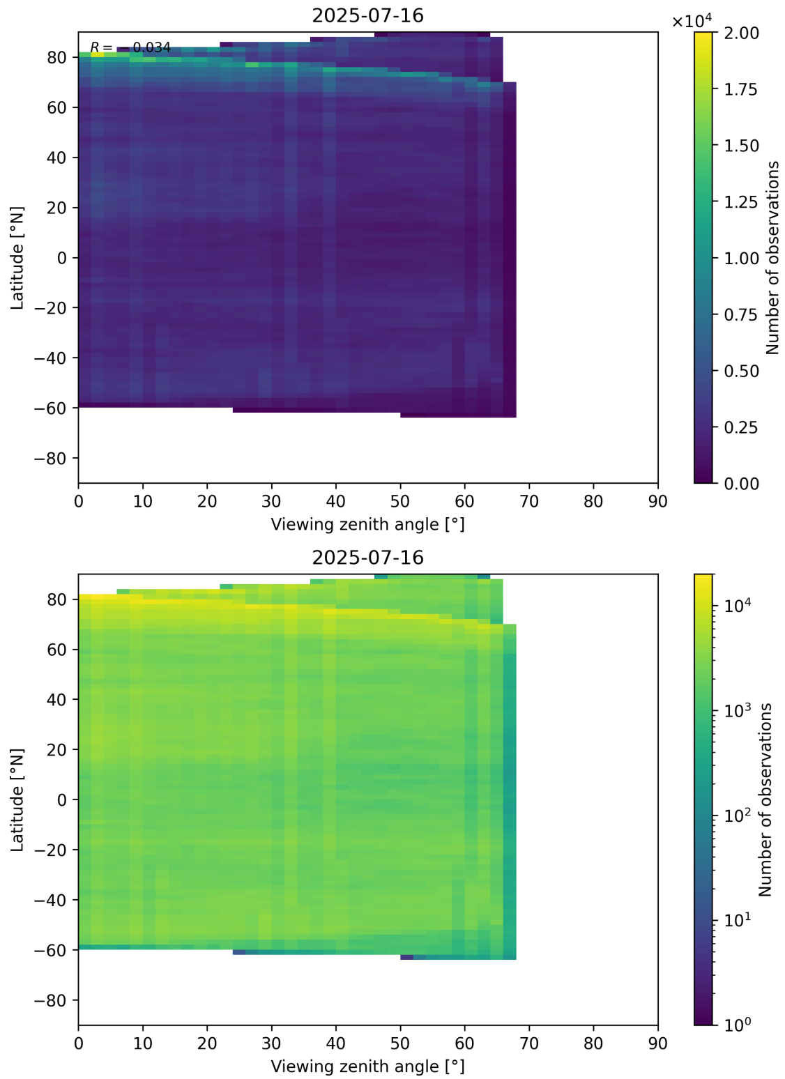
Figure 74: Scatter density plot of “Viewing zenith angle” against “Latitude” for 2025-07-15 to 2025-07-17.
