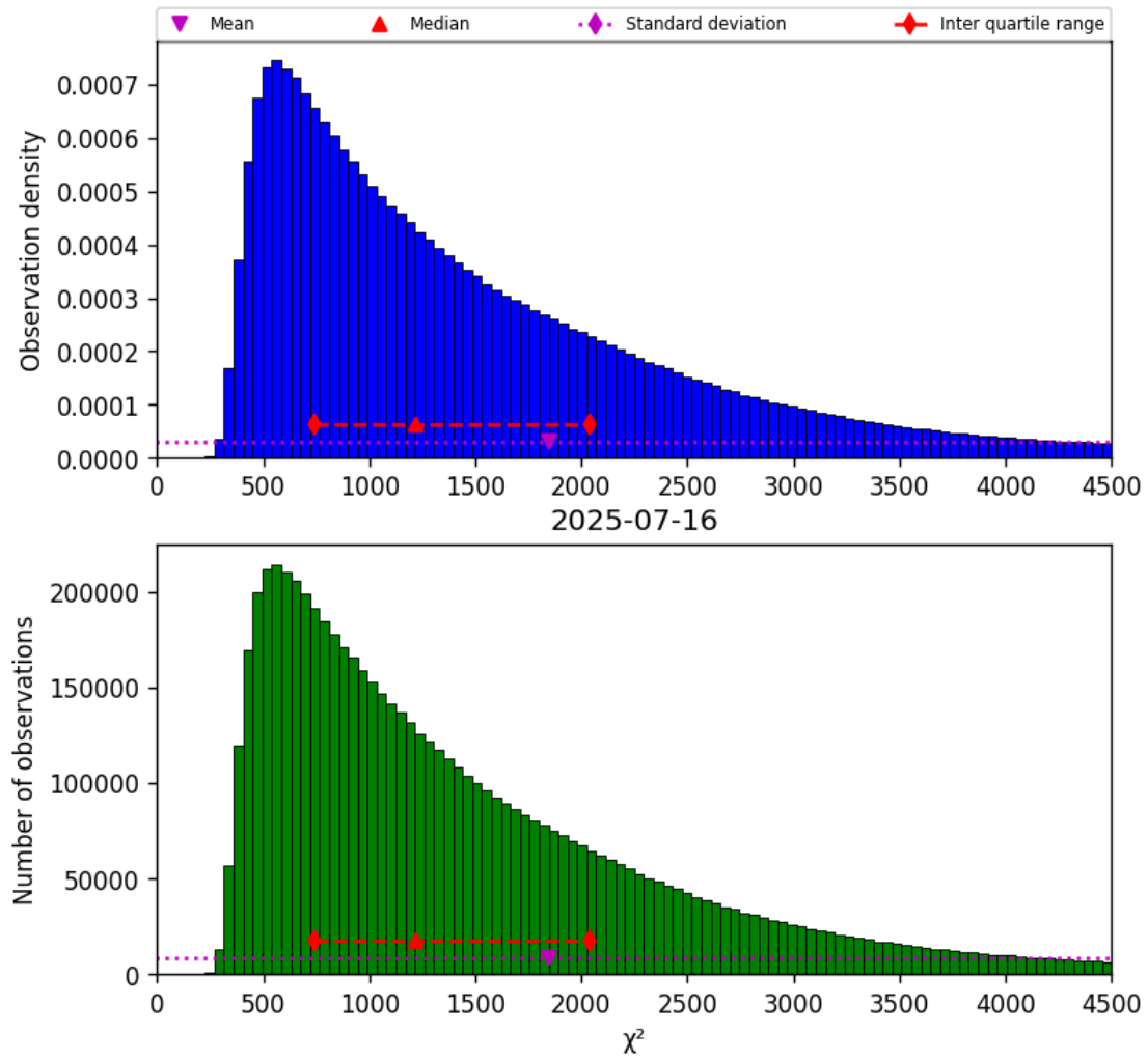
Figure 22: Histogram of “ \chi^2 ” for 2025-07-15 to 2025-07-17
