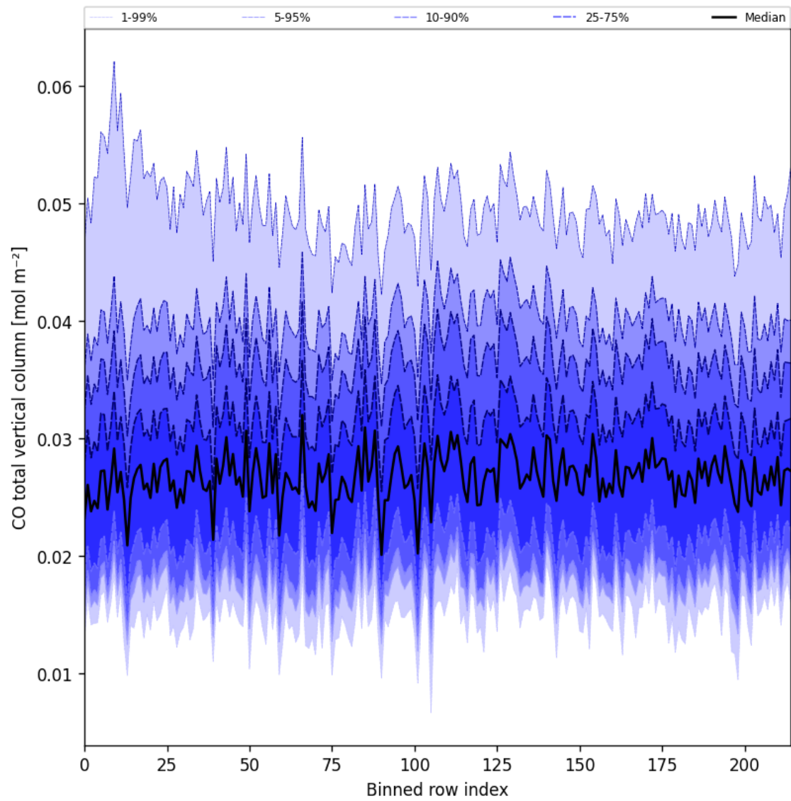
Figure 26: Along track statistics of “CO total vertical column” for 2025-07-15 to 2025-07-17
