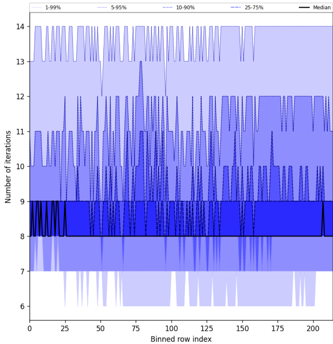
Figure 32: Along track statistics of “Number of iterations” for 2025-07-15 to 2025-07-17
