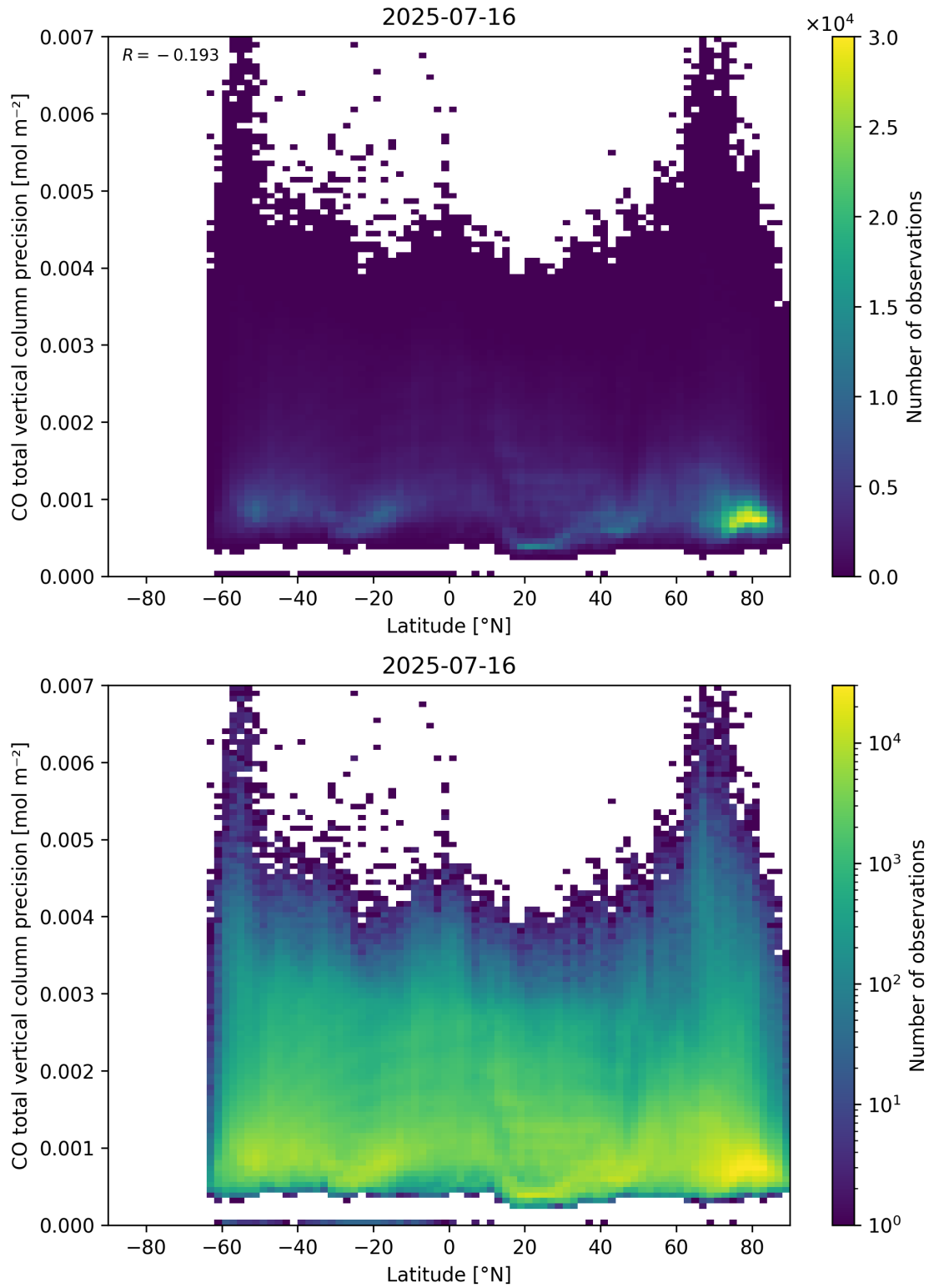
Figure 53: Scatter density plot of “Latitude” against “CO total vertical column precision” for 2025-07-15 to 2025-07-17.
