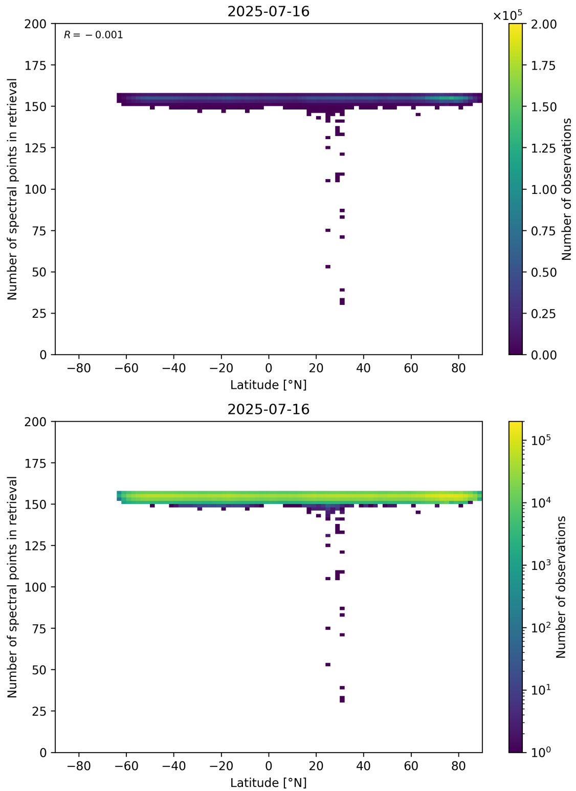
Figure 57: Scatter density plot of “Latitude” against “Number of spectral points in retrieval” for 2025-07-15 to 2025-07-17.
