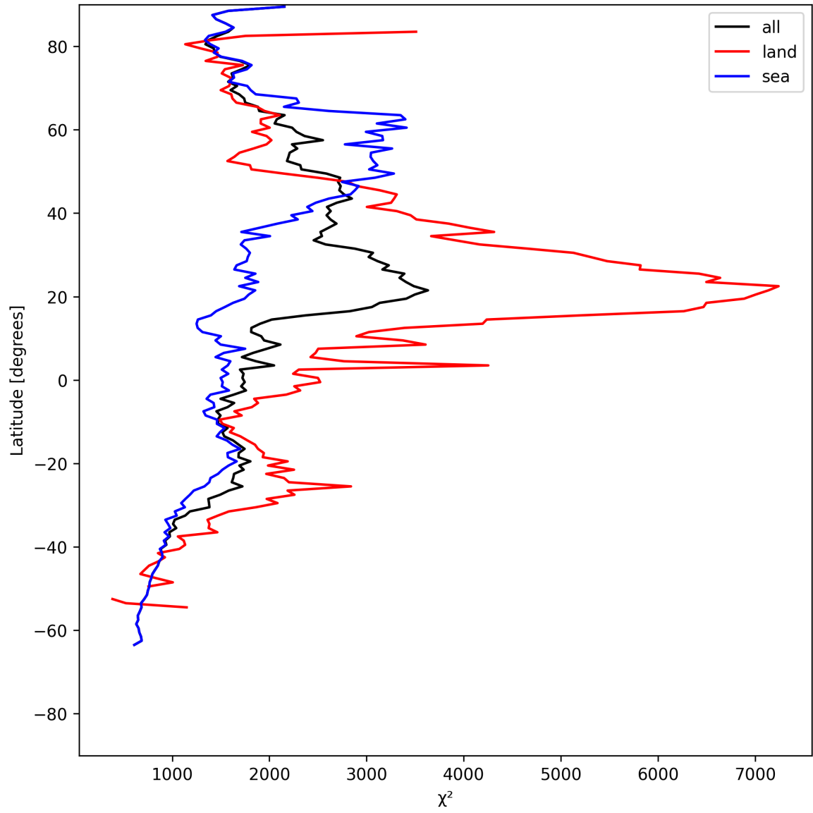
Figure 14: Zonal average of “ \chi^2 ” for 2025-07-15 to 2025-07-17.
