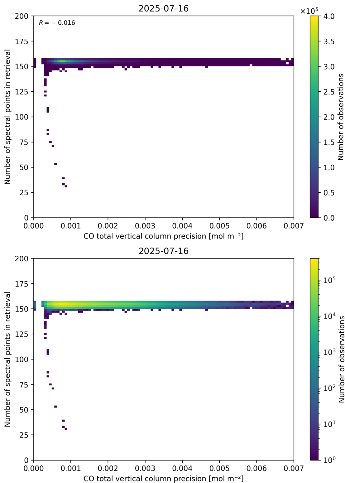
Figure 47: Scatter density plot of “CO total vertical column precision” against “Number of spectral points in retrieval” for 2025-07-15 to 2025-07-17.
