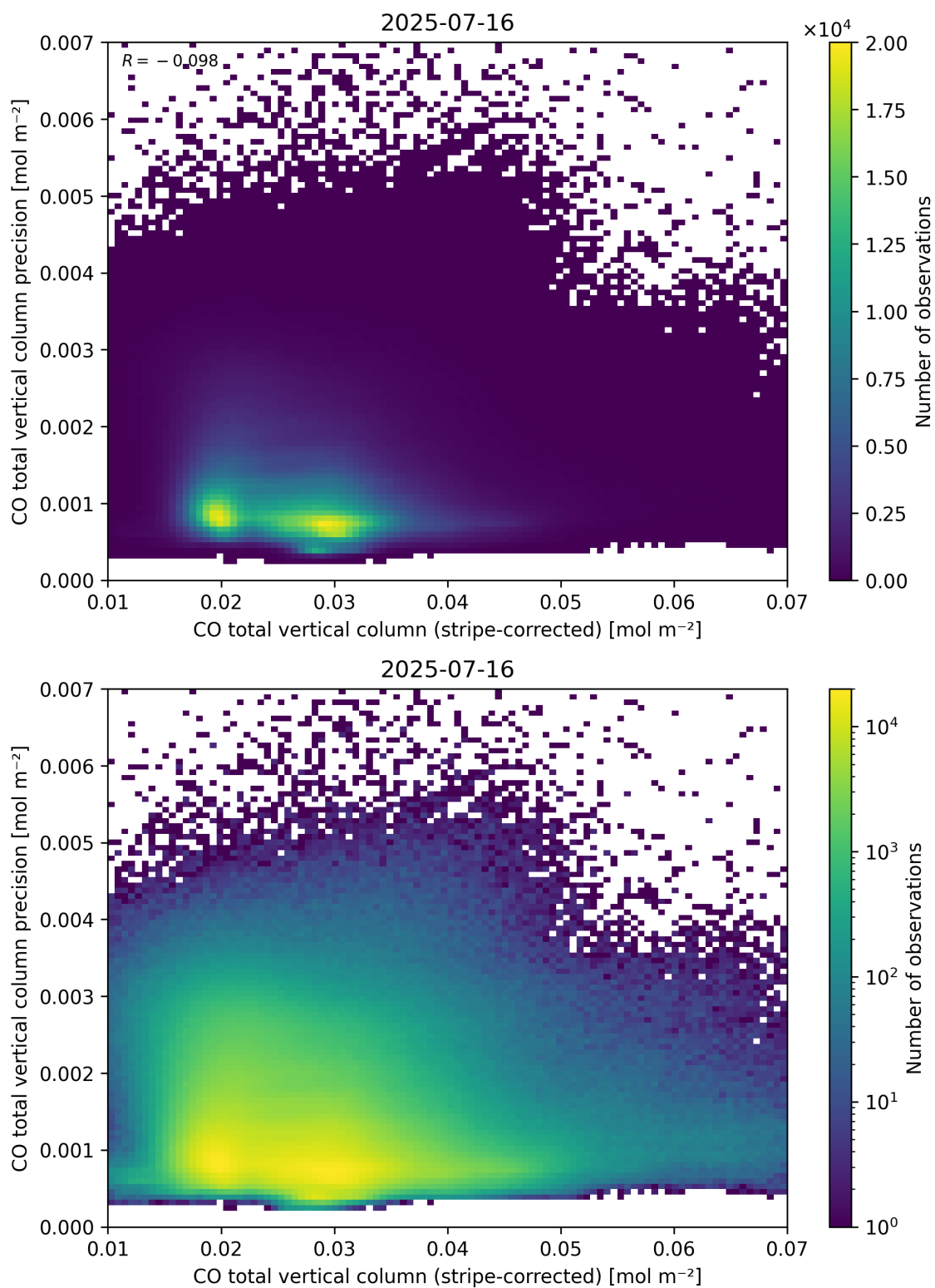
Figure 36: Scatter density plot of “CO total vertical column (stripe-corrected)” against “CO total vertical column precision” for 2025-07-15 to 2025-07-17.
