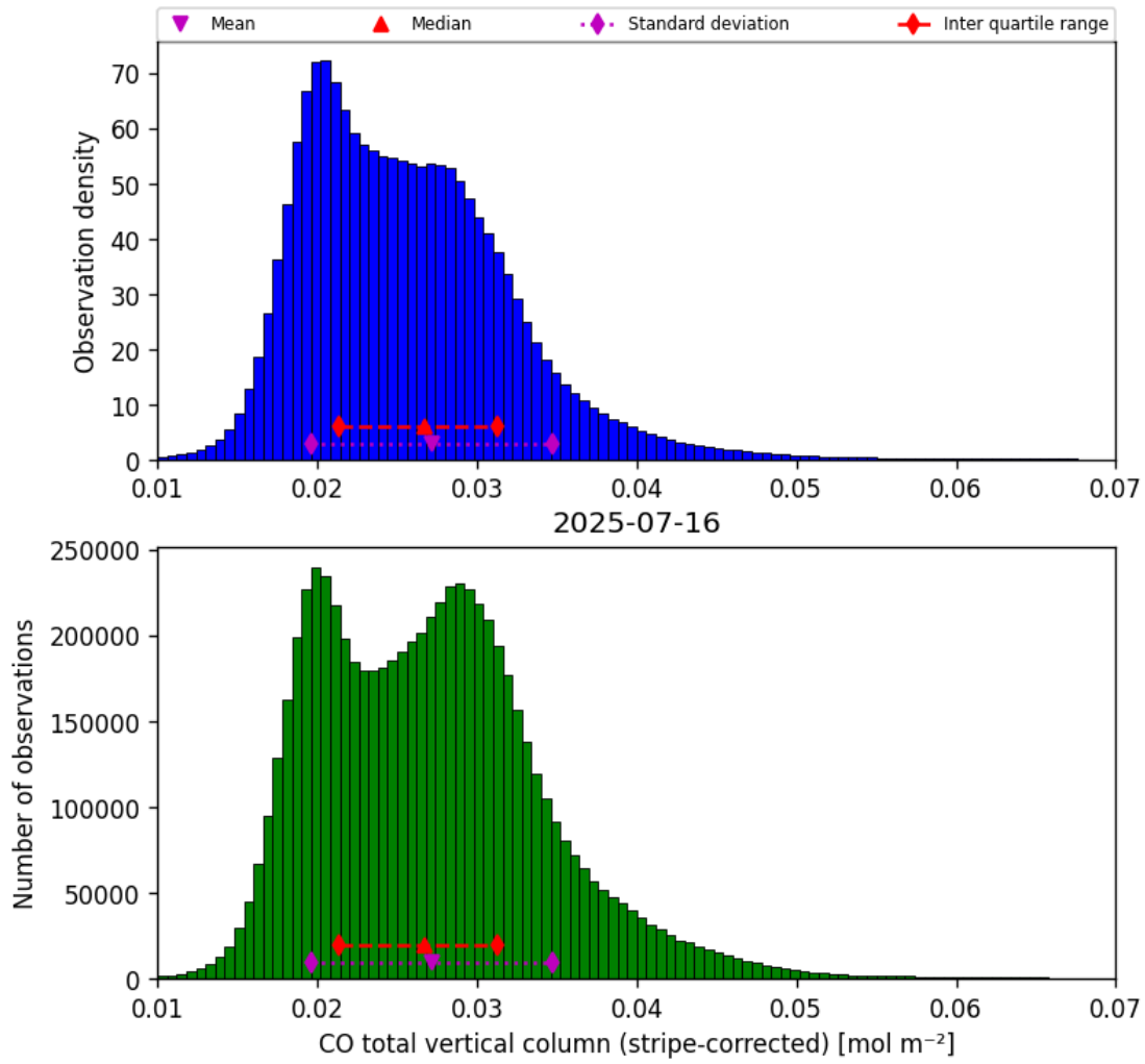
Figure 19: Histogram of “CO total vertical column (stripe-corrected)” for 2025-07-15 to 2025-07-17
