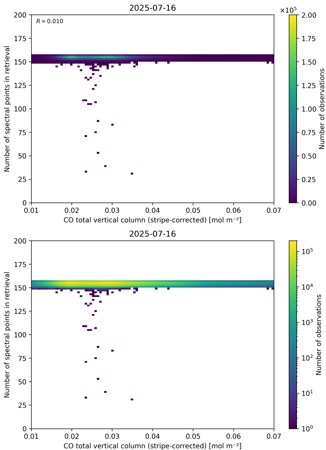
Figure 40: Scatter density plot of “CO total vertical column (stripe-corrected)” against “Number of spectral points in retrieval” for 2025-07-15 to 2025-07-17.
