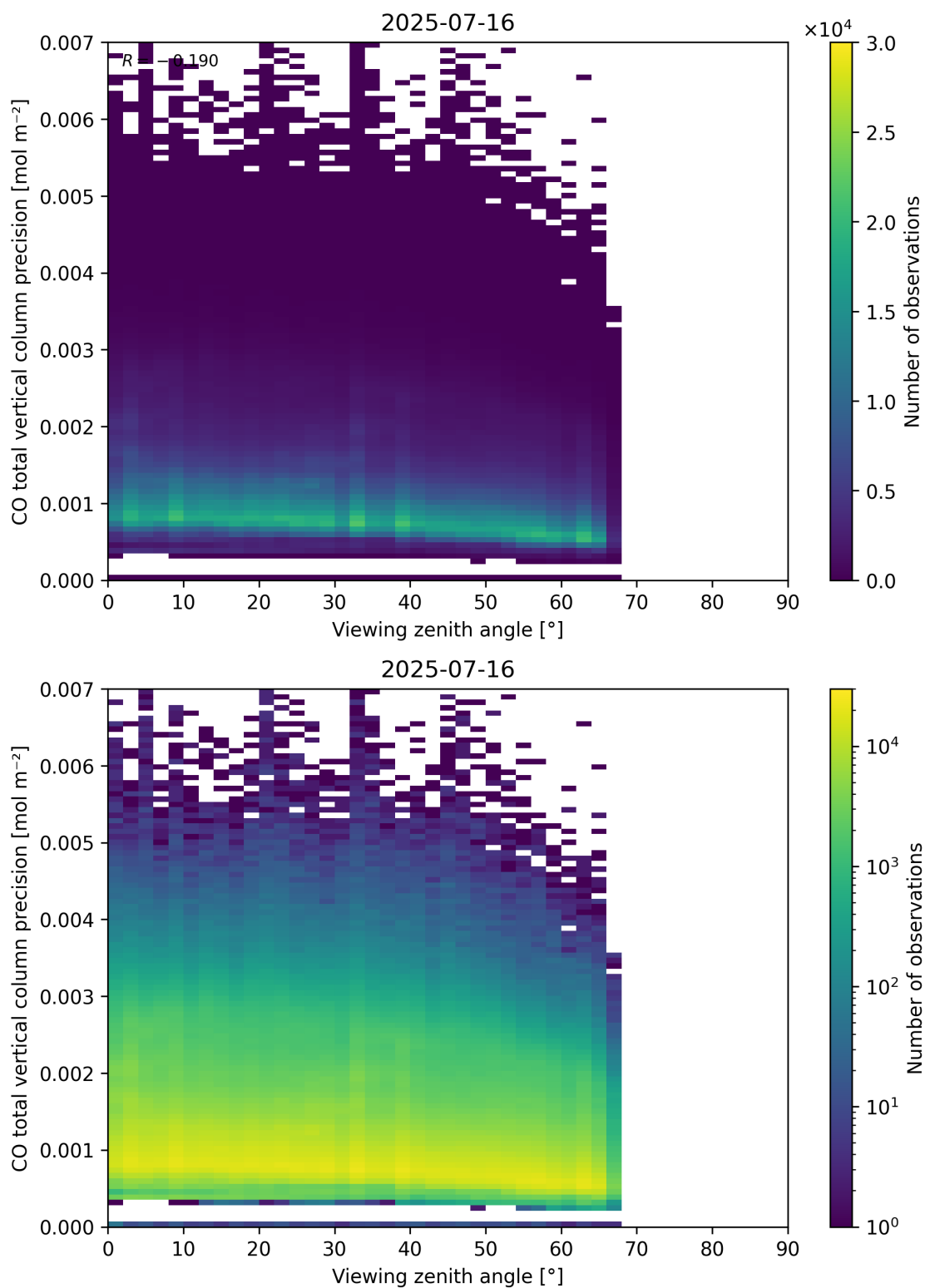
Figure 71: Scatter density plot of “Viewing zenith angle” against “CO total vertical column precision” for 2025-07-15 to 2025-07-17.
