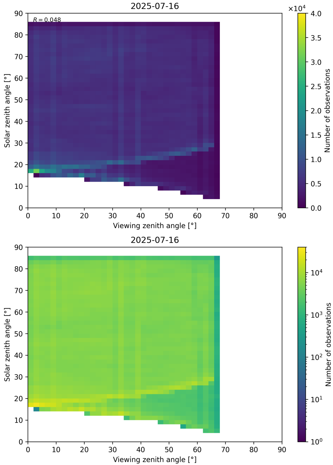
Figure 77: Scatter density plot of “Viewing zenith angle” against “Solar zenith angle” for 2025-07-15 to 2025-07-17.
