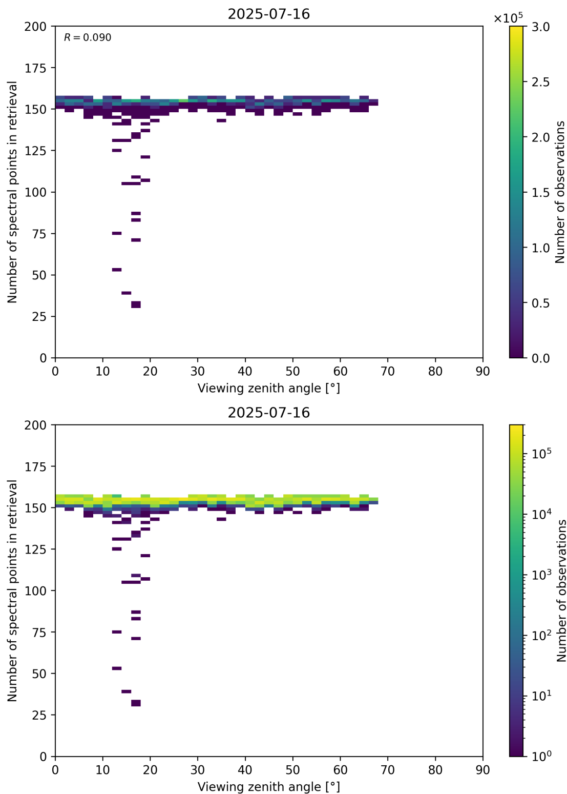
Figure 76: Scatter density plot of “Viewing zenith angle” against “Number of spectral points in retrieval” for 2025-07-15 to 2025-07-17.
