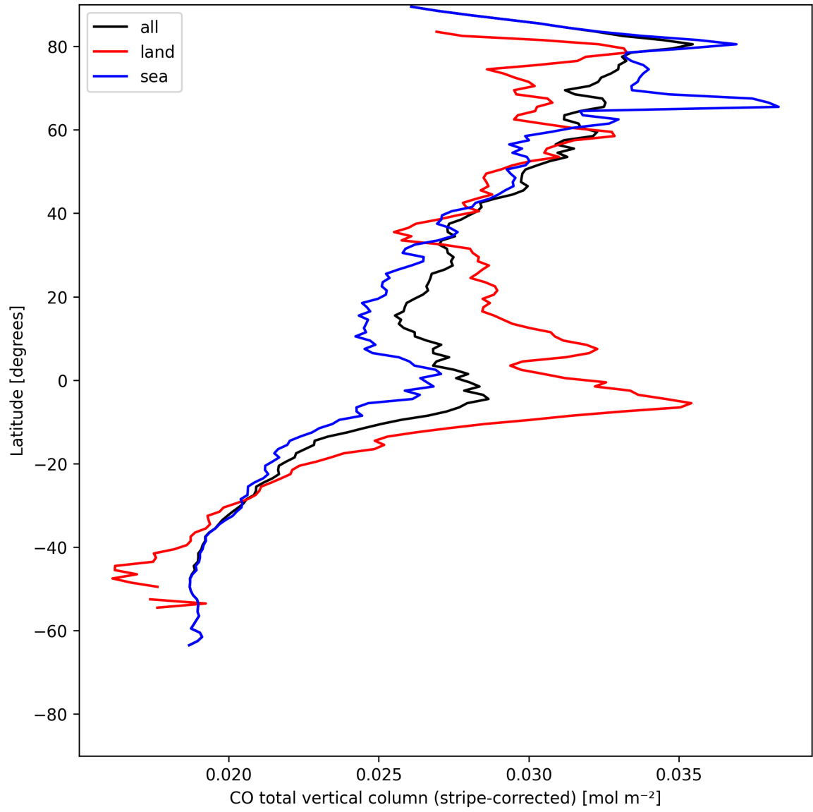
Figure 11: Zonal average of “CO total vertical column (stripe-corrected)” for 2025-07-15 to 2025-07-17.
