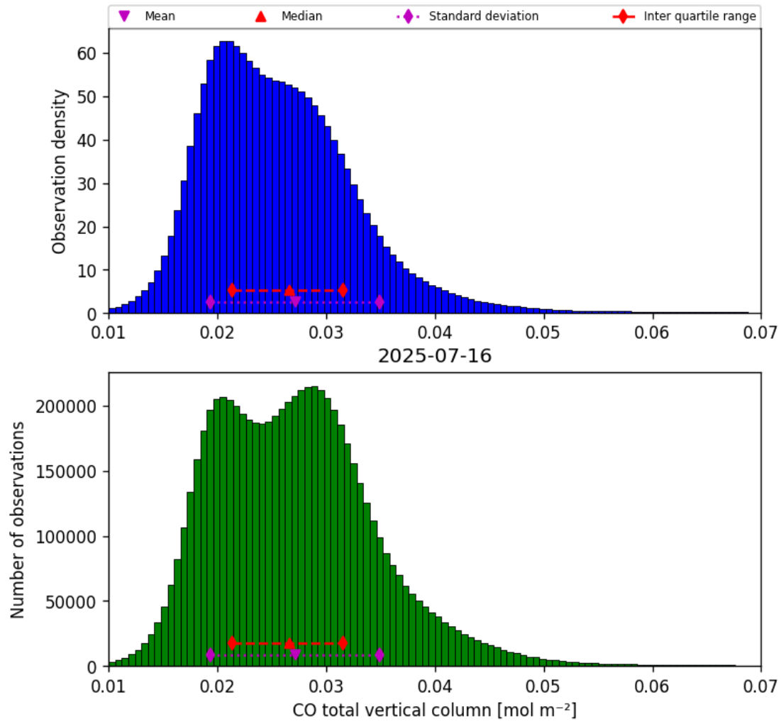
Figure 18: Histogram of “CO total vertical column” for 2025-07-15 to 2025-07-17
