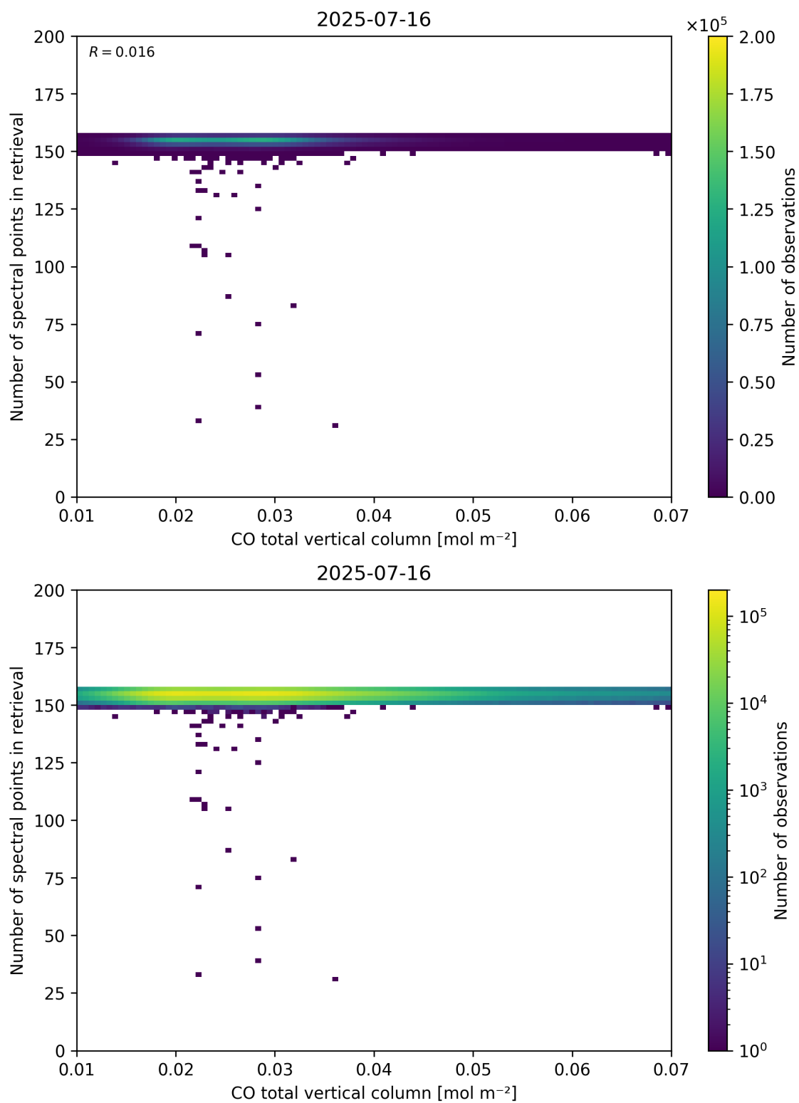
Figure 43: Scatter density plot of “CO total vertical column” against “Number of spectral points in retrieval” for 2025-07-15 to 2025-07-17.
