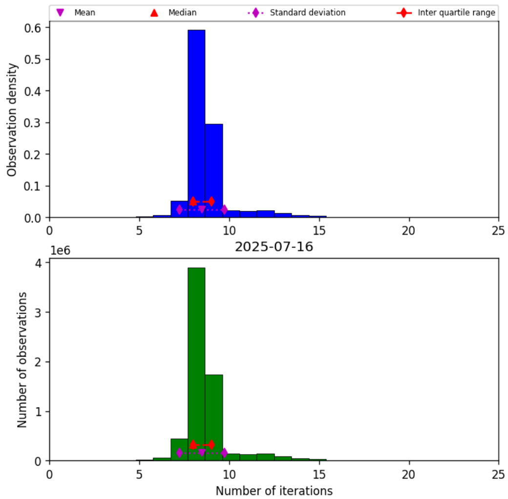
Figure 24: Histogram of “Number of iterations” for 2025-07-15 to 2025-07-17
