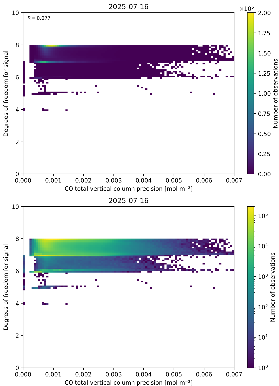
Figure 45: Scatter density plot of “CO total vertical column precision” against “Degrees of freedom for signal” for 2025-07-15 to 2025-07-17.
