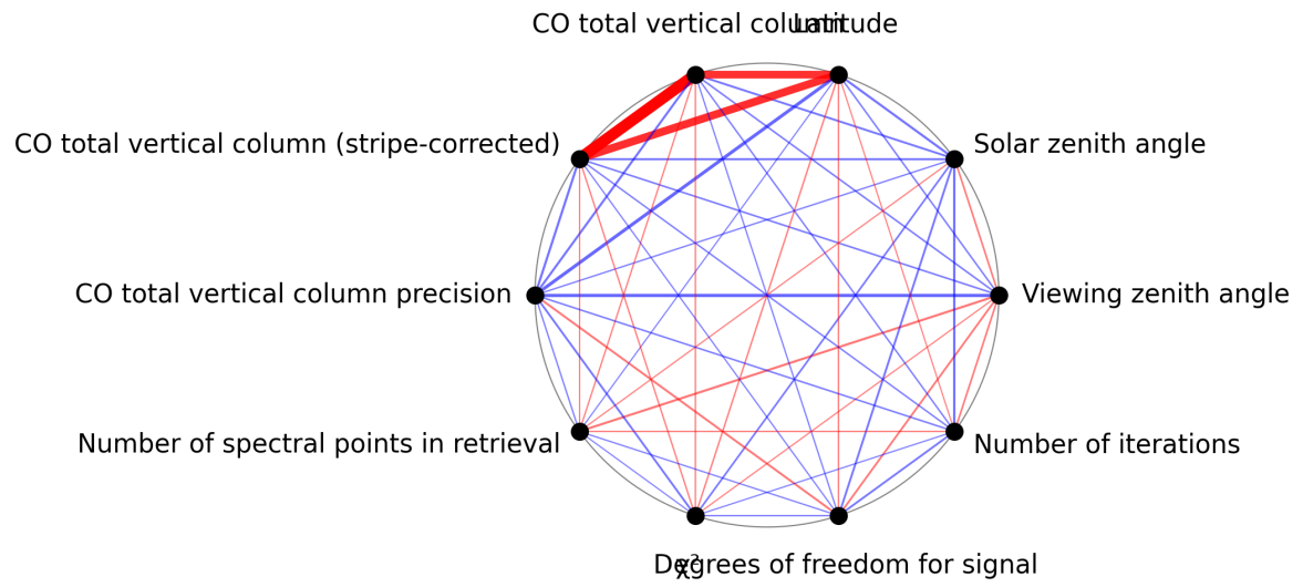
Figure 1: Map of correlation graph for 2025-07-15 to 2025-07-17.
