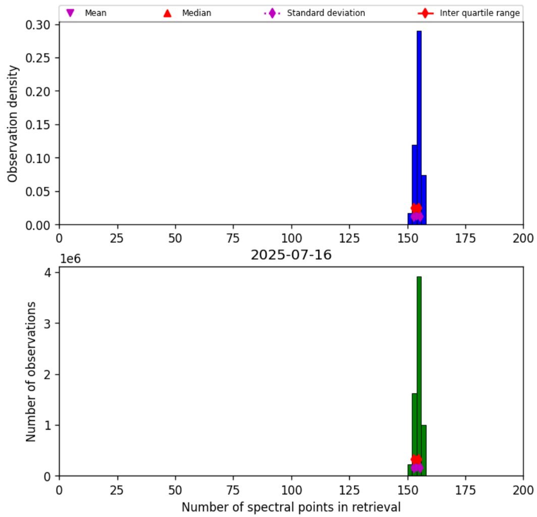
Figure 21: Histogram of “Number of spectral points in retrieval” for 2025-07-15 to 2025-07-17
