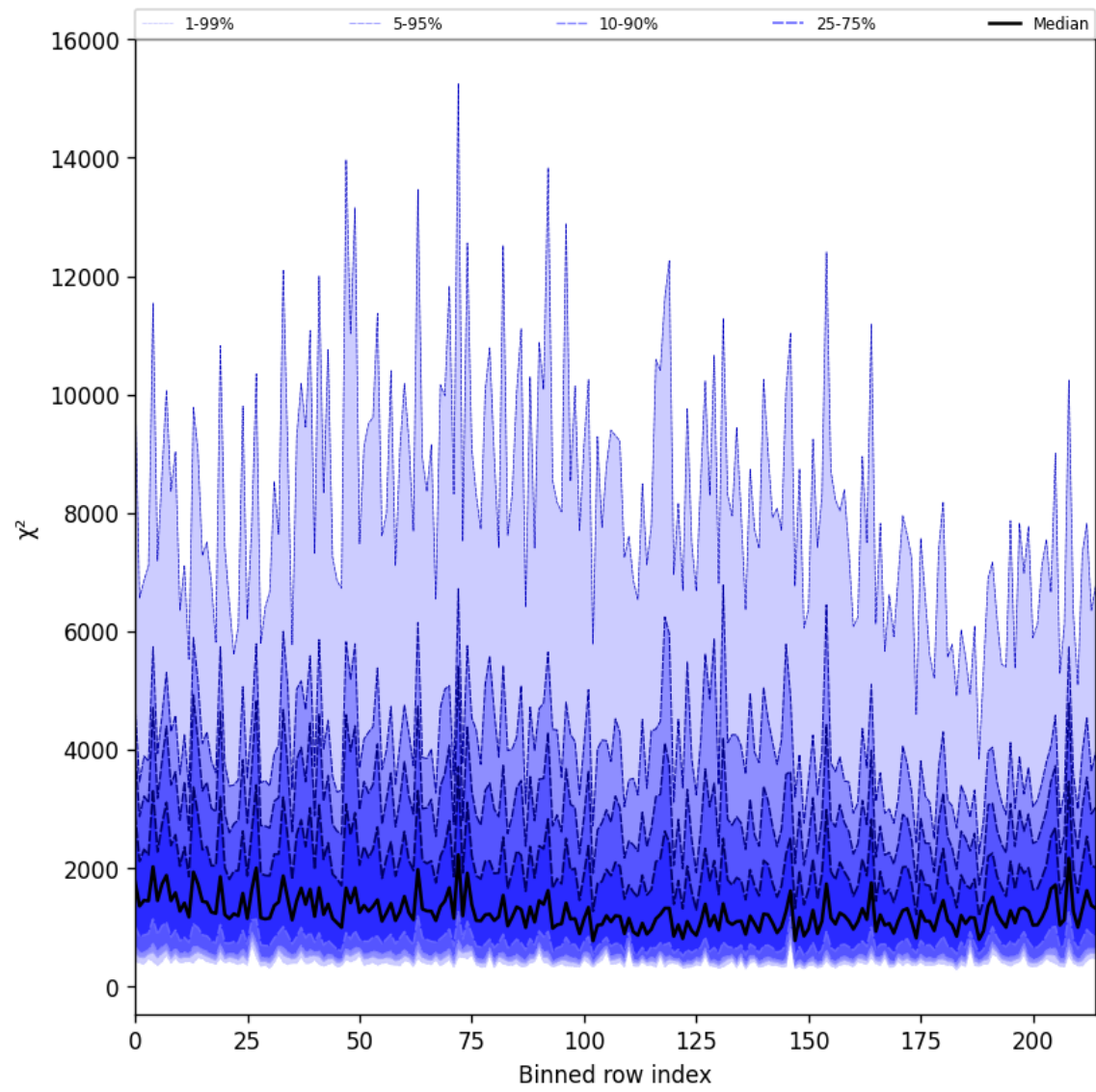
Figure 30: Along track statistics of “ \chi^2 ” for 2025-07-15 to 2025-07-17
