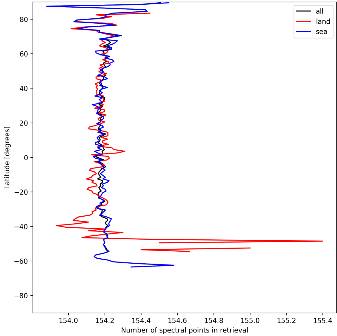
Figure 13: Zonal average of “Number of spectral points in retrieval” for 2025-07-15 to 2025-07-17.
