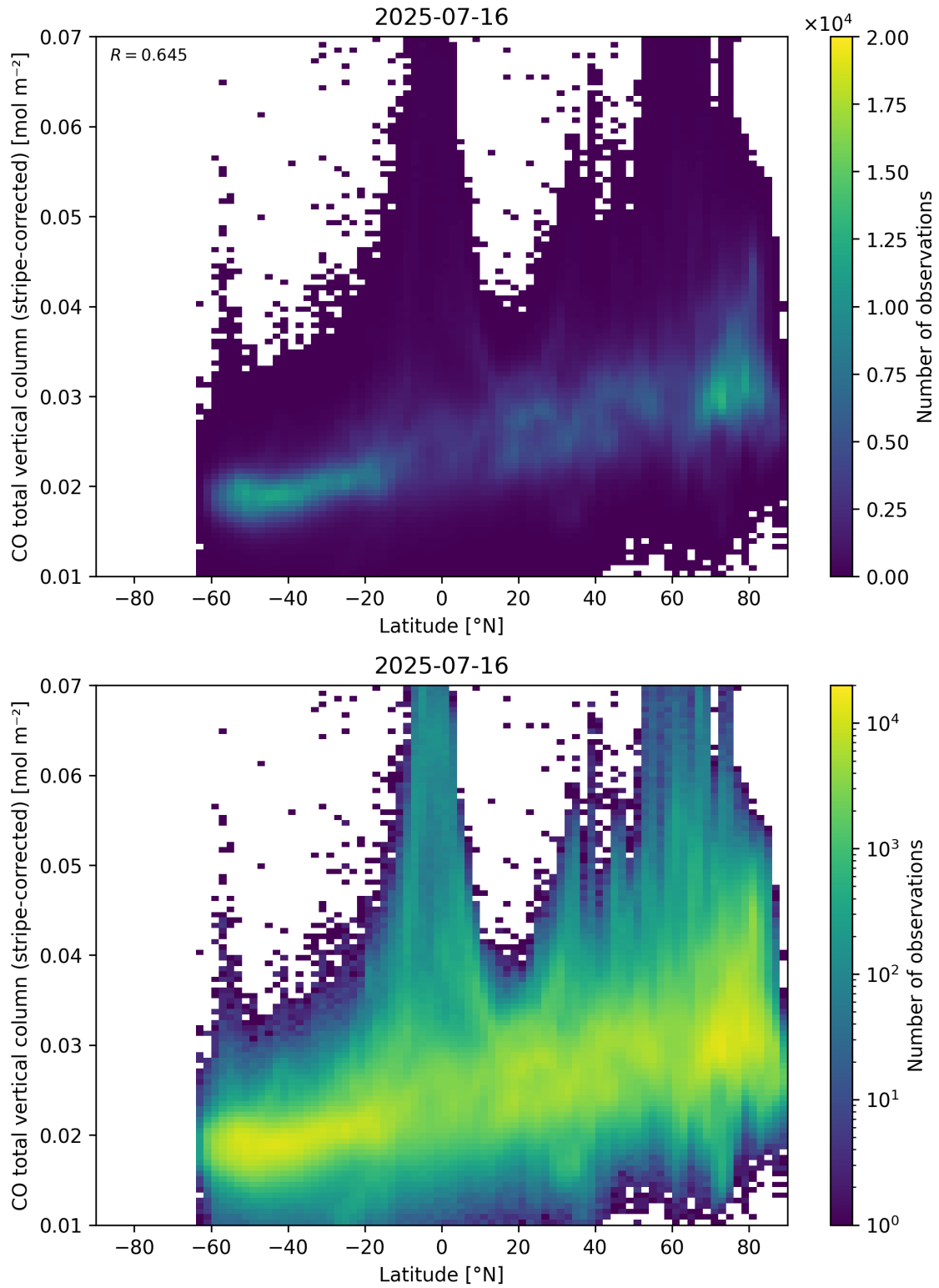
Figure 52: Scatter density plot of “Latitude” against “CO total vertical column (stripe-corrected)” for 2025-07-15 to 2025-07-17.
