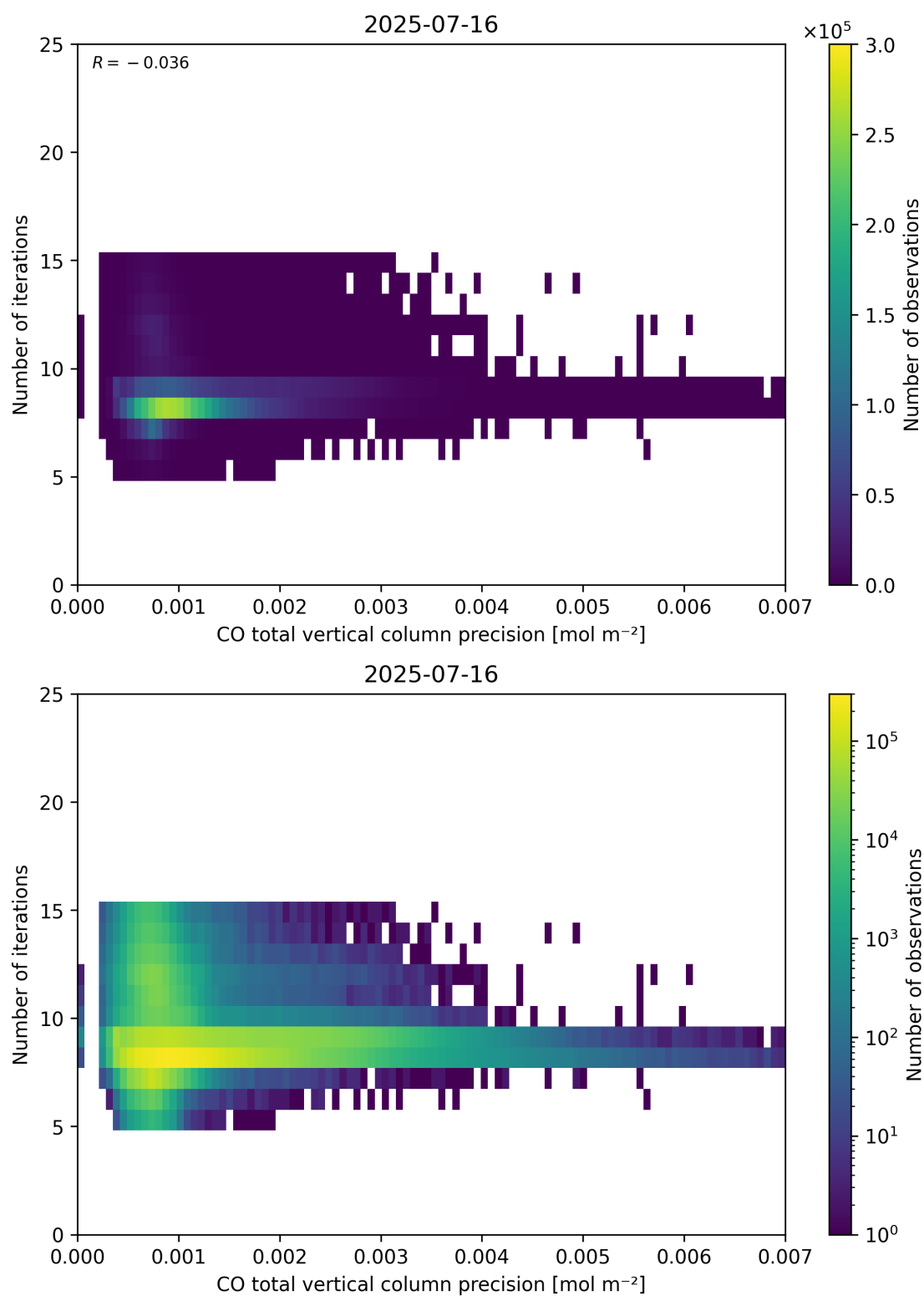
Figure 46: Scatter density plot of “CO total vertical column precision” against “Number of iterations” for 2025-07-15 to 2025-07-17.
