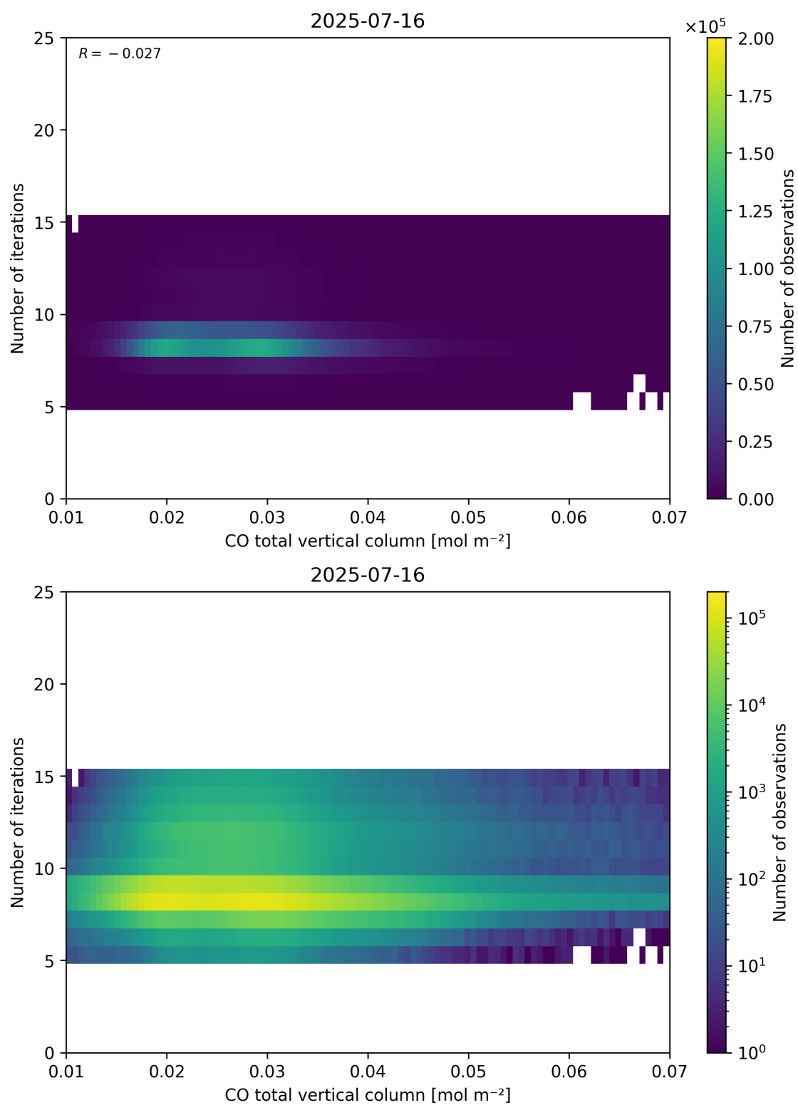
Figure 42: Scatter density plot of “CO total vertical column” against “Number of iterations” for 2025-07-15 to 2025-07-17.
