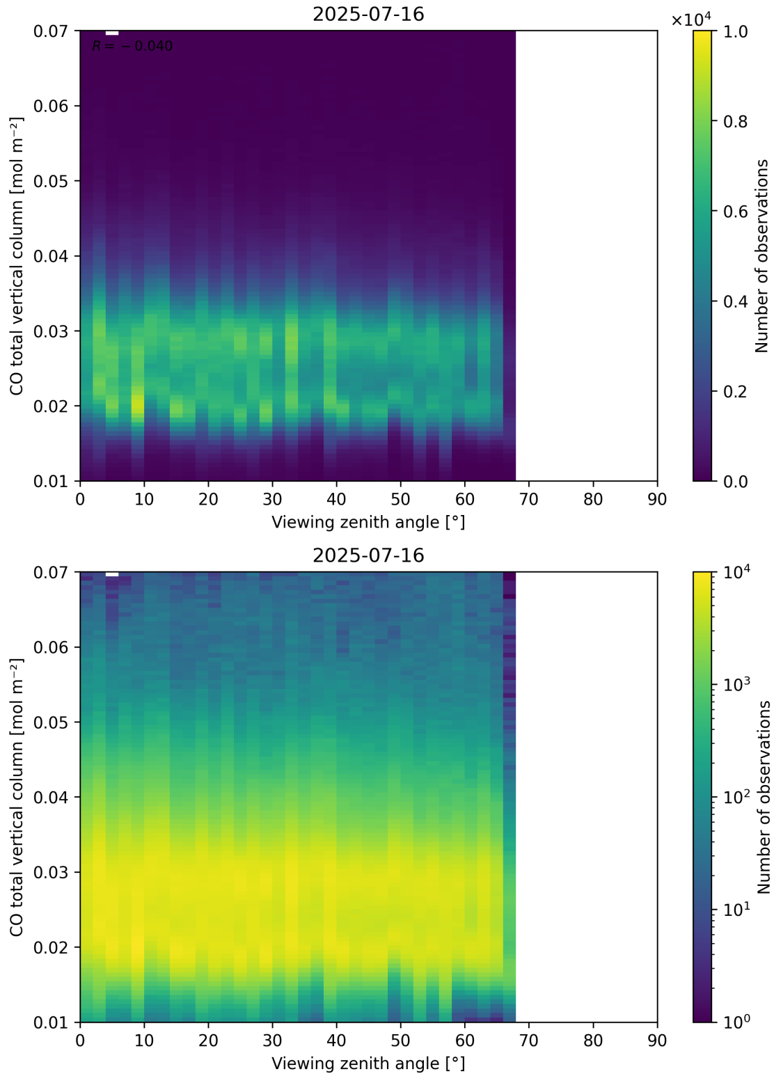
Figure 69: Scatter density plot of “Viewing zenith angle” against “CO total vertical column” for 2025-07-15 to 2025-07-17.
