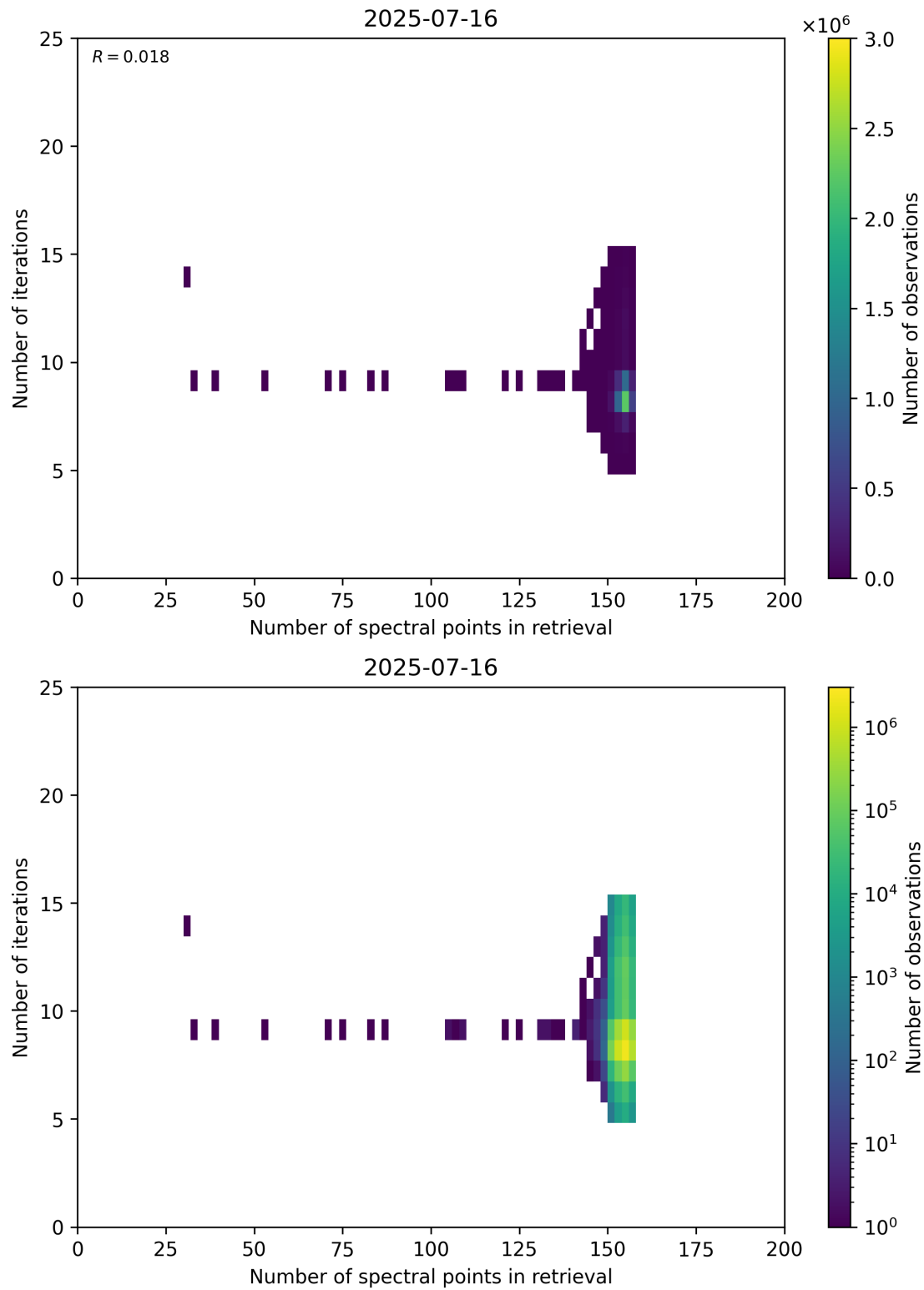
Figure 60: Scatter density plot of “Number of spectral points in retrieval” against “Number of iterations” for 2025-07-15 to 2025-07-17.
