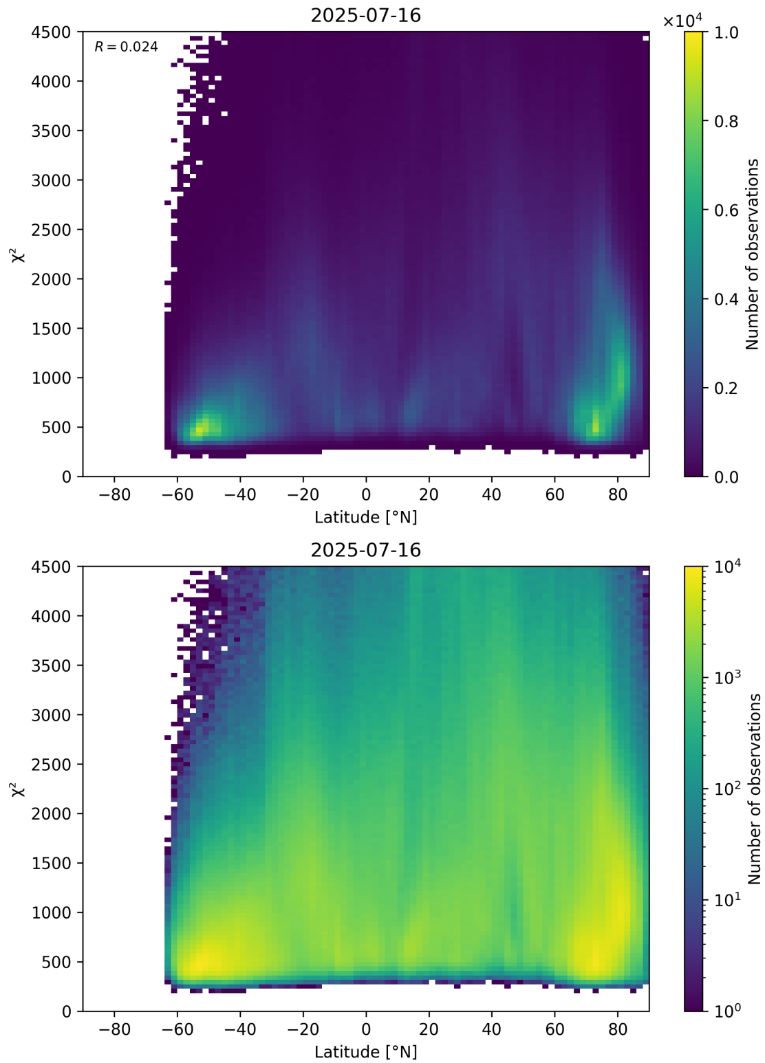
Figure 54: Scatter density plot of “Latitude” against “ \chi^2 ” for 2025-07-15 to 2025-07-17.
