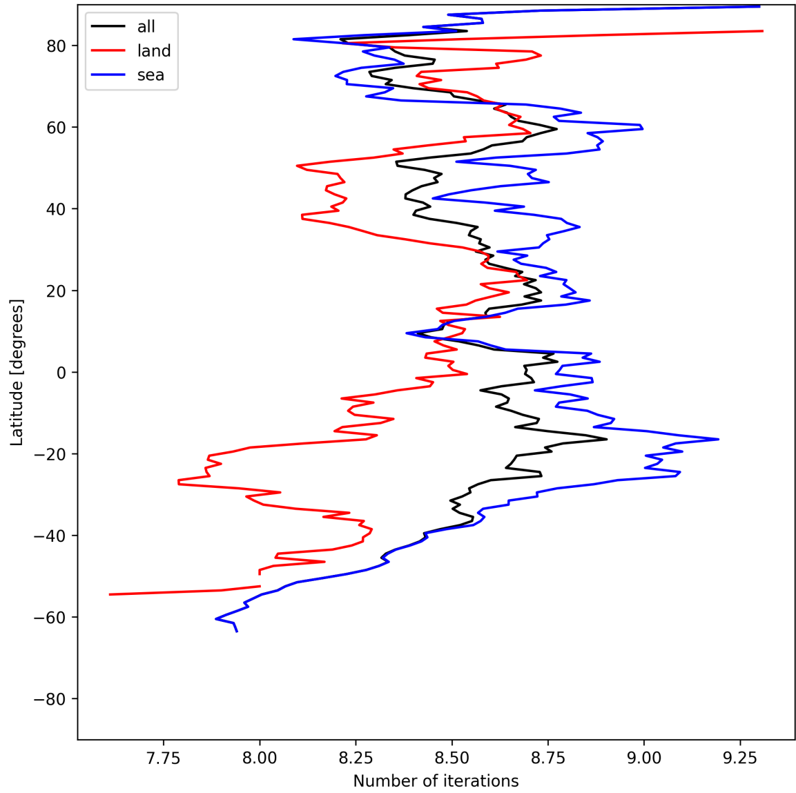
Figure 16: Zonal average of “Number of iterations” for 2025-07-15 to 2025-07-17.
