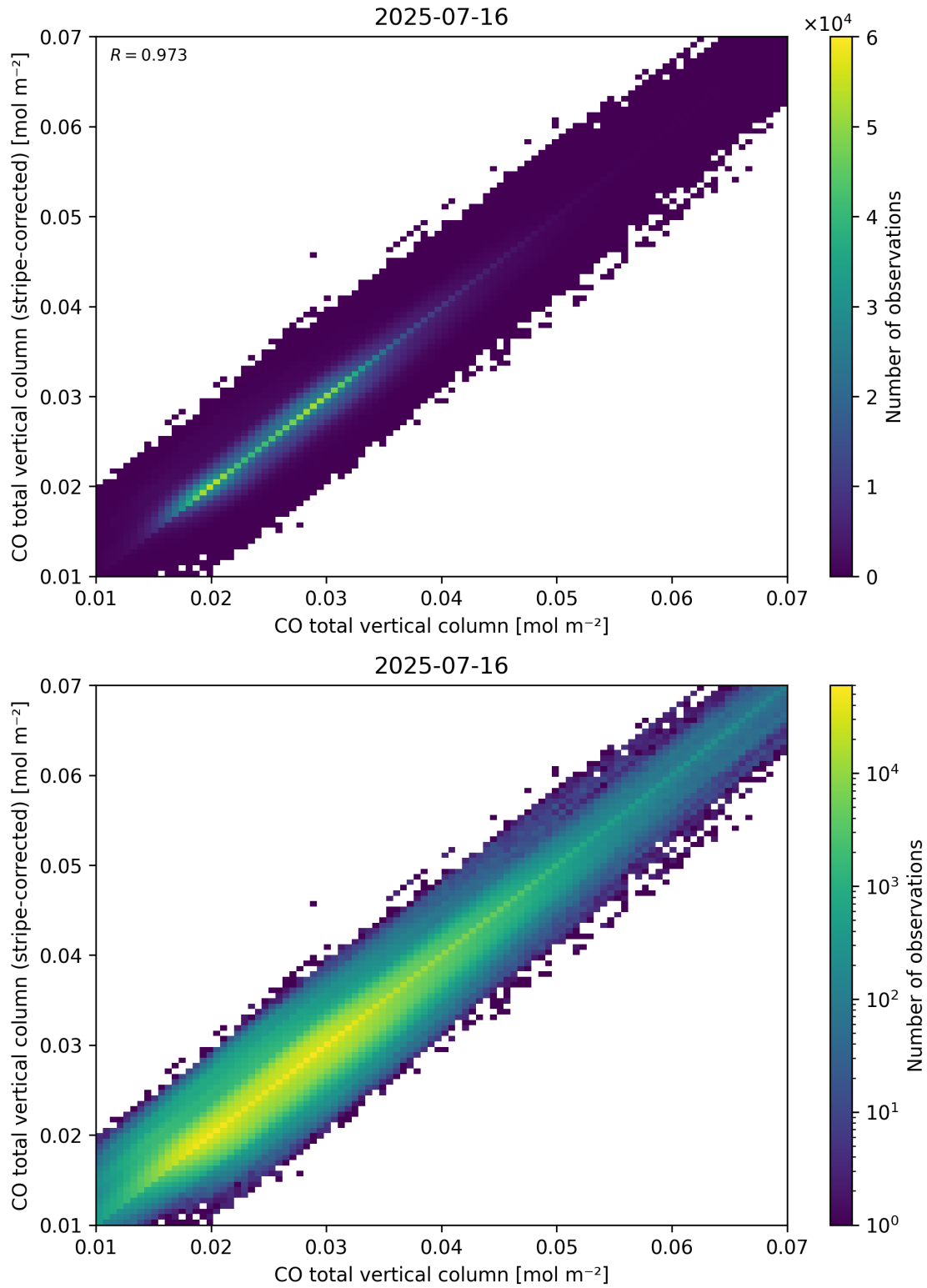
Figure 33: Scatter density plot of “CO total vertical column” against “CO total vertical column (stripe-corrected)” for 2025-07-15 to 2025-07-17.
