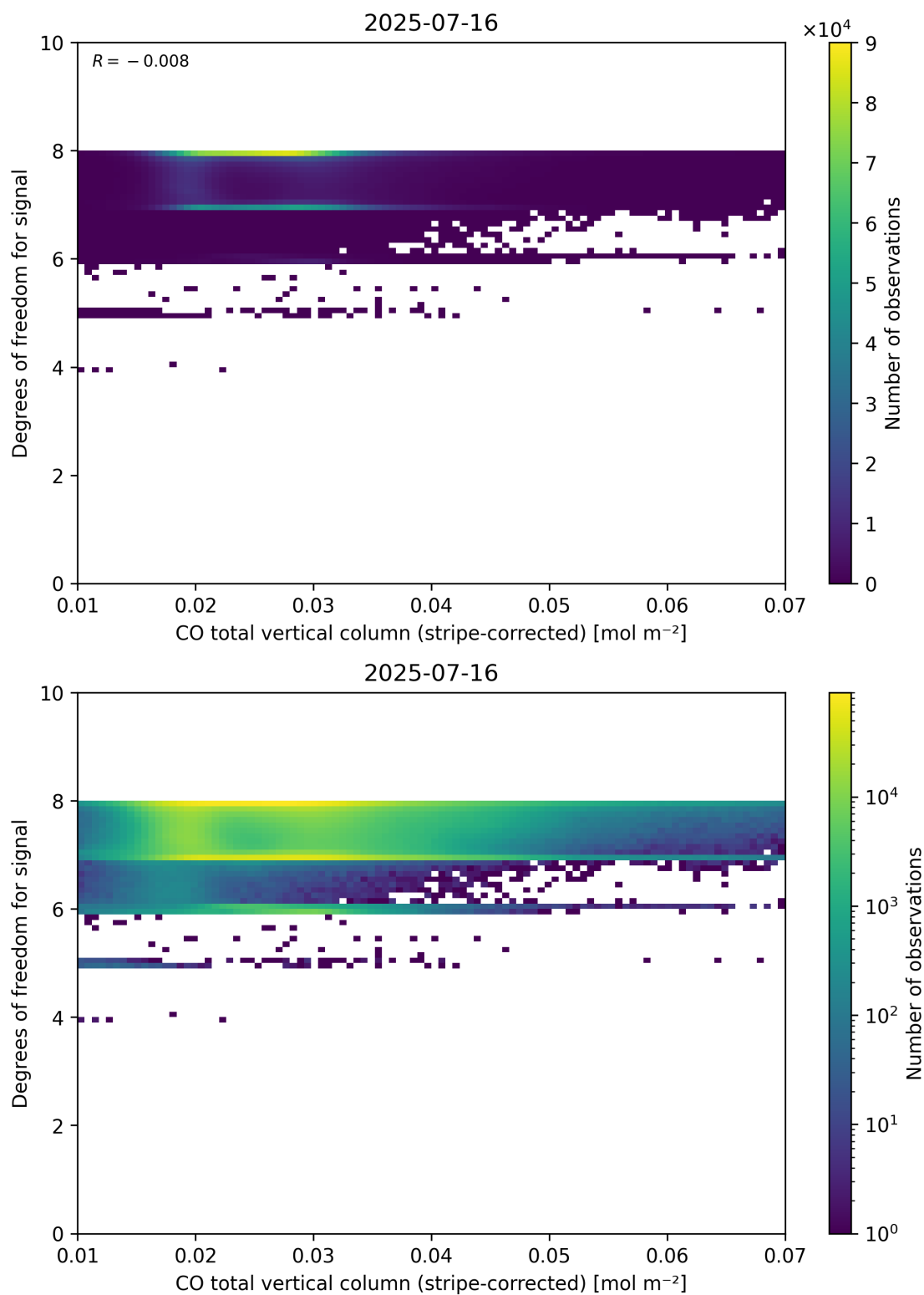
Figure 38: Scatter density plot of “CO total vertical column (stripe-corrected)” against “Degrees of freedom for signal” for 2025-07-15 to 2025-07-17.
