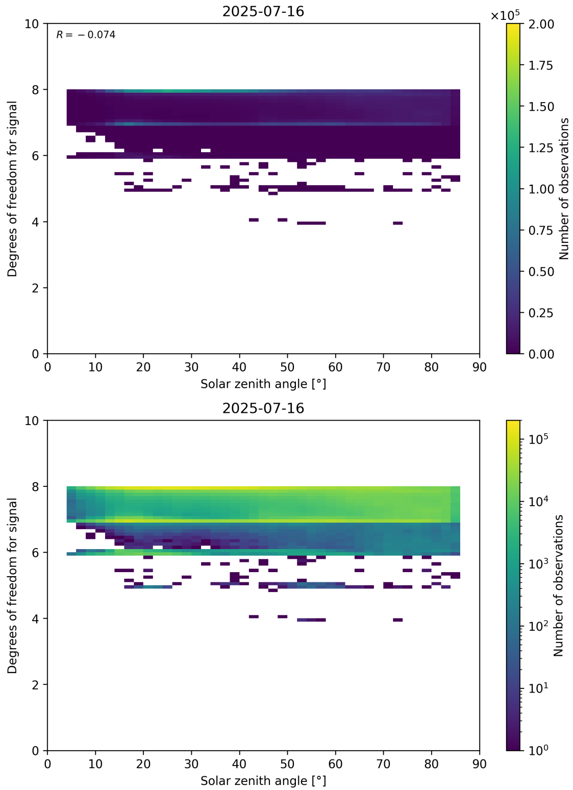
Figure 65: Scatter density plot of “Solar zenith angle” against “Degrees of freedom for signal” for 2025-07-15 to 2025-07-17.
