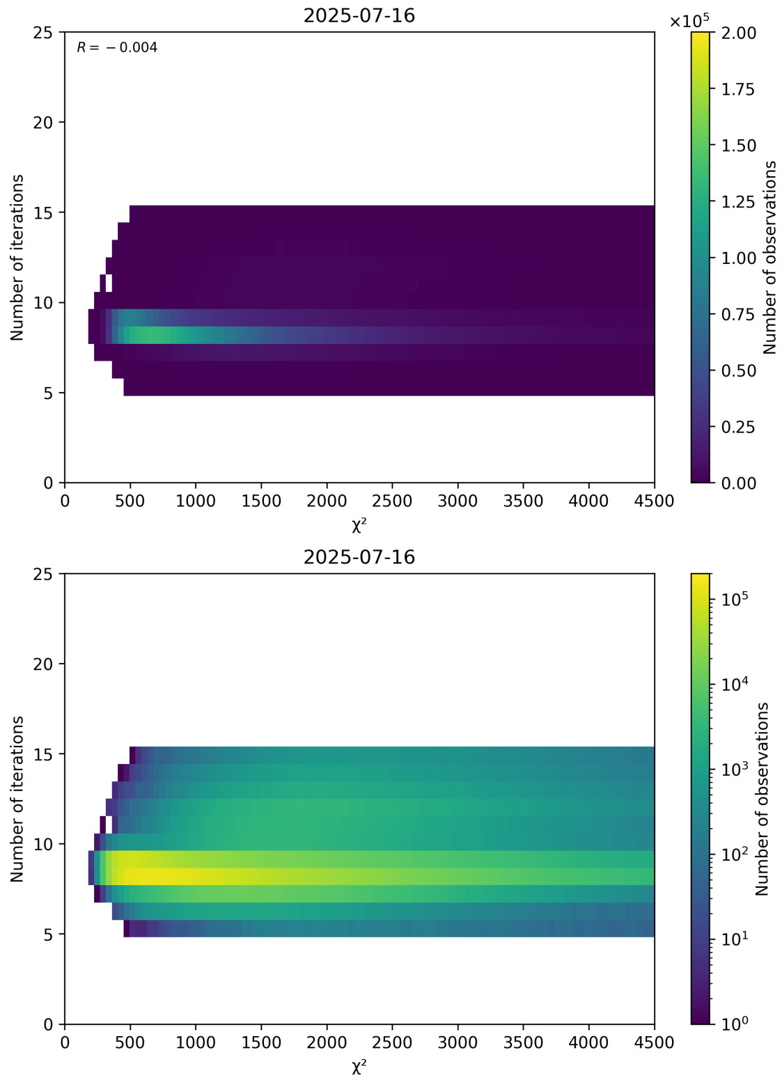
Figure 49: Scatter density plot of “ \chi^2 ” against “Number of iterations” for 2025-07-15 to 2025-07-17.
