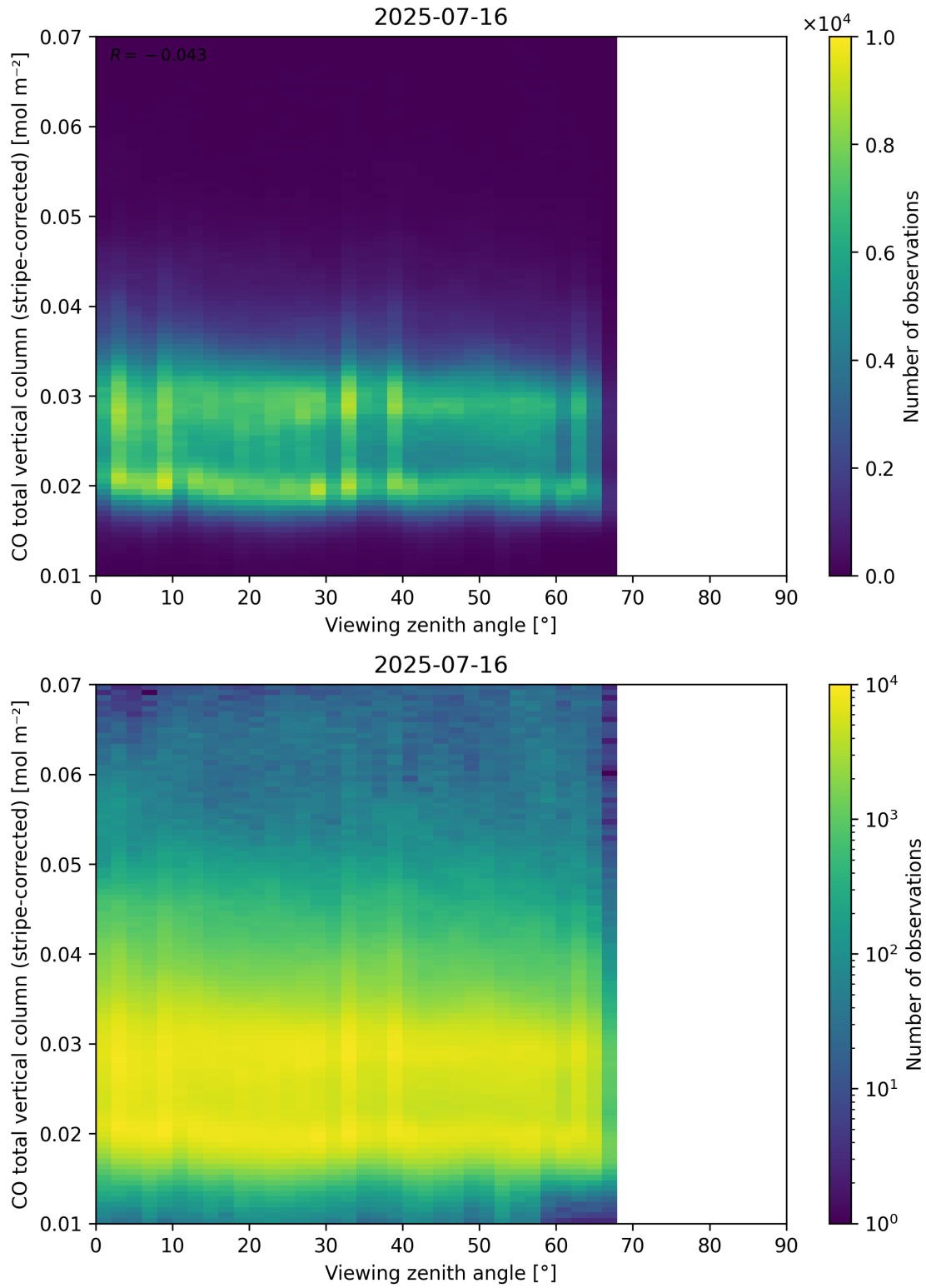
Figure 70: Scatter density plot of “Viewing zenith angle” against “CO total vertical column (stripe-corrected)” for 2025-07-15 to 2025-07-17.
