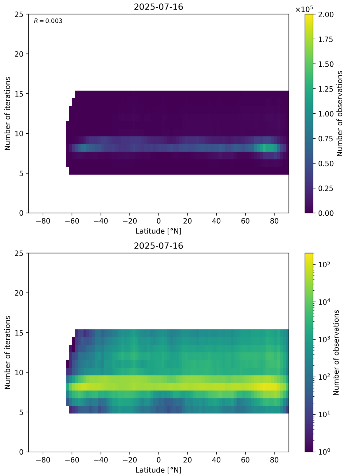
Figure 56: Scatter density plot of “Latitude” against “Number of iterations” for 2025-07-15 to 2025-07-17.
