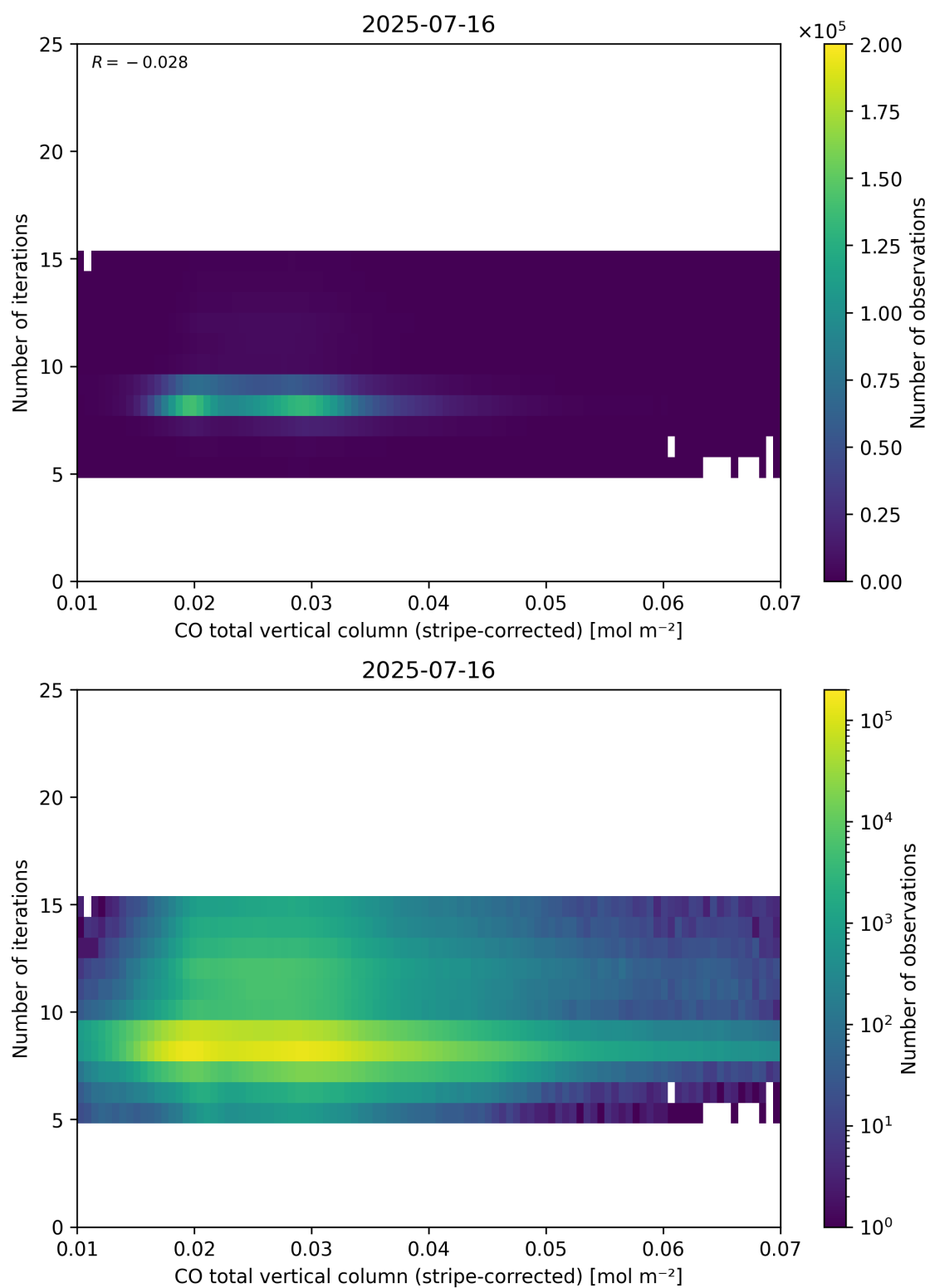
Figure 39: Scatter density plot of “CO total vertical column (stripe-corrected)” against “Number of iterations” for 2025-07-15 to 2025-07-17.
