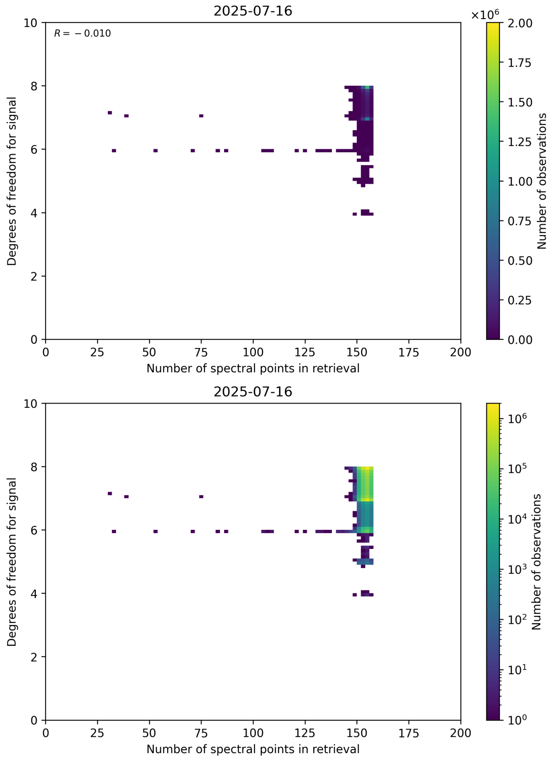
Figure 59: Scatter density plot of “Number of spectral points in retrieval” against “Degrees of freedom for signal” for 2025-07-15 to 2025-07-17.
