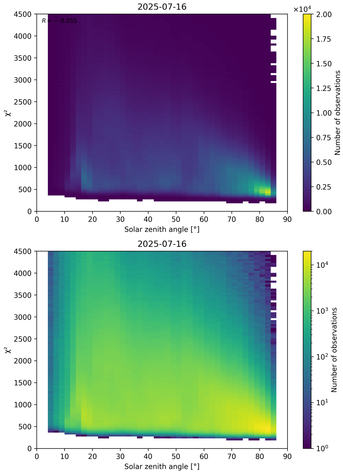
Figure 64: Scatter density plot of “Solar zenith angle” against “ \chi^2 ” for 2025-07-15 to 2025-07-17.
