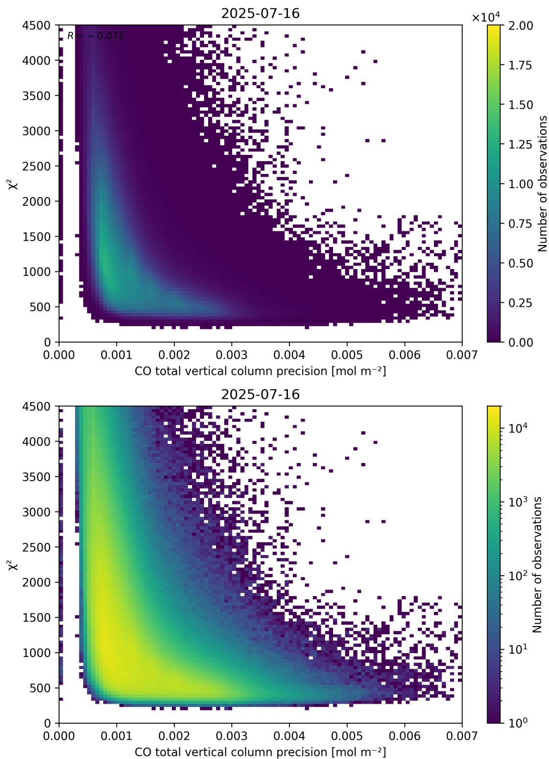
Figure 44: Scatter density plot of “CO total vertical column precision” against “ \chi^2 ” for 2025-07-15 to 2025-07-17.
