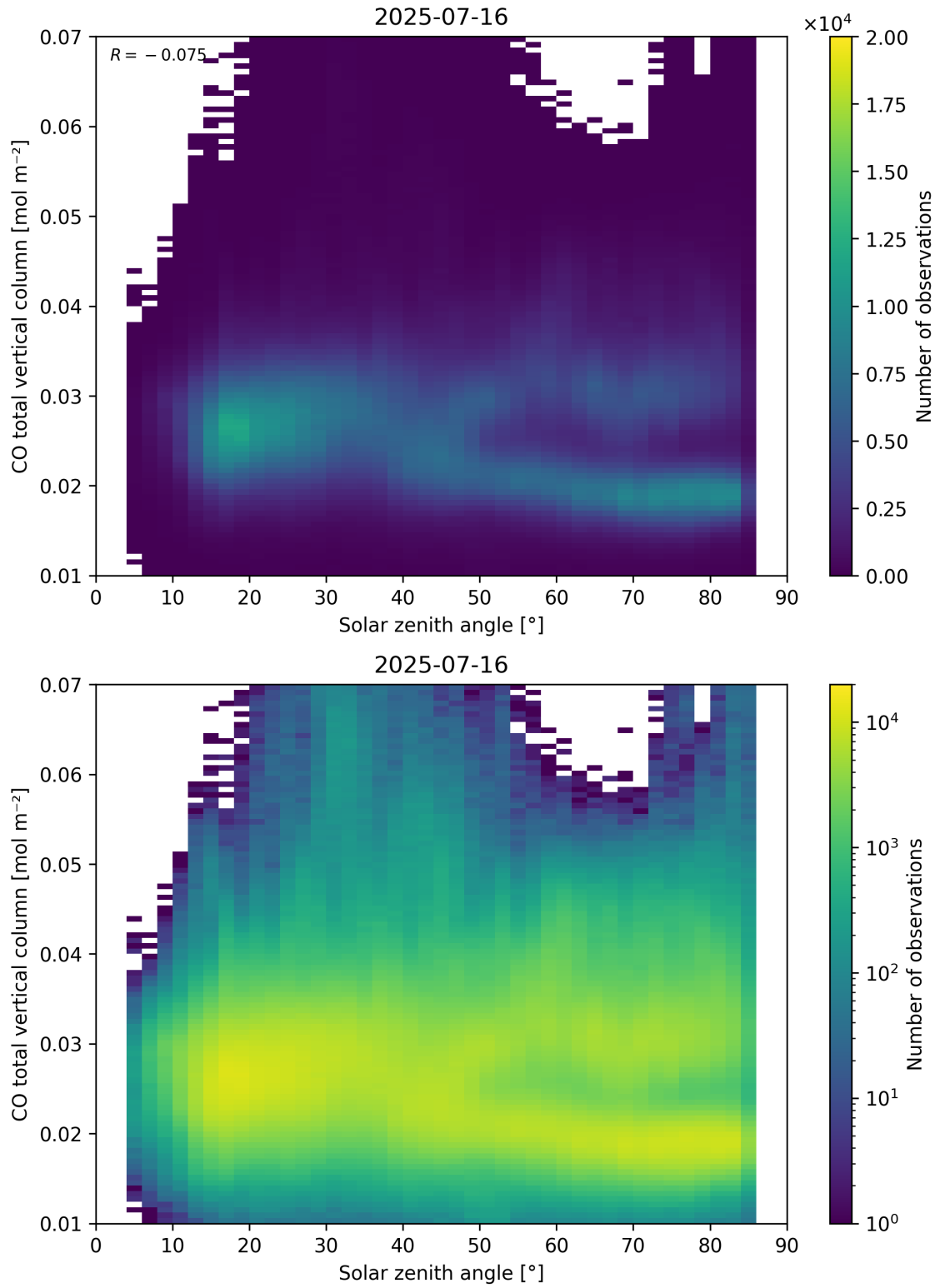
Figure 61: Scatter density plot of “Solar zenith angle” against “CO total vertical column” for 2025-07-15 to 2025-07-17.
