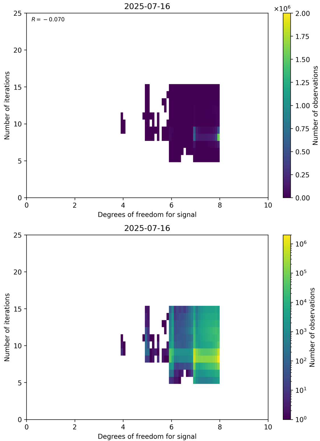
Figure 50: Scatter density plot of “Degrees of freedom for signal” against “Number of iterations” for 2025-07-15 to 2025-07-17.
