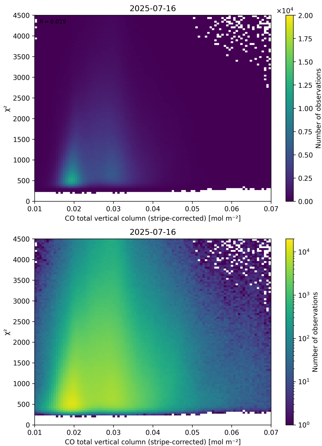
Figure 37: Scatter density plot of “CO total vertical column (stripe-corrected)” against “ \chi^2 ” for 2025-07-15 to 2025-07-17.
