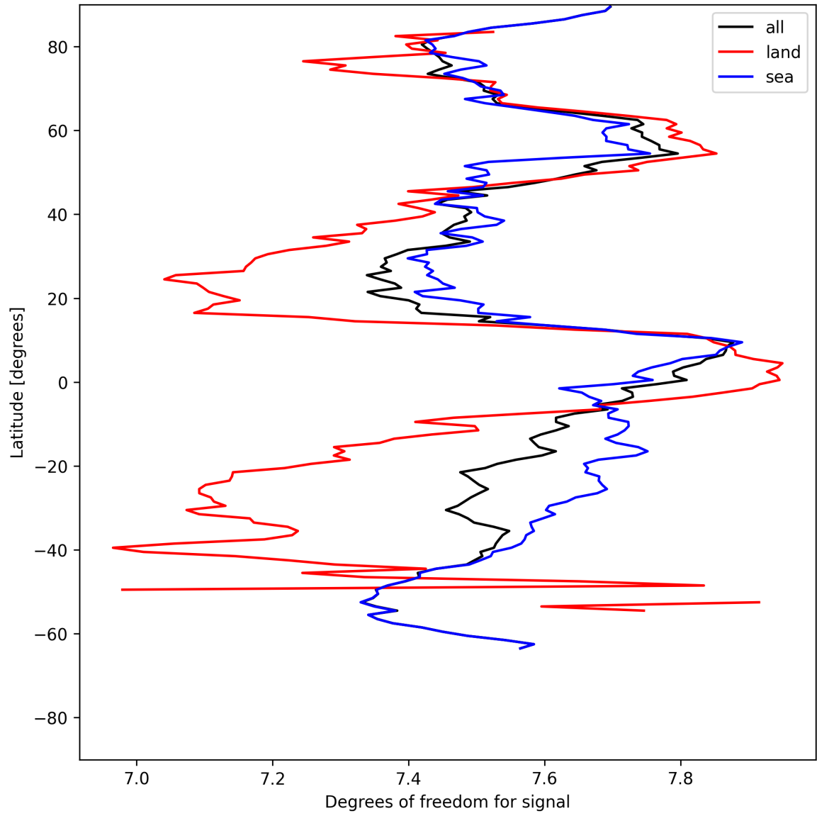
Figure 15: Zonal average of “Degrees of freedom for signal” for 2025-07-15 to 2025-07-17.
