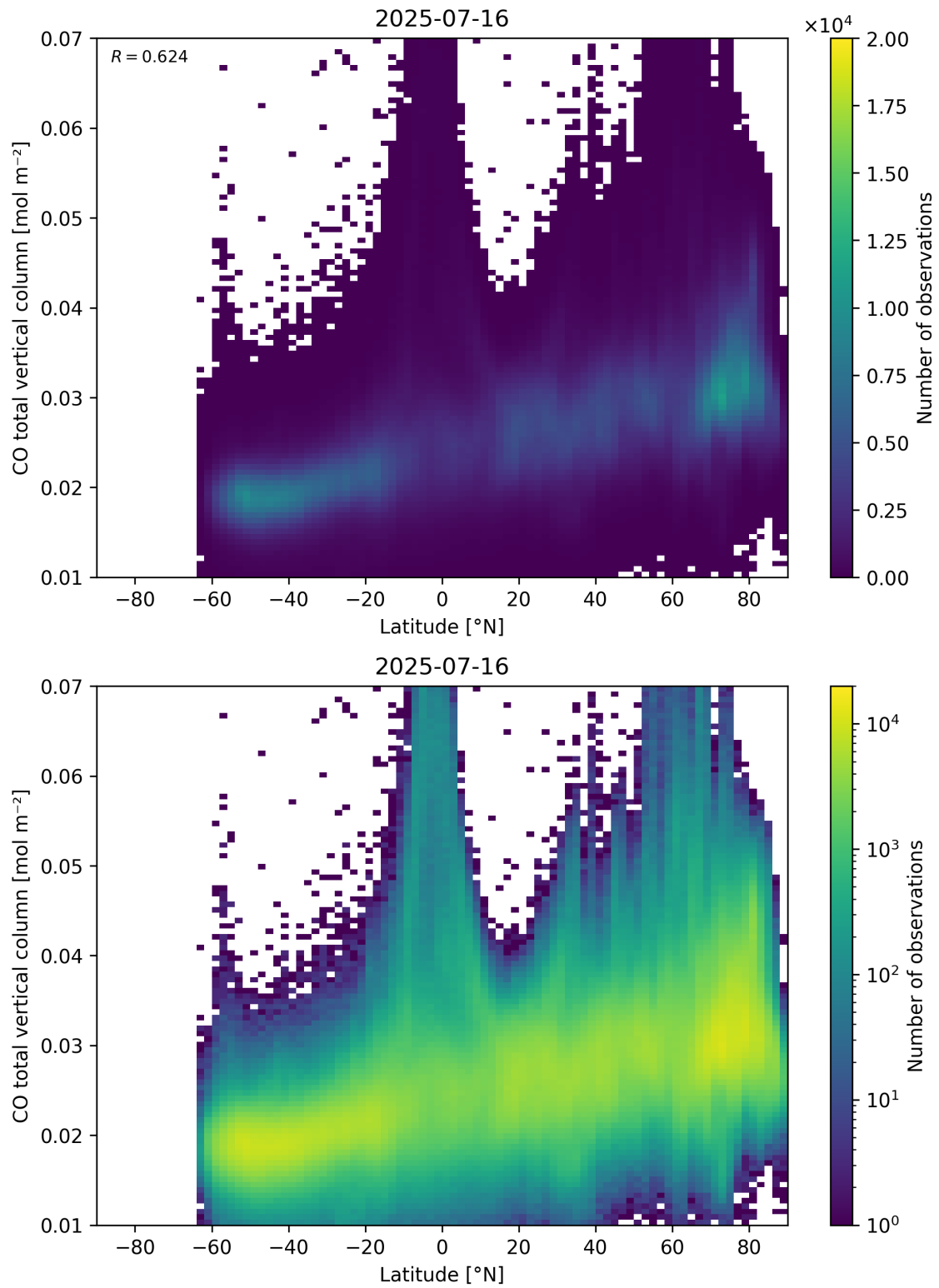
Figure 51: Scatter density plot of “Latitude” against “CO total vertical column” for 2025-07-15 to 2025-07-17.
