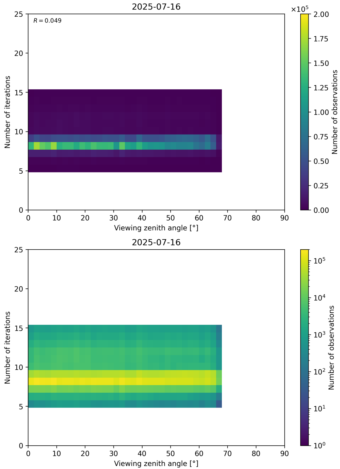
Figure 75: Scatter density plot of “Viewing zenith angle” against “Number of iterations” for 2025-07-15 to 2025-07-17.
