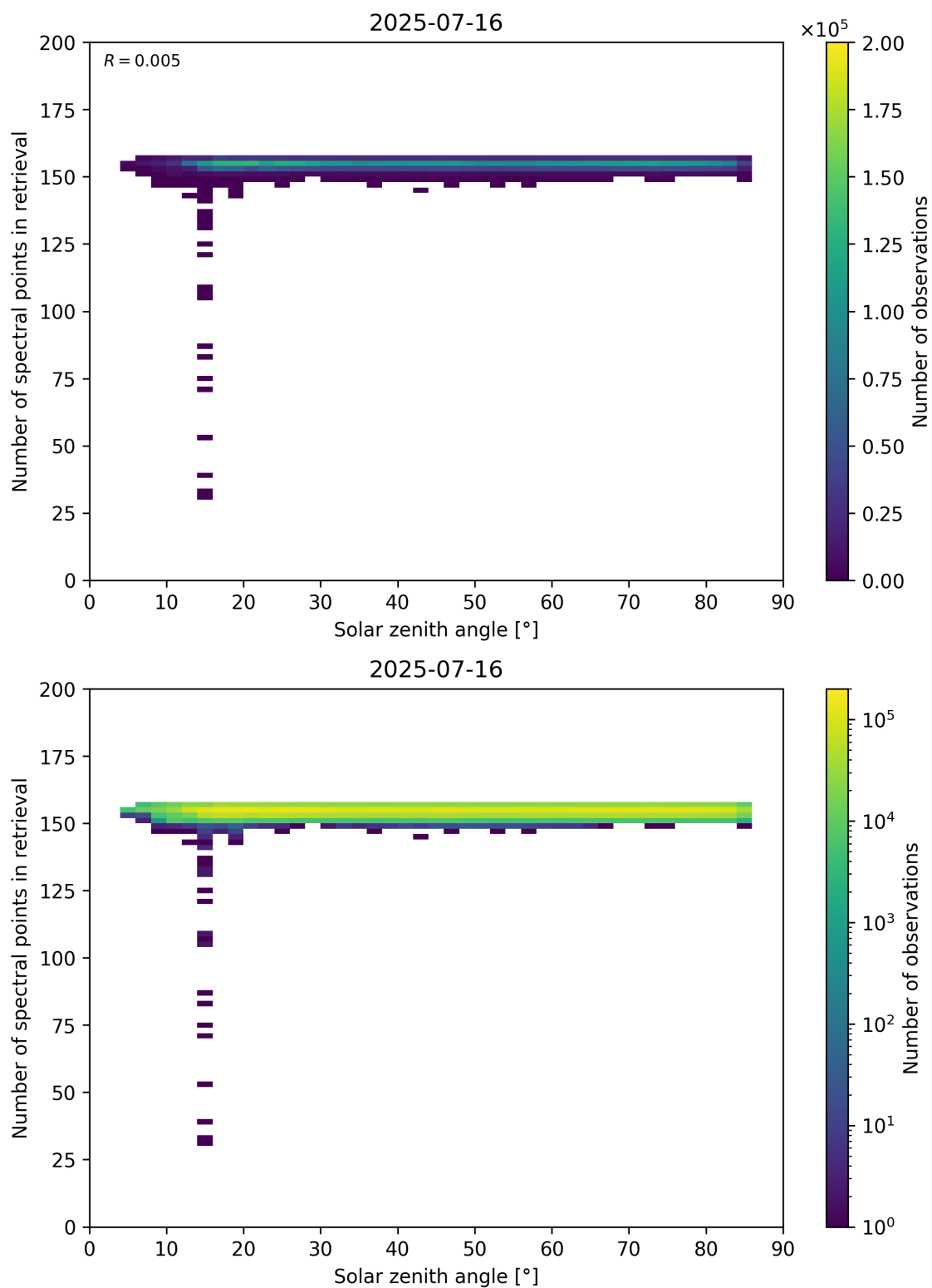
Figure 68: Scatter density plot of “Solar zenith angle” against “Number of spectral points in retrieval” for 2025-07-15 to 2025-07-17.
