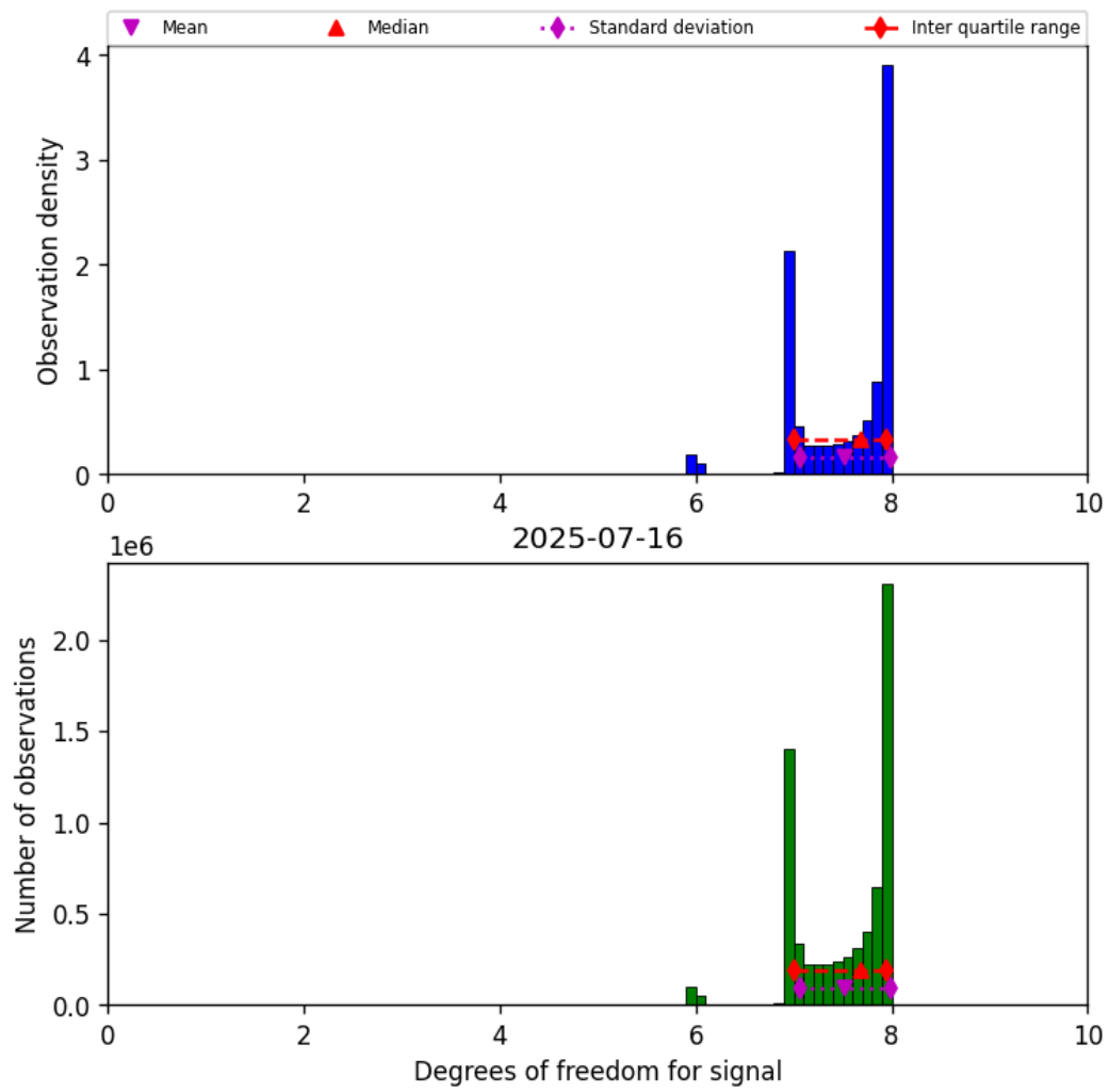
Figure 23: Histogram of “Degrees of freedom for signal” for 2025-07-15 to 2025-07-17
