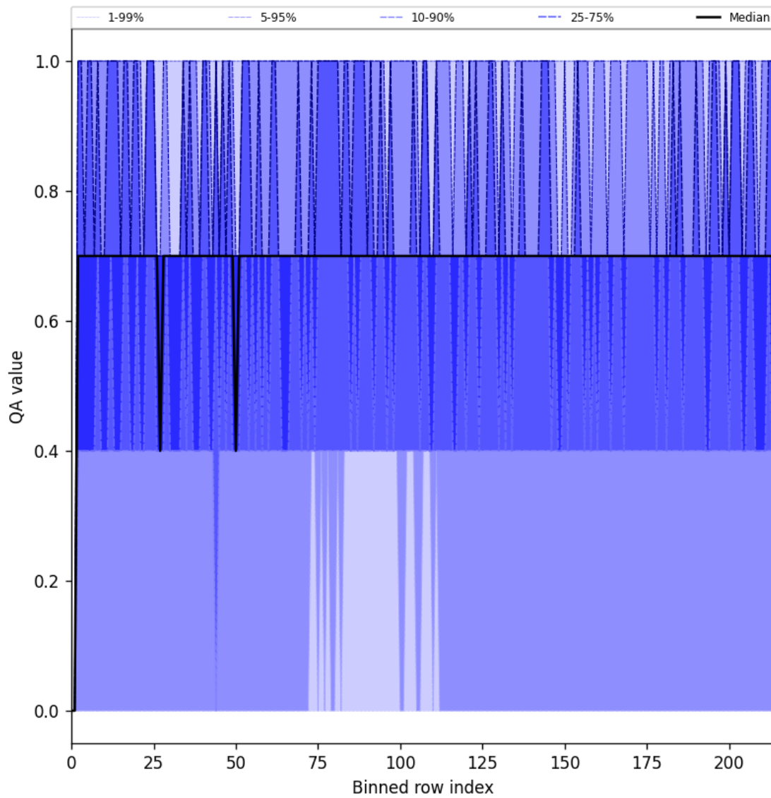
Figure 25: Along track statistics of “QA value” for 2025-07-15 to 2025-07-17
