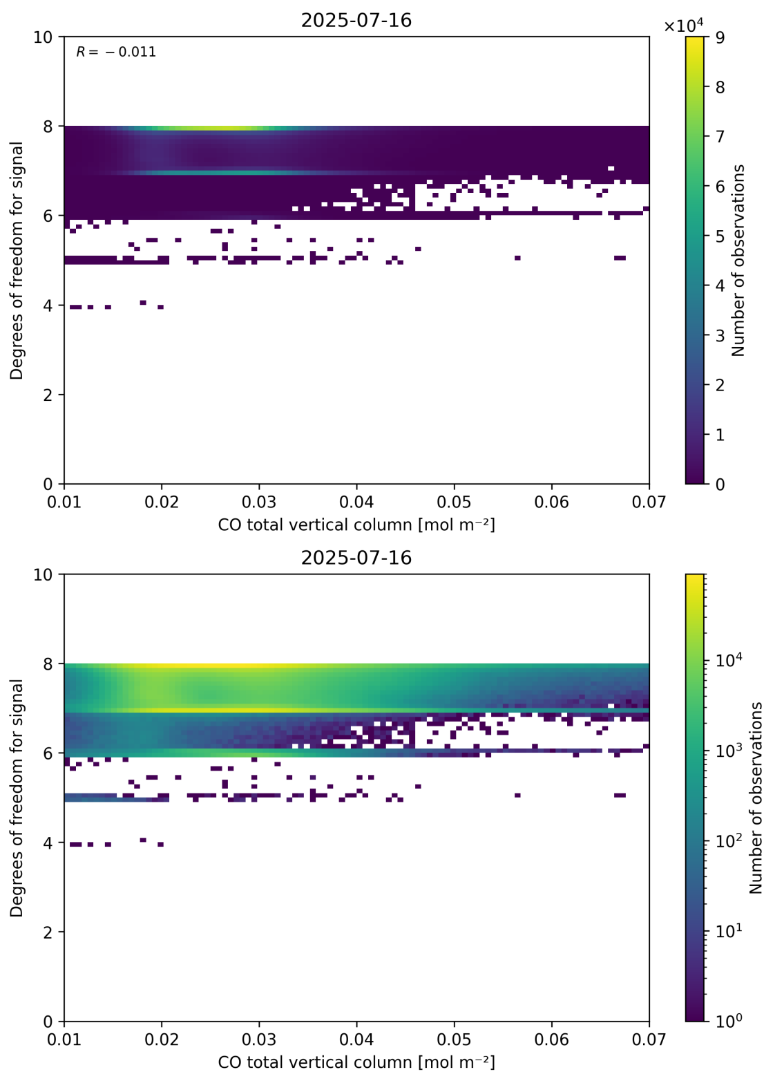
Figure 41: Scatter density plot of “CO total vertical column” against “Degrees of freedom for signal” for 2025-07-15 to 2025-07-17.
