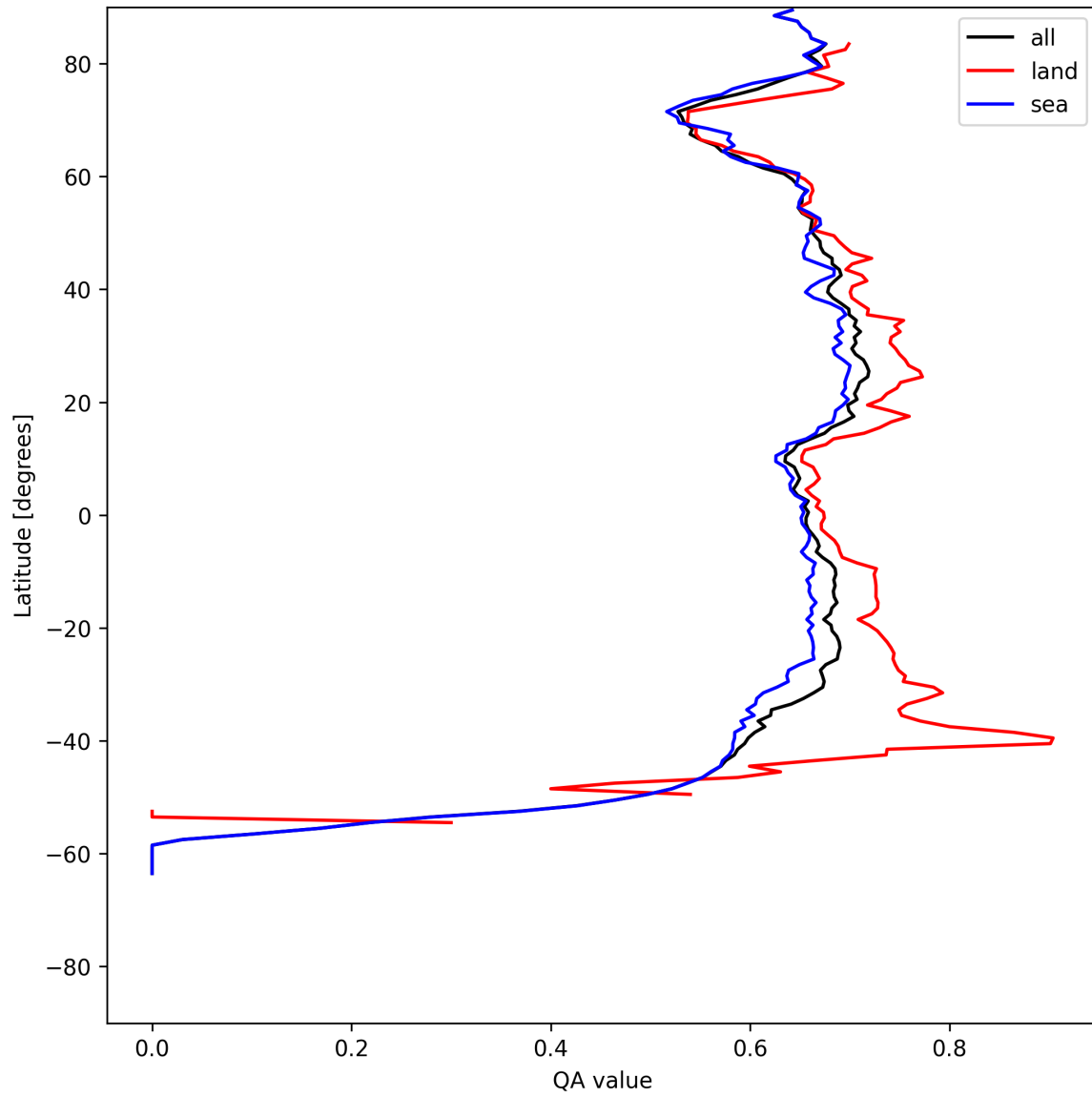
Figure 9: Zonal average of “QA value” for 2025-07-15 to 2025-07-17.
