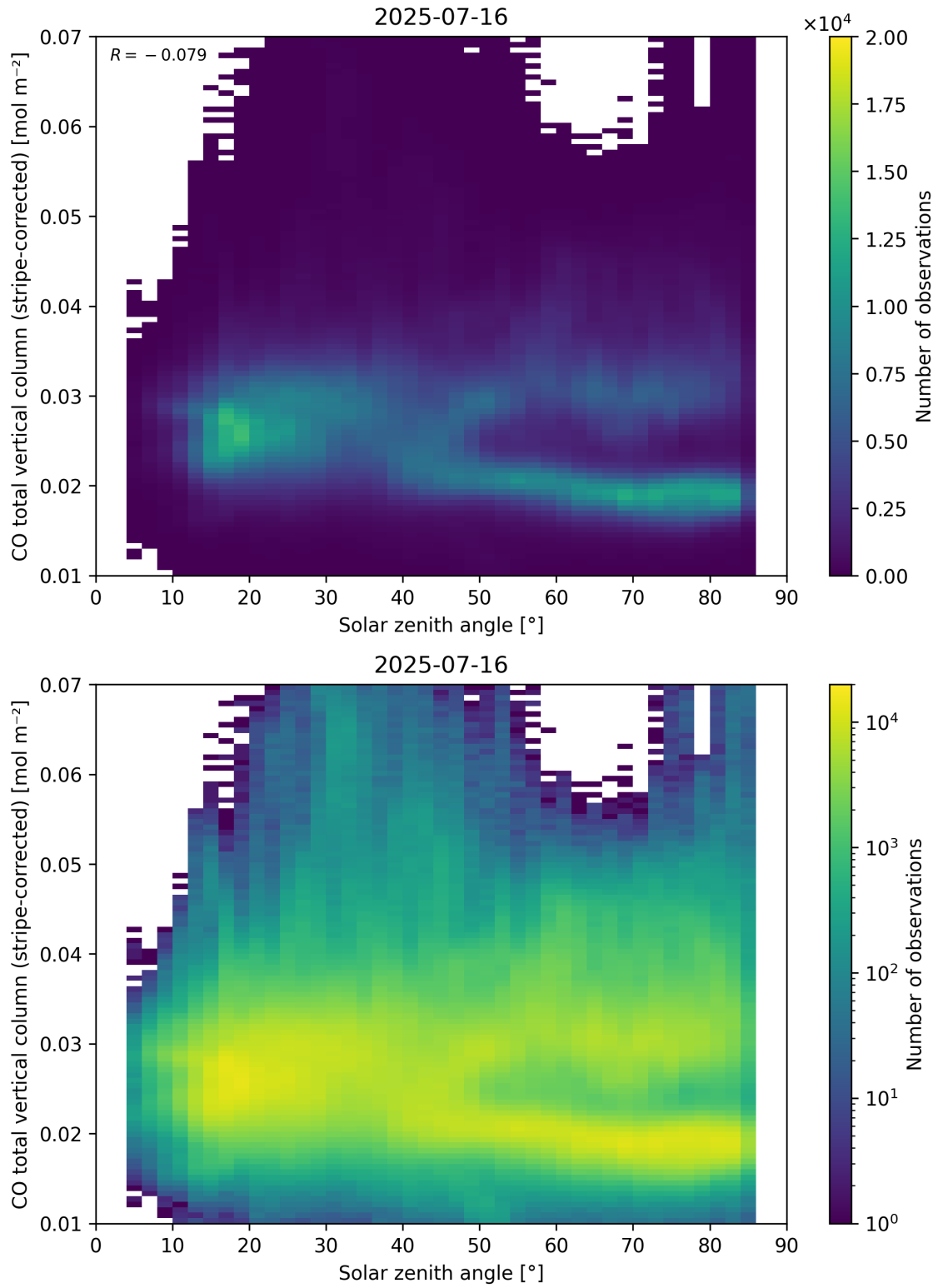
Figure 62: Scatter density plot of “Solar zenith angle” against “CO total vertical column (stripe-corrected)” for 2025-07-15 to 2025-07-17.
