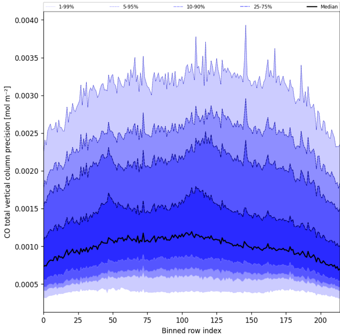
Figure 28: Along track statistics of “CO total vertical column precision” for 2025-07-15 to 2025-07-17
