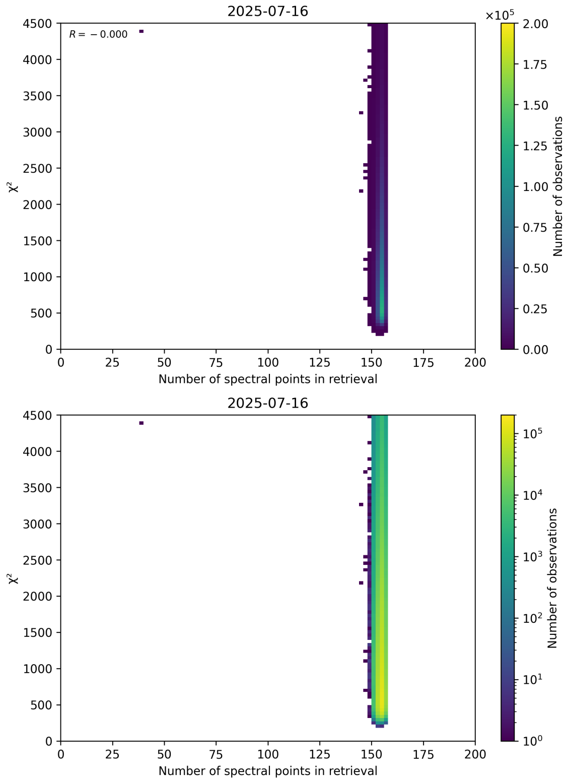
Figure 58: Scatter density plot of “Number of spectral points in retrieval” against “ \chi^2 ” for 2025-07-15 to 2025-07-17.
