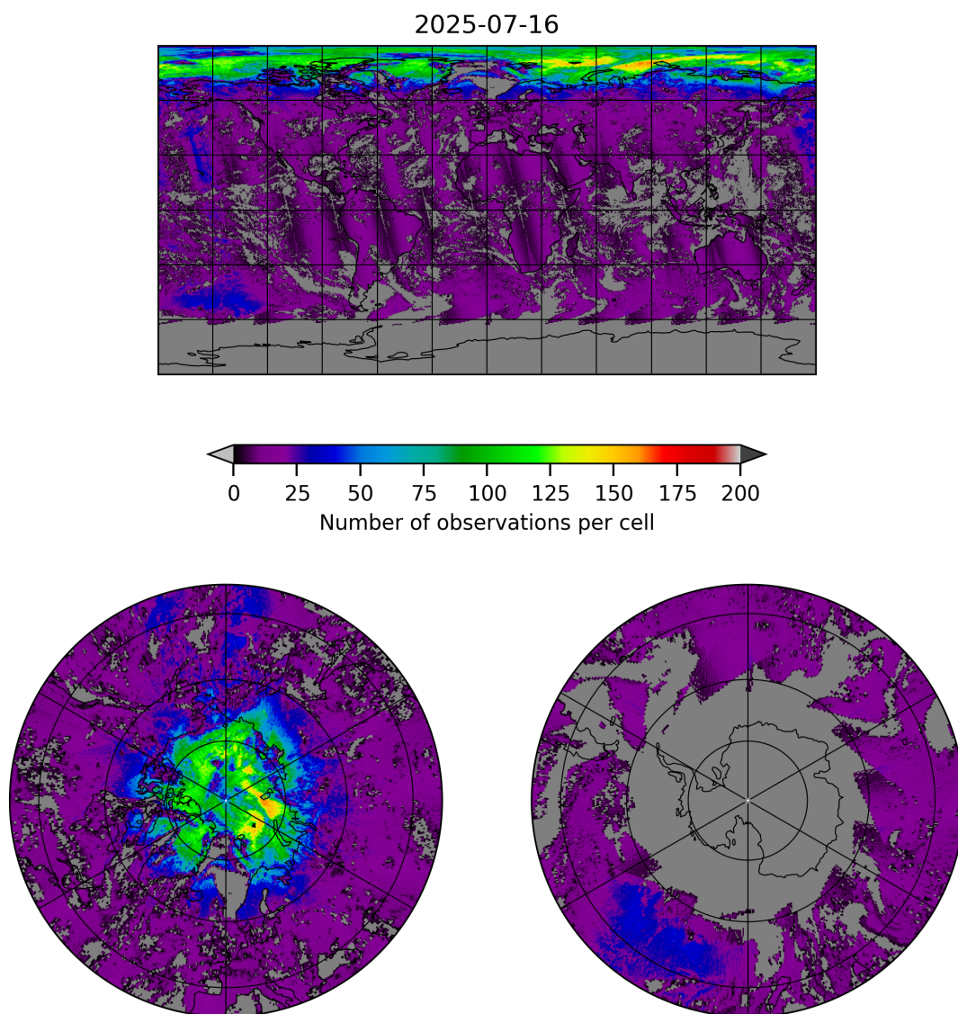
Figure 8: Map of the number of observations for 2025-07-15 to 2025-07-17
