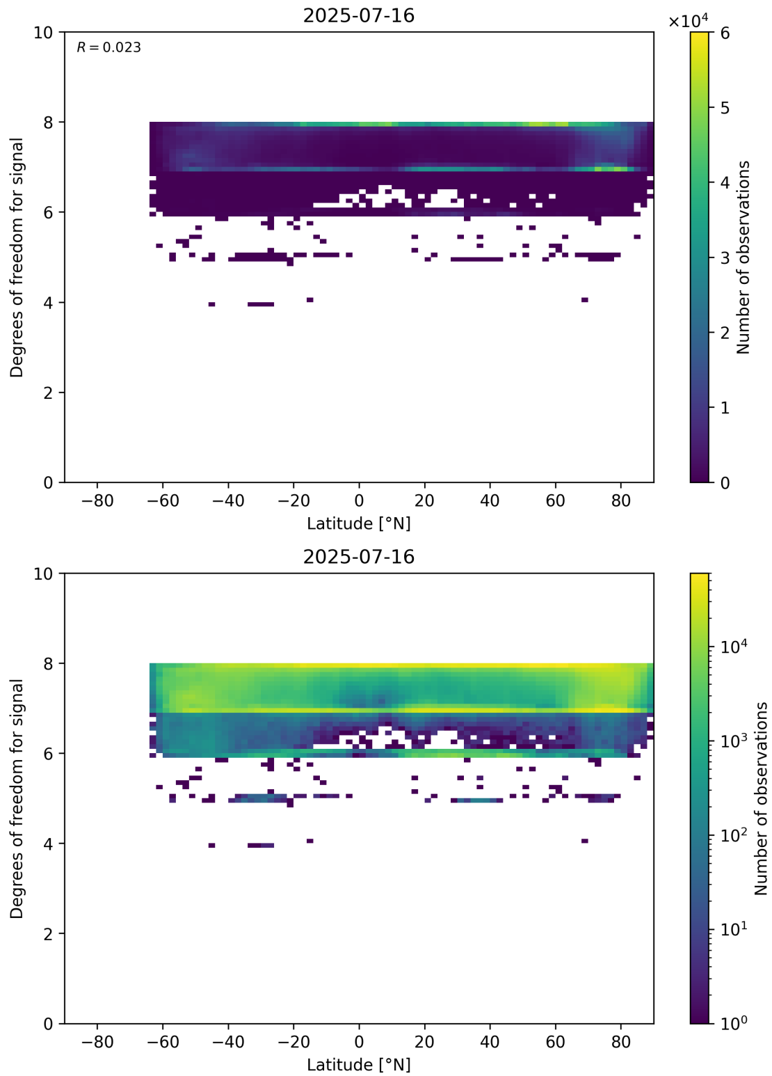
Figure 55: Scatter density plot of “Latitude” against “Degrees of freedom for signal” for 2025-07-15 to 2025-07-17.
