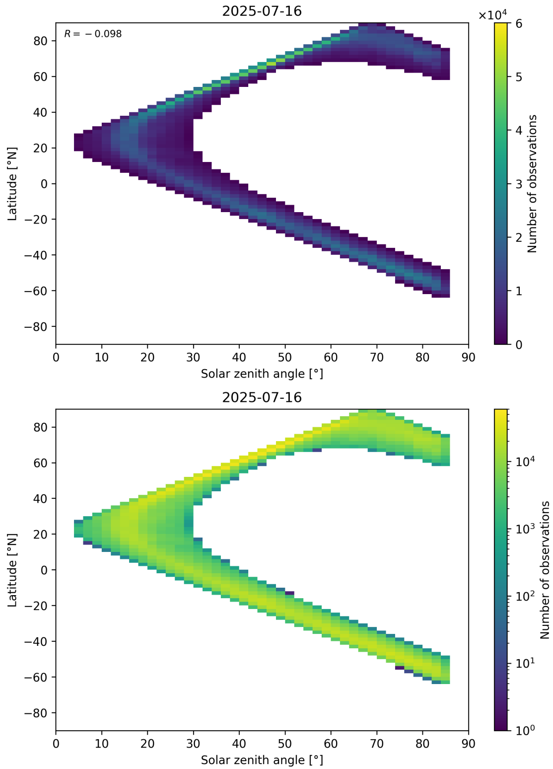
Figure 66: Scatter density plot of “Solar zenith angle” against “Latitude” for 2025-07-15 to 2025-07-17.
