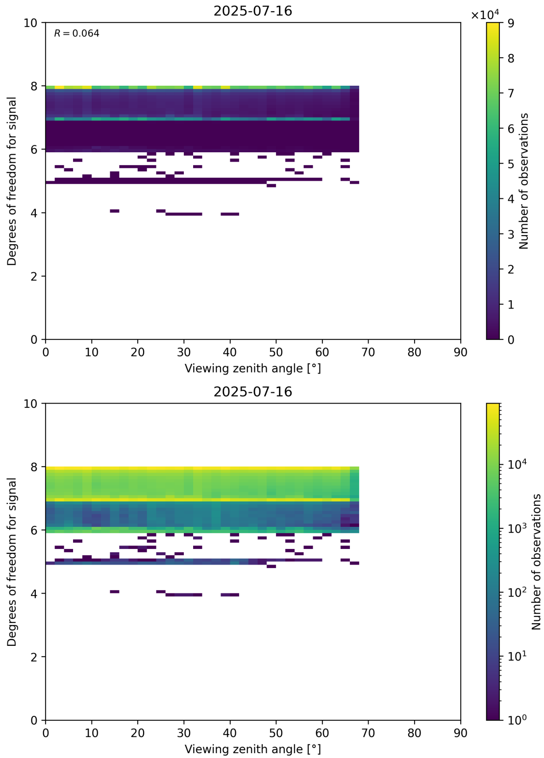
Figure 73: Scatter density plot of “Viewing zenith angle” against “Degrees of freedom for signal” for 2025-07-15 to 2025-07-17.
