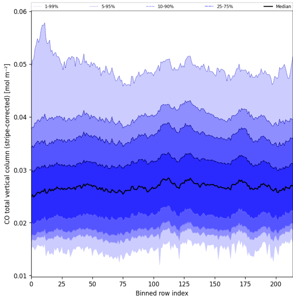
Figure 27: Along track statistics of “CO total vertical column (stripe-corrected)” for 2025-07-15 to 2025-07-17
