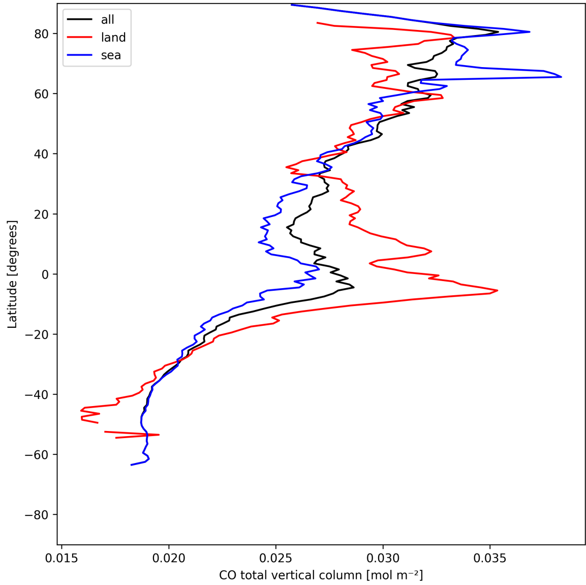
Figure 10: Zonal average of “CO total vertical column” for 2025-07-15 to 2025-07-17.
