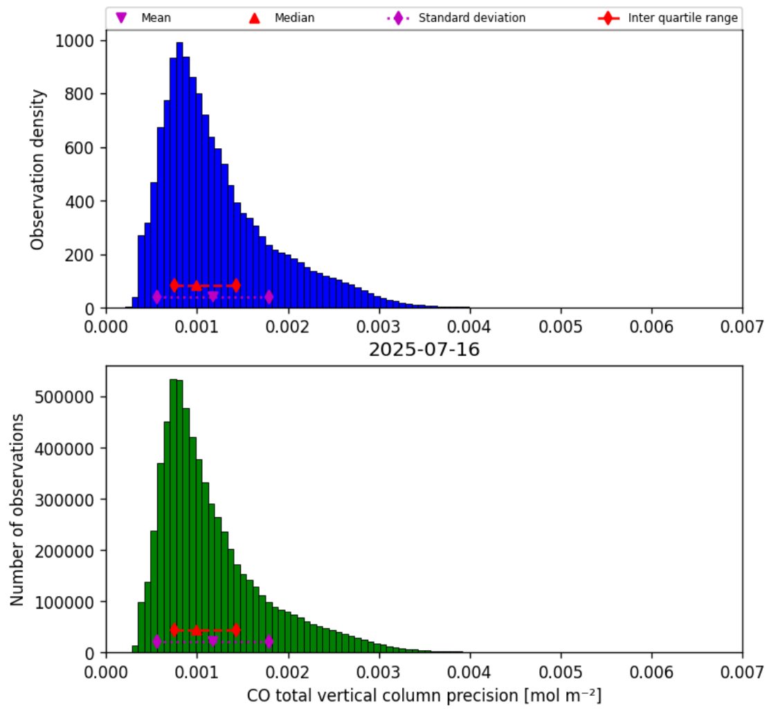
Figure 20: Histogram of “CO total vertical column precision” for 2025-07-15 to 2025-07-17
