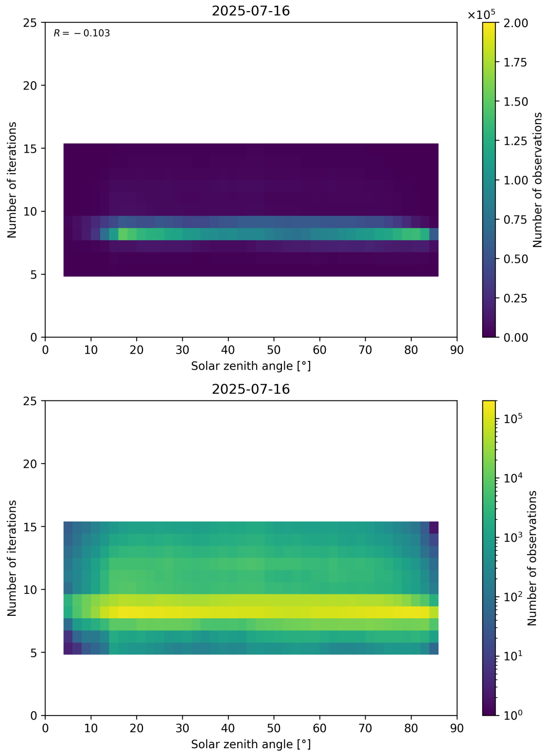
Figure 67: Scatter density plot of “Solar zenith angle” against “Number of iterations” for 2025-07-15 to 2025-07-17.
