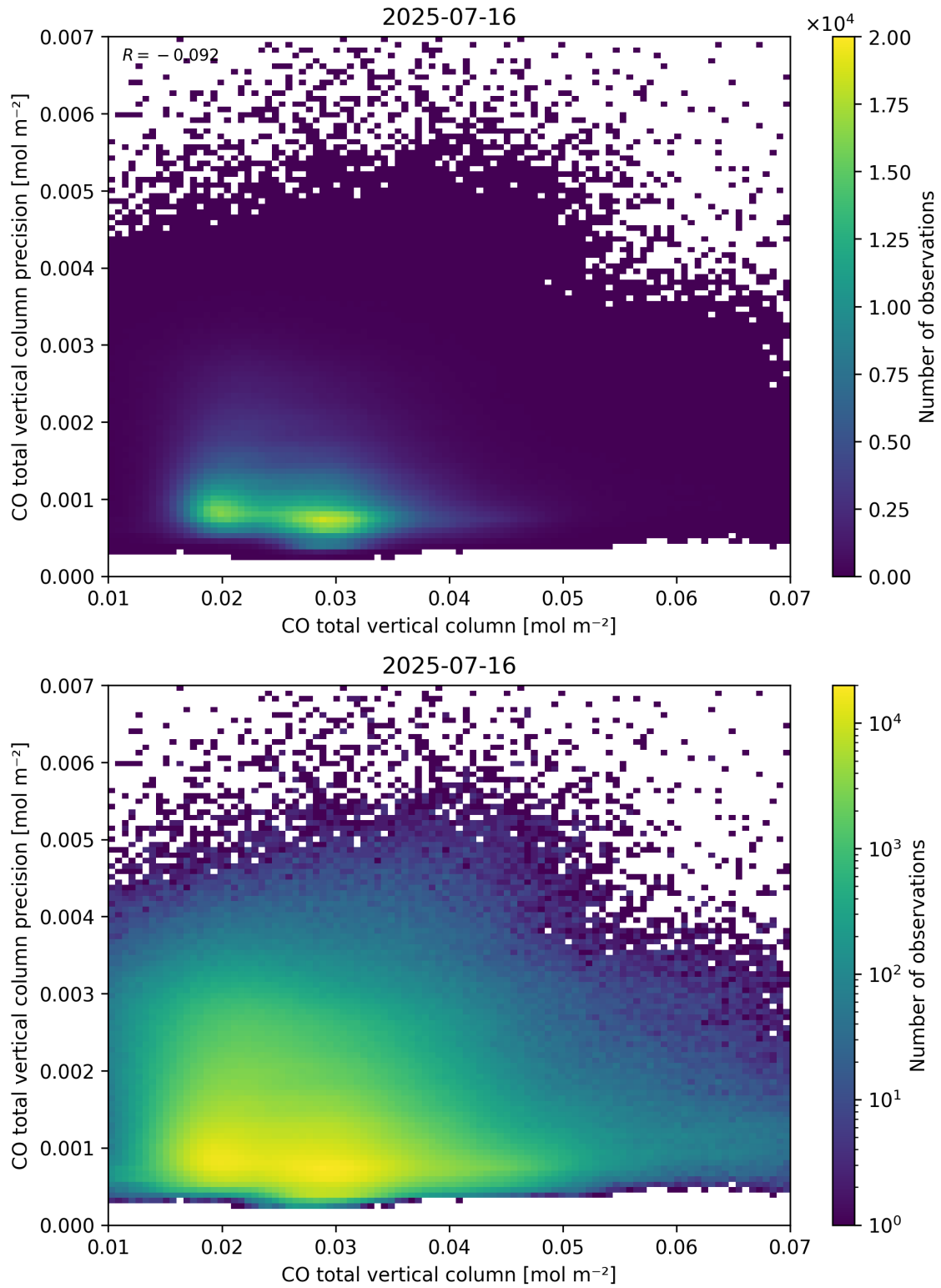
Figure 34: Scatter density plot of “CO total vertical column” against “CO total vertical column precision” for 2025-07-15 to 2025-07-17.
