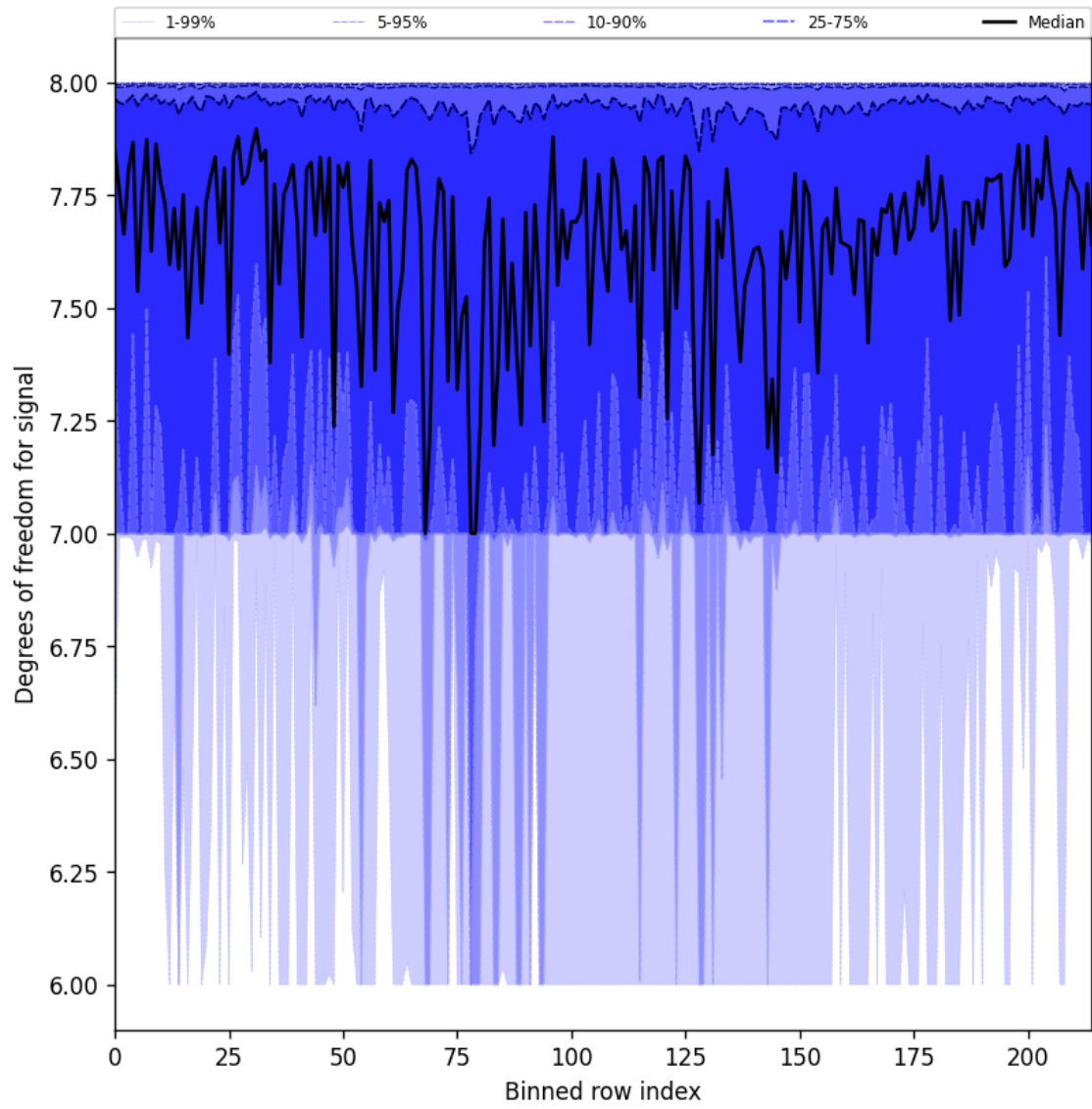
Figure 31: Along track statistics of “Degrees of freedom for signal” for 2025-07-15 to 2025-07-17
