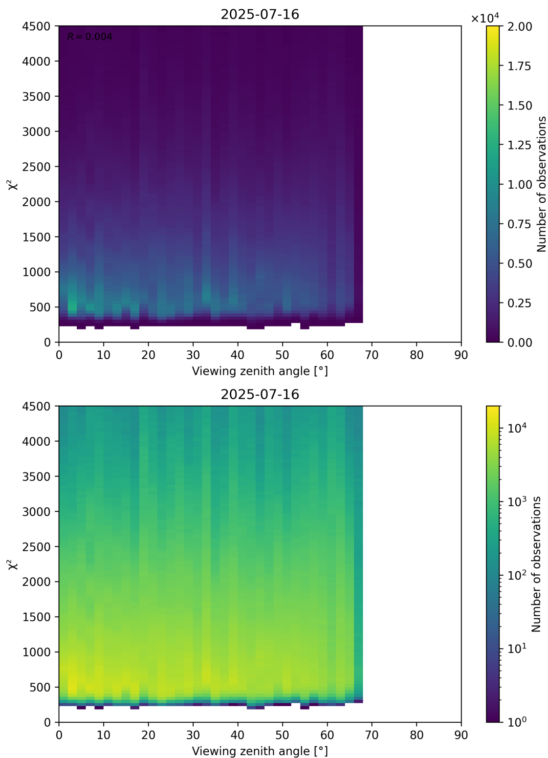
Figure 72: Scatter density plot of “Viewing zenith angle” against “ \chi^2 ” for 2025-07-15 to 2025-07-17.
