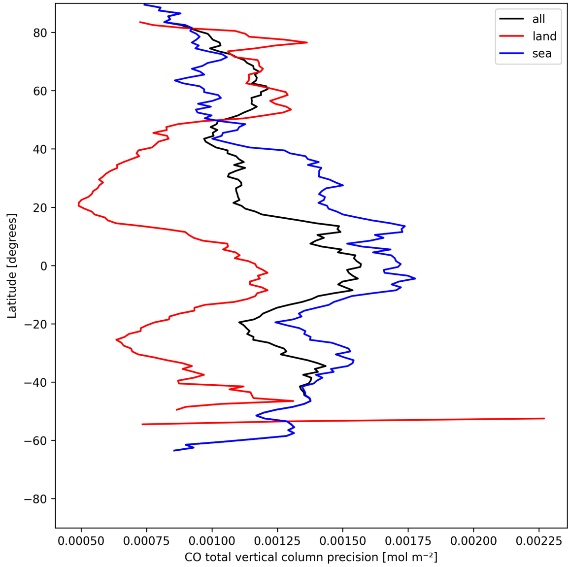
Figure 12: Zonal average of “CO total vertical column precision” for 2025-07-15 to 2025-07-17.
