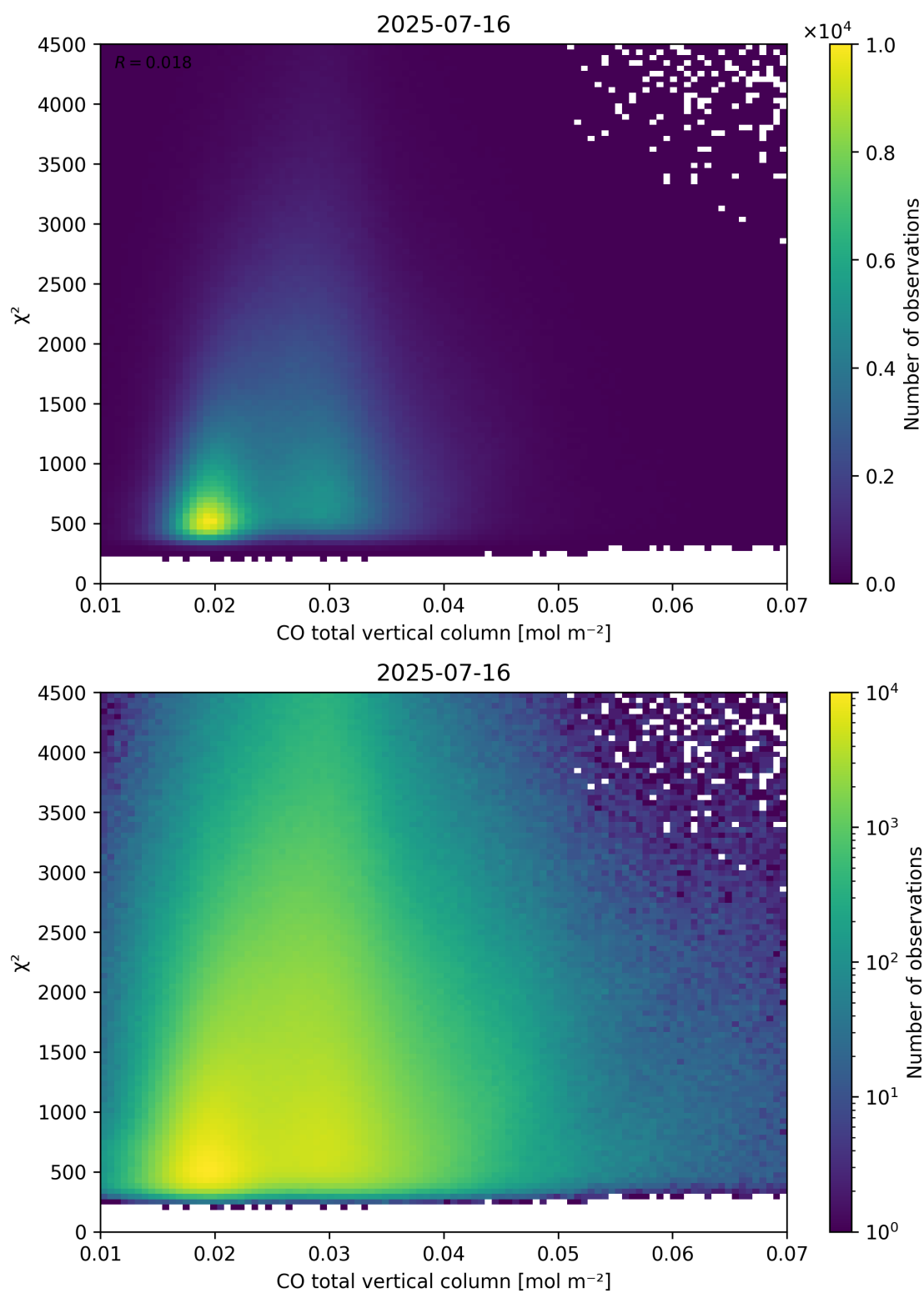
Figure 35: Scatter density plot of “CO total vertical column” against “ \chi^2 ” for 2025-07-15 to 2025-07-17.
