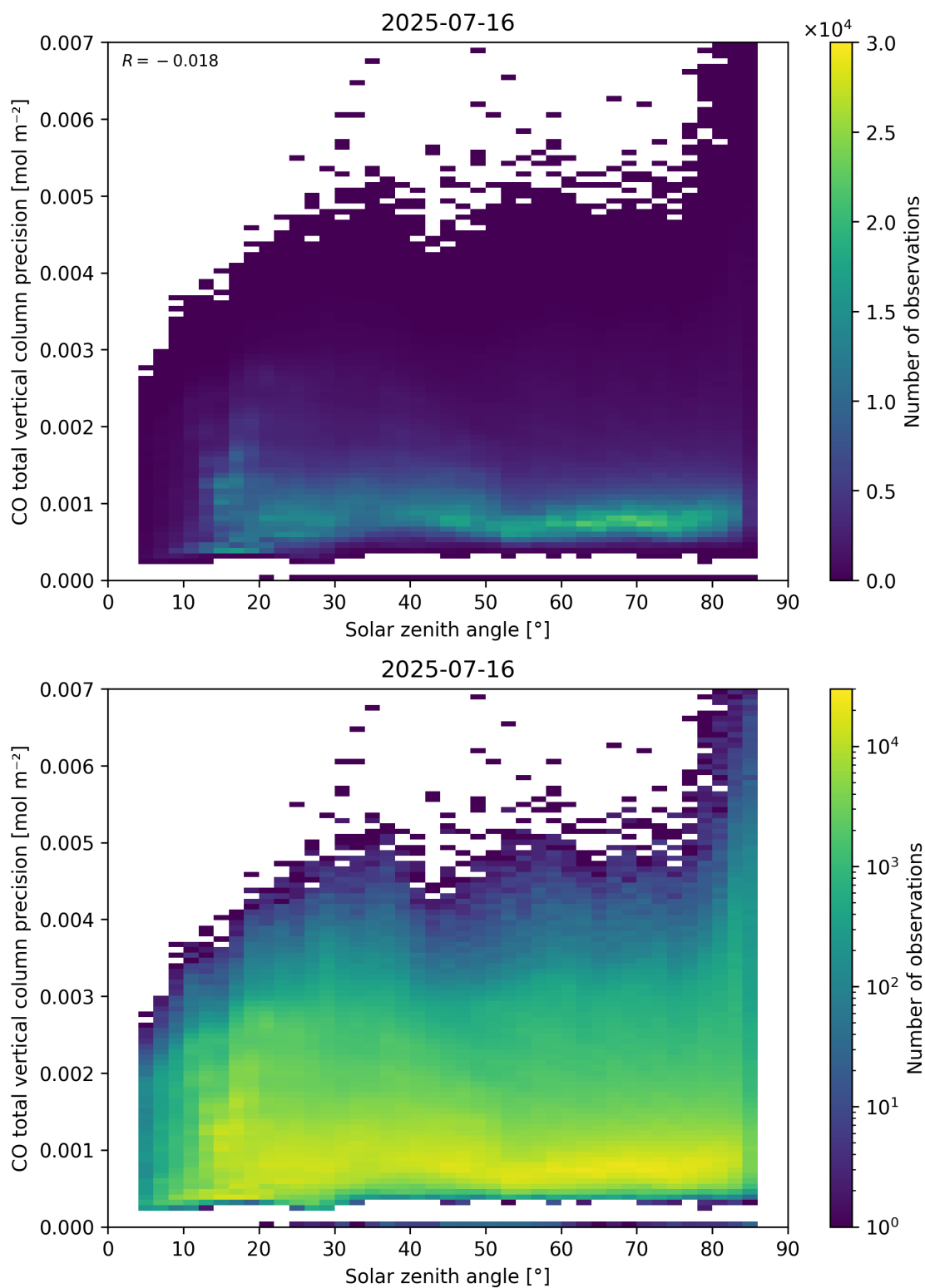
Figure 63: Scatter density plot of “Solar zenith angle” against “CO total vertical column precision” for 2025-07-15 to 2025-07-17.
