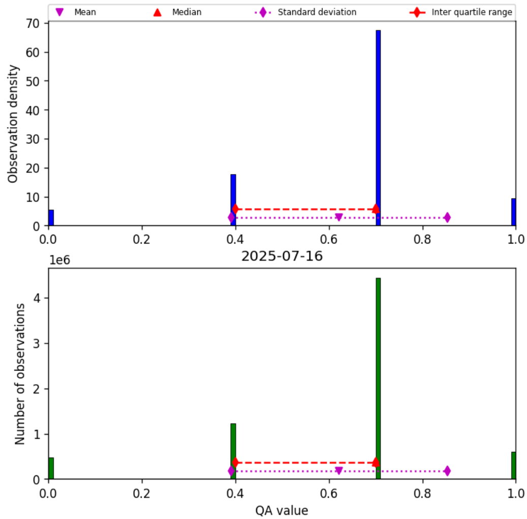
Figure 17: Histogram of “QA value” for 2025-07-15 to 2025-07-17
