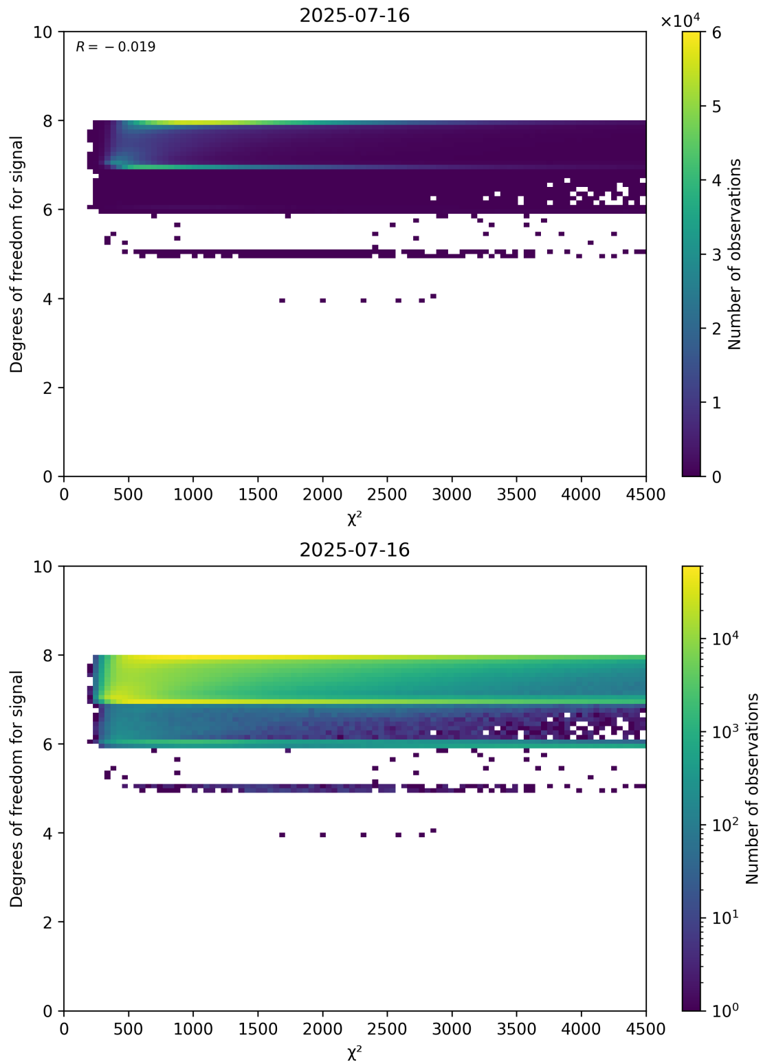
Figure 48: Scatter density plot of “ \chi^2 ” against “Degrees of freedom for signal” for 2025-07-15 to 2025-07-17.
