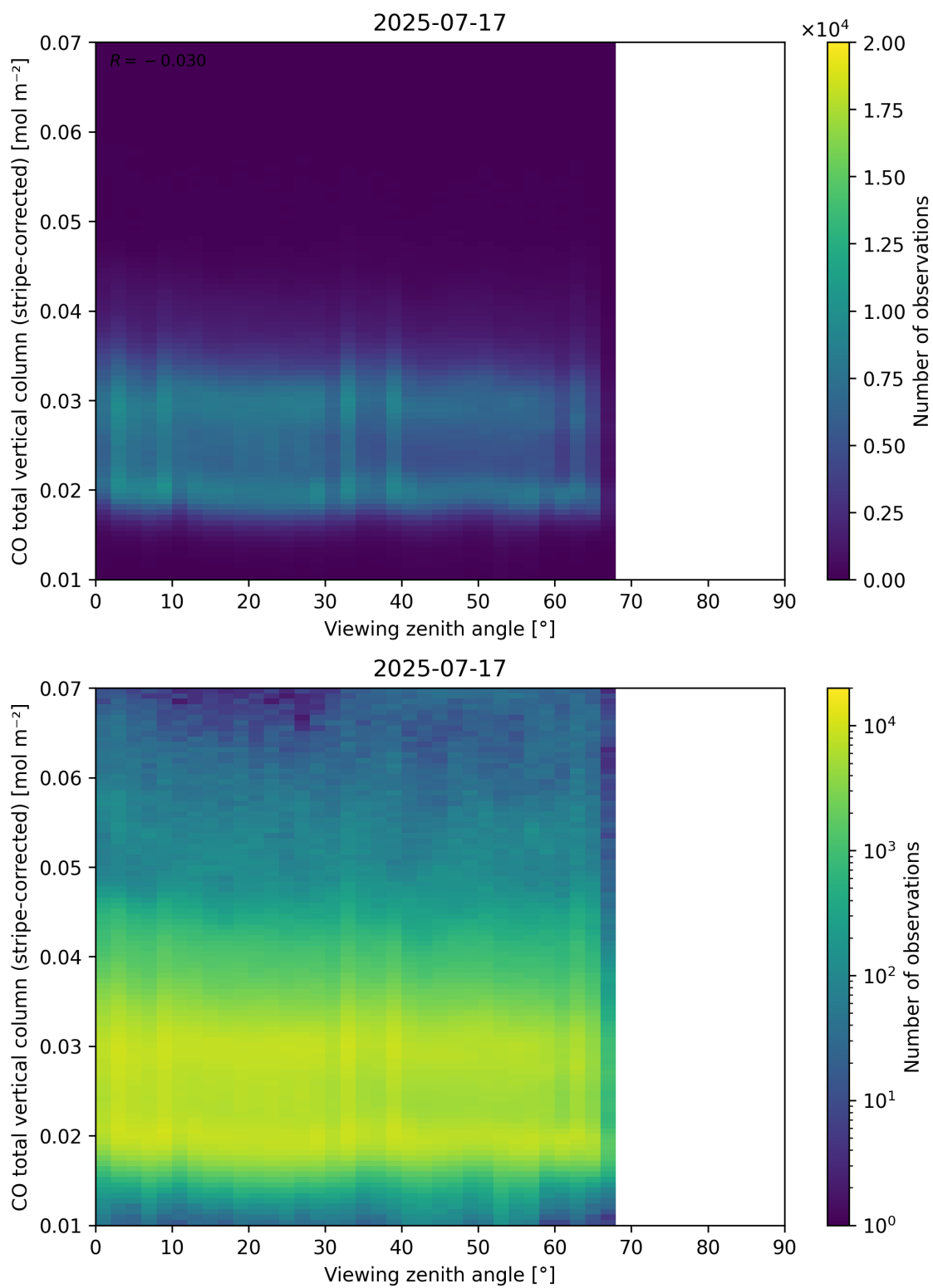
Figure 70: Scatter density plot of “Viewing zenith angle” against “CO total vertical column (stripe-corrected)” for 2025-07-16 to 2025-07-18.
