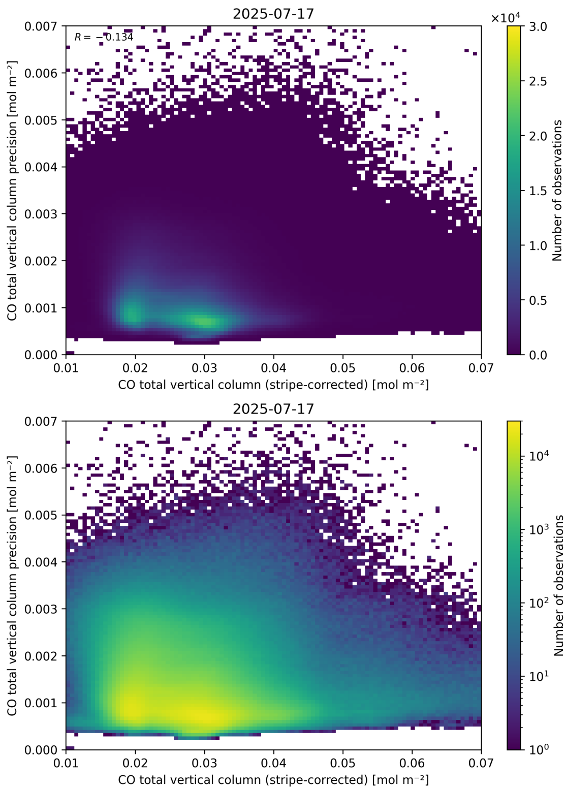
Figure 36: Scatter density plot of “CO total vertical column (stripe-corrected)” against “CO total vertical column precision” for 2025-07-16 to 2025-07-18.
