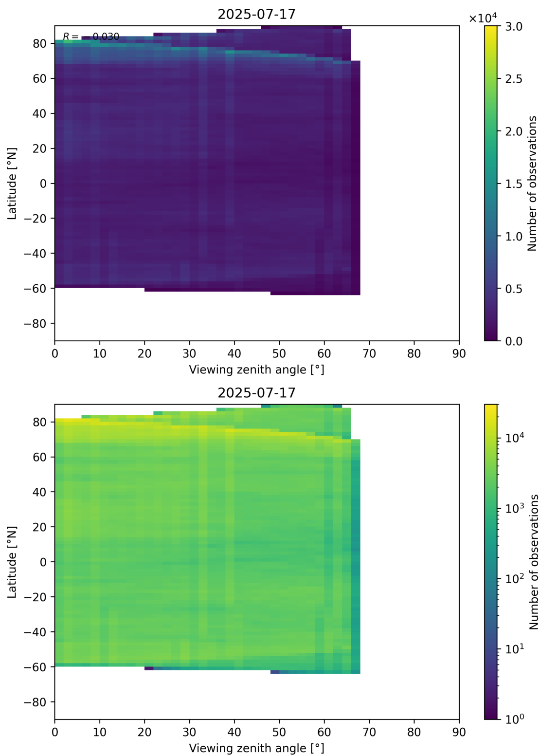
Figure 74: Scatter density plot of “Viewing zenith angle” against “Latitude” for 2025-07-16 to 2025-07-18.
