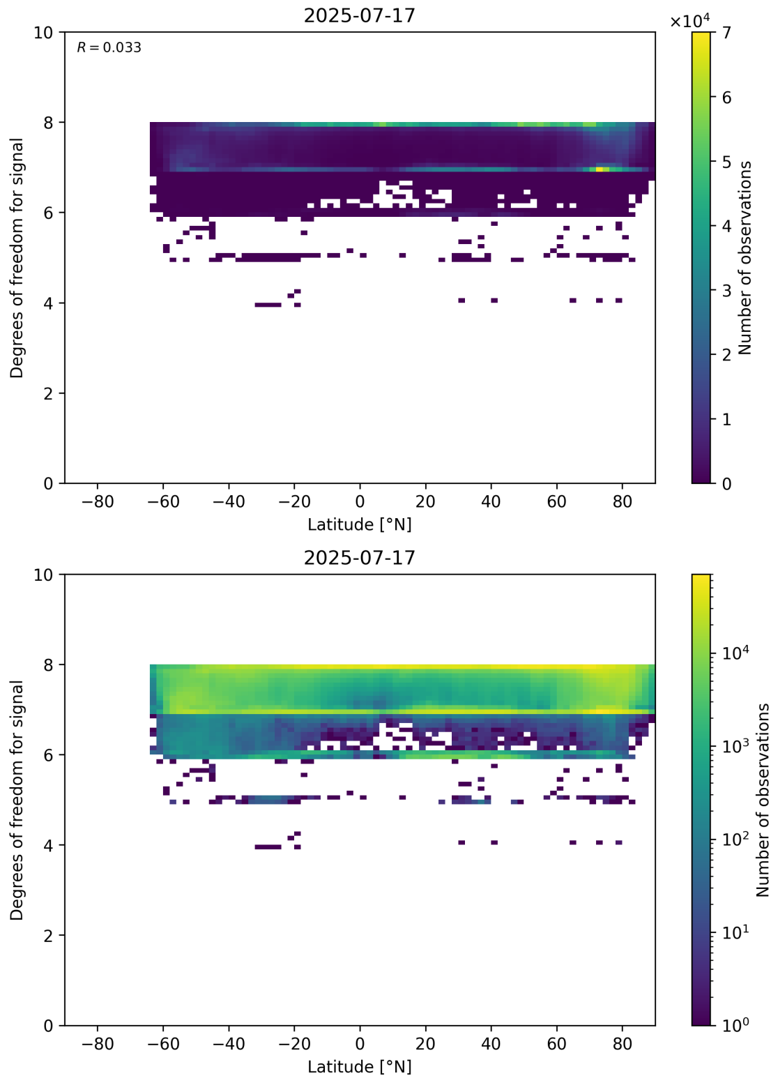
Figure 55: Scatter density plot of “Latitude” against “Degrees of freedom for signal” for 2025-07-16 to 2025-07-18.
