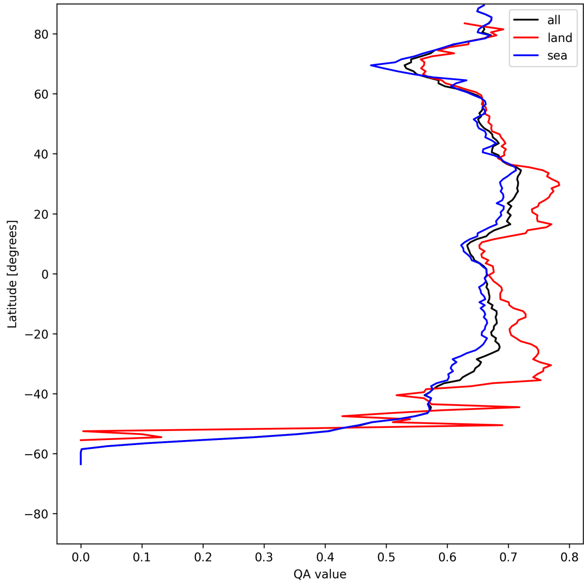
Figure 9: Zonal average of “QA value” for 2025-07-16 to 2025-07-18.
