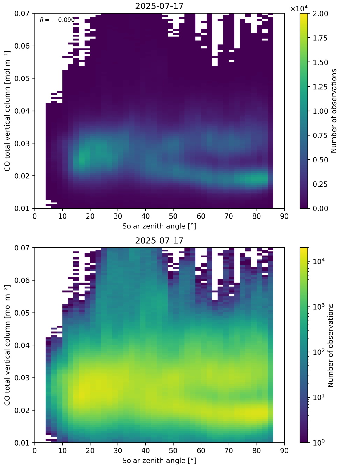
Figure 61: Scatter density plot of “Solar zenith angle” against “CO total vertical column” for 2025-07-16 to 2025-07-18.
