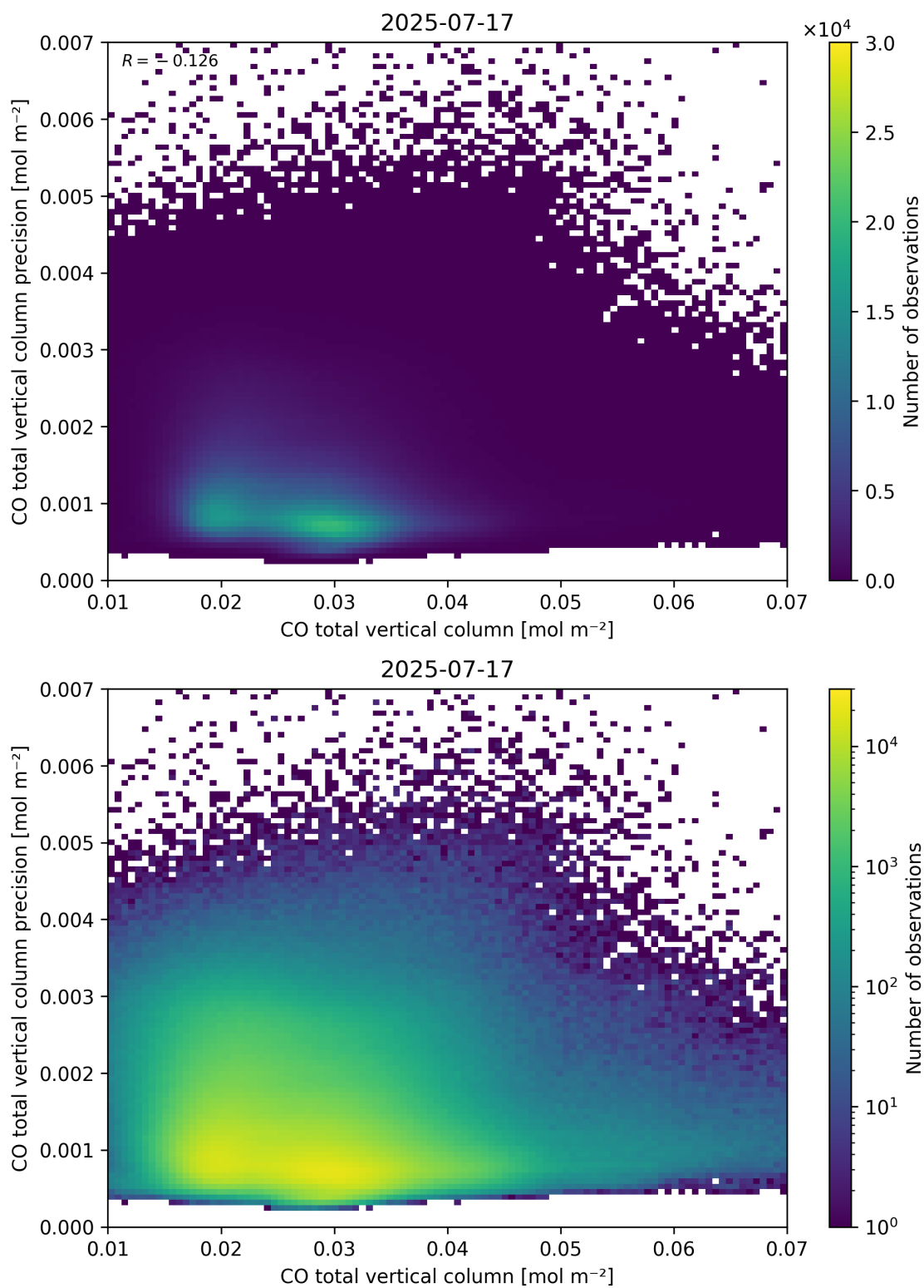
Figure 34: Scatter density plot of “CO total vertical column” against “CO total vertical column precision” for 2025-07-16 to 2025-07-18.
