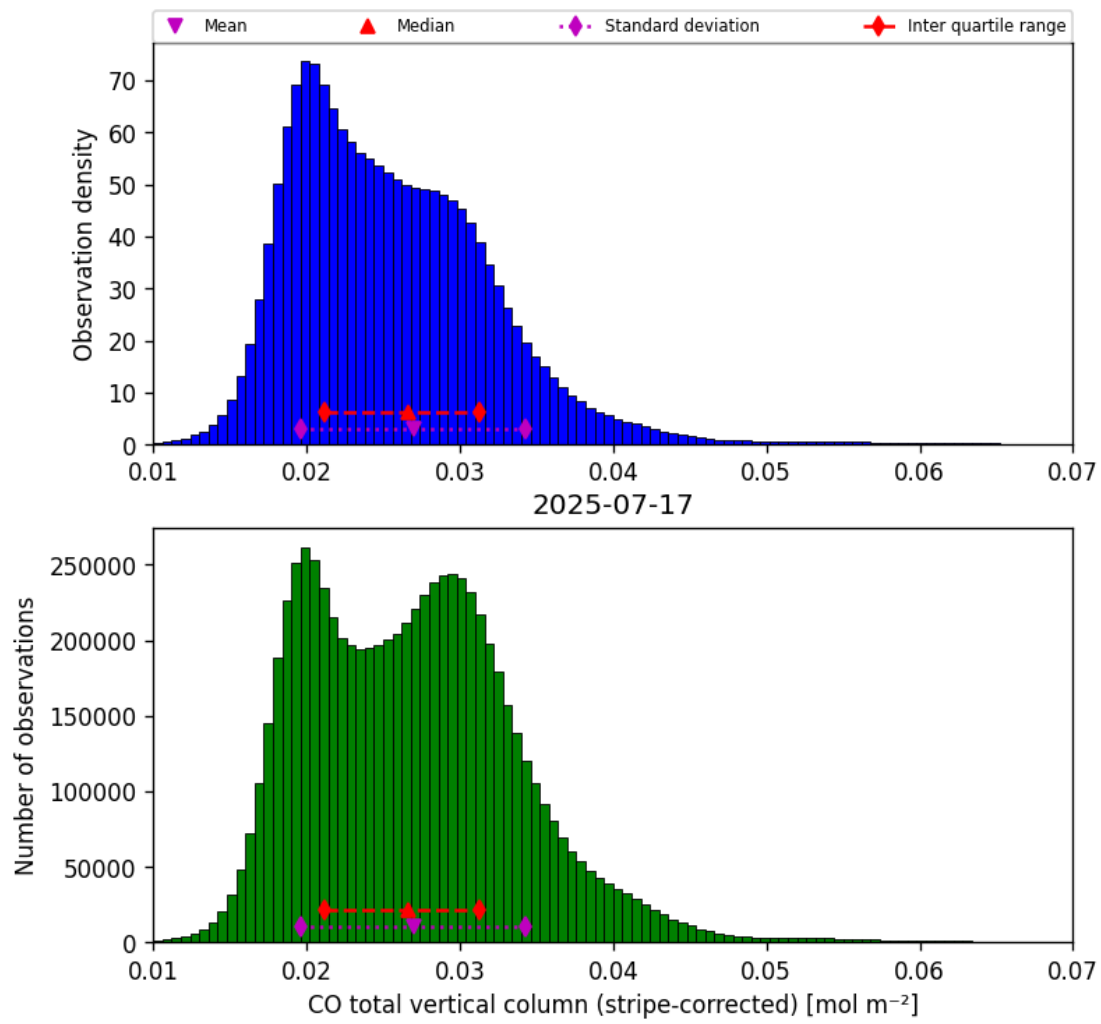
Figure 19: Histogram of “CO total vertical column (stripe-corrected)” for 2025-07-16 to 2025-07-18
