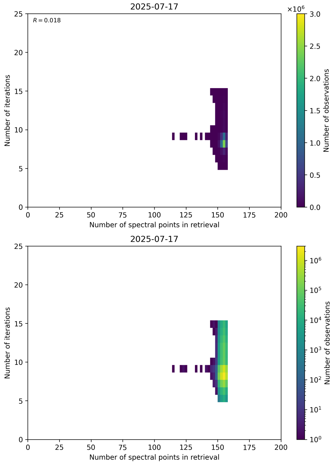
Figure 60: Scatter density plot of “Number of spectral points in retrieval” against “Number of iterations” for 2025-07-16 to 2025-07-18.
