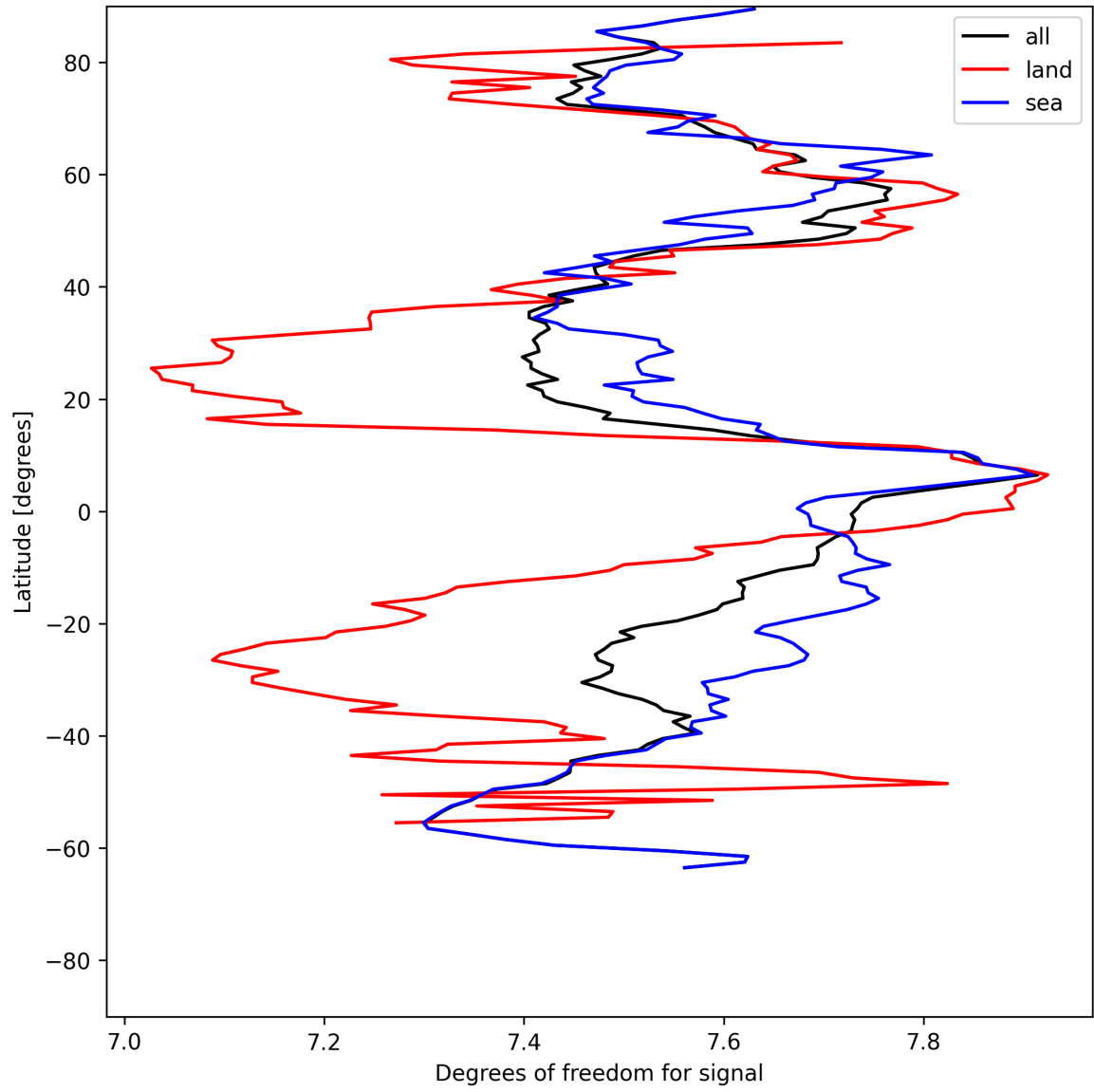
Figure 15: Zonal average of “Degrees of freedom for signal” for 2025-07-16 to 2025-07-18.
