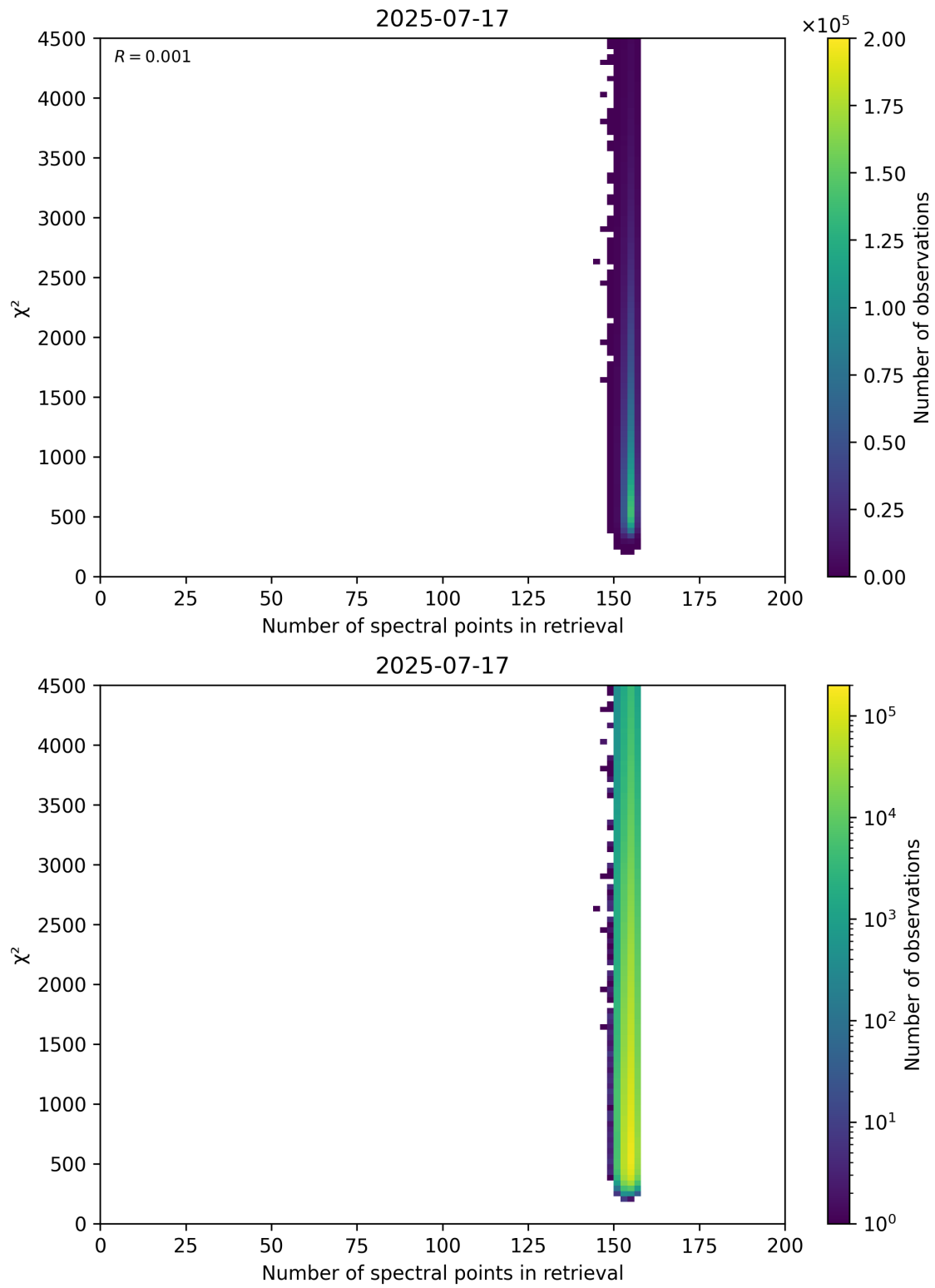
Figure 58: Scatter density plot of “Number of spectral points in retrieval” against “ \chi^2 ” for 2025-07-16 to 2025-07-18.
