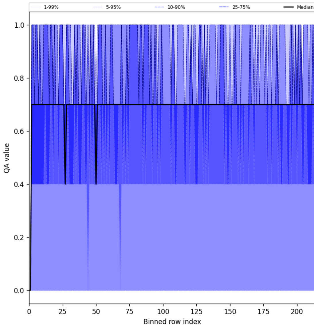
Figure 25: Along track statistics of “QA value” for 2025-07-16 to 2025-07-18
