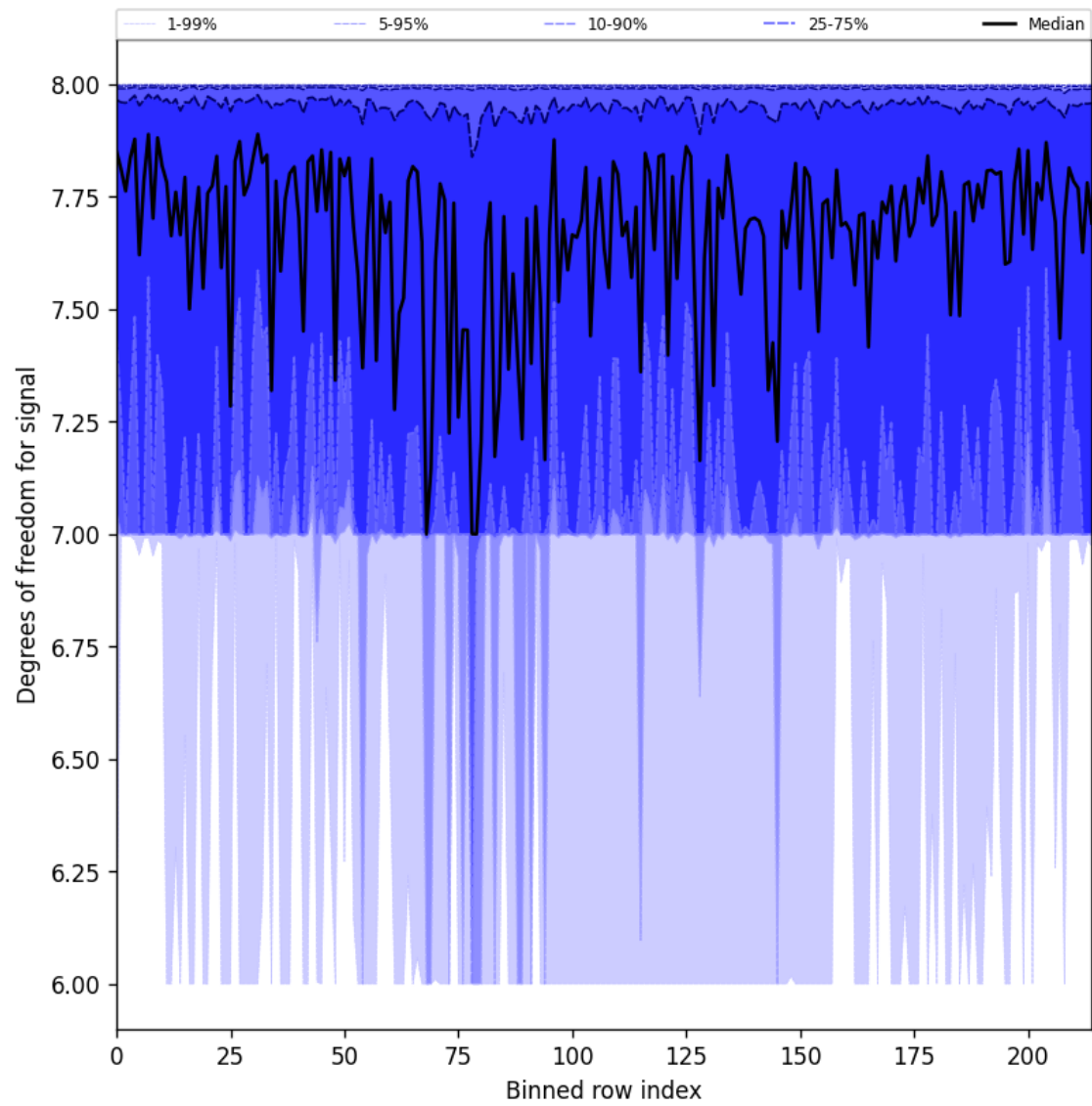
Figure 31: Along track statistics of “Degrees of freedom for signal” for 2025-07-16 to 2025-07-18
