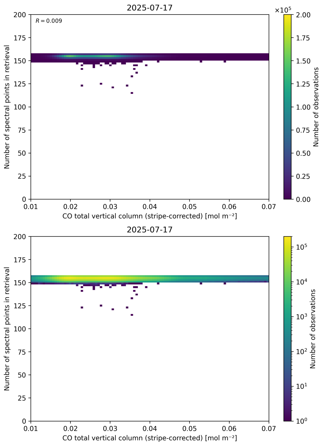
Figure 40: Scatter density plot of “CO total vertical column (stripe-corrected)” against “Number of spectral points in retrieval” for 2025-07-16 to 2025-07-18.
