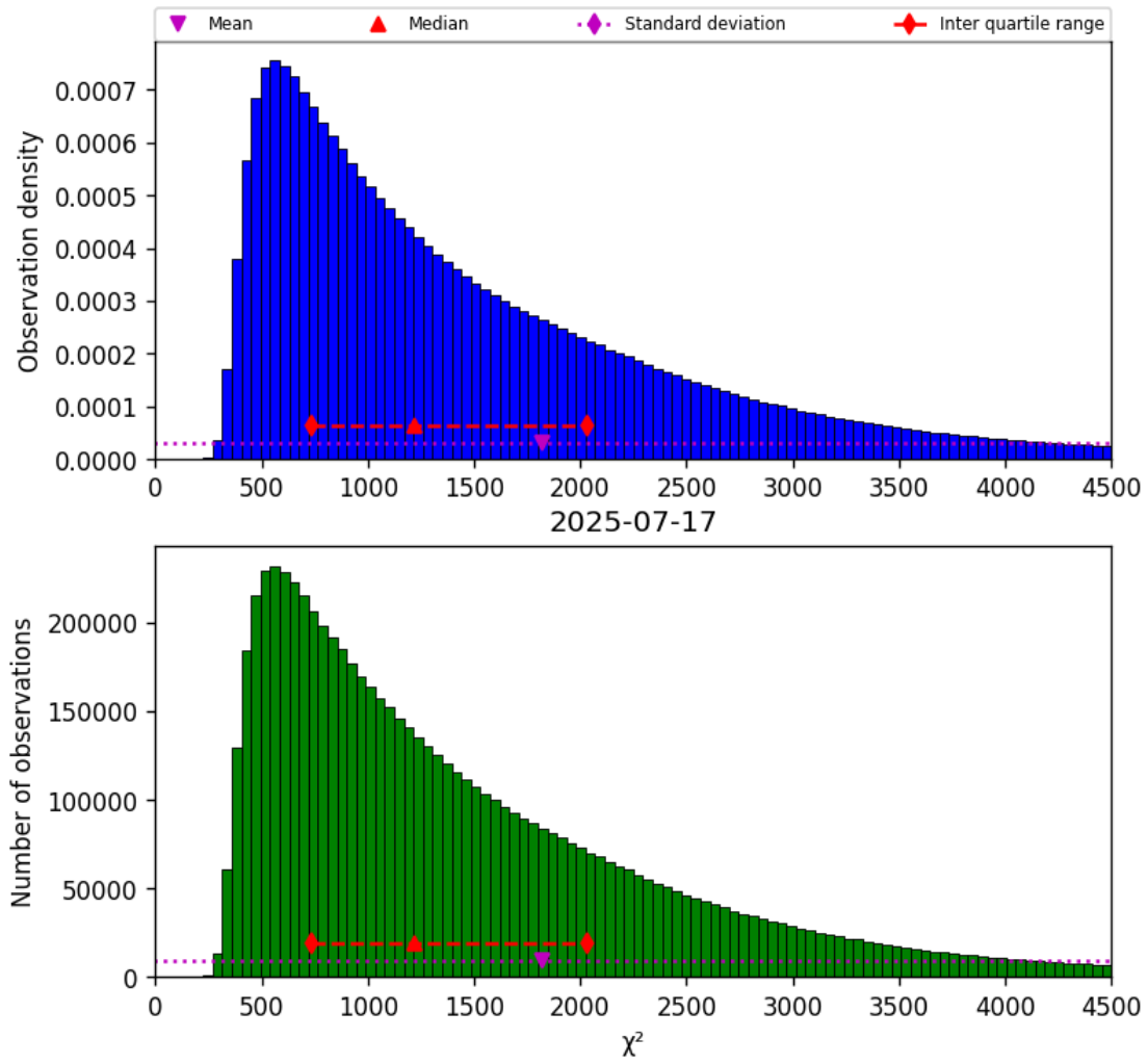
Figure 22: Histogram of " \chi^2 " for 2025-07-16 to 2025-07-18
