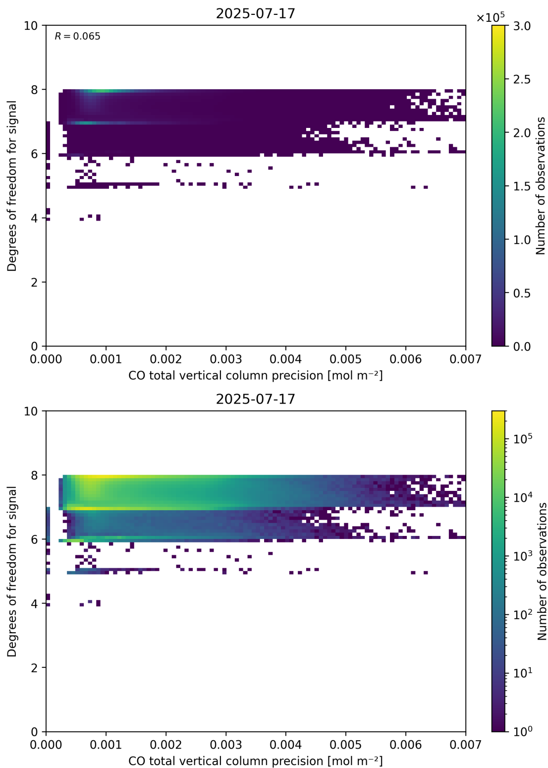
Figure 45: Scatter density plot of “CO total vertical column precision” against “Degrees of freedom for signal” for 2025-07-16 to 2025-07-18.
