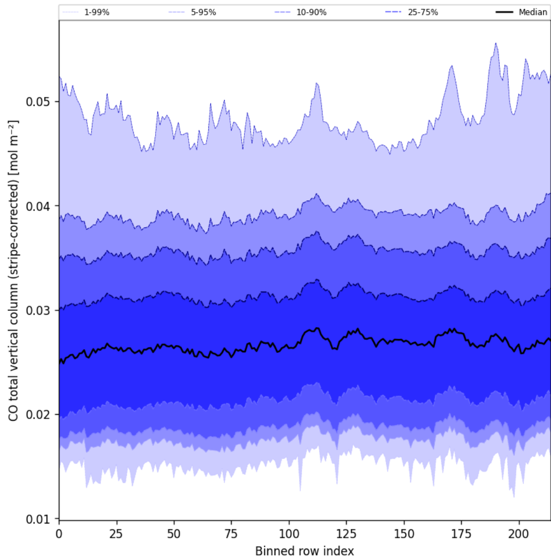
Figure 27: Along track statistics of “CO total vertical column (stripe-corrected)” for 2025-07-16 to 2025-07-18
