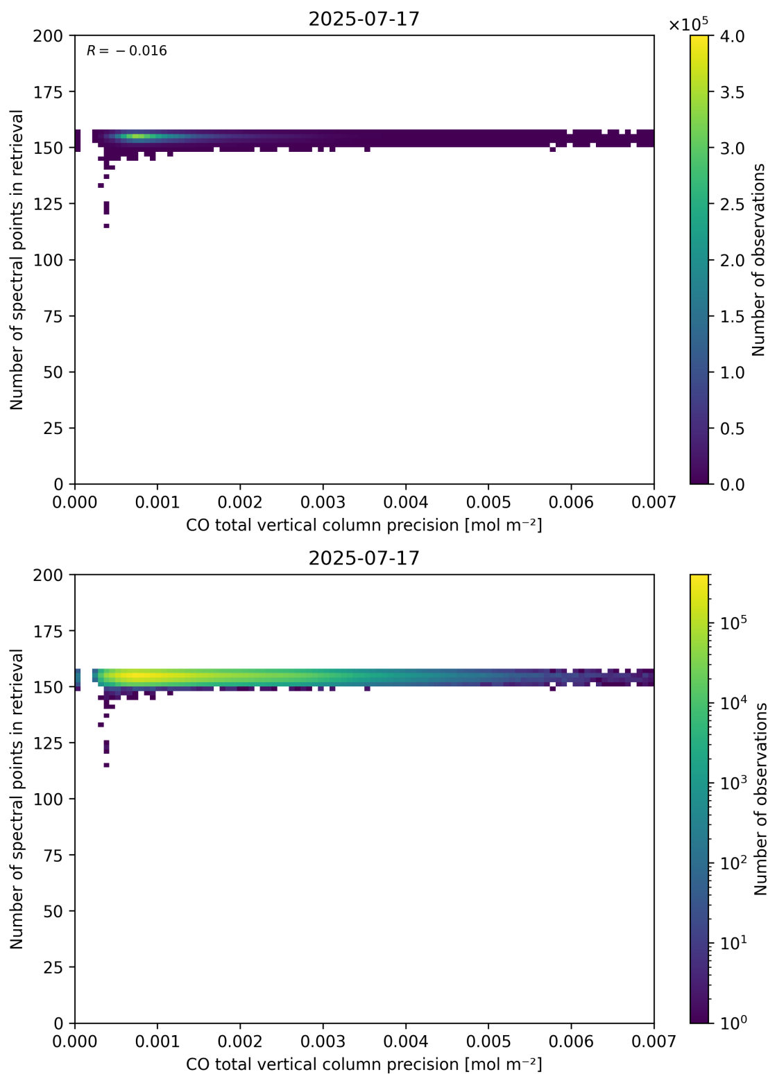
Figure 47: Scatter density plot of “CO total vertical column precision” against “Number of spectral points in retrieval” for 2025-07-16 to 2025-07-18.
