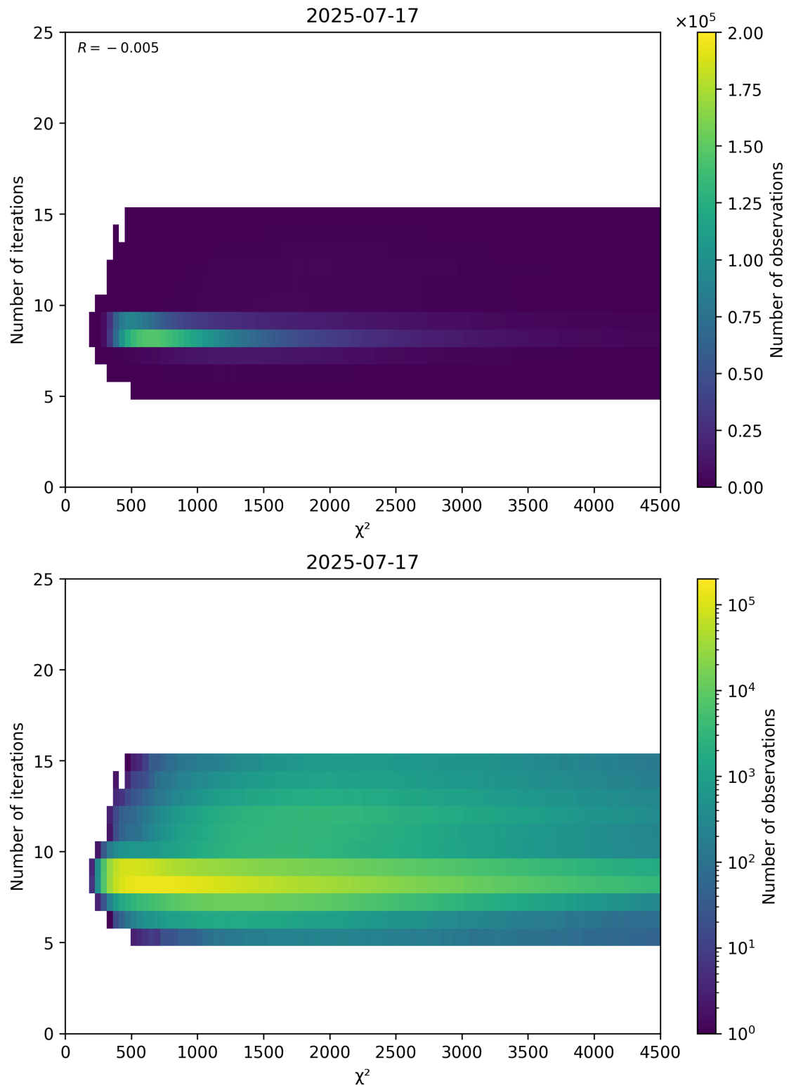
Figure 49: Scatter density plot of “ \chi^2 ” against “Number of iterations” for 2025-07-16 to 2025-07-18.
