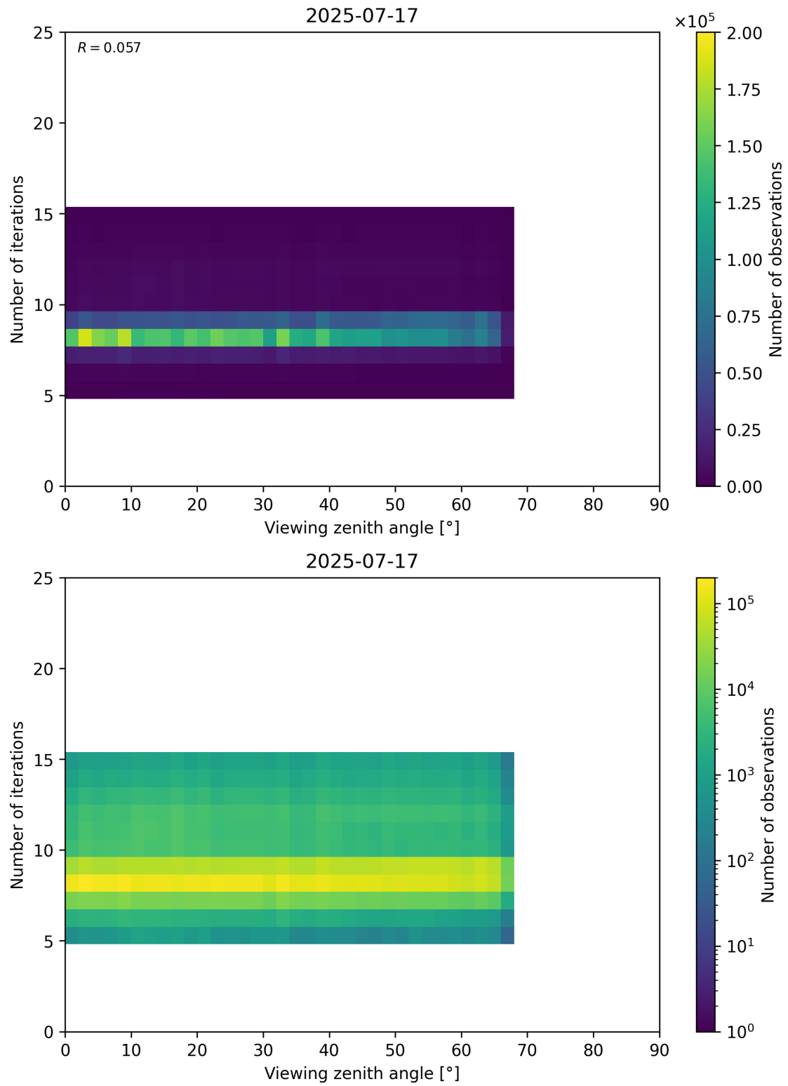
Figure 75: Scatter density plot of “Viewing zenith angle” against “Number of iterations” for 2025-07-16 to 2025-07-18.
