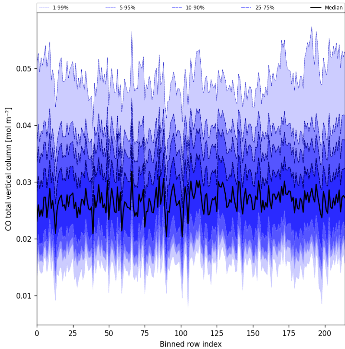
Figure 26: Along track statistics of “CO total vertical column” for 2025-07-16 to 2025-07-18
