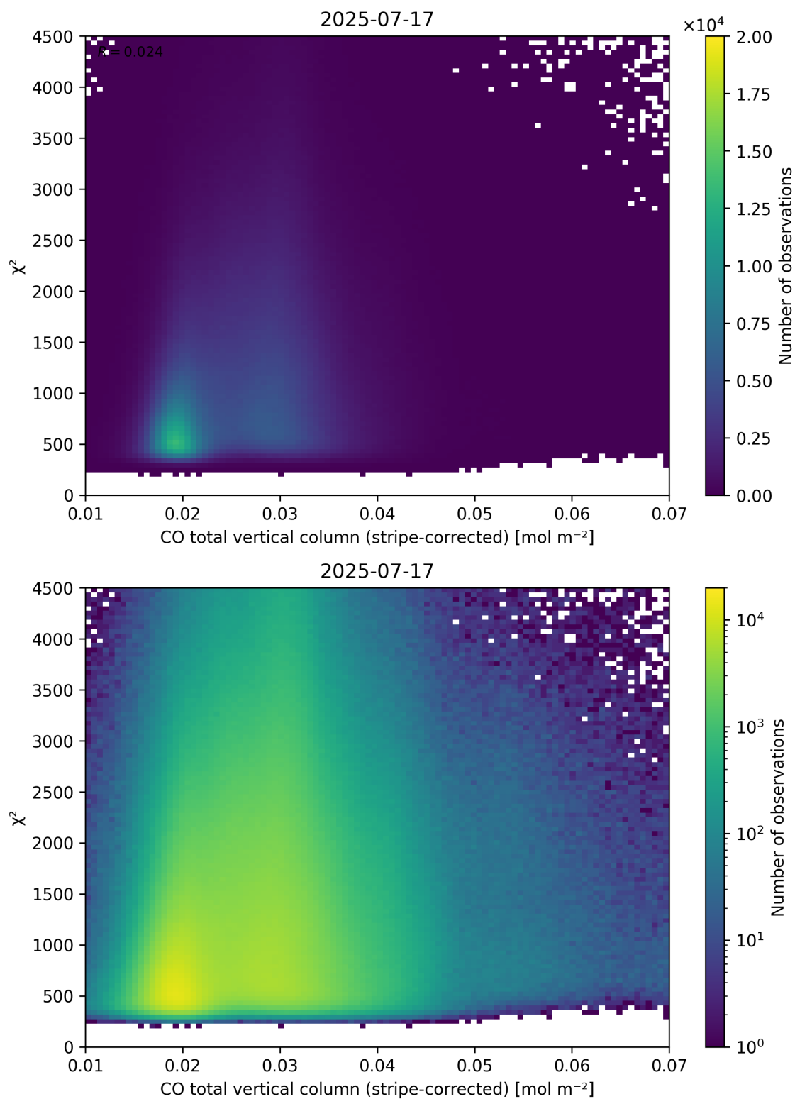
Figure 37: Scatter density plot of “CO total vertical column (stripe-corrected)” against “ \chi^2 ” for 2025-07-16 to 2025-07-18.
