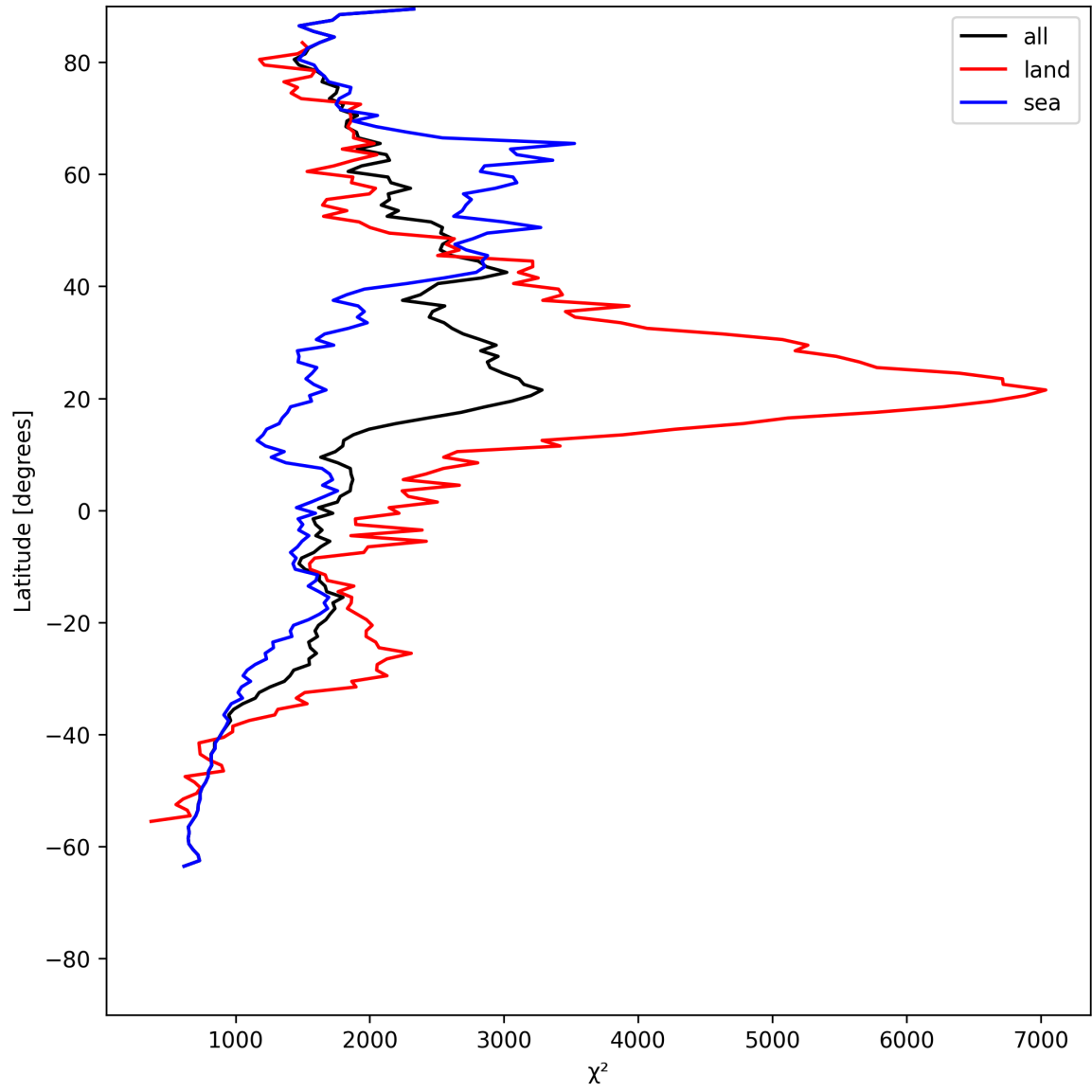
Figure 14: Zonal average of “ \chi^2 ” for 2025-07-16 to 2025-07-18.
