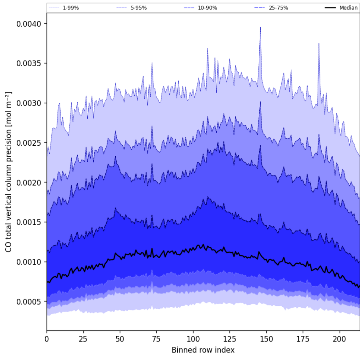
Figure 28: Along track statistics of “CO total vertical column precision” for 2025-07-16 to 2025-07-18
