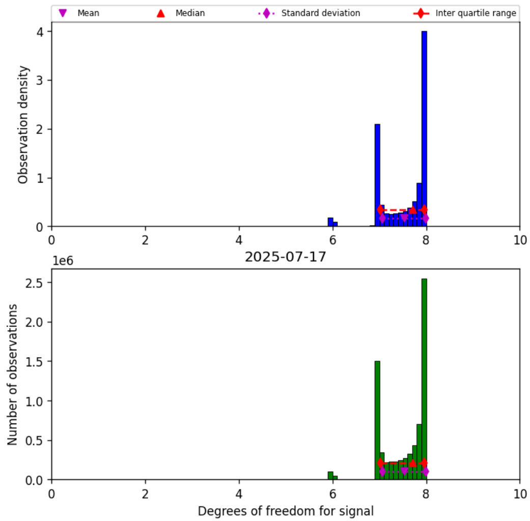
Figure 23: Histogram of “Degrees of freedom for signal” for 2025-07-16 to 2025-07-18
