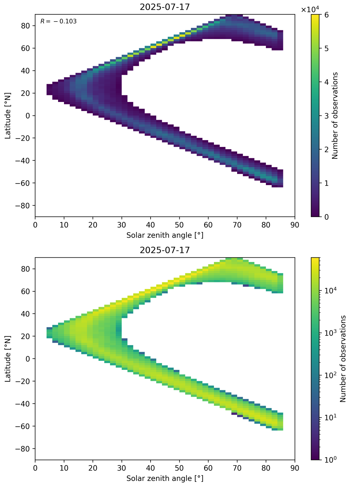
Figure 66: Scatter density plot of “Solar zenith angle” against “Latitude” for 2025-07-16 to 2025-07-18.
