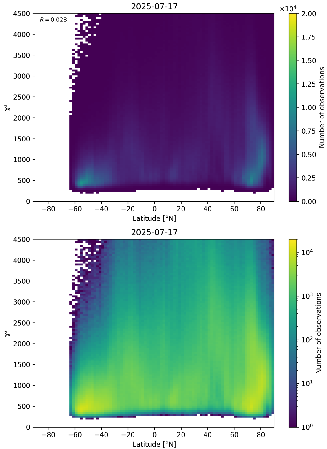
Figure 54: Scatter density plot of “Latitude” against “ \chi^2 ” for 2025-07-16 to 2025-07-18.
