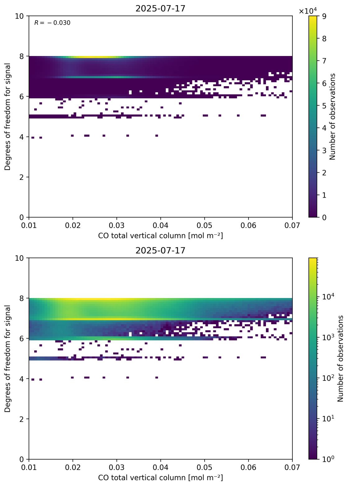
Figure 41: Scatter density plot of “CO total vertical column” against “Degrees of freedom for signal” for 2025-07-16 to 2025-07-18.
