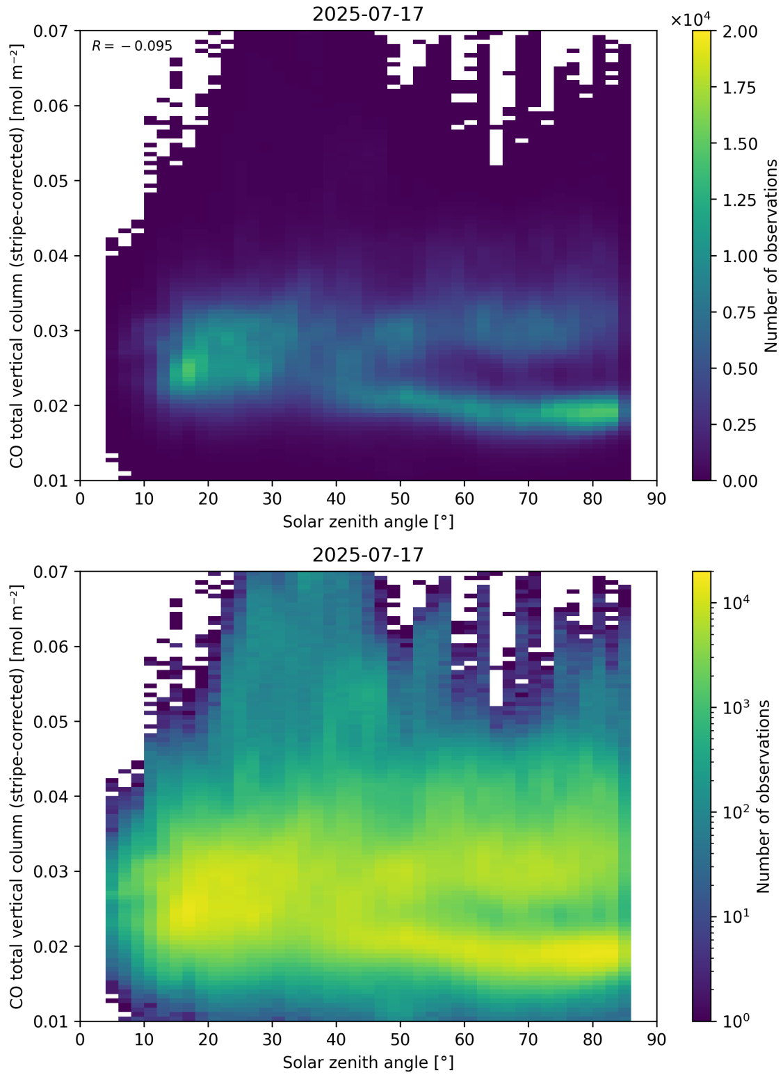
Figure 62: Scatter density plot of “Solar zenith angle” against “CO total vertical column (stripe-corrected)” for 2025-07-16 to 2025-07-18.
