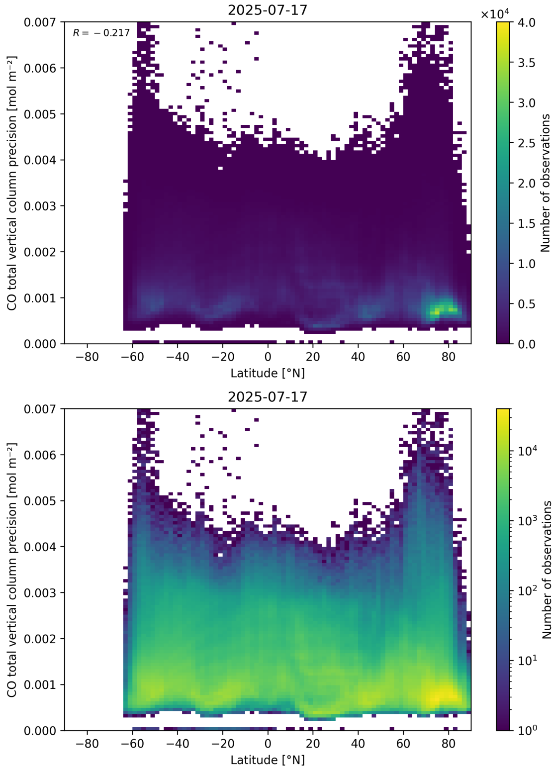
Figure 53: Scatter density plot of “Latitude” against “CO total vertical column precision” for 2025-07-16 to 2025-07-18.
