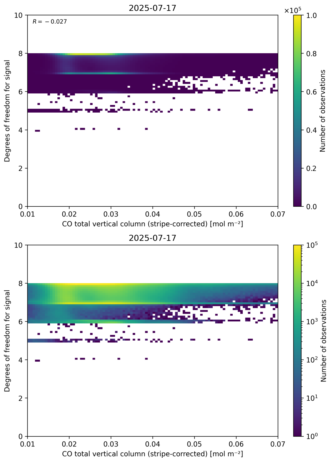
Figure 38: Scatter density plot of “CO total vertical column (stripe-corrected)” against “Degrees of freedom for signal” for 2025-07-16 to 2025-07-18.
