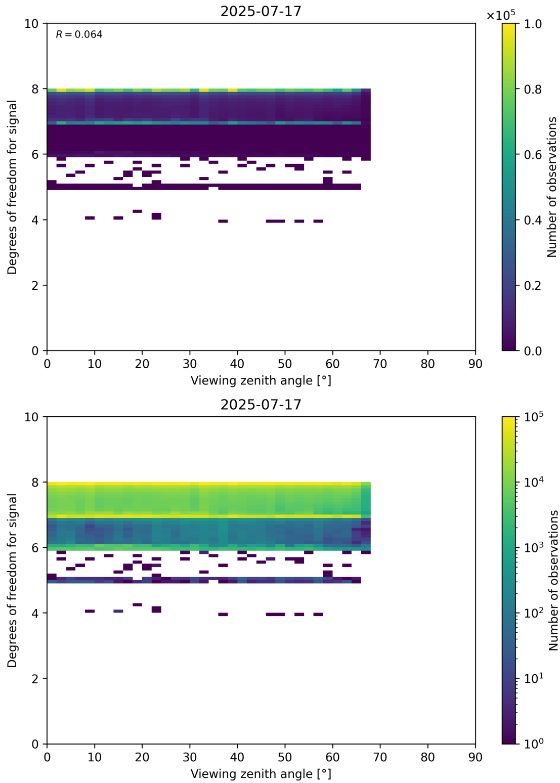
Figure 73: Scatter density plot of “Viewing zenith angle” against “Degrees of freedom for signal” for 2025-07-16 to 2025-07-18.
