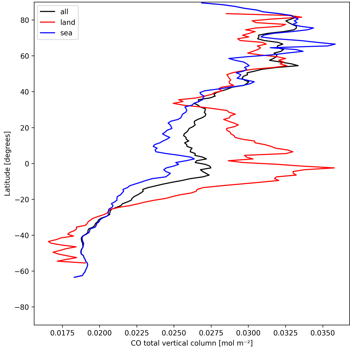
Figure 10: Zonal average of “CO total vertical column” for 2025-07-16 to 2025-07-18.
