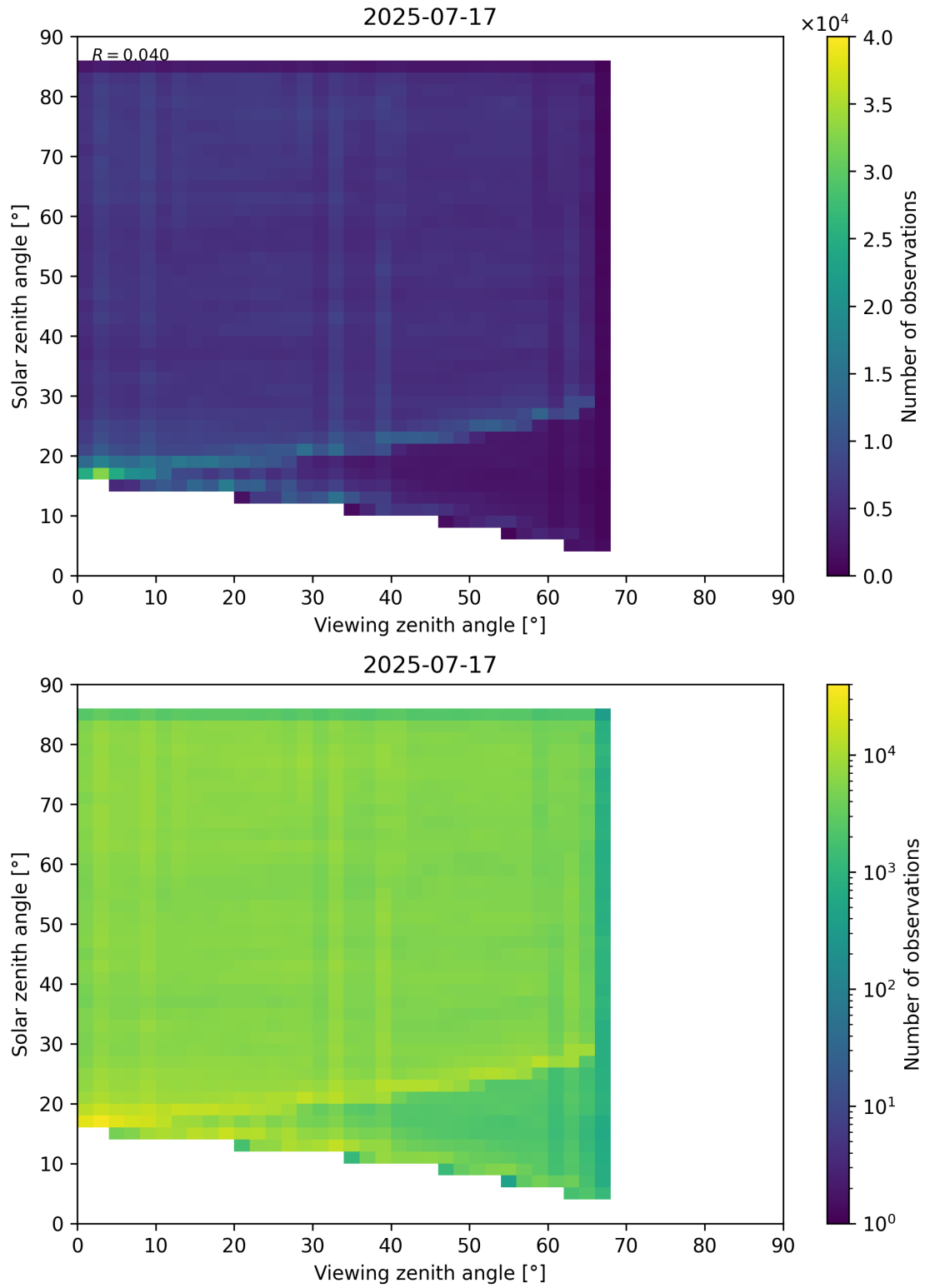
Figure 77: Scatter density plot of “Viewing zenith angle” against “Solar zenith angle” for 2025-07-16 to 2025-07-18.
