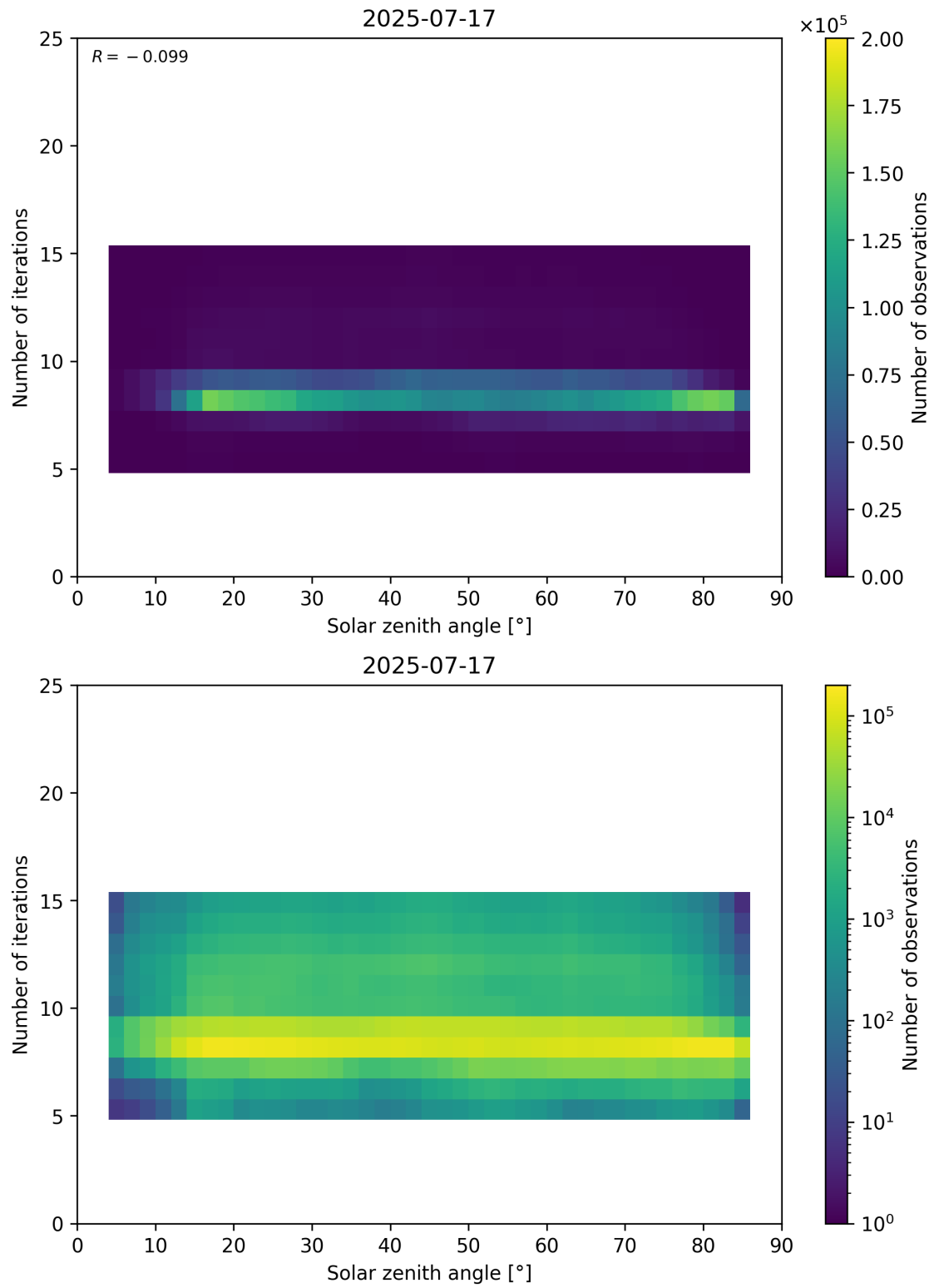
Figure 67: Scatter density plot of “Solar zenith angle” against “Number of iterations” for 2025-07-16 to 2025-07-18.
