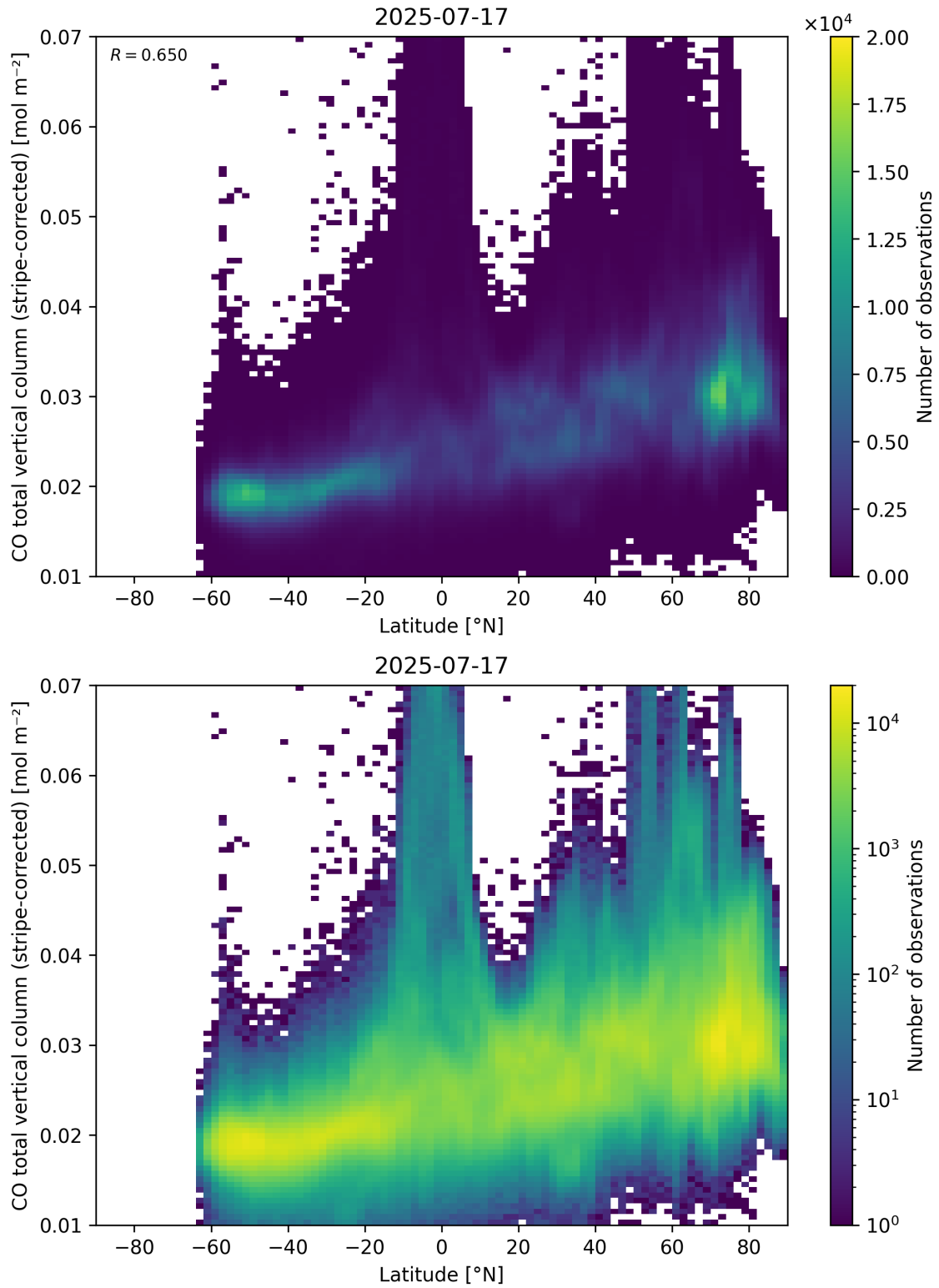
Figure 52: Scatter density plot of “Latitude” against “CO total vertical column (stripe-corrected)” for 2025-07-16 to 2025-07-18.
