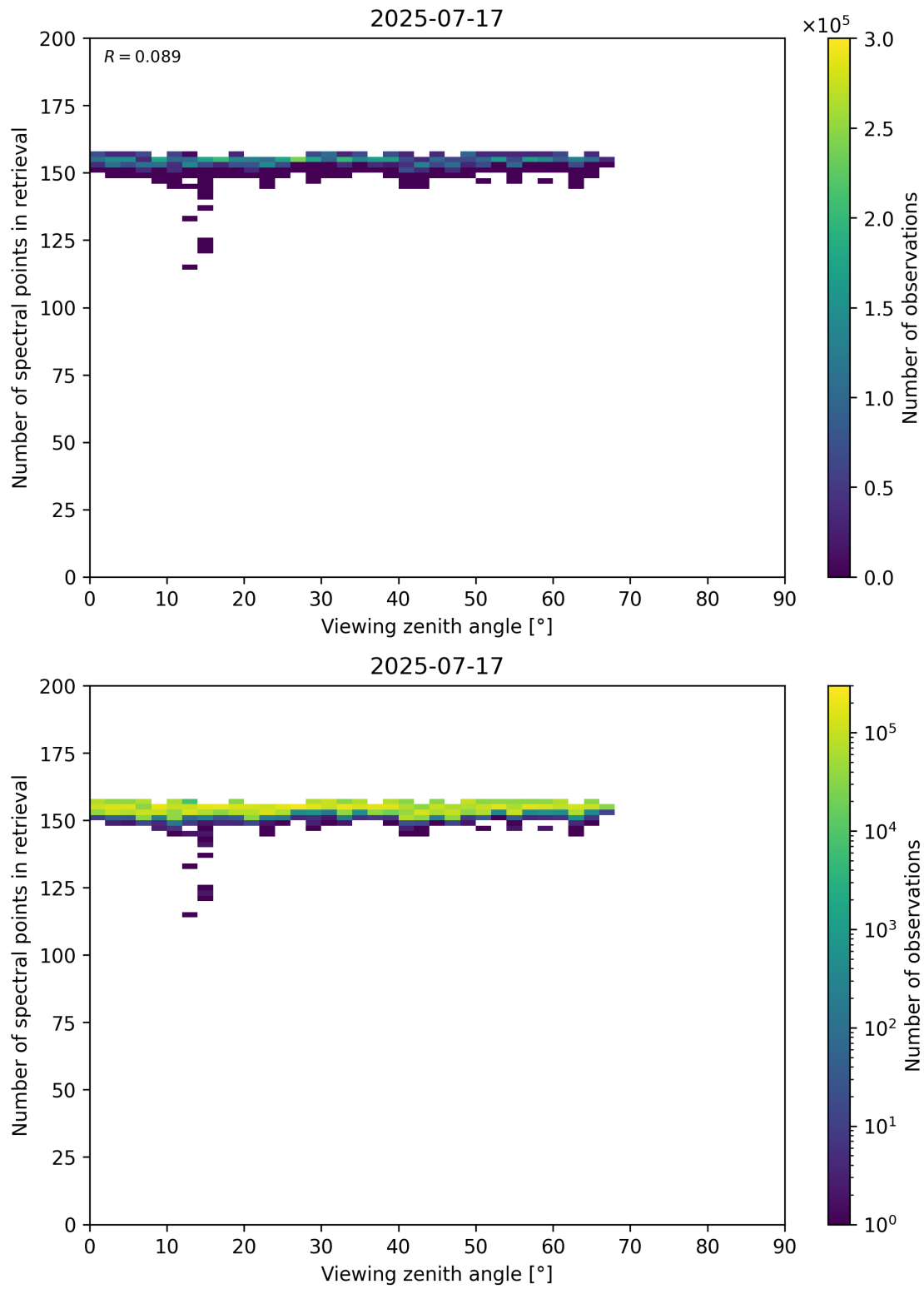
Figure 76: Scatter density plot of “Viewing zenith angle” against “Number of spectral points in retrieval” for 2025-07-16 to 2025-07-18.
