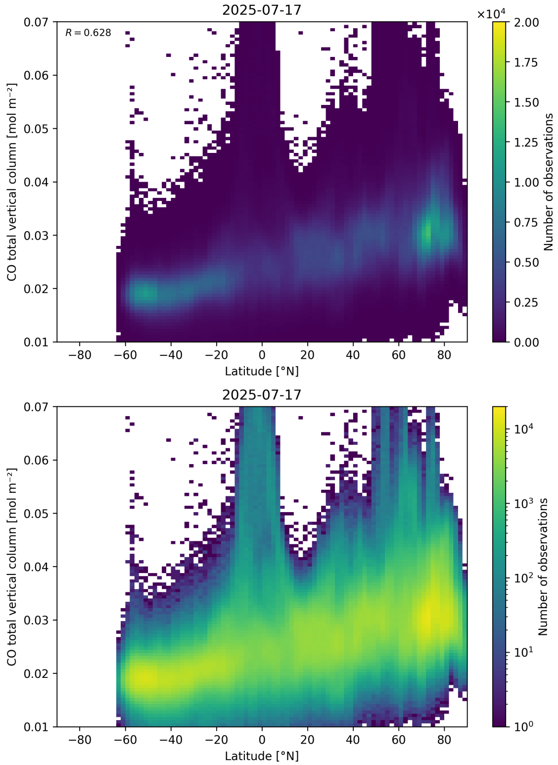
Figure 51: Scatter density plot of “Latitude” against “CO total vertical column” for 2025-07-16 to 2025-07-18.
