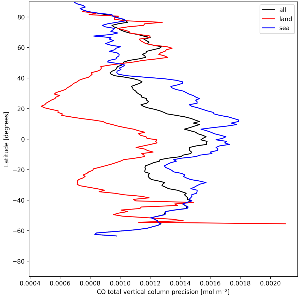
Figure 12: Zonal average of “CO total vertical column precision” for 2025-07-16 to 2025-07-18.
