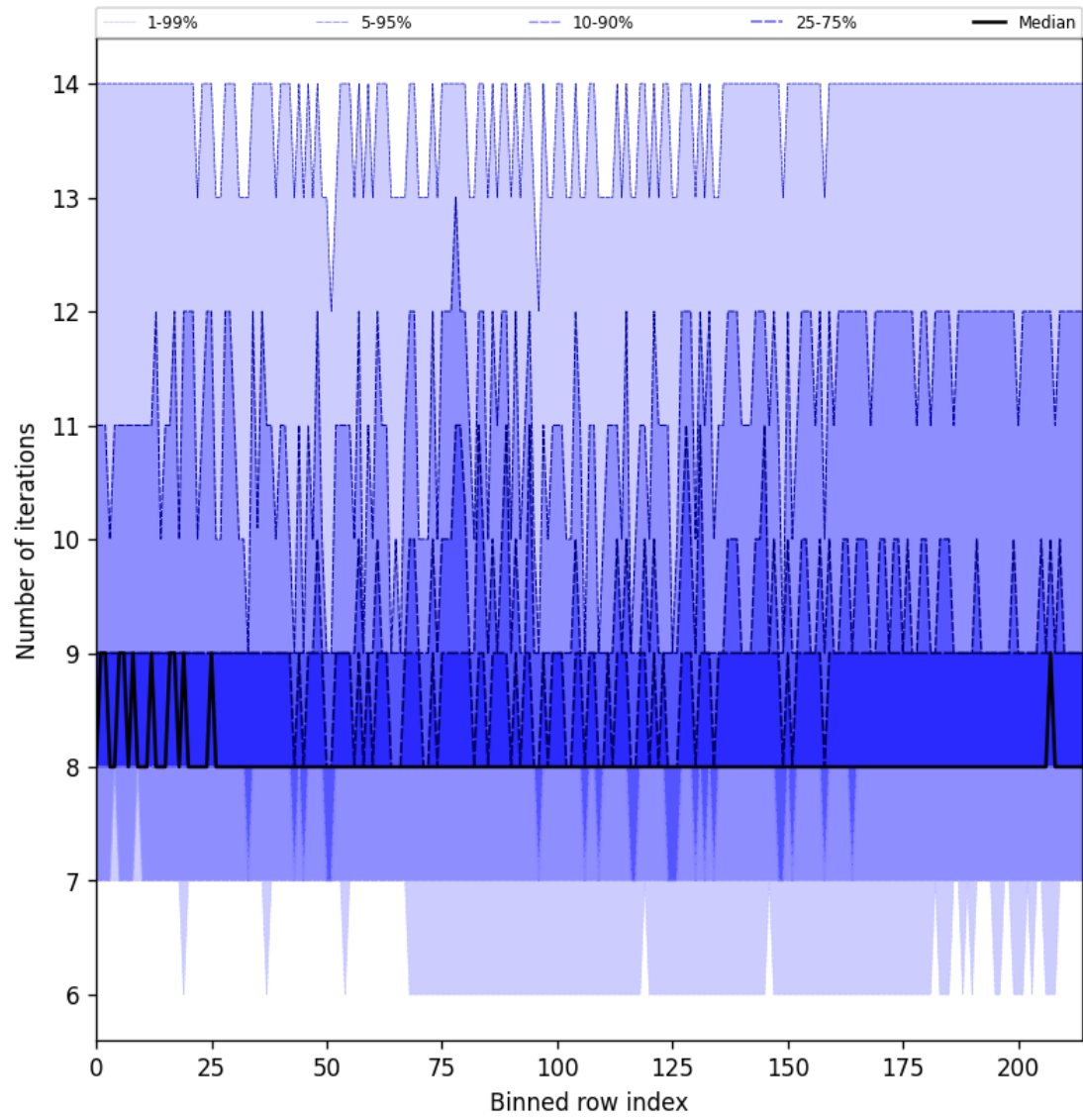
Figure 32: Along track statistics of “Number of iterations” for 2025-07-16 to 2025-07-18
