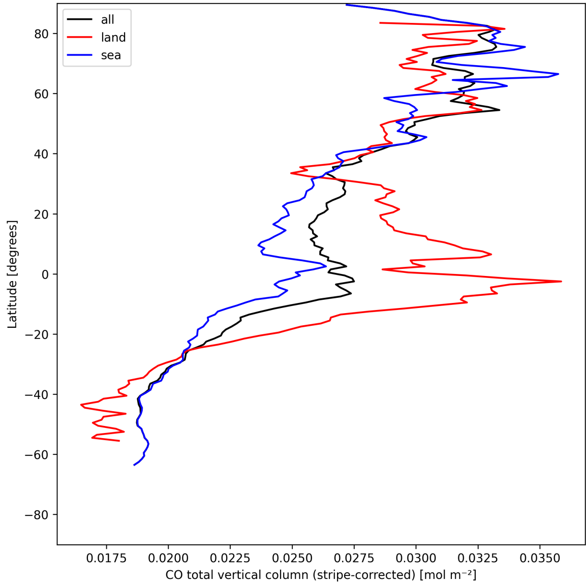
Figure 11: Zonal average of “CO total vertical column (stripe-corrected)” for 2025-07-16 to 2025-07-18.
