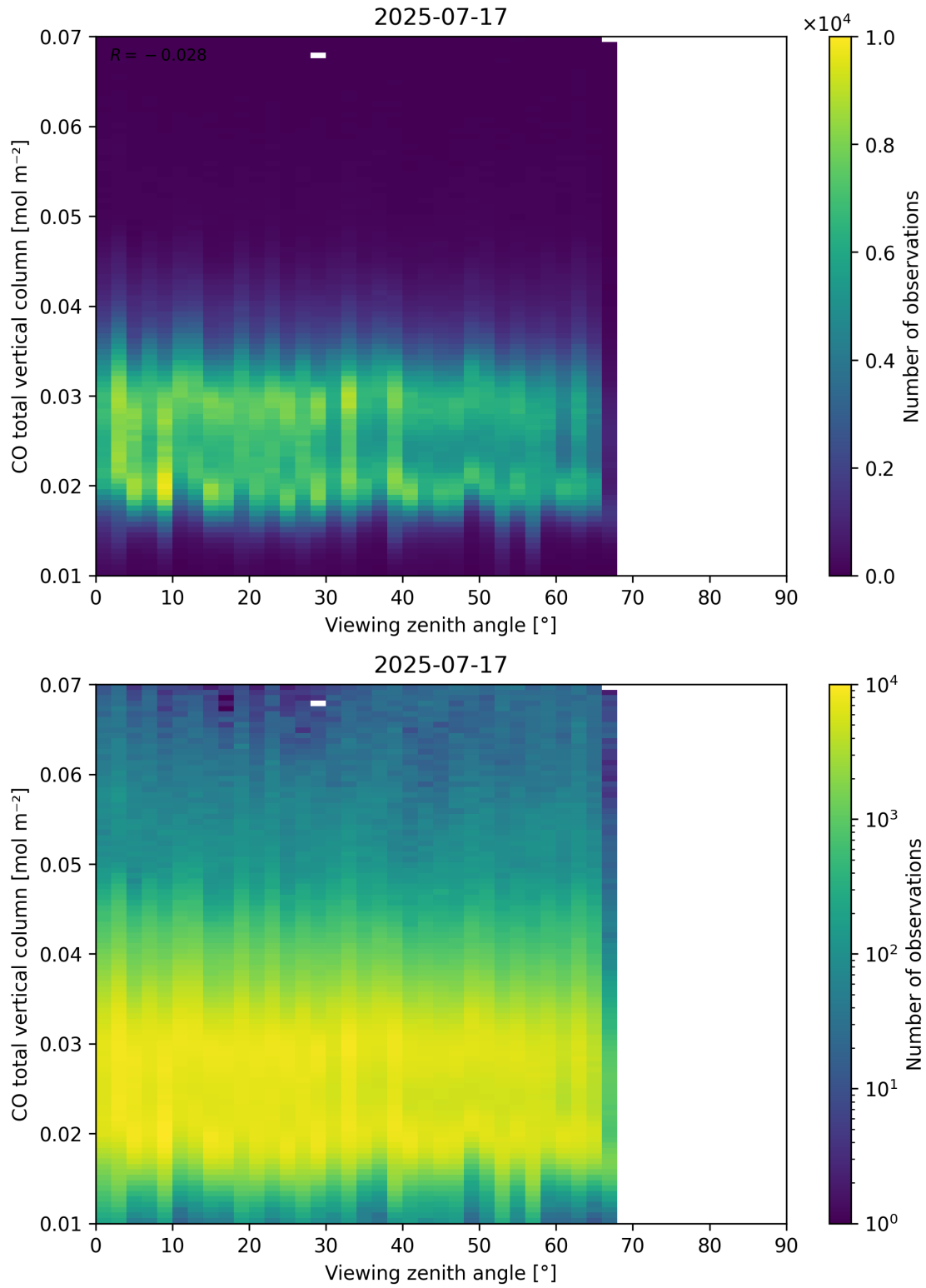
Figure 69: Scatter density plot of “Viewing zenith angle” against “CO total vertical column” for 2025-07-16 to 2025-07-18.
