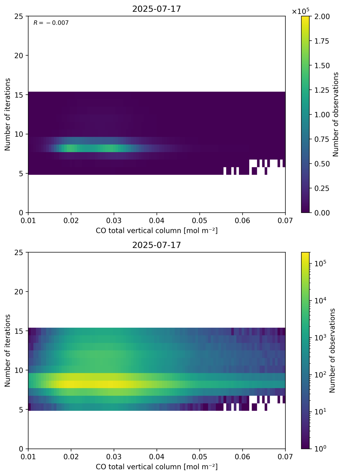
Figure 42: Scatter density plot of “CO total vertical column” against “Number of iterations” for 2025-07-16 to 2025-07-18.
