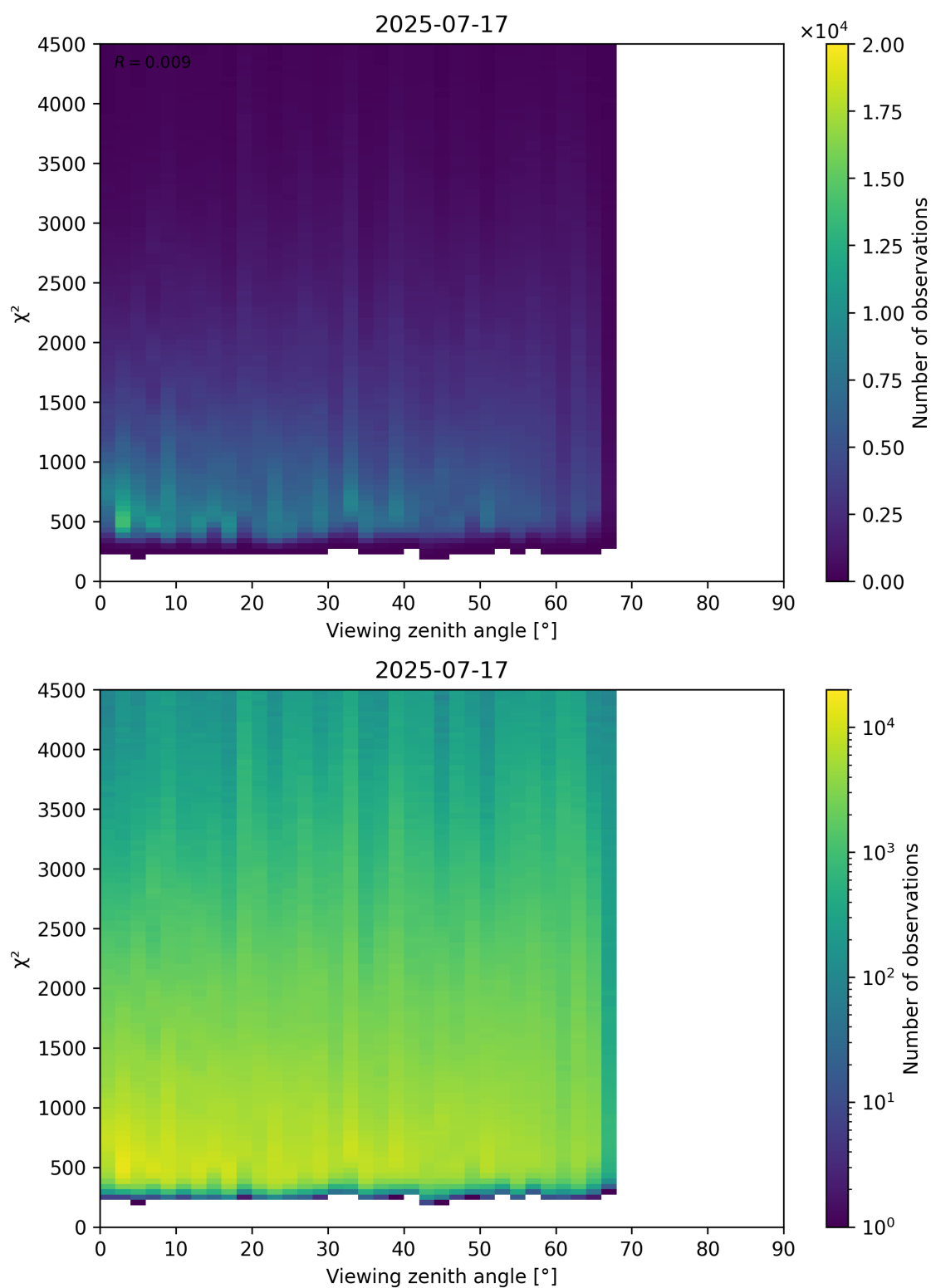
Figure 72: Scatter density plot of "Viewing zenith angle" against " \chi^2 " for 2025-07-16 to 2025-07-18.
