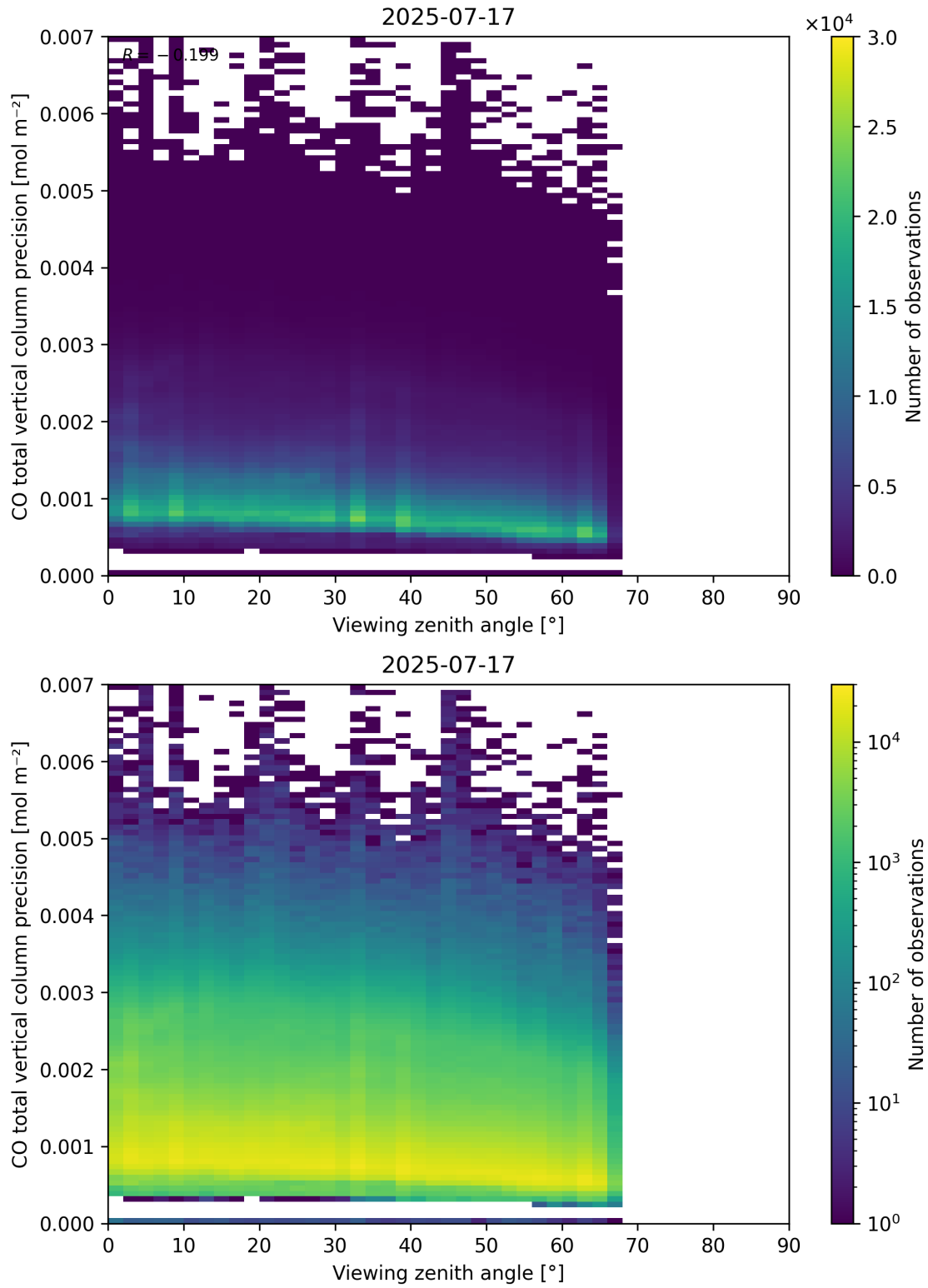
Figure 71: Scatter density plot of “Viewing zenith angle” against “CO total vertical column precision” for 2025-07-16 to 2025-07-18.
