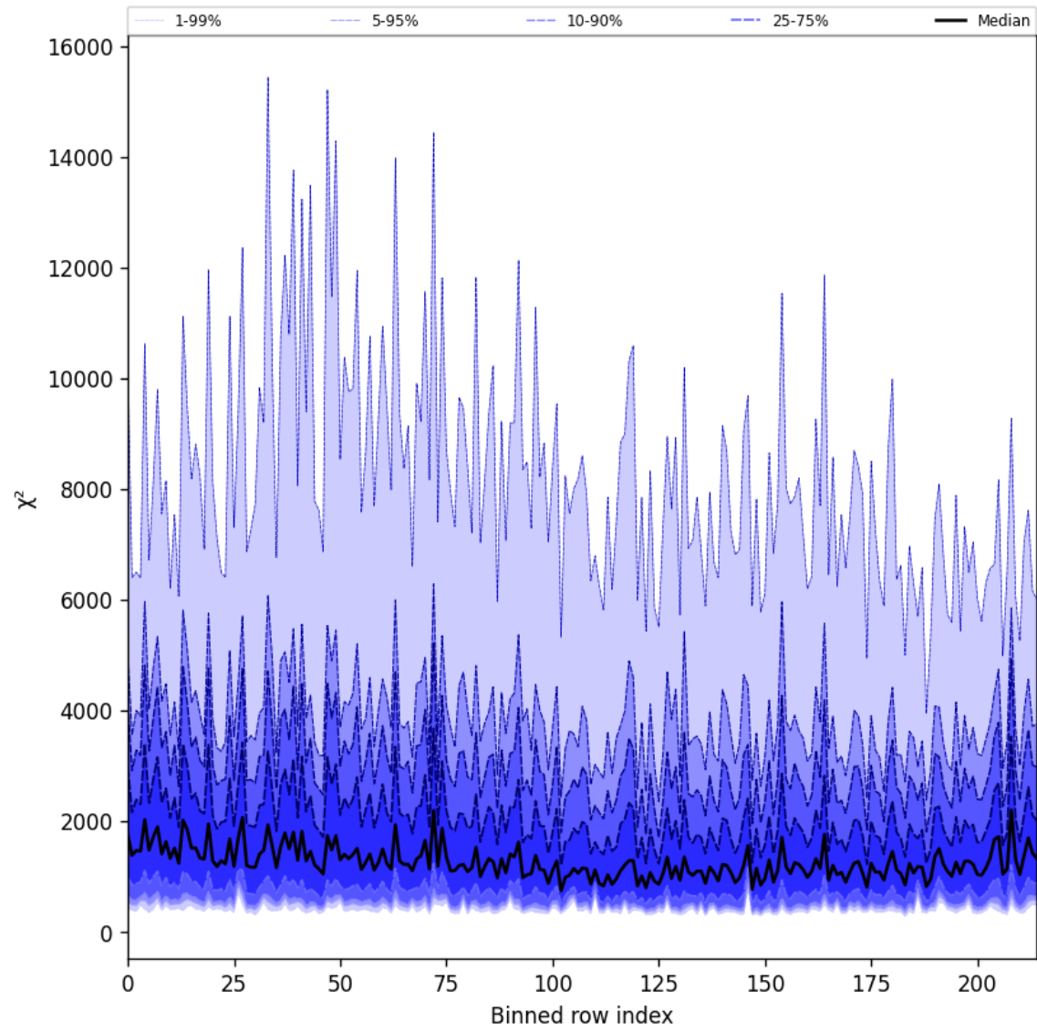
Figure 30: Along track statistics of “ \chi^2 ” for 2025-07-16 to 2025-07-18
