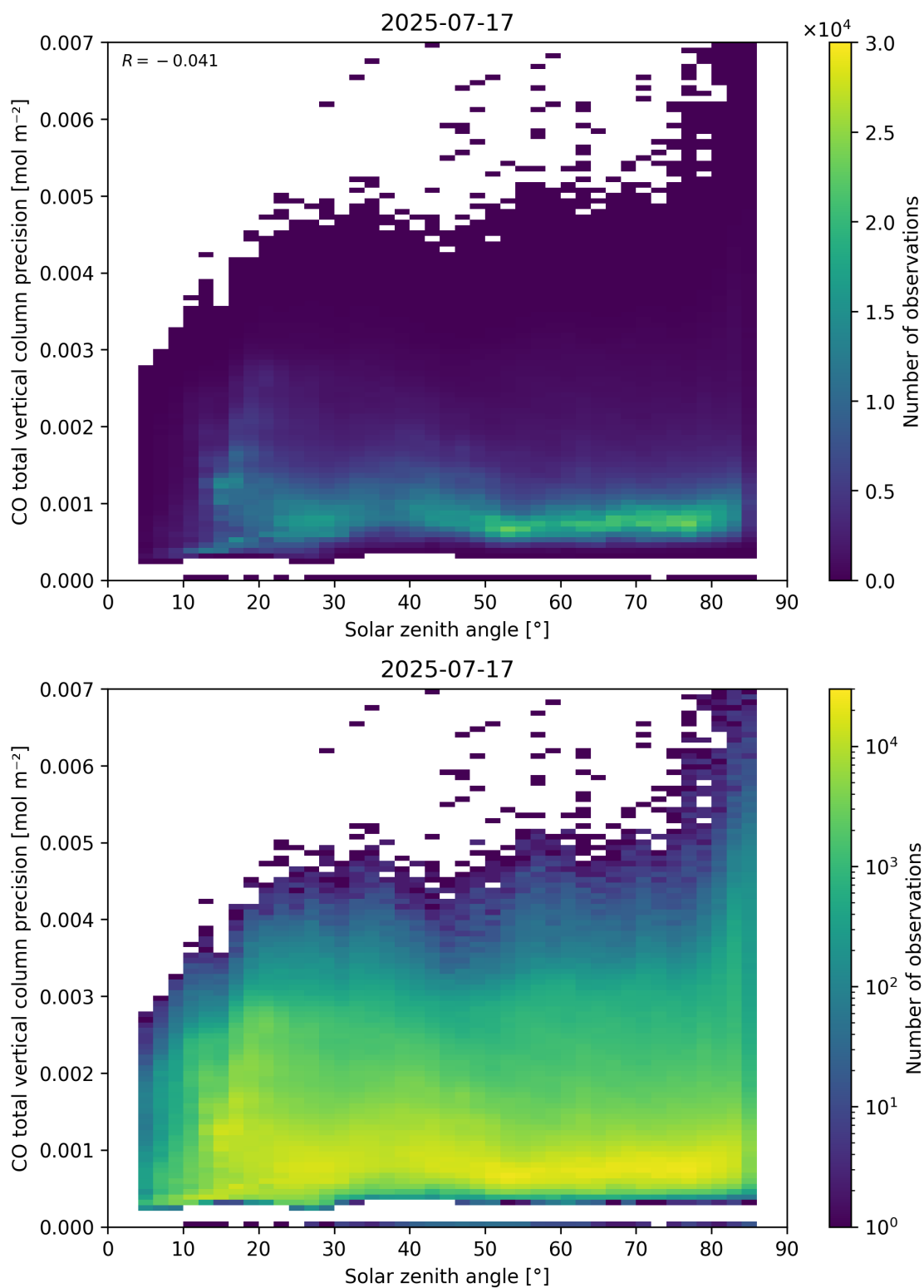
Figure 63: Scatter density plot of “Solar zenith angle” against “CO total vertical column precision” for 2025-07-16 to 2025-07-18.
