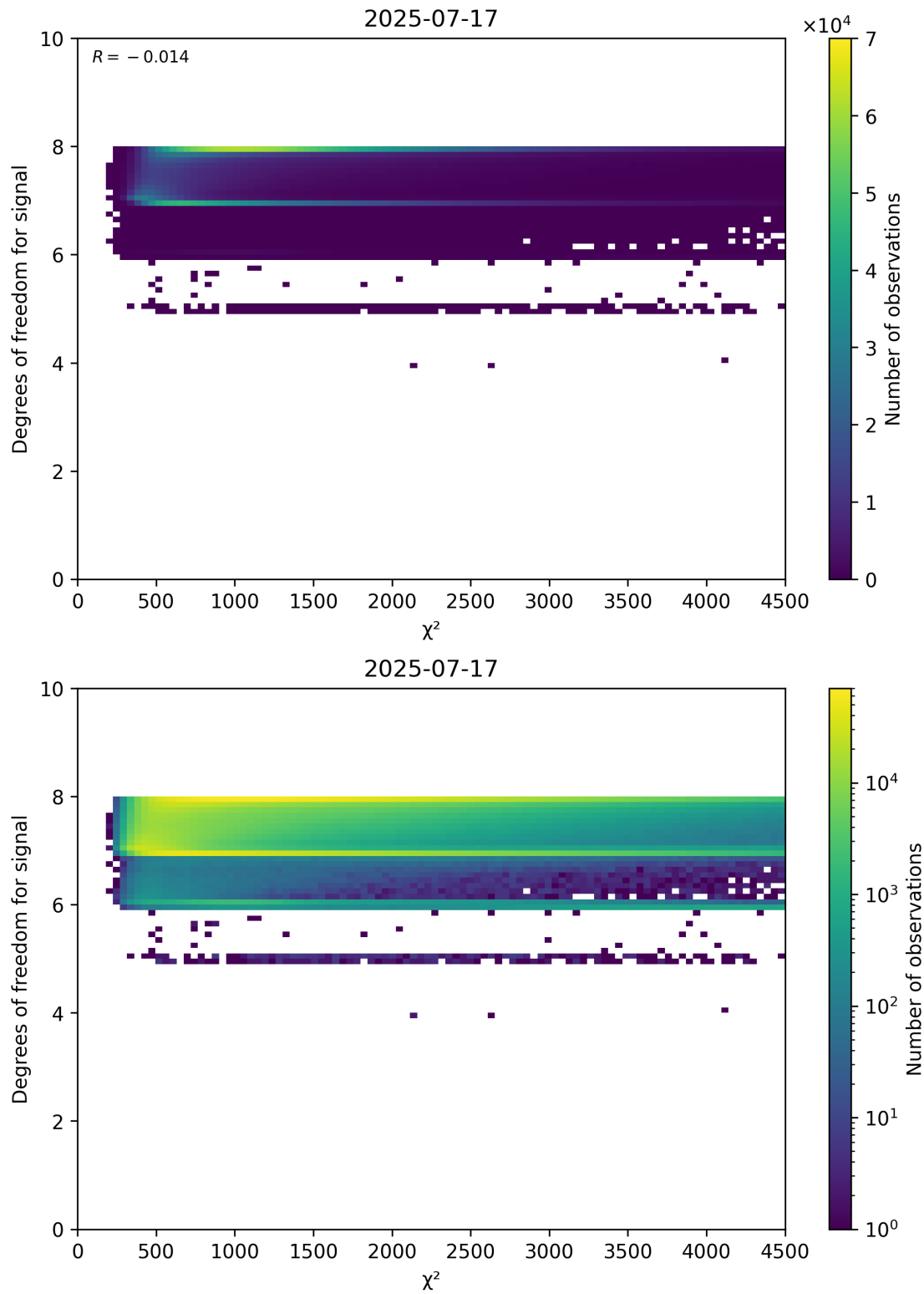
Figure 48: Scatter density plot of “ \chi^2 ” against “Degrees of freedom for signal” for 2025-07-16 to 2025-07-18.
