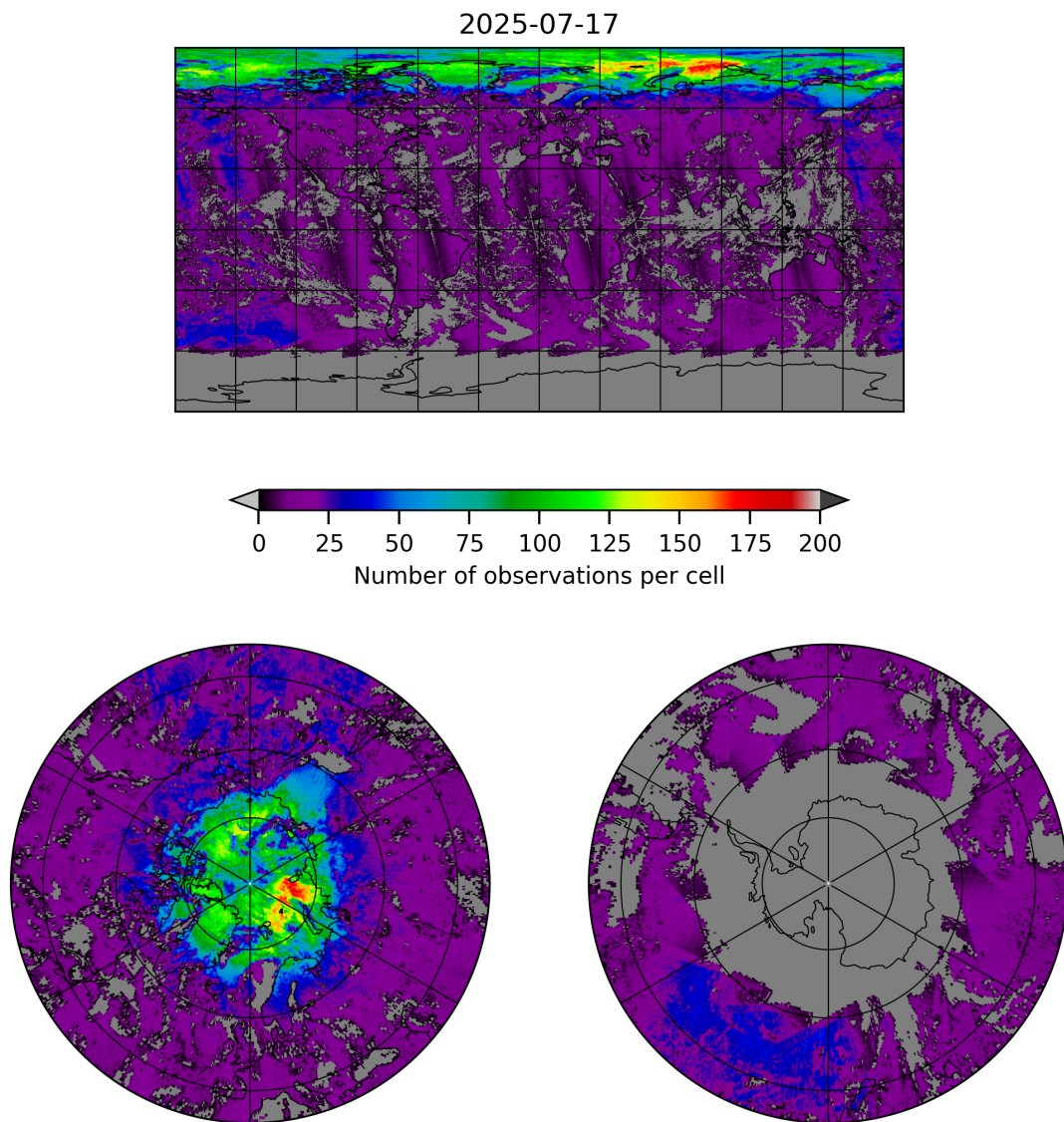
Figure 8: Map of the number of observations for 2025-07-16 to 2025-07-18
