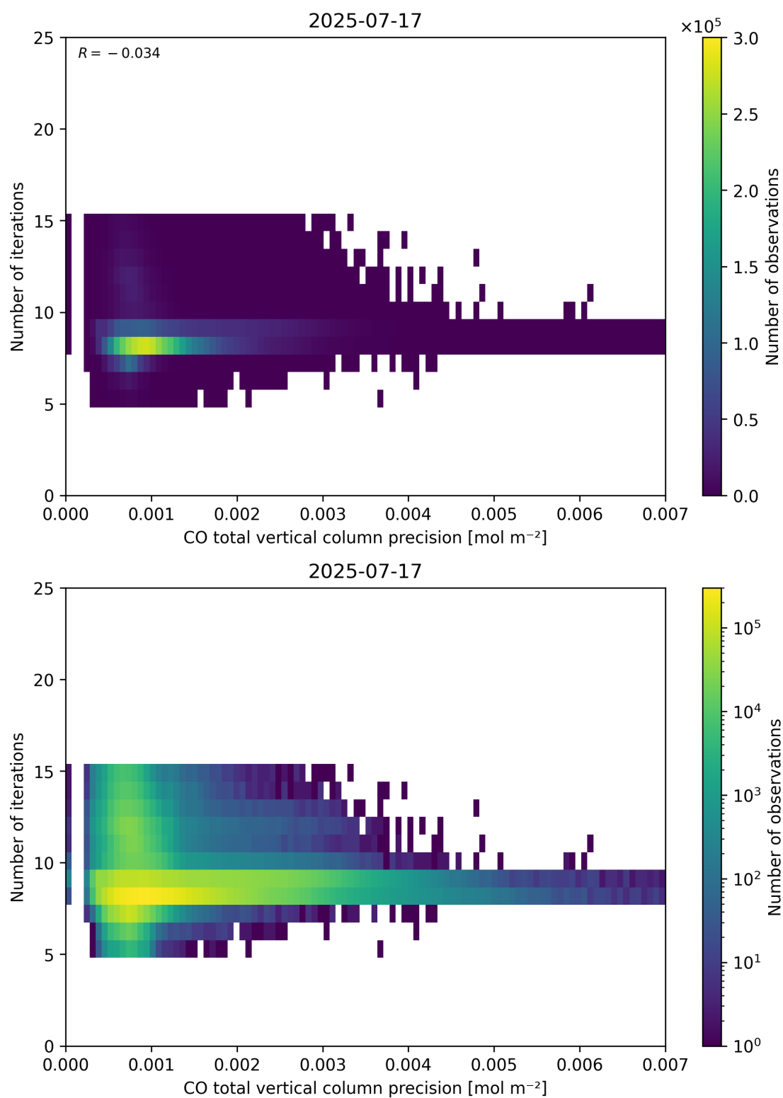
Figure 46: Scatter density plot of “CO total vertical column precision” against “Number of iterations” for 2025-07-16 to 2025-07-18.
