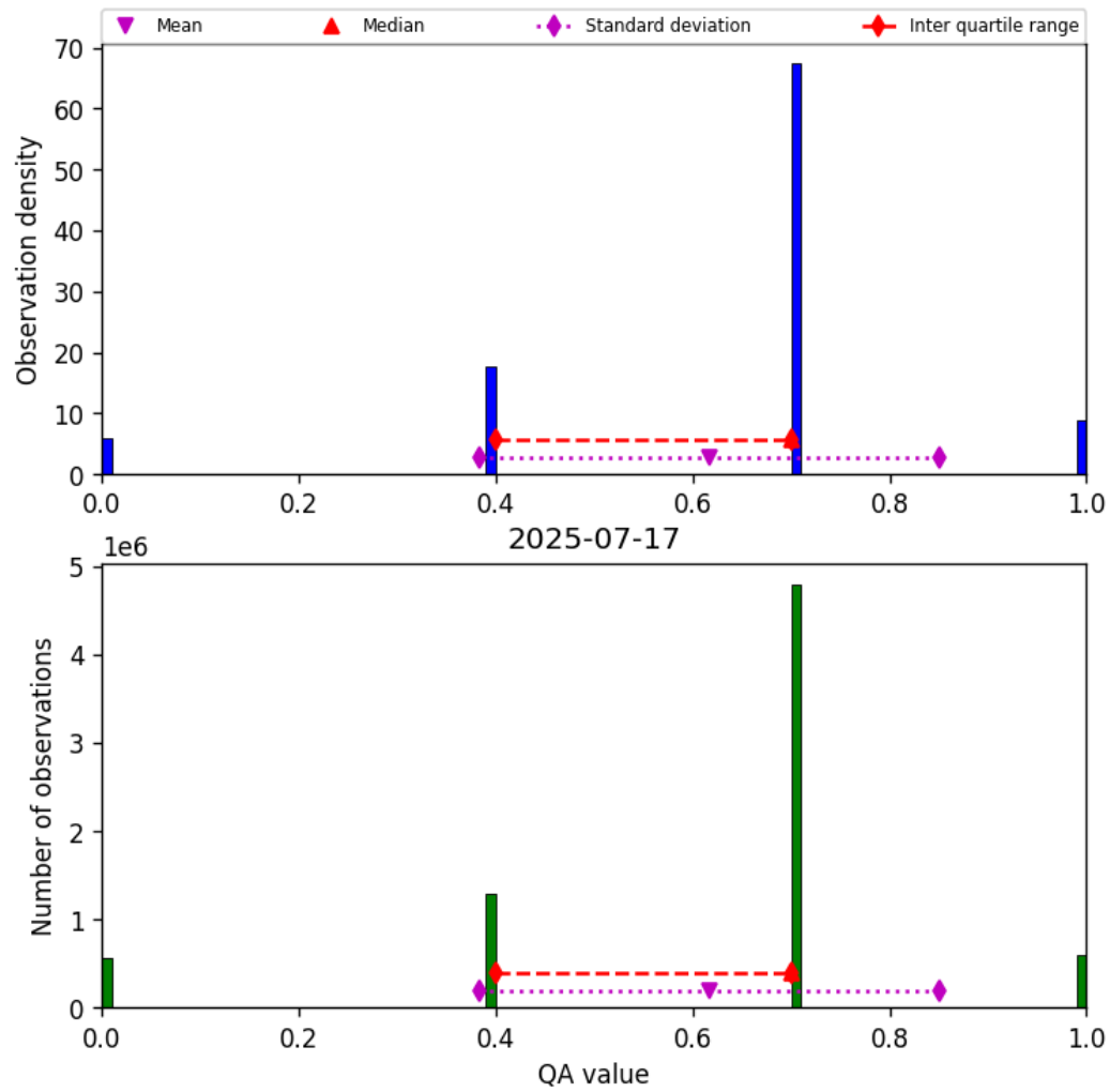
Figure 17: Histogram of “QA value” for 2025-07-16 to 2025-07-18
