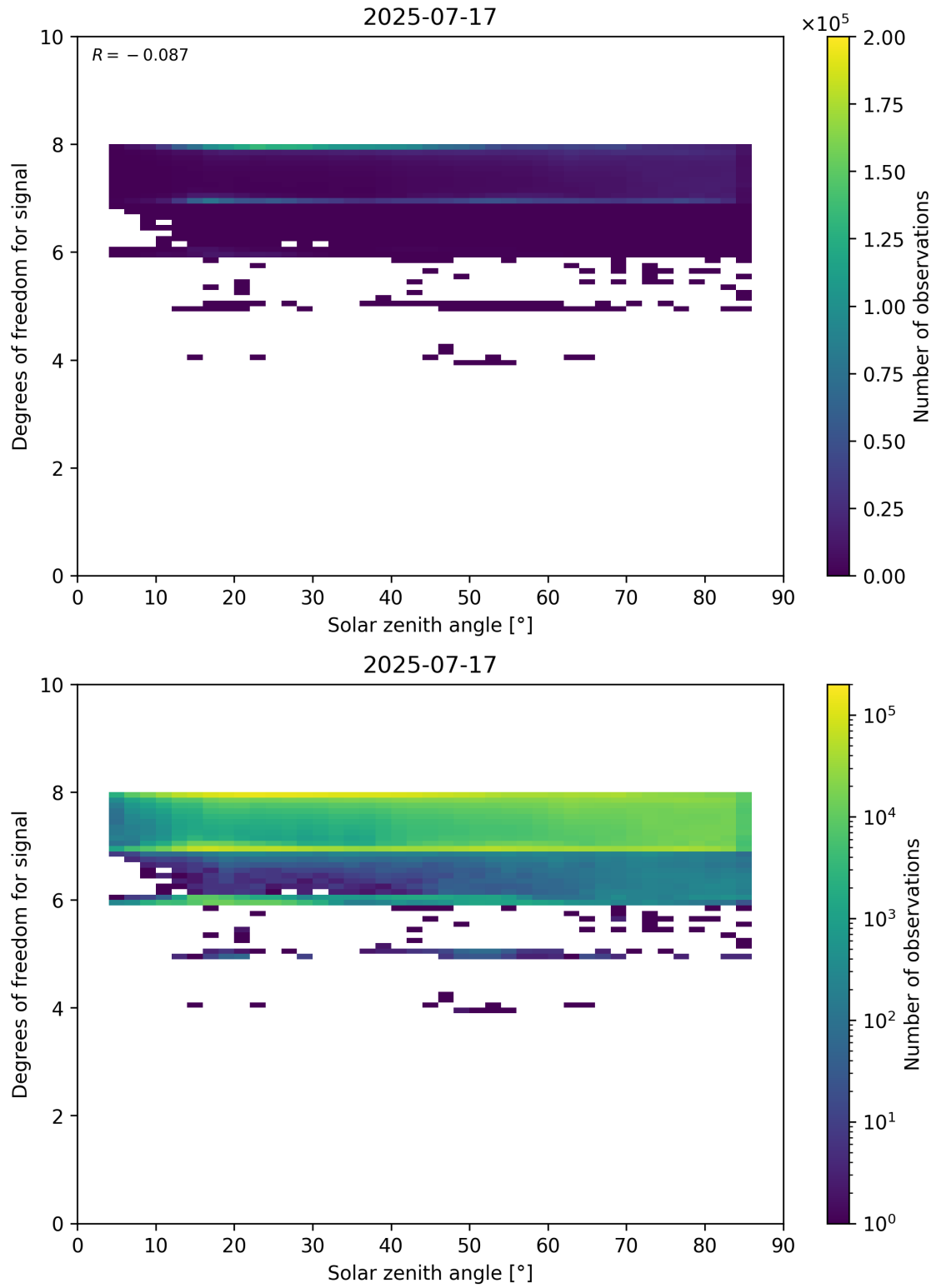
Figure 65: Scatter density plot of “Solar zenith angle” against “Degrees of freedom for signal” for 2025-07-16 to 2025-07-18.
