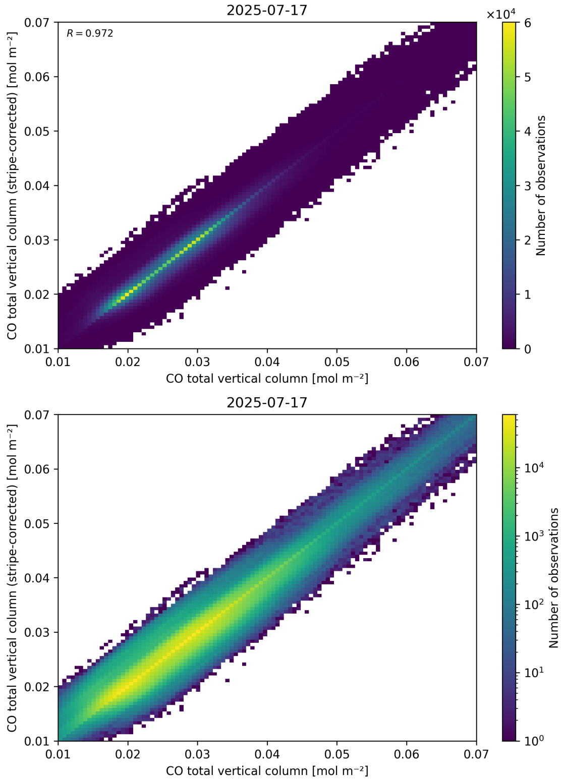
Figure 33: Scatter density plot of “CO total vertical column” against “CO total vertical column (stripe-corrected)” for 2025-07-16 to 2025-07-18.
