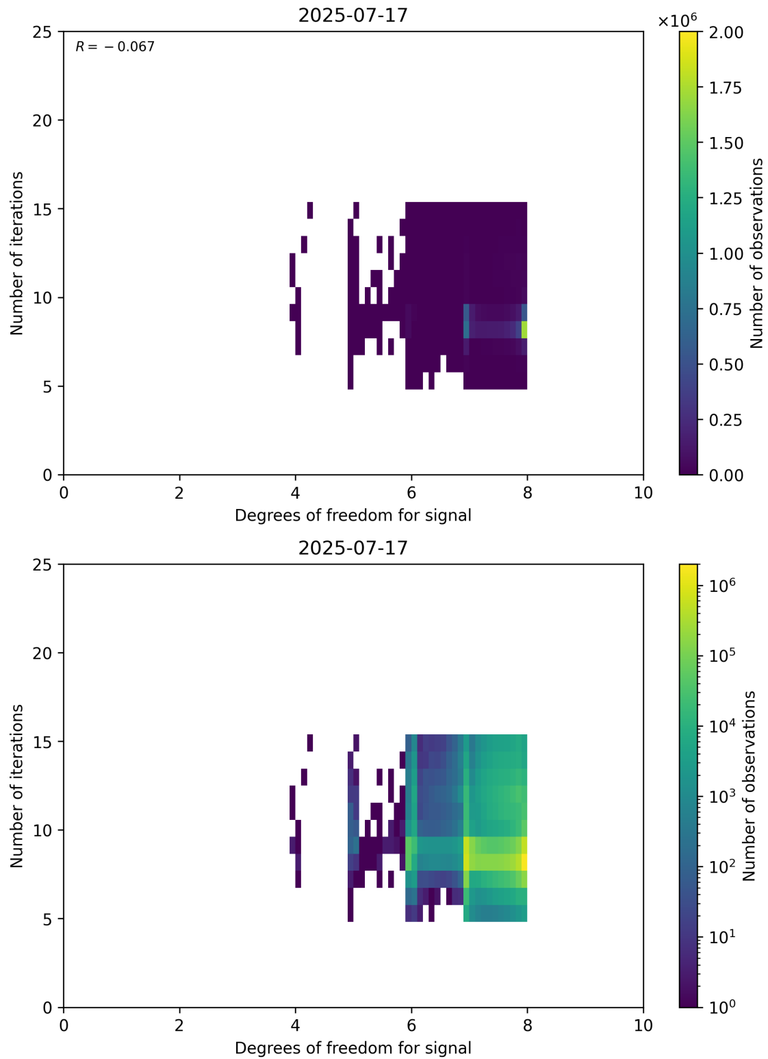
Figure 50: Scatter density plot of “Degrees of freedom for signal” against “Number of iterations” for 2025-07-16 to 2025-07-18.
