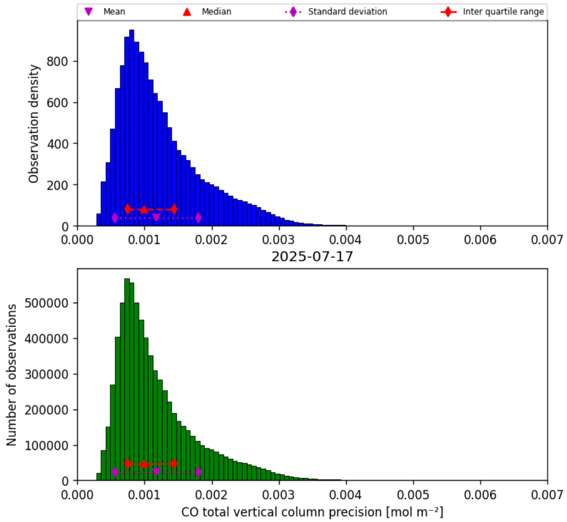
Figure 20: Histogram of “CO total vertical column precision” for 2025-07-16 to 2025-07-18
