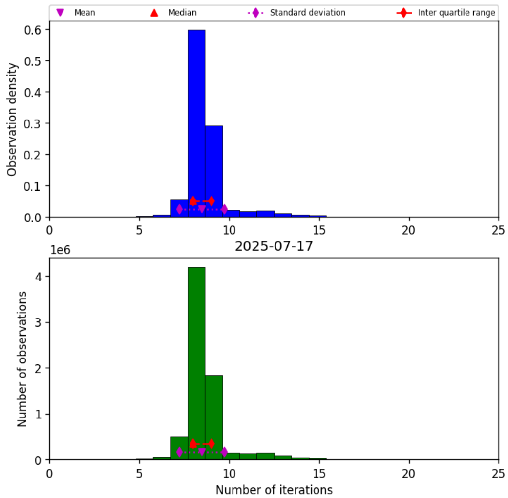
Figure 24: Histogram of “Number of iterations” for 2025-07-16 to 2025-07-18
