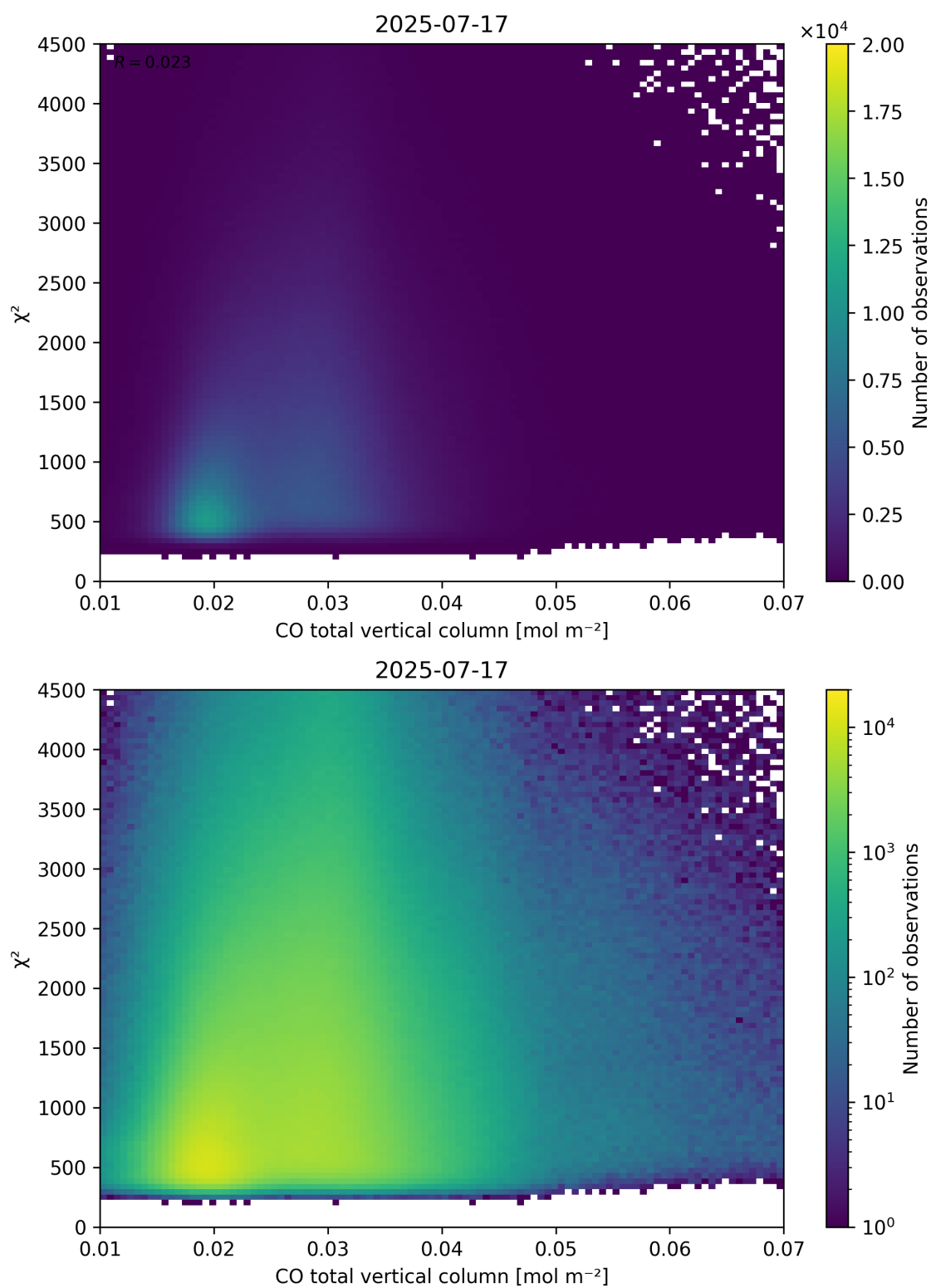
Figure 35: Scatter density plot of “CO total vertical column” against “ \chi^2 ” for 2025-07-16 to 2025-07-18.
