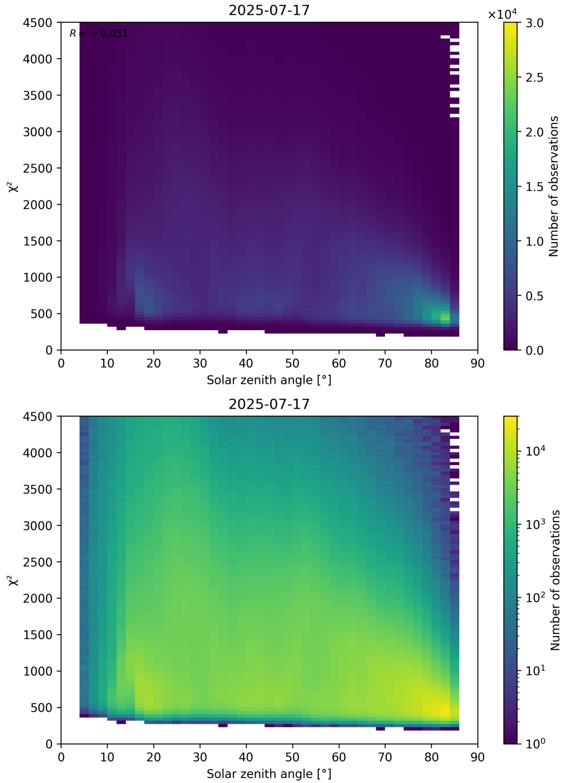
Figure 64: Scatter density plot of “Solar zenith angle” against “ \chi^2 ” for 2025-07-16 to 2025-07-18.
