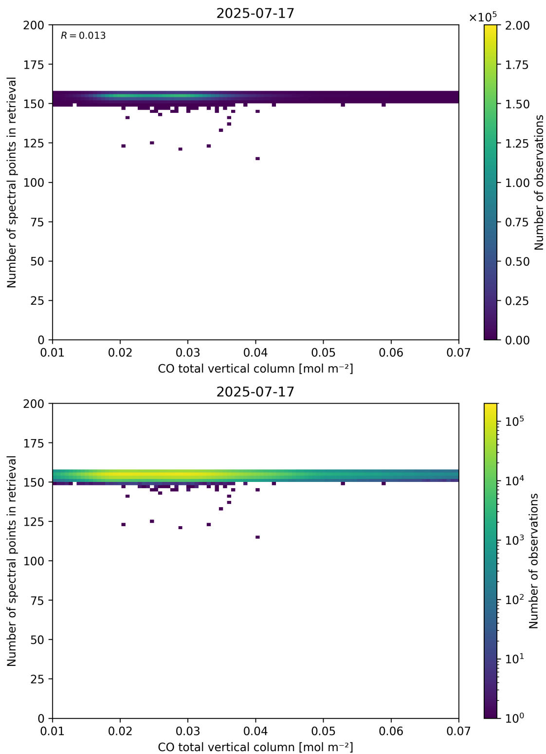
Figure 43: Scatter density plot of “CO total vertical column” against “Number of spectral points in retrieval” for 2025-07-16 to 2025-07-18.
