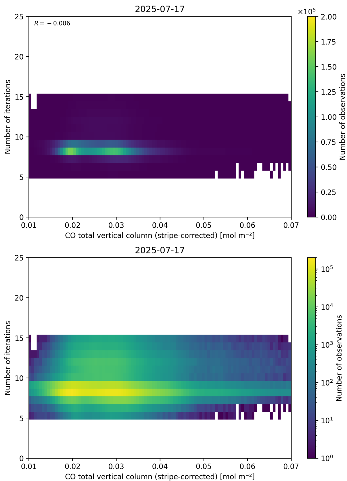
Figure 39: Scatter density plot of “CO total vertical column (stripe-corrected)” against “Number of iterations” for 2025-07-16 to 2025-07-18.
