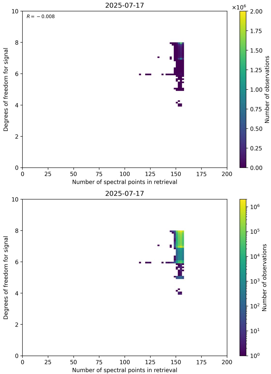
Figure 59: Scatter density plot of “Number of spectral points in retrieval” against “Degrees of freedom for signal” for 2025-07-16 to 2025-07-18.
