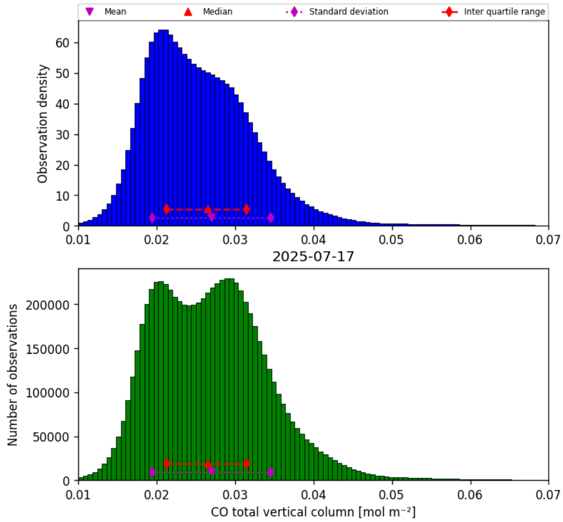
Figure 18: Histogram of “CO total vertical column” for 2025-07-16 to 2025-07-18
