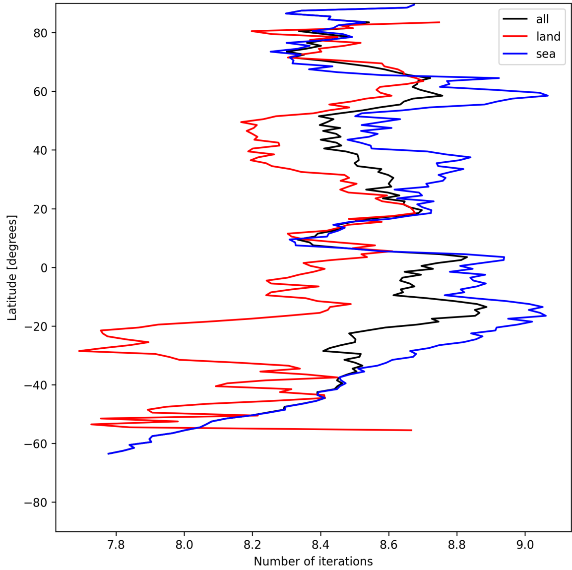
Figure 16: Zonal average of “Number of iterations” for 2025-07-16 to 2025-07-18.
