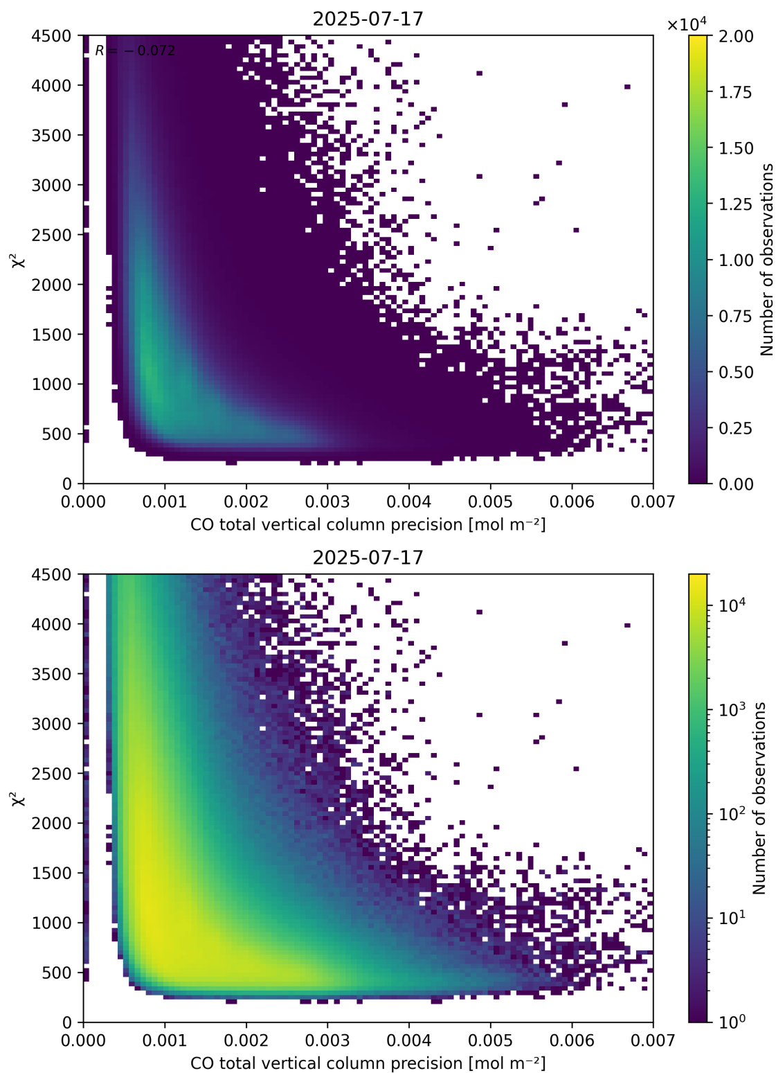
Figure 44: Scatter density plot of “CO total vertical column precision” against “ \chi^2 ” for 2025-07-16 to 2025-07-18.
