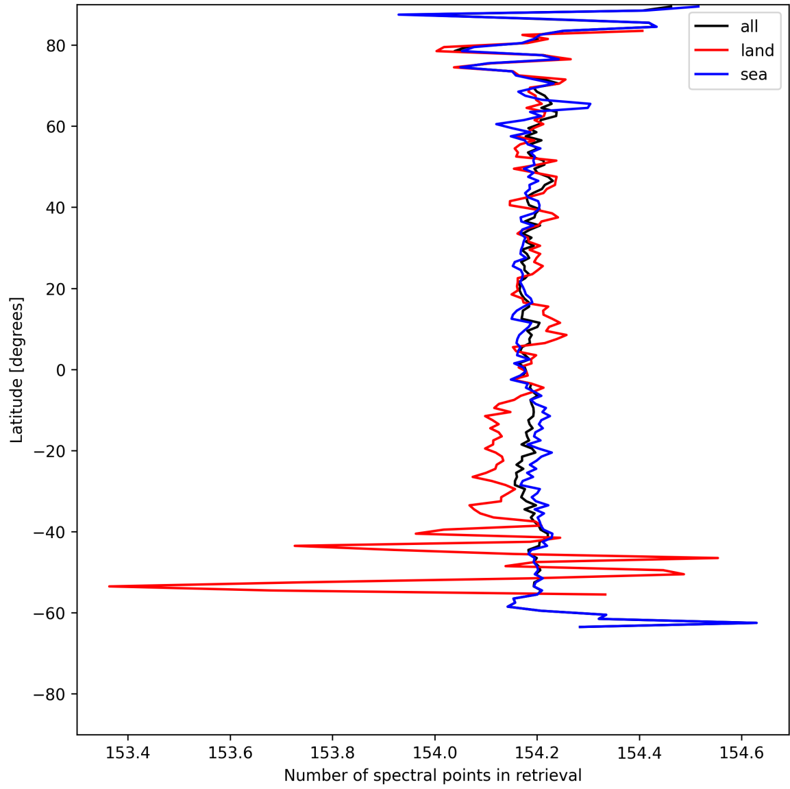
Figure 13: Zonal average of “Number of spectral points in retrieval” for 2025-07-16 to 2025-07-18.
