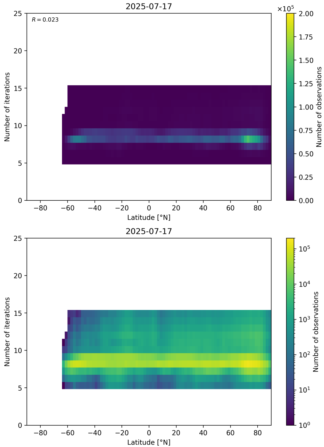
Figure 56: Scatter density plot of “Latitude” against “Number of iterations” for 2025-07-16 to 2025-07-18.
