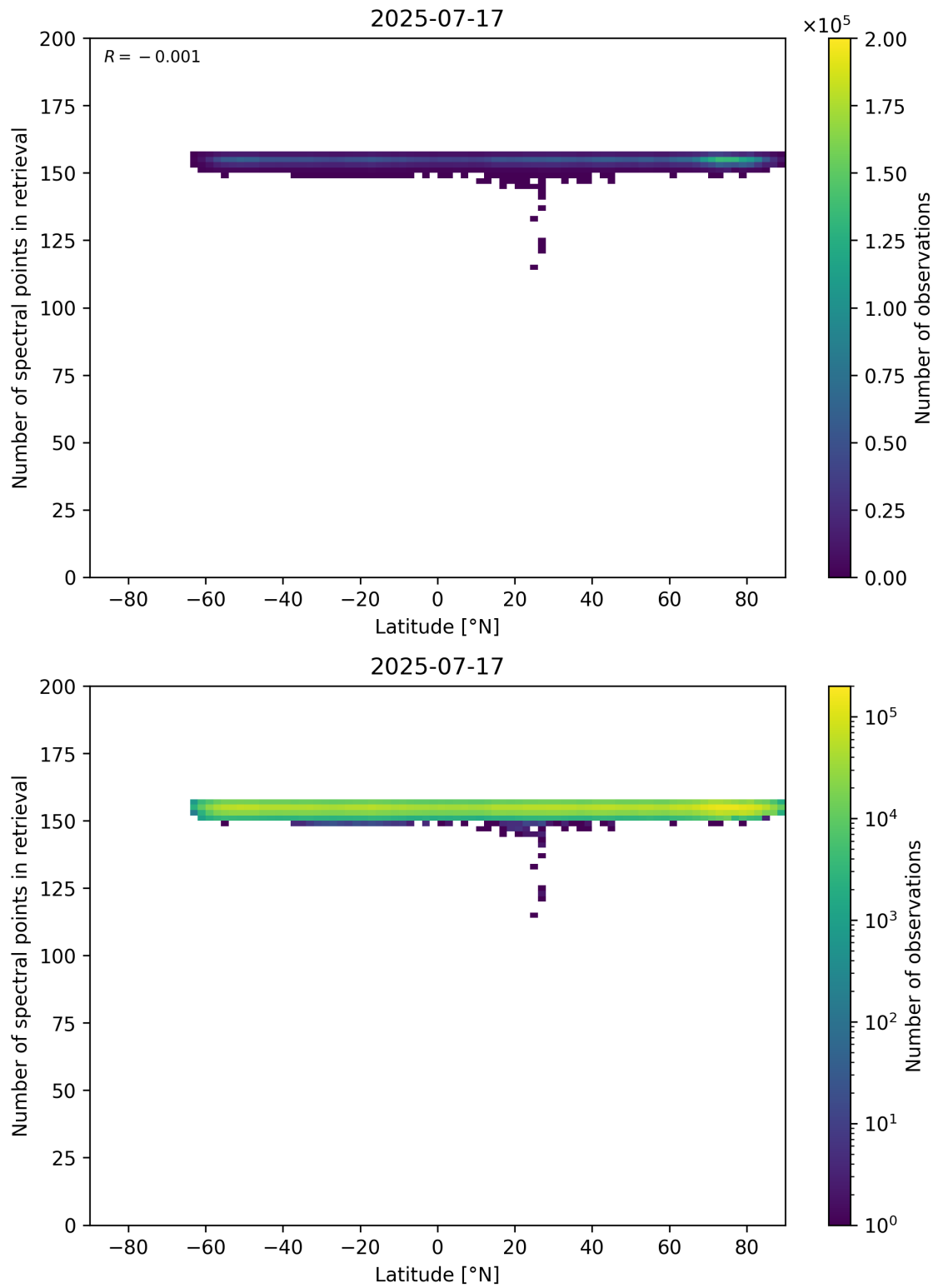
Figure 57: Scatter density plot of “Latitude” against “Number of spectral points in retrieval” for 2025-07-16 to 2025-07-18.
