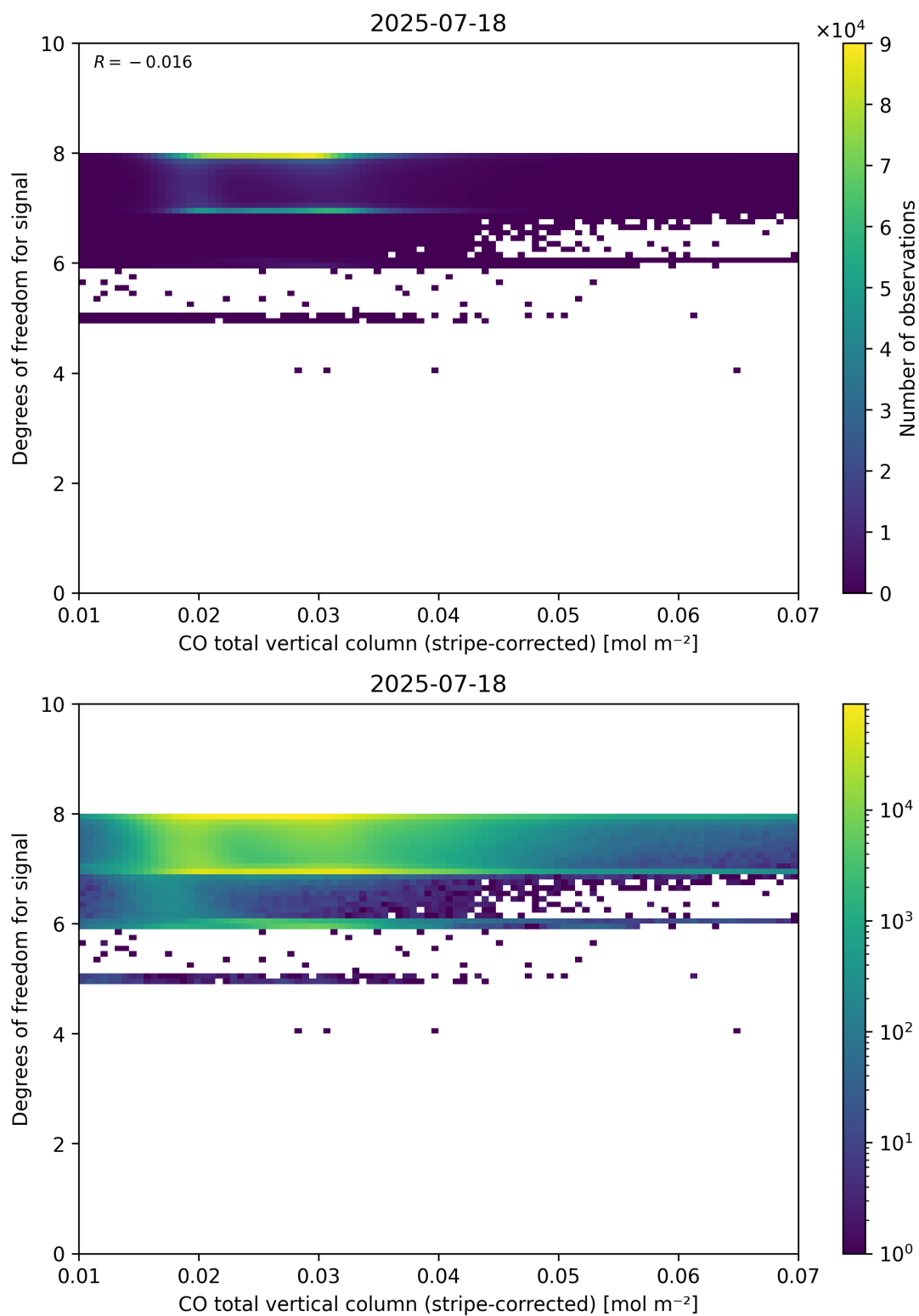
Figure 38: Scatter density plot of “CO total vertical column (stripe-corrected)” against “Degrees of freedom for signal” for 2025-07-18 to 2025-07-19.
