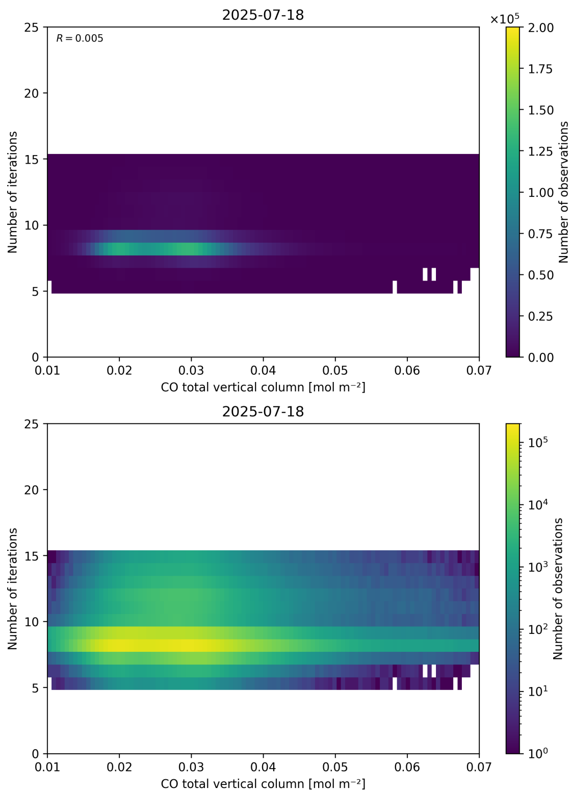
Figure 42: Scatter density plot of “CO total vertical column” against “Number of iterations” for 2025-07-18 to 2025-07-19.
