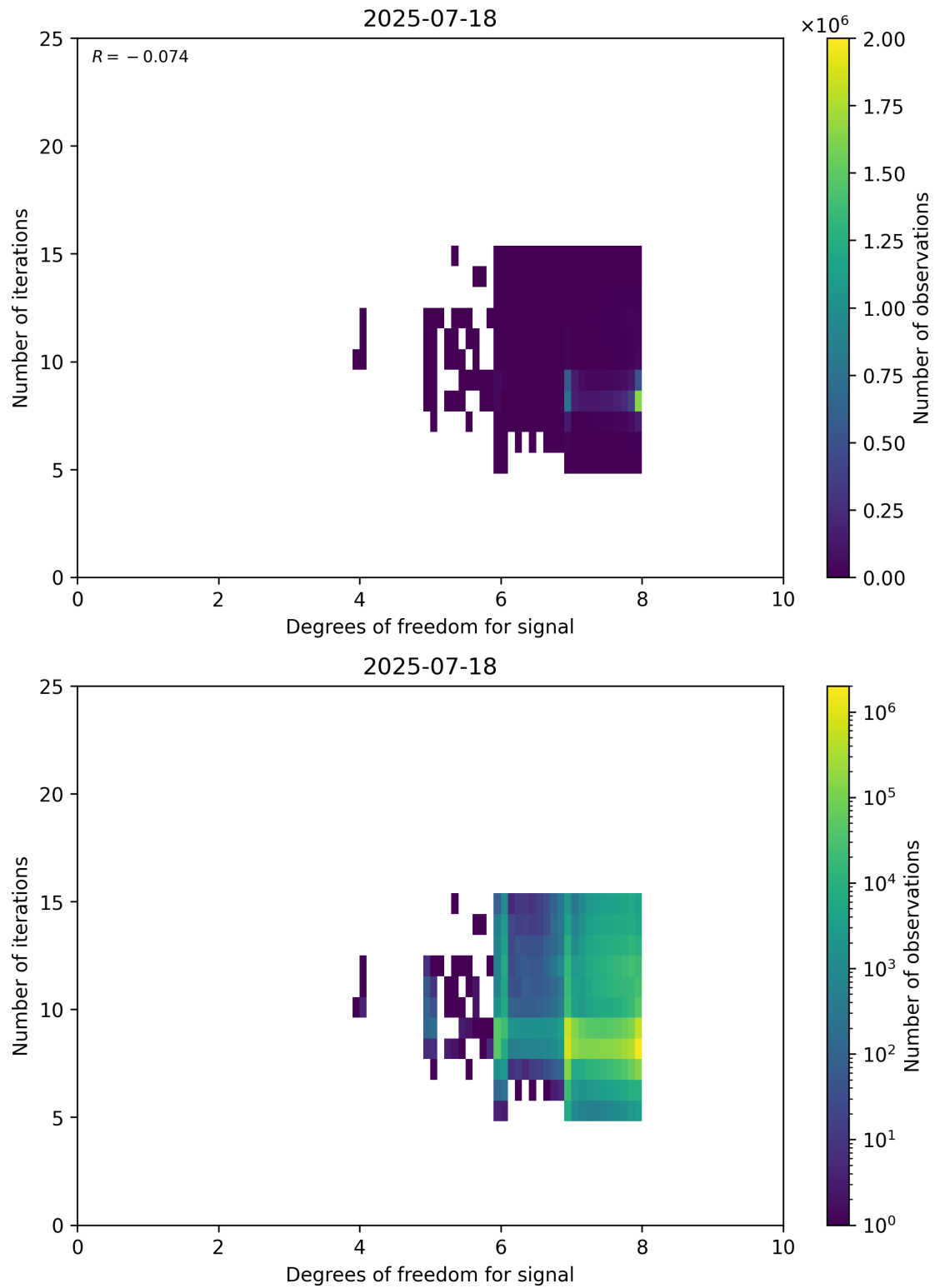
Figure 50: Scatter density plot of “Degrees of freedom for signal” against “Number of iterations” for 2025-07-18 to 2025-07-19.
