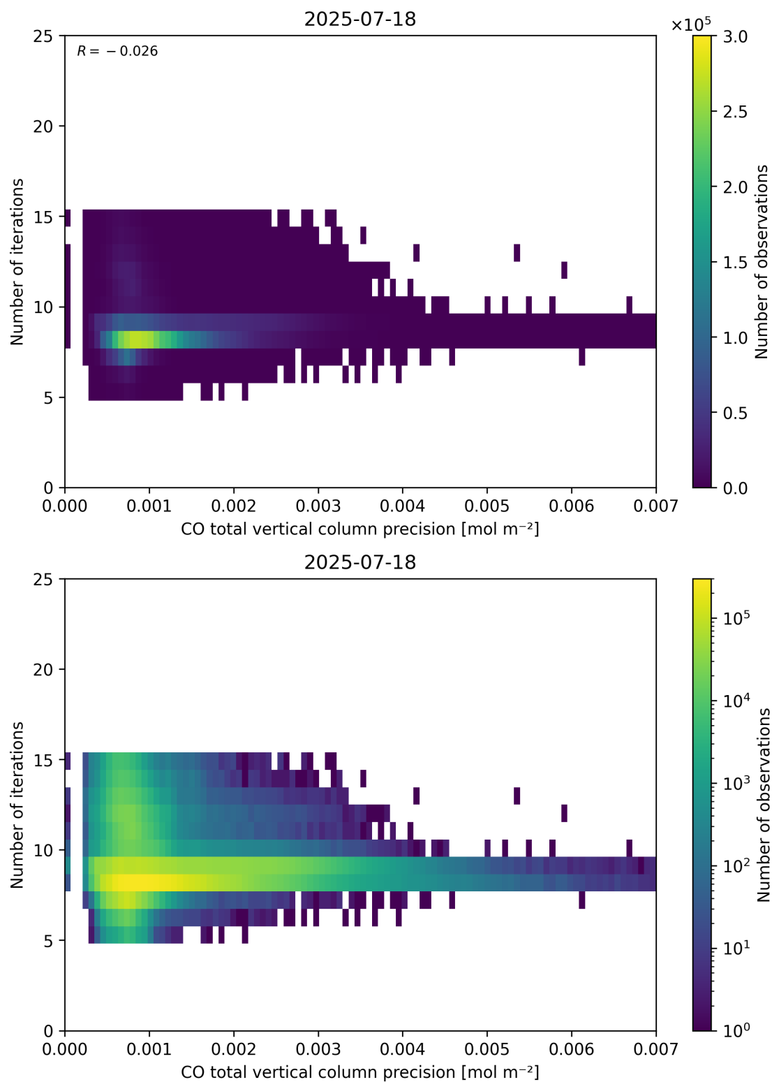
Figure 46: Scatter density plot of “CO total vertical column precision” against “Number of iterations” for 2025-07-18 to 2025-07-19.
