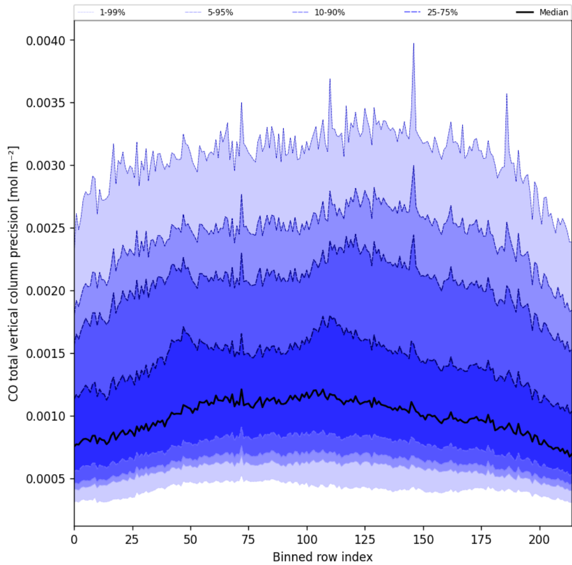
Figure 28: Along track statistics of “CO total vertical column precision” for 2025-07-18 to 2025-07-19
