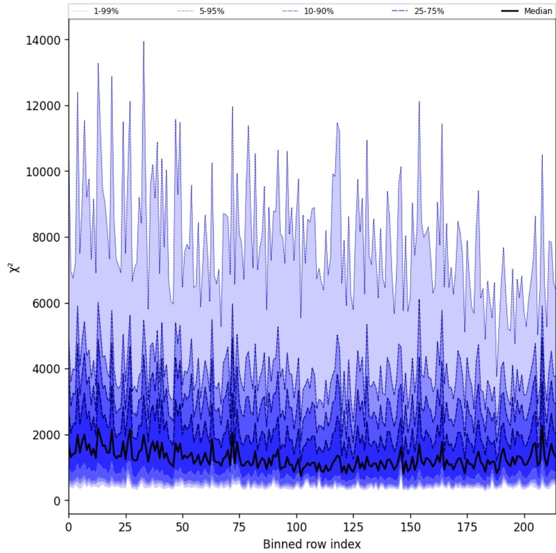
Figure 30: Along track statistics of “ \chi^2 ” for 2025-07-18 to 2025-07-19
