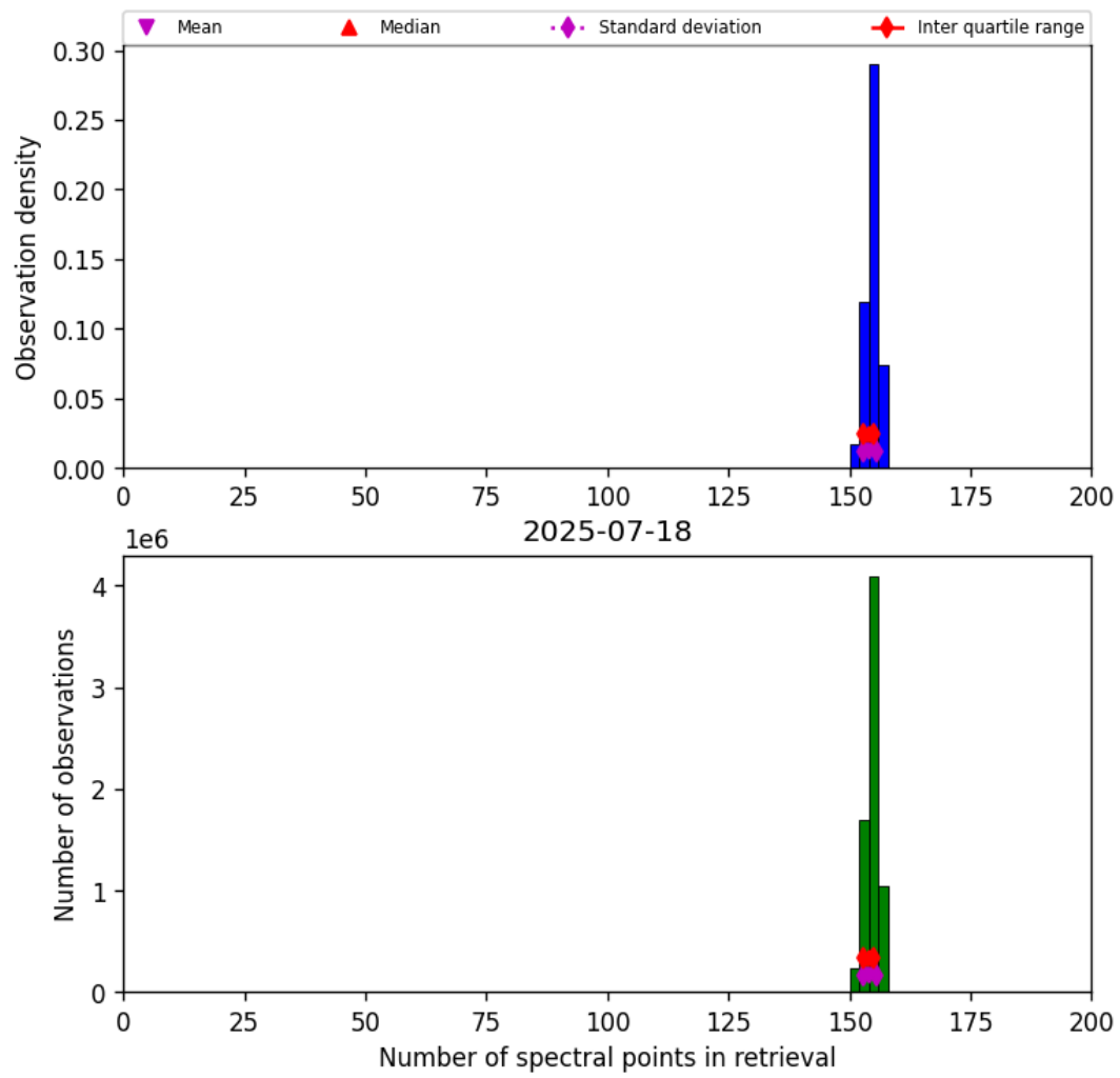
Figure 21: Histogram of “Number of spectral points in retrieval” for 2025-07-18 to 2025-07-19
