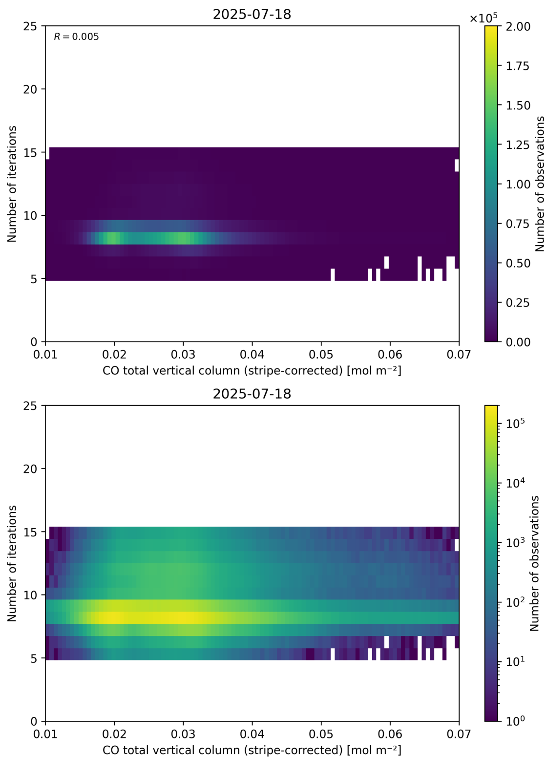
Figure 39: Scatter density plot of “CO total vertical column (stripe-corrected)” against “Number of iterations” for 2025-07-18 to 2025-07-19.
