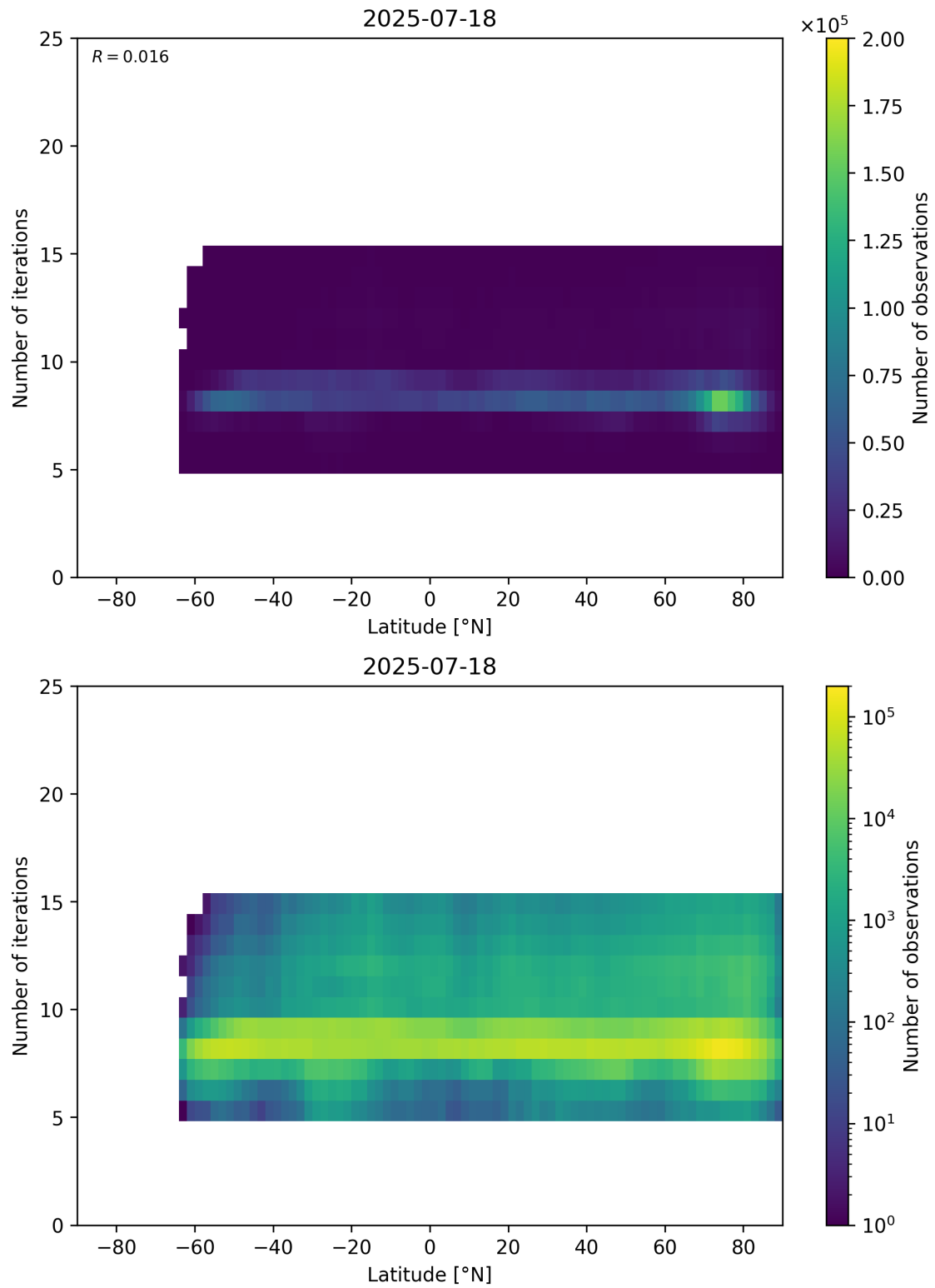
Figure 56: Scatter density plot of “Latitude” against “Number of iterations” for 2025-07-18 to 2025-07-19.
