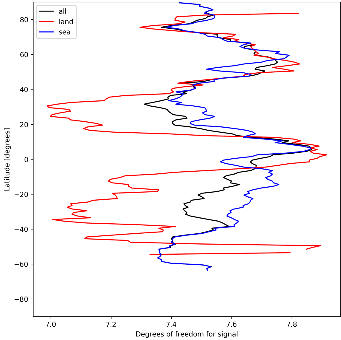
Figure 15: Zonal average of “Degrees of freedom for signal” for 2025-07-18 to 2025-07-19.
