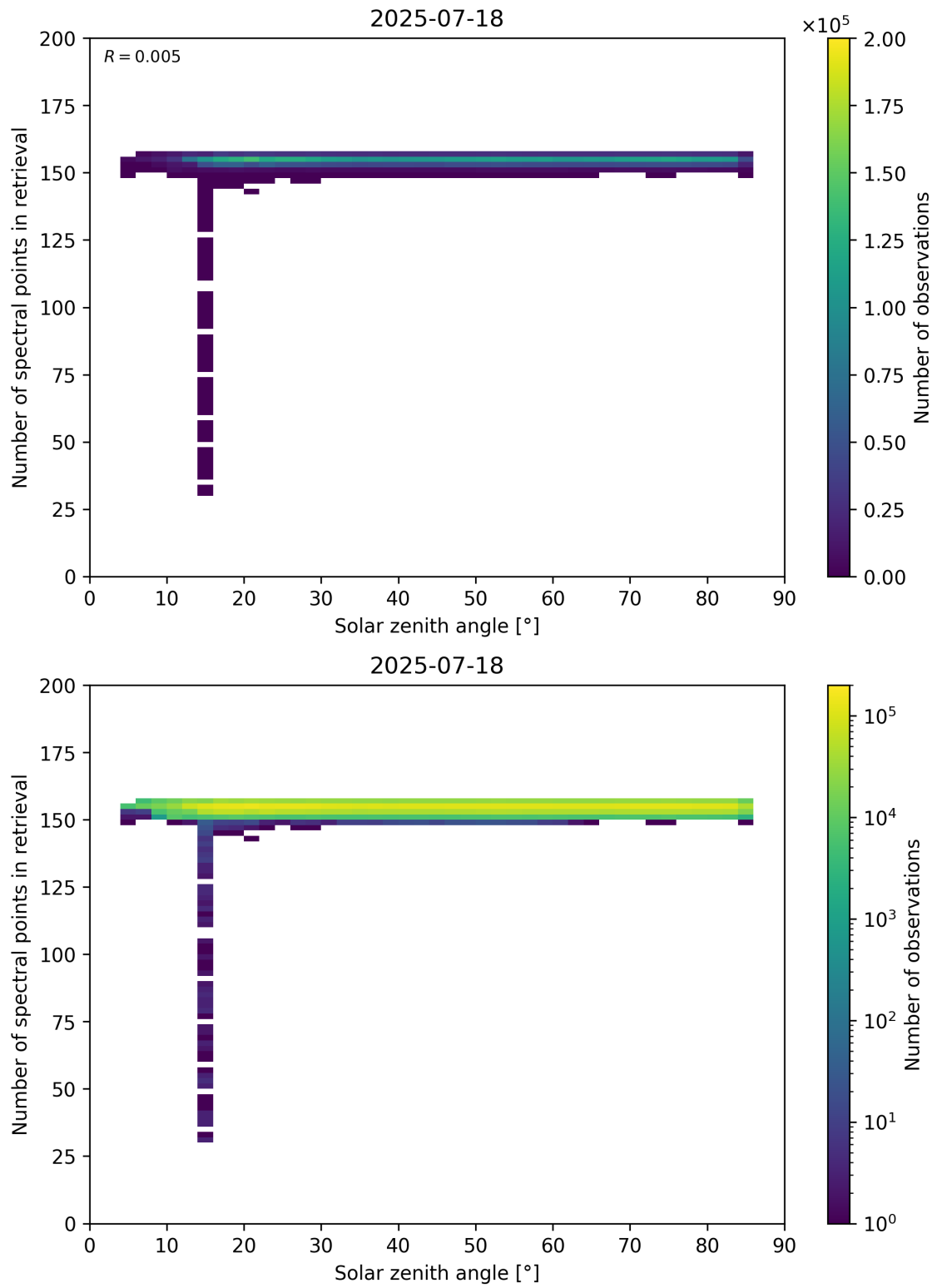
Figure 68: Scatter density plot of “Solar zenith angle” against “Number of spectral points in retrieval” for 2025-07-18 to 2025-07-19.
