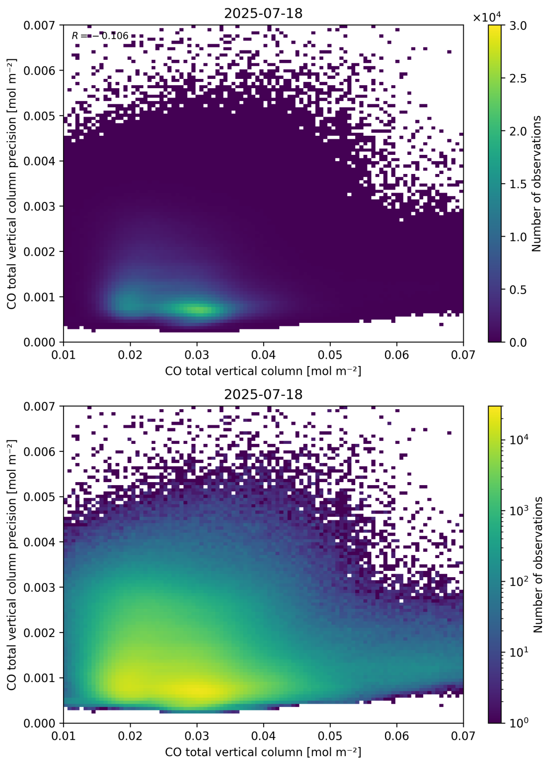
Figure 34: Scatter density plot of “CO total vertical column” against “CO total vertical column precision” for 2025-07-18 to 2025-07-19.
