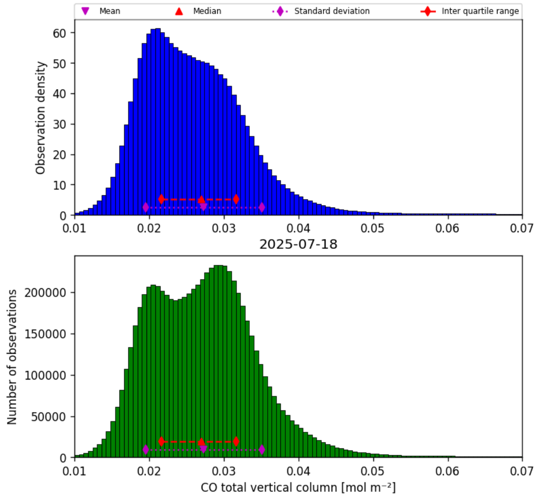
Figure 18: Histogram of “CO total vertical column” for 2025-07-18 to 2025-07-19
