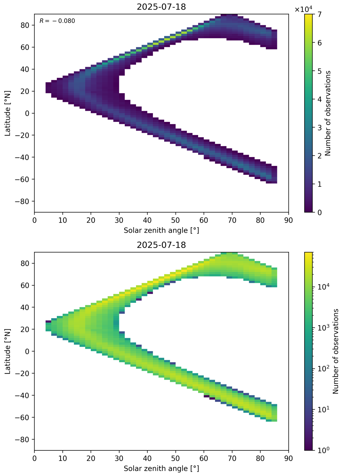
Figure 66: Scatter density plot of “Solar zenith angle” against “Latitude” for 2025-07-18 to 2025-07-19.
