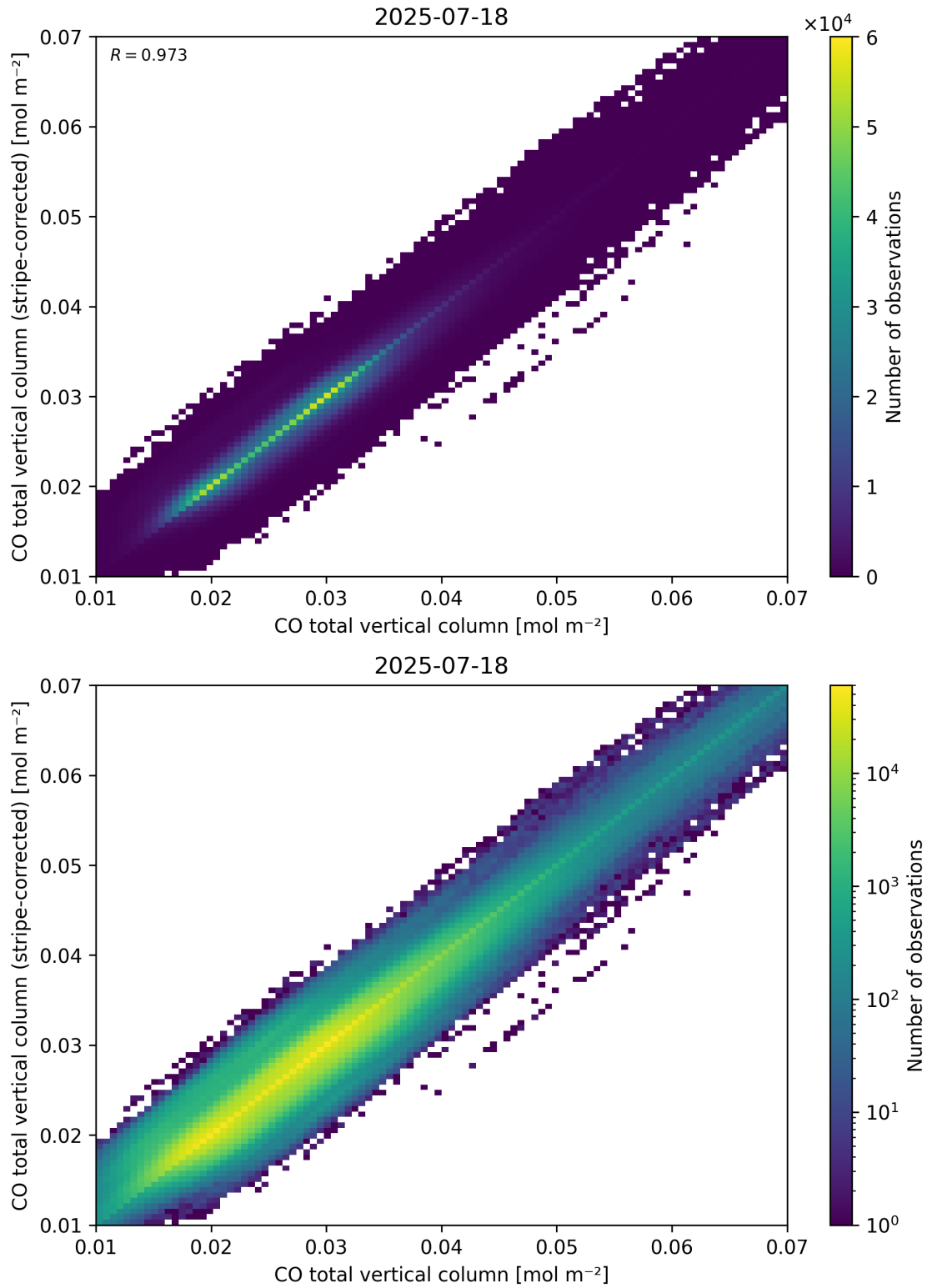
Figure 33: Scatter density plot of “CO total vertical column” against “CO total vertical column (stripe-corrected)” for 2025-07-18 to 2025-07-19.
