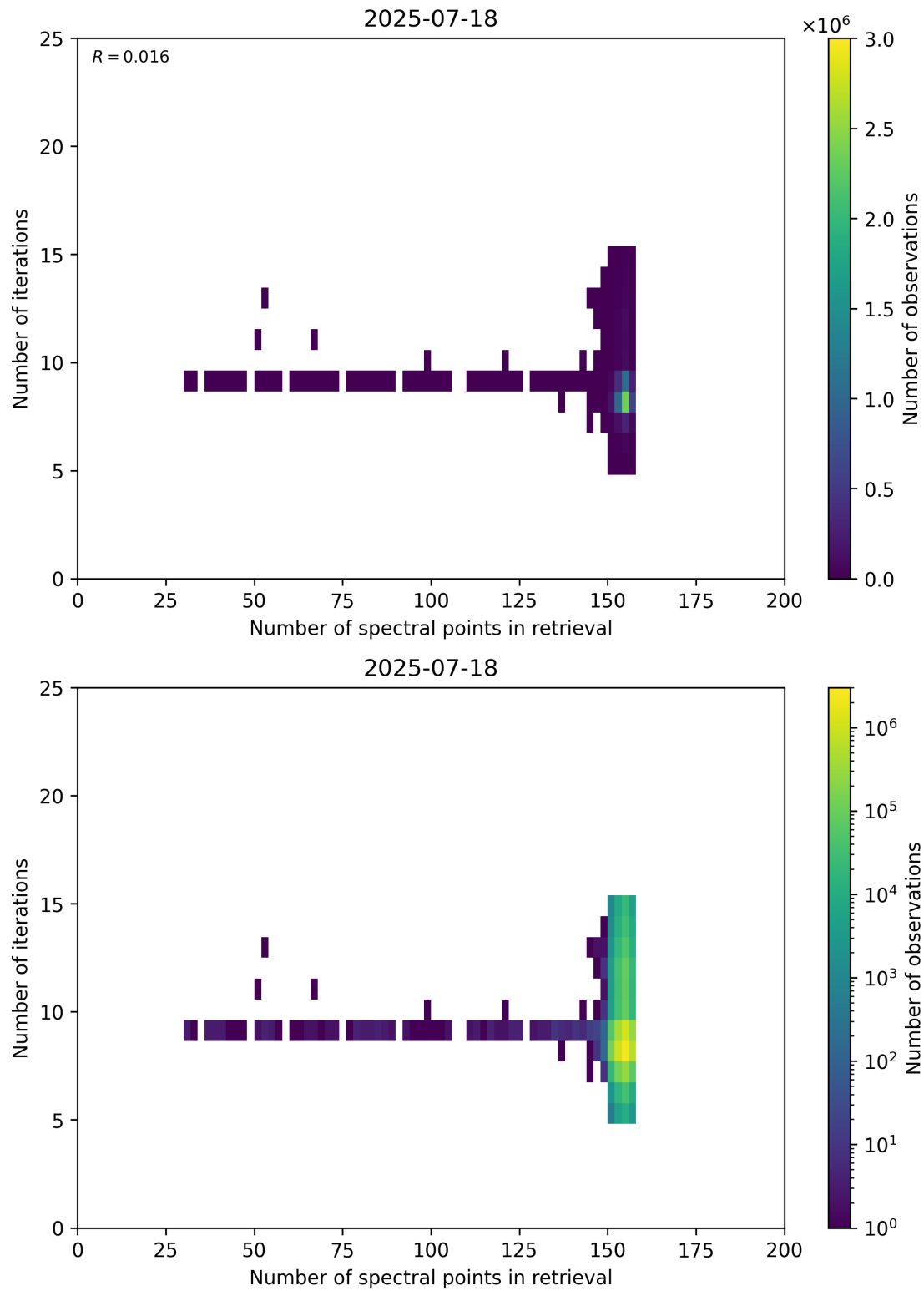
Figure 60: Scatter density plot of “Number of spectral points in retrieval” against “Number of iterations” for 2025-07-18 to 2025-07-19.
