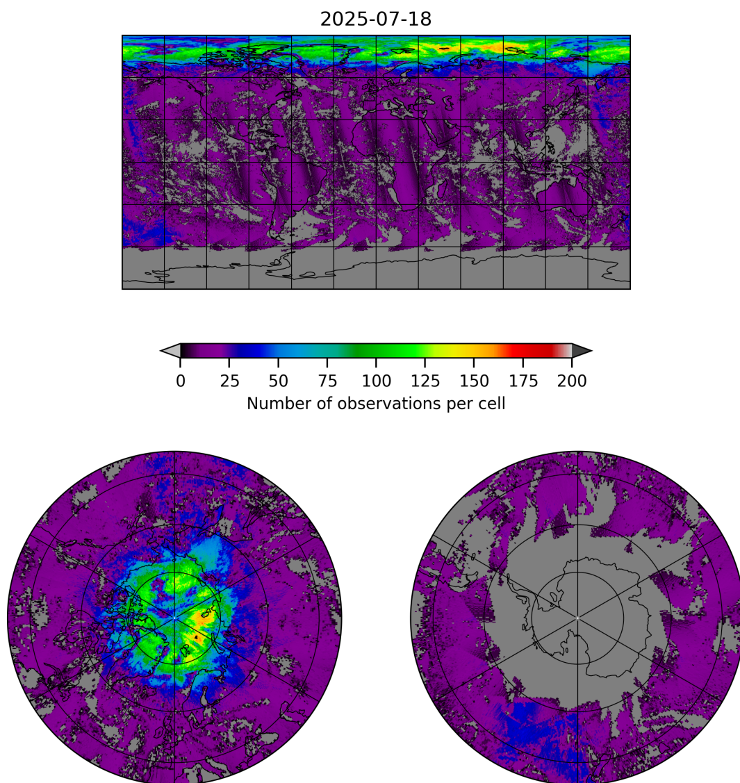
Figure 8: Map of the number of observations for 2025-07-18 to 2025-07-19
