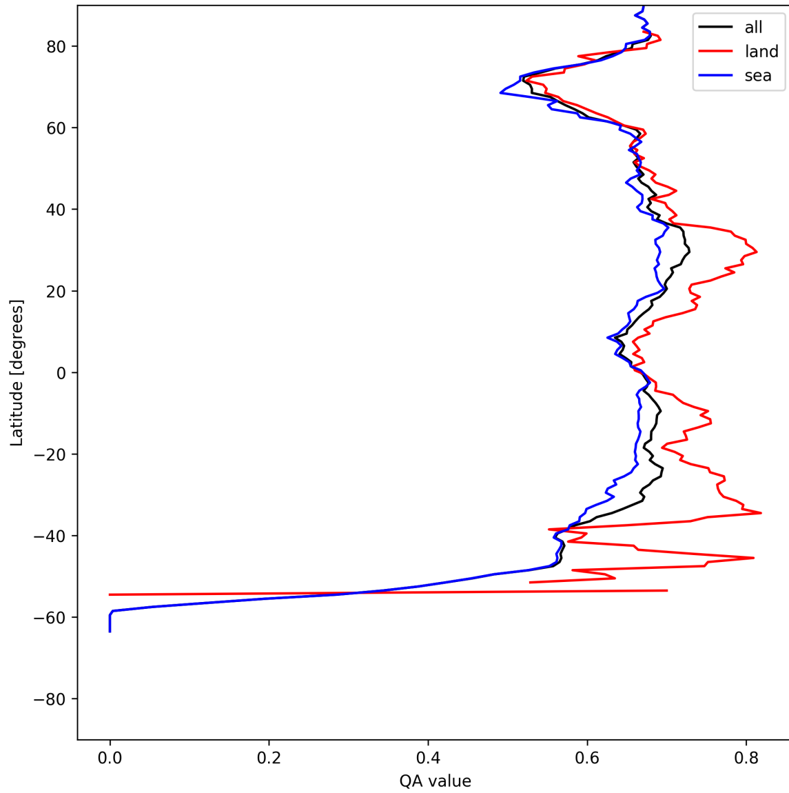
Figure 9: Zonal average of “QA value” for 2025-07-18 to 2025-07-19.
