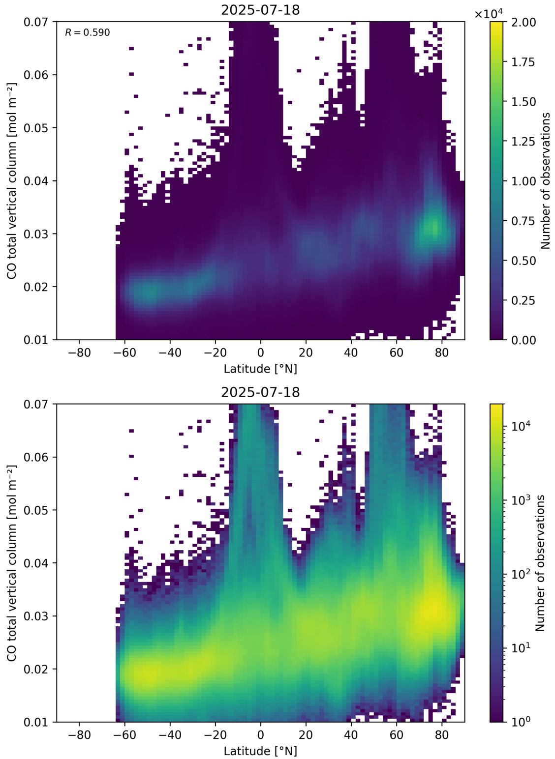
Figure 51: Scatter density plot of “Latitude” against “CO total vertical column” for 2025-07-18 to 2025-07-19.
