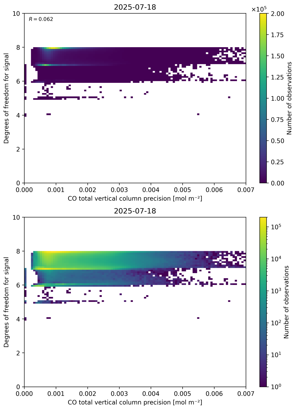
Figure 45: Scatter density plot of “CO total vertical column precision” against “Degrees of freedom for signal” for 2025-07-18 to 2025-07-19.
