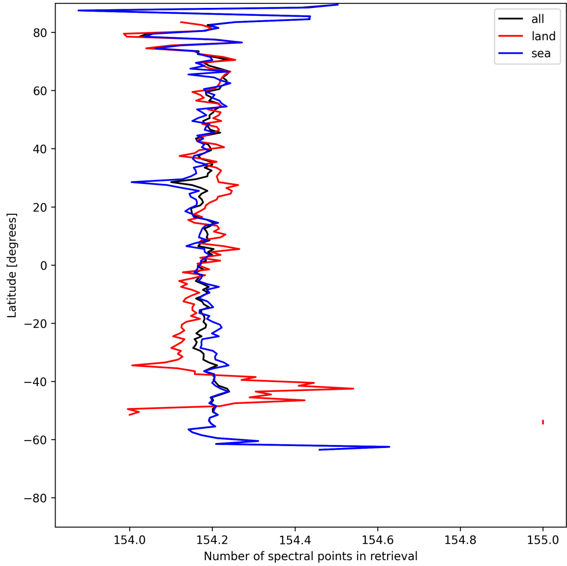
Figure 13: Zonal average of “Number of spectral points in retrieval” for 2025-07-18 to 2025-07-19.
