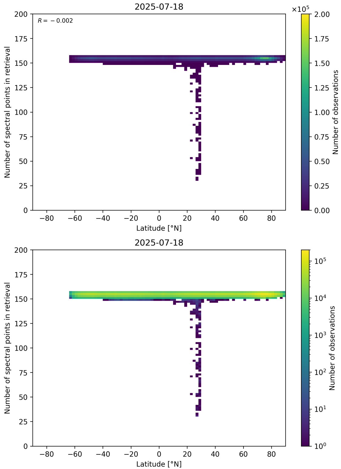
Figure 57: Scatter density plot of “Latitude” against “Number of spectral points in retrieval” for 2025-07-18 to 2025-07-19.
