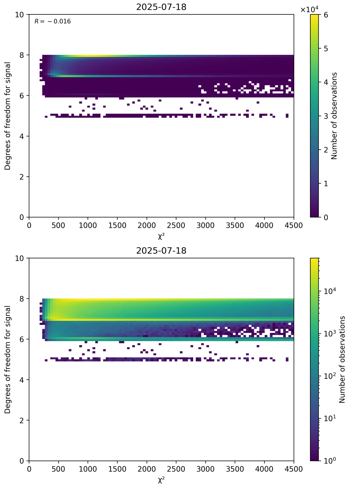
Figure 48: Scatter density plot of “ \chi^2 ” against “Degrees of freedom for signal” for 2025-07-18 to 2025-07-19.
