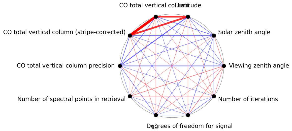
Figure 1: Map of correlation graph for 2025-07-18 to 2025-07-19.
