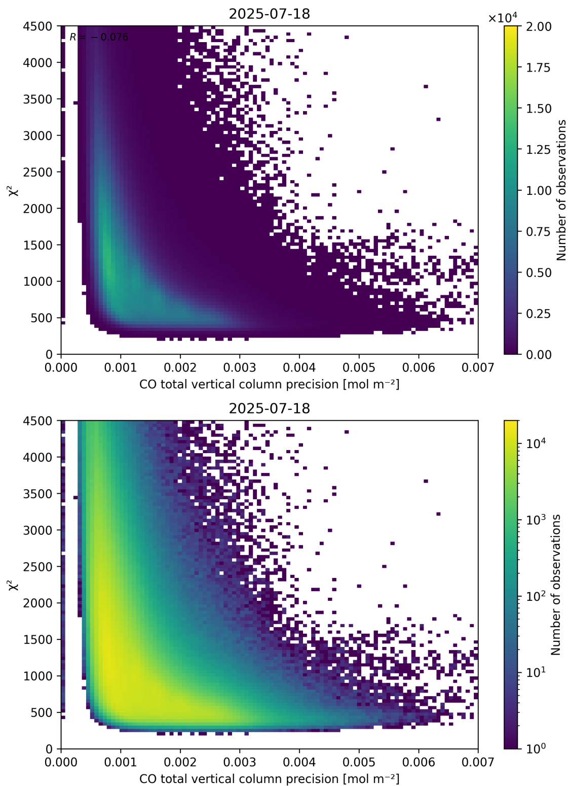
Figure 44: Scatter density plot of “CO total vertical column precision” against “ \chi^2 ” for 2025-07-18 to 2025-07-19.
