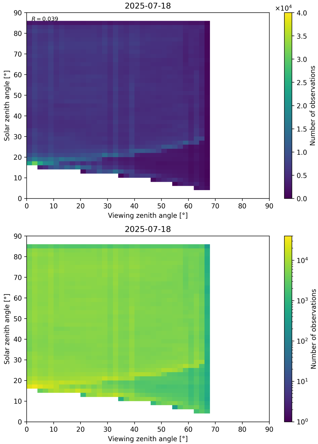
Figure 77: Scatter density plot of “Viewing zenith angle” against “Solar zenith angle” for 2025-07-18 to 2025-07-19.
