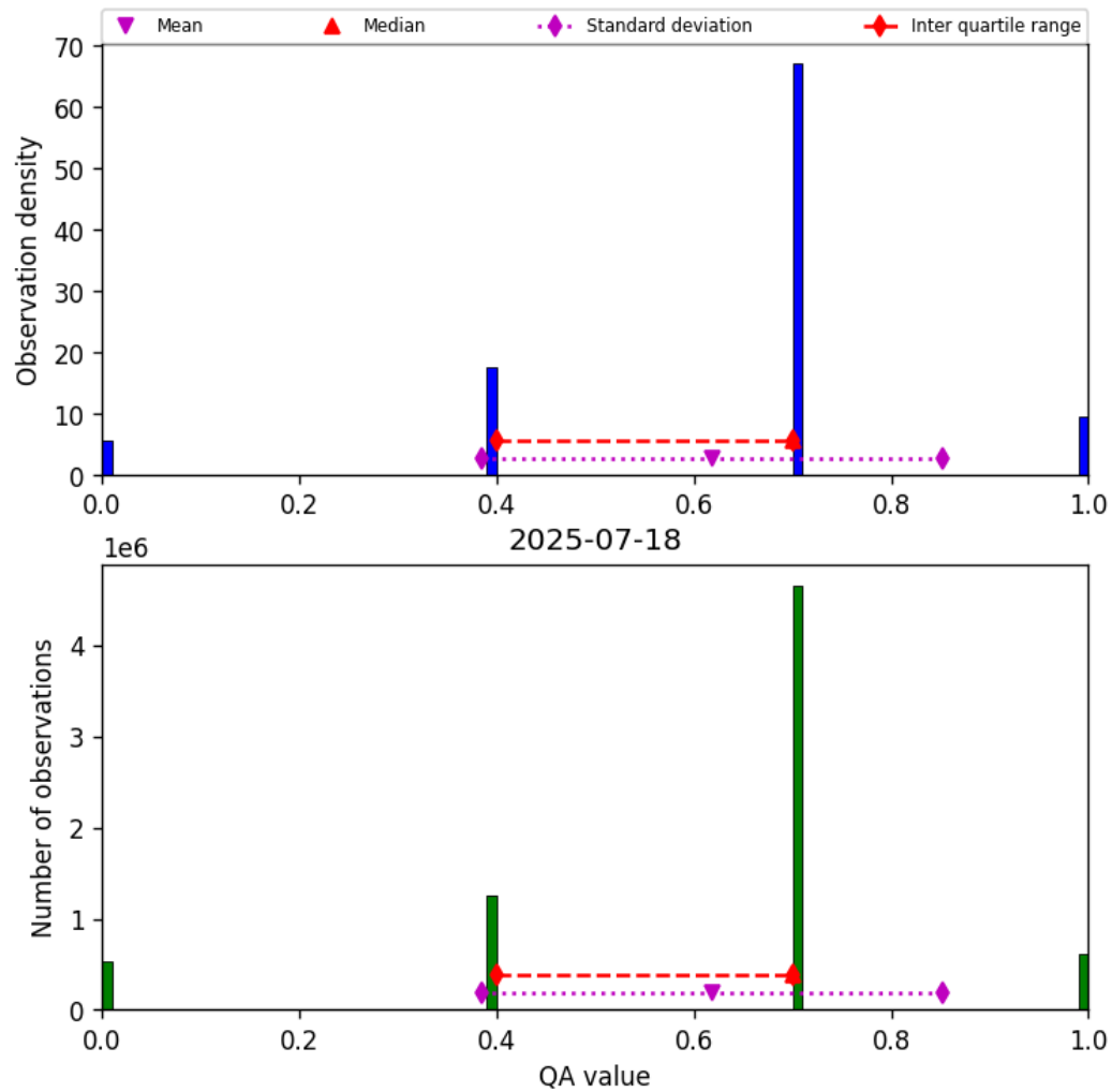
Figure 17: Histogram of “QA value” for 2025-07-18 to 2025-07-19
