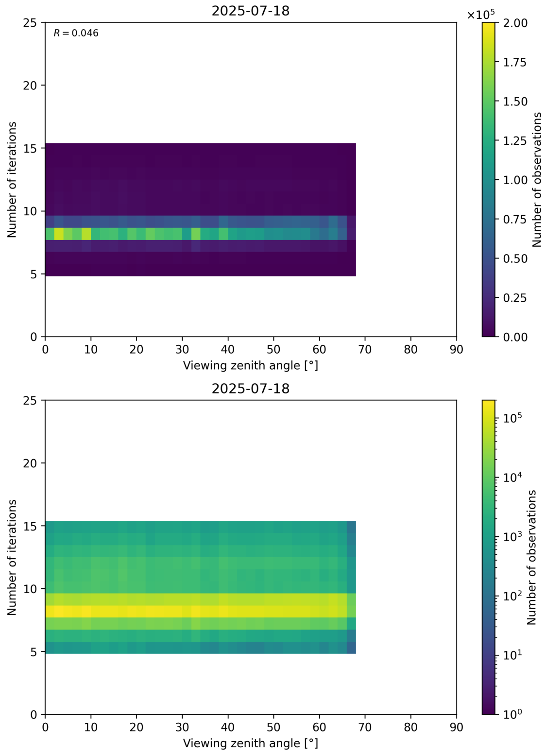
Figure 75: Scatter density plot of “Viewing zenith angle” against “Number of iterations” for 2025-07-18 to 2025-07-19.
