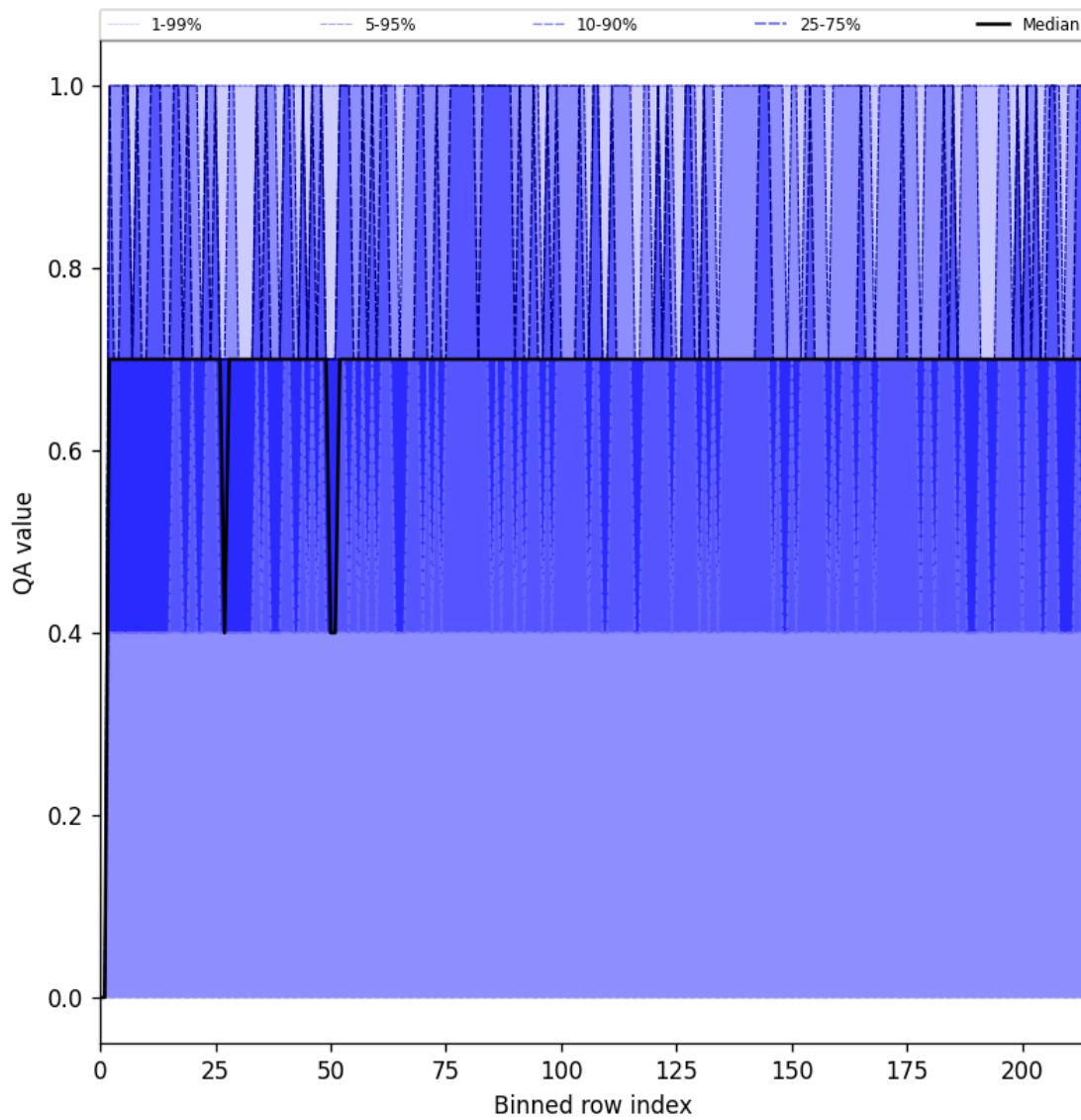
Figure 25: Along track statistics of “QA value” for 2025-07-18 to 2025-07-19
