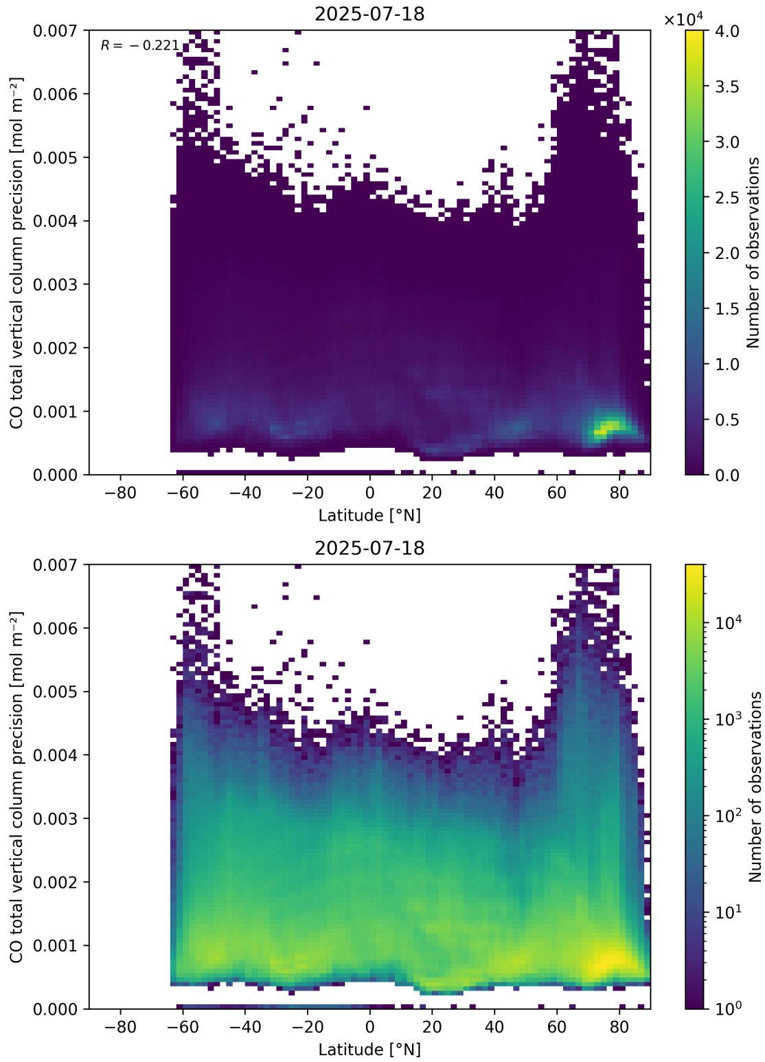
Figure 53: Scatter density plot of “Latitude” against “CO total vertical column precision” for 2025-07-18 to 2025-07-19.
