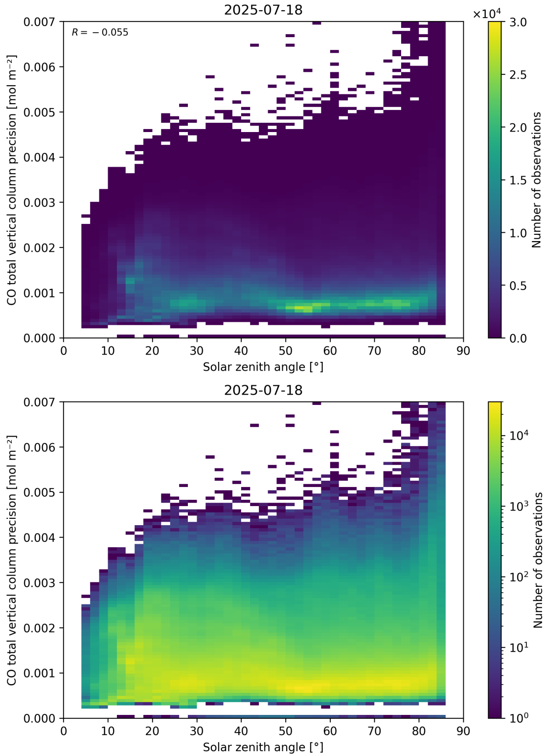
Figure 63: Scatter density plot of “Solar zenith angle” against “CO total vertical column precision” for 2025-07-18 to 2025-07-19.
