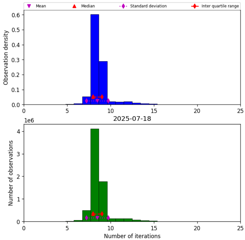
Figure 24: Histogram of “Number of iterations” for 2025-07-18 to 2025-07-19
