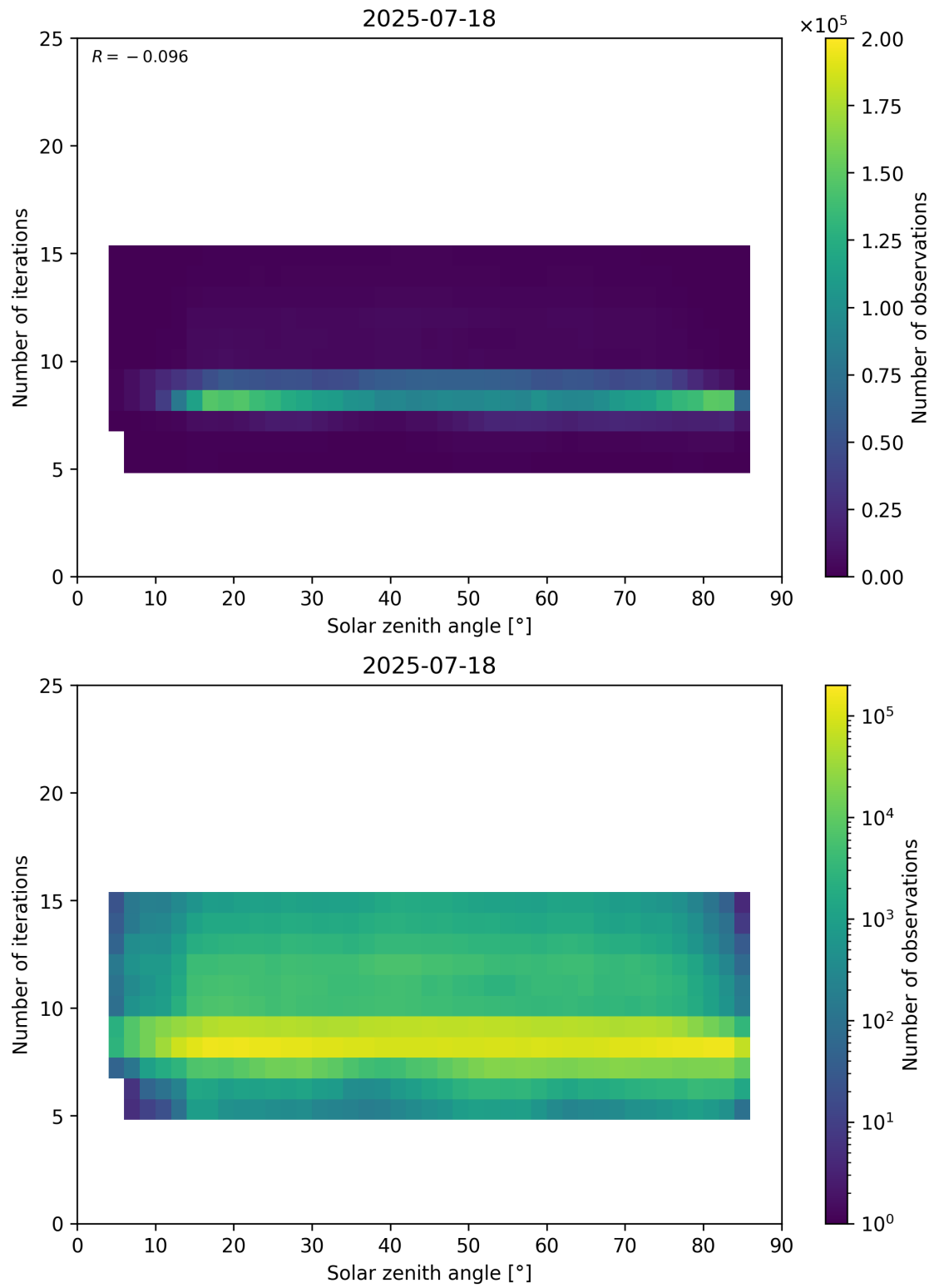
Figure 67: Scatter density plot of “Solar zenith angle” against “Number of iterations” for 2025-07-18 to 2025-07-19.
