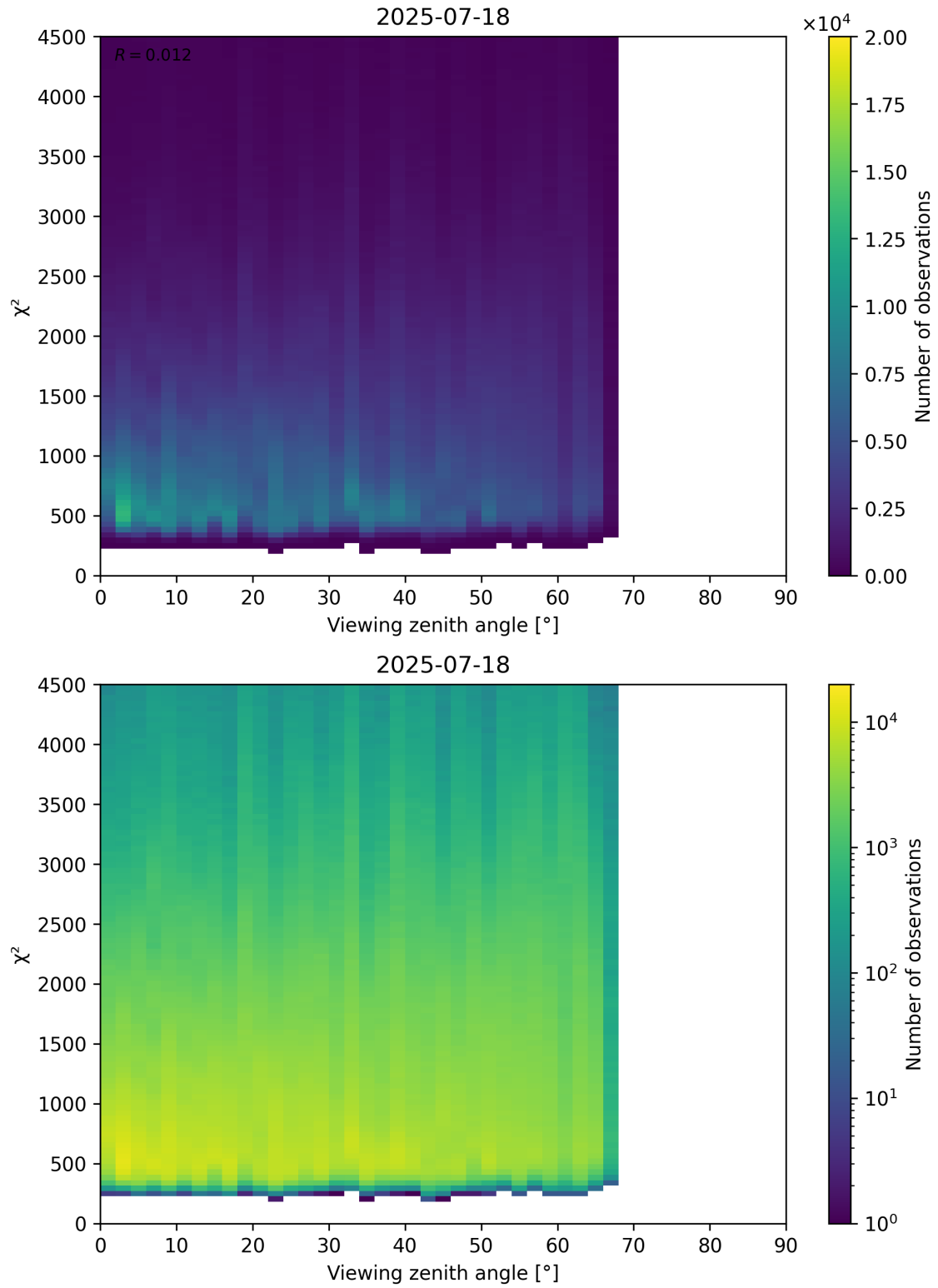
Figure 72: Scatter density plot of “Viewing zenith angle” against “ \chi^2 ” for 2025-07-18 to 2025-07-19.
