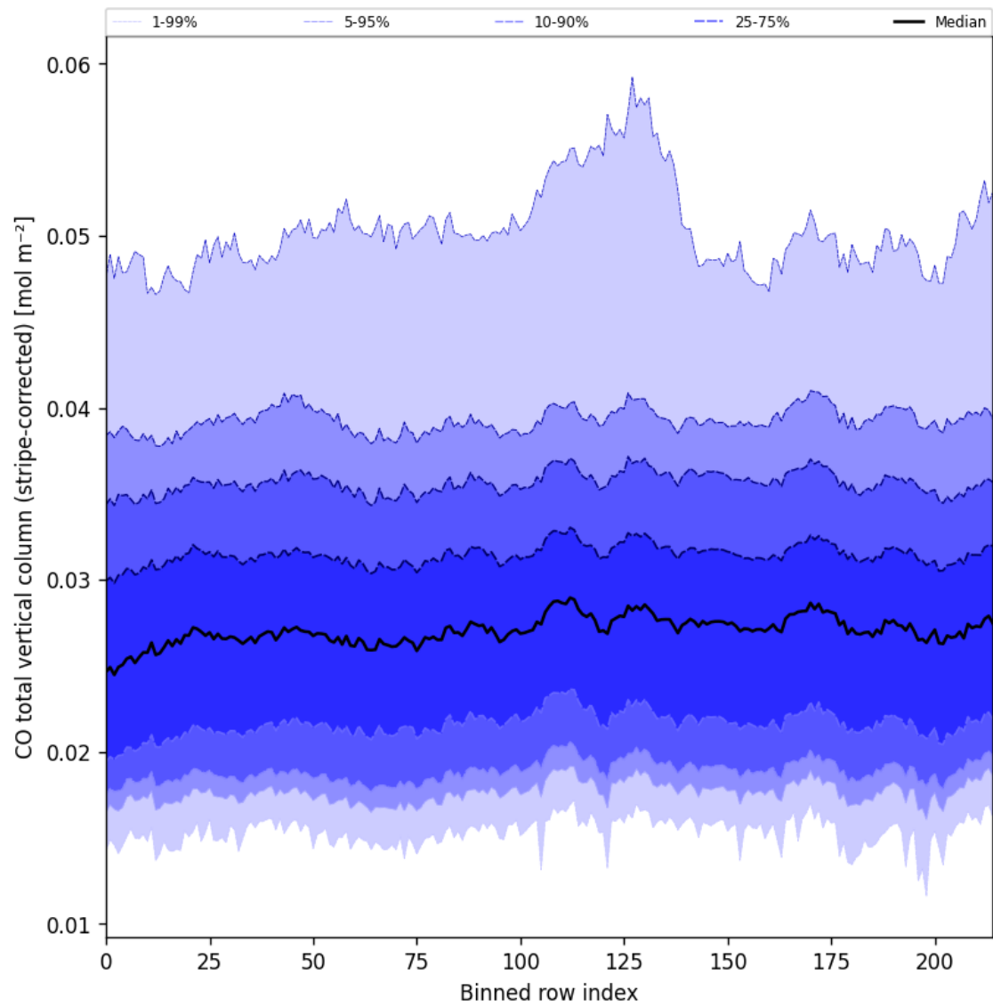
Figure 27: Along track statistics of “CO total vertical column (stripe-corrected)” for 2025-07-18 to 2025-07-19
