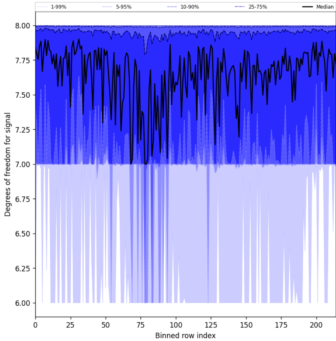
Figure 31: Along track statistics of “Degrees of freedom for signal” for 2025-07-18 to 2025-07-19
