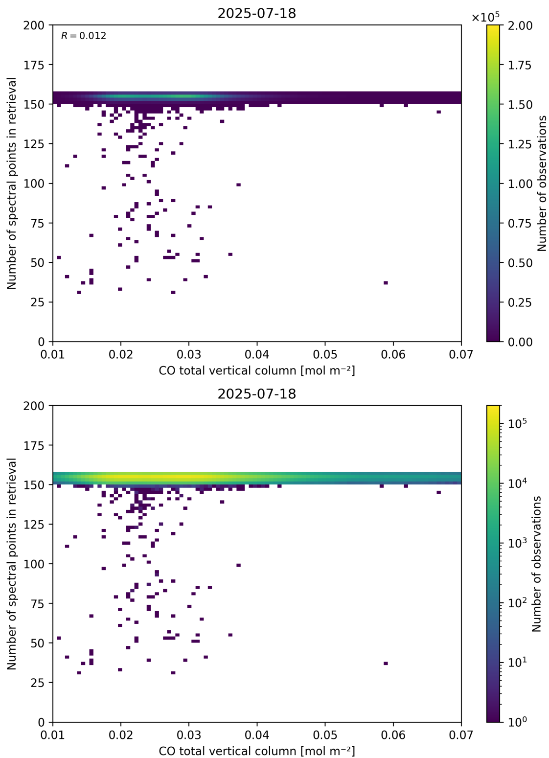
Figure 43: Scatter density plot of “CO total vertical column” against “Number of spectral points in retrieval” for 2025-07-18 to 2025-07-19.
