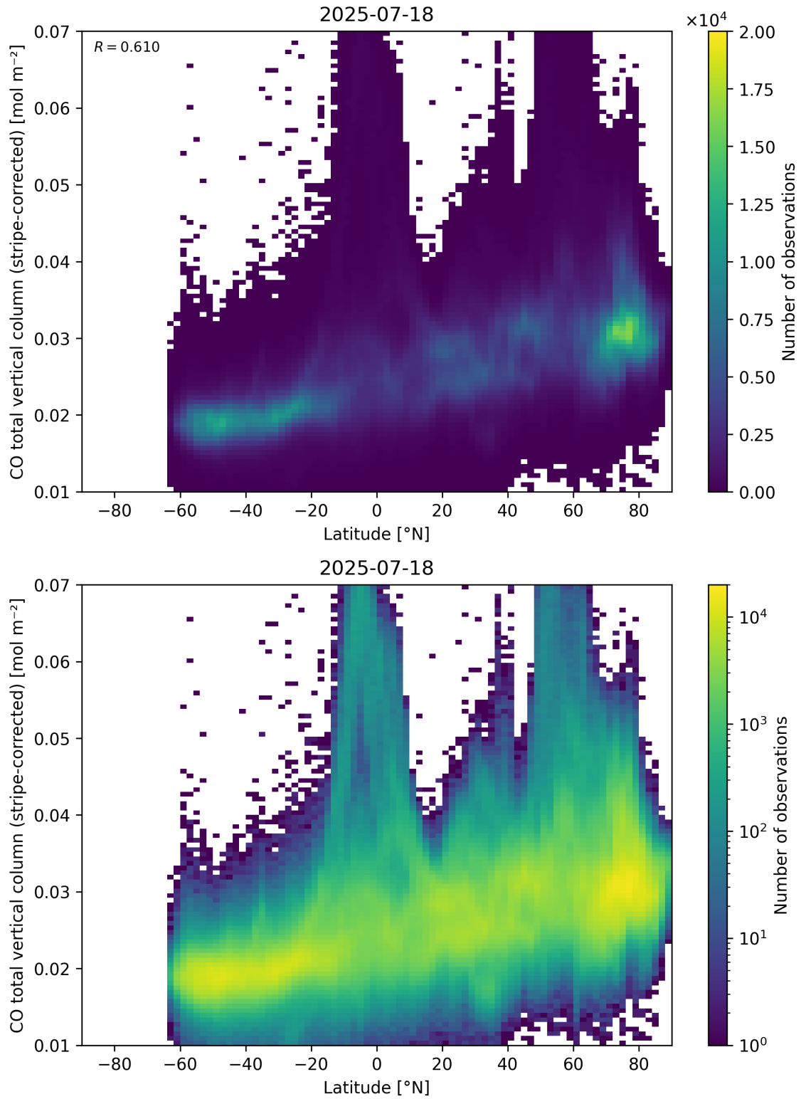
Figure 52: Scatter density plot of “Latitude” against “CO total vertical column (stripe-corrected)” for 2025-07-18 to 2025-07-19.
