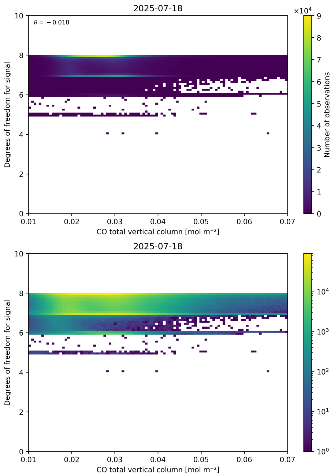
Figure 41: Scatter density plot of “CO total vertical column” against “Degrees of freedom for signal” for 2025-07-18 to 2025-07-19.
