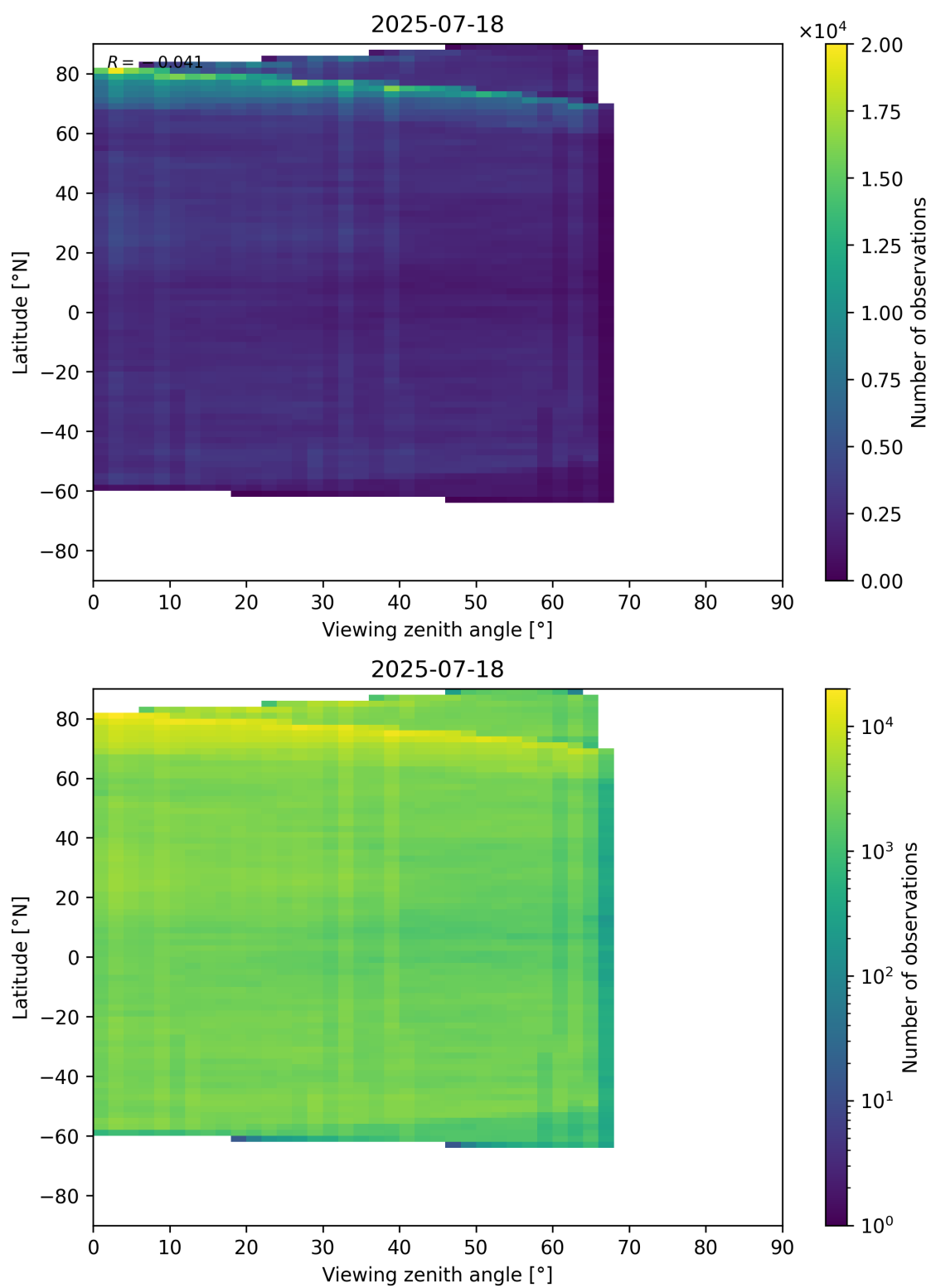
Figure 74: Scatter density plot of “Viewing zenith angle” against “Latitude” for 2025-07-18 to 2025-07-19.
