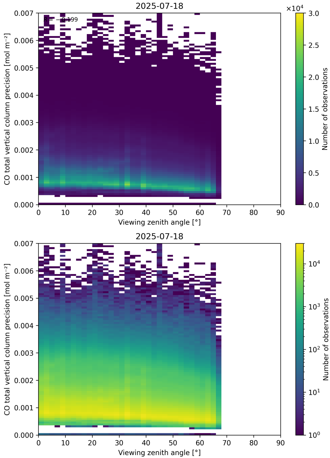
Figure 71: Scatter density plot of “Viewing zenith angle” against “CO total vertical column precision” for 2025-07-18 to 2025-07-19.
