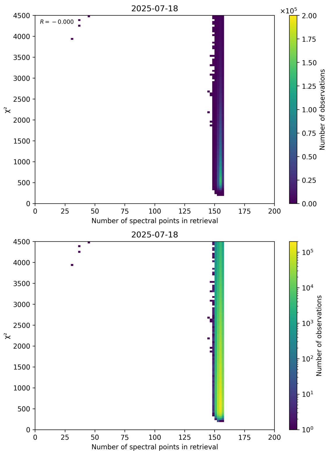
Figure 58: Scatter density plot of “Number of spectral points in retrieval” against “ \chi^2 ” for 2025-07-18 to 2025-07-19.
