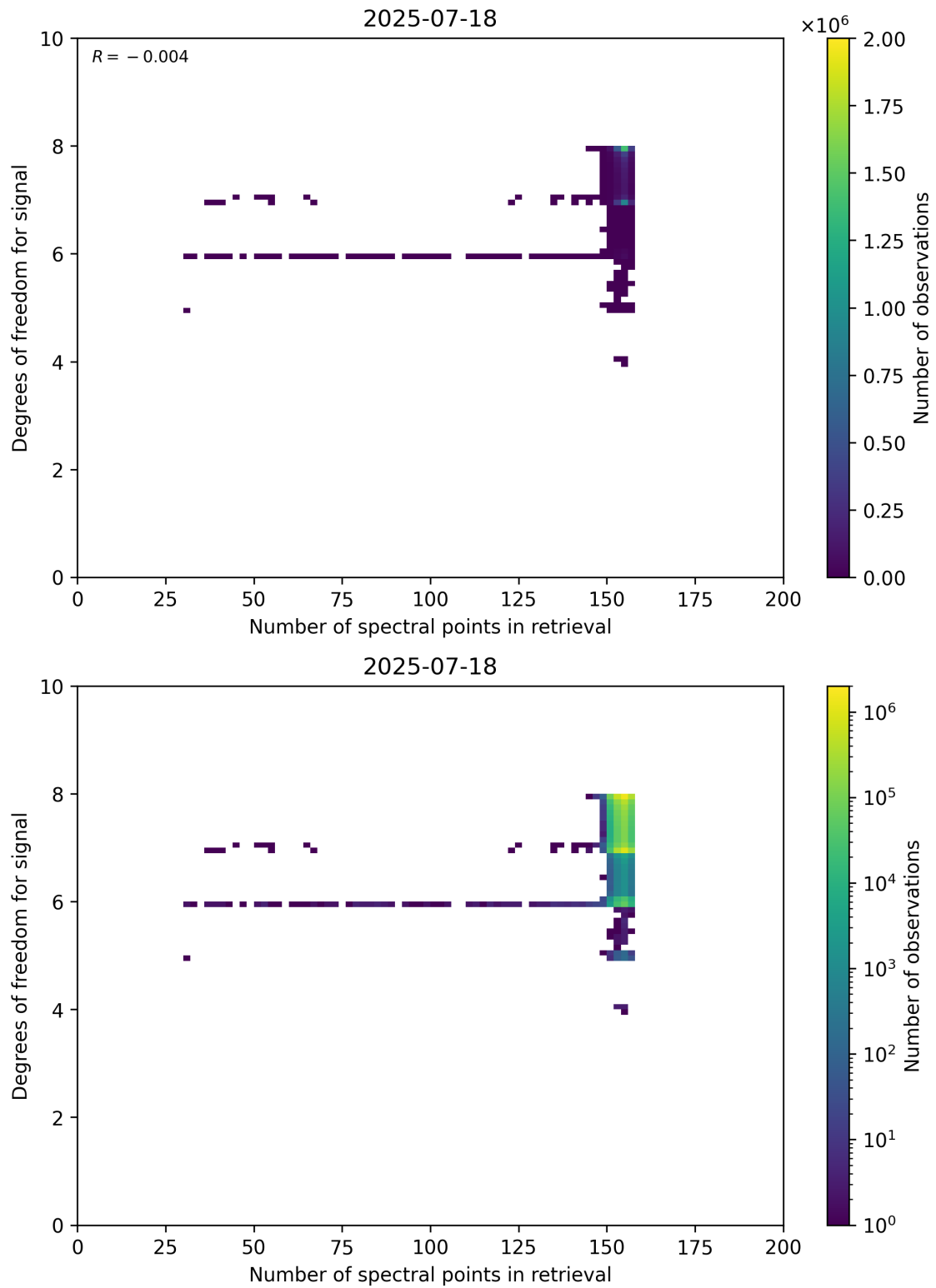
Figure 59: Scatter density plot of “Number of spectral points in retrieval” against “Degrees of freedom for signal” for 2025-07-18 to 2025-07-19.
