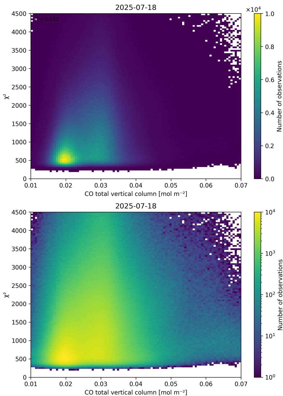
Figure 35: Scatter density plot of “CO total vertical column” against “ \chi^2 ” for 2025-07-18 to 2025-07-19.
