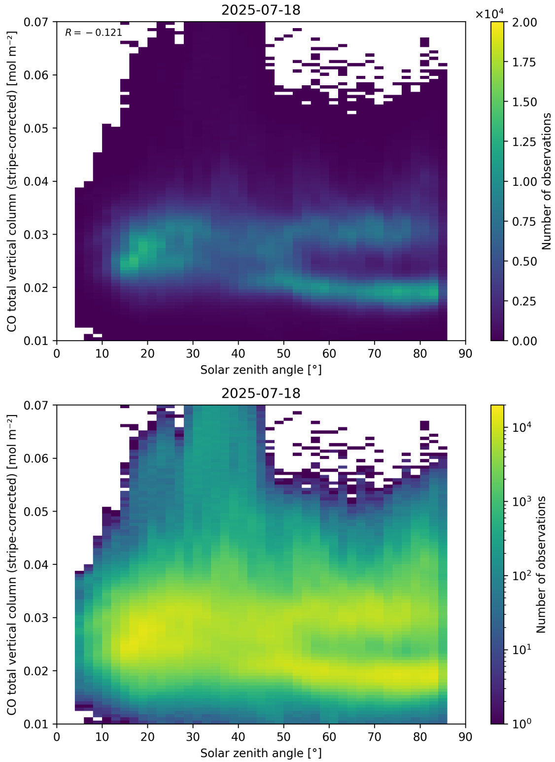
Figure 62: Scatter density plot of “Solar zenith angle” against “CO total vertical column (stripe-corrected)” for 2025-07-18 to 2025-07-19.
