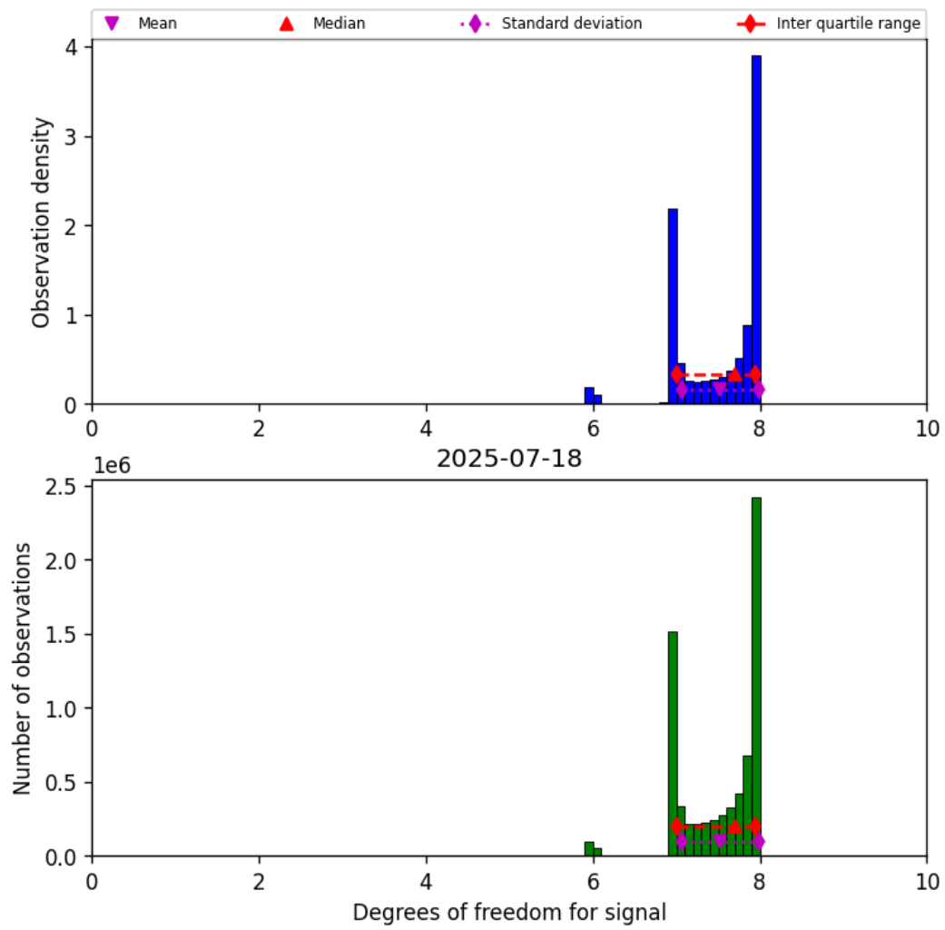
Figure 23: Histogram of “Degrees of freedom for signal” for 2025-07-18 to 2025-07-19
