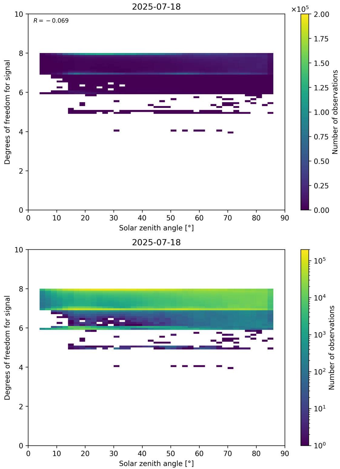
Figure 65: Scatter density plot of “Solar zenith angle” against “Degrees of freedom for signal” for 2025-07-18 to 2025-07-19.
