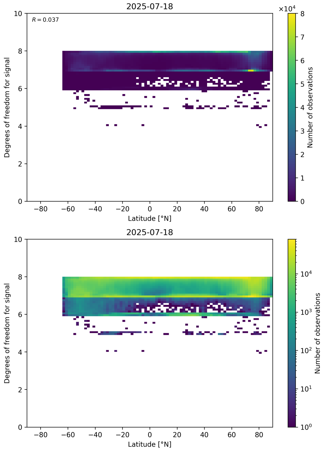
Figure 55: Scatter density plot of “Latitude” against “Degrees of freedom for signal” for 2025-07-18 to 2025-07-19.
