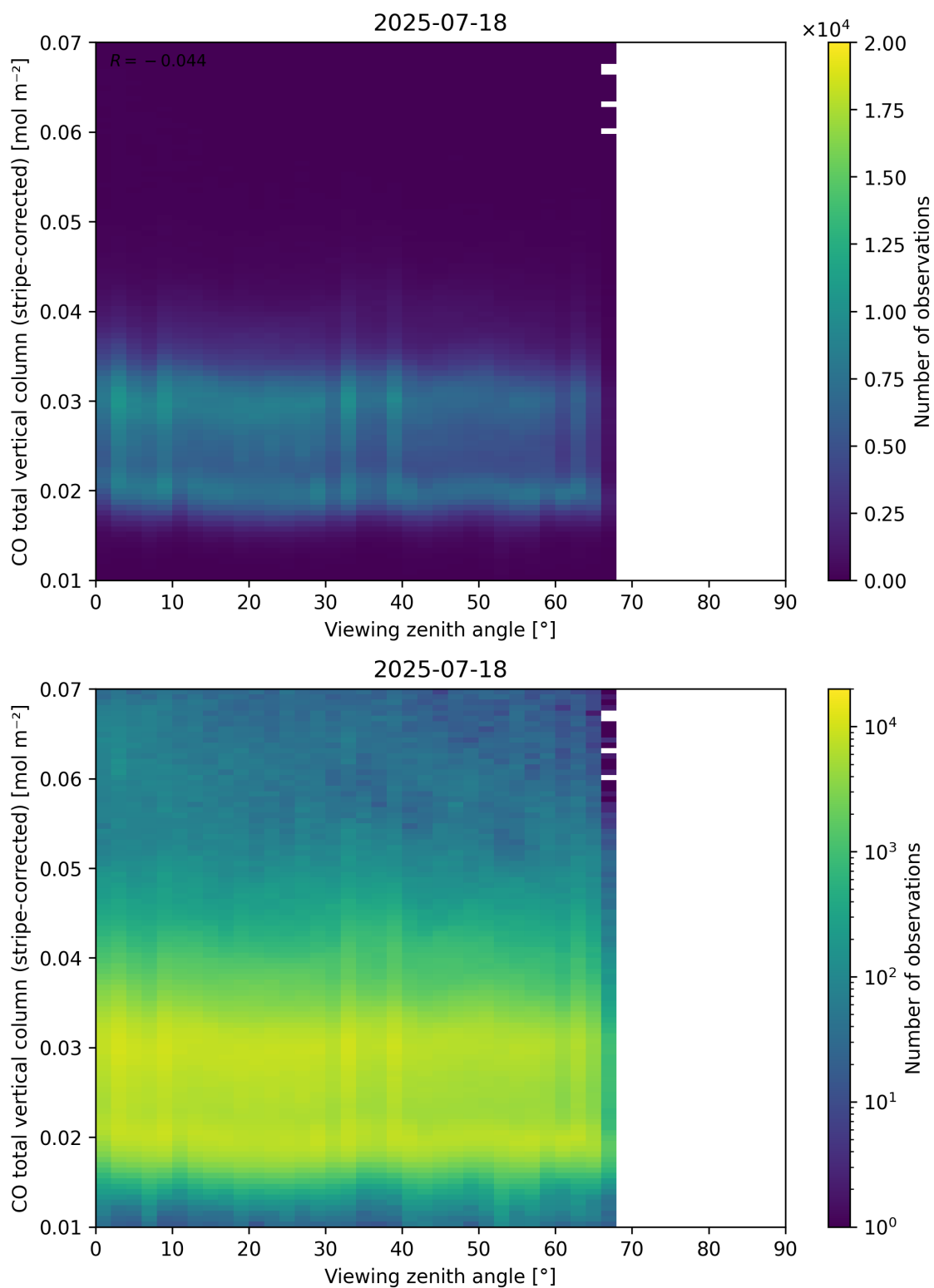
Figure 70: Scatter density plot of “Viewing zenith angle” against “CO total vertical column (stripe-corrected)” for 2025-07-18 to 2025-07-19.
