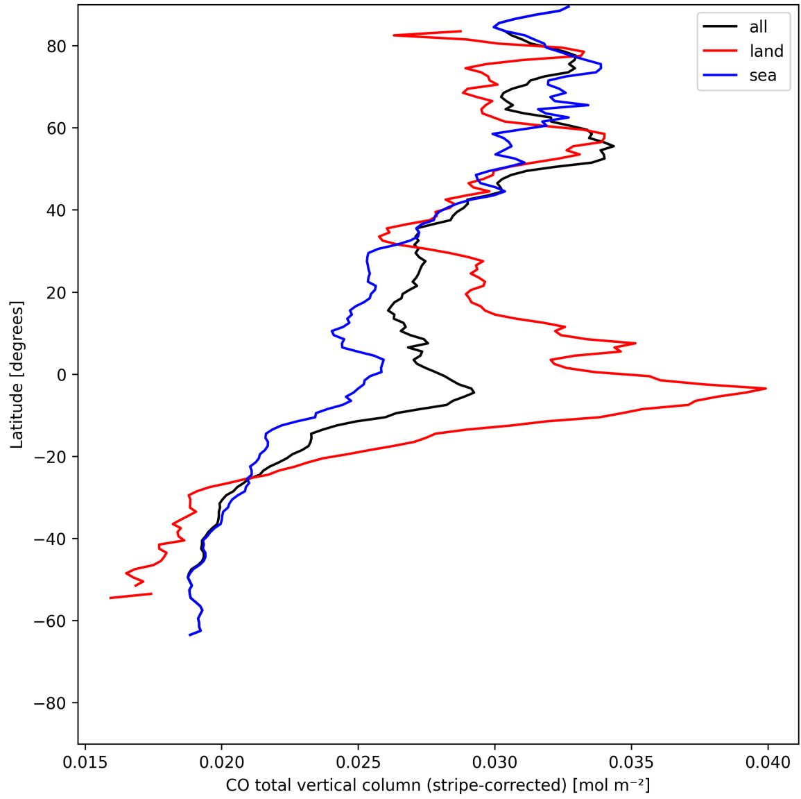
Figure 11: Zonal average of “CO total vertical column (stripe-corrected)” for 2025-07-18 to 2025-07-19.
