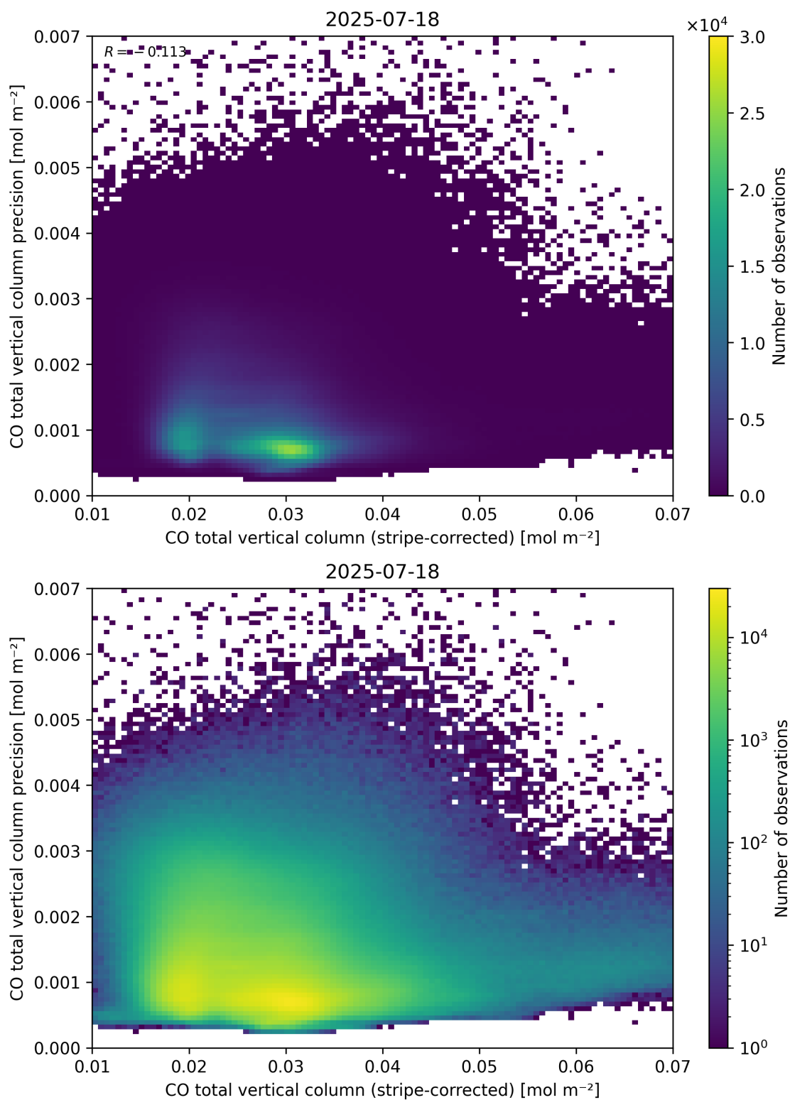
Figure 36: Scatter density plot of “CO total vertical column (stripe-corrected)” against “CO total vertical column precision” for 2025-07-18 to 2025-07-19.
