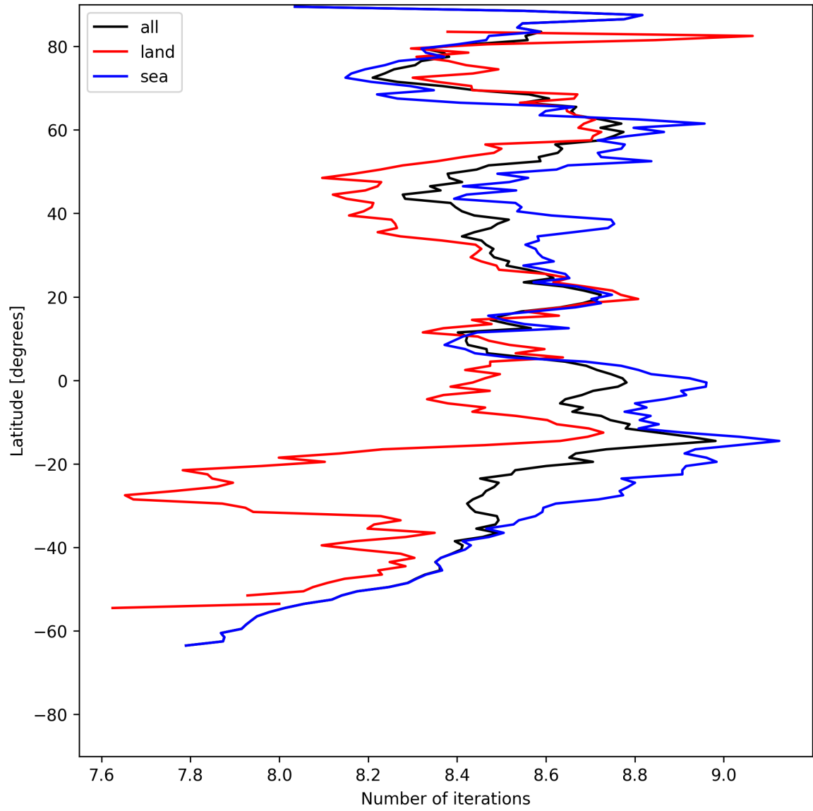
Figure 16: Zonal average of “Number of iterations” for 2025-07-18 to 2025-07-19.
