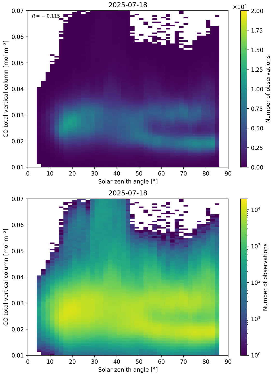
Figure 61: Scatter density plot of “Solar zenith angle” against “CO total vertical column” for 2025-07-18 to 2025-07-19.
