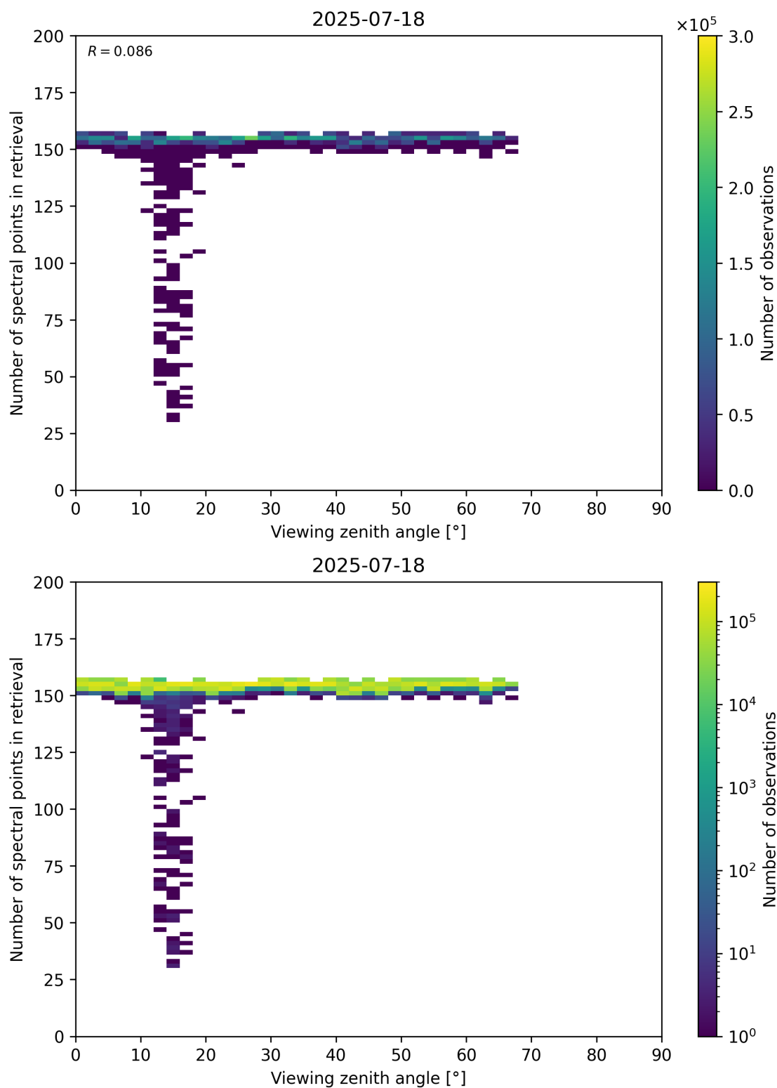
Figure 76: Scatter density plot of “Viewing zenith angle” against “Number of spectral points in retrieval” for 2025-07-18 to 2025-07-19.
