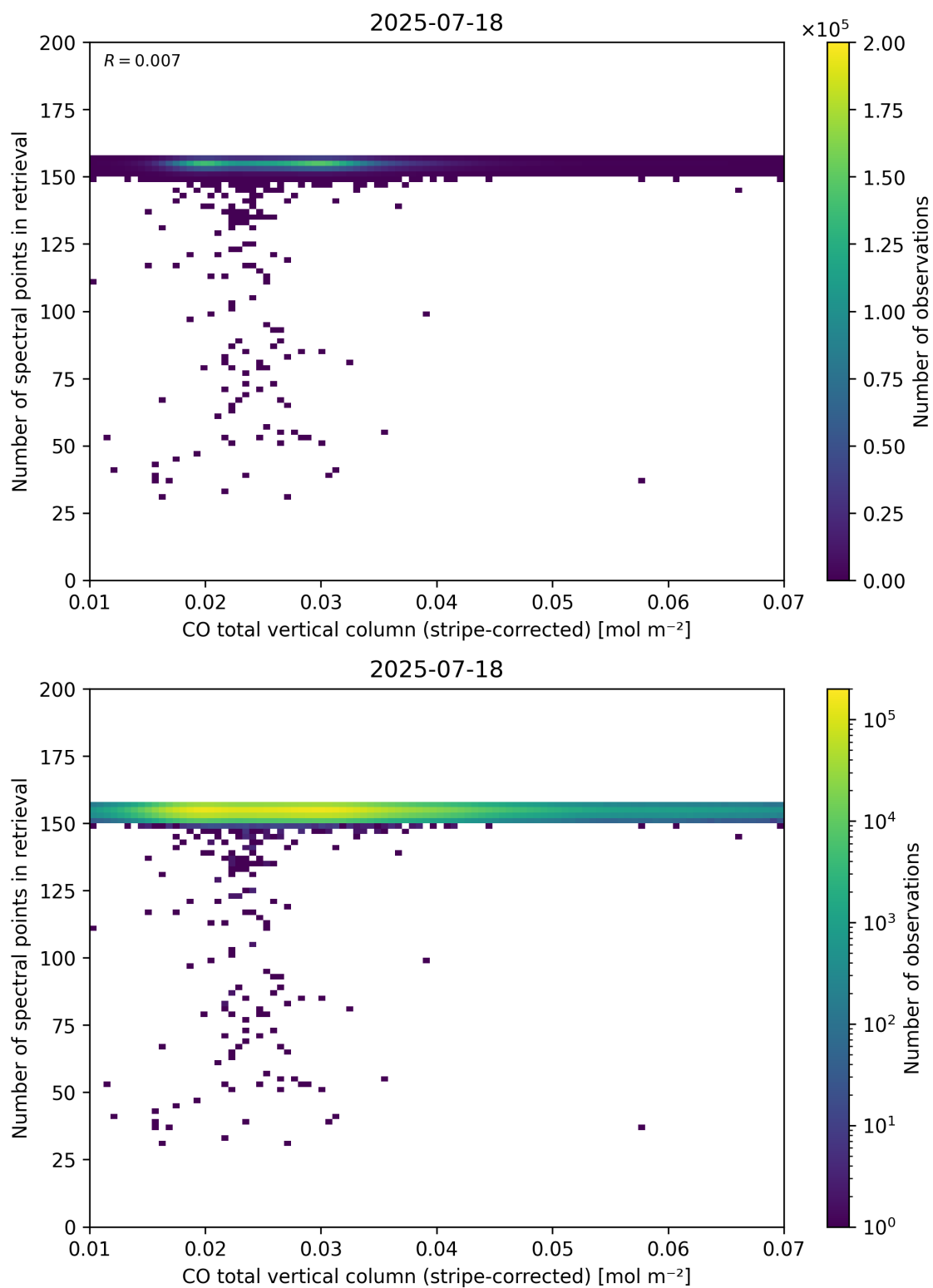
Figure 40: Scatter density plot of “CO total vertical column (stripe-corrected)” against “Number of spectral points in retrieval” for 2025-07-18 to 2025-07-19.
