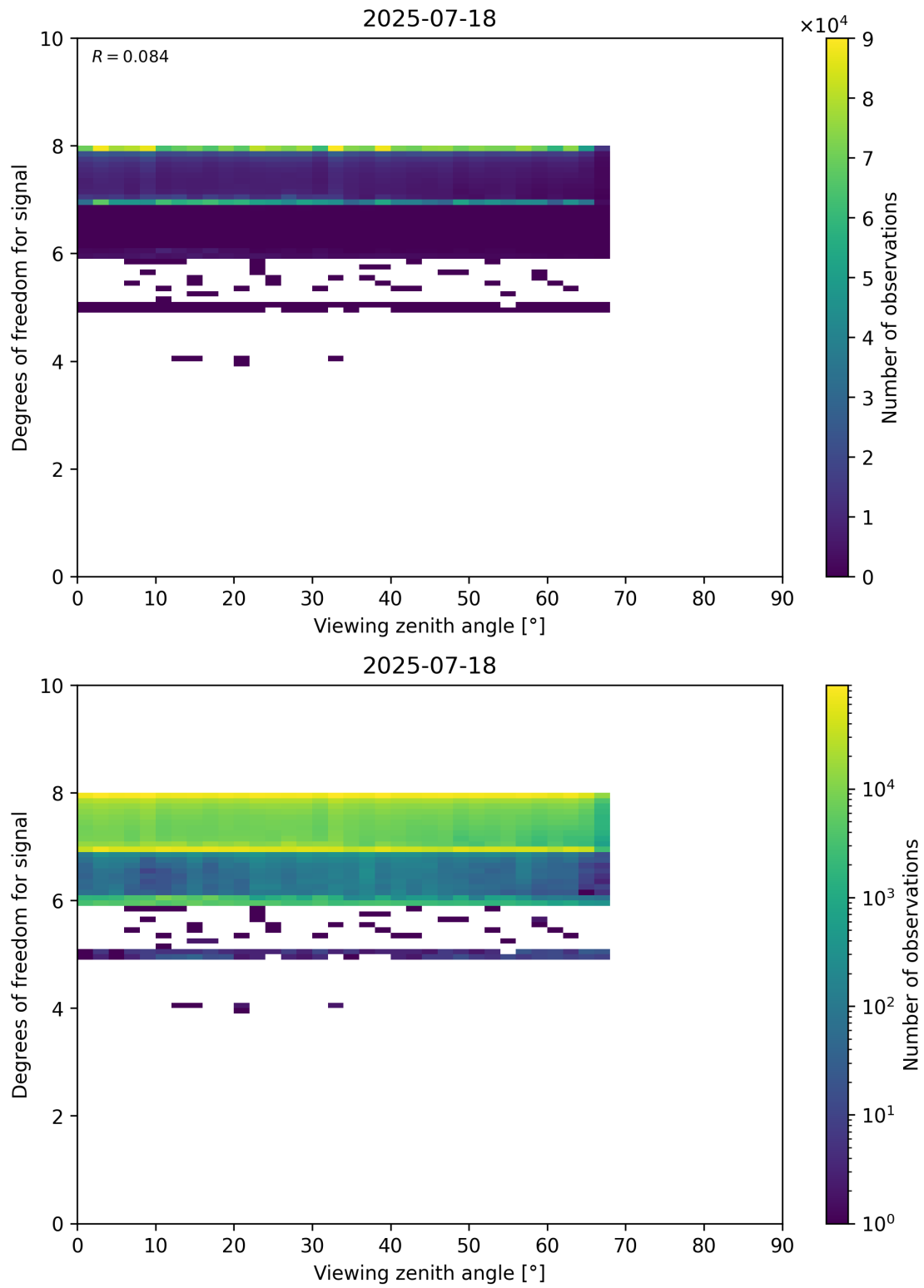
Figure 73: Scatter density plot of “Viewing zenith angle” against “Degrees of freedom for signal” for 2025-07-18 to 2025-07-19.
