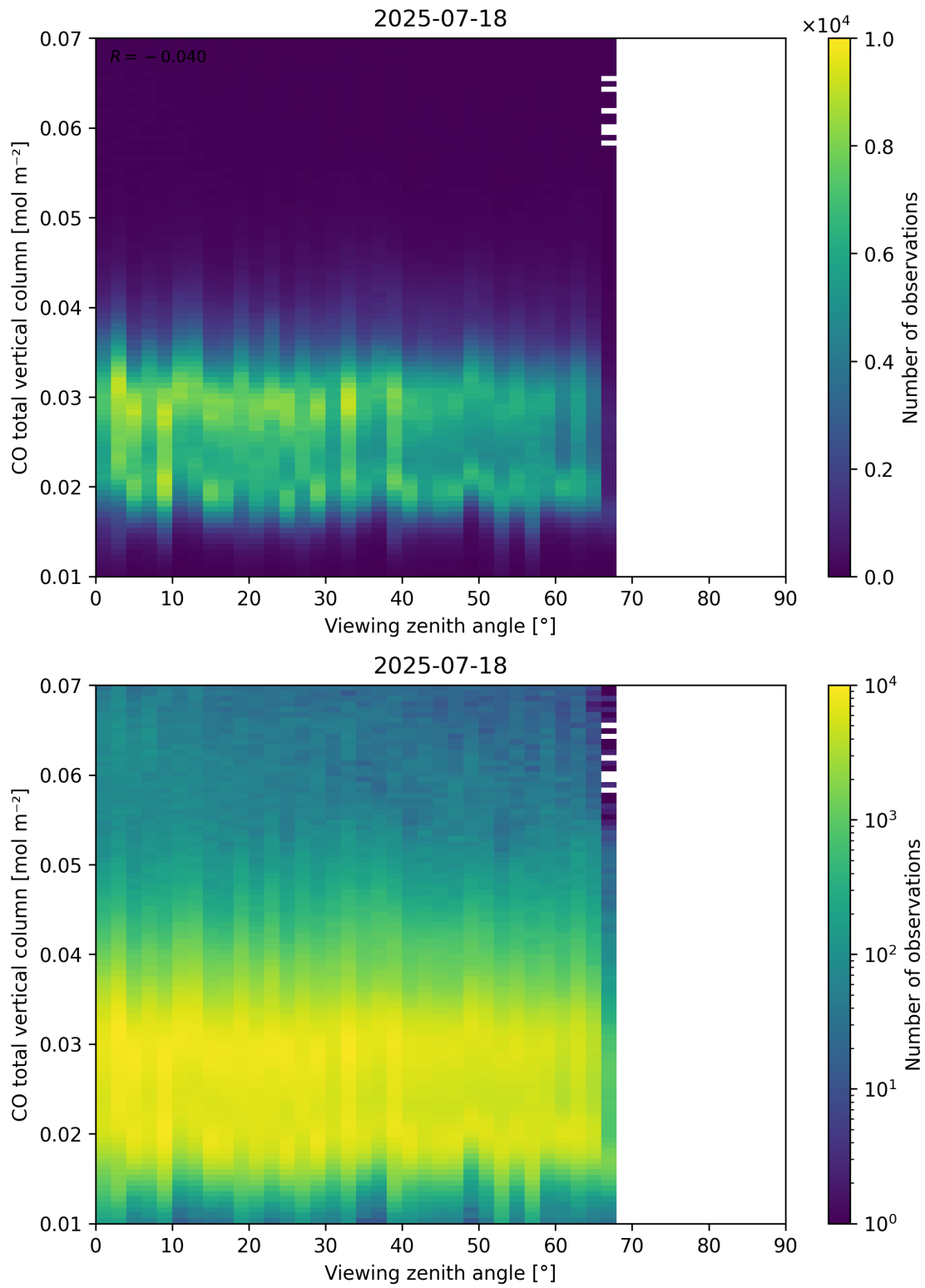
Figure 69: Scatter density plot of “Viewing zenith angle” against “CO total vertical column” for 2025-07-18 to 2025-07-19.
