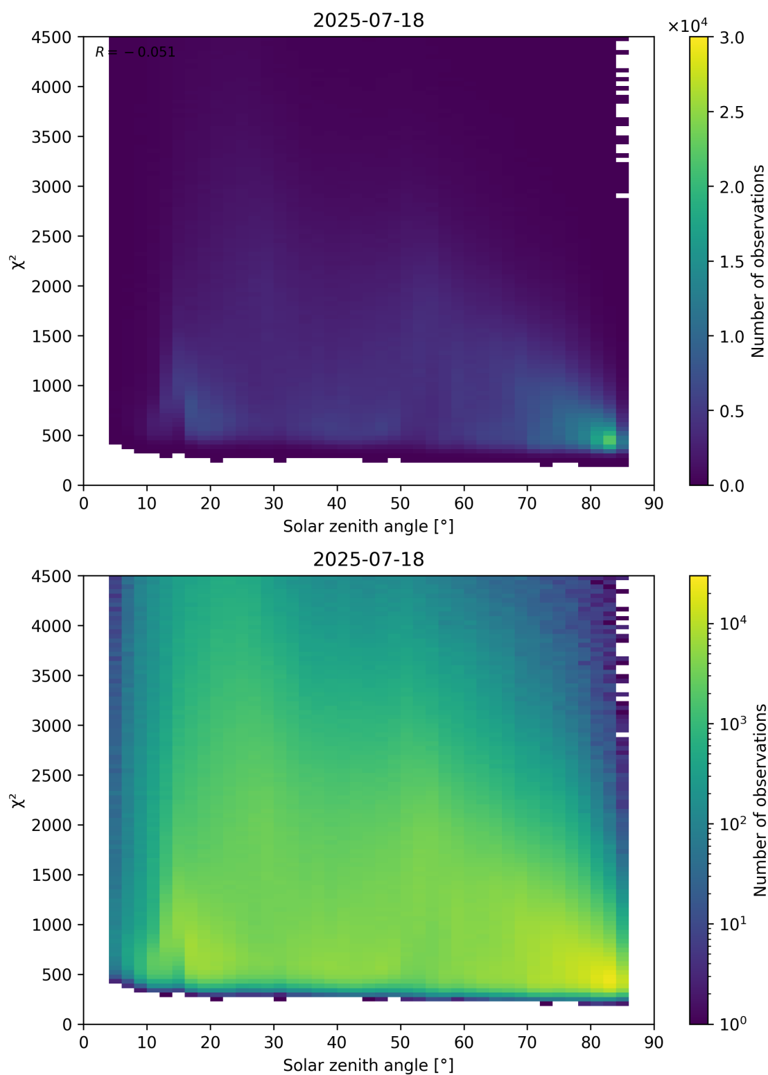
Figure 64: Scatter density plot of “Solar zenith angle” against “ \chi^2 ” for 2025-07-18 to 2025-07-19.
