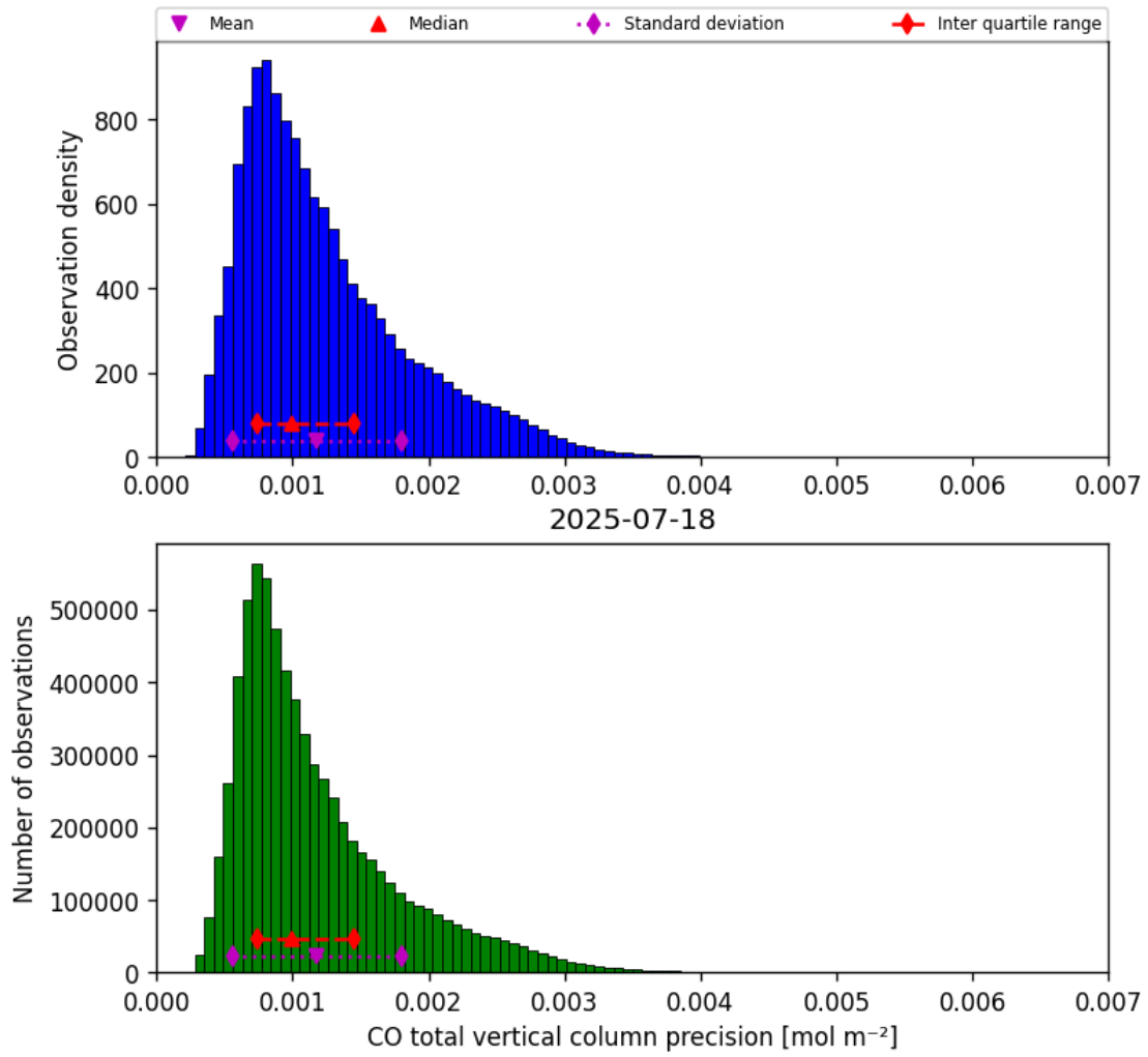
Figure 20: Histogram of “CO total vertical column precision” for 2025-07-18 to 2025-07-19
