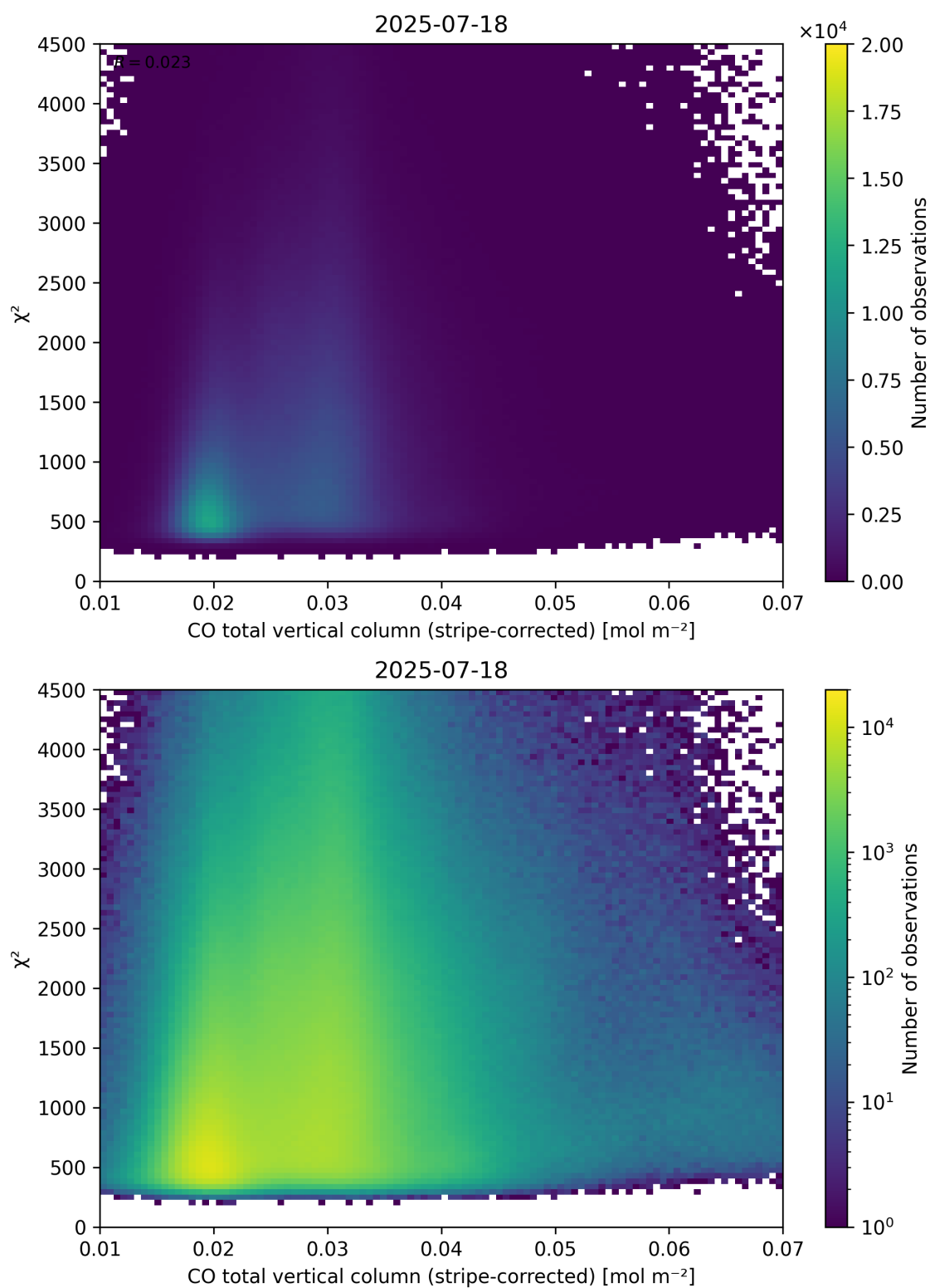
Figure 37: Scatter density plot of “CO total vertical column (stripe-corrected)” against “ \chi^2 ” for 2025-07-18 to 2025-07-19.
