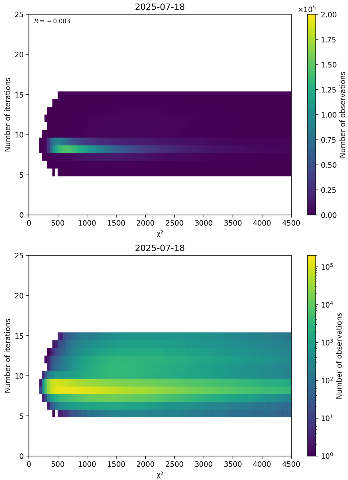
Figure 49: Scatter density plot of “ \chi^2 ” against “Number of iterations” for 2025-07-18 to 2025-07-19.
