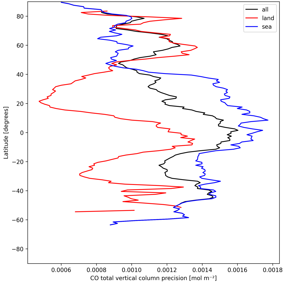
Figure 12: Zonal average of “CO total vertical column precision” for 2025-07-18 to 2025-07-19.
