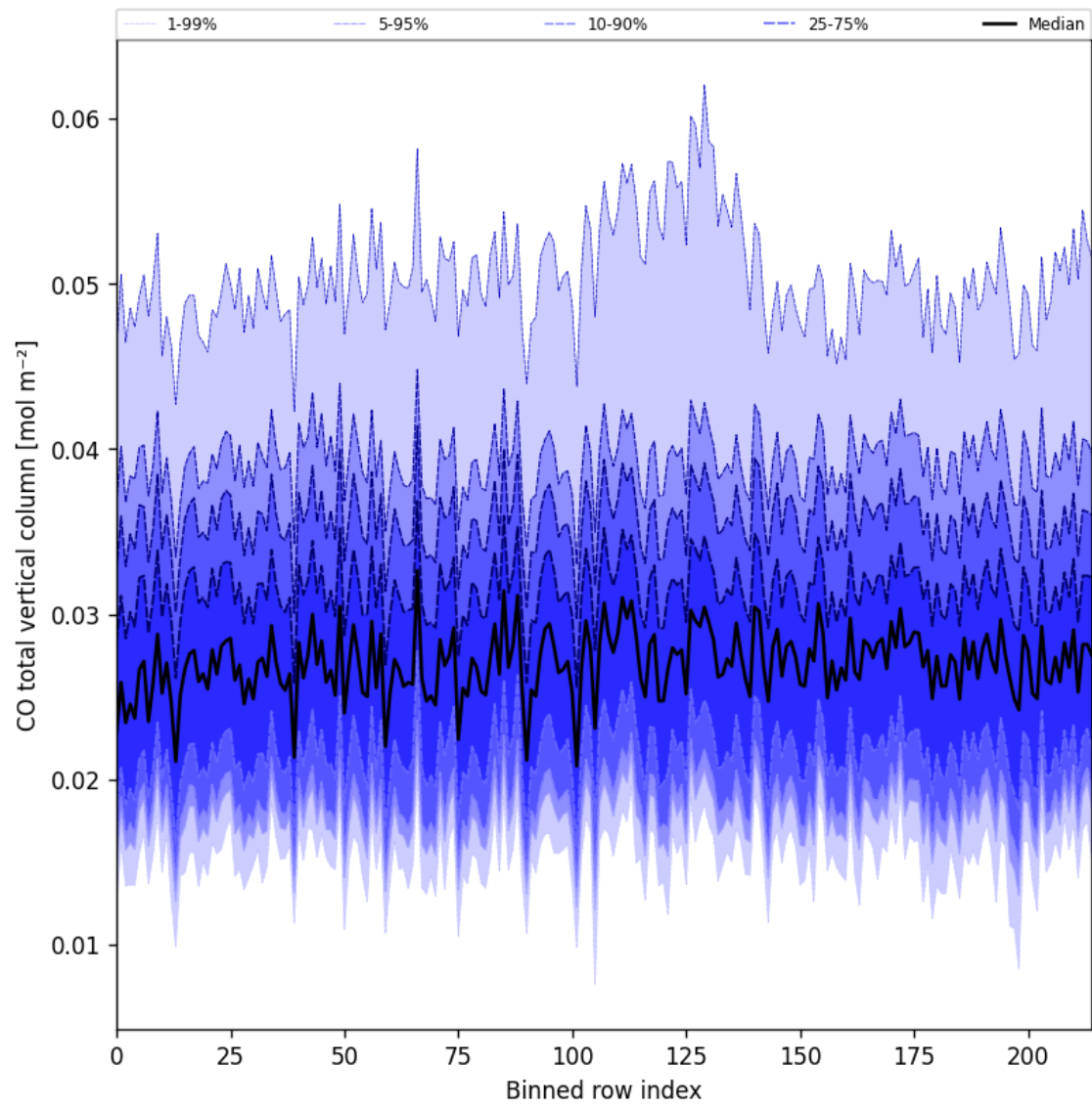
Figure 26: Along track statistics of “CO total vertical column” for 2025-07-18 to 2025-07-19
