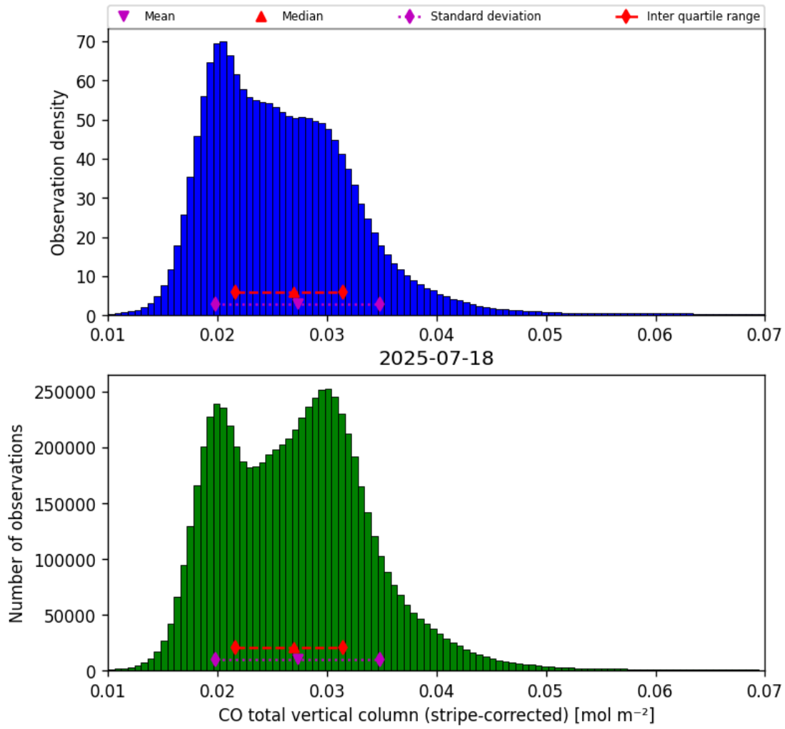
Figure 19: Histogram of “CO total vertical column (stripe-corrected)” for 2025-07-18 to 2025-07-19
