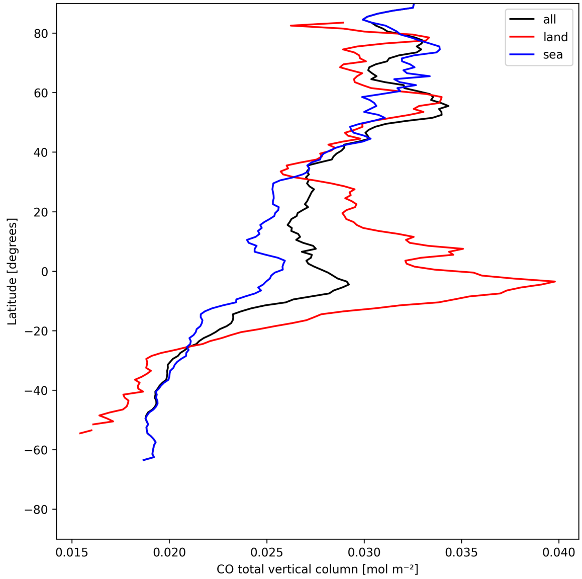
Figure 10: Zonal average of “CO total vertical column” for 2025-07-18 to 2025-07-19.
