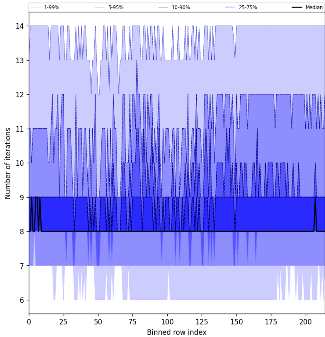
Figure 32: Along track statistics of “Number of iterations” for 2025-07-18 to 2025-07-19
