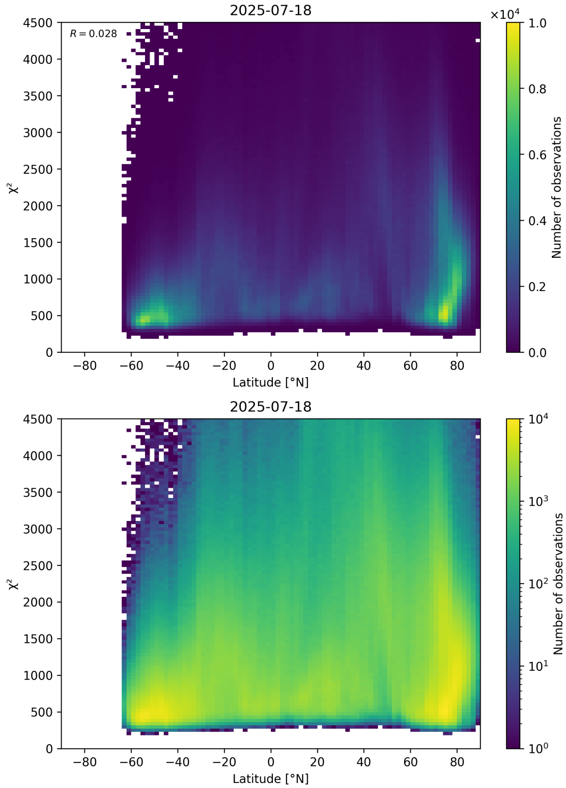
Figure 54: Scatter density plot of “Latitude” against “ \chi^2 ” for 2025-07-18 to 2025-07-19.
