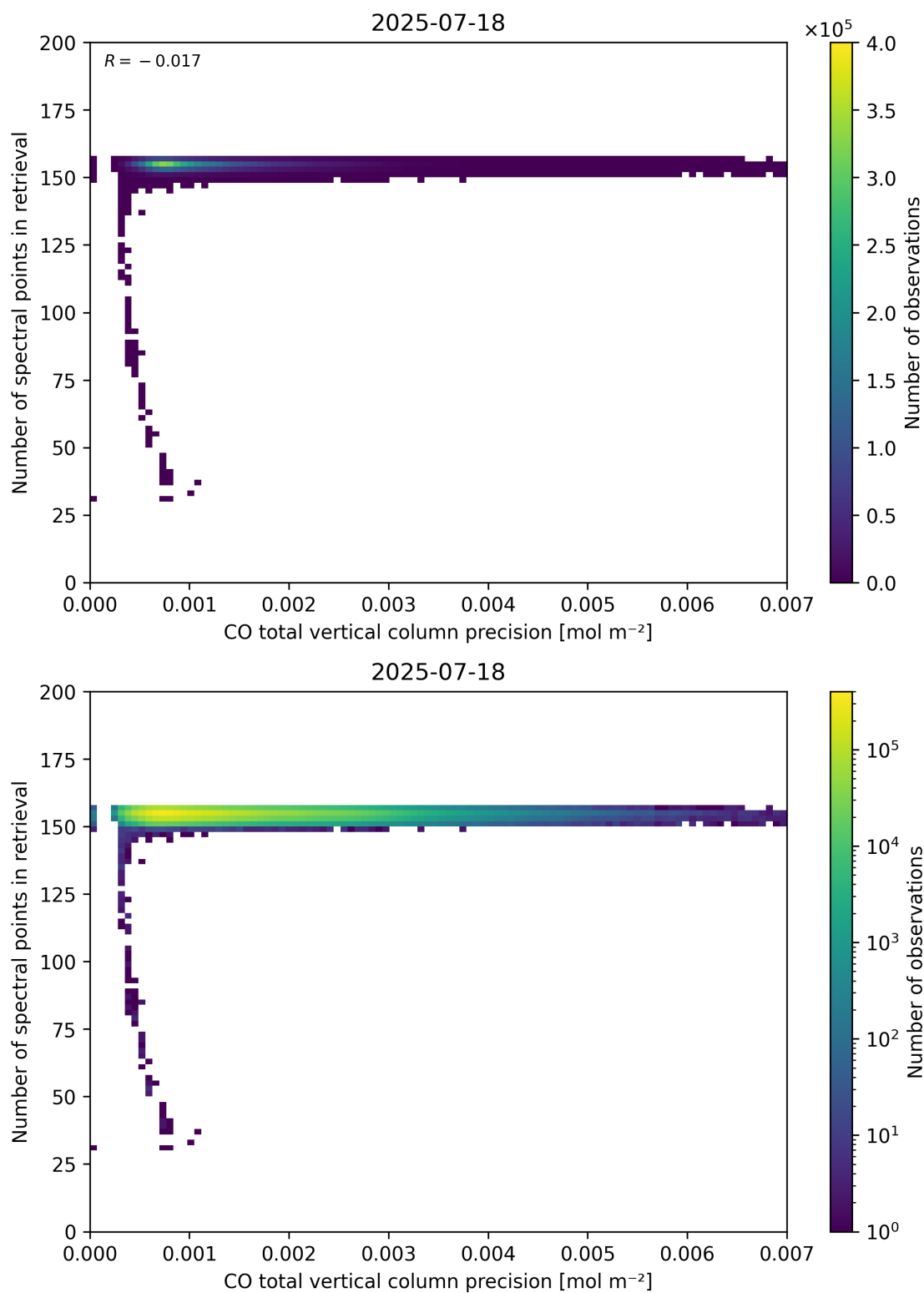
Figure 47: Scatter density plot of “CO total vertical column precision” against “Number of spectral points in retrieval” for 2025-07-18 to 2025-07-19.
