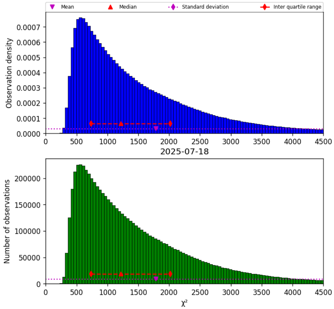
Figure 22: Histogram of “ \chi^2 ” for 2025-07-18 to 2025-07-19
