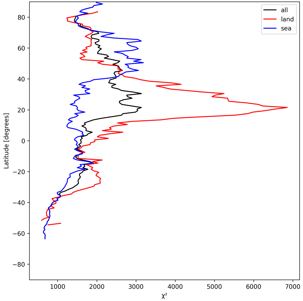
Figure 14: Zonal average of “ \chi^2 ” for 2025-07-18 to 2025-07-19.
