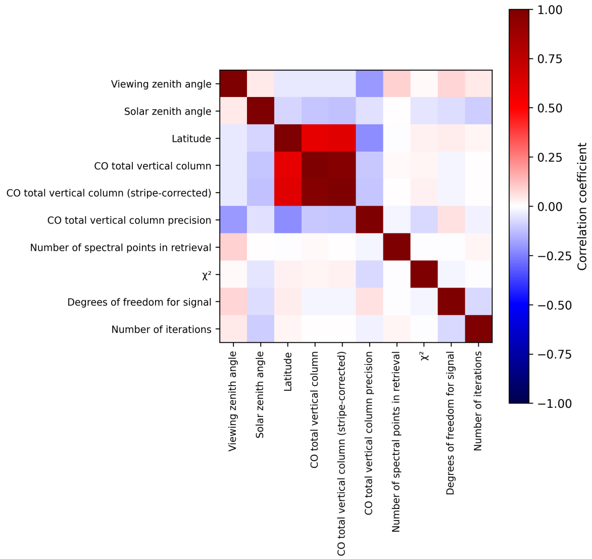
Figure 2: Map of correlation matrix for 2025-07-18 to 2025-07-19.
