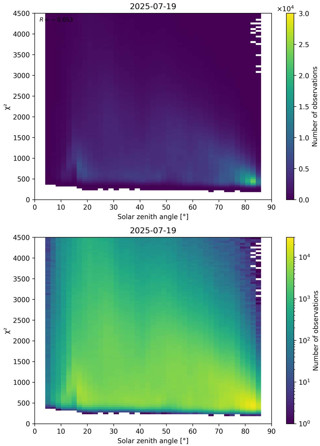
Figure 64: Scatter density plot of “Solar zenith angle” against “ \chi^2 ” for 2025-07-19 to 2025-07-20.
