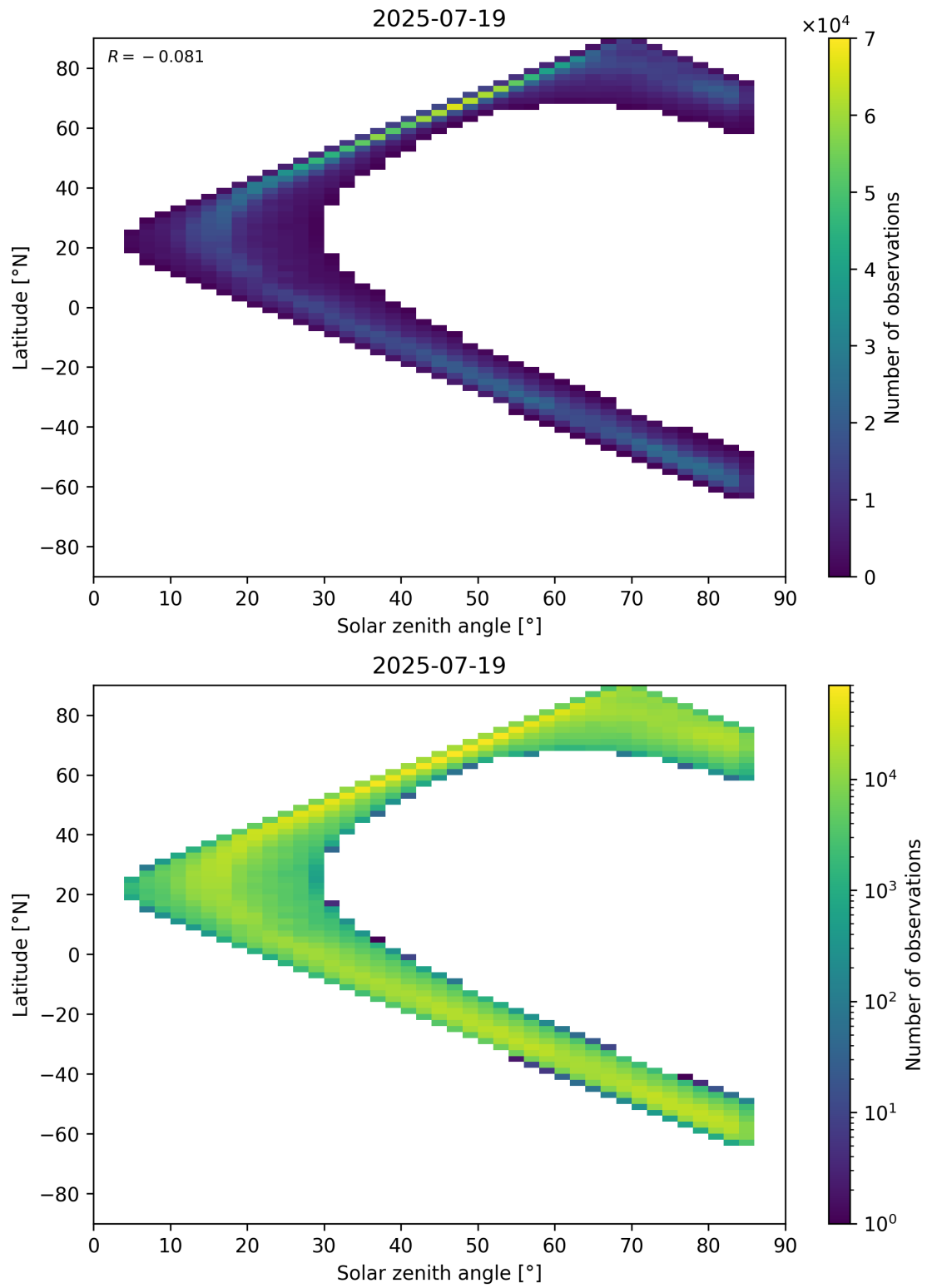
Figure 66: Scatter density plot of “Solar zenith angle” against “Latitude” for 2025-07-19 to 2025-07-20.
