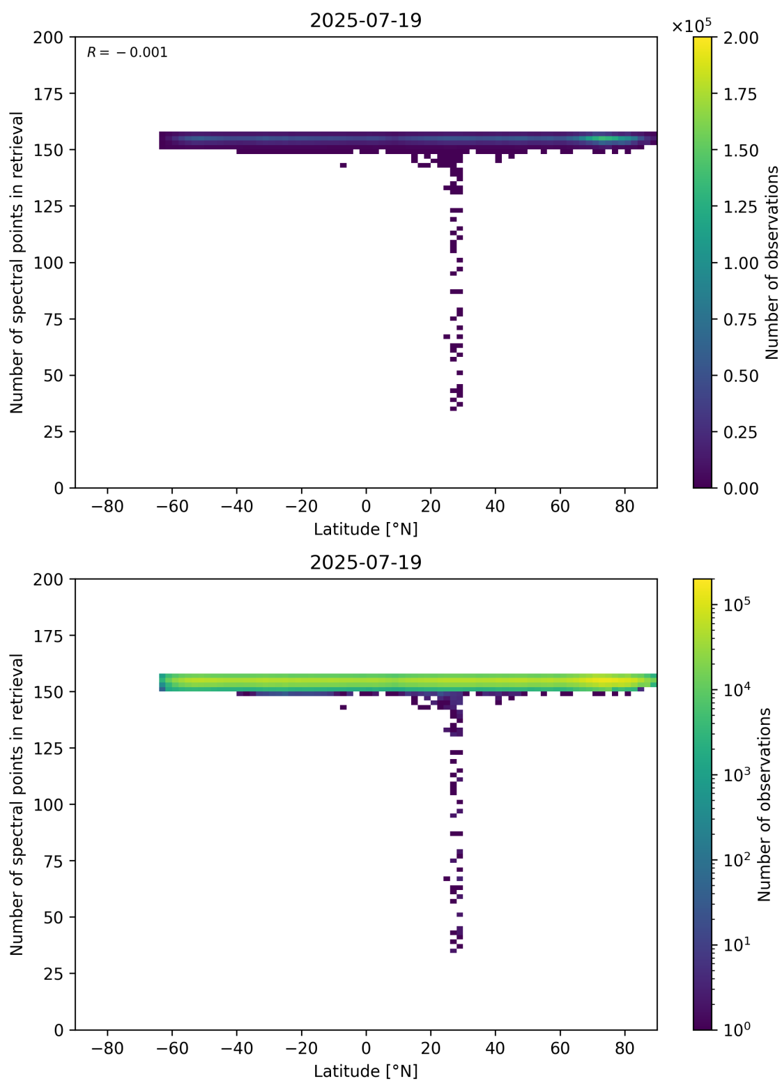
Figure 57: Scatter density plot of “Latitude” against “Number of spectral points in retrieval” for 2025-07-19 to 2025-07-20.
