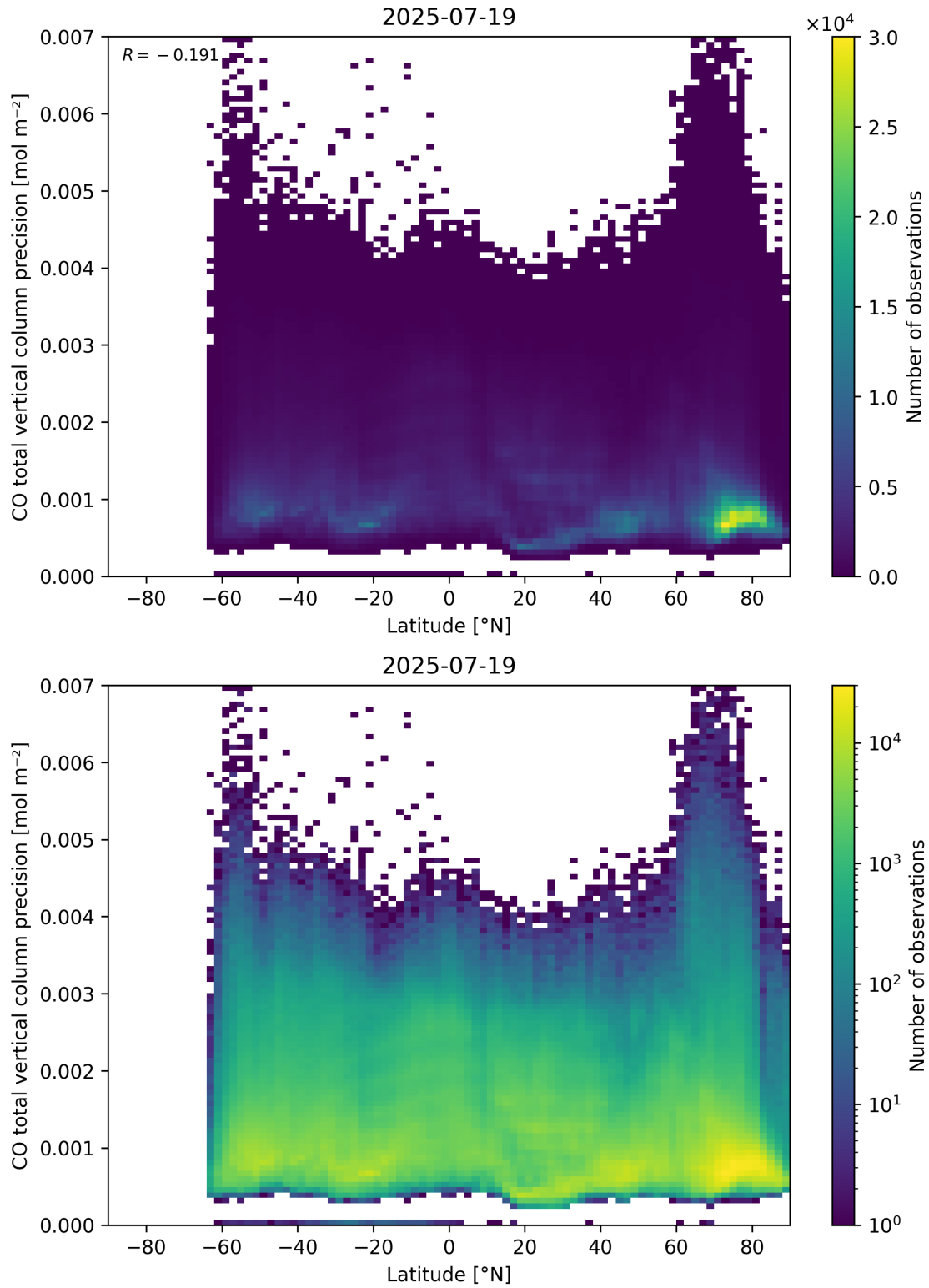
Figure 53: Scatter density plot of “Latitude” against “CO total vertical column precision” for 2025-07-19 to 2025-07-20.
