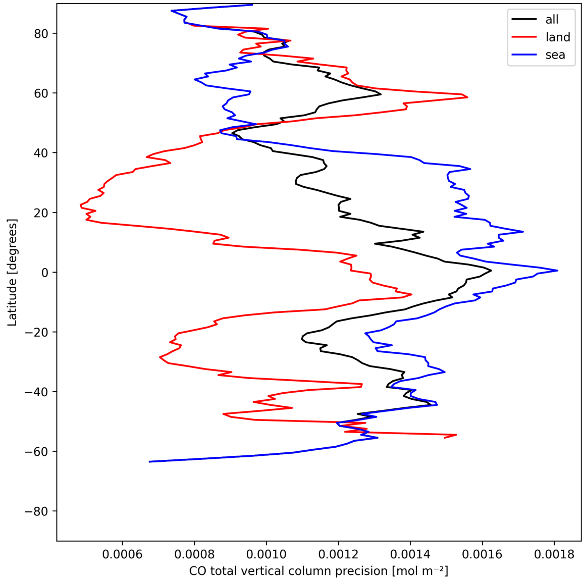
Figure 12: Zonal average of “CO total vertical column precision” for 2025-07-19 to 2025-07-20.
