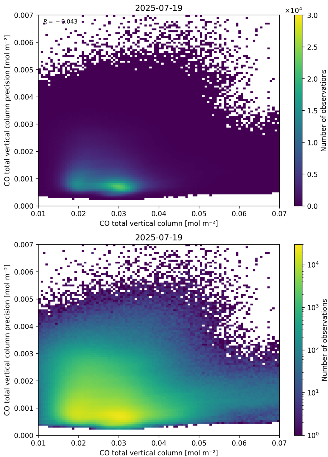
Figure 34: Scatter density plot of “CO total vertical column” against “CO total vertical column precision” for 2025-07-19 to 2025-07-20.
