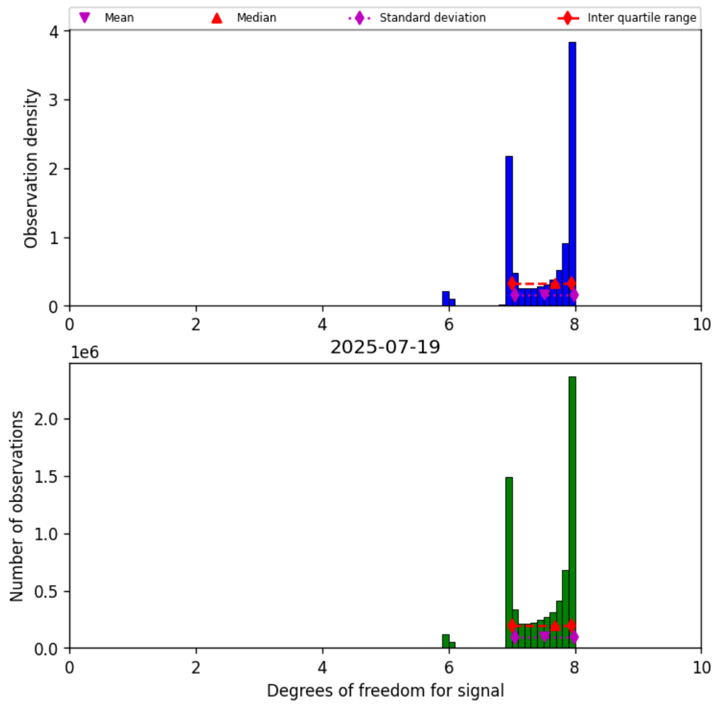
Figure 23: Histogram of “Degrees of freedom for signal” for 2025-07-19 to 2025-07-20
