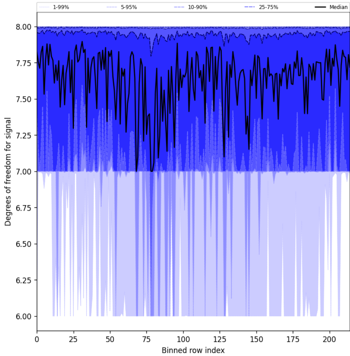
Figure 31: Along track statistics of “Degrees of freedom for signal” for 2025-07-19 to 2025-07-20
