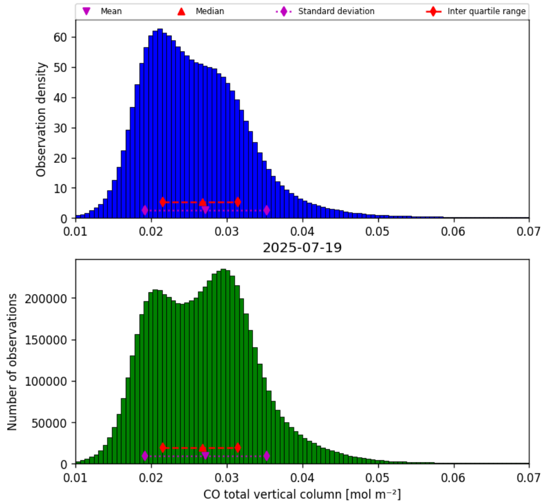
Figure 18: Histogram of “CO total vertical column” for 2025-07-19 to 2025-07-20
