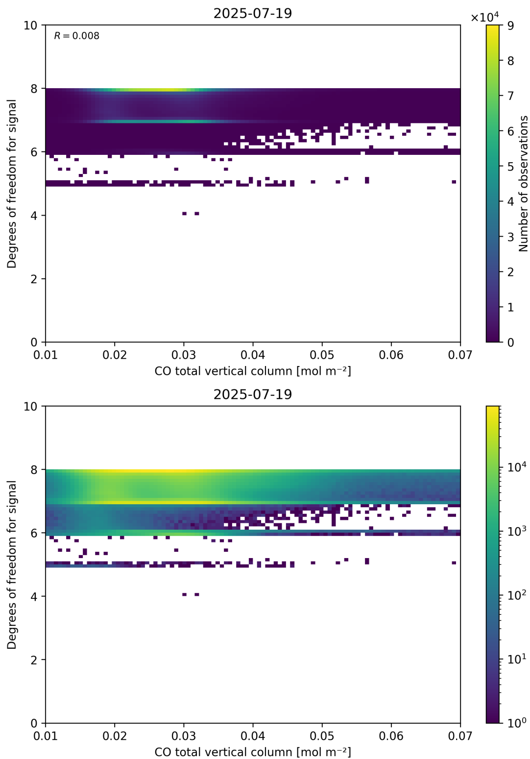
Figure 41: Scatter density plot of “CO total vertical column” against “Degrees of freedom for signal” for 2025-07-19 to 2025-07-20.
