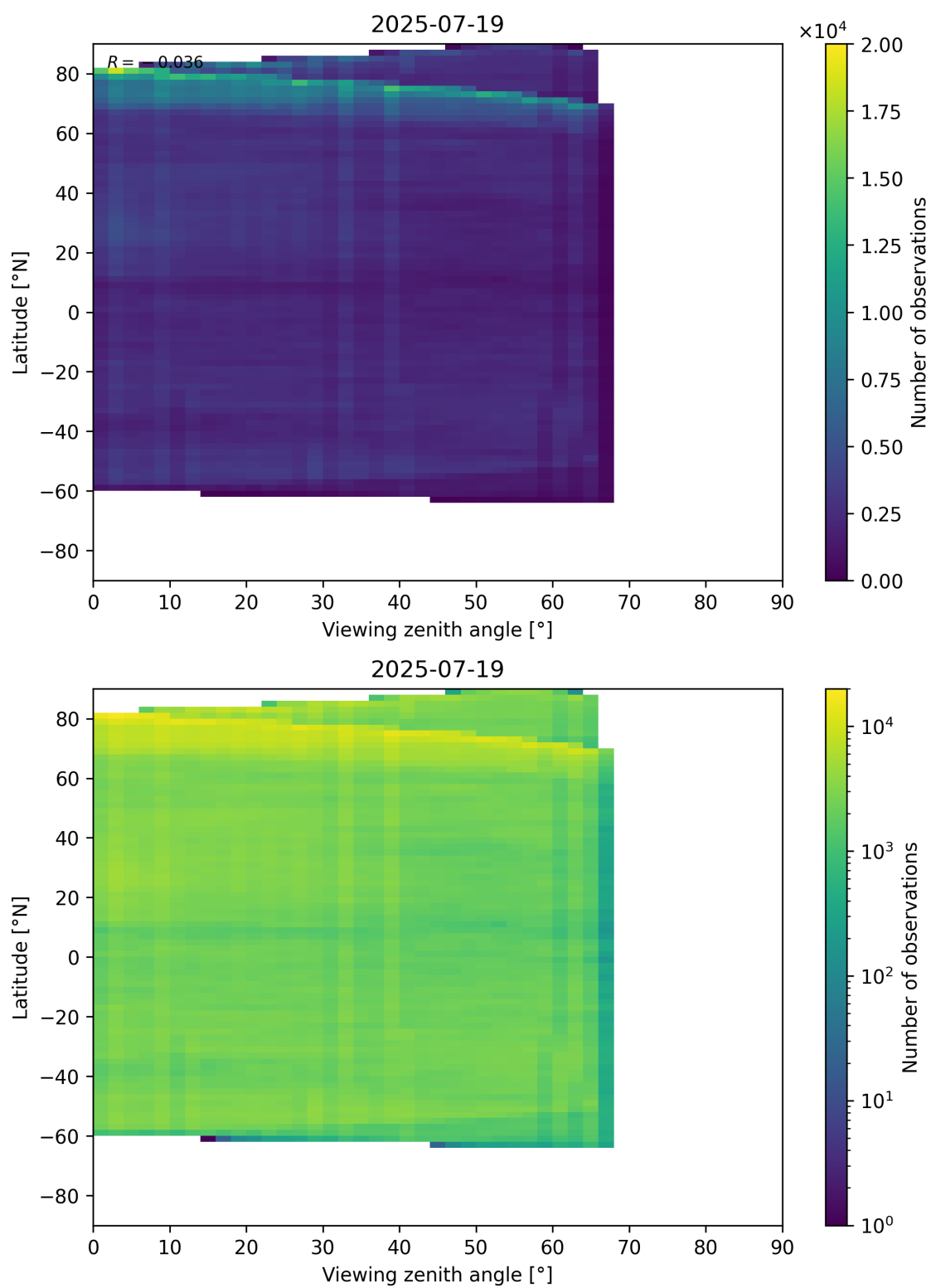
Figure 74: Scatter density plot of “Viewing zenith angle” against “Latitude” for 2025-07-19 to 2025-07-20.
