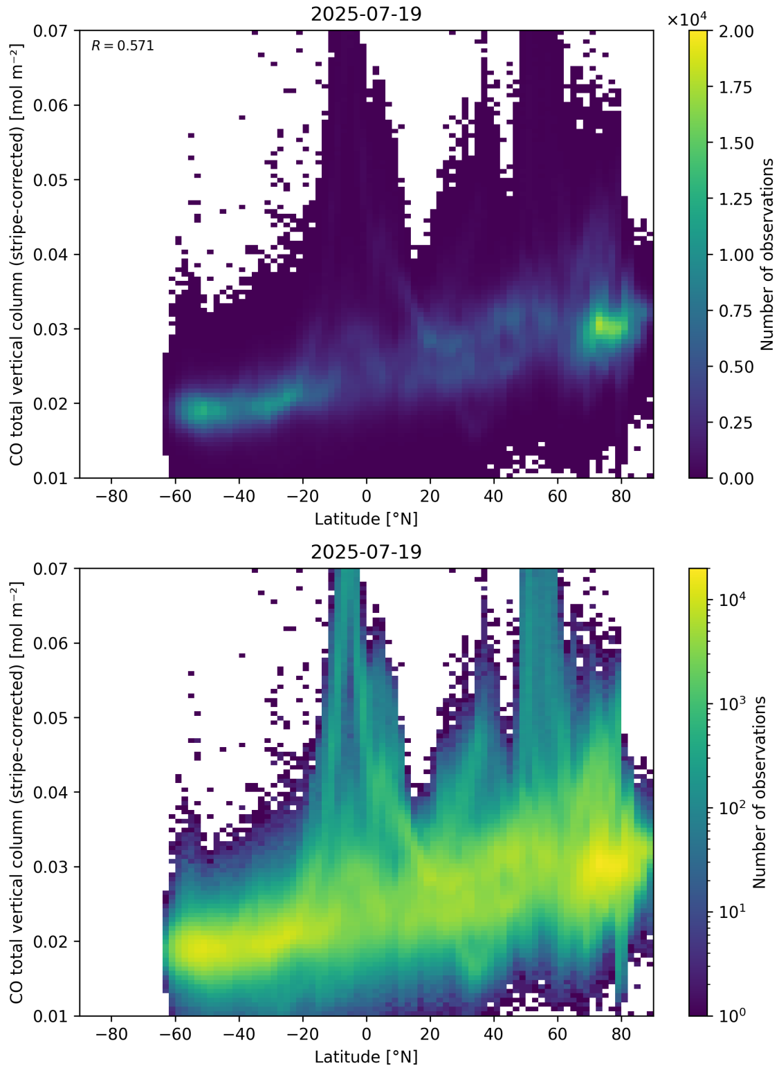
Figure 52: Scatter density plot of “Latitude” against “CO total vertical column (stripe-corrected)” for 2025-07-19 to 2025-07-20.
