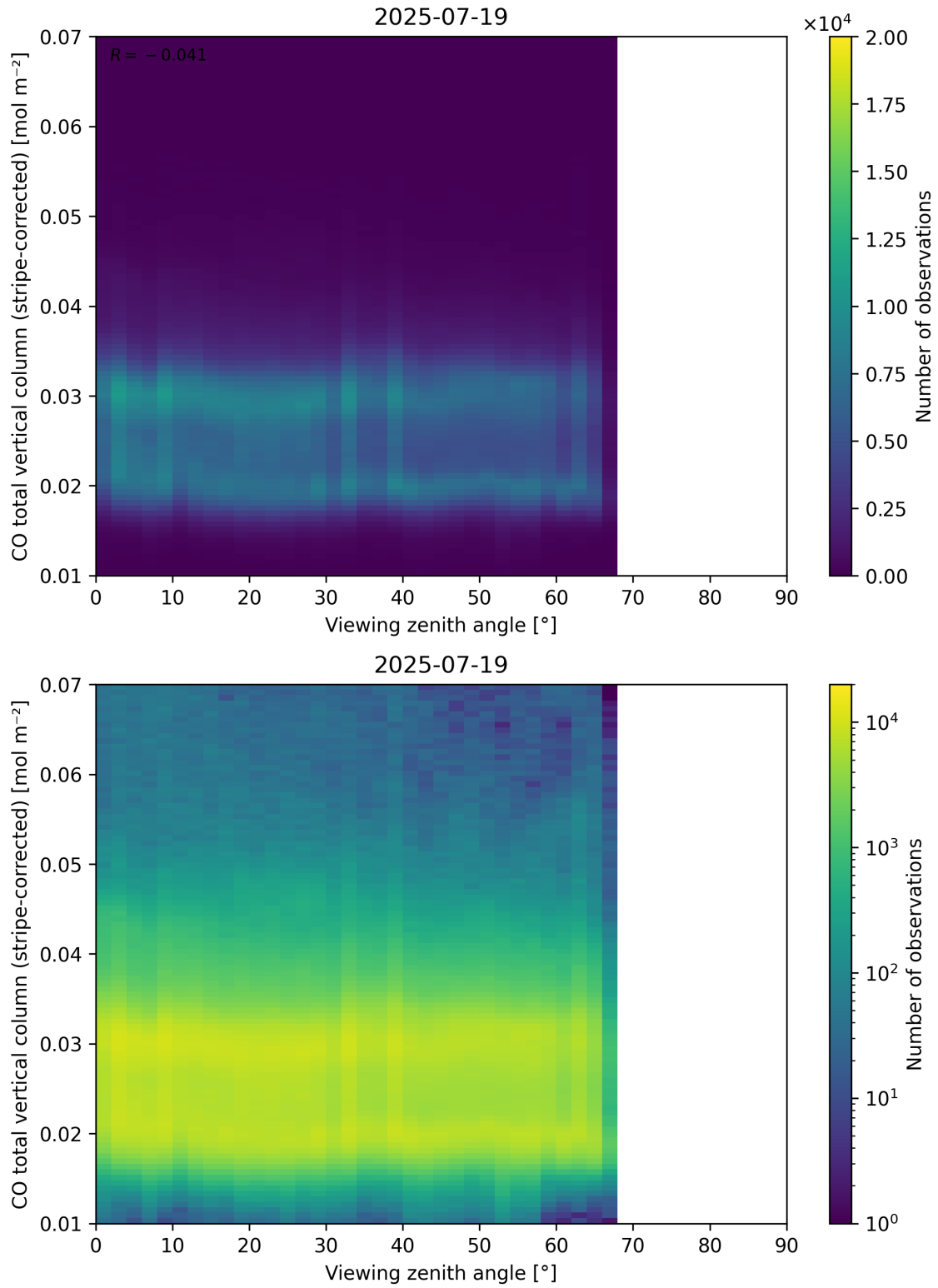
Figure 70: Scatter density plot of “Viewing zenith angle” against “CO total vertical column (stripe-corrected)” for 2025-07-19 to 2025-07-20.
