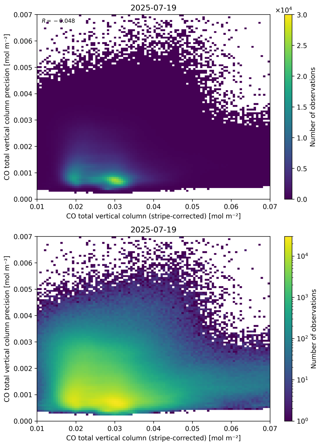
Figure 36: Scatter density plot of “CO total vertical column (stripe-corrected)” against “CO total vertical column precision” for 2025-07-19 to 2025-07-20.
