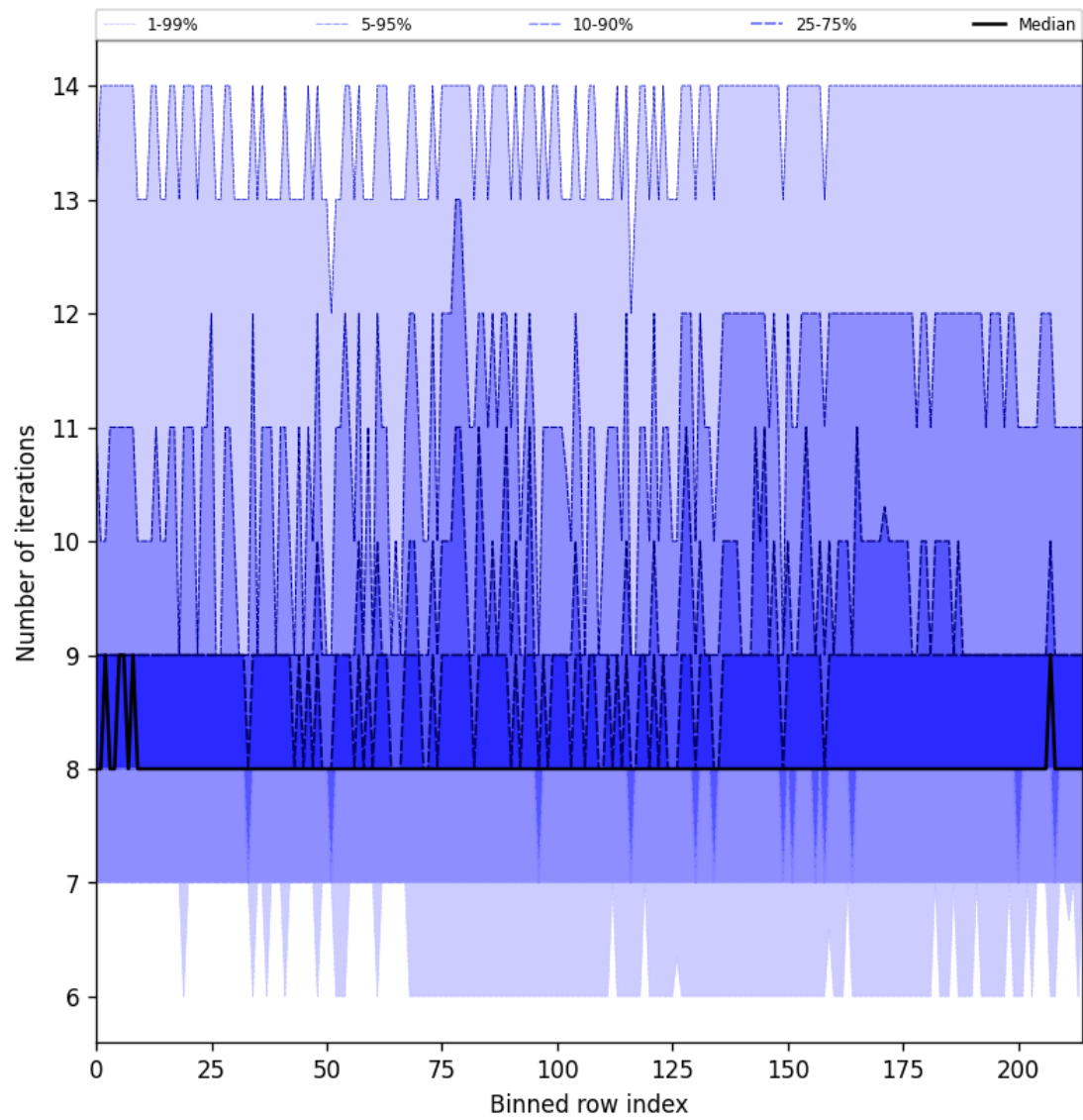
Figure 32: Along track statistics of “Number of iterations” for 2025-07-19 to 2025-07-20
