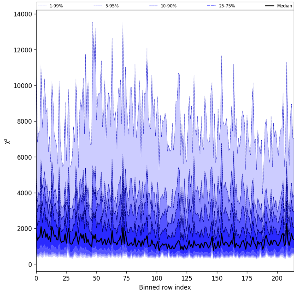
Figure 30: Along track statistics of “ \chi^2 ” for 2025-07-19 to 2025-07-20
