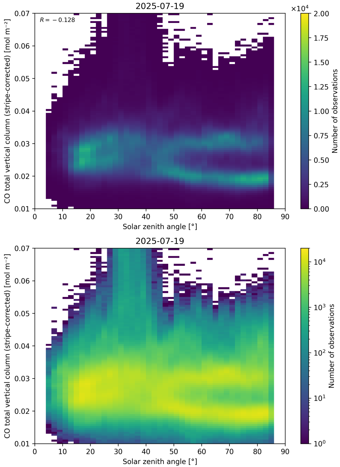
Figure 62: Scatter density plot of “Solar zenith angle” against “CO total vertical column (stripe-corrected)” for 2025-07-19 to 2025-07-20.
