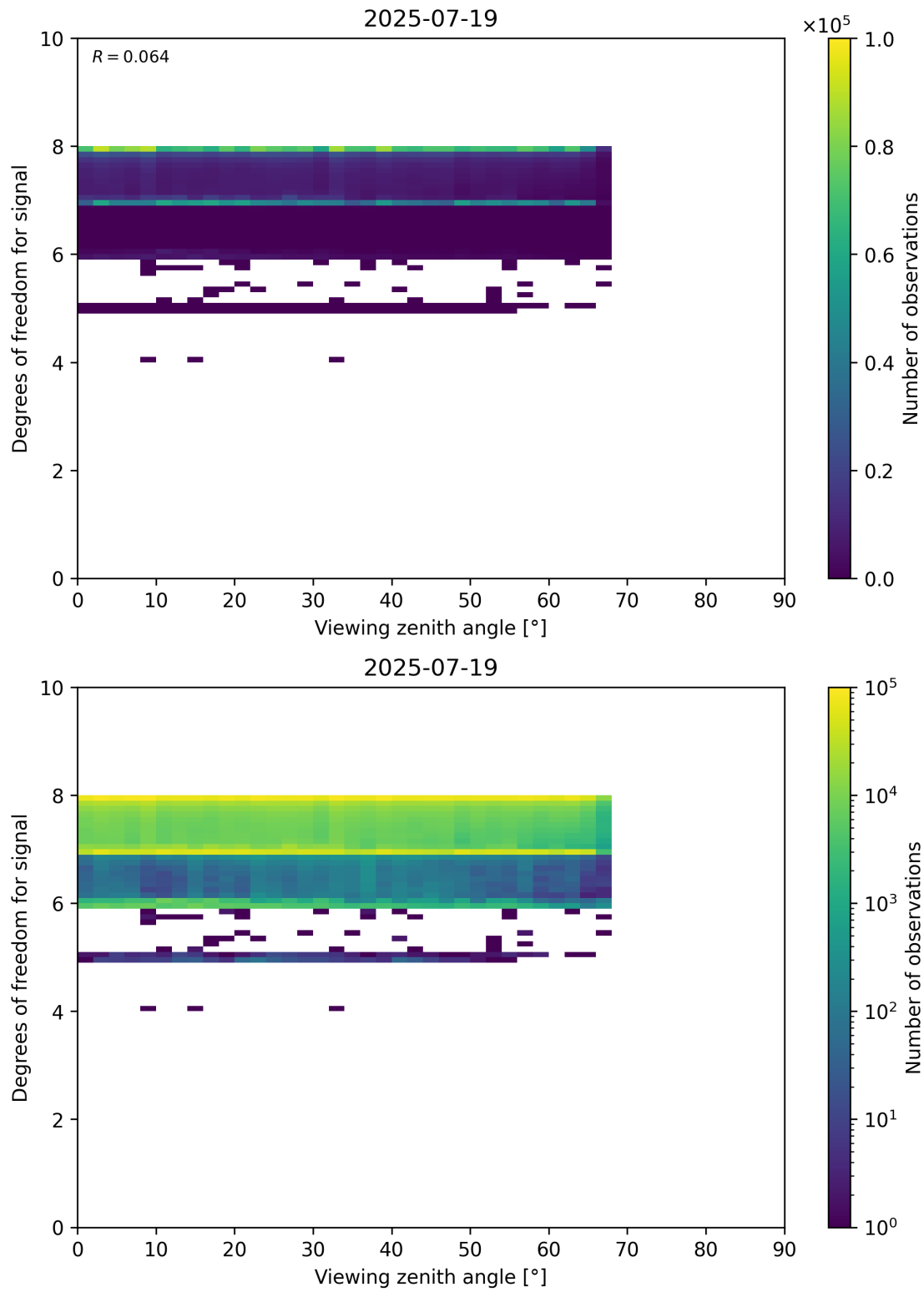
Figure 73: Scatter density plot of “Viewing zenith angle” against “Degrees of freedom for signal” for 2025-07-19 to 2025-07-20.
