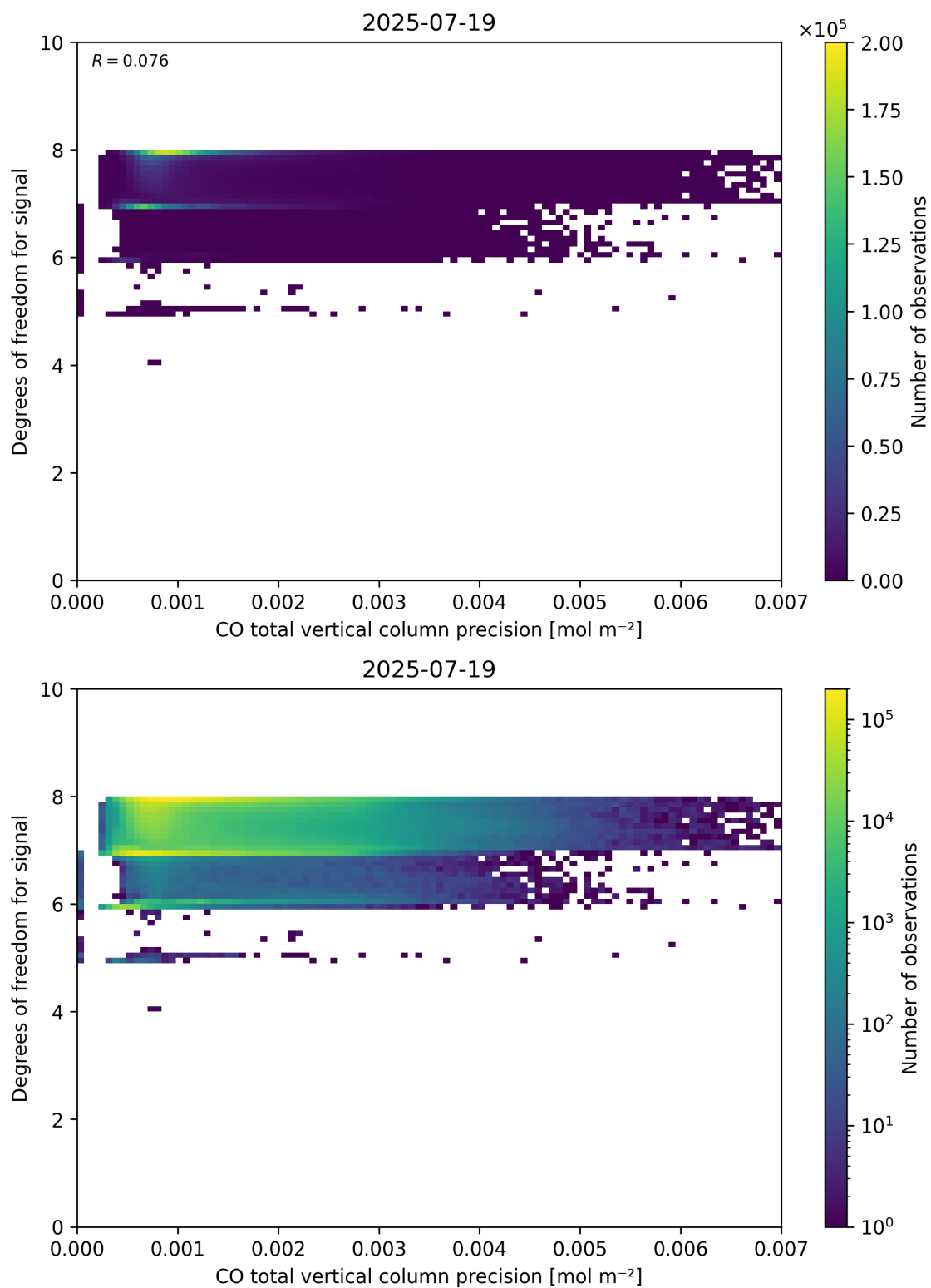
Figure 45: Scatter density plot of “CO total vertical column precision” against “Degrees of freedom for signal” for 2025-07-19 to 2025-07-20.
