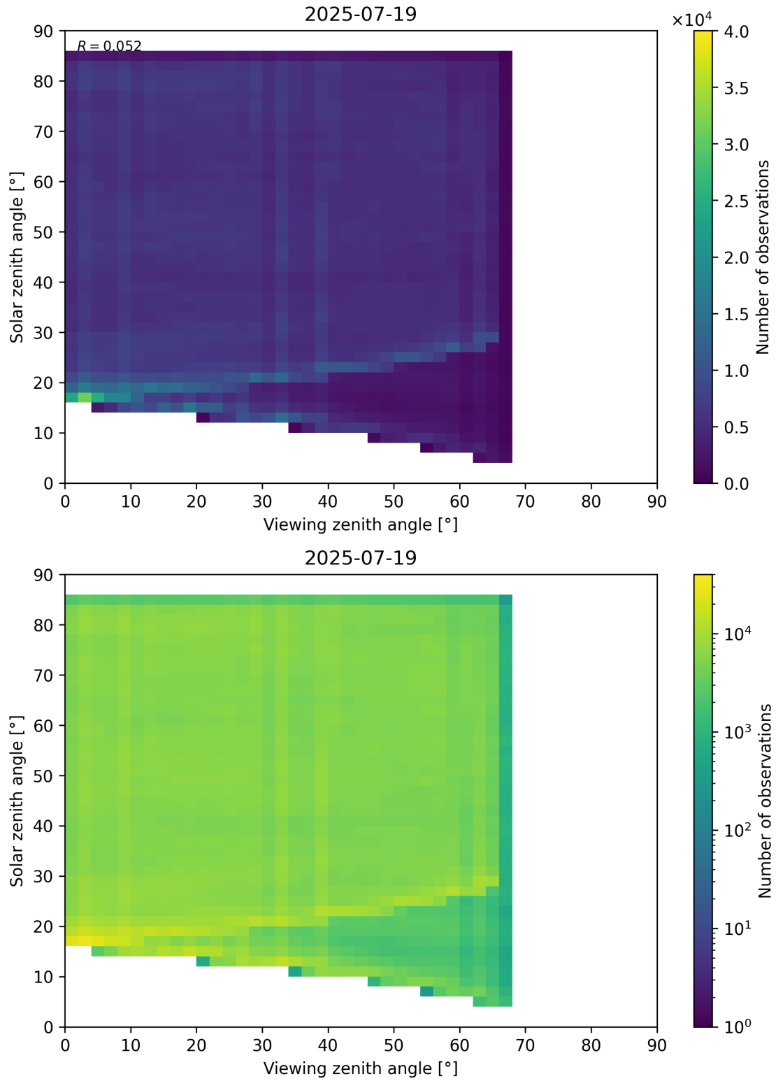
Figure 77: Scatter density plot of “Viewing zenith angle” against “Solar zenith angle” for 2025-07-19 to 2025-07-20.
