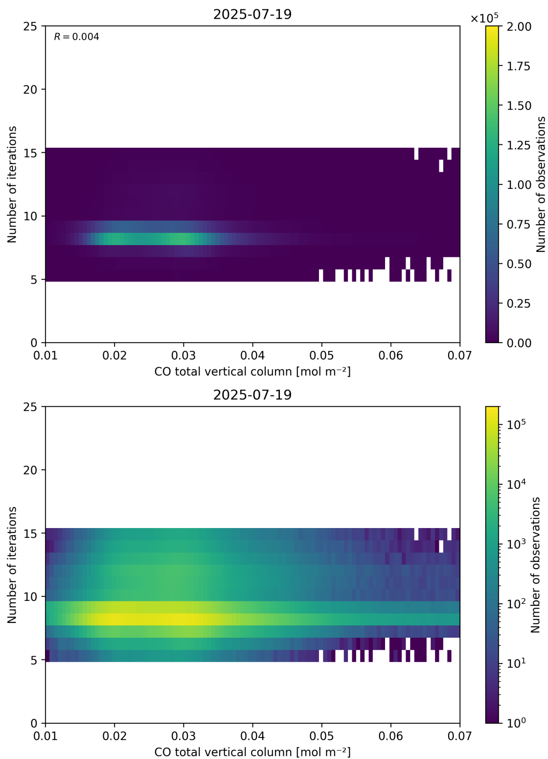
Figure 42: Scatter density plot of “CO total vertical column” against “Number of iterations” for 2025-07-19 to 2025-07-20.
