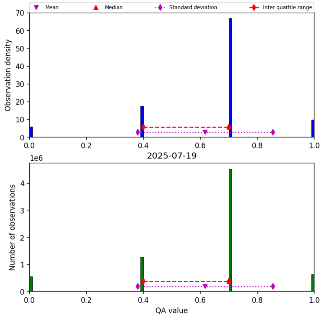
Figure 17: Histogram of “QA value” for 2025-07-19 to 2025-07-20
