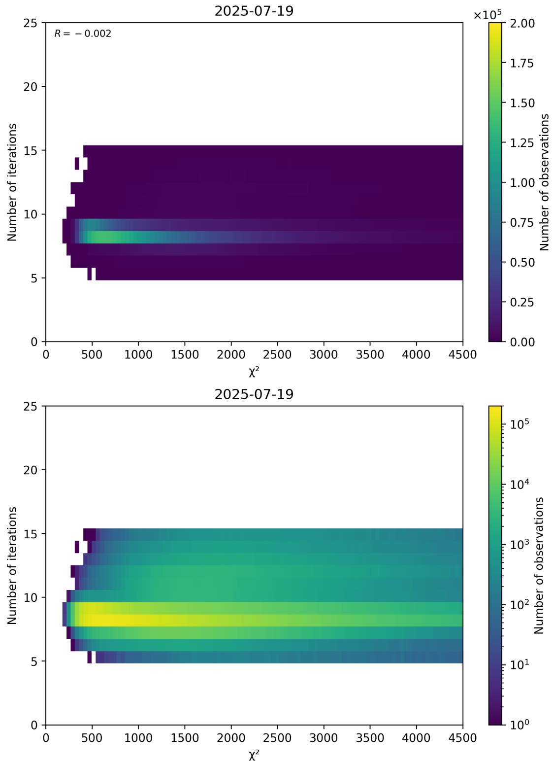
Figure 49: Scatter density plot of “ \chi^2 ” against “Number of iterations” for 2025-07-19 to 2025-07-20.
