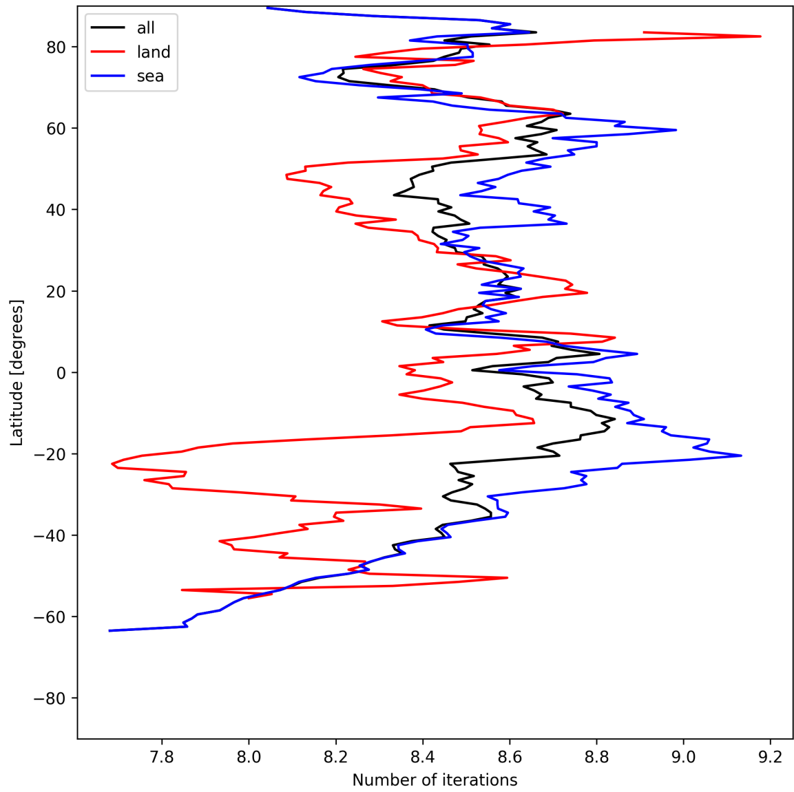
Figure 16: Zonal average of “Number of iterations” for 2025-07-19 to 2025-07-20.
