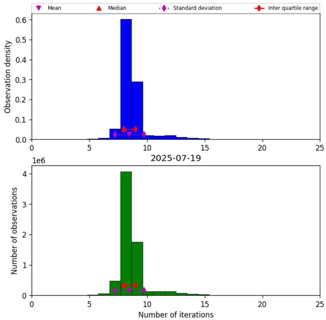
Figure 24: Histogram of “Number of iterations” for 2025-07-19 to 2025-07-20
