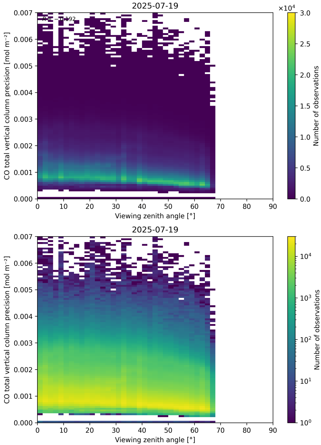
Figure 71: Scatter density plot of “Viewing zenith angle” against “CO total vertical column precision” for 2025-07-19 to 2025-07-20.
