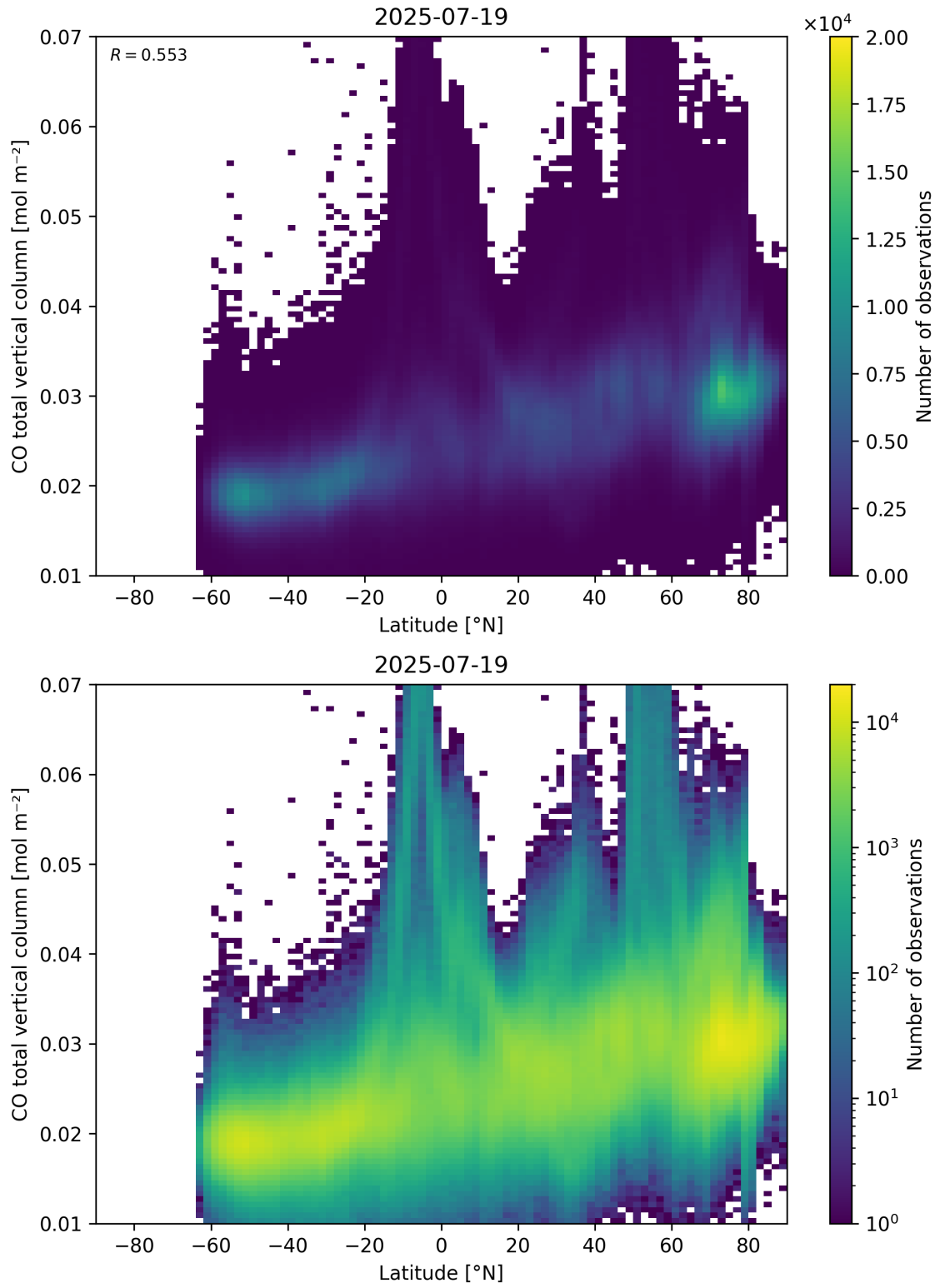
Figure 51: Scatter density plot of “Latitude” against “CO total vertical column” for 2025-07-19 to 2025-07-20.
