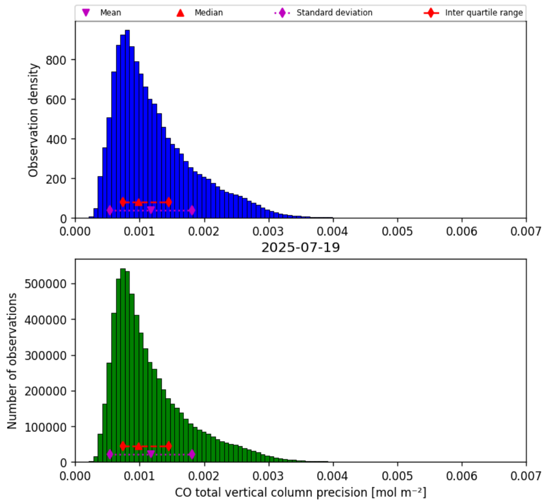
Figure 20: Histogram of “CO total vertical column precision” for 2025-07-19 to 2025-07-20
