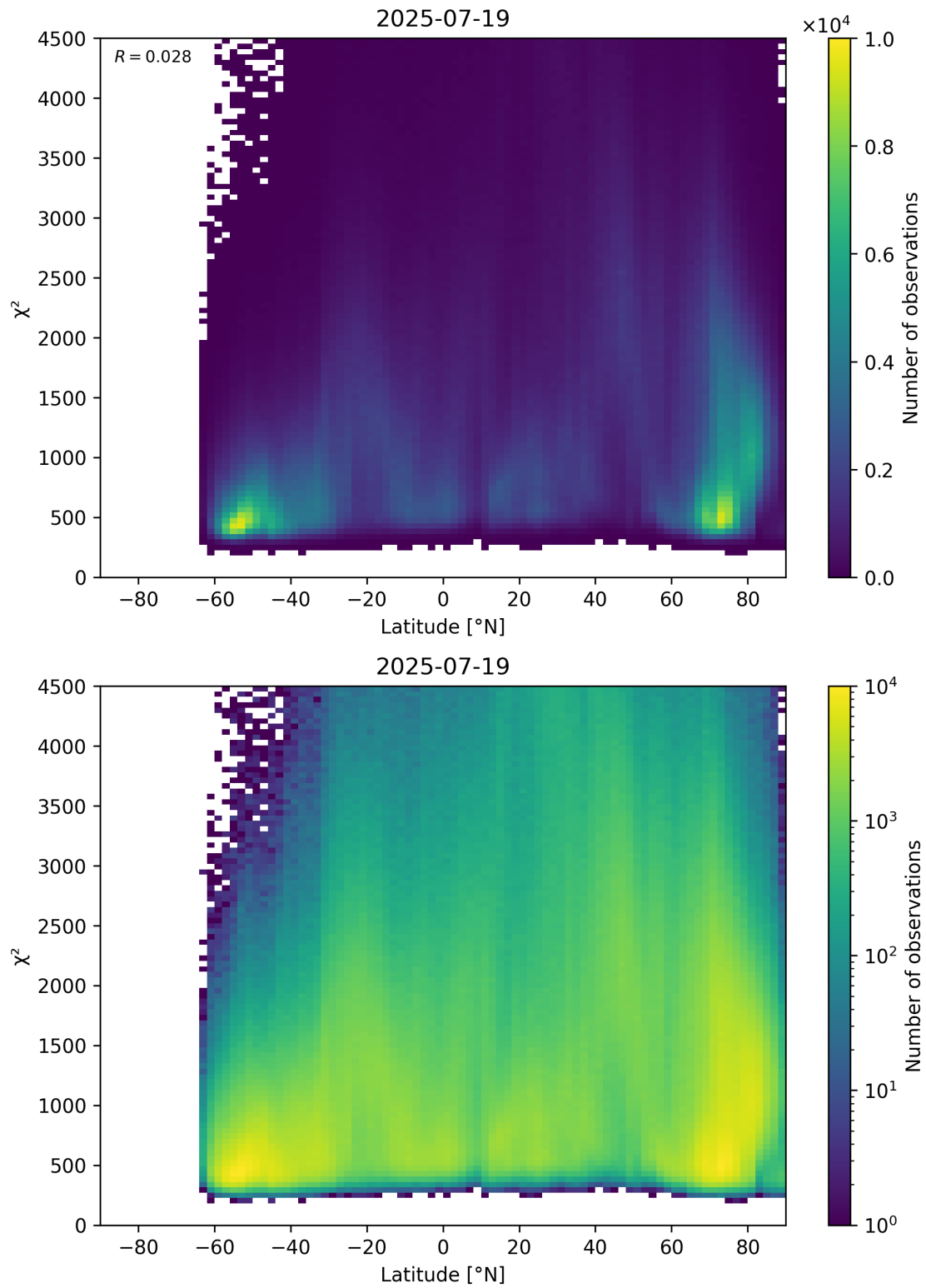
Figure 54: Scatter density plot of “Latitude” against “ \chi^2 ” for 2025-07-19 to 2025-07-20.
