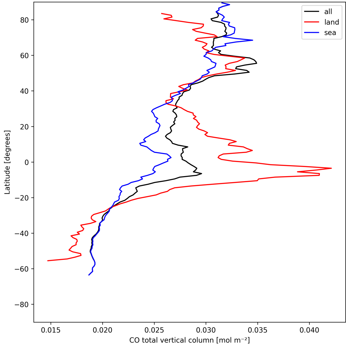
Figure 10: Zonal average of “CO total vertical column” for 2025-07-19 to 2025-07-20.
