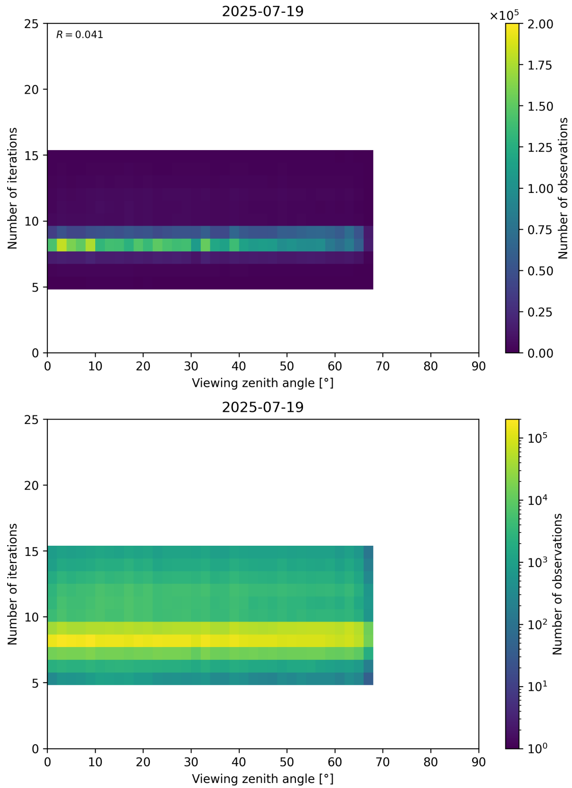
Figure 75: Scatter density plot of “Viewing zenith angle” against “Number of iterations” for 2025-07-19 to 2025-07-20.
