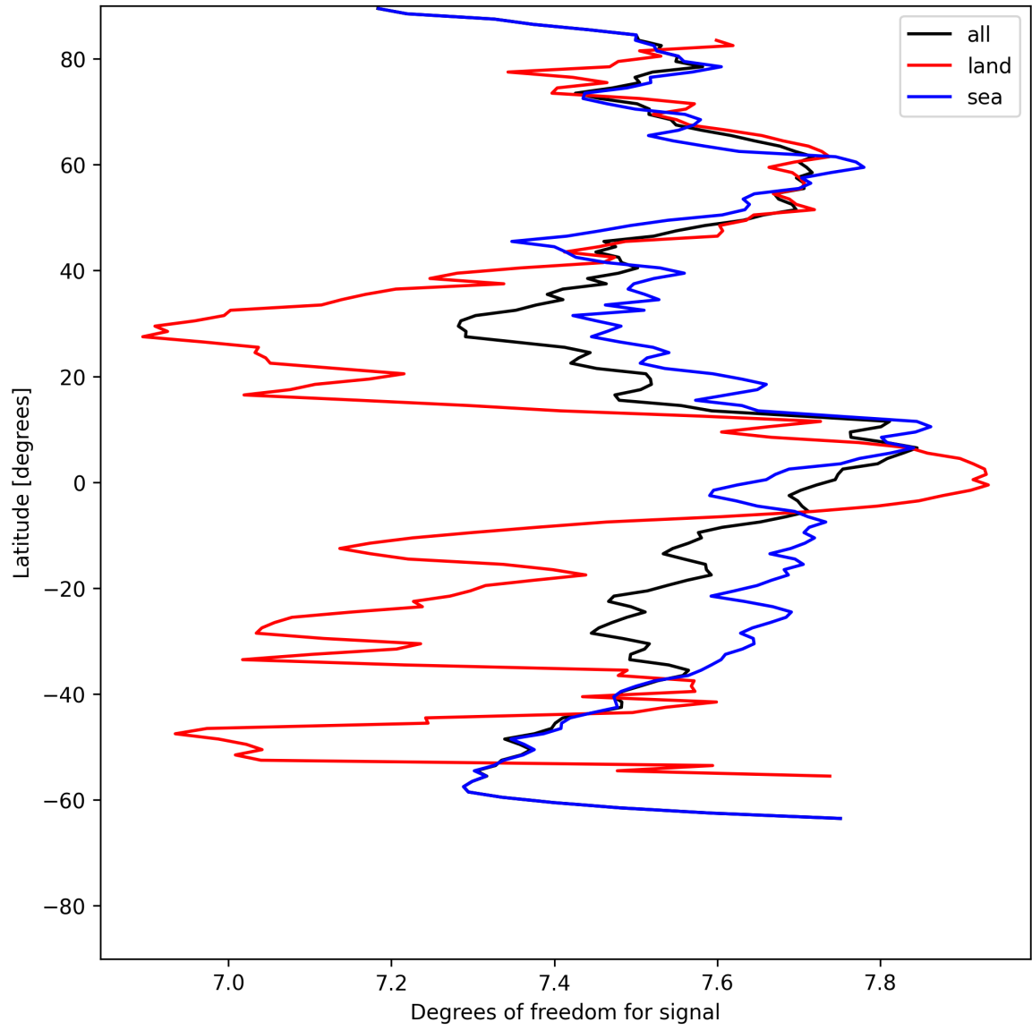
Figure 15: Zonal average of “Degrees of freedom for signal” for 2025-07-19 to 2025-07-20.
