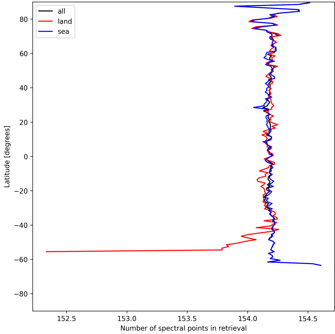
Figure 13: Zonal average of “Number of spectral points in retrieval” for 2025-07-19 to 2025-07-20.
