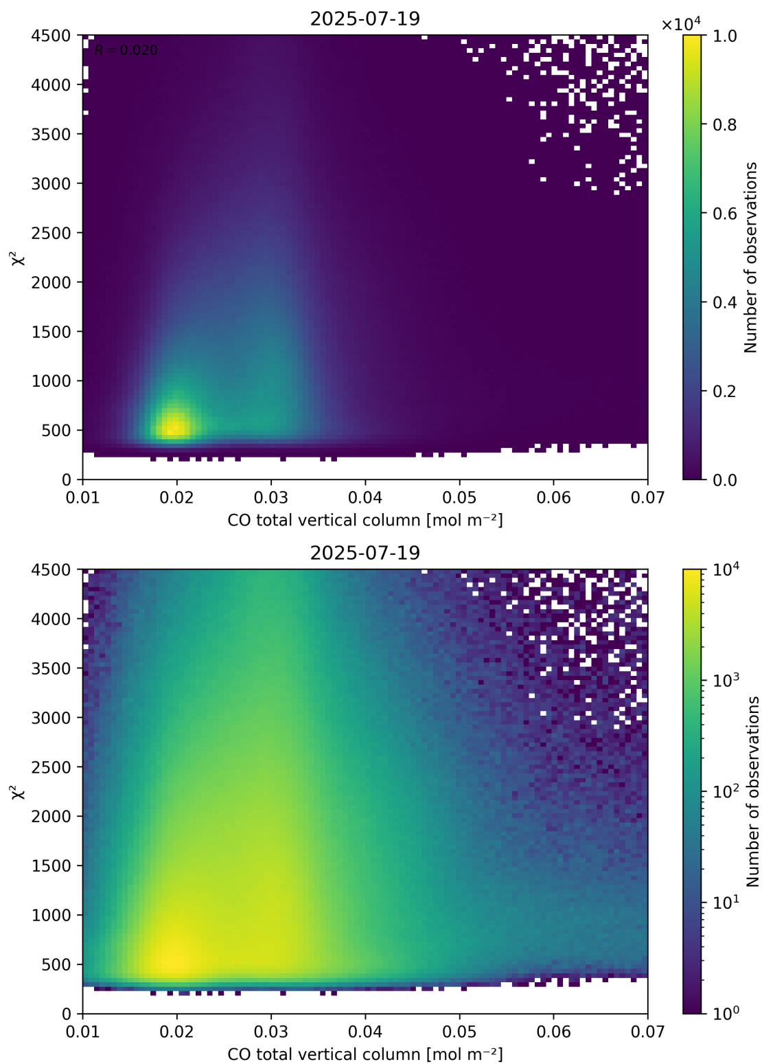
Figure 35: Scatter density plot of “CO total vertical column” against “ \chi^2 ” for 2025-07-19 to 2025-07-20.
