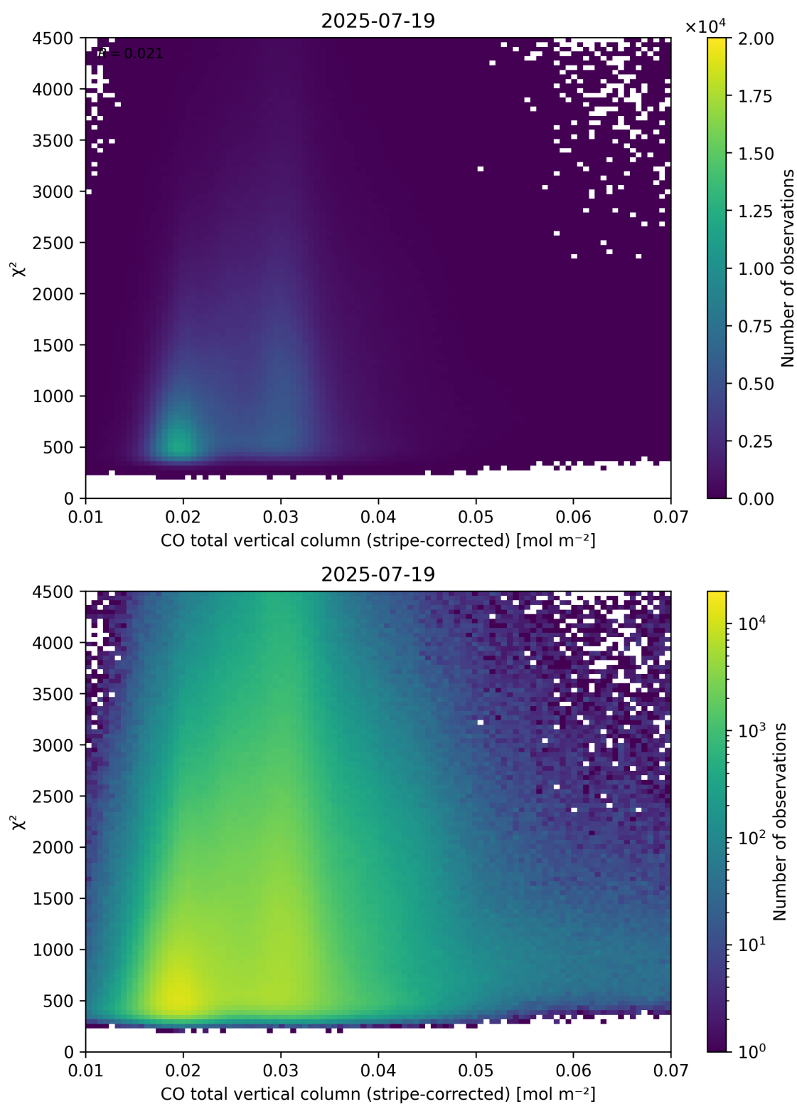
Figure 37: Scatter density plot of “CO total vertical column (stripe-corrected)” against “ \chi^2 ” for 2025-07-19 to 2025-07-20.
