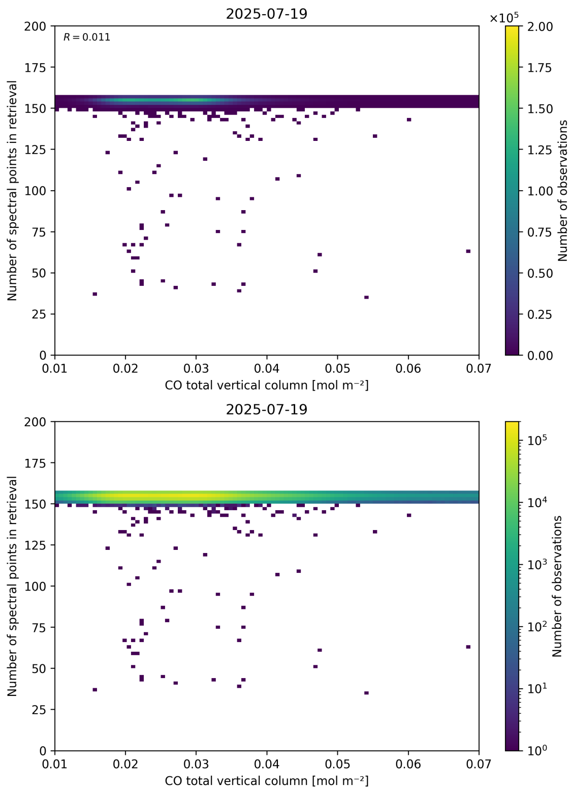
Figure 43: Scatter density plot of “CO total vertical column” against “Number of spectral points in retrieval” for 2025-07-19 to 2025-07-20.
