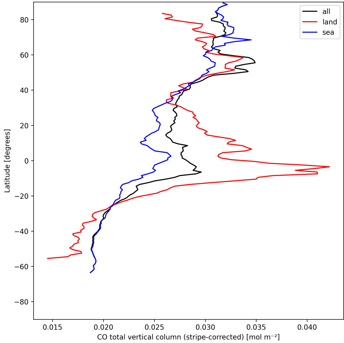
Figure 11: Zonal average of “CO total vertical column (stripe-corrected)” for 2025-07-19 to 2025-07-20.
