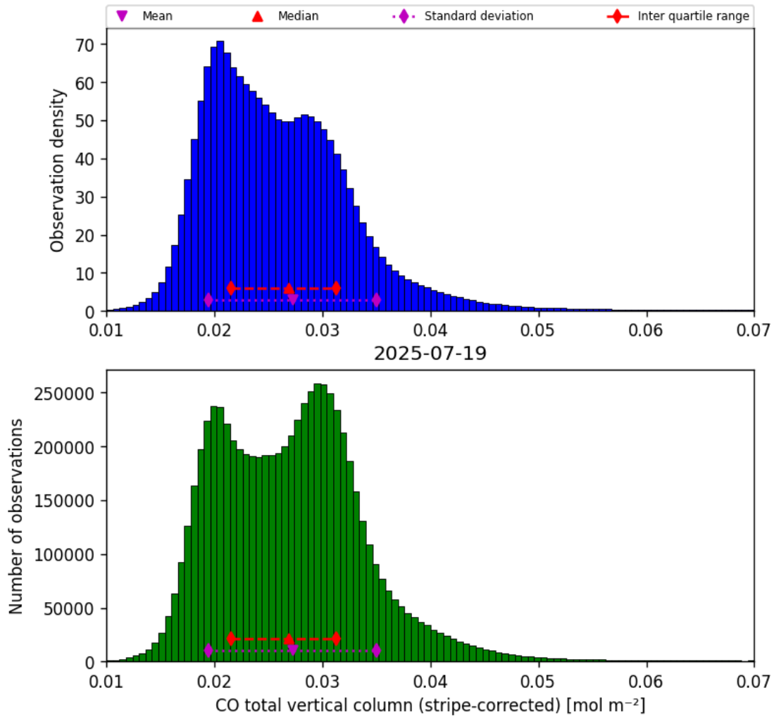
Figure 19: Histogram of “CO total vertical column (stripe-corrected)” for 2025-07-19 to 2025-07-20
