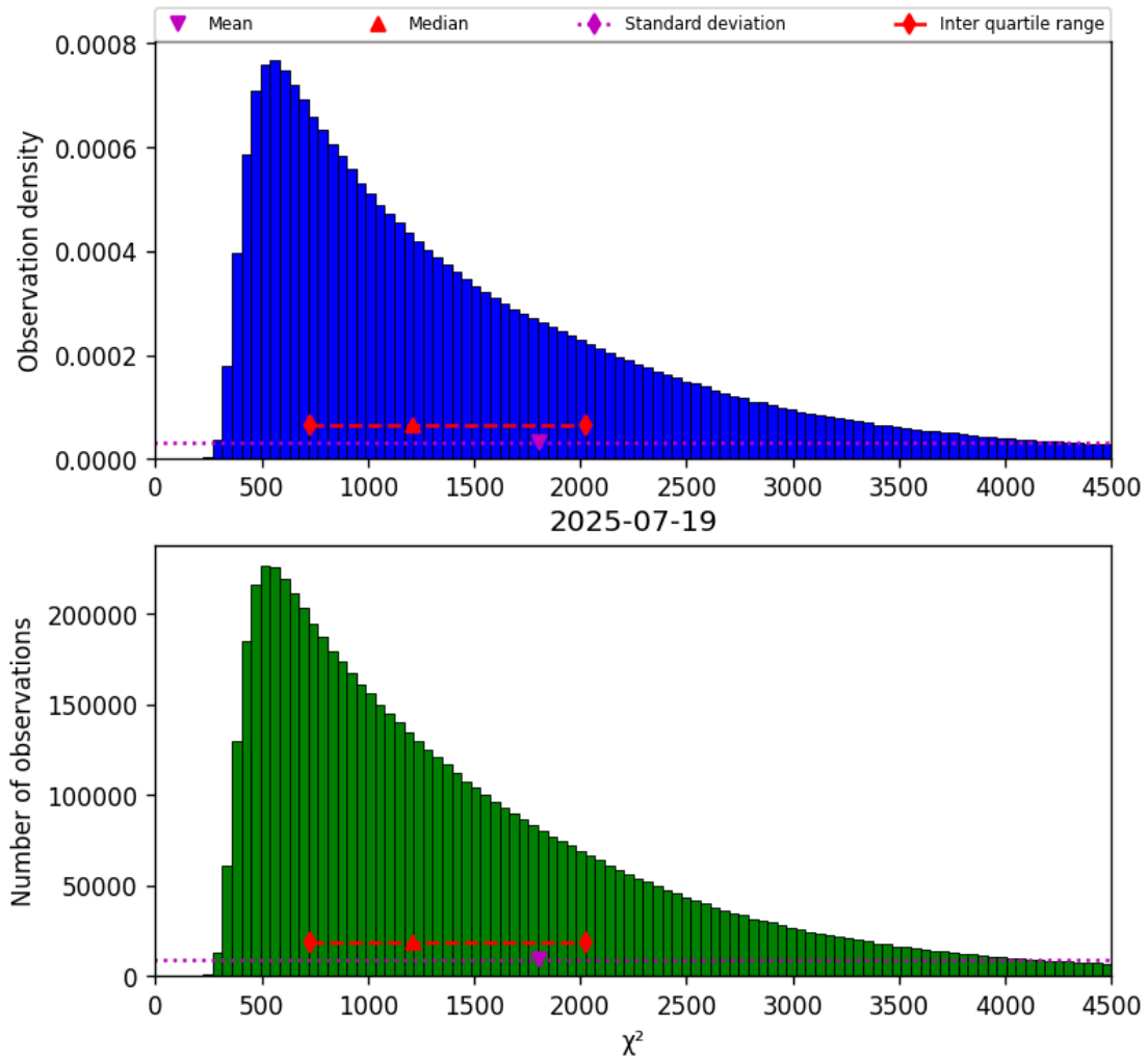
Figure 22: Histogram of “ \chi^2 ” for 2025-07-19 to 2025-07-20
