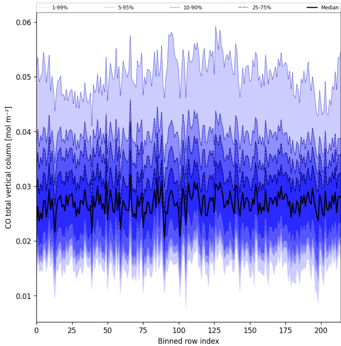
Figure 26: Along track statistics of “CO total vertical column” for 2025-07-19 to 2025-07-20
