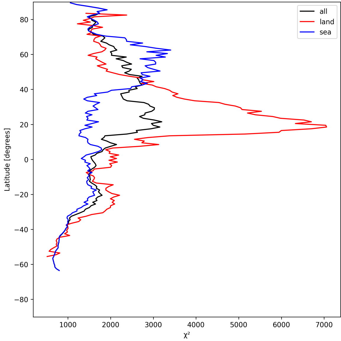
Figure 14: Zonal average of “ \chi^2 ” for 2025-07-19 to 2025-07-20.
