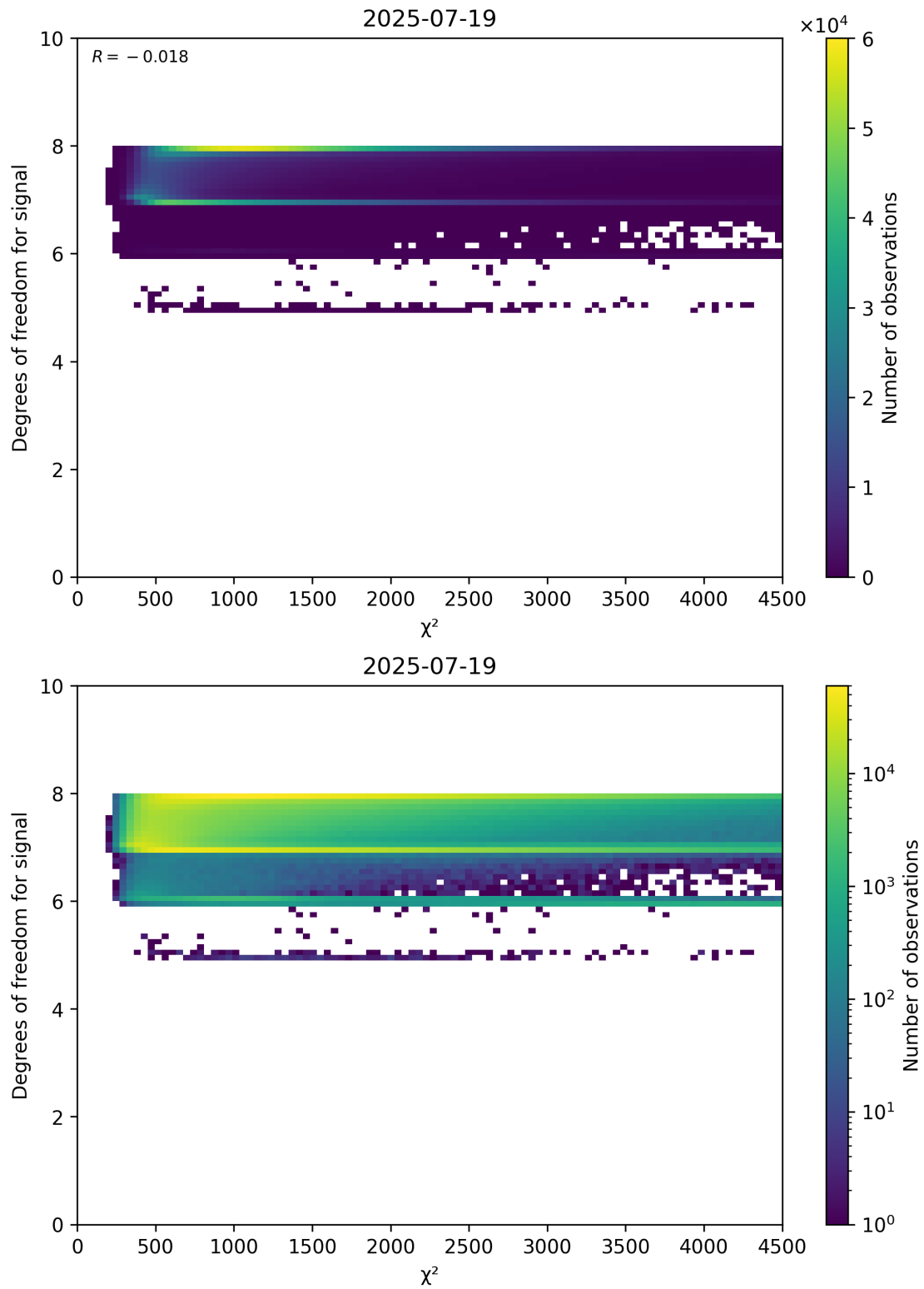
Figure 48: Scatter density plot of “ \chi^2 ” against “Degrees of freedom for signal” for 2025-07-19 to 2025-07-20.
