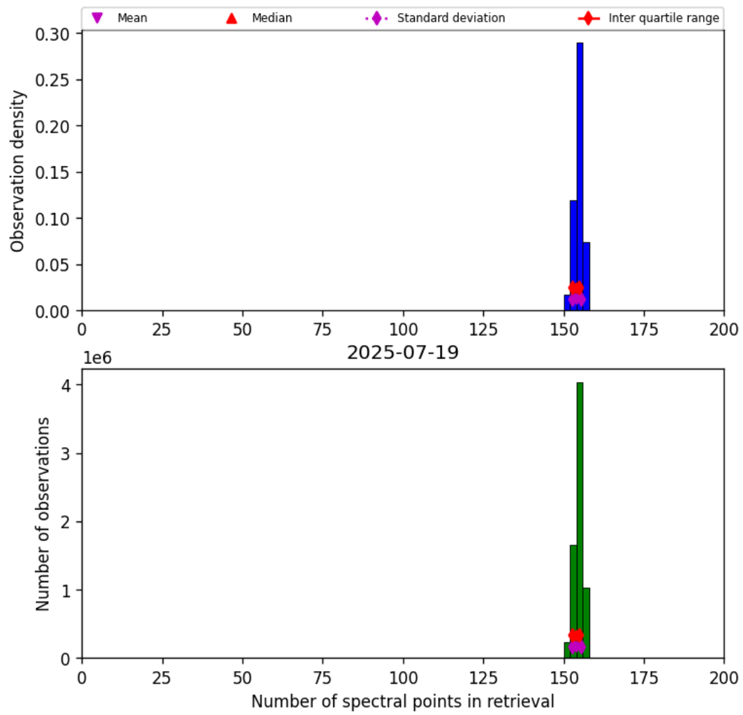
Figure 21: Histogram of “Number of spectral points in retrieval” for 2025-07-19 to 2025-07-20
