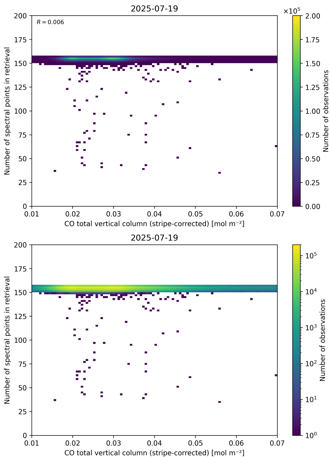
Figure 40: Scatter density plot of “CO total vertical column (stripe-corrected)” against “Number of spectral points in retrieval” for 2025-07-19 to 2025-07-20.
