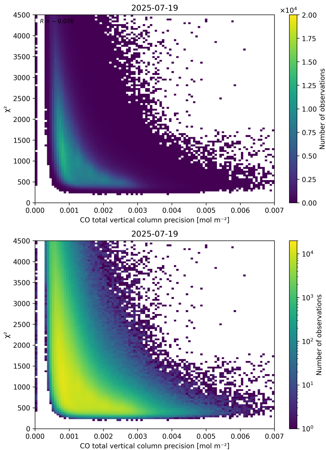
Figure 44: Scatter density plot of “CO total vertical column precision” against “ \chi^2 ” for 2025-07-19 to 2025-07-20.
