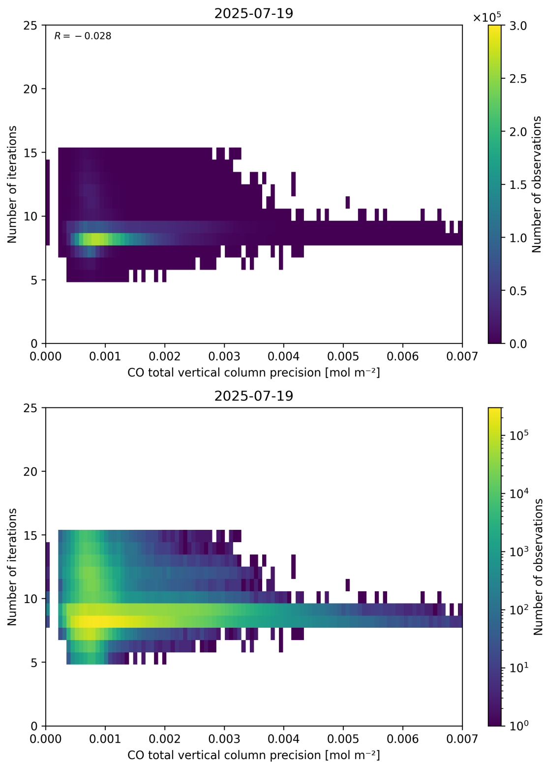
Figure 46: Scatter density plot of “CO total vertical column precision” against “Number of iterations” for 2025-07-19 to 2025-07-20.
