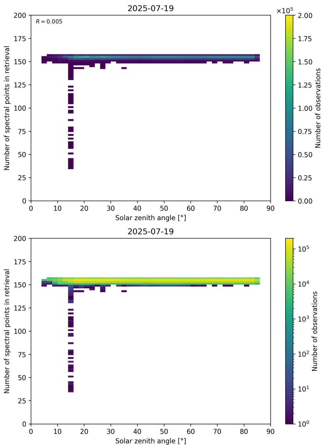
Figure 68: Scatter density plot of “Solar zenith angle” against “Number of spectral points in retrieval” for 2025-07-19 to 2025-07-20.
