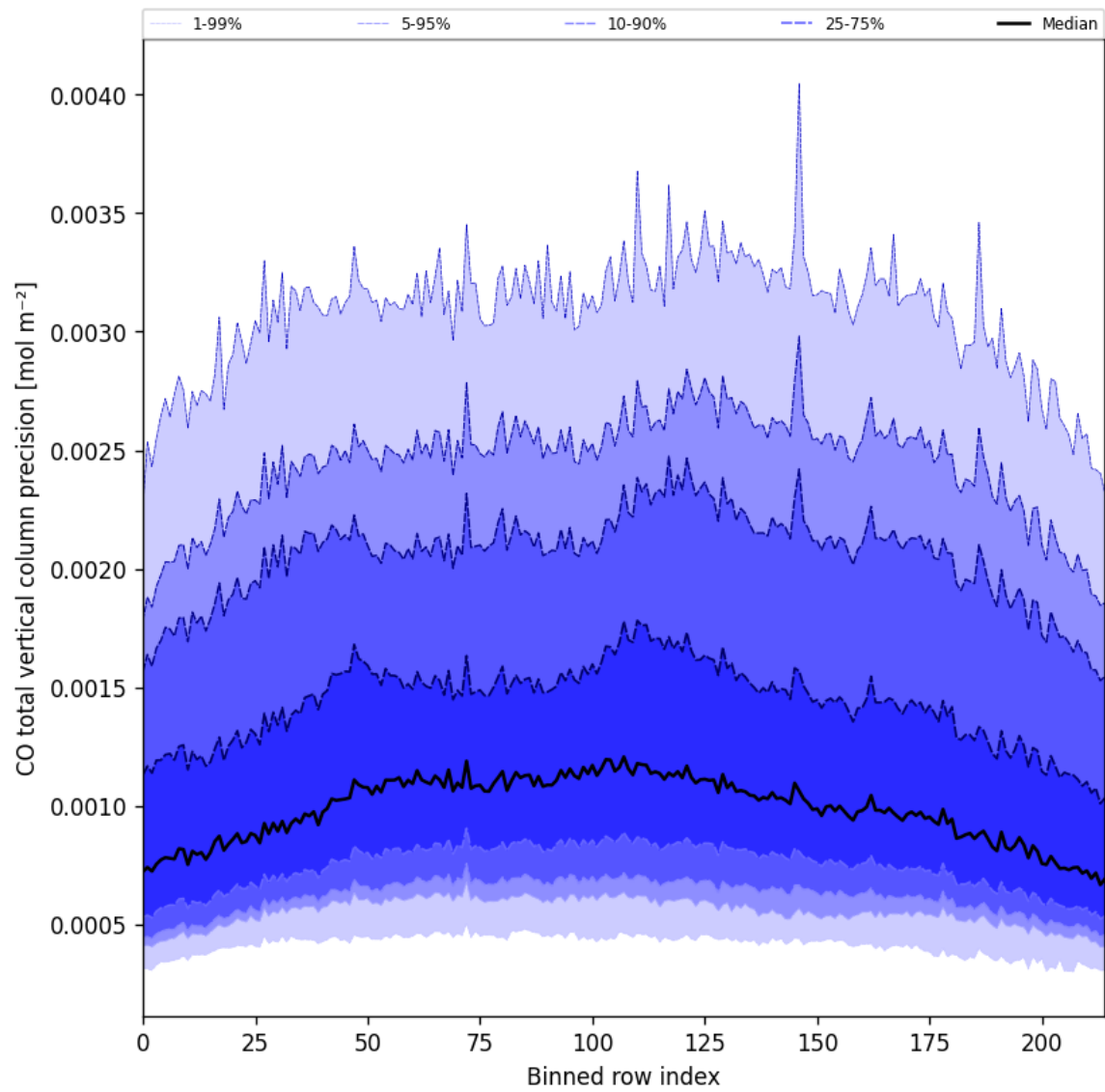
Figure 28: Along track statistics of “CO total vertical column precision” for 2025-07-19 to 2025-07-20
