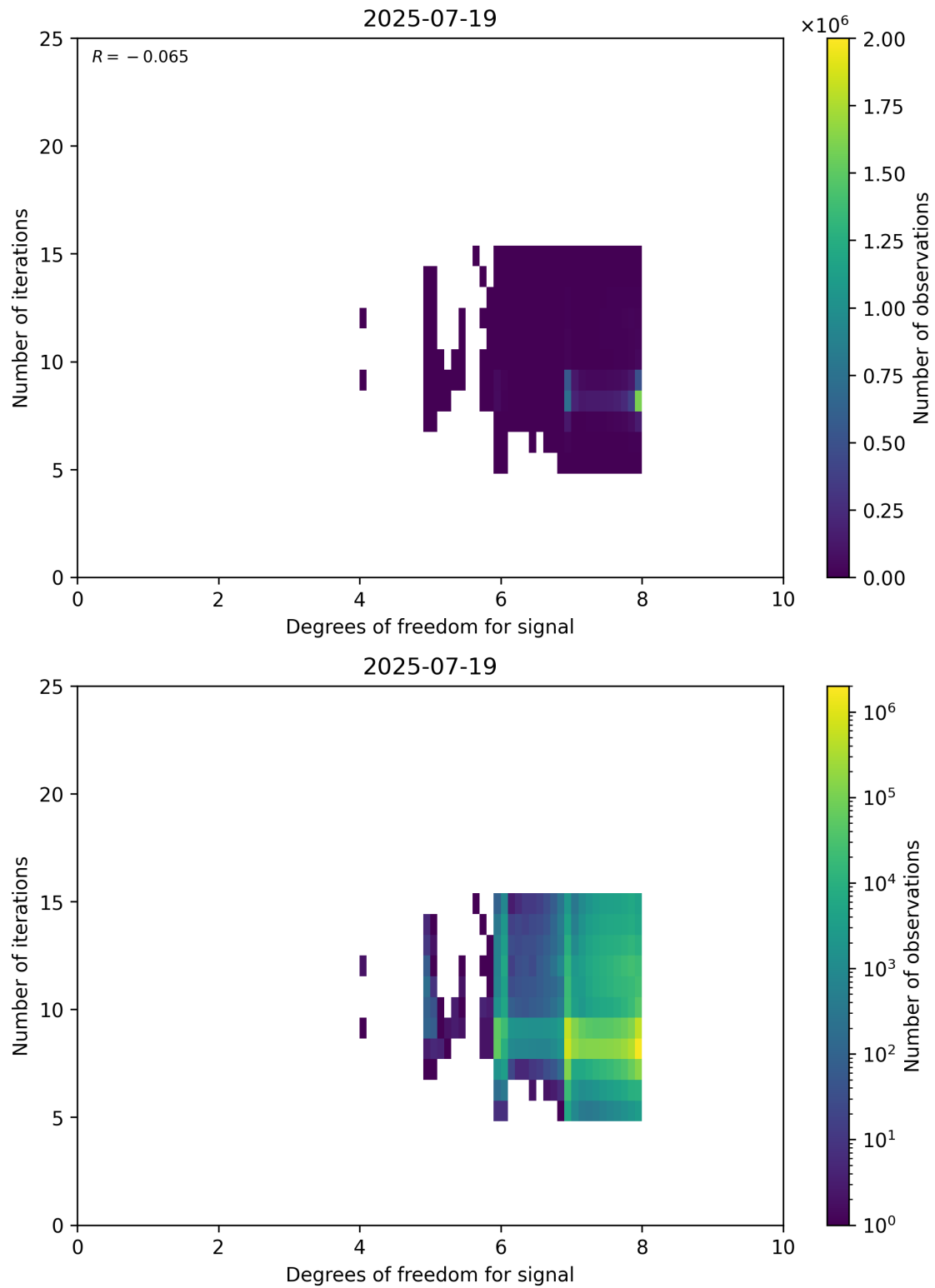
Figure 50: Scatter density plot of “Degrees of freedom for signal” against “Number of iterations” for 2025-07-19 to 2025-07-20.
