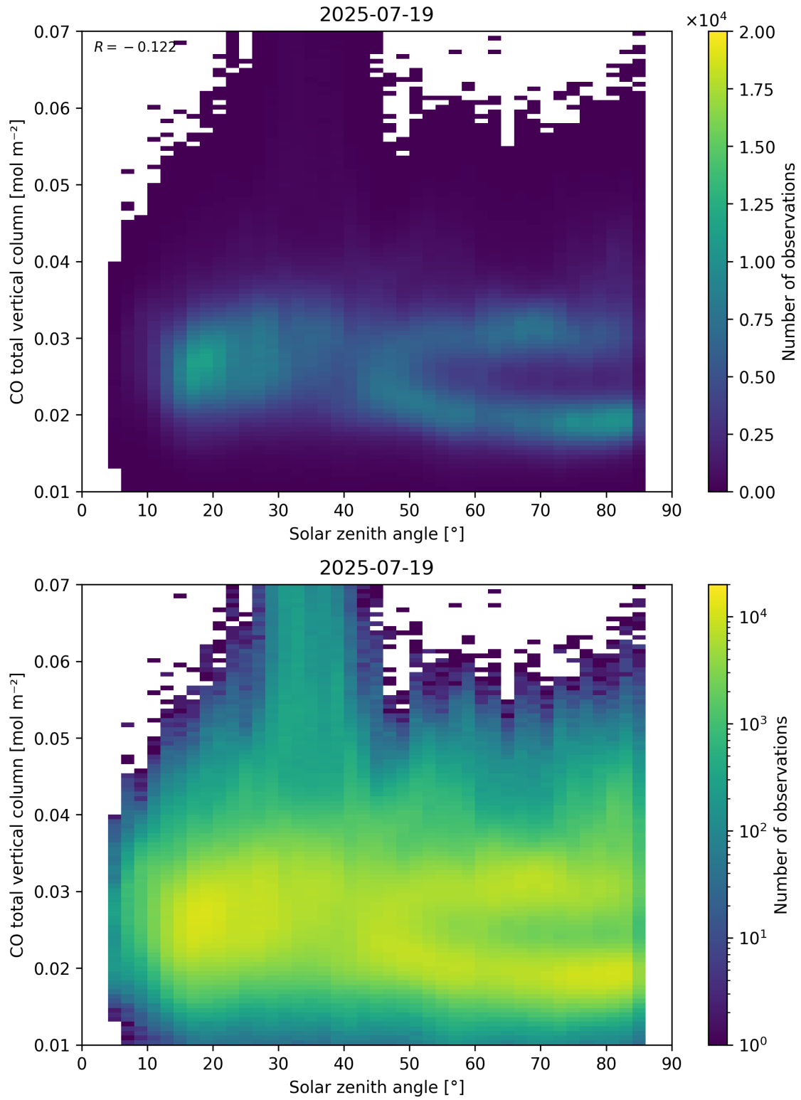
Figure 61: Scatter density plot of “Solar zenith angle” against “CO total vertical column” for 2025-07-19 to 2025-07-20.
