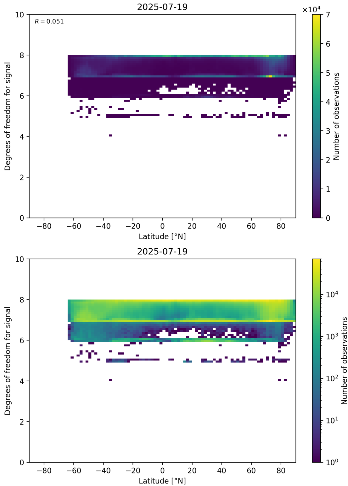
Figure 55: Scatter density plot of “Latitude” against “Degrees of freedom for signal” for 2025-07-19 to 2025-07-20.
