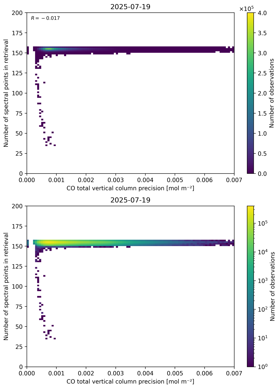
Figure 47: Scatter density plot of “CO total vertical column precision” against “Number of spectral points in retrieval” for 2025-07-19 to 2025-07-20.
