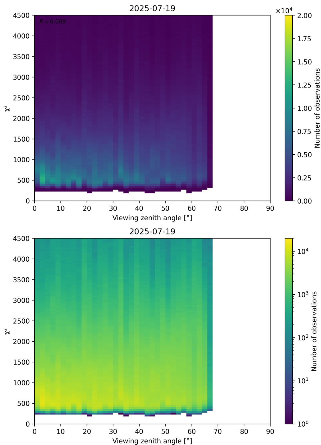
Figure 72: Scatter density plot of “Viewing zenith angle” against “ \chi^2 ” for 2025-07-19 to 2025-07-20.
