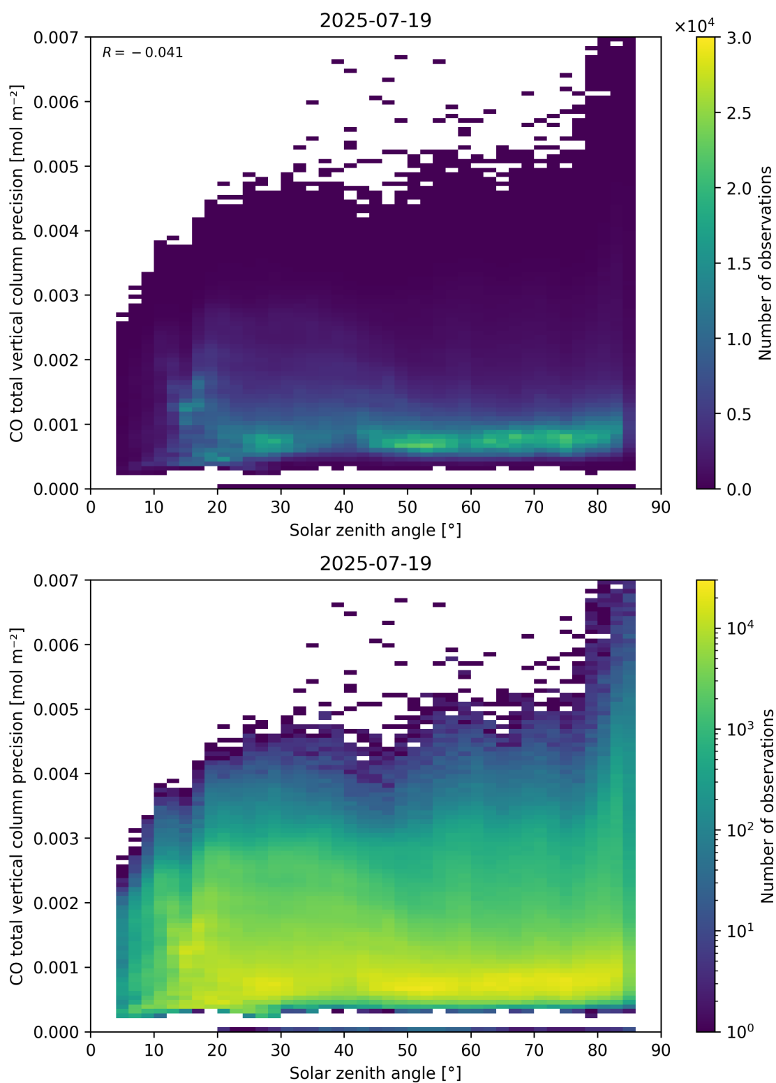
Figure 63: Scatter density plot of “Solar zenith angle” against “CO total vertical column precision” for 2025-07-19 to 2025-07-20.
