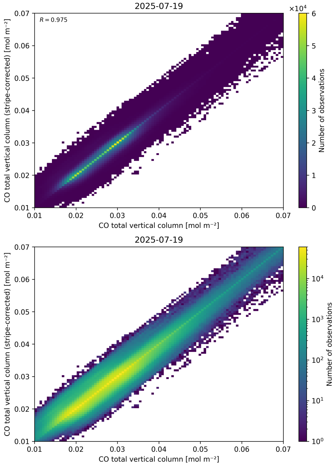
Figure 33: Scatter density plot of “CO total vertical column” against “CO total vertical column (stripe-corrected)” for 2025-07-19 to 2025-07-20.
