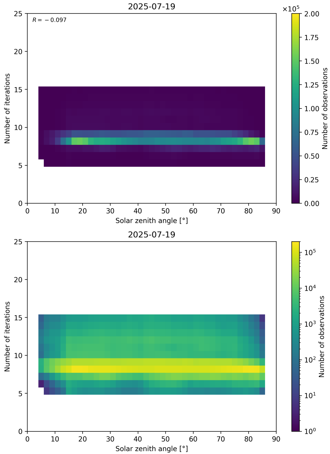
Figure 67: Scatter density plot of “Solar zenith angle” against “Number of iterations” for 2025-07-19 to 2025-07-20.
