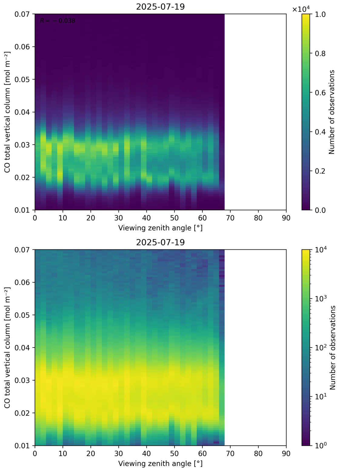
Figure 69: Scatter density plot of “Viewing zenith angle” against “CO total vertical column” for 2025-07-19 to 2025-07-20.
