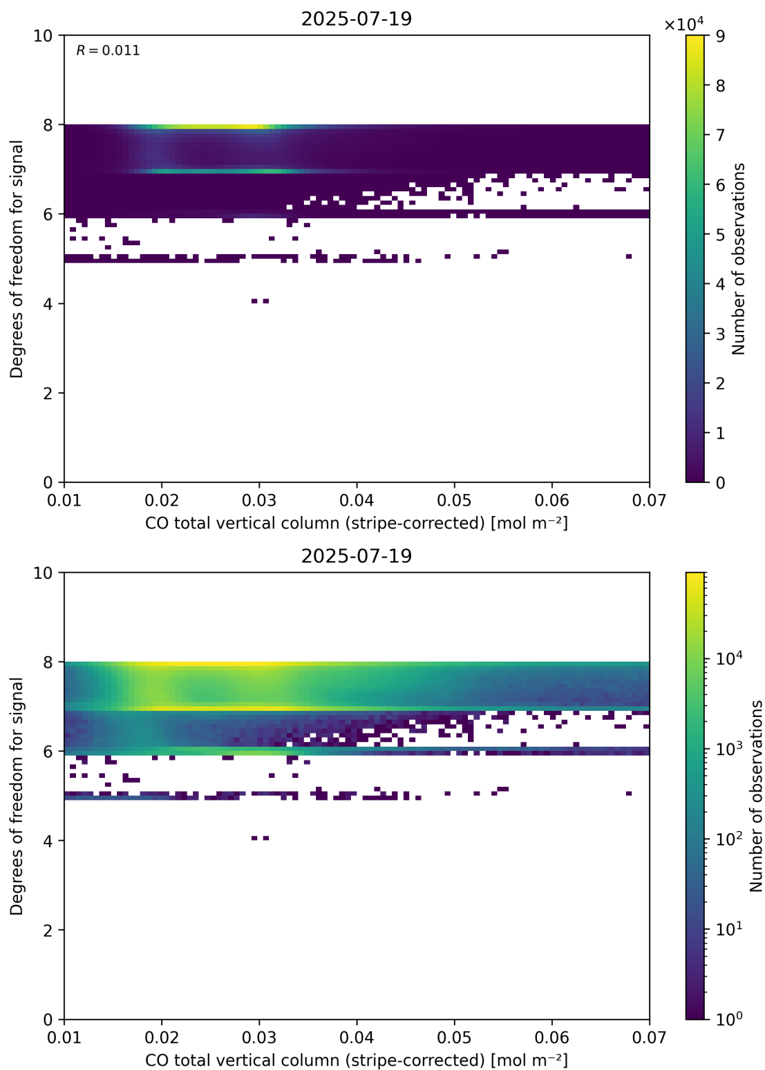
Figure 38: Scatter density plot of “CO total vertical column (stripe-corrected)” against “Degrees of freedom for signal” for 2025-07-19 to 2025-07-20.
