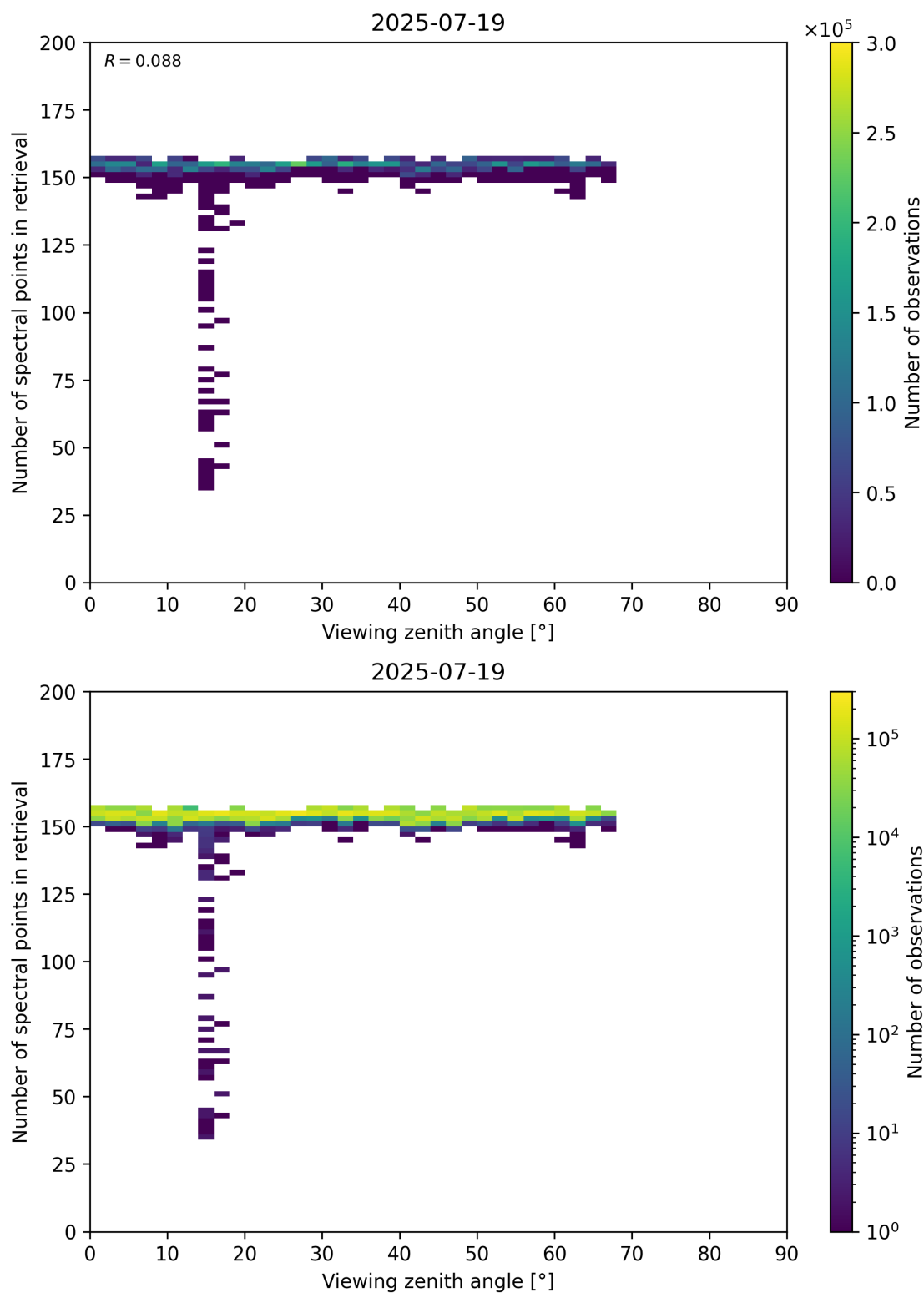
Figure 76: Scatter density plot of “Viewing zenith angle” against “Number of spectral points in retrieval” for 2025-07-19 to 2025-07-20.
