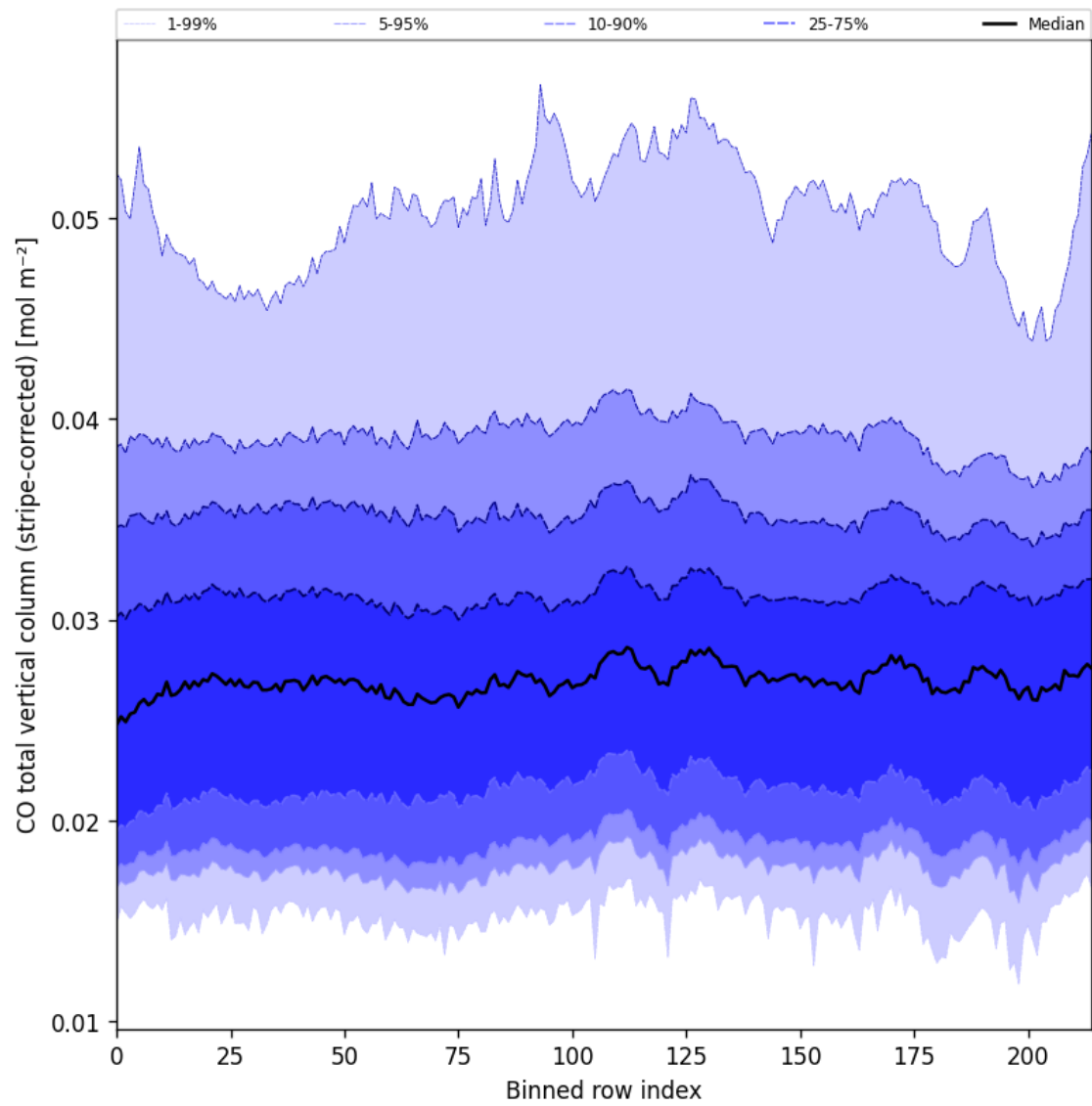
Figure 27: Along track statistics of “CO total vertical column (stripe-corrected)” for 2025-07-19 to 2025-07-20
