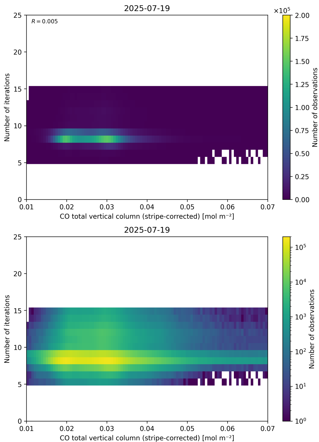
Figure 39: Scatter density plot of “CO total vertical column (stripe-corrected)” against “Number of iterations” for 2025-07-19 to 2025-07-20.
