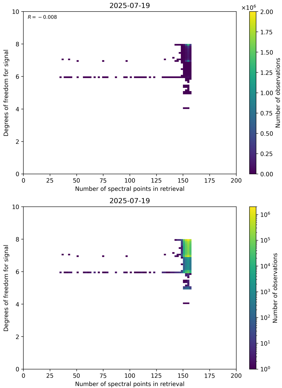
Figure 59: Scatter density plot of “Number of spectral points in retrieval” against “Degrees of freedom for signal” for 2025-07-19 to 2025-07-20.
