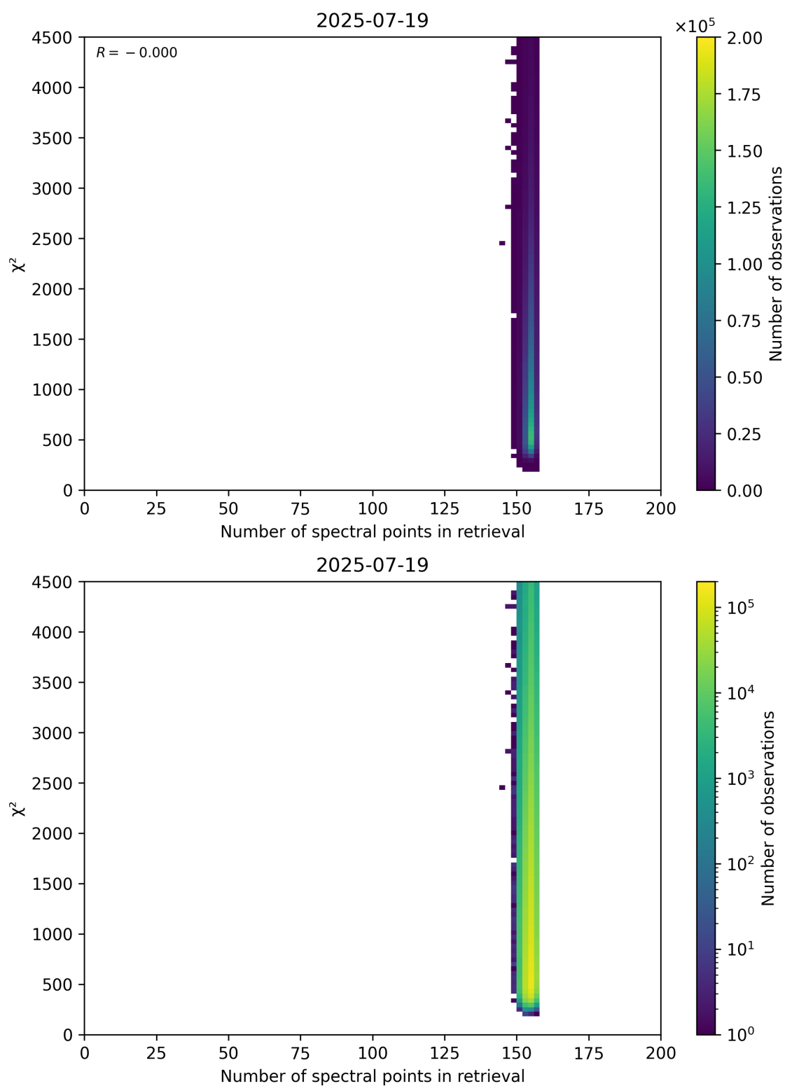
Figure 58: Scatter density plot of “Number of spectral points in retrieval” against “ \chi^2 ” for 2025-07-19 to 2025-07-20.
