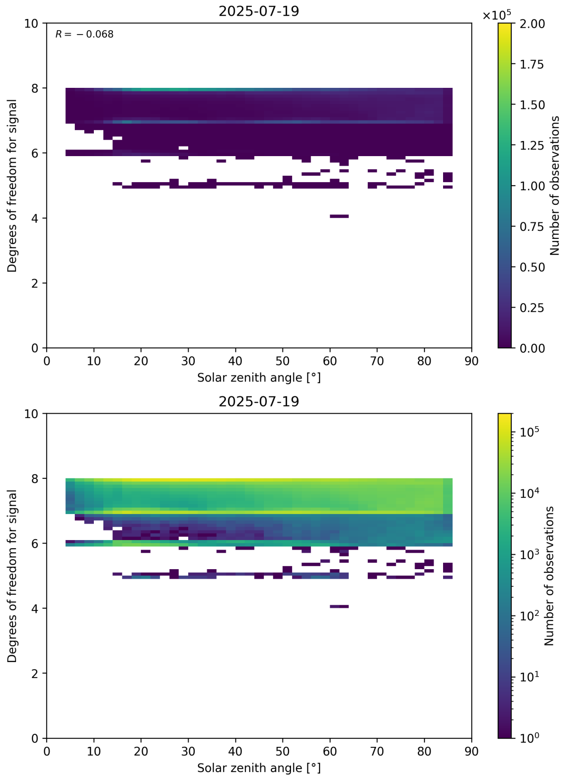
Figure 65: Scatter density plot of “Solar zenith angle” against “Degrees of freedom for signal” for 2025-07-19 to 2025-07-20.
