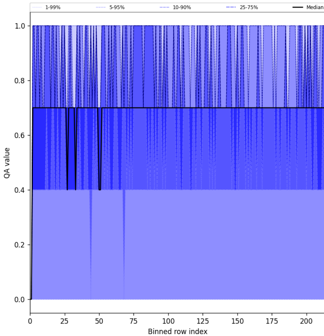
Figure 25: Along track statistics of “QA value” for 2025-07-19 to 2025-07-20
