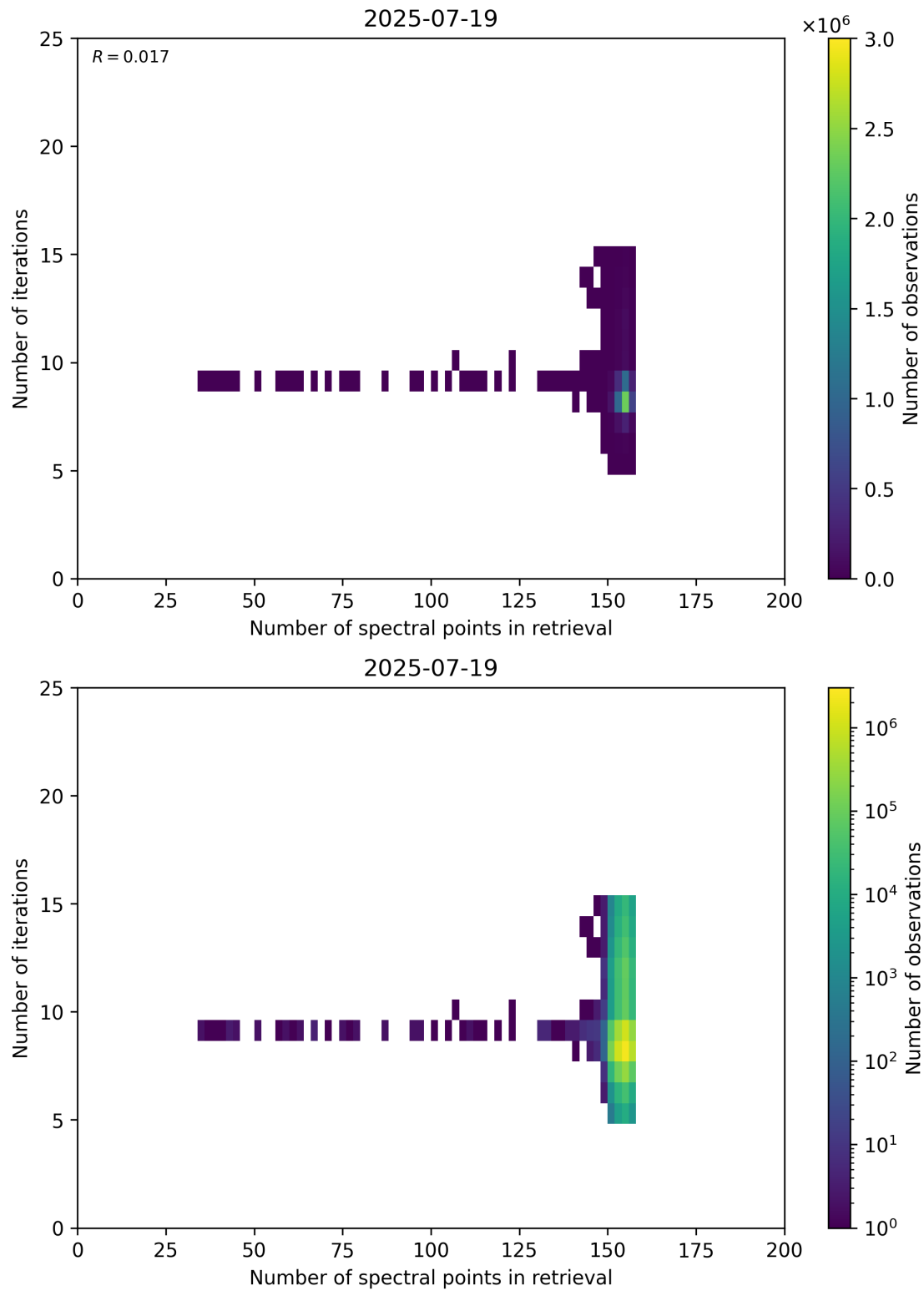
Figure 60: Scatter density plot of “Number of spectral points in retrieval” against “Number of iterations” for 2025-07-19 to 2025-07-20.
