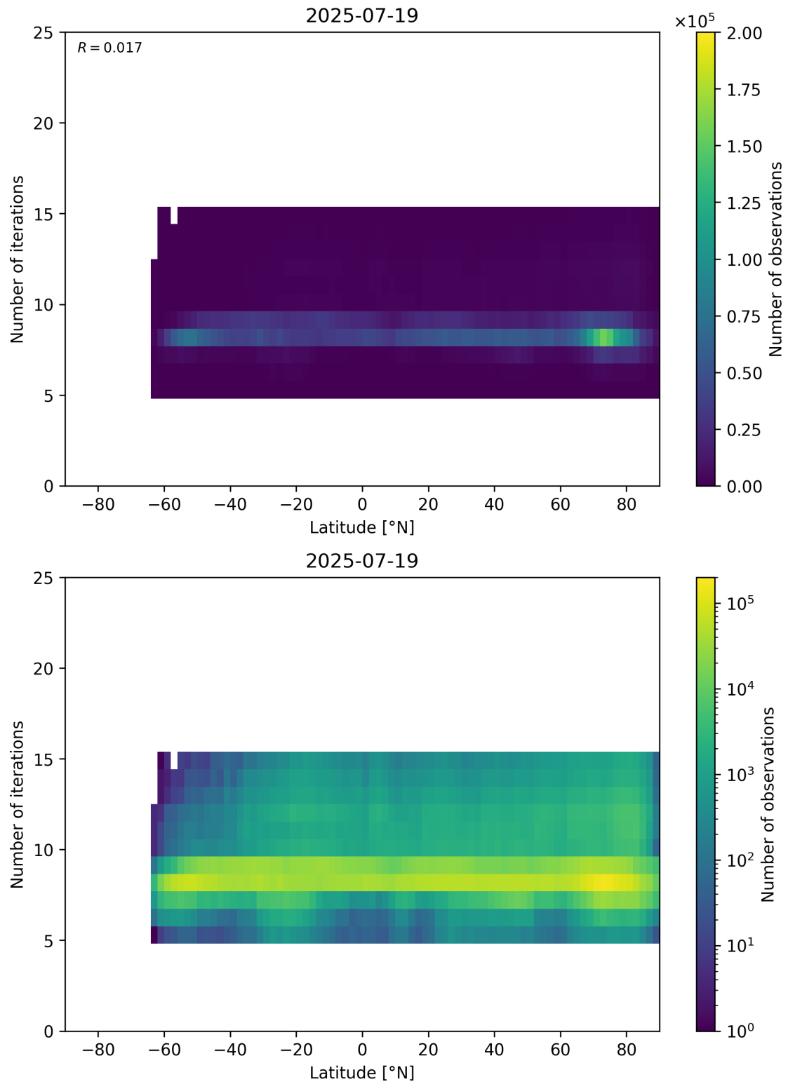
Figure 56: Scatter density plot of “Latitude” against “Number of iterations” for 2025-07-19 to 2025-07-20.
