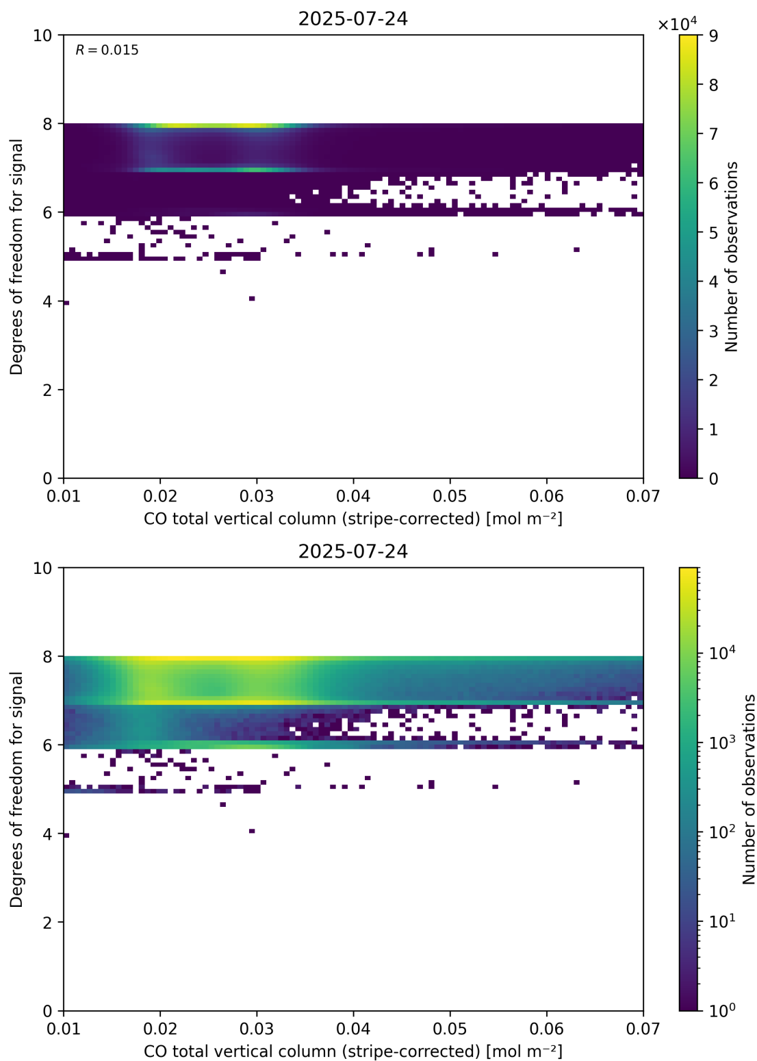
Figure 38: Scatter density plot of “CO total vertical column (stripe-corrected)” against “Degrees of freedom for signal” for 2025-07-24 to 2025-07-25.
