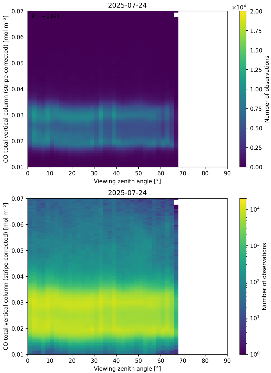
Figure 70: Scatter density plot of “Viewing zenith angle” against “CO total vertical column (stripe-corrected)” for 2025-07-24 to 2025-07-25.
