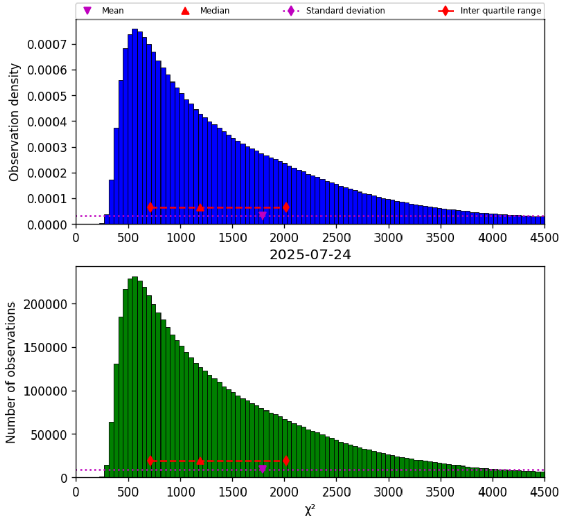
Figure 22: Histogram of “ \chi^2 ” for 2025-07-24 to 2025-07-25
