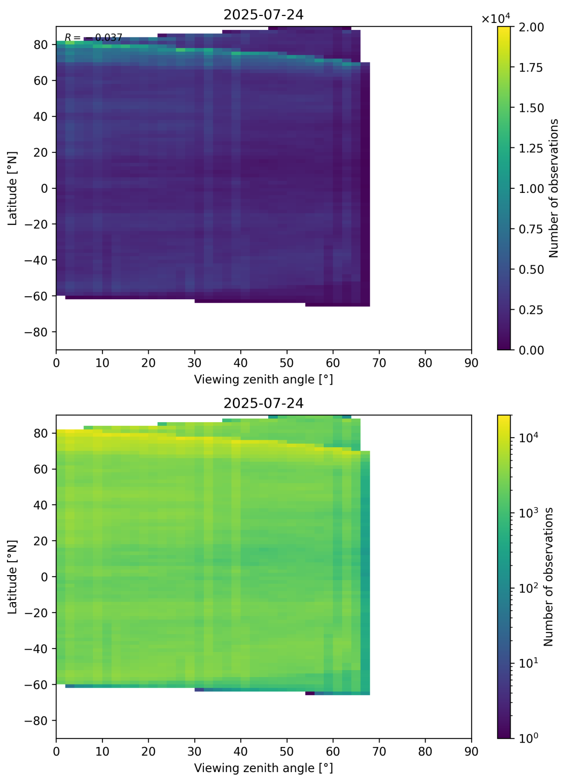
Figure 74: Scatter density plot of “Viewing zenith angle” against “Latitude” for 2025-07-24 to 2025-07-25.
