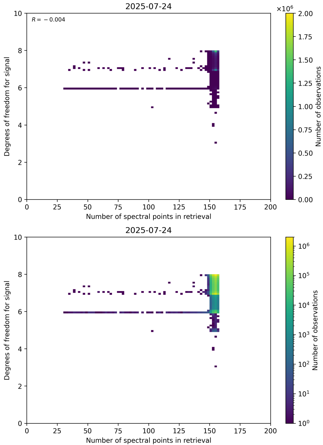
Figure 59: Scatter density plot of “Number of spectral points in retrieval” against “Degrees of freedom for signal” for 2025-07-24 to 2025-07-25.
