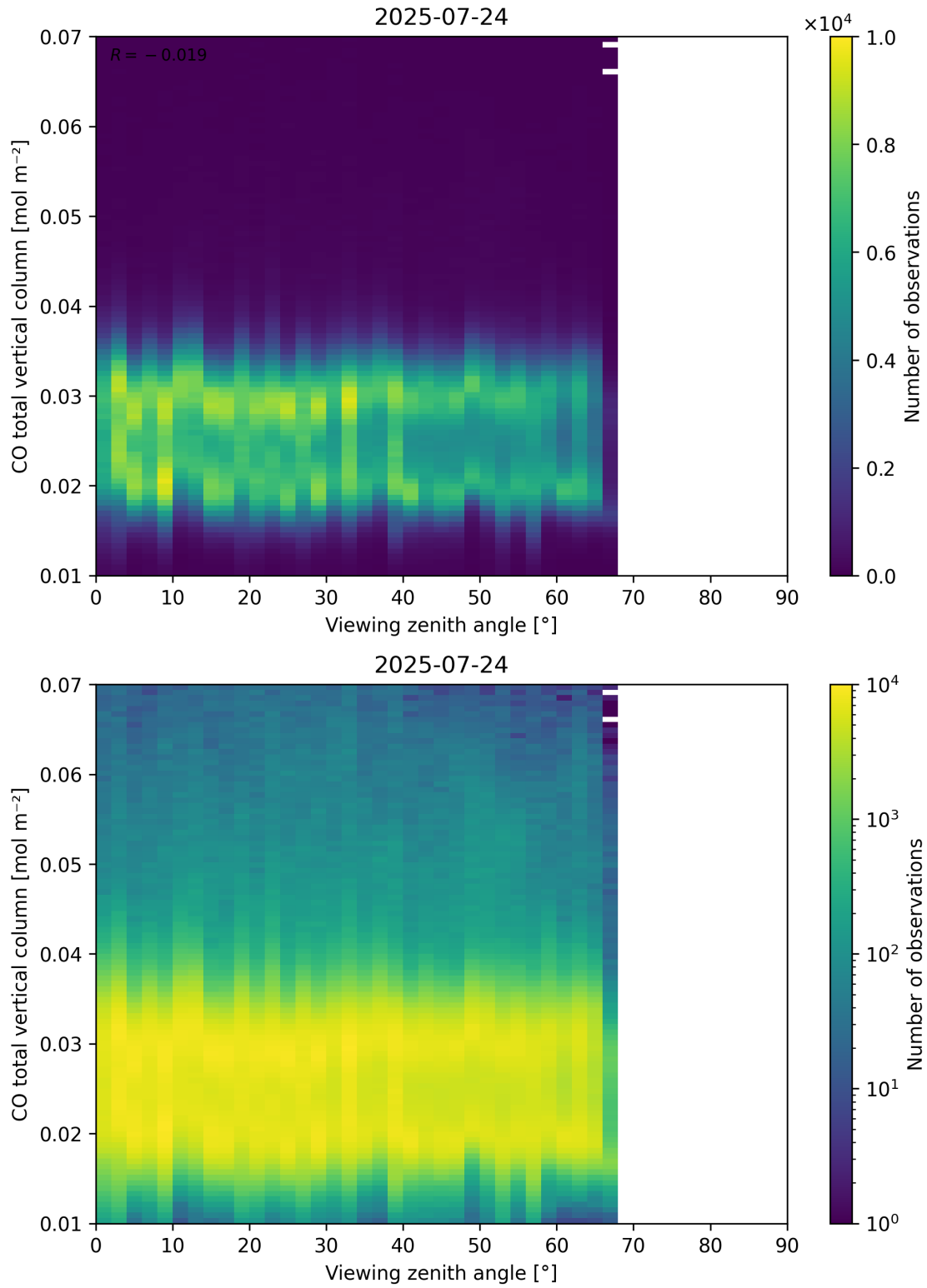
Figure 69: Scatter density plot of “Viewing zenith angle” against “CO total vertical column” for 2025-07-24 to 2025-07-25.
