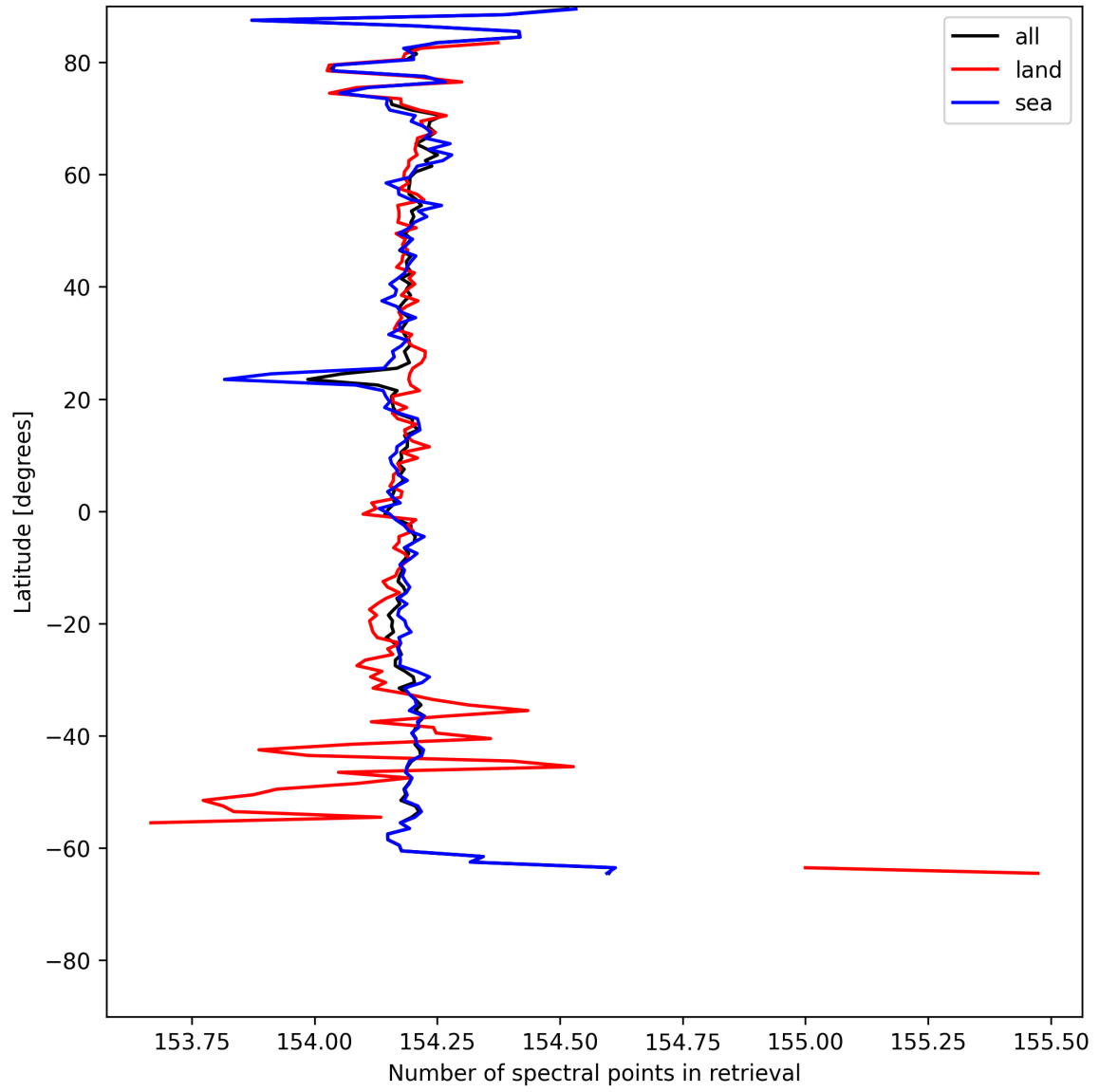
Figure 13: Zonal average of “Number of spectral points in retrieval” for 2025-07-24 to 2025-07-25.
