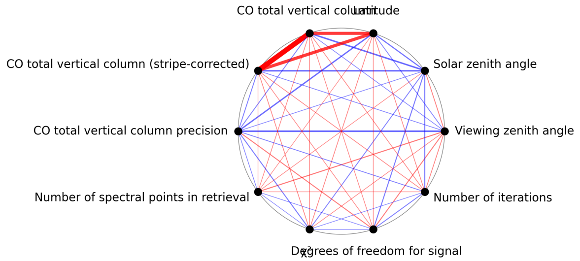
Figure 1: Map of correlation graph for 2025-07-24 to 2025-07-25.
