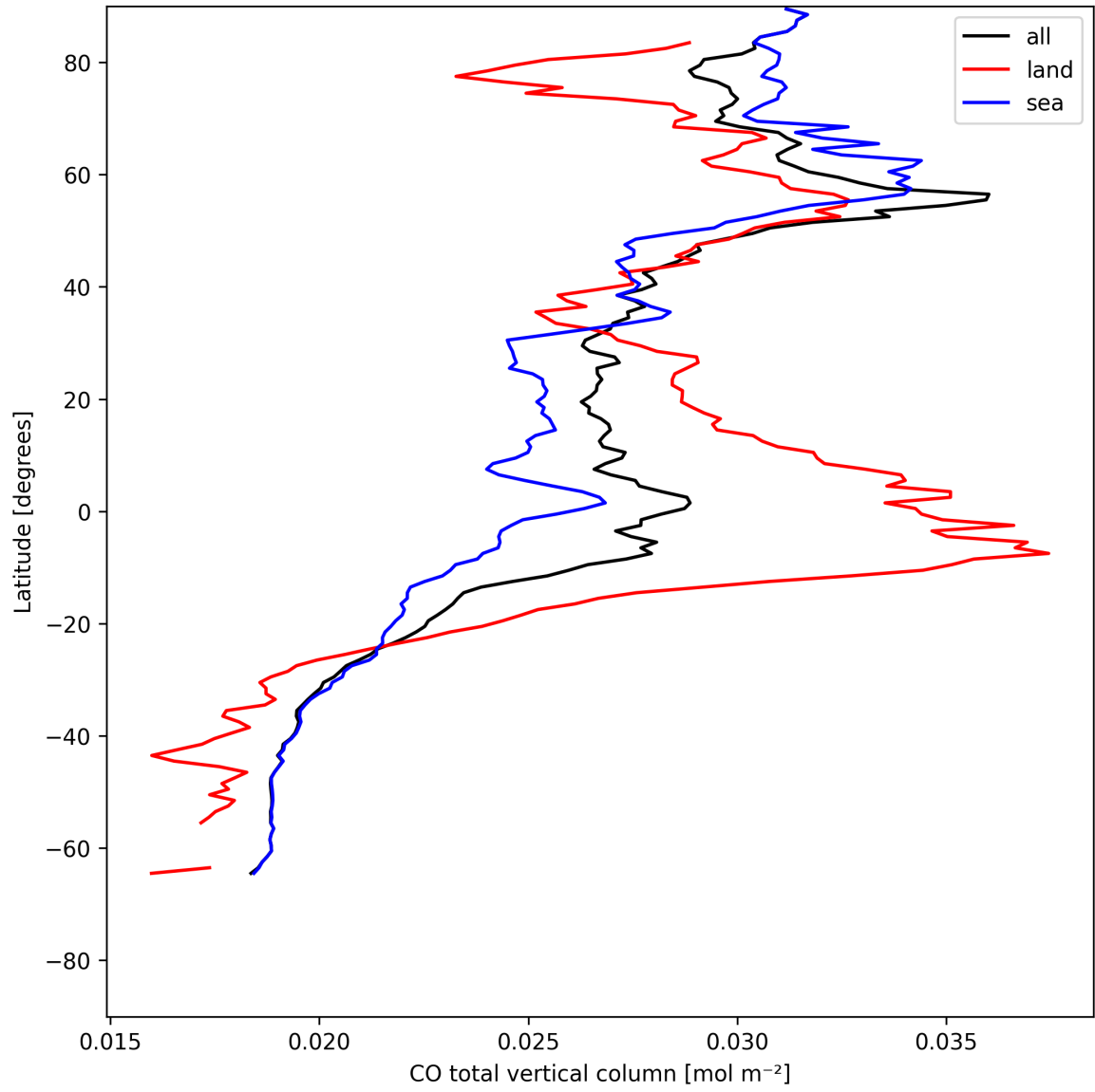
Figure 10: Zonal average of “CO total vertical column” for 2025-07-24 to 2025-07-25.
