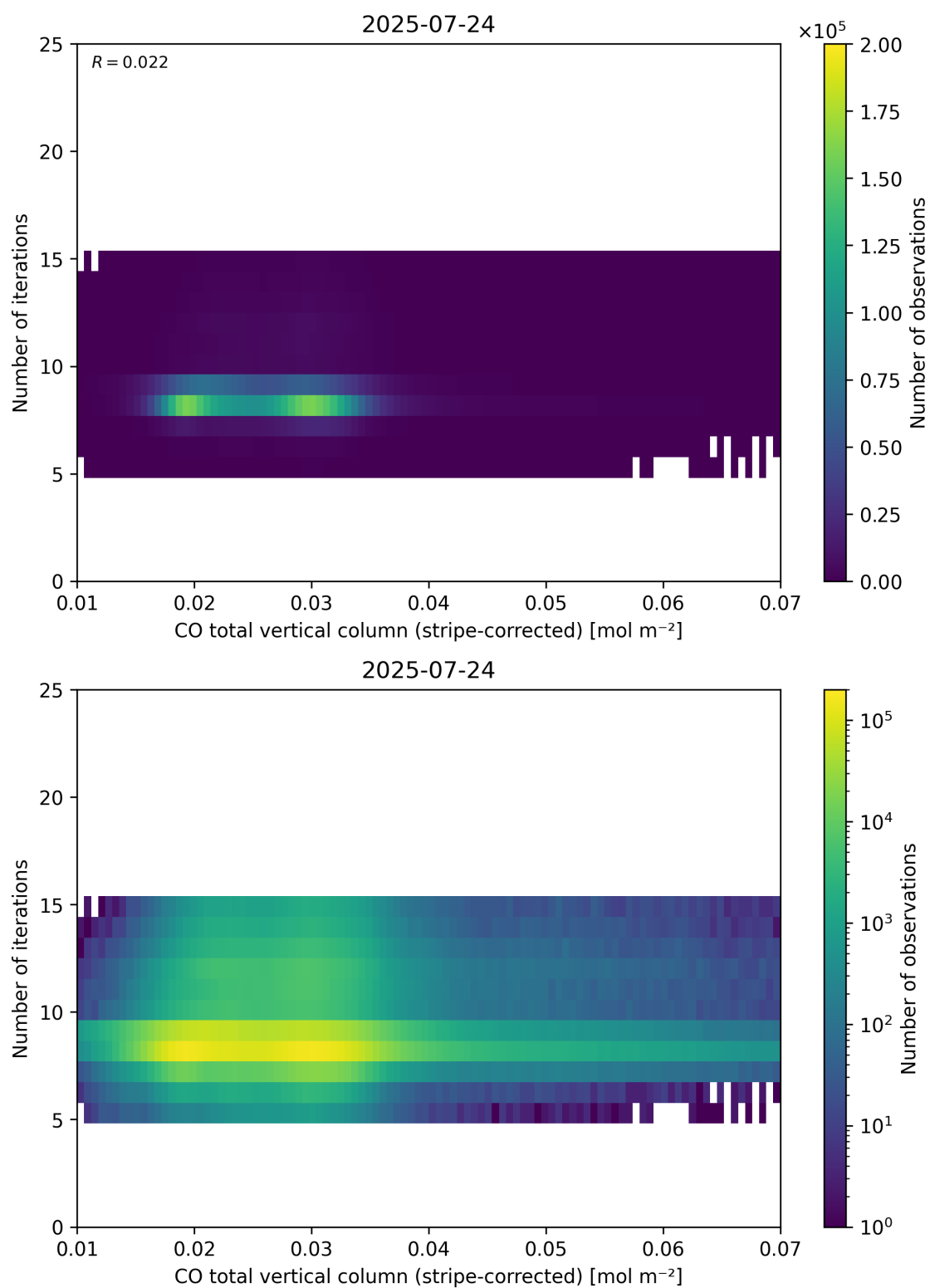
Figure 39: Scatter density plot of “CO total vertical column (stripe-corrected)” against “Number of iterations” for 2025-07-24 to 2025-07-25.
