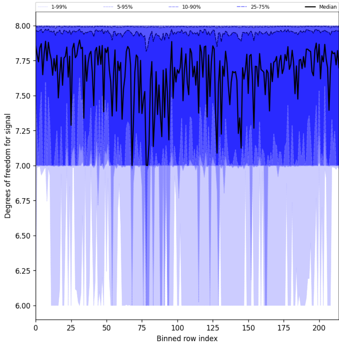
Figure 31: Along track statistics of “Degrees of freedom for signal” for 2025-07-24 to 2025-07-25
