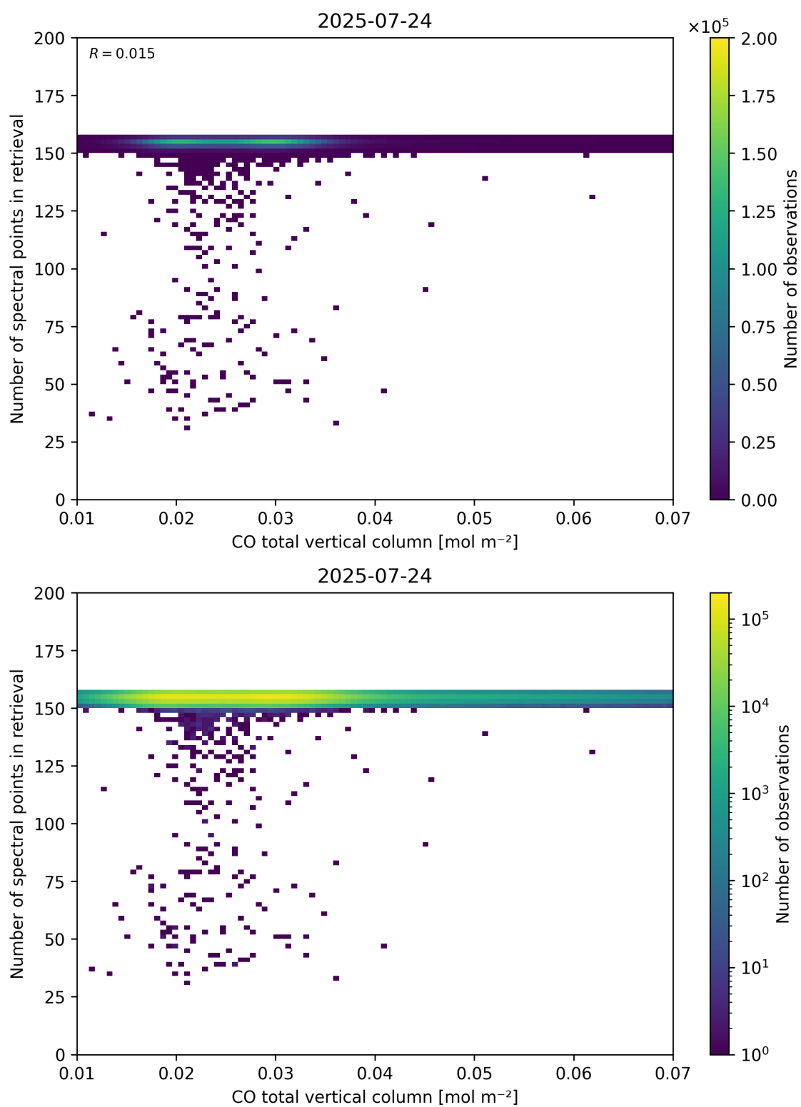
Figure 43: Scatter density plot of “CO total vertical column” against “Number of spectral points in retrieval” for 2025-07-24 to 2025-07-25.
