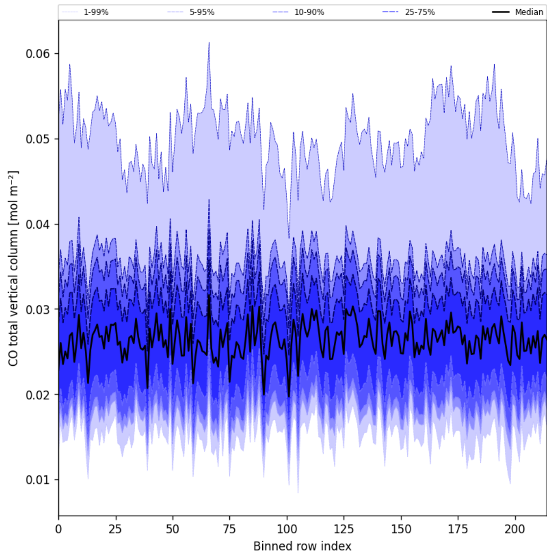
Figure 26: Along track statistics of “CO total vertical column” for 2025-07-24 to 2025-07-25
