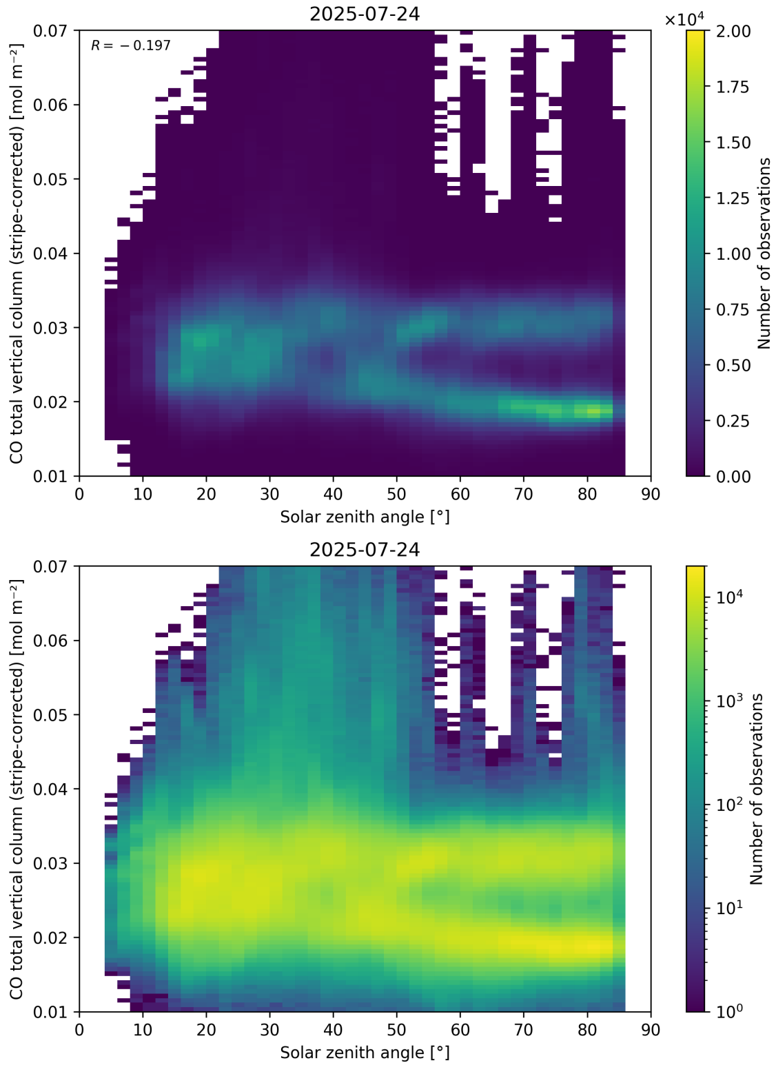
Figure 62: Scatter density plot of “Solar zenith angle” against “CO total vertical column (stripe-corrected)” for 2025-07-24 to 2025-07-25.
