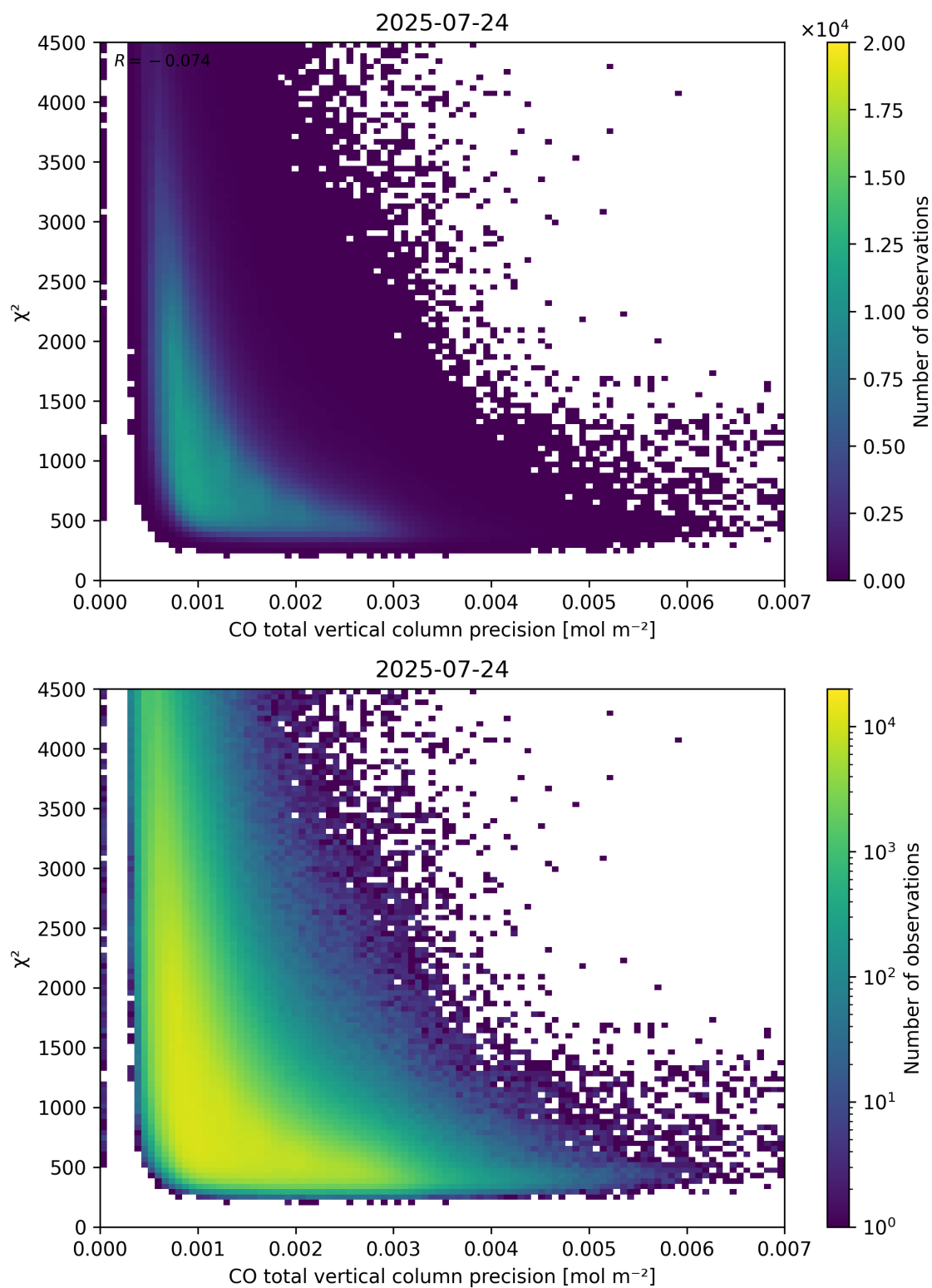
Figure 44: Scatter density plot of “CO total vertical column precision” against “ \chi^2 ” for 2025-07-24 to 2025-07-25.
