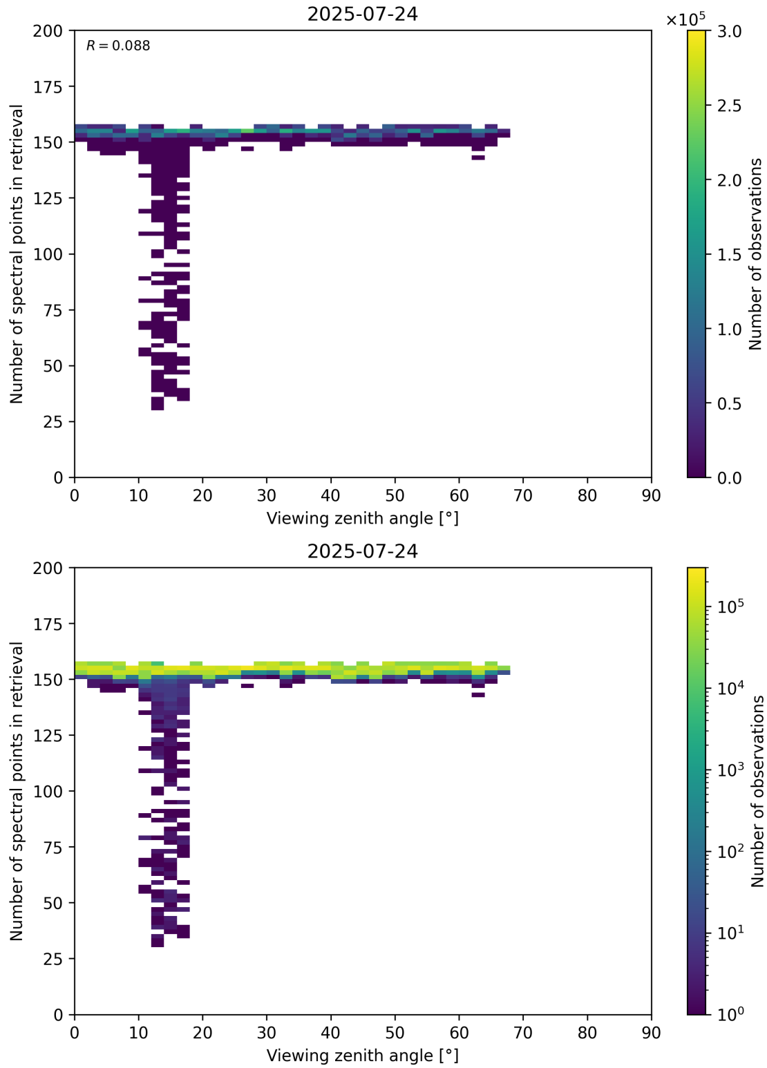
Figure 76: Scatter density plot of “Viewing zenith angle” against “Number of spectral points in retrieval” for 2025-07-24 to 2025-07-25.
