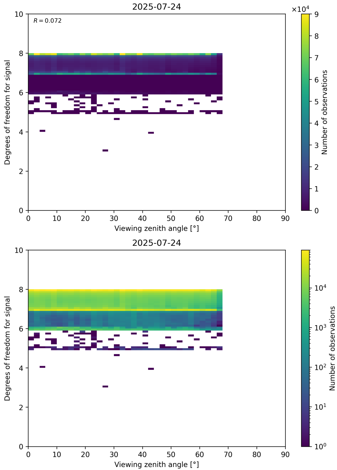
Figure 73: Scatter density plot of “Viewing zenith angle” against “Degrees of freedom for signal” for 2025-07-24 to 2025-07-25.
