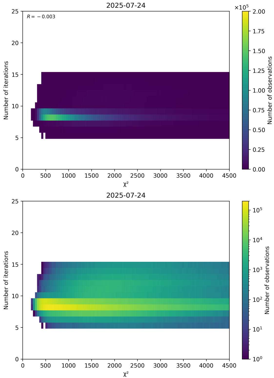
Figure 49: Scatter density plot of “ \chi^2 ” against “Number of iterations” for 2025-07-24 to 2025-07-25.
