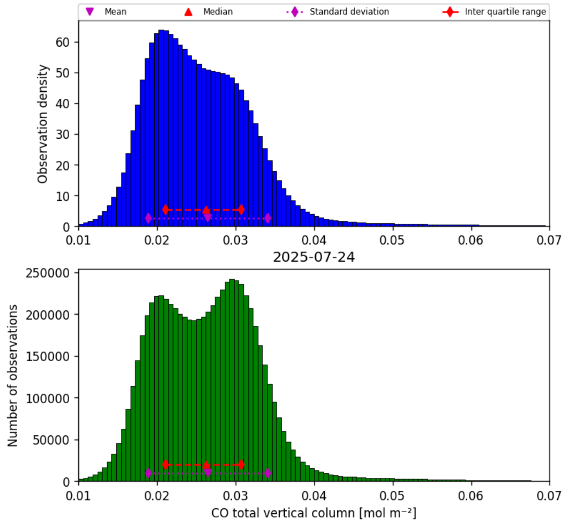
Figure 18: Histogram of “CO total vertical column” for 2025-07-24 to 2025-07-25
