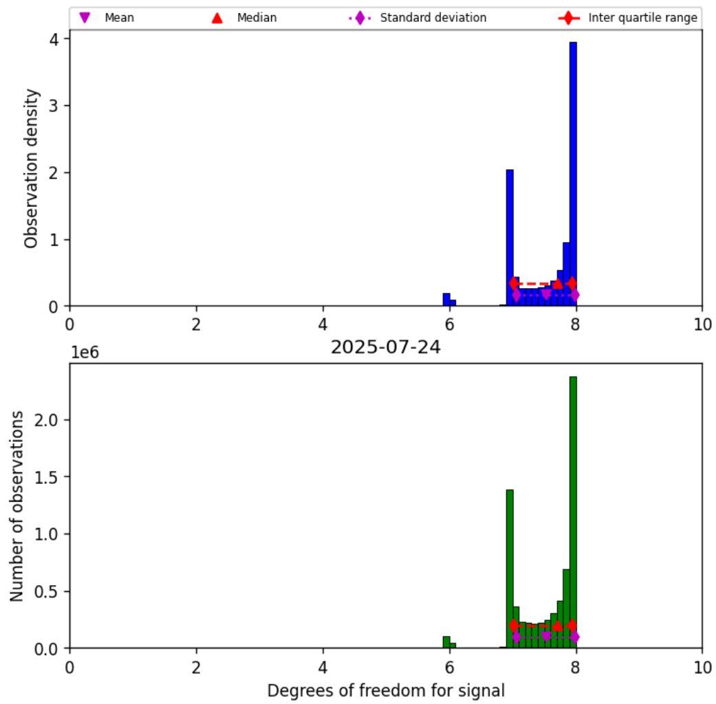
Figure 23: Histogram of “Degrees of freedom for signal” for 2025-07-24 to 2025-07-25
