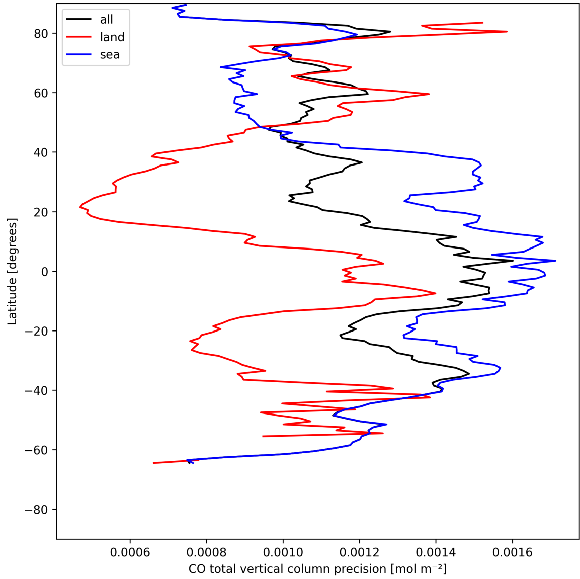
Figure 12: Zonal average of “CO total vertical column precision” for 2025-07-24 to 2025-07-25.
