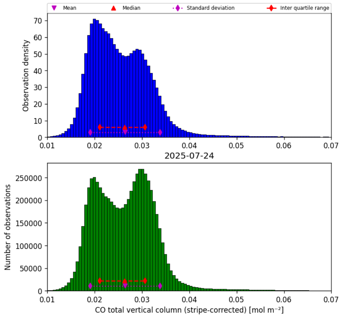
Figure 19: Histogram of “CO total vertical column (stripe-corrected)” for 2025-07-24 to 2025-07-25
