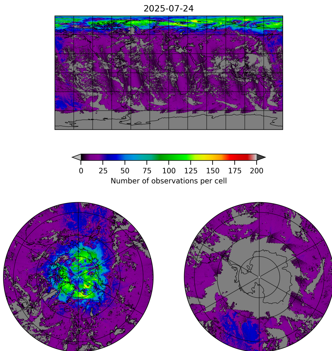
Figure 8: Map of the number of observations for 2025-07-24 to 2025-07-25
