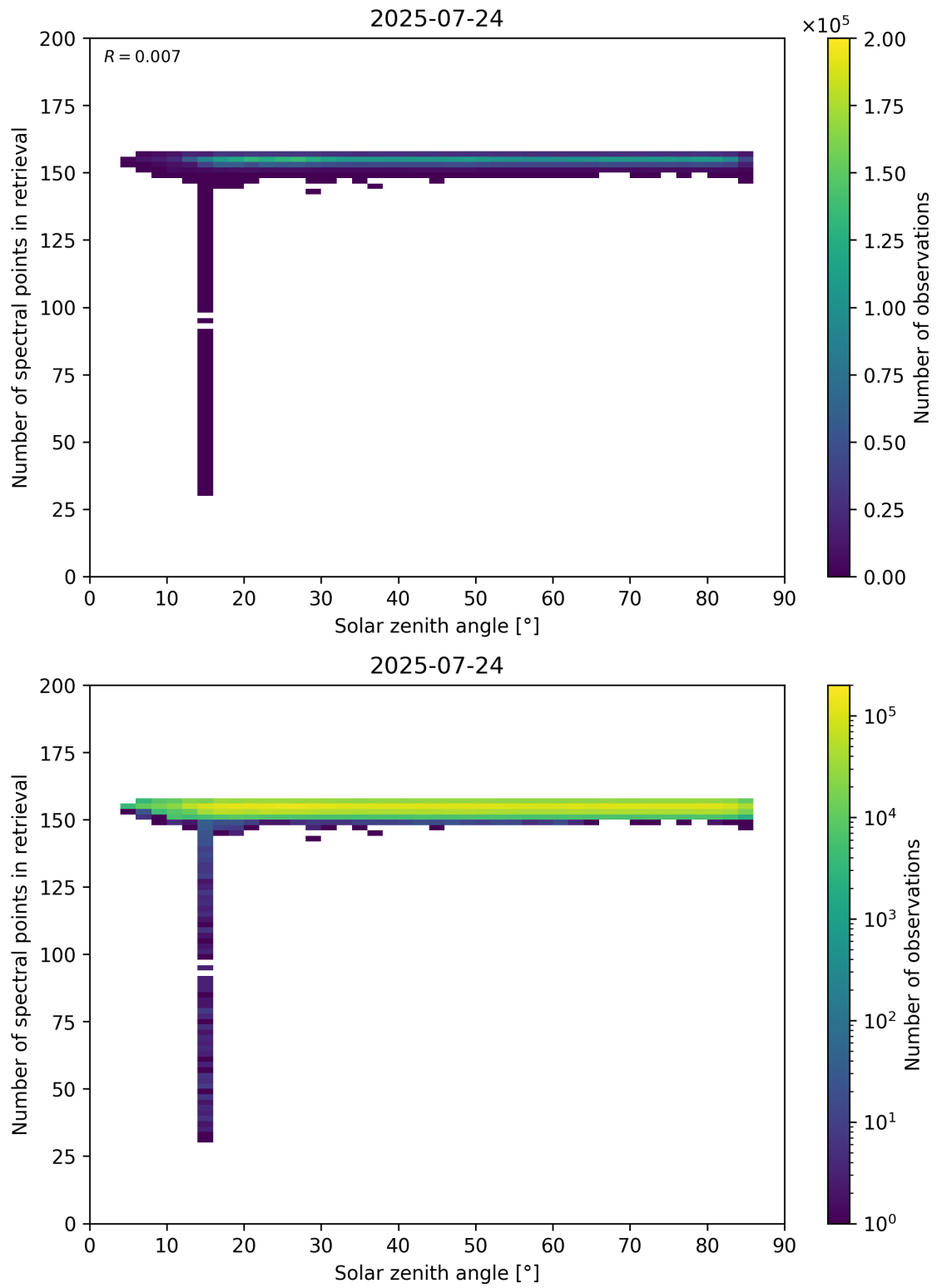
Figure 68: Scatter density plot of “Solar zenith angle” against “Number of spectral points in retrieval” for 2025-07-24 to 2025-07-25.
