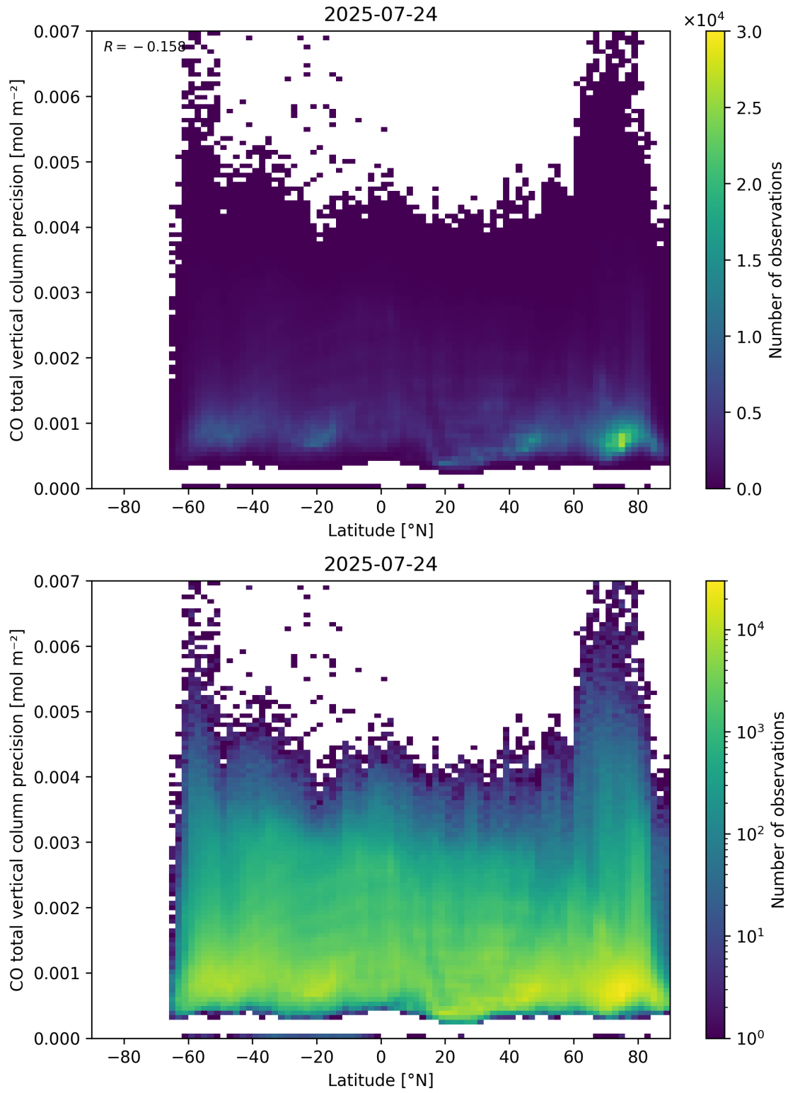
Figure 53: Scatter density plot of “Latitude” against “CO total vertical column precision” for 2025-07-24 to 2025-07-25.
