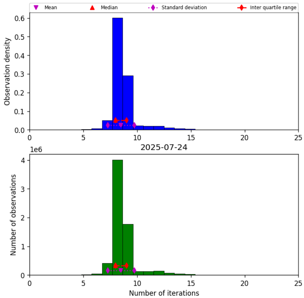
Figure 24: Histogram of “Number of iterations” for 2025-07-24 to 2025-07-25
