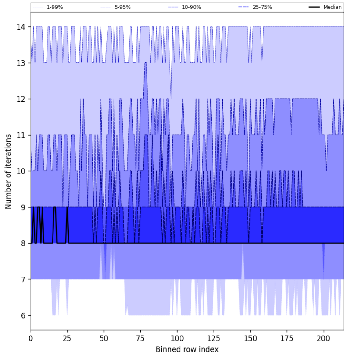
Figure 32: Along track statistics of “Number of iterations” for 2025-07-24 to 2025-07-25
