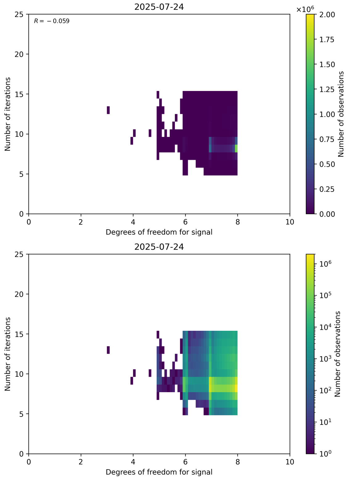
Figure 50: Scatter density plot of “Degrees of freedom for signal” against “Number of iterations” for 2025-07-24 to 2025-07-25.
