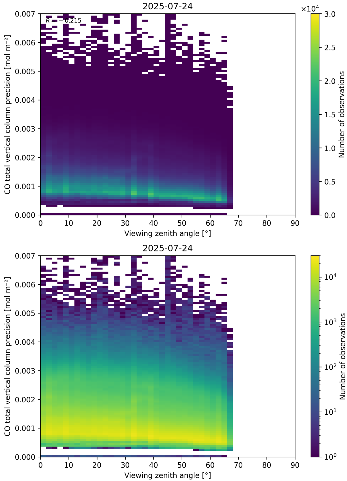
Figure 71: Scatter density plot of “Viewing zenith angle” against “CO total vertical column precision” for 2025-07-24 to 2025-07-25.
