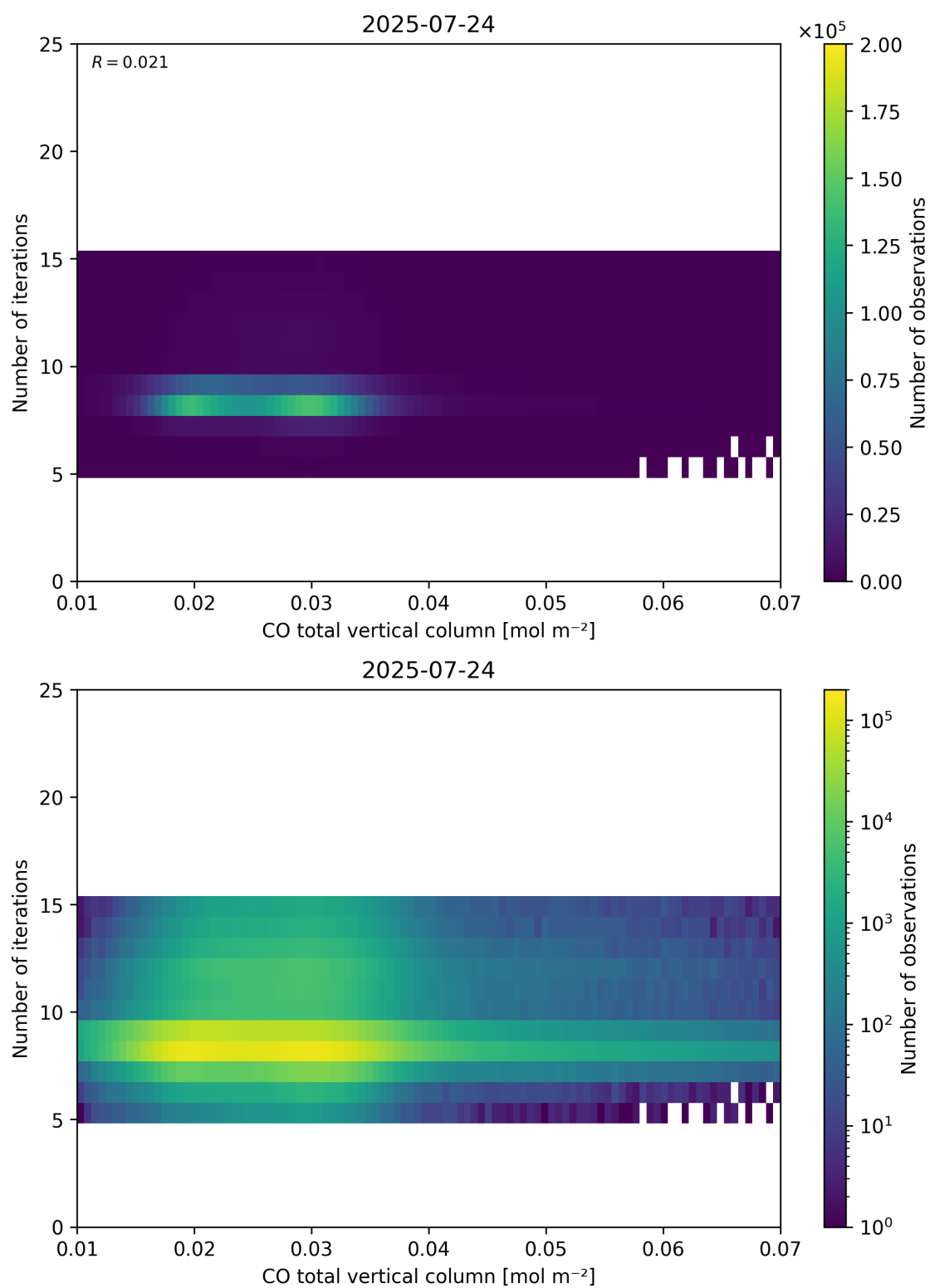
Figure 42: Scatter density plot of “CO total vertical column” against “Number of iterations” for 2025-07-24 to 2025-07-25.
