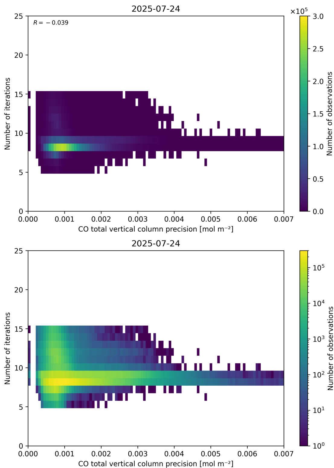
Figure 46: Scatter density plot of “CO total vertical column precision” against “Number of iterations” for 2025-07-24 to 2025-07-25.
