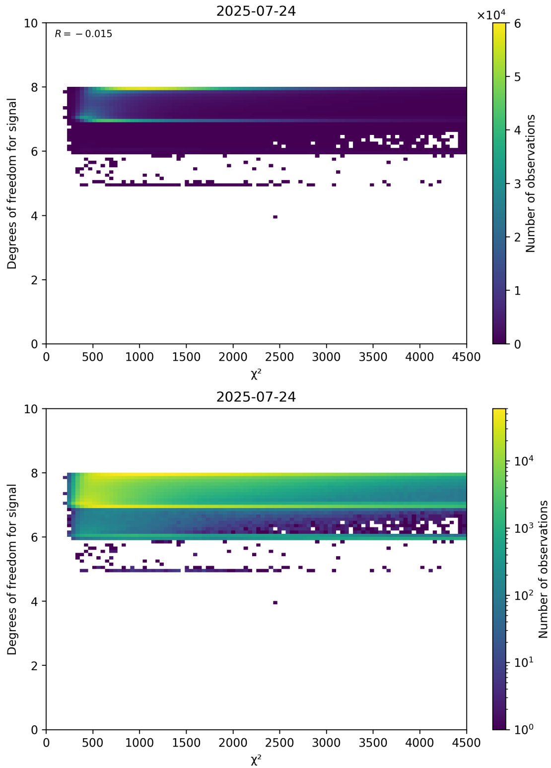
Figure 48: Scatter density plot of " \chi^2 " against "Degrees of freedom for signal" for 2025-07-24 to 2025-07-25.
