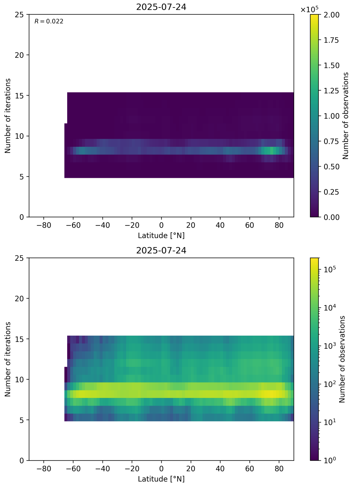
Figure 56: Scatter density plot of “Latitude” against “Number of iterations” for 2025-07-24 to 2025-07-25.
