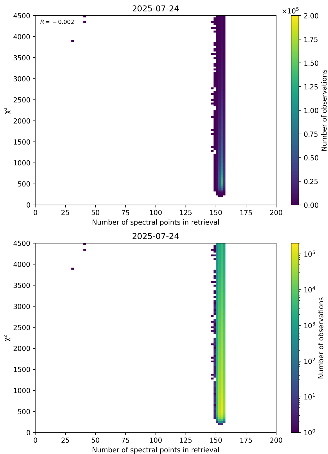
Figure 58: Scatter density plot of “Number of spectral points in retrieval” against “ \chi^2 ” for 2025-07-24 to 2025-07-25.
