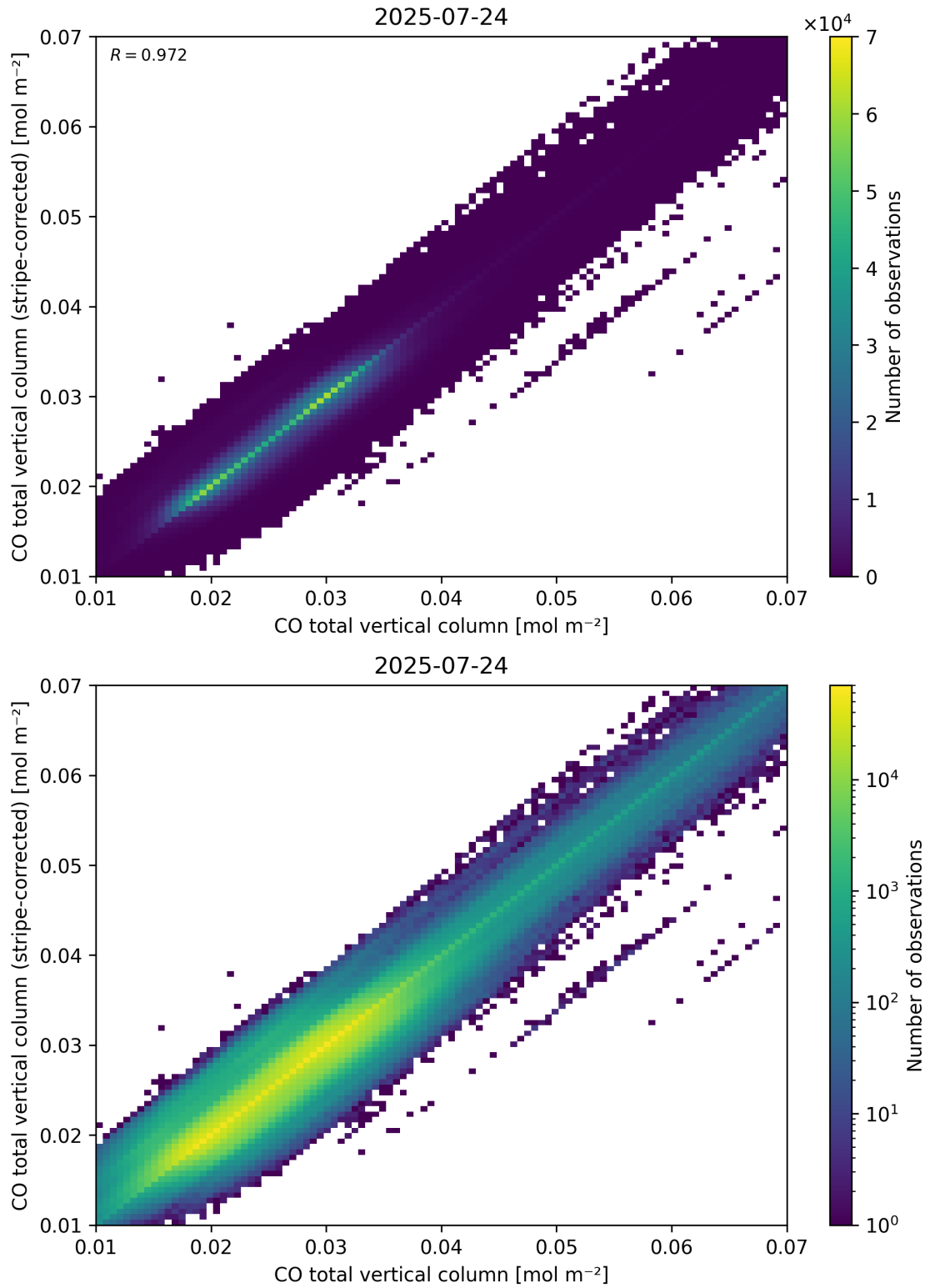
Figure 33: Scatter density plot of “CO total vertical column” against “CO total vertical column (stripe-corrected)” for 2025-07-24 to 2025-07-25.
