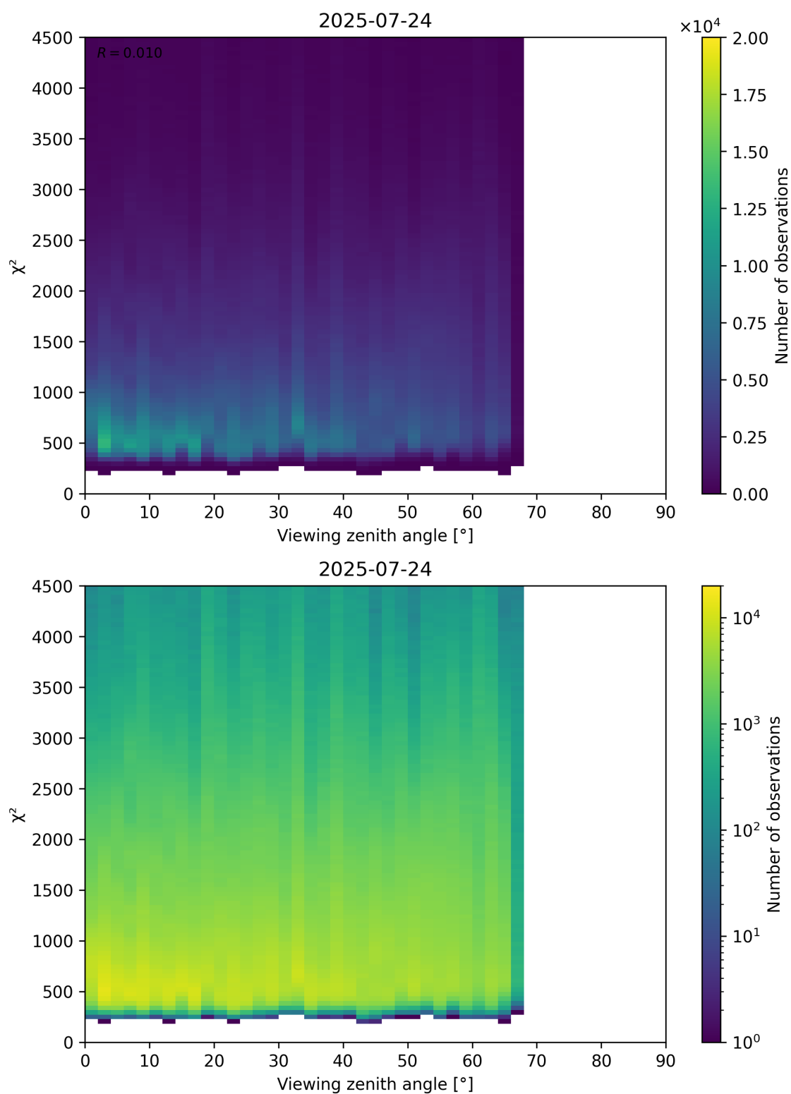
Figure 72: Scatter density plot of “Viewing zenith angle” against “ \chi^2 ” for 2025-07-24 to 2025-07-25.
