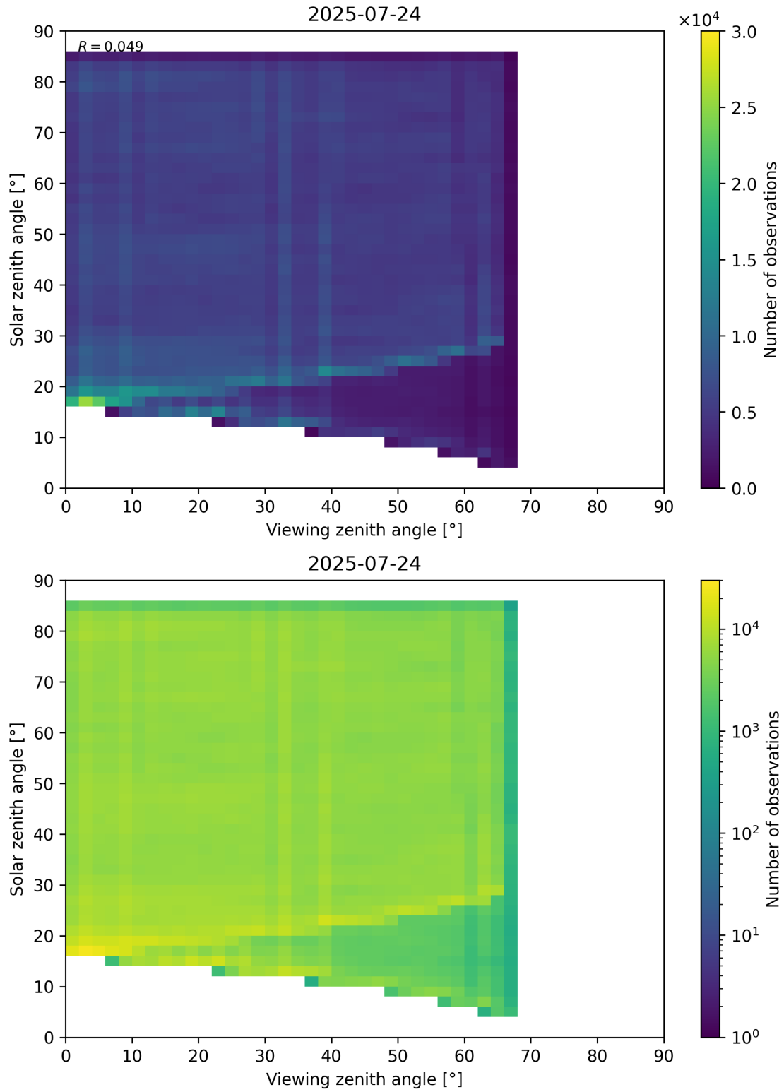
Figure 77: Scatter density plot of “Viewing zenith angle” against “Solar zenith angle” for 2025-07-24 to 2025-07-25.
