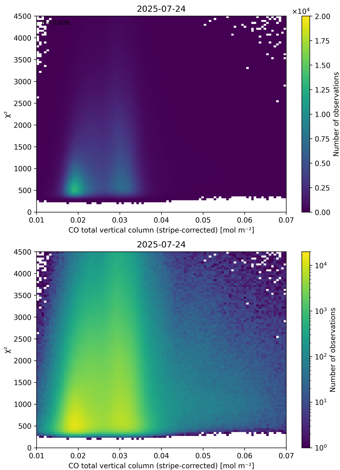
Figure 37: Scatter density plot of “CO total vertical column (stripe-corrected)” against “ \chi^2 ” for 2025-07-24 to 2025-07-25.
