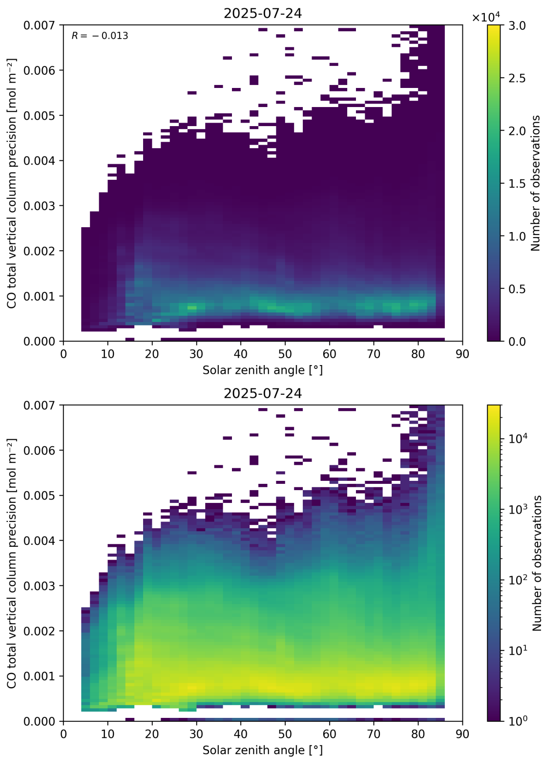
Figure 63: Scatter density plot of “Solar zenith angle” against “CO total vertical column precision” for 2025-07-24 to 2025-07-25.
