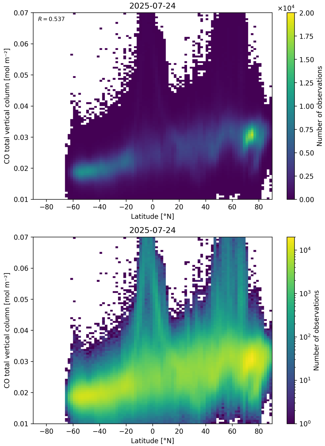
Figure 51: Scatter density plot of “Latitude” against “CO total vertical column” for 2025-07-24 to 2025-07-25.
