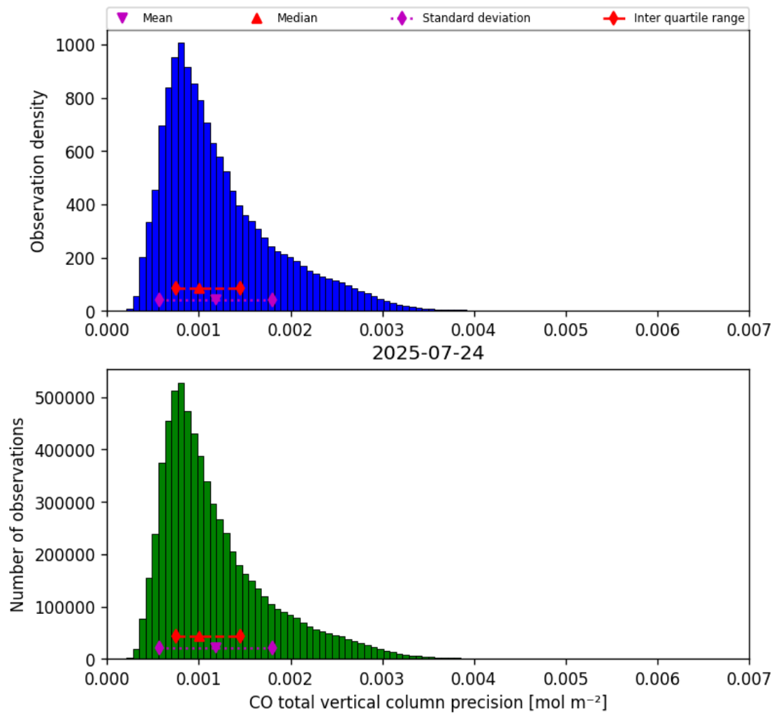
Figure 20: Histogram of “CO total vertical column precision” for 2025-07-24 to 2025-07-25
