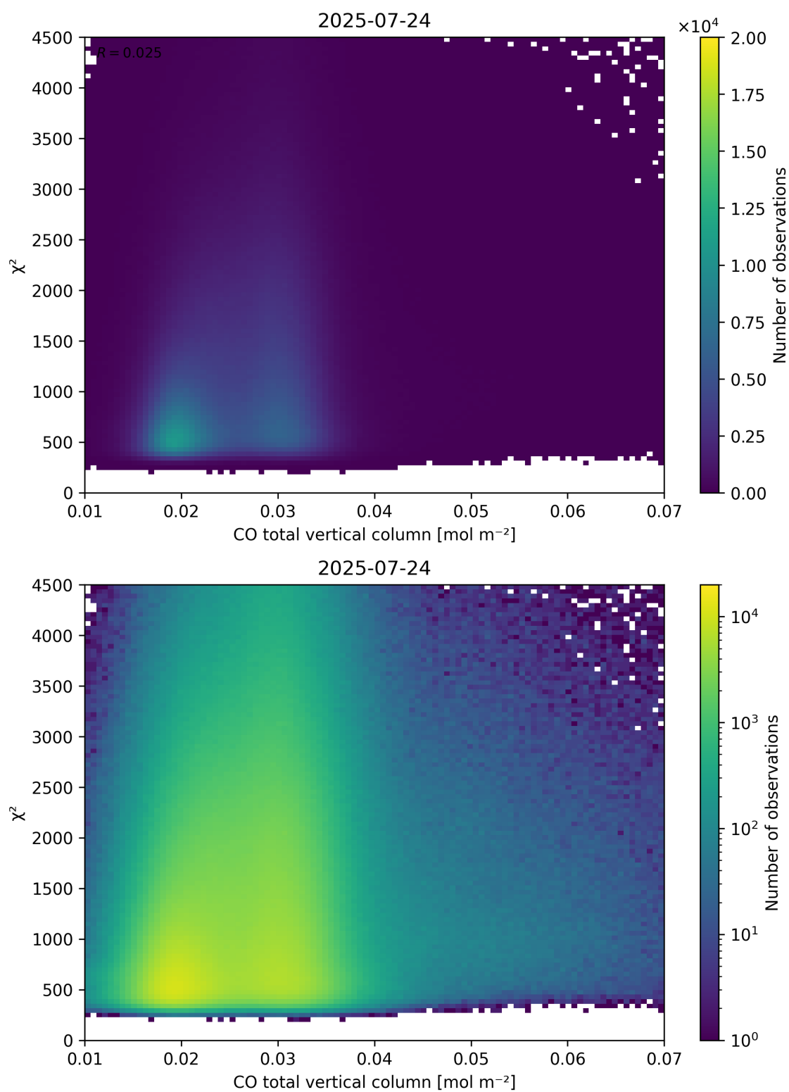
Figure 35: Scatter density plot of “CO total vertical column” against “ \chi^2 ” for 2025-07-24 to 2025-07-25.
