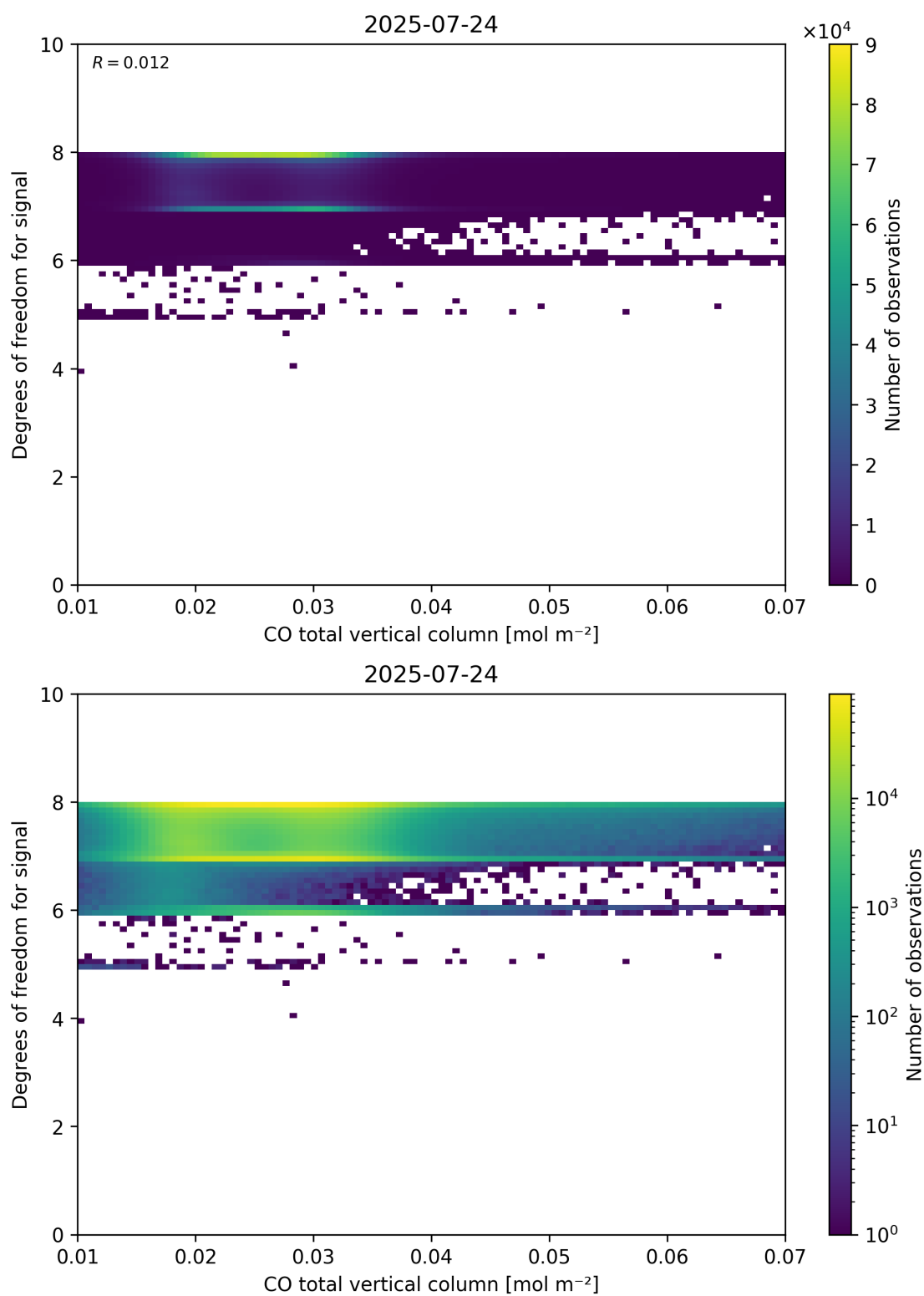
Figure 41: Scatter density plot of “CO total vertical column” against “Degrees of freedom for signal” for 2025-07-24 to 2025-07-25.
