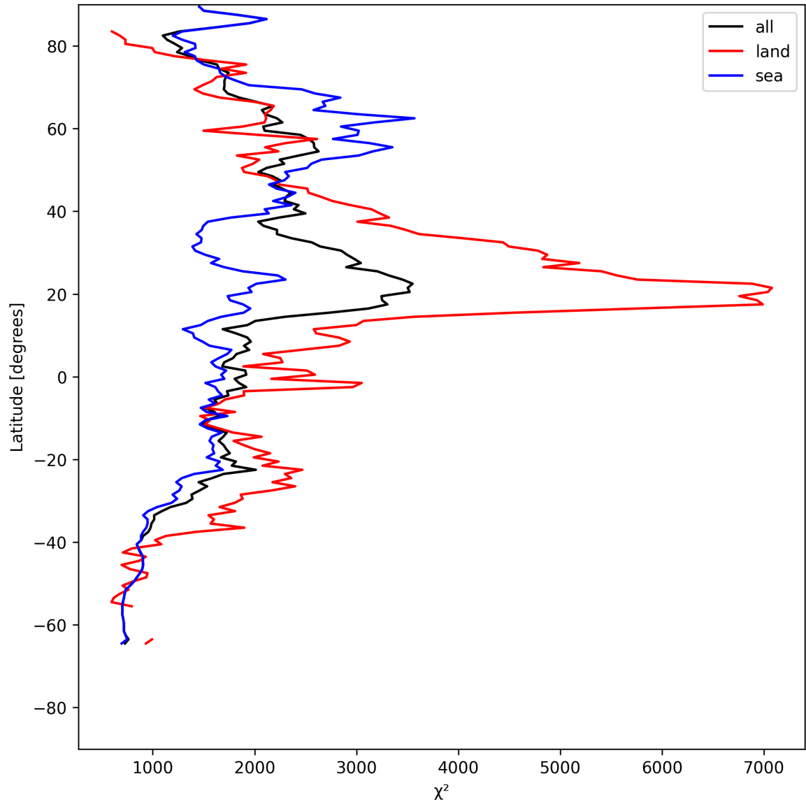
Figure 14: Zonal average of “ \chi^2 ” for 2025-07-24 to 2025-07-25.
