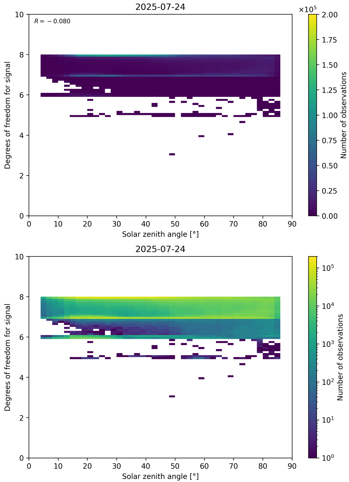
Figure 65: Scatter density plot of “Solar zenith angle” against “Degrees of freedom for signal” for 2025-07-24 to 2025-07-25.
