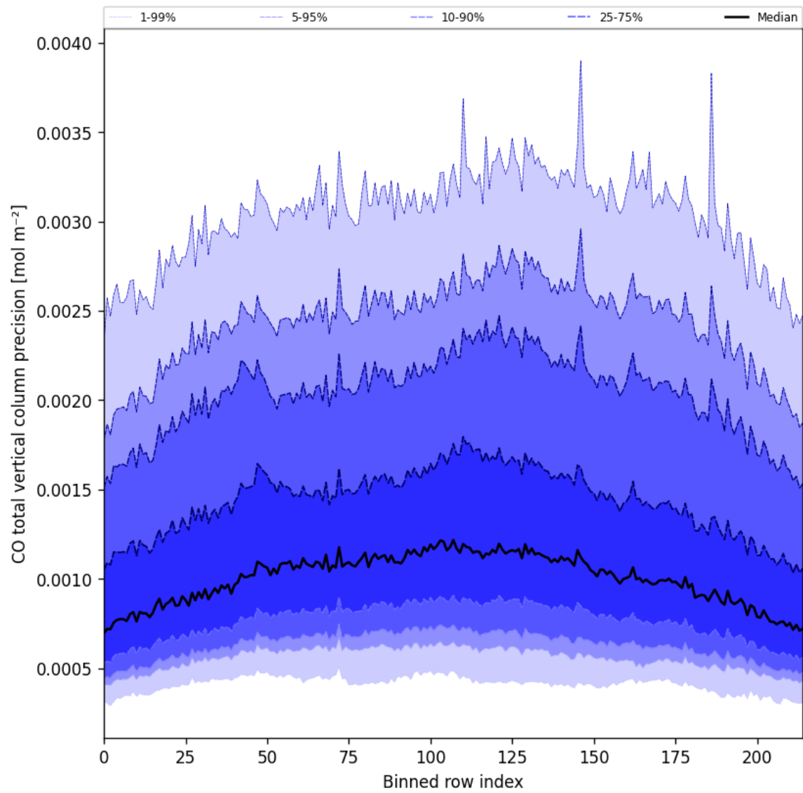
Figure 28: Along track statistics of “CO total vertical column precision” for 2025-07-24 to 2025-07-25
