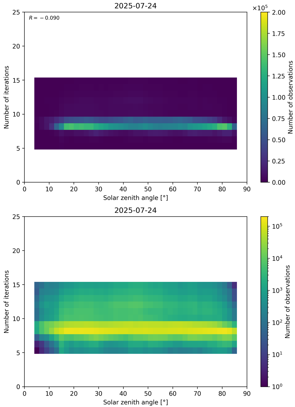
Figure 67: Scatter density plot of “Solar zenith angle” against “Number of iterations” for 2025-07-24 to 2025-07-25.
