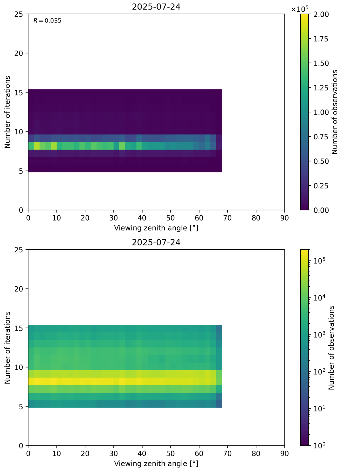
Figure 75: Scatter density plot of “Viewing zenith angle” against “Number of iterations” for 2025-07-24 to 2025-07-25.
