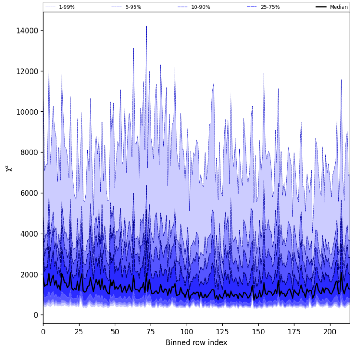
Figure 30: Along track statistics of “ \chi^2 ” for 2025-07-24 to 2025-07-25
