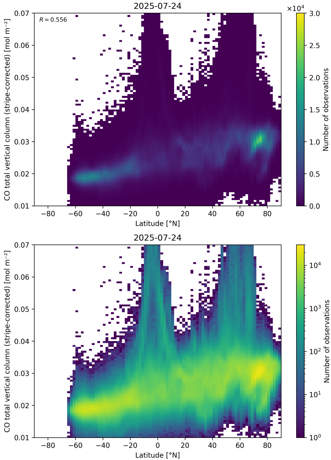
Figure 52: Scatter density plot of “Latitude” against “CO total vertical column (stripe-corrected)” for 2025-07-24 to 2025-07-25.
