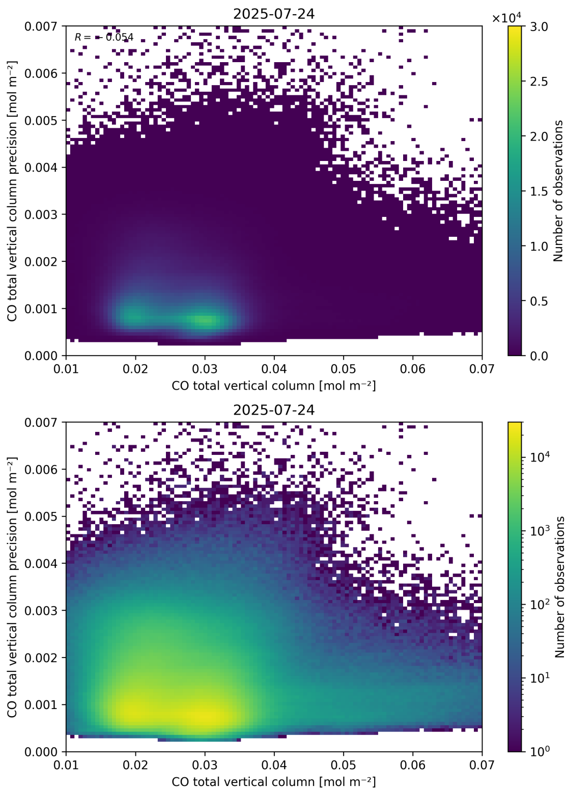
Figure 34: Scatter density plot of “CO total vertical column” against “CO total vertical column precision” for 2025-07-24 to 2025-07-25.
