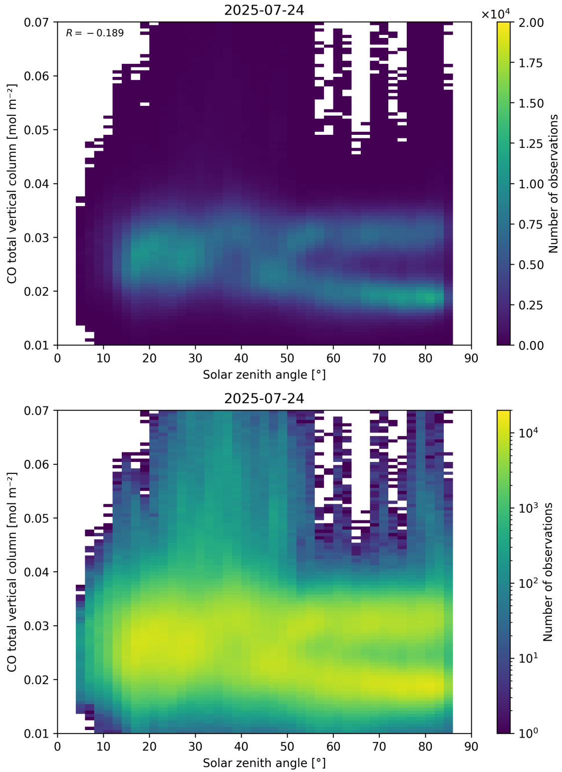
Figure 61: Scatter density plot of “Solar zenith angle” against “CO total vertical column” for 2025-07-24 to 2025-07-25.
