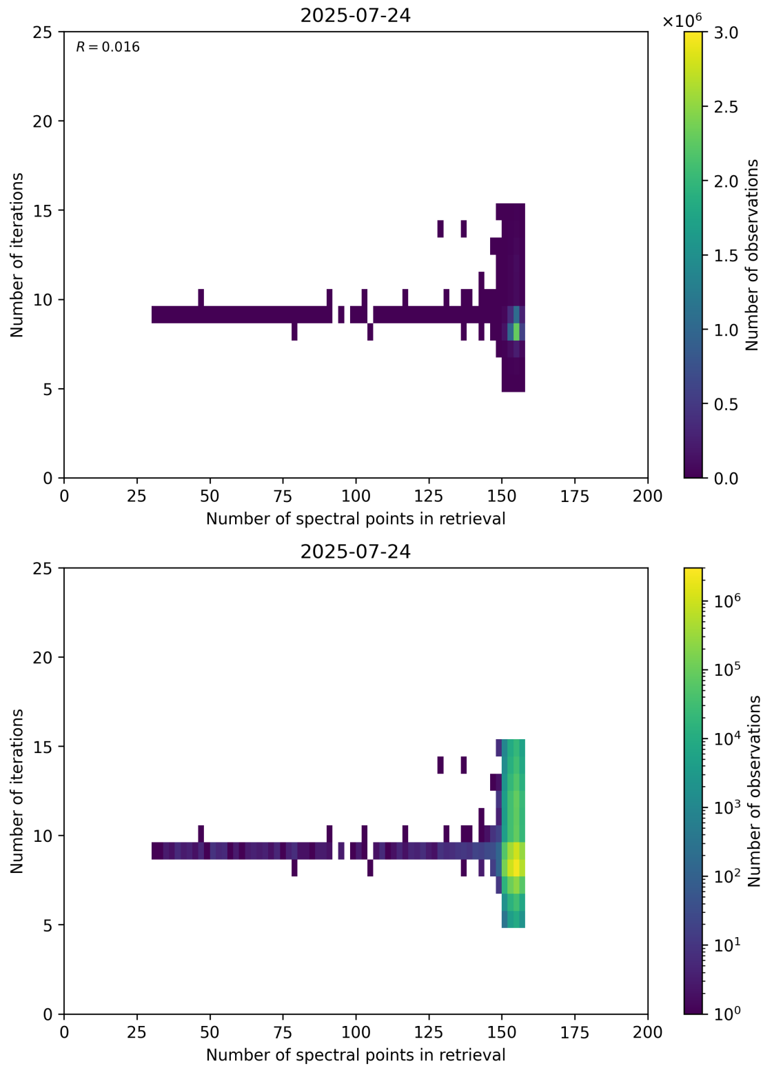
Figure 60: Scatter density plot of “Number of spectral points in retrieval” against “Number of iterations” for 2025-07-24 to 2025-07-25.
