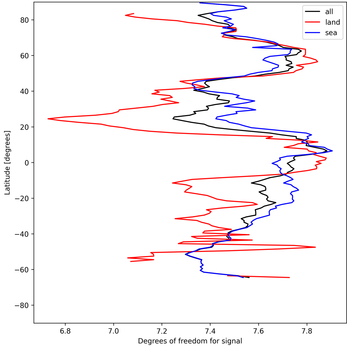
Figure 15: Zonal average of “Degrees of freedom for signal” for 2025-07-24 to 2025-07-25.
