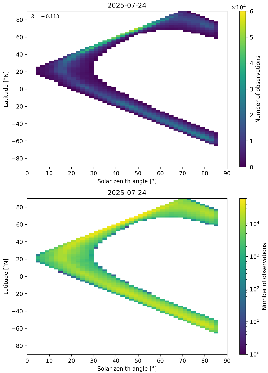
Figure 66: Scatter density plot of “Solar zenith angle” against “Latitude” for 2025-07-24 to 2025-07-25.
