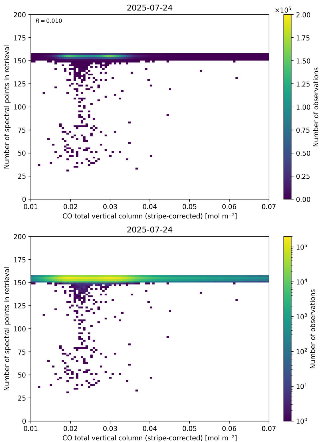
Figure 40: Scatter density plot of “CO total vertical column (stripe-corrected)” against “Number of spectral points in retrieval” for 2025-07-24 to 2025-07-25.
