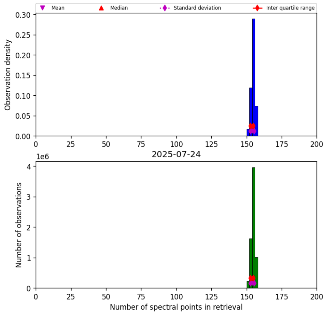
Figure 21: Histogram of “Number of spectral points in retrieval” for 2025-07-24 to 2025-07-25
