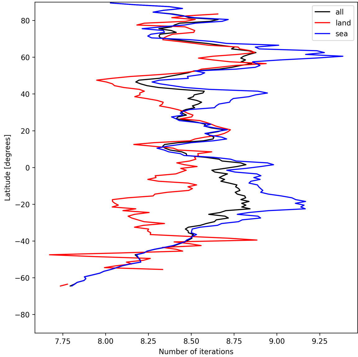
Figure 16: Zonal average of “Number of iterations” for 2025-07-24 to 2025-07-25.
