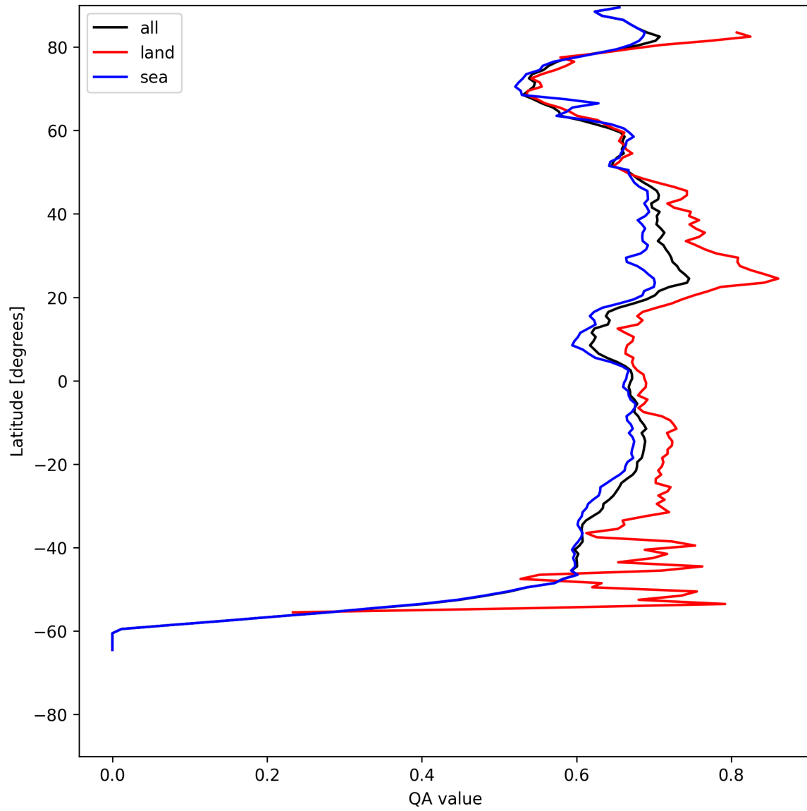
Figure 9: Zonal average of “QA value” for 2025-07-24 to 2025-07-25.
