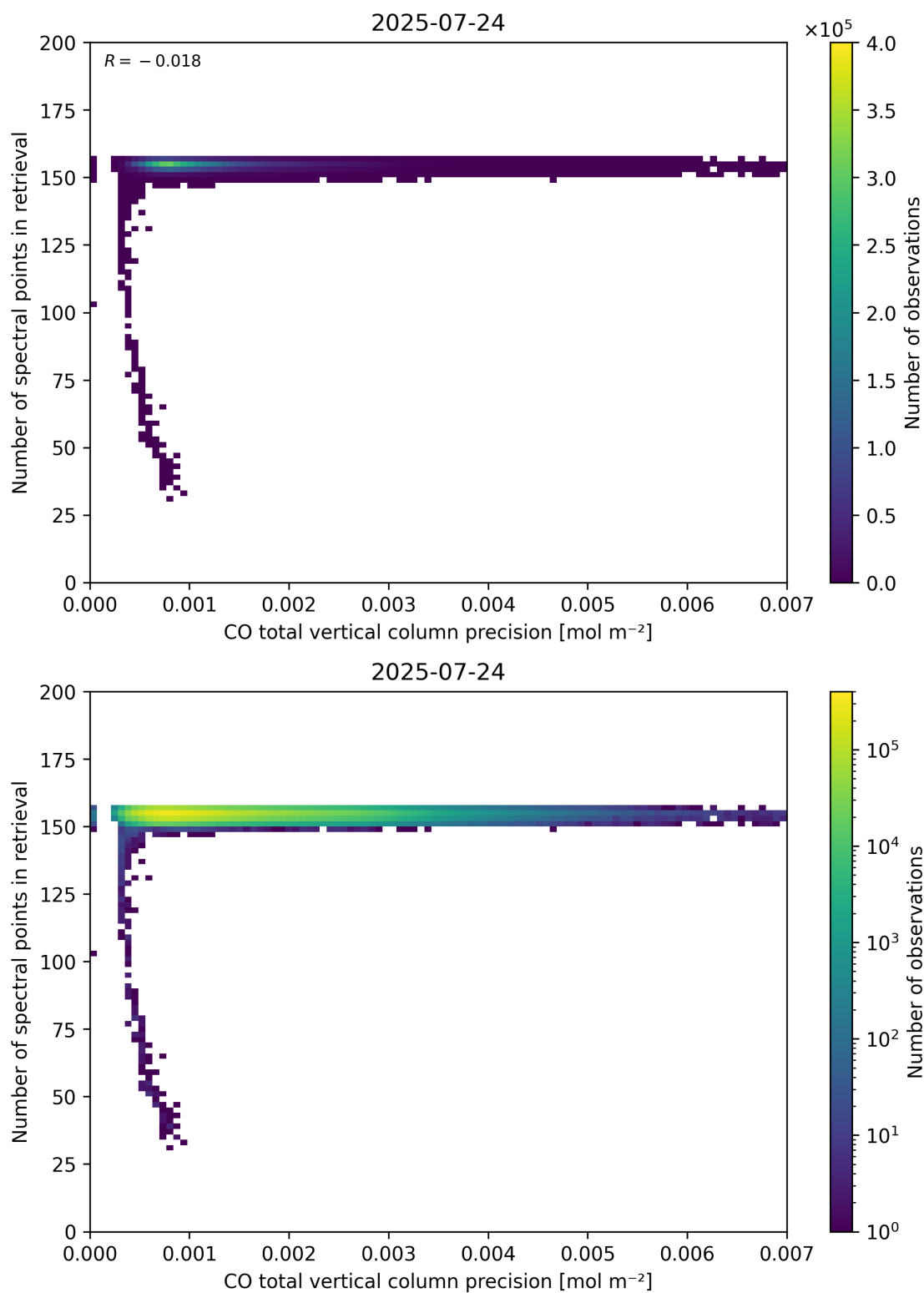
Figure 47: Scatter density plot of “CO total vertical column precision” against “Number of spectral points in retrieval” for 2025-07-24 to 2025-07-25.
