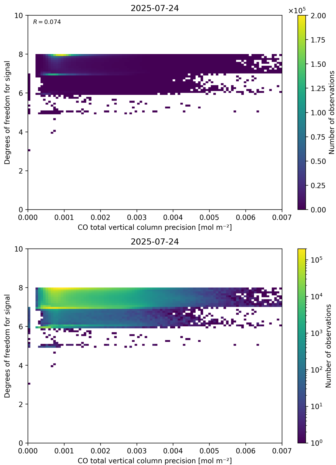
Figure 45: Scatter density plot of “CO total vertical column precision” against “Degrees of freedom for signal” for 2025-07-24 to 2025-07-25.
