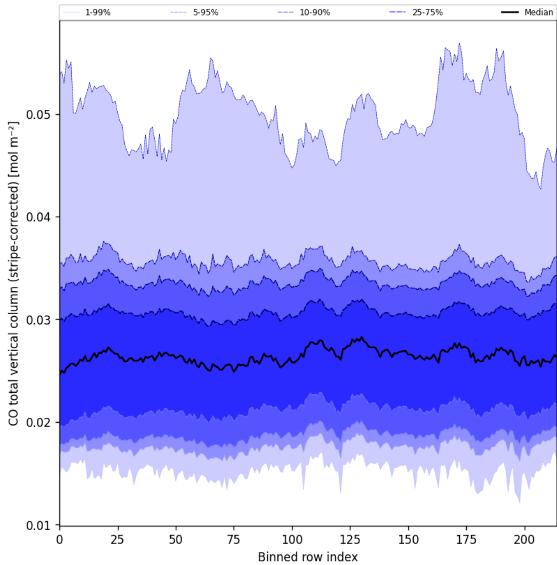
Figure 27: Along track statistics of “CO total vertical column (stripe-corrected)” for 2025-07-24 to 2025-07-25
