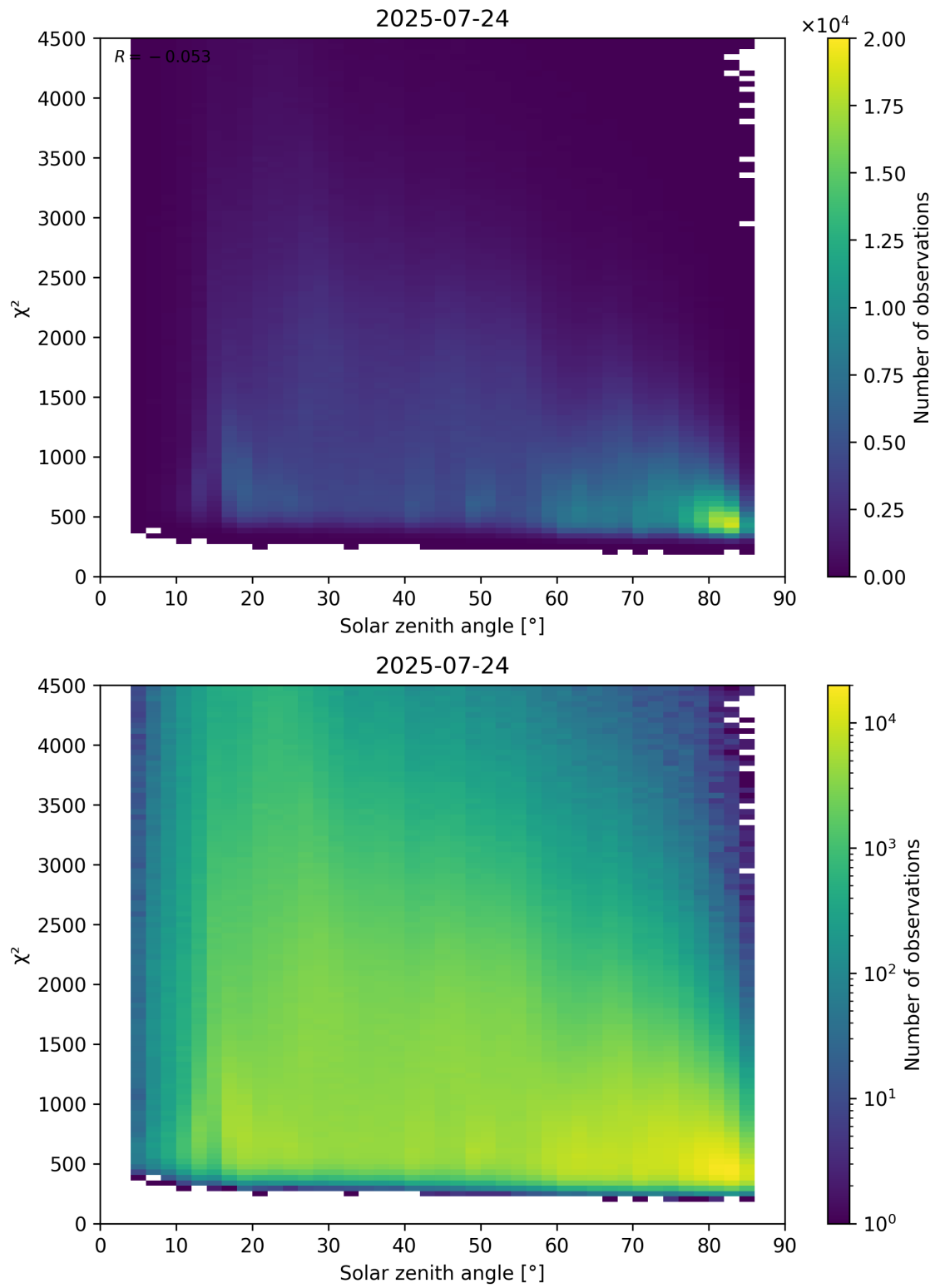
Figure 64: Scatter density plot of “Solar zenith angle” against “ \chi^2 ” for 2025-07-24 to 2025-07-25.
