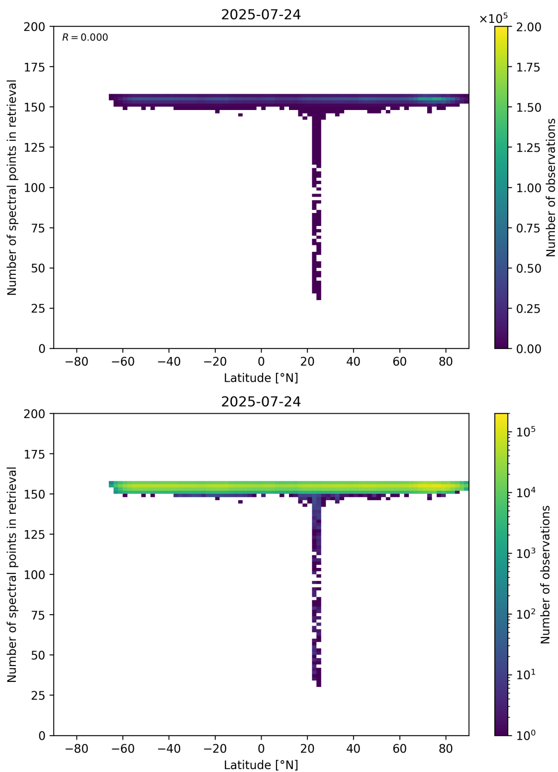
Figure 57: Scatter density plot of “Latitude” against “Number of spectral points in retrieval” for 2025-07-24 to 2025-07-25.
