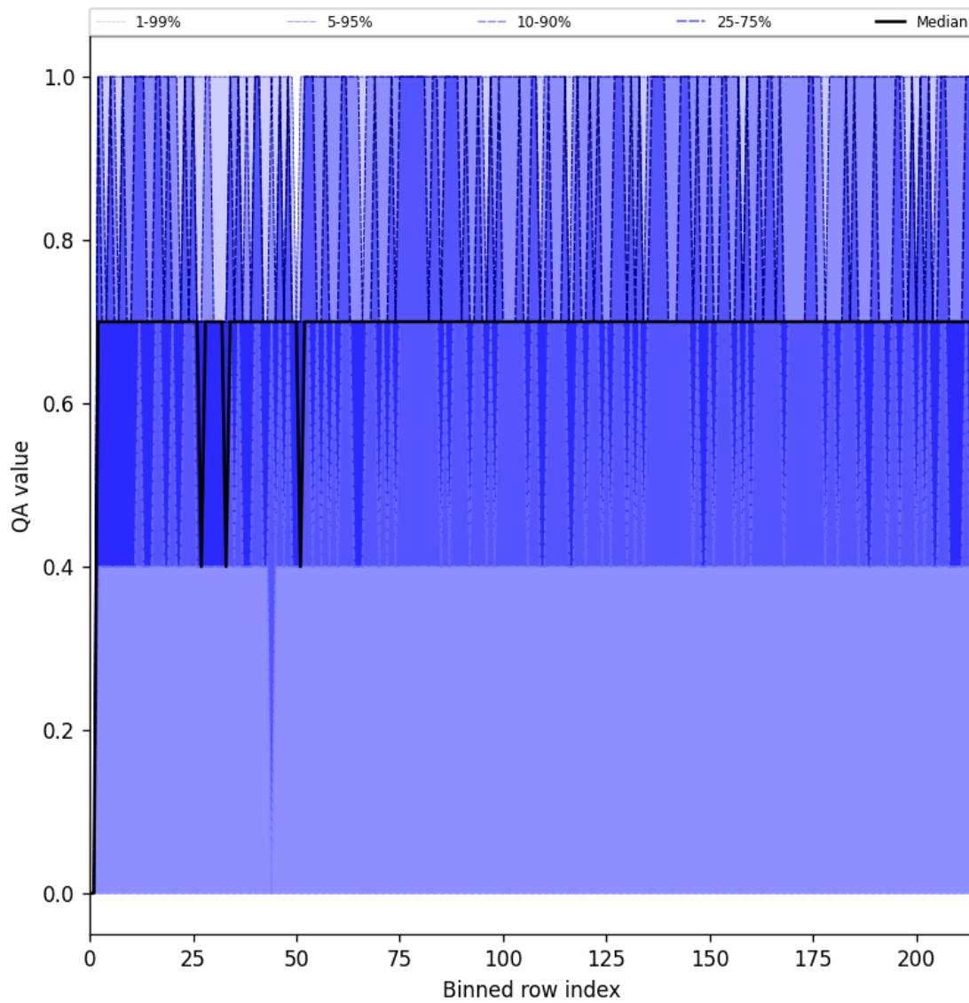
Figure 25: Along track statistics of “QA value” for 2025-07-24 to 2025-07-25
