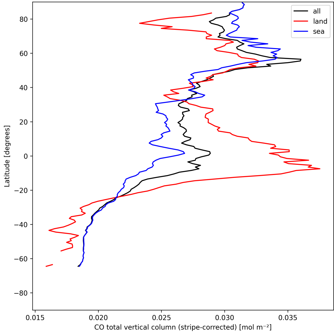
Figure 11: Zonal average of “CO total vertical column (stripe-corrected)” for 2025-07-24 to 2025-07-25.
