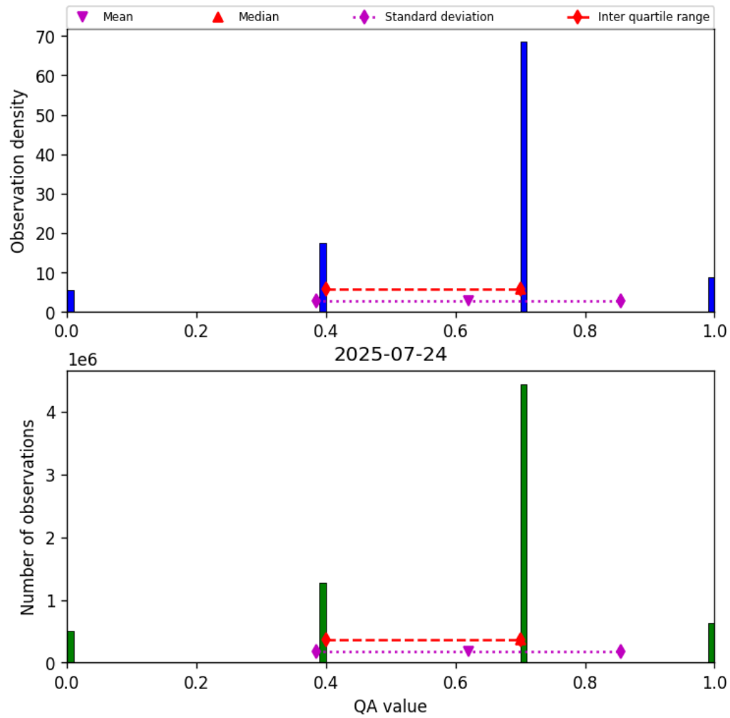
Figure 17: Histogram of “QA value” for 2025-07-24 to 2025-07-25
