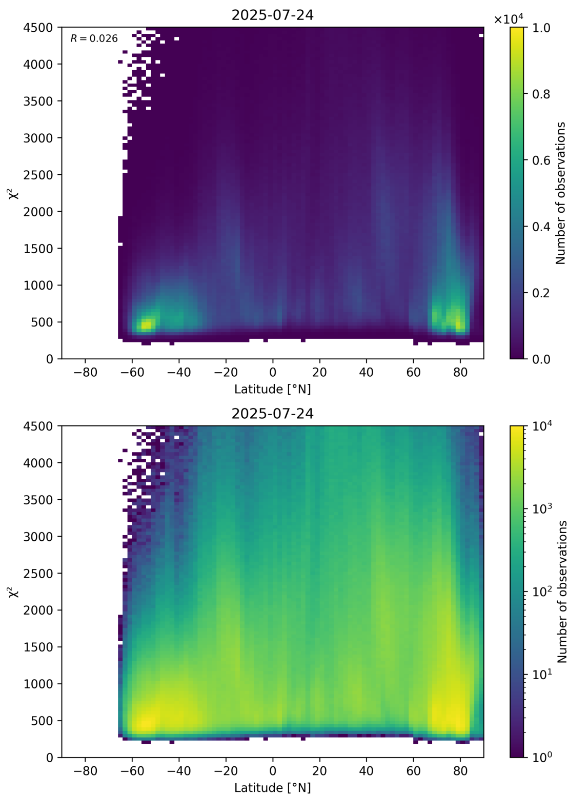
Figure 54: Scatter density plot of “Latitude” against “ \chi^2 ” for 2025-07-24 to 2025-07-25.
