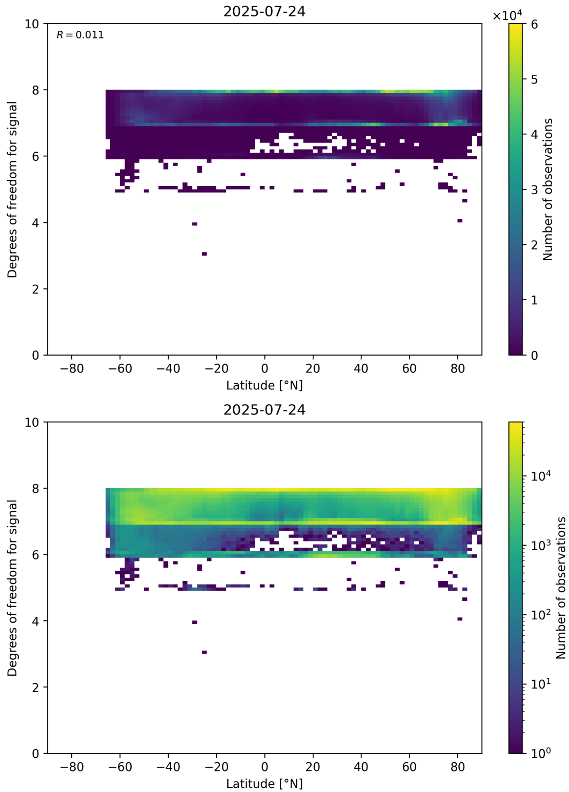
Figure 55: Scatter density plot of “Latitude” against “Degrees of freedom for signal” for 2025-07-24 to 2025-07-25.
