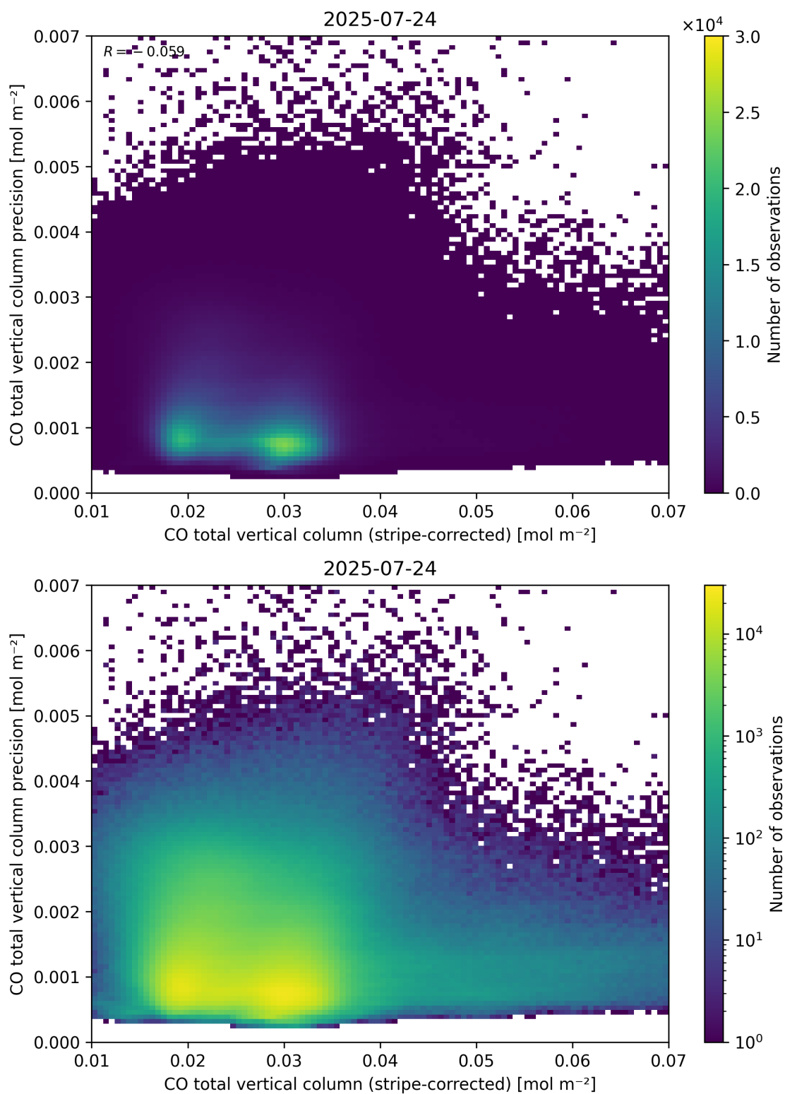
Figure 36: Scatter density plot of “CO total vertical column (stripe-corrected)” against “CO total vertical column precision” for 2025-07-24 to 2025-07-25.
