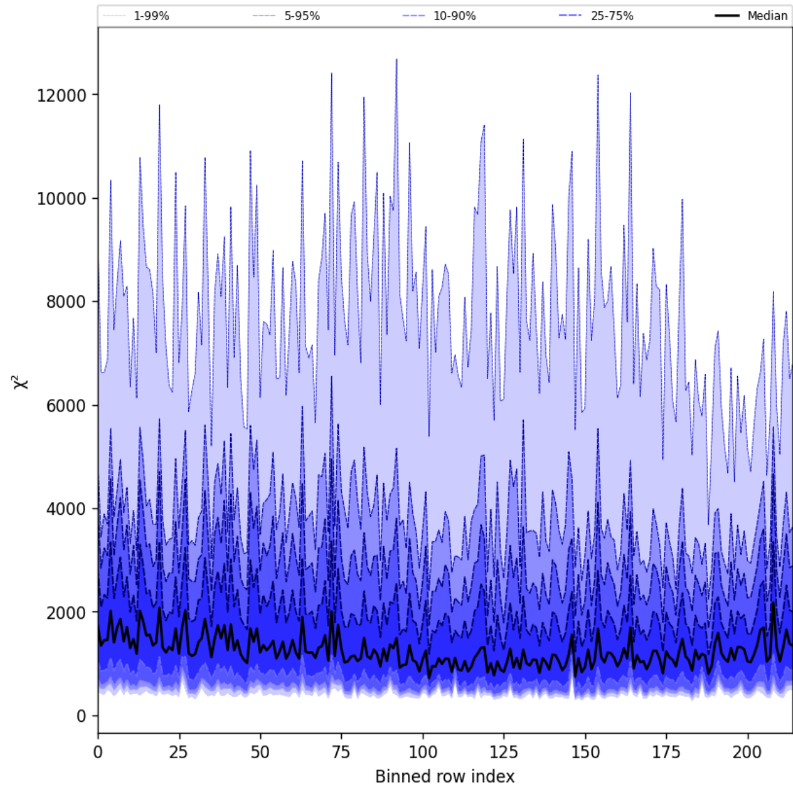
Figure 30: Along track statistics of “ \chi^2 ” for 2025-07-25 to 2025-07-27
