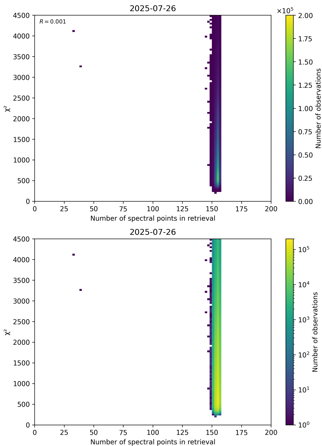
Figure 58: Scatter density plot of “Number of spectral points in retrieval” against “ \chi^2 ” for 2025-07-25 to 2025-07-27.
