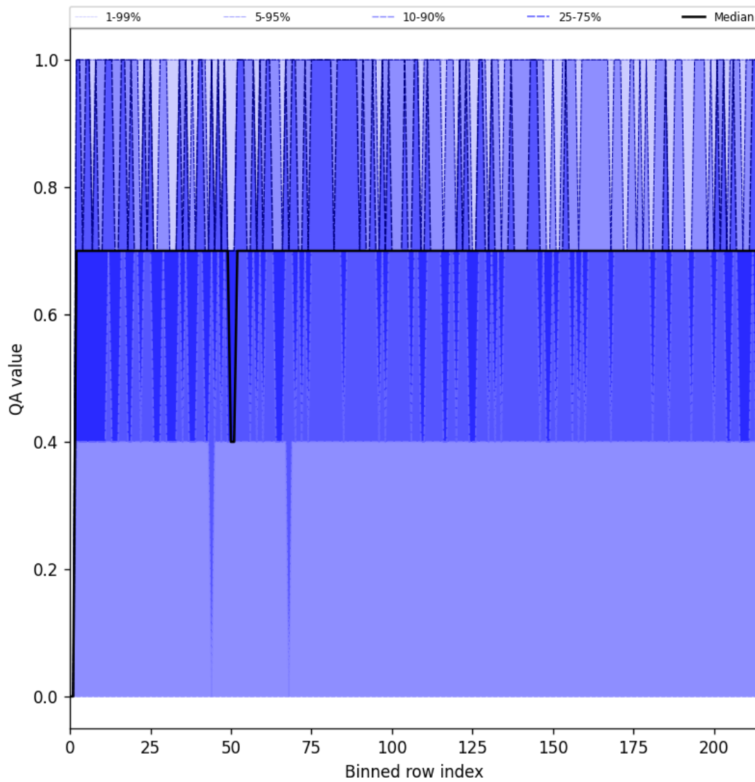
Figure 25: Along track statistics of “QA value” for 2025-07-25 to 2025-07-27
