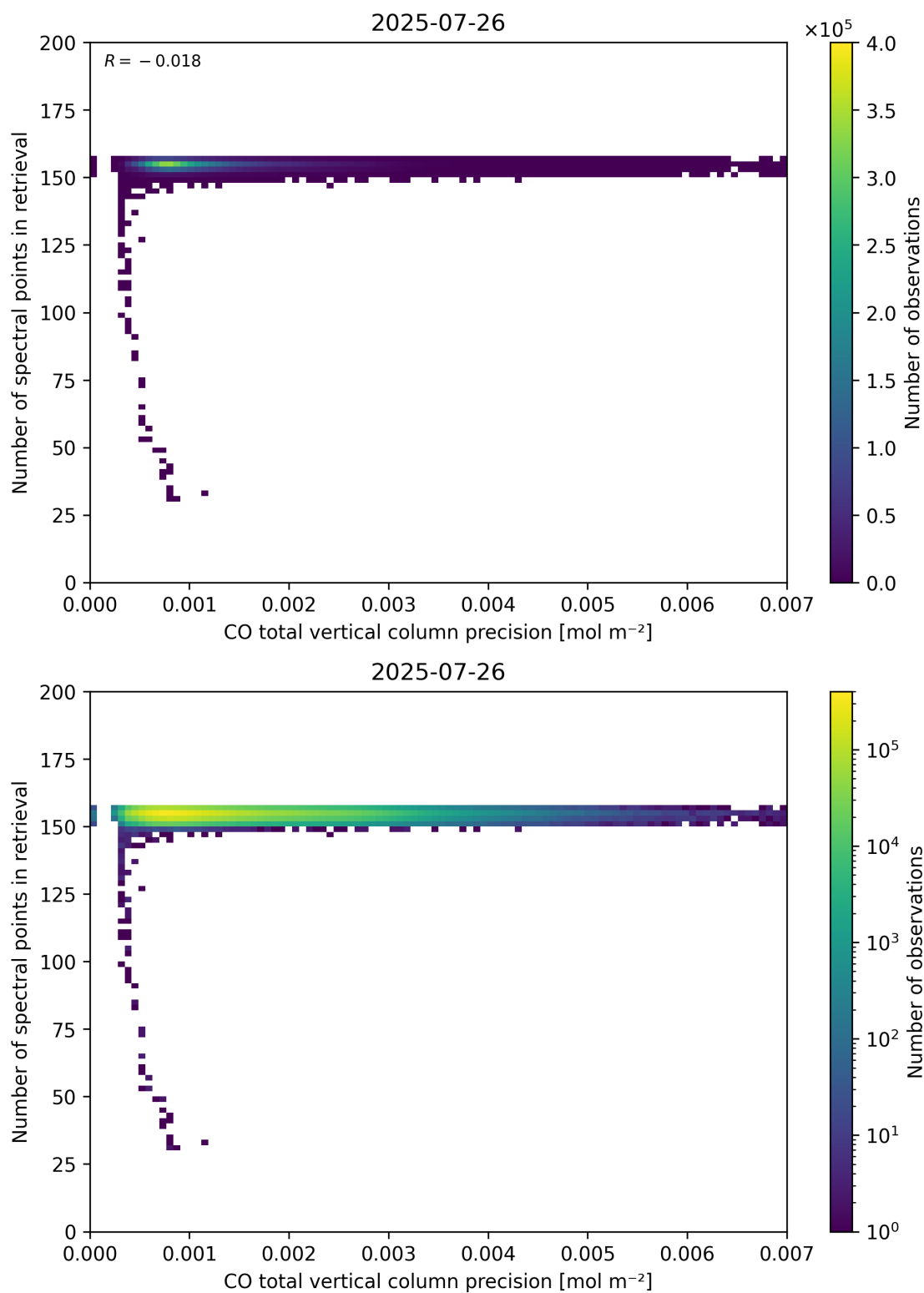
Figure 47: Scatter density plot of “CO total vertical column precision” against “Number of spectral points in retrieval” for 2025-07-25 to 2025-07-27.
