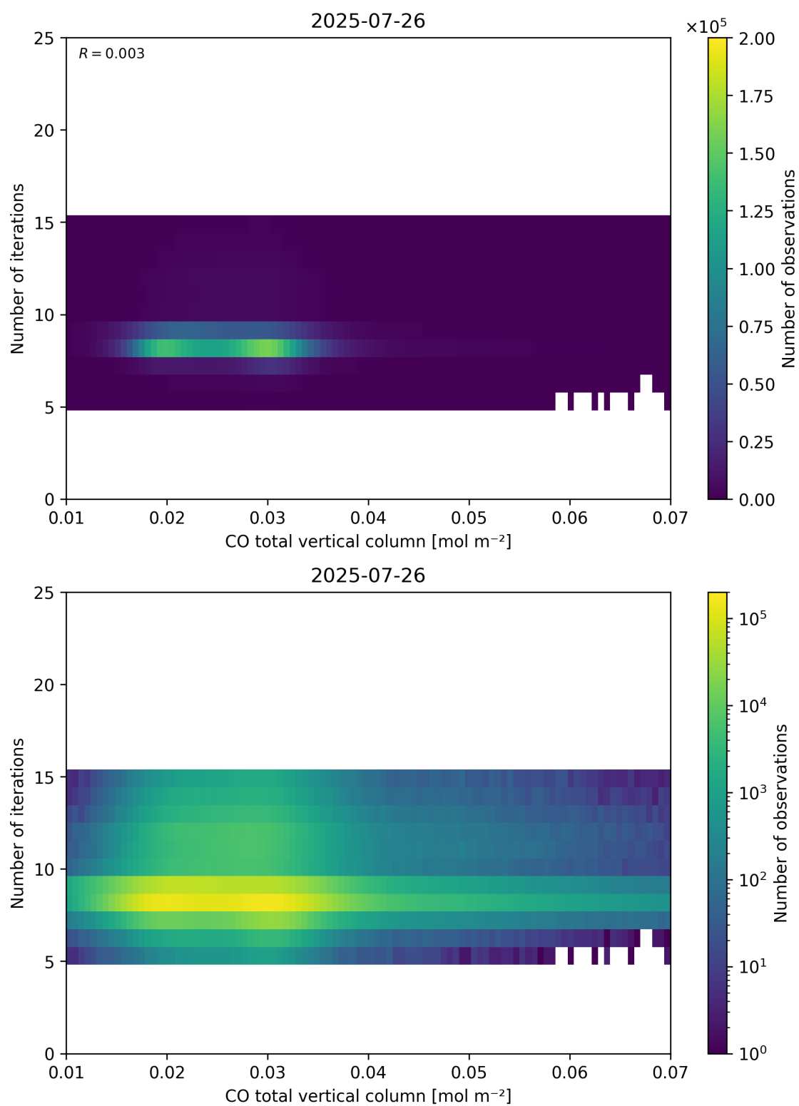
Figure 42: Scatter density plot of “CO total vertical column” against “Number of iterations” for 2025-07-25 to 2025-07-27.
