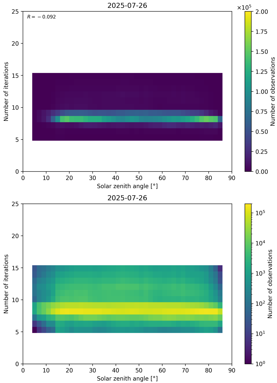
Figure 67: Scatter density plot of “Solar zenith angle” against “Number of iterations” for 2025-07-25 to 2025-07-27.
