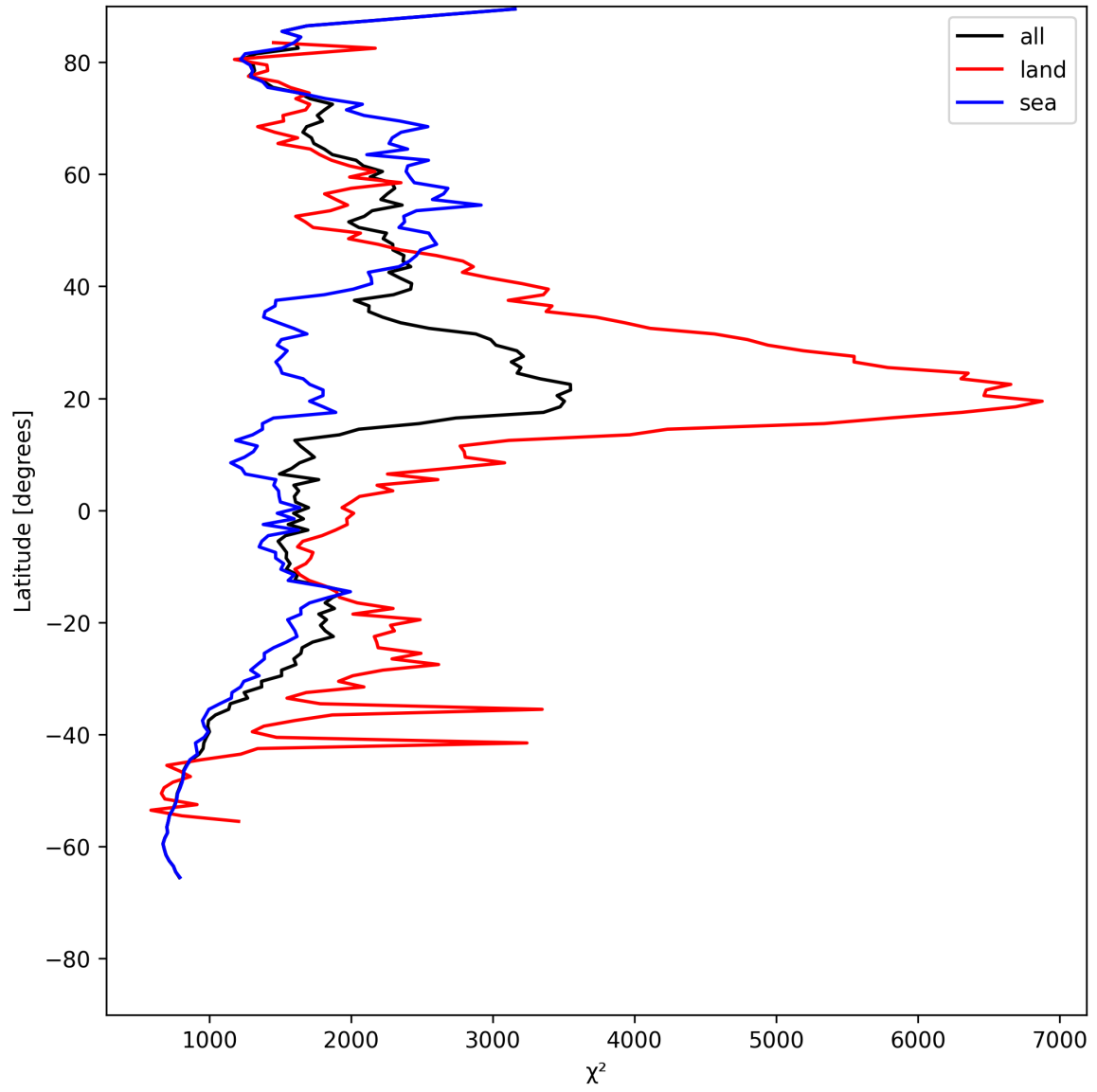
Figure 14: Zonal average of “ \chi^2 ” for 2025-07-25 to 2025-07-27.
