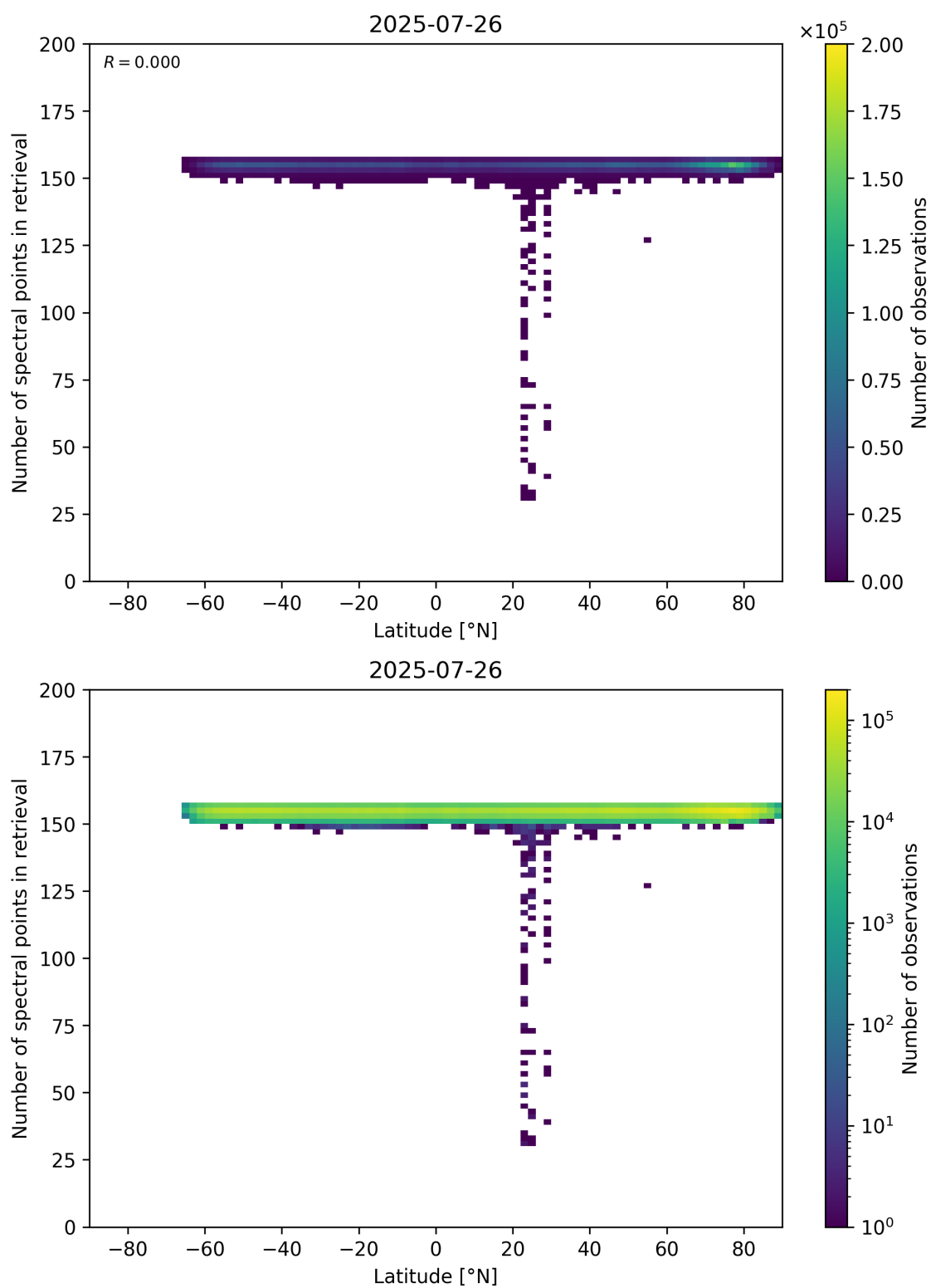
Figure 57: Scatter density plot of “Latitude” against “Number of spectral points in retrieval” for 2025-07-25 to 2025-07-27.
