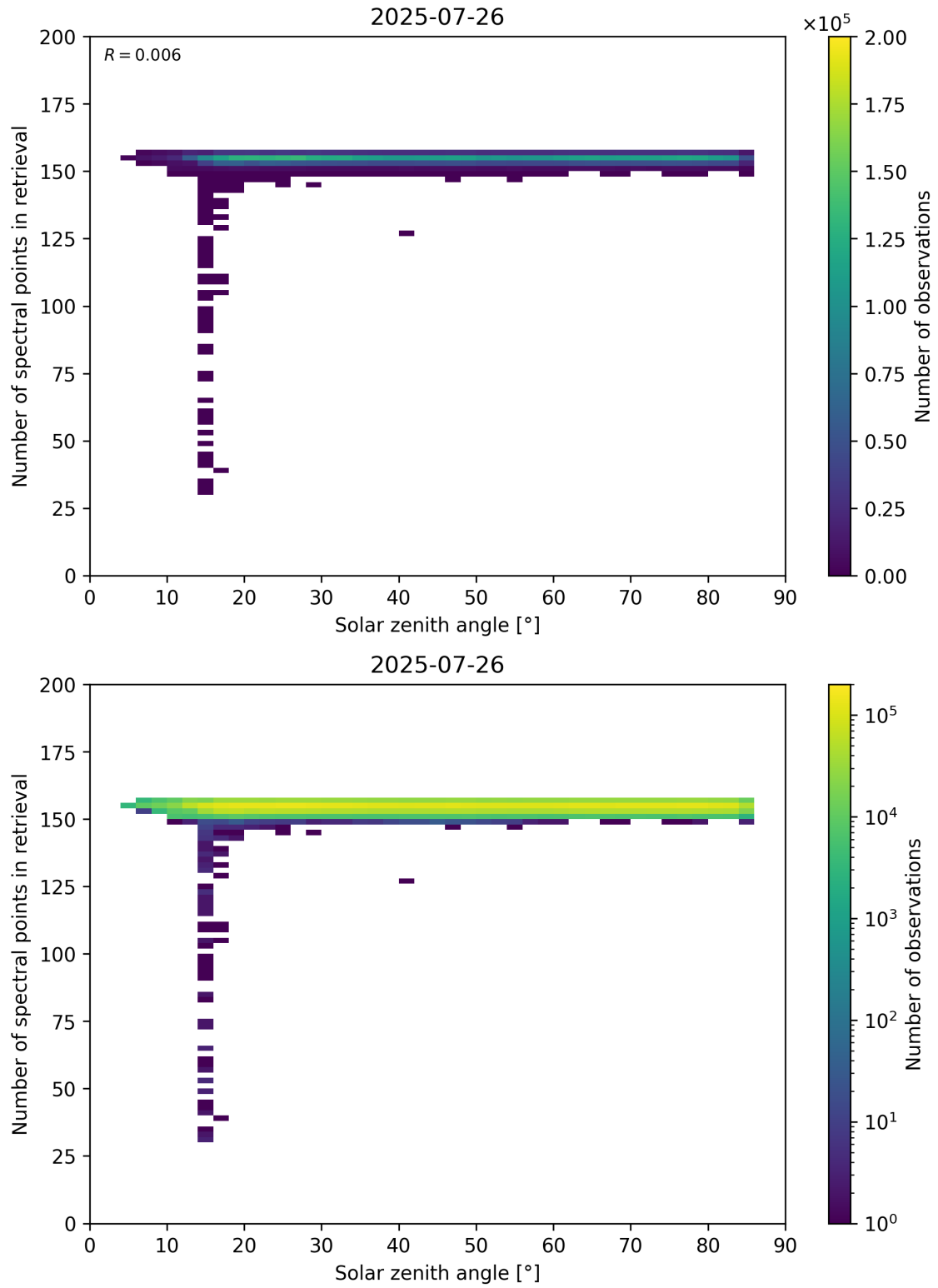
Figure 68: Scatter density plot of “Solar zenith angle” against “Number of spectral points in retrieval” for 2025-07-25 to 2025-07-27.
