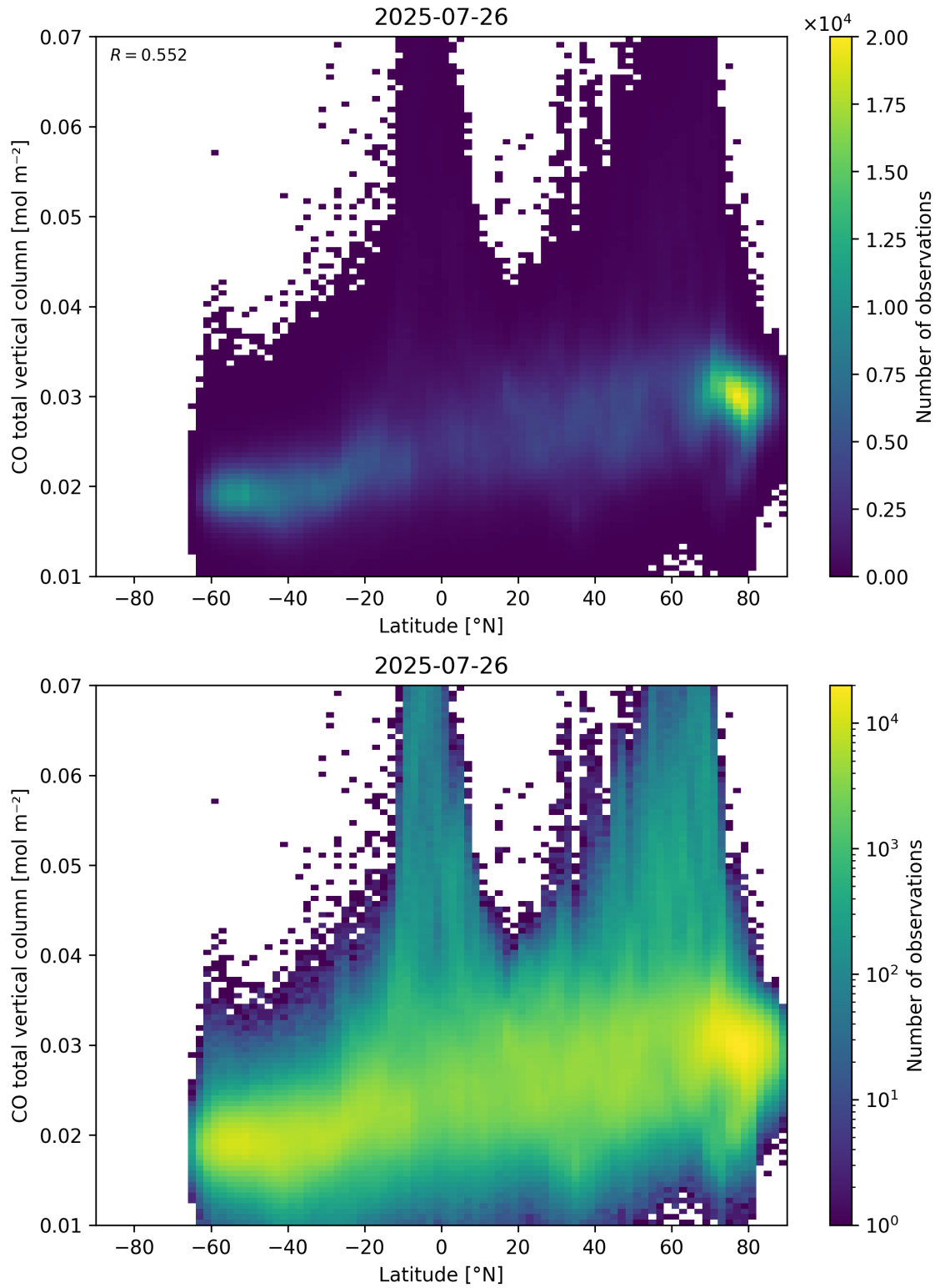
Figure 51: Scatter density plot of “Latitude” against “CO total vertical column” for 2025-07-25 to 2025-07-27.
