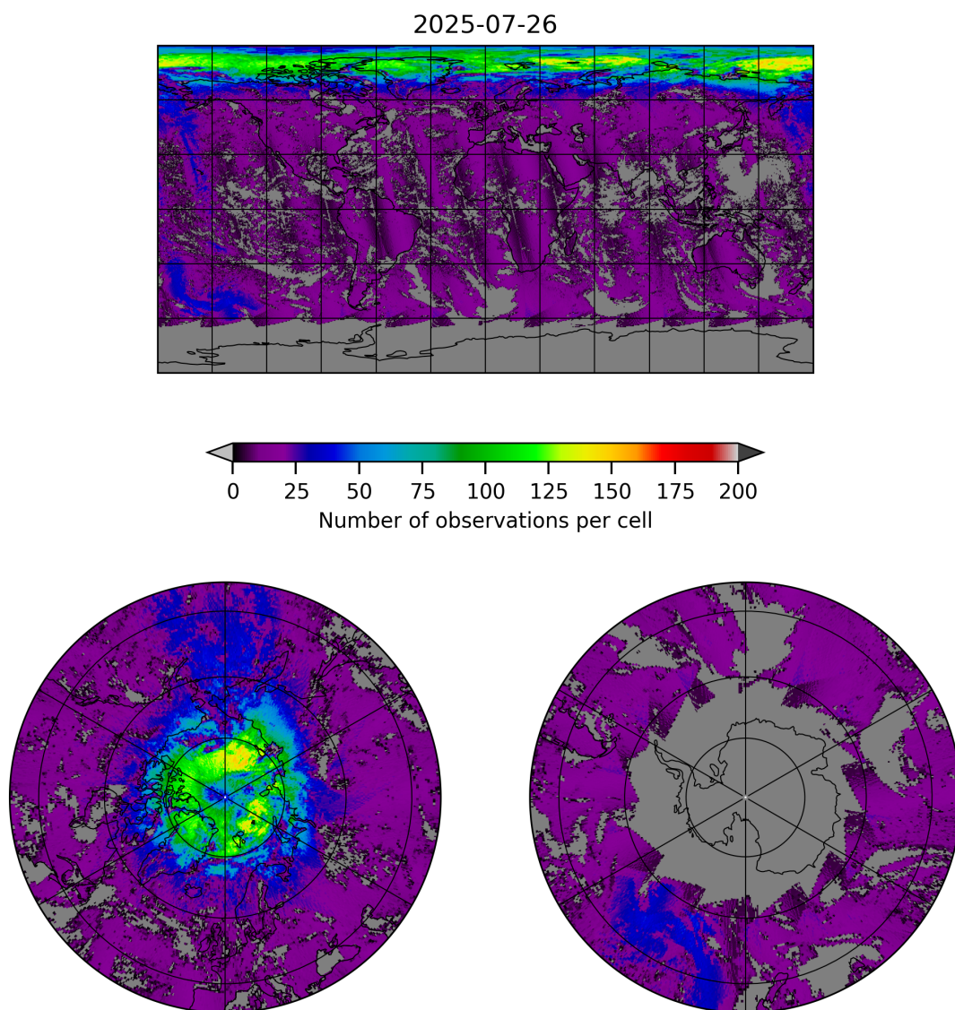
Figure 8: Map of the number of observations for 2025-07-25 to 2025-07-27
