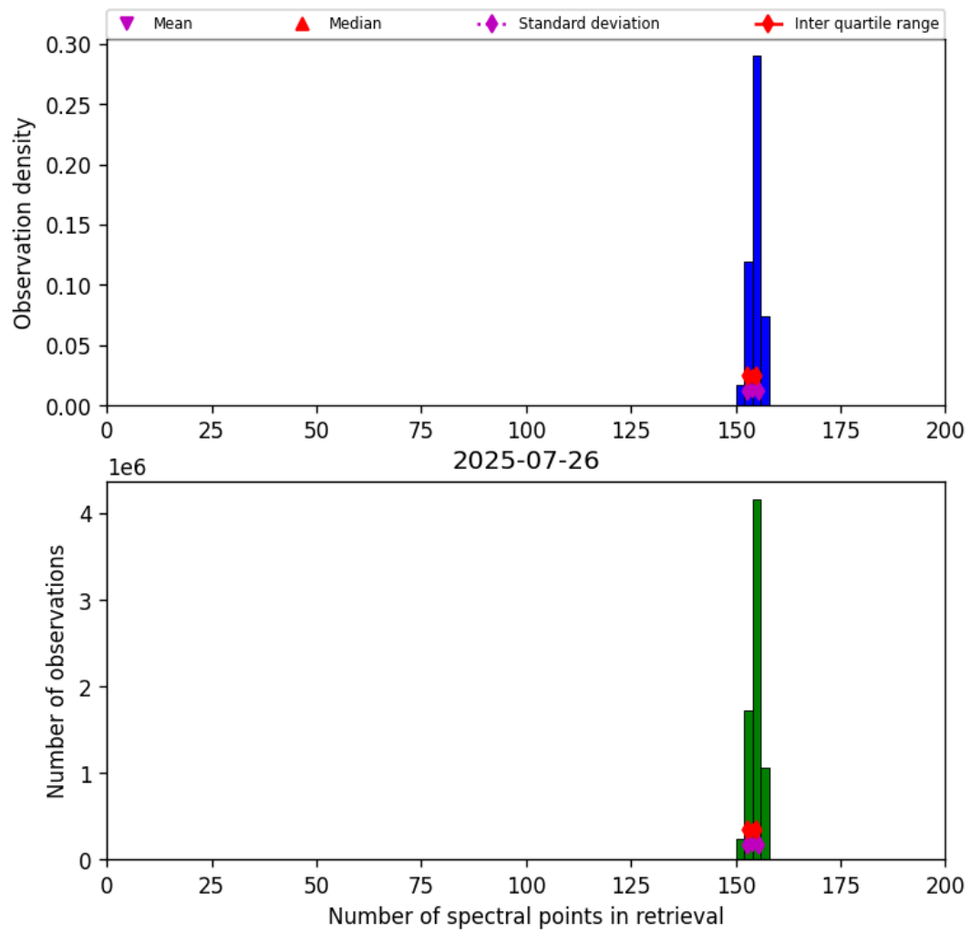
Figure 21: Histogram of “Number of spectral points in retrieval” for 2025-07-25 to 2025-07-27
