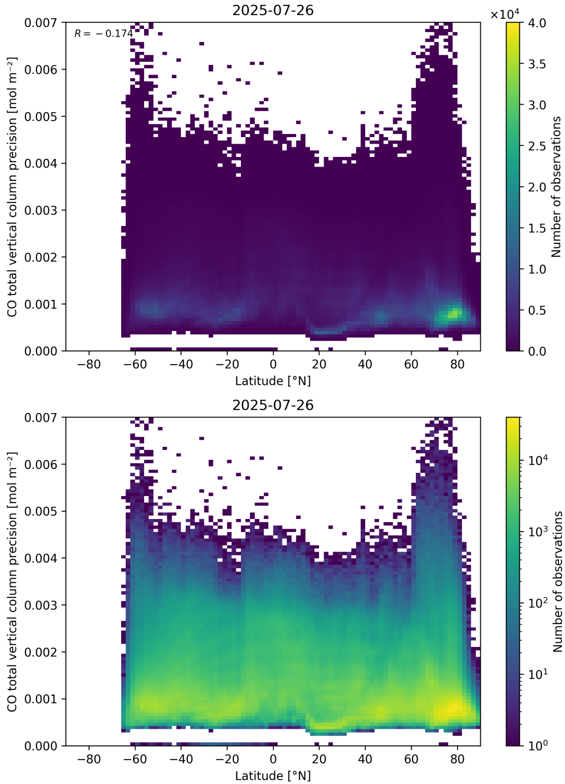
Figure 53: Scatter density plot of “Latitude” against “CO total vertical column precision” for 2025-07-25 to 2025-07-27.
