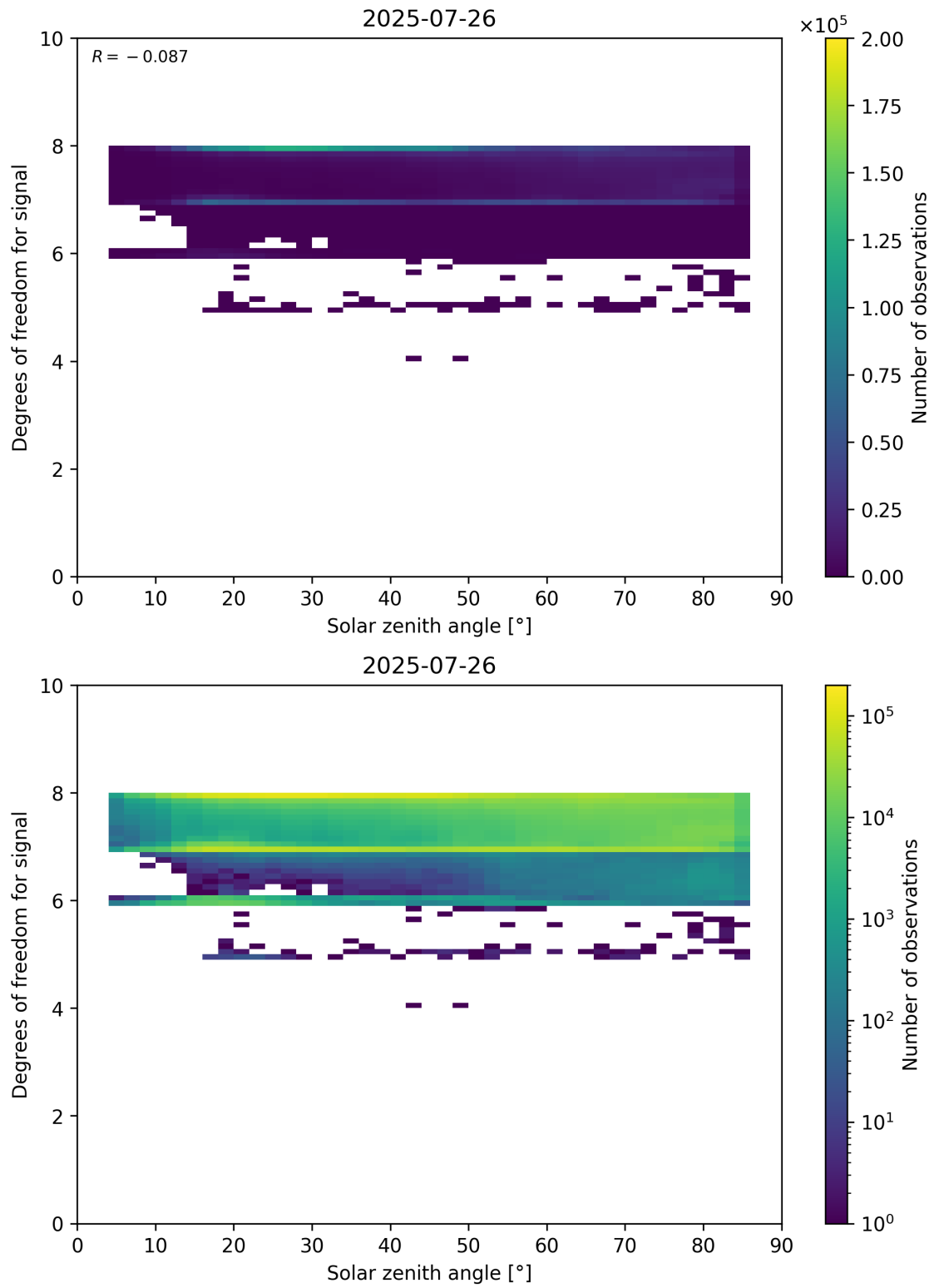
Figure 65: Scatter density plot of “Solar zenith angle” against “Degrees of freedom for signal” for 2025-07-25 to 2025-07-27.
