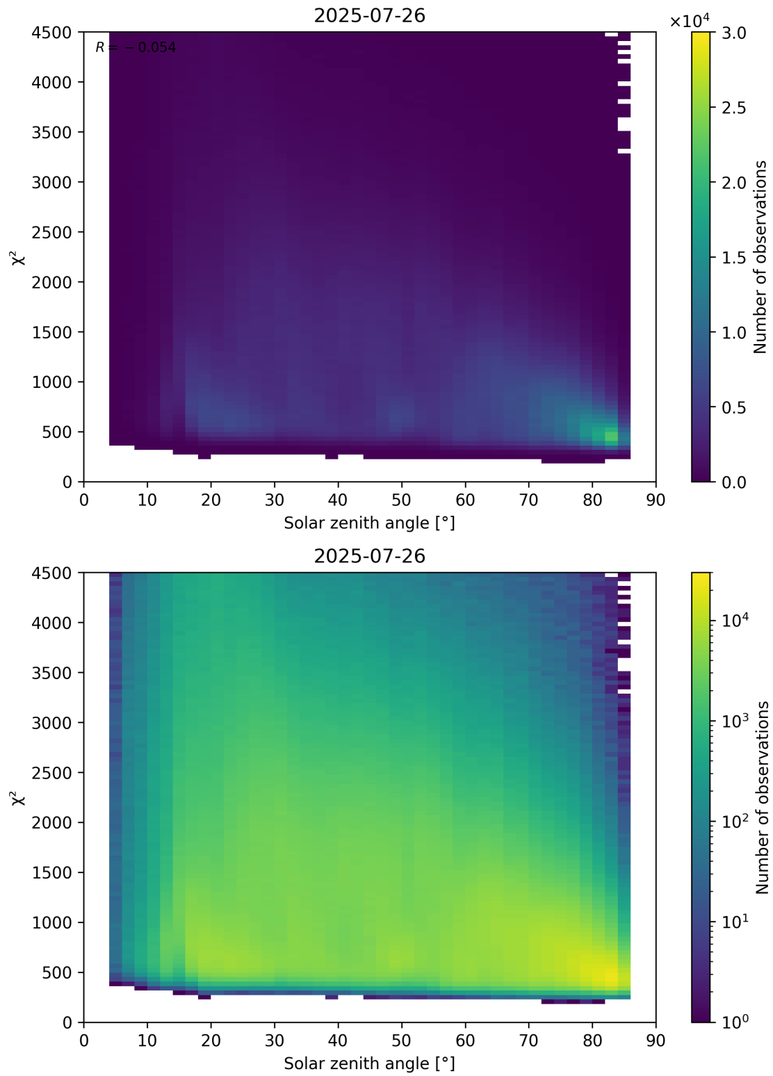
Figure 64: Scatter density plot of “Solar zenith angle” against “ \chi^2 ” for 2025-07-25 to 2025-07-27.
