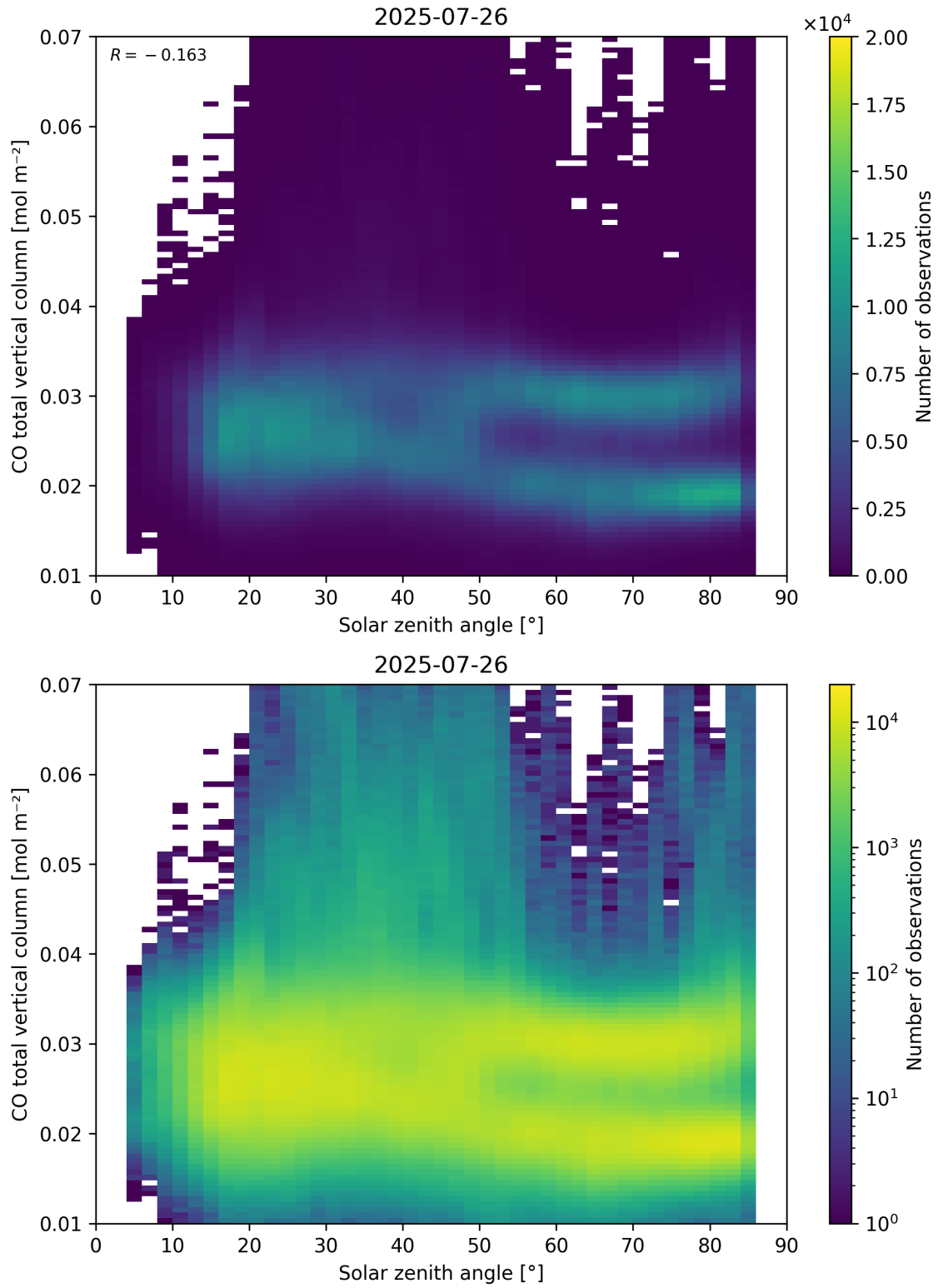
Figure 61: Scatter density plot of “Solar zenith angle” against “CO total vertical column” for 2025-07-25 to 2025-07-27.
