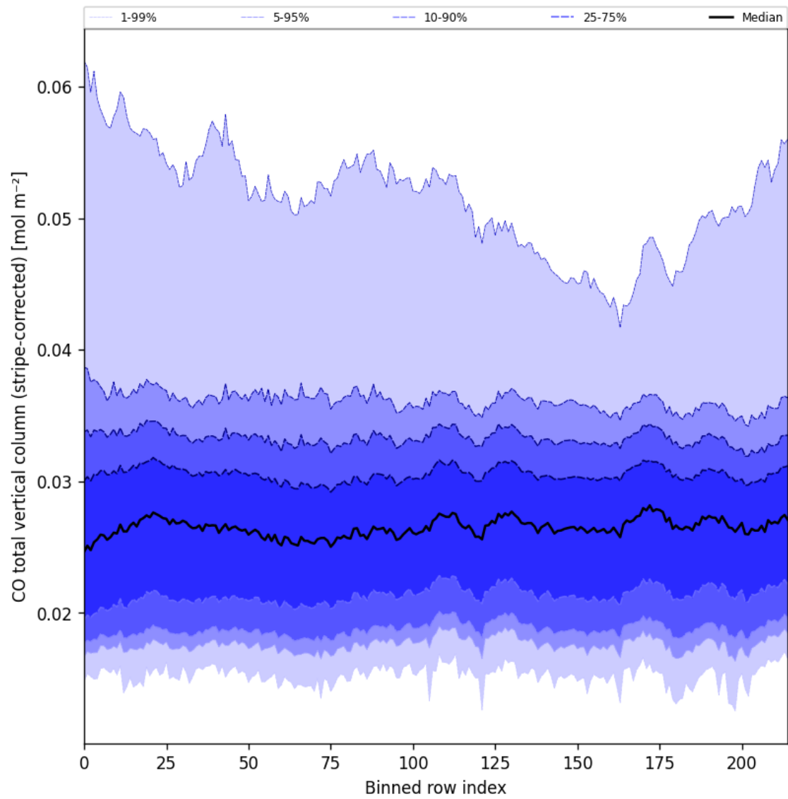
Figure 27: Along track statistics of “CO total vertical column (stripe-corrected)” for 2025-07-25 to 2025-07-27
