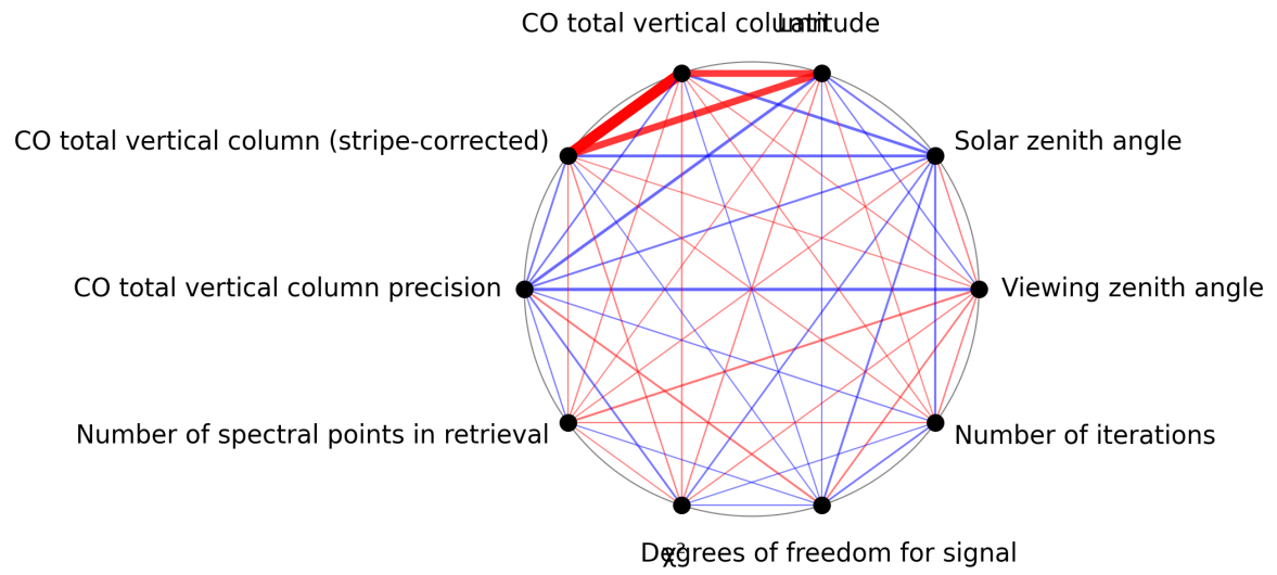
Figure 1: Map of correlation graph for 2025-07-25 to 2025-07-27.
