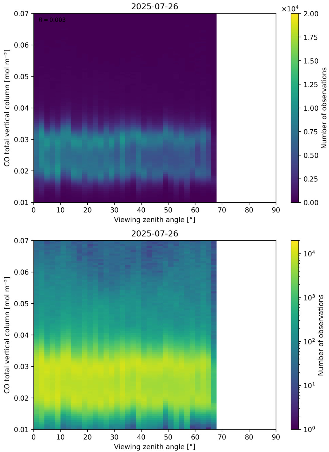
Figure 69: Scatter density plot of “Viewing zenith angle” against “CO total vertical column” for 2025-07-25 to 2025-07-27.
