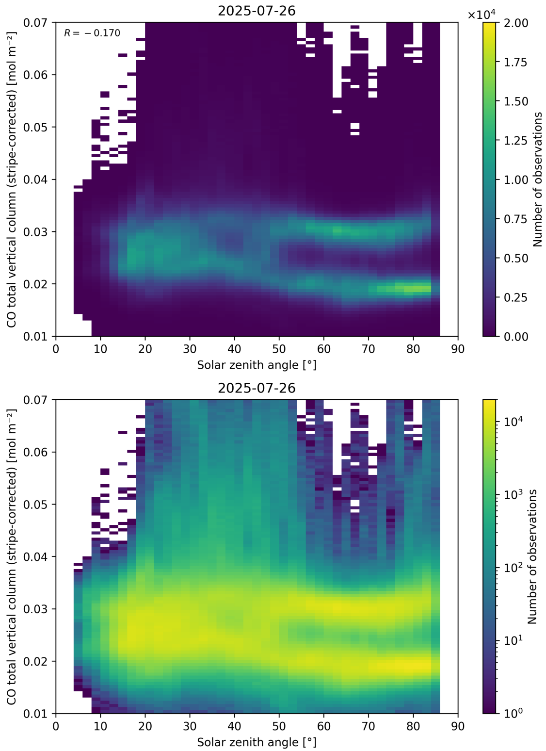
Figure 62: Scatter density plot of “Solar zenith angle” against “CO total vertical column (stripe-corrected)” for 2025-07-25 to 2025-07-27.
