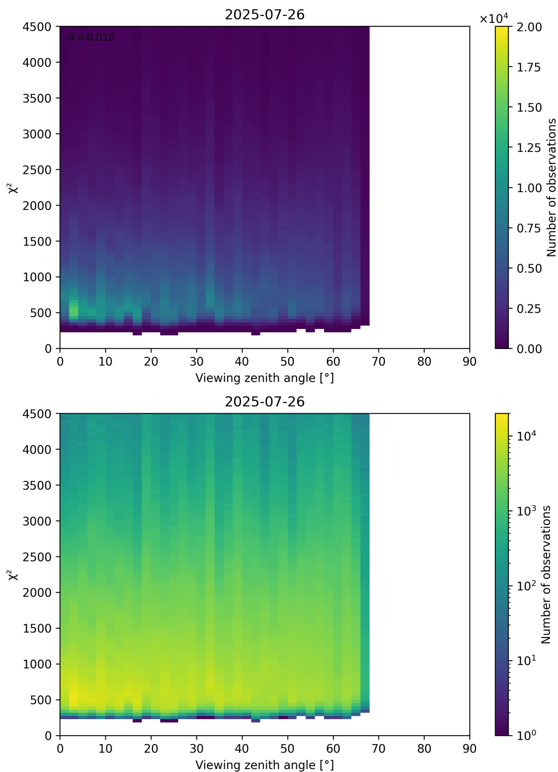
Figure 72: Scatter density plot of “Viewing zenith angle” against “ \chi^2 ” for 2025-07-25 to 2025-07-27.
