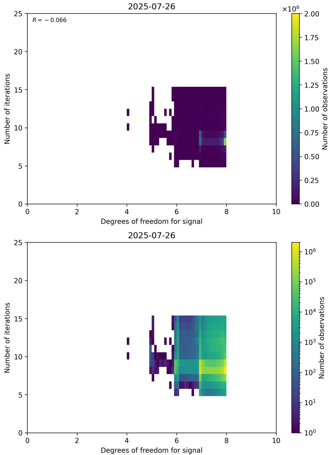
Figure 50: Scatter density plot of “Degrees of freedom for signal” against “Number of iterations” for 2025-07-25 to 2025-07-27.
