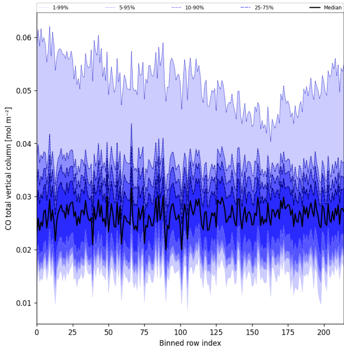
Figure 26: Along track statistics of “CO total vertical column” for 2025-07-25 to 2025-07-27
