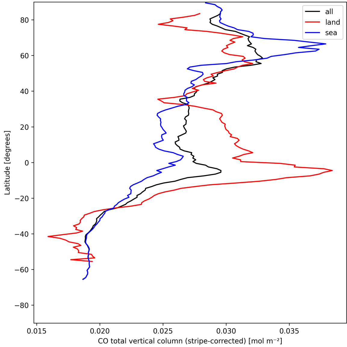
Figure 11: Zonal average of “CO total vertical column (stripe-corrected)” for 2025-07-25 to 2025-07-27.
