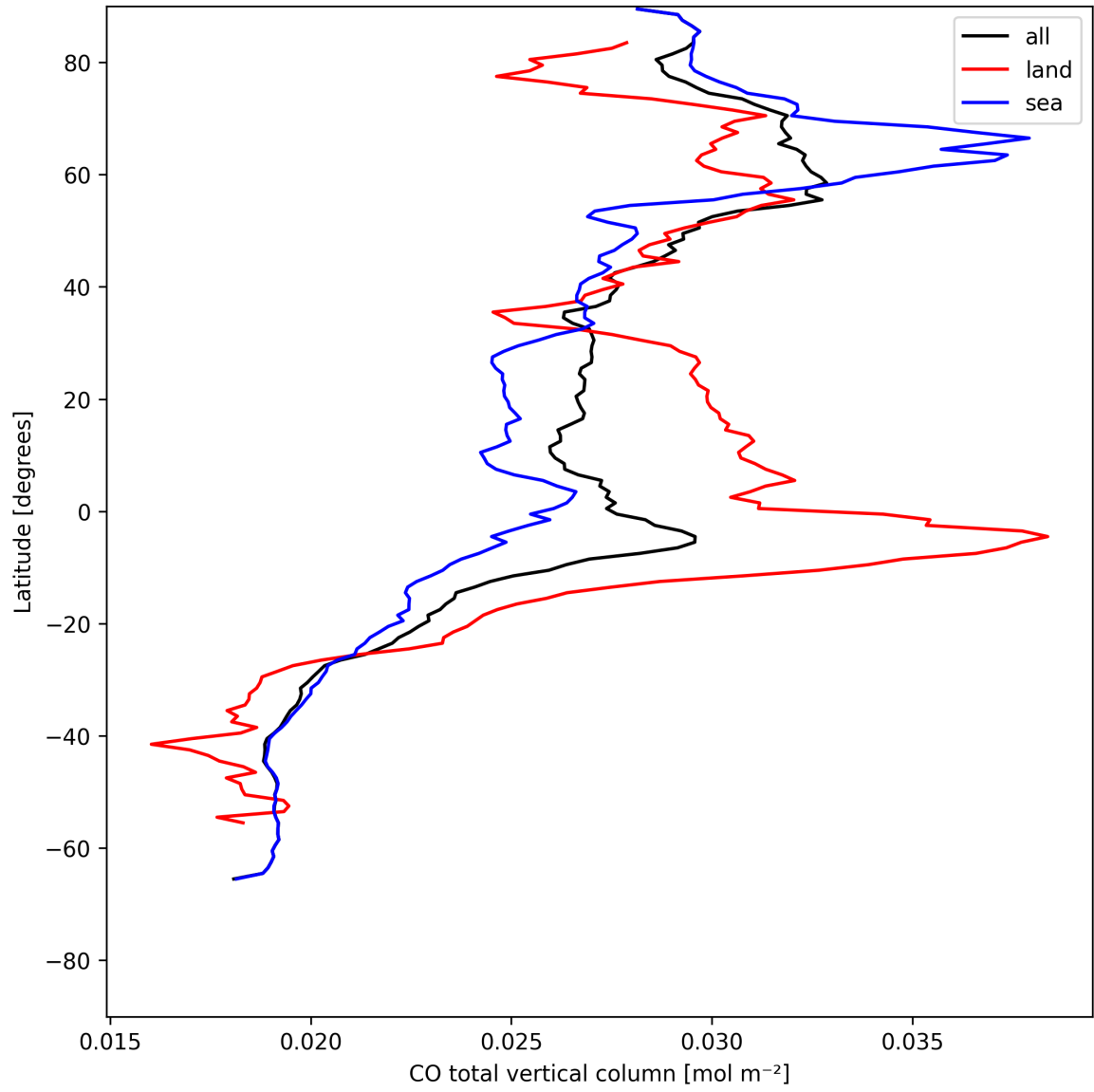
Figure 10: Zonal average of “CO total vertical column” for 2025-07-25 to 2025-07-27.
