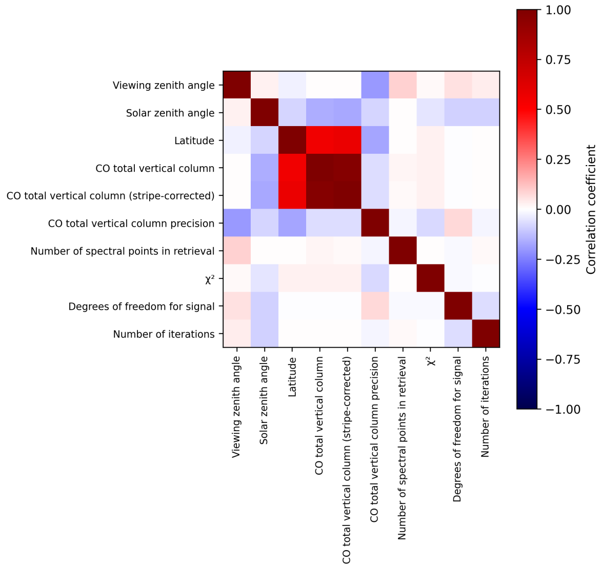
Figure 2: Map of correlation matrix for 2025-07-25 to 2025-07-27.
