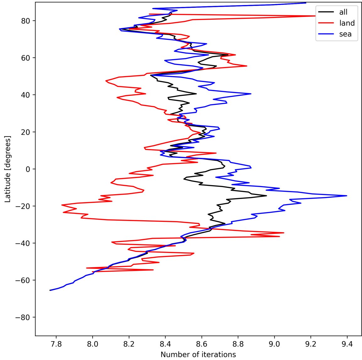
Figure 16: Zonal average of “Number of iterations” for 2025-07-25 to 2025-07-27.
