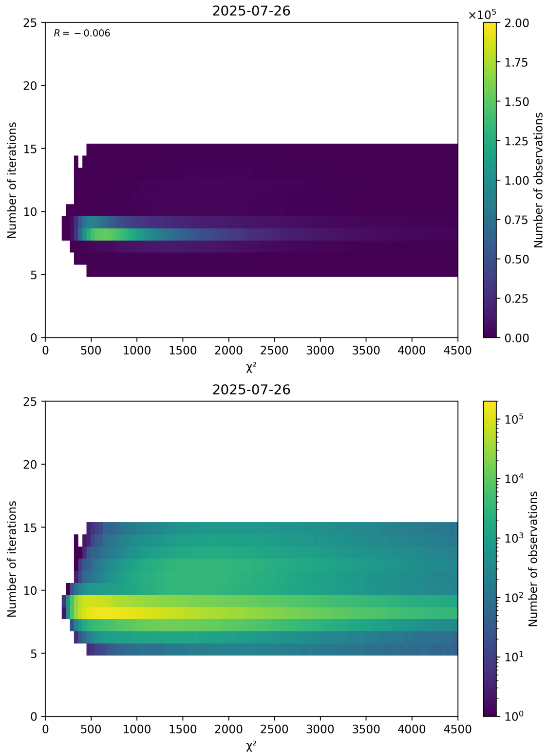
Figure 49: Scatter density plot of “ \chi^2 ” against “Number of iterations” for 2025-07-25 to 2025-07-27.
