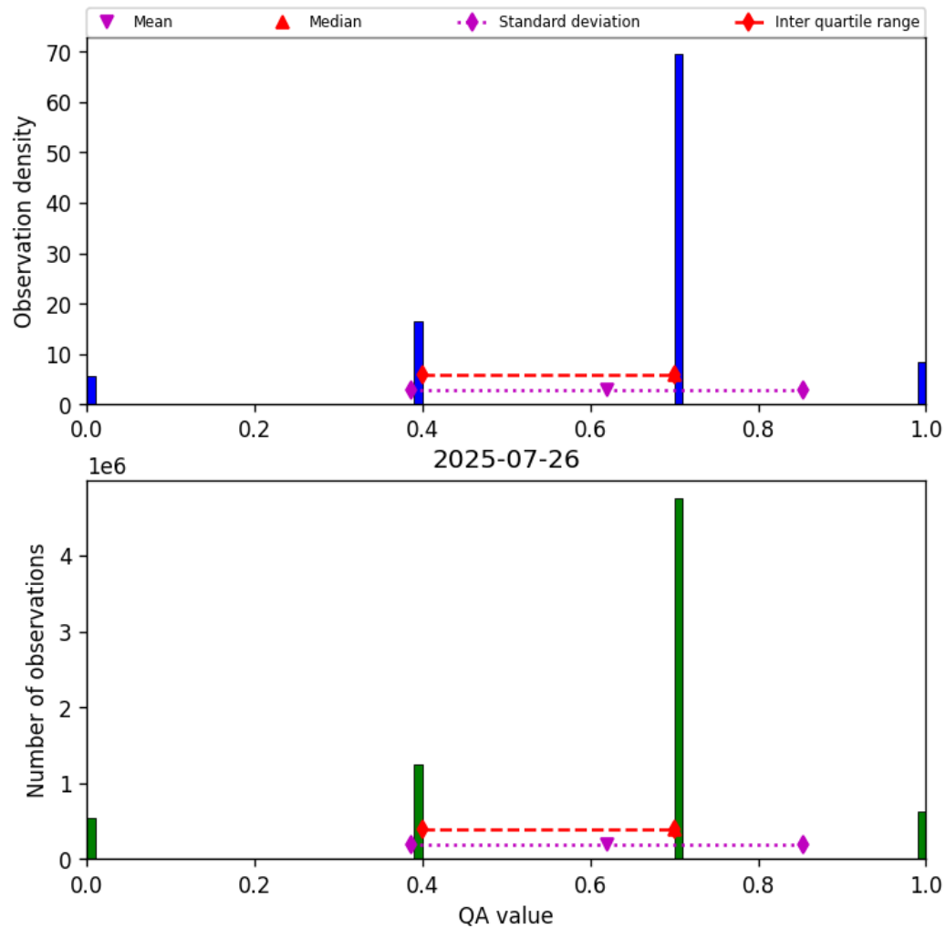
Figure 17: Histogram of “QA value” for 2025-07-25 to 2025-07-27
