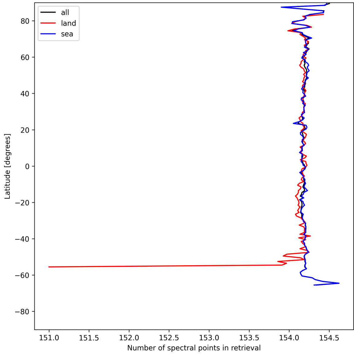
Figure 13: Zonal average of “Number of spectral points in retrieval” for 2025-07-25 to 2025-07-27.
