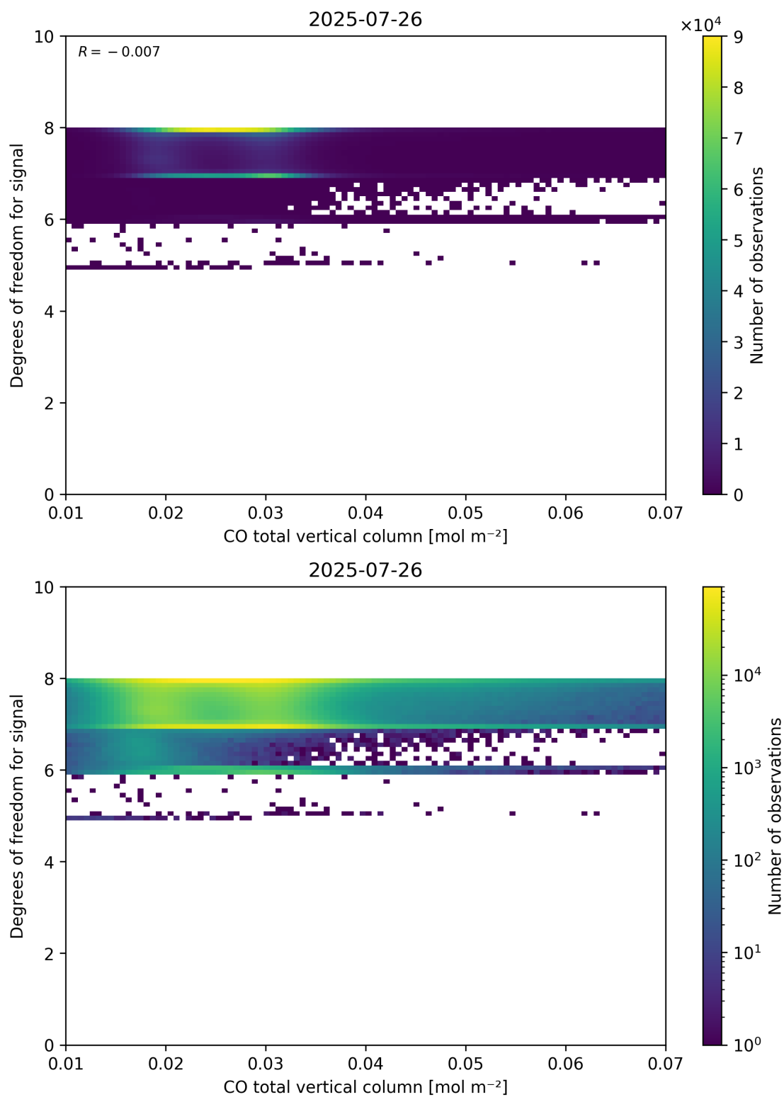
Figure 41: Scatter density plot of “CO total vertical column” against “Degrees of freedom for signal” for 2025-07-25 to 2025-07-27.
