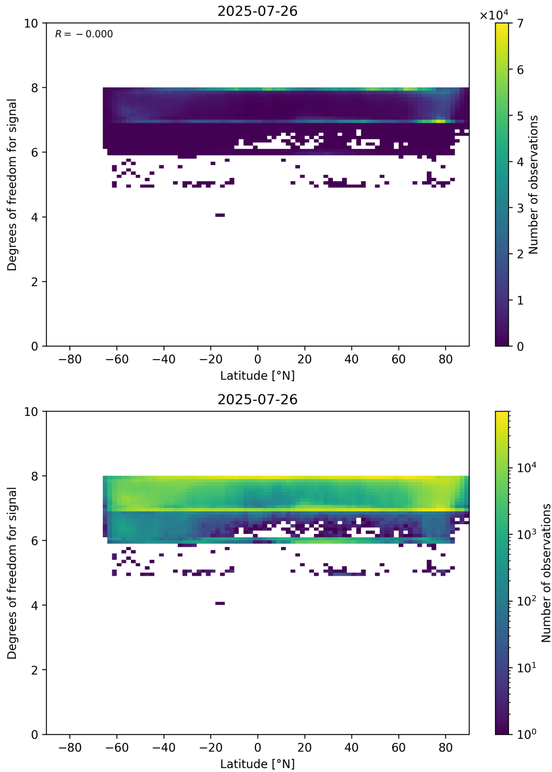
Figure 55: Scatter density plot of “Latitude” against “Degrees of freedom for signal” for 2025-07-25 to 2025-07-27.
