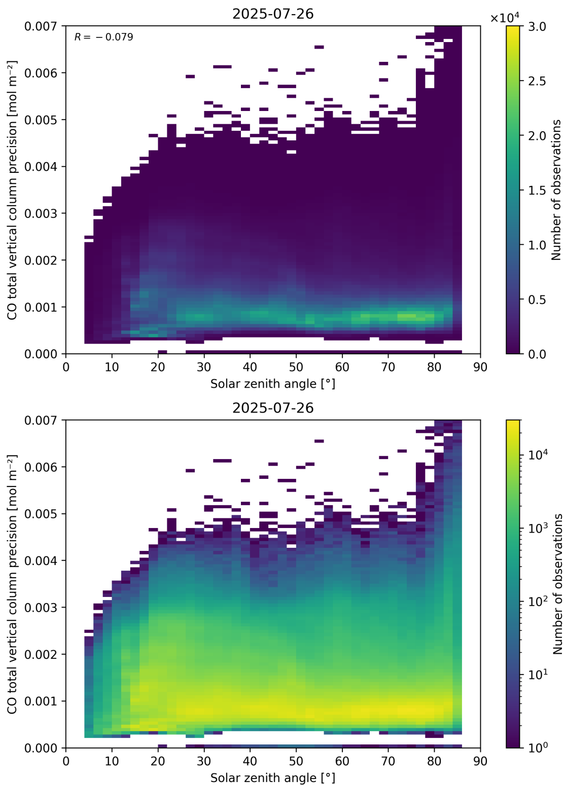
Figure 63: Scatter density plot of “Solar zenith angle” against “CO total vertical column precision” for 2025-07-25 to 2025-07-27.
