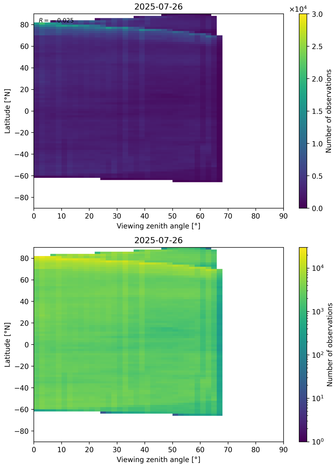
Figure 74: Scatter density plot of “Viewing zenith angle” against “Latitude” for 2025-07-25 to 2025-07-27.
