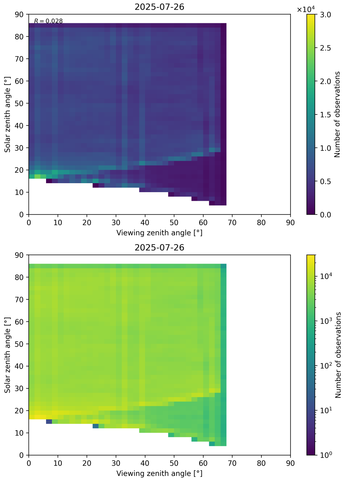
Figure 77: Scatter density plot of “Viewing zenith angle” against “Solar zenith angle” for 2025-07-25 to 2025-07-27.
