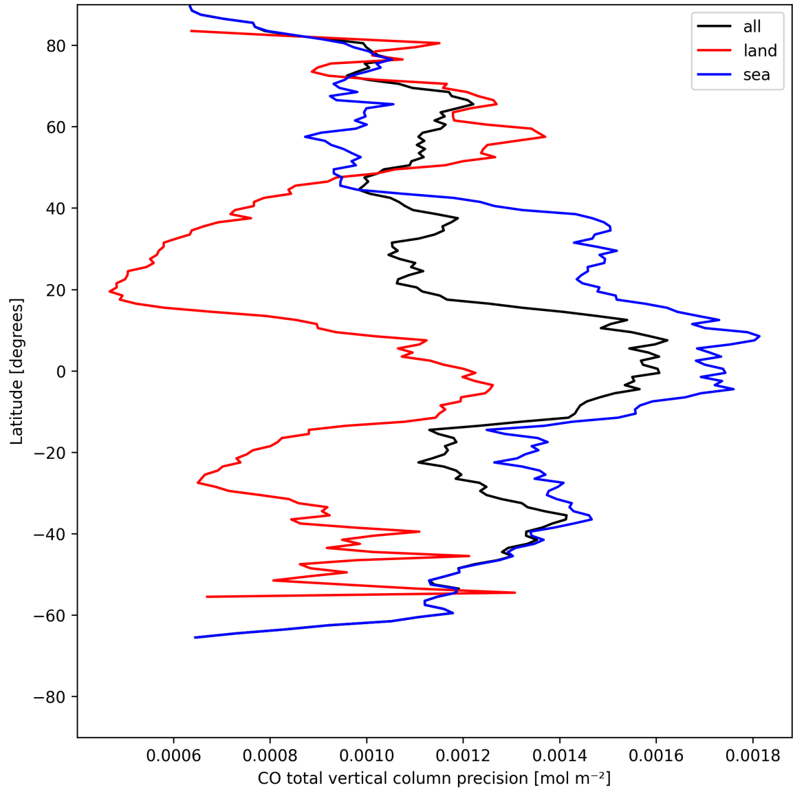
Figure 12: Zonal average of “CO total vertical column precision” for 2025-07-25 to 2025-07-27.
