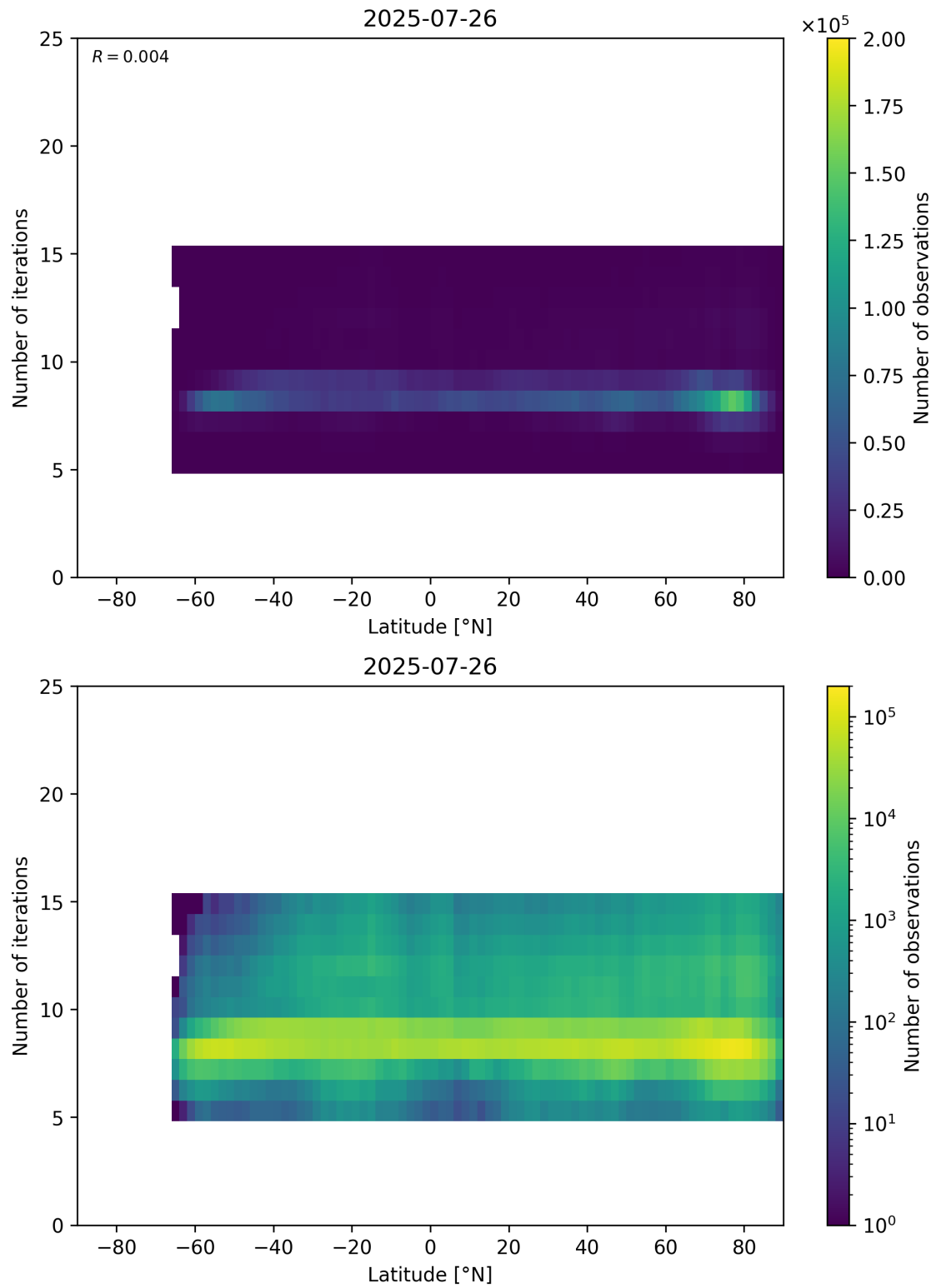
Figure 56: Scatter density plot of “Latitude” against “Number of iterations” for 2025-07-25 to 2025-07-27.
