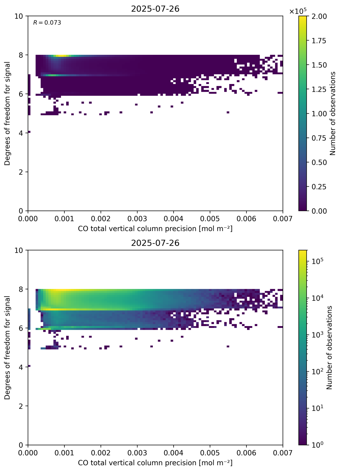
Figure 45: Scatter density plot of “CO total vertical column precision” against “Degrees of freedom for signal” for 2025-07-25 to 2025-07-27.
