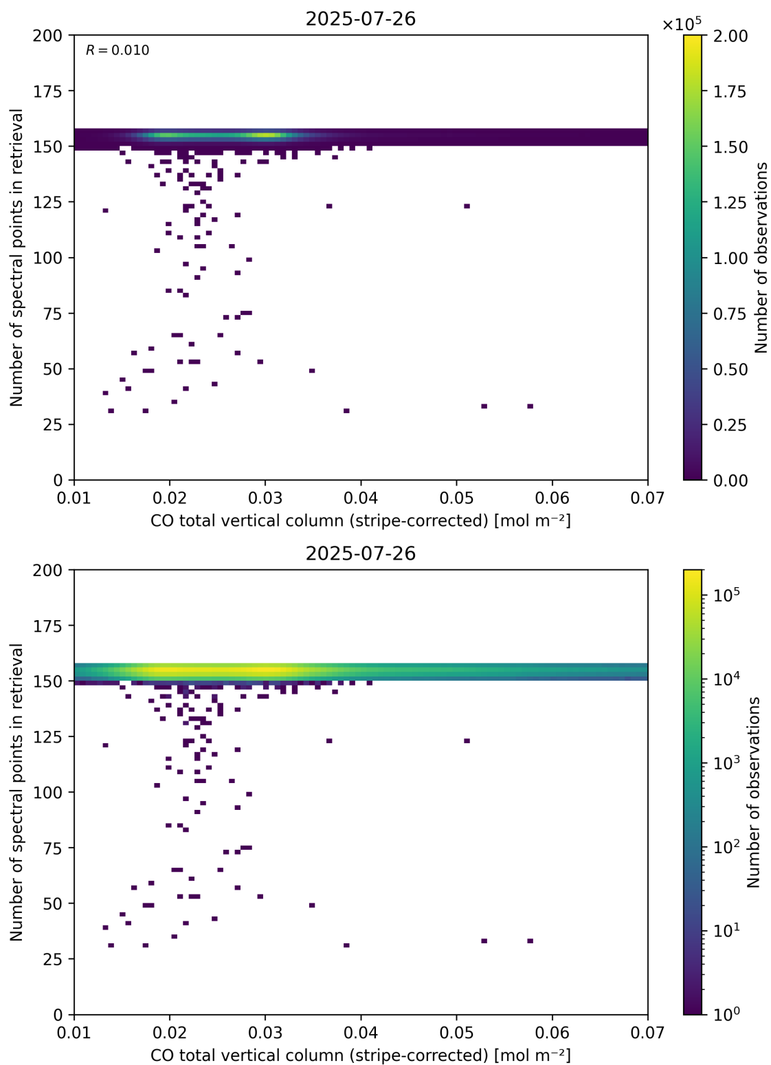
Figure 40: Scatter density plot of “CO total vertical column (stripe-corrected)” against “Number of spectral points in retrieval” for 2025-07-25 to 2025-07-27.
