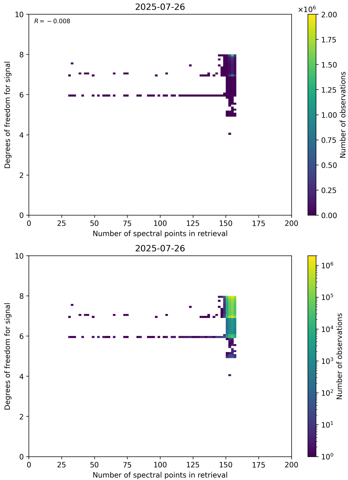
Figure 59: Scatter density plot of “Number of spectral points in retrieval” against “Degrees of freedom for signal” for 2025-07-25 to 2025-07-27.
