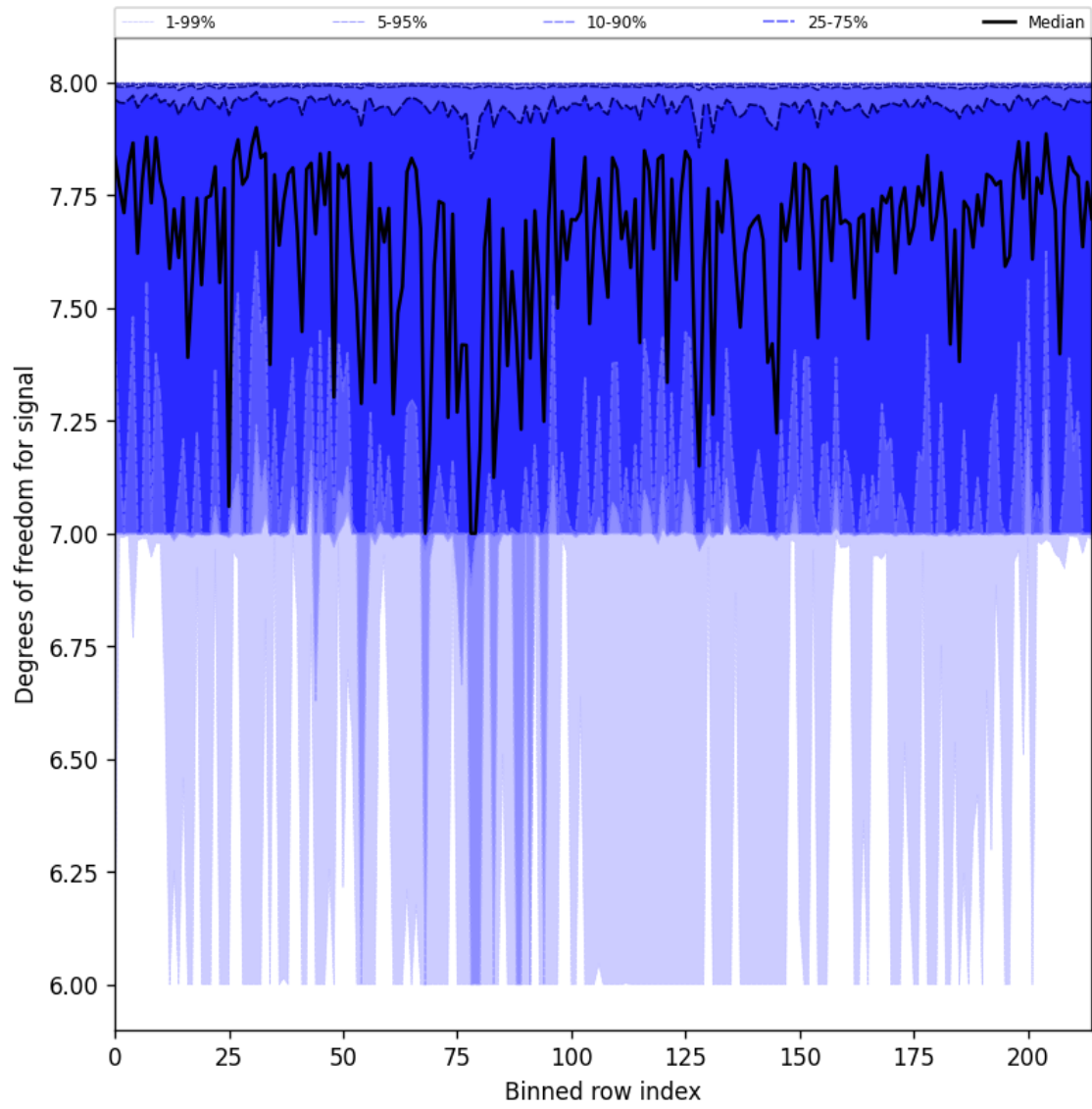
Figure 31: Along track statistics of “Degrees of freedom for signal” for 2025-07-25 to 2025-07-27
