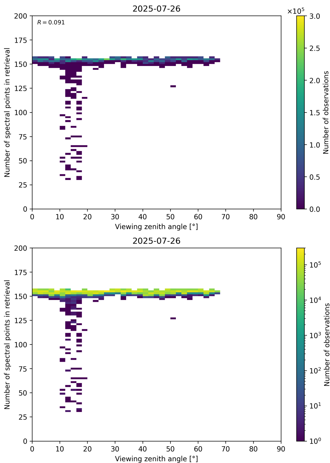
Figure 76: Scatter density plot of “Viewing zenith angle” against “Number of spectral points in retrieval” for 2025-07-25 to 2025-07-27.
