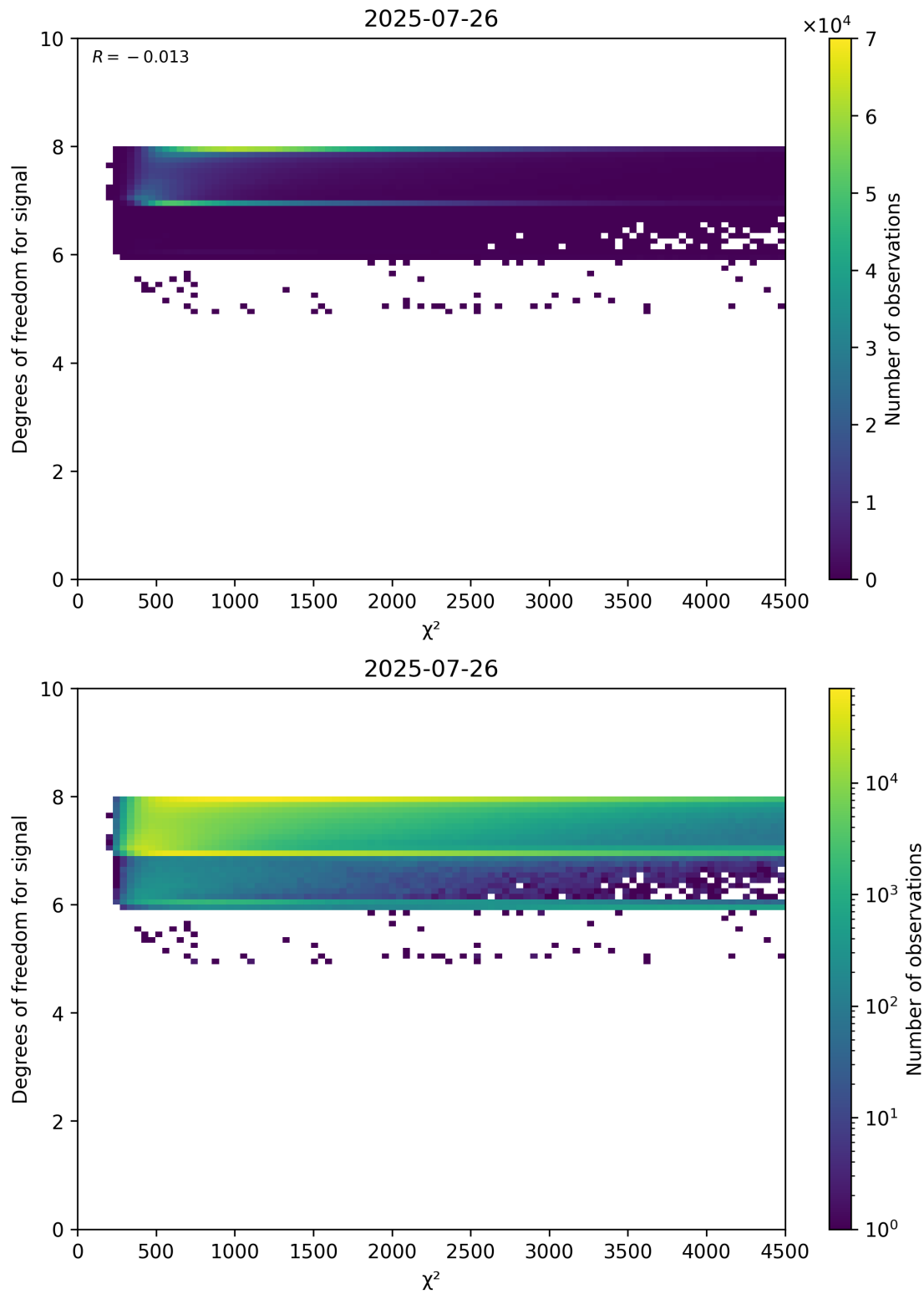
Figure 48: Scatter density plot of “ \chi^2 ” against “Degrees of freedom for signal” for 2025-07-25 to 2025-07-27.
