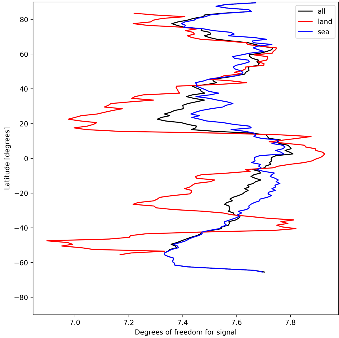
Figure 15: Zonal average of “Degrees of freedom for signal” for 2025-07-25 to 2025-07-27.
