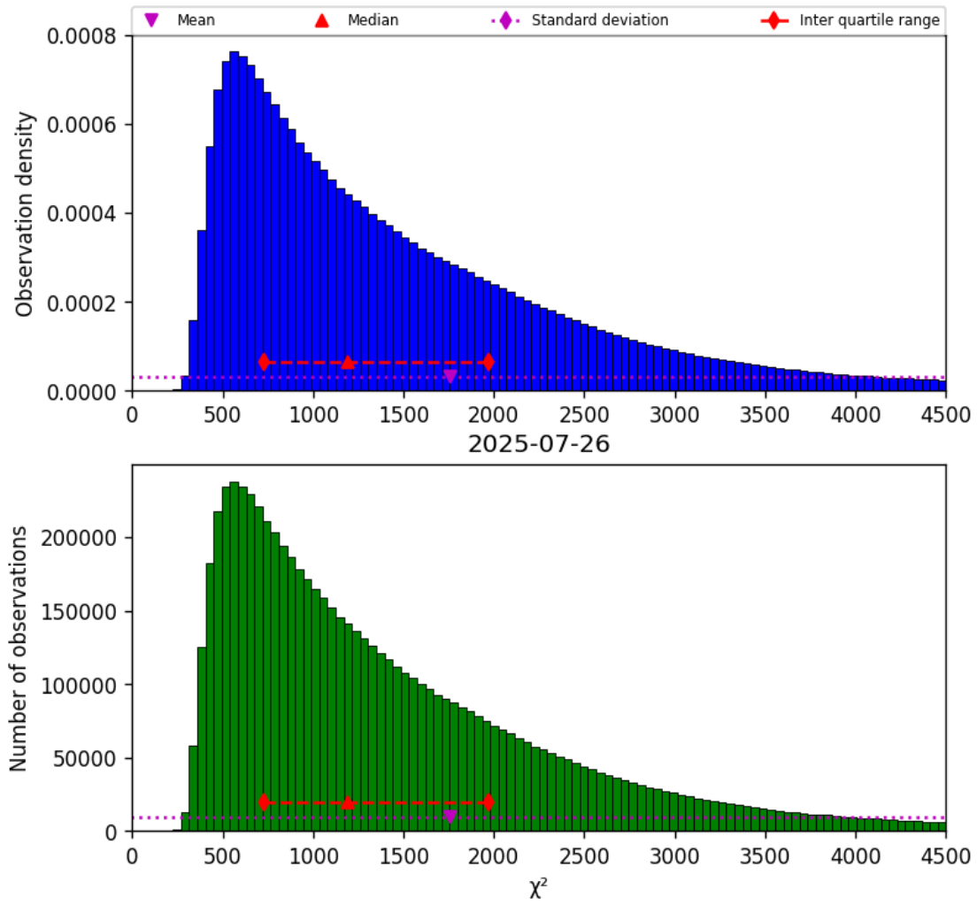
Figure 22: Histogram of “ \chi^2 ” for 2025-07-25 to 2025-07-27
