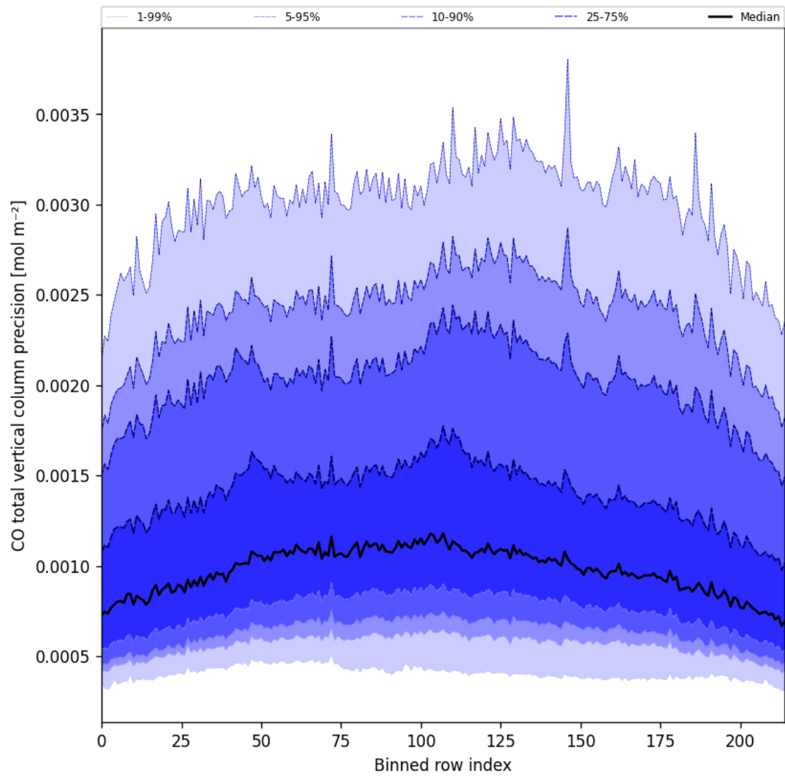
Figure 28: Along track statistics of “CO total vertical column precision” for 2025-07-25 to 2025-07-27
