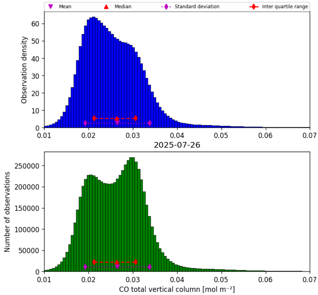
Figure 18: Histogram of “CO total vertical column” for 2025-07-25 to 2025-07-27
