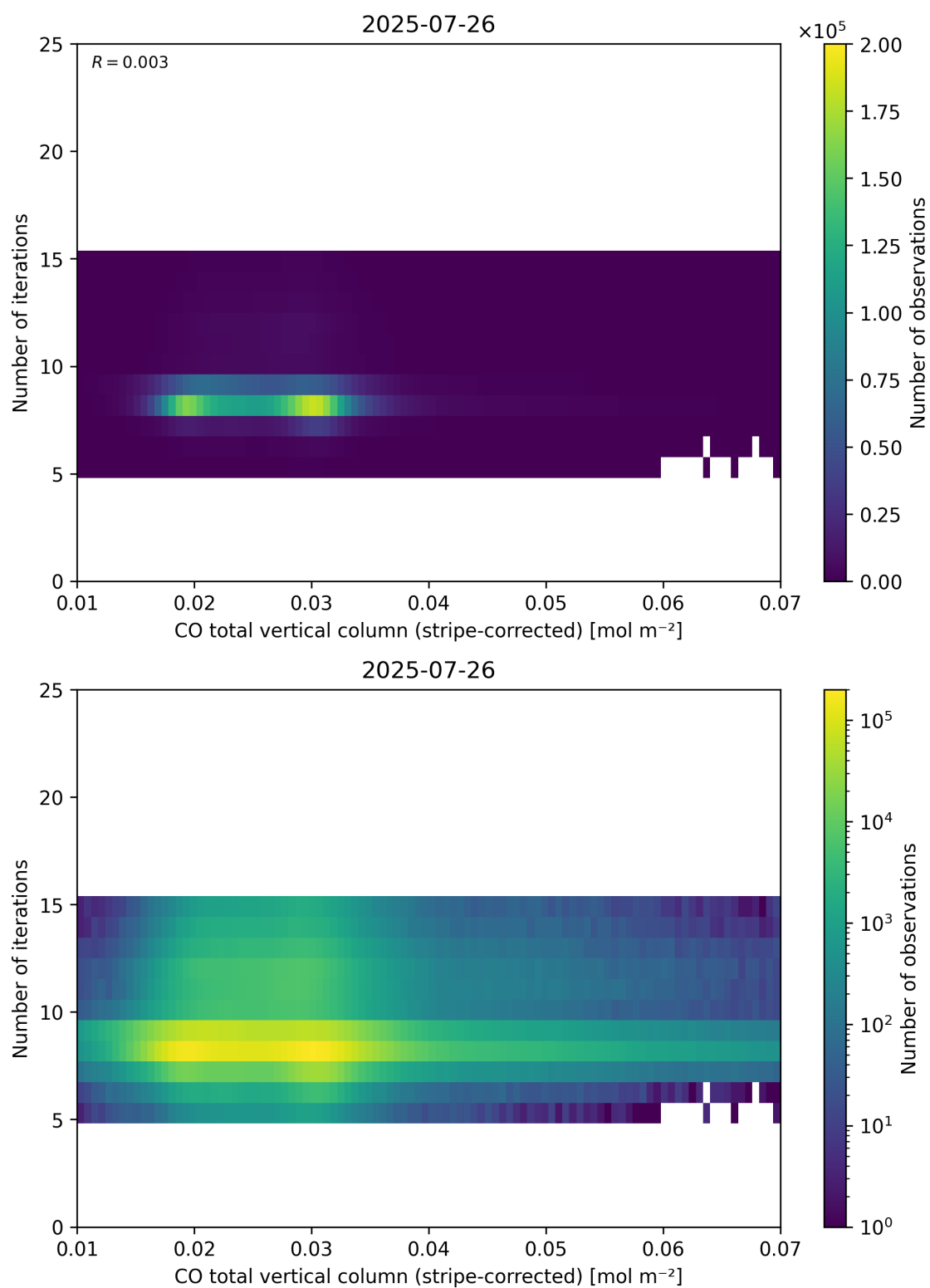
Figure 39: Scatter density plot of “CO total vertical column (stripe-corrected)” against “Number of iterations” for 2025-07-25 to 2025-07-27.
