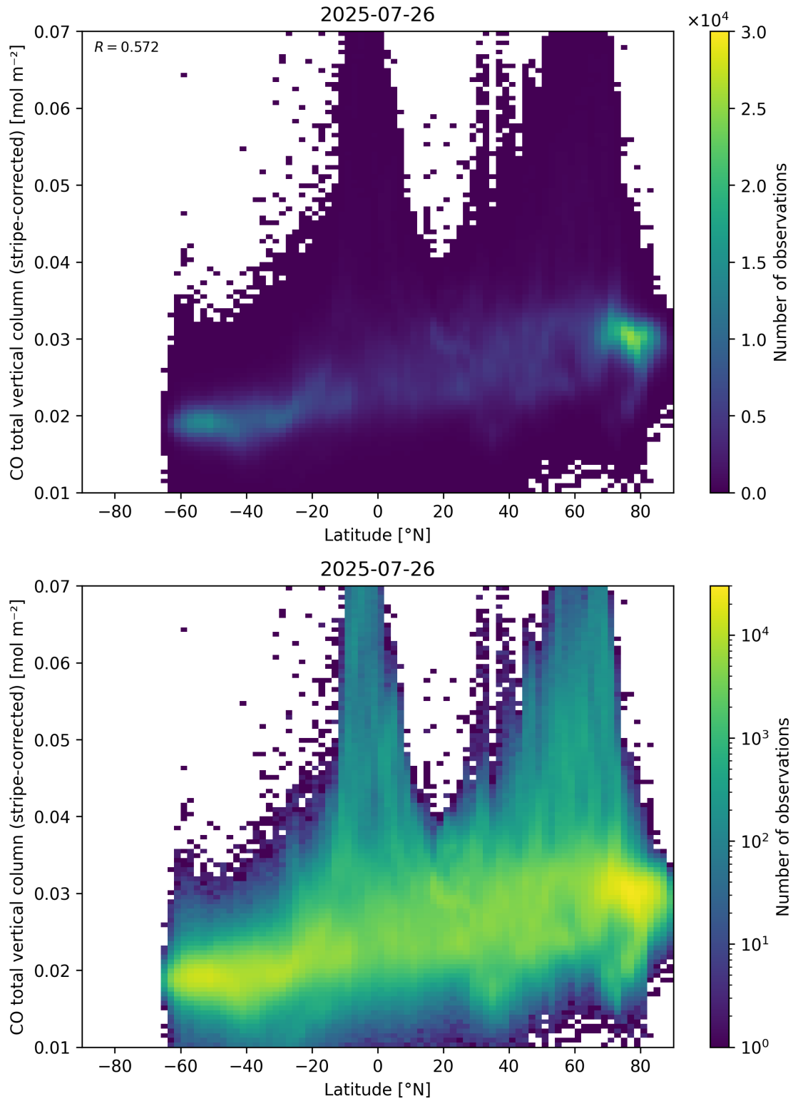
Figure 52: Scatter density plot of “Latitude” against “CO total vertical column (stripe-corrected)” for 2025-07-25 to 2025-07-27.
