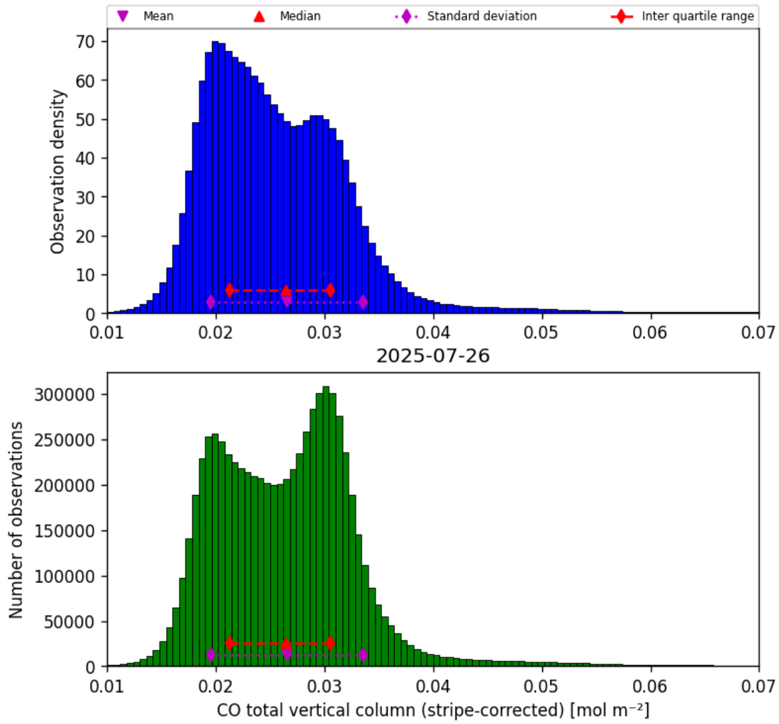
Figure 19: Histogram of “CO total vertical column (stripe-corrected)” for 2025-07-25 to 2025-07-27
