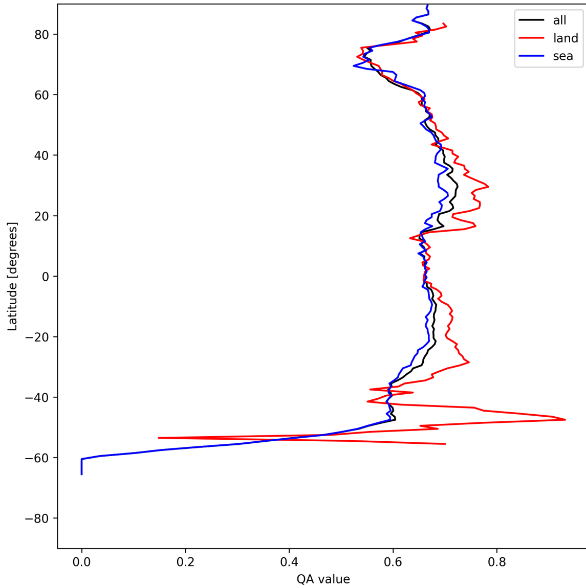
Figure 9: Zonal average of “QA value” for 2025-07-25 to 2025-07-27.
