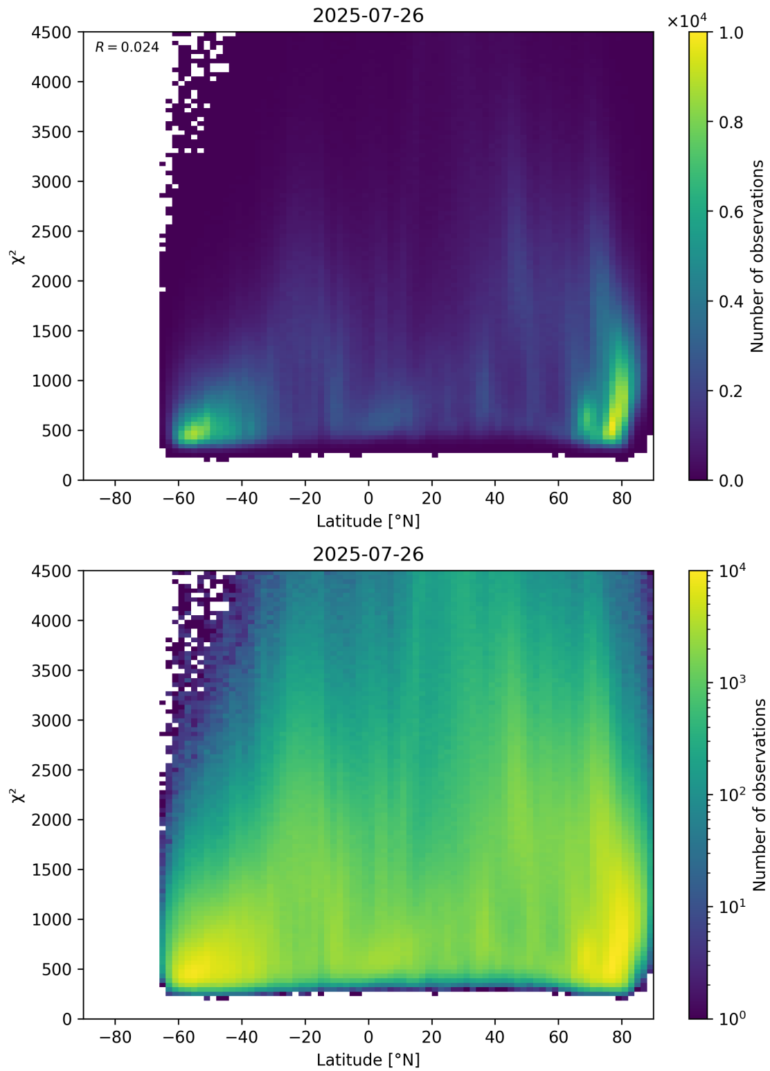
Figure 54: Scatter density plot of “Latitude” against “ \chi^2 ” for 2025-07-25 to 2025-07-27.
