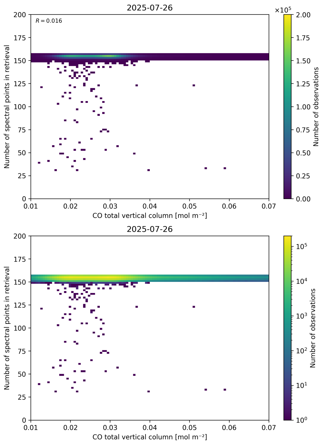
Figure 43: Scatter density plot of “CO total vertical column” against “Number of spectral points in retrieval” for 2025-07-25 to 2025-07-27.
