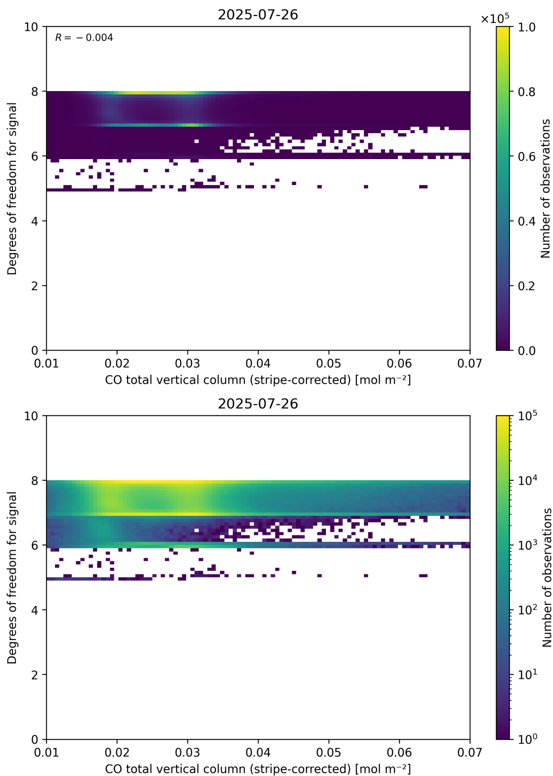
Figure 38: Scatter density plot of “CO total vertical column (stripe-corrected)” against “Degrees of freedom for signal” for 2025-07-25 to 2025-07-27.
