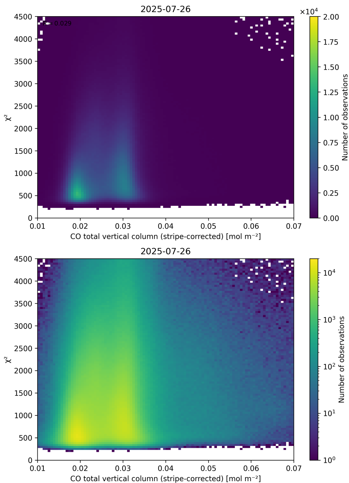
Figure 37: Scatter density plot of “CO total vertical column (stripe-corrected)” against “ \chi^2 ” for 2025-07-25 to 2025-07-27.
