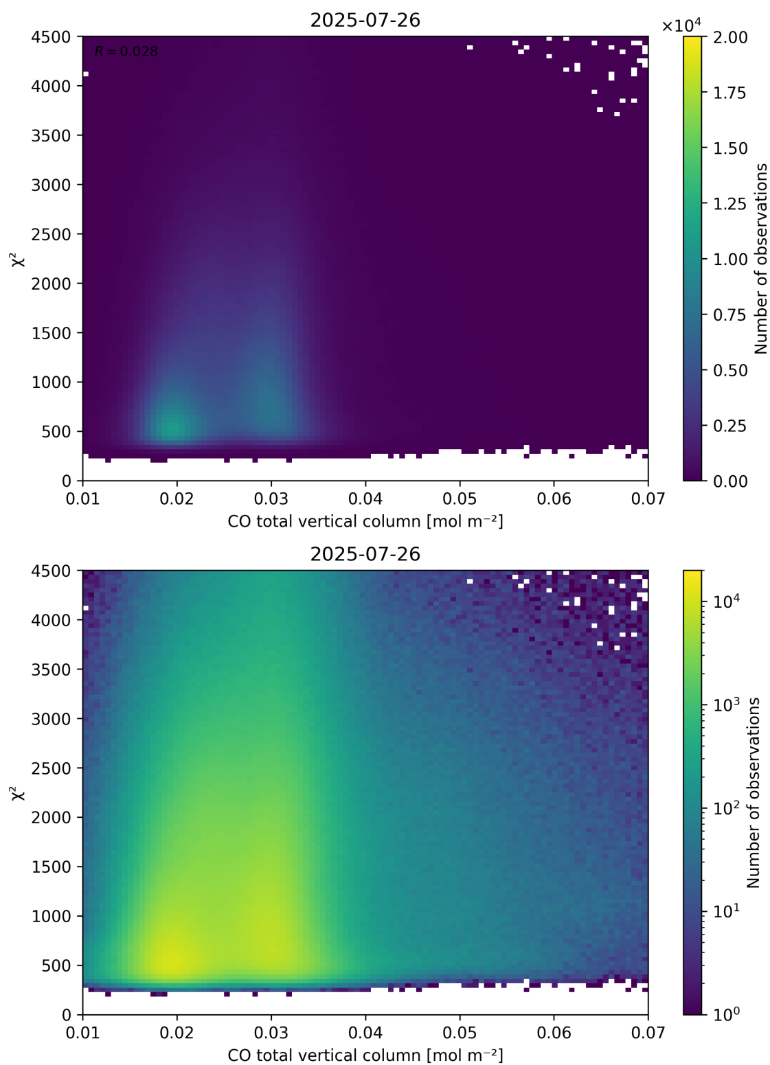
Figure 35: Scatter density plot of “CO total vertical column” against “ \chi^2 ” for 2025-07-25 to 2025-07-27.
