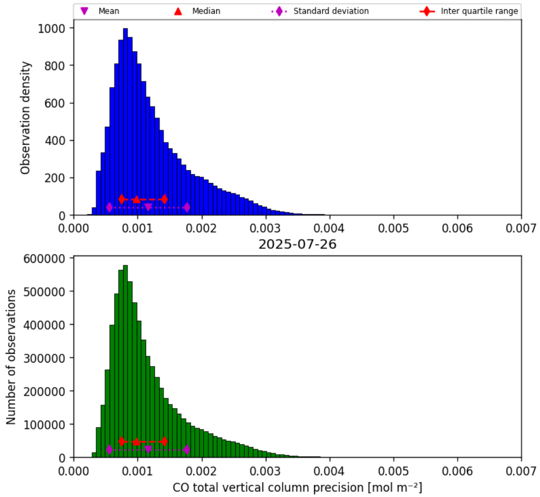
Figure 20: Histogram of “CO total vertical column precision” for 2025-07-25 to 2025-07-27
