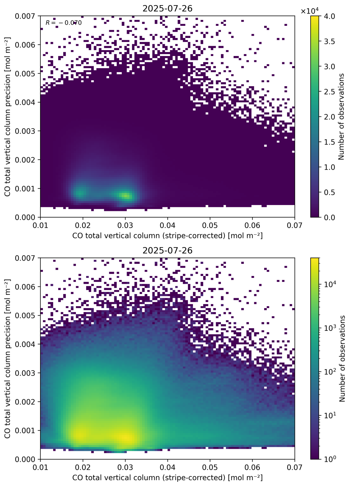
Figure 36: Scatter density plot of “CO total vertical column (stripe-corrected)” against “CO total vertical column precision” for 2025-07-25 to 2025-07-27.
