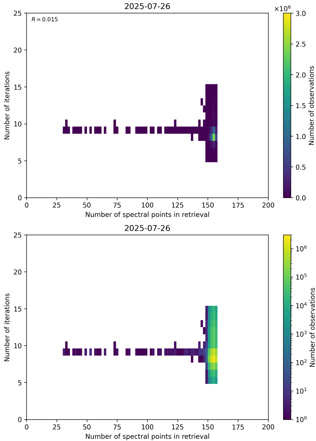
Figure 60: Scatter density plot of “Number of spectral points in retrieval” against “Number of iterations” for 2025-07-25 to 2025-07-27.
