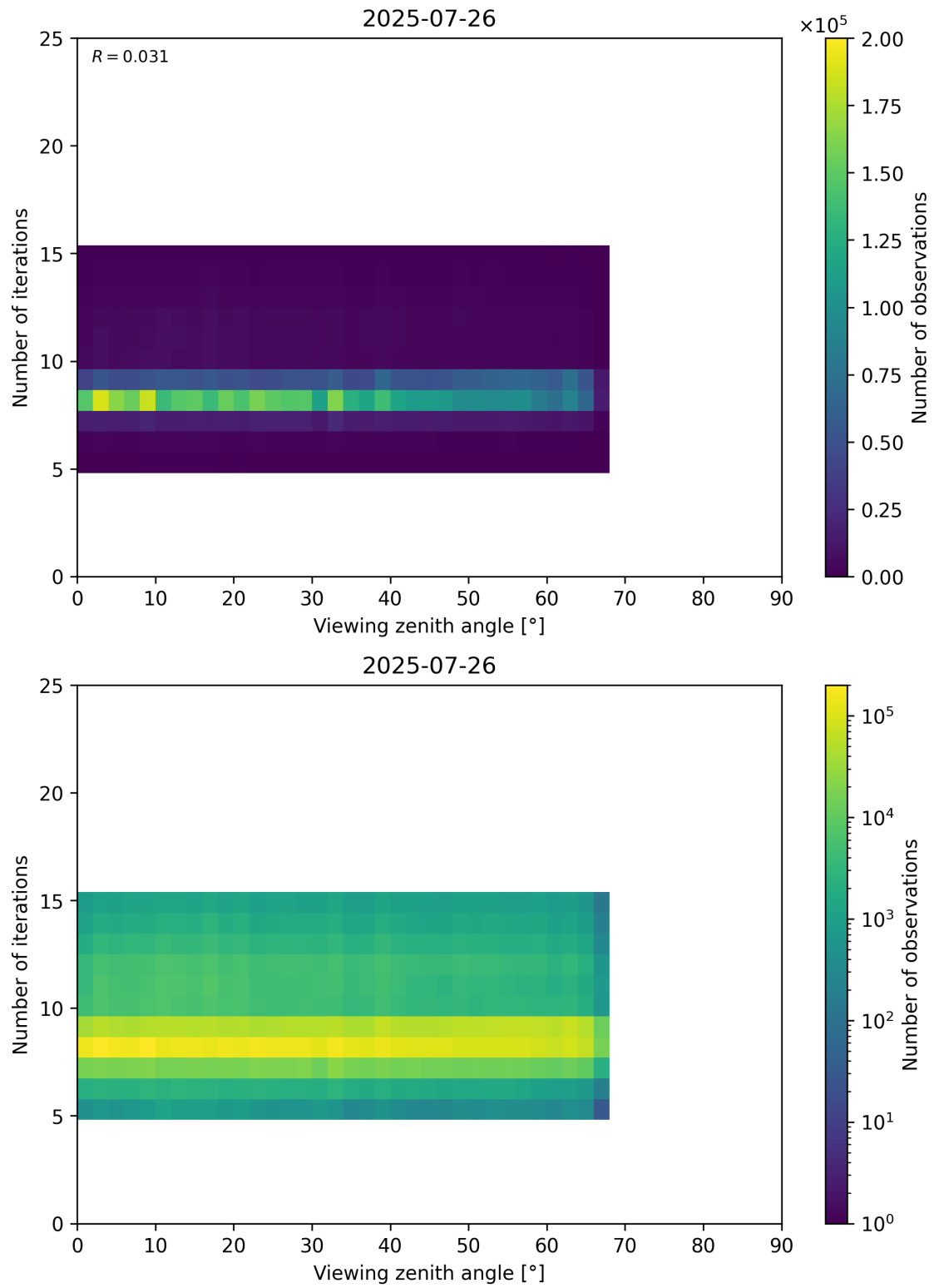
Figure 75: Scatter density plot of “Viewing zenith angle” against “Number of iterations” for 2025-07-25 to 2025-07-27.
