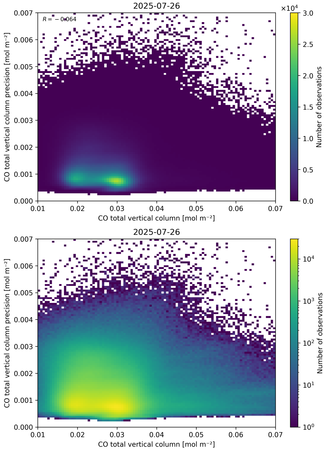
Figure 34: Scatter density plot of “CO total vertical column” against “CO total vertical column precision” for 2025-07-25 to 2025-07-27.
