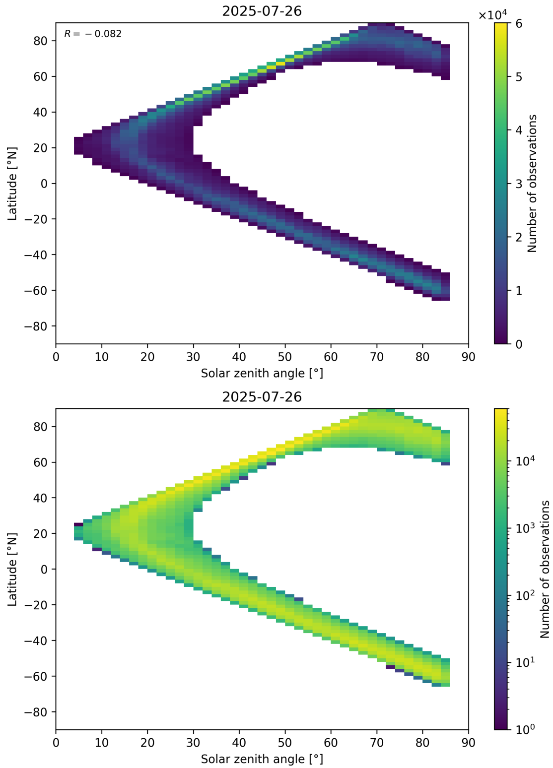
Figure 66: Scatter density plot of “Solar zenith angle” against “Latitude” for 2025-07-25 to 2025-07-27.
