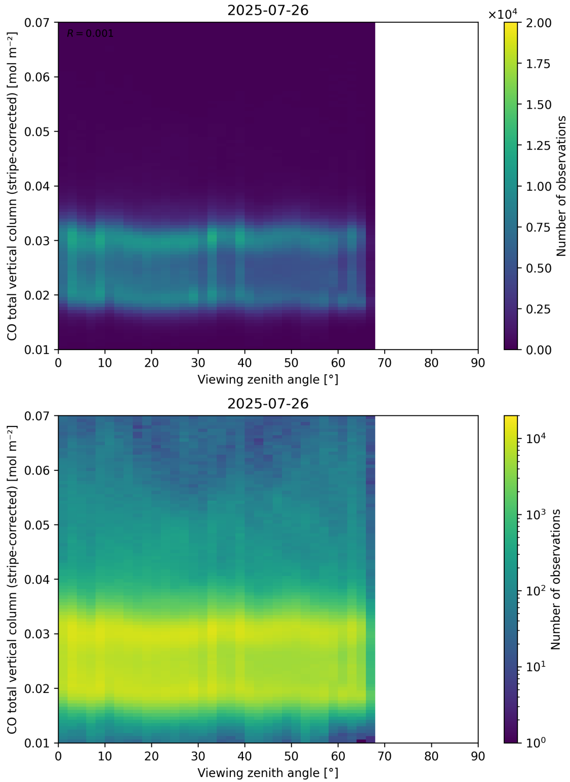
Figure 70: Scatter density plot of “Viewing zenith angle” against “CO total vertical column (stripe-corrected)” for 2025-07-25 to 2025-07-27.
