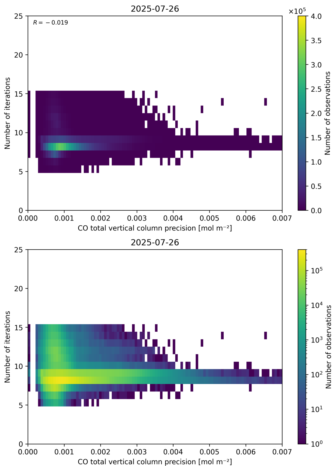
Figure 46: Scatter density plot of “CO total vertical column precision” against “Number of iterations” for 2025-07-25 to 2025-07-27.
