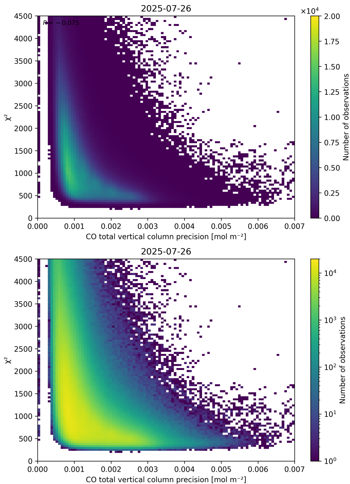
Figure 44: Scatter density plot of “CO total vertical column precision” against “ \chi^2 ” for 2025-07-25 to 2025-07-27.
