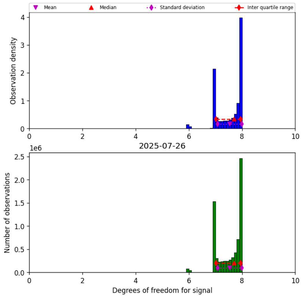
Figure 23: Histogram of “Degrees of freedom for signal” for 2025-07-25 to 2025-07-27
