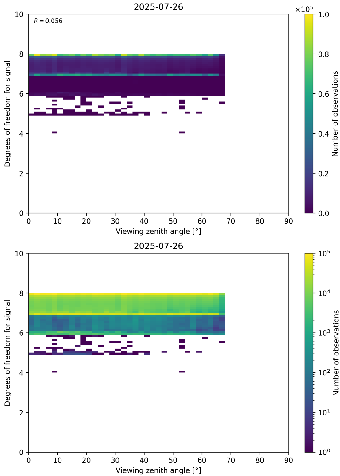
Figure 73: Scatter density plot of “Viewing zenith angle” against “Degrees of freedom for signal” for 2025-07-25 to 2025-07-27.
