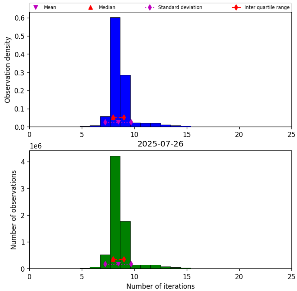
Figure 24: Histogram of “Number of iterations” for 2025-07-25 to 2025-07-27
