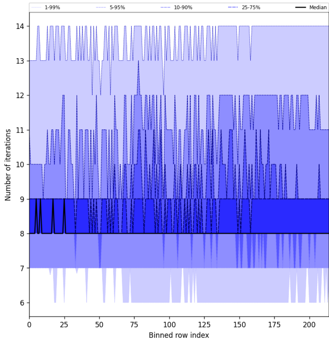
Figure 32: Along track statistics of “Number of iterations” for 2025-07-25 to 2025-07-27
