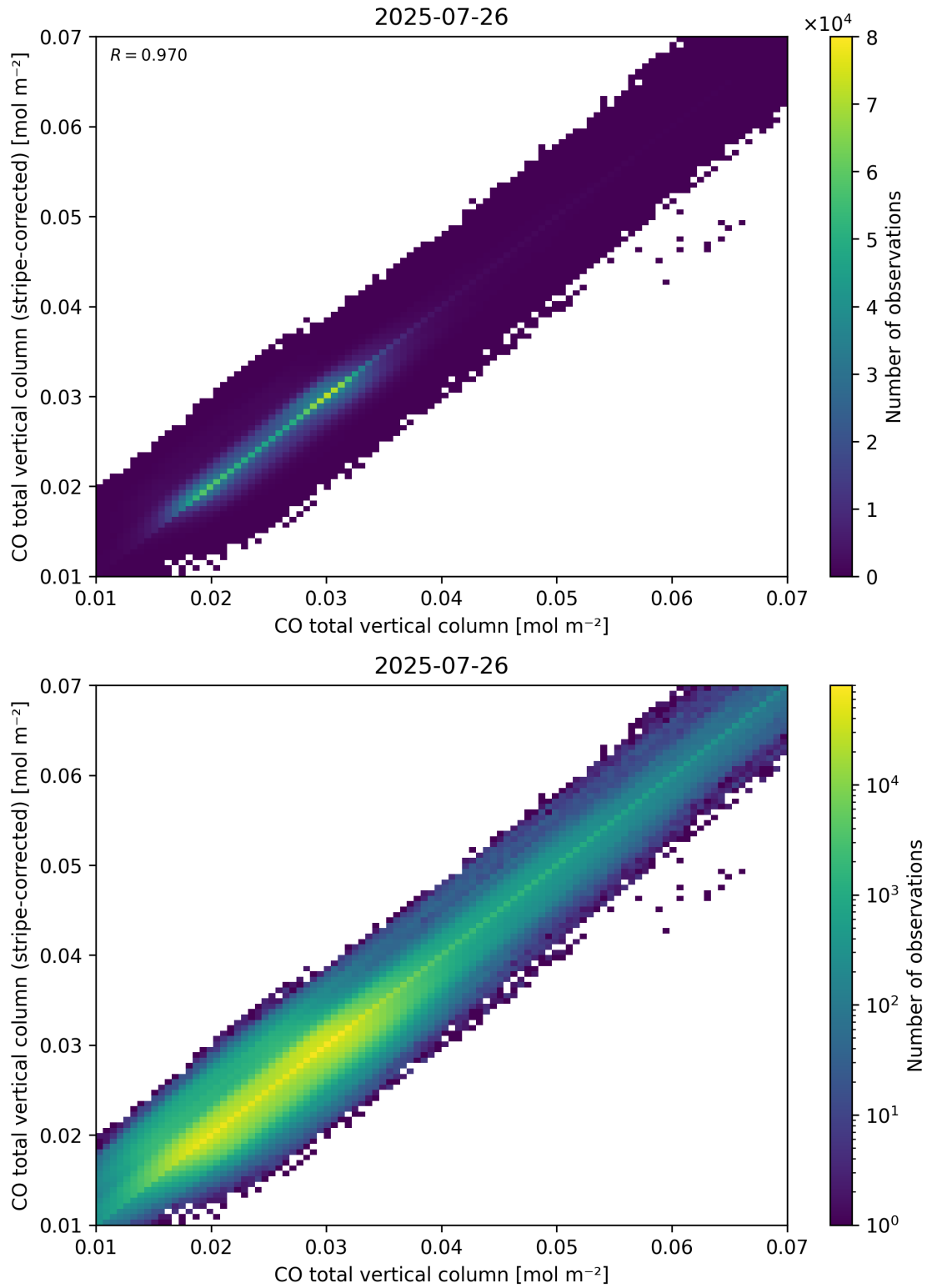
Figure 33: Scatter density plot of “CO total vertical column” against “CO total vertical column (stripe-corrected)” for 2025-07-25 to 2025-07-27.
