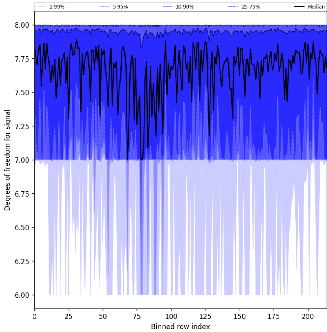
Figure 31: Along track statistics of “Degrees of freedom for signal” for 2025-07-26 to 2025-07-28
