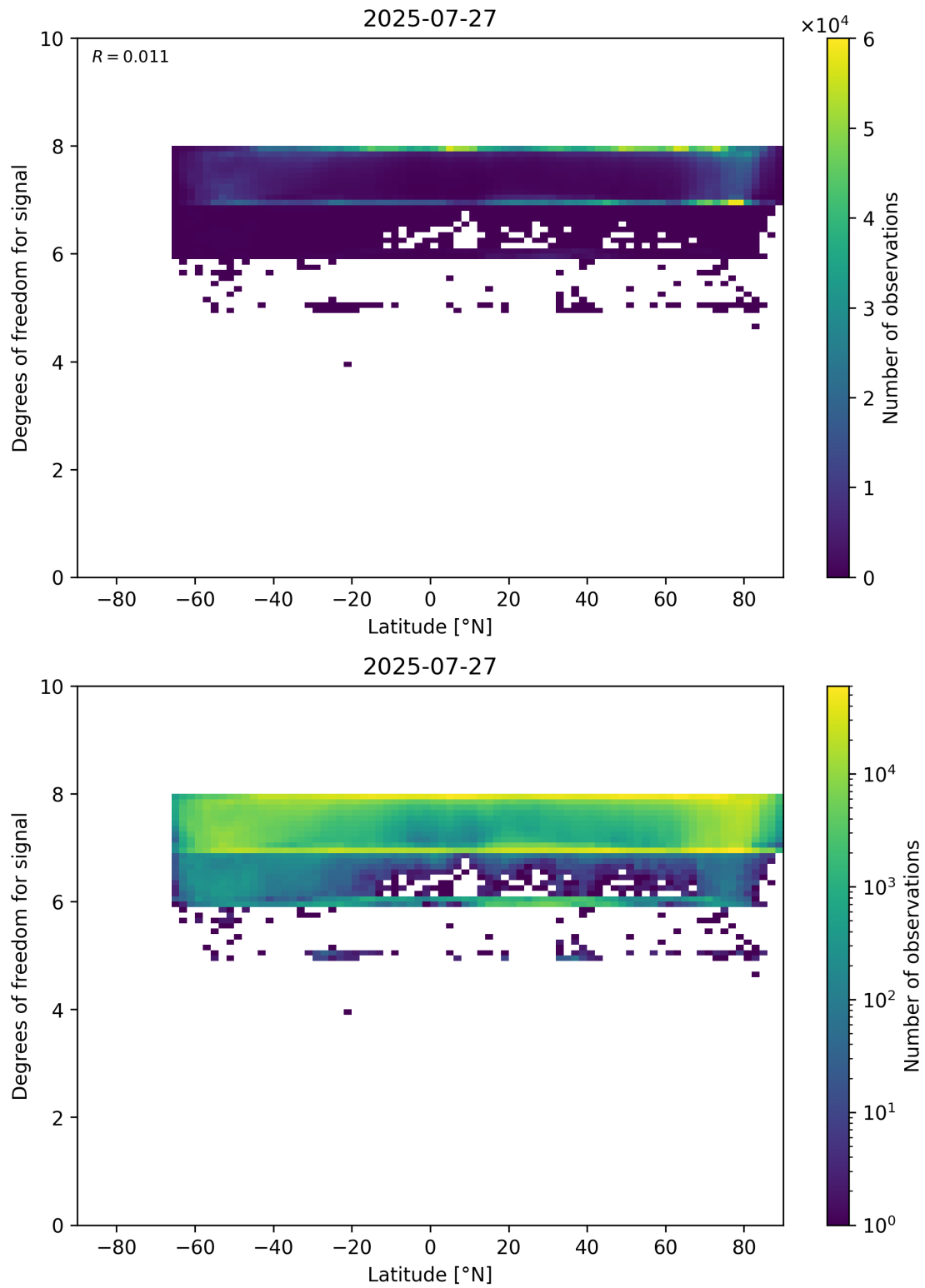
Figure 55: Scatter density plot of “Latitude” against “Degrees of freedom for signal” for 2025-07-26 to 2025-07-28.
