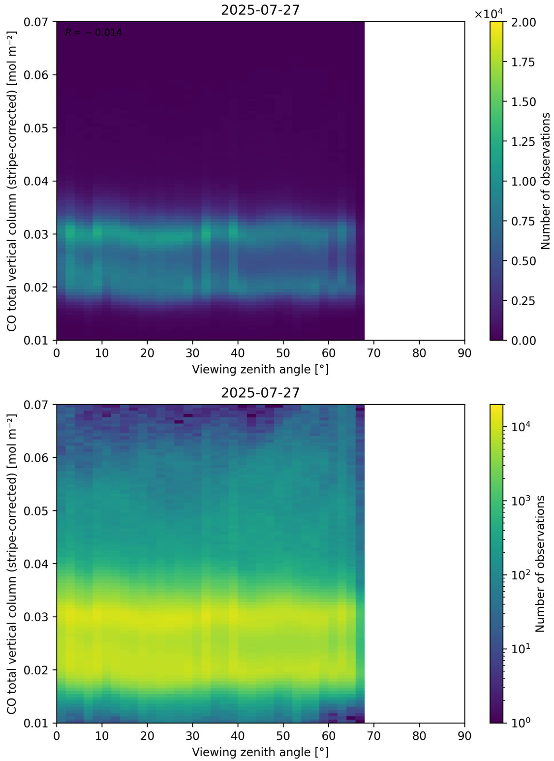
Figure 70: Scatter density plot of “Viewing zenith angle” against “CO total vertical column (stripe-corrected)” for 2025-07-26 to 2025-07-28.
