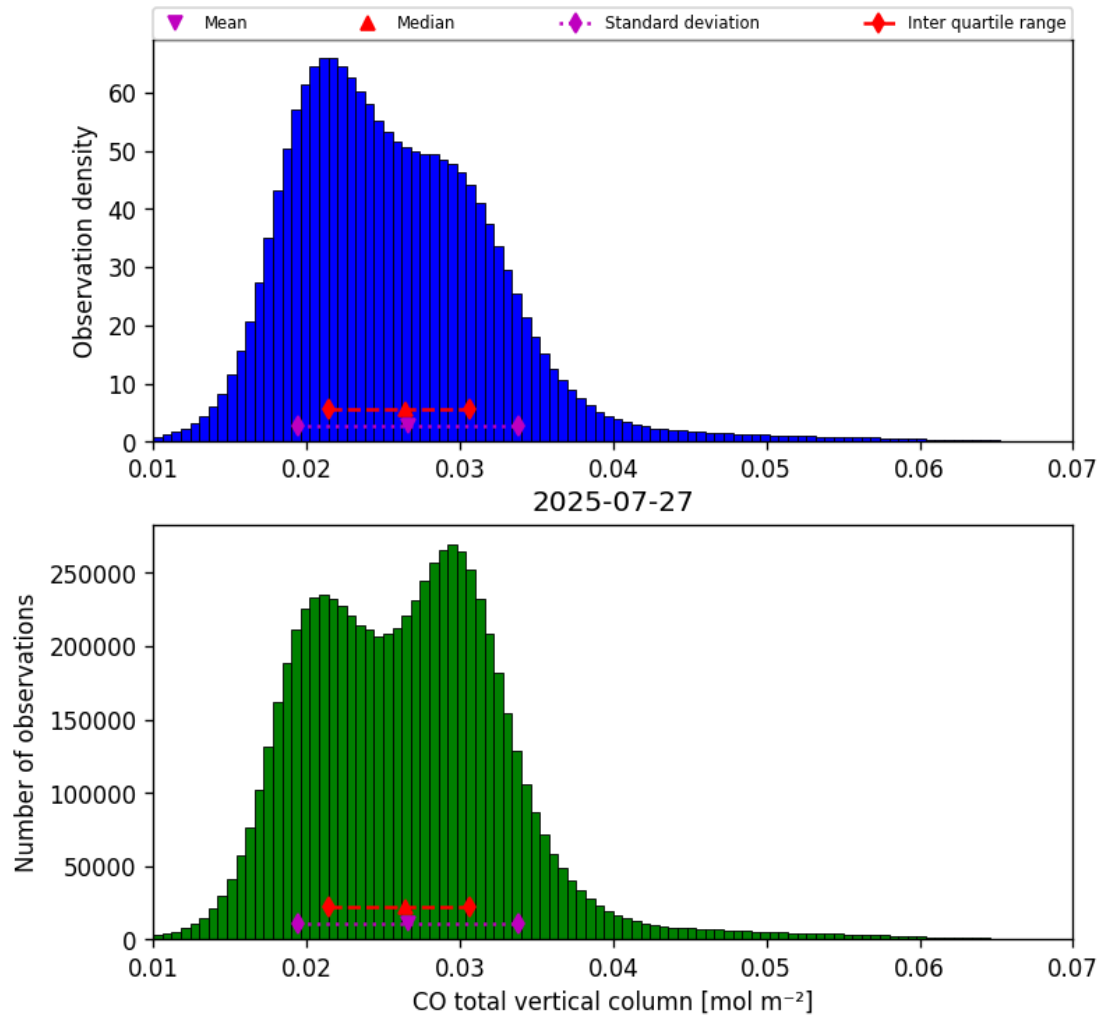
Figure 18: Histogram of “CO total vertical column” for 2025-07-26 to 2025-07-28
