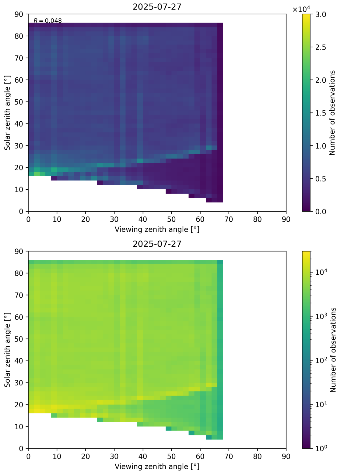
Figure 77: Scatter density plot of “Viewing zenith angle” against “Solar zenith angle” for 2025-07-26 to 2025-07-28.
