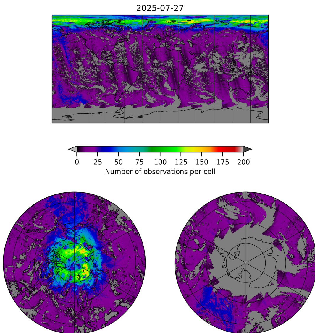
Figure 8: Map of the number of observations for 2025-07-26 to 2025-07-28
