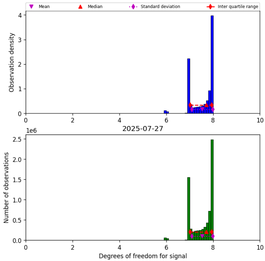
Figure 23: Histogram of “Degrees of freedom for signal” for 2025-07-26 to 2025-07-28
