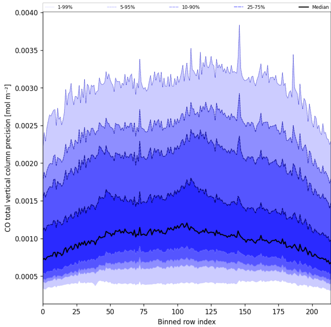
Figure 28: Along track statistics of “CO total vertical column precision” for 2025-07-26 to 2025-07-28
