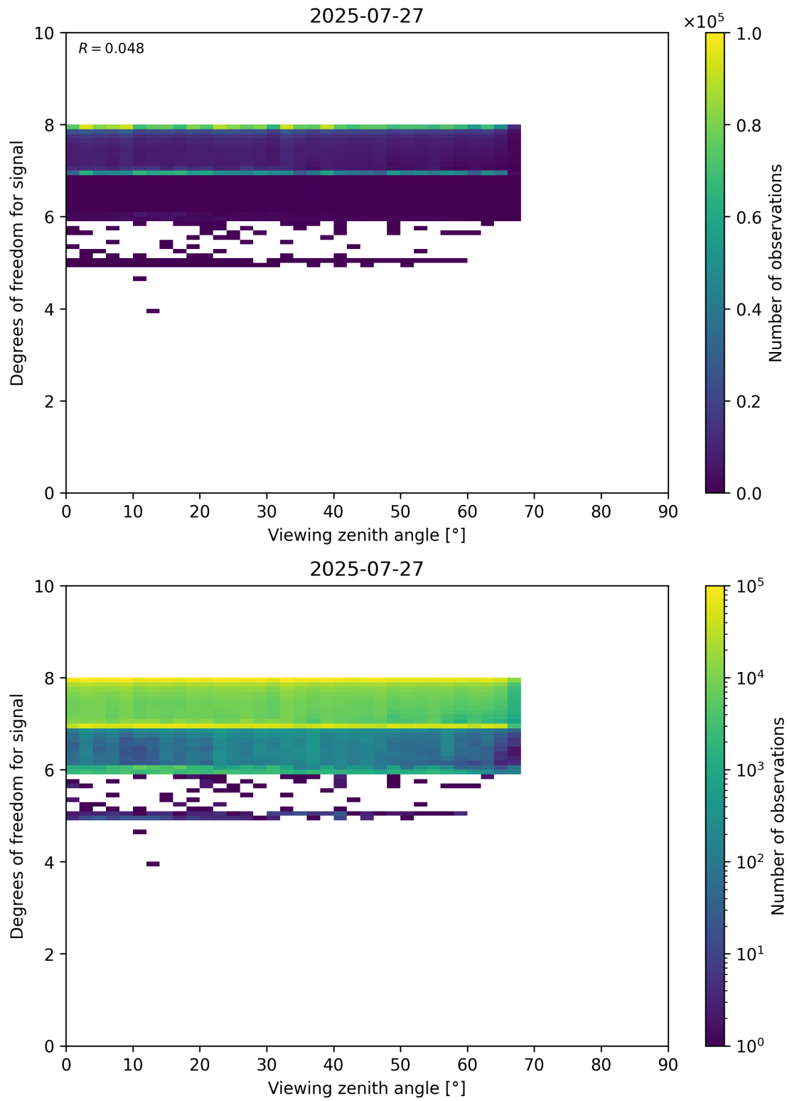
Figure 73: Scatter density plot of “Viewing zenith angle” against “Degrees of freedom for signal” for 2025-07-26 to 2025-07-28.
