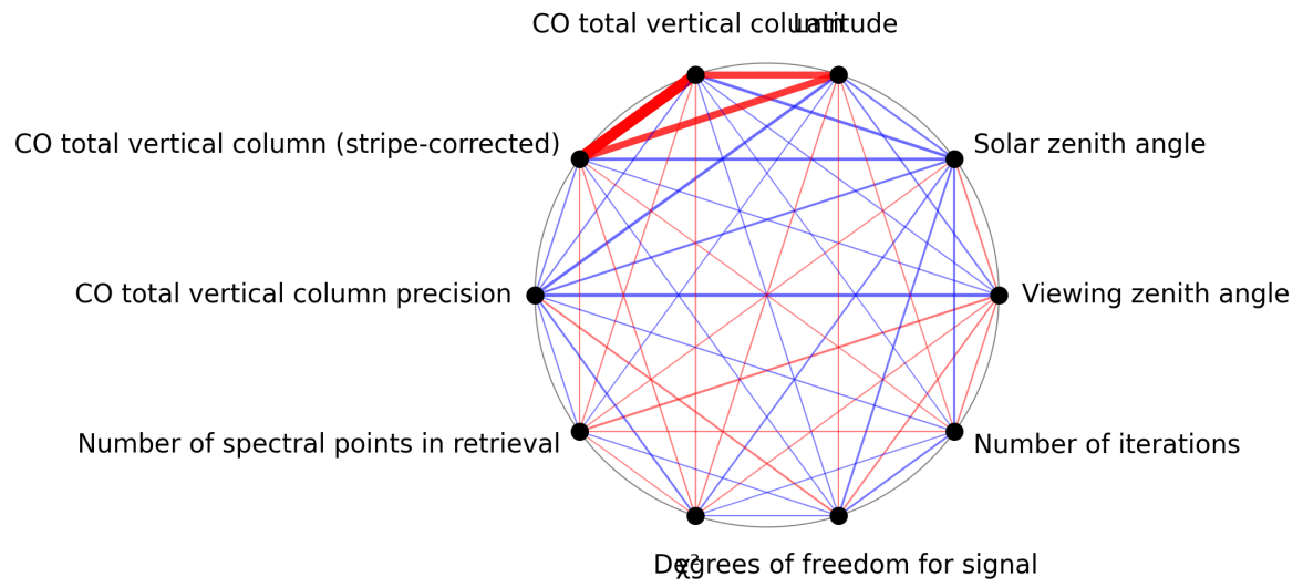
Figure 1: Map of correlation graph for 2025-07-26 to 2025-07-28.
