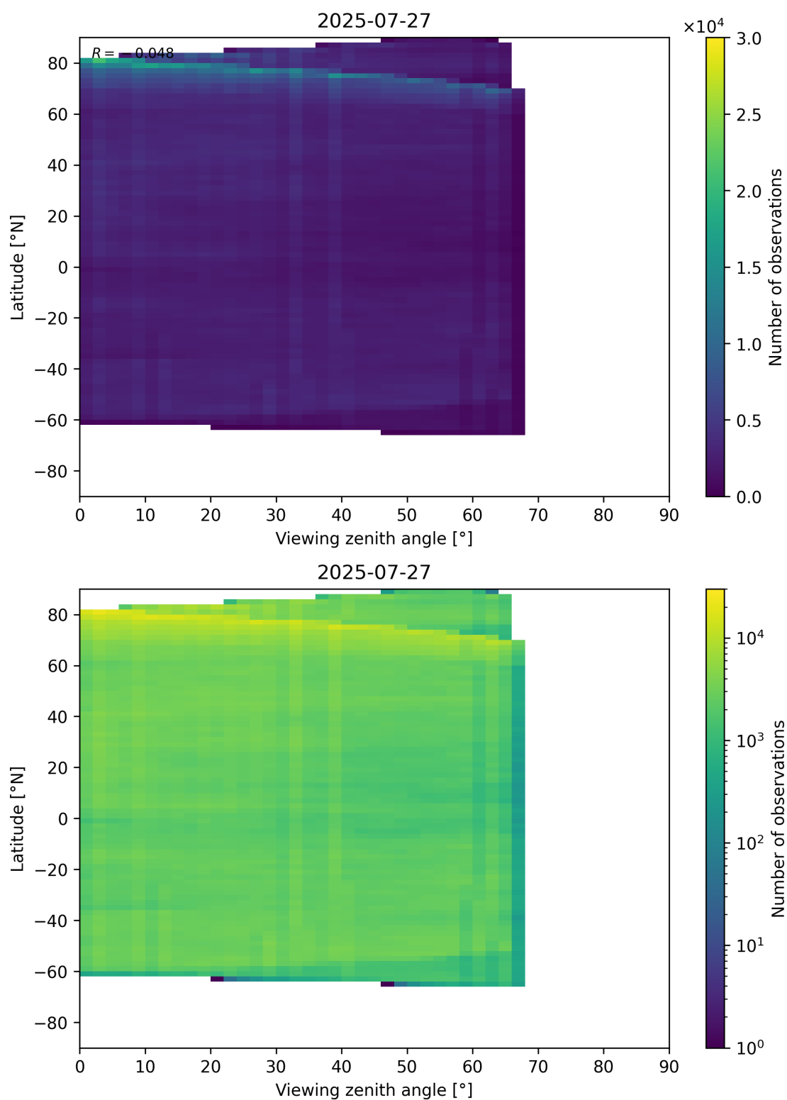
Figure 74: Scatter density plot of “Viewing zenith angle” against “Latitude” for 2025-07-26 to 2025-07-28.
