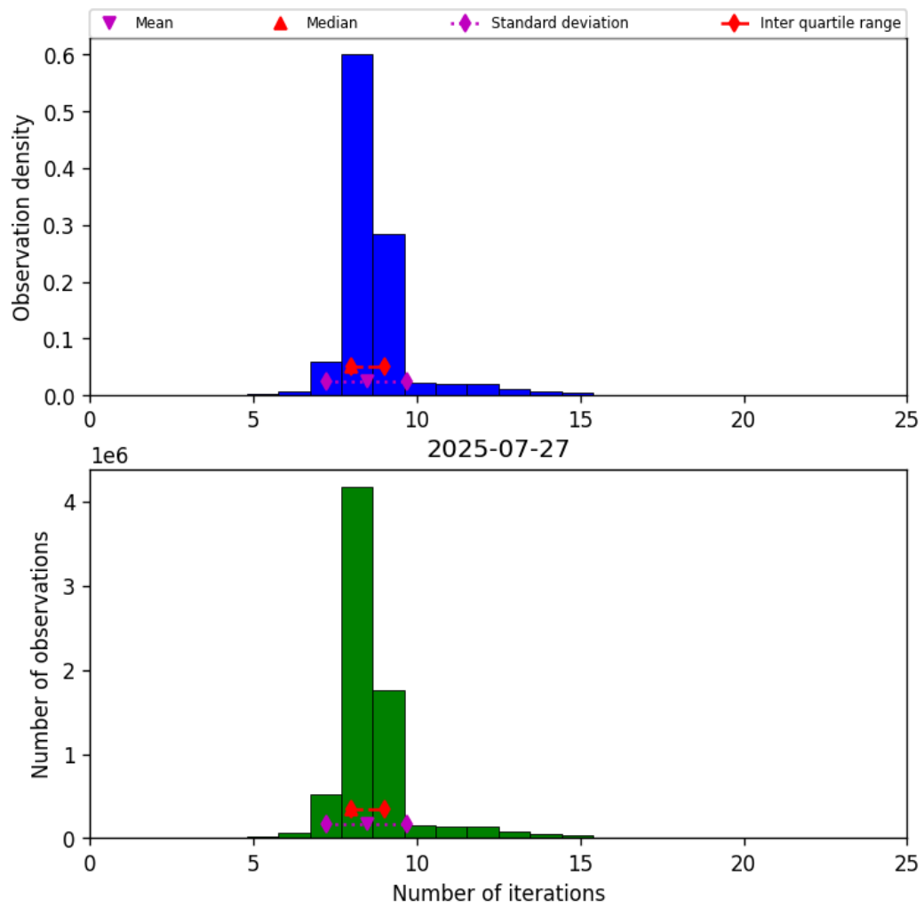
Figure 24: Histogram of “Number of iterations” for 2025-07-26 to 2025-07-28
