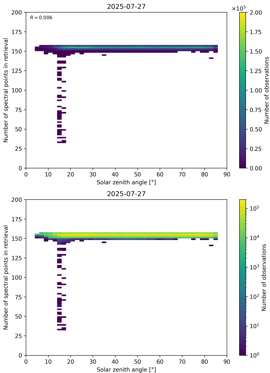
Figure 68: Scatter density plot of “Solar zenith angle” against “Number of spectral points in retrieval” for 2025-07-26 to 2025-07-28.
