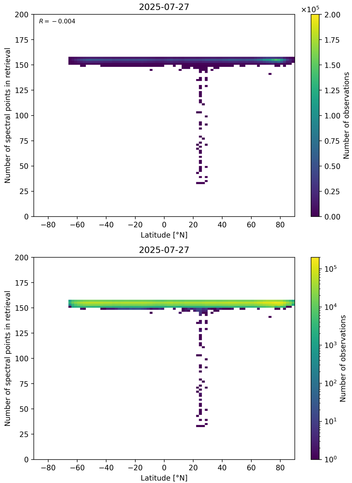
Figure 57: Scatter density plot of “Latitude” against “Number of spectral points in retrieval” for 2025-07-26 to 2025-07-28.
