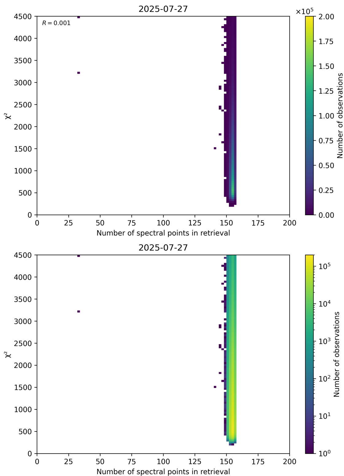
Figure 58: Scatter density plot of “Number of spectral points in retrieval” against “ \chi^2 ” for 2025-07-26 to 2025-07-28.
