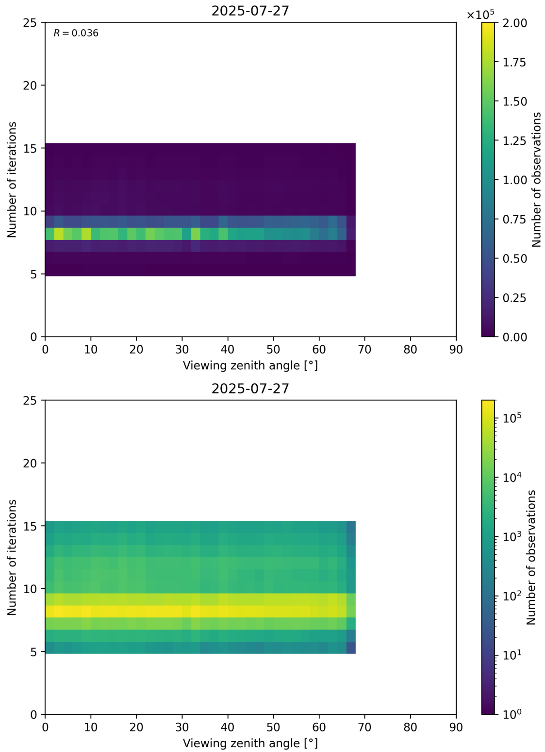
Figure 75: Scatter density plot of “Viewing zenith angle” against “Number of iterations” for 2025-07-26 to 2025-07-28.
