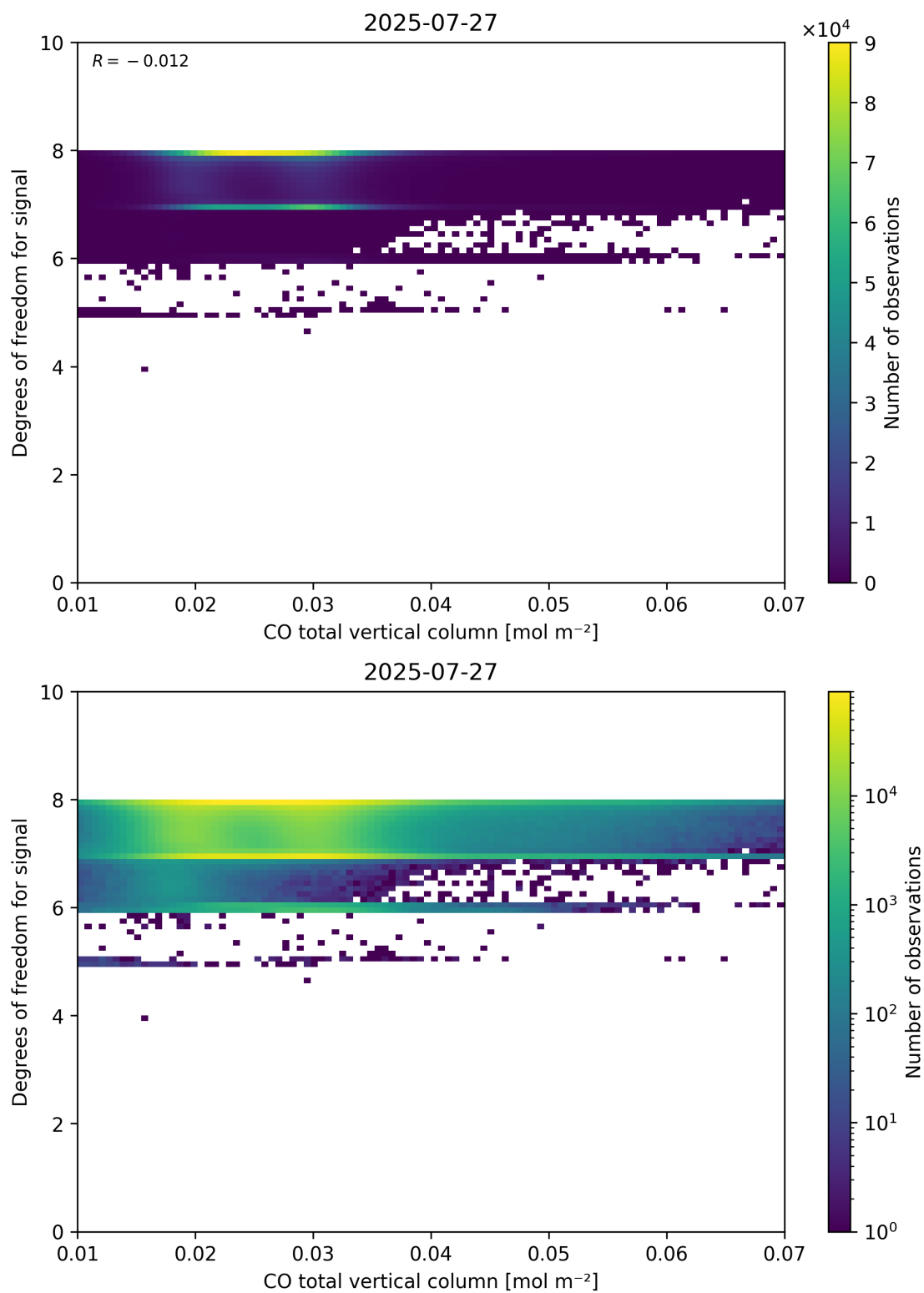
Figure 41: Scatter density plot of “CO total vertical column” against “Degrees of freedom for signal” for 2025-07-26 to 2025-07-28.
