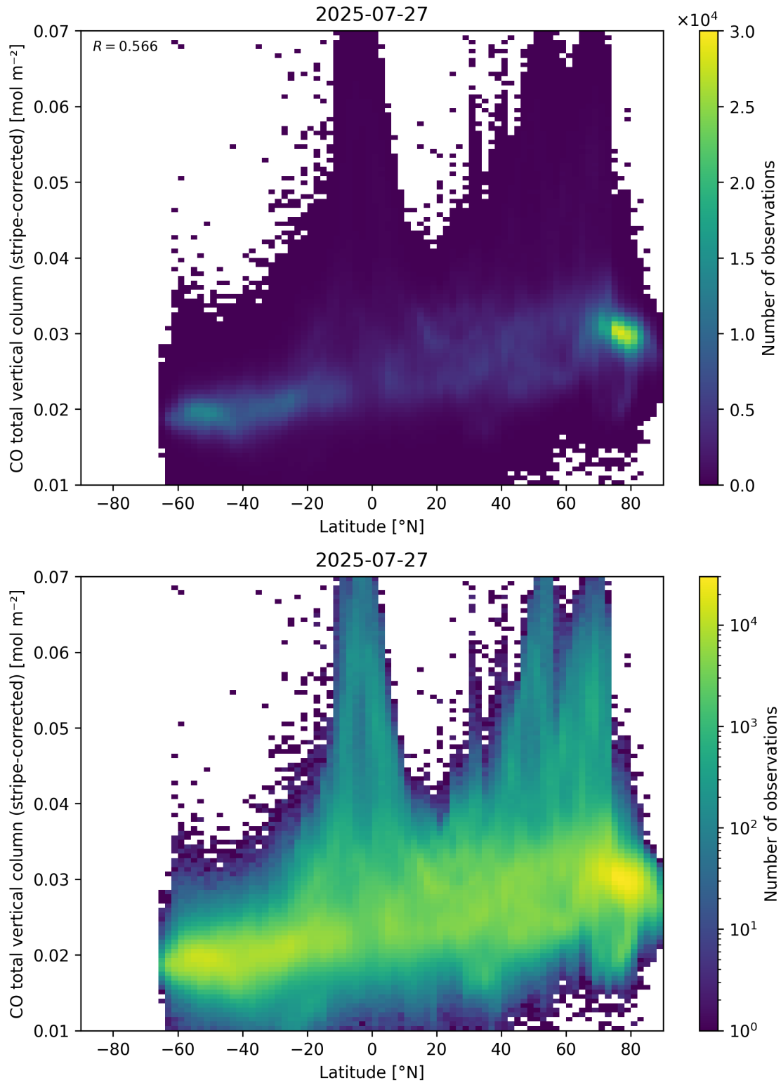
Figure 52: Scatter density plot of “Latitude” against “CO total vertical column (stripe-corrected)” for 2025-07-26 to 2025-07-28.
