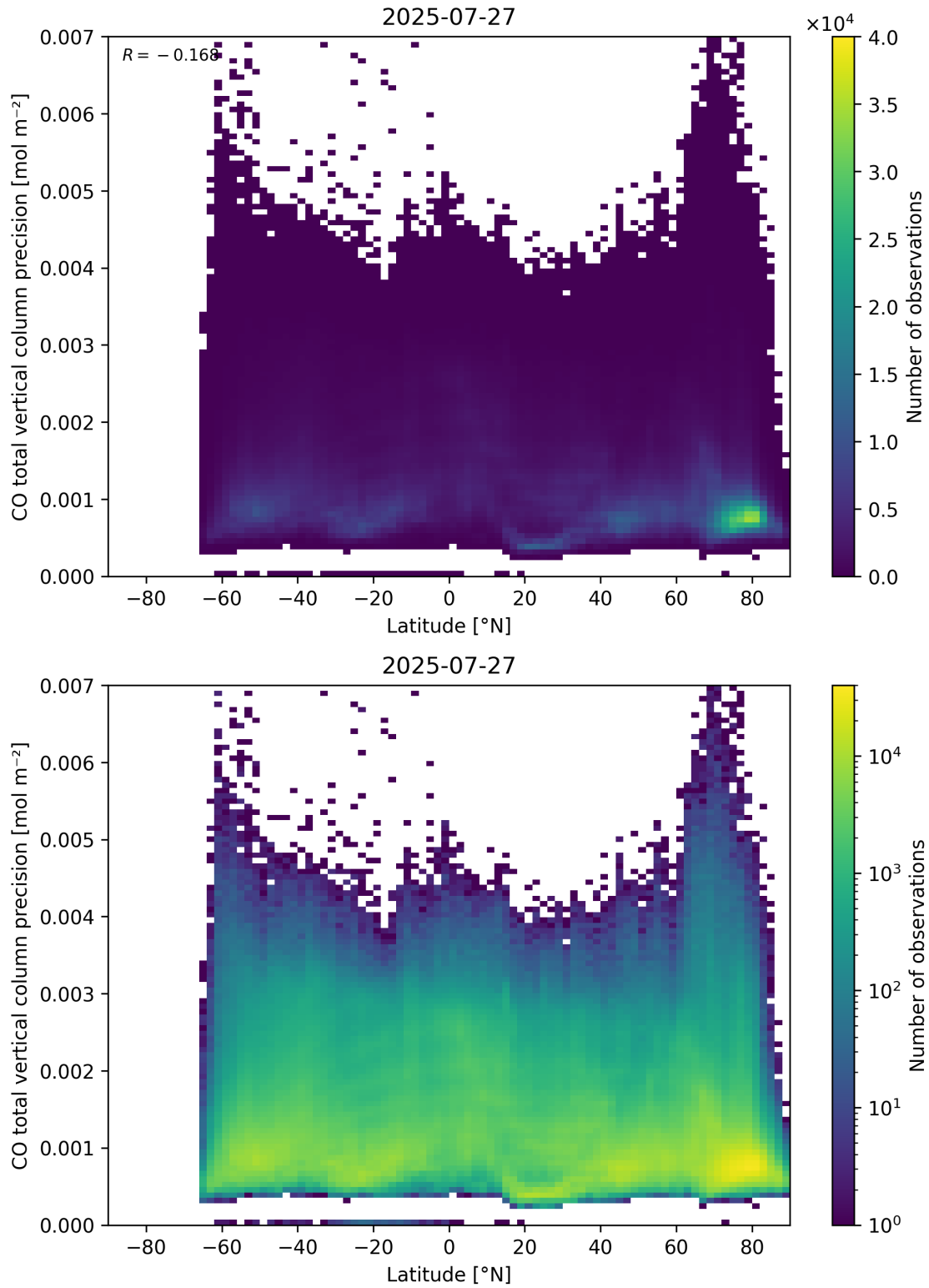
Figure 53: Scatter density plot of “Latitude” against “CO total vertical column precision” for 2025-07-26 to 2025-07-28.
