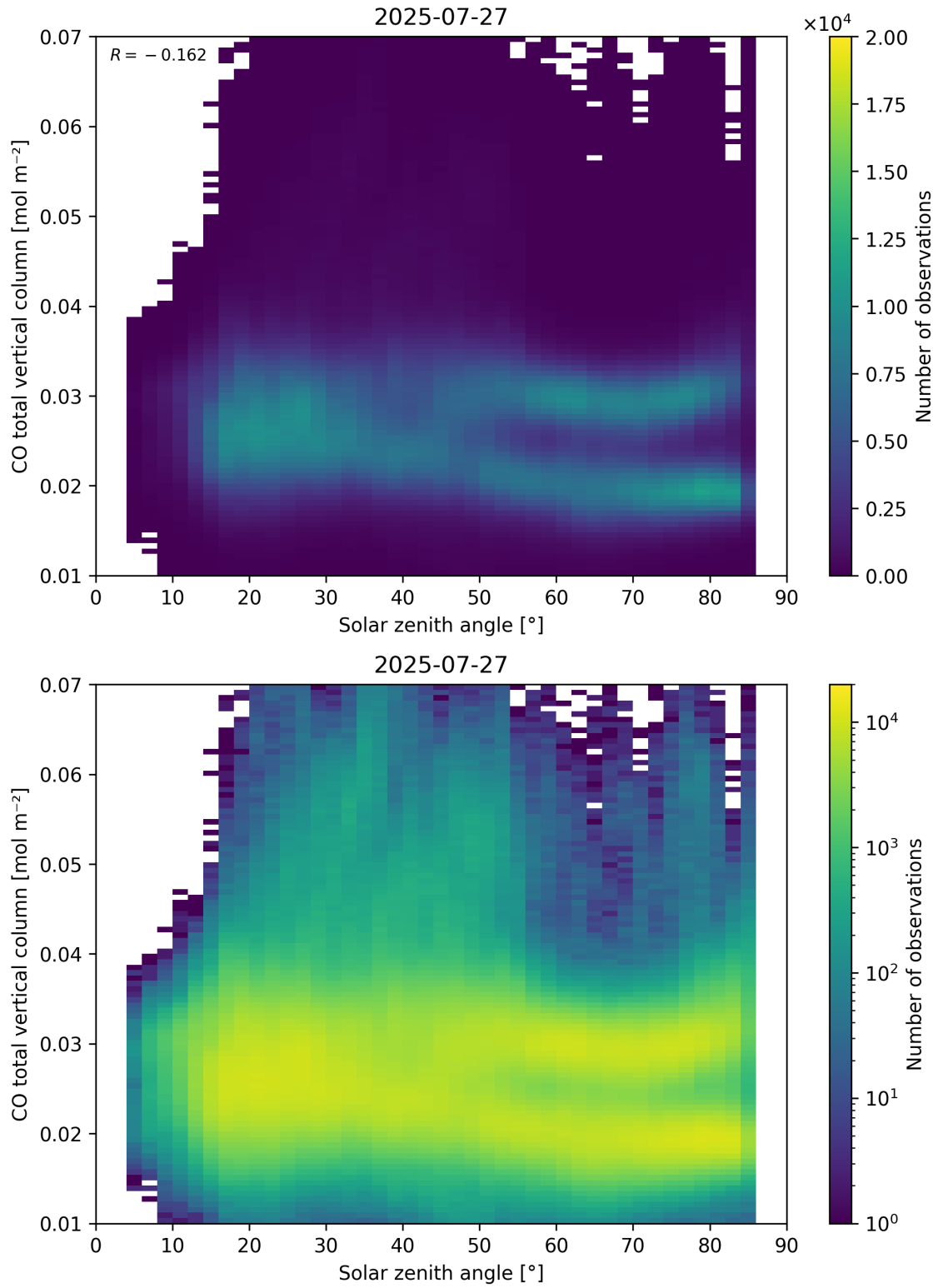
Figure 61: Scatter density plot of “Solar zenith angle” against “CO total vertical column” for 2025-07-26 to 2025-07-28.
