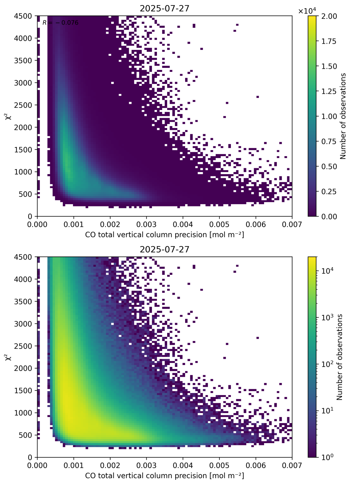
Figure 44: Scatter density plot of “CO total vertical column precision” against “ \chi^2 ” for 2025-07-26 to 2025-07-28.
