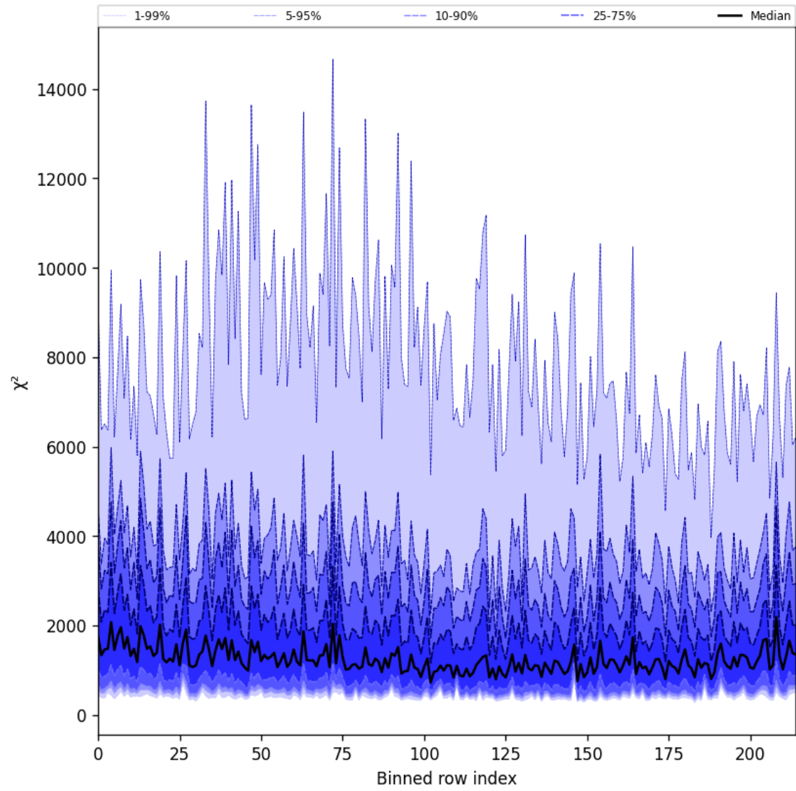
Figure 30: Along track statistics of “ \chi^2 ” for 2025-07-26 to 2025-07-28
