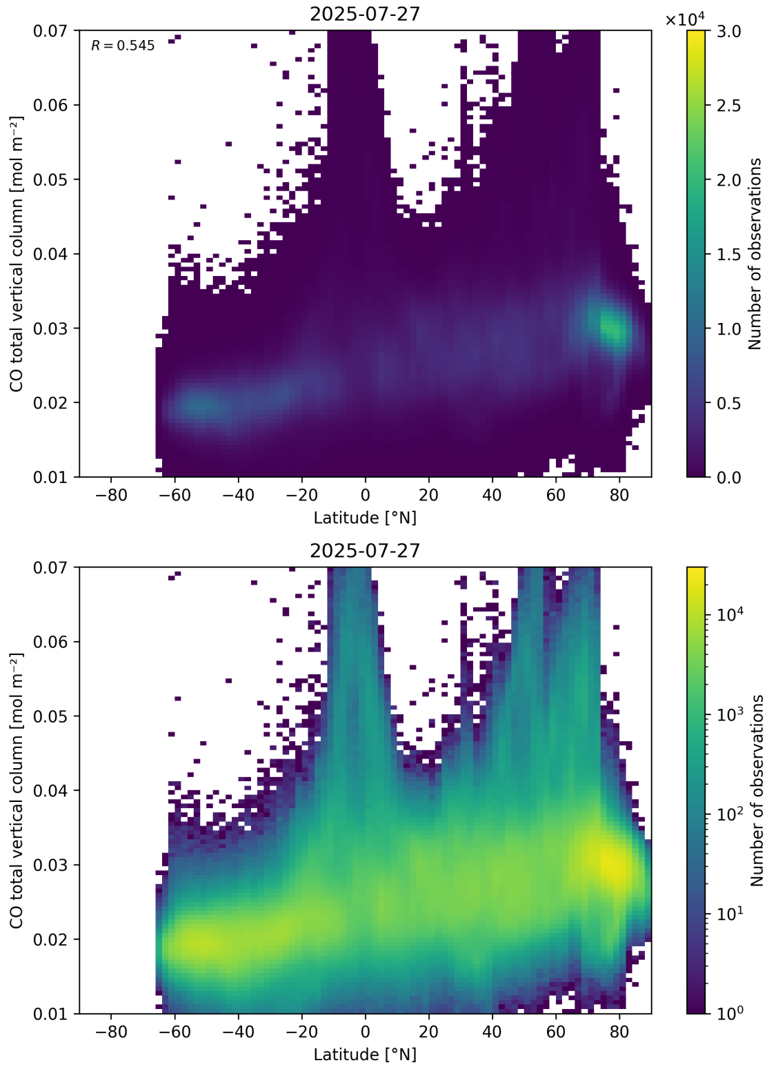
Figure 51: Scatter density plot of “Latitude” against “CO total vertical column” for 2025-07-26 to 2025-07-28.
