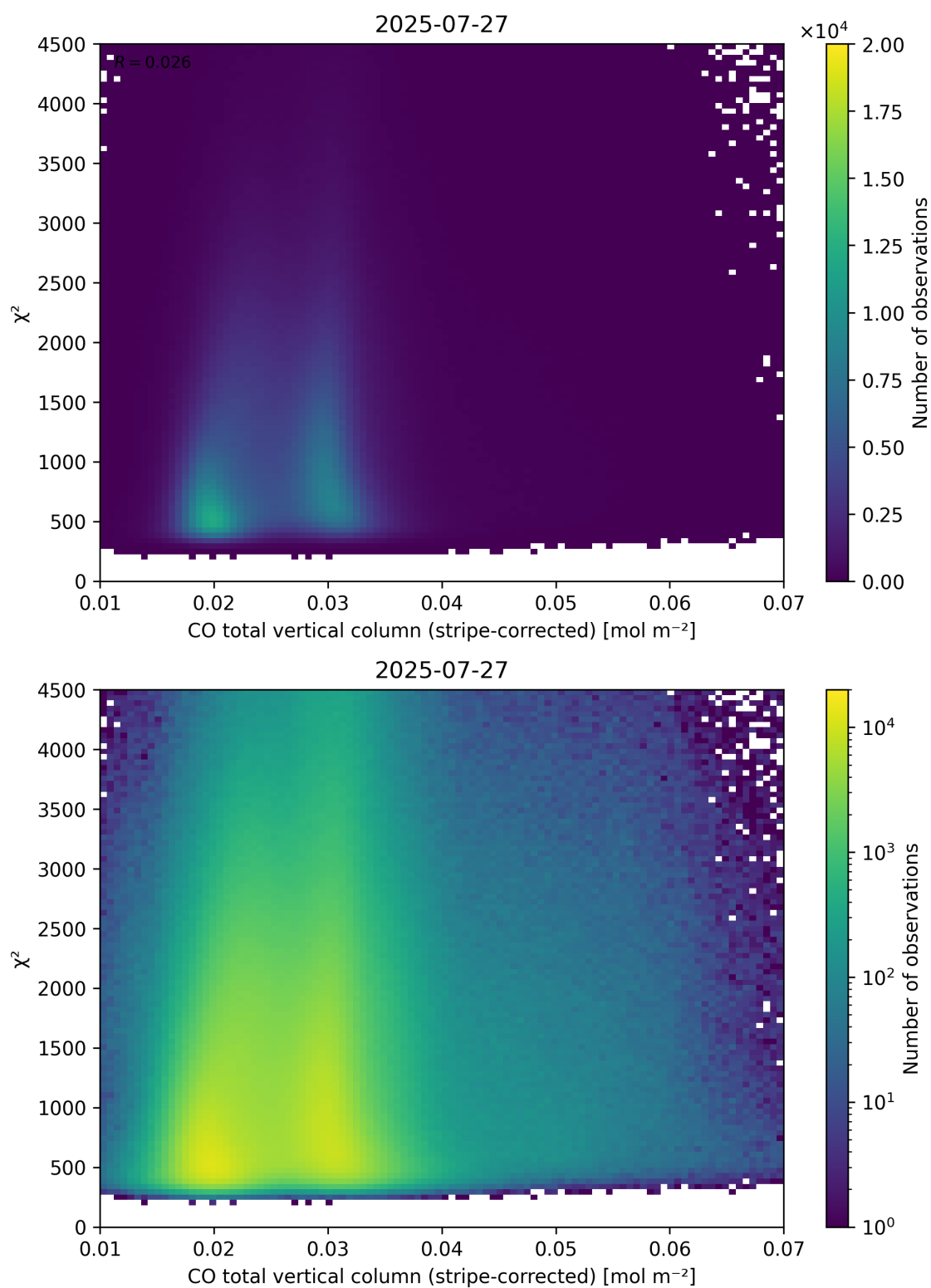
Figure 37: Scatter density plot of “CO total vertical column (stripe-corrected)” against “ \chi^2 ” for 2025-07-26 to 2025-07-28.
