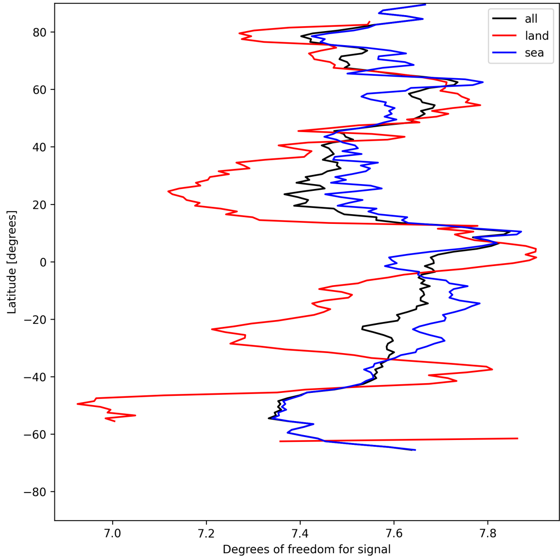
Figure 15: Zonal average of “Degrees of freedom for signal” for 2025-07-26 to 2025-07-28.
