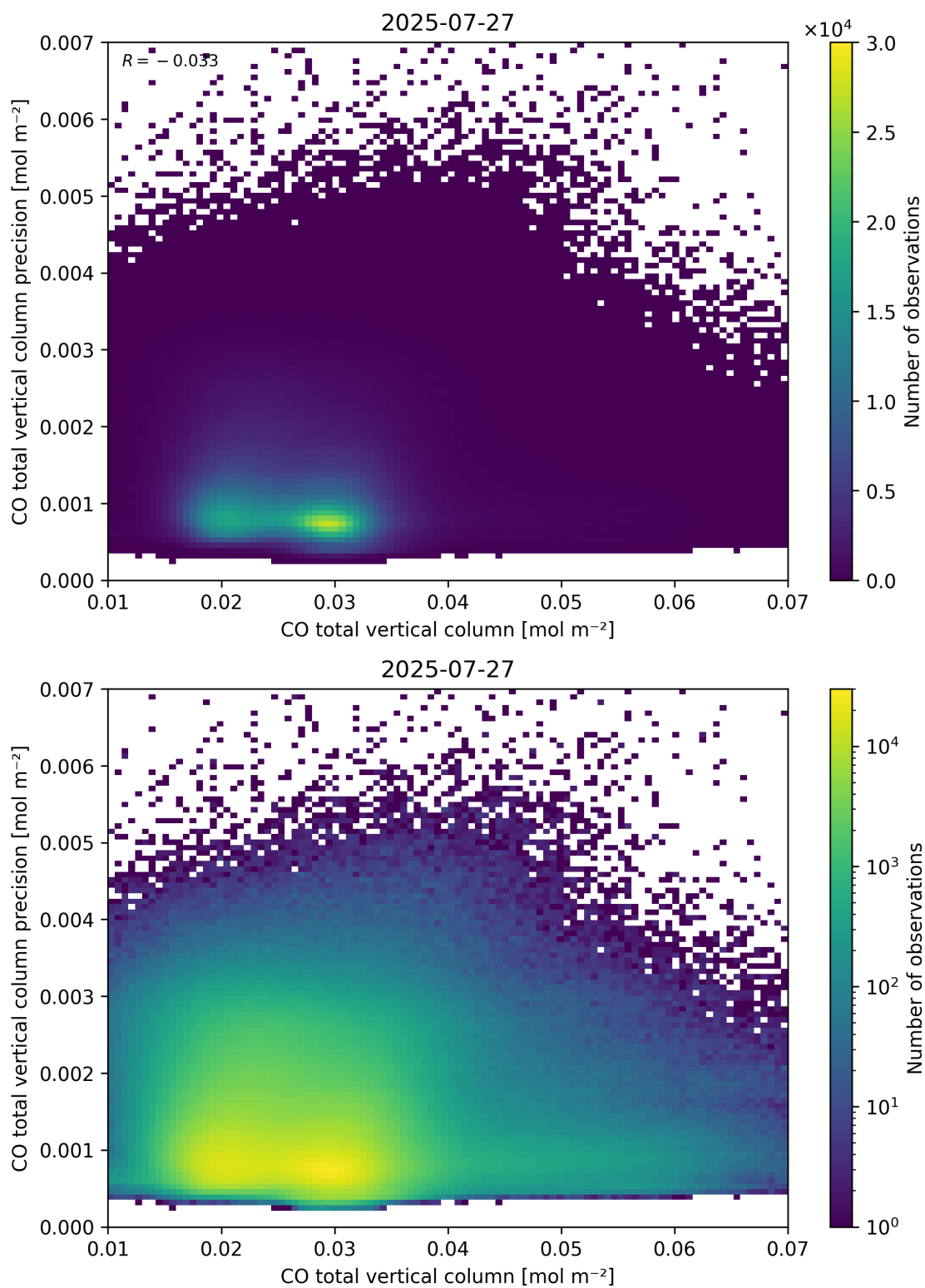
Figure 34: Scatter density plot of “CO total vertical column” against “CO total vertical column precision” for 2025-07-26 to 2025-07-28.
