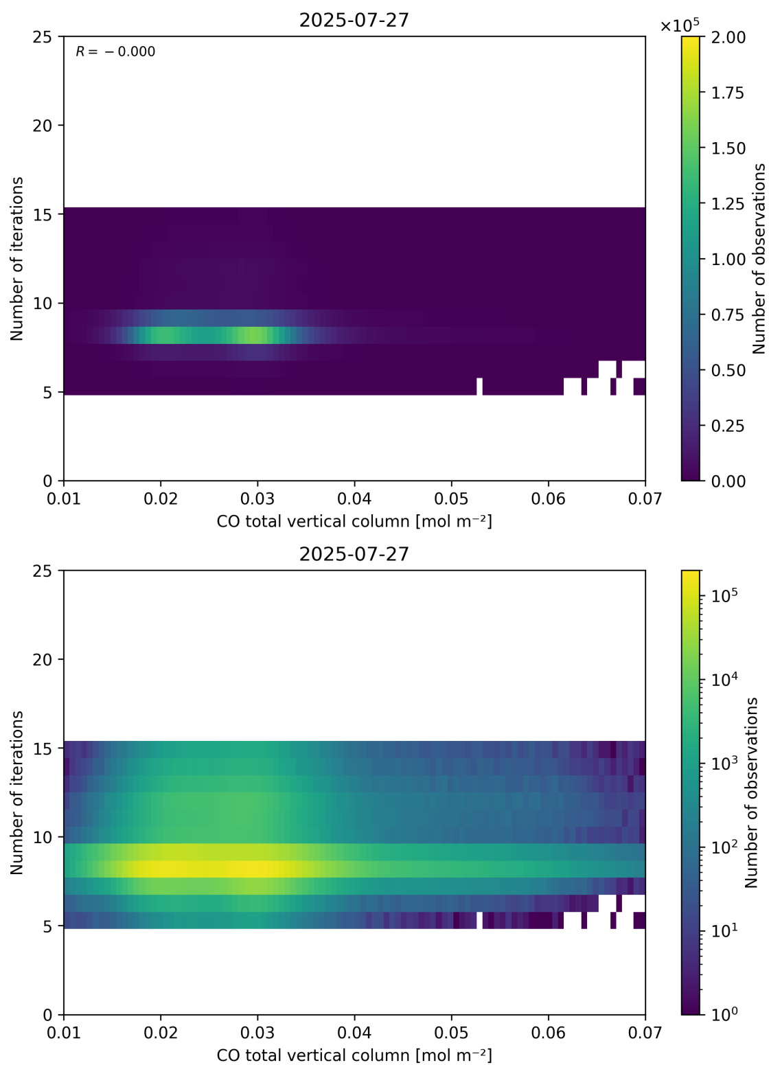
Figure 42: Scatter density plot of “CO total vertical column” against “Number of iterations” for 2025-07-26 to 2025-07-28.
