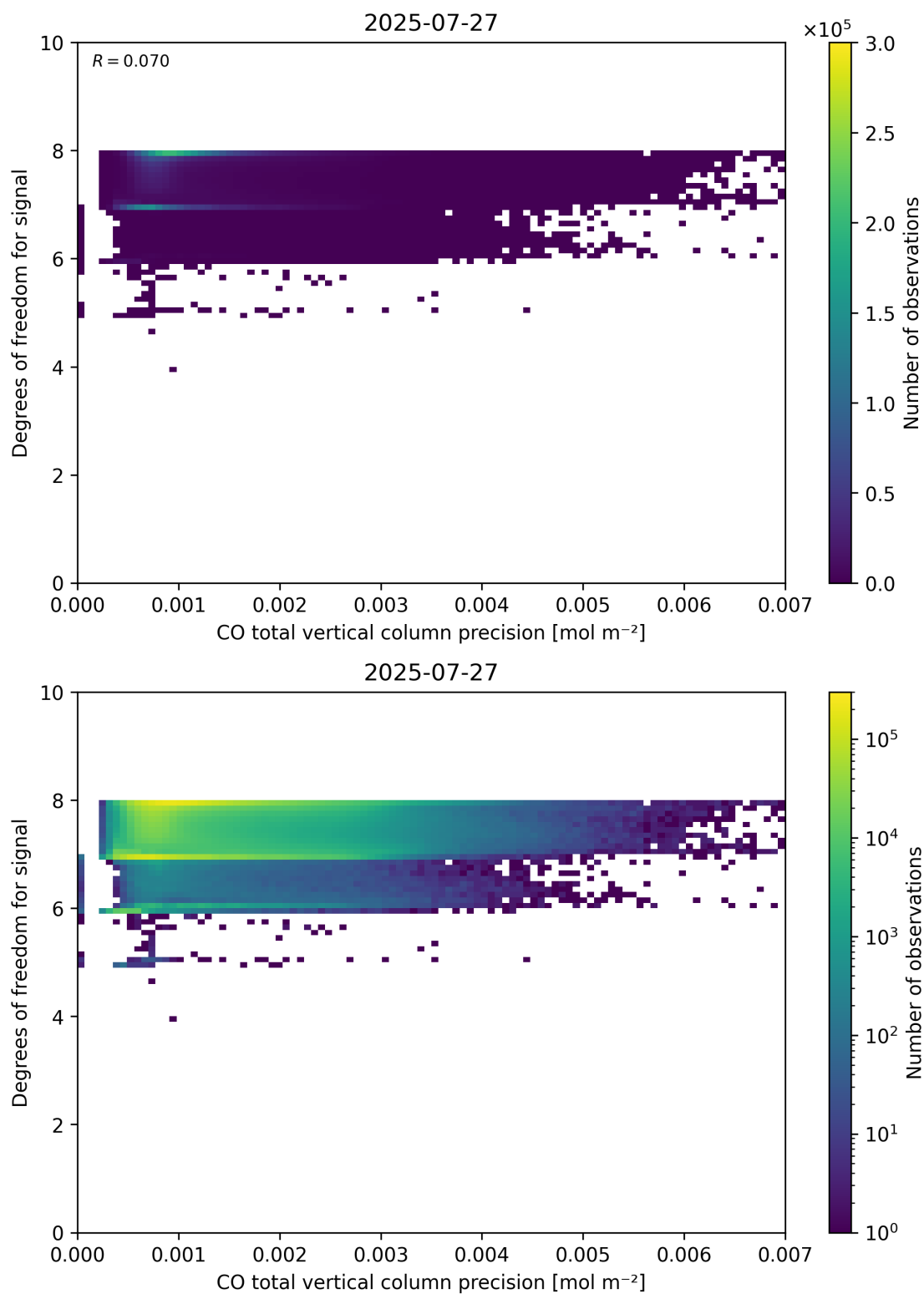
Figure 45: Scatter density plot of “CO total vertical column precision” against “Degrees of freedom for signal” for 2025-07-26 to 2025-07-28.
