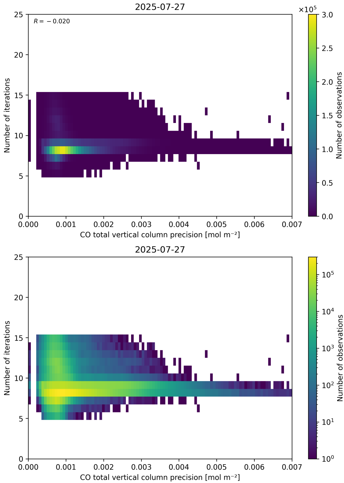
Figure 46: Scatter density plot of “CO total vertical column precision” against “Number of iterations” for 2025-07-26 to 2025-07-28.
