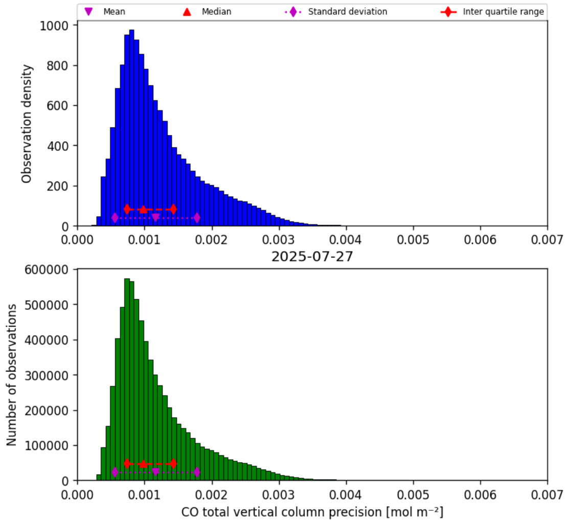
Figure 20: Histogram of “CO total vertical column precision” for 2025-07-26 to 2025-07-28
