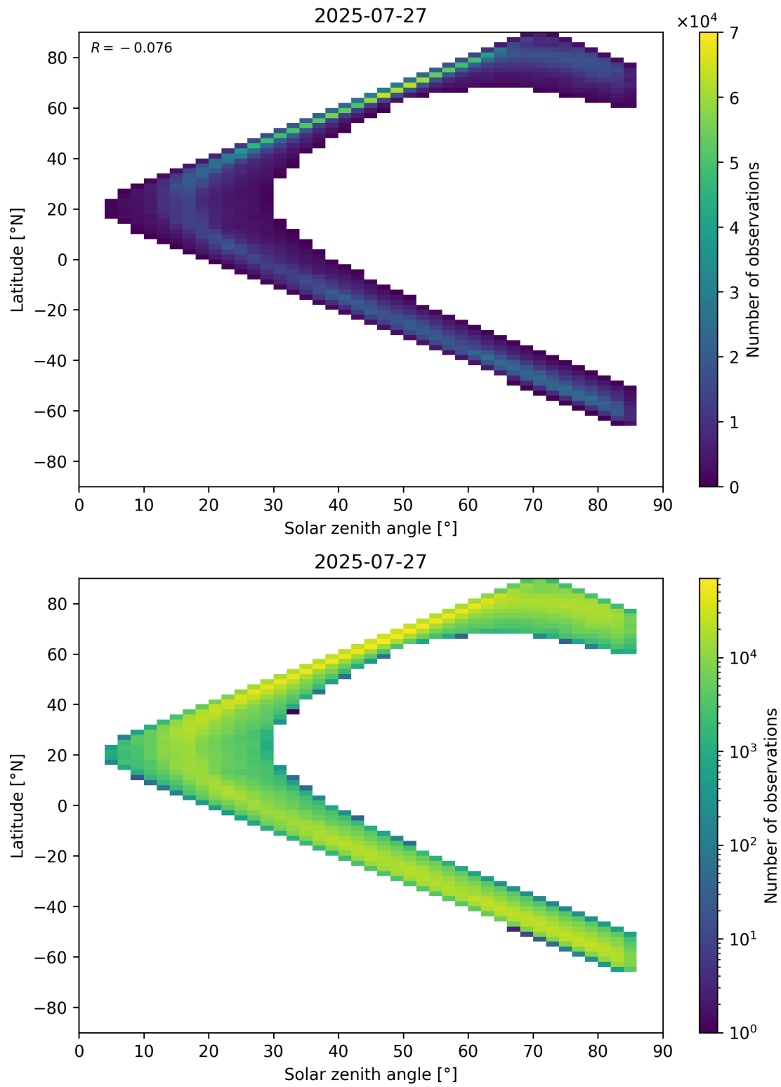
Figure 66: Scatter density plot of “Solar zenith angle” against “Latitude” for 2025-07-26 to 2025-07-28.
