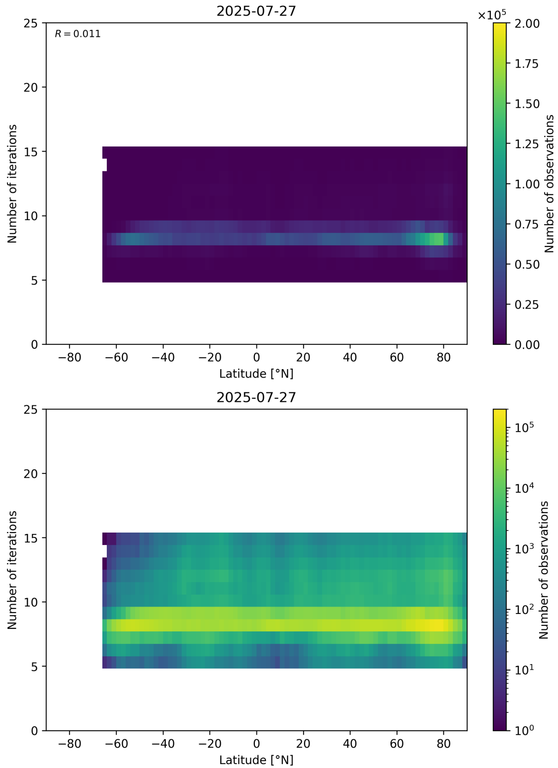
Figure 56: Scatter density plot of “Latitude” against “Number of iterations” for 2025-07-26 to 2025-07-28.
