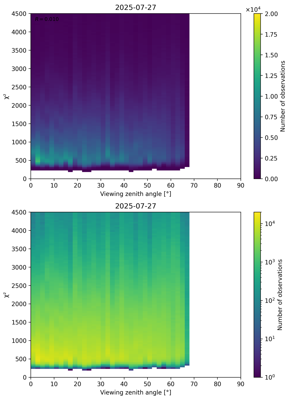
Figure 72: Scatter density plot of “Viewing zenith angle” against “ \chi^2 ” for 2025-07-26 to 2025-07-28.
