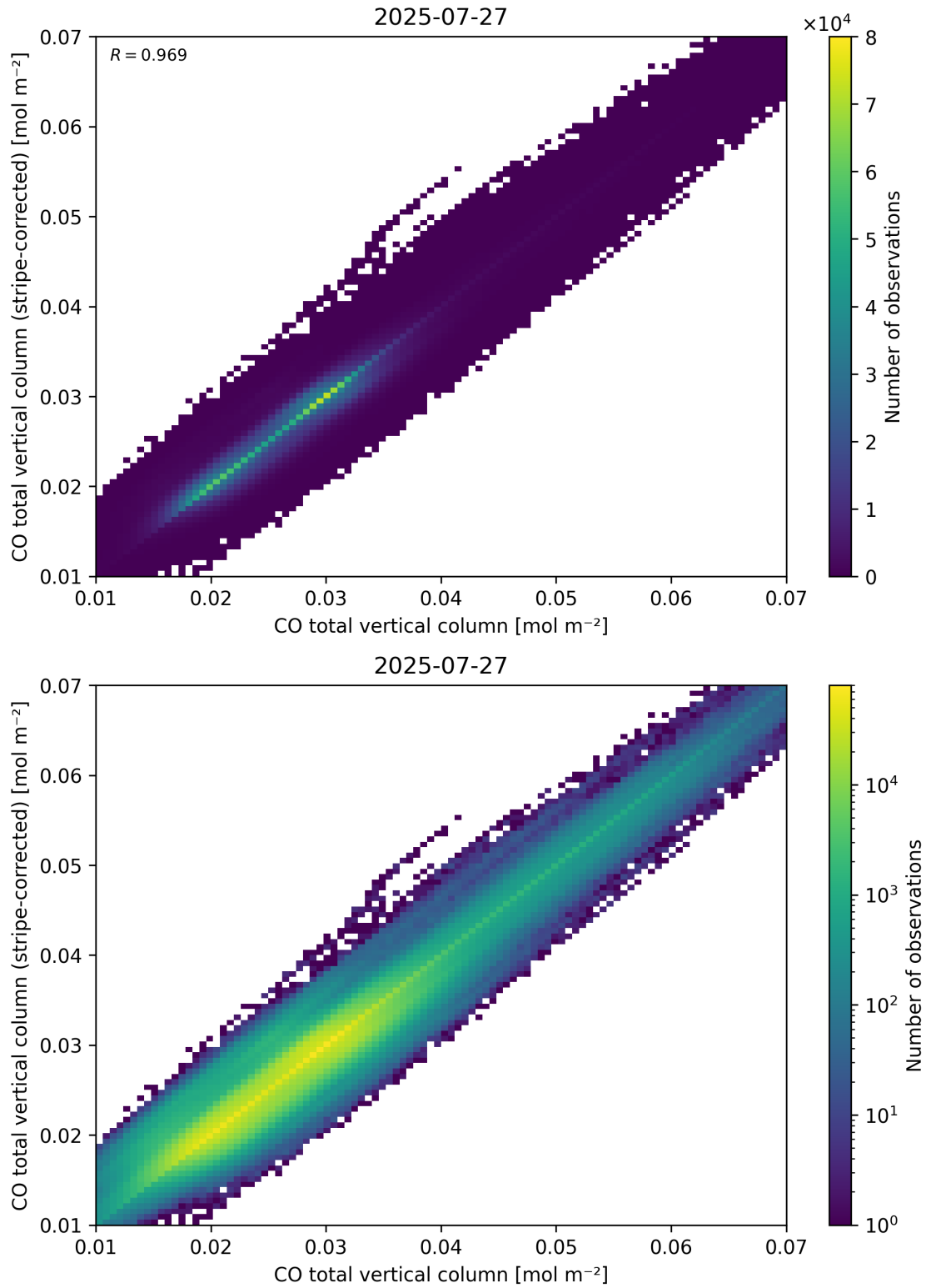
Figure 33: Scatter density plot of “CO total vertical column” against “CO total vertical column (stripe-corrected)” for 2025-07-26 to 2025-07-28.
