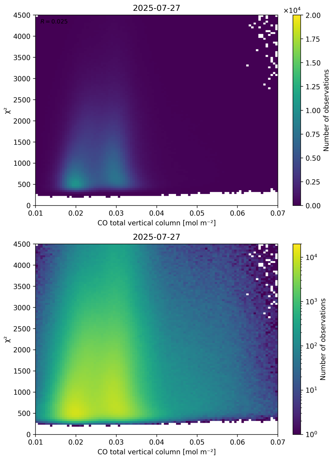
Figure 35: Scatter density plot of “CO total vertical column” against “ \chi^2 ” for 2025-07-26 to 2025-07-28.
