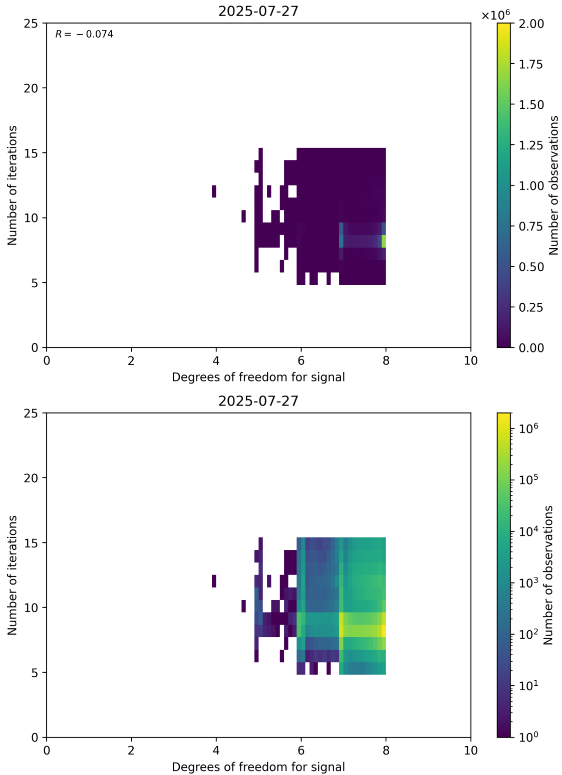
Figure 50: Scatter density plot of “Degrees of freedom for signal” against “Number of iterations” for 2025-07-26 to 2025-07-28.
