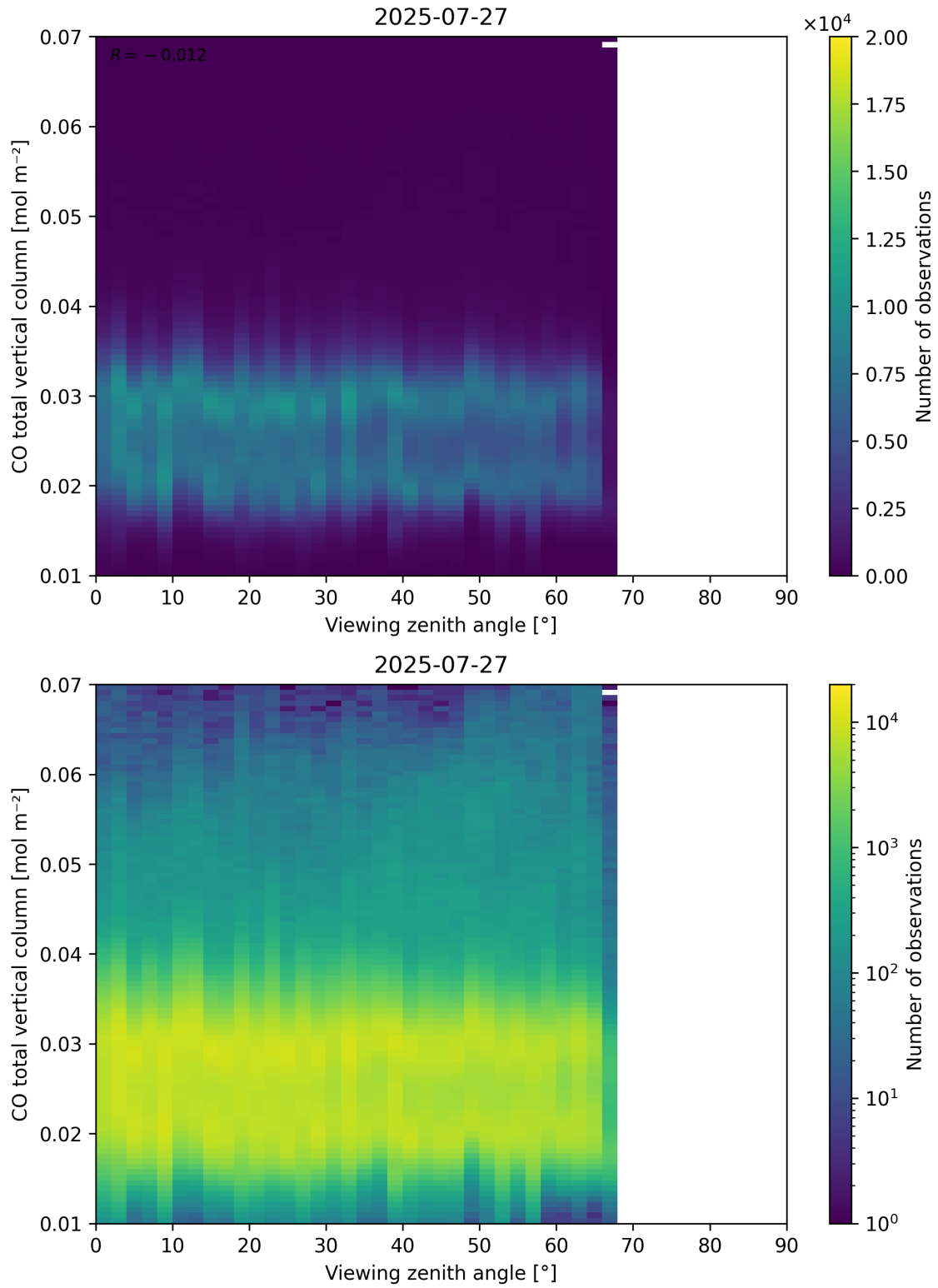
Figure 69: Scatter density plot of “Viewing zenith angle” against “CO total vertical column” for 2025-07-26 to 2025-07-28.
