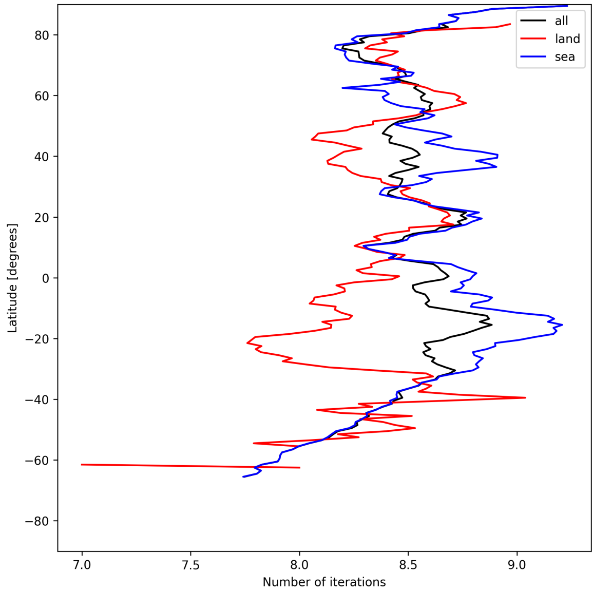
Figure 16: Zonal average of “Number of iterations” for 2025-07-26 to 2025-07-28.
