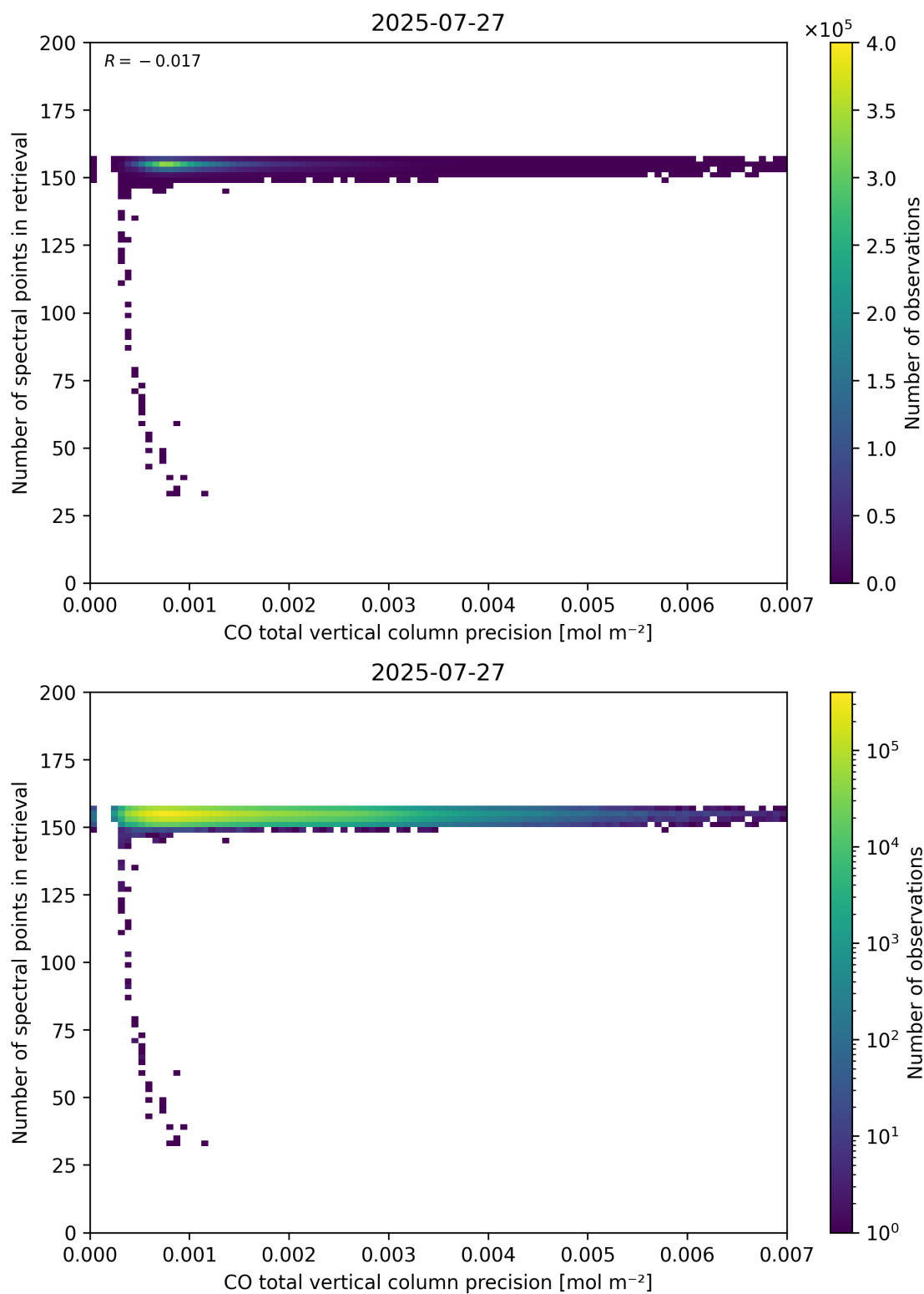
Figure 47: Scatter density plot of “CO total vertical column precision” against “Number of spectral points in retrieval” for 2025-07-26 to 2025-07-28.
