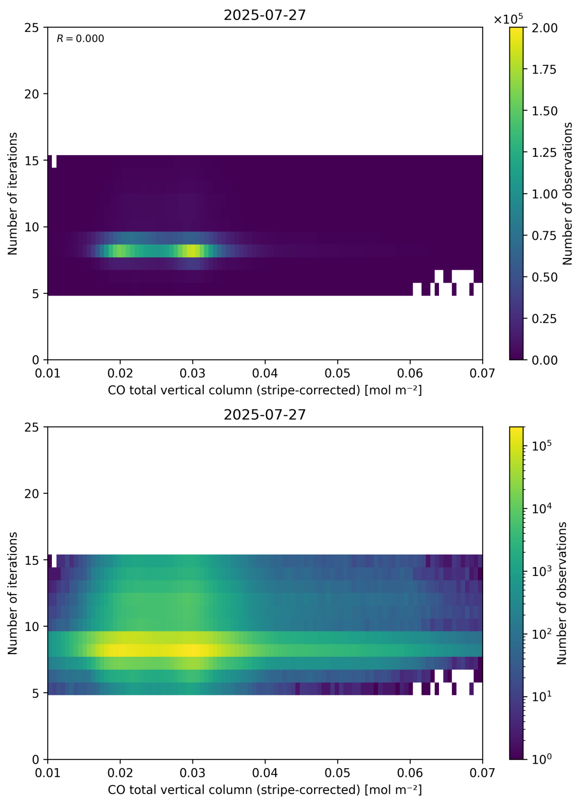
Figure 39: Scatter density plot of “CO total vertical column (stripe-corrected)” against “Number of iterations” for 2025-07-26 to 2025-07-28.
