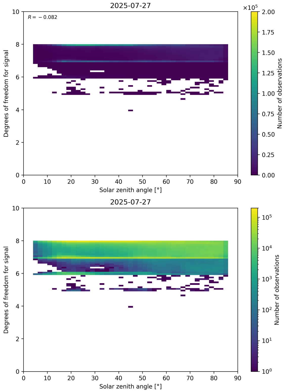
Figure 65: Scatter density plot of “Solar zenith angle” against “Degrees of freedom for signal” for 2025-07-26 to 2025-07-28.
