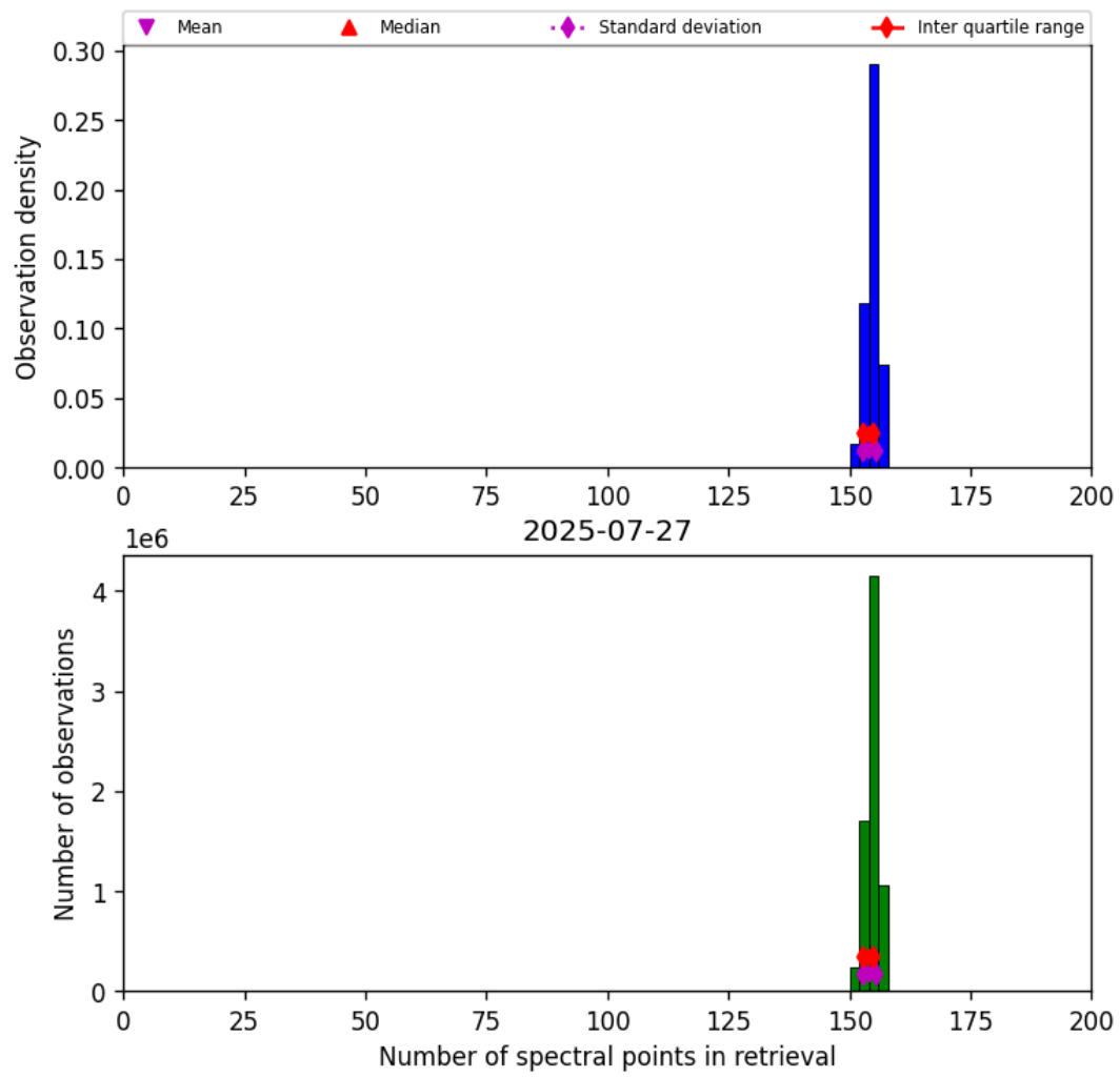
Figure 21: Histogram of “Number of spectral points in retrieval” for 2025-07-26 to 2025-07-28
