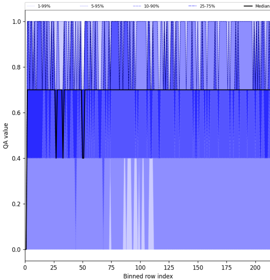
Figure 25: Along track statistics of “QA value” for 2025-07-26 to 2025-07-28
