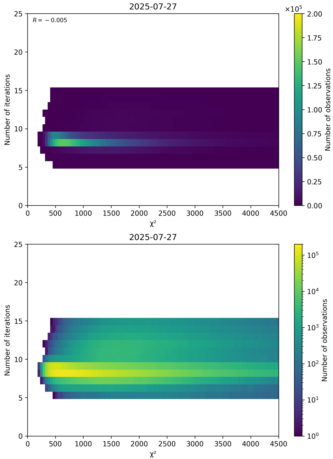
Figure 49: Scatter density plot of “ \chi^2 ” against “Number of iterations” for 2025-07-26 to 2025-07-28.
