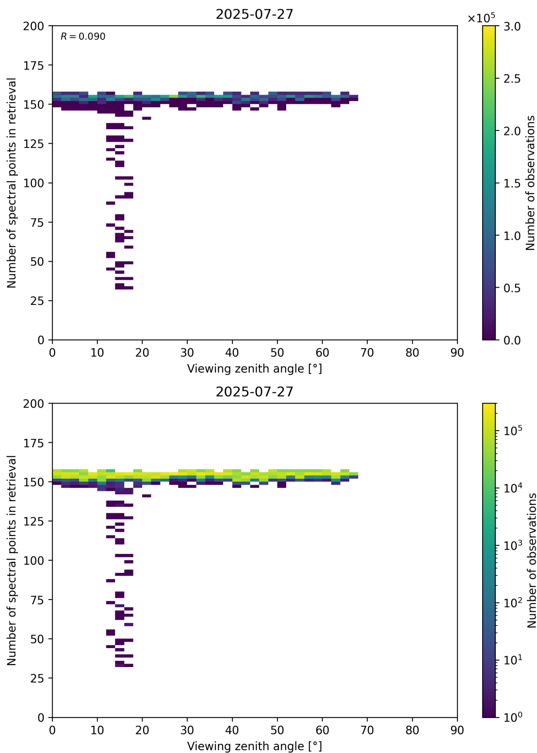
Figure 76: Scatter density plot of “Viewing zenith angle” against “Number of spectral points in retrieval” for 2025-07-26 to 2025-07-28.
