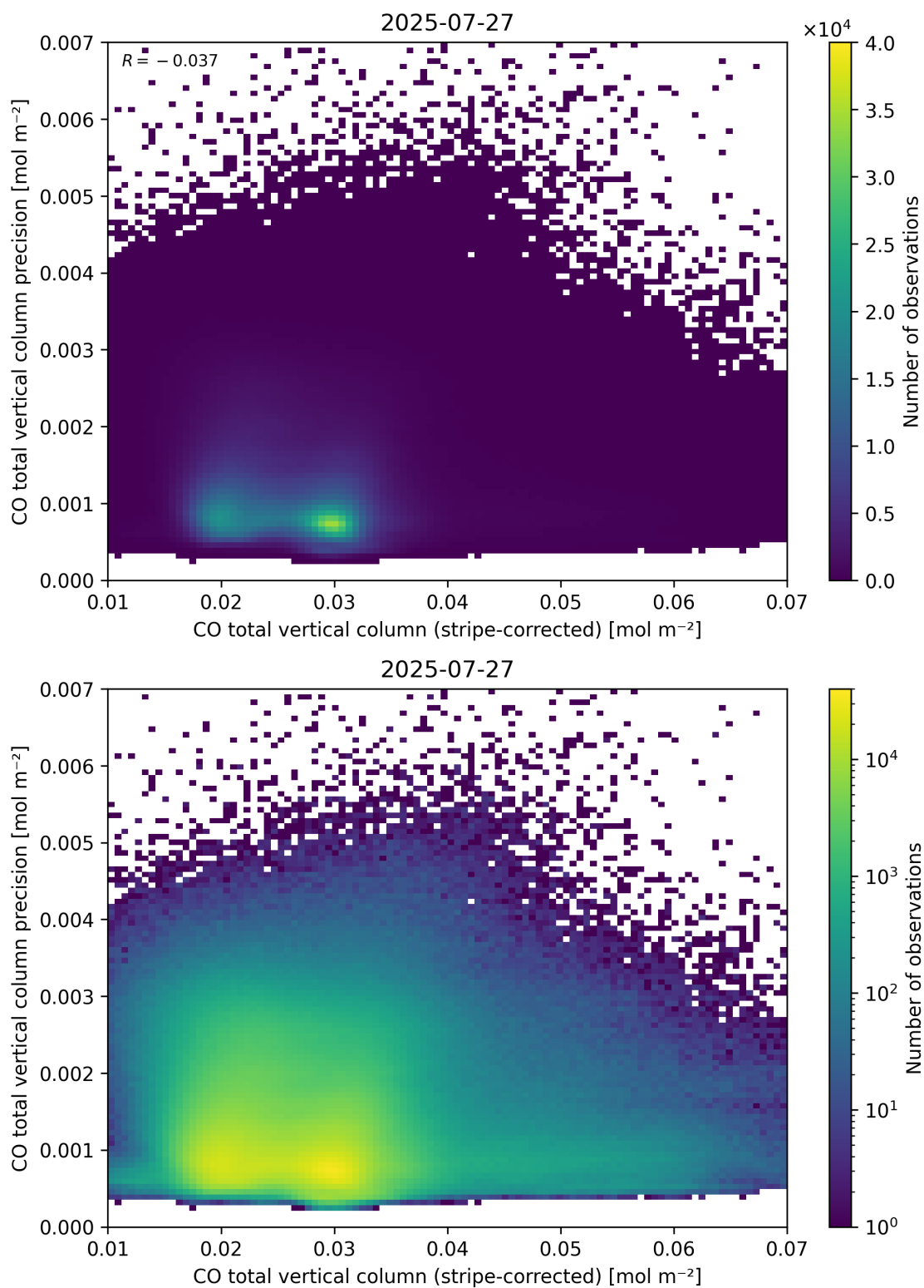
Figure 36: Scatter density plot of “CO total vertical column (stripe-corrected)” against “CO total vertical column precision” for 2025-07-26 to 2025-07-28.
