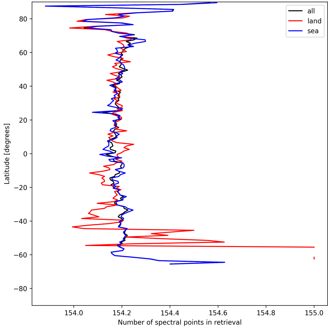
Figure 13: Zonal average of “Number of spectral points in retrieval” for 2025-07-26 to 2025-07-28.
