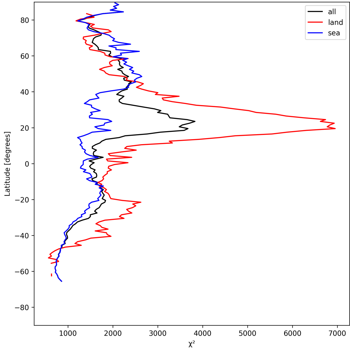
Figure 14: Zonal average of “ \chi^2 ” for 2025-07-26 to 2025-07-28.
