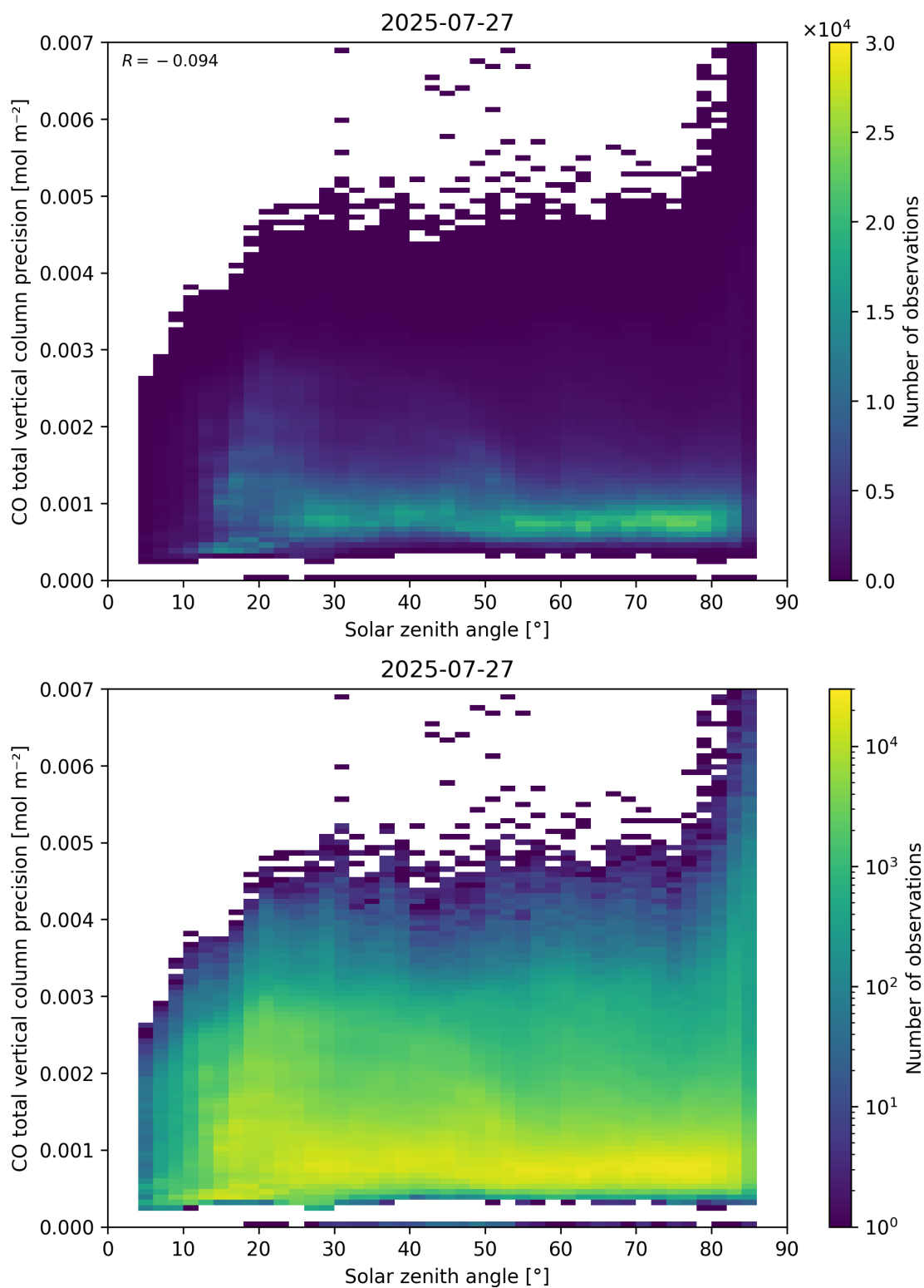
Figure 63: Scatter density plot of “Solar zenith angle” against “CO total vertical column precision” for 2025-07-26 to 2025-07-28.
