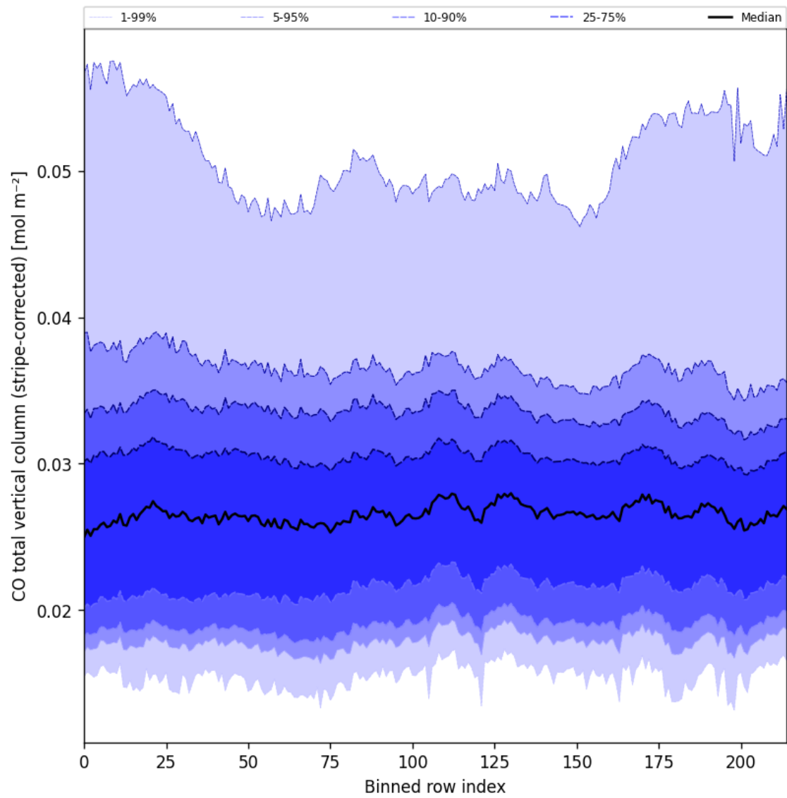
Figure 27: Along track statistics of “CO total vertical column (stripe-corrected)” for 2025-07-26 to 2025-07-28
