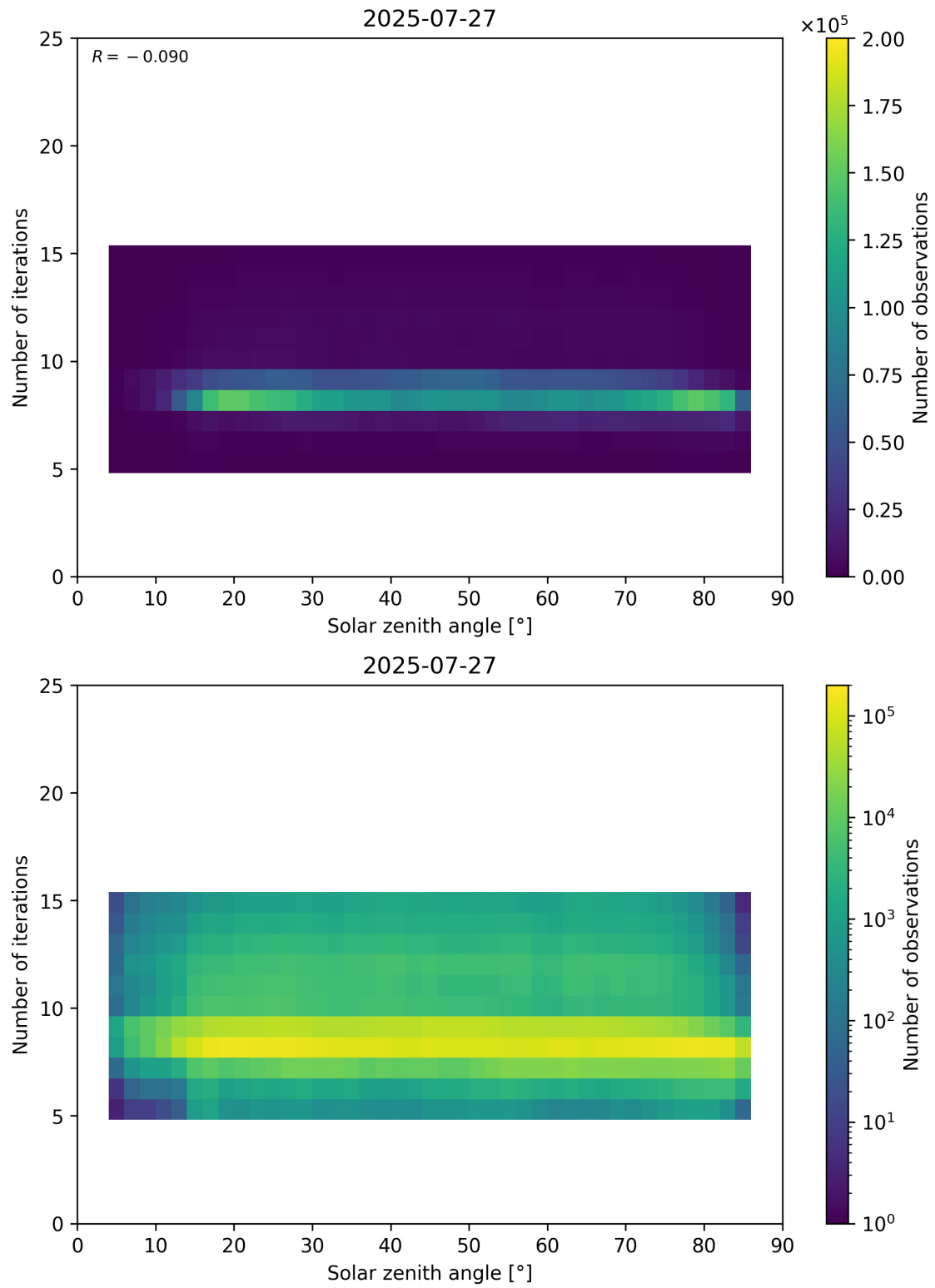
Figure 67: Scatter density plot of “Solar zenith angle” against “Number of iterations” for 2025-07-26 to 2025-07-28.
