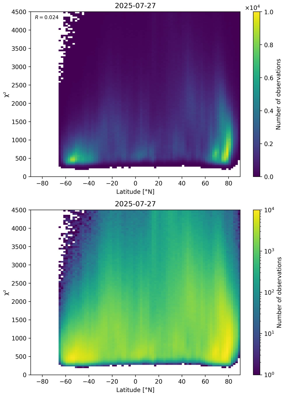
Figure 54: Scatter density plot of “Latitude” against “ \chi^2 ” for 2025-07-26 to 2025-07-28.
