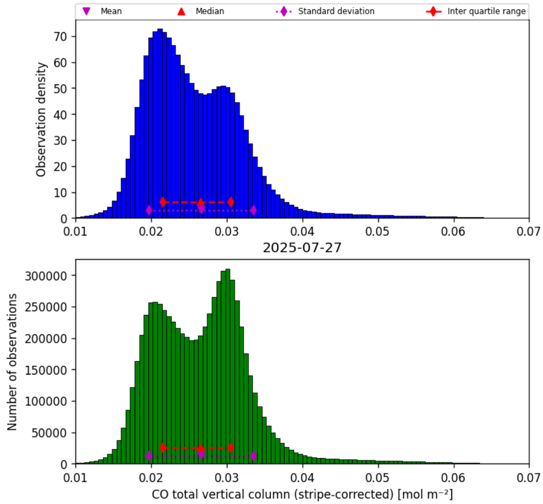
Figure 19: Histogram of “CO total vertical column (stripe-corrected)” for 2025-07-26 to 2025-07-28
