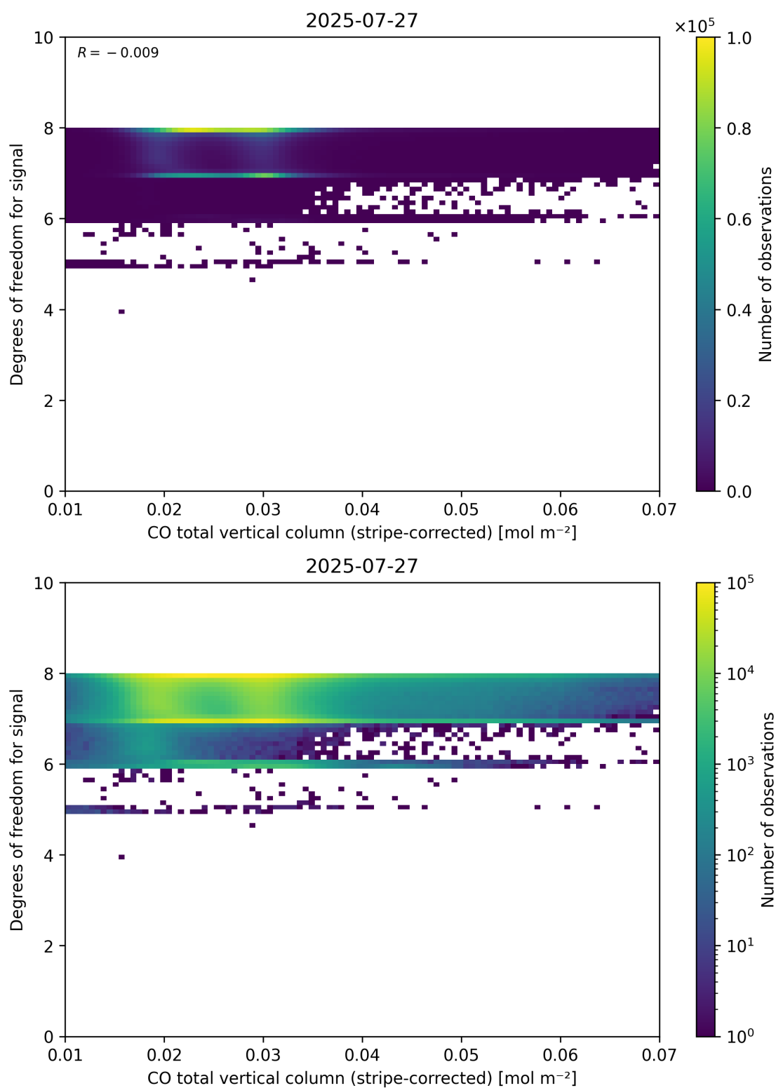
Figure 38: Scatter density plot of “CO total vertical column (stripe-corrected)” against “Degrees of freedom for signal” for 2025-07-26 to 2025-07-28.
