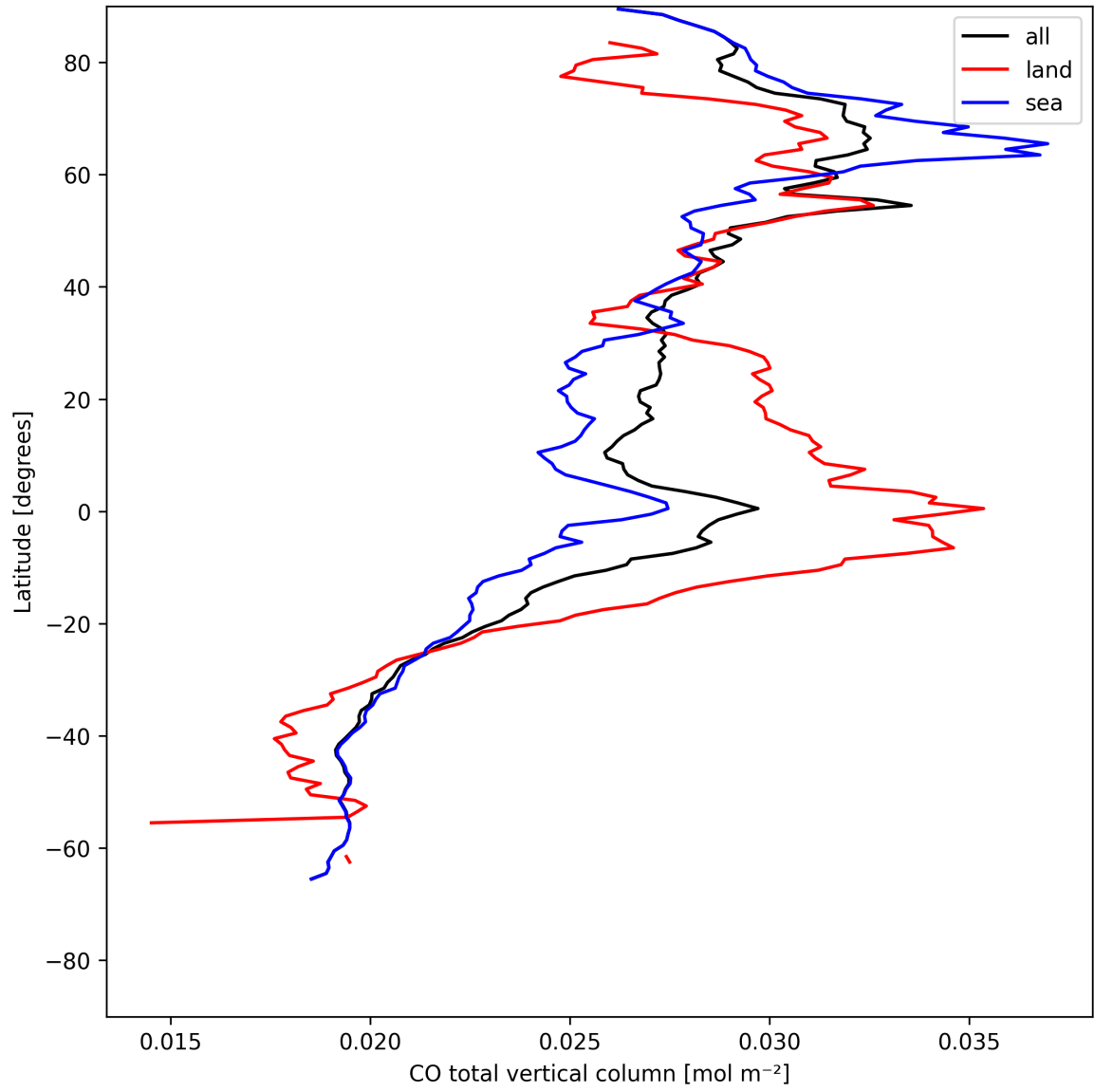
Figure 10: Zonal average of “CO total vertical column” for 2025-07-26 to 2025-07-28.
