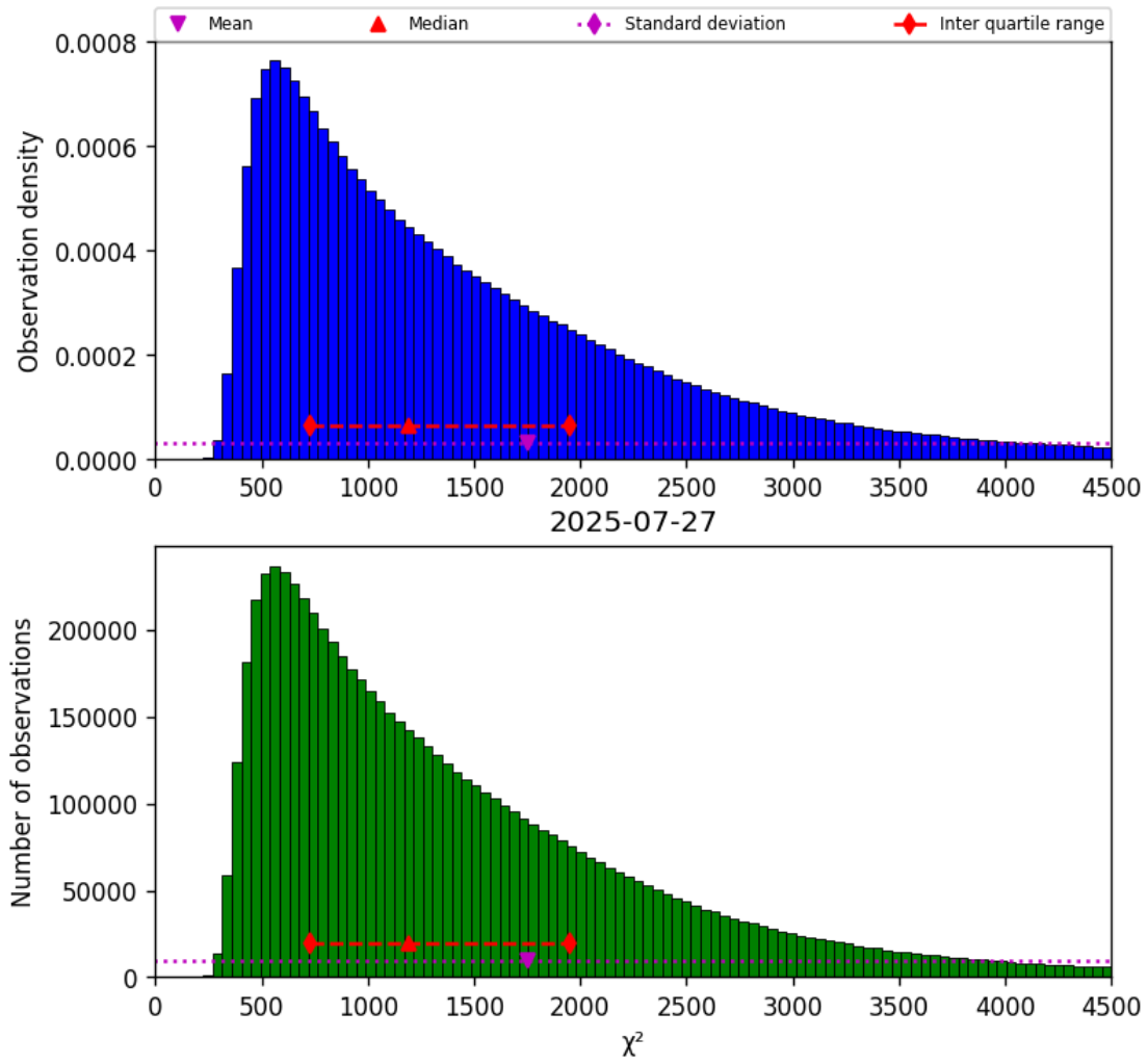
Figure 22: Histogram of “ \chi^2 ” for 2025-07-26 to 2025-07-28
