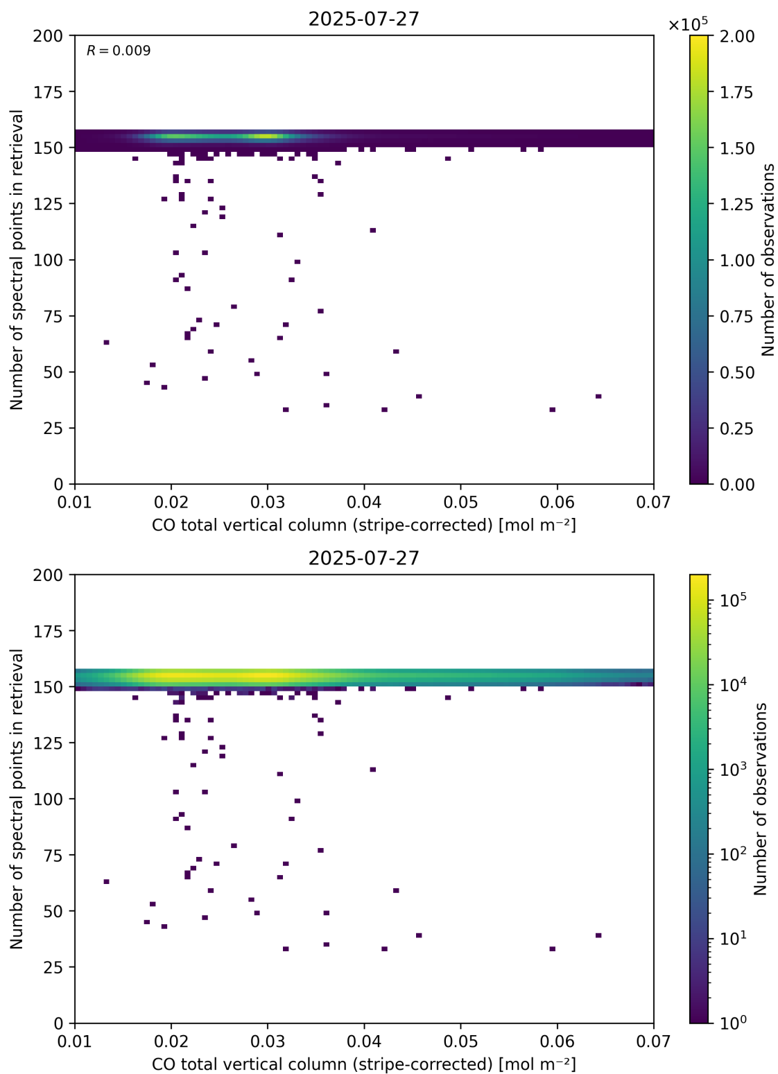
Figure 40: Scatter density plot of “CO total vertical column (stripe-corrected)” against “Number of spectral points in retrieval” for 2025-07-26 to 2025-07-28.
