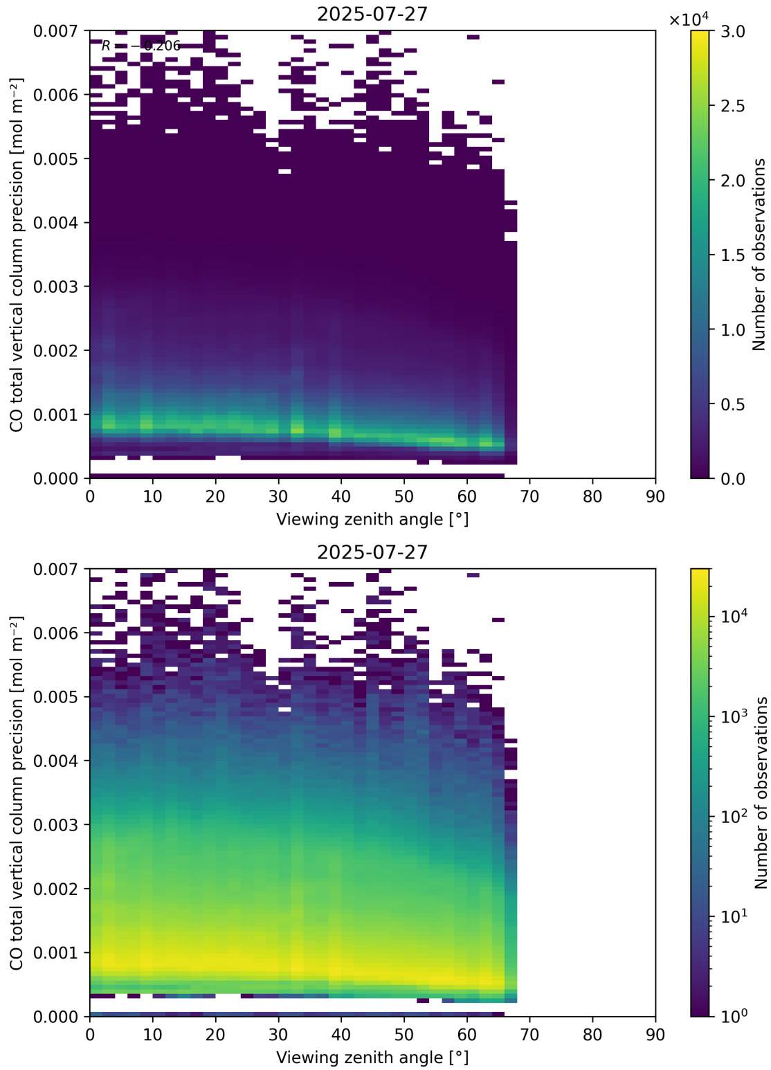
Figure 71: Scatter density plot of “Viewing zenith angle” against “CO total vertical column precision” for 2025-07-26 to 2025-07-28.
