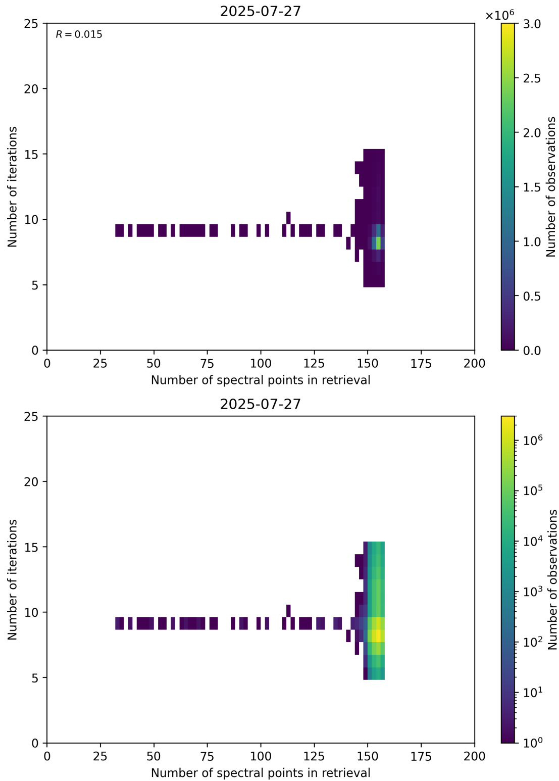
Figure 60: Scatter density plot of “Number of spectral points in retrieval” against “Number of iterations” for 2025-07-26 to 2025-07-28.
