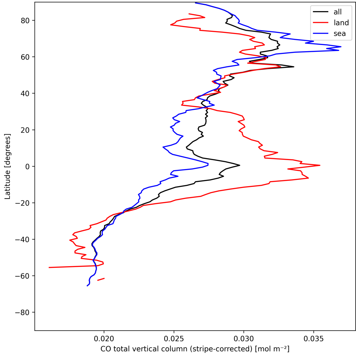
Figure 11: Zonal average of “CO total vertical column (stripe-corrected)” for 2025-07-26 to 2025-07-28.
