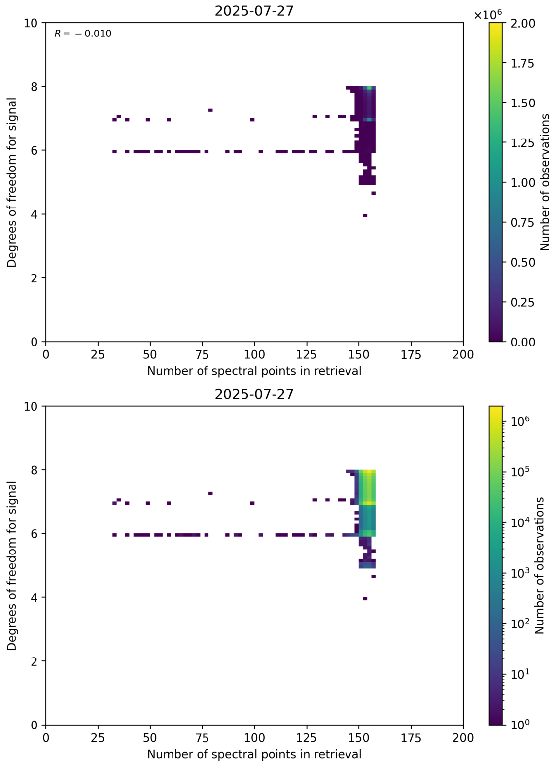
Figure 59: Scatter density plot of “Number of spectral points in retrieval” against “Degrees of freedom for signal” for 2025-07-26 to 2025-07-28.
