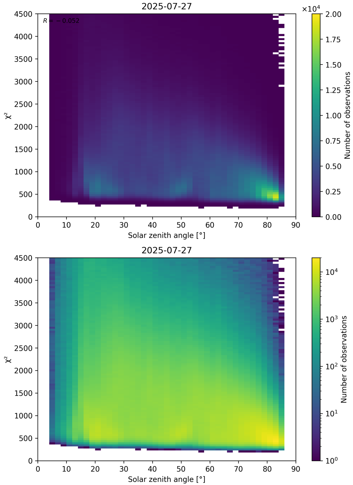
Figure 64: Scatter density plot of “Solar zenith angle” against “ \chi^2 ” for 2025-07-26 to 2025-07-28.
