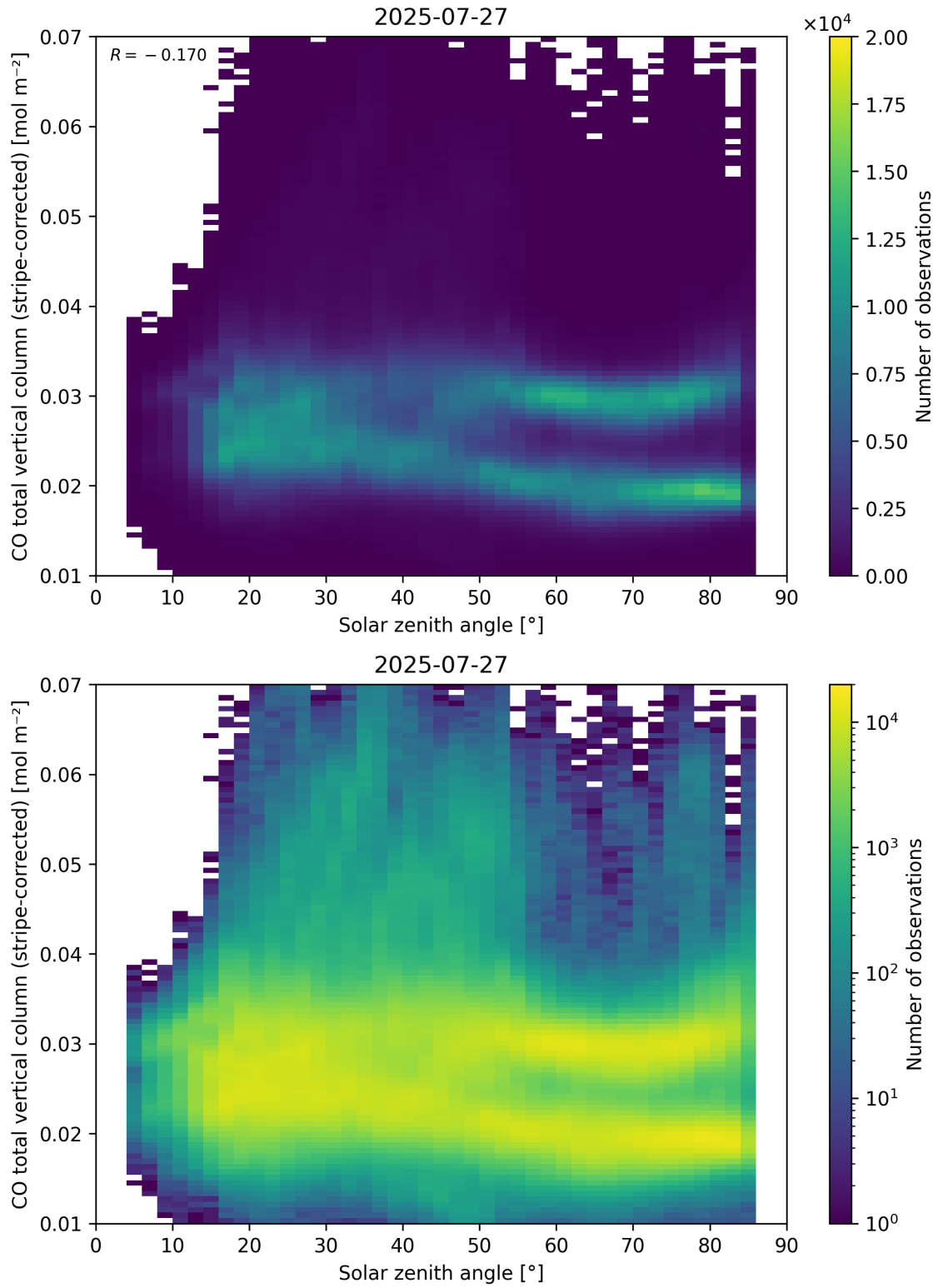
Figure 62: Scatter density plot of “Solar zenith angle” against “CO total vertical column (stripe-corrected)” for 2025-07-26 to 2025-07-28.
