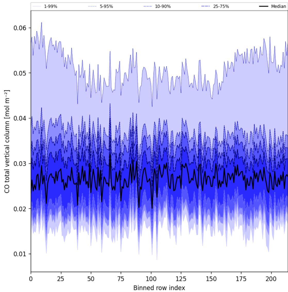
Figure 26: Along track statistics of “CO total vertical column” for 2025-07-26 to 2025-07-28
