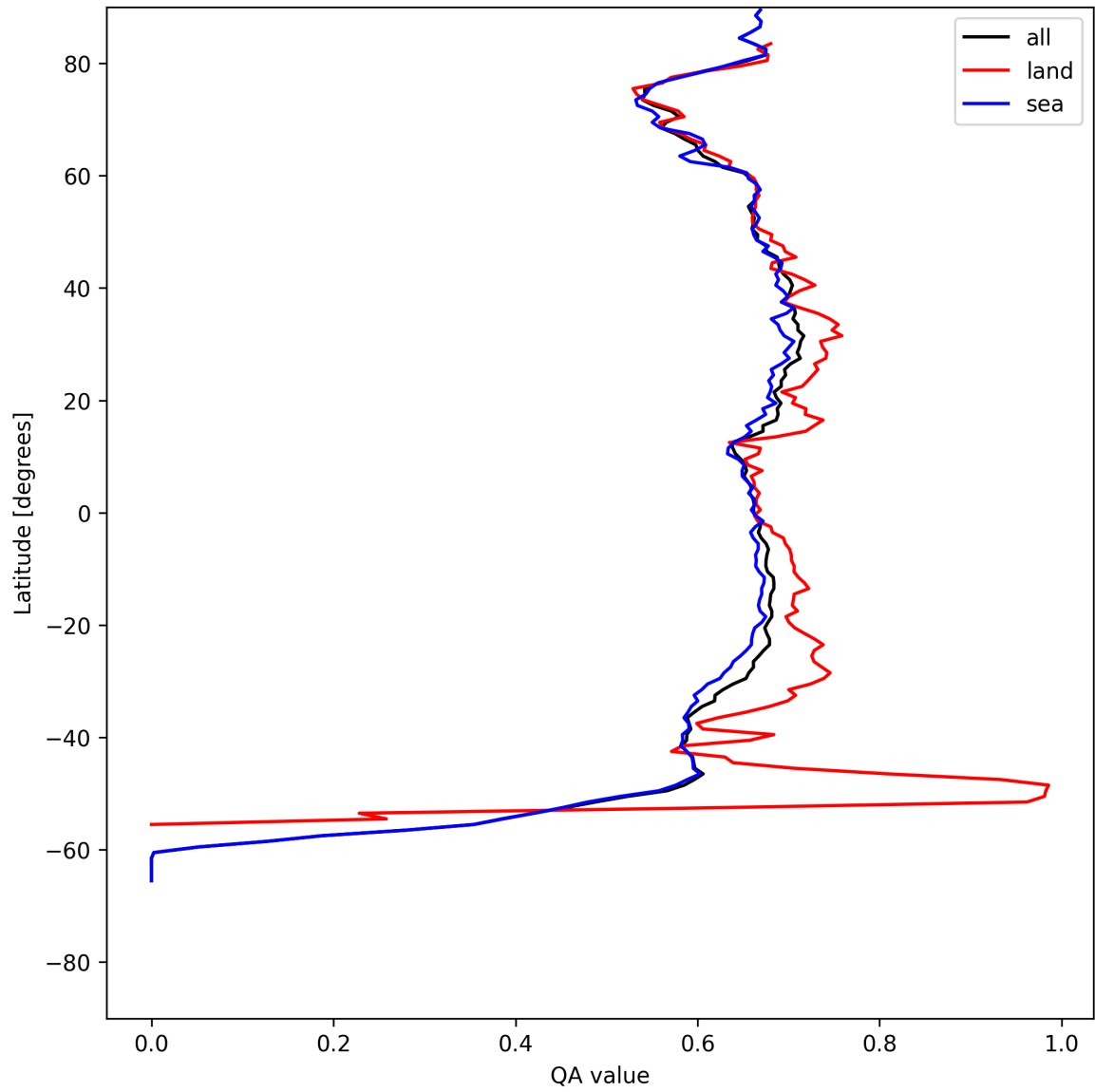
Figure 9: Zonal average of “QA value” for 2025-07-26 to 2025-07-28.
