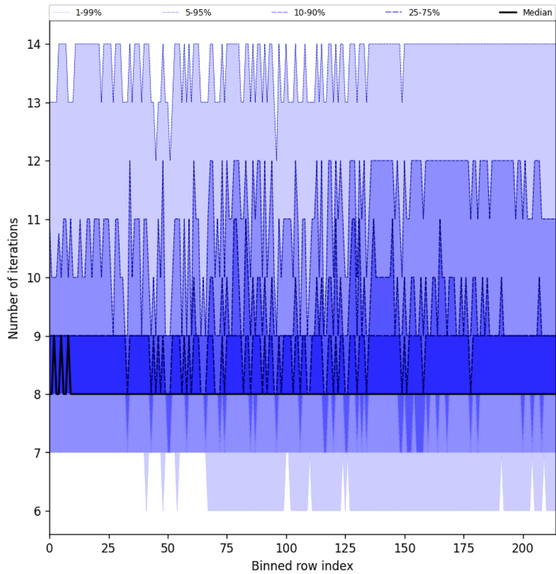
Figure 32: Along track statistics of “Number of iterations” for 2025-07-26 to 2025-07-28
