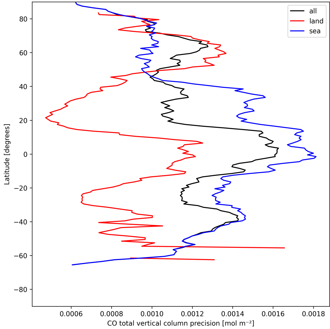
Figure 12: Zonal average of “CO total vertical column precision” for 2025-07-26 to 2025-07-28.
