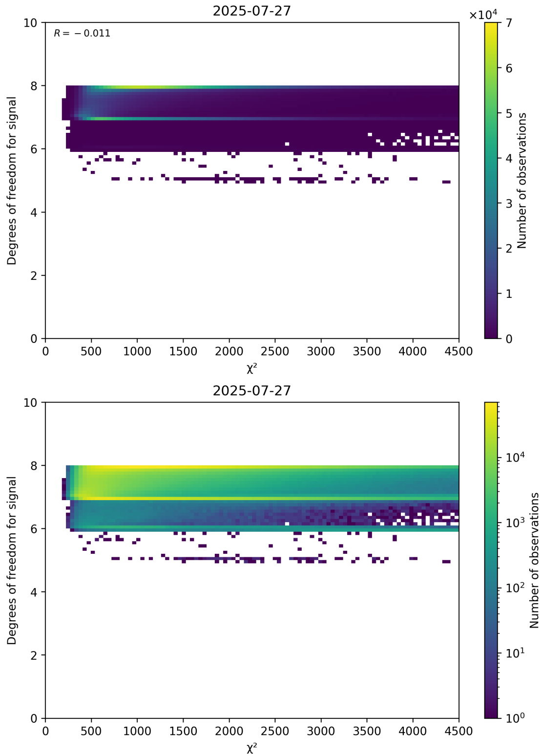
Figure 48: Scatter density plot of “ \chi^2 ” against “Degrees of freedom for signal” for 2025-07-26 to 2025-07-28.
