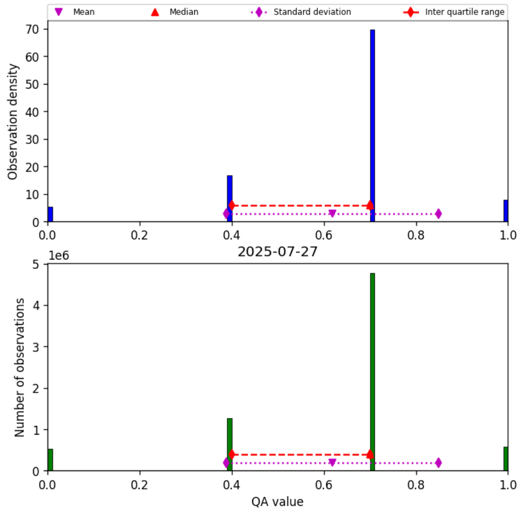
Figure 17: Histogram of “QA value” for 2025-07-26 to 2025-07-28
