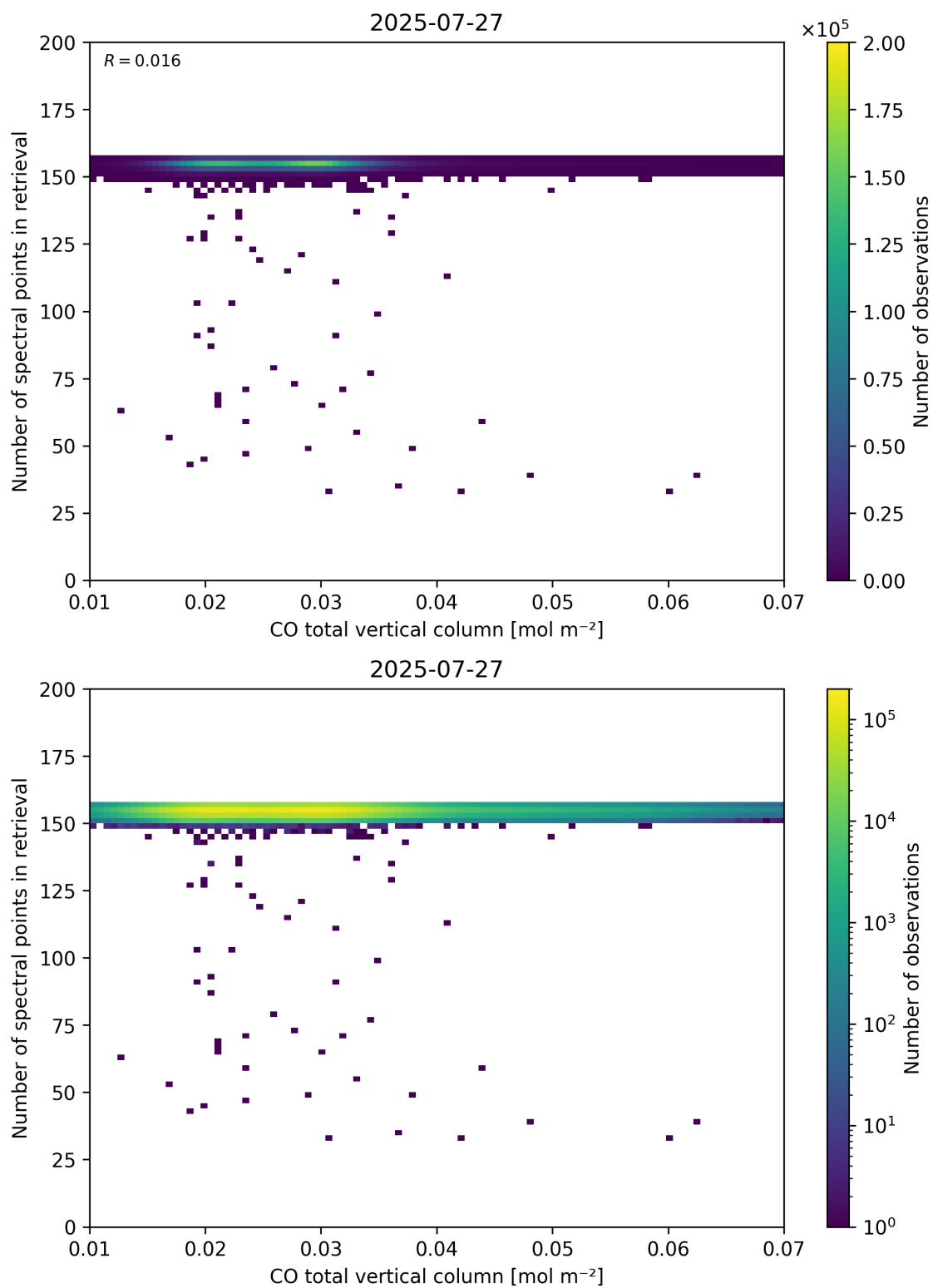
Figure 43: Scatter density plot of “CO total vertical column” against “Number of spectral points in retrieval” for 2025-07-26 to 2025-07-28.
