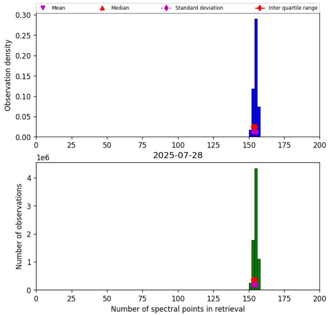
Figure 21: Histogram of “Number of spectral points in retrieval” for 2025-07-27 to 2025-07-29
