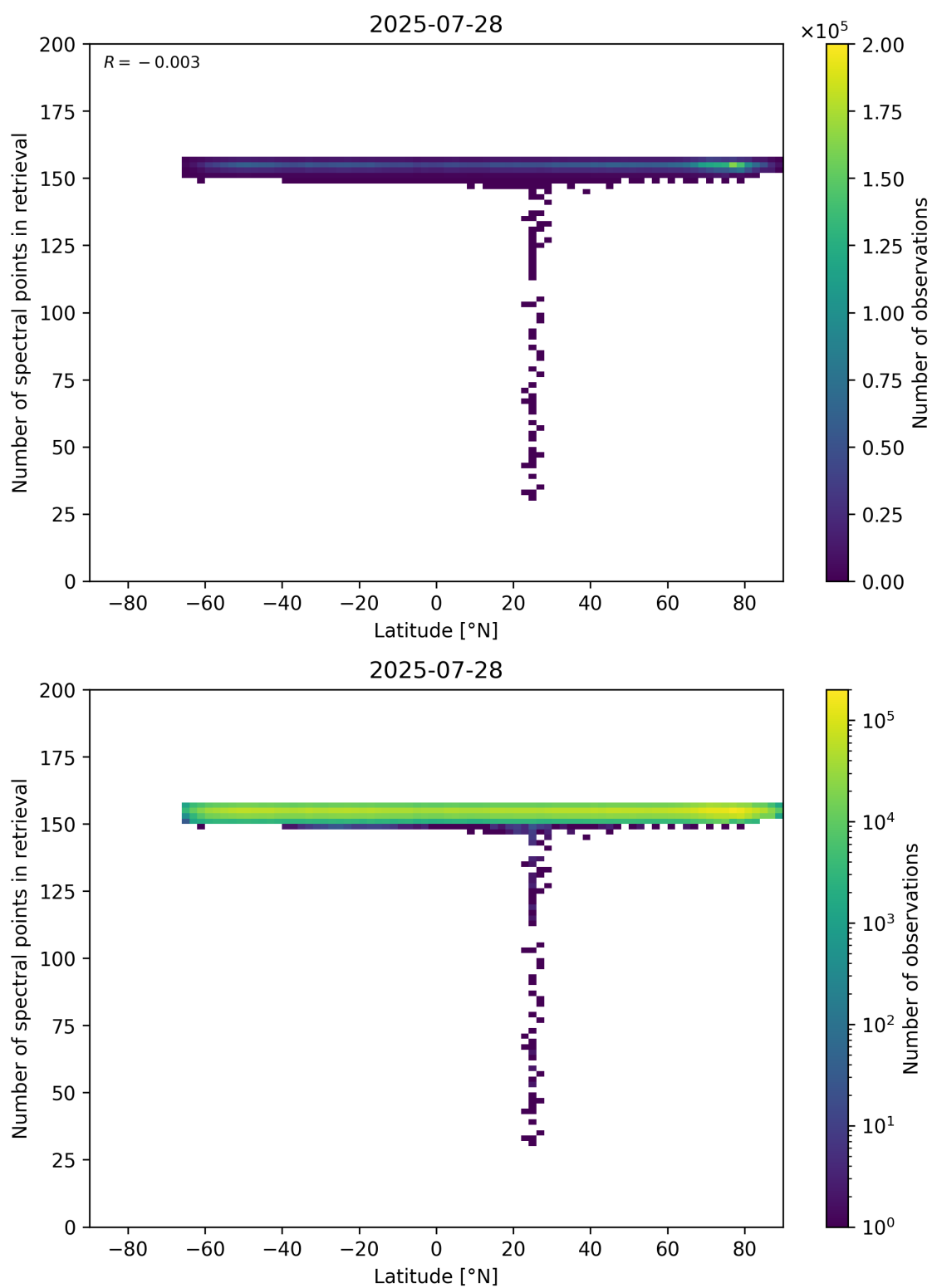
Figure 57: Scatter density plot of “Latitude” against “Number of spectral points in retrieval” for 2025-07-27 to 2025-07-29.
