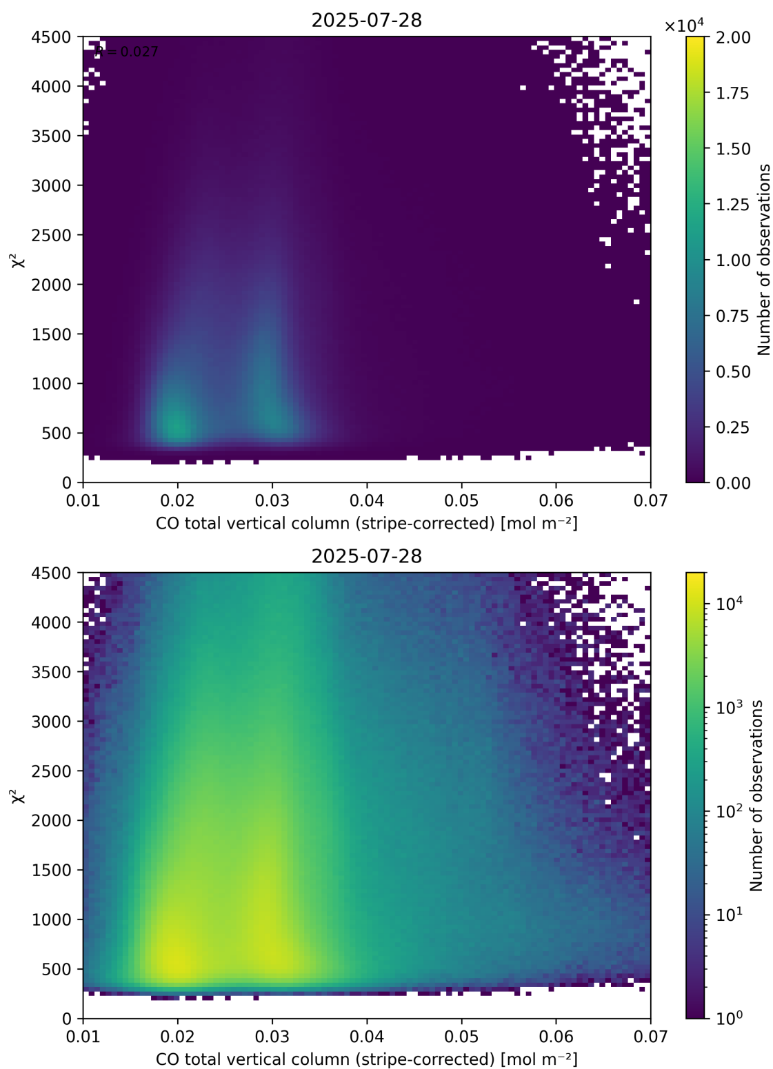
Figure 37: Scatter density plot of “CO total vertical column (stripe-corrected)” against “ \chi^2 ” for 2025-07-27 to 2025-07-29.
