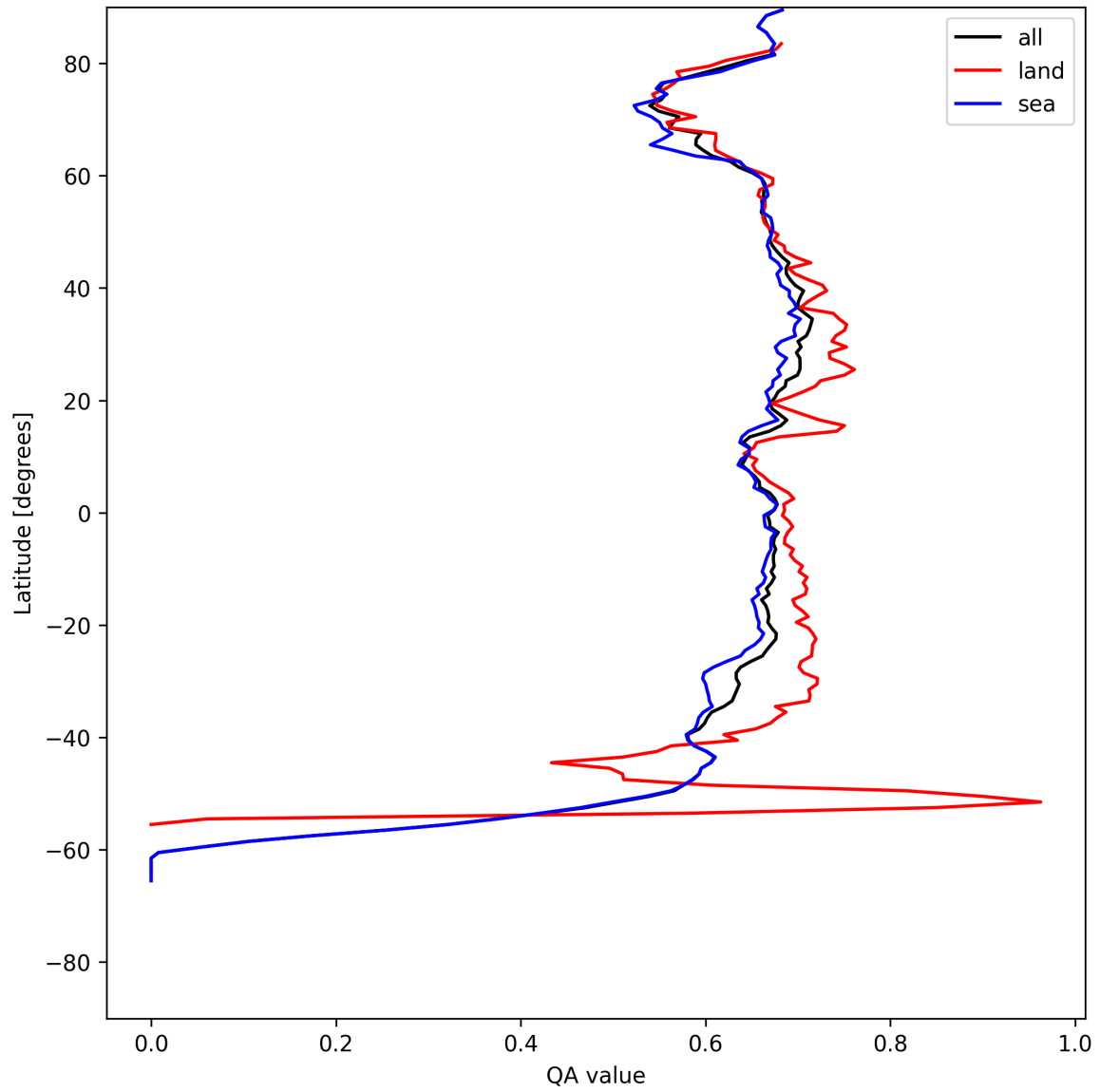
Figure 9: Zonal average of “QA value” for 2025-07-27 to 2025-07-29.
