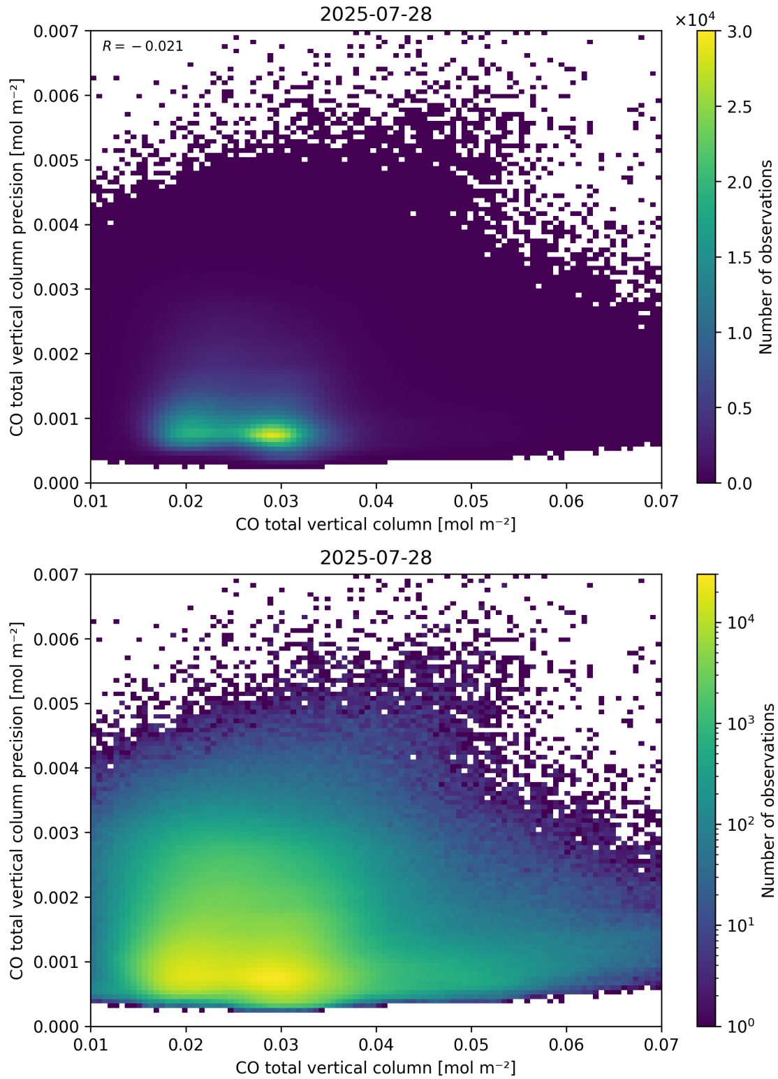
Figure 34: Scatter density plot of “CO total vertical column” against “CO total vertical column precision” for 2025-07-27 to 2025-07-29.
