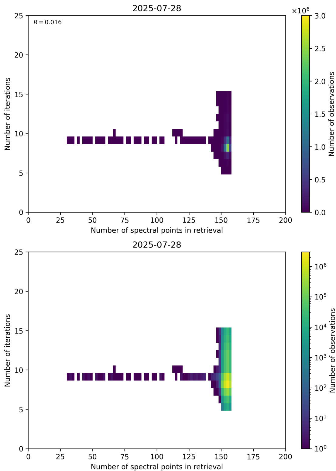
Figure 60: Scatter density plot of “Number of spectral points in retrieval” against “Number of iterations” for 2025-07-27 to 2025-07-29.
