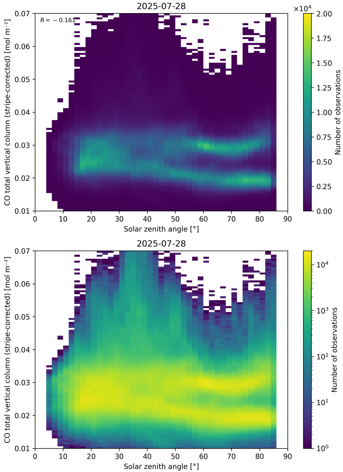
Figure 62: Scatter density plot of “Solar zenith angle” against “CO total vertical column (stripe-corrected)” for 2025-07-27 to 2025-07-29.
