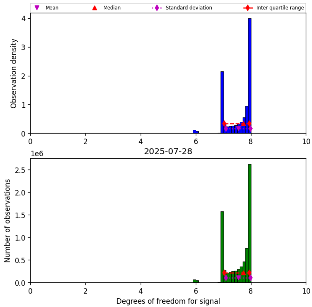
Figure 23: Histogram of “Degrees of freedom for signal” for 2025-07-27 to 2025-07-29
