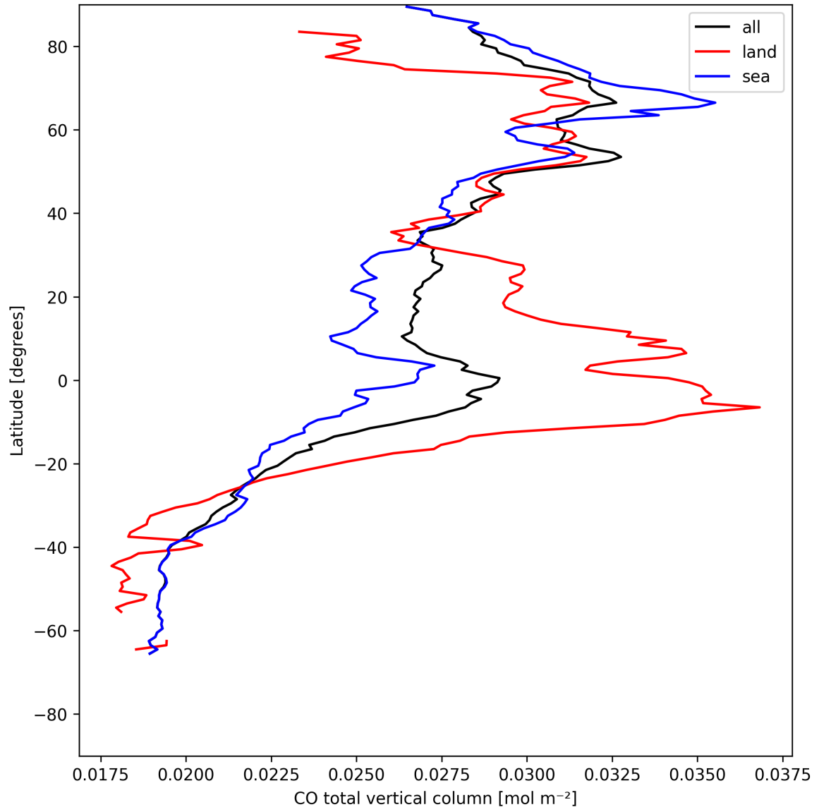
Figure 10: Zonal average of “CO total vertical column” for 2025-07-27 to 2025-07-29.
