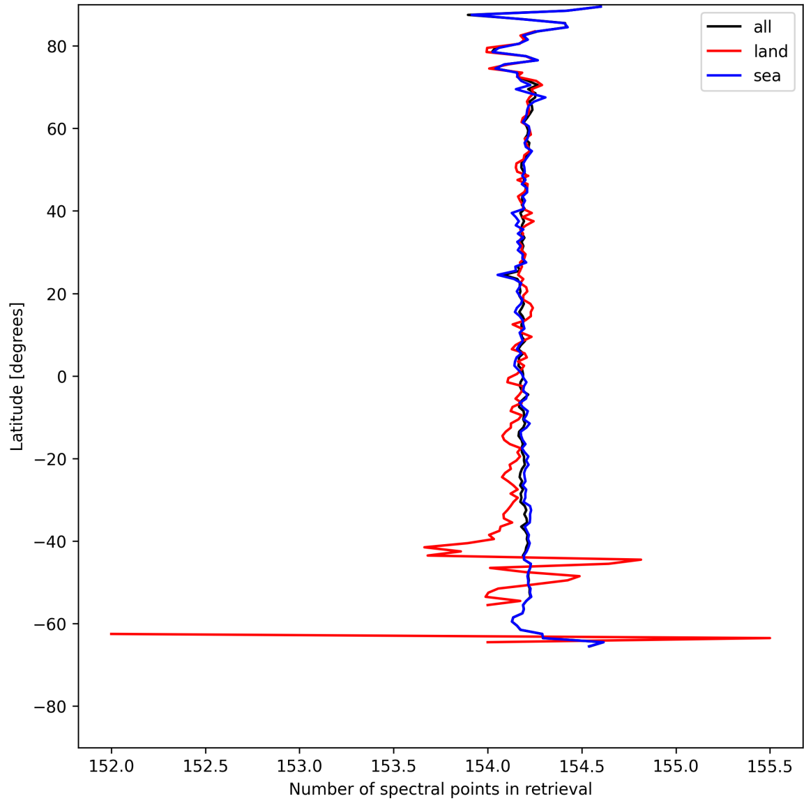
Figure 13: Zonal average of “Number of spectral points in retrieval” for 2025-07-27 to 2025-07-29.
