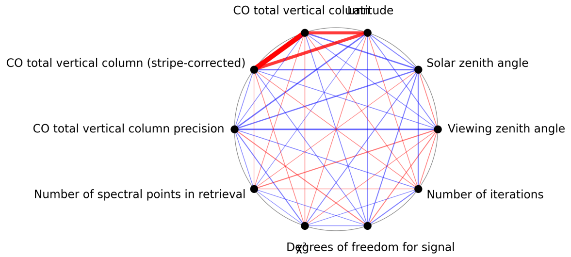
Figure 1: Map of correlation graph for 2025-07-27 to 2025-07-29.
