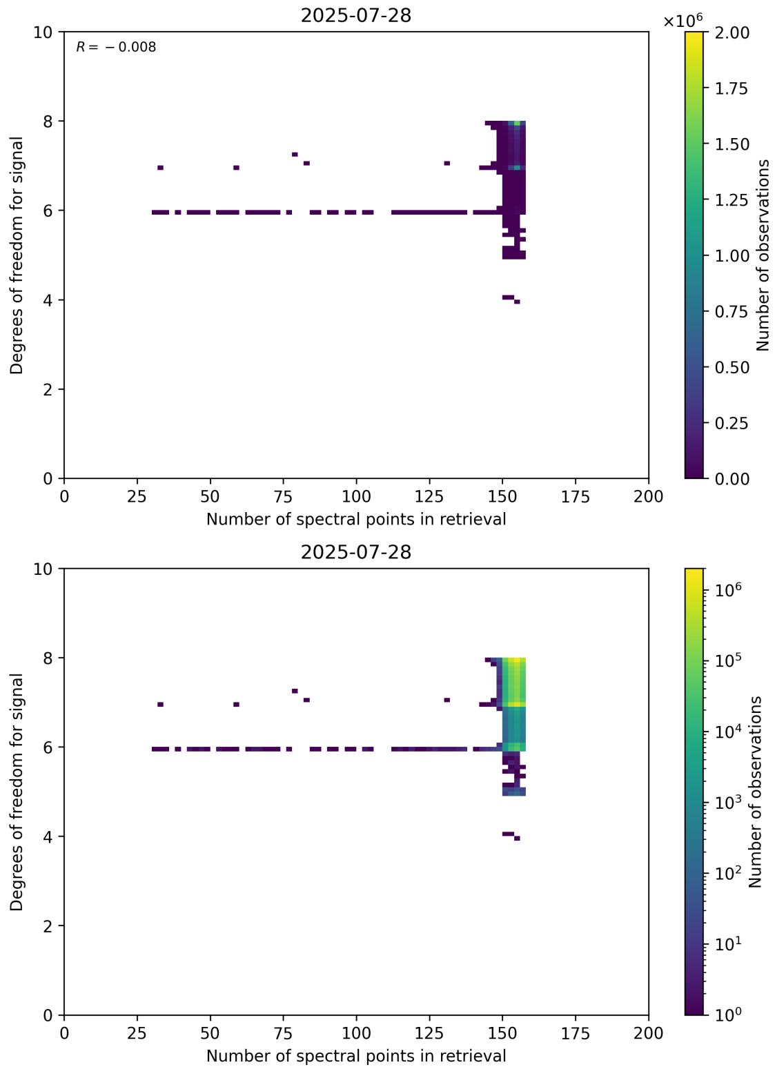
Figure 59: Scatter density plot of “Number of spectral points in retrieval” against “Degrees of freedom for signal” for 2025-07-27 to 2025-07-29.
