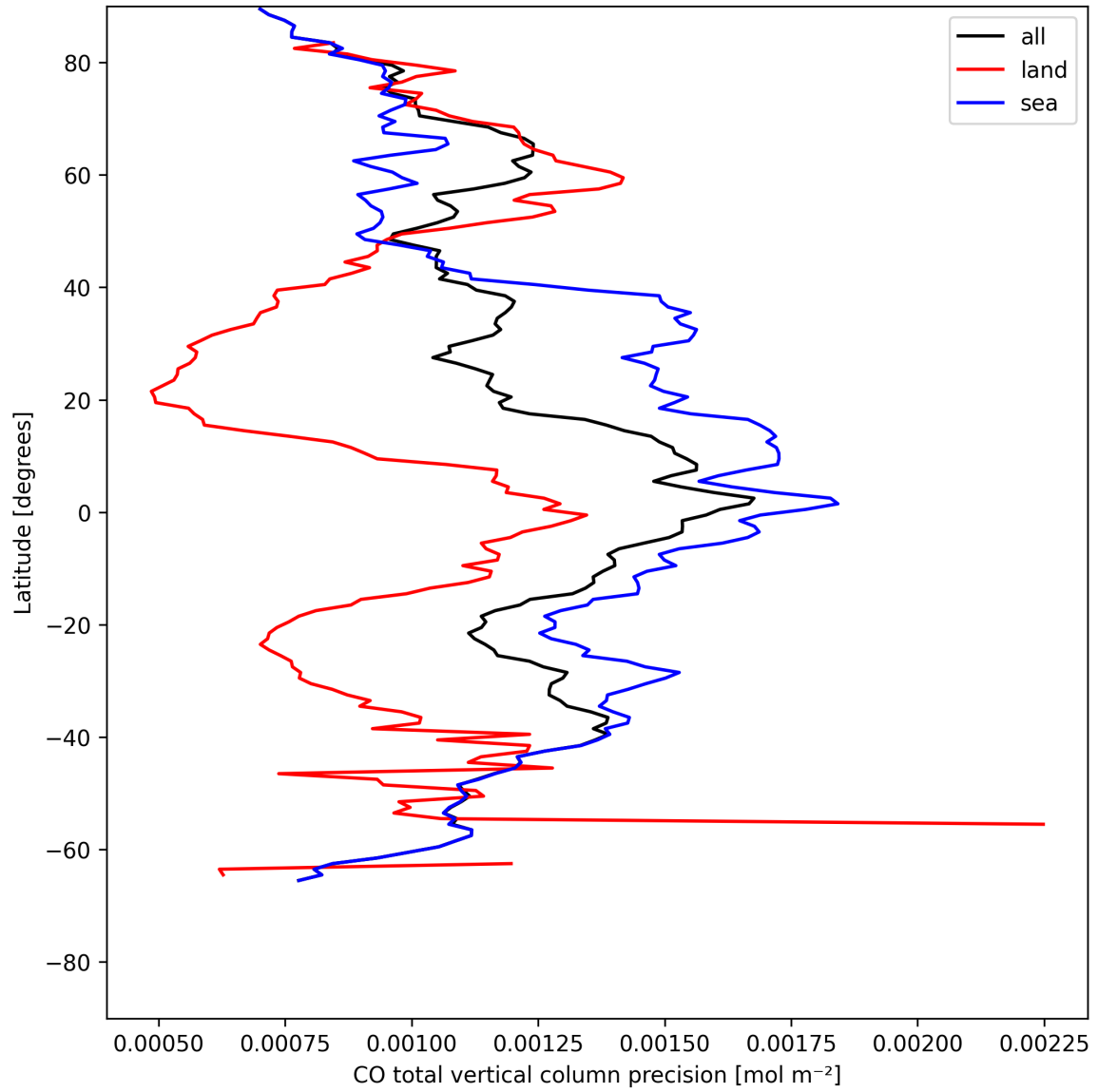
Figure 12: Zonal average of "CO total vertical column precision" for 2025-07-27 to 2025-07-29.
