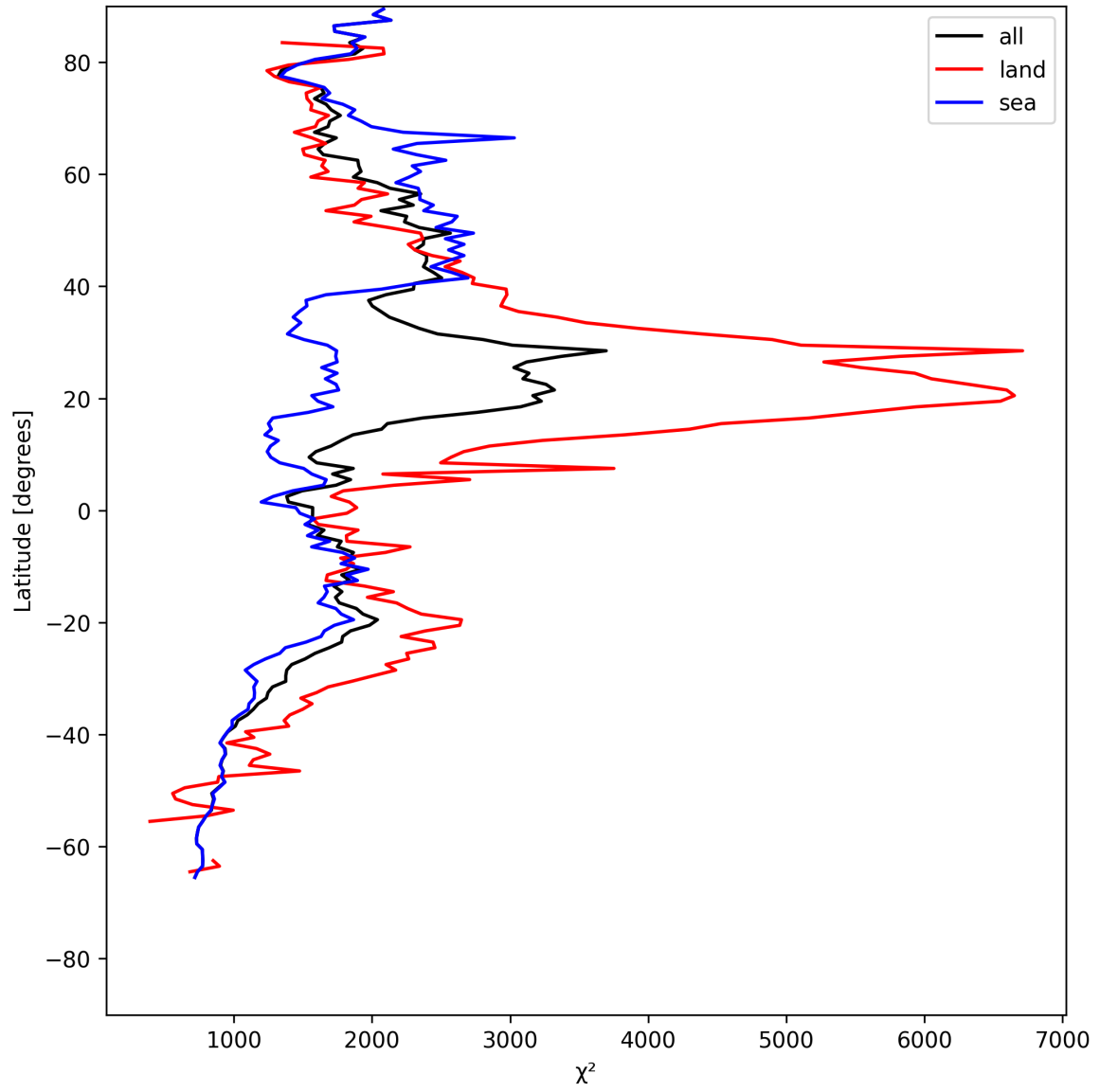
Figure 14: Zonal average of “ \chi^2 ” for 2025-07-27 to 2025-07-29.
