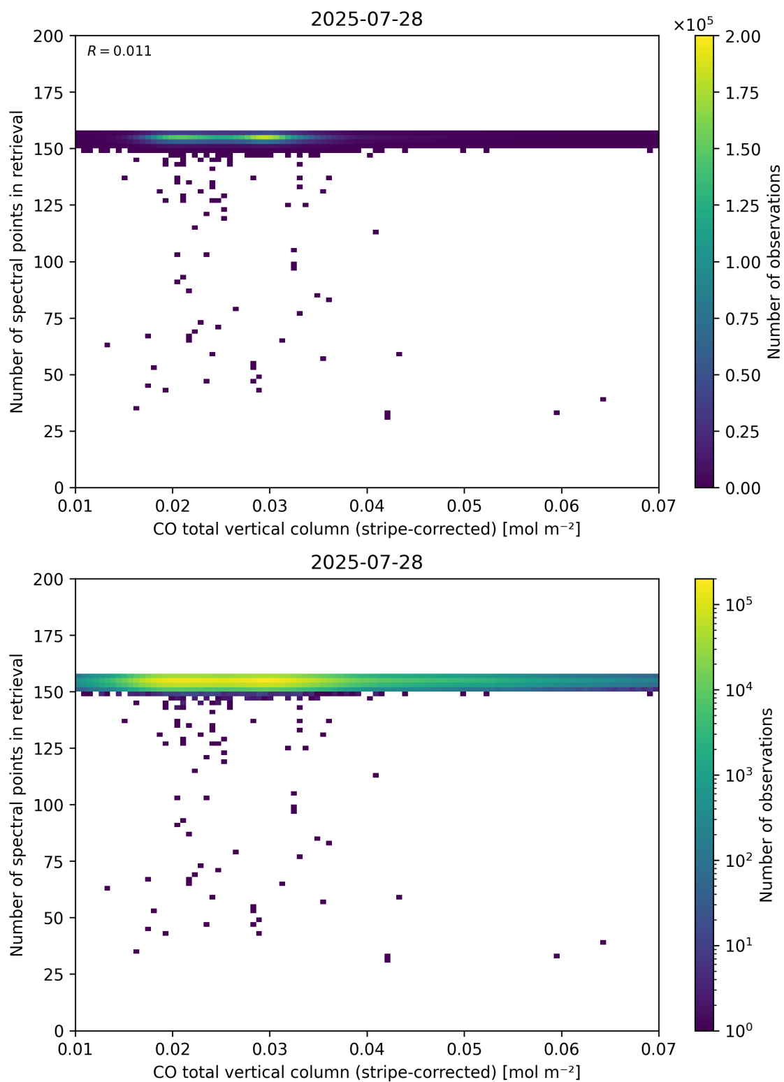
Figure 40: Scatter density plot of “CO total vertical column (stripe-corrected)” against “Number of spectral points in retrieval” for 2025-07-27 to 2025-07-29.
