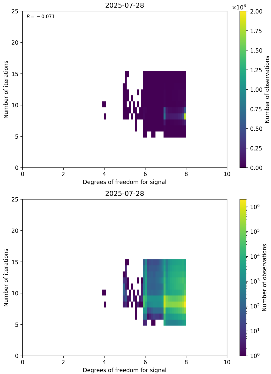
Figure 50: Scatter density plot of “Degrees of freedom for signal” against “Number of iterations” for 2025-07-27 to 2025-07-29.
