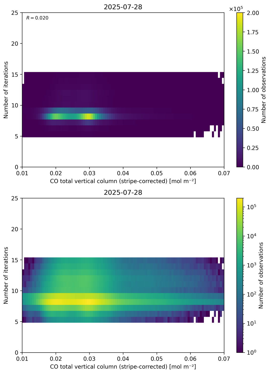
Figure 39: Scatter density plot of “CO total vertical column (stripe-corrected)” against “Number of iterations” for 2025-07-27 to 2025-07-29.
