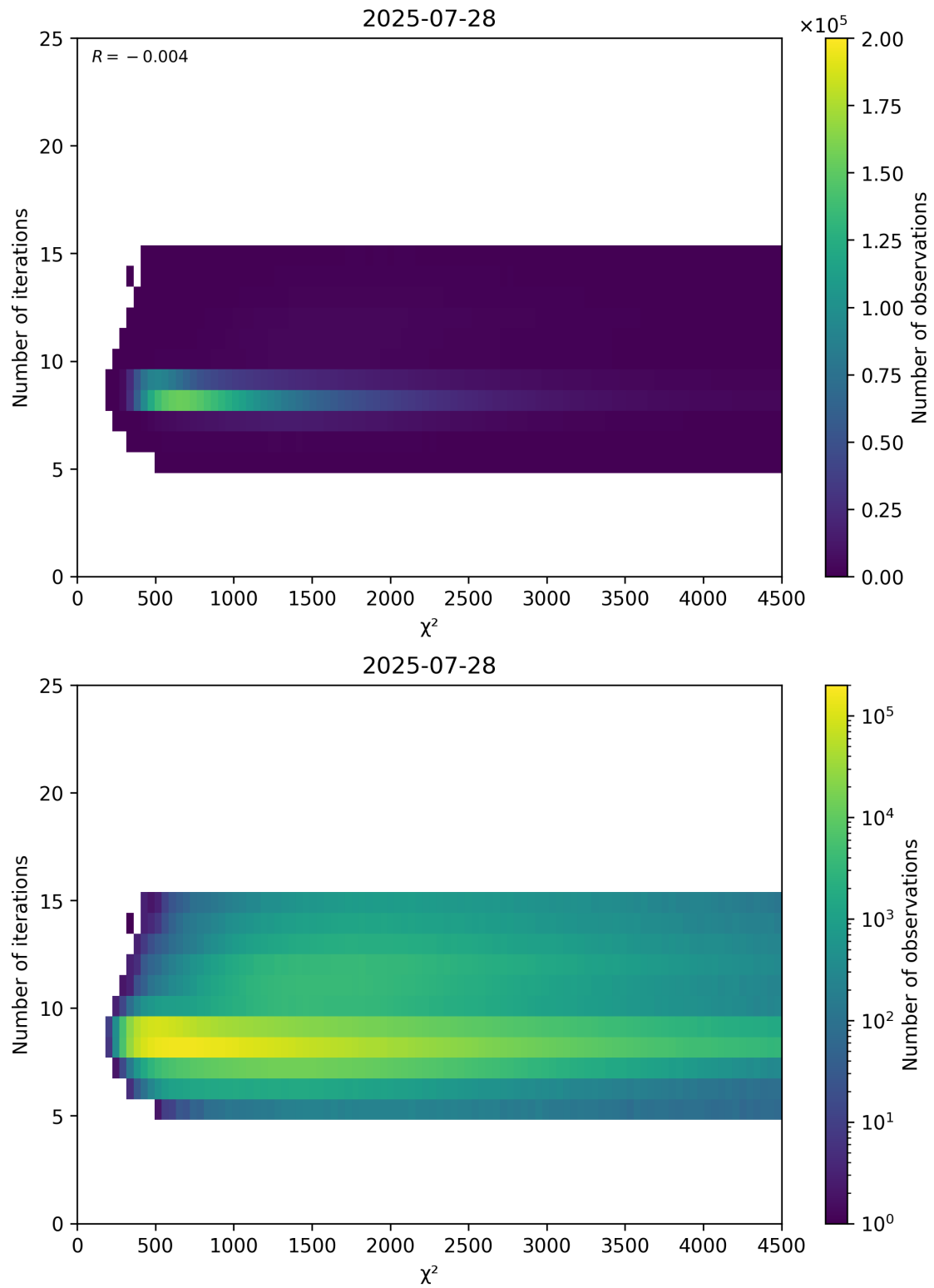
Figure 49: Scatter density plot of “ \chi^2 ” against “Number of iterations” for 2025-07-27 to 2025-07-29.
