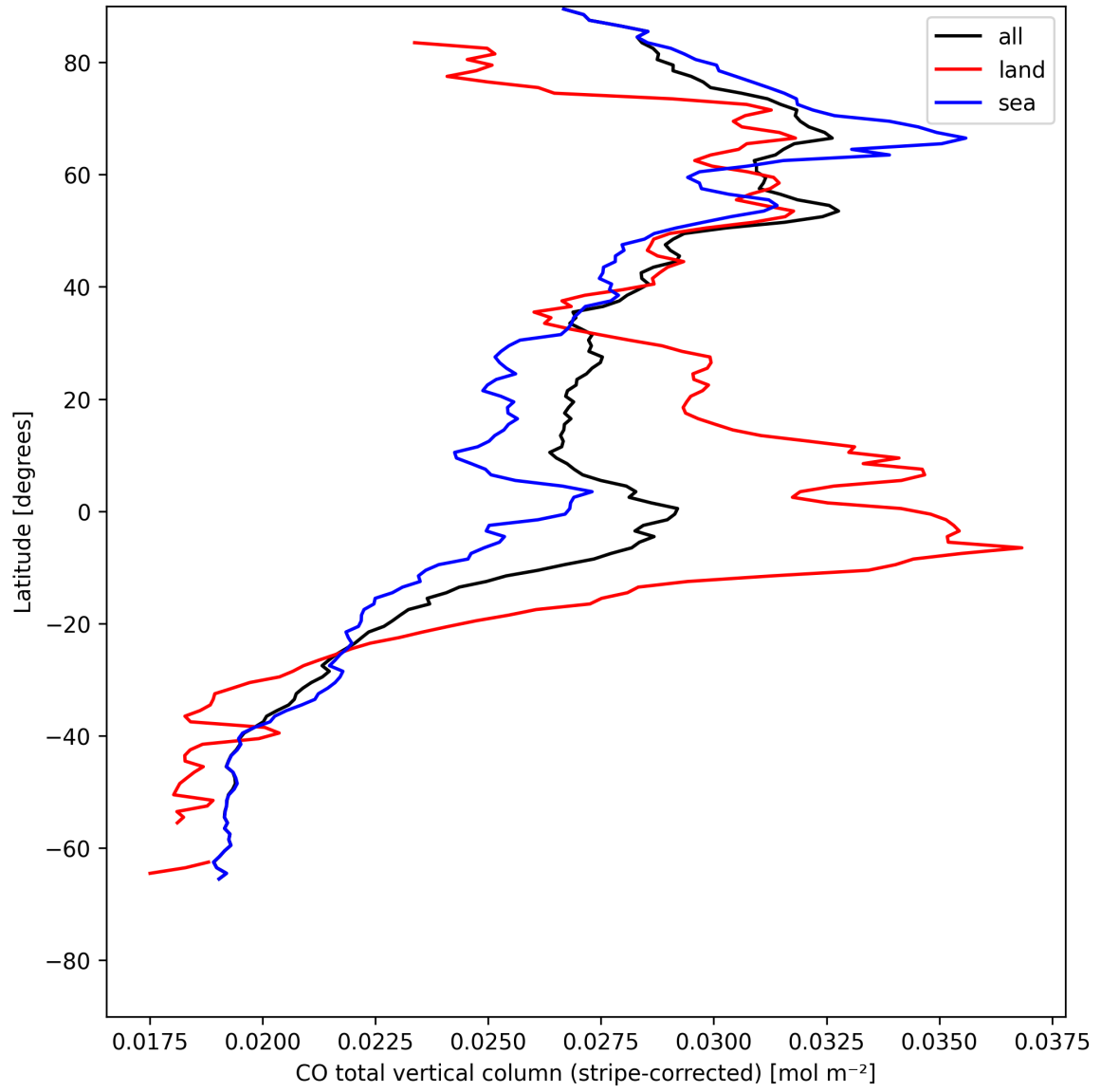
Figure 11: Zonal average of “CO total vertical column (stripe-corrected)” for 2025-07-27 to 2025-07-29.
