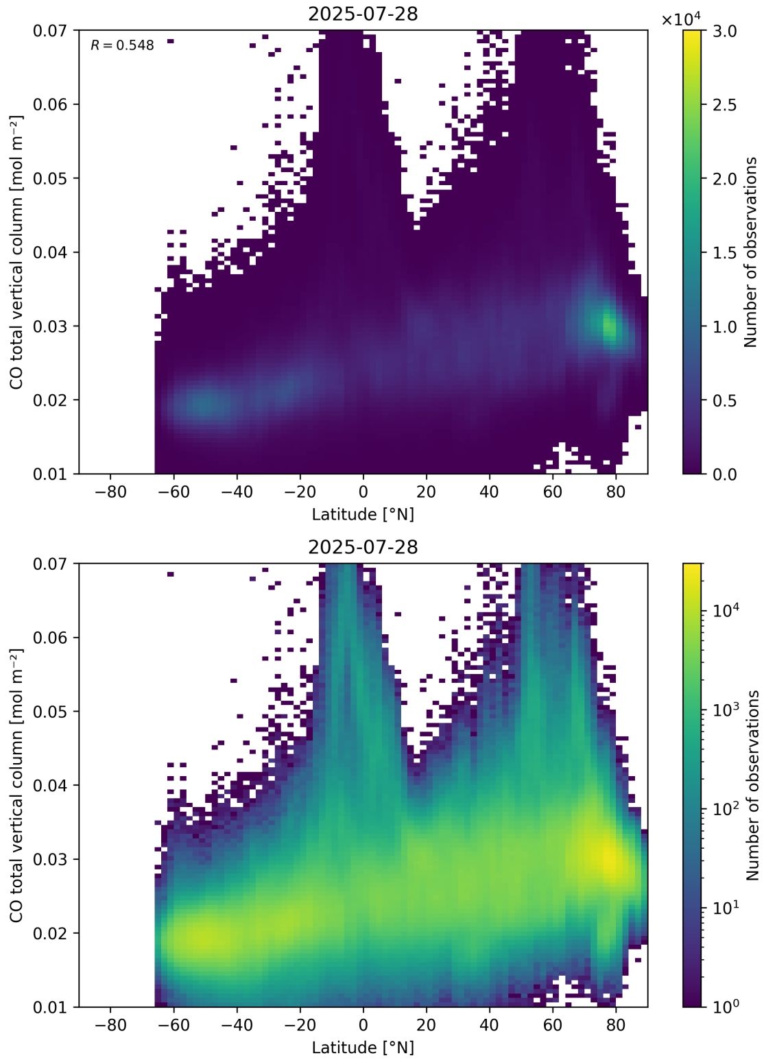
Figure 51: Scatter density plot of “Latitude” against “CO total vertical column” for 2025-07-27 to 2025-07-29.
