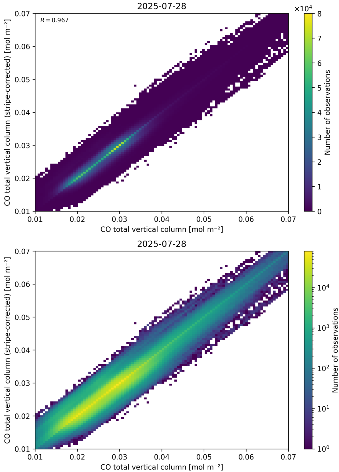
Figure 33: Scatter density plot of “CO total vertical column” against “CO total vertical column (stripe-corrected)” for 2025-07-27 to 2025-07-29.
