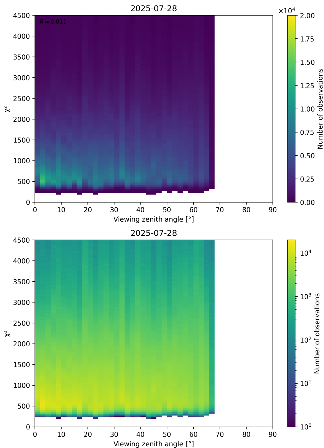
Figure 72: Scatter density plot of “Viewing zenith angle” against “ \chi^2 ” for 2025-07-27 to 2025-07-29.
