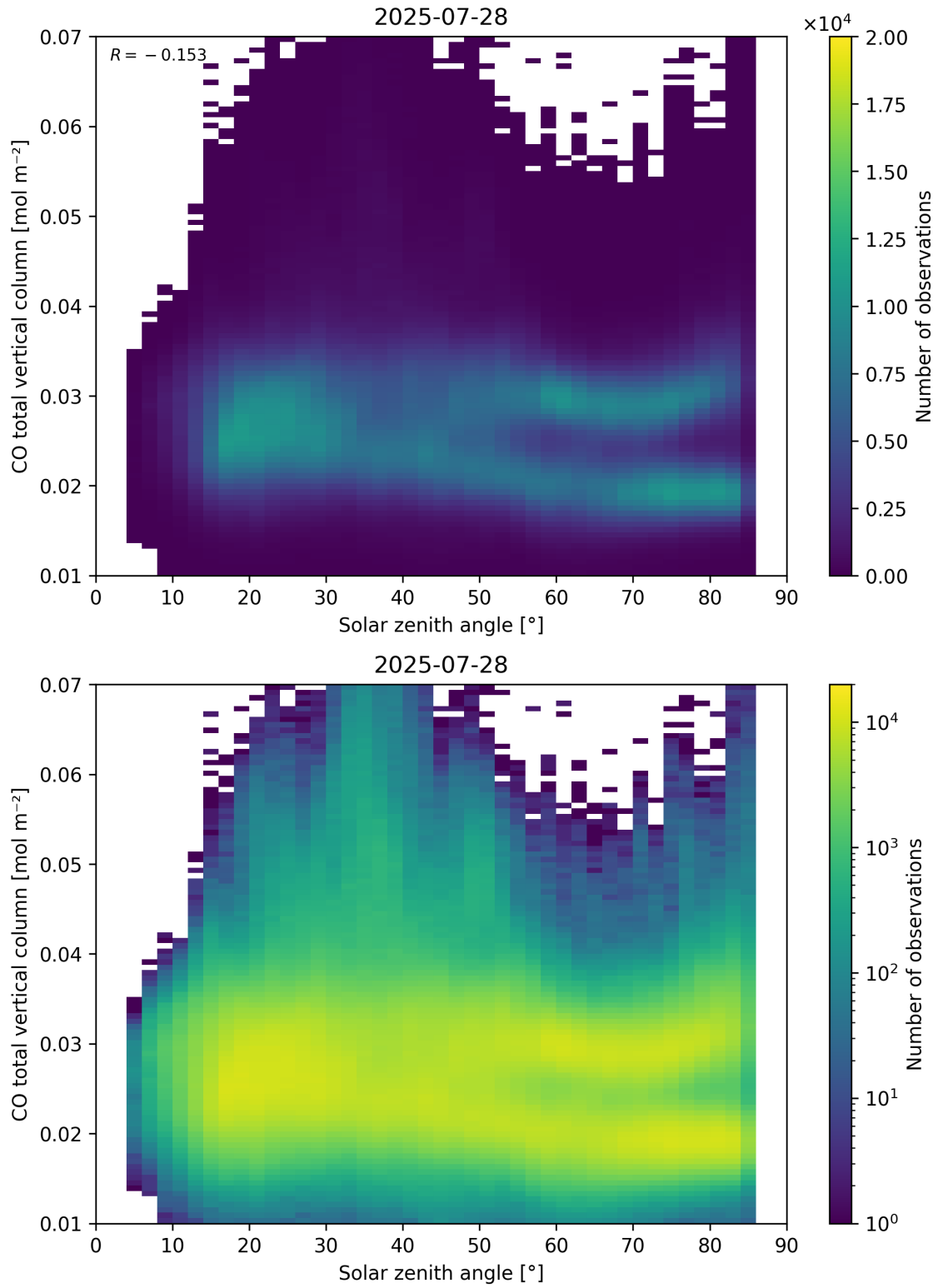
Figure 61: Scatter density plot of “Solar zenith angle” against “CO total vertical column” for 2025-07-27 to 2025-07-29.
