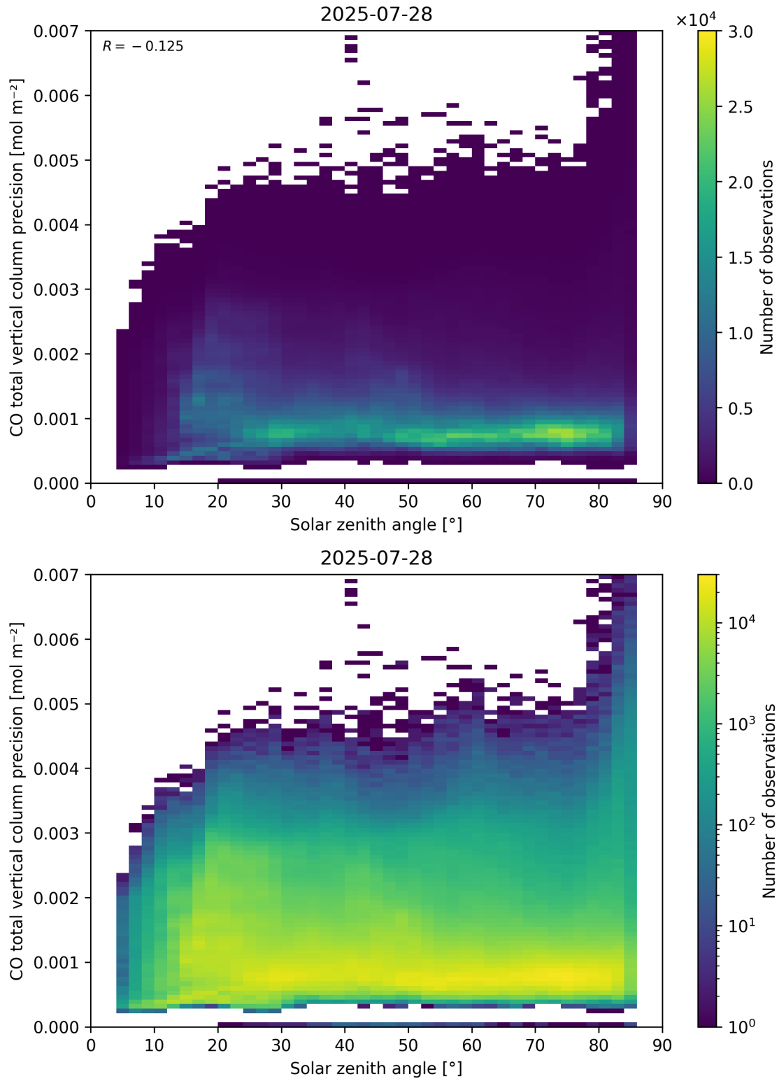
Figure 63: Scatter density plot of “Solar zenith angle” against “CO total vertical column precision” for 2025-07-27 to 2025-07-29.
