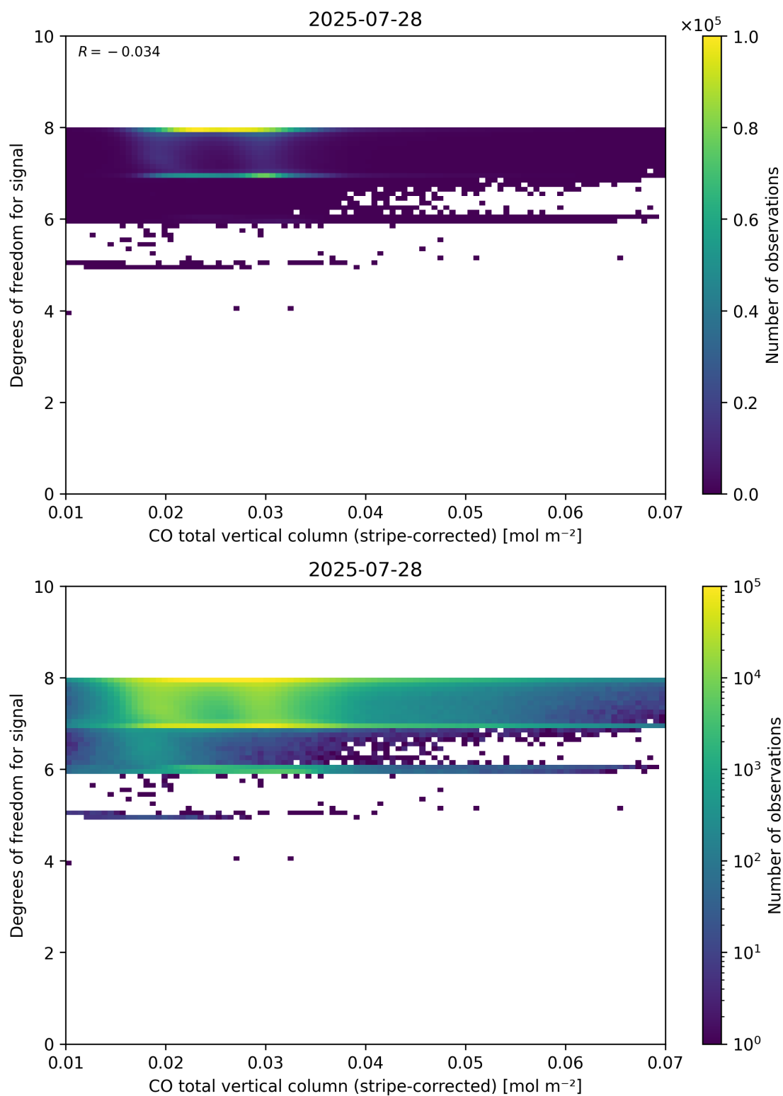
Figure 38: Scatter density plot of “CO total vertical column (stripe-corrected)” against “Degrees of freedom for signal” for 2025-07-27 to 2025-07-29.
