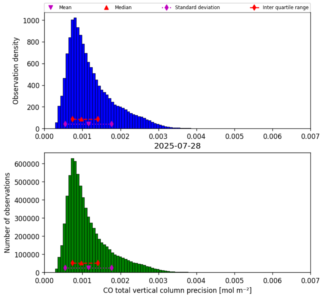
Figure 20: Histogram of “CO total vertical column precision” for 2025-07-27 to 2025-07-29
