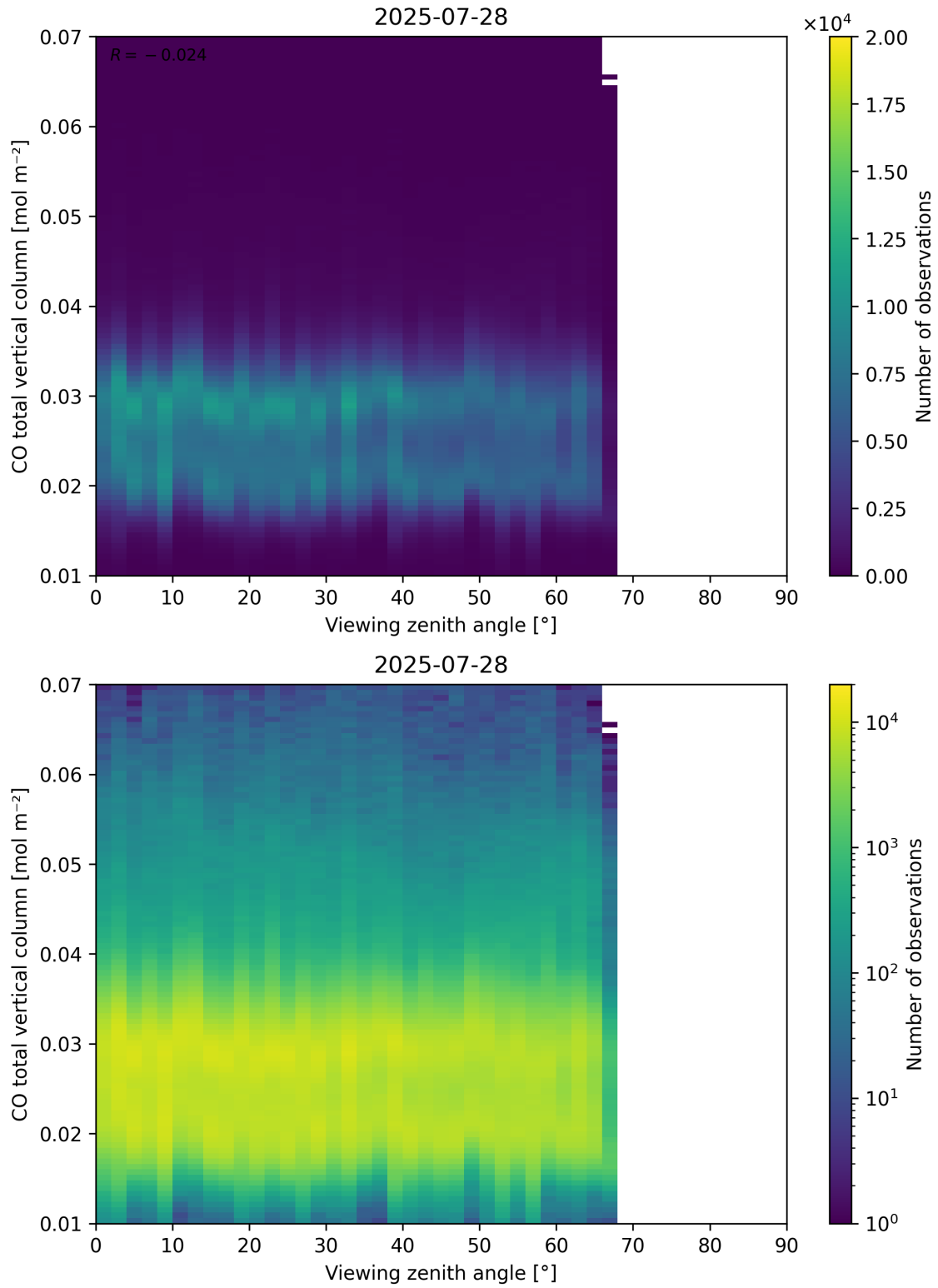
Figure 69: Scatter density plot of “Viewing zenith angle” against “CO total vertical column” for 2025-07-27 to 2025-07-29.
