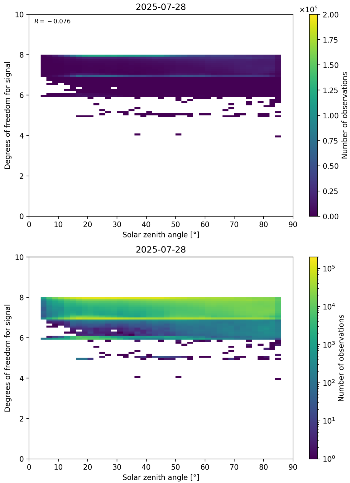
Figure 65: Scatter density plot of “Solar zenith angle” against “Degrees of freedom for signal” for 2025-07-27 to 2025-07-29.
