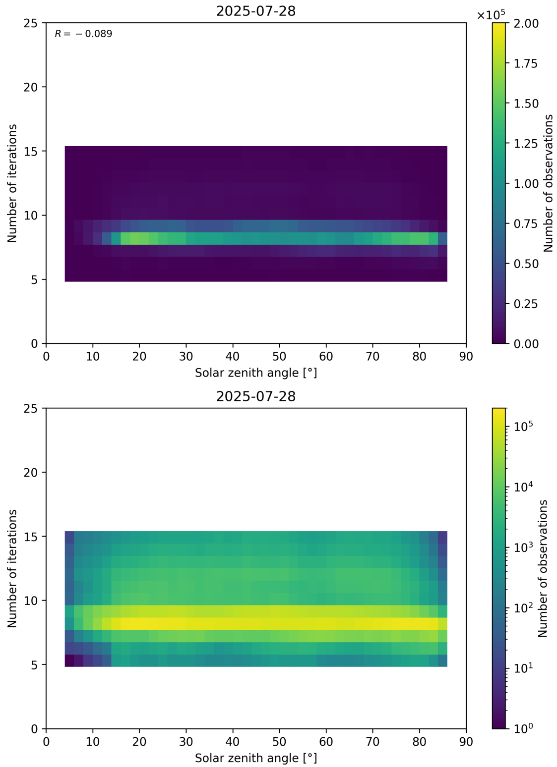
Figure 67: Scatter density plot of “Solar zenith angle” against “Number of iterations” for 2025-07-27 to 2025-07-29.
