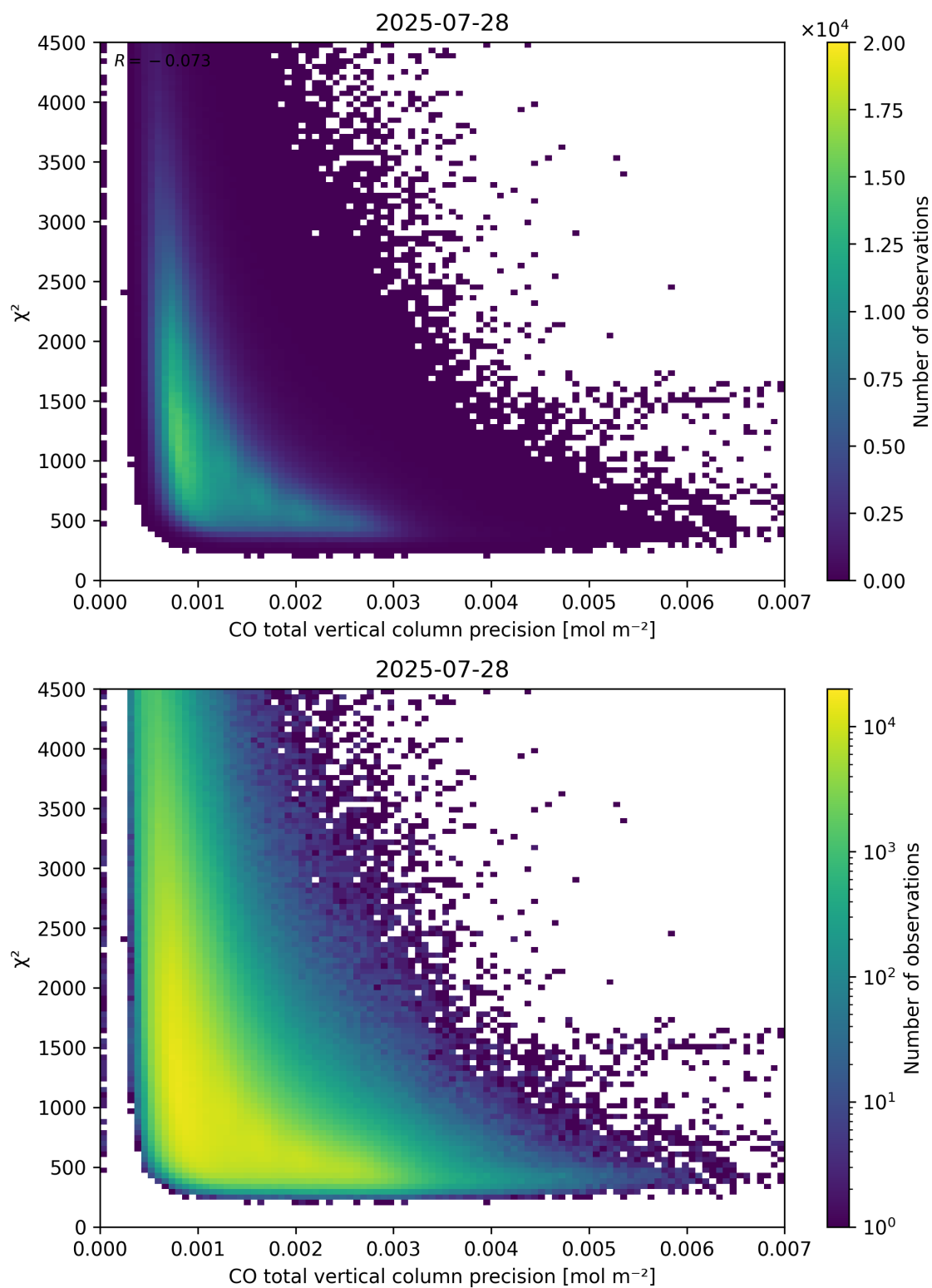
Figure 44: Scatter density plot of “CO total vertical column precision” against “ \chi^2 ” for 2025-07-27 to 2025-07-29.
