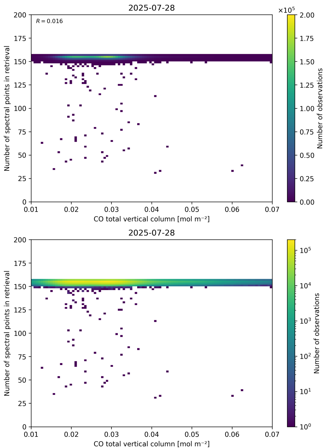
Figure 43: Scatter density plot of “CO total vertical column” against “Number of spectral points in retrieval” for 2025-07-27 to 2025-07-29.
