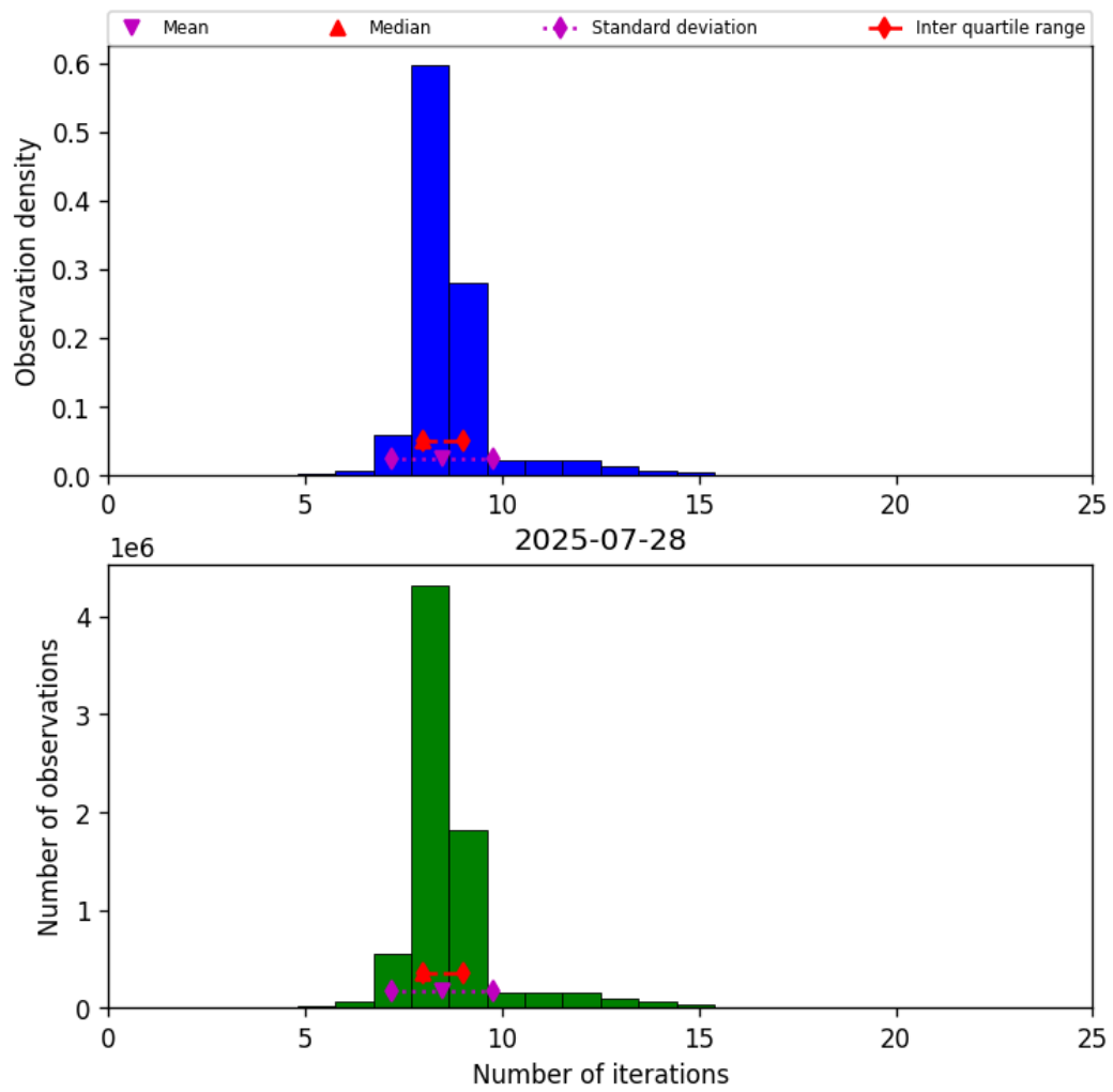
Figure 24: Histogram of “Number of iterations” for 2025-07-27 to 2025-07-29
