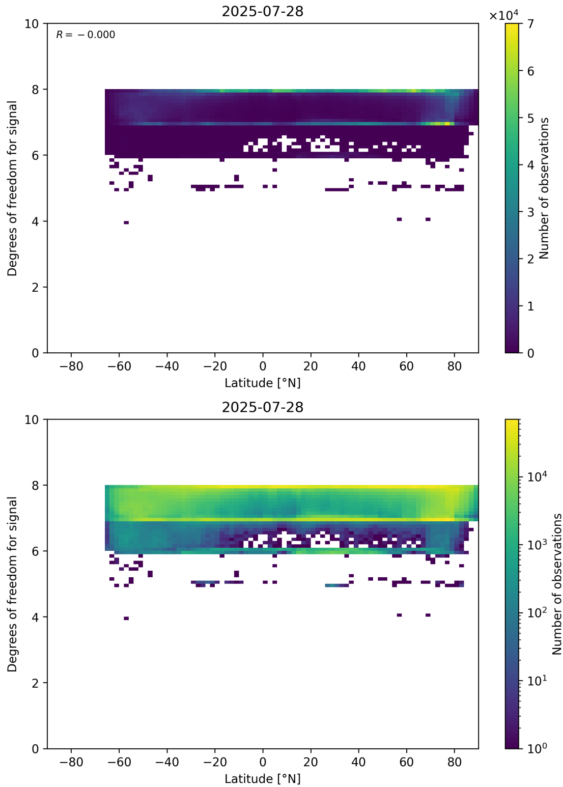
Figure 55: Scatter density plot of “Latitude” against “Degrees of freedom for signal” for 2025-07-27 to 2025-07-29.
