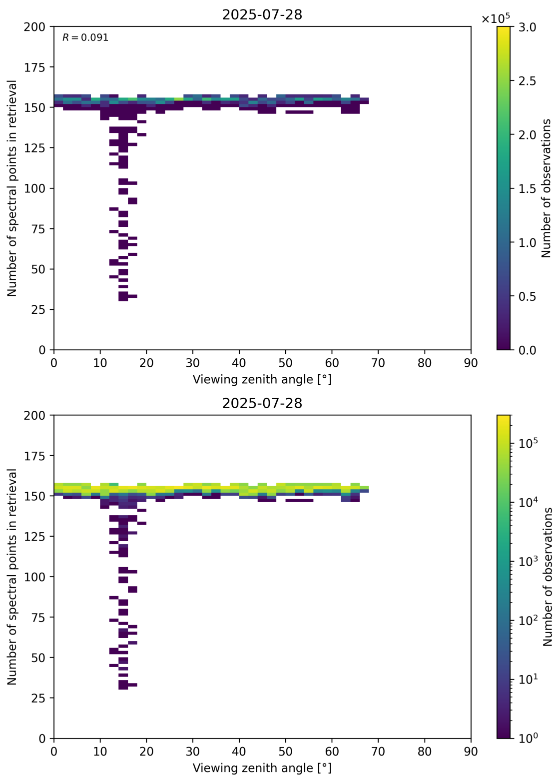
Figure 76: Scatter density plot of “Viewing zenith angle” against “Number of spectral points in retrieval” for 2025-07-27 to 2025-07-29.
