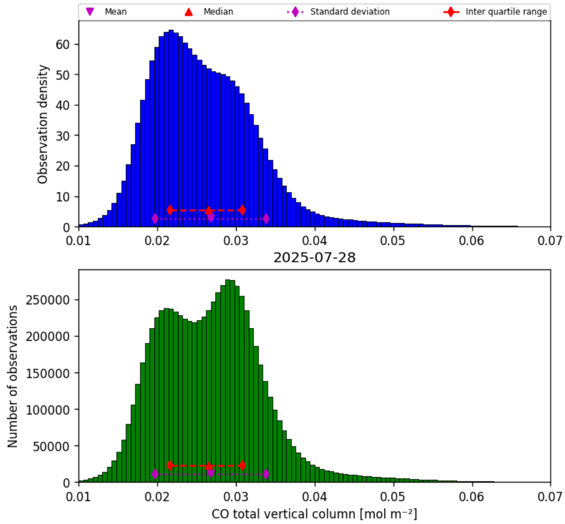
Figure 18: Histogram of “CO total vertical column” for 2025-07-27 to 2025-07-29
