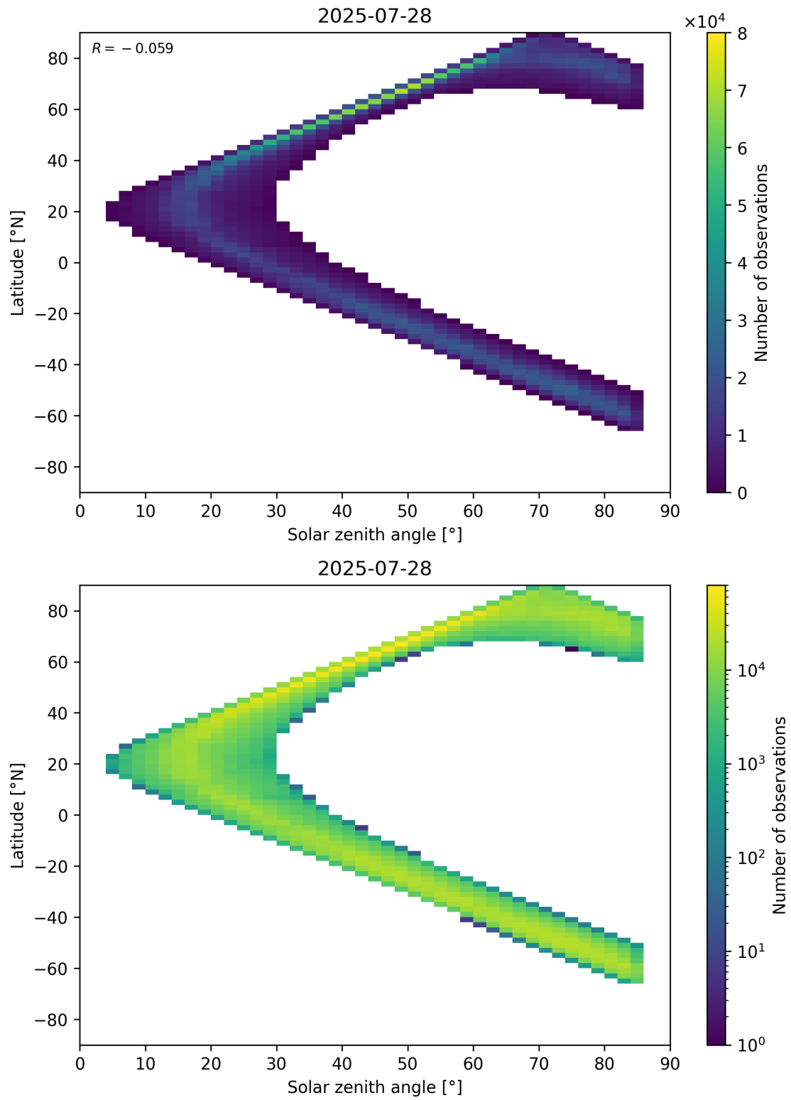
Figure 66: Scatter density plot of “Solar zenith angle” against “Latitude” for 2025-07-27 to 2025-07-29.
