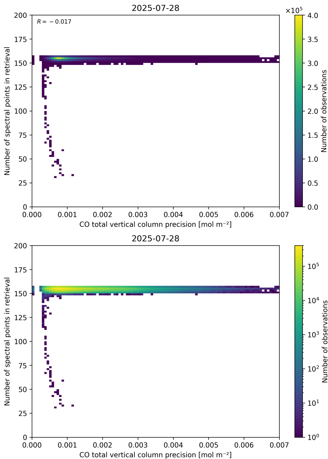
Figure 47: Scatter density plot of “CO total vertical column precision” against “Number of spectral points in retrieval” for 2025-07-27 to 2025-07-29.
