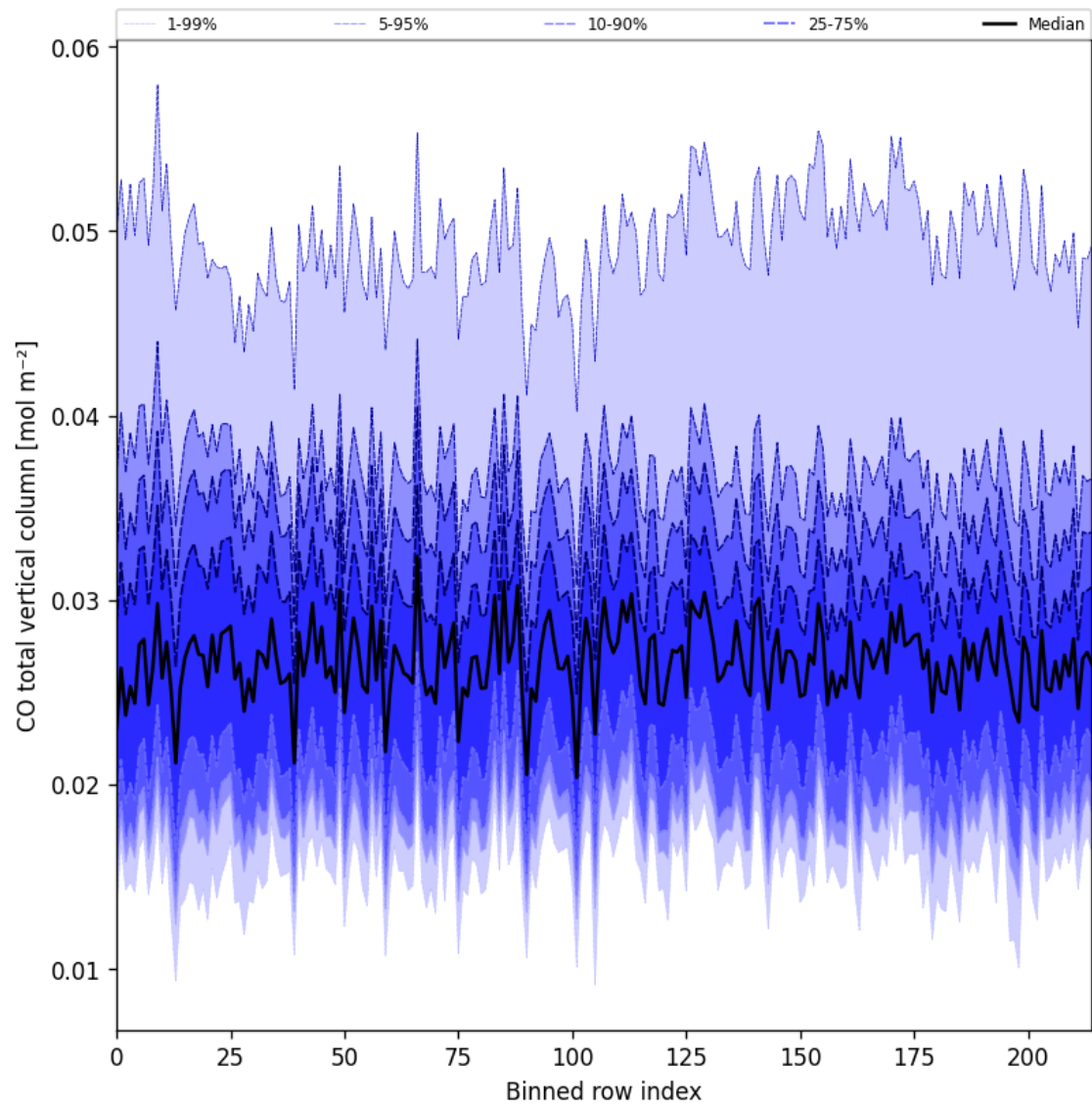
Figure 26: Along track statistics of “CO total vertical column” for 2025-07-27 to 2025-07-29
