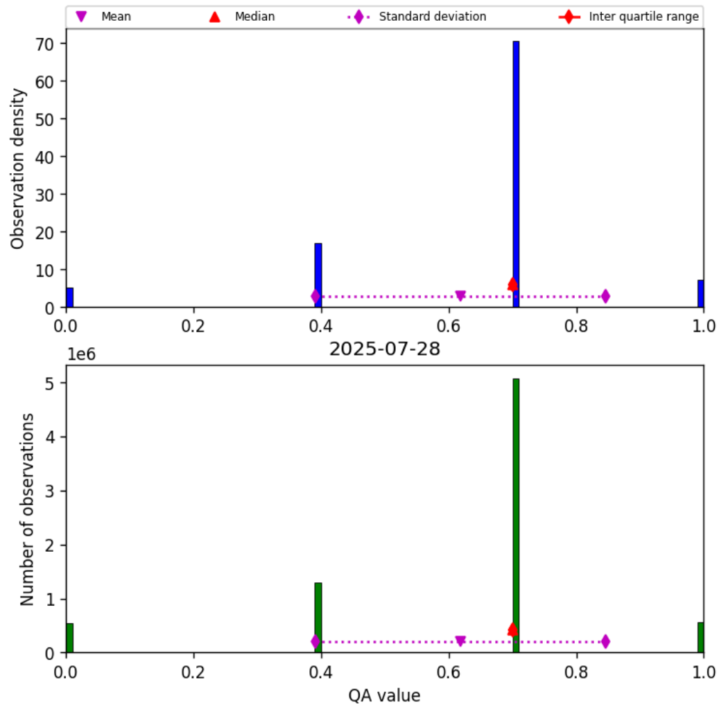
Figure 17: Histogram of “QA value” for 2025-07-27 to 2025-07-29
