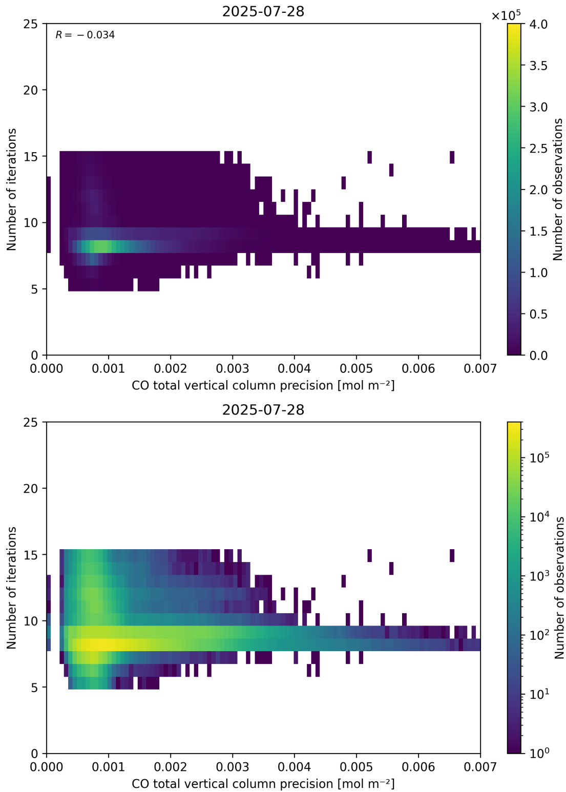
Figure 46: Scatter density plot of “CO total vertical column precision” against “Number of iterations” for 2025-07-27 to 2025-07-29.
