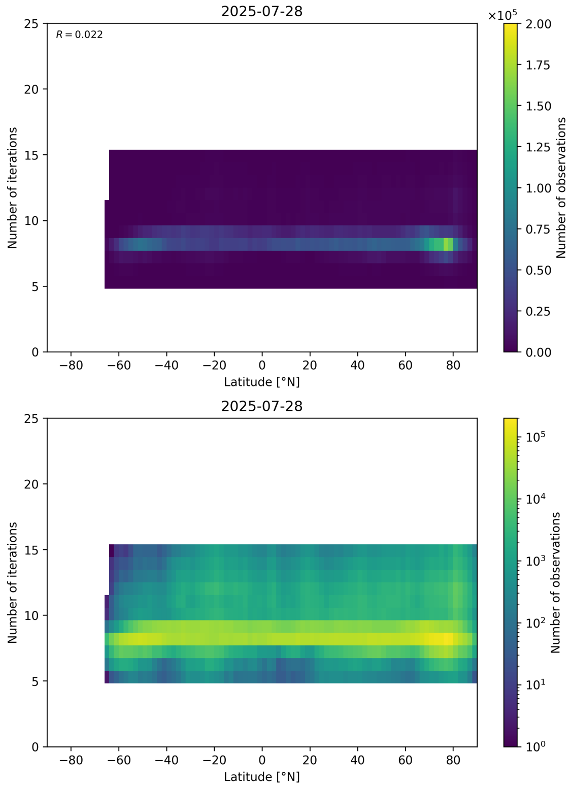
Figure 56: Scatter density plot of “Latitude” against “Number of iterations” for 2025-07-27 to 2025-07-29.
