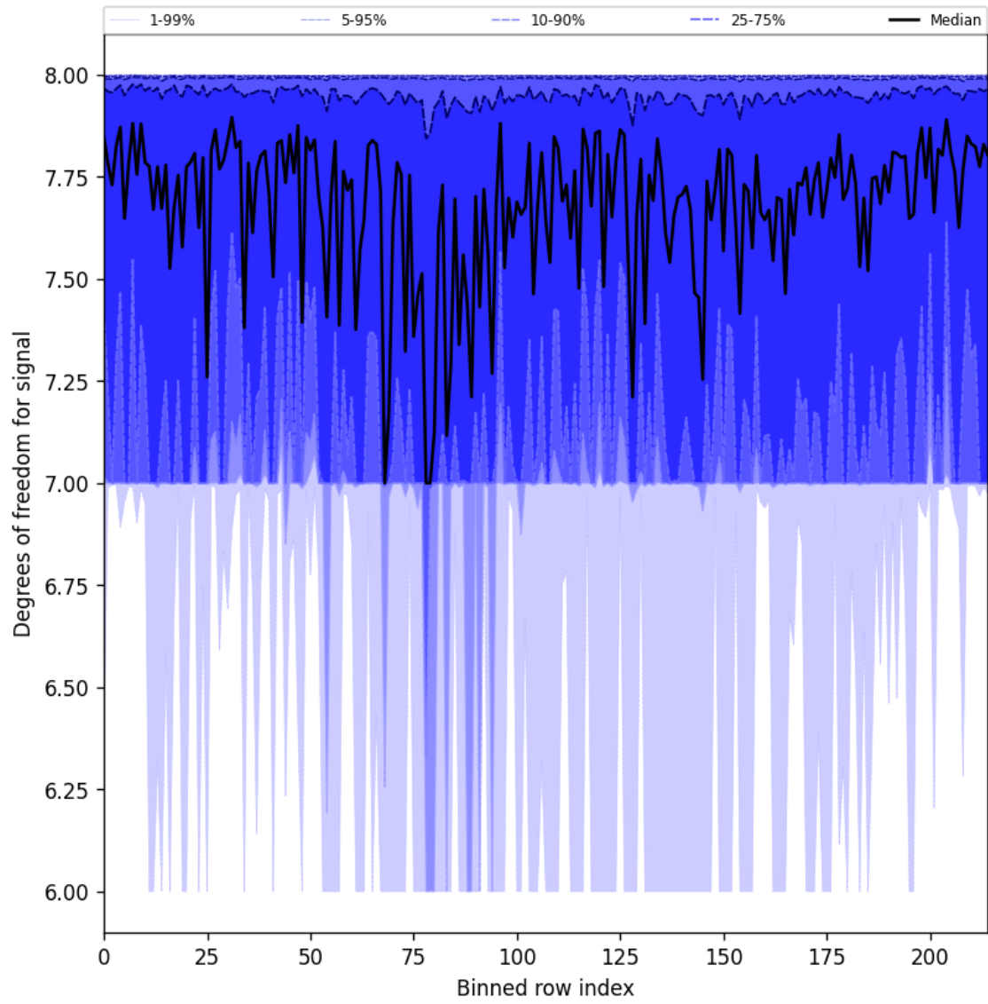
Figure 31: Along track statistics of “Degrees of freedom for signal” for 2025-07-27 to 2025-07-29
