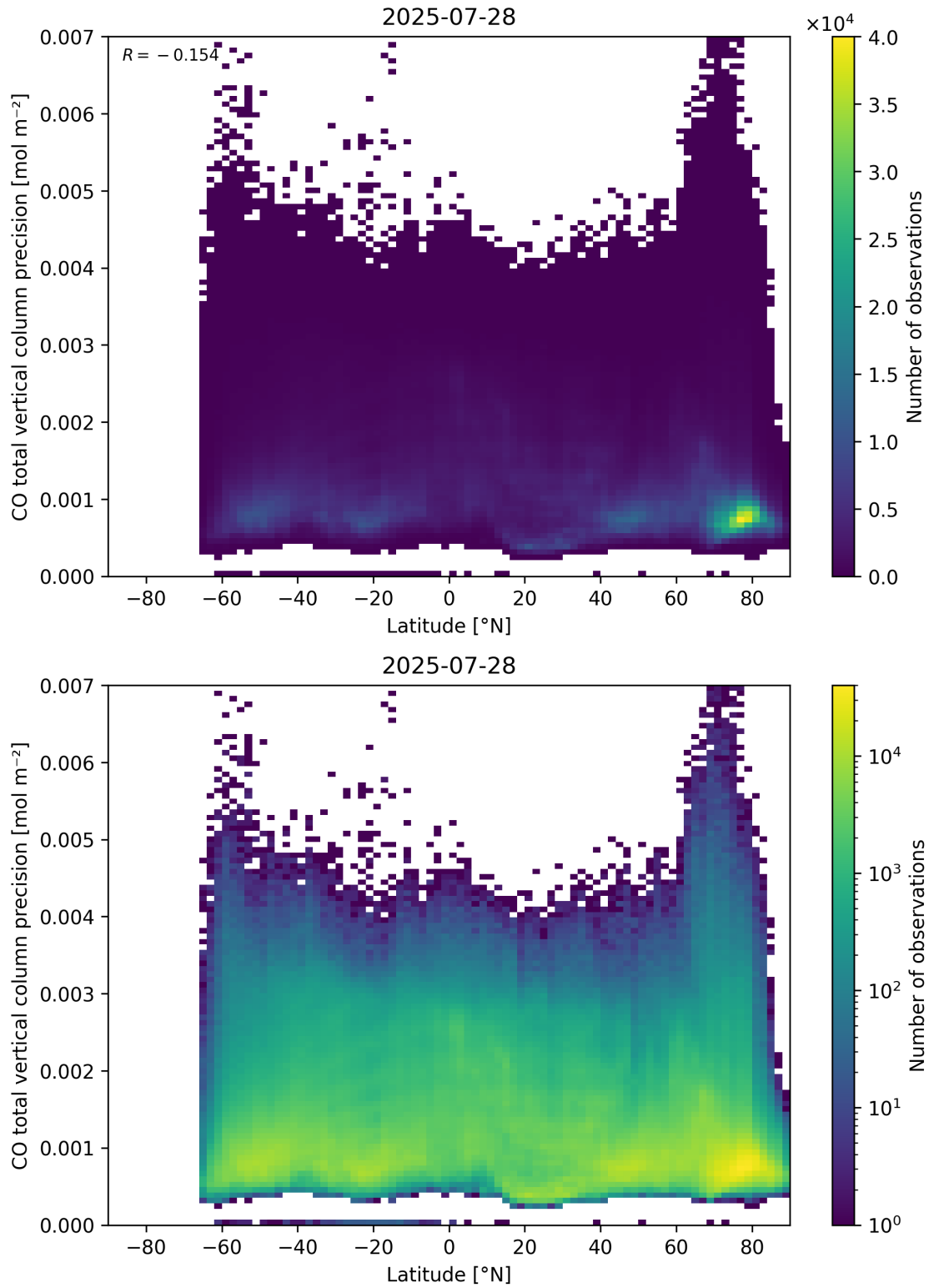
Figure 53: Scatter density plot of “Latitude” against “CO total vertical column precision” for 2025-07-27 to 2025-07-29.
