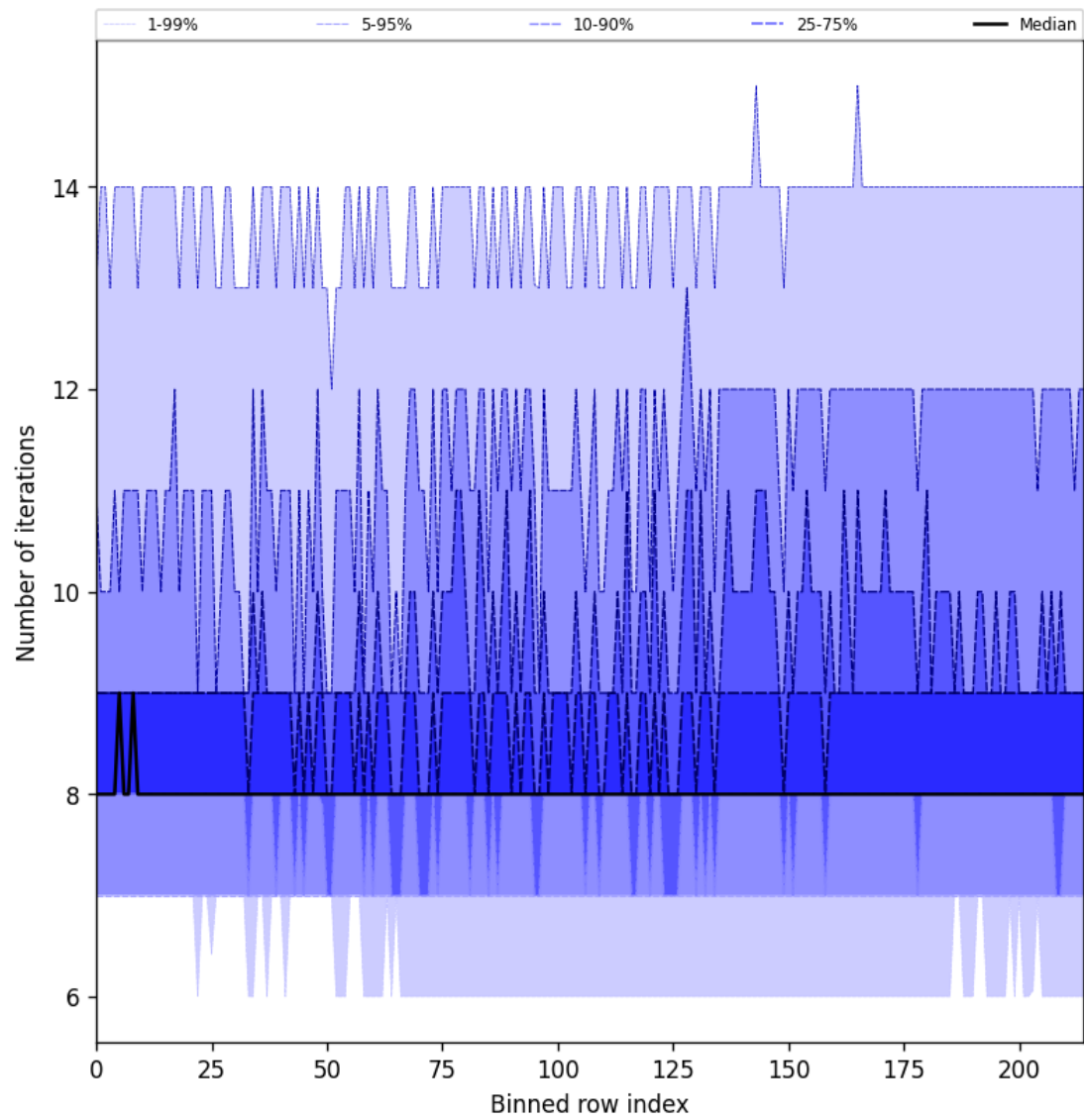
Figure 32: Along track statistics of “Number of iterations” for 2025-07-27 to 2025-07-29
