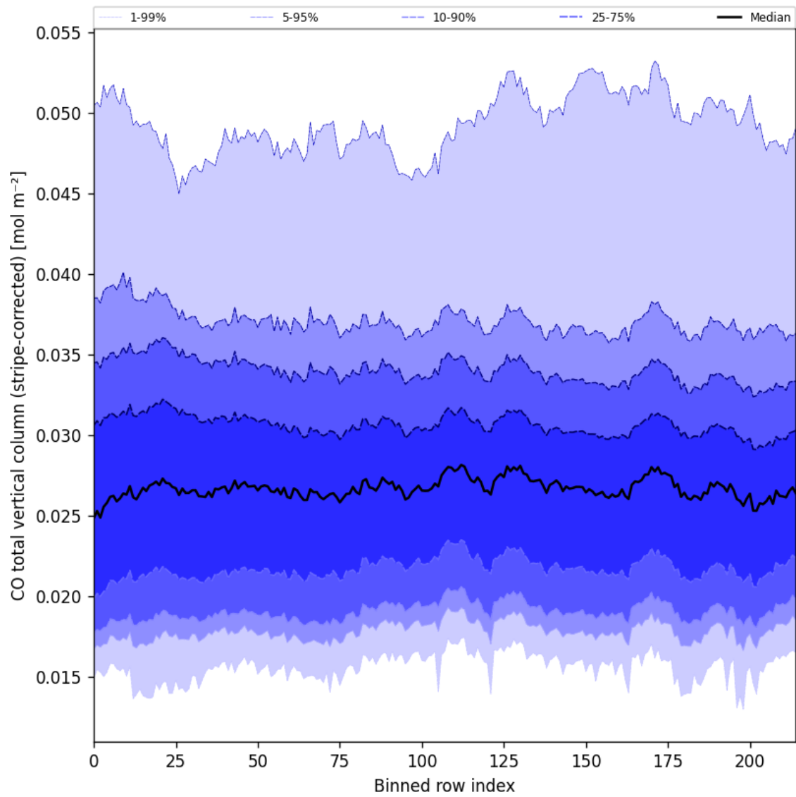
Figure 27: Along track statistics of “CO total vertical column (stripe-corrected)” for 2025-07-27 to 2025-07-29
