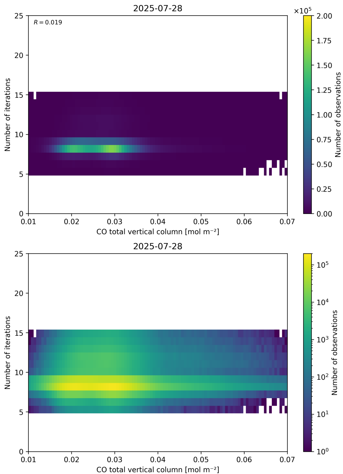
Figure 42: Scatter density plot of “CO total vertical column” against “Number of iterations” for 2025-07-27 to 2025-07-29.
