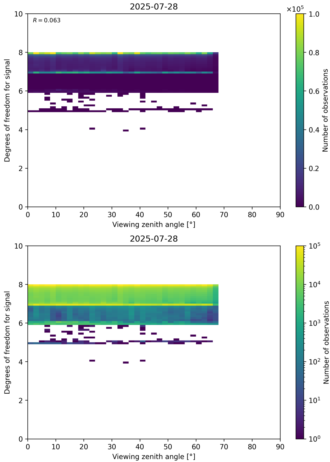
Figure 73: Scatter density plot of “Viewing zenith angle” against “Degrees of freedom for signal” for 2025-07-27 to 2025-07-29.
