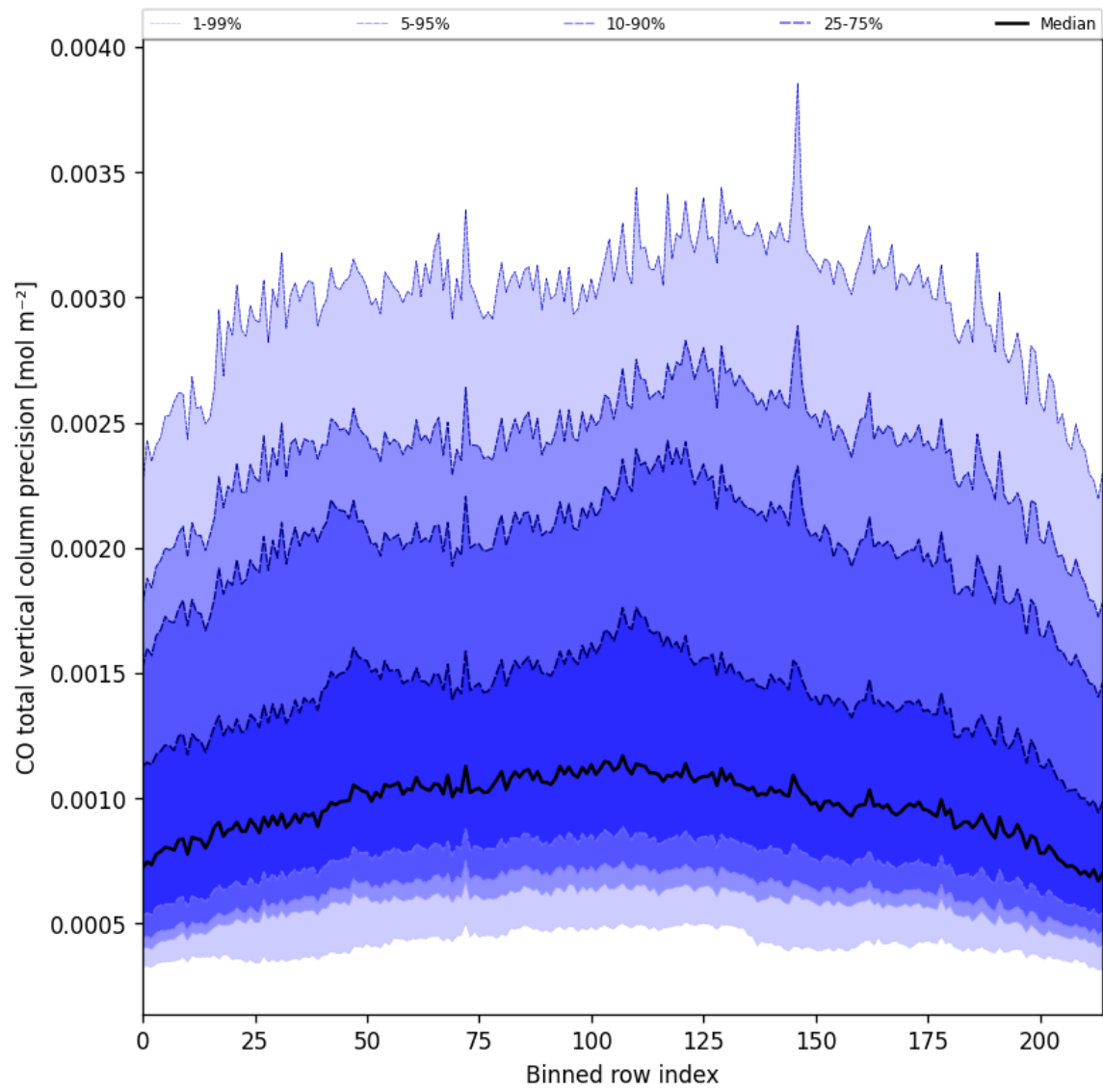
Figure 28: Along track statistics of “CO total vertical column precision” for 2025-07-27 to 2025-07-29
