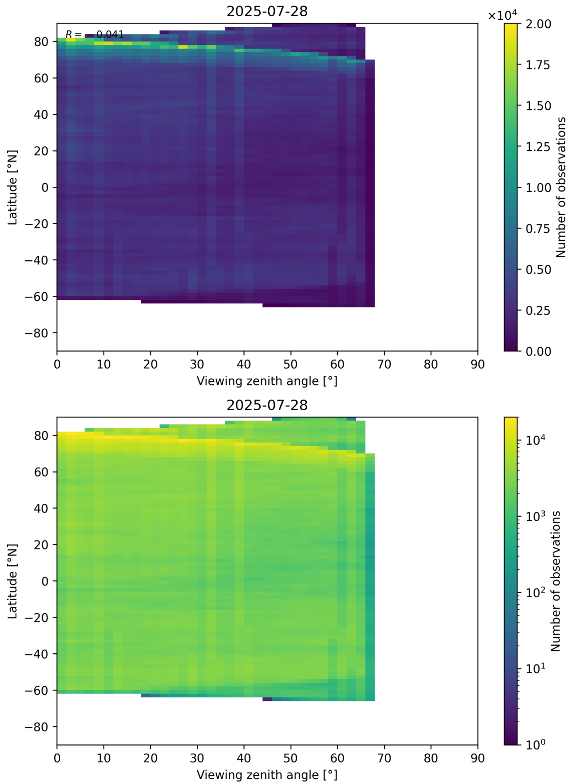
Figure 74: Scatter density plot of “Viewing zenith angle” against “Latitude” for 2025-07-27 to 2025-07-29.
