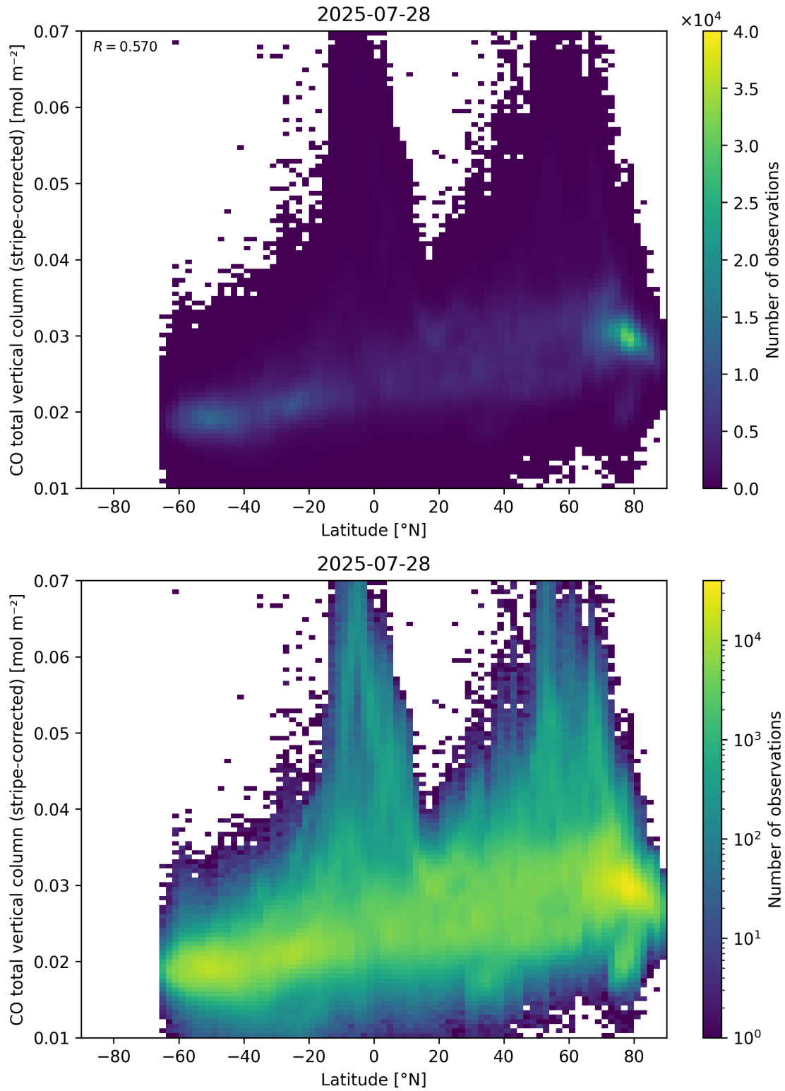
Figure 52: Scatter density plot of “Latitude” against “CO total vertical column (stripe-corrected)” for 2025-07-27 to 2025-07-29.
