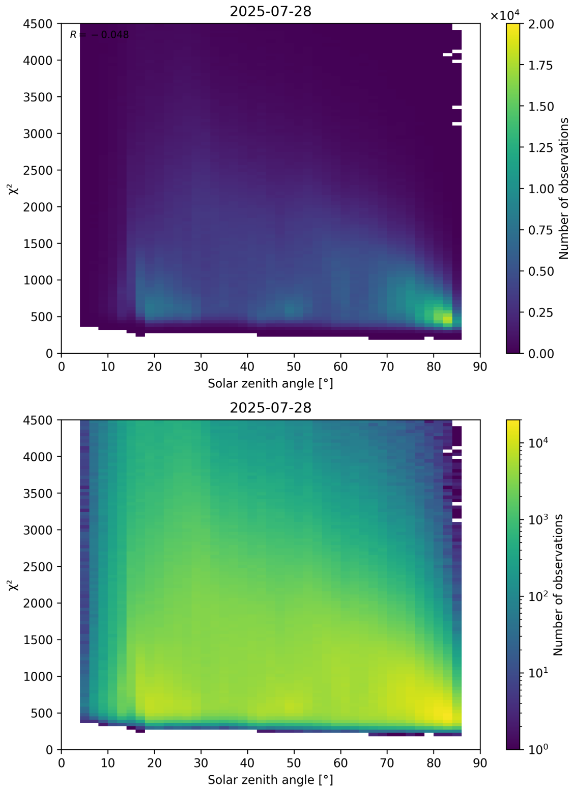
Figure 64: Scatter density plot of “Solar zenith angle” against “ \chi^2 ” for 2025-07-27 to 2025-07-29.
