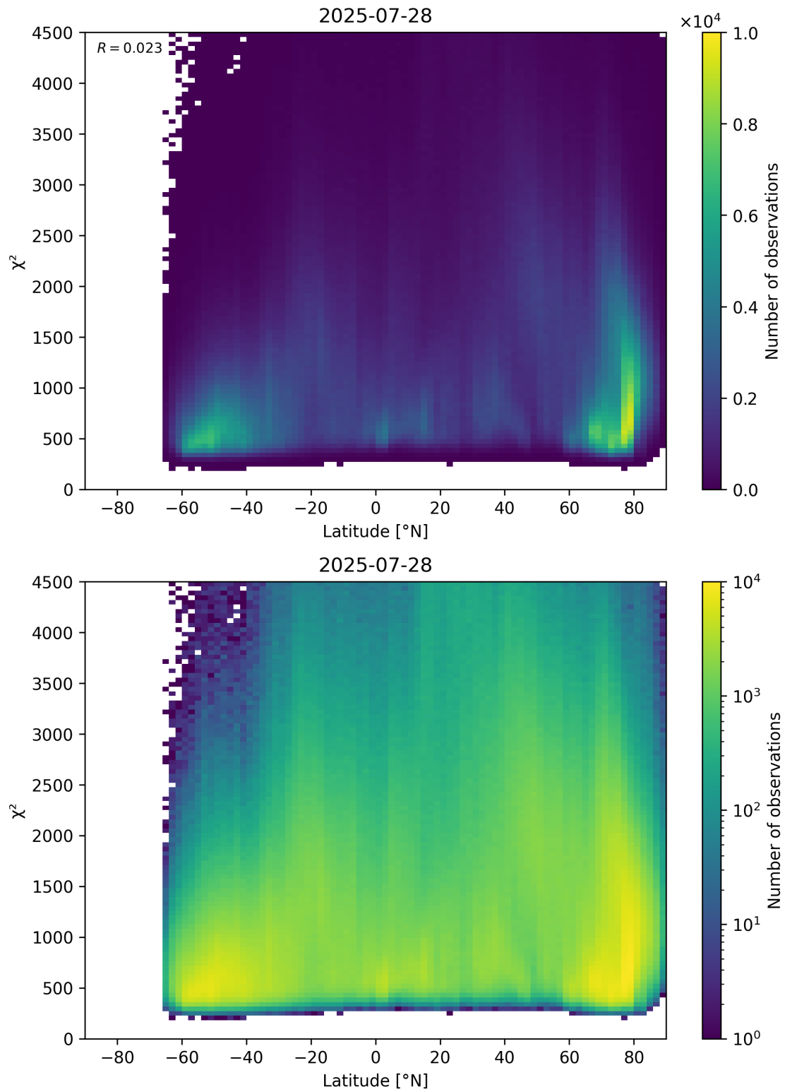
Figure 54: Scatter density plot of “Latitude” against “ \chi^2 ” for 2025-07-27 to 2025-07-29.
