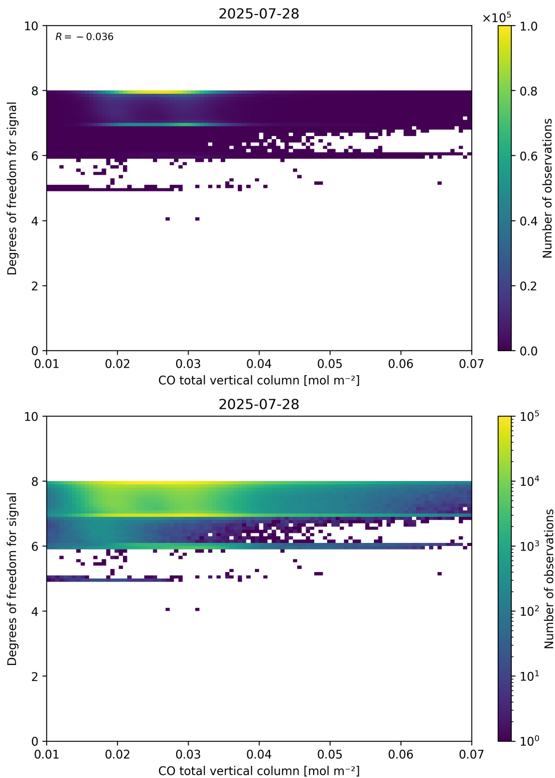
Figure 41: Scatter density plot of “CO total vertical column” against “Degrees of freedom for signal” for 2025-07-27 to 2025-07-29.
