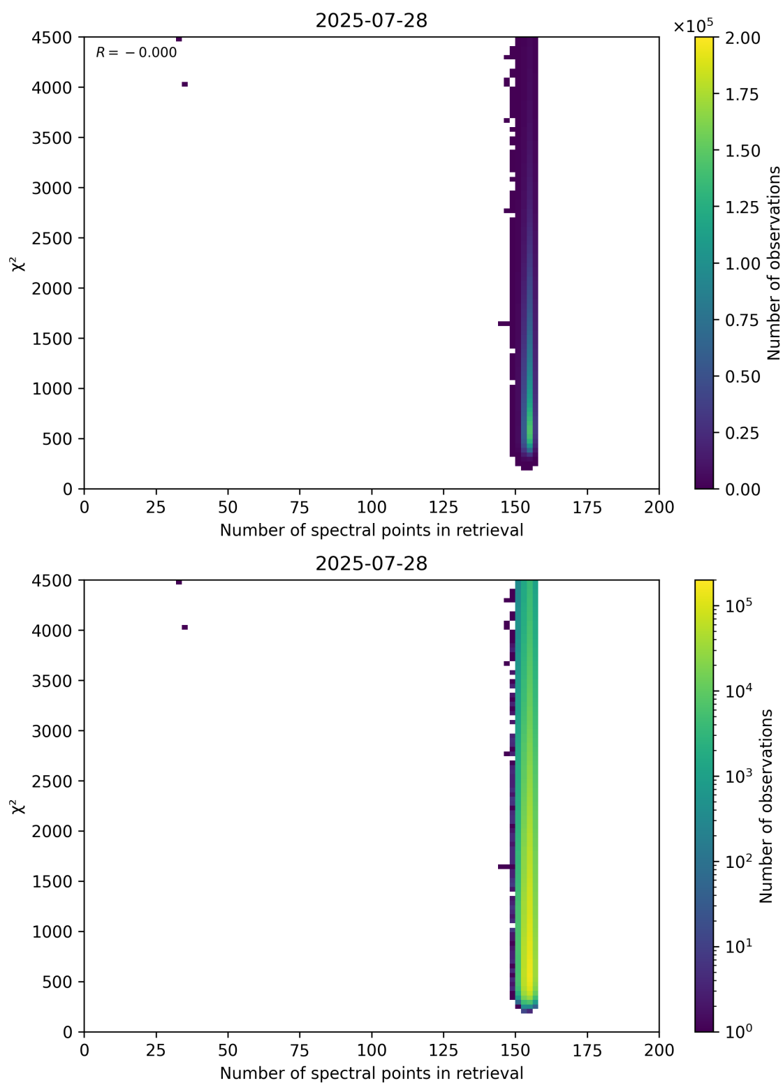
Figure 58: Scatter density plot of “Number of spectral points in retrieval” against “ \chi^2 ” for 2025-07-27 to 2025-07-29.
