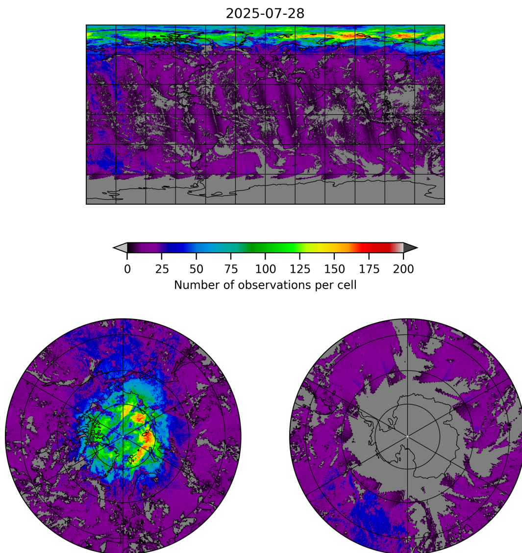
Figure 8: Map of the number of observations for 2025-07-27 to 2025-07-29
