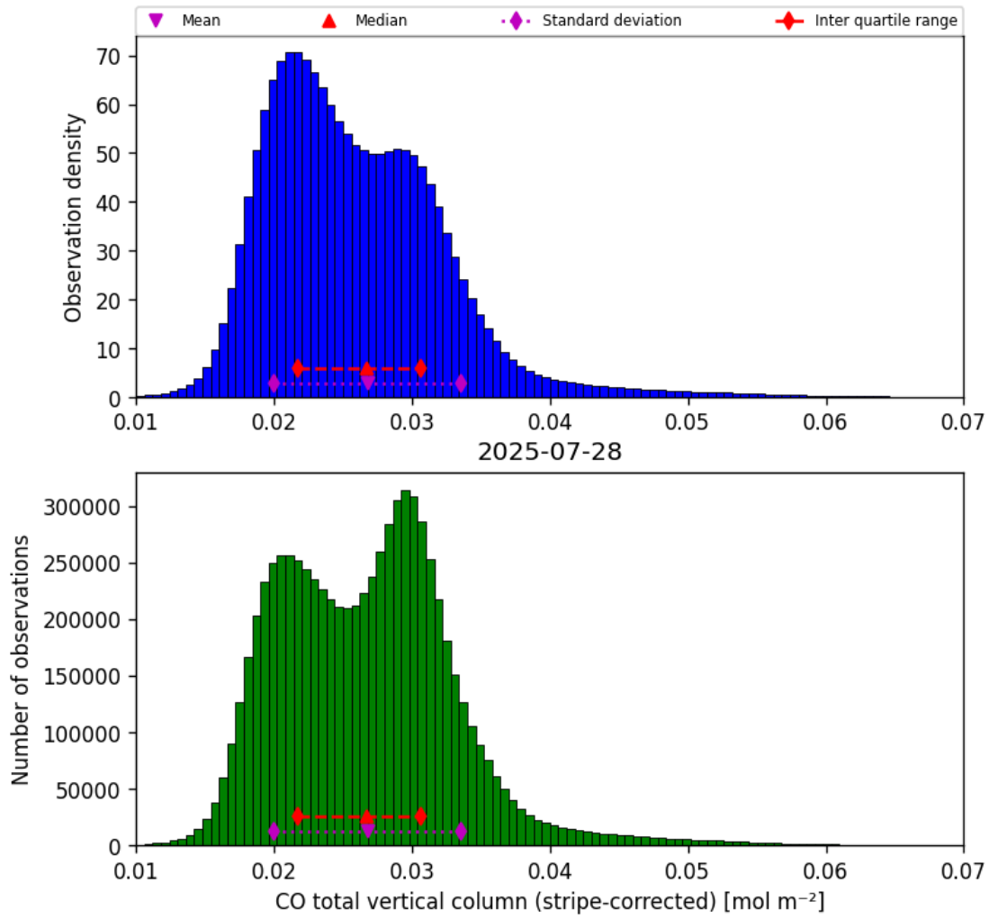
Figure 19: Histogram of “CO total vertical column (stripe-corrected)” for 2025-07-27 to 2025-07-29
