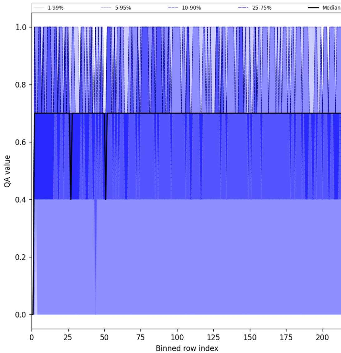
Figure 25: Along track statistics of “QA value” for 2025-07-27 to 2025-07-29
