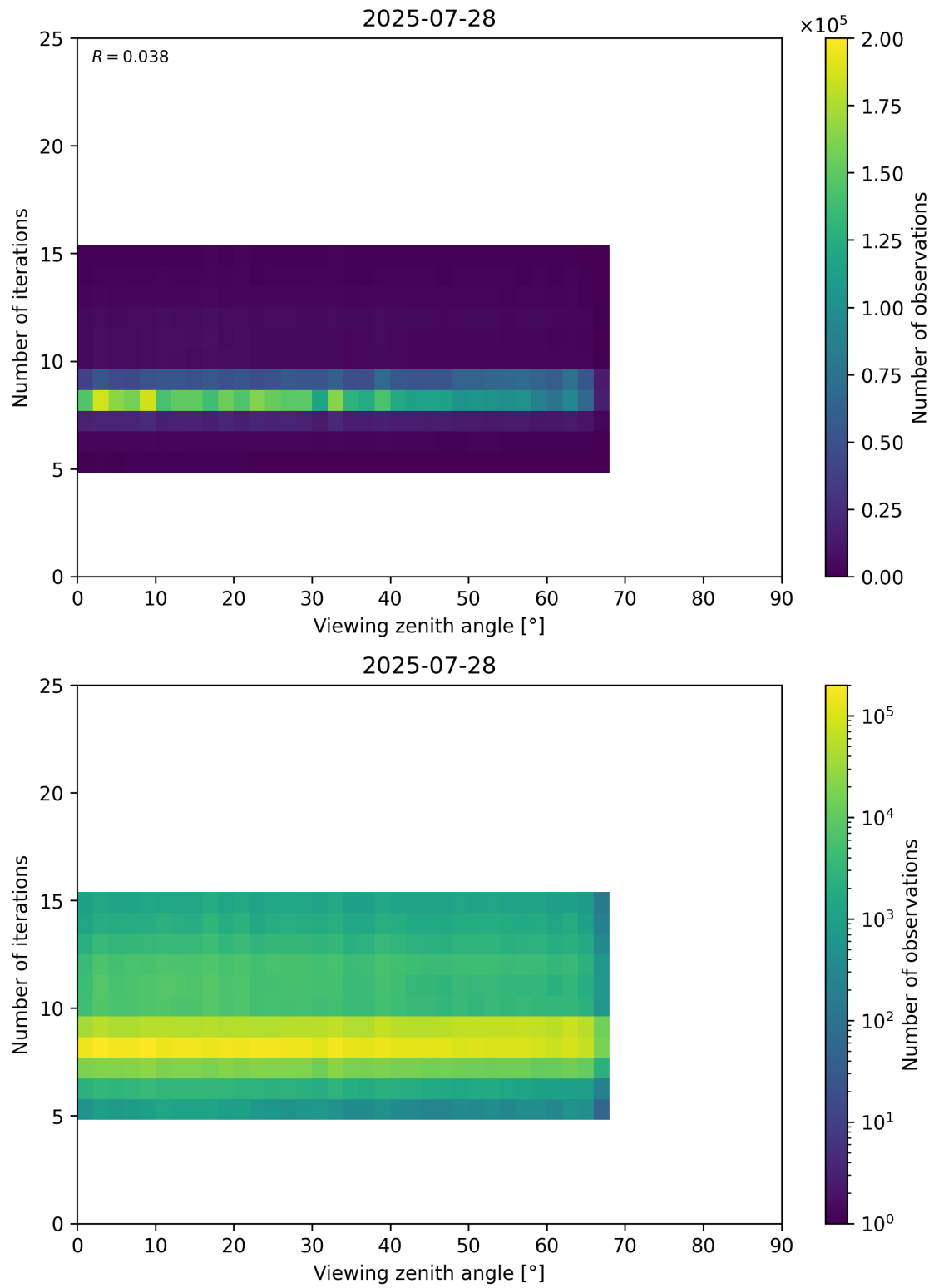
Figure 75: Scatter density plot of “Viewing zenith angle” against “Number of iterations” for 2025-07-27 to 2025-07-29.
