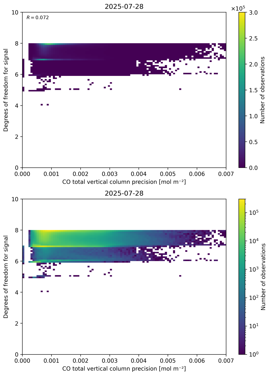
Figure 45: Scatter density plot of “CO total vertical column precision” against “Degrees of freedom for signal” for 2025-07-27 to 2025-07-29.
