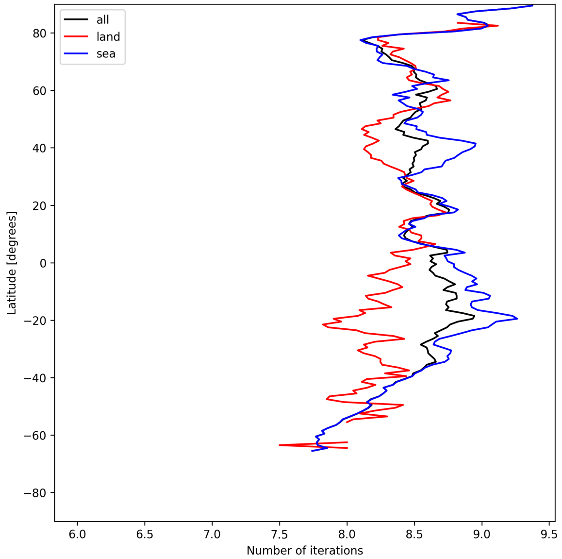
Figure 16: Zonal average of “Number of iterations” for 2025-07-27 to 2025-07-29.
