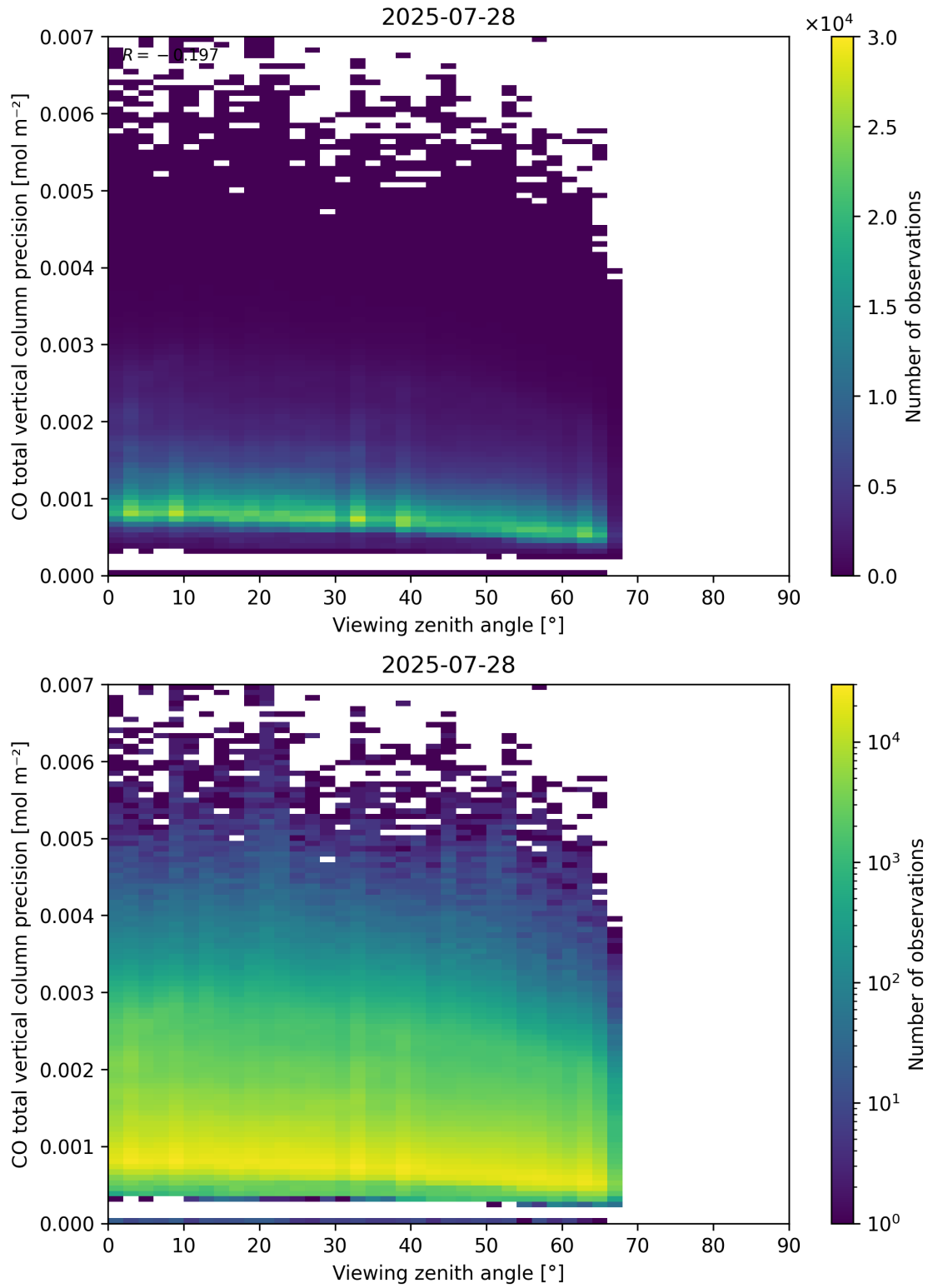
Figure 71: Scatter density plot of “Viewing zenith angle” against “CO total vertical column precision” for 2025-07-27 to 2025-07-29.
