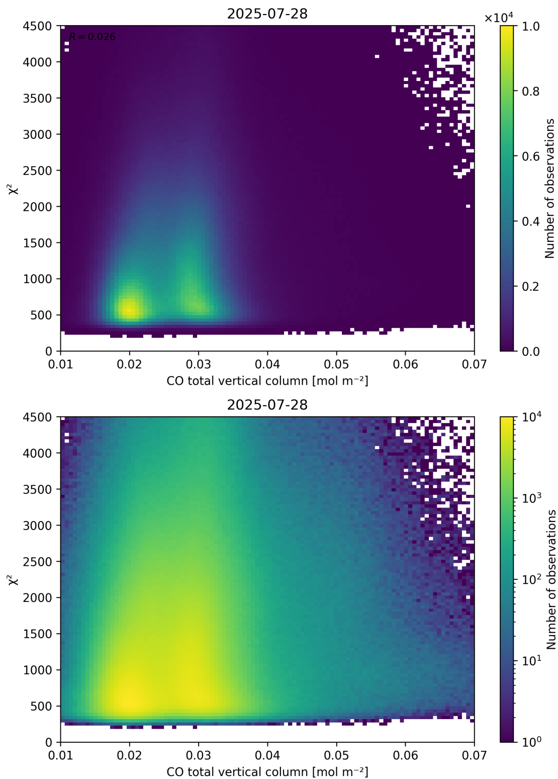
Figure 35: Scatter density plot of “CO total vertical column” against “ \chi^2 ” for 2025-07-27 to 2025-07-29.
