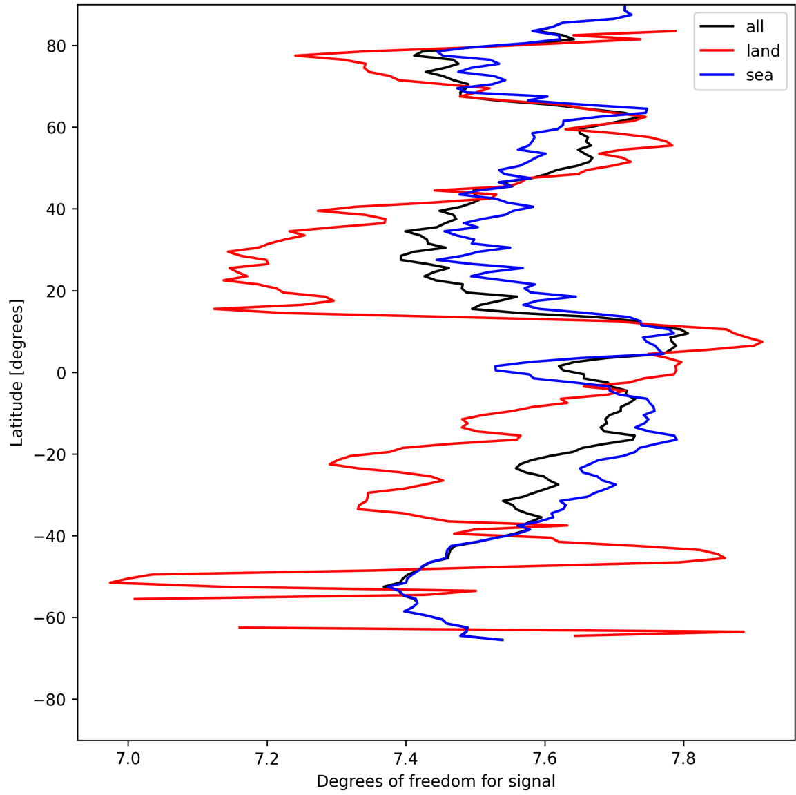
Figure 15: Zonal average of “Degrees of freedom for signal” for 2025-07-27 to 2025-07-29.
