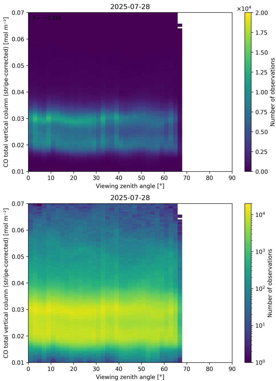
Figure 70: Scatter density plot of “Viewing zenith angle” against “CO total vertical column (stripe-corrected)” for 2025-07-27 to 2025-07-29.
