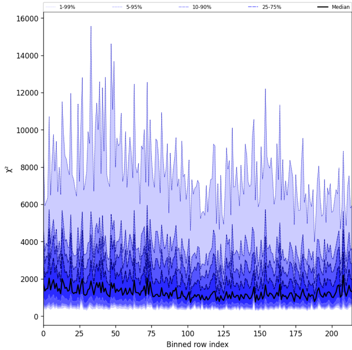
Figure 30: Along track statistics of “ \chi^2 ” for 2025-07-27 to 2025-07-29
