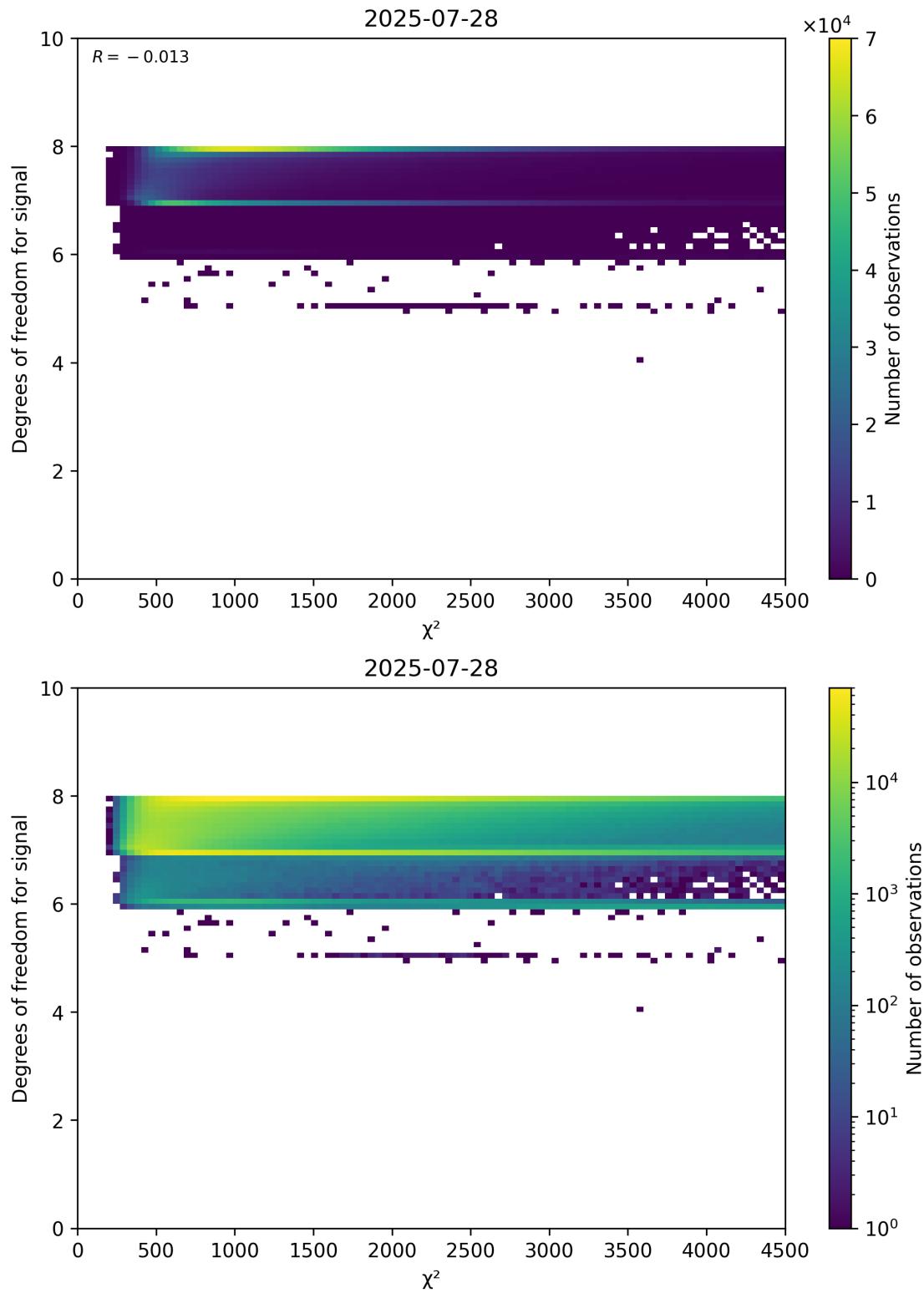
Figure 48: Scatter density plot of “ \chi^2 ” against “Degrees of freedom for signal” for 2025-07-27 to 2025-07-29.
