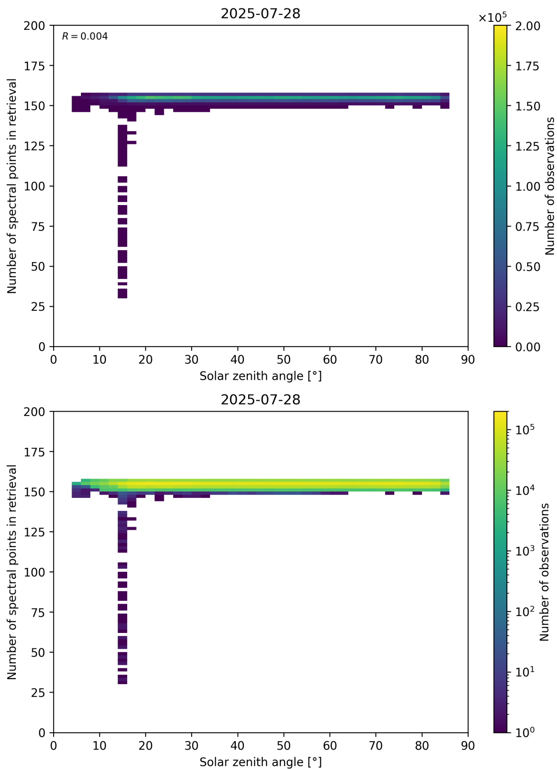
Figure 68: Scatter density plot of “Solar zenith angle” against “Number of spectral points in retrieval” for 2025-07-27 to 2025-07-29.
