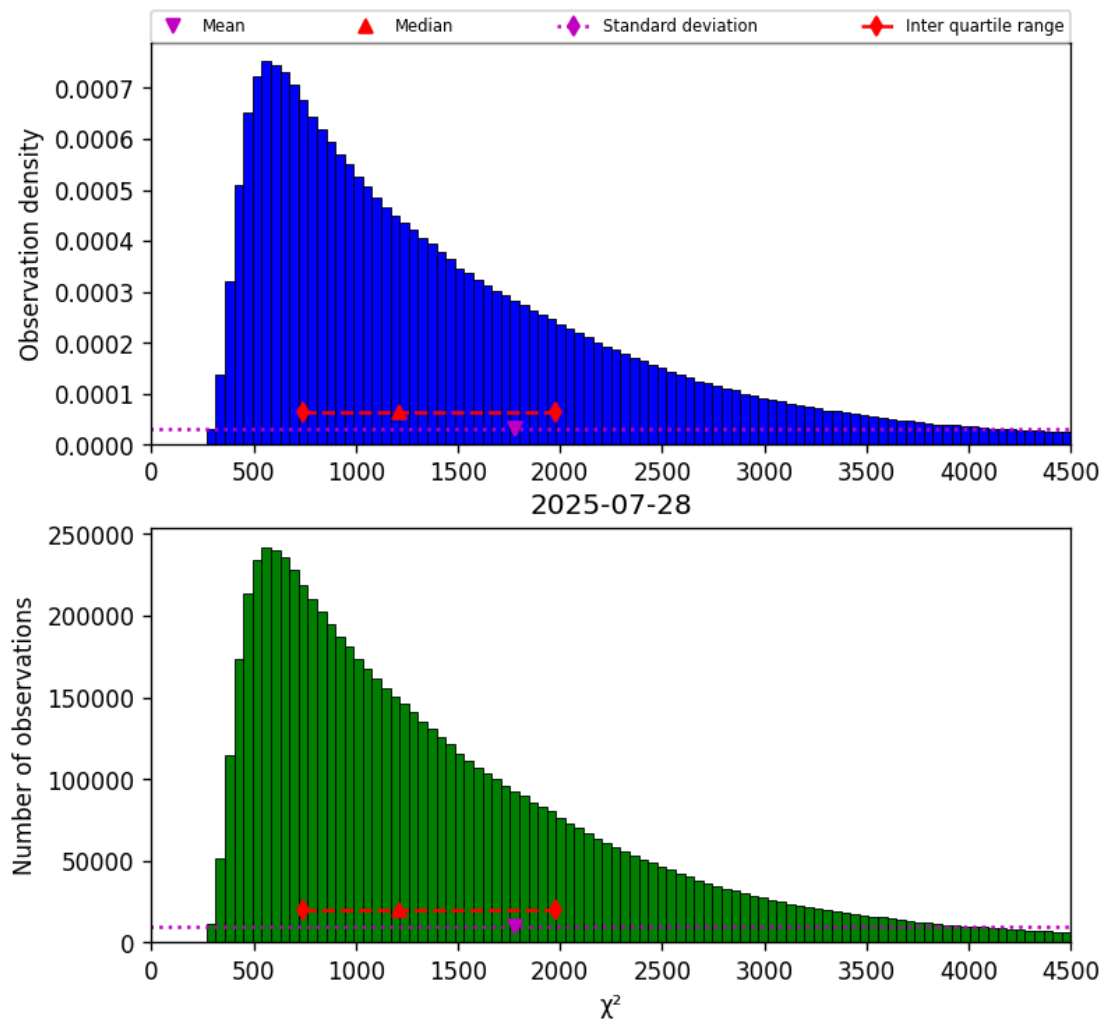
Figure 22: Histogram of “ \chi^2 ” for 2025-07-27 to 2025-07-29
