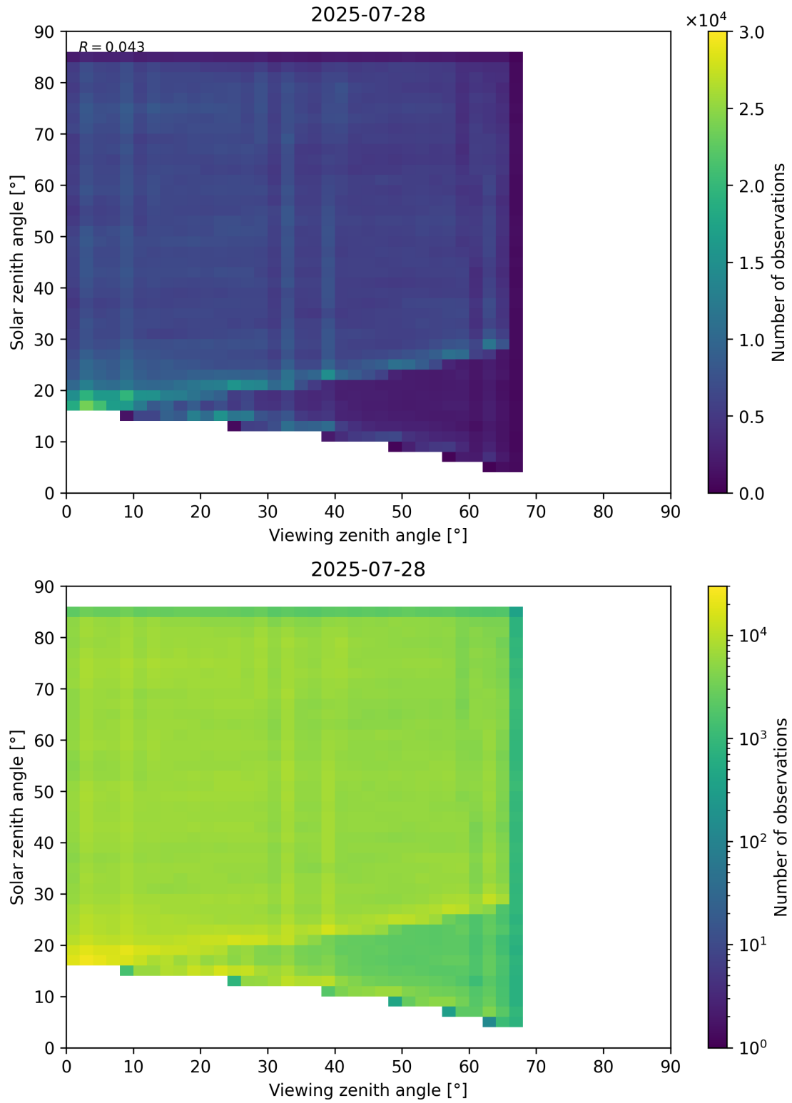
Figure 77: Scatter density plot of “Viewing zenith angle” against “Solar zenith angle” for 2025-07-27 to 2025-07-29.
