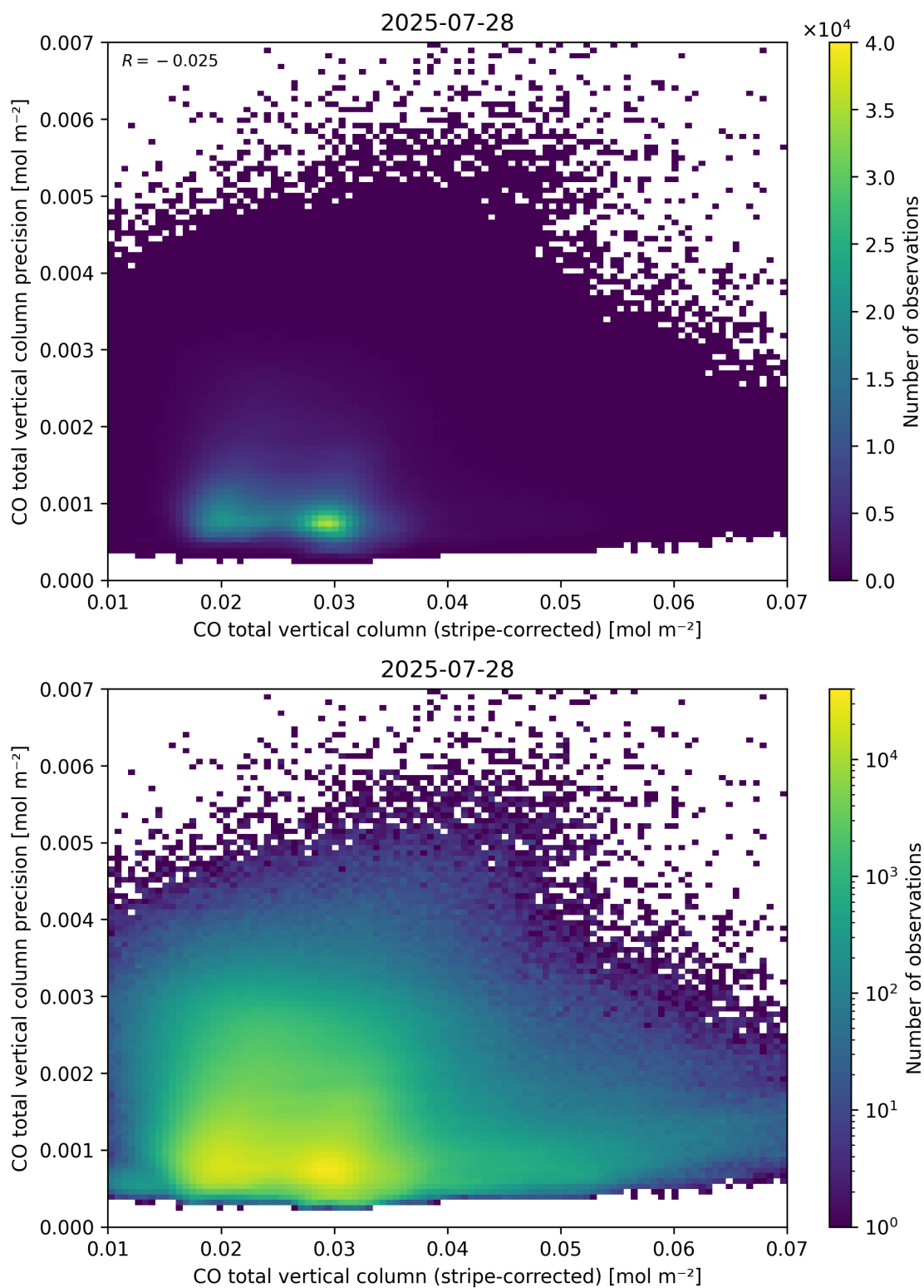
Figure 36: Scatter density plot of “CO total vertical column (stripe-corrected)” against “CO total vertical column precision” for 2025-07-27 to 2025-07-29.
