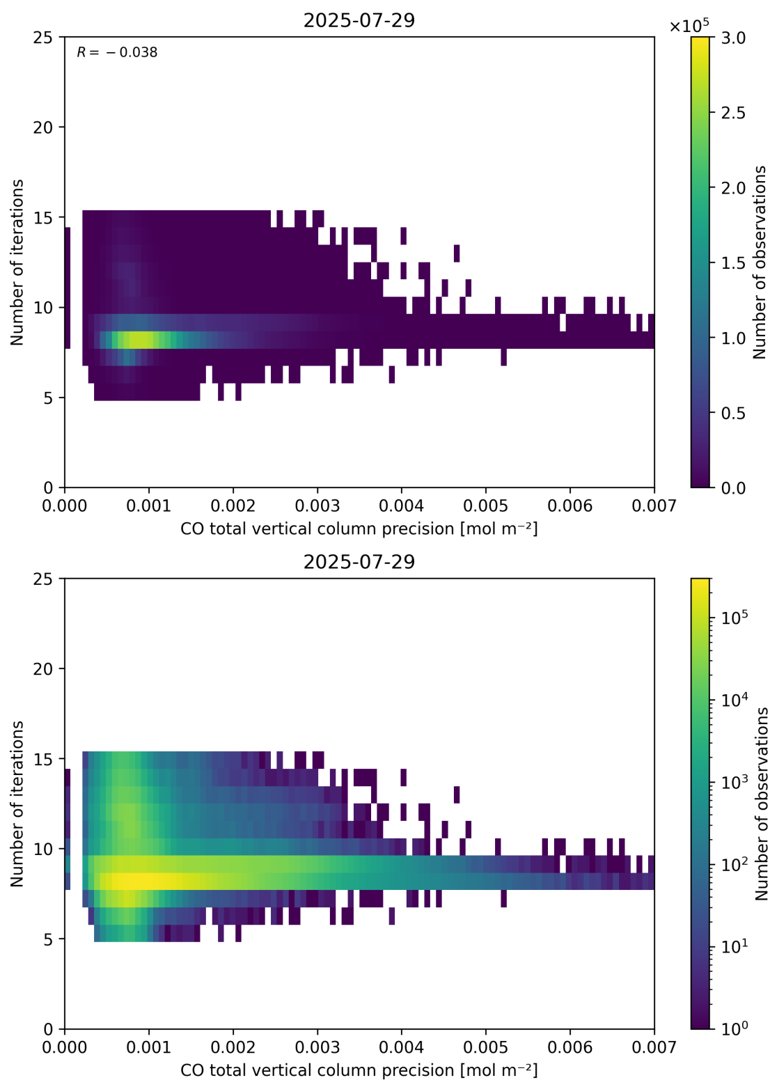
Figure 46: Scatter density plot of “CO total vertical column precision” against “Number of iterations” for 2025-07-29 to 2025-07-30.
