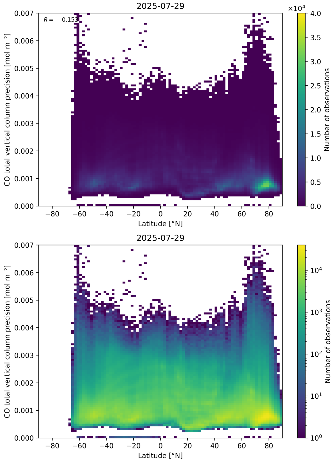
Figure 53: Scatter density plot of “Latitude” against “CO total vertical column precision” for 2025-07-29 to 2025-07-30.
