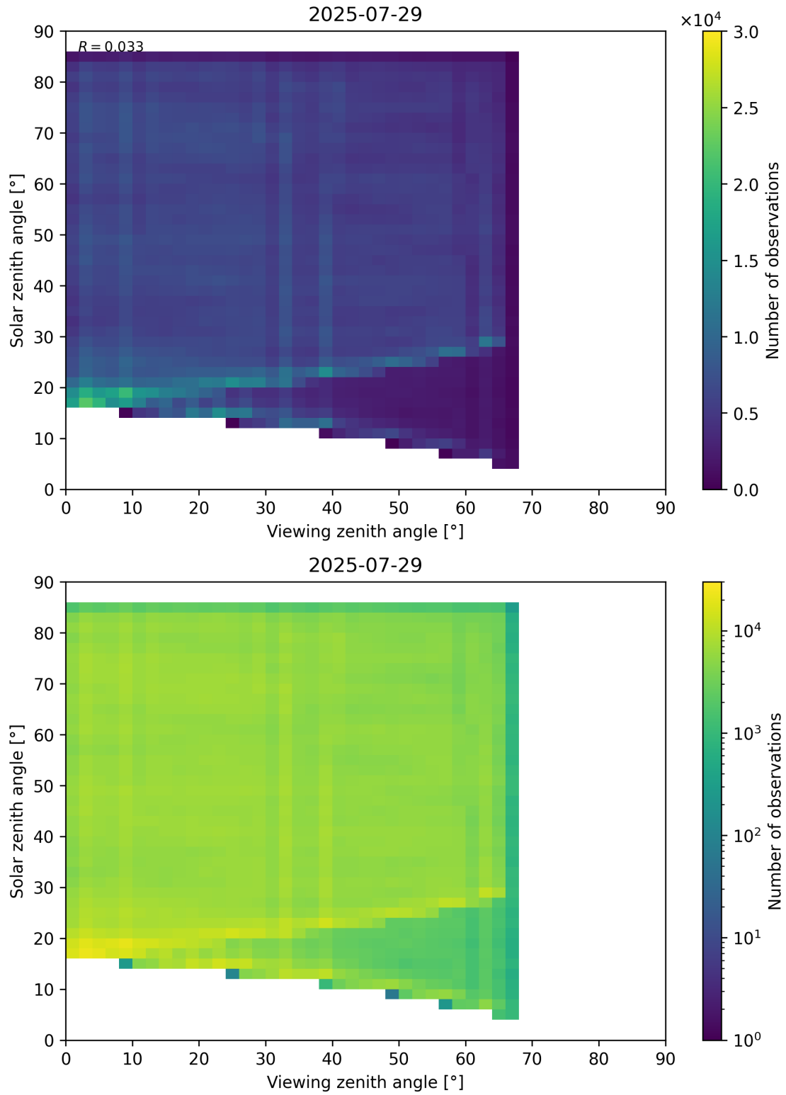
Figure 77: Scatter density plot of “Viewing zenith angle” against “Solar zenith angle” for 2025-07-29 to 2025-07-30.
