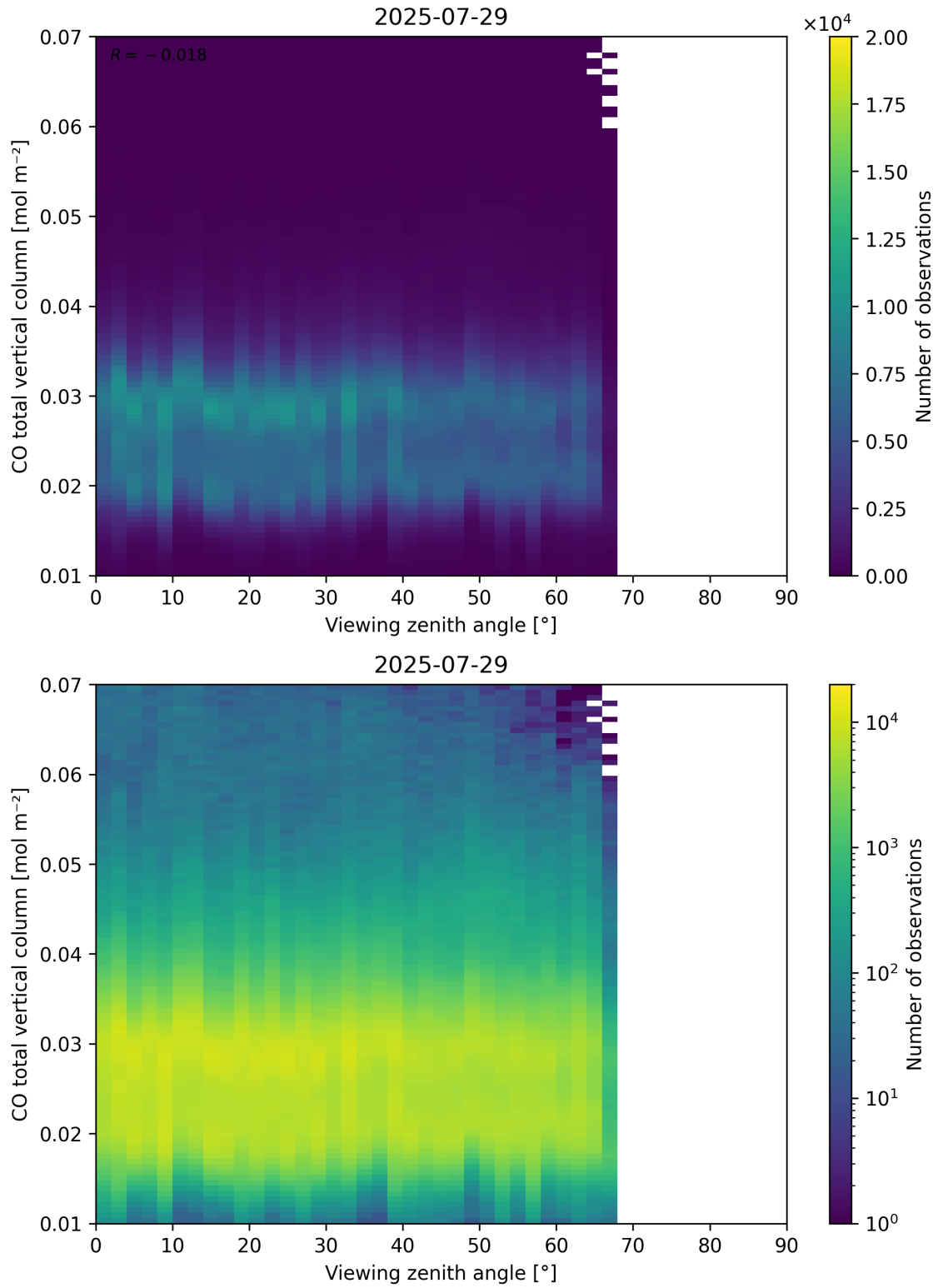
Figure 69: Scatter density plot of “Viewing zenith angle” against “CO total vertical column” for 2025-07-29 to 2025-07-30.
