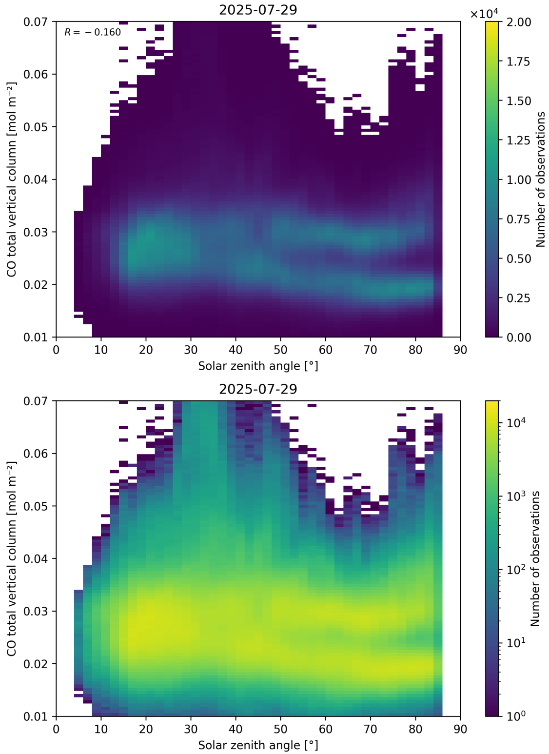
Figure 61: Scatter density plot of “Solar zenith angle” against “CO total vertical column” for 2025-07-29 to 2025-07-30.
