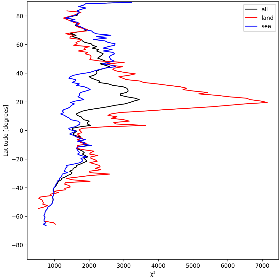
Figure 14: Zonal average of “ \chi^2 ” for 2025-07-29 to 2025-07-30.
