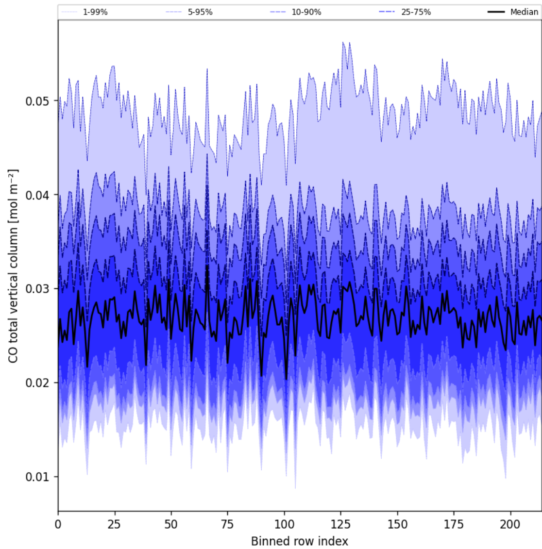
Figure 26: Along track statistics of “CO total vertical column” for 2025-07-29 to 2025-07-30
