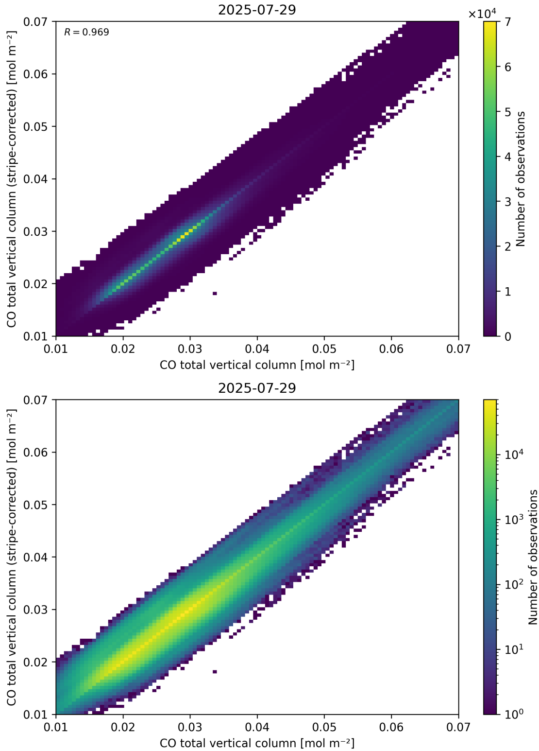
Figure 33: Scatter density plot of “CO total vertical column” against “CO total vertical column (stripe-corrected)” for 2025-07-29 to 2025-07-30.
