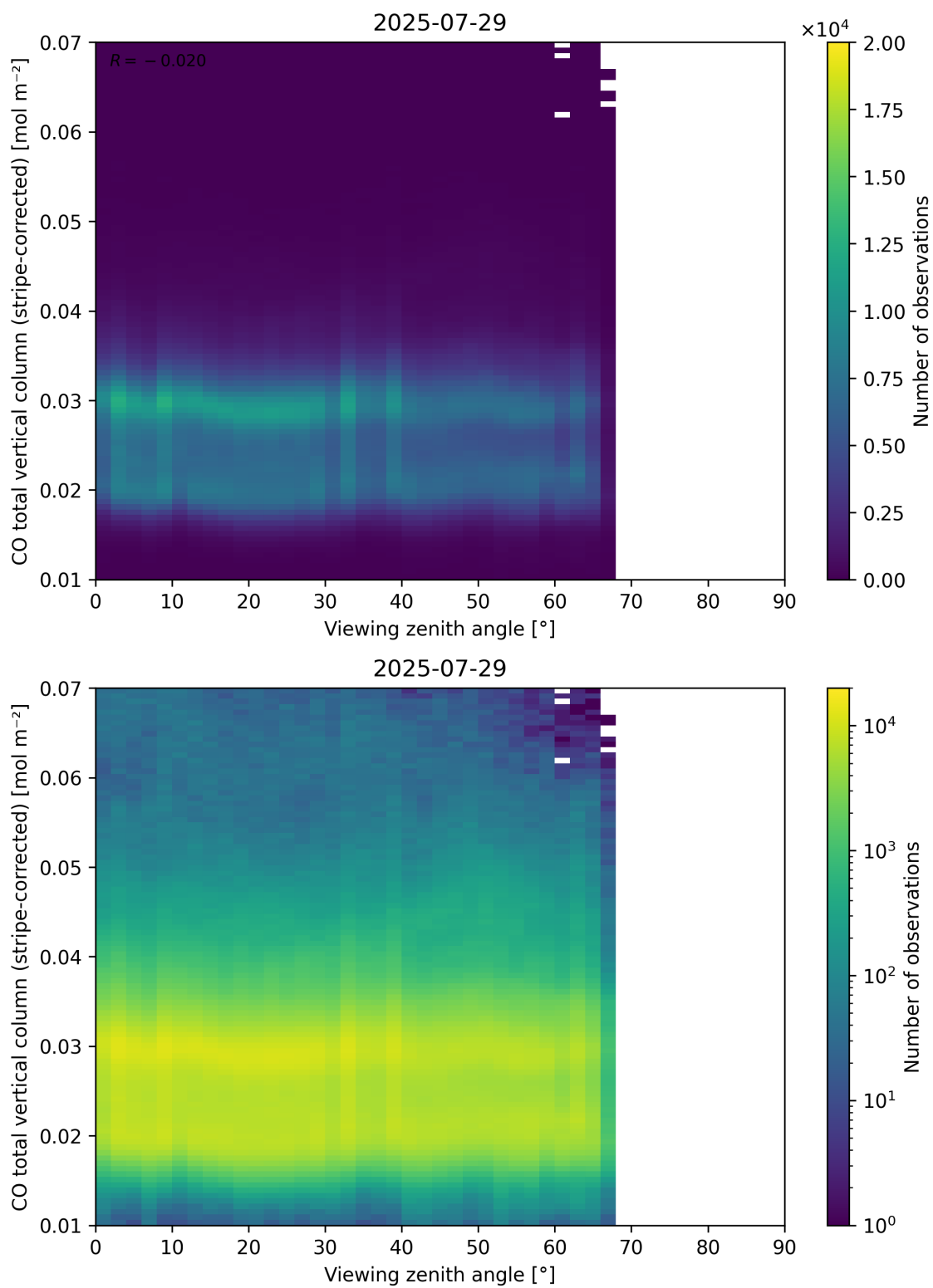
Figure 70: Scatter density plot of “Viewing zenith angle” against “CO total vertical column (stripe-corrected)” for 2025-07-29 to 2025-07-30.
