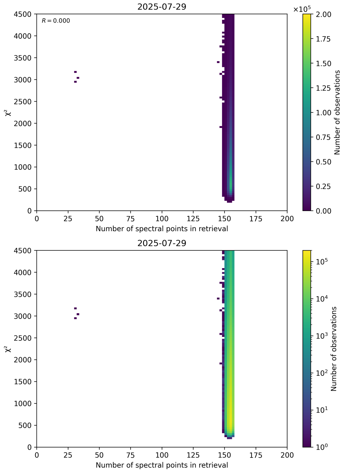
Figure 58: Scatter density plot of “Number of spectral points in retrieval” against “ \chi^2 ” for 2025-07-29 to 2025-07-30.
