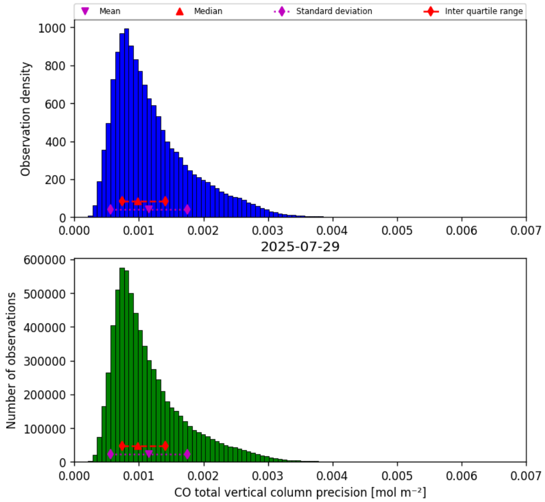
Figure 20: Histogram of “CO total vertical column precision” for 2025-07-29 to 2025-07-30
