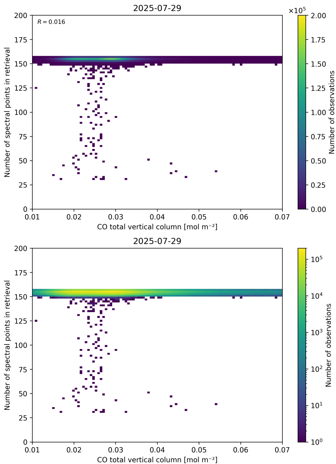
Figure 43: Scatter density plot of “CO total vertical column” against “Number of spectral points in retrieval” for 2025-07-29 to 2025-07-30.
