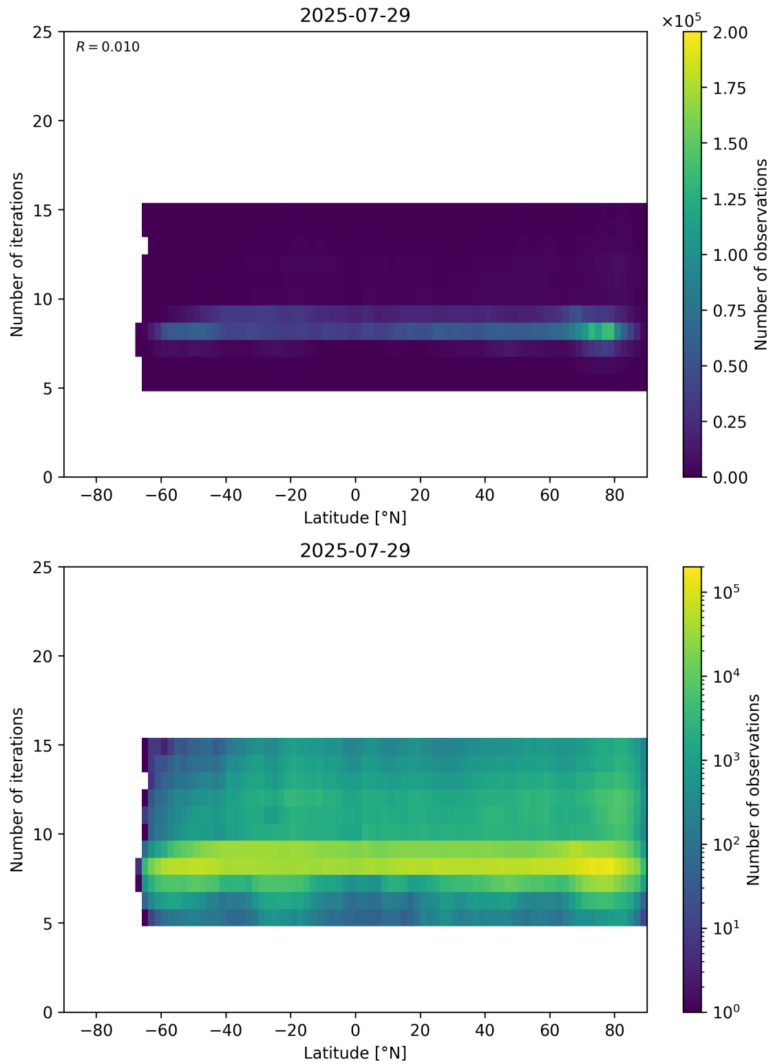
Figure 56: Scatter density plot of “Latitude” against “Number of iterations” for 2025-07-29 to 2025-07-30.
