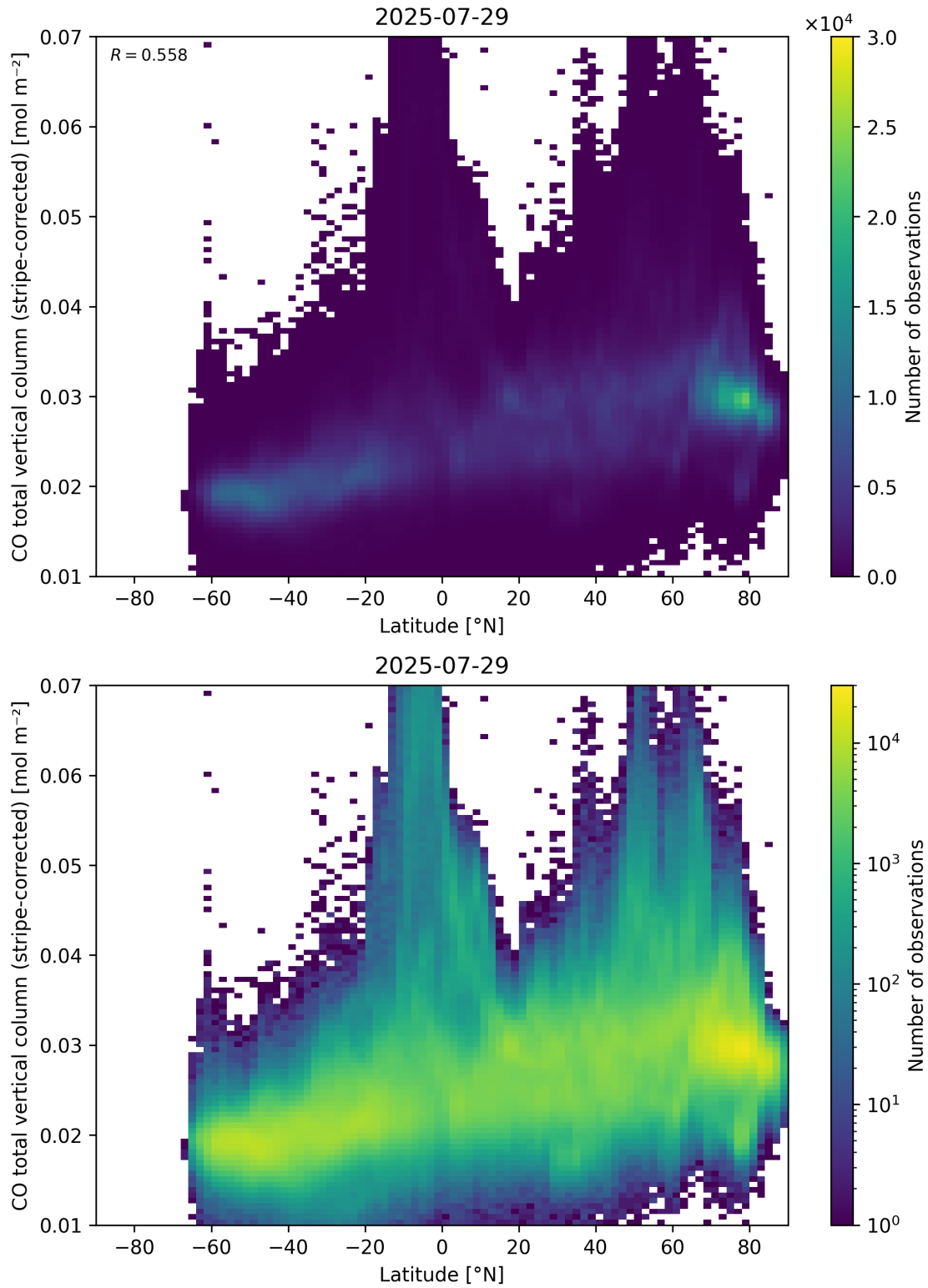
Figure 52: Scatter density plot of “Latitude” against “CO total vertical column (stripe-corrected)” for 2025-07-29 to 2025-07-30.
