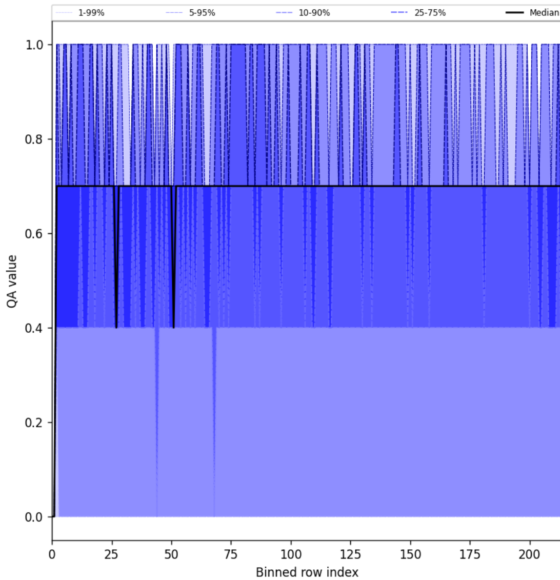
Figure 25: Along track statistics of “QA value” for 2025-07-29 to 2025-07-30
