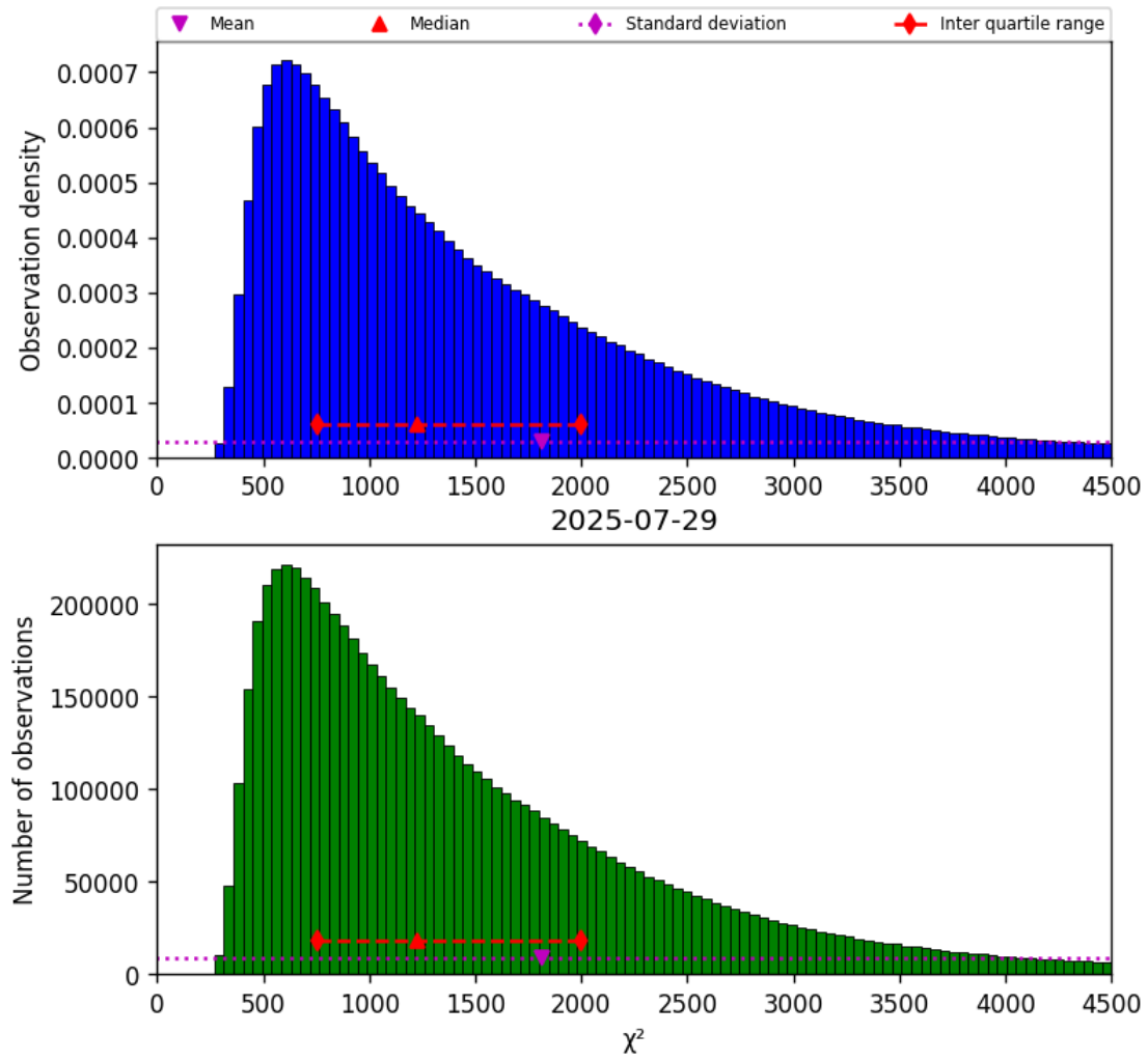
Figure 22: Histogram of “ \chi^2 ” for 2025-07-29 to 2025-07-30
