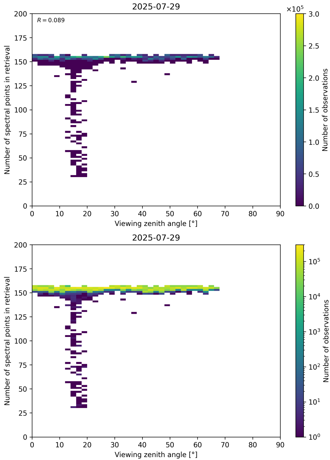
Figure 76: Scatter density plot of “Viewing zenith angle” against “Number of spectral points in retrieval” for 2025-07-29 to 2025-07-30.
