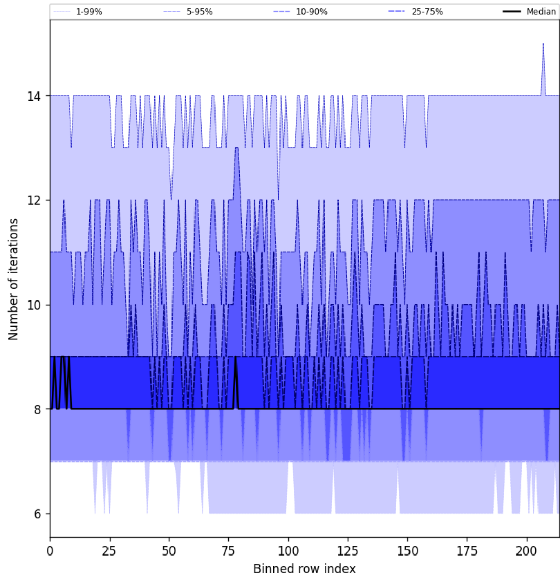
Figure 32: Along track statistics of “Number of iterations” for 2025-07-29 to 2025-07-30
