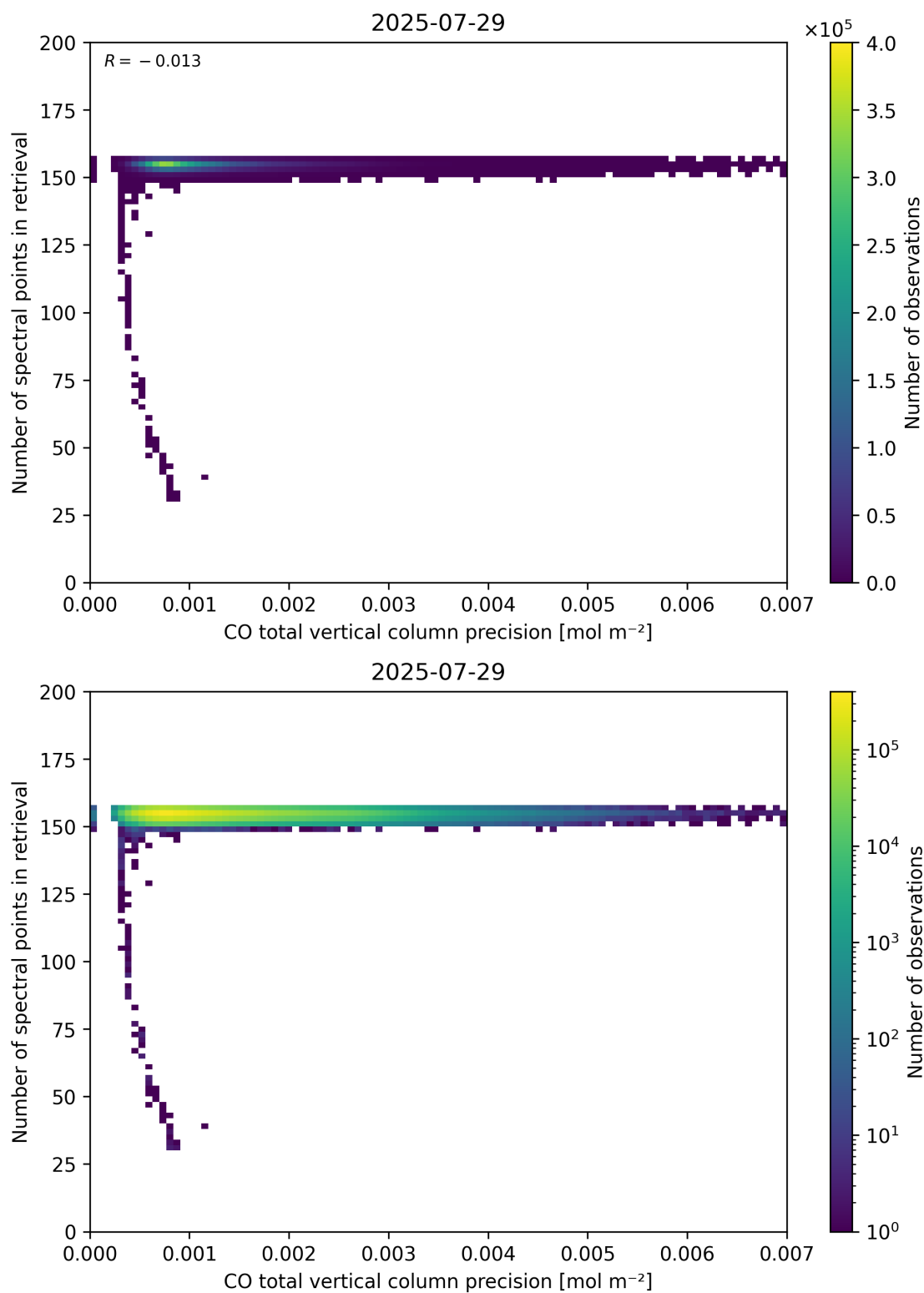
Figure 47: Scatter density plot of “CO total vertical column precision” against “Number of spectral points in retrieval” for 2025-07-29 to 2025-07-30.
