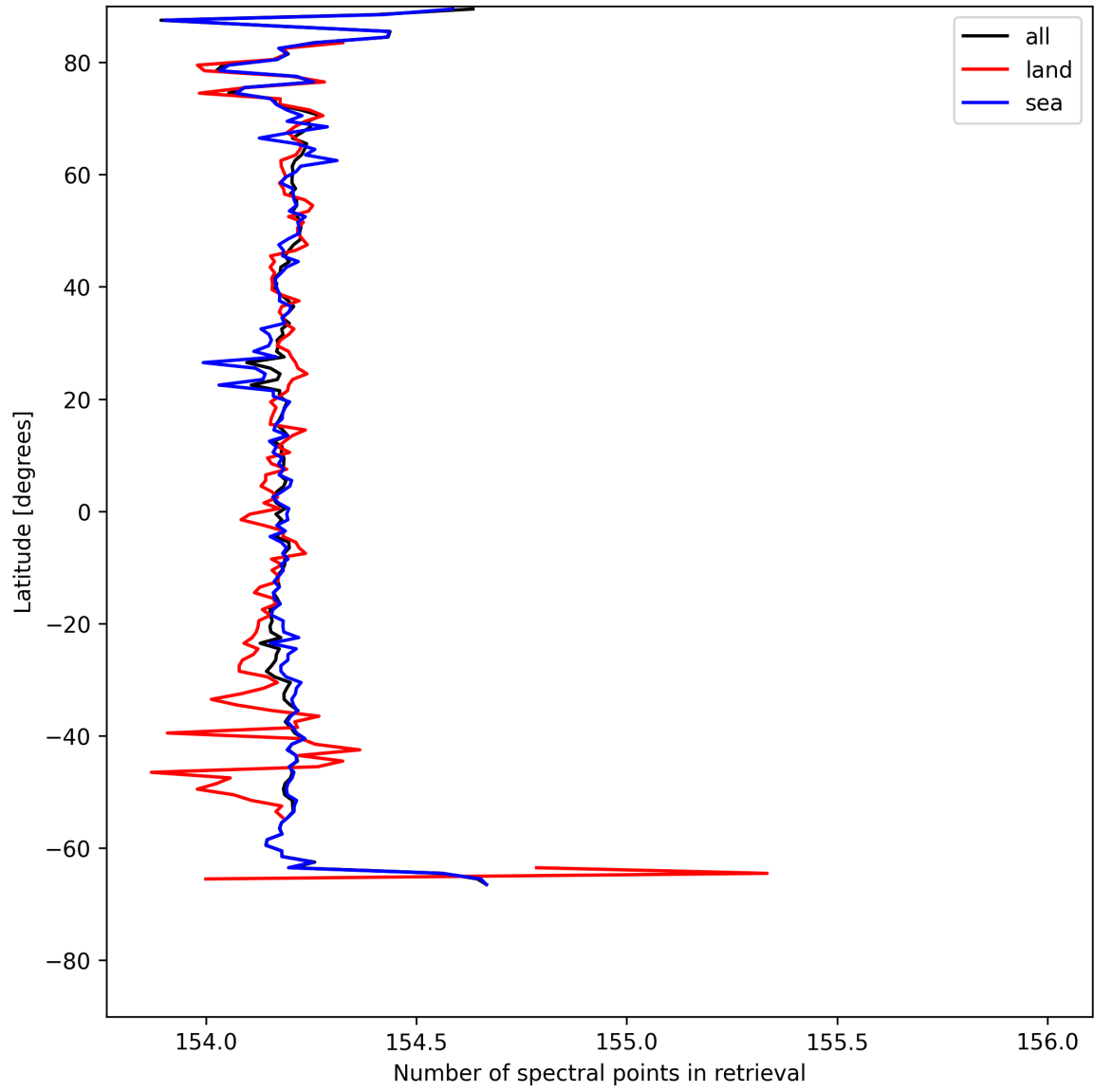
Figure 13: Zonal average of “Number of spectral points in retrieval” for 2025-07-29 to 2025-07-30.
