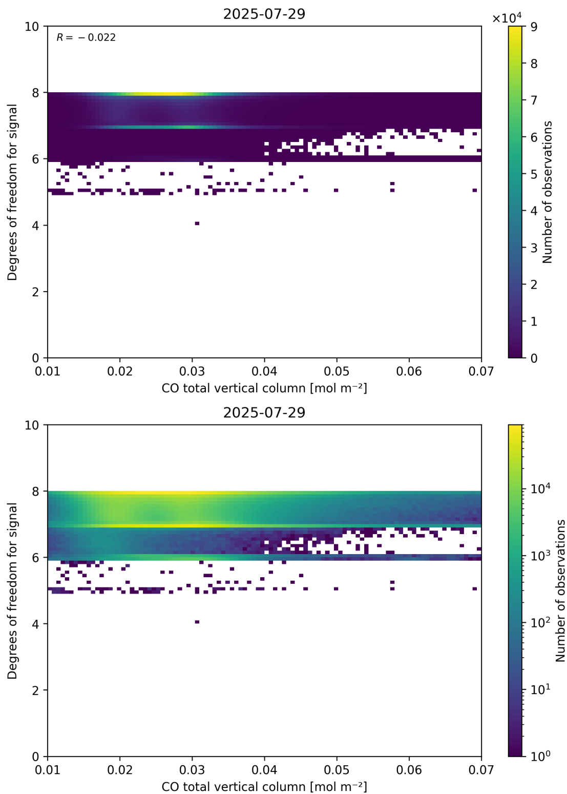
Figure 41: Scatter density plot of “CO total vertical column” against “Degrees of freedom for signal” for 2025-07-29 to 2025-07-30.
