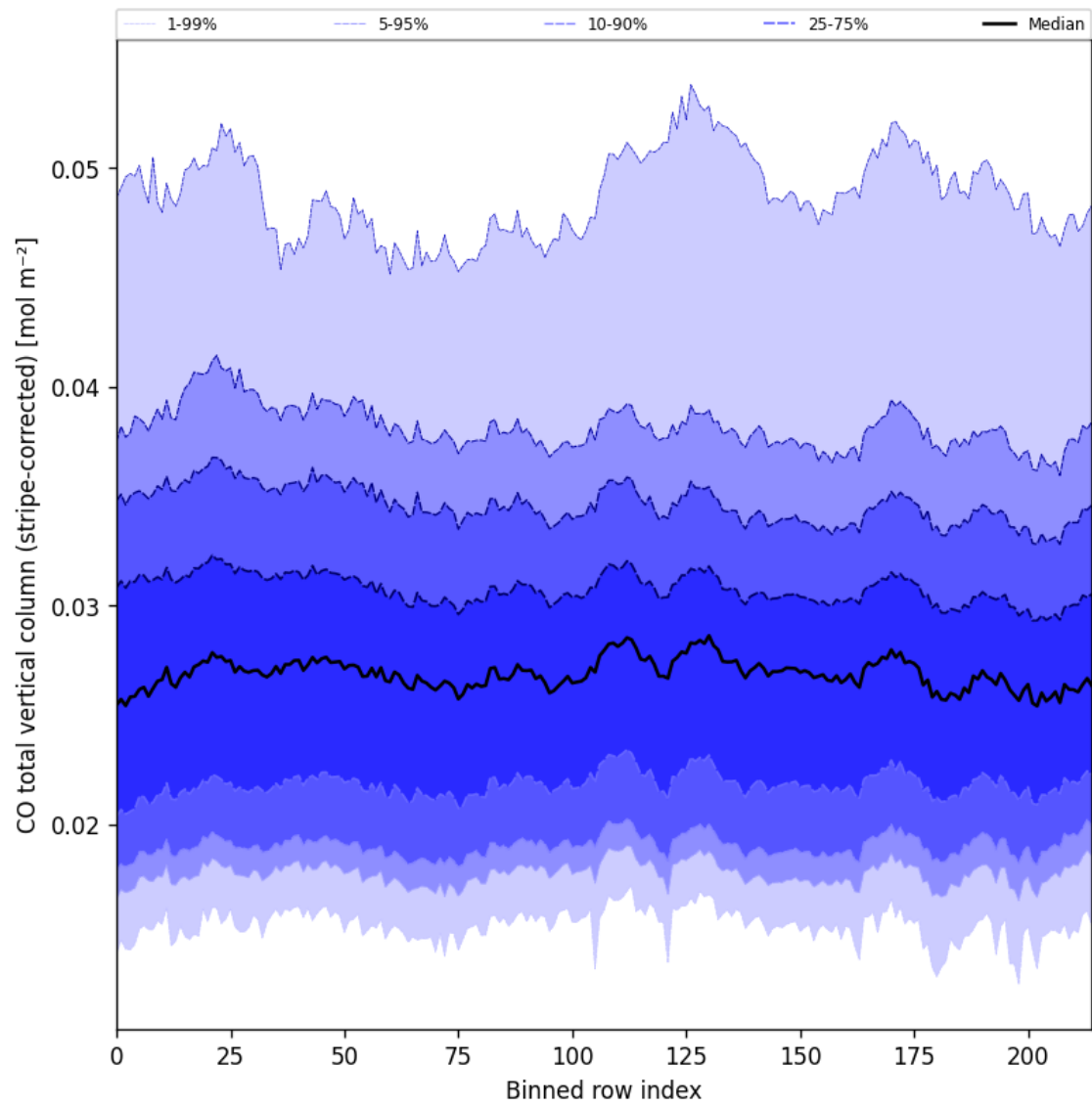
Figure 27: Along track statistics of “CO total vertical column (stripe-corrected)” for 2025-07-29 to 2025-07-30
