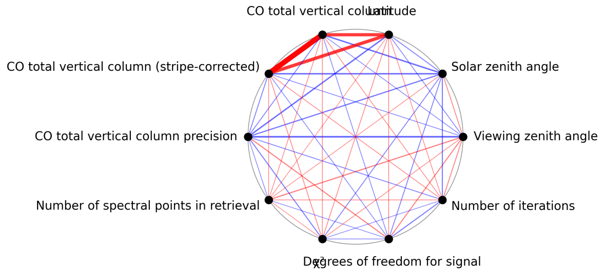
Figure 1: Map of correlation graph for 2025-07-29 to 2025-07-30.
