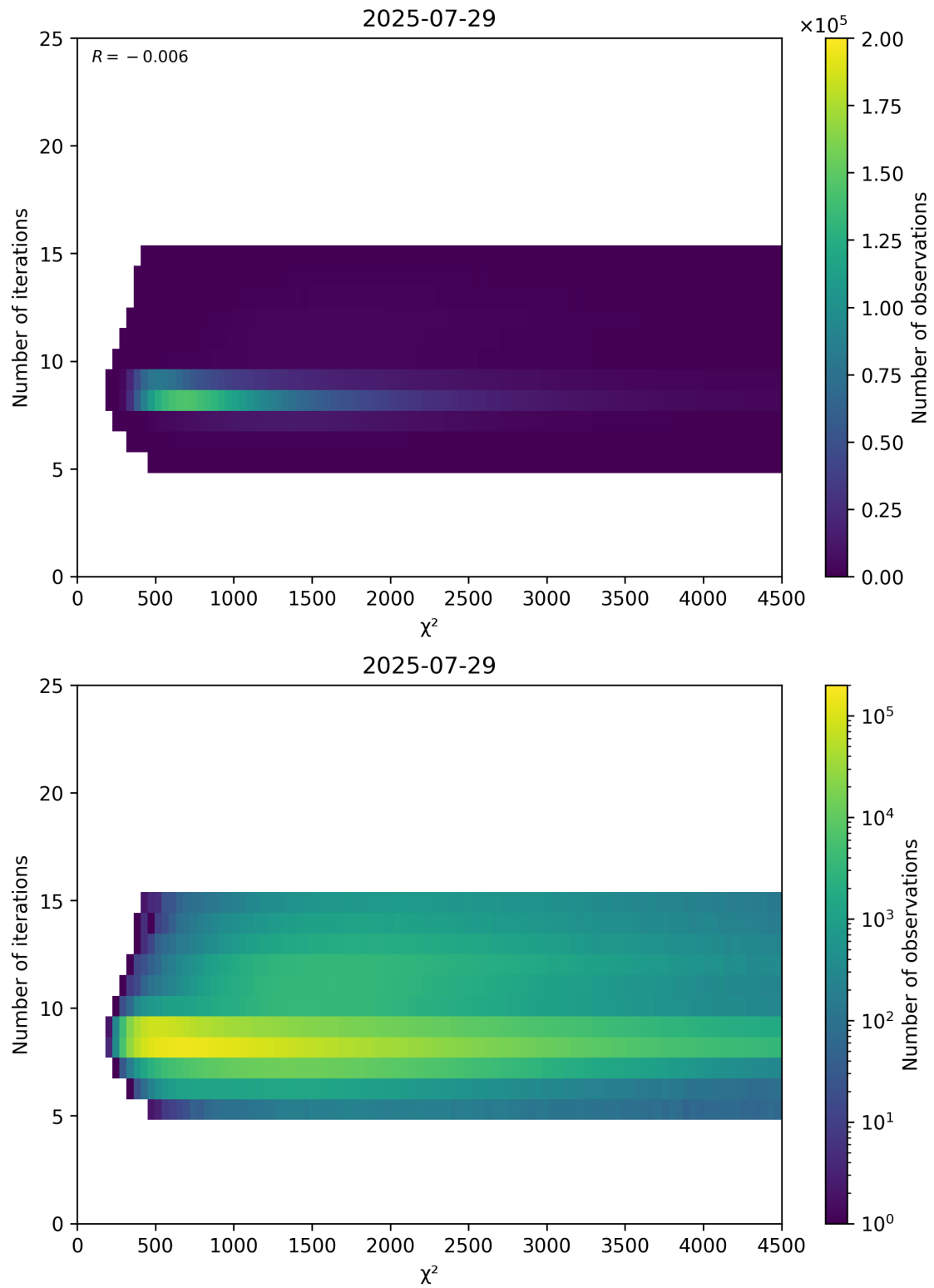
Figure 49: Scatter density plot of “ \chi^2 ” against “Number of iterations” for 2025-07-29 to 2025-07-30.
