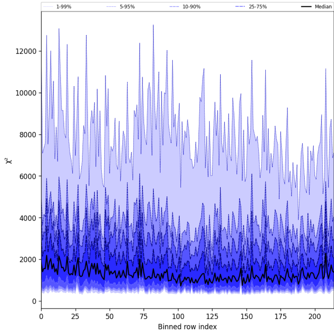
Figure 30: Along track statistics of “ \chi^2 ” for 2025-07-29 to 2025-07-30
