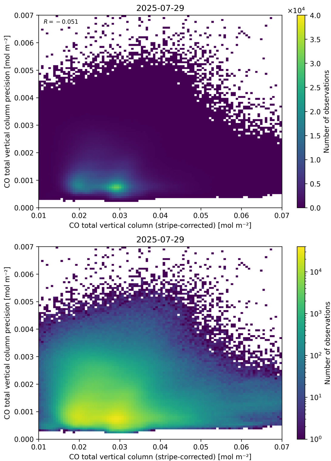
Figure 36: Scatter density plot of “CO total vertical column (stripe-corrected)” against “CO total vertical column precision” for 2025-07-29 to 2025-07-30.
