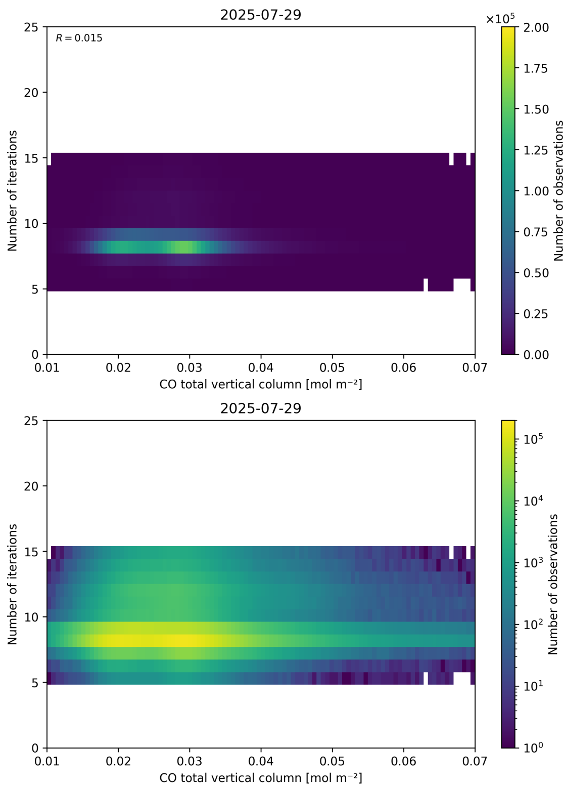
Figure 42: Scatter density plot of “CO total vertical column” against “Number of iterations” for 2025-07-29 to 2025-07-30.
