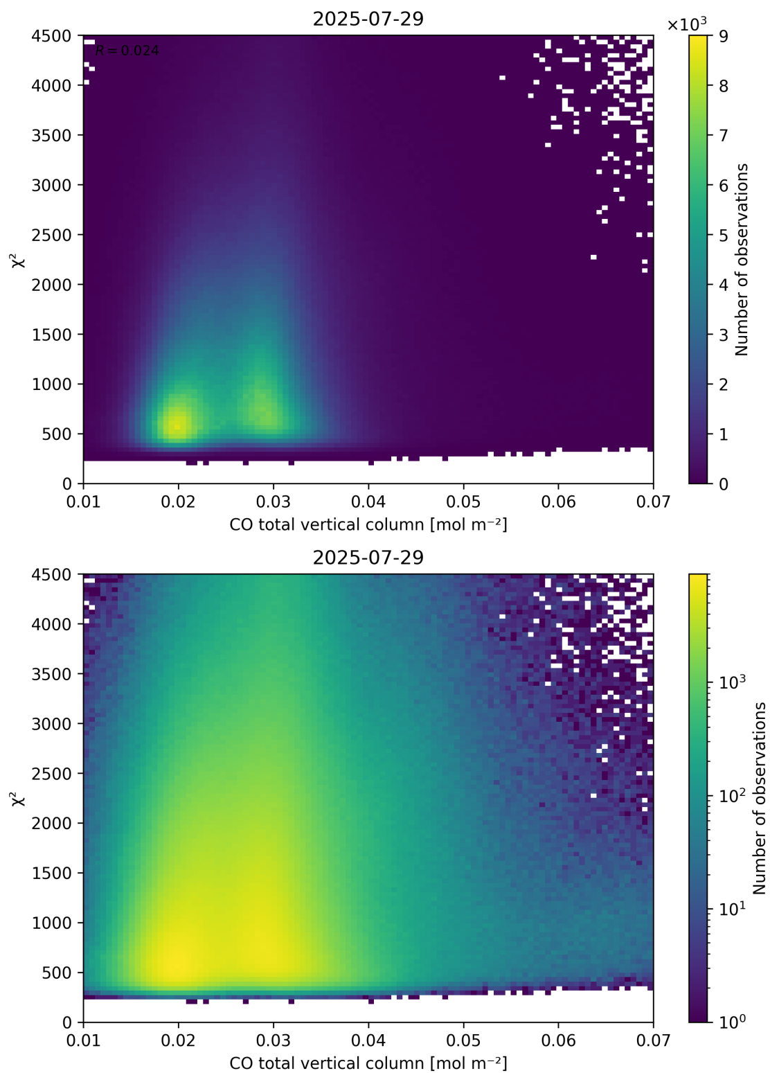
Figure 35: Scatter density plot of “CO total vertical column” against “ \chi^2 ” for 2025-07-29 to 2025-07-30.
