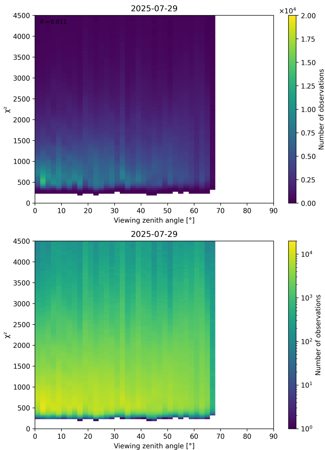
Figure 72: Scatter density plot of “Viewing zenith angle” against “ \chi^2 ” for 2025-07-29 to 2025-07-30.
