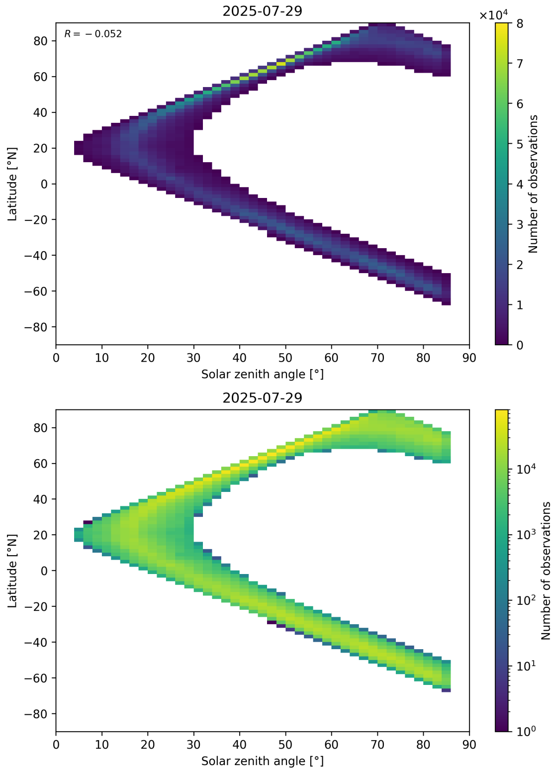
Figure 66: Scatter density plot of “Solar zenith angle” against “Latitude” for 2025-07-29 to 2025-07-30.
