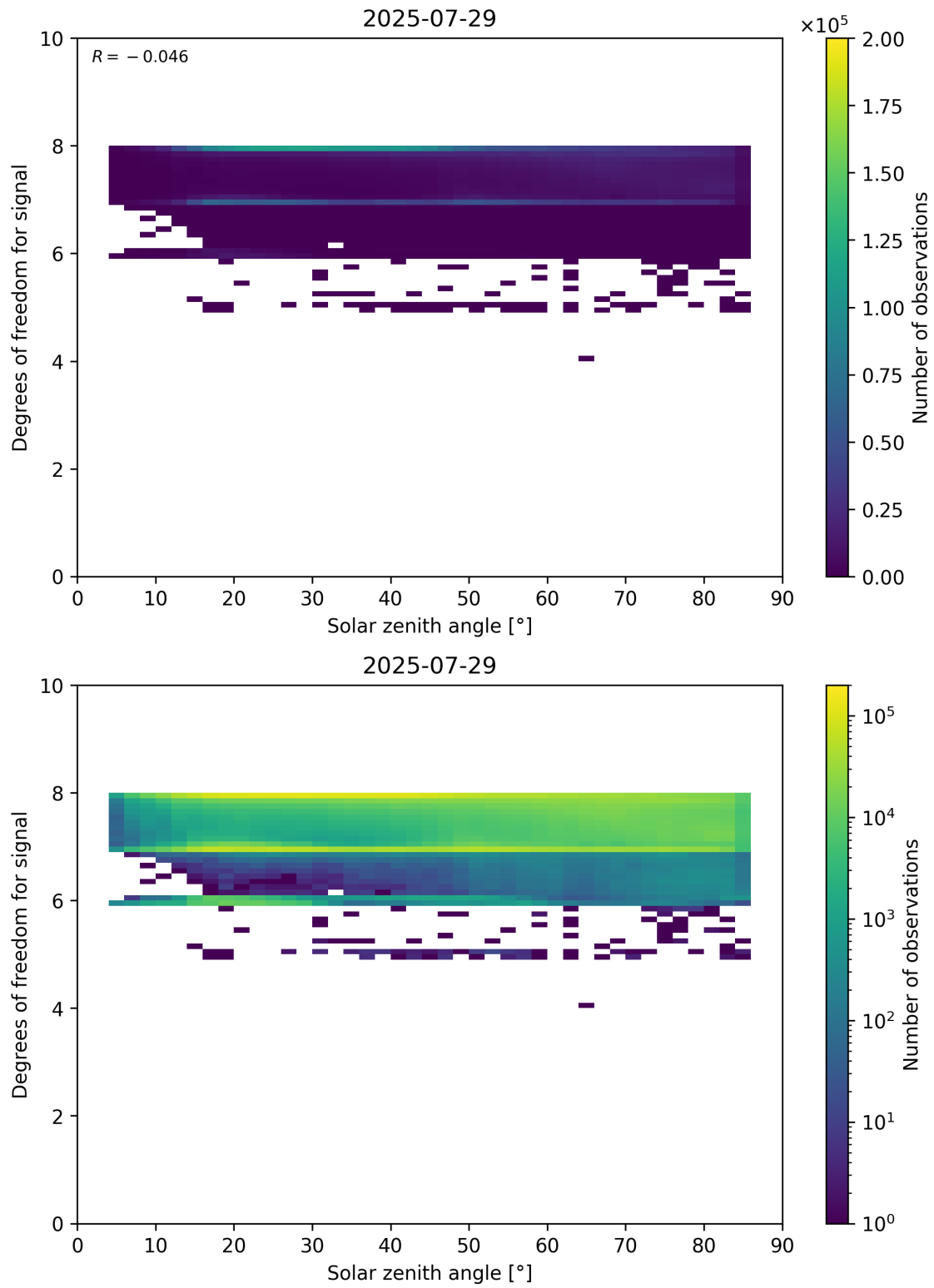
Figure 65: Scatter density plot of “Solar zenith angle” against “Degrees of freedom for signal” for 2025-07-29 to 2025-07-30.
