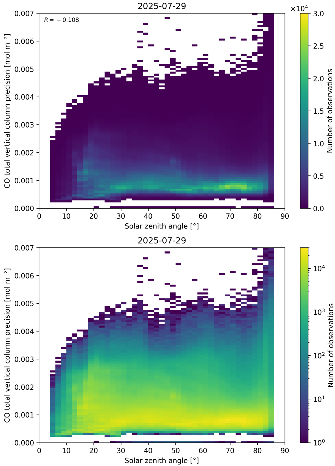
Figure 63: Scatter density plot of “Solar zenith angle” against “CO total vertical column precision” for 2025-07-29 to 2025-07-30.
