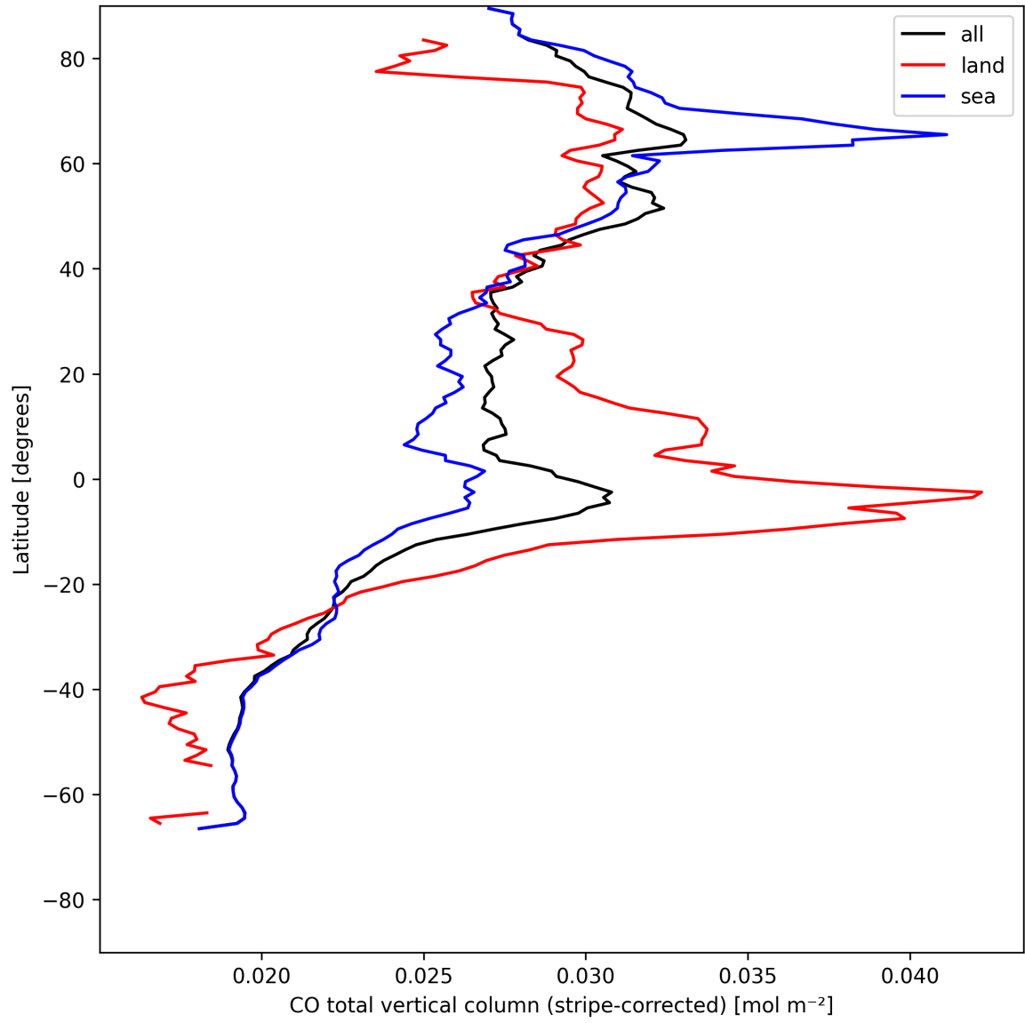
Figure 11: Zonal average of “CO total vertical column (stripe-corrected)” for 2025-07-29 to 2025-07-30.
