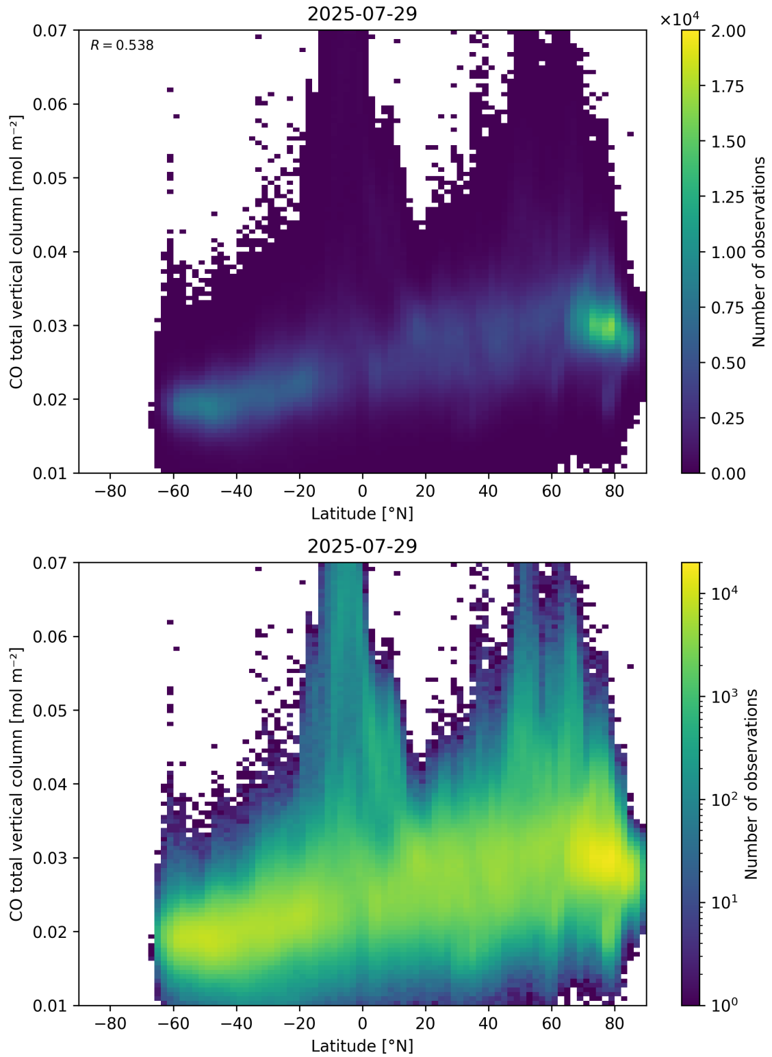
Figure 51: Scatter density plot of “Latitude” against “CO total vertical column” for 2025-07-29 to 2025-07-30.
