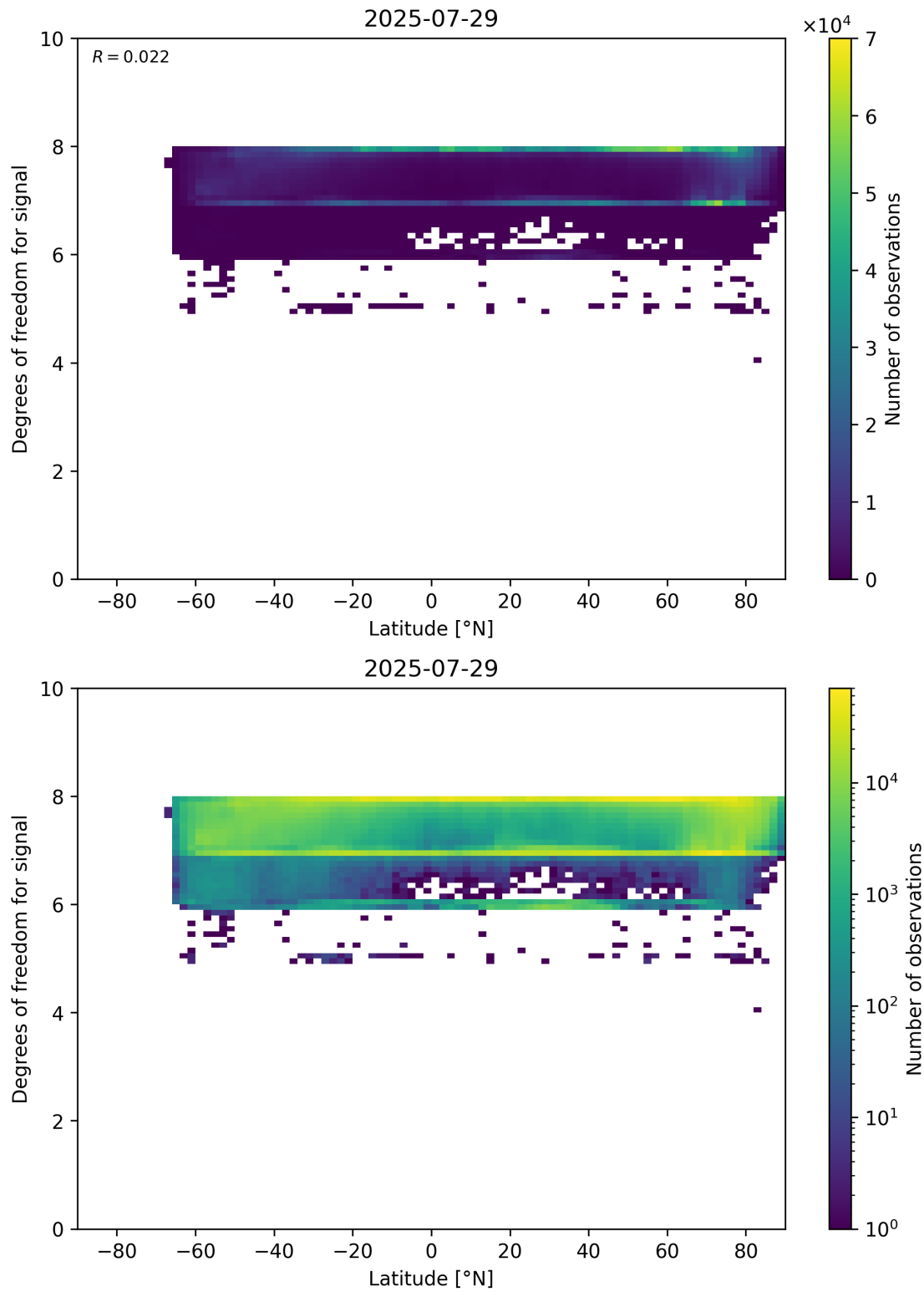
Figure 55: Scatter density plot of “Latitude” against “Degrees of freedom for signal” for 2025-07-29 to 2025-07-30.
