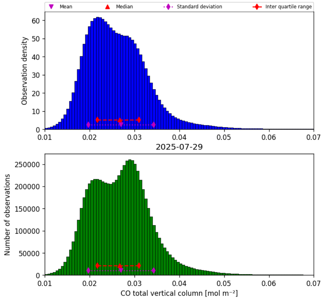
Figure 18: Histogram of “CO total vertical column” for 2025-07-29 to 2025-07-30
