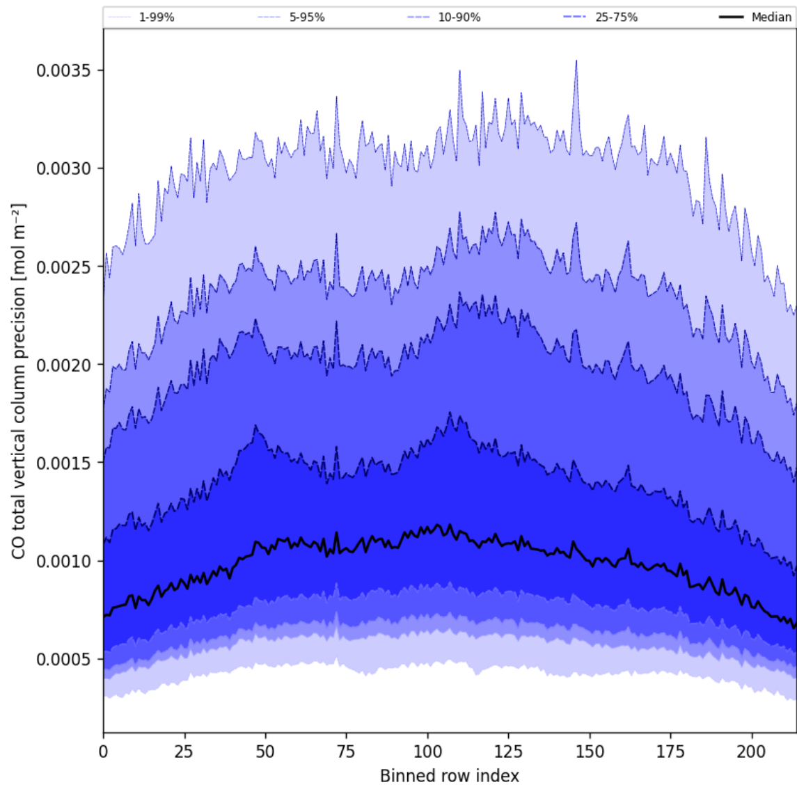
Figure 28: Along track statistics of “CO total vertical column precision” for 2025-07-29 to 2025-07-30
