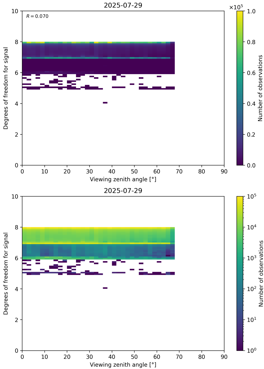
Figure 73: Scatter density plot of “Viewing zenith angle” against “Degrees of freedom for signal” for 2025-07-29 to 2025-07-30.
