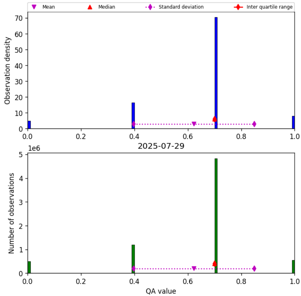
Figure 17: Histogram of “QA value” for 2025-07-29 to 2025-07-30
