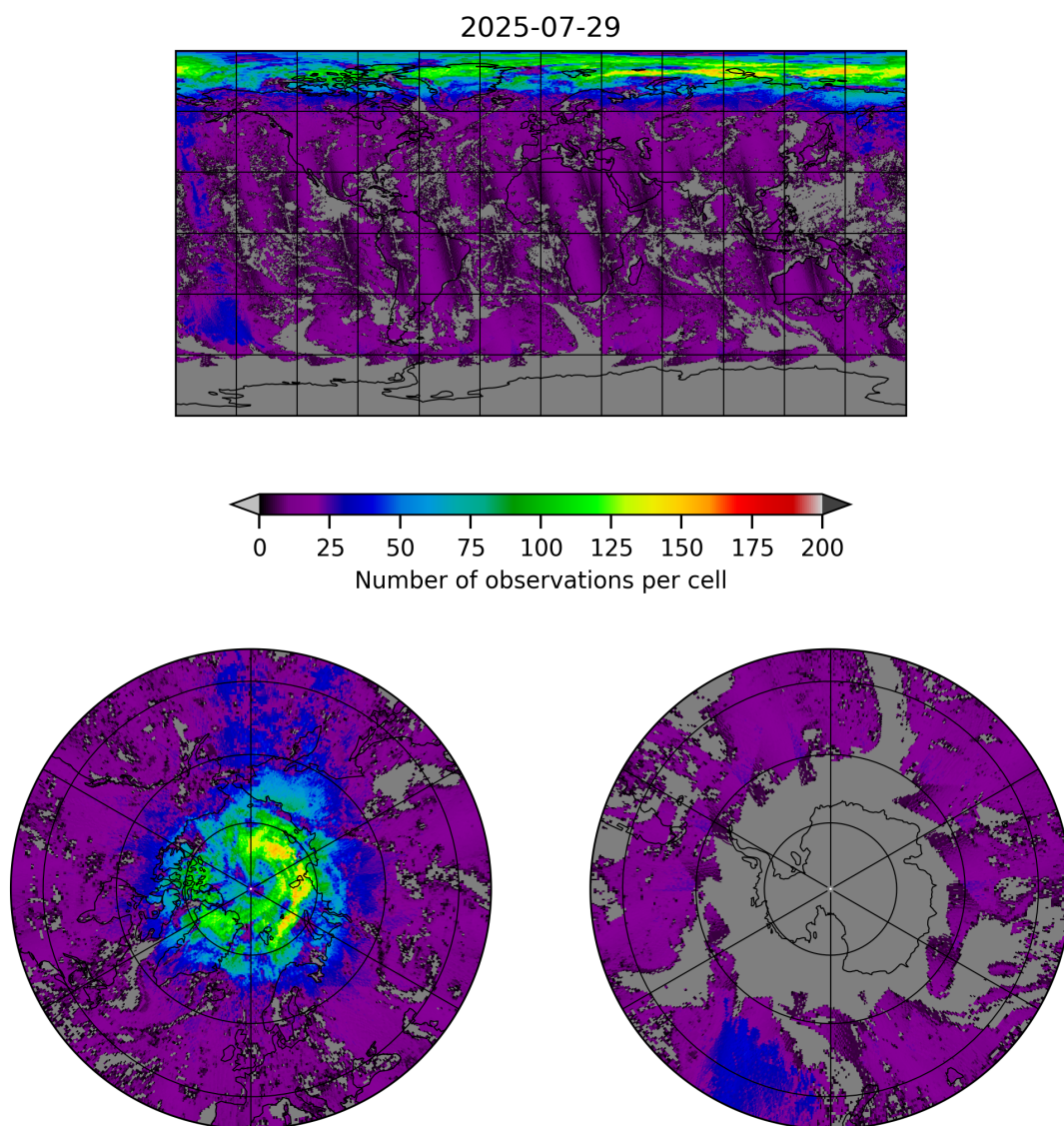
Figure 8: Map of the number of observations for 2025-07-29 to 2025-07-30
