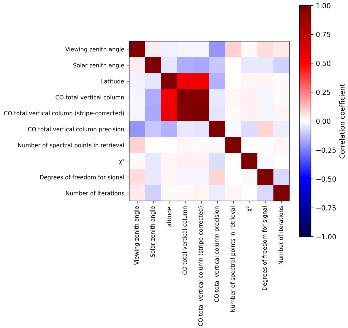
Figure 2: Map of correlation matrix for 2025-07-29 to 2025-07-30.
