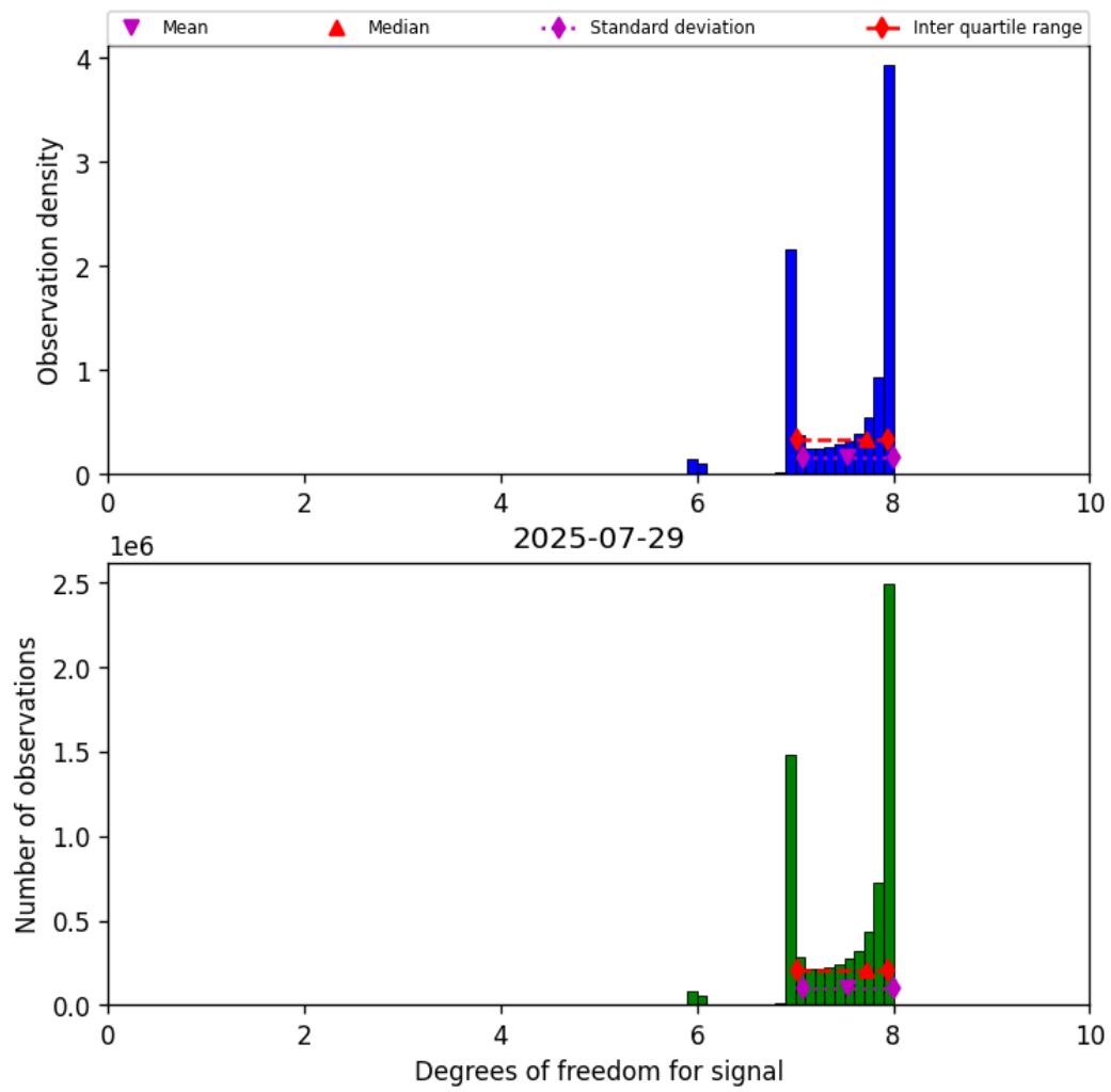
Figure 23: Histogram of “Degrees of freedom for signal” for 2025-07-29 to 2025-07-30
