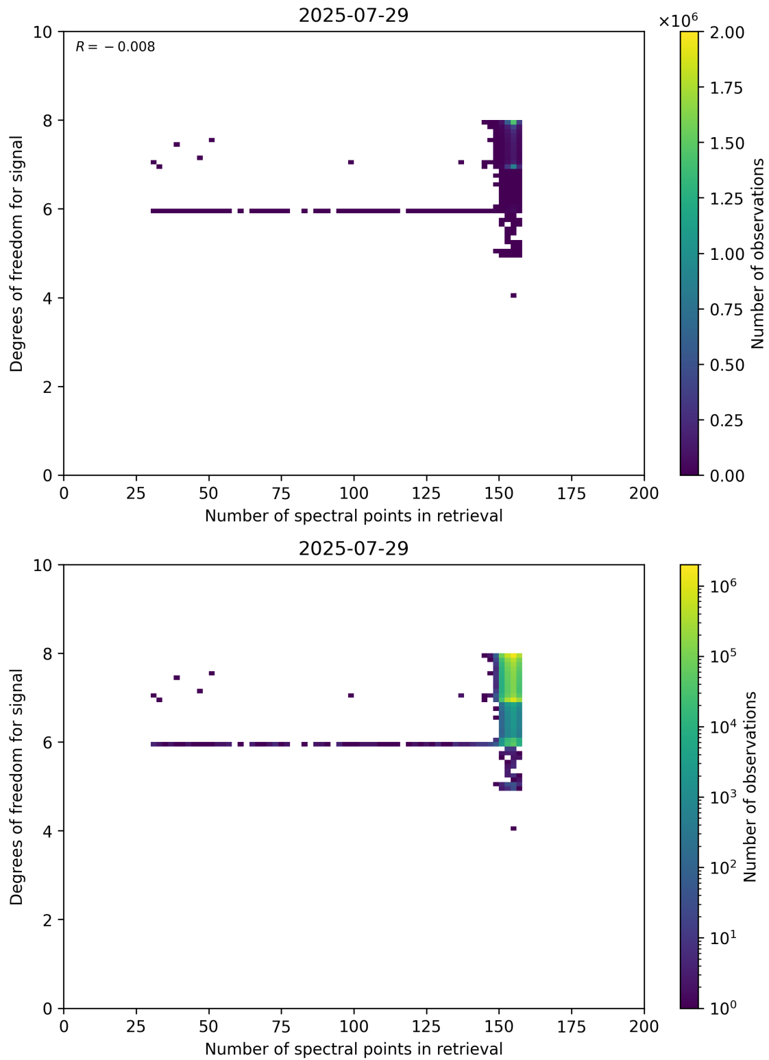
Figure 59: Scatter density plot of “Number of spectral points in retrieval” against “Degrees of freedom for signal” for 2025-07-29 to 2025-07-30.
