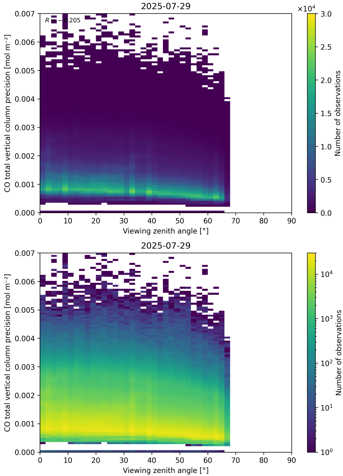
Figure 71: Scatter density plot of “Viewing zenith angle” against “CO total vertical column precision” for 2025-07-29 to 2025-07-30.
