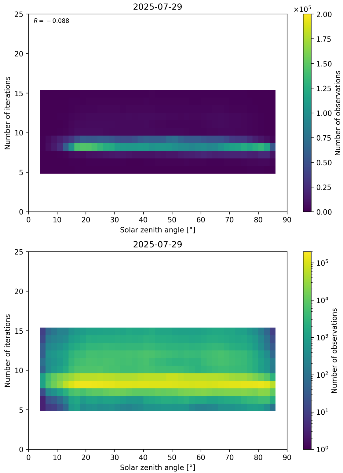
Figure 67: Scatter density plot of “Solar zenith angle” against “Number of iterations” for 2025-07-29 to 2025-07-30.
