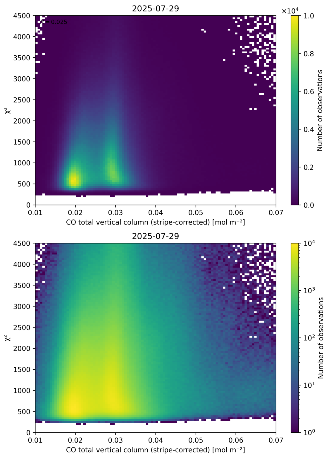
Figure 37: Scatter density plot of “CO total vertical column (stripe-corrected)” against “ \chi^2 ” for 2025-07-29 to 2025-07-30.
