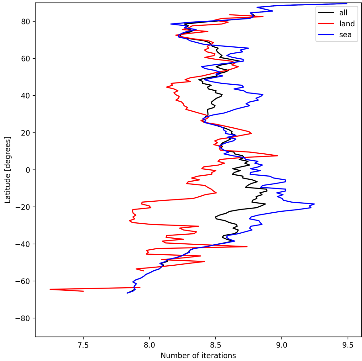
Figure 16: Zonal average of “Number of iterations” for 2025-07-29 to 2025-07-30.
