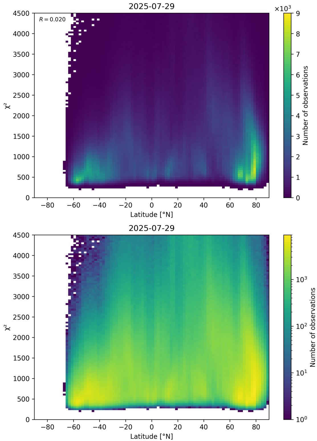
Figure 54: Scatter density plot of “Latitude” against “ \chi^2 ” for 2025-07-29 to 2025-07-30.
