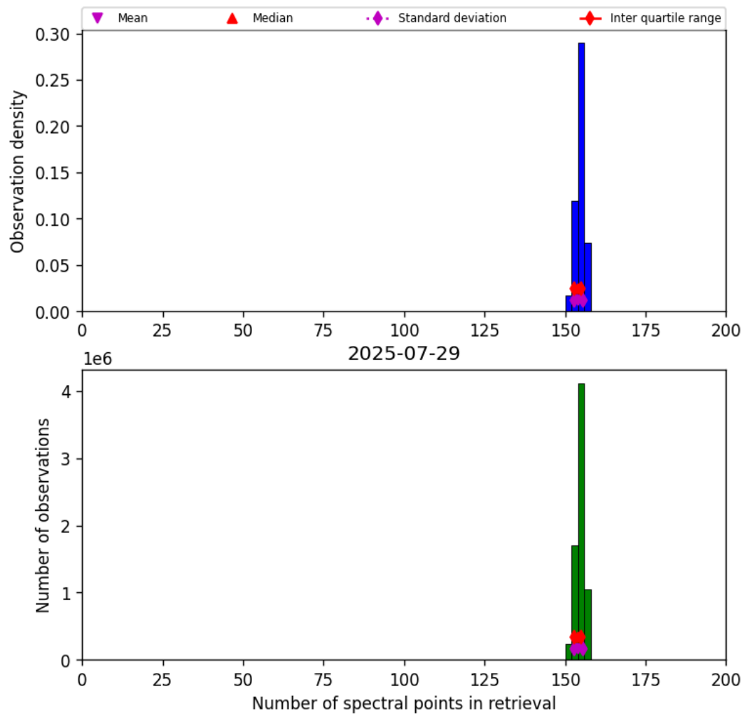
Figure 21: Histogram of “Number of spectral points in retrieval” for 2025-07-29 to 2025-07-30
