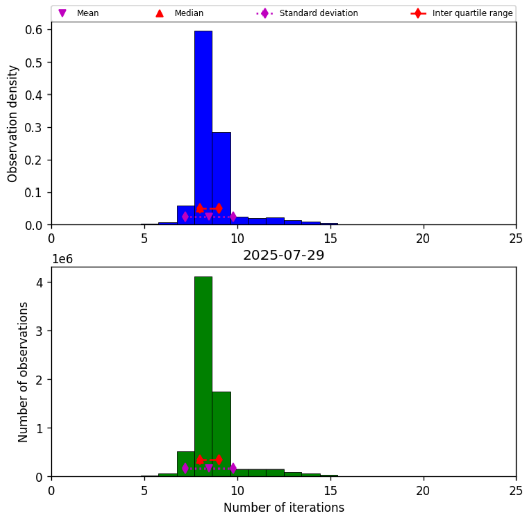
Figure 24: Histogram of “Number of iterations” for 2025-07-29 to 2025-07-30
