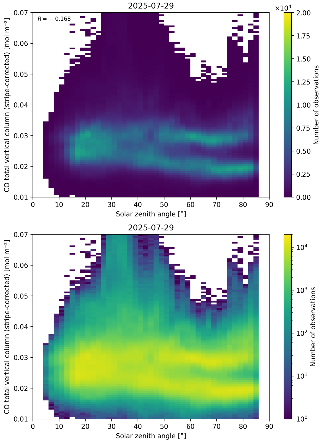
Figure 62: Scatter density plot of “Solar zenith angle” against “CO total vertical column (stripe-corrected)” for 2025-07-29 to 2025-07-30.
