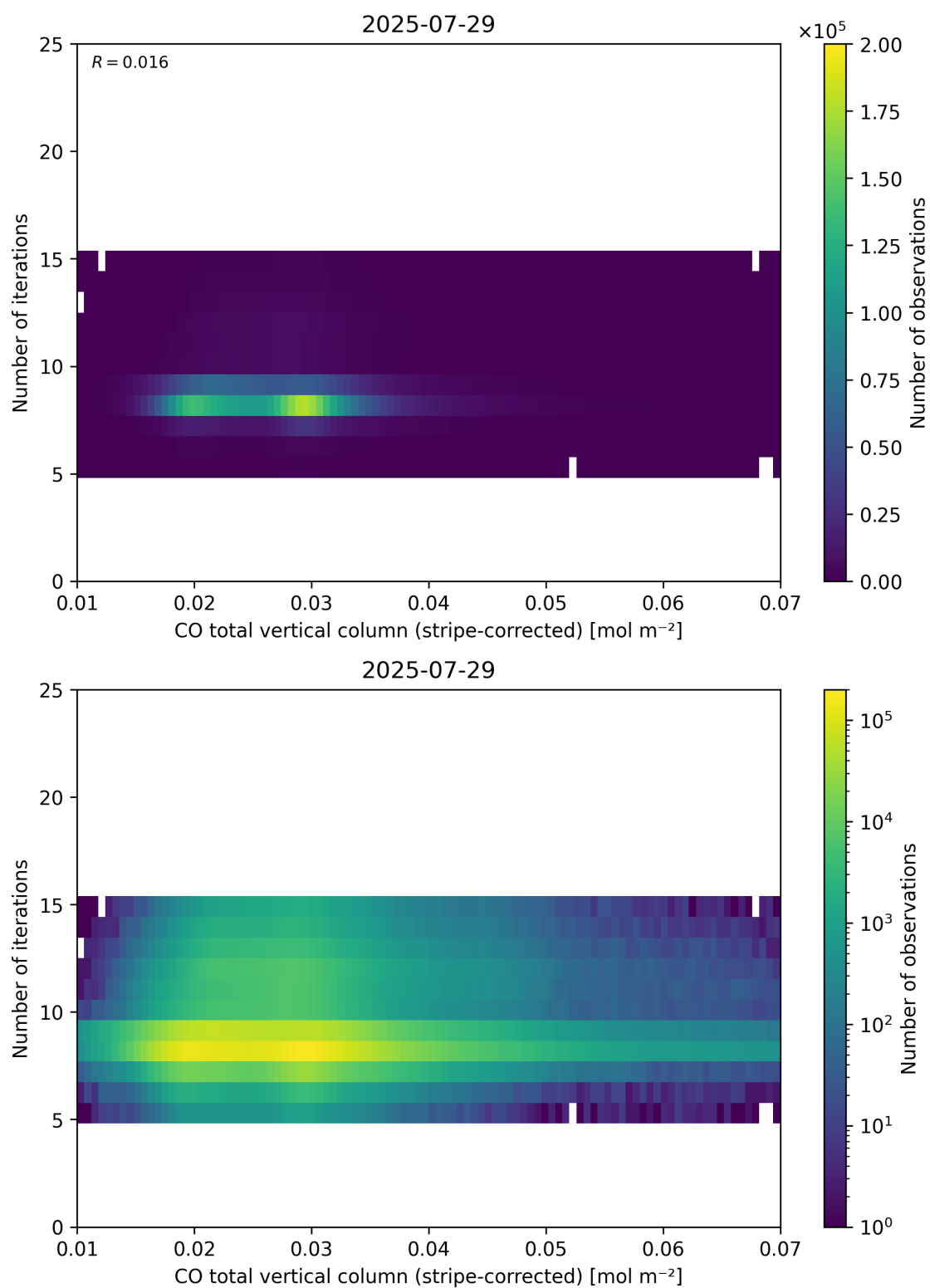
Figure 39: Scatter density plot of “CO total vertical column (stripe-corrected)” against “Number of iterations” for 2025-07-29 to 2025-07-30.
