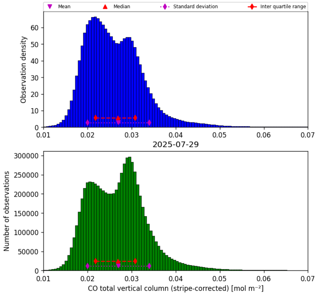
Figure 19: Histogram of “CO total vertical column (stripe-corrected)” for 2025-07-29 to 2025-07-30
