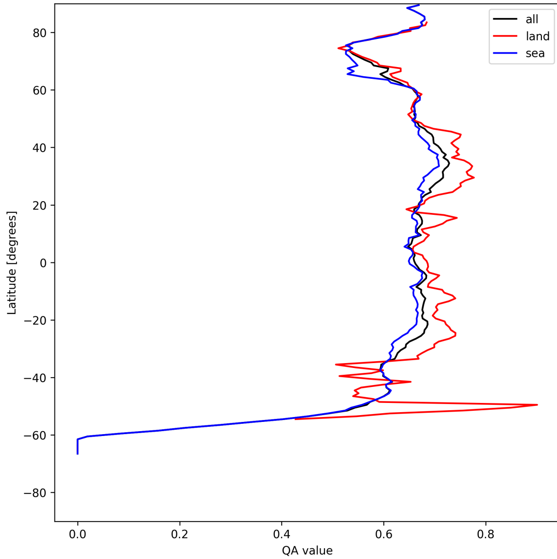
Figure 9: Zonal average of “QA value” for 2025-07-29 to 2025-07-30.
