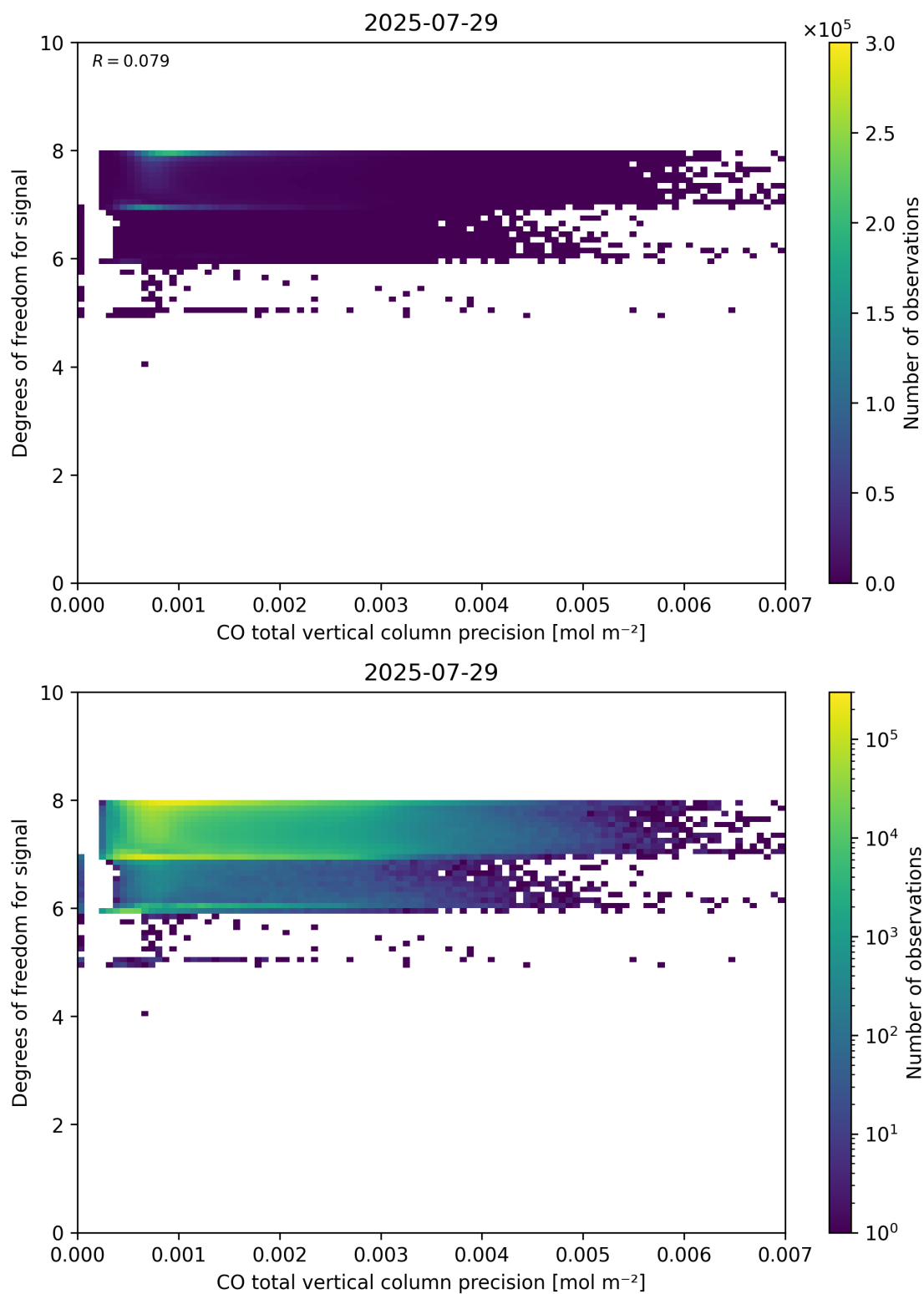
Figure 45: Scatter density plot of “CO total vertical column precision” against “Degrees of freedom for signal” for 2025-07-29 to 2025-07-30.
