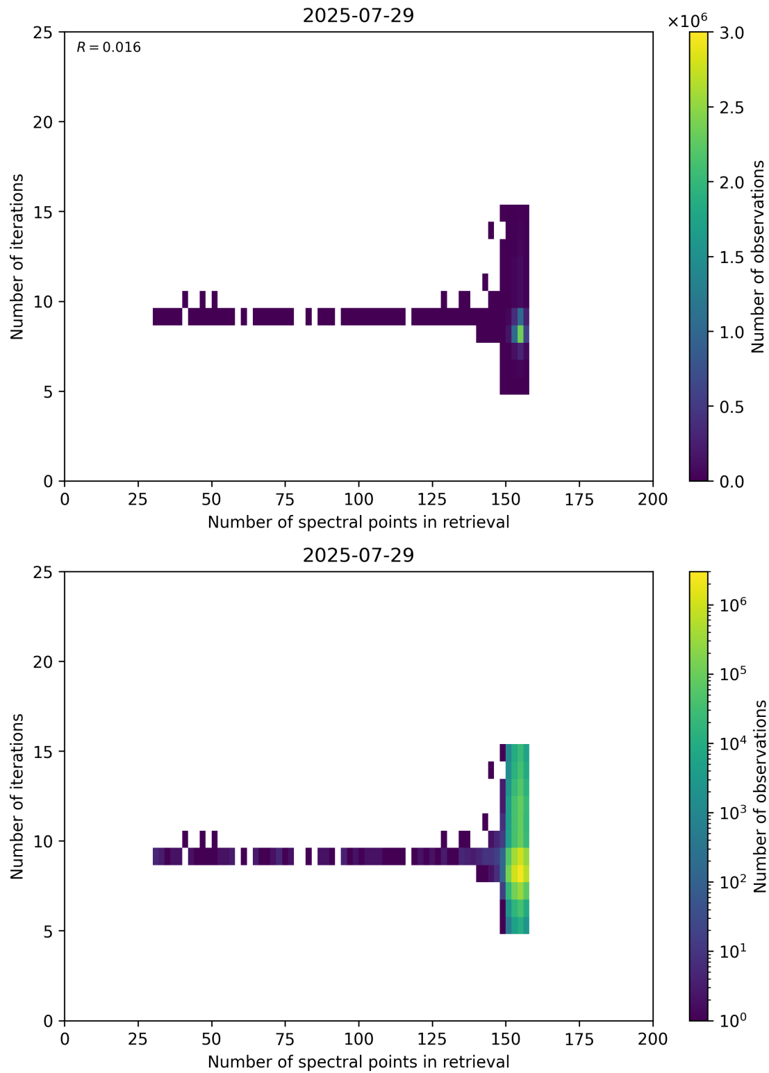
Figure 60: Scatter density plot of “Number of spectral points in retrieval” against “Number of iterations” for 2025-07-29 to 2025-07-30.
