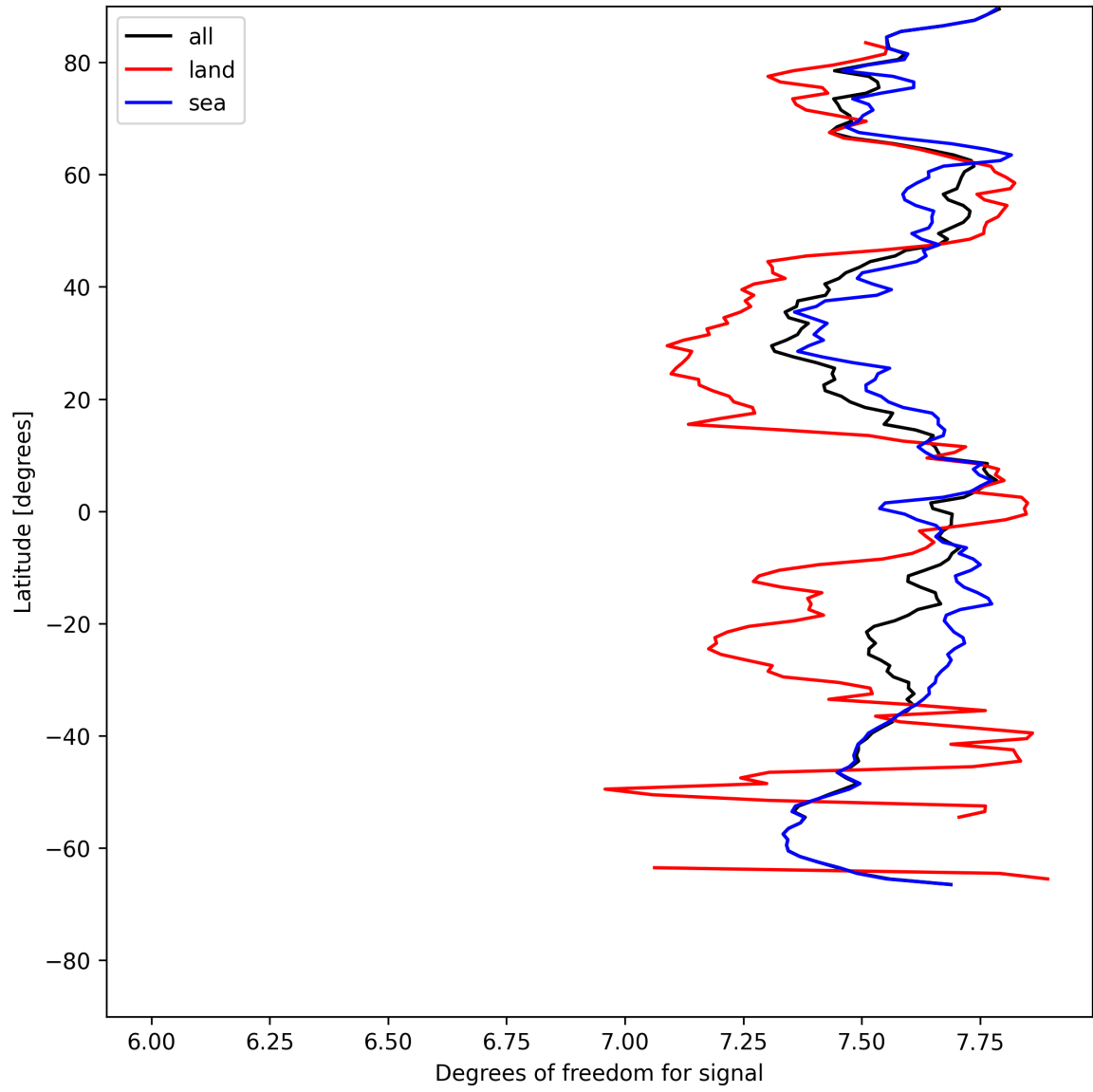
Figure 15: Zonal average of “Degrees of freedom for signal” for 2025-07-29 to 2025-07-30.
