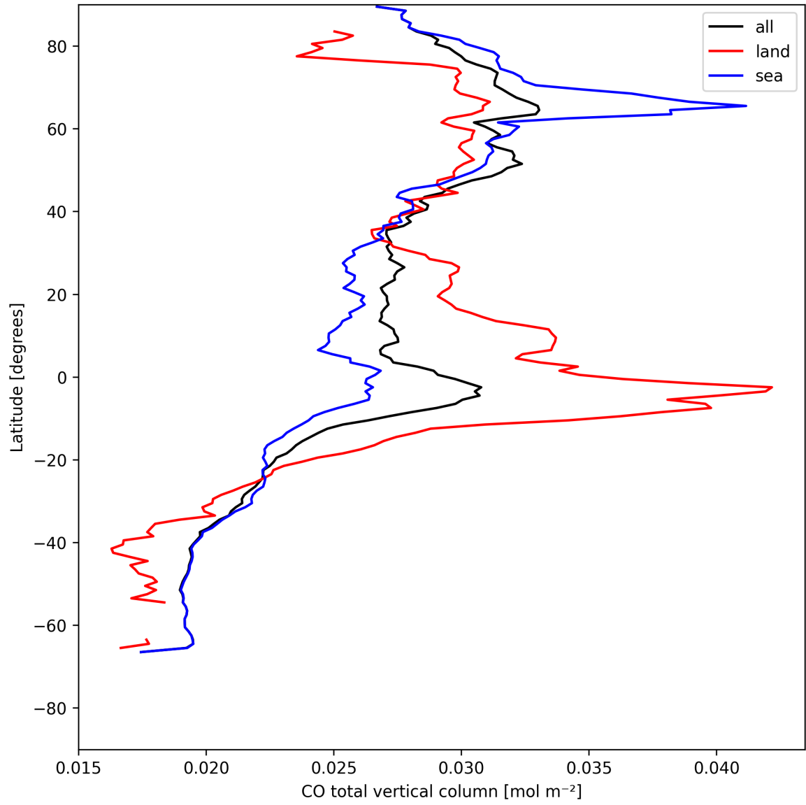
Figure 10: Zonal average of “CO total vertical column” for 2025-07-29 to 2025-07-30.
