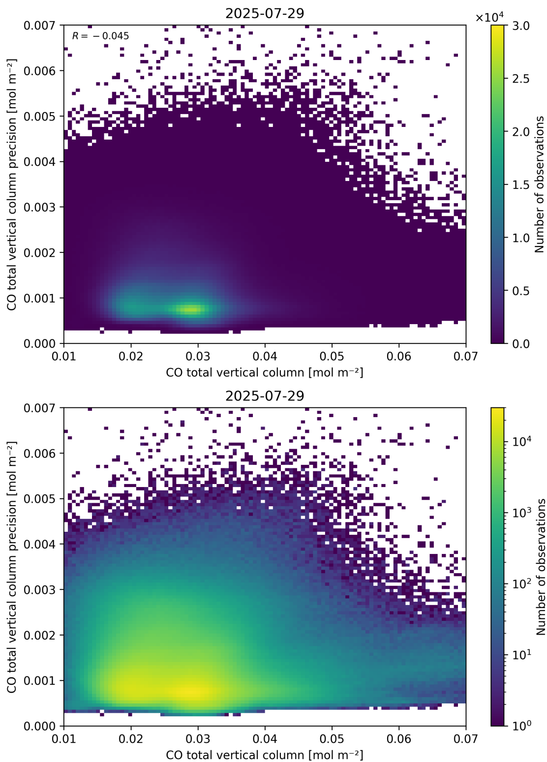
Figure 34: Scatter density plot of “CO total vertical column” against “CO total vertical column precision” for 2025-07-29 to 2025-07-30.
