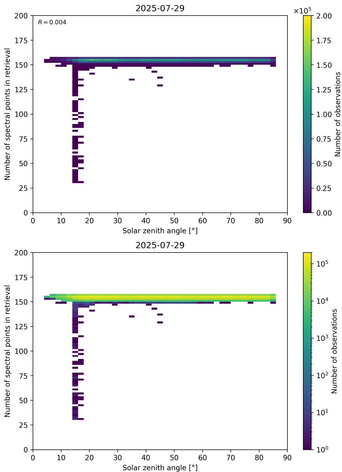
Figure 68: Scatter density plot of “Solar zenith angle” against “Number of spectral points in retrieval” for 2025-07-29 to 2025-07-30.
