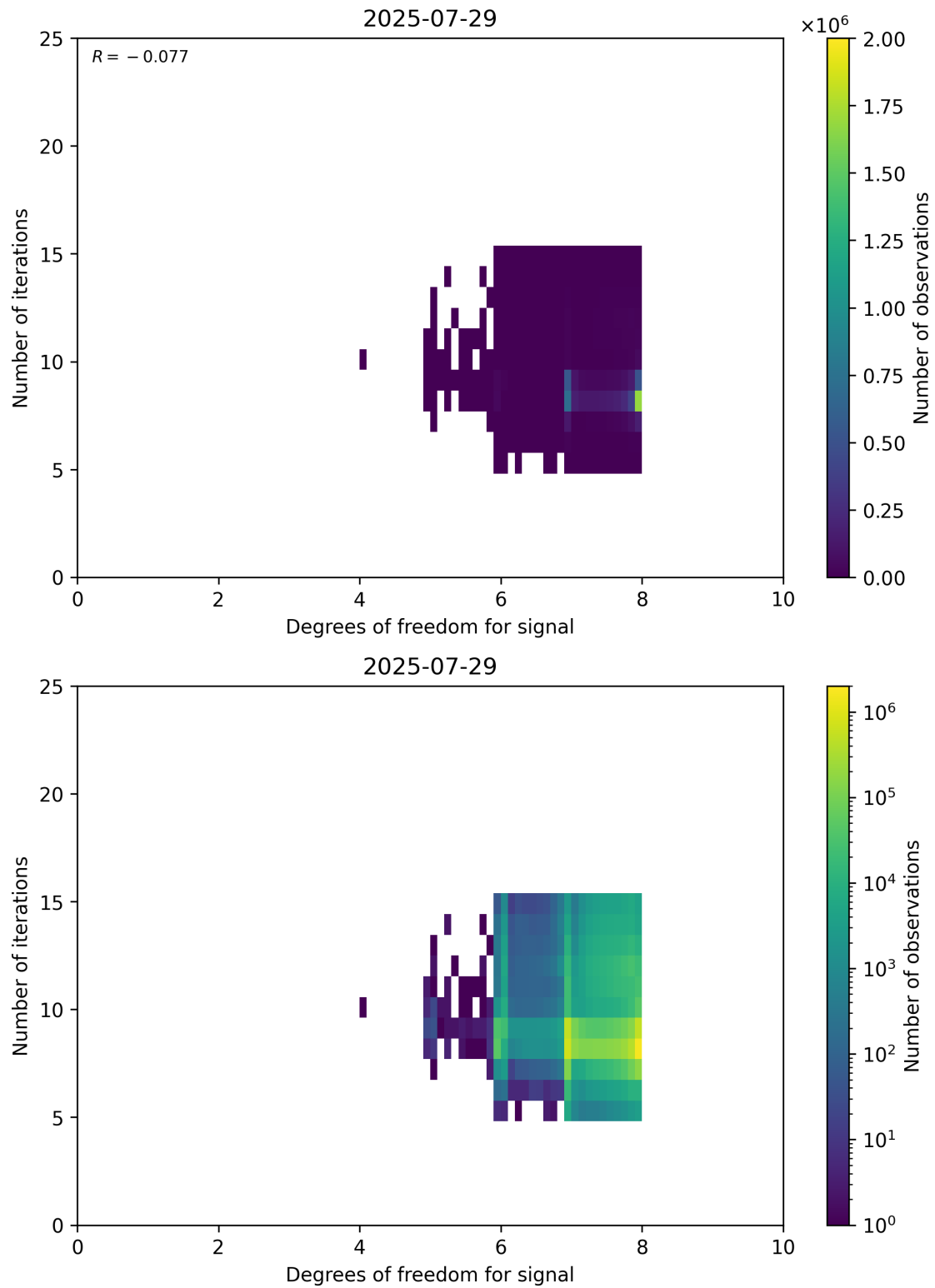
Figure 50: Scatter density plot of “Degrees of freedom for signal” against “Number of iterations” for 2025-07-29 to 2025-07-30.
