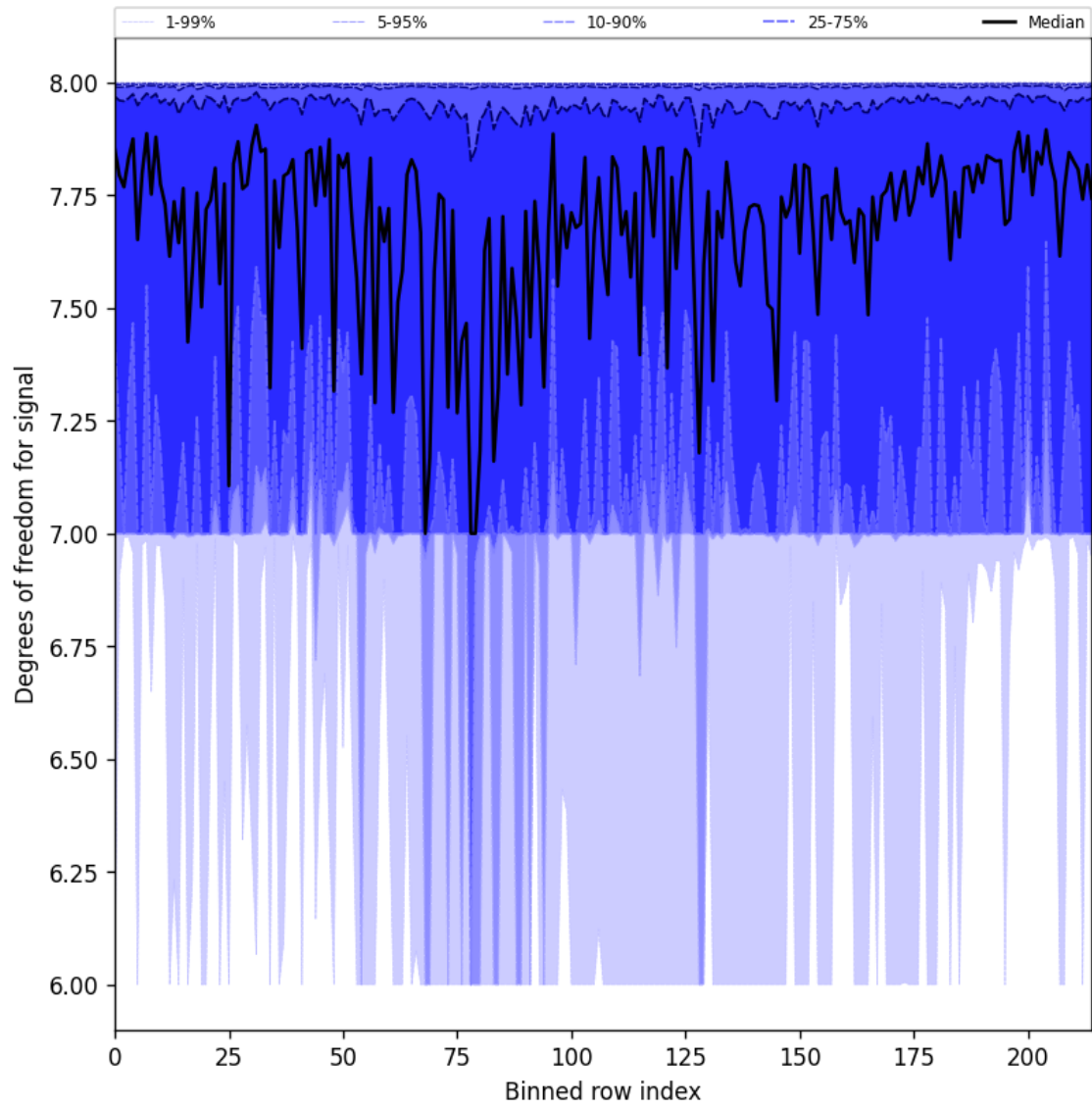
Figure 31: Along track statistics of “Degrees of freedom for signal” for 2025-07-29 to 2025-07-30
