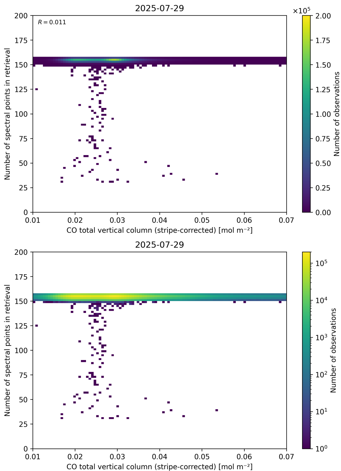
Figure 40: Scatter density plot of “CO total vertical column (stripe-corrected)” against “Number of spectral points in retrieval” for 2025-07-29 to 2025-07-30.
