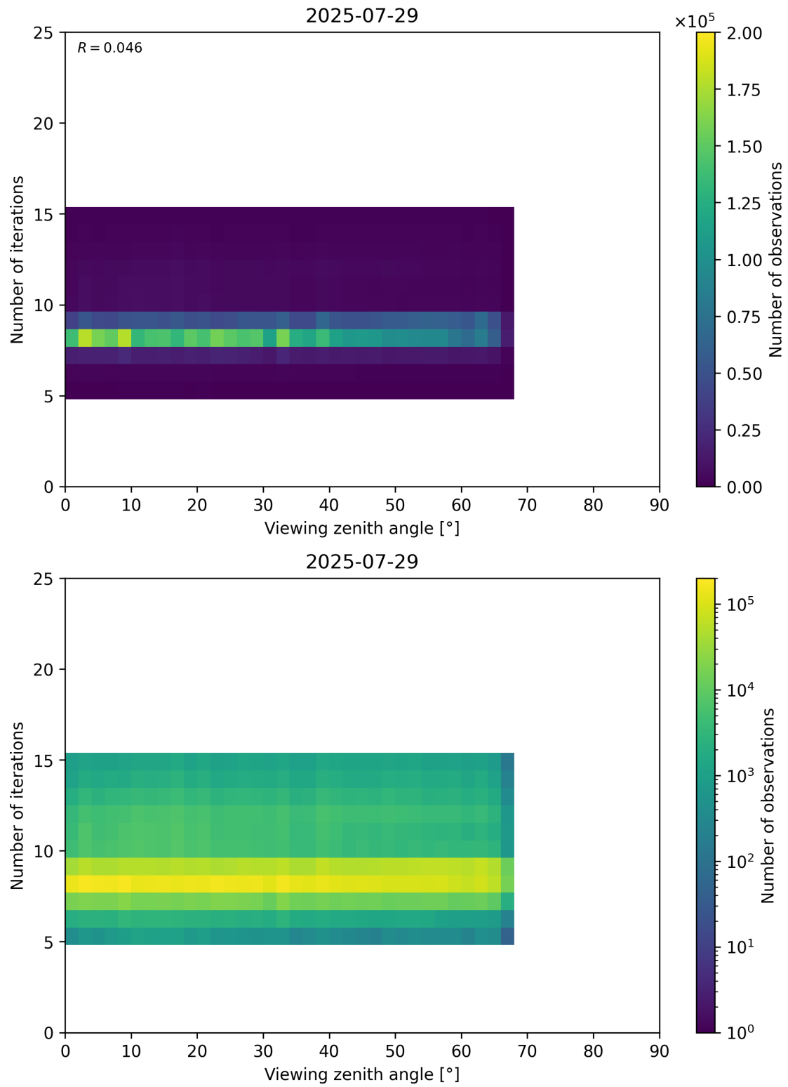
Figure 75: Scatter density plot of “Viewing zenith angle” against “Number of iterations” for 2025-07-29 to 2025-07-30.
