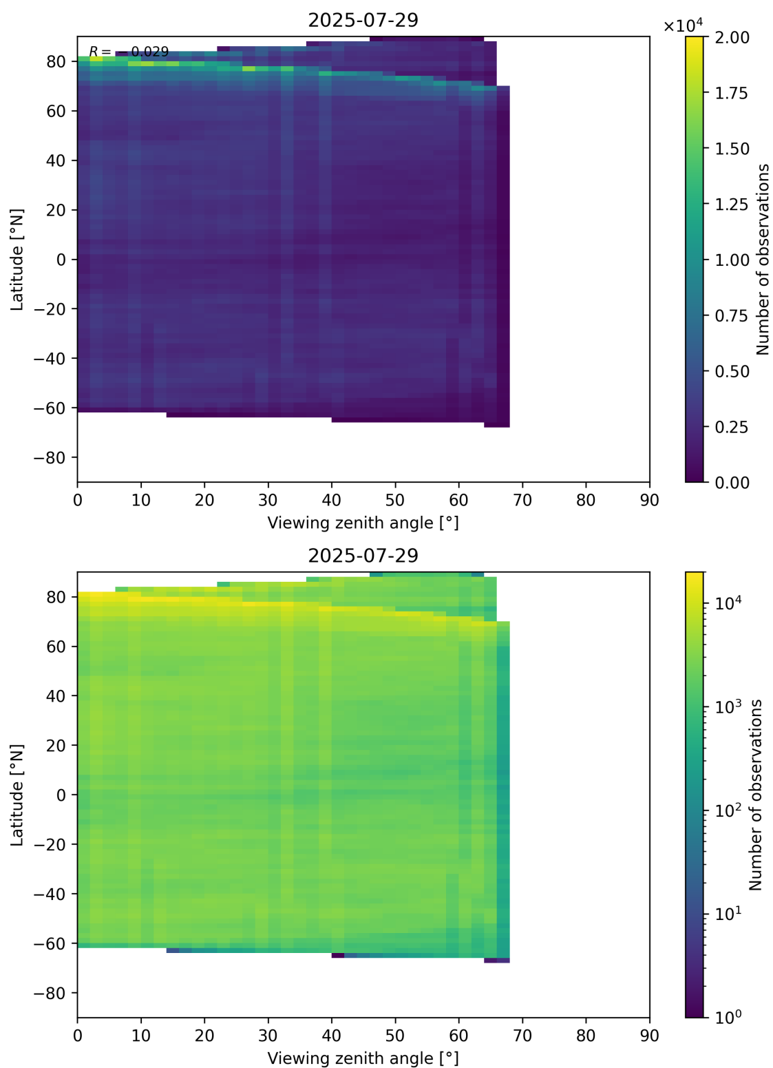
Figure 74: Scatter density plot of “Viewing zenith angle” against “Latitude” for 2025-07-29 to 2025-07-30.
