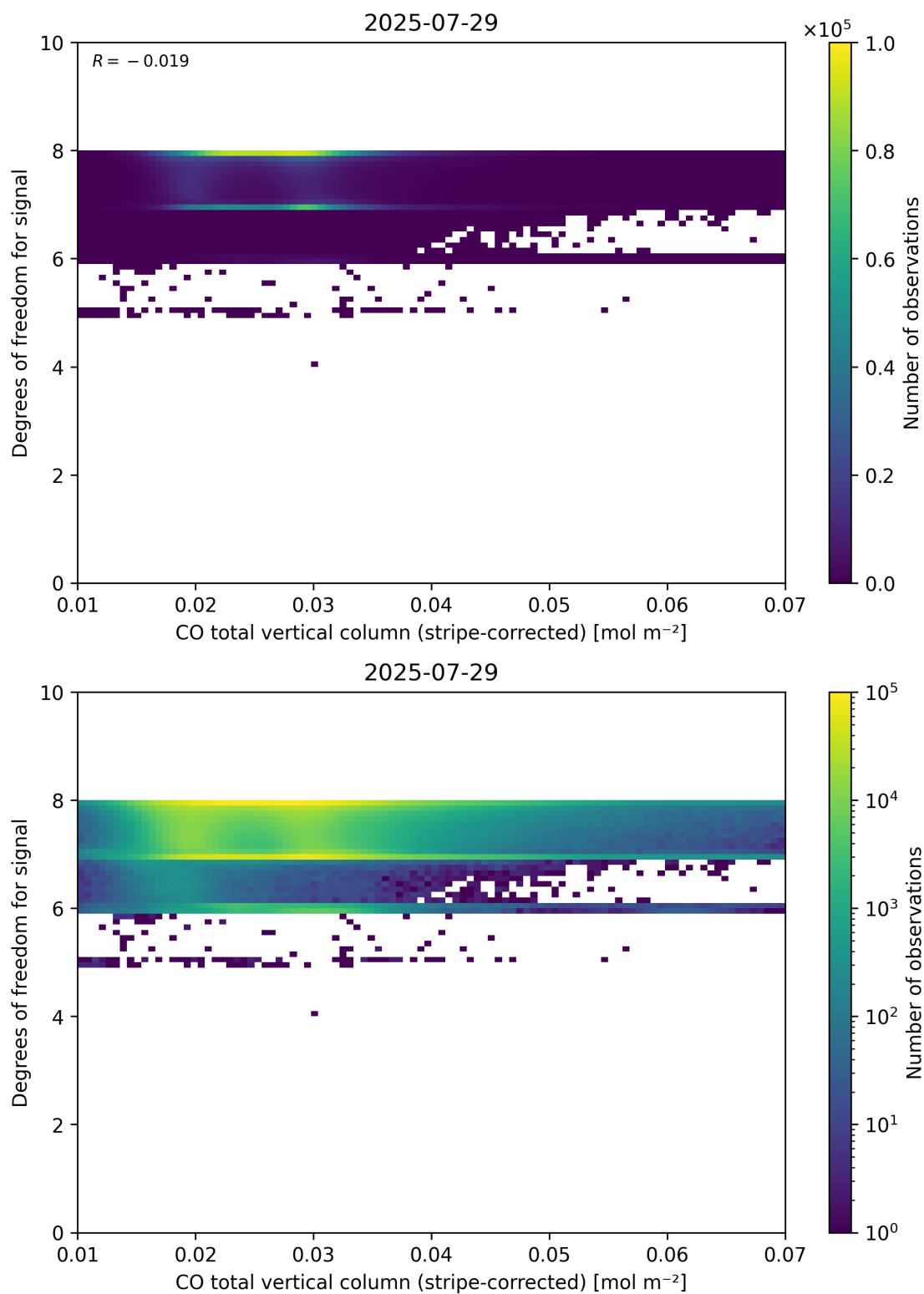
Figure 38: Scatter density plot of “CO total vertical column (stripe-corrected)” against “Degrees of freedom for signal” for 2025-07-29 to 2025-07-30.
