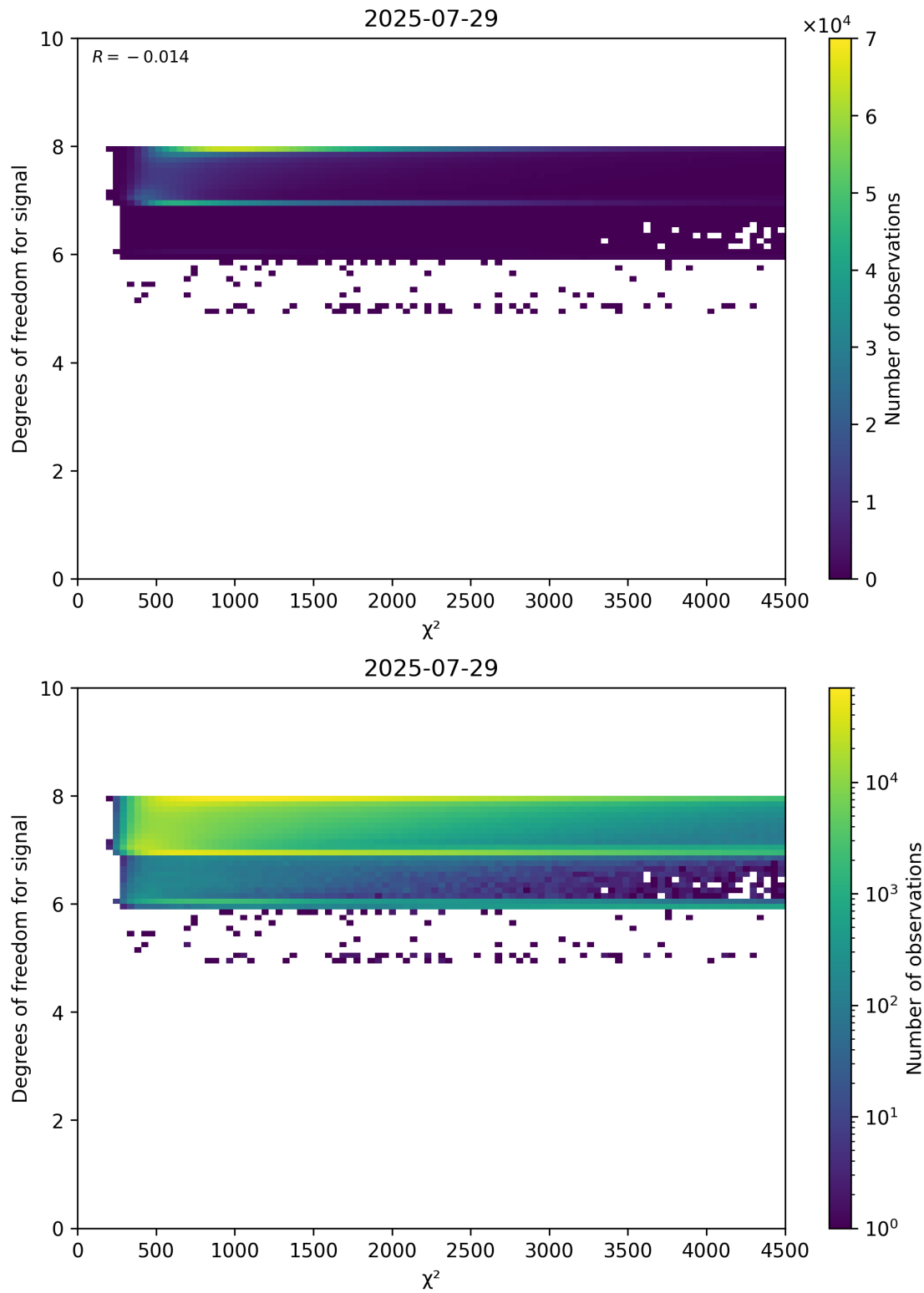
Figure 48: Scatter density plot of " \chi^2 " against "Degrees of freedom for signal" for 2025-07-29 to 2025-07-30.
