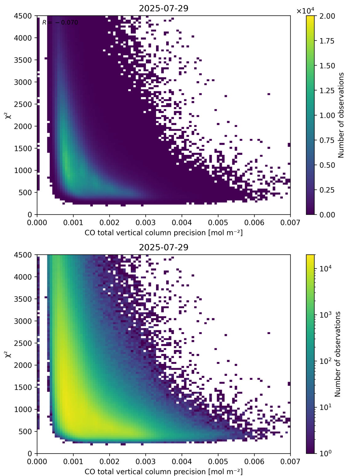
Figure 44: Scatter density plot of “CO total vertical column precision” against “ \chi^2 ” for 2025-07-29 to 2025-07-30.
