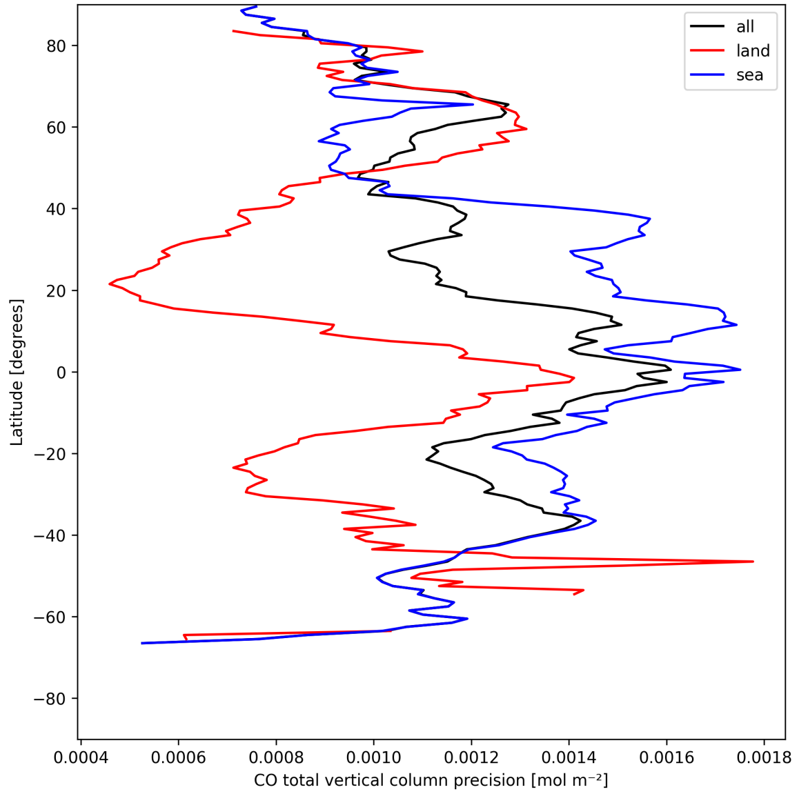
Figure 12: Zonal average of “CO total vertical column precision” for 2025-07-29 to 2025-07-30.
