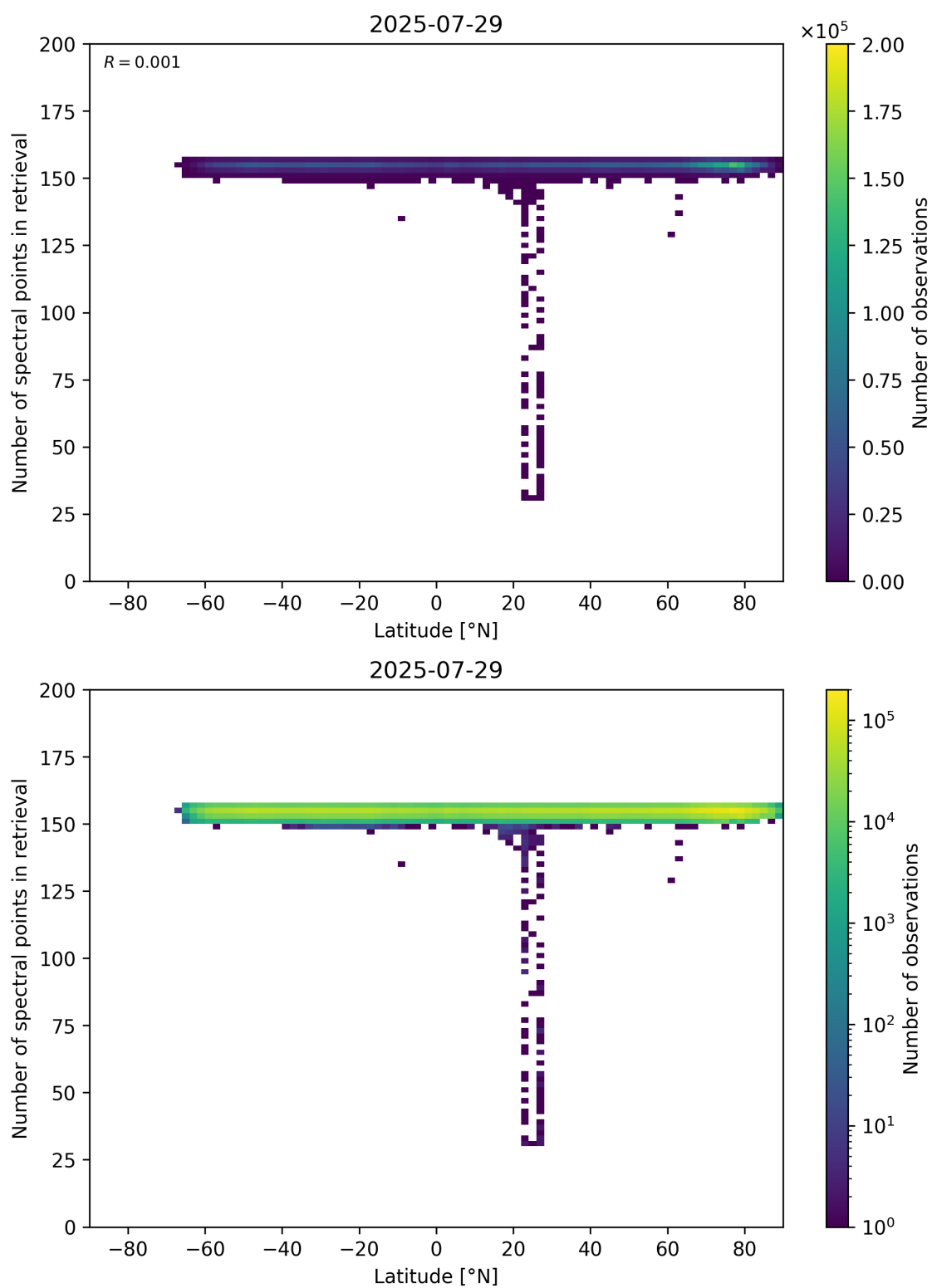
Figure 57: Scatter density plot of “Latitude” against “Number of spectral points in retrieval” for 2025-07-29 to 2025-07-30.
