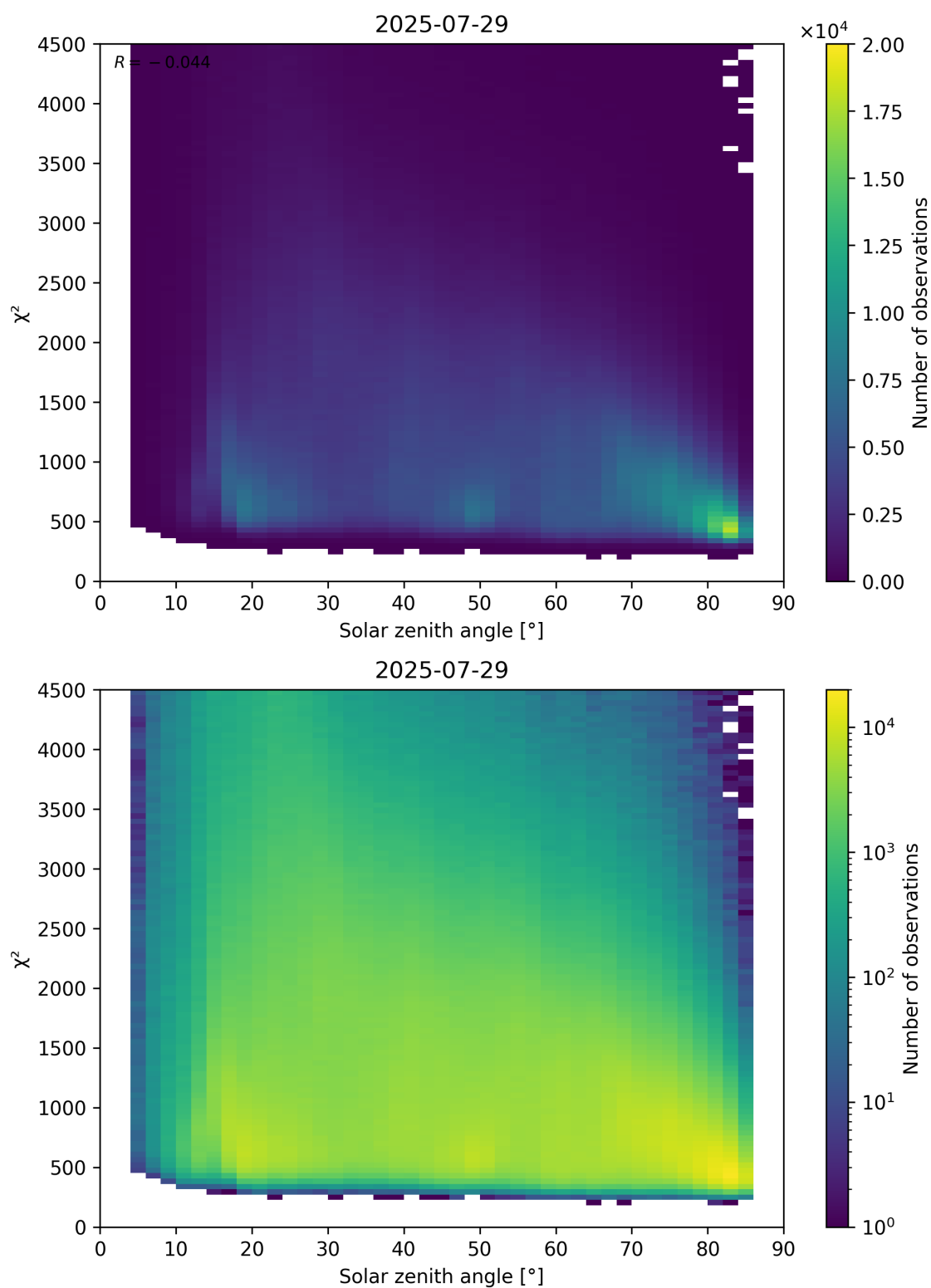
Figure 64: Scatter density plot of “Solar zenith angle” against “ \chi^2 ” for 2025-07-29 to 2025-07-30.
