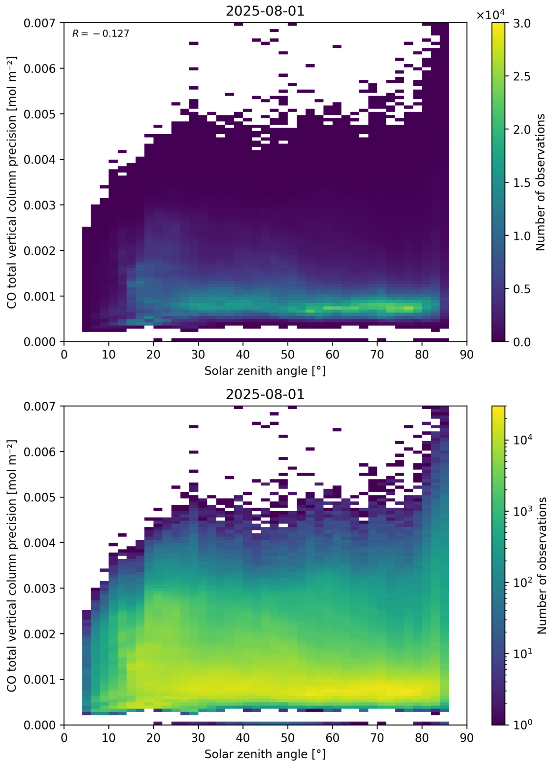
Figure 63: Scatter density plot of “Solar zenith angle” against “CO total vertical column precision” for 2025-07-31 to 2025-08-02.
