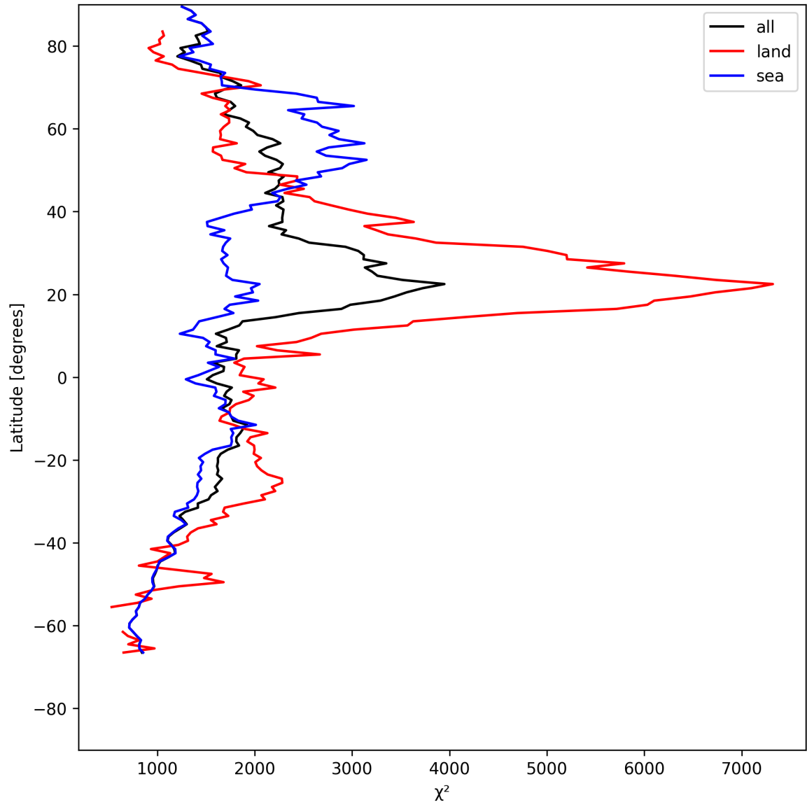
Figure 14: Zonal average of “ \chi^2 ” for 2025-07-31 to 2025-08-02.
