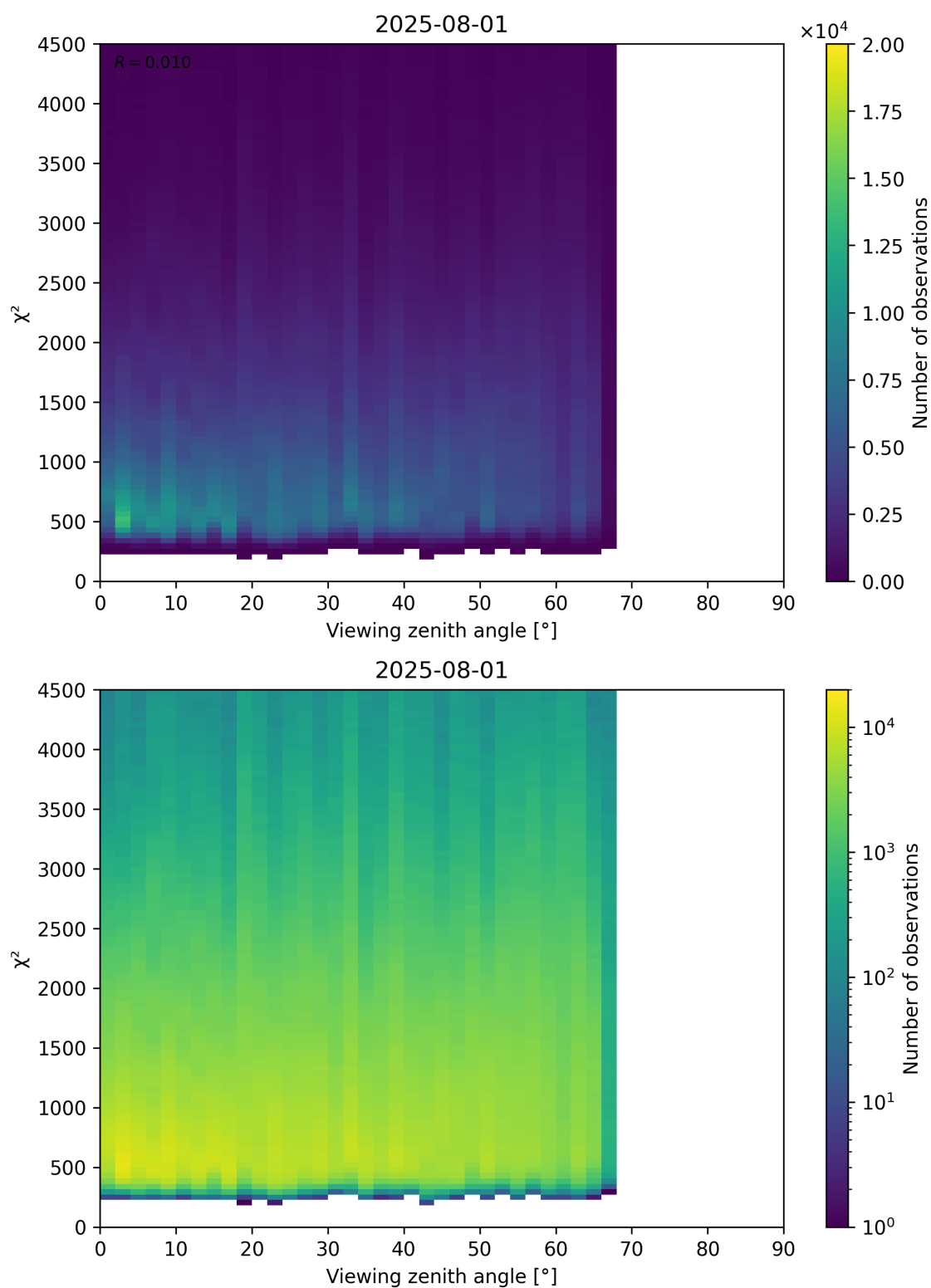
Figure 72: Scatter density plot of “Viewing zenith angle” against “ \chi^2 ” for 2025-07-31 to 2025-08-02.
