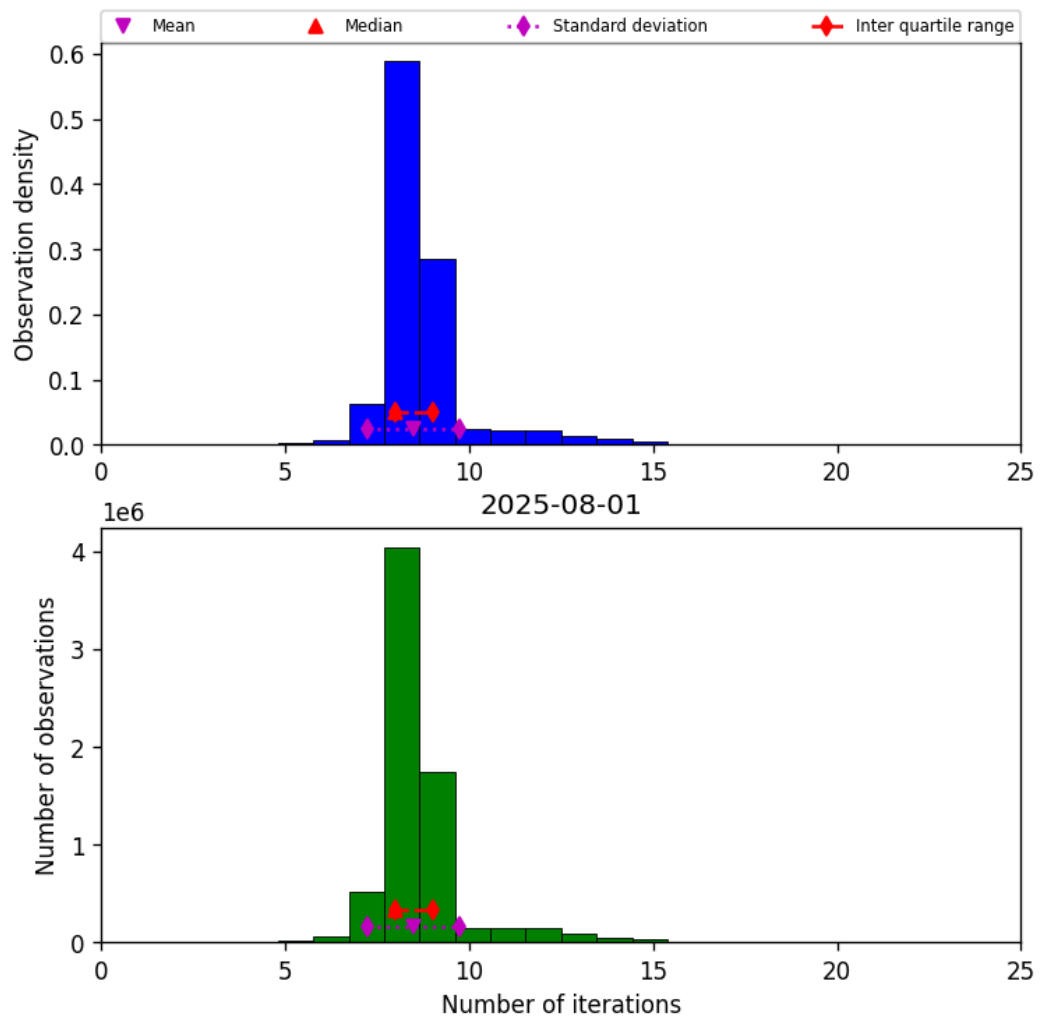
Figure 24: Histogram of “Number of iterations” for 2025-07-31 to 2025-08-02
