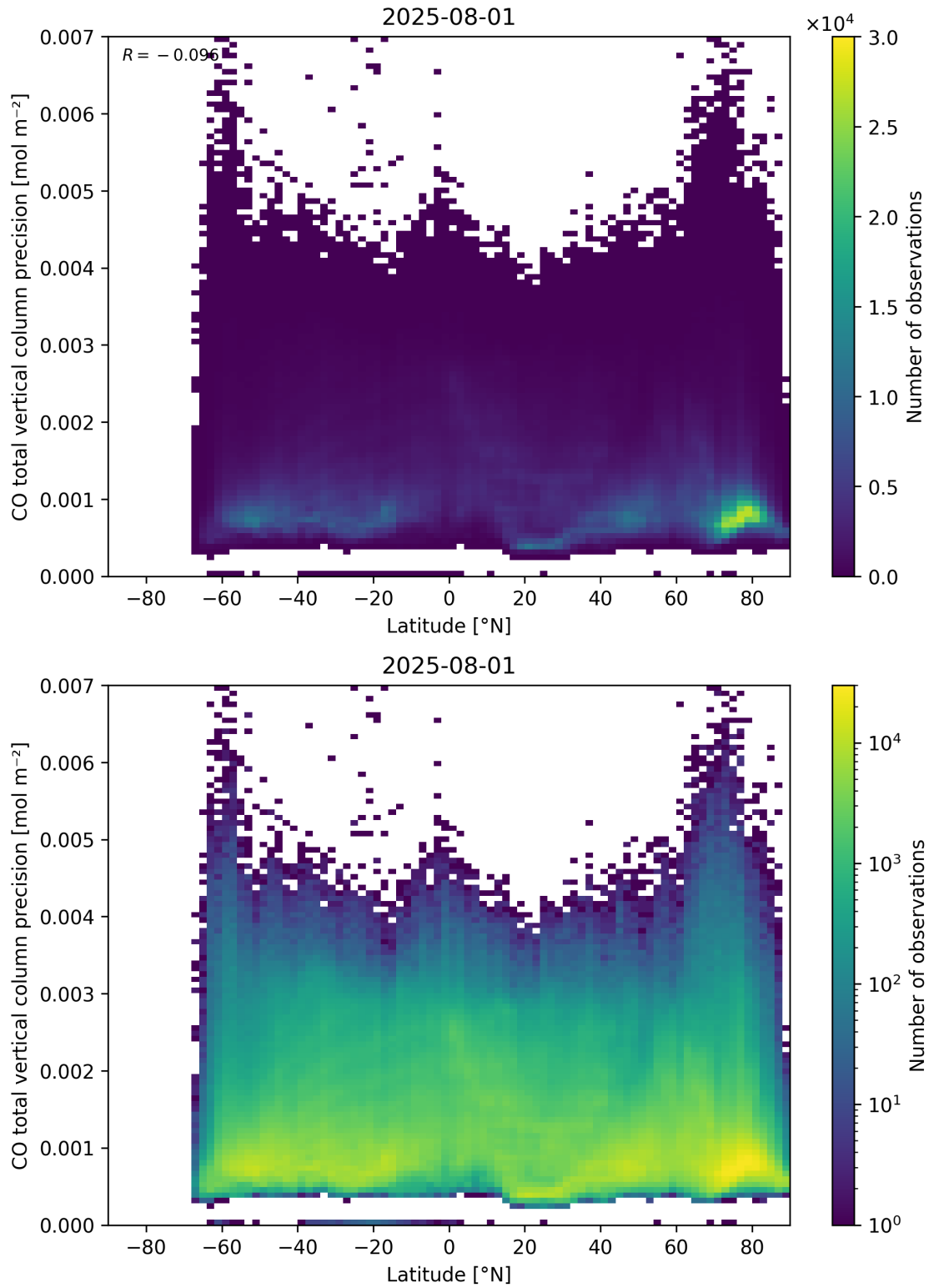
Figure 53: Scatter density plot of “Latitude” against “CO total vertical column precision” for 2025-07-31 to 2025-08-02.
