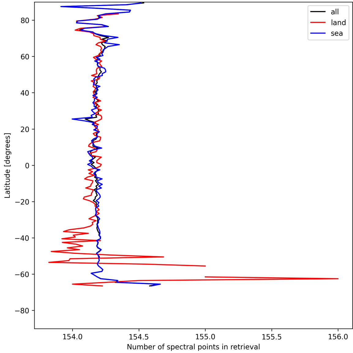
Figure 13: Zonal average of “Number of spectral points in retrieval” for 2025-07-31 to 2025-08-02.
