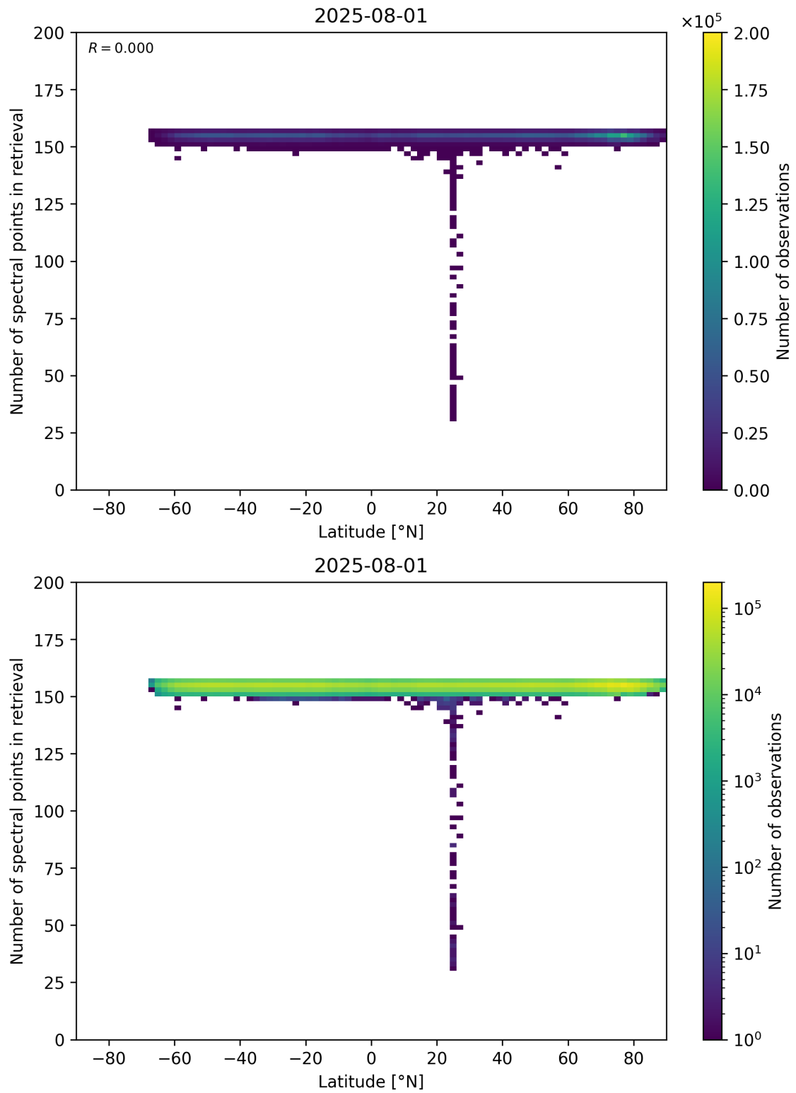
Figure 57: Scatter density plot of “Latitude” against “Number of spectral points in retrieval” for 2025-07-31 to 2025-08-02.
