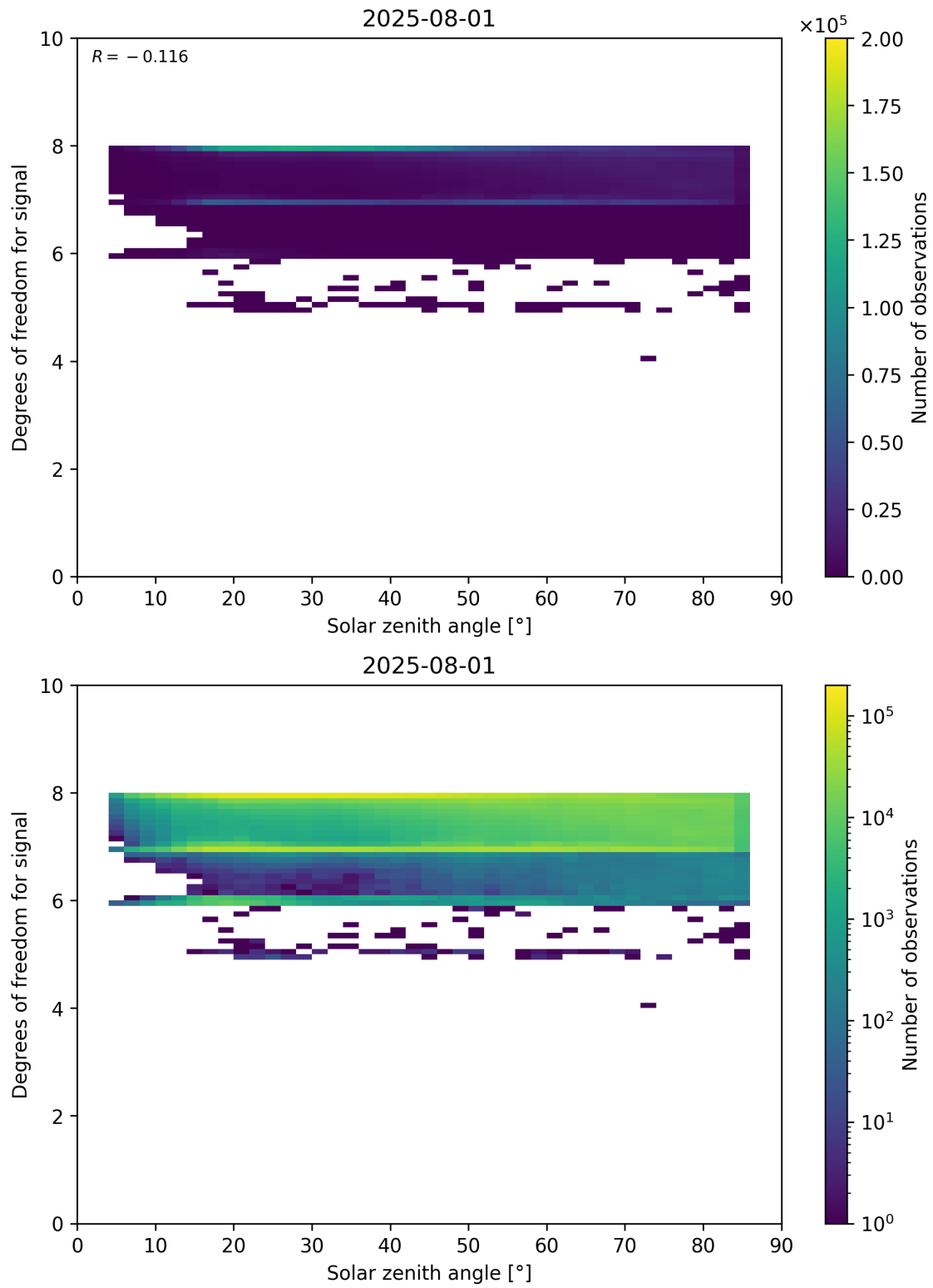
Figure 65: Scatter density plot of “Solar zenith angle” against “Degrees of freedom for signal” for 2025-07-31 to 2025-08-02.
