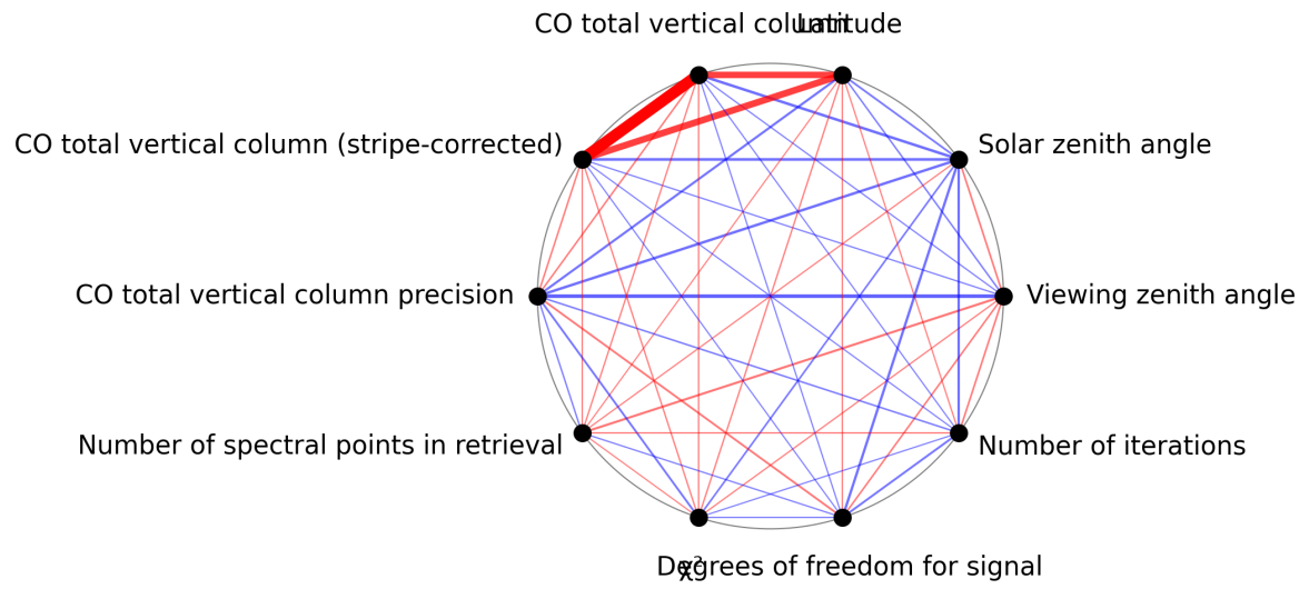
Figure 1: Map of correlation graph for 2025-07-31 to 2025-08-02.
