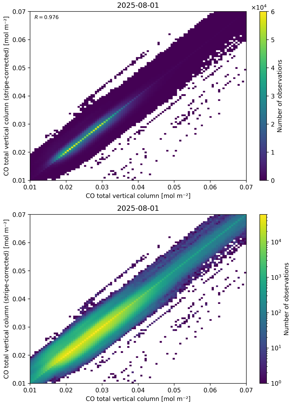
Figure 33: Scatter density plot of “CO total vertical column” against “CO total vertical column (stripe-corrected)” for 2025-07-31 to 2025-08-02.
