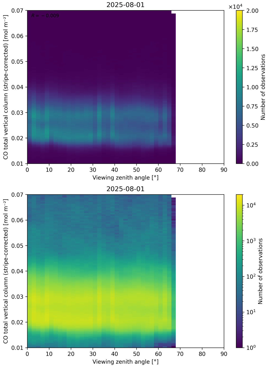
Figure 70: Scatter density plot of “Viewing zenith angle” against “CO total vertical column (stripe-corrected)” for 2025-07-31 to 2025-08-02.
