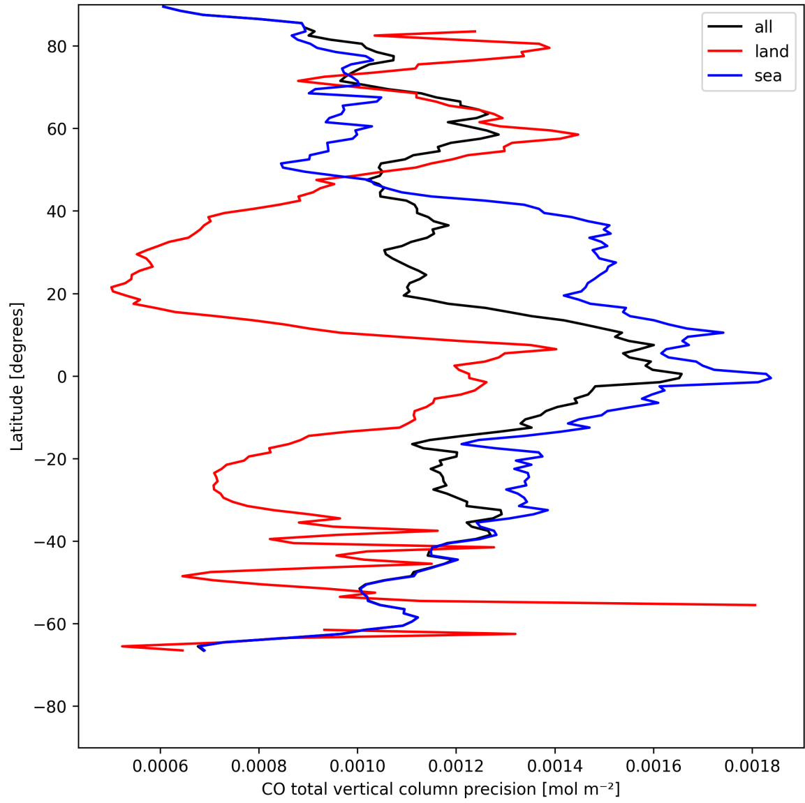
Figure 12: Zonal average of “CO total vertical column precision” for 2025-07-31 to 2025-08-02.
