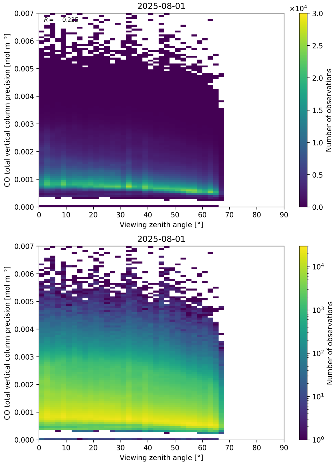
Figure 71: Scatter density plot of “Viewing zenith angle” against “CO total vertical column precision” for 2025-07-31 to 2025-08-02.
