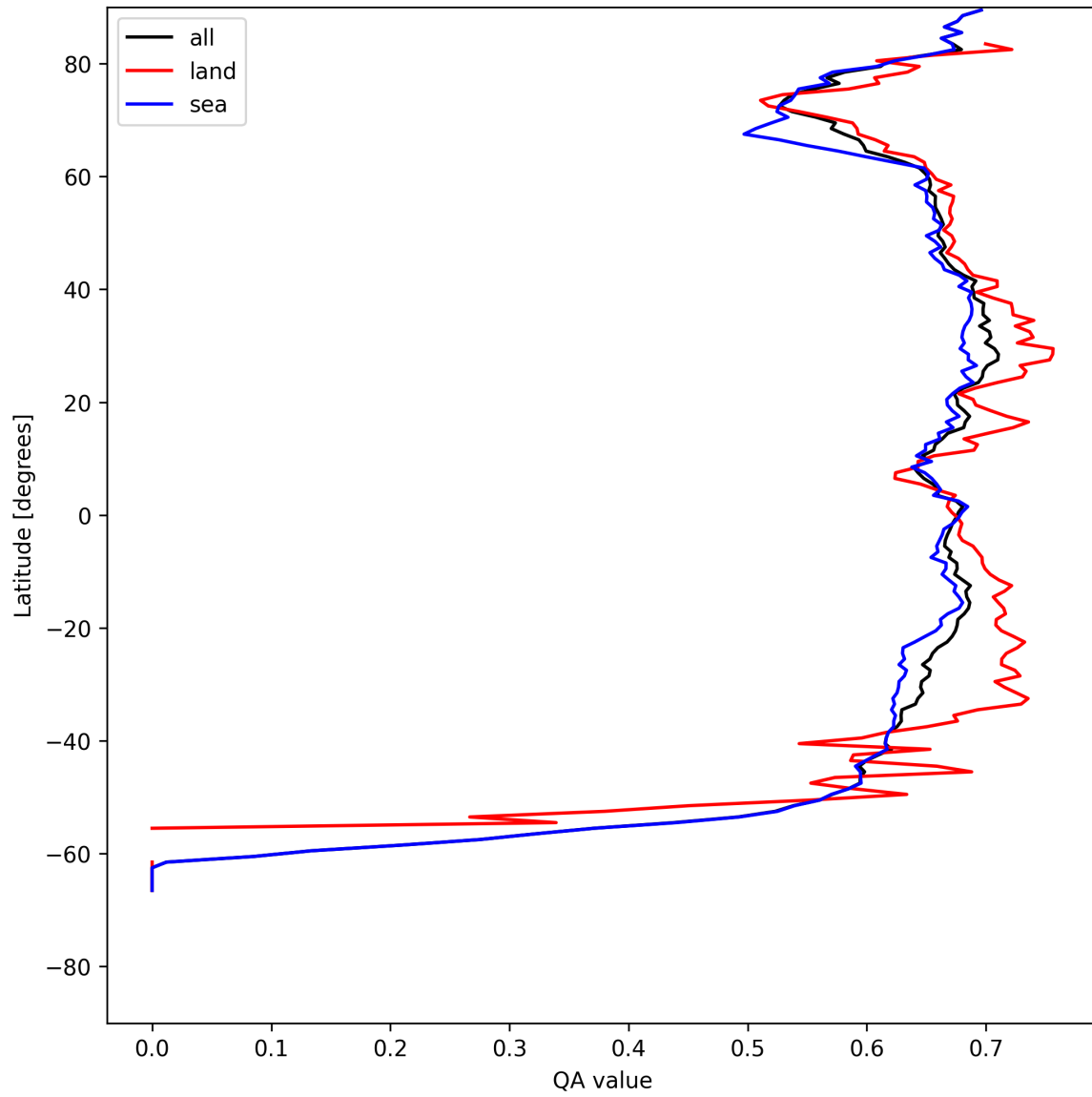
Figure 9: Zonal average of “QA value” for 2025-07-31 to 2025-08-02.
