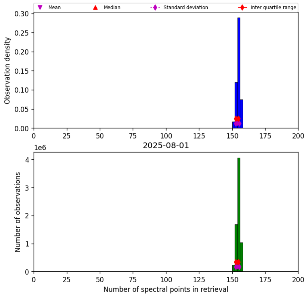
Figure 21: Histogram of “Number of spectral points in retrieval” for 2025-07-31 to 2025-08-02
