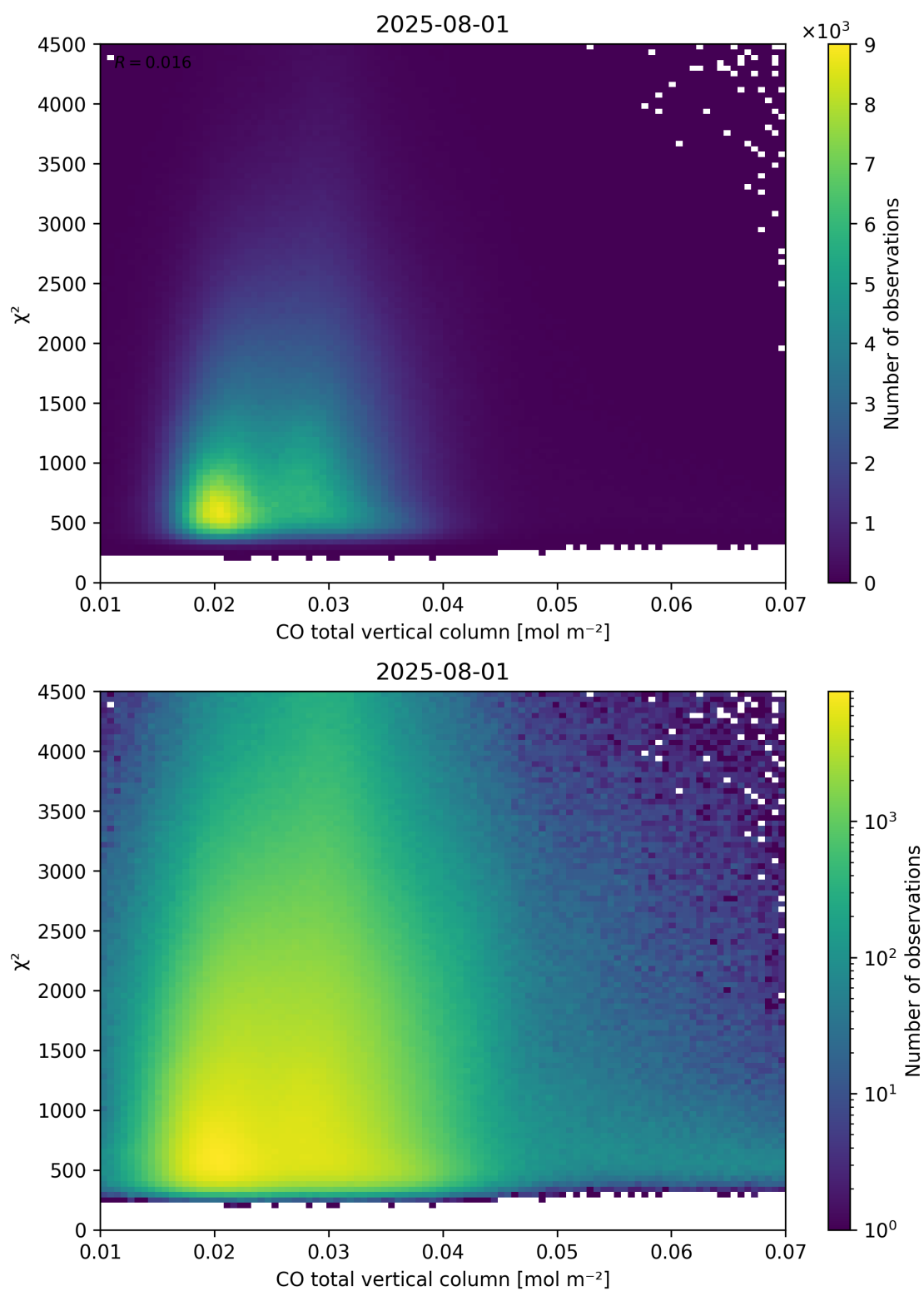
Figure 35: Scatter density plot of “CO total vertical column” against “ \chi^2 ” for 2025-07-31 to 2025-08-02.
