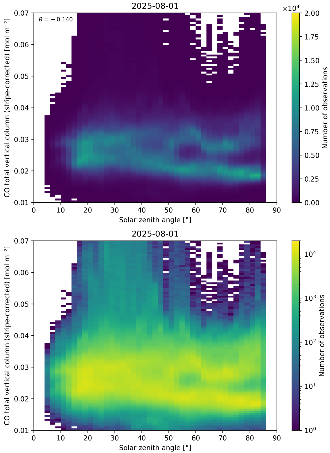
Figure 62: Scatter density plot of “Solar zenith angle” against “CO total vertical column (stripe-corrected)” for 2025-07-31 to 2025-08-02.
