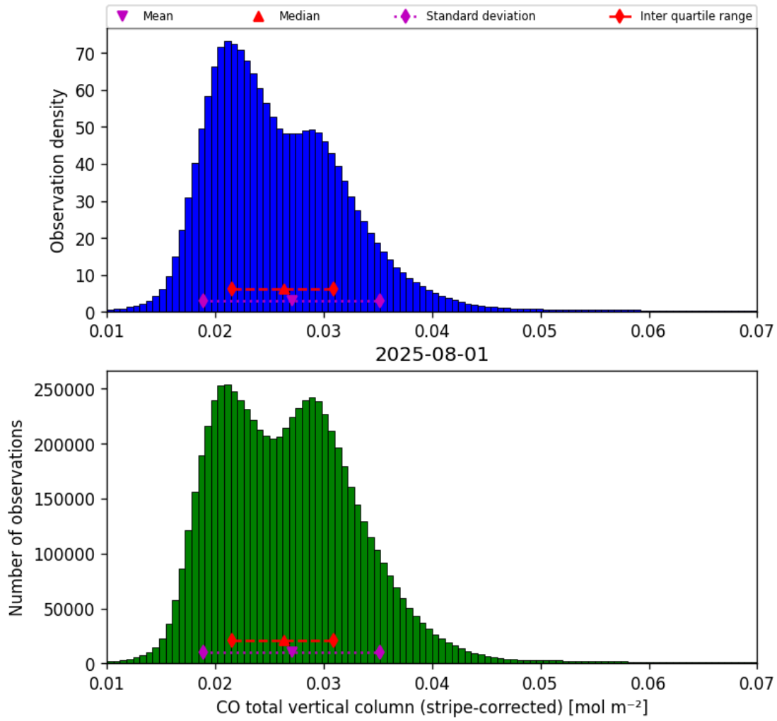
Figure 19: Histogram of “CO total vertical column (stripe-corrected)” for 2025-07-31 to 2025-08-02
