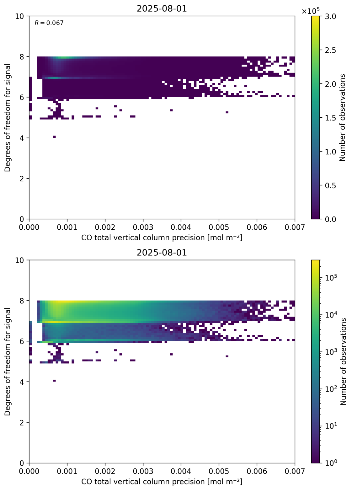
Figure 45: Scatter density plot of “CO total vertical column precision” against “Degrees of freedom for signal” for 2025-07-31 to 2025-08-02.
