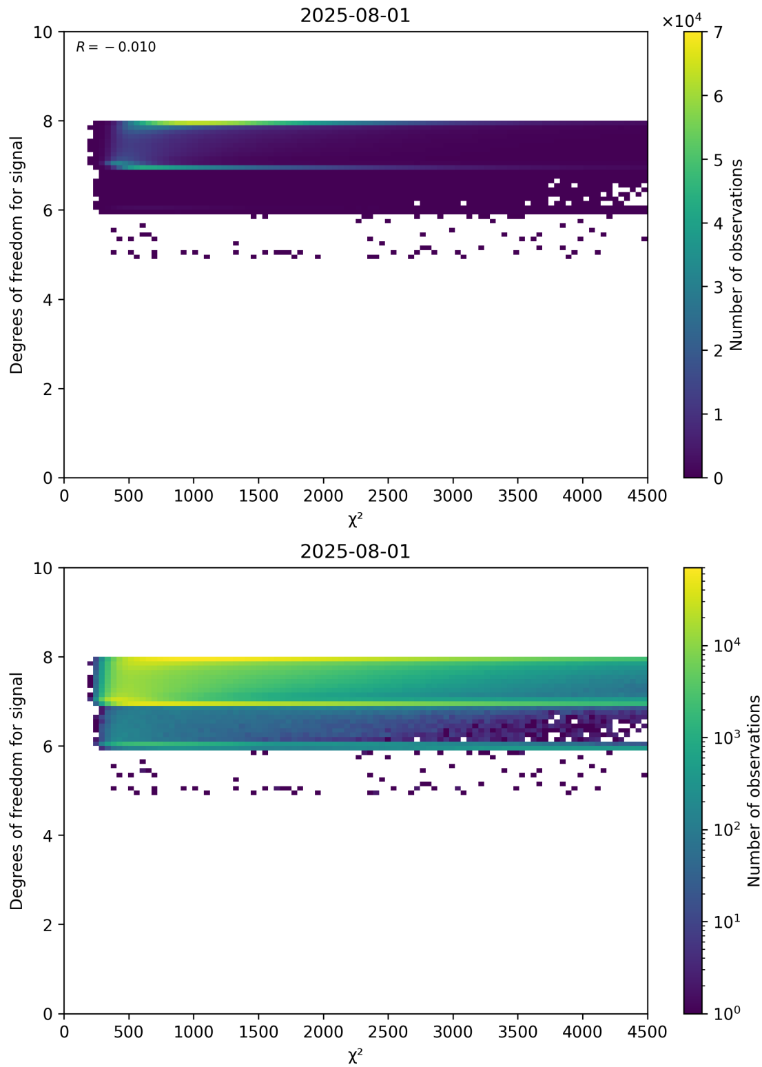
Figure 48: Scatter density plot of “ \chi^2 ” against “Degrees of freedom for signal” for 2025-07-31 to 2025-08-02.
