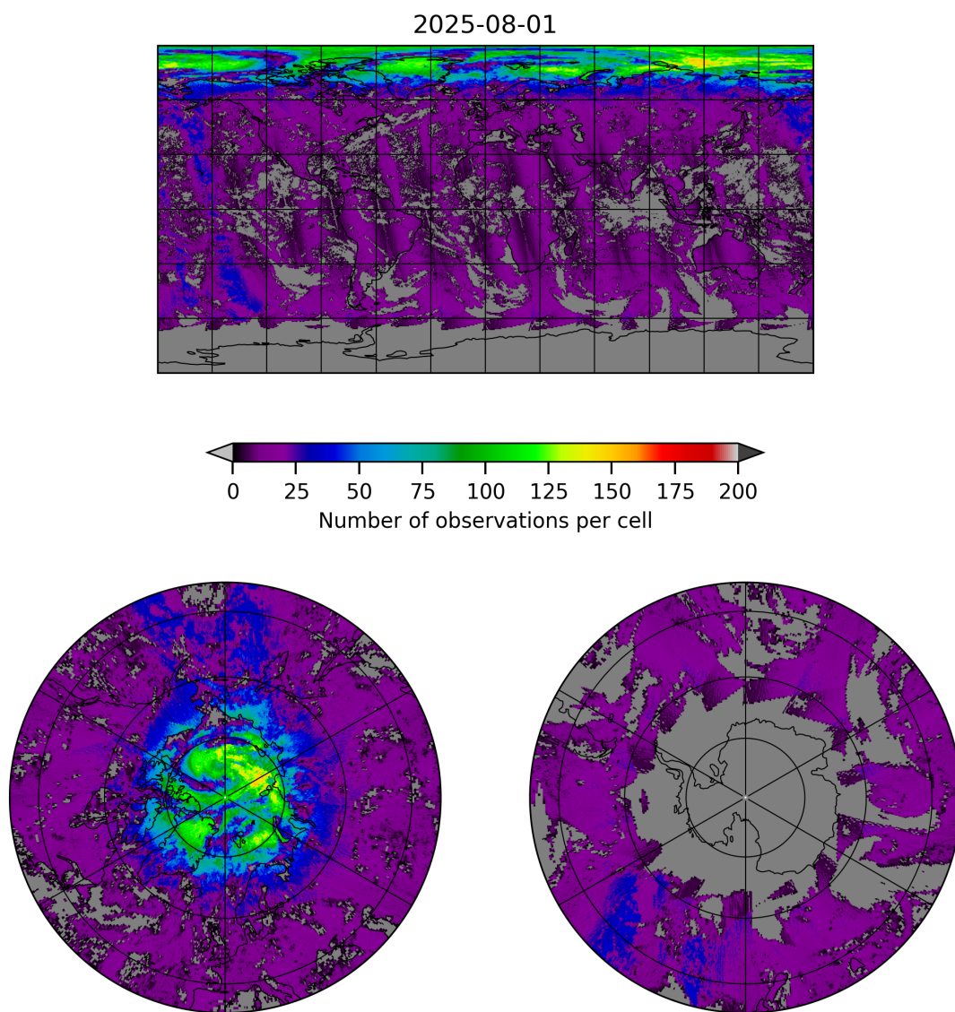
Figure 8: Map of the number of observations for 2025-07-31 to 2025-08-02
