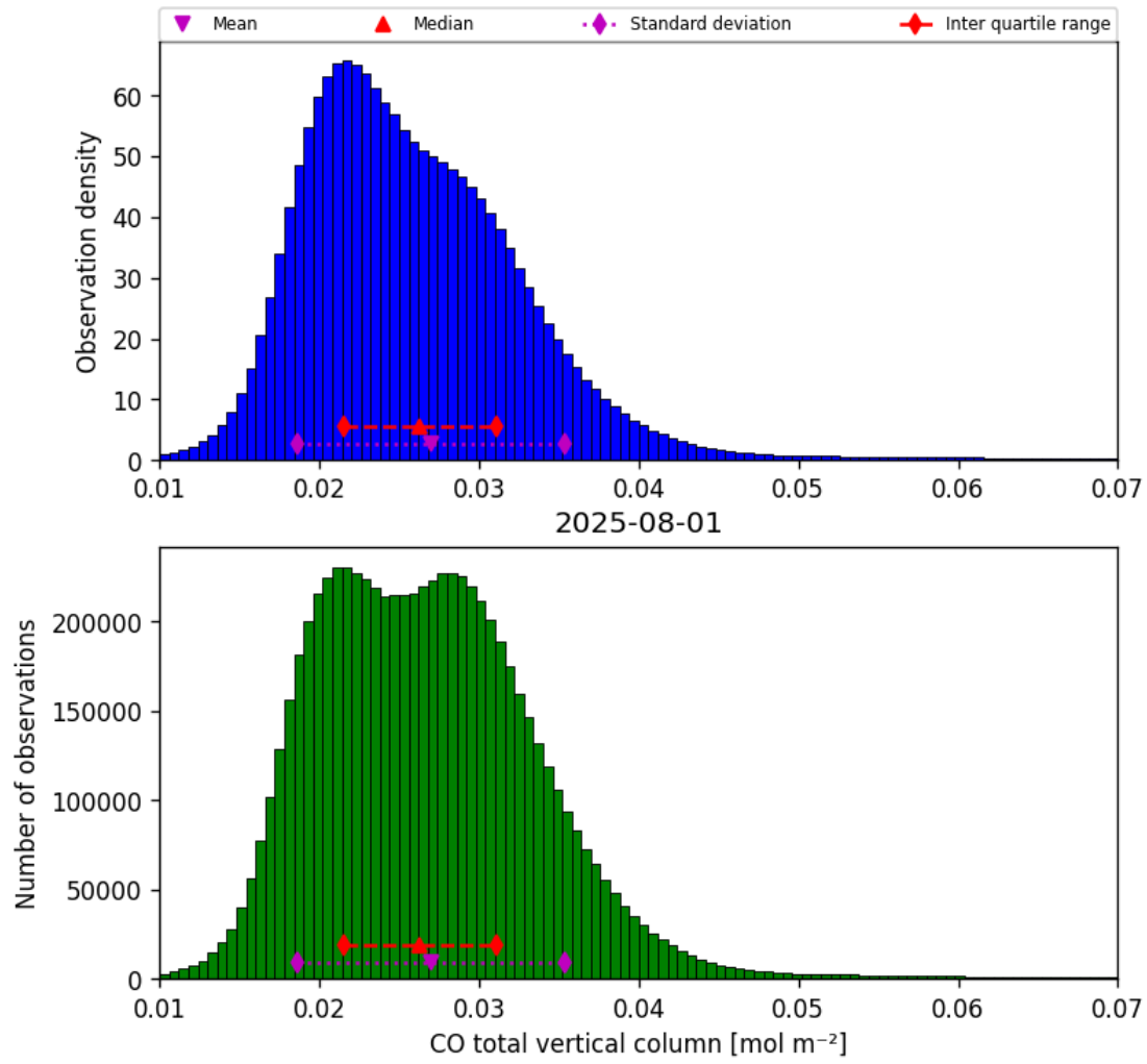
Figure 18: Histogram of “CO total vertical column” for 2025-07-31 to 2025-08-02
