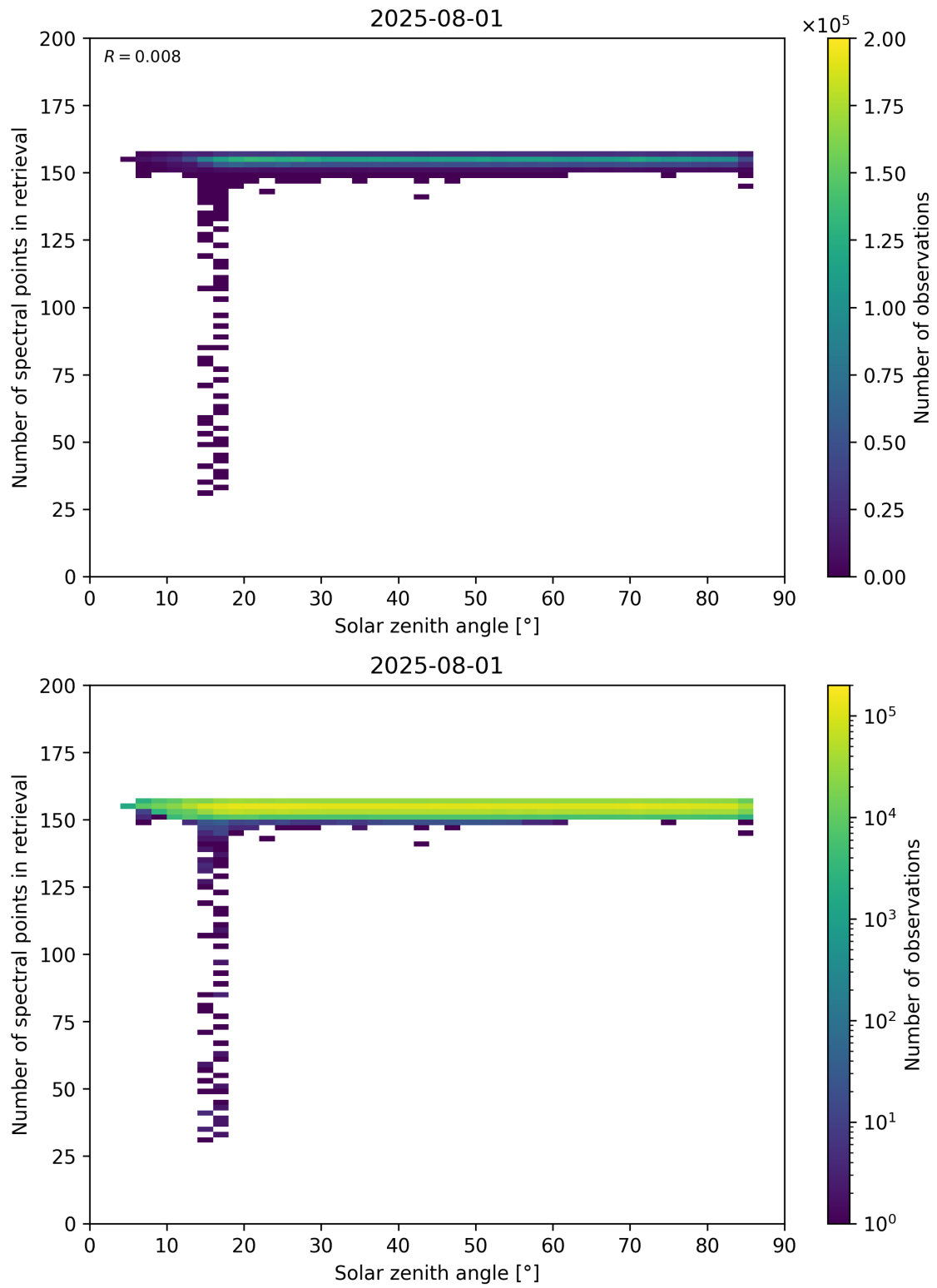
Figure 68: Scatter density plot of “Solar zenith angle” against “Number of spectral points in retrieval” for 2025-07-31 to 2025-08-02.
