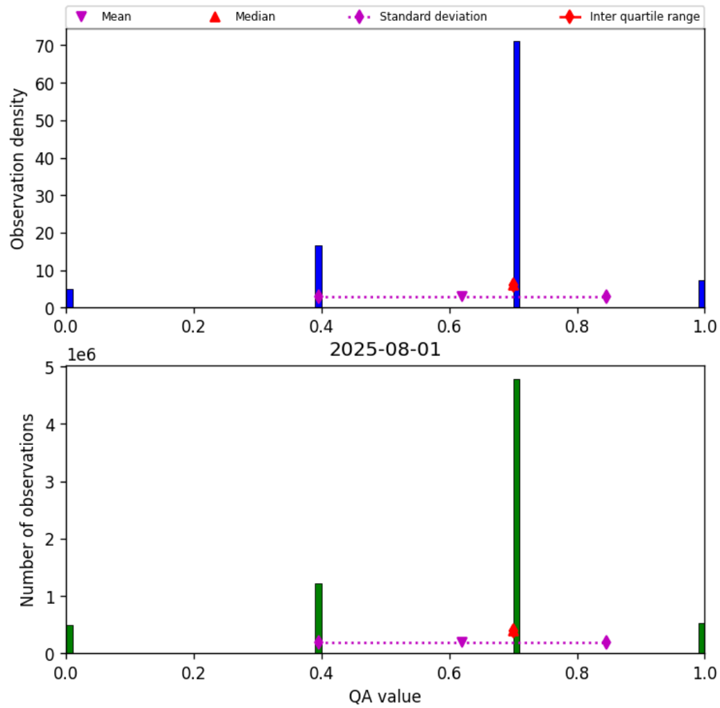
Figure 17: Histogram of “QA value” for 2025-07-31 to 2025-08-02
