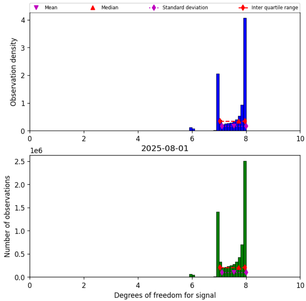
Figure 23: Histogram of “Degrees of freedom for signal” for 2025-07-31 to 2025-08-02
