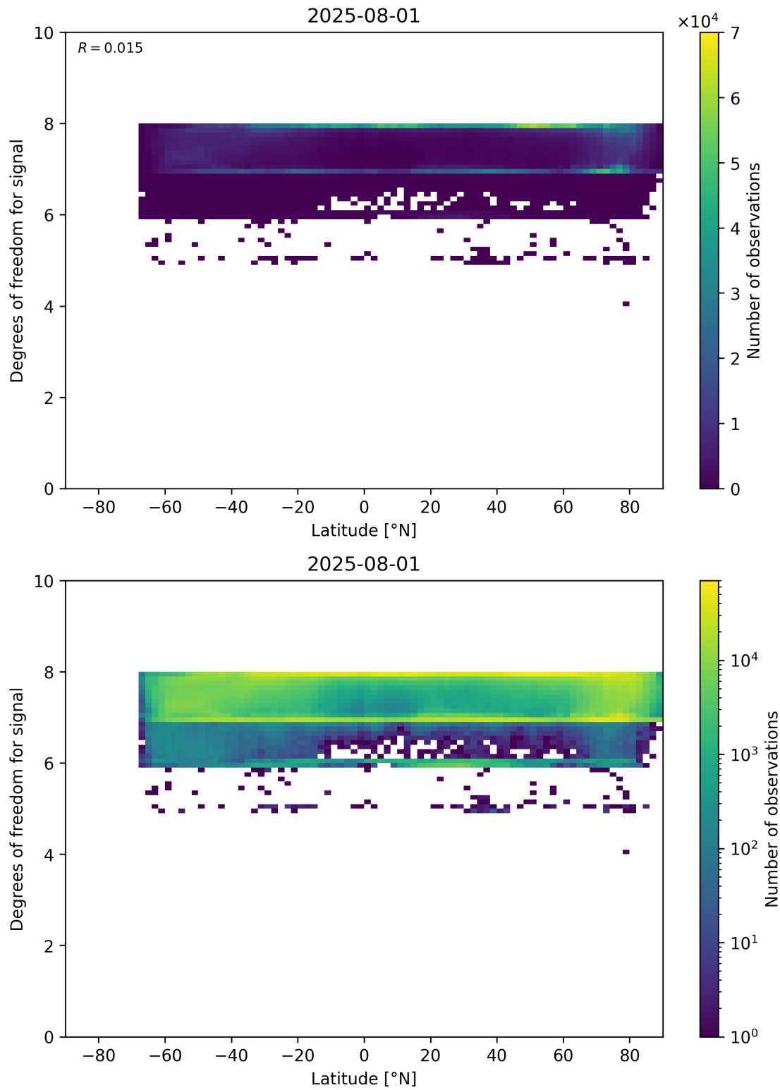
Figure 55: Scatter density plot of “Latitude” against “Degrees of freedom for signal” for 2025-07-31 to 2025-08-02.
