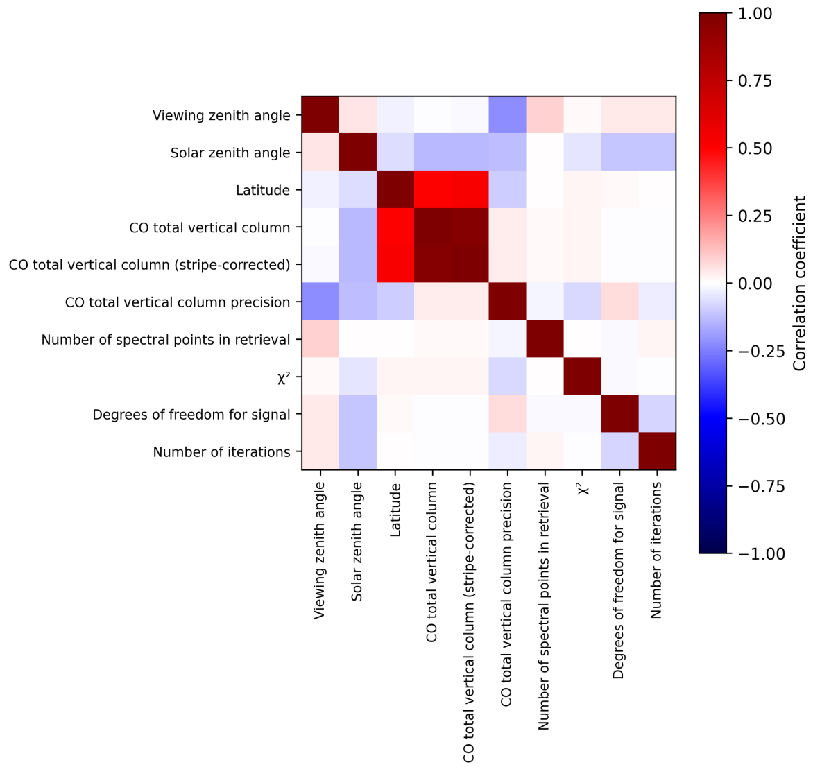
Figure 2: Map of correlation matrix for 2025-07-31 to 2025-08-02.
