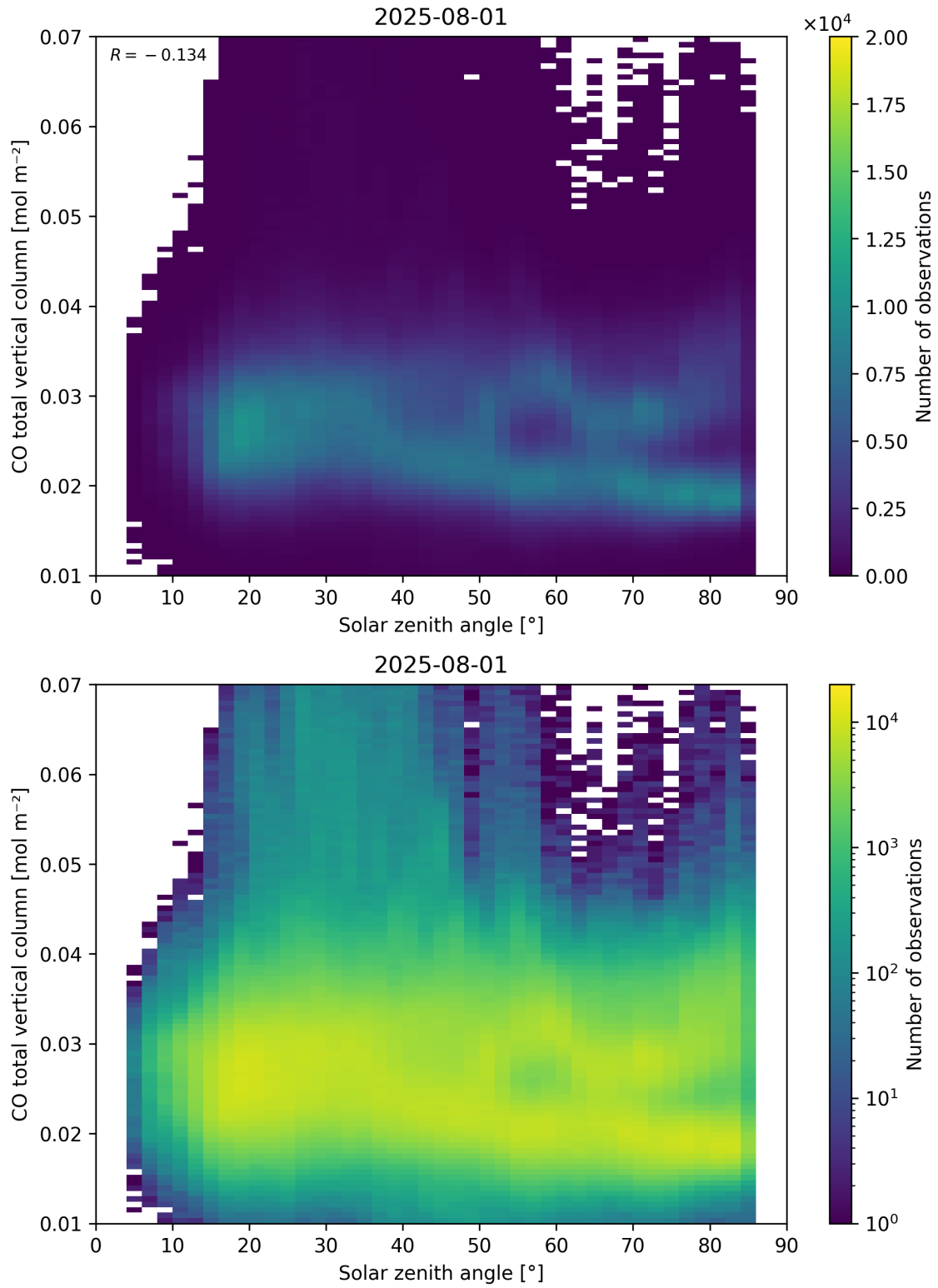
Figure 61: Scatter density plot of “Solar zenith angle” against “CO total vertical column” for 2025-07-31 to 2025-08-02.
