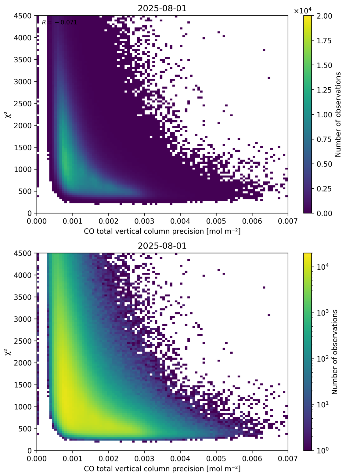
Figure 44: Scatter density plot of “CO total vertical column precision” against “ \chi^2 ” for 2025-07-31 to 2025-08-02.
