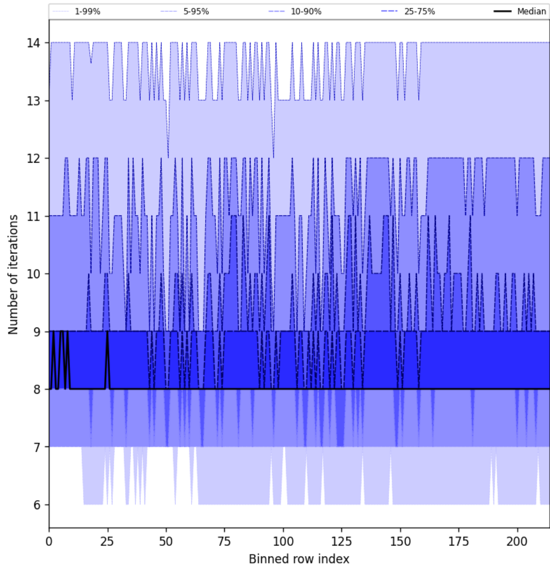
Figure 32: Along track statistics of “Number of iterations” for 2025-07-31 to 2025-08-02
