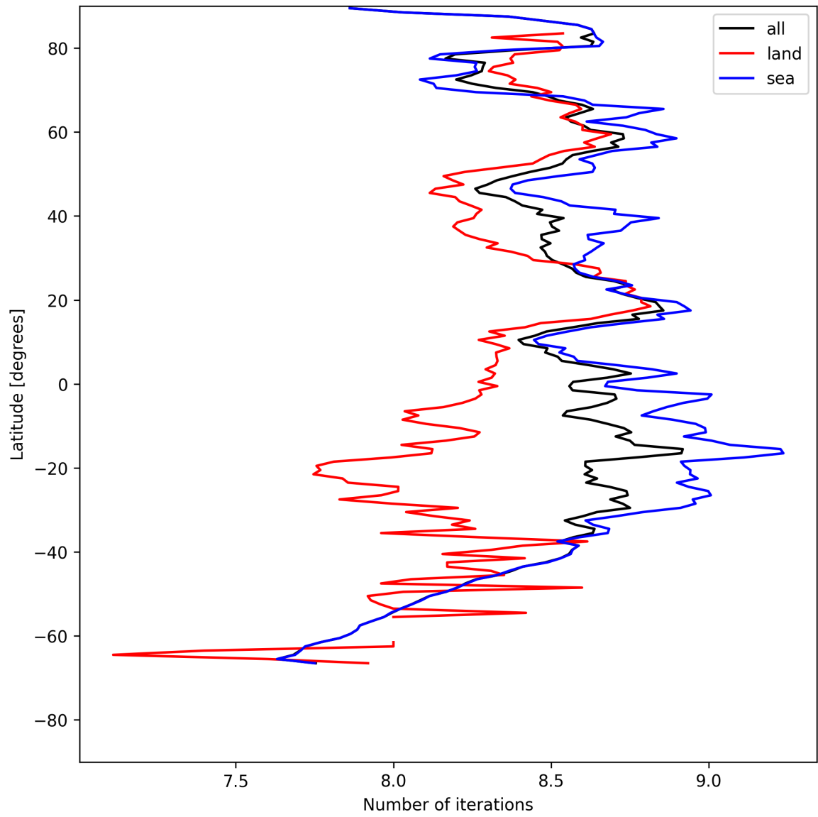
Figure 16: Zonal average of “Number of iterations” for 2025-07-31 to 2025-08-02.
