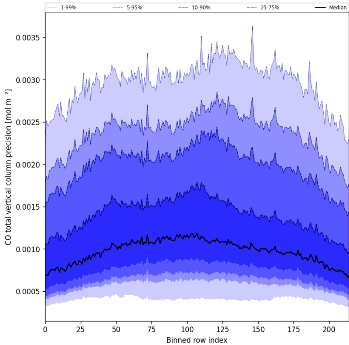
Figure 28: Along track statistics of “CO total vertical column precision” for 2025-07-31 to 2025-08-02
