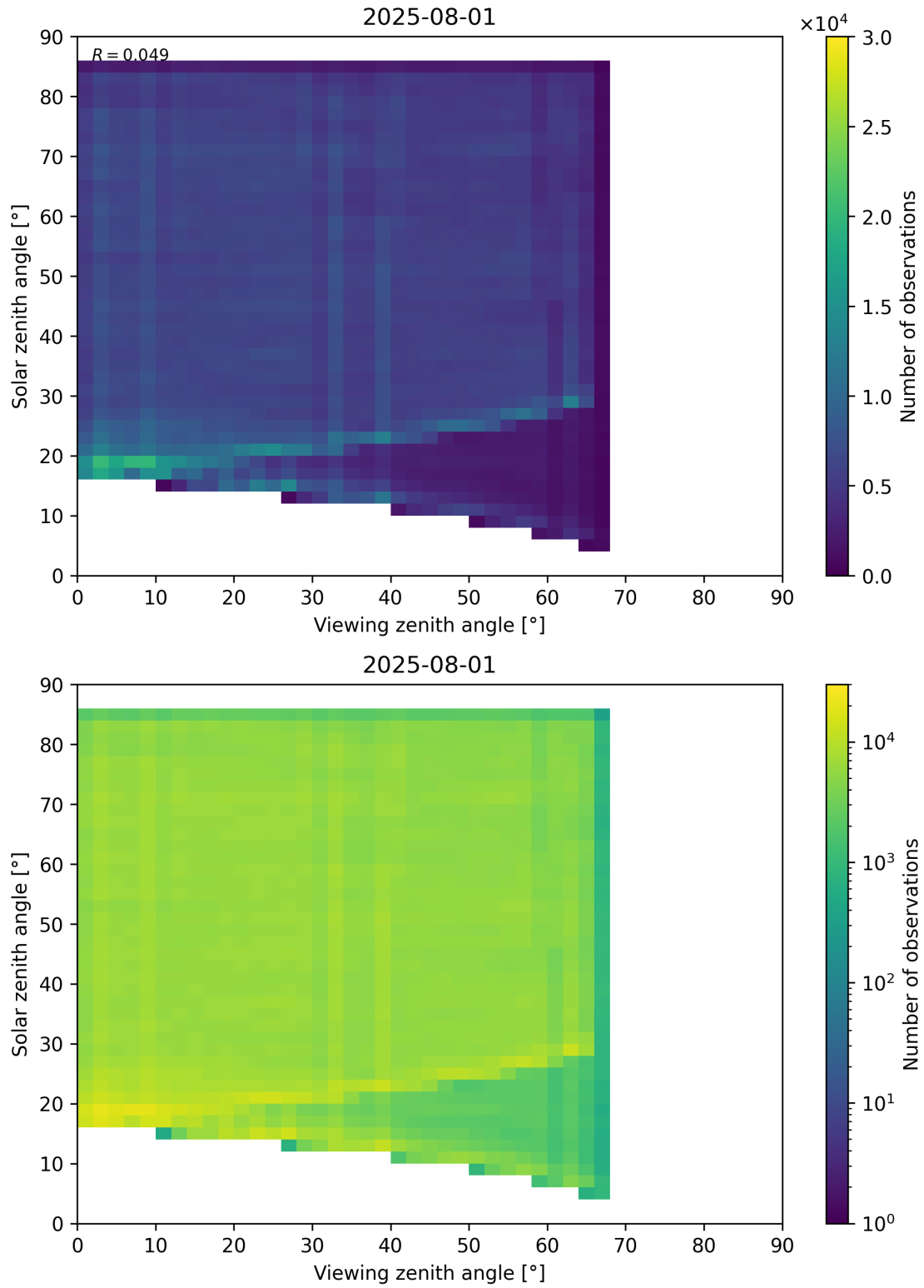
Figure 77: Scatter density plot of “Viewing zenith angle” against “Solar zenith angle” for 2025-07-31 to 2025-08-02.
