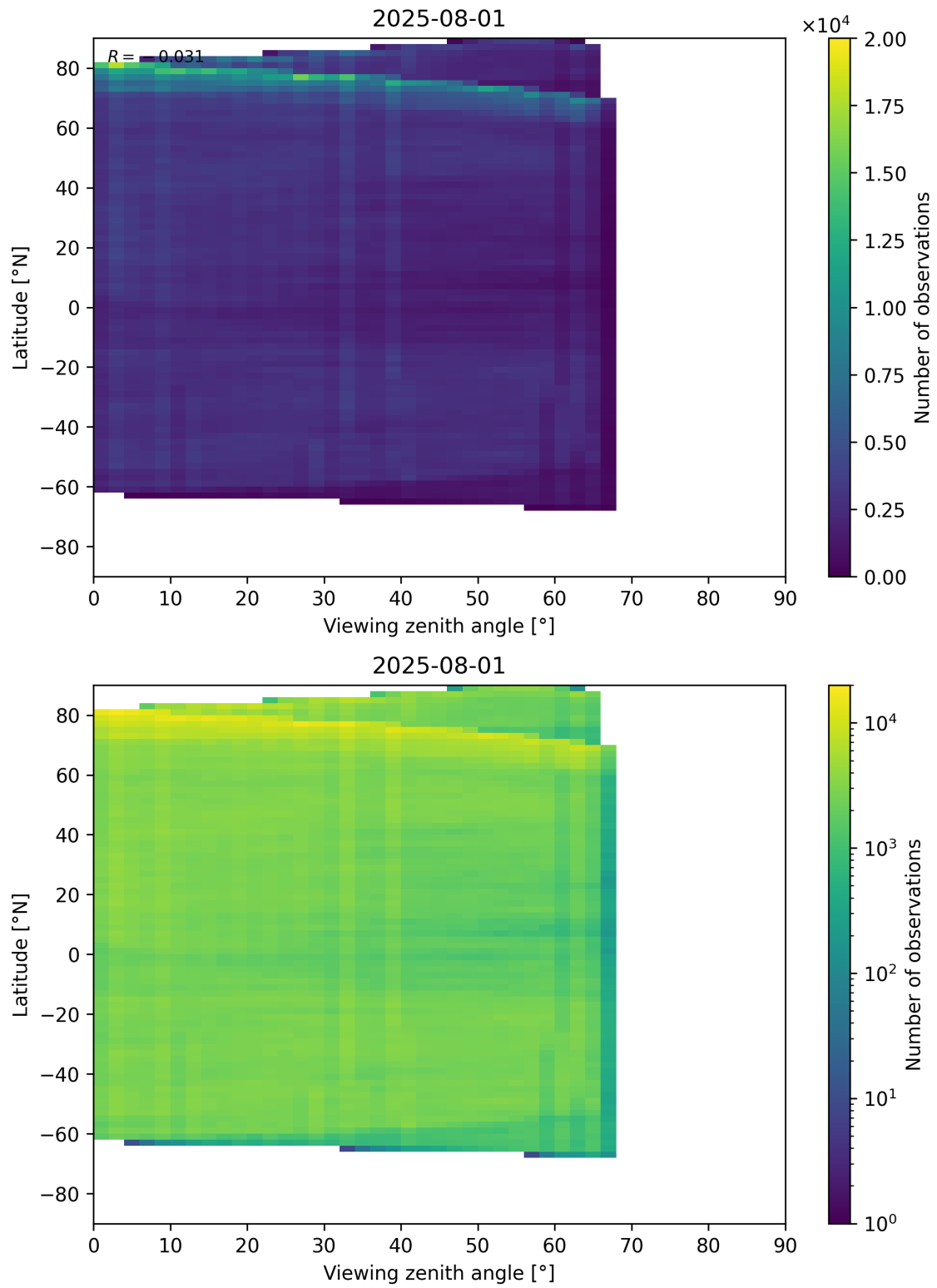
Figure 74: Scatter density plot of “Viewing zenith angle” against “Latitude” for 2025-07-31 to 2025-08-02.
