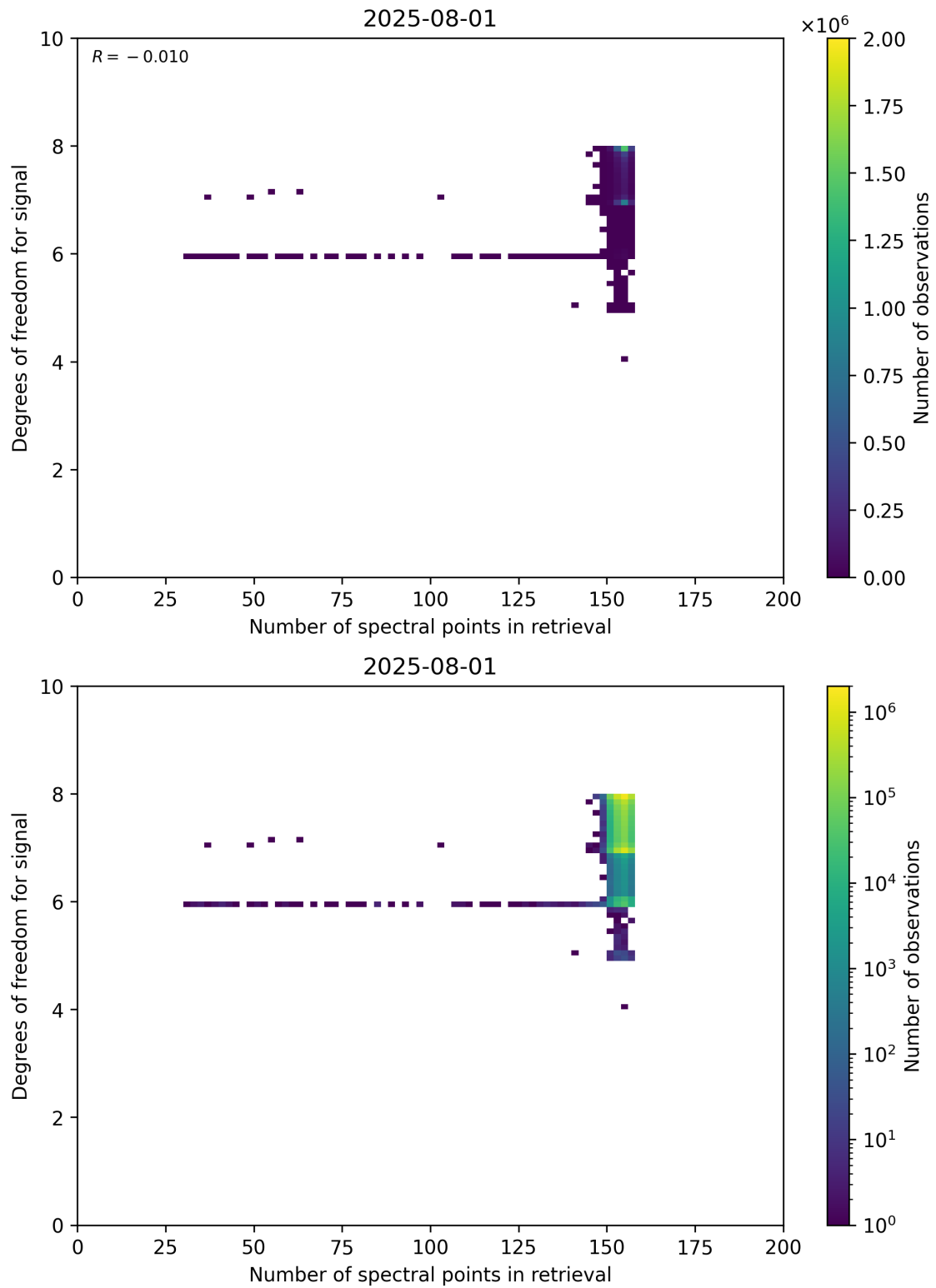
Figure 59: Scatter density plot of “Number of spectral points in retrieval” against “Degrees of freedom for signal” for 2025-07-31 to 2025-08-02.
