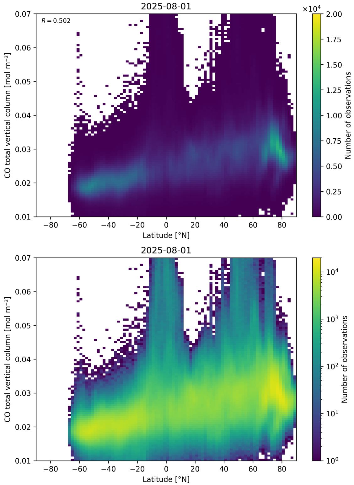
Figure 51: Scatter density plot of “Latitude” against “CO total vertical column” for 2025-07-31 to 2025-08-02.
