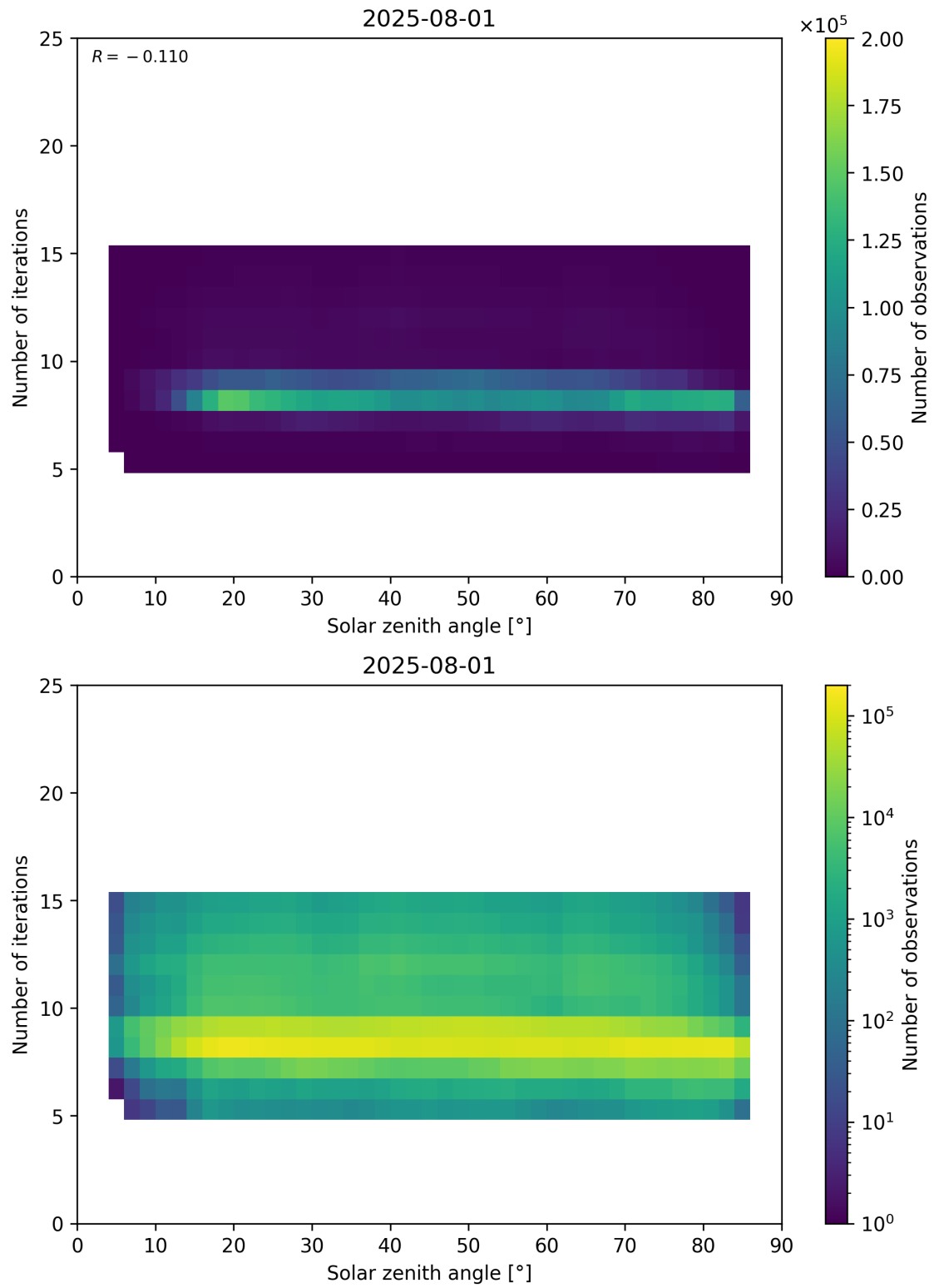
Figure 67: Scatter density plot of “Solar zenith angle” against “Number of iterations” for 2025-07-31 to 2025-08-02.
