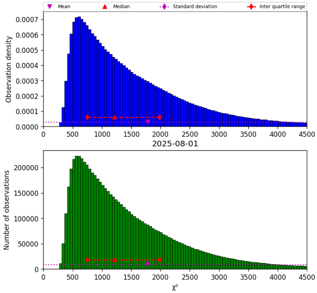
Figure 22: Histogram of “ \chi^2 ” for 2025-07-31 to 2025-08-02
