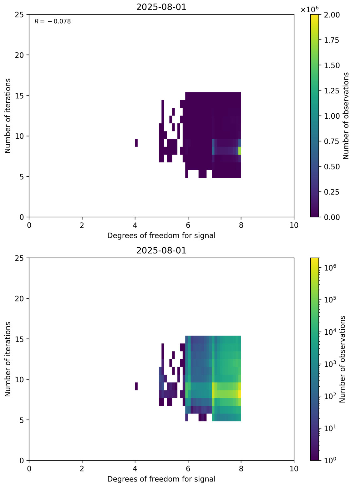
Figure 50: Scatter density plot of “Degrees of freedom for signal” against “Number of iterations” for 2025-07-31 to 2025-08-02.
