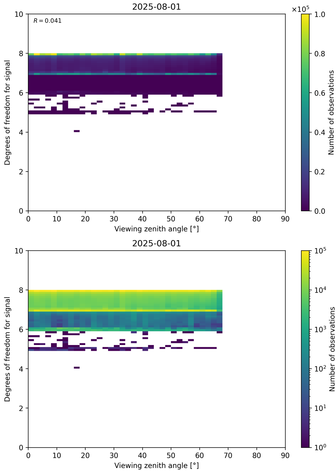
Figure 73: Scatter density plot of “Viewing zenith angle” against “Degrees of freedom for signal” for 2025-07-31 to 2025-08-02.
