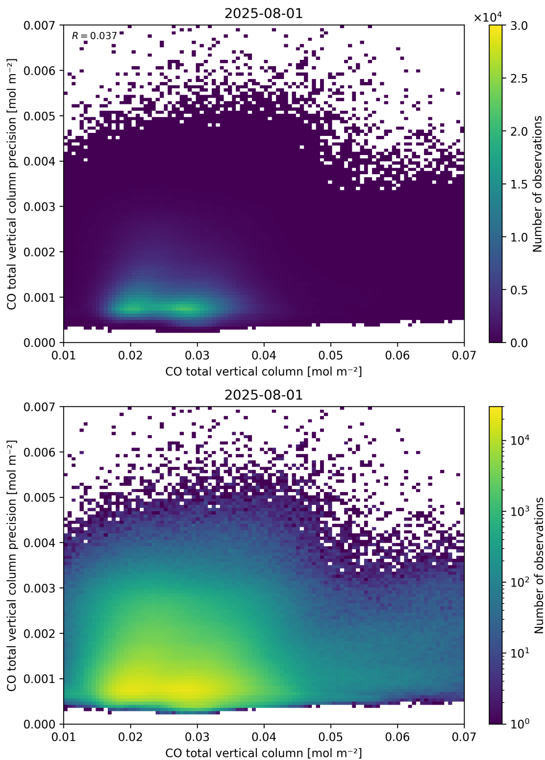
Figure 34: Scatter density plot of “CO total vertical column” against “CO total vertical column precision” for 2025-07-31 to 2025-08-02.
