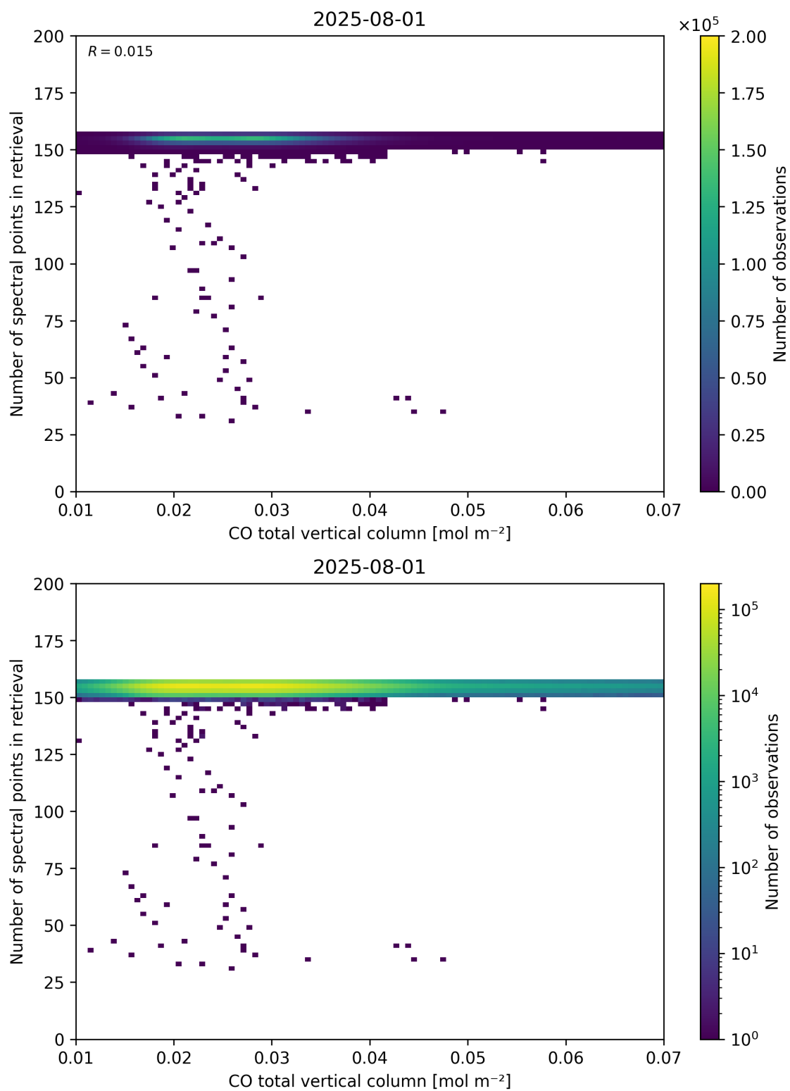
Figure 43: Scatter density plot of “CO total vertical column” against “Number of spectral points in retrieval” for 2025-07-31 to 2025-08-02.
