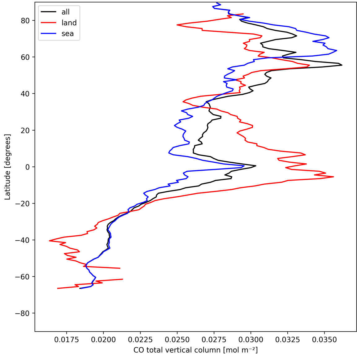
Figure 10: Zonal average of “CO total vertical column” for 2025-07-31 to 2025-08-02.
