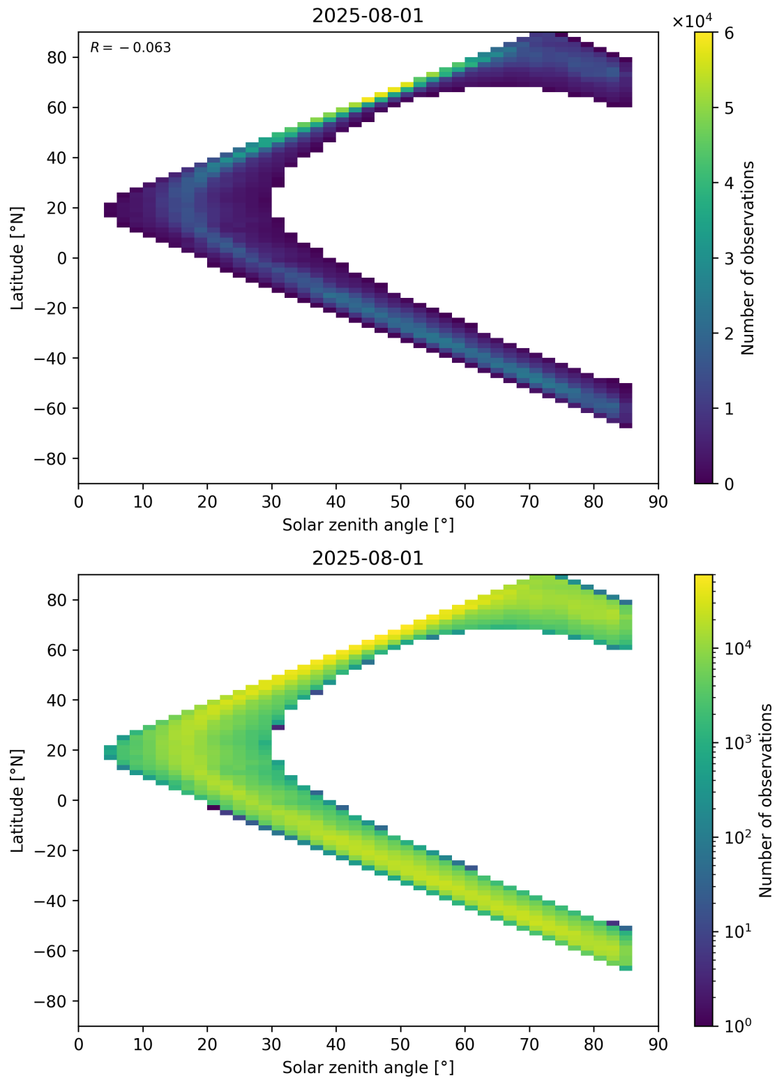
Figure 66: Scatter density plot of “Solar zenith angle” against “Latitude” for 2025-07-31 to 2025-08-02.
