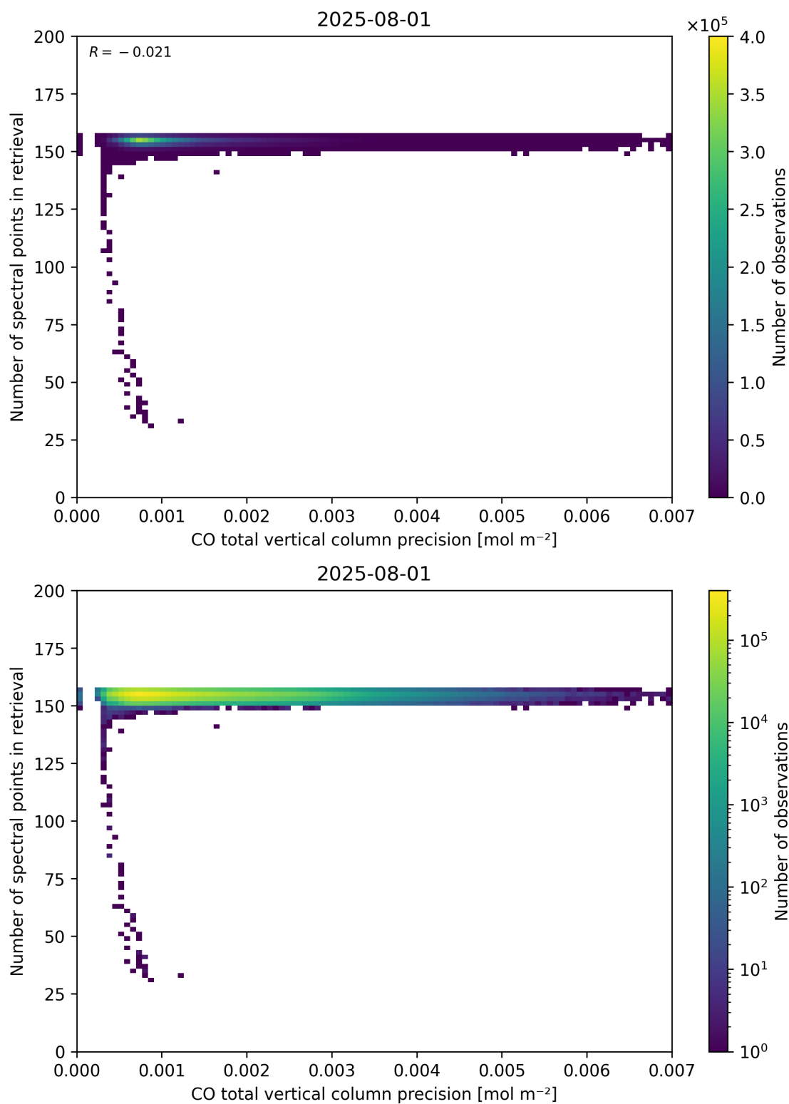
Figure 47: Scatter density plot of “CO total vertical column precision” against “Number of spectral points in retrieval” for 2025-07-31 to 2025-08-02.
