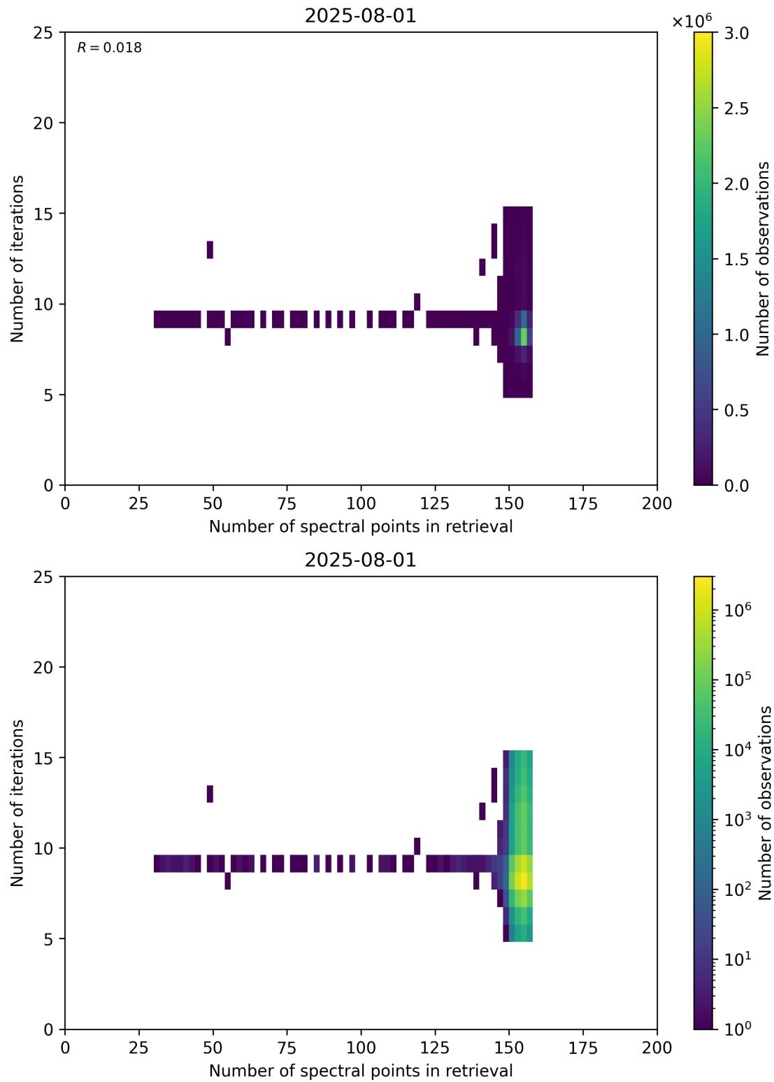
Figure 60: Scatter density plot of “Number of spectral points in retrieval” against “Number of iterations” for 2025-07-31 to 2025-08-02.
