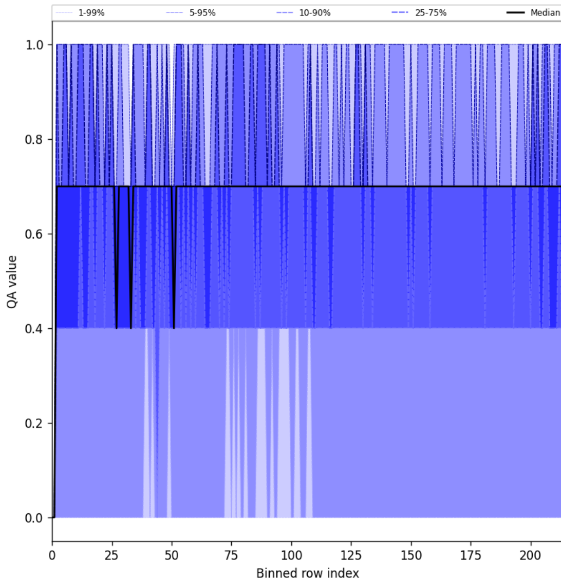
Figure 25: Along track statistics of “QA value” for 2025-07-31 to 2025-08-02
