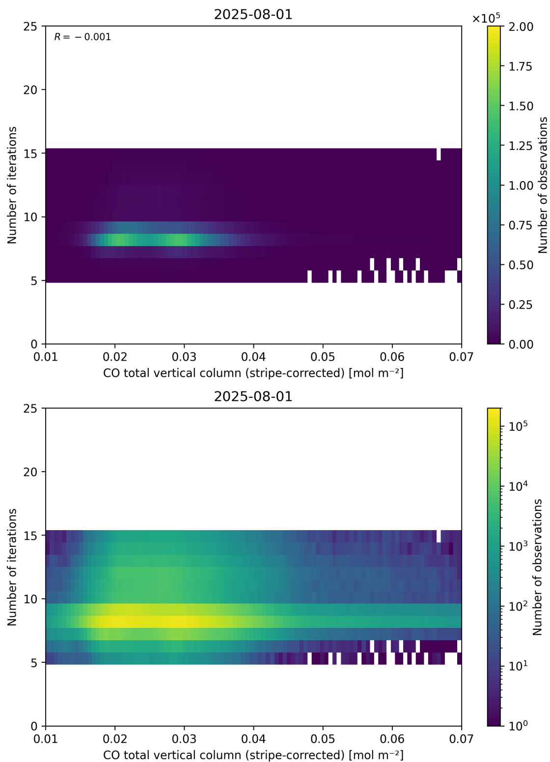
Figure 39: Scatter density plot of “CO total vertical column (stripe-corrected)” against “Number of iterations” for 2025-07-31 to 2025-08-02.
