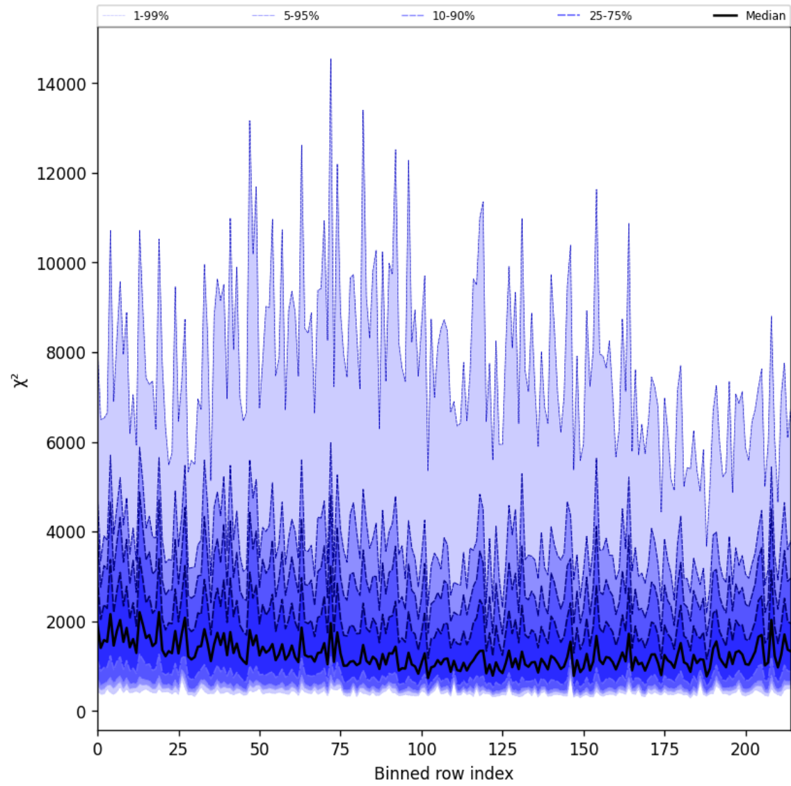
Figure 30: Along track statistics of “ \chi^2 ” for 2025-07-31 to 2025-08-02
