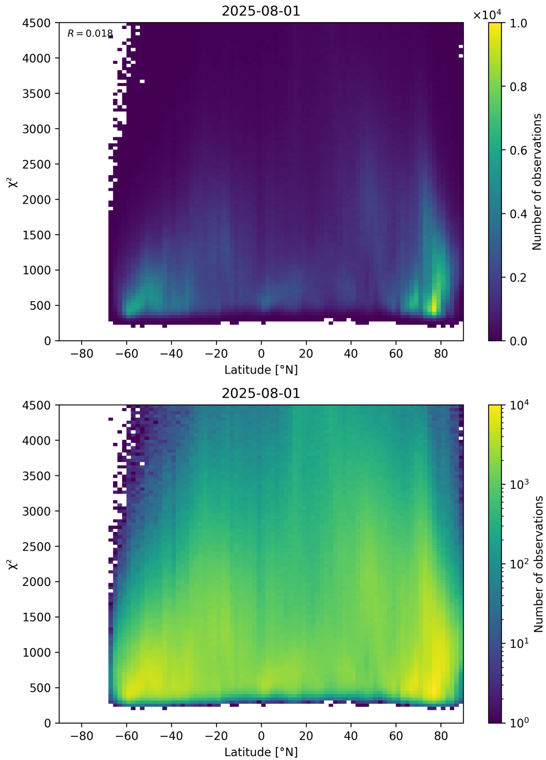
Figure 54: Scatter density plot of “Latitude” against “ \chi^2 ” for 2025-07-31 to 2025-08-02.
