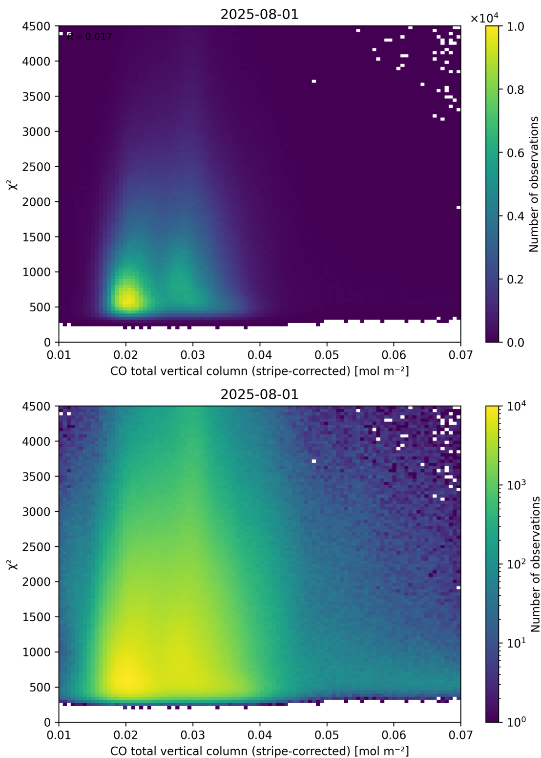
Figure 37: Scatter density plot of “CO total vertical column (stripe-corrected)” against “ \chi^2 ” for 2025-07-31 to 2025-08-02.
