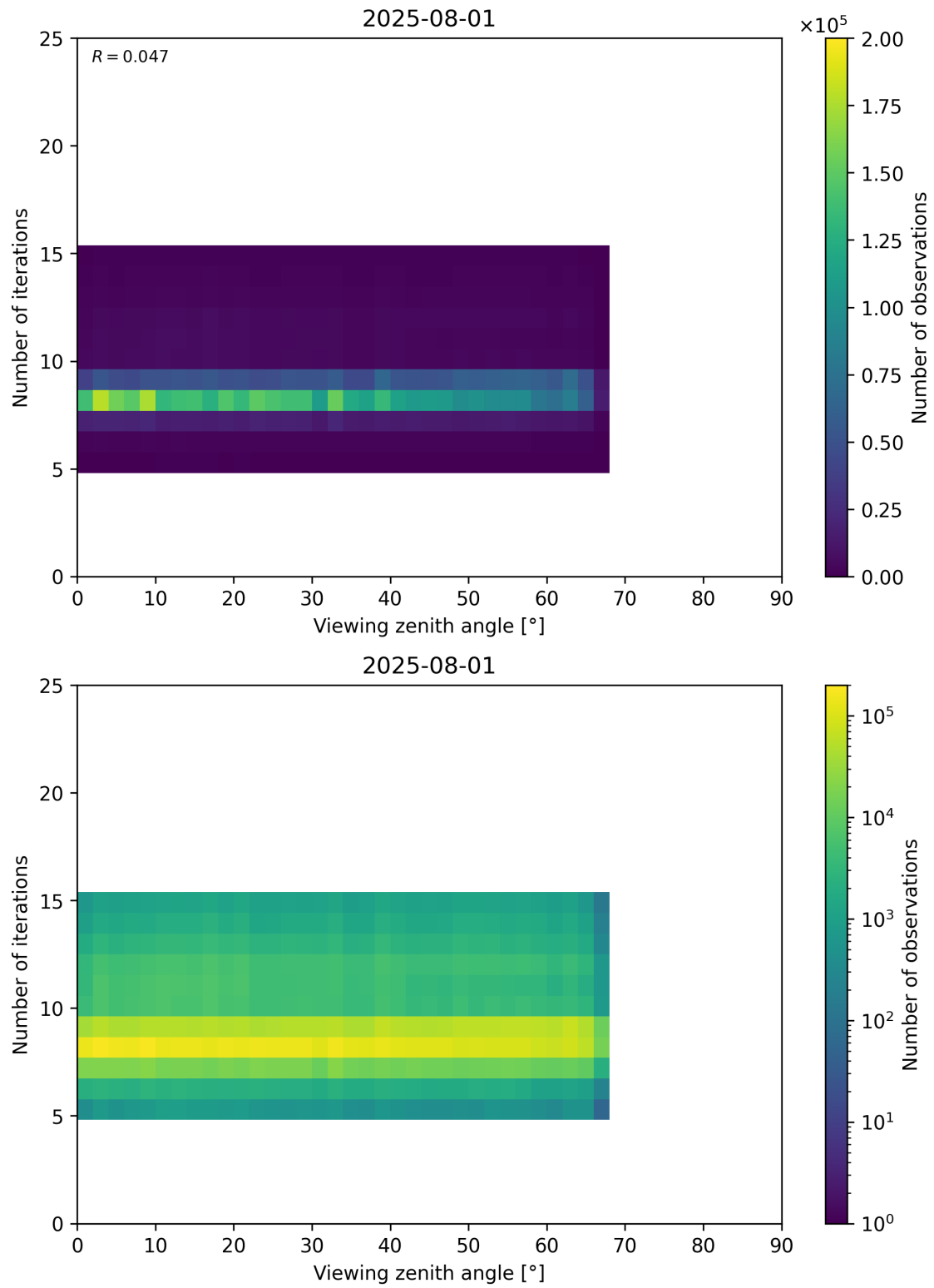
Figure 75: Scatter density plot of “Viewing zenith angle” against “Number of iterations” for 2025-07-31 to 2025-08-02.
