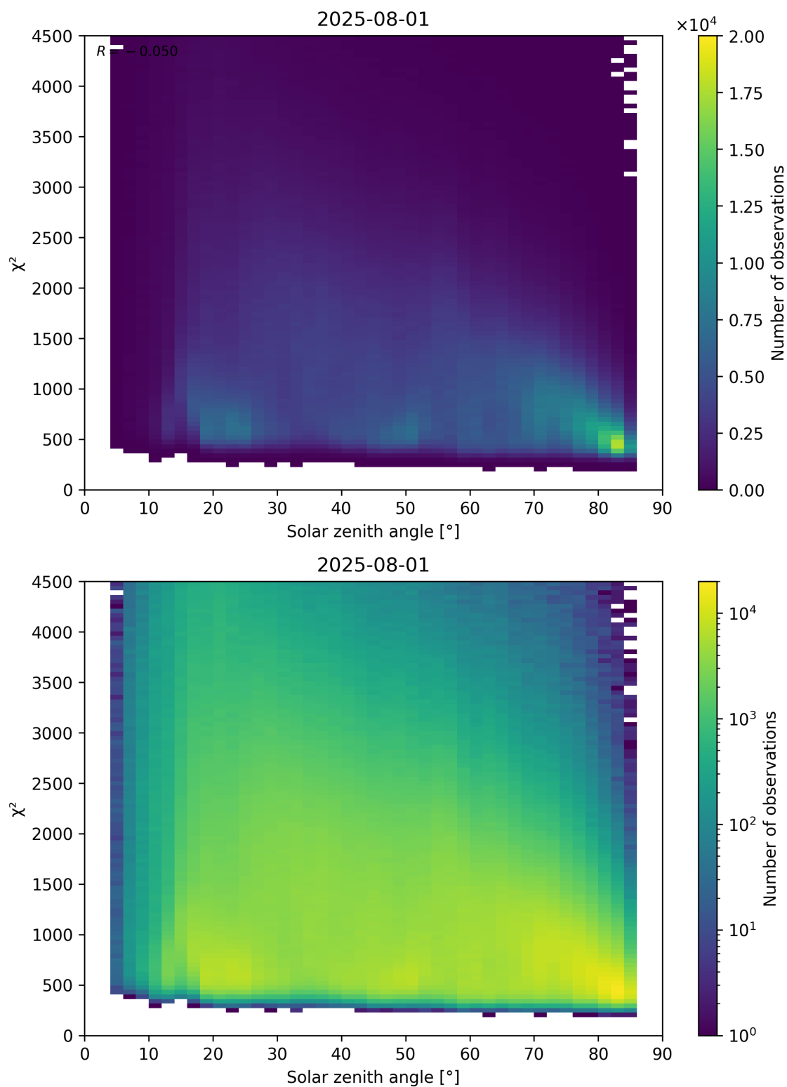
Figure 64: Scatter density plot of “Solar zenith angle” against “ \chi^2 ” for 2025-07-31 to 2025-08-02.
