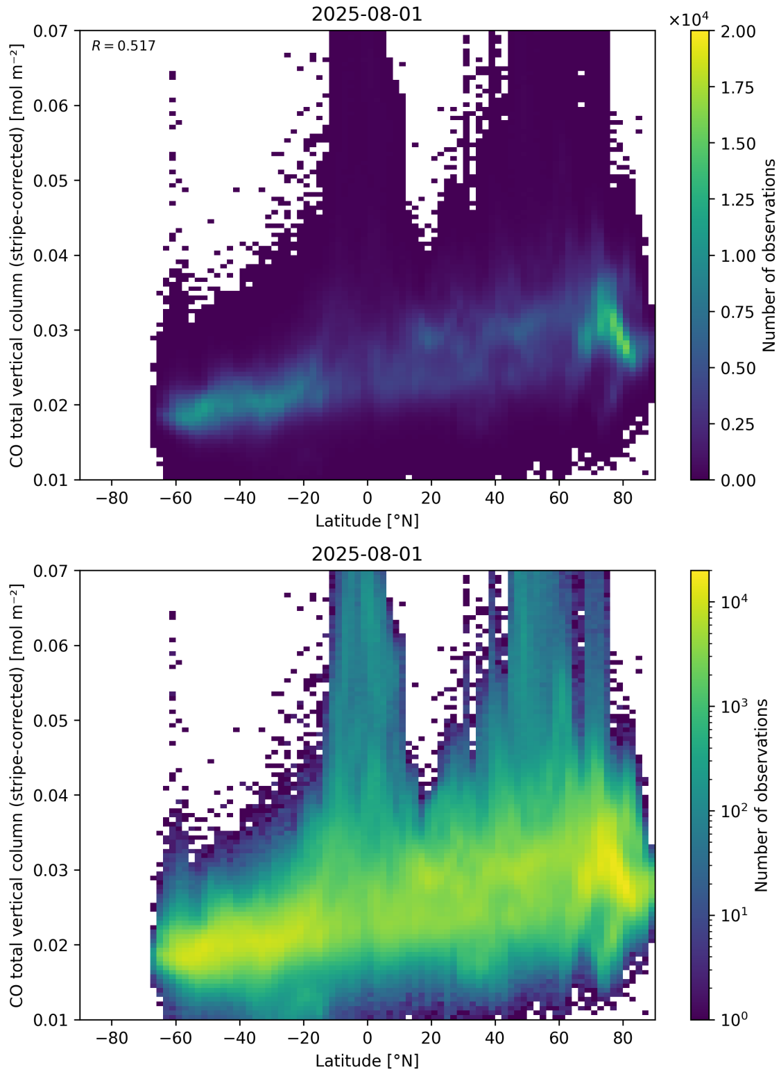
Figure 52: Scatter density plot of “Latitude” against “CO total vertical column (stripe-corrected)” for 2025-07-31 to 2025-08-02.
