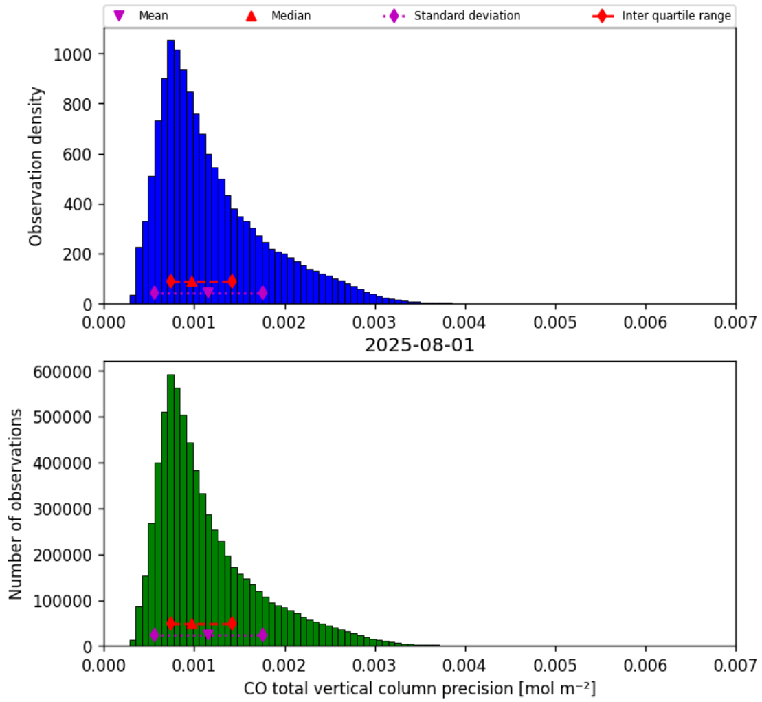
Figure 20: Histogram of “CO total vertical column precision” for 2025-07-31 to 2025-08-02
