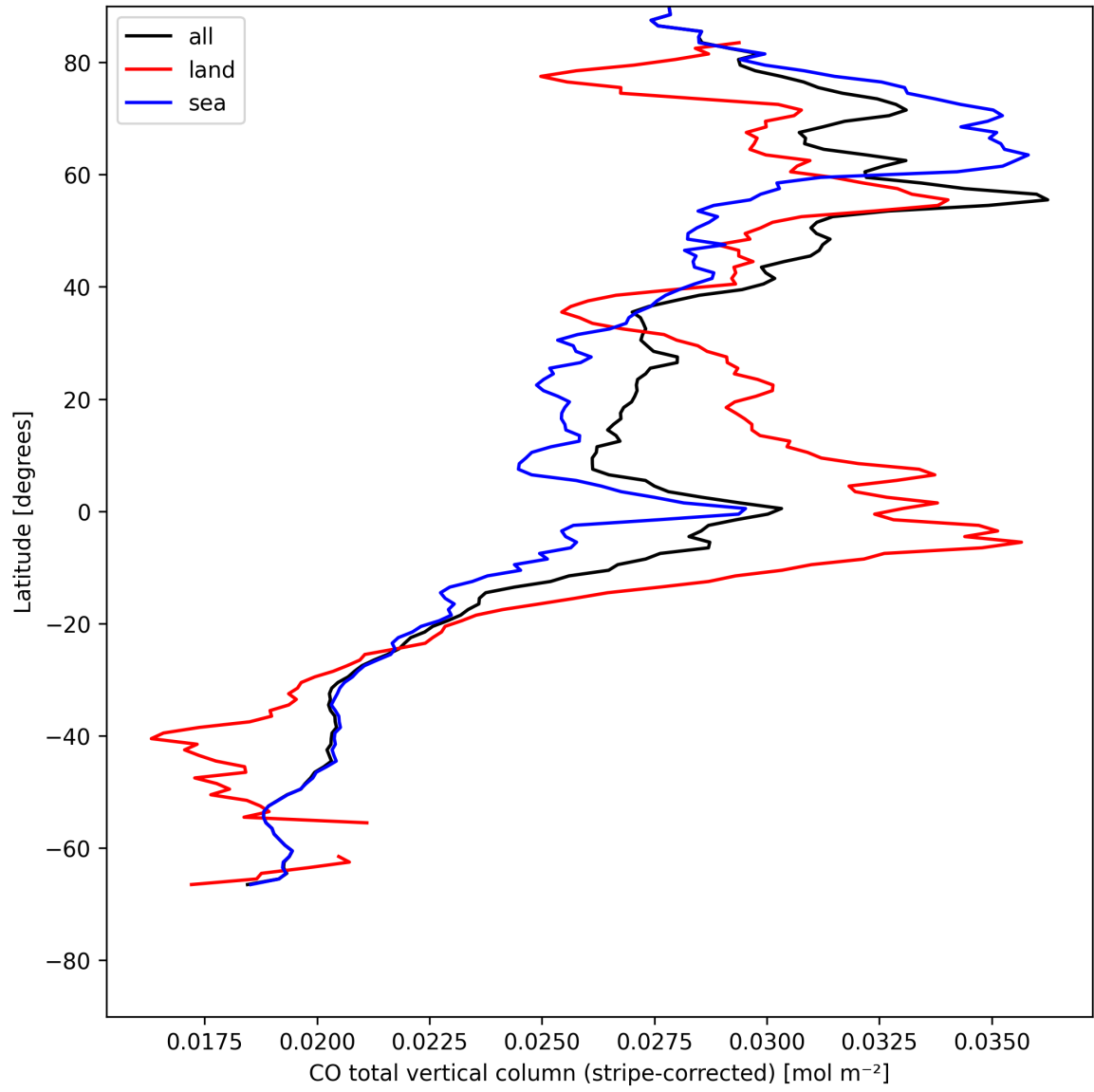
Figure 11: Zonal average of “CO total vertical column (stripe-corrected)” for 2025-07-31 to 2025-08-02.
