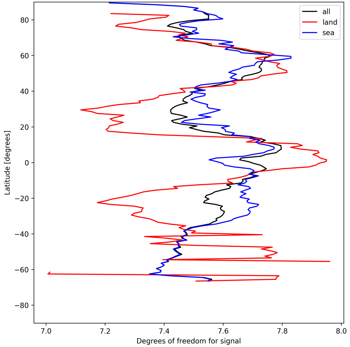
Figure 15: Zonal average of “Degrees of freedom for signal” for 2025-07-31 to 2025-08-02.
