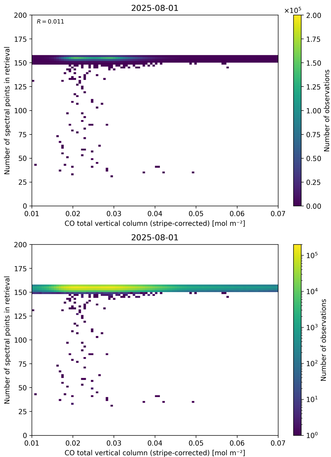
Figure 40: Scatter density plot of “CO total vertical column (stripe-corrected)” against “Number of spectral points in retrieval” for 2025-07-31 to 2025-08-02.
