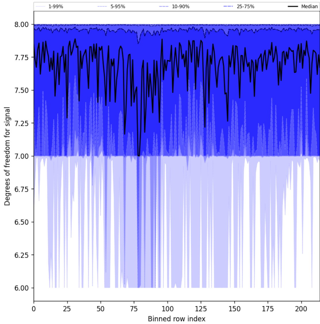
Figure 31: Along track statistics of “Degrees of freedom for signal” for 2025-07-31 to 2025-08-02
