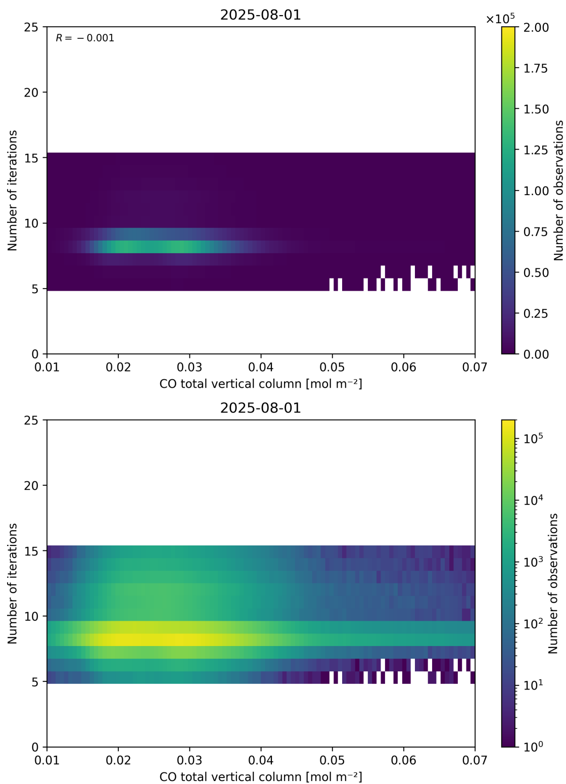
Figure 42: Scatter density plot of “CO total vertical column” against “Number of iterations” for 2025-07-31 to 2025-08-02.
