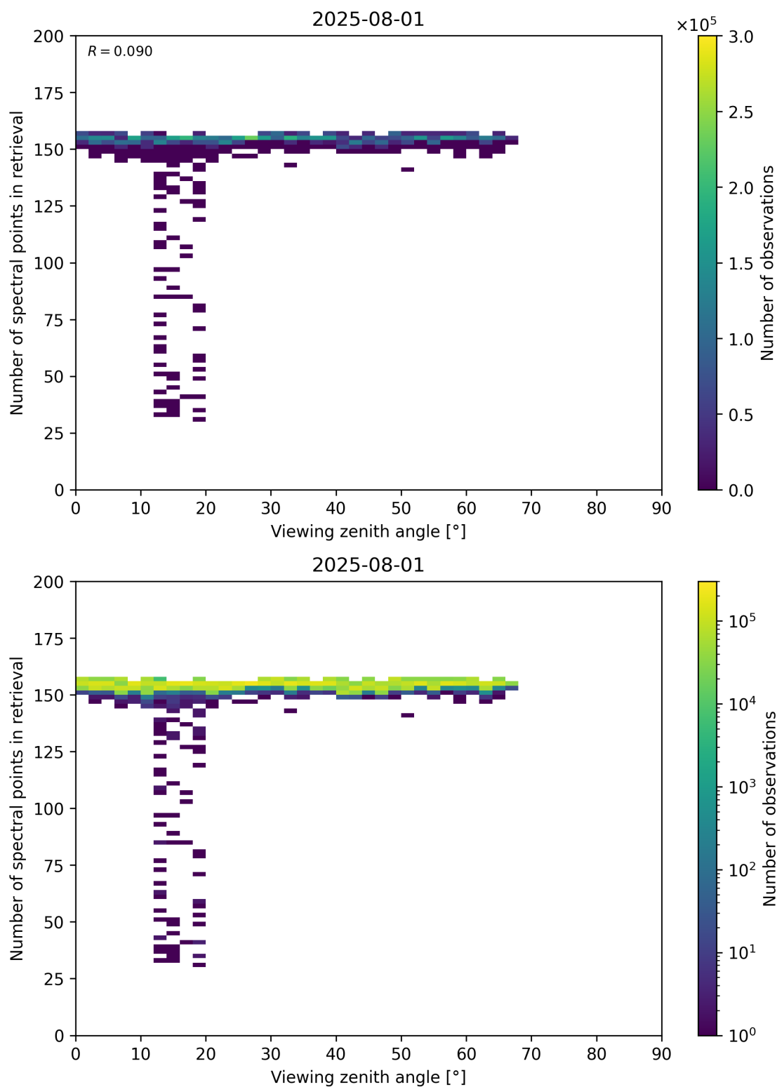
Figure 76: Scatter density plot of “Viewing zenith angle” against “Number of spectral points in retrieval” for 2025-07-31 to 2025-08-02.
