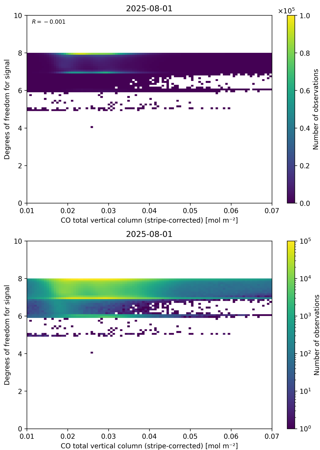
Figure 38: Scatter density plot of “CO total vertical column (stripe-corrected)” against “Degrees of freedom for signal” for 2025-07-31 to 2025-08-02.
