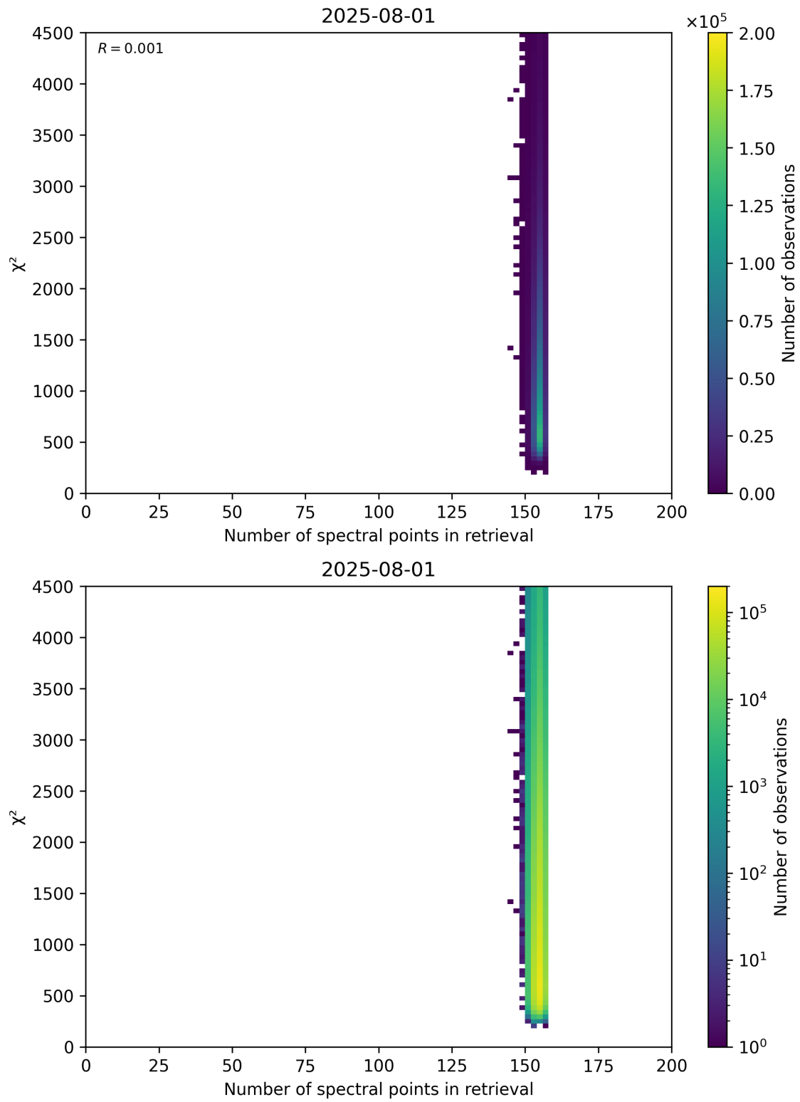
Figure 58: Scatter density plot of “Number of spectral points in retrieval” against “ \chi^2 ” for 2025-07-31 to 2025-08-02.
