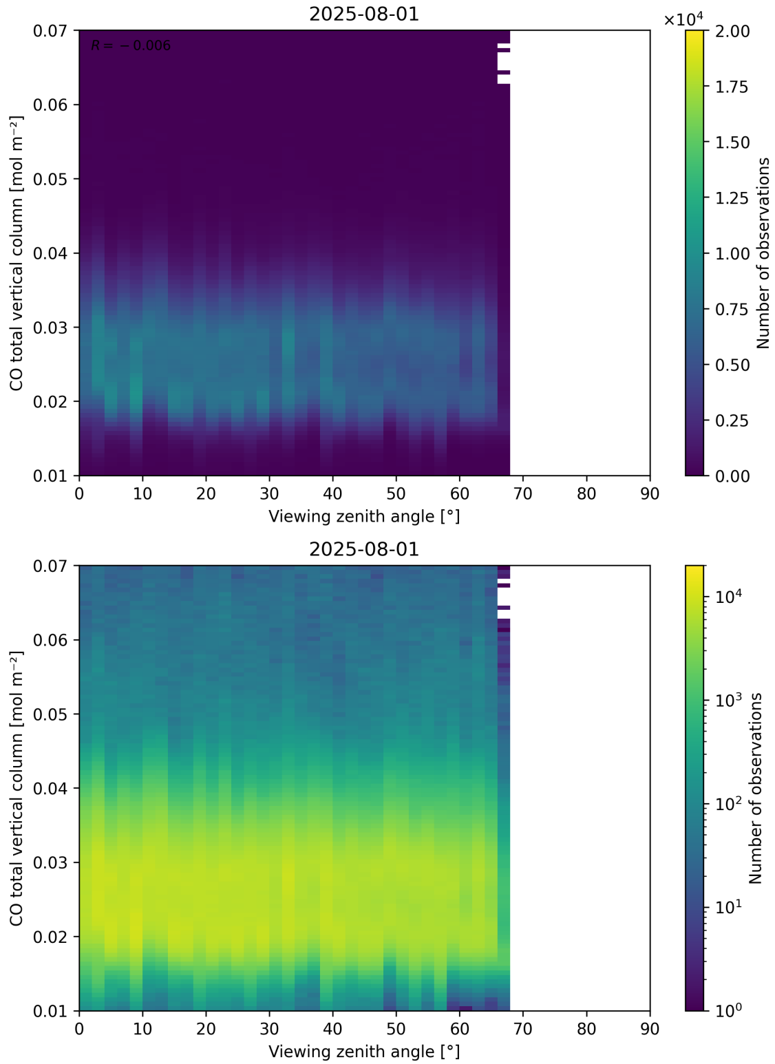
Figure 69: Scatter density plot of “Viewing zenith angle” against “CO total vertical column” for 2025-07-31 to 2025-08-02.
