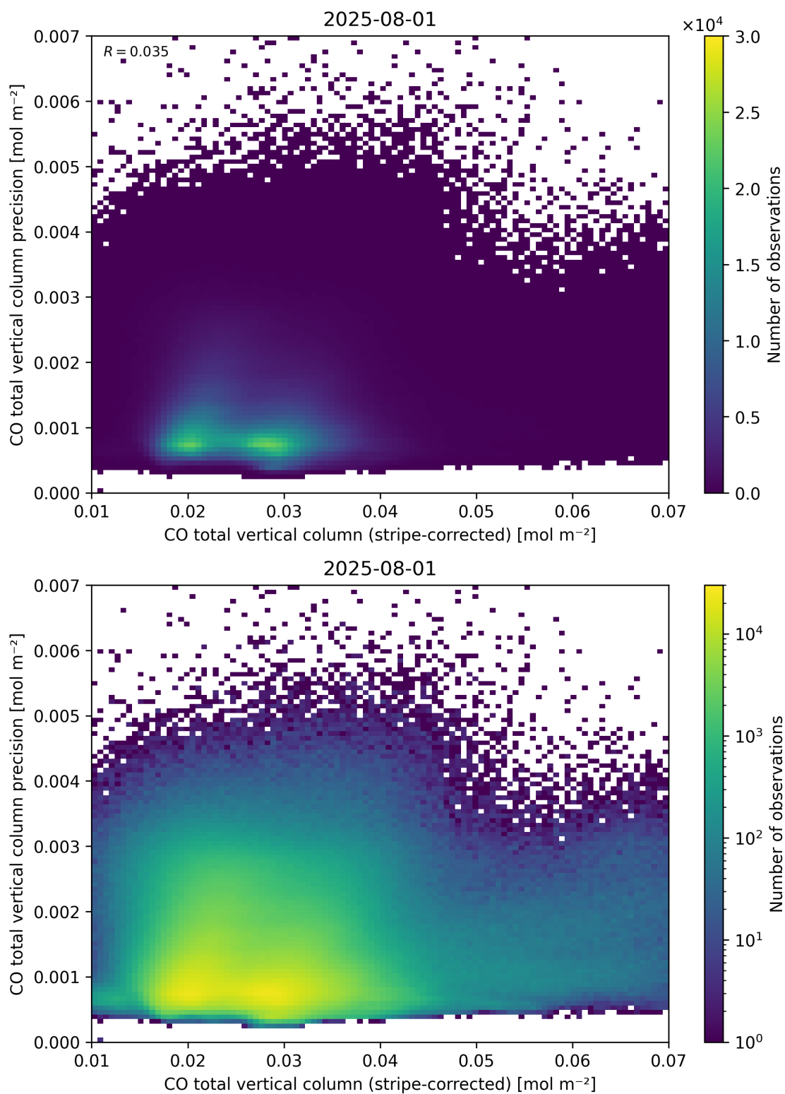
Figure 36: Scatter density plot of “CO total vertical column (stripe-corrected)” against “CO total vertical column precision” for 2025-07-31 to 2025-08-02.
