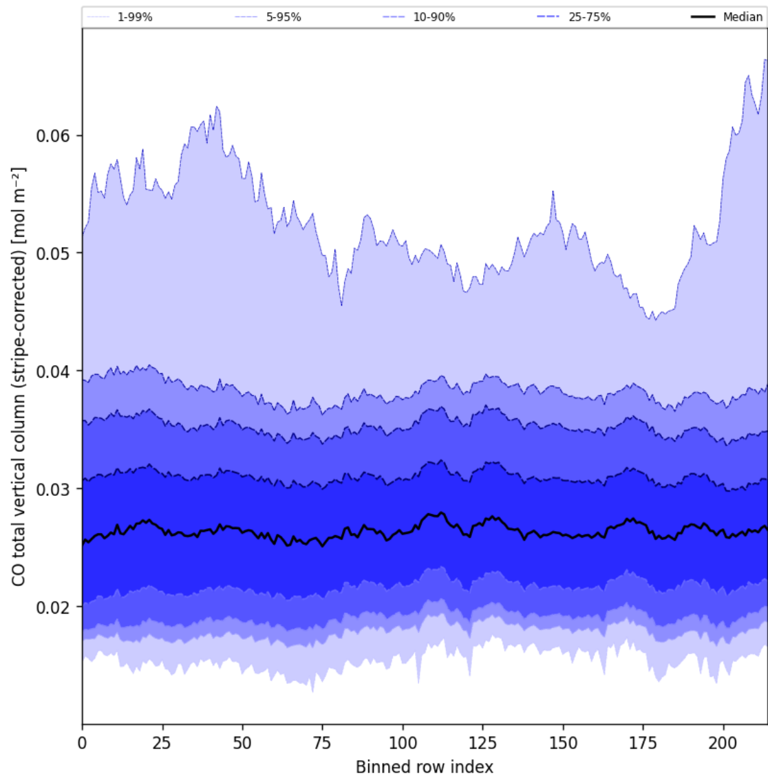
Figure 27: Along track statistics of “CO total vertical column (stripe-corrected)” for 2025-07-31 to 2025-08-02
