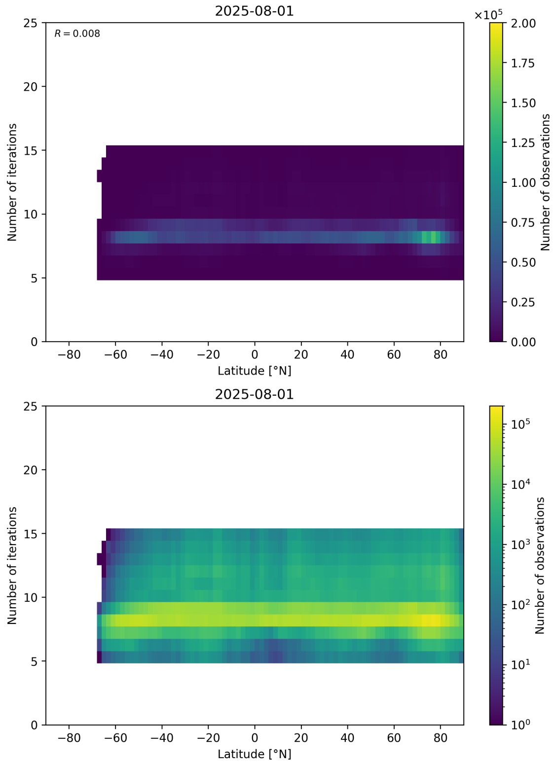
Figure 56: Scatter density plot of “Latitude” against “Number of iterations” for 2025-07-31 to 2025-08-02.
