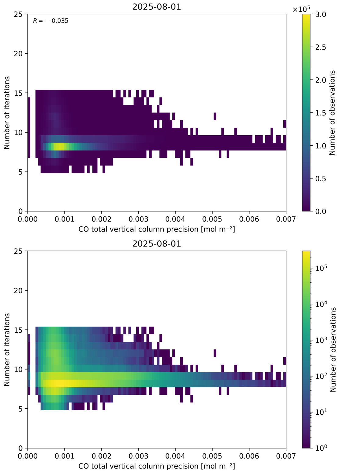
Figure 46: Scatter density plot of “CO total vertical column precision” against “Number of iterations” for 2025-07-31 to 2025-08-02.
