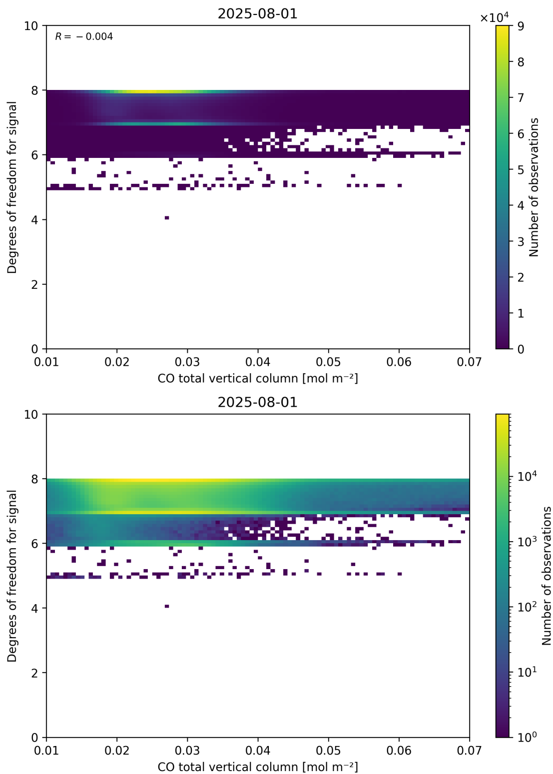
Figure 41: Scatter density plot of “CO total vertical column” against “Degrees of freedom for signal” for 2025-07-31 to 2025-08-02.
