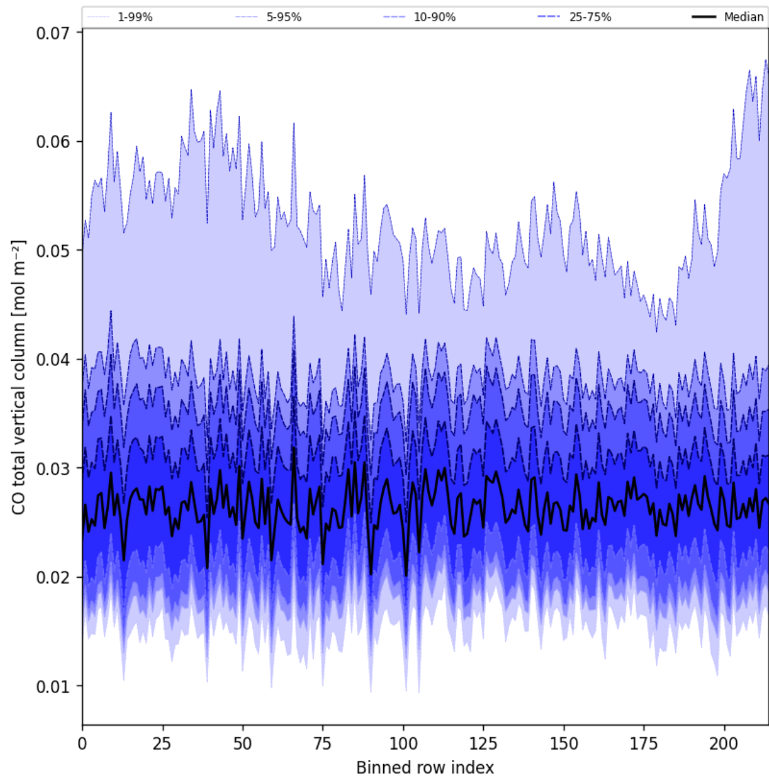
Figure 26: Along track statistics of “CO total vertical column” for 2025-07-31 to 2025-08-02
