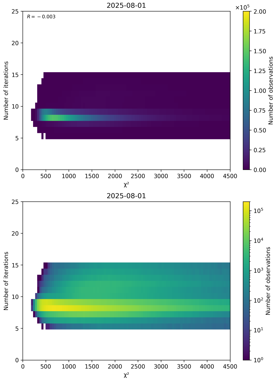
Figure 49: Scatter density plot of “ \chi^2 ” against “Number of iterations” for 2025-07-31 to 2025-08-02.
