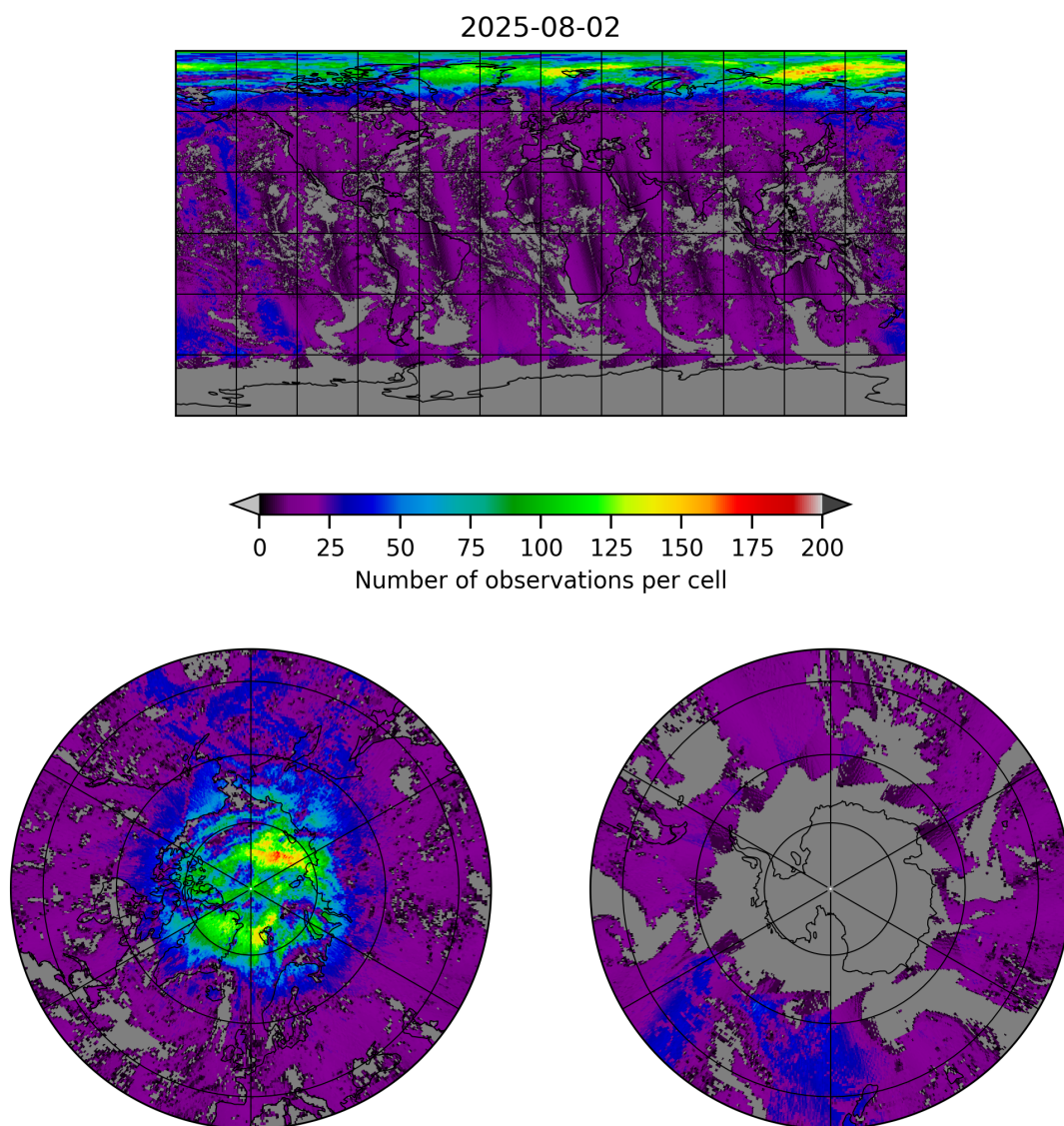
Figure 8: Map of the number of observations for 2025-08-01 to 2025-08-03
