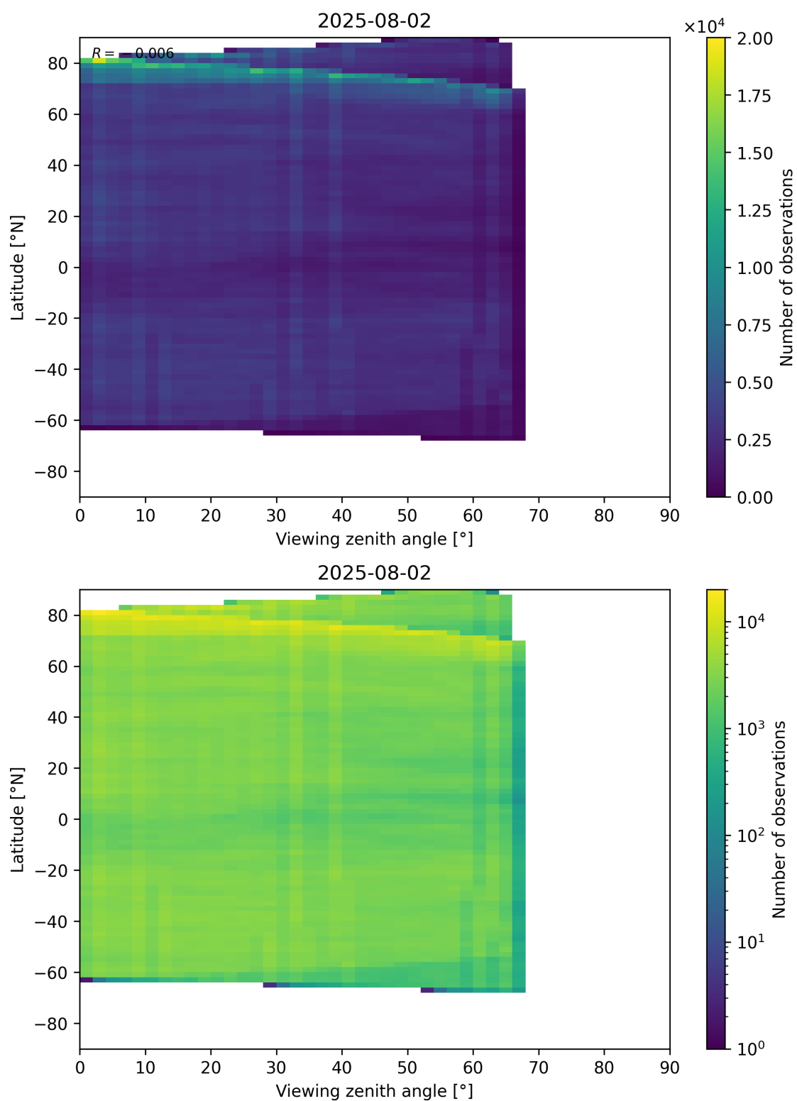
Figure 74: Scatter density plot of “Viewing zenith angle” against “Latitude” for 2025-08-01 to 2025-08-03.
