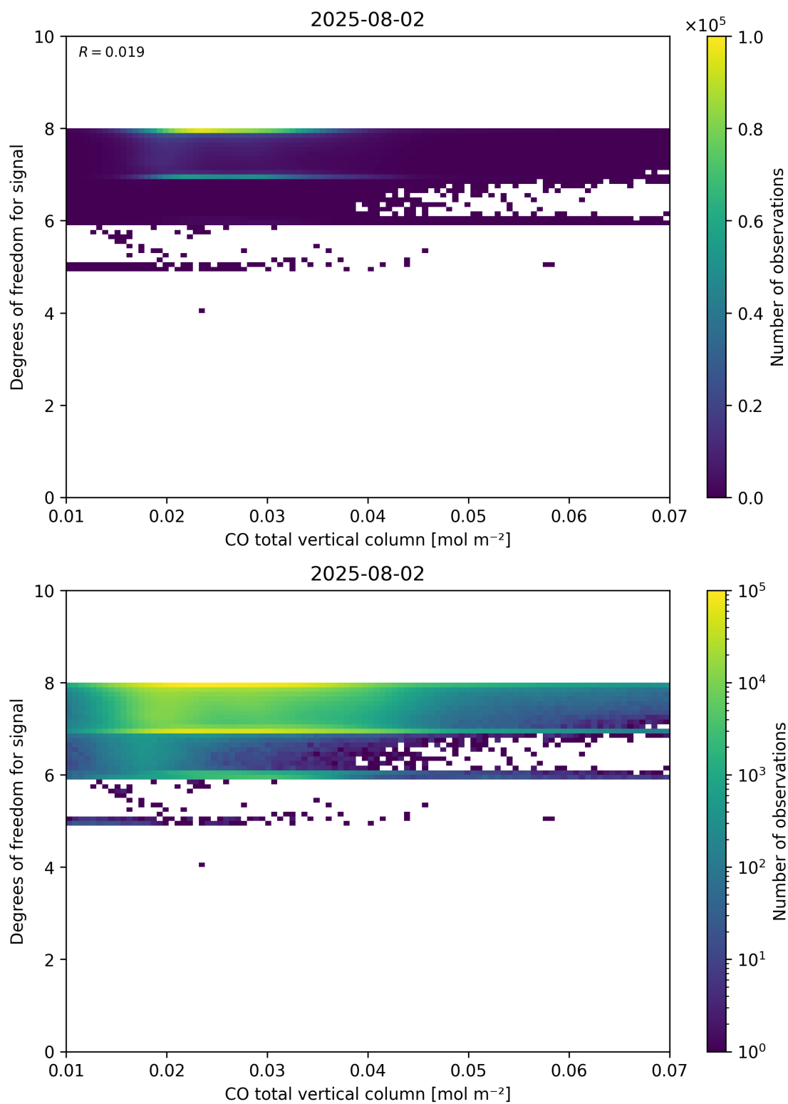
Figure 41: Scatter density plot of “CO total vertical column” against “Degrees of freedom for signal” for 2025-08-01 to 2025-08-03.
