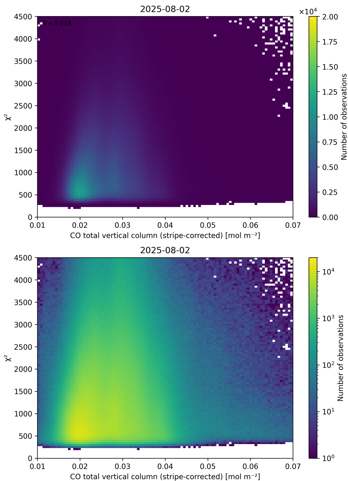
Figure 37: Scatter density plot of “CO total vertical column (stripe-corrected)” against “ \chi^2 ” for 2025-08-01 to 2025-08-03.
