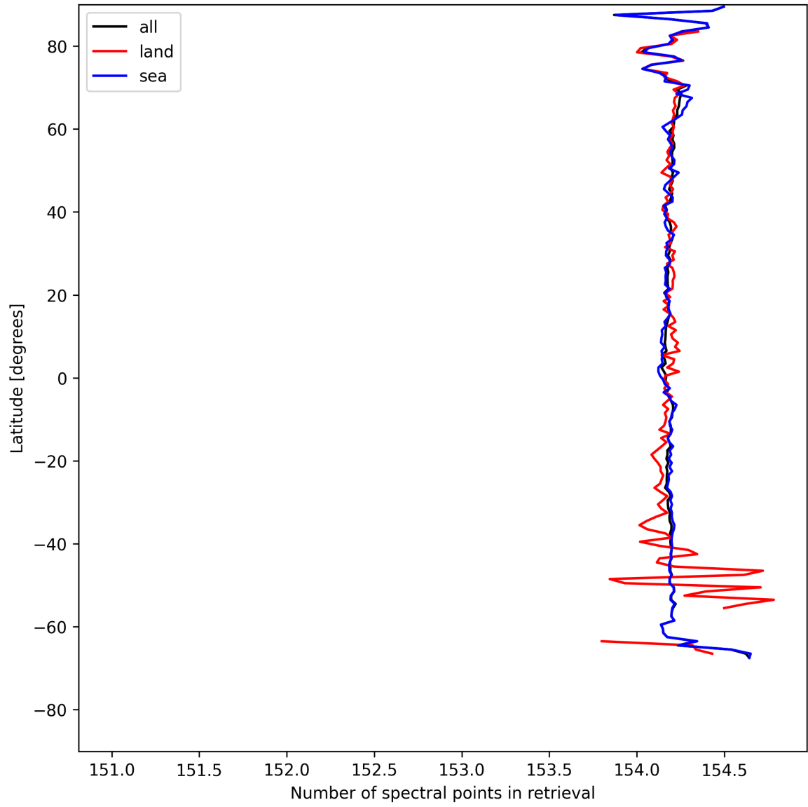
Figure 13: Zonal average of “Number of spectral points in retrieval” for 2025-08-01 to 2025-08-03.
