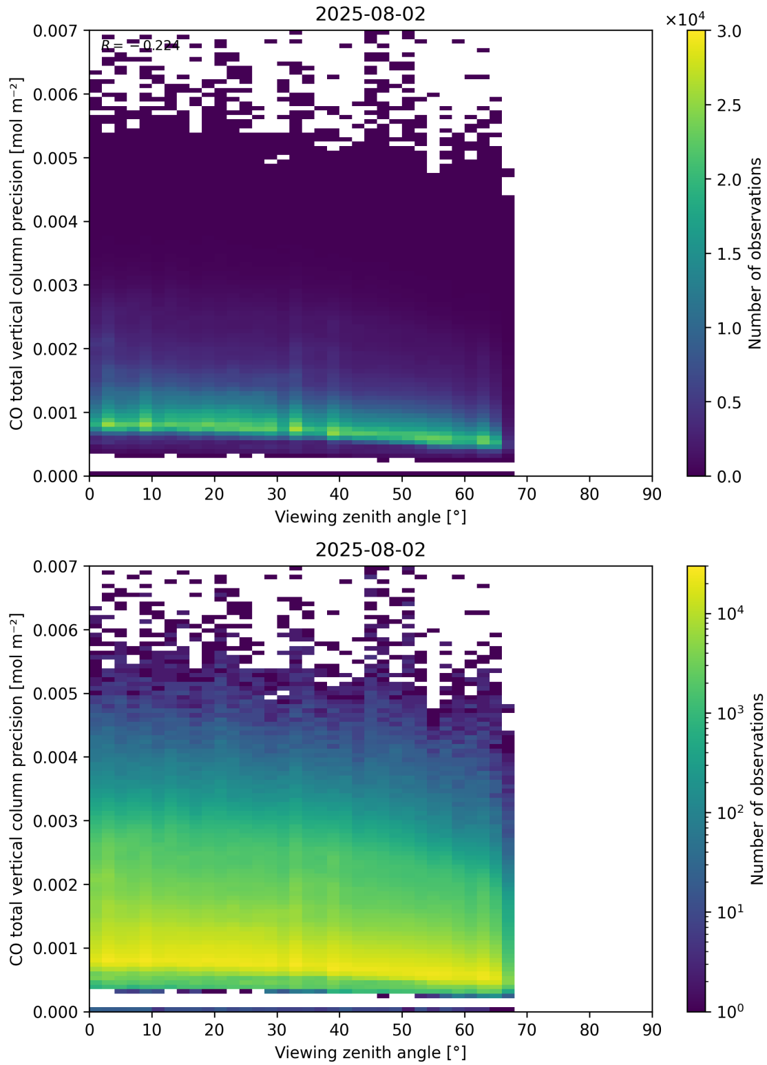
Figure 71: Scatter density plot of “Viewing zenith angle” against “CO total vertical column precision” for 2025-08-01 to 2025-08-03.
