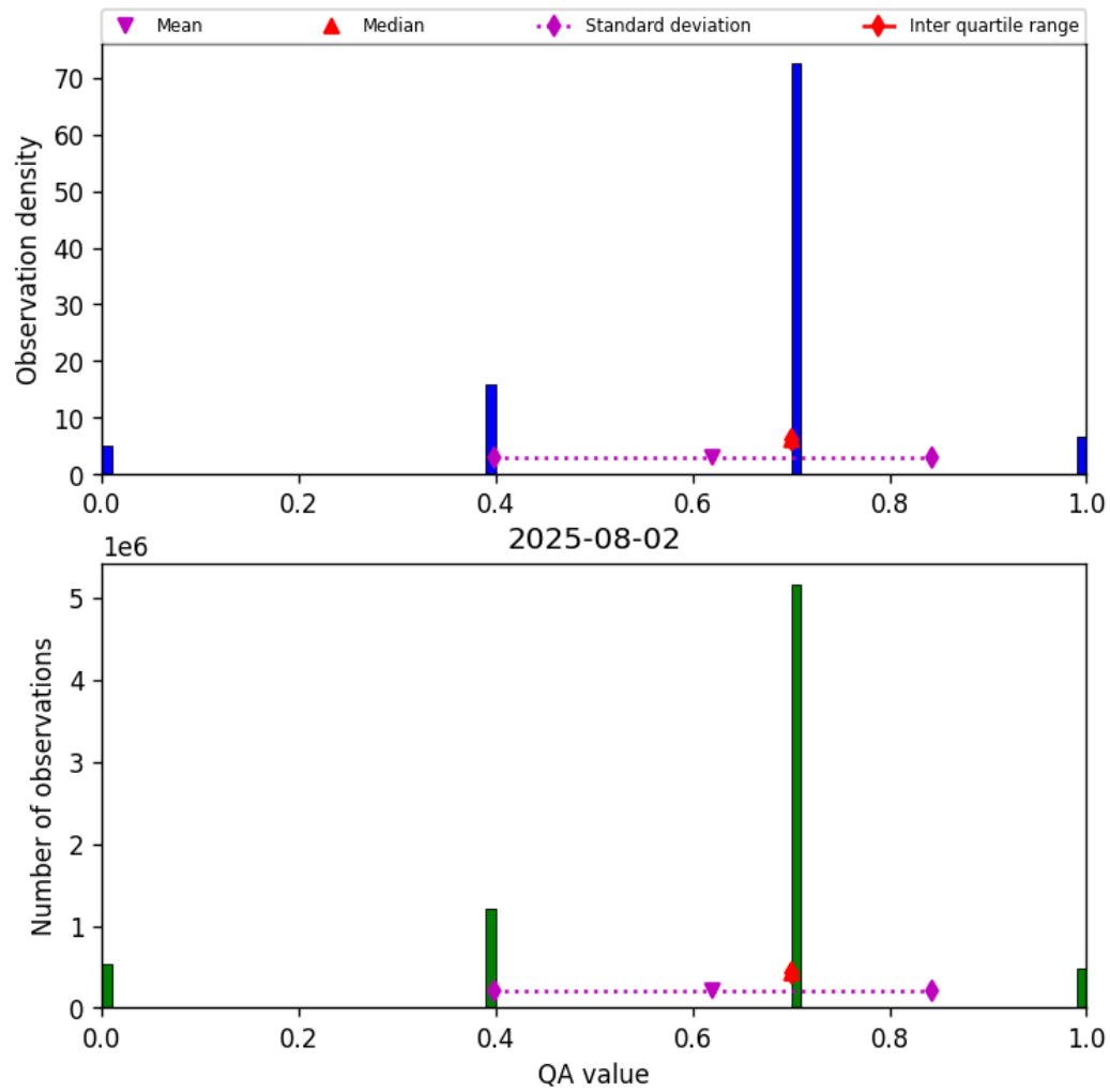
Figure 17: Histogram of “QA value” for 2025-08-01 to 2025-08-03
