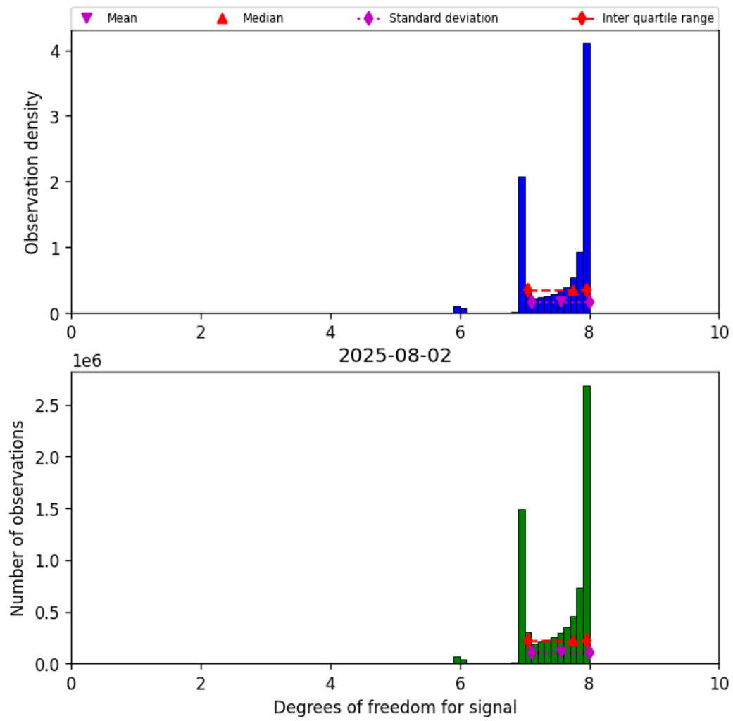
Figure 23: Histogram of “Degrees of freedom for signal” for 2025-08-01 to 2025-08-03
