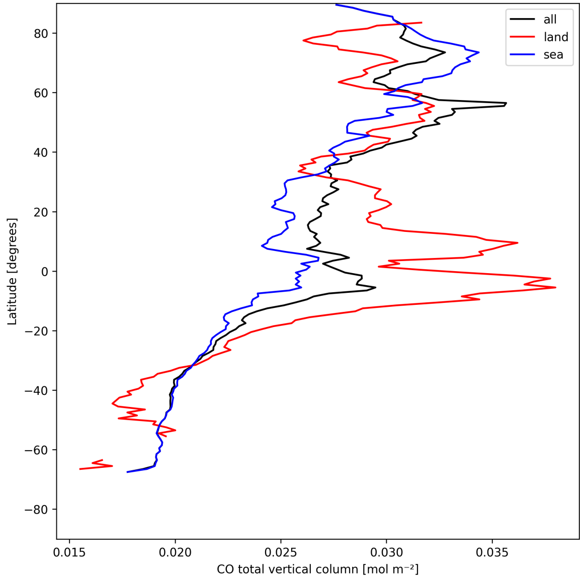
Figure 10: Zonal average of “CO total vertical column” for 2025-08-01 to 2025-08-03.
