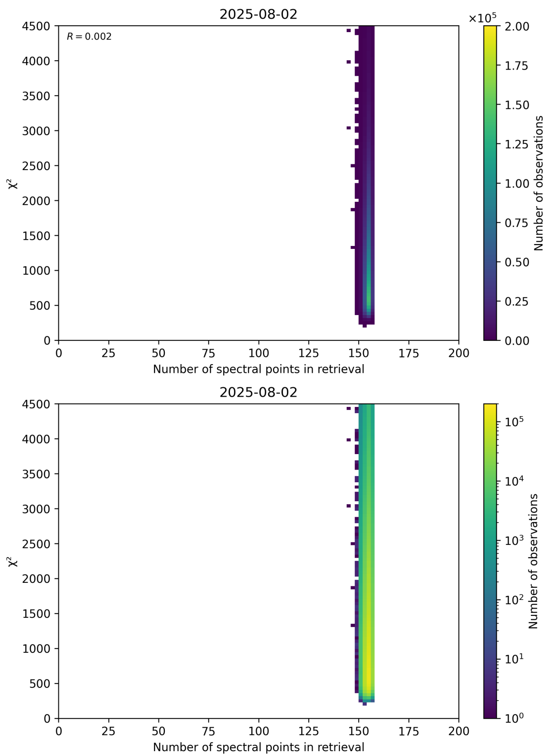
Figure 58: Scatter density plot of “Number of spectral points in retrieval” against “ \chi^2 ” for 2025-08-01 to 2025-08-03.
