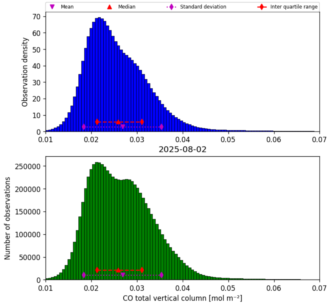
Figure 18: Histogram of “CO total vertical column” for 2025-08-01 to 2025-08-03
