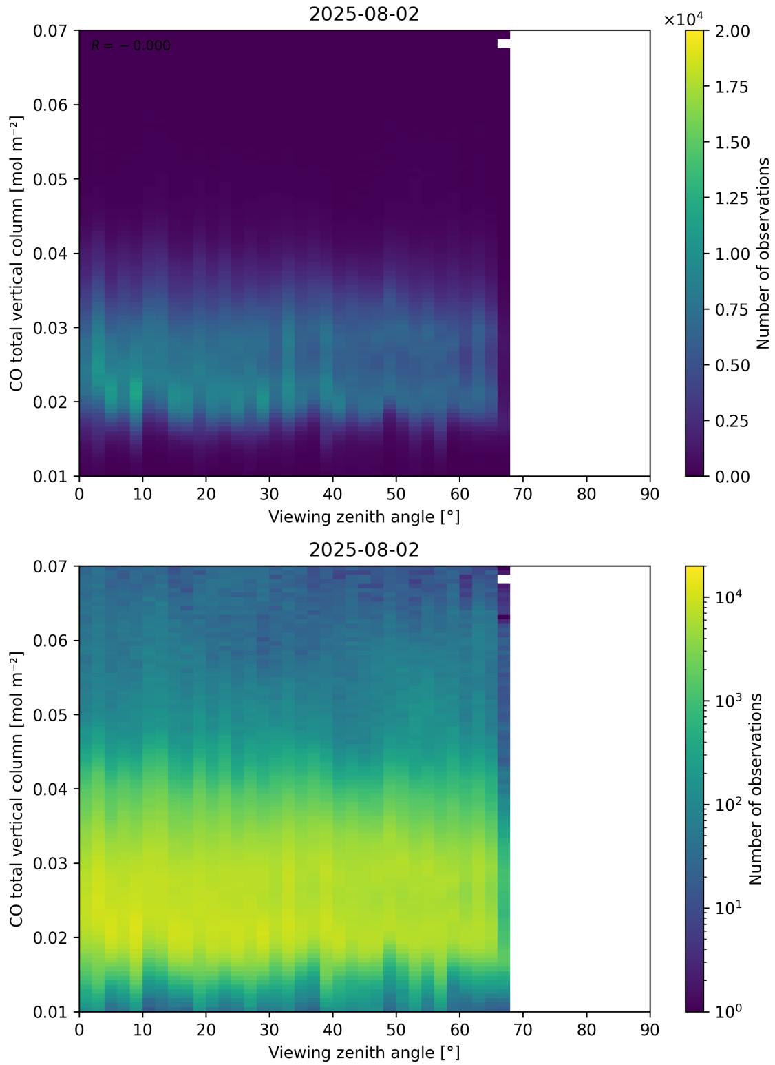
Figure 69: Scatter density plot of “Viewing zenith angle” against “CO total vertical column” for 2025-08-01 to 2025-08-03.
