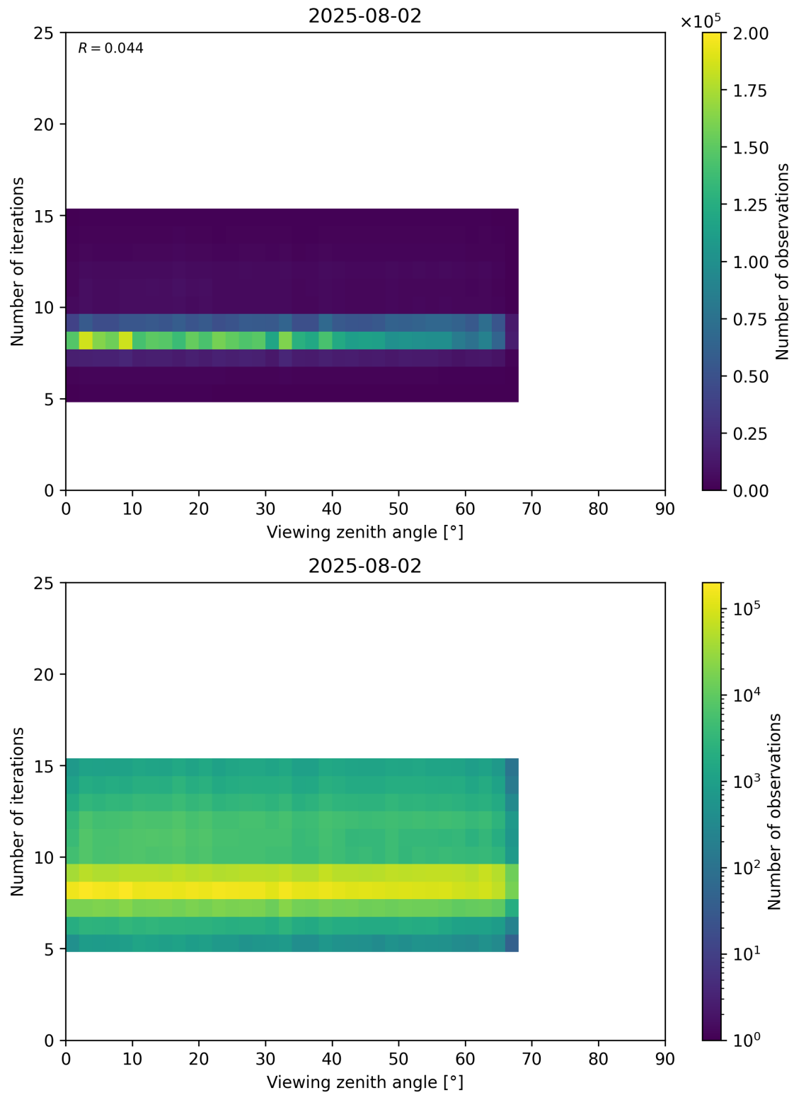
Figure 75: Scatter density plot of “Viewing zenith angle” against “Number of iterations” for 2025-08-01 to 2025-08-03.
