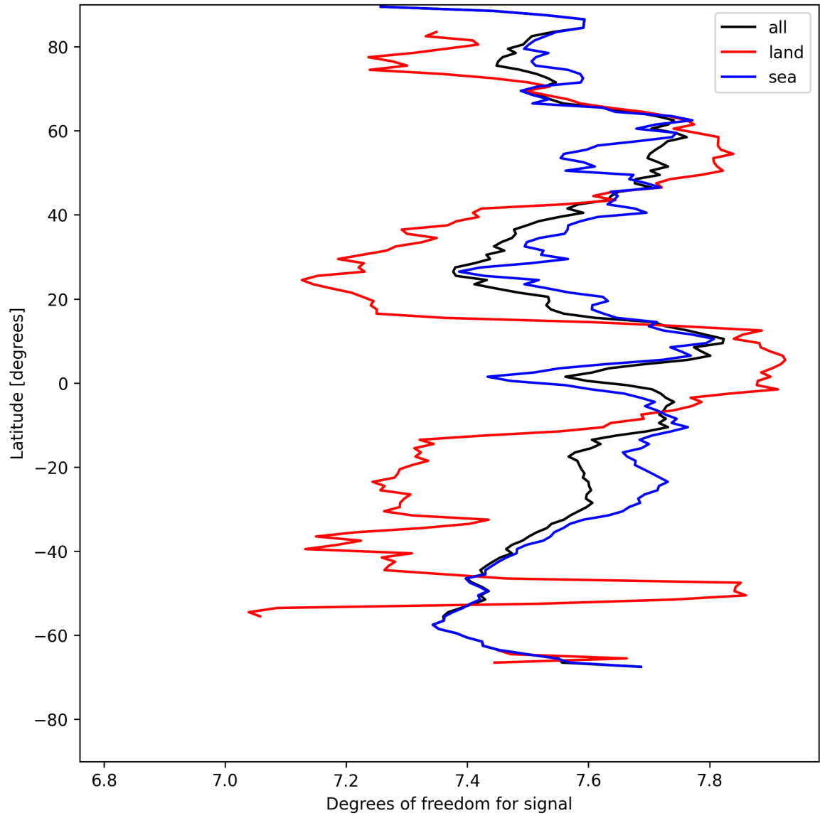
Figure 15: Zonal average of “Degrees of freedom for signal” for 2025-08-01 to 2025-08-03.
