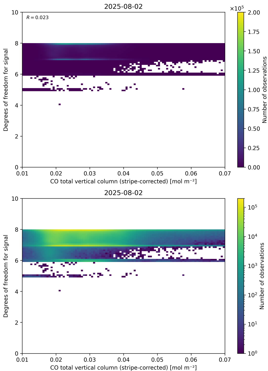
Figure 38: Scatter density plot of “CO total vertical column (stripe-corrected)” against “Degrees of freedom for signal” for 2025-08-01 to 2025-08-03.
