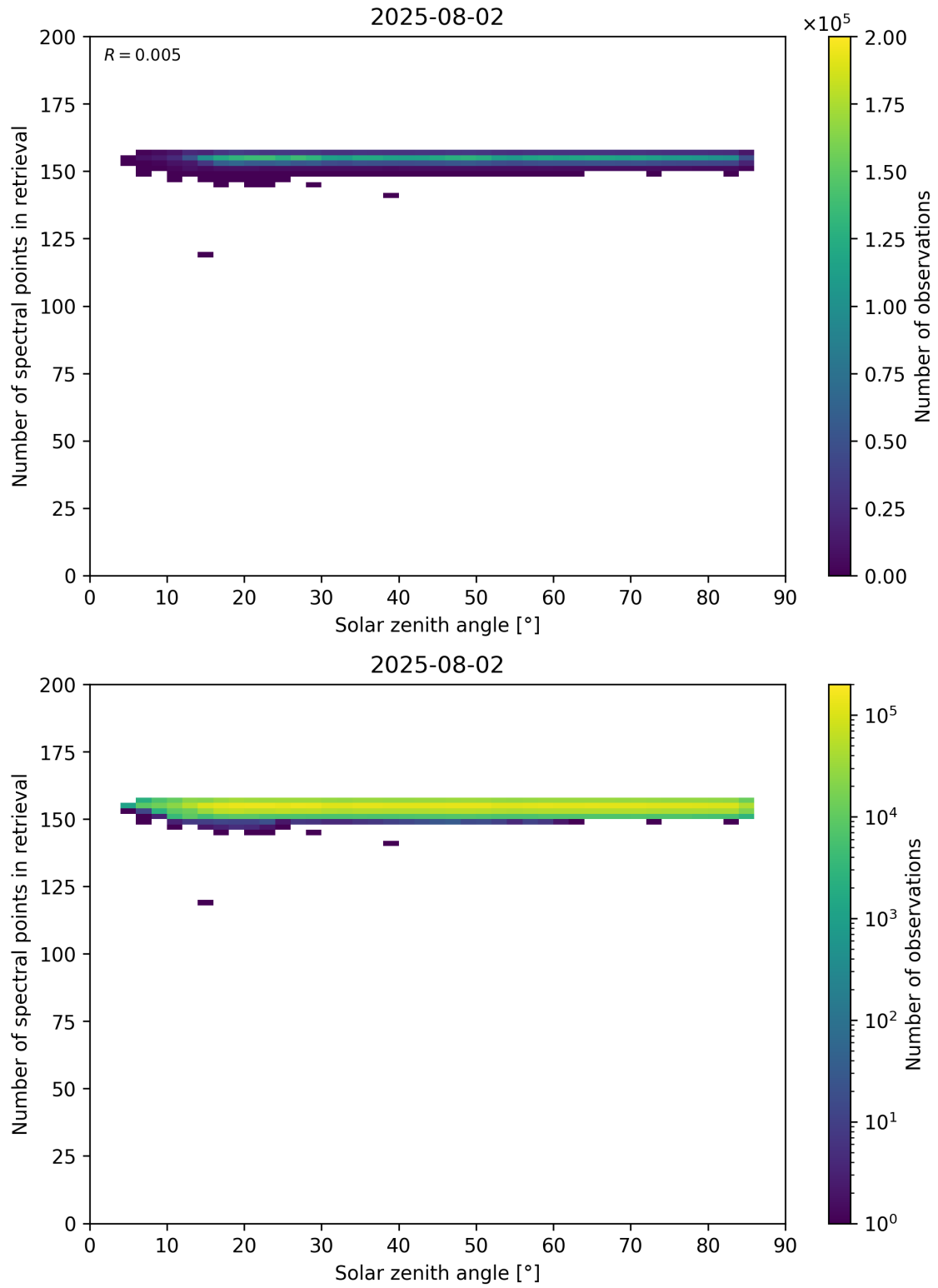
Figure 68: Scatter density plot of “Solar zenith angle” against “Number of spectral points in retrieval” for 2025-08-01 to 2025-08-03.
