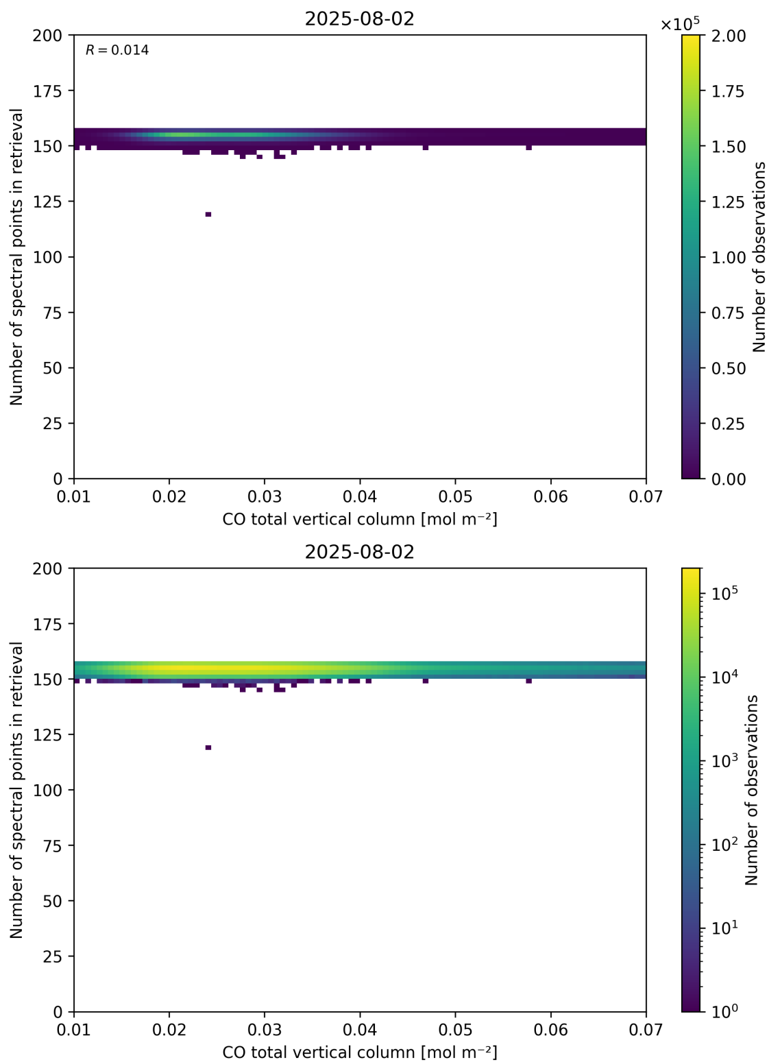
Figure 43: Scatter density plot of “CO total vertical column” against “Number of spectral points in retrieval” for 2025-08-01 to 2025-08-03.
