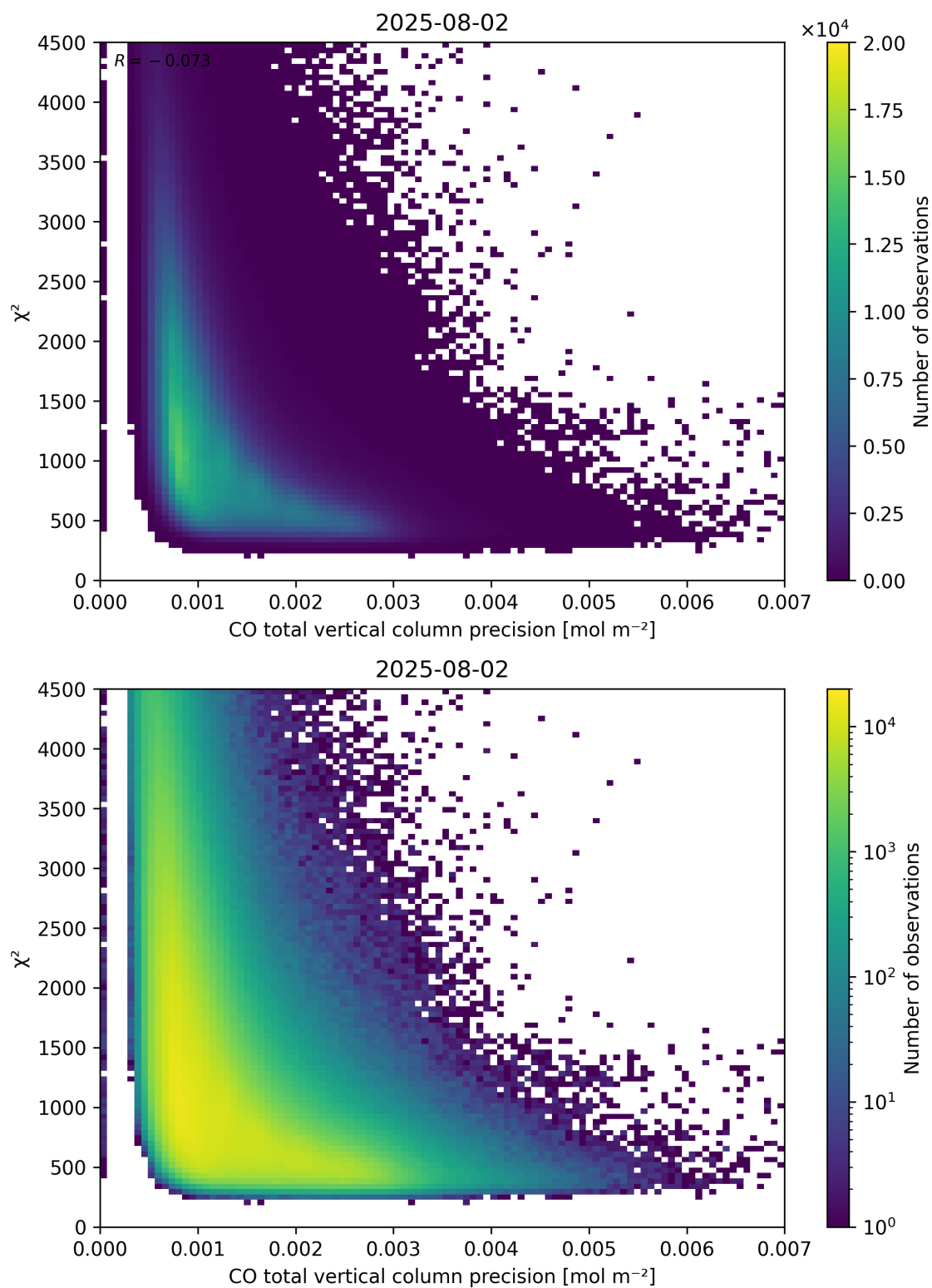
Figure 44: Scatter density plot of “CO total vertical column precision” against “ \chi^2 ” for 2025-08-01 to 2025-08-03.
