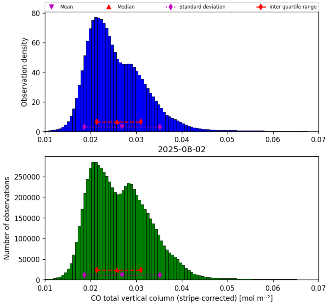
Figure 19: Histogram of “CO total vertical column (stripe-corrected)” for 2025-08-01 to 2025-08-03
