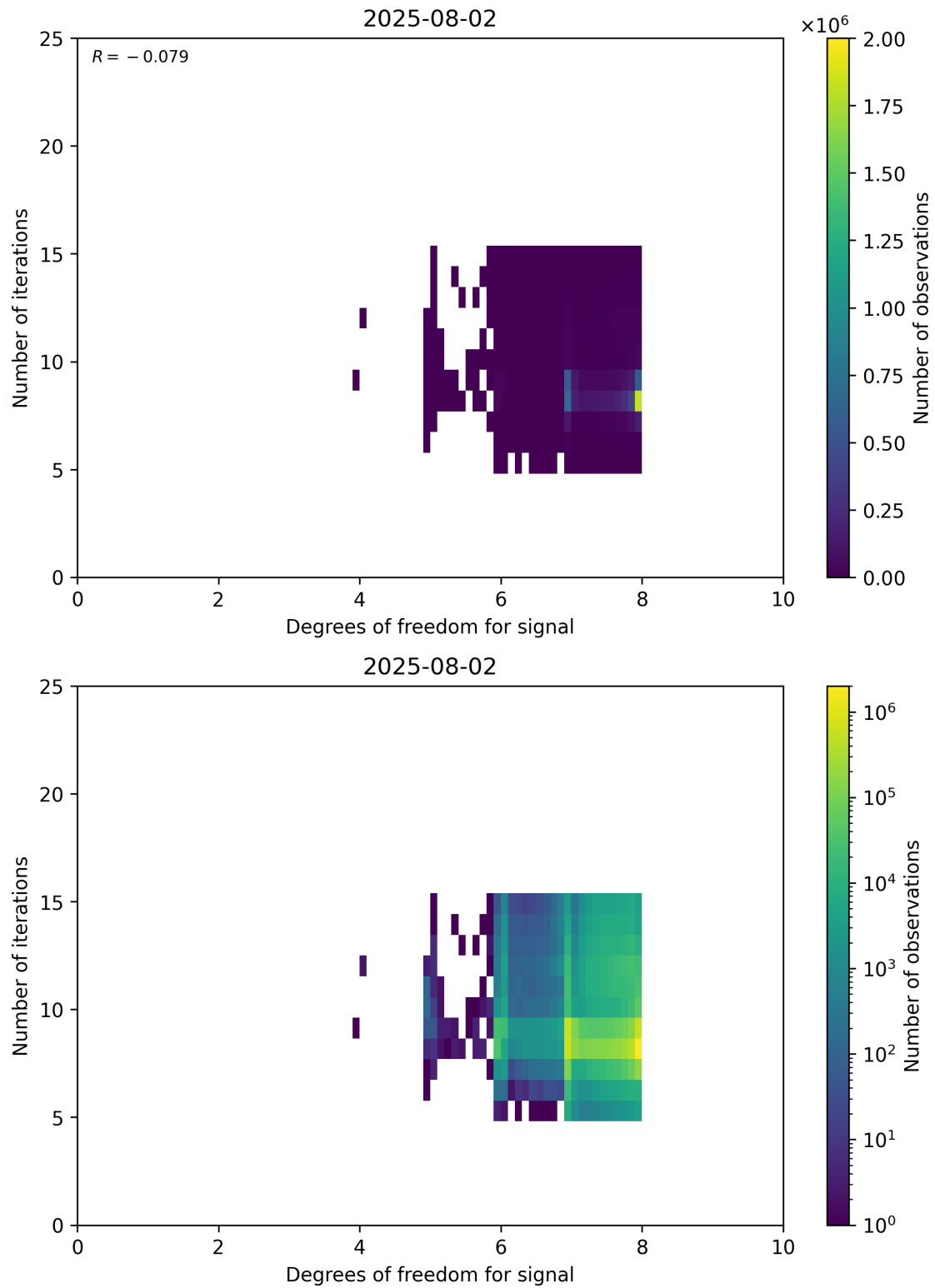
Figure 50: Scatter density plot of “Degrees of freedom for signal” against “Number of iterations” for 2025-08-01 to 2025-08-03.
