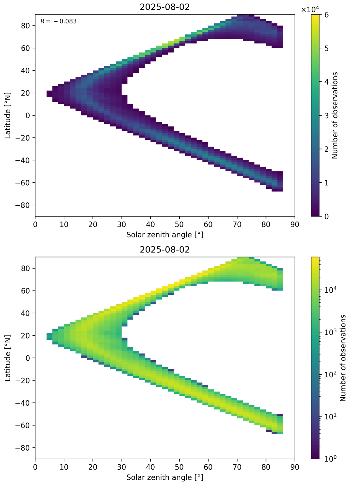
Figure 66: Scatter density plot of “Solar zenith angle” against “Latitude” for 2025-08-01 to 2025-08-03.
