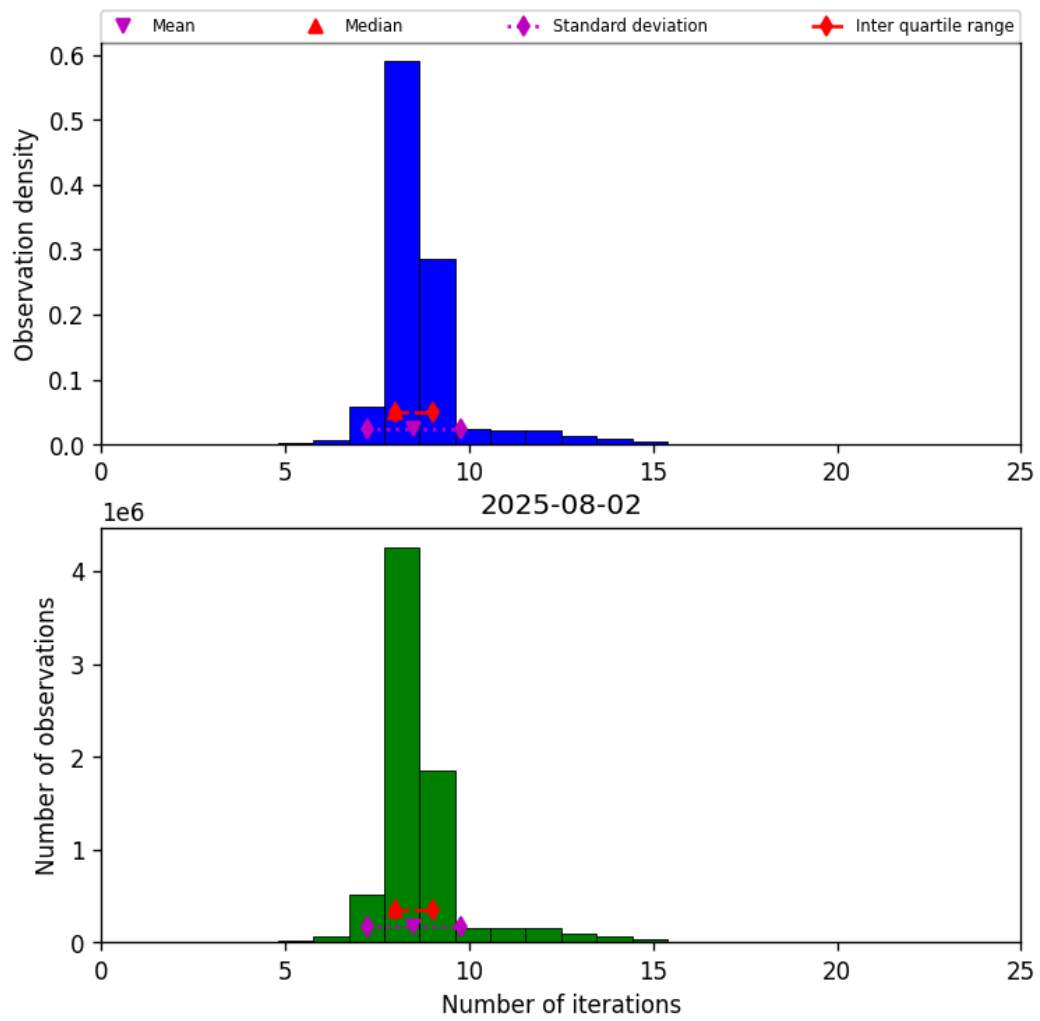
Figure 24: Histogram of “Number of iterations” for 2025-08-01 to 2025-08-03
