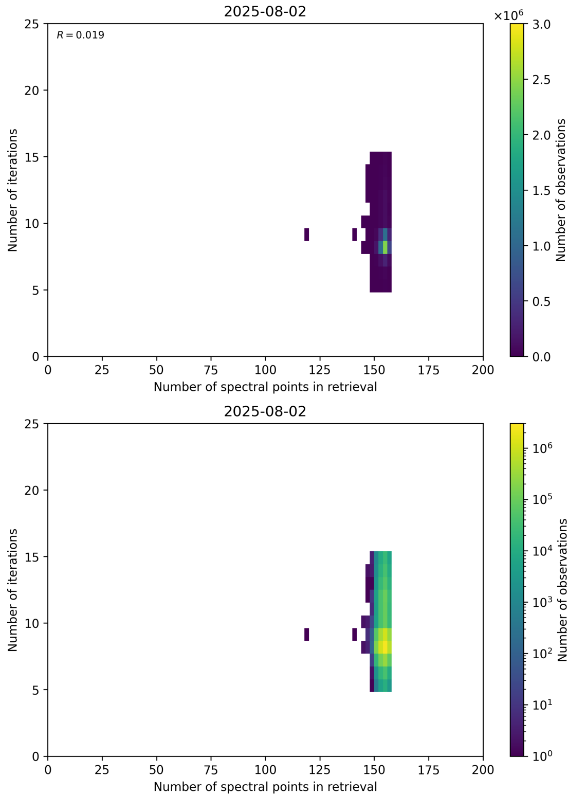
Figure 60: Scatter density plot of “Number of spectral points in retrieval” against “Number of iterations” for 2025-08-01 to 2025-08-03.
