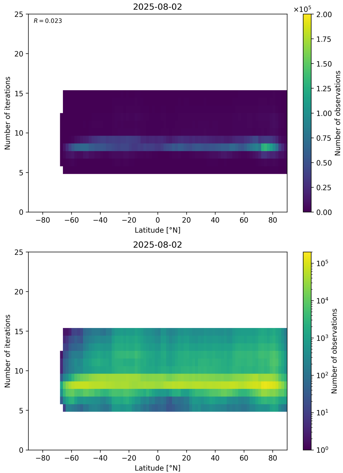
Figure 56: Scatter density plot of “Latitude” against “Number of iterations” for 2025-08-01 to 2025-08-03.
