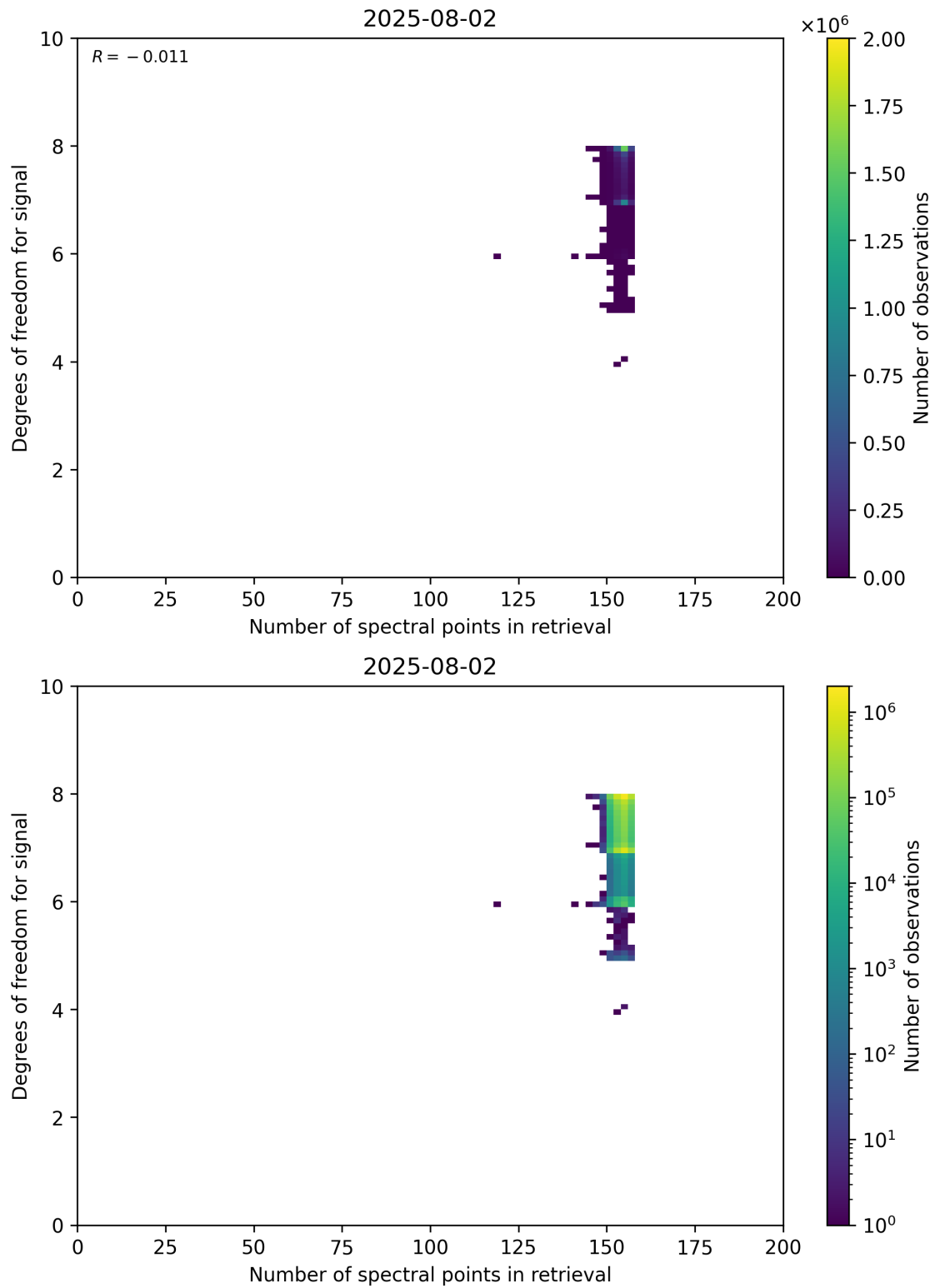
Figure 59: Scatter density plot of “Number of spectral points in retrieval” against “Degrees of freedom for signal” for 2025-08-01 to 2025-08-03.
