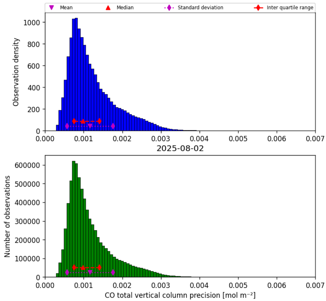
Figure 20: Histogram of “CO total vertical column precision” for 2025-08-01 to 2025-08-03
