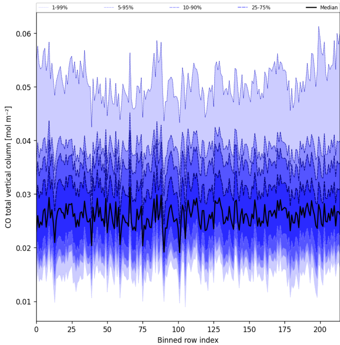
Figure 26: Along track statistics of “CO total vertical column” for 2025-08-01 to 2025-08-03
