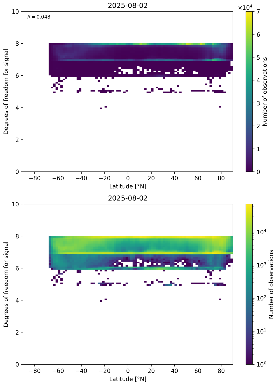
Figure 55: Scatter density plot of “Latitude” against “Degrees of freedom for signal” for 2025-08-01 to 2025-08-03.
