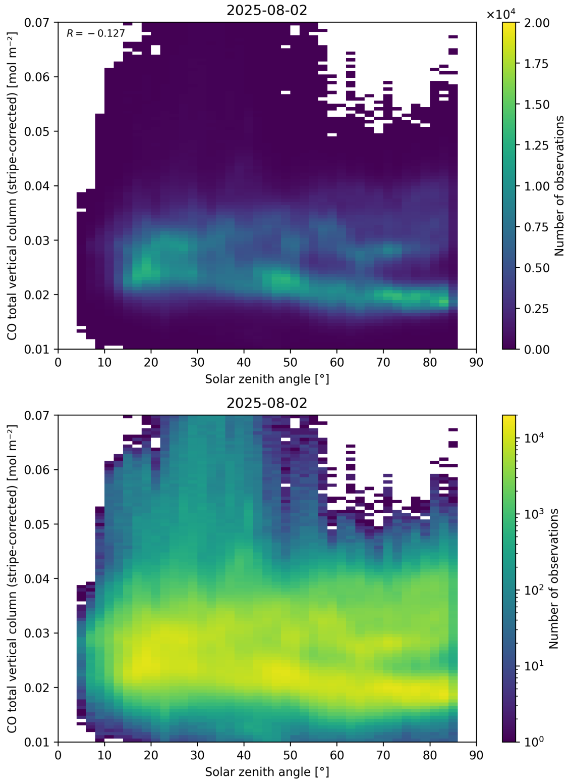
Figure 62: Scatter density plot of “Solar zenith angle” against “CO total vertical column (stripe-corrected)” for 2025-08-01 to 2025-08-03.
