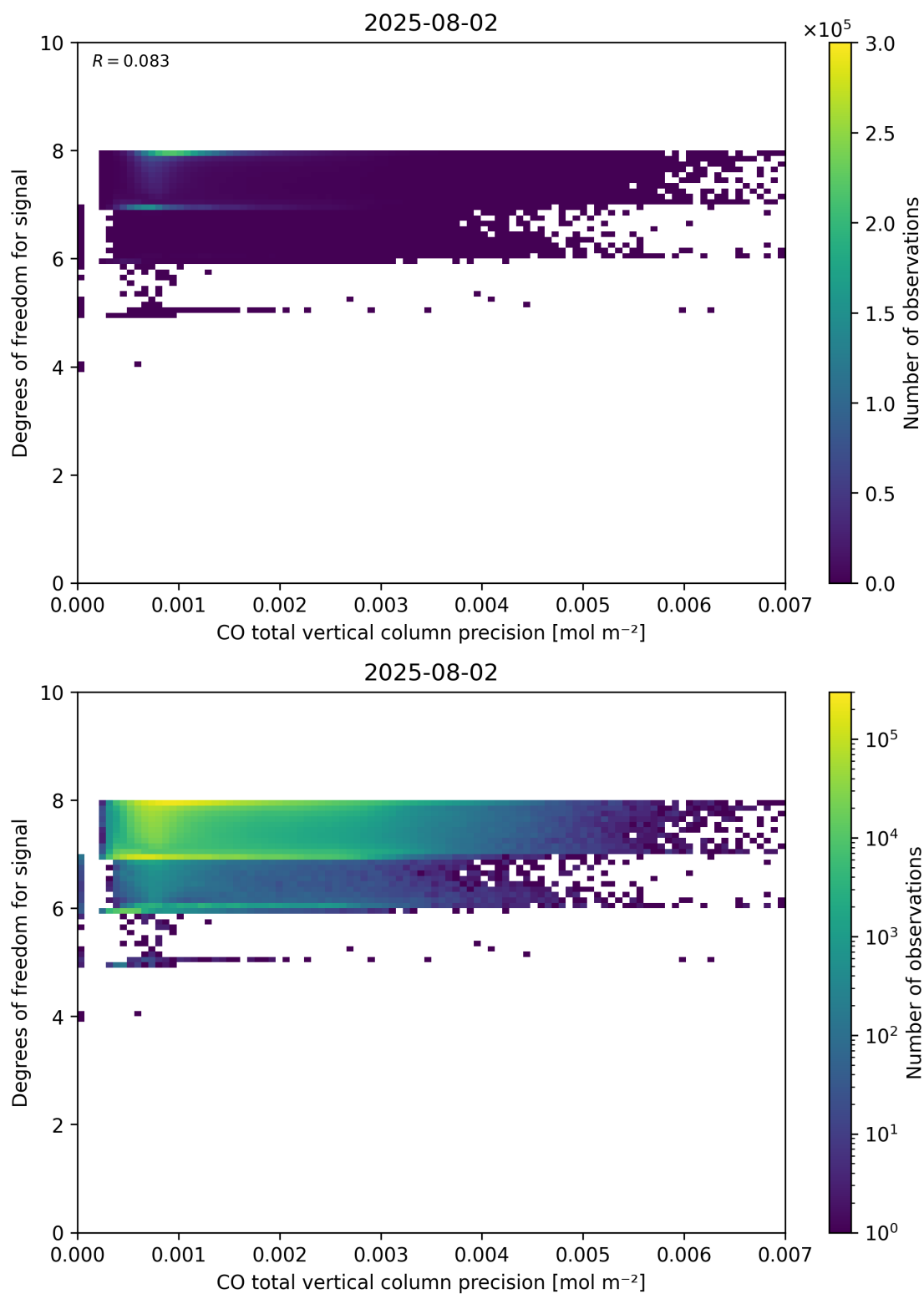
Figure 45: Scatter density plot of “CO total vertical column precision” against “Degrees of freedom for signal” for 2025-08-01 to 2025-08-03.
