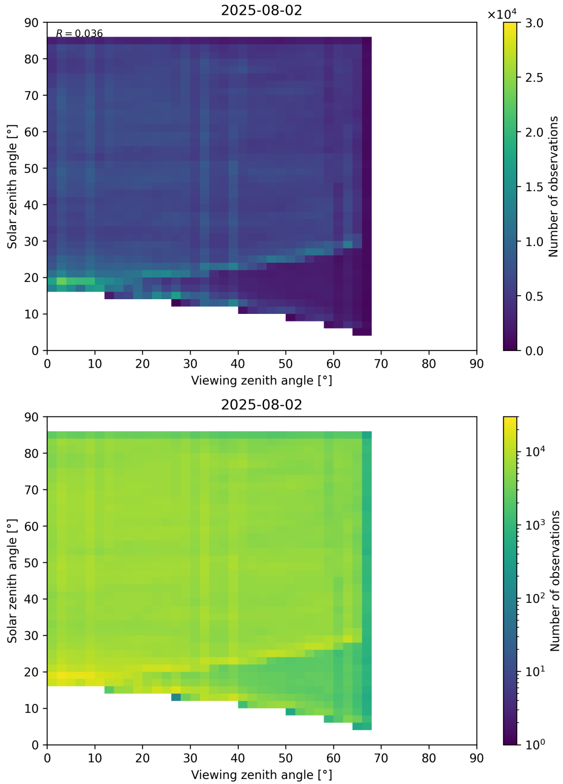
Figure 77: Scatter density plot of “Viewing zenith angle” against “Solar zenith angle” for 2025-08-01 to 2025-08-03.
