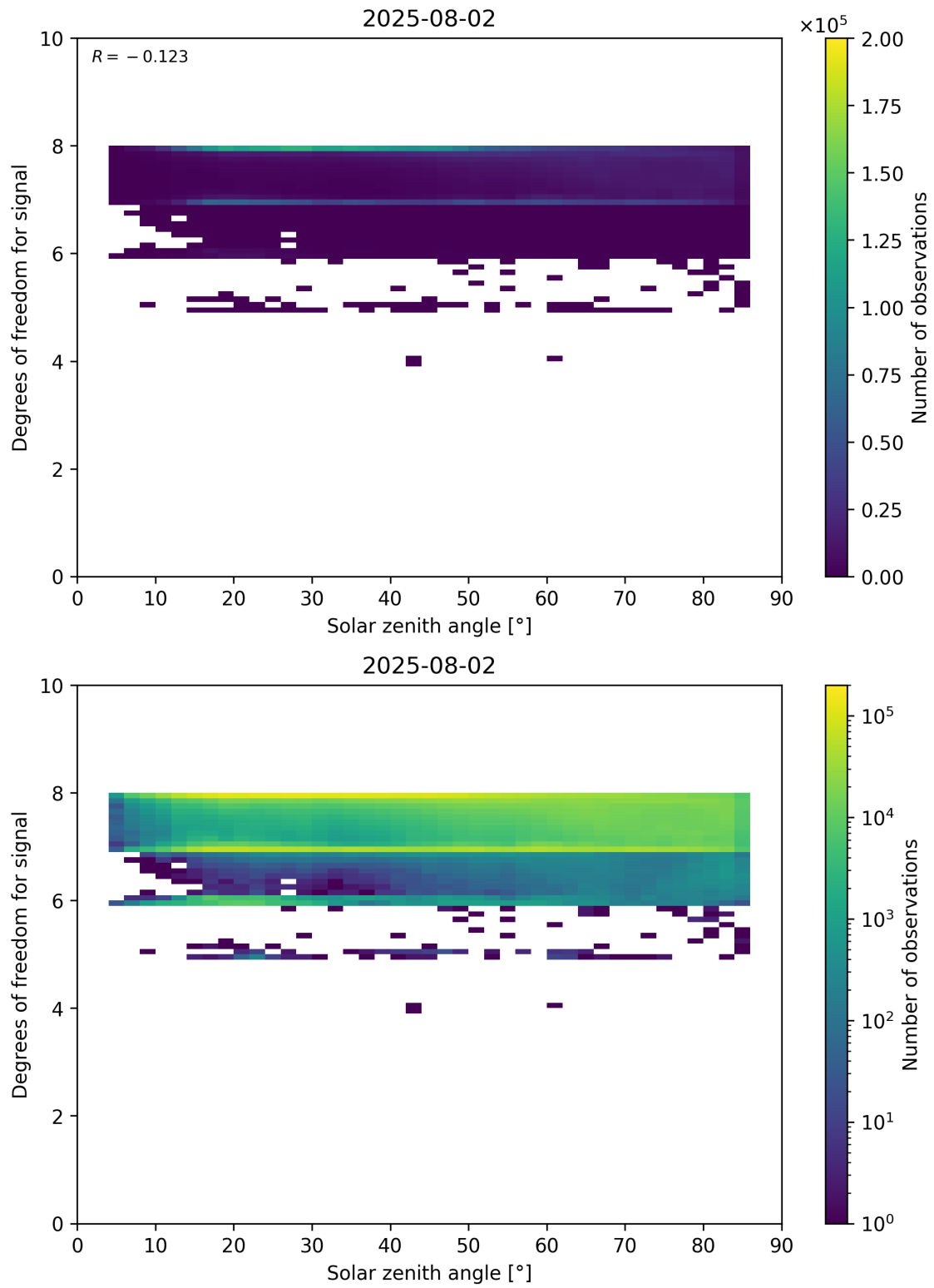
Figure 65: Scatter density plot of “Solar zenith angle” against “Degrees of freedom for signal” for 2025-08-01 to 2025-08-03.
