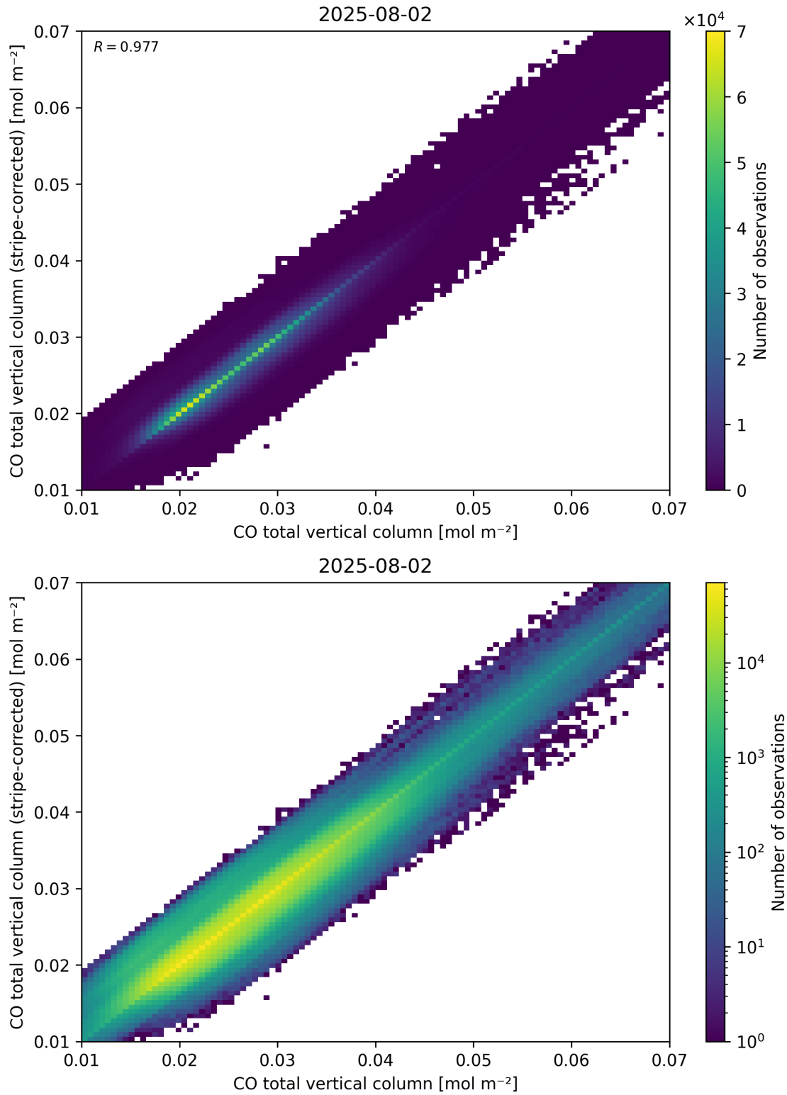
Figure 33: Scatter density plot of “CO total vertical column” against “CO total vertical column (stripe-corrected)” for 2025-08-01 to 2025-08-03.
