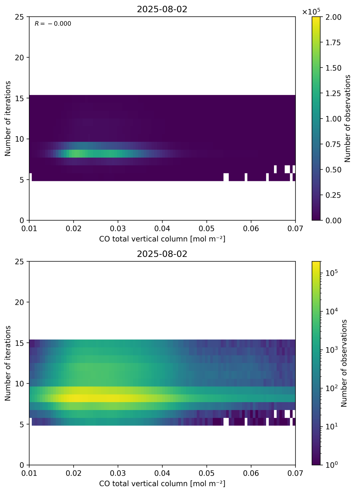
Figure 42: Scatter density plot of “CO total vertical column” against “Number of iterations” for 2025-08-01 to 2025-08-03.
