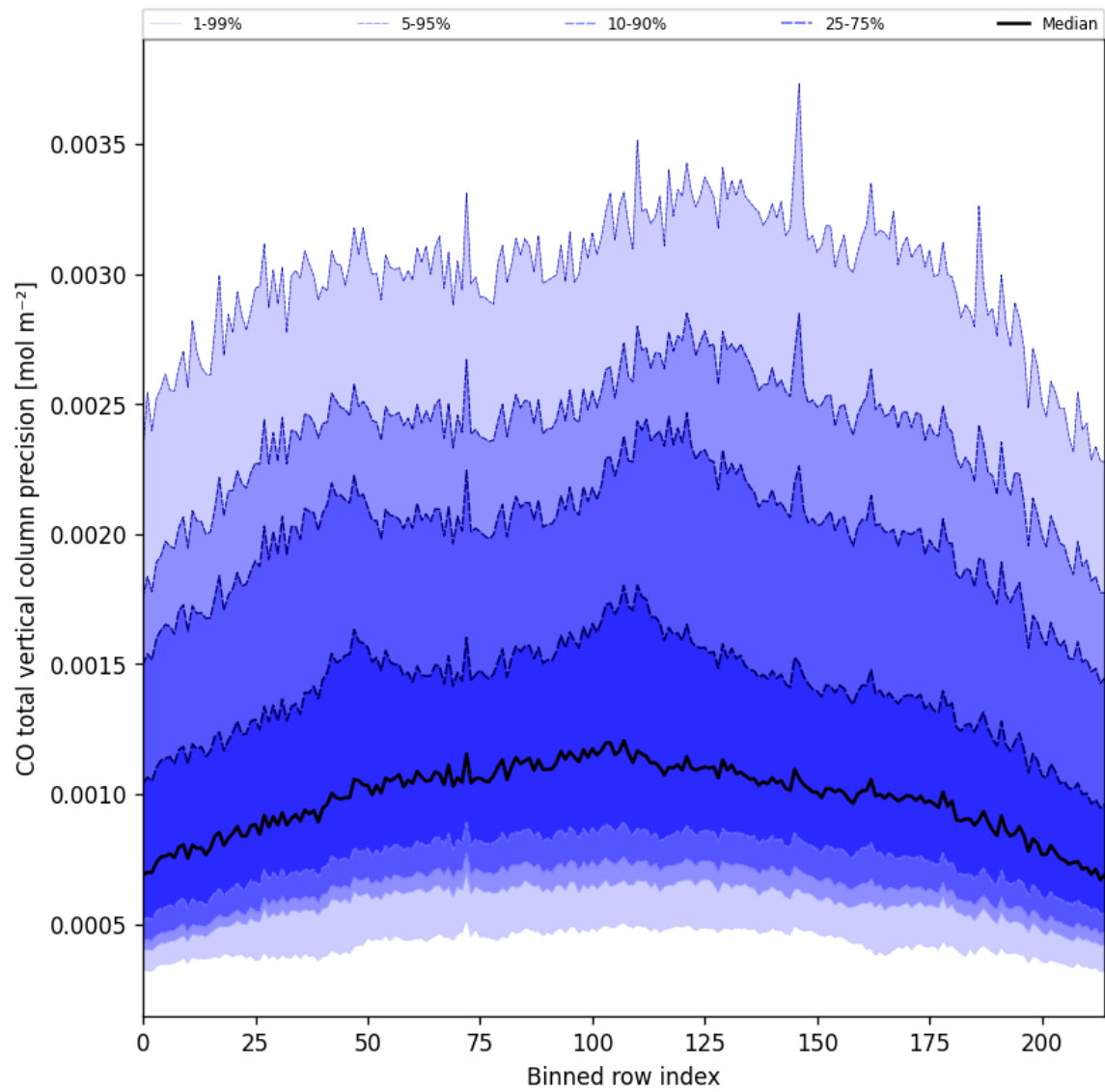
Figure 28: Along track statistics of “CO total vertical column precision” for 2025-08-01 to 2025-08-03
