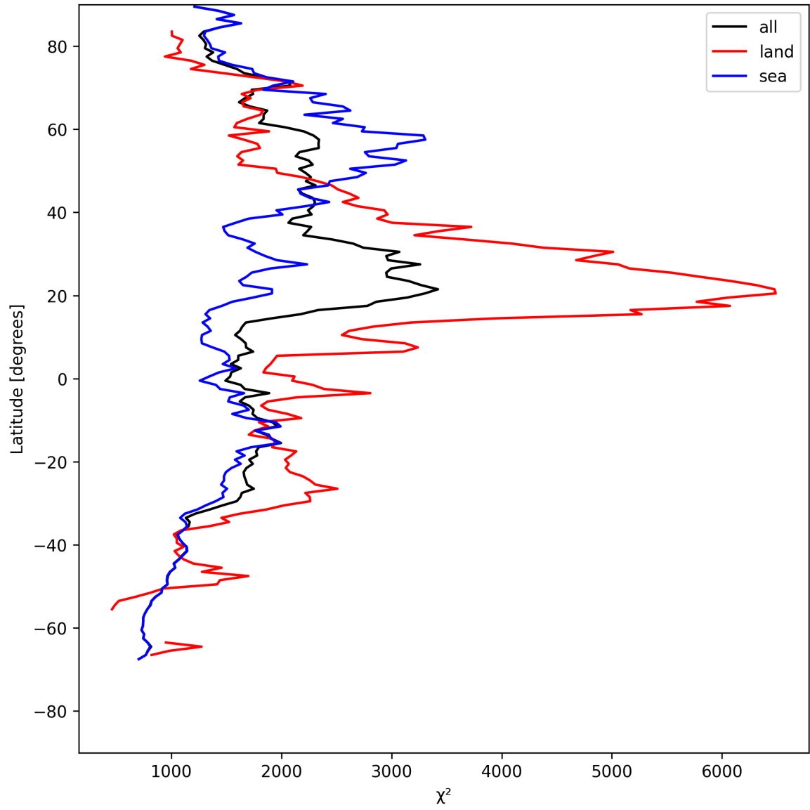
Figure 14: Zonal average of “ \chi^2 ” for 2025-08-01 to 2025-08-03.
