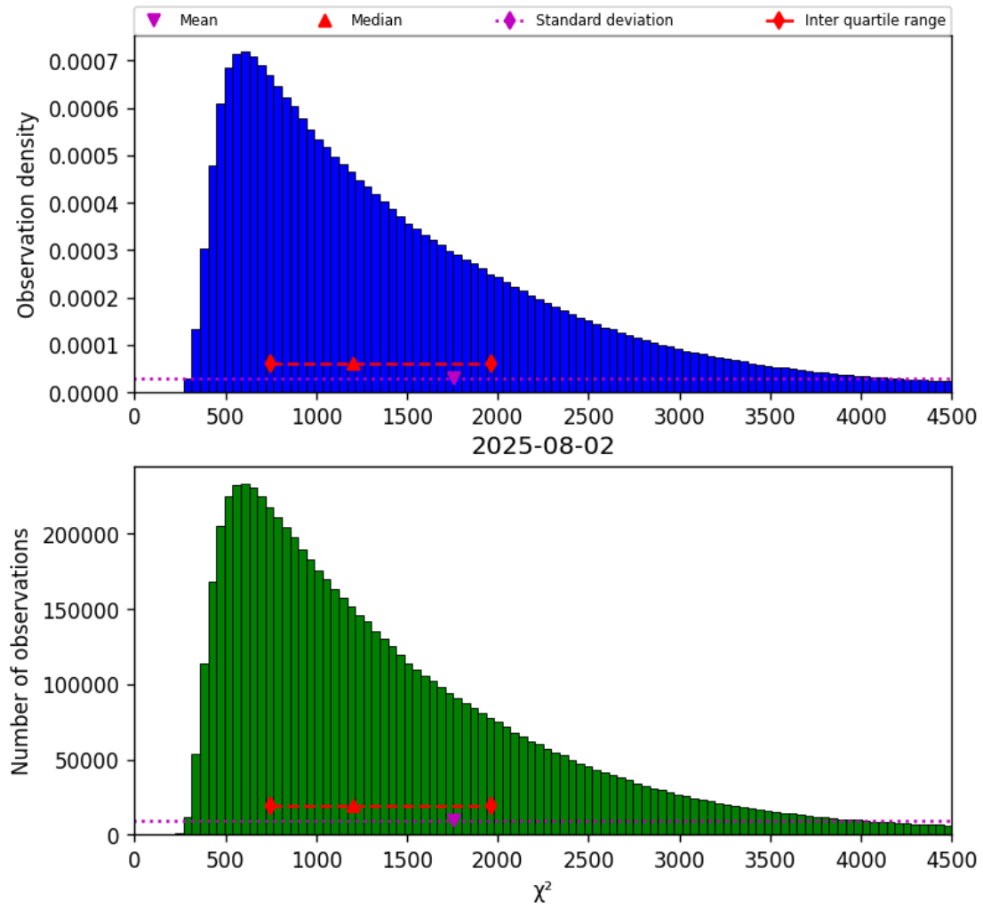
Figure 22: Histogram of " \chi^2 " for 2025-08-01 to 2025-08-03
