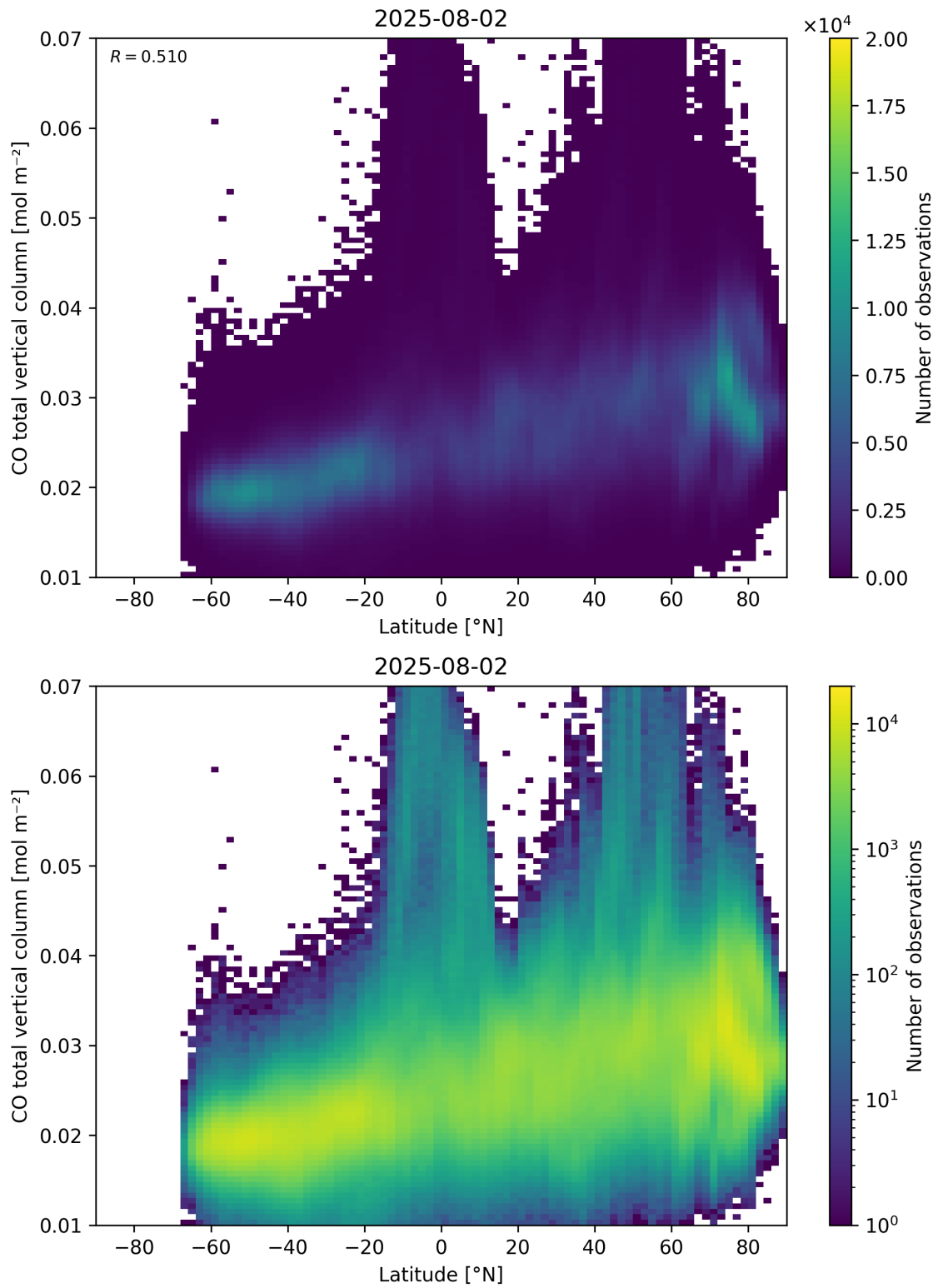
Figure 51: Scatter density plot of “Latitude” against “CO total vertical column” for 2025-08-01 to 2025-08-03.
