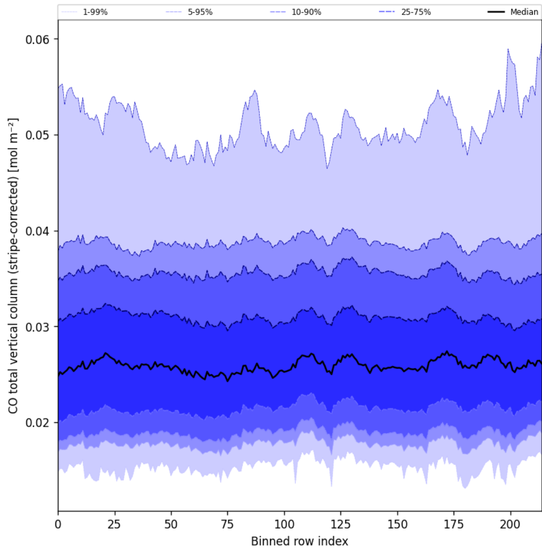
Figure 27: Along track statistics of “CO total vertical column (stripe-corrected)” for 2025-08-01 to 2025-08-03
