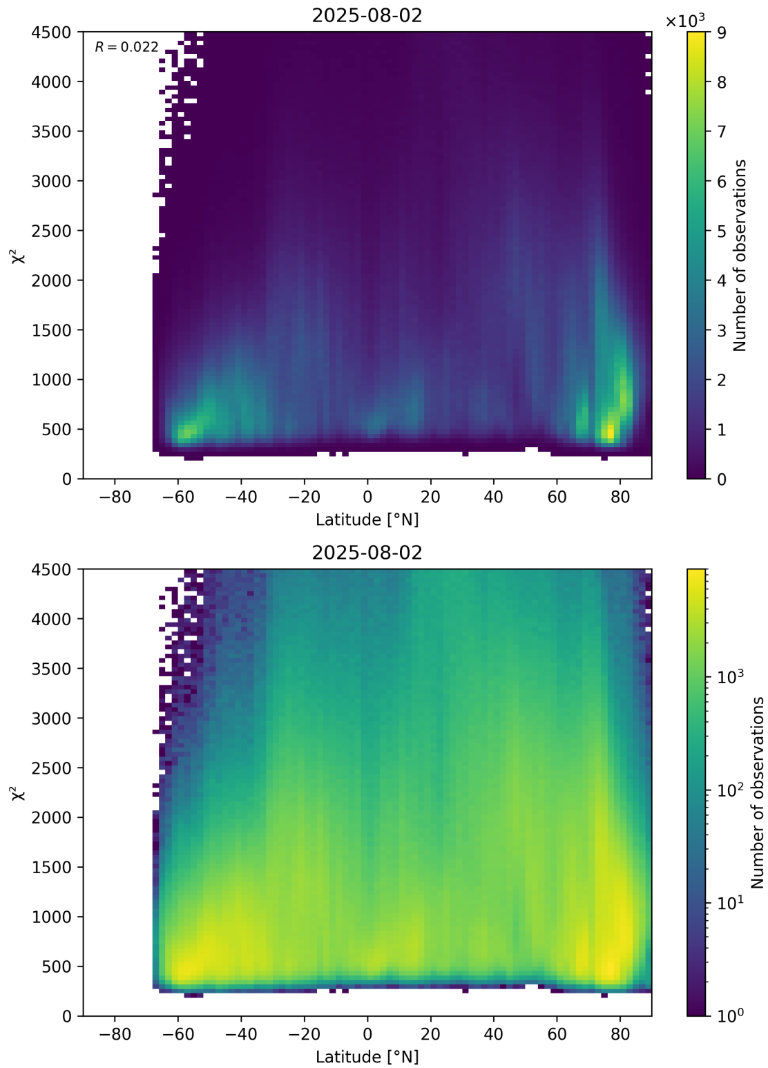
Figure 54: Scatter density plot of “Latitude” against “ \chi^2 ” for 2025-08-01 to 2025-08-03.
