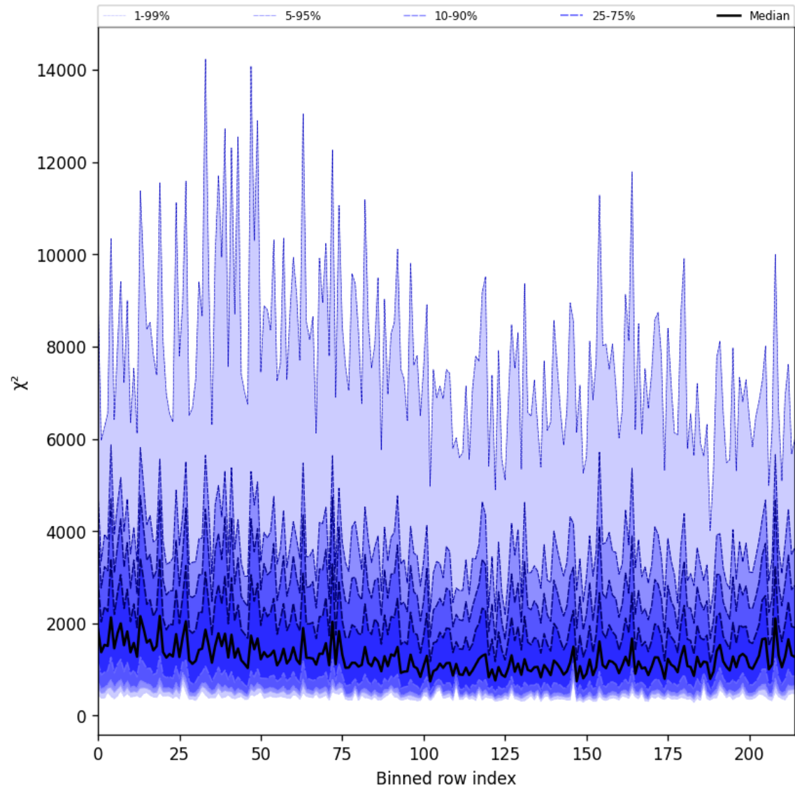
Figure 30: Along track statistics of “ \chi^2 ” for 2025-08-01 to 2025-08-03
