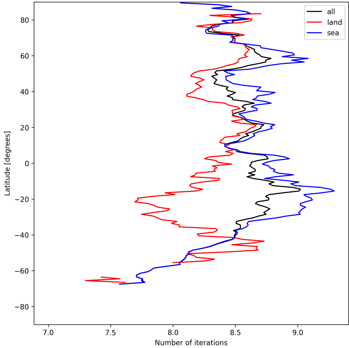
Figure 16: Zonal average of “Number of iterations” for 2025-08-01 to 2025-08-03.
