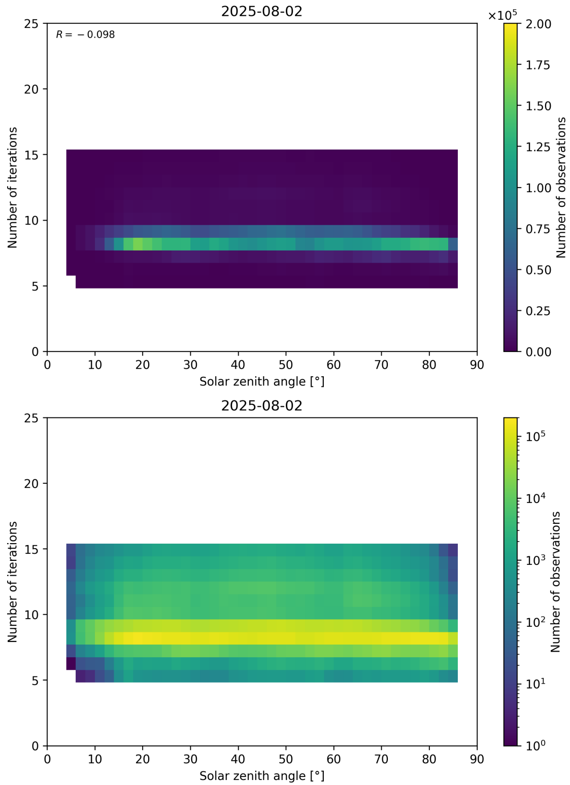
Figure 67: Scatter density plot of “Solar zenith angle” against “Number of iterations” for 2025-08-01 to 2025-08-03.
