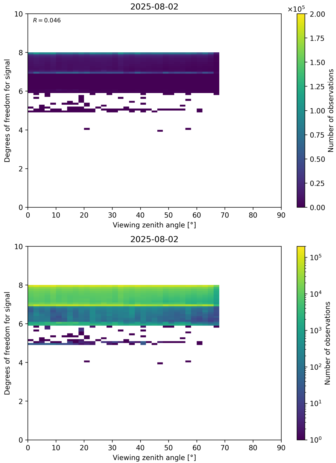
Figure 73: Scatter density plot of “Viewing zenith angle” against “Degrees of freedom for signal” for 2025-08-01 to 2025-08-03.
