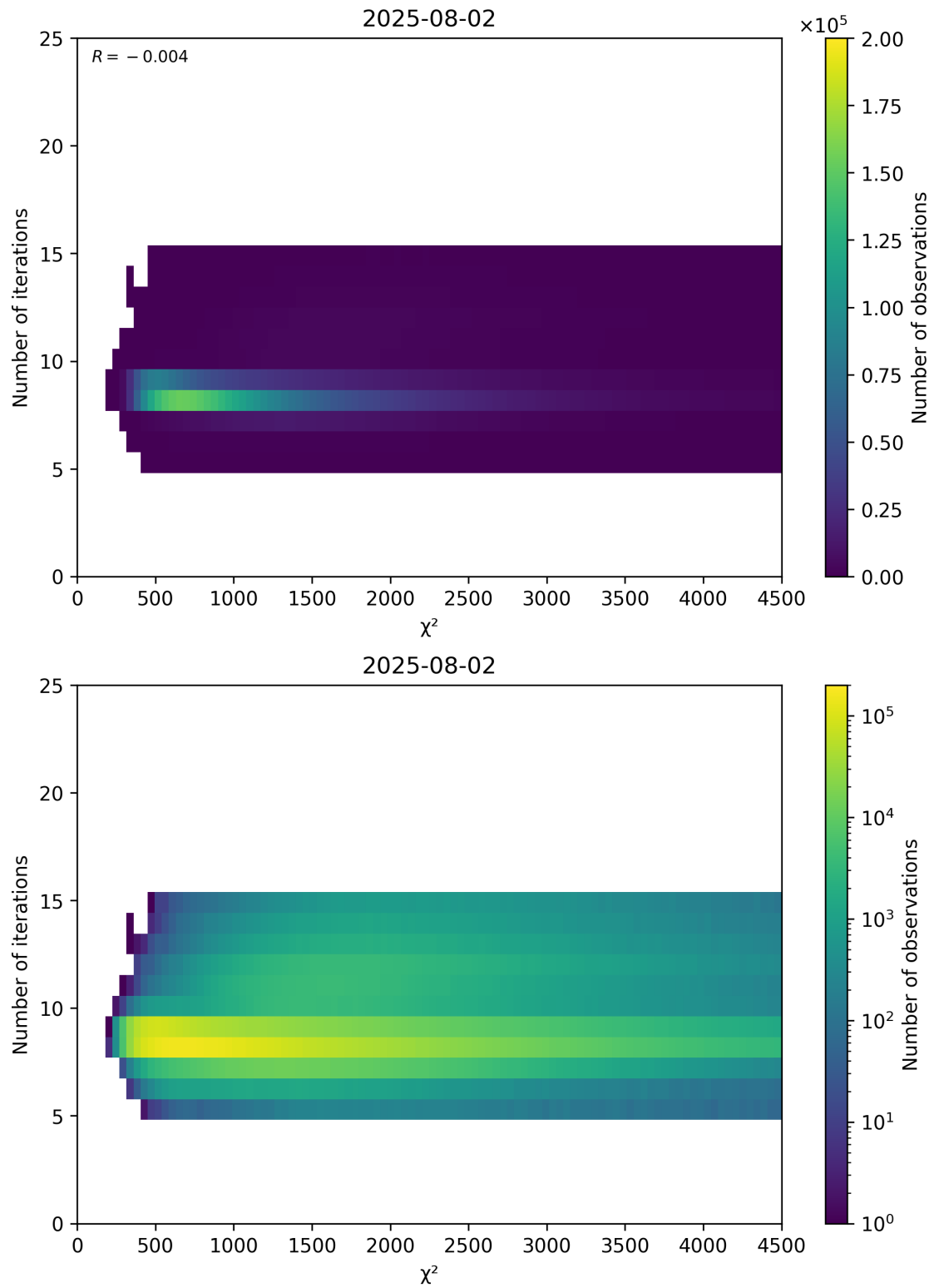
Figure 49: Scatter density plot of “ \chi^2 ” against “Number of iterations” for 2025-08-01 to 2025-08-03.
