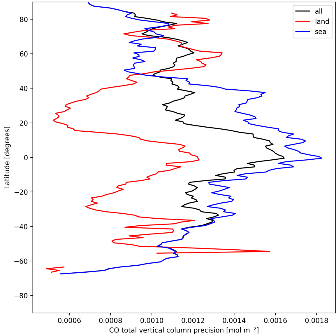
Figure 12: Zonal average of "CO total vertical column precision" for 2025-08-01 to 2025-08-03.
