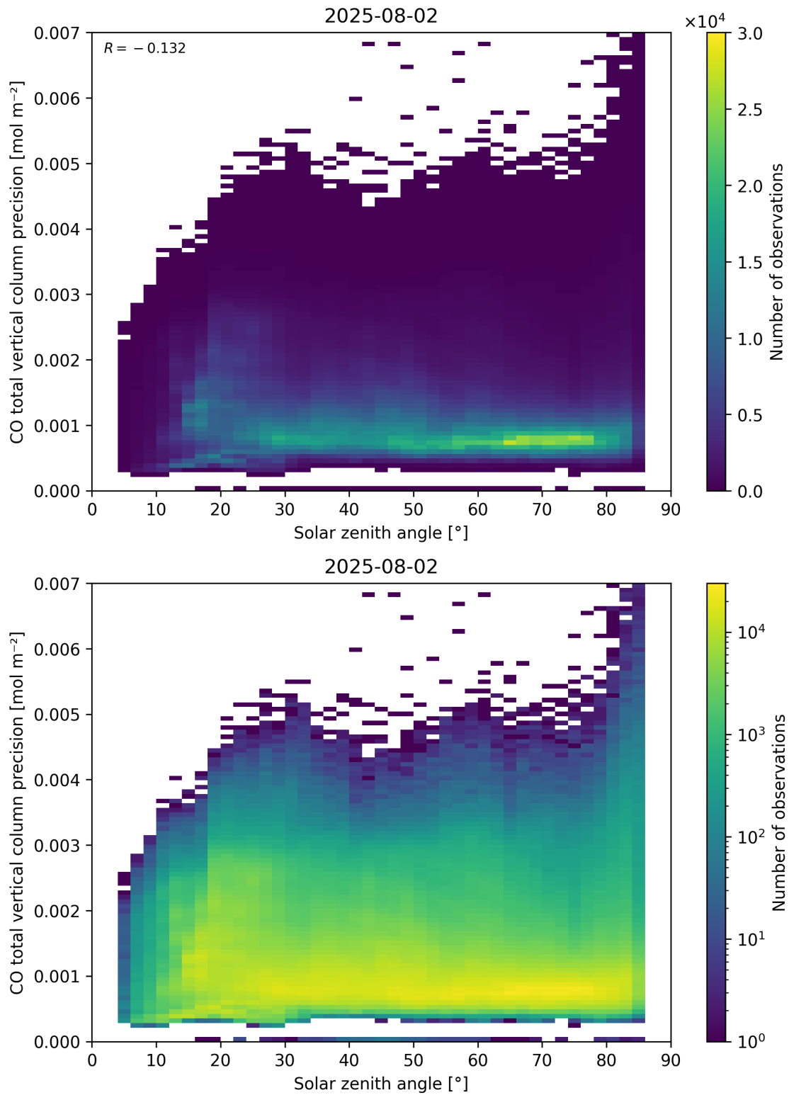
Figure 63: Scatter density plot of “Solar zenith angle” against “CO total vertical column precision” for 2025-08-01 to 2025-08-03.
