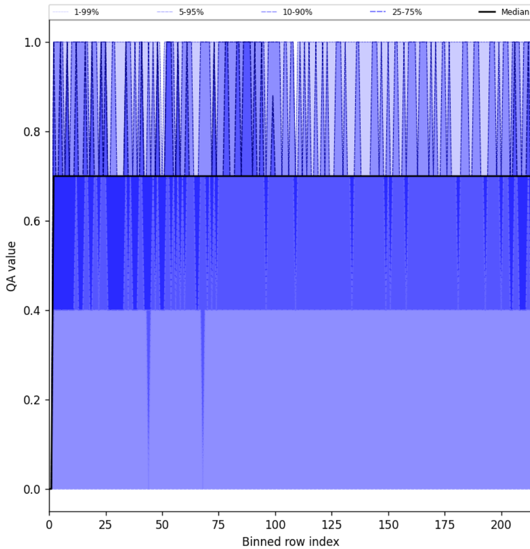
Figure 25: Along track statistics of “QA value” for 2025-08-01 to 2025-08-03
