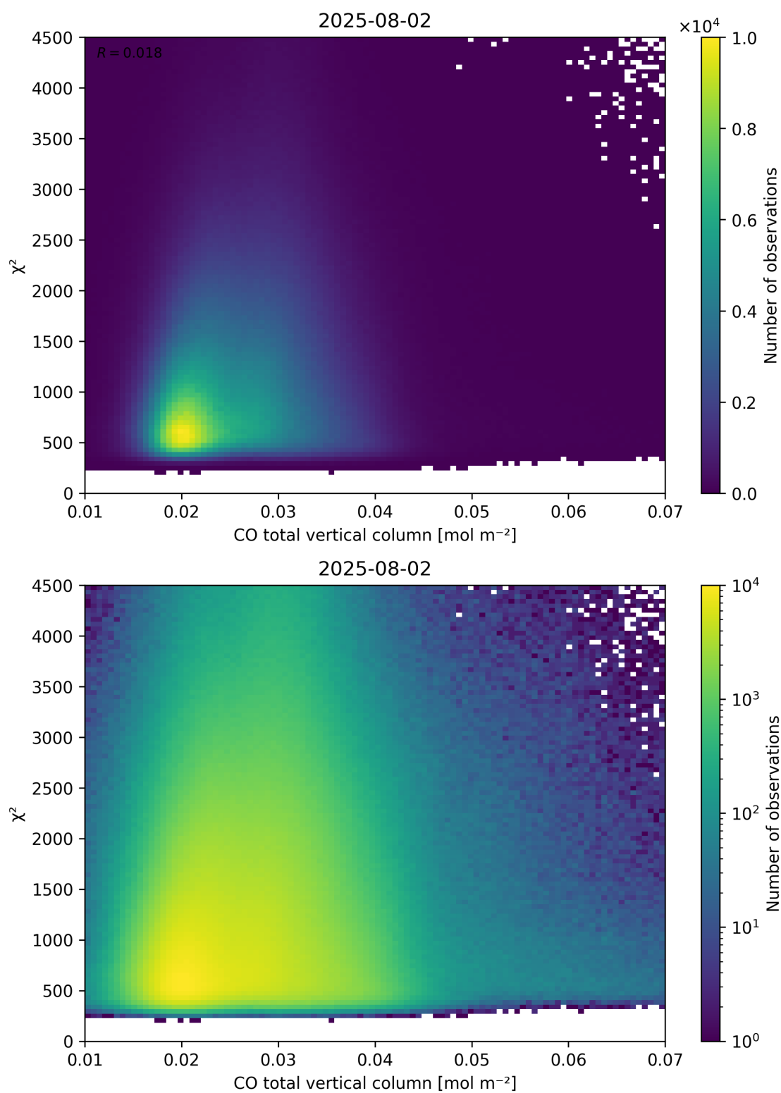
Figure 35: Scatter density plot of “CO total vertical column” against “ \chi^2 ” for 2025-08-01 to 2025-08-03.
