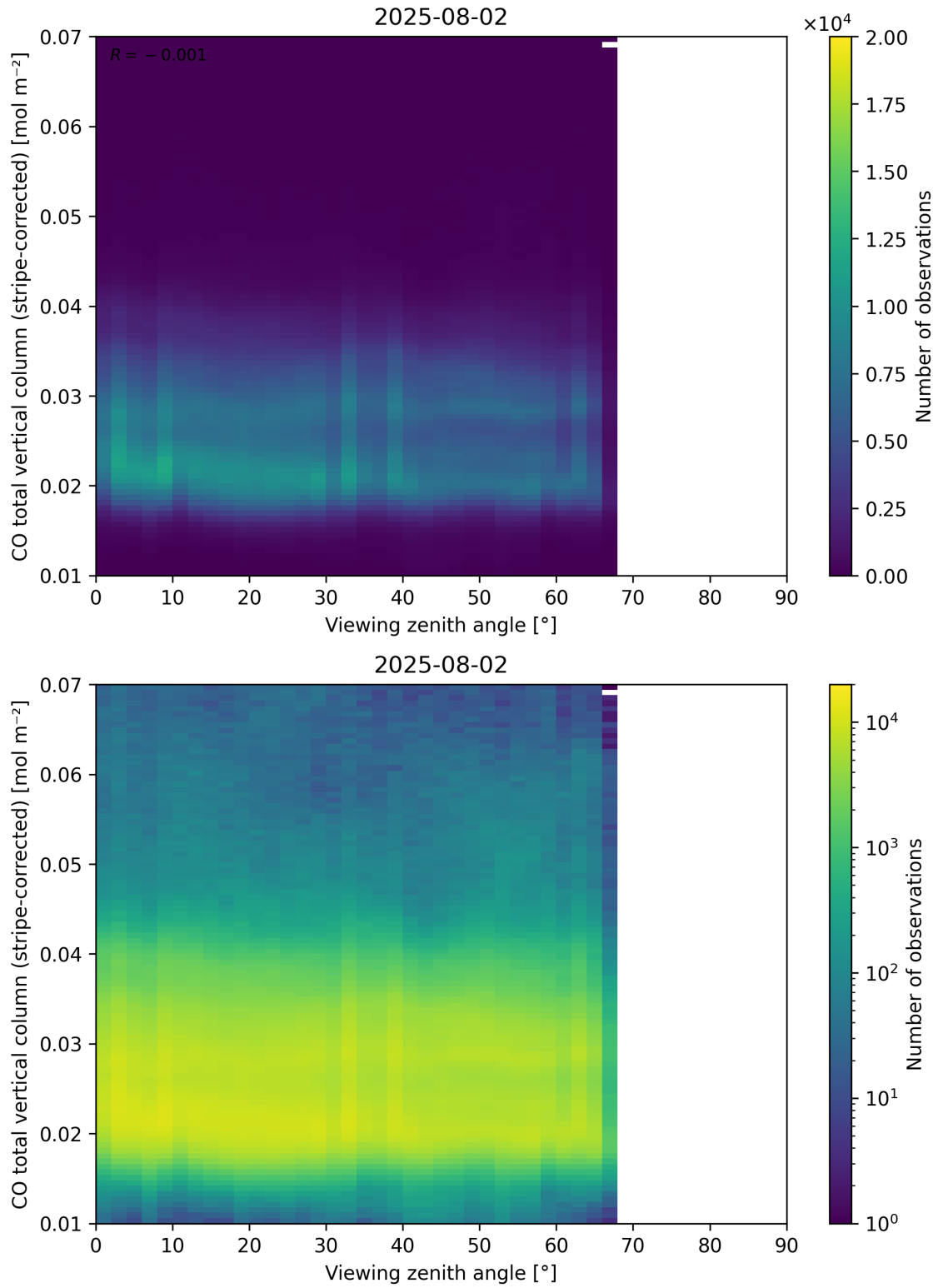
Figure 70: Scatter density plot of “Viewing zenith angle” against “CO total vertical column (stripe-corrected)” for 2025-08-01 to 2025-08-03.
