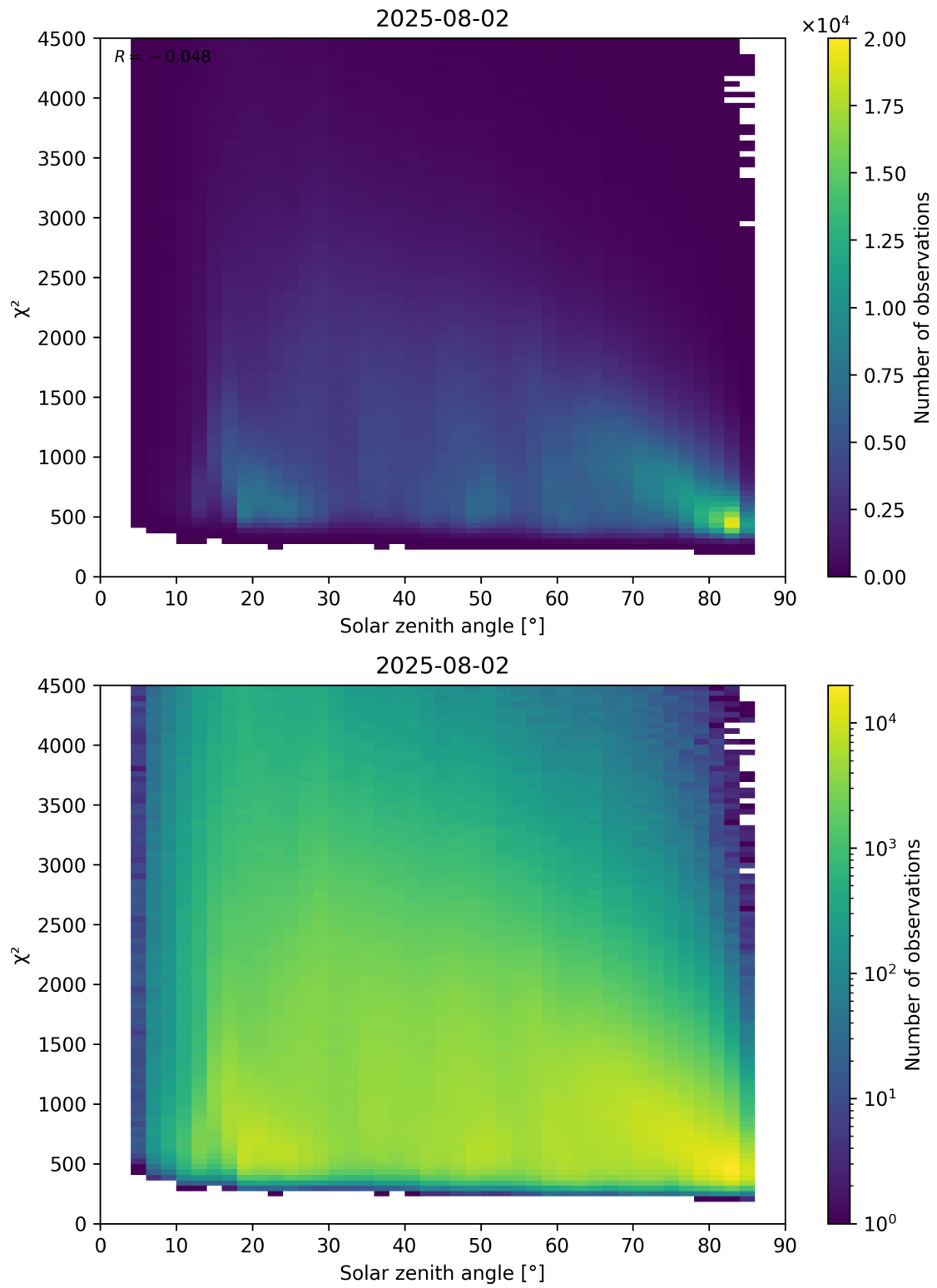
Figure 64: Scatter density plot of “Solar zenith angle” against “ \chi^2 ” for 2025-08-01 to 2025-08-03.
