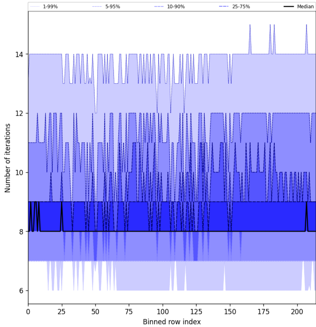
Figure 32: Along track statistics of “Number of iterations” for 2025-08-01 to 2025-08-03
