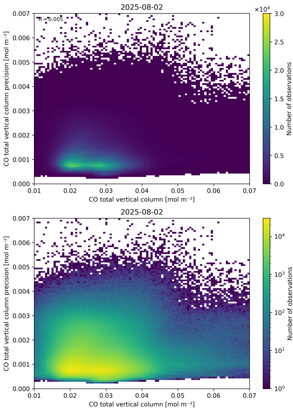
Figure 34: Scatter density plot of “CO total vertical column” against “CO total vertical column precision” for 2025-08-01 to 2025-08-03.
