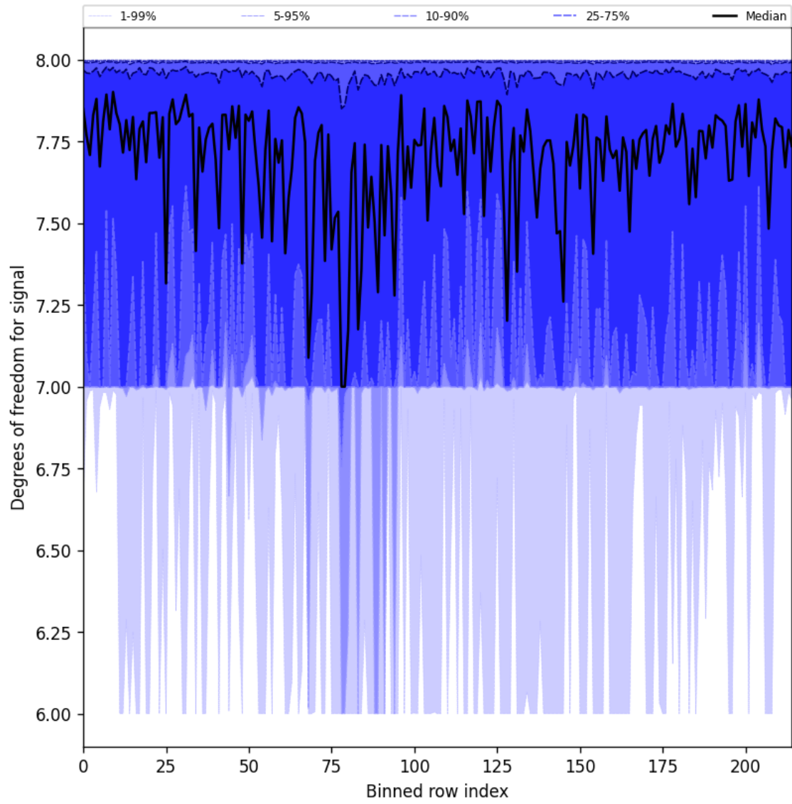
Figure 31: Along track statistics of “Degrees of freedom for signal” for 2025-08-01 to 2025-08-03
