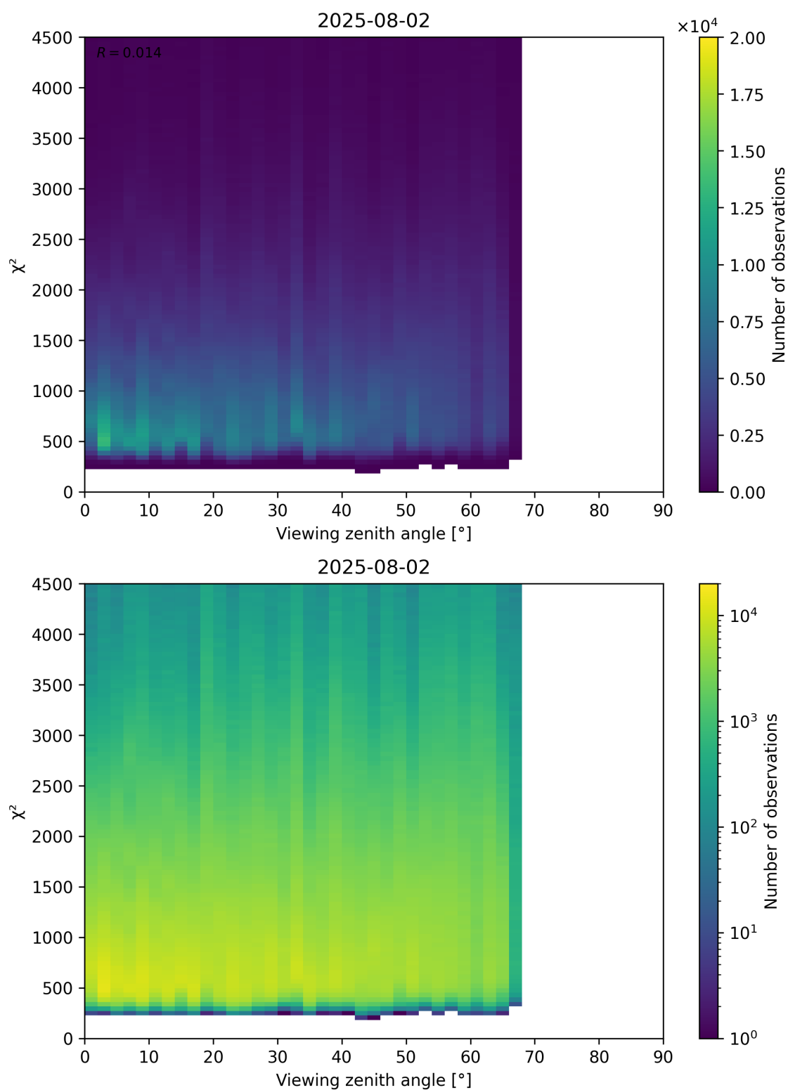
Figure 72: Scatter density plot of “Viewing zenith angle” against “ \chi^2 ” for 2025-08-01 to 2025-08-03.
