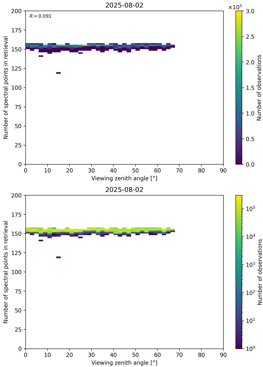
Figure 76: Scatter density plot of “Viewing zenith angle” against “Number of spectral points in retrieval” for 2025-08-01 to 2025-08-03.
