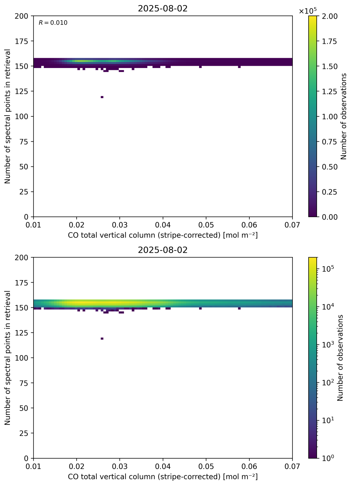
Figure 40: Scatter density plot of “CO total vertical column (stripe-corrected)” against “Number of spectral points in retrieval” for 2025-08-01 to 2025-08-03.
