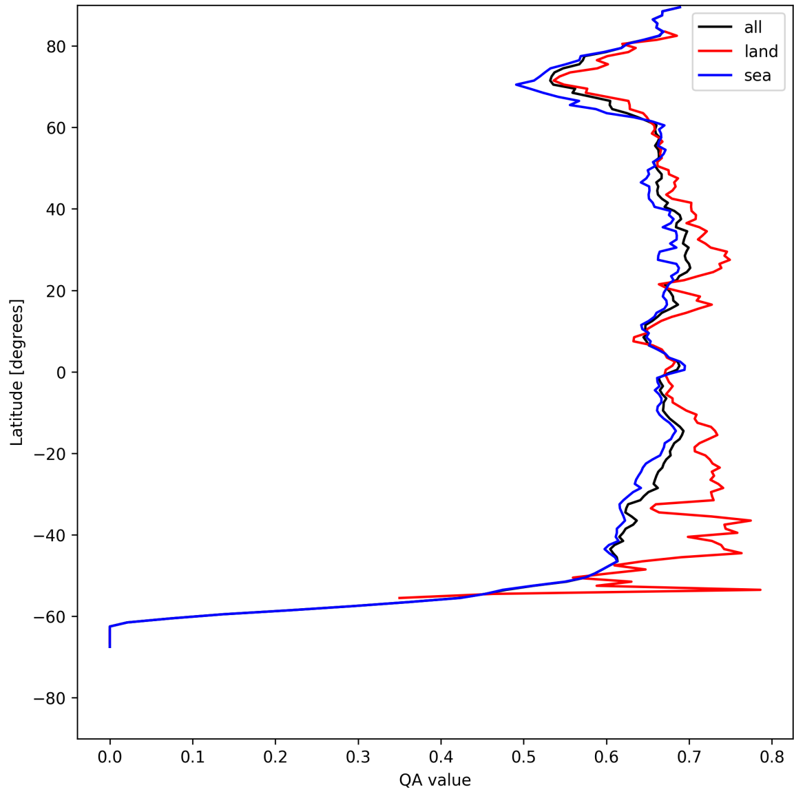
Figure 9: Zonal average of “QA value” for 2025-08-01 to 2025-08-03.
