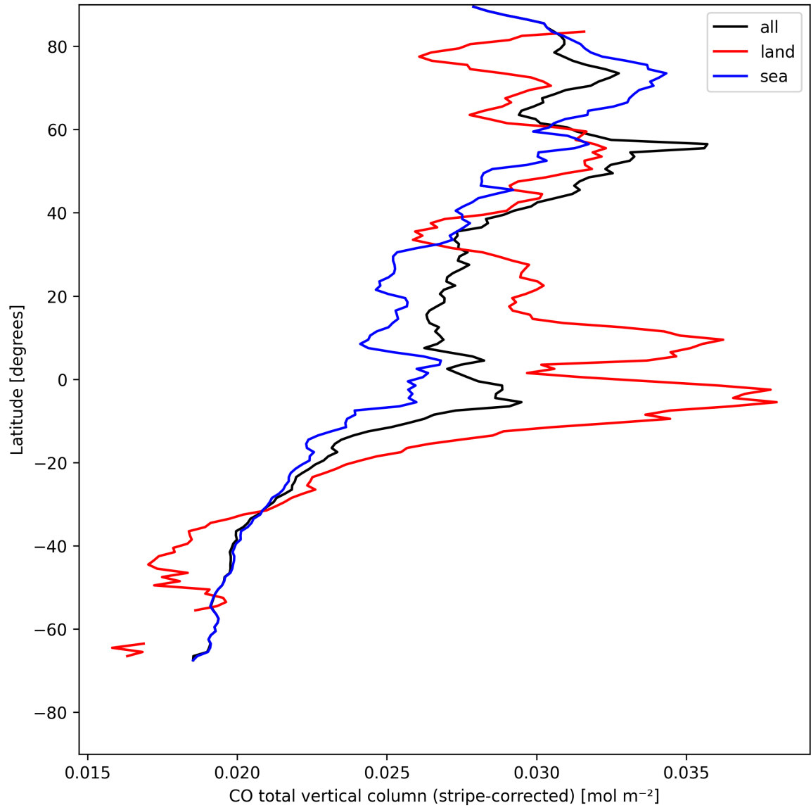
Figure 11: Zonal average of “CO total vertical column (stripe-corrected)” for 2025-08-01 to 2025-08-03.
