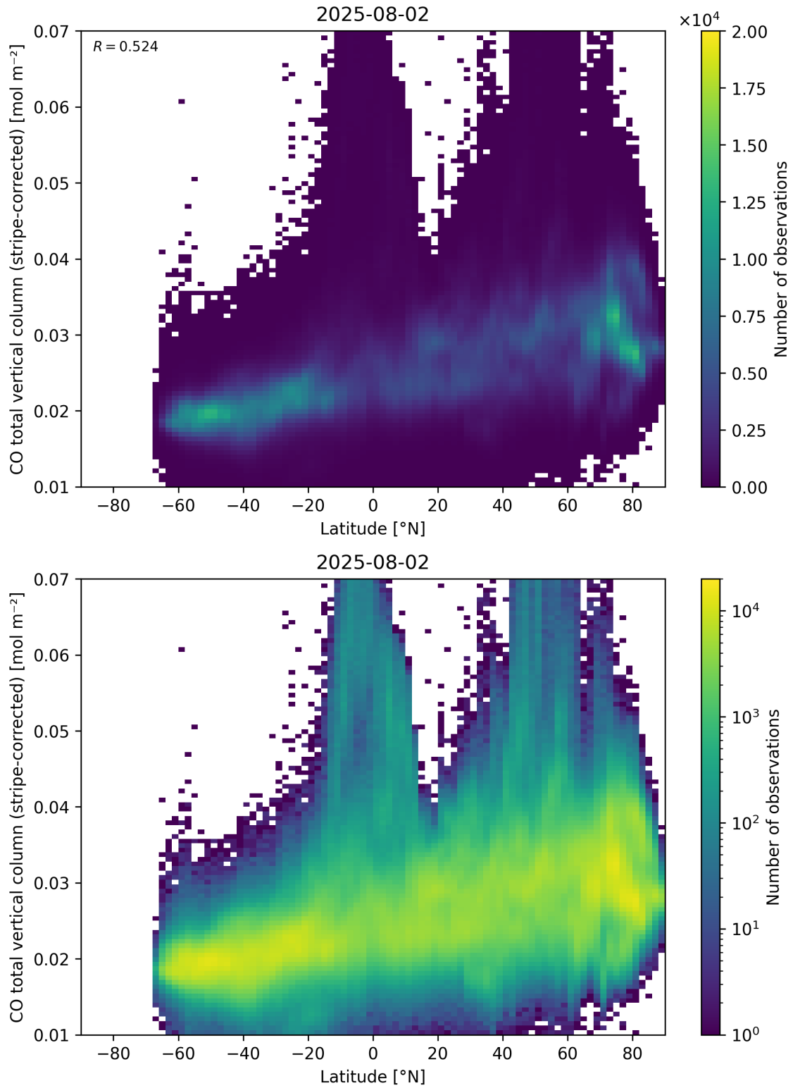
Figure 52: Scatter density plot of “Latitude” against “CO total vertical column (stripe-corrected)” for 2025-08-01 to 2025-08-03.
