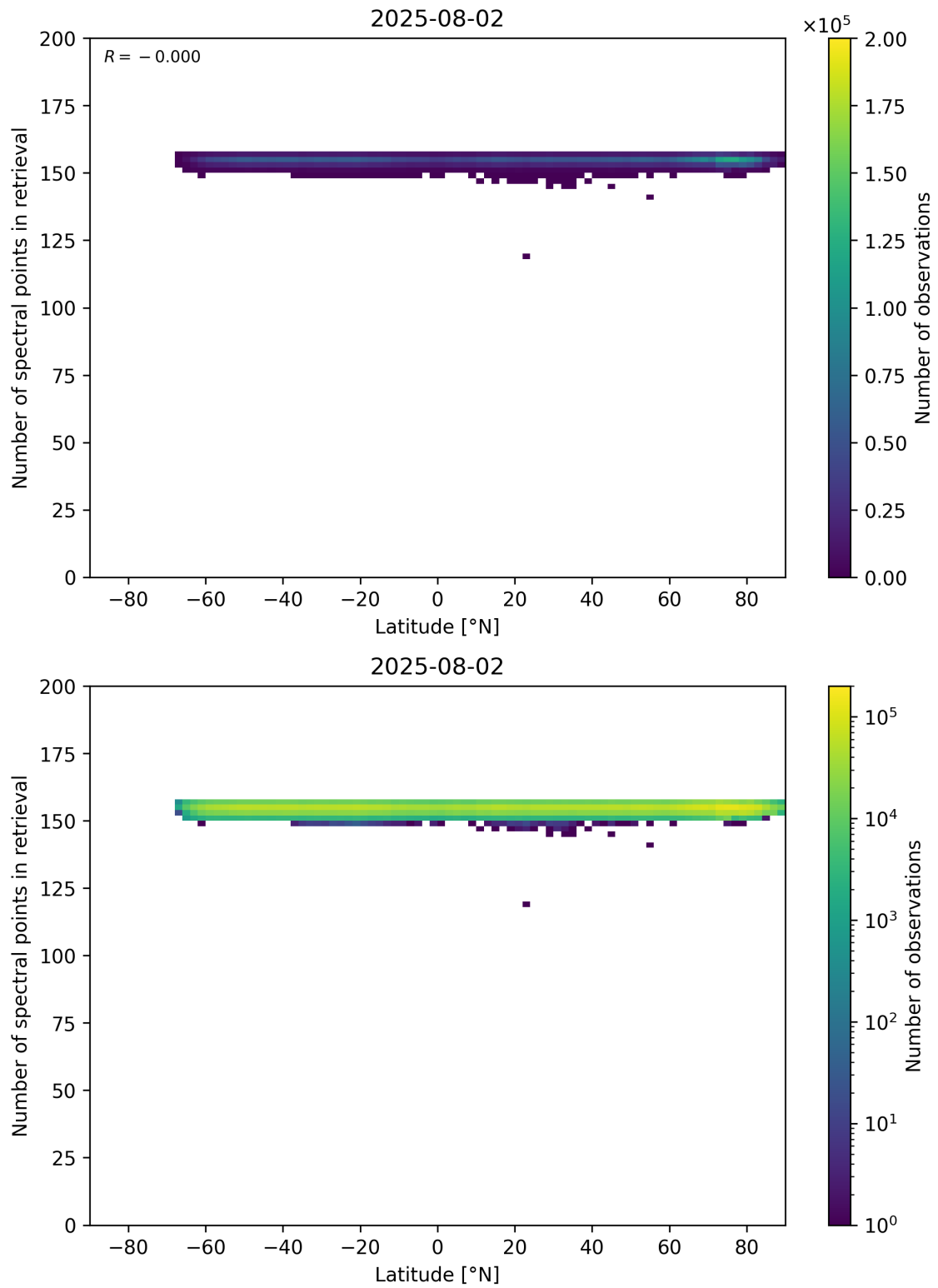
Figure 57: Scatter density plot of “Latitude” against “Number of spectral points in retrieval” for 2025-08-01 to 2025-08-03.
