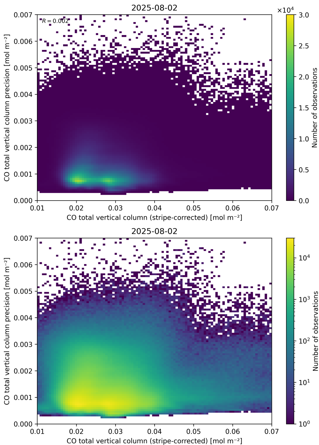
Figure 36: Scatter density plot of “CO total vertical column (stripe-corrected)” against “CO total vertical column precision” for 2025-08-01 to 2025-08-03.
