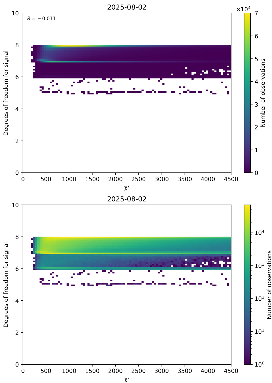
Figure 48: Scatter density plot of “ \chi^2 ” against “Degrees of freedom for signal” for 2025-08-01 to 2025-08-03.
