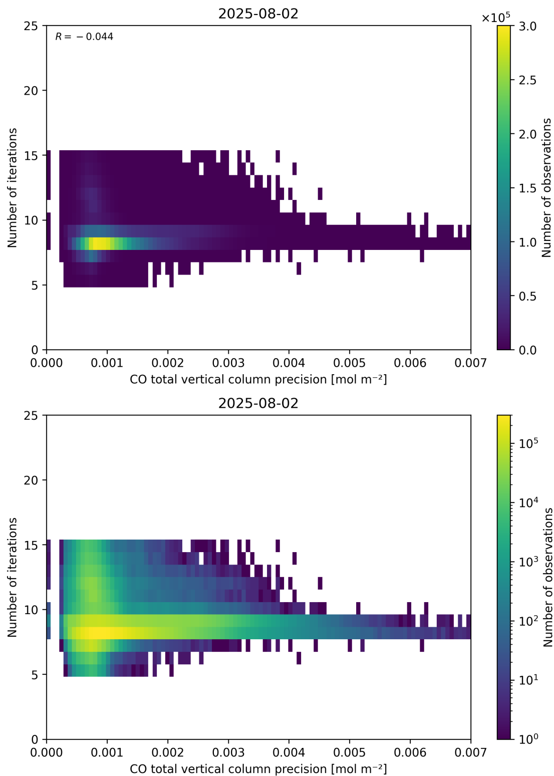
Figure 46: Scatter density plot of “CO total vertical column precision” against “Number of iterations” for 2025-08-01 to 2025-08-03.
