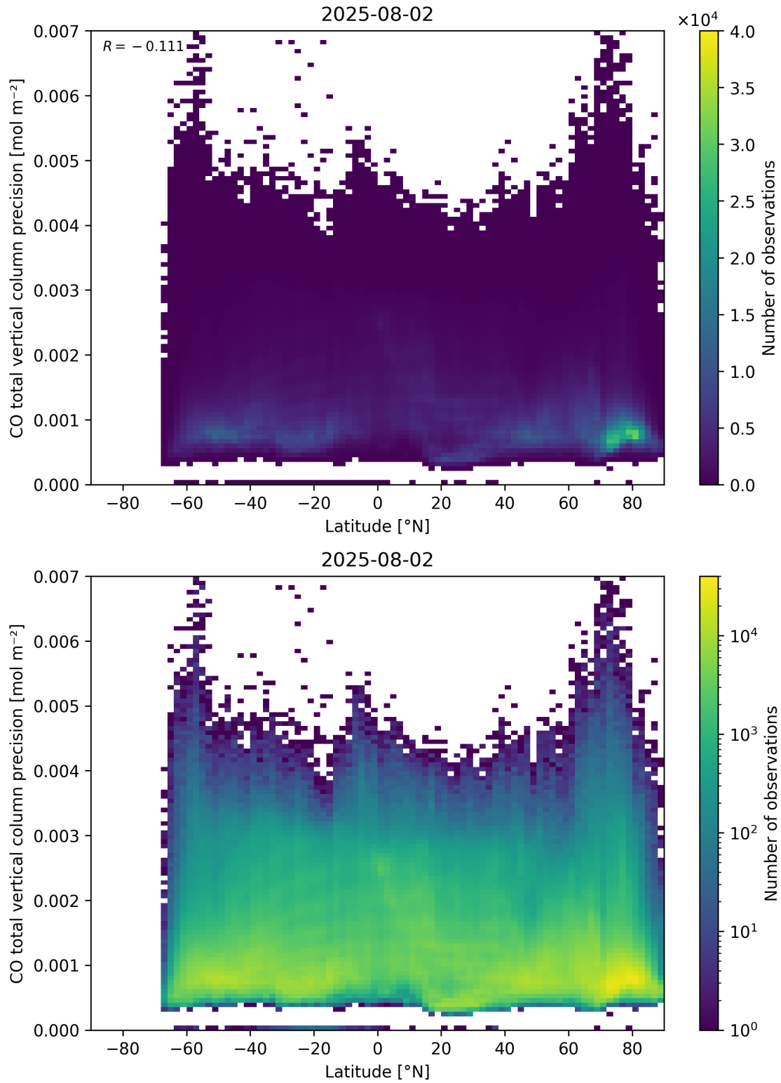
Figure 53: Scatter density plot of “Latitude” against “CO total vertical column precision” for 2025-08-01 to 2025-08-03.
