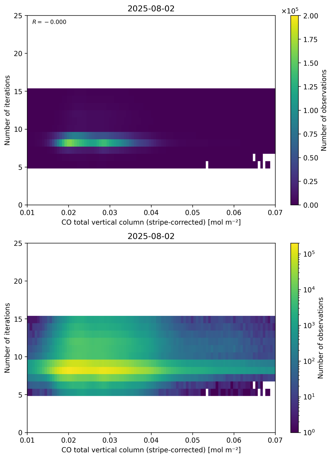
Figure 39: Scatter density plot of “CO total vertical column (stripe-corrected)” against “Number of iterations” for 2025-08-01 to 2025-08-03.
