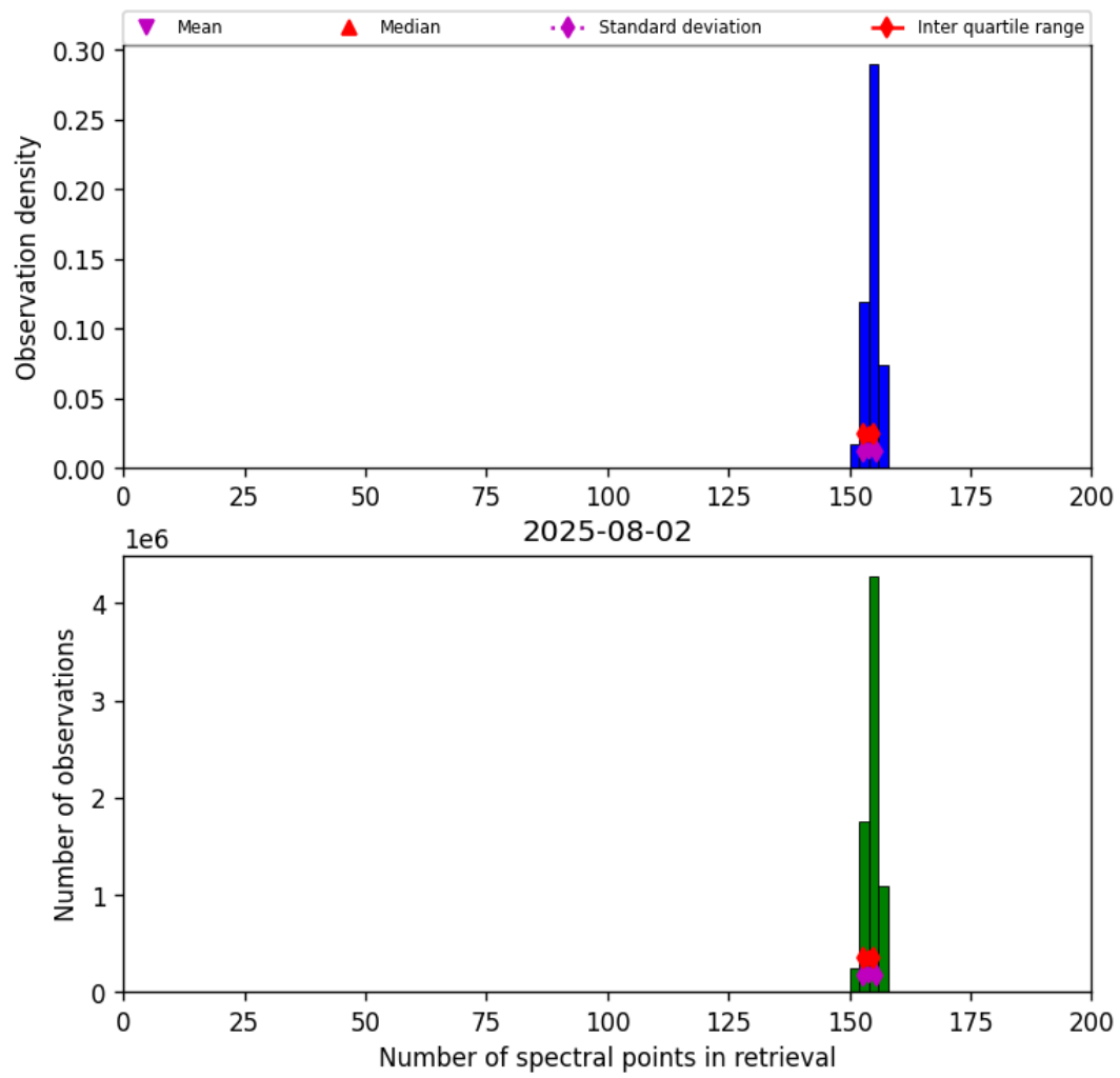
Figure 21: Histogram of “Number of spectral points in retrieval” for 2025-08-01 to 2025-08-03
