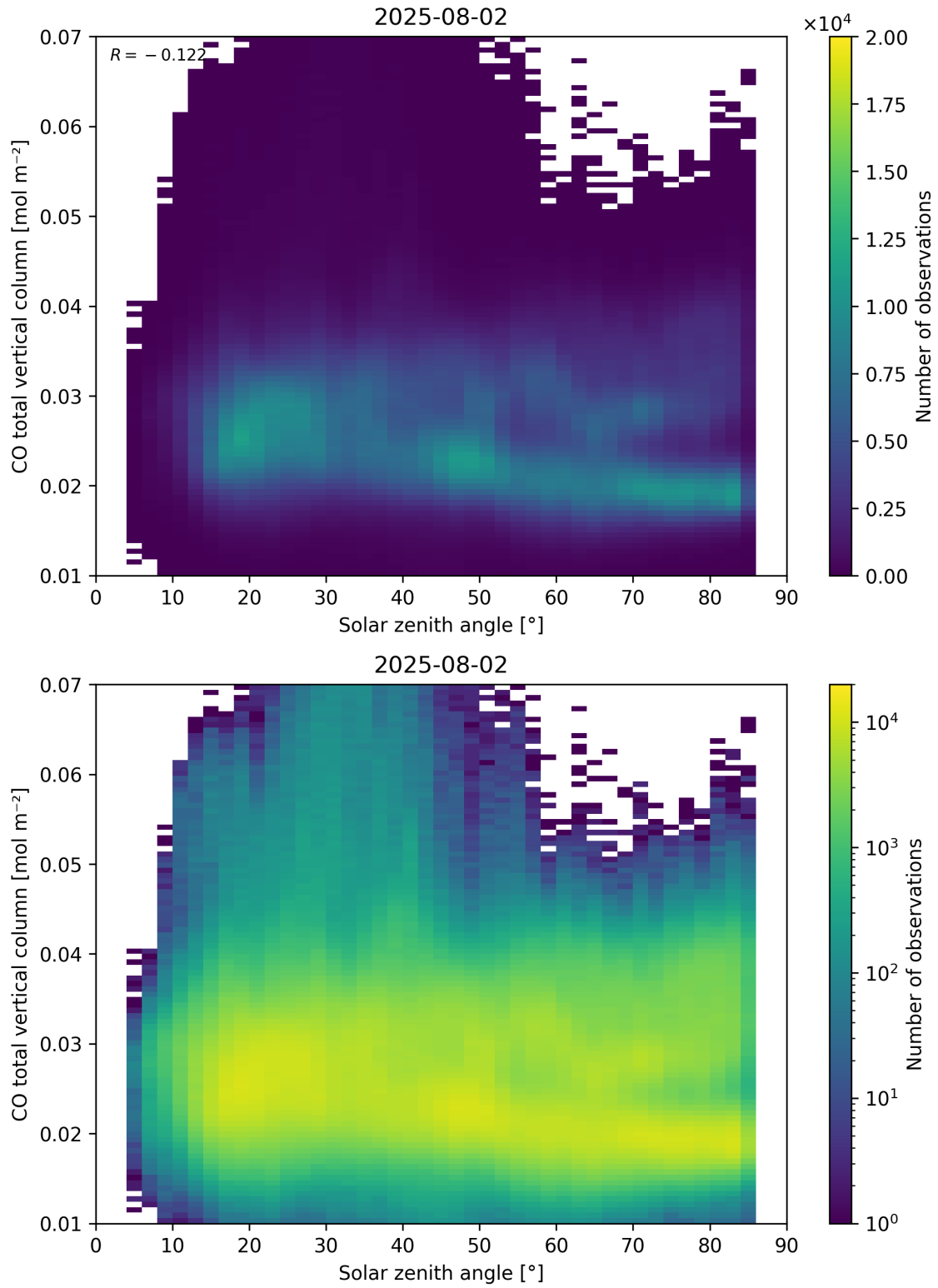
Figure 61: Scatter density plot of “Solar zenith angle” against “CO total vertical column” for 2025-08-01 to 2025-08-03.
