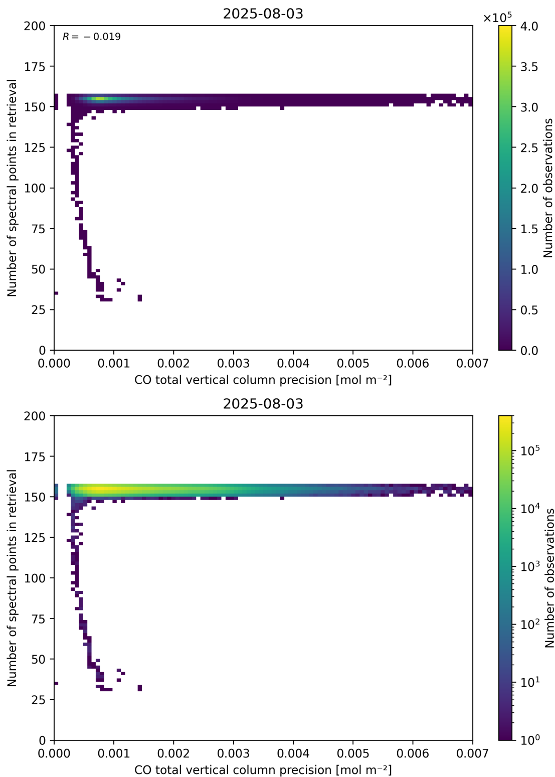
Figure 47: Scatter density plot of “CO total vertical column precision” against “Number of spectral points in retrieval” for 2025-08-03 to 2025-08-04.
