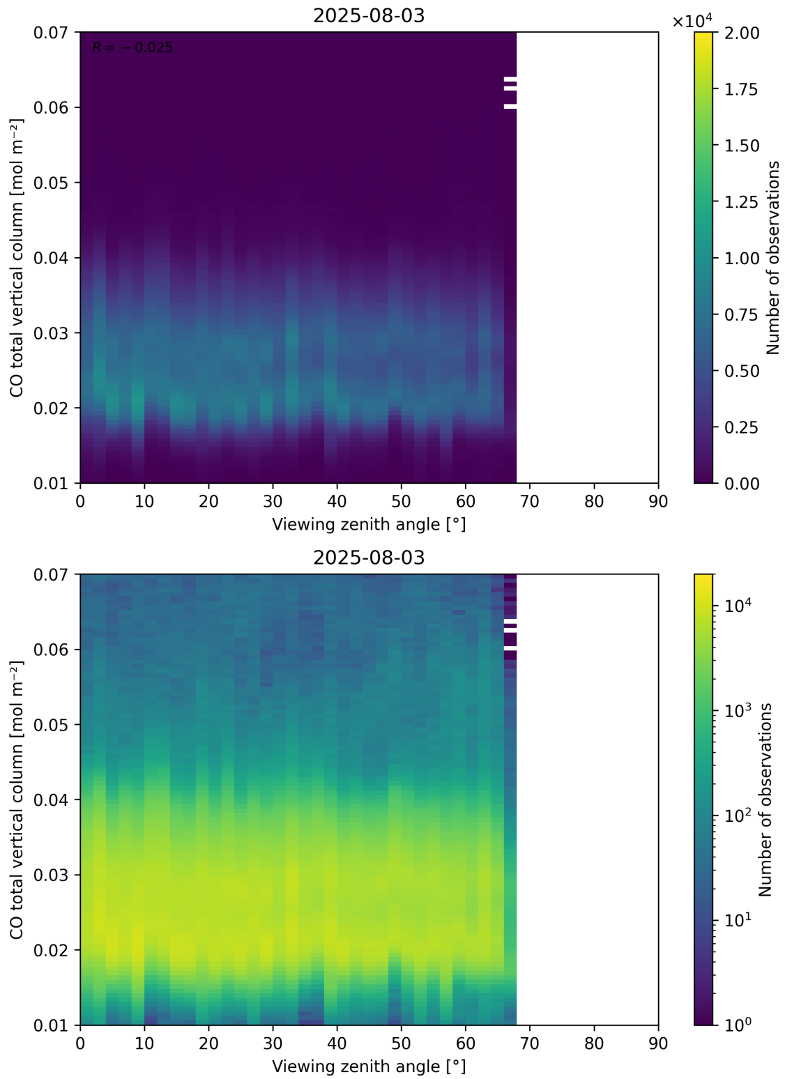
Figure 69: Scatter density plot of “Viewing zenith angle” against “CO total vertical column” for 2025-08-03 to 2025-08-04.
