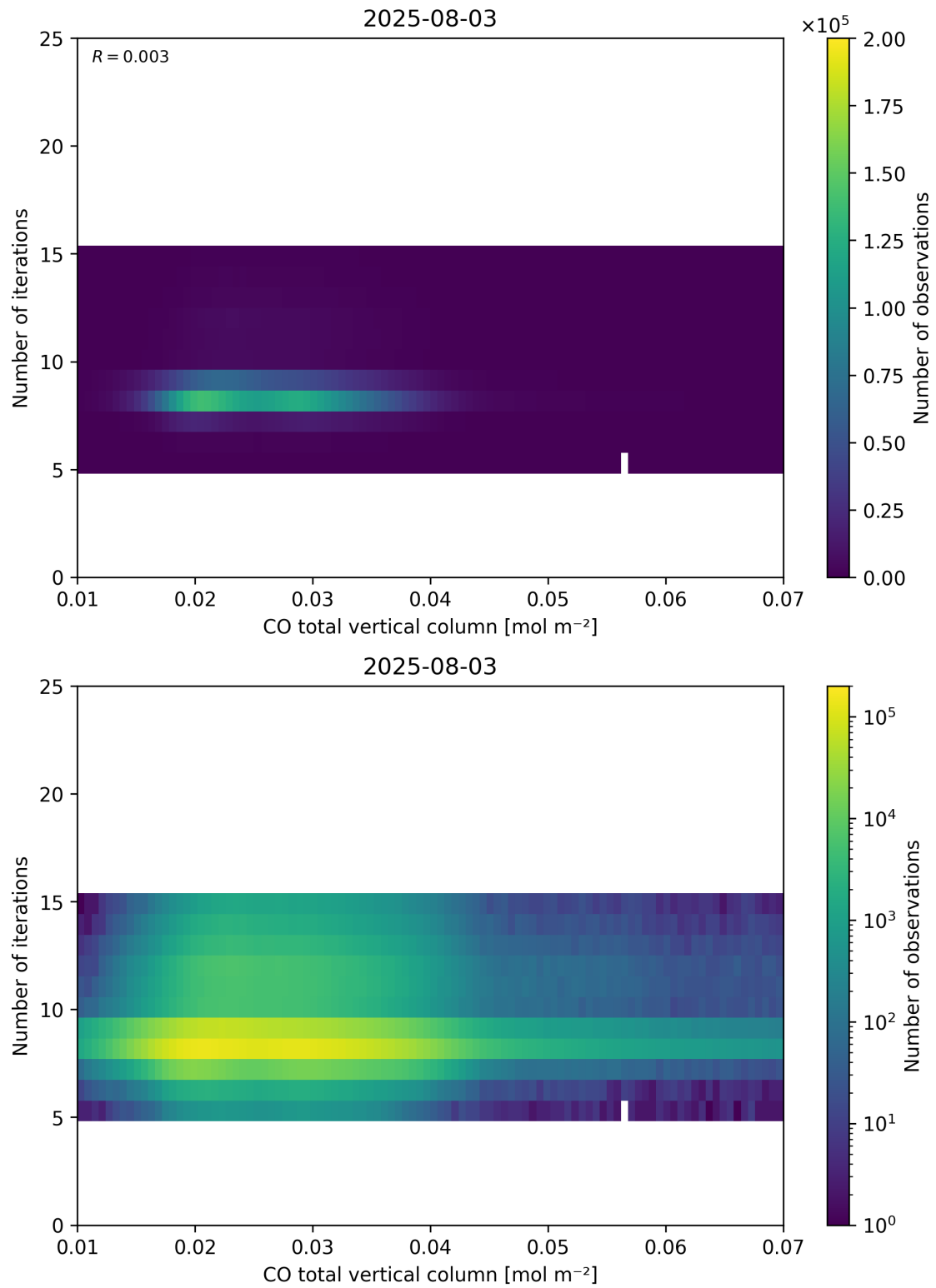
Figure 42: Scatter density plot of “CO total vertical column” against “Number of iterations” for 2025-08-03 to 2025-08-04.
