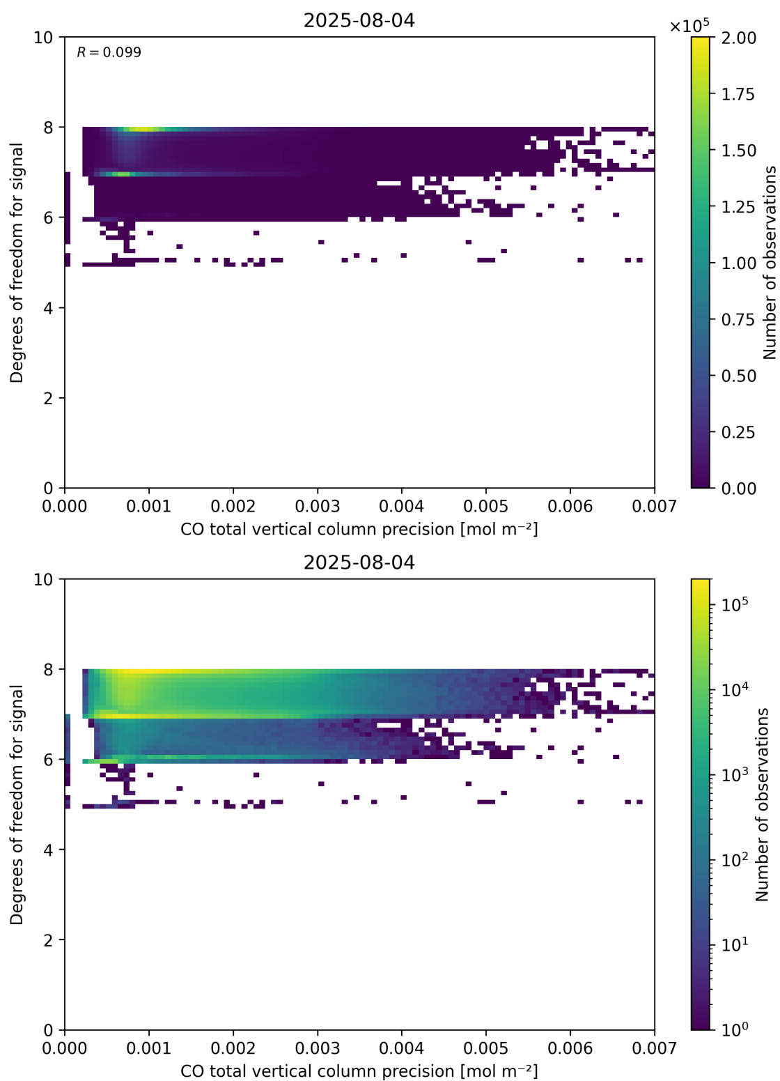
Figure 45: Scatter density plot of “CO total vertical column precision” against “Degrees of freedom for signal” for 2025-08-04 to 2025-08-05.
