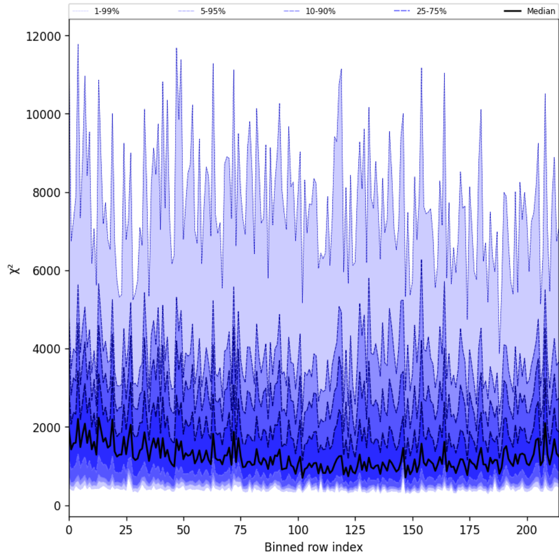
Figure 30: Along track statistics of “ \chi^2 ” for 2025-08-04 to 2025-08-05
