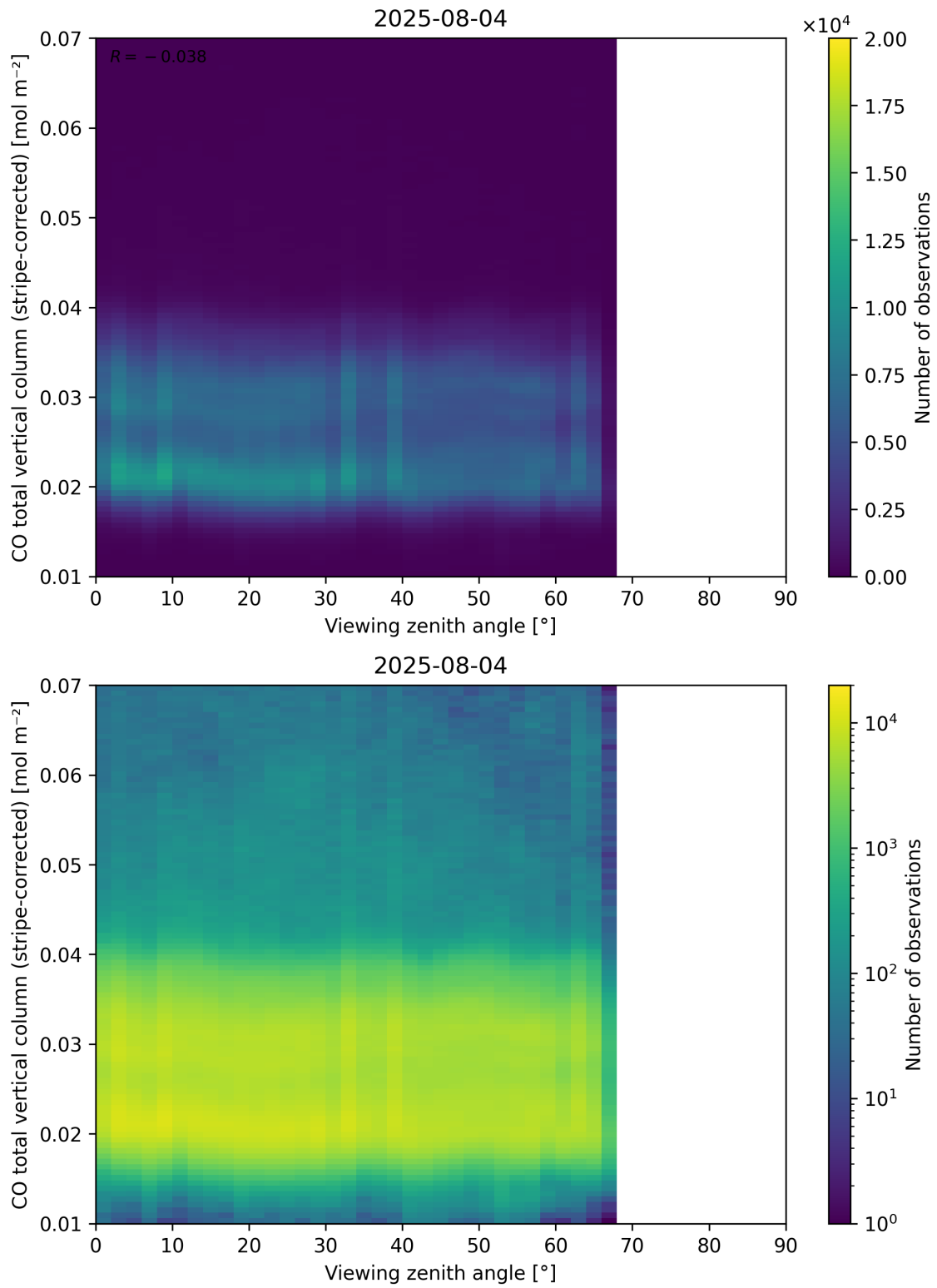
Figure 70: Scatter density plot of “Viewing zenith angle” against “CO total vertical column (stripe-corrected)” for 2025-08-04 to 2025-08-05.
