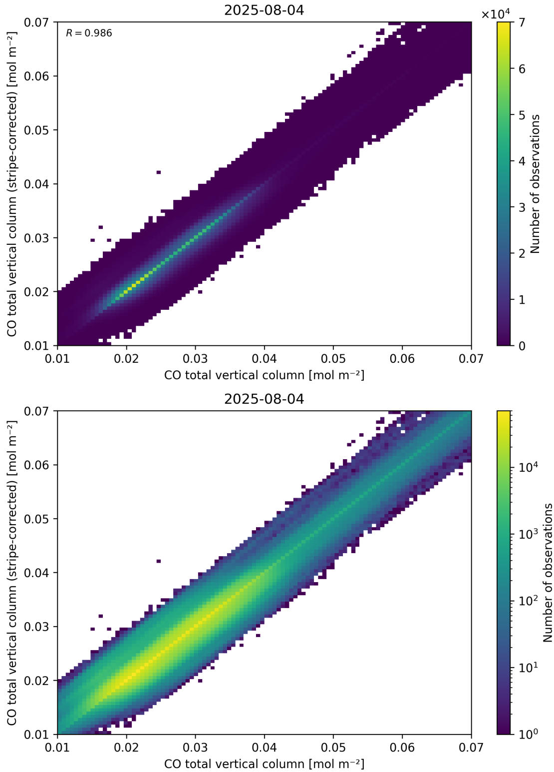
Figure 33: Scatter density plot of “CO total vertical column” against “CO total vertical column (stripe-corrected)” for 2025-08-04 to 2025-08-05.
