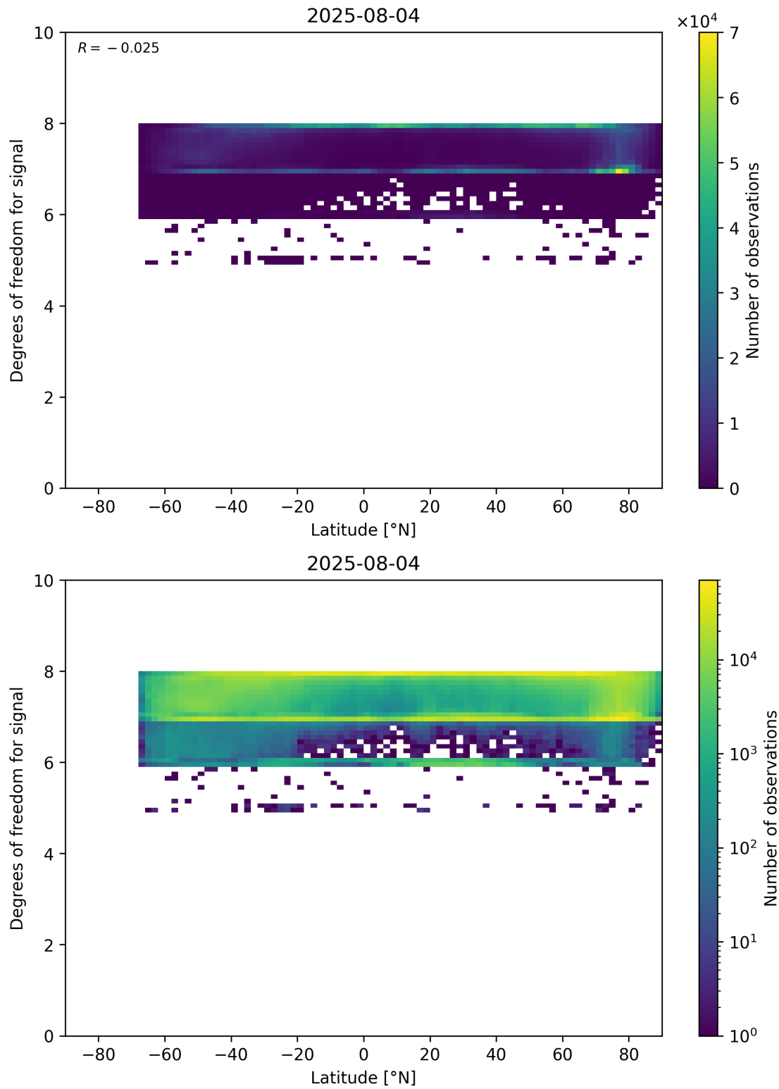
Figure 55: Scatter density plot of “Latitude” against “Degrees of freedom for signal” for 2025-08-04 to 2025-08-05.
