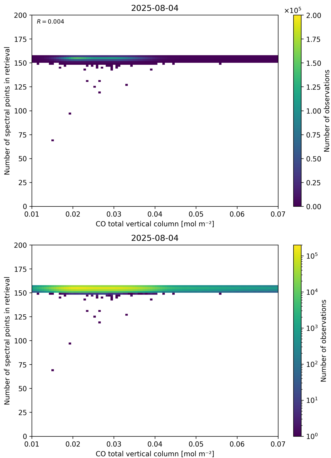
Figure 43: Scatter density plot of “CO total vertical column” against “Number of spectral points in retrieval” for 2025-08-04 to 2025-08-05.
