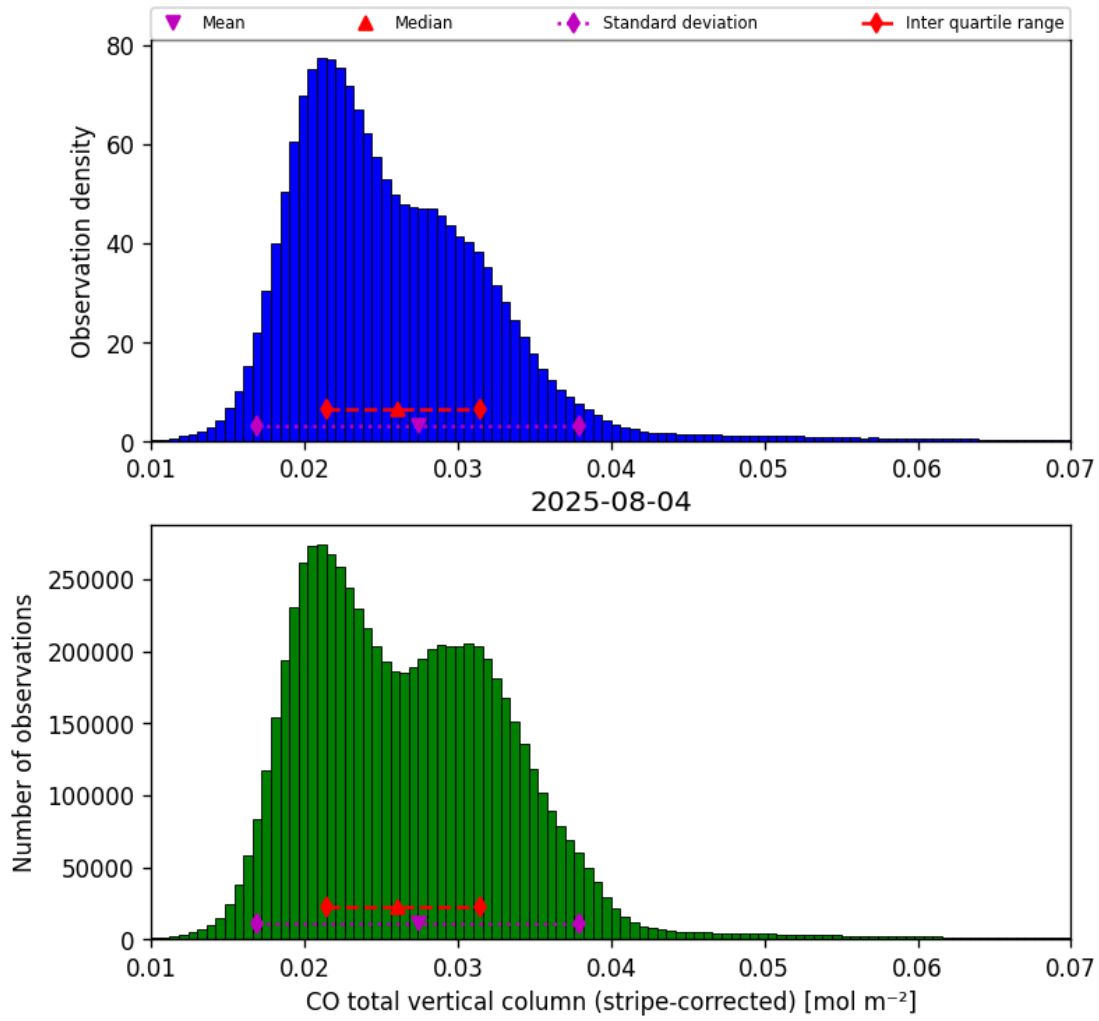
Figure 19: Histogram of “CO total vertical column (stripe-corrected)” for 2025-08-04 to 2025-08-05
