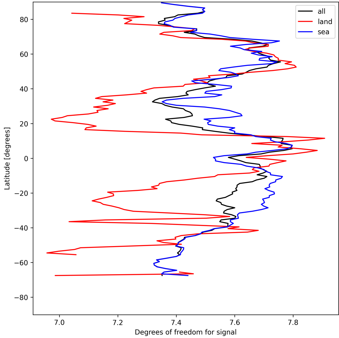
Figure 15: Zonal average of “Degrees of freedom for signal” for 2025-08-04 to 2025-08-05.
