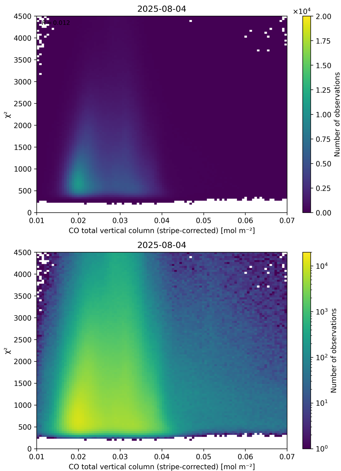
Figure 37: Scatter density plot of “CO total vertical column (stripe-corrected)” against “ \chi^2 ” for 2025-08-04 to 2025-08-05.
