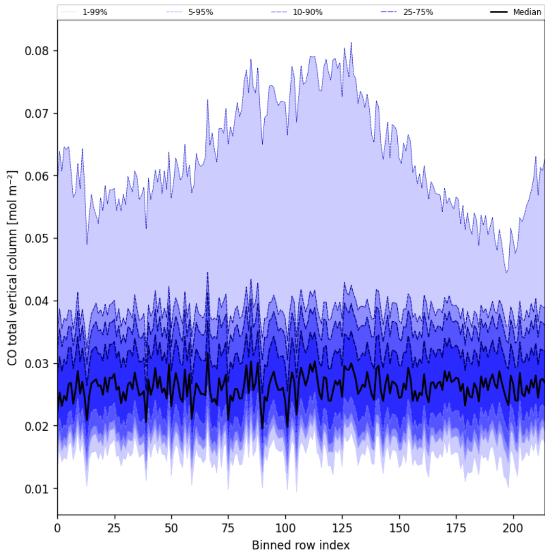
Figure 26: Along track statistics of “CO total vertical column” for 2025-08-04 to 2025-08-05
