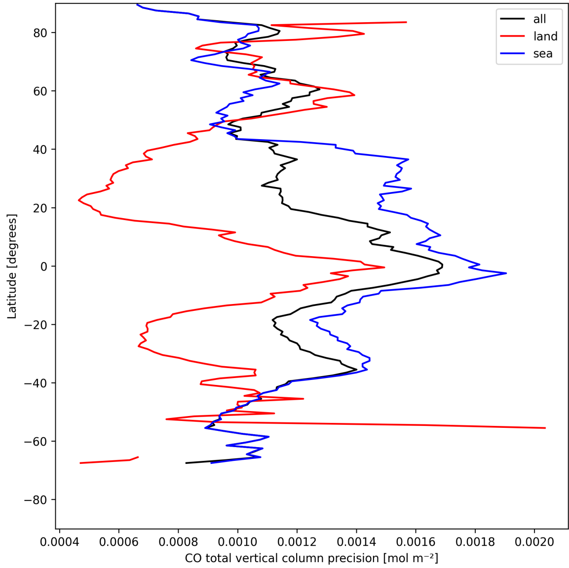
Figure 12: Zonal average of “CO total vertical column precision” for 2025-08-04 to 2025-08-05.
