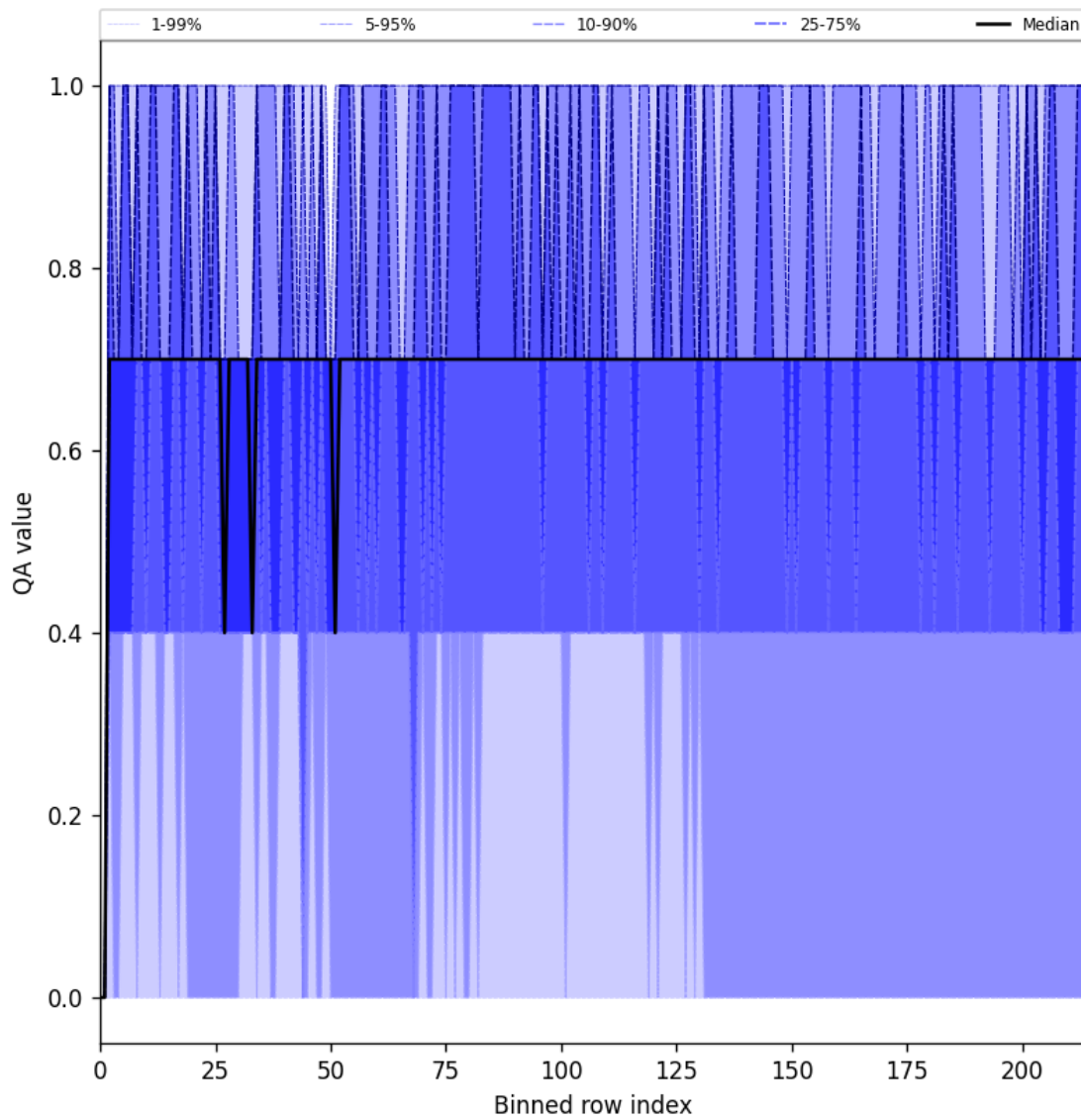
Figure 25: Along track statistics of “QA value” for 2025-08-04 to 2025-08-05
