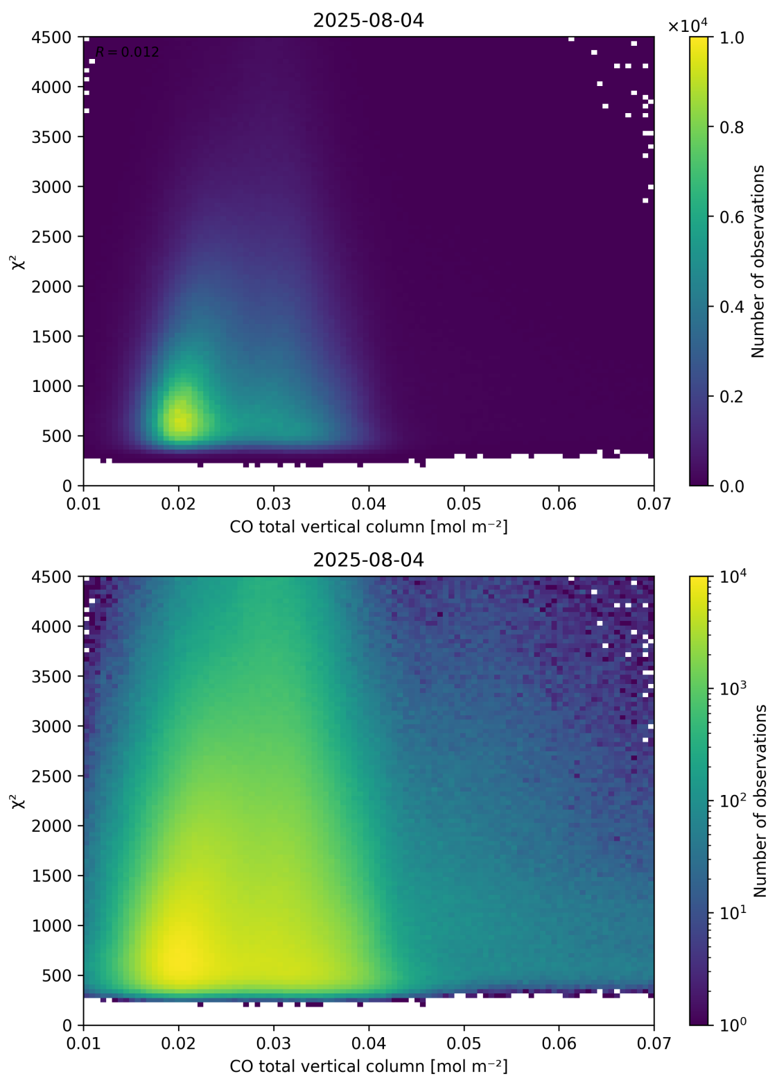
Figure 35: Scatter density plot of “CO total vertical column” against “ \chi^2 ” for 2025-08-04 to 2025-08-05.
