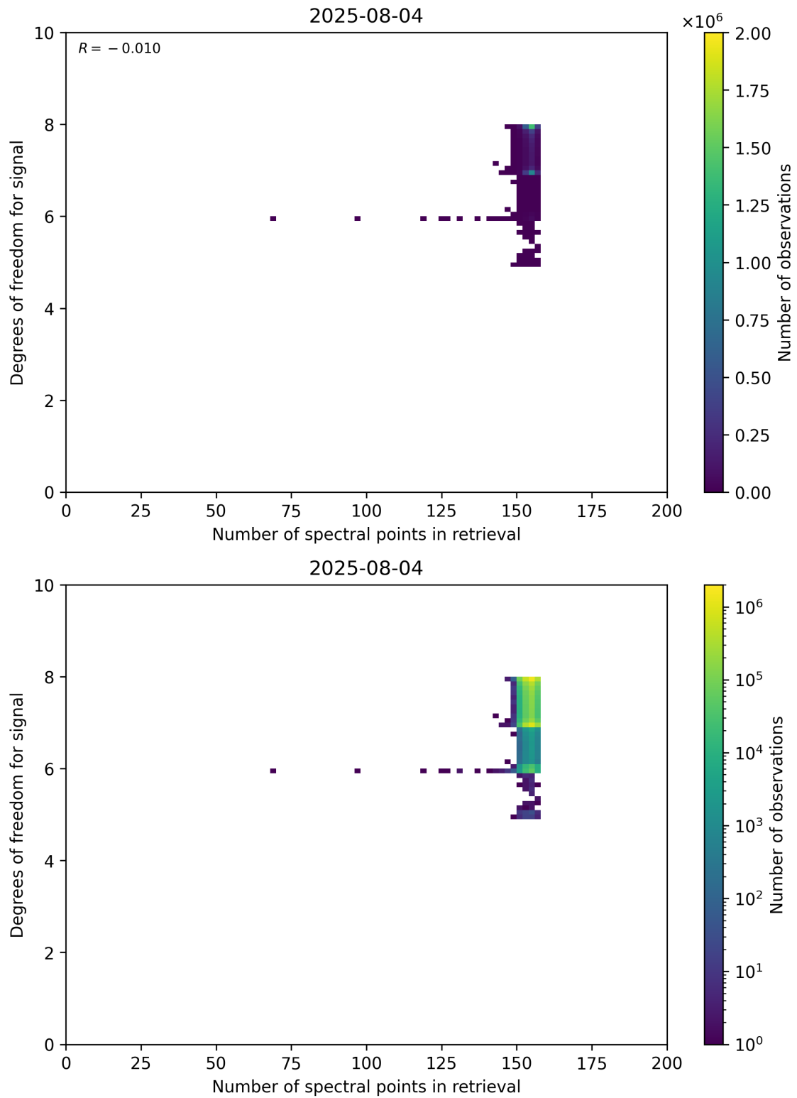
Figure 59: Scatter density plot of “Number of spectral points in retrieval” against “Degrees of freedom for signal” for 2025-08-04 to 2025-08-05.
