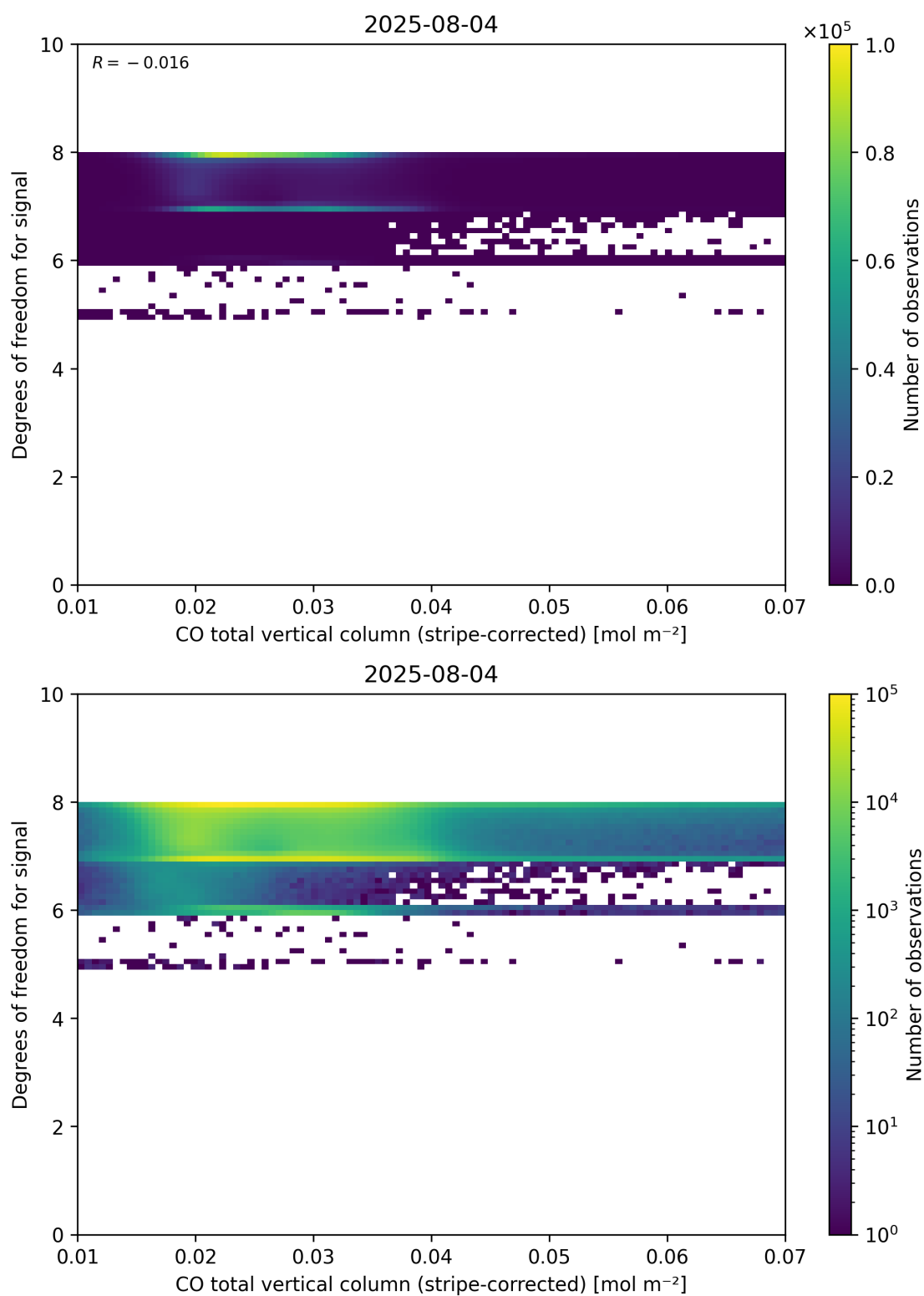
Figure 38: Scatter density plot of “CO total vertical column (stripe-corrected)” against “Degrees of freedom for signal” for 2025-08-04 to 2025-08-05.
