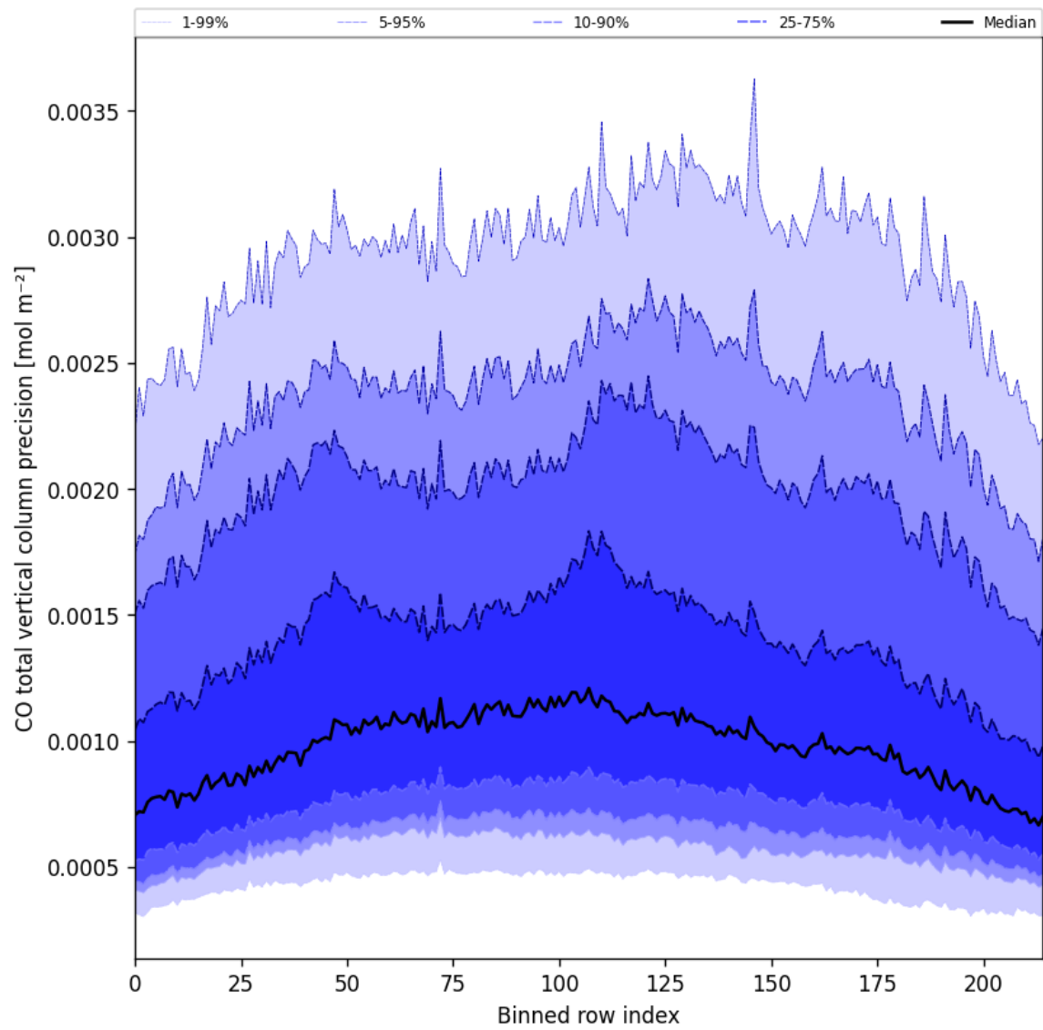
Figure 28: Along track statistics of “CO total vertical column precision” for 2025-08-04 to 2025-08-05
