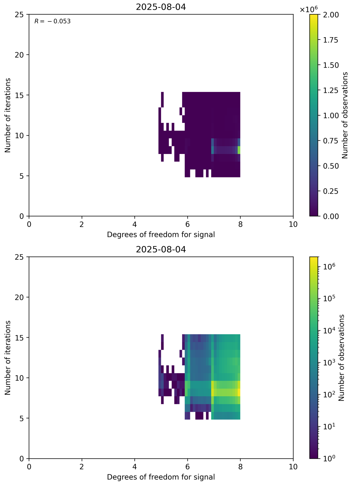
Figure 50: Scatter density plot of “Degrees of freedom for signal” against “Number of iterations” for 2025-08-04 to 2025-08-05.
