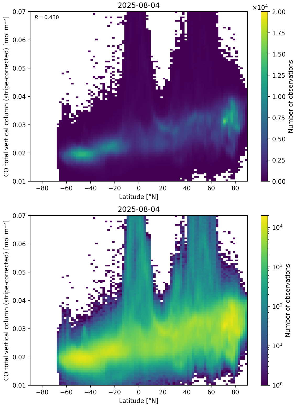
Figure 52: Scatter density plot of “Latitude” against “CO total vertical column (stripe-corrected)” for 2025-08-04 to 2025-08-05.
