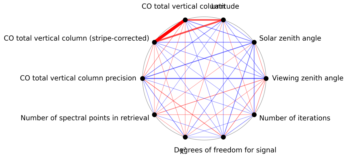
Figure 1: Map of correlation graph for 2025-08-04 to 2025-08-05.
