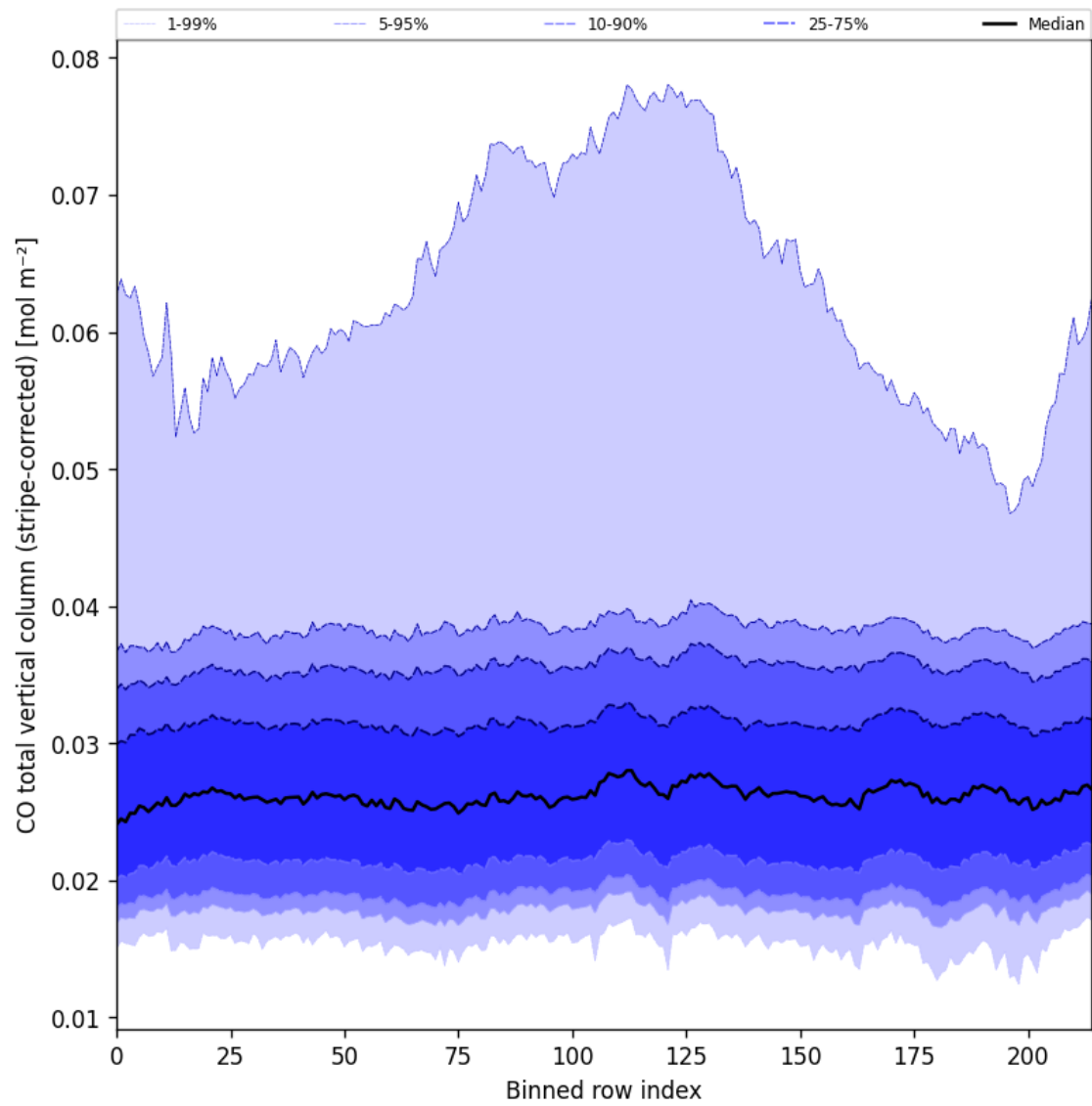
Figure 27: Along track statistics of “CO total vertical column (stripe-corrected)” for 2025-08-04 to 2025-08-05
