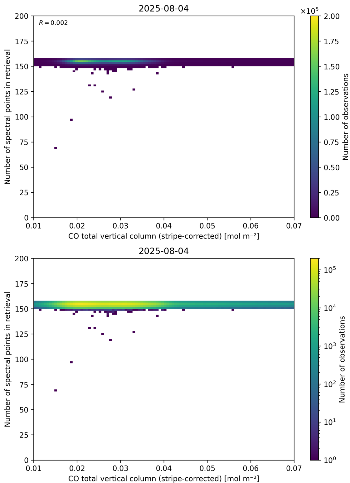
Figure 40: Scatter density plot of “CO total vertical column (stripe-corrected)” against “Number of spectral points in retrieval” for 2025-08-04 to 2025-08-05.
