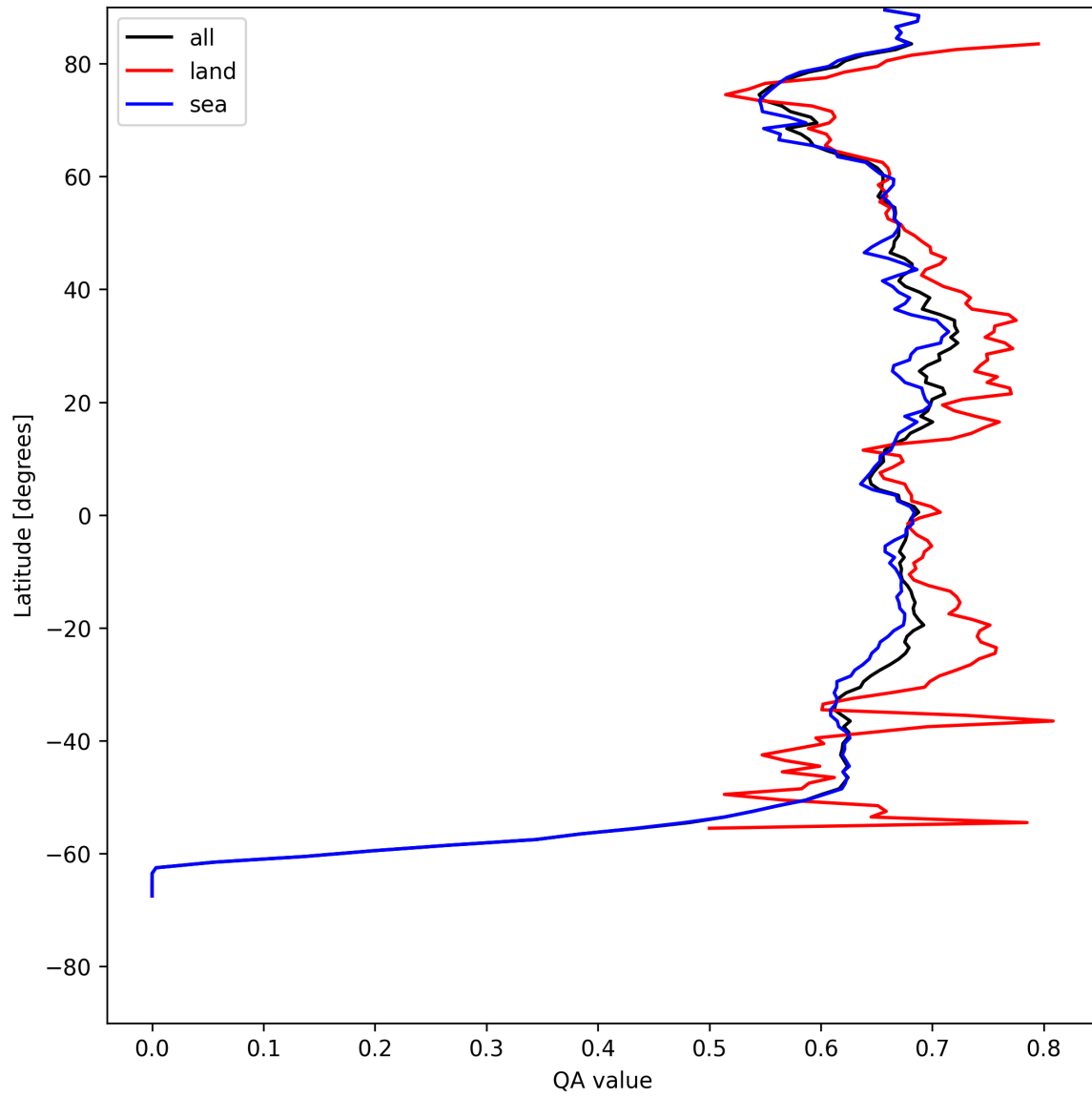
Figure 9: Zonal average of “QA value” for 2025-08-04 to 2025-08-05.
