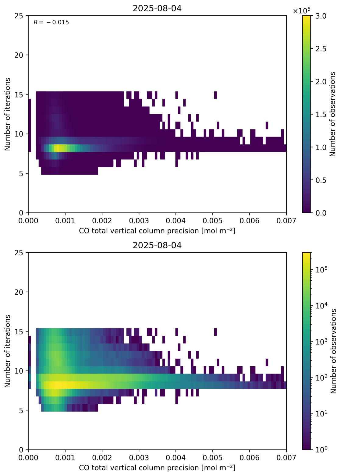
Figure 46: Scatter density plot of “CO total vertical column precision” against “Number of iterations” for 2025-08-04 to 2025-08-05.
