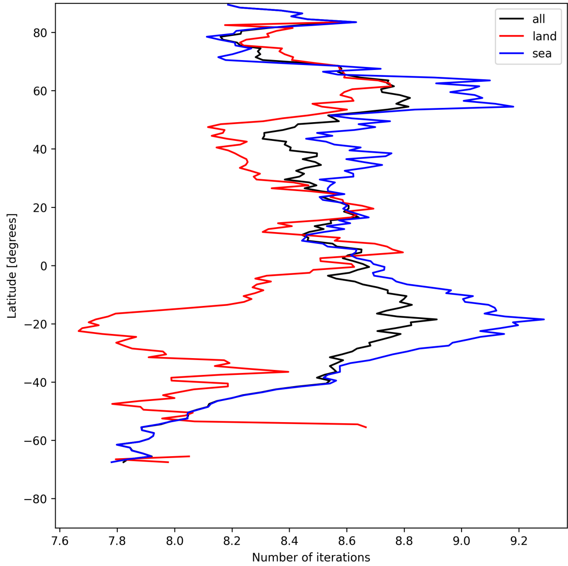
Figure 16: Zonal average of “Number of iterations” for 2025-08-04 to 2025-08-05.
