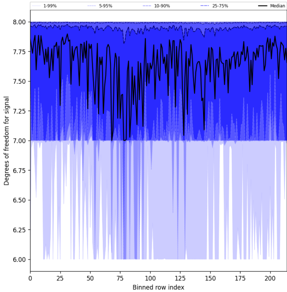
Figure 31: Along track statistics of “Degrees of freedom for signal” for 2025-08-04 to 2025-08-05
