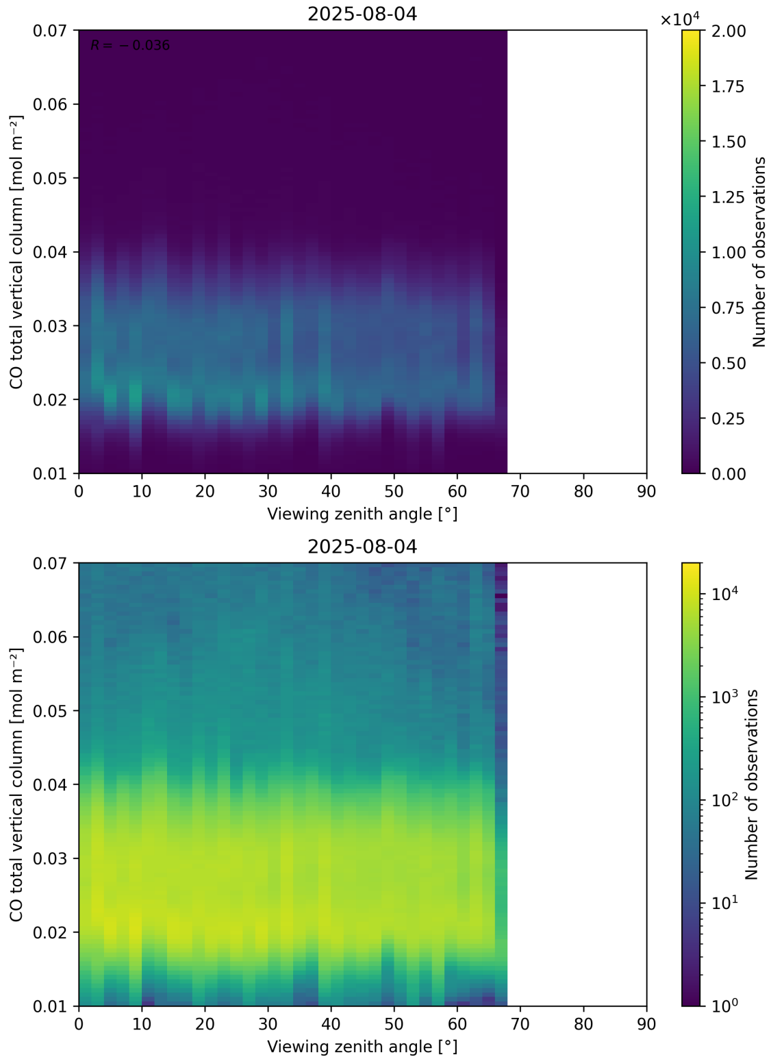
Figure 69: Scatter density plot of “Viewing zenith angle” against “CO total vertical column” for 2025-08-04 to 2025-08-05.
