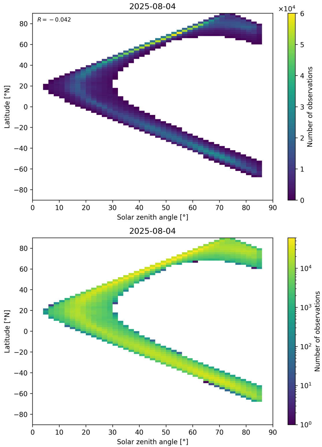
Figure 66: Scatter density plot of “Solar zenith angle” against “Latitude” for 2025-08-04 to 2025-08-05.
