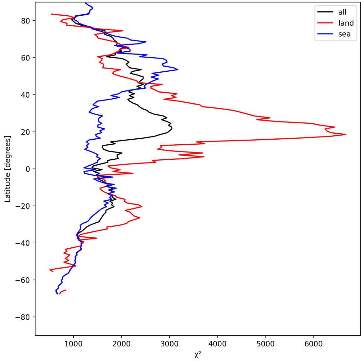
Figure 14: Zonal average of “ \chi^2 ” for 2025-08-04 to 2025-08-05.
