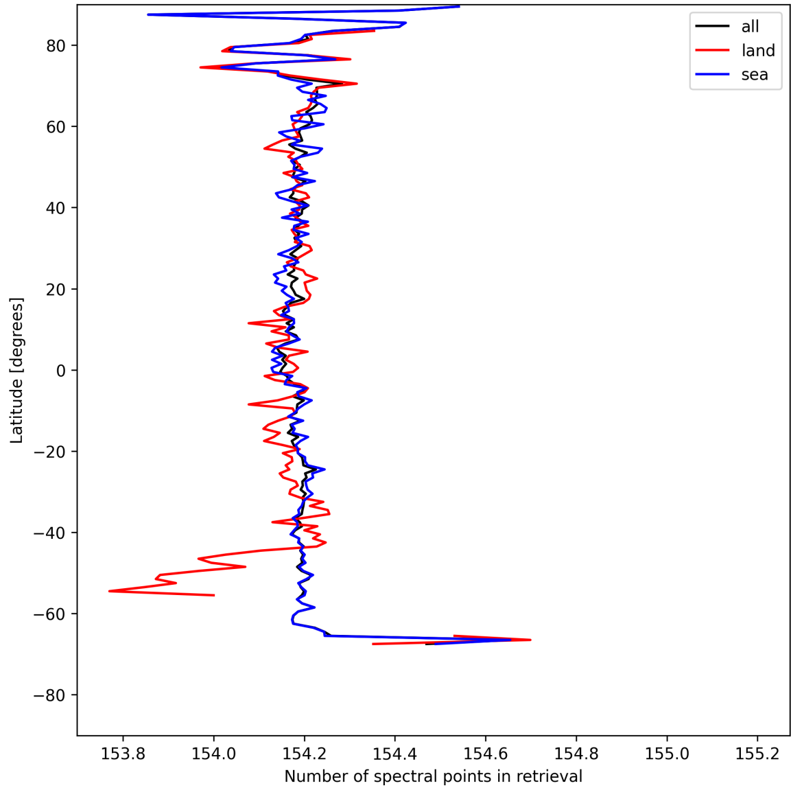
Figure 13: Zonal average of “Number of spectral points in retrieval” for 2025-08-04 to 2025-08-05.
