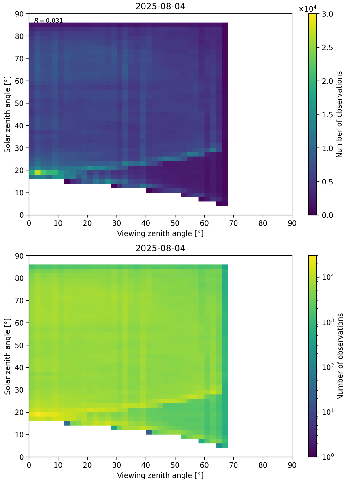
Figure 77: Scatter density plot of “Viewing zenith angle” against “Solar zenith angle” for 2025-08-04 to 2025-08-05.
