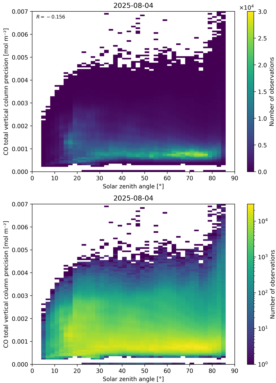
Figure 63: Scatter density plot of “Solar zenith angle” against “CO total vertical column precision” for 2025-08-04 to 2025-08-05.
