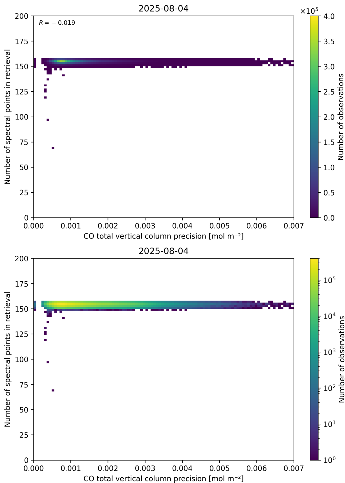
Figure 47: Scatter density plot of “CO total vertical column precision” against “Number of spectral points in retrieval” for 2025-08-04 to 2025-08-05.
