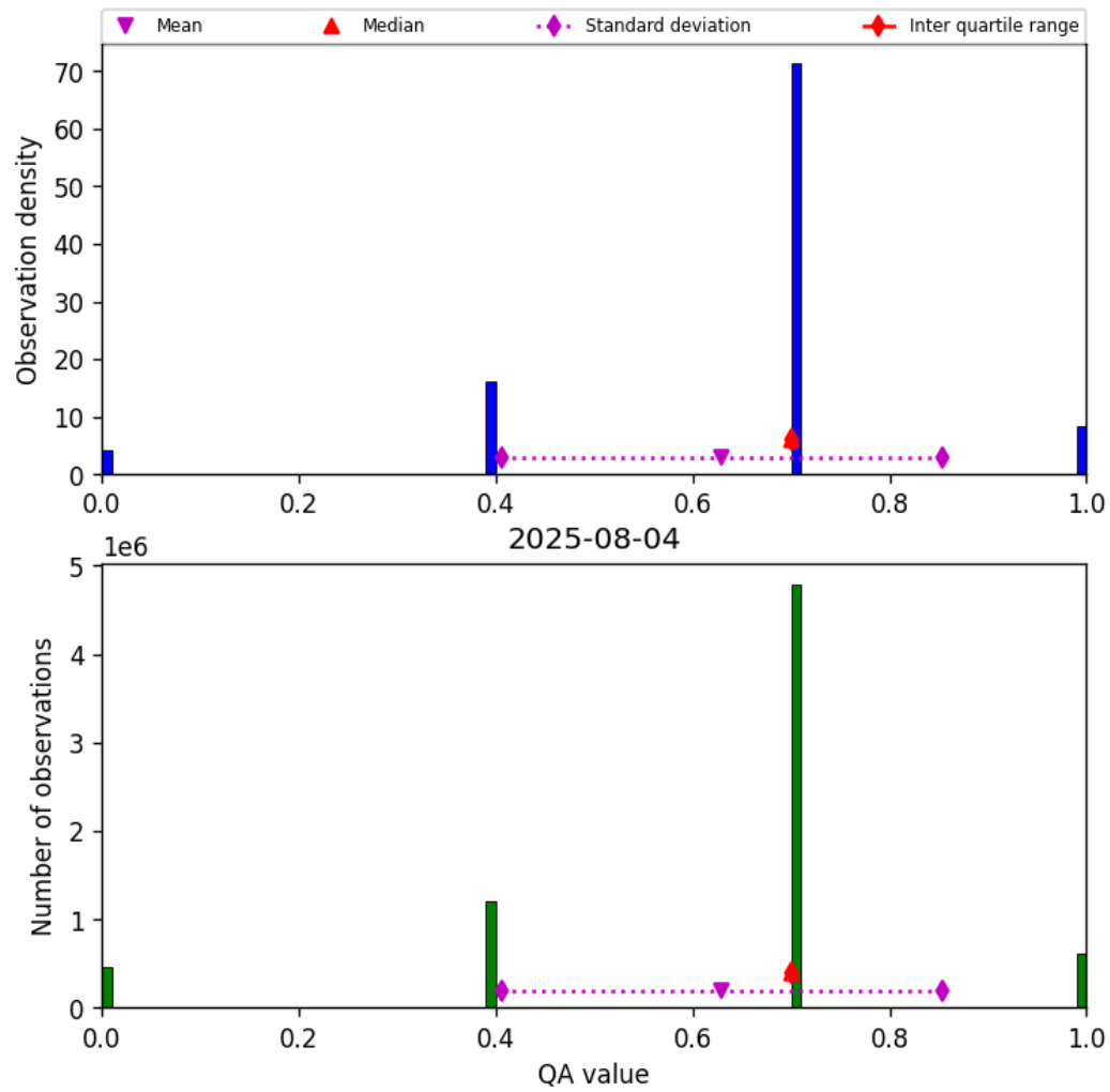
Figure 17: Histogram of “QA value” for 2025-08-04 to 2025-08-05
