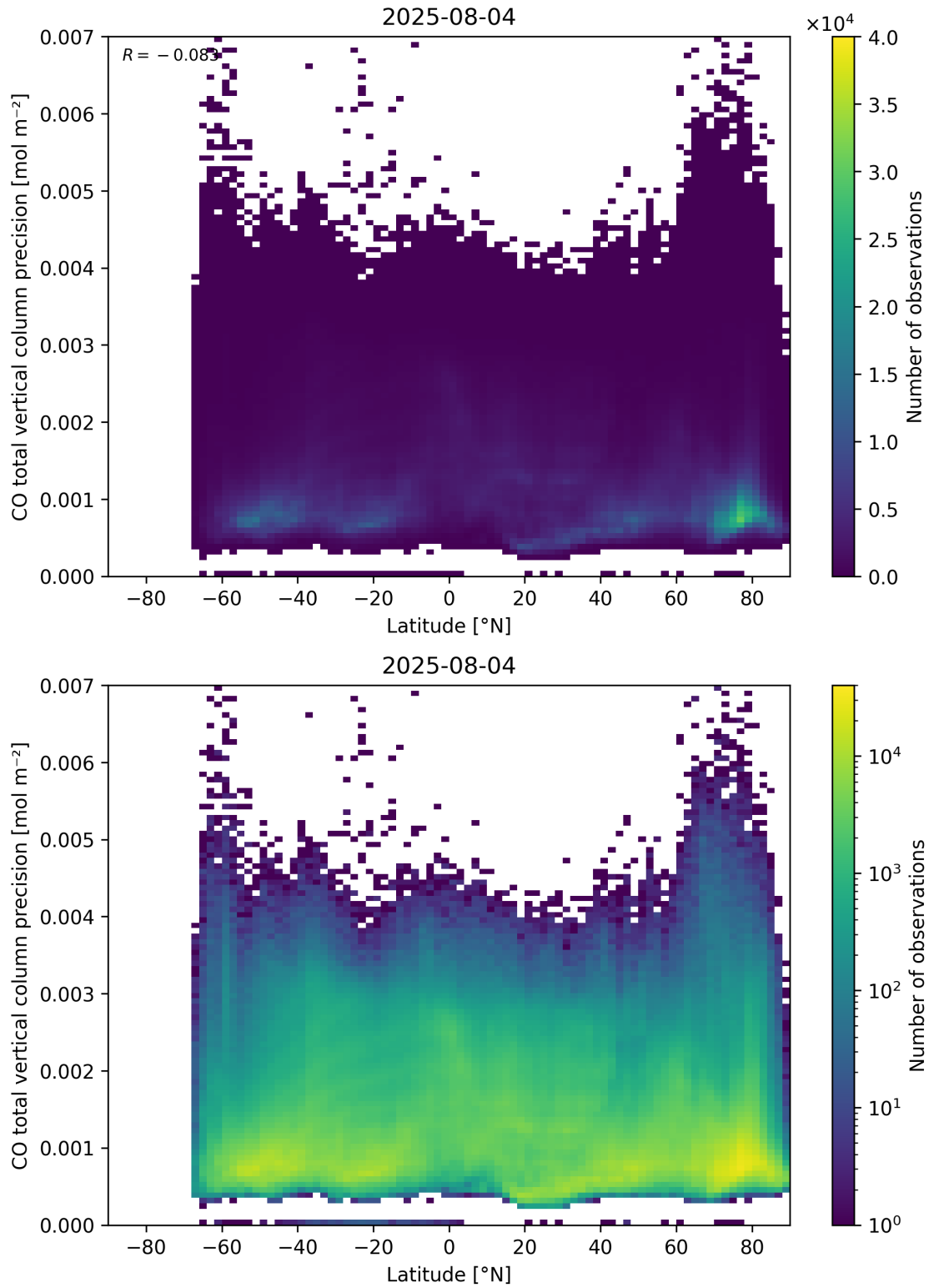
Figure 53: Scatter density plot of “Latitude” against “CO total vertical column precision” for 2025-08-04 to 2025-08-05.
