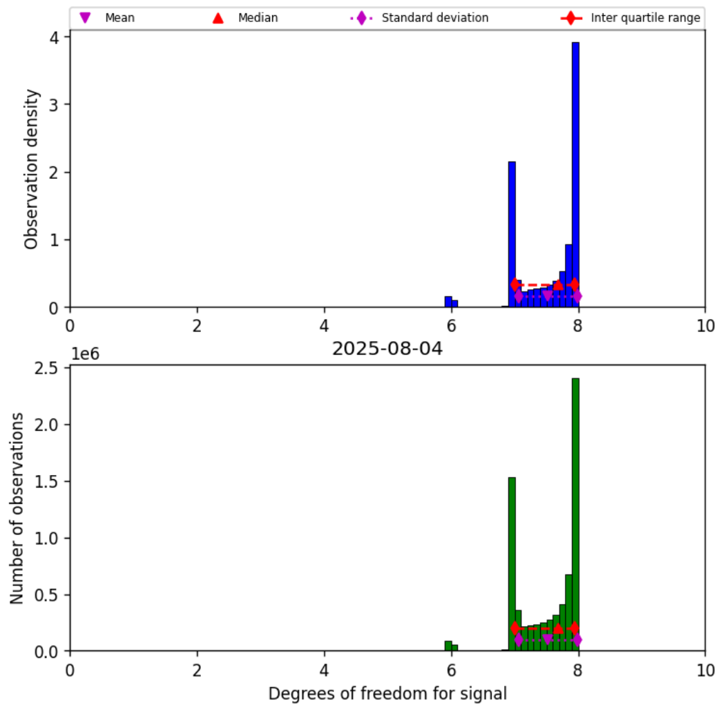
Figure 23: Histogram of “Degrees of freedom for signal” for 2025-08-04 to 2025-08-05
