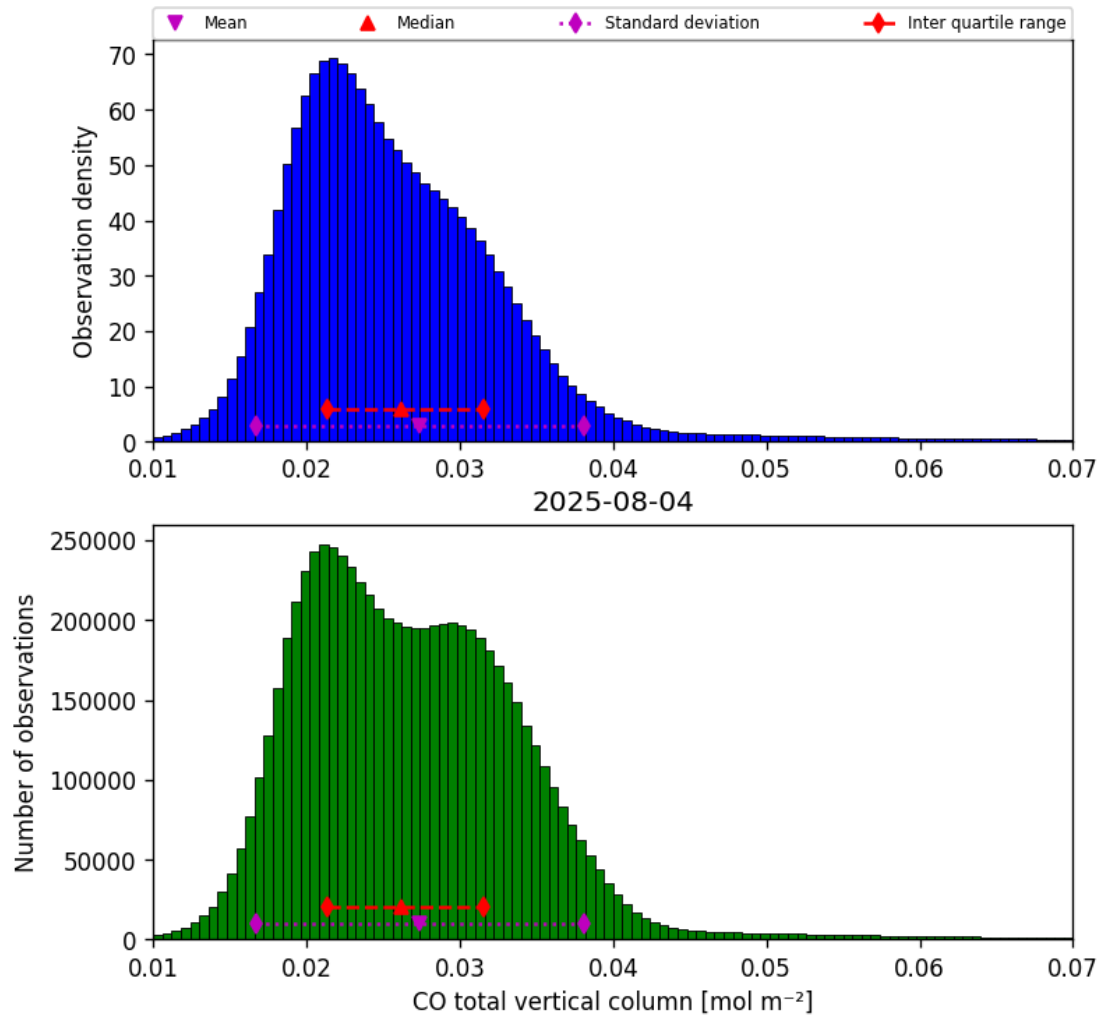
Figure 18: Histogram of “CO total vertical column” for 2025-08-04 to 2025-08-05
