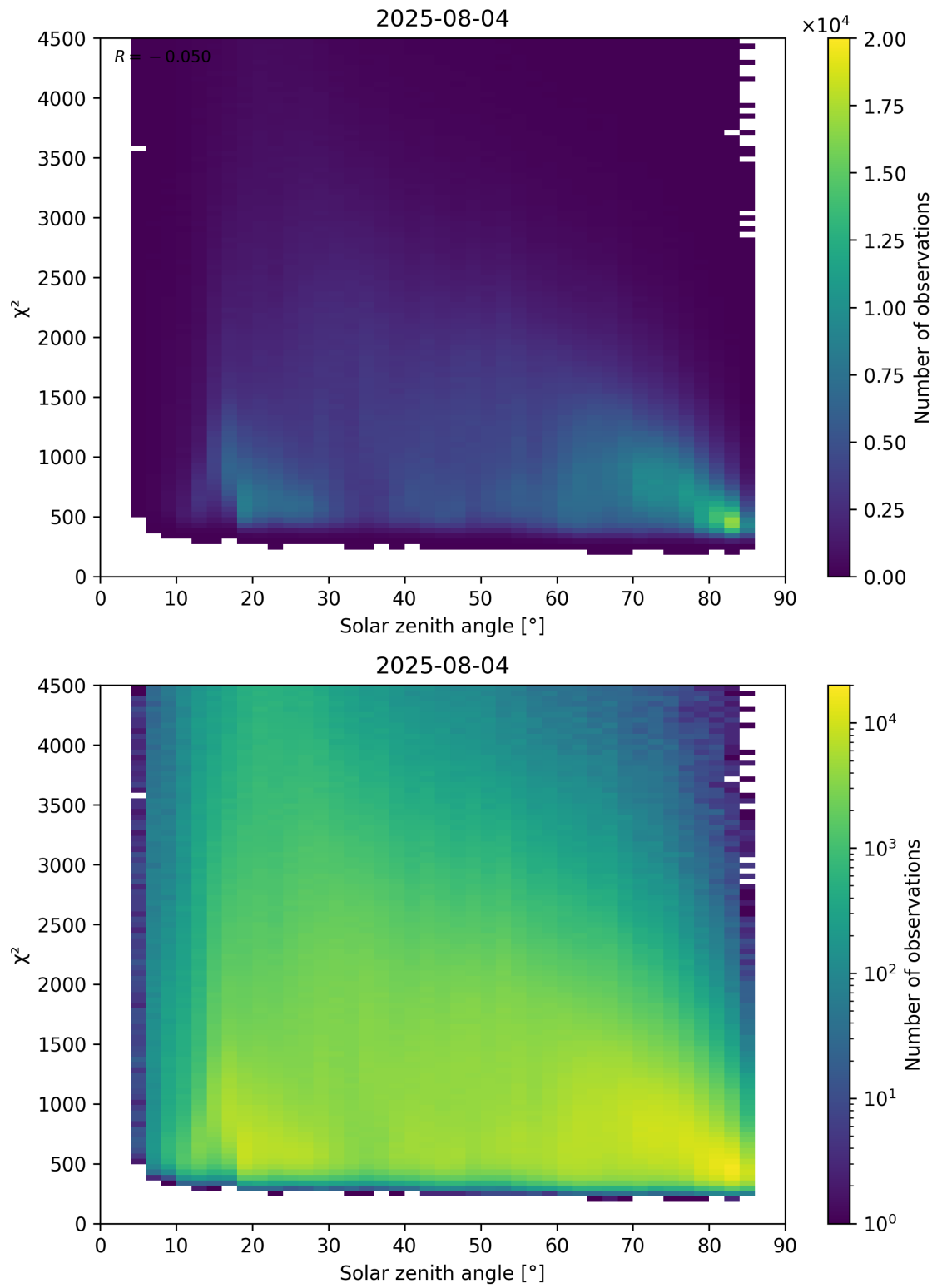
Figure 64: Scatter density plot of “Solar zenith angle” against “ \chi^2 ” for 2025-08-04 to 2025-08-05.
