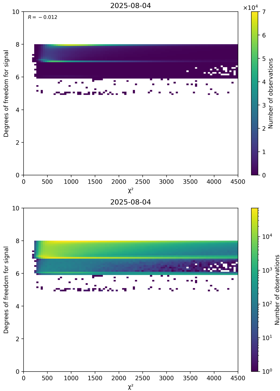
Figure 48: Scatter density plot of " \chi^2 " against "Degrees of freedom for signal" for 2025-08-04 to 2025-08-05.
