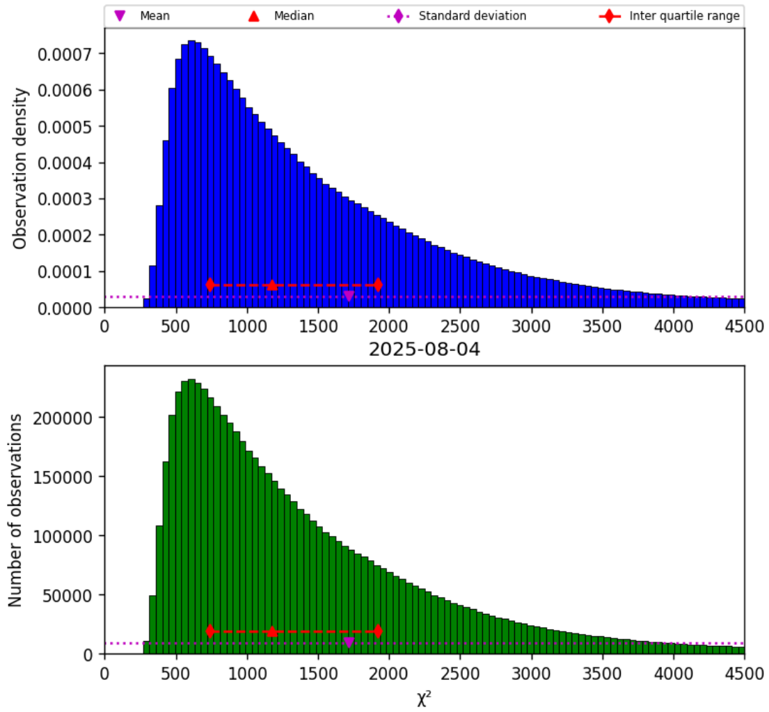
Figure 22: Histogram of " \chi^2 " for 2025-08-04 to 2025-08-05
