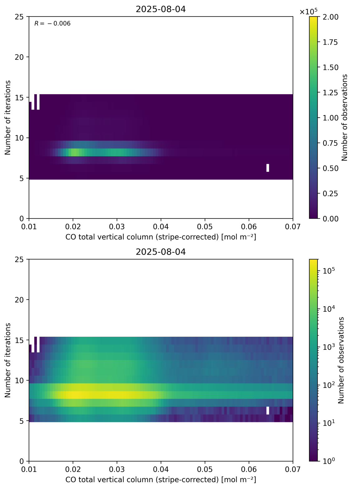
Figure 39: Scatter density plot of “CO total vertical column (stripe-corrected)” against “Number of iterations” for 2025-08-04 to 2025-08-05.
