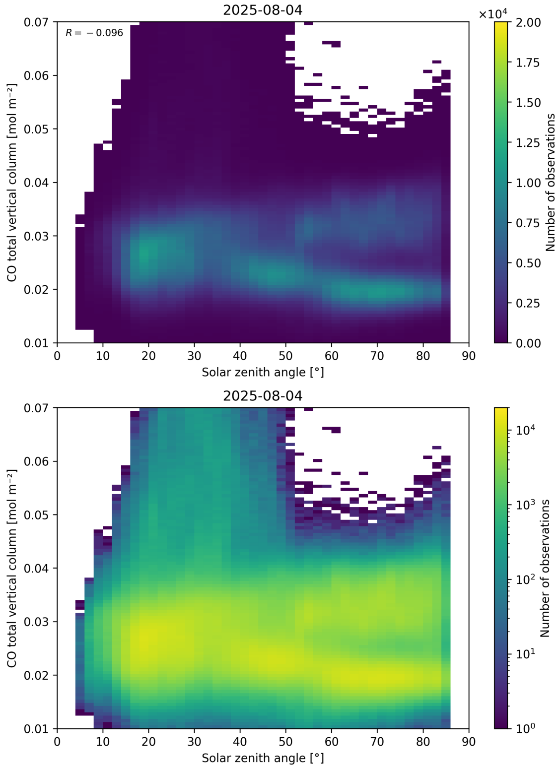
Figure 61: Scatter density plot of “Solar zenith angle” against “CO total vertical column” for 2025-08-04 to 2025-08-05.
