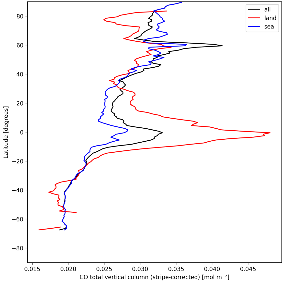
Figure 11: Zonal average of “CO total vertical column (stripe-corrected)” for 2025-08-04 to 2025-08-05.
