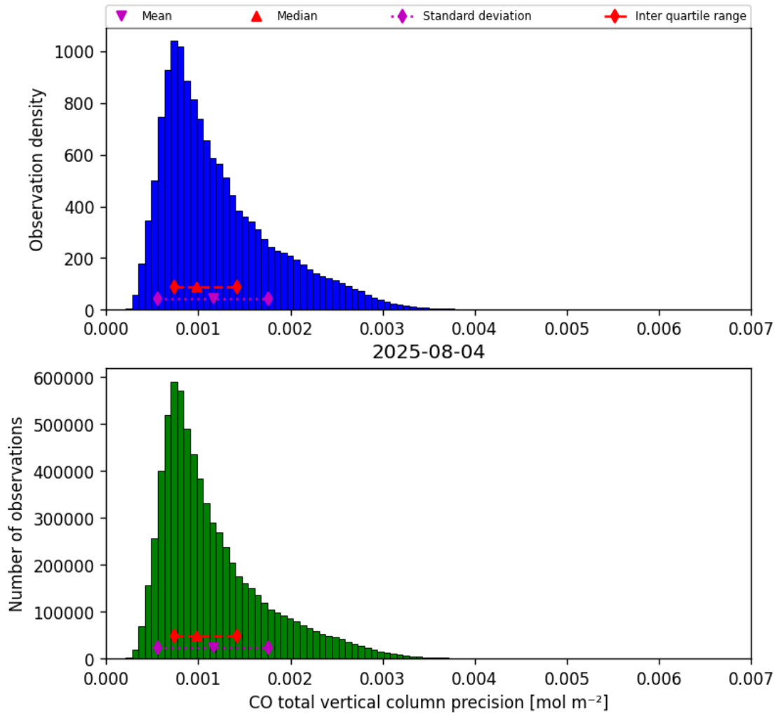
Figure 20: Histogram of “CO total vertical column precision” for 2025-08-04 to 2025-08-05
