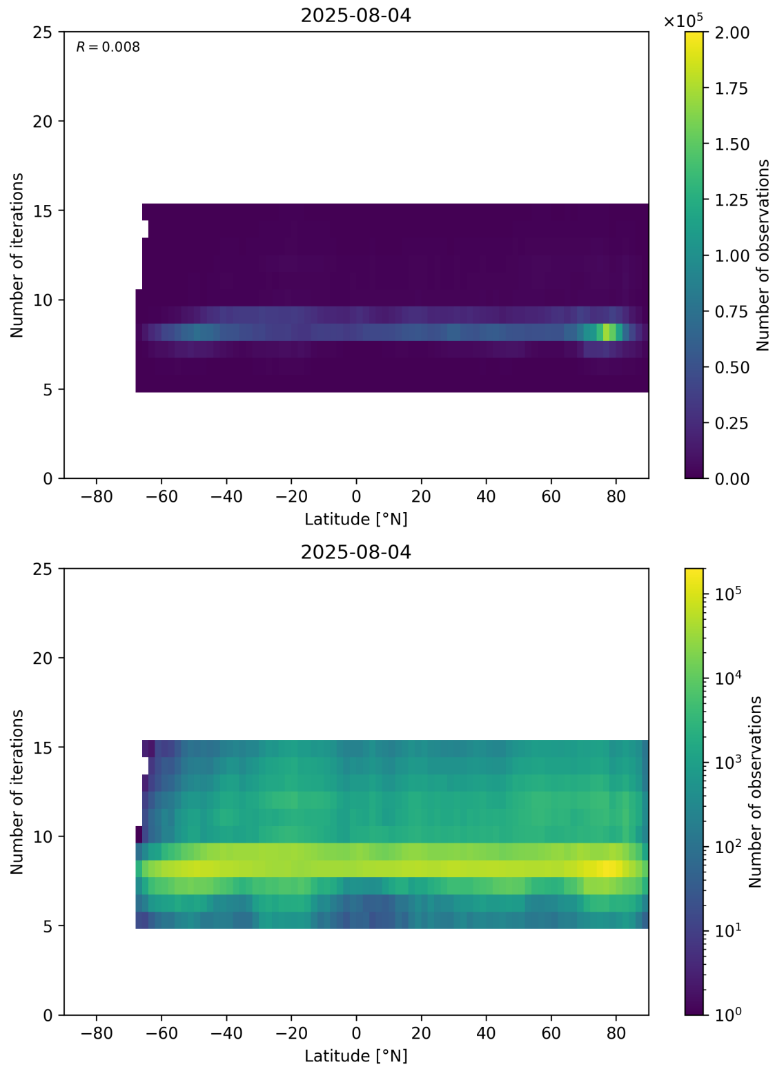
Figure 56: Scatter density plot of “Latitude” against “Number of iterations” for 2025-08-04 to 2025-08-05.
