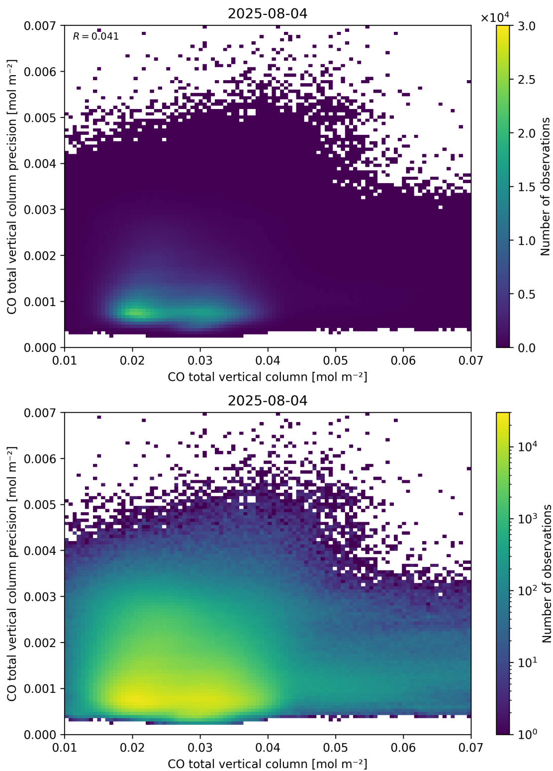
Figure 34: Scatter density plot of “CO total vertical column” against “CO total vertical column precision” for 2025-08-04 to 2025-08-05.
