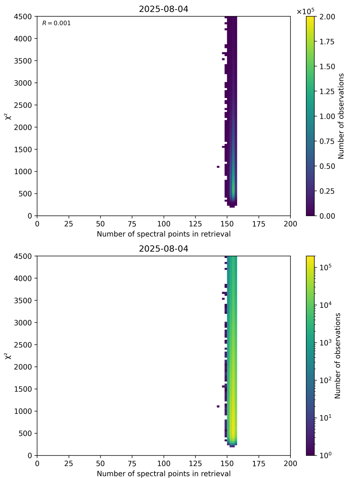
Figure 58: Scatter density plot of “Number of spectral points in retrieval” against “ \chi^2 ” for 2025-08-04 to 2025-08-05.
