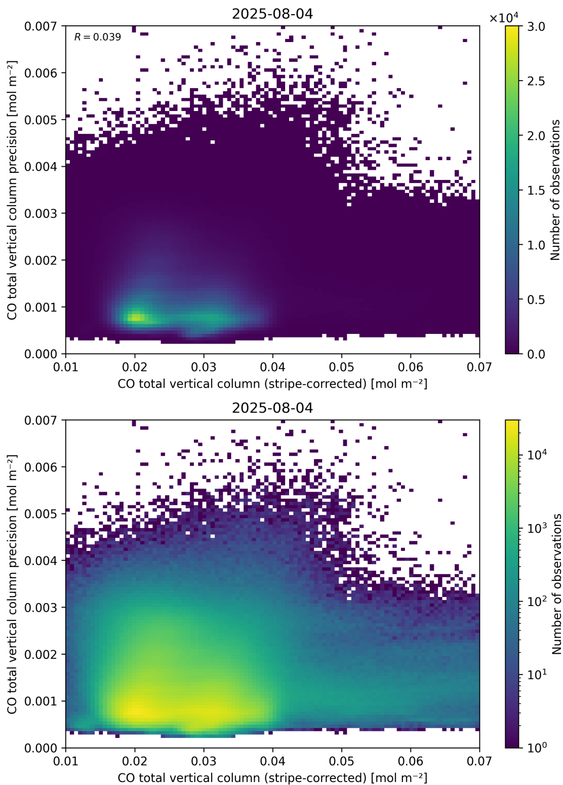
Figure 36: Scatter density plot of “CO total vertical column (stripe-corrected)” against “CO total vertical column precision” for 2025-08-04 to 2025-08-05.
