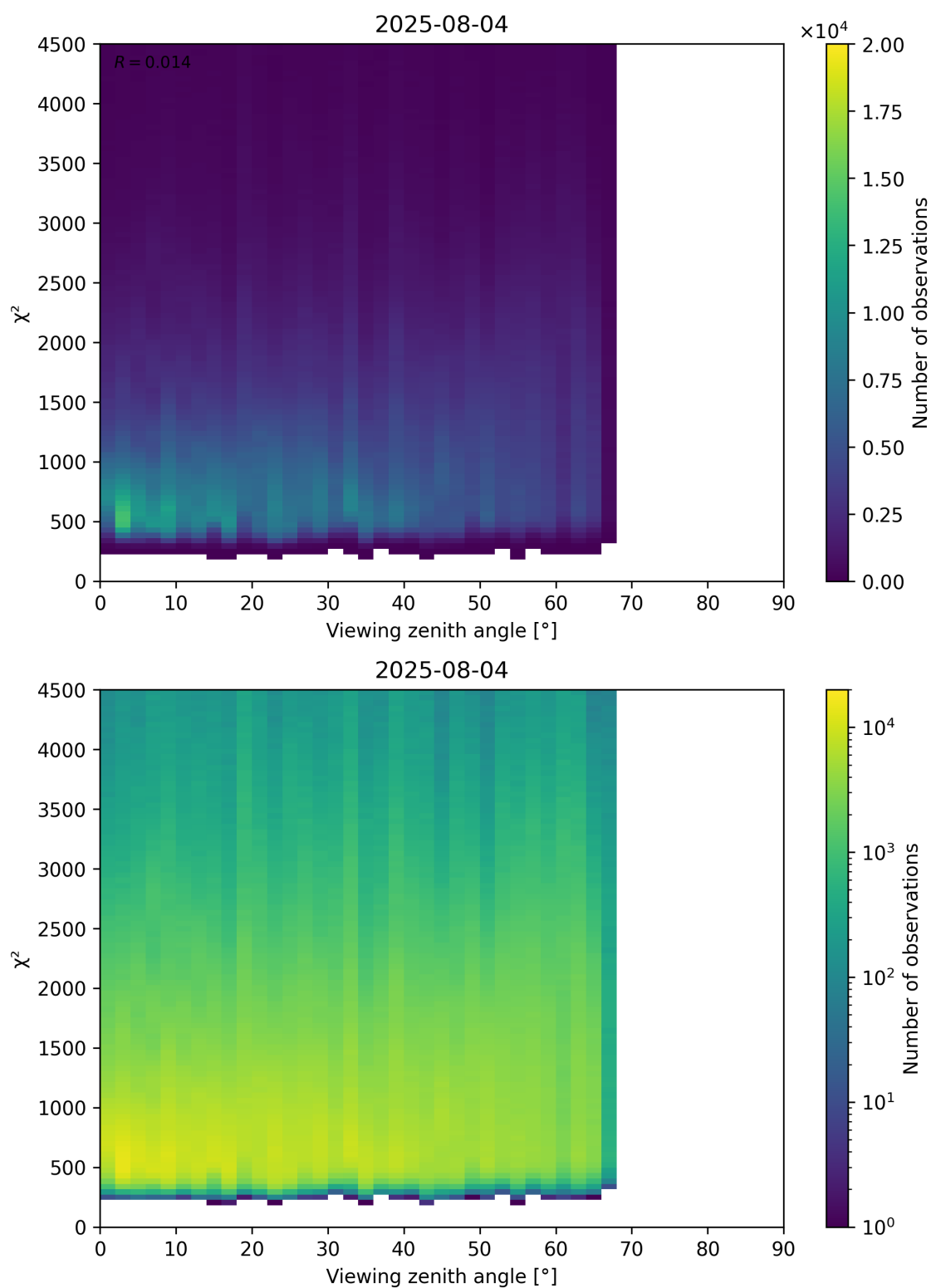
Figure 72: Scatter density plot of “Viewing zenith angle” against “ \chi^2 ” for 2025-08-04 to 2025-08-05.
