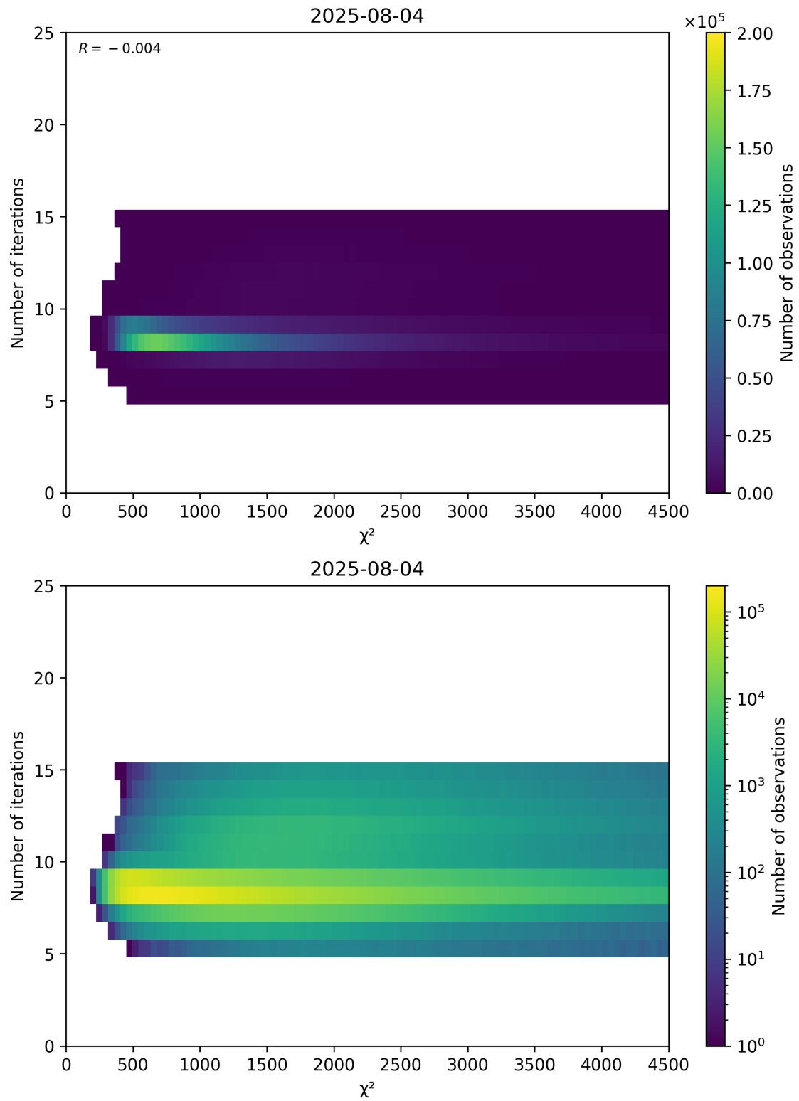
Figure 49: Scatter density plot of “ \chi^2 ” against “Number of iterations” for 2025-08-04 to 2025-08-05.
