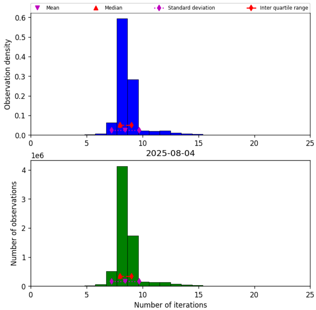
Figure 24: Histogram of “Number of iterations” for 2025-08-04 to 2025-08-05
