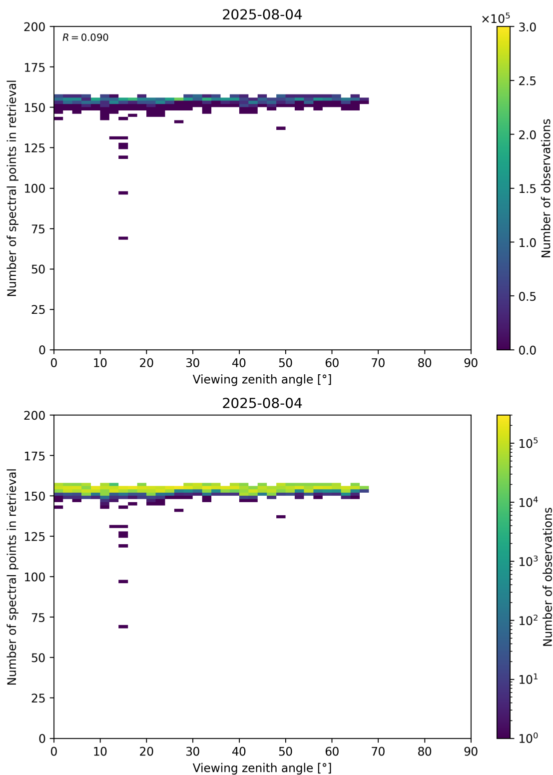
Figure 76: Scatter density plot of “Viewing zenith angle” against “Number of spectral points in retrieval” for 2025-08-04 to 2025-08-05.
