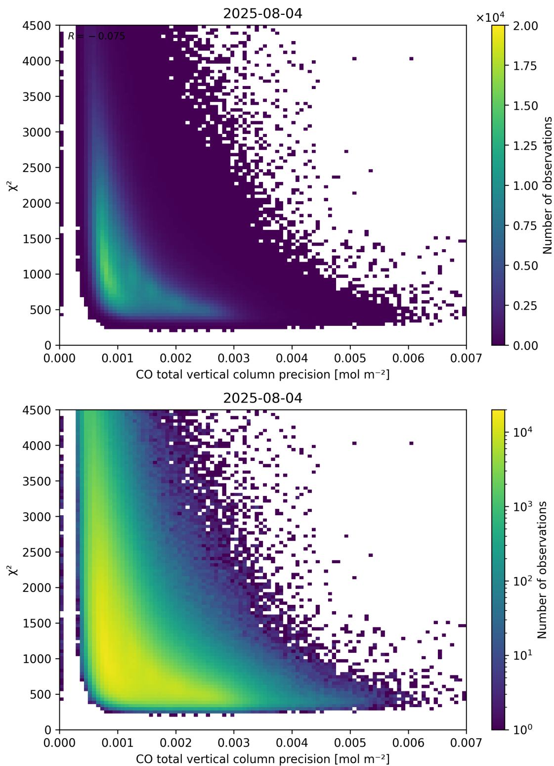
Figure 44: Scatter density plot of “CO total vertical column precision” against “ \chi^2 ” for 2025-08-04 to 2025-08-05.
