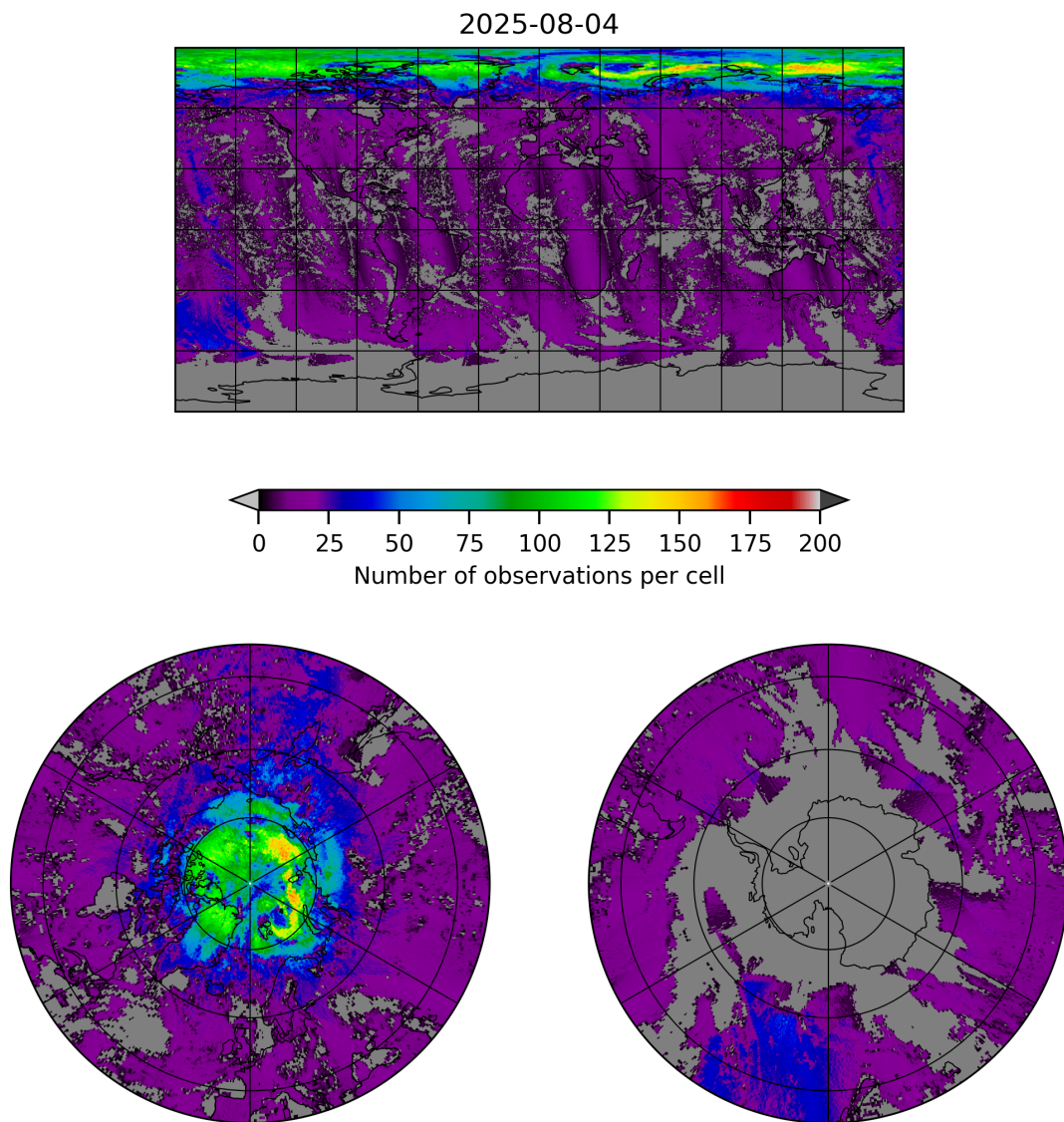
Figure 8: Map of the number of observations for 2025-08-04 to 2025-08-05
