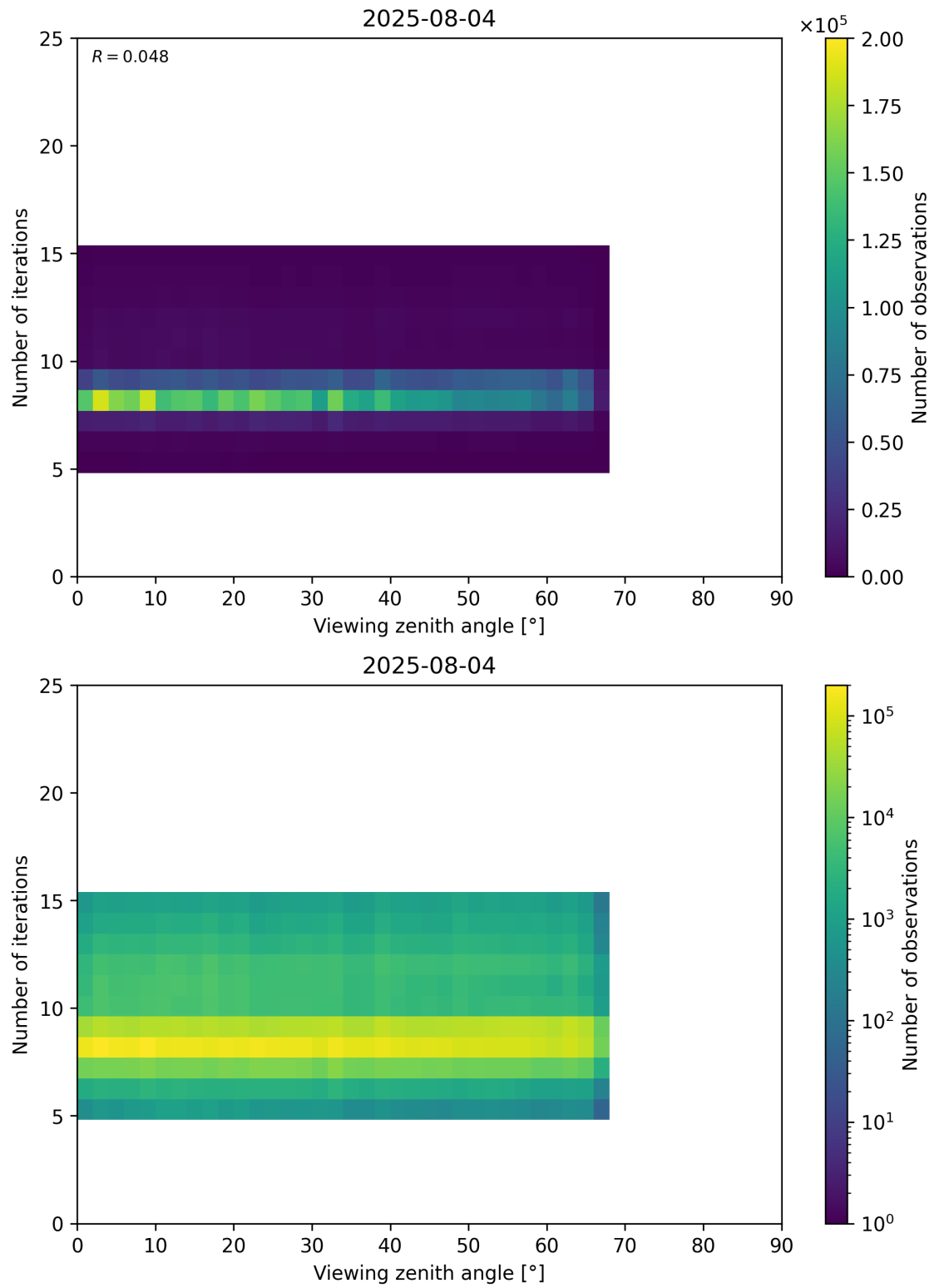
Figure 75: Scatter density plot of “Viewing zenith angle” against “Number of iterations” for 2025-08-04 to 2025-08-05.
