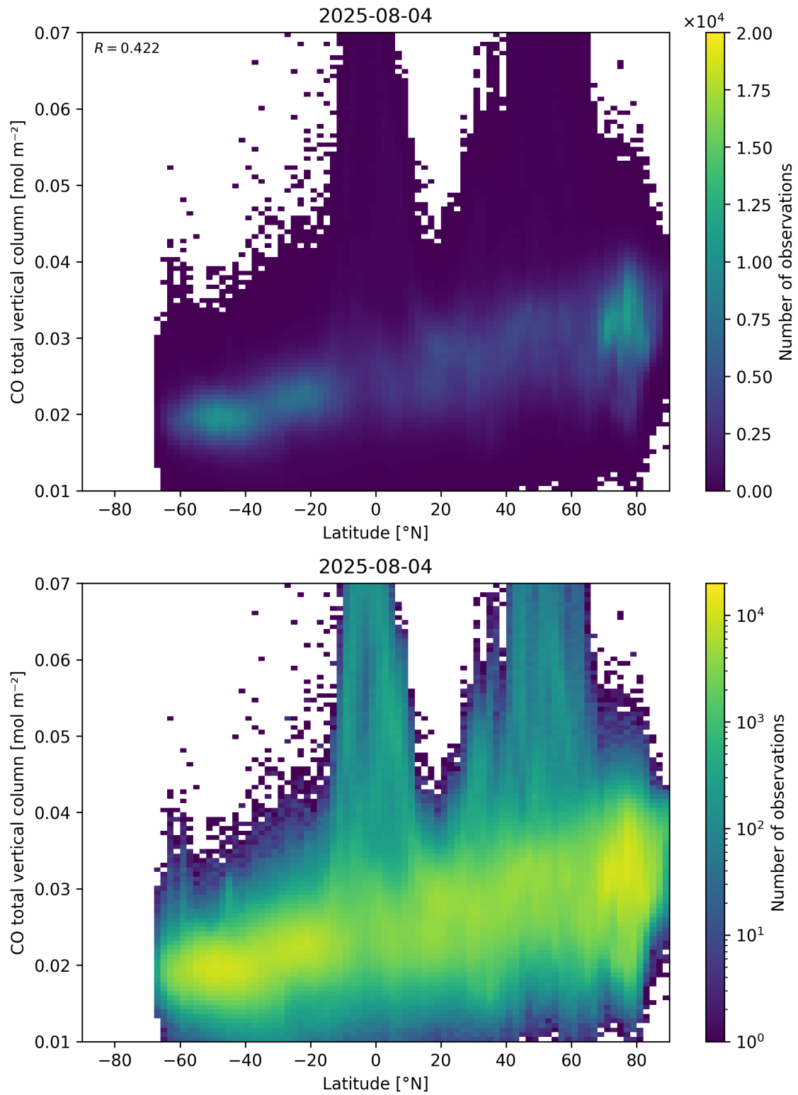
Figure 51: Scatter density plot of “Latitude” against “CO total vertical column” for 2025-08-04 to 2025-08-05.
