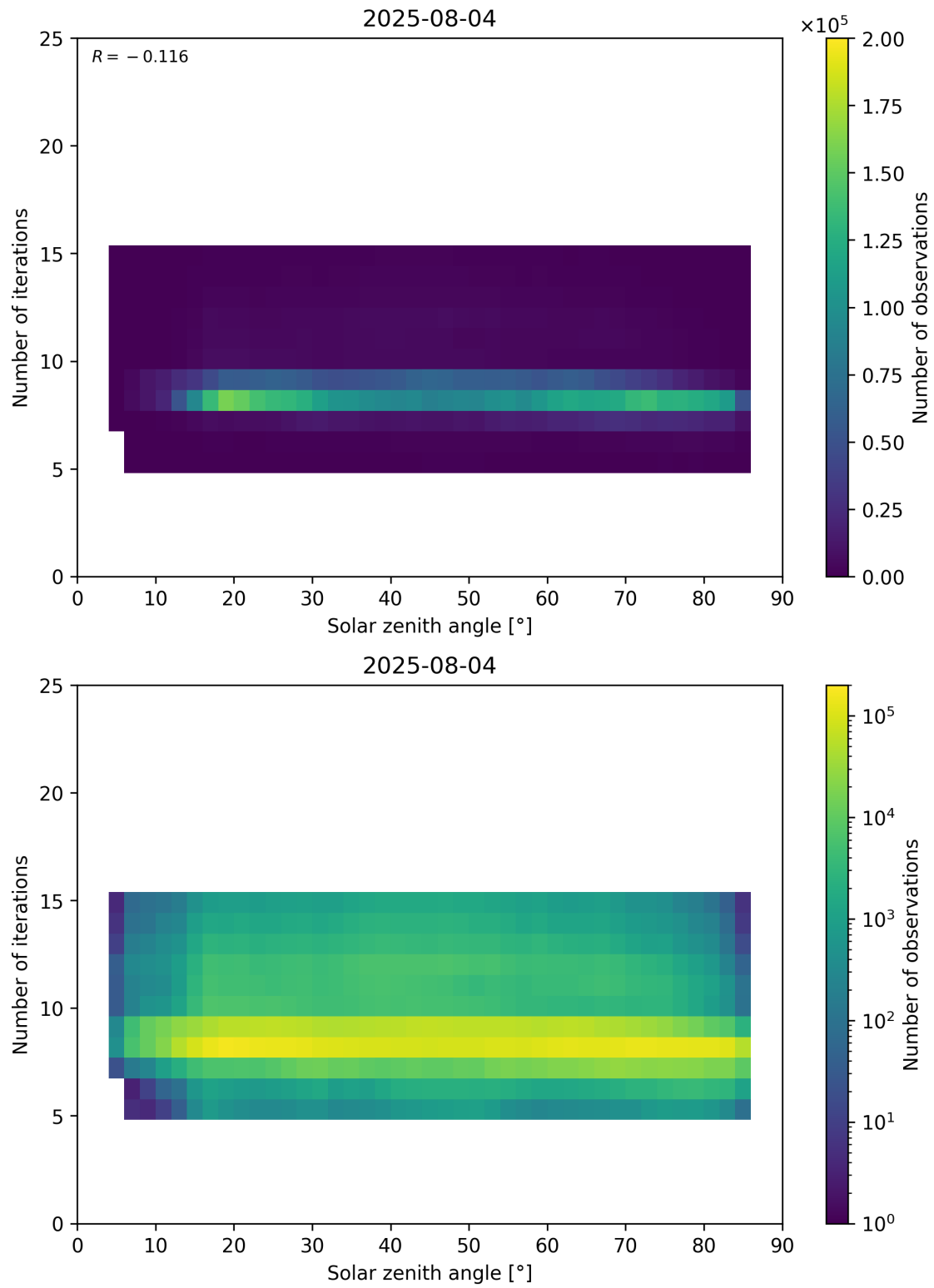
Figure 67: Scatter density plot of “Solar zenith angle” against “Number of iterations” for 2025-08-04 to 2025-08-05.
