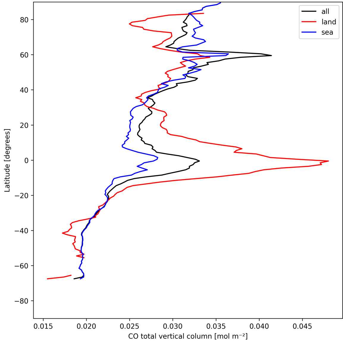
Figure 10: Zonal average of “CO total vertical column” for 2025-08-04 to 2025-08-05.
