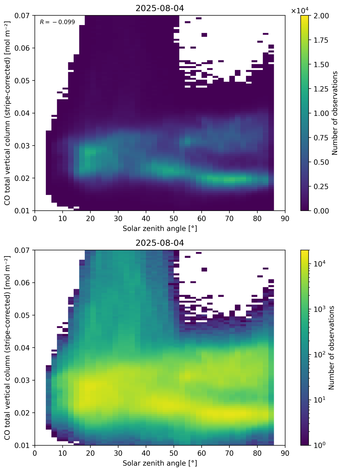
Figure 62: Scatter density plot of “Solar zenith angle” against “CO total vertical column (stripe-corrected)” for 2025-08-04 to 2025-08-05.
