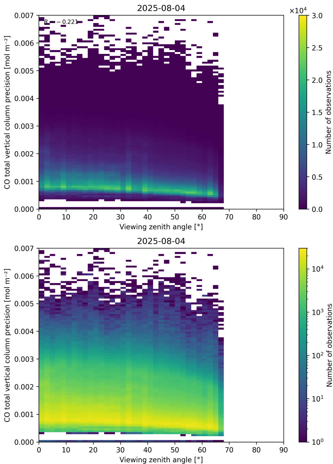
Figure 71: Scatter density plot of “Viewing zenith angle” against “CO total vertical column precision” for 2025-08-04 to 2025-08-05.
