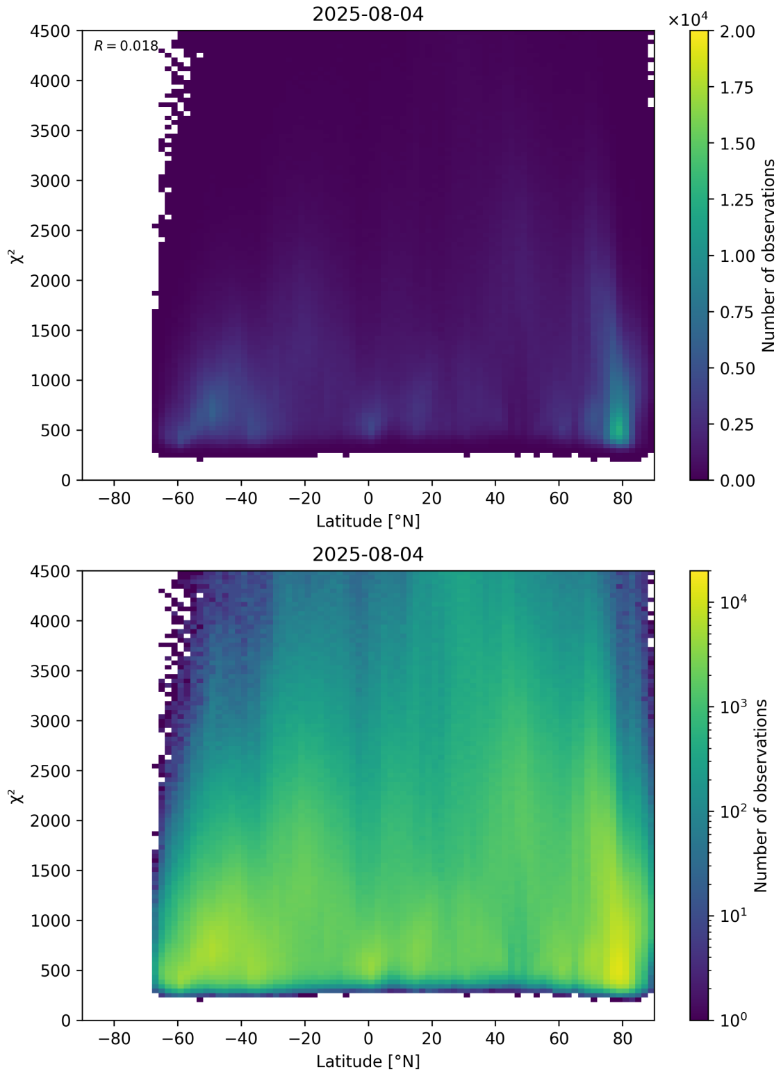
Figure 54: Scatter density plot of “Latitude” against “ \chi^2 ” for 2025-08-04 to 2025-08-05.
