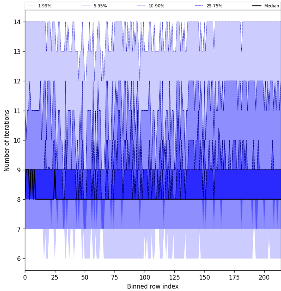
Figure 32: Along track statistics of “Number of iterations” for 2025-08-04 to 2025-08-05
