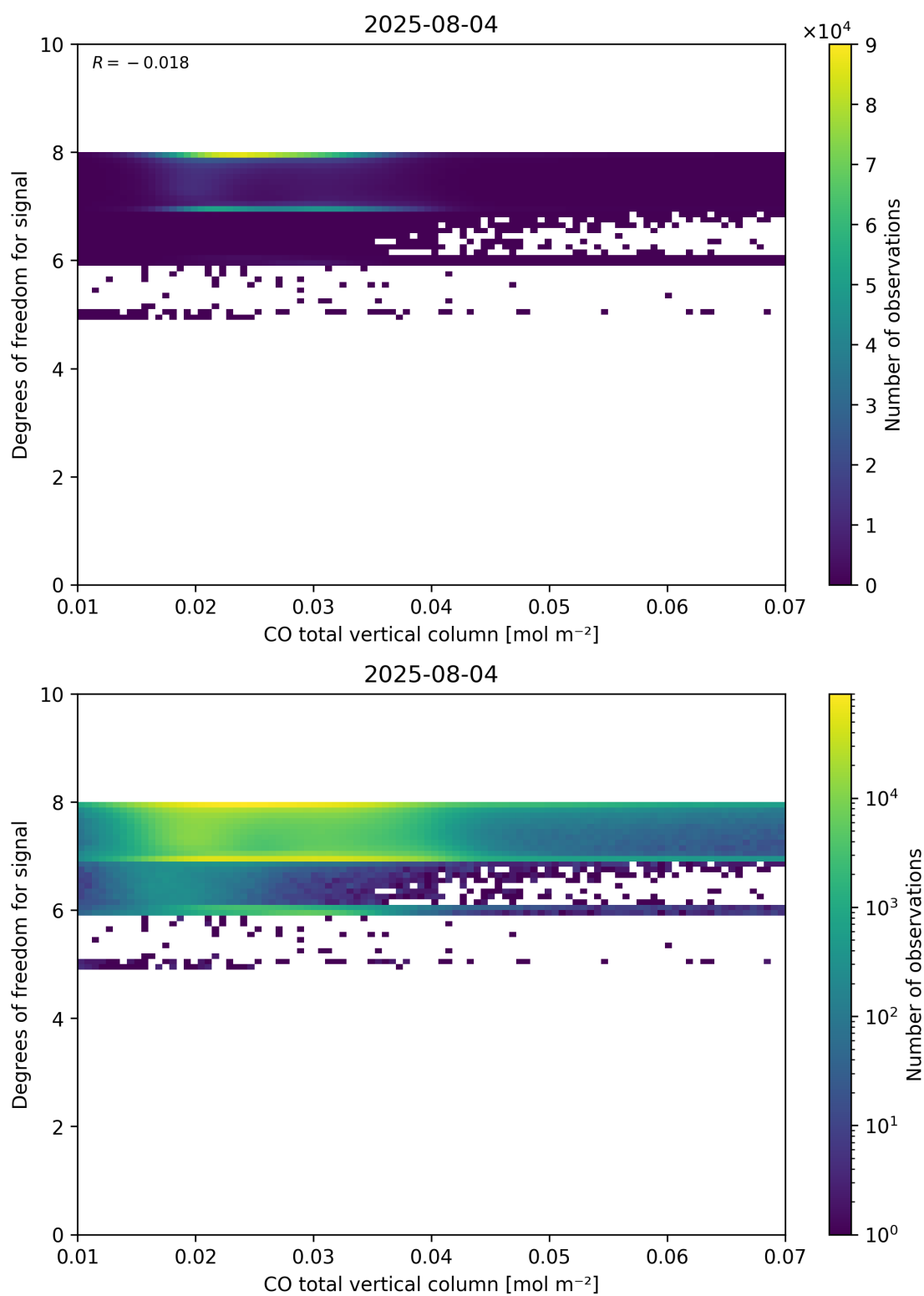
Figure 41: Scatter density plot of “CO total vertical column” against “Degrees of freedom for signal” for 2025-08-04 to 2025-08-05.
