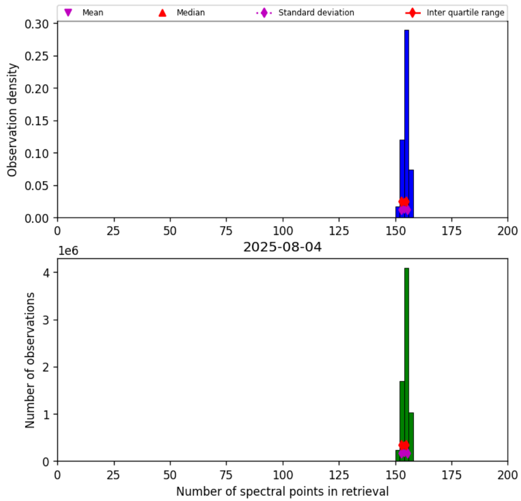
Figure 21: Histogram of “Number of spectral points in retrieval” for 2025-08-04 to 2025-08-05
