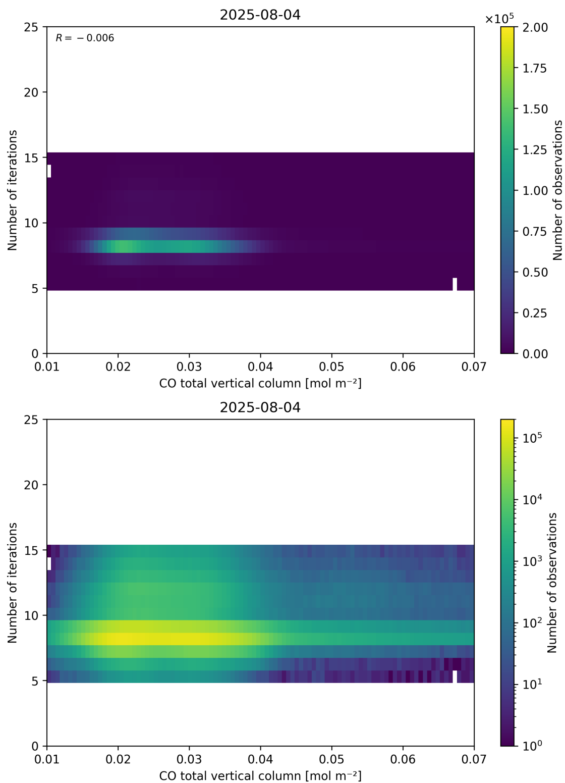
Figure 42: Scatter density plot of “CO total vertical column” against “Number of iterations” for 2025-08-04 to 2025-08-05.
