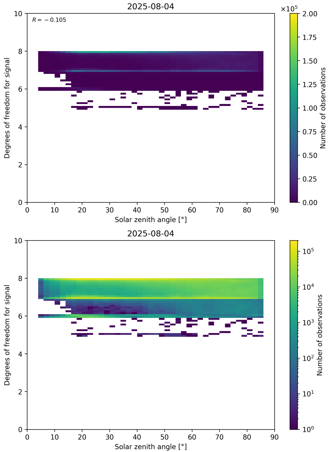
Figure 65: Scatter density plot of “Solar zenith angle” against “Degrees of freedom for signal” for 2025-08-04 to 2025-08-05.
