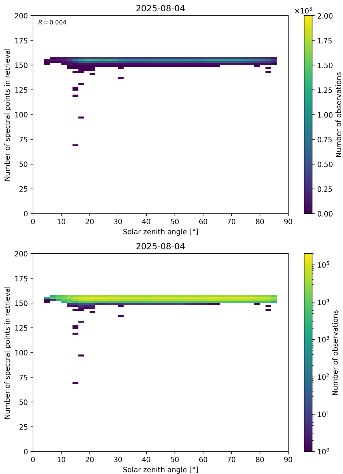
Figure 68: Scatter density plot of “Solar zenith angle” against “Number of spectral points in retrieval” for 2025-08-04 to 2025-08-05.
