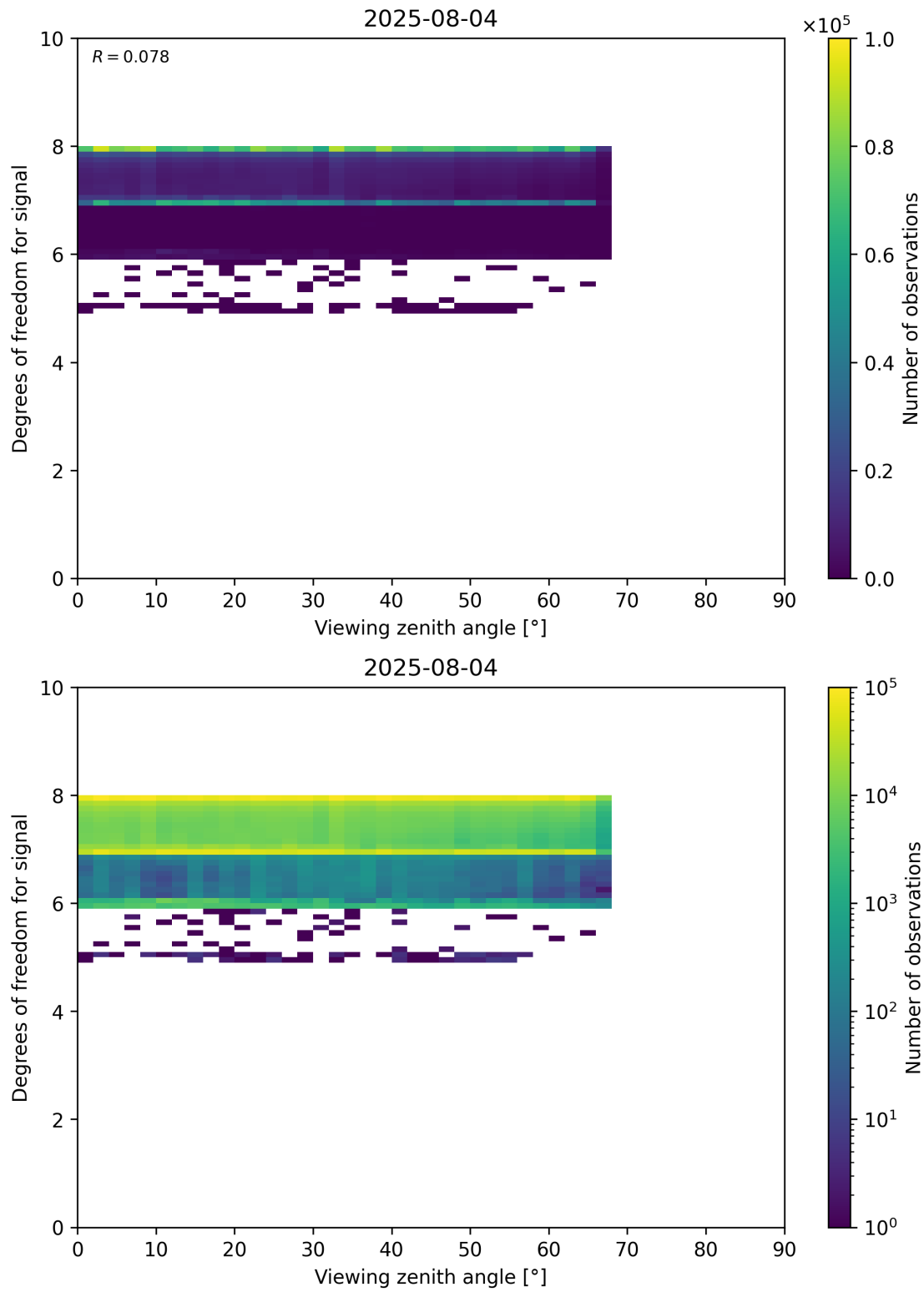
Figure 73: Scatter density plot of “Viewing zenith angle” against “Degrees of freedom for signal” for 2025-08-04 to 2025-08-05.
