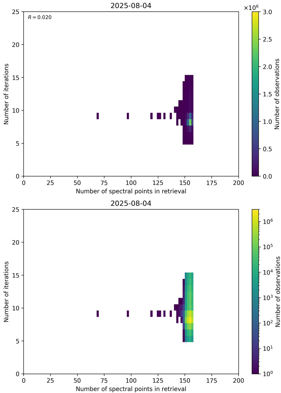
Figure 60: Scatter density plot of “Number of spectral points in retrieval” against “Number of iterations” for 2025-08-04 to 2025-08-05.
