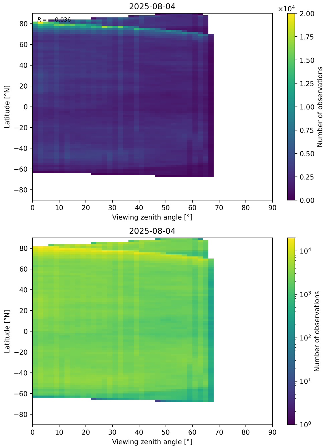
Figure 74: Scatter density plot of “Viewing zenith angle” against “Latitude” for 2025-08-04 to 2025-08-05.
