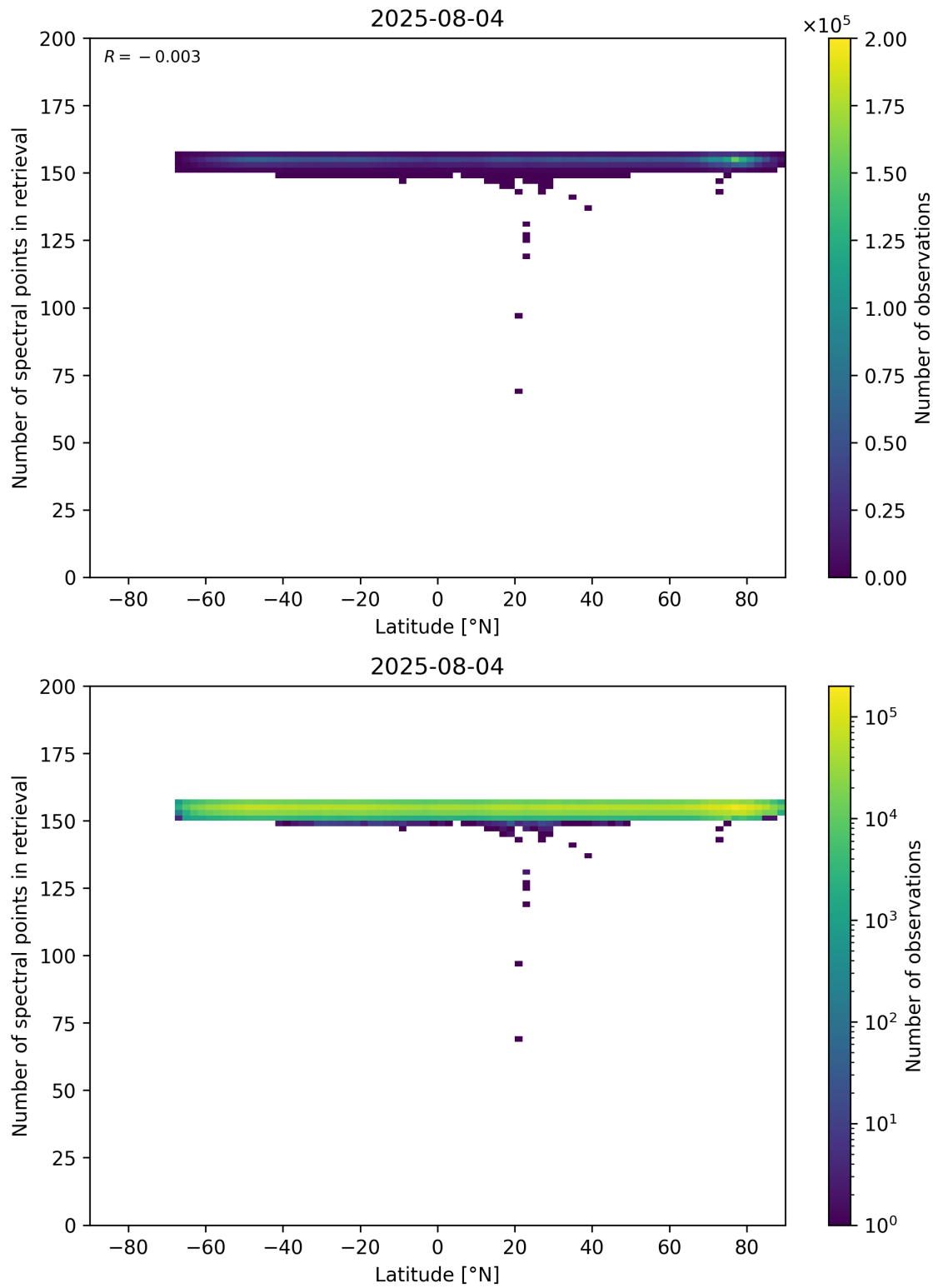
Figure 57: Scatter density plot of “Latitude” against “Number of spectral points in retrieval” for 2025-08-04 to 2025-08-05.
