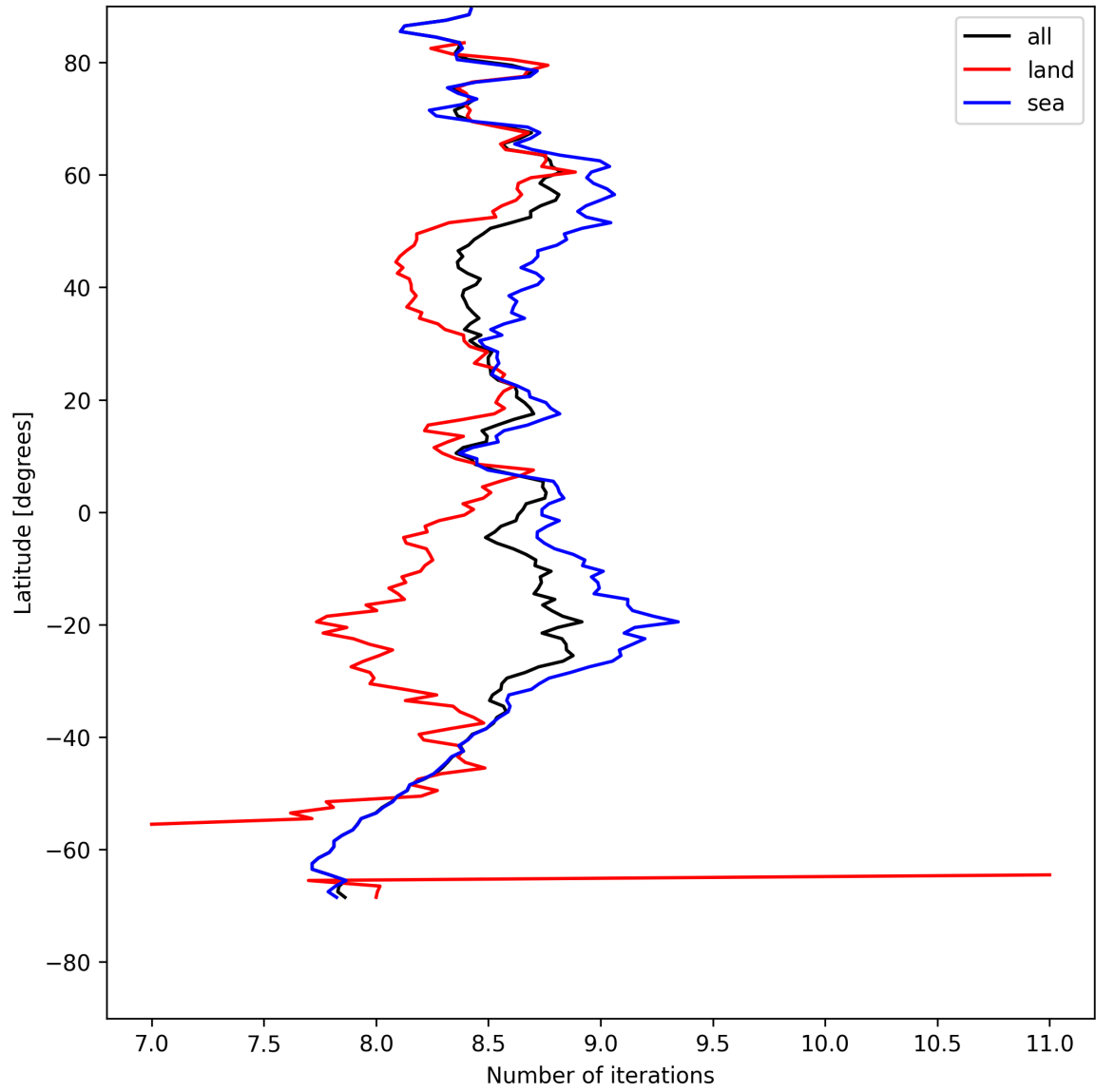
Figure 16: Zonal average of “Number of iterations” for 2025-08-06 to 2025-08-08.
