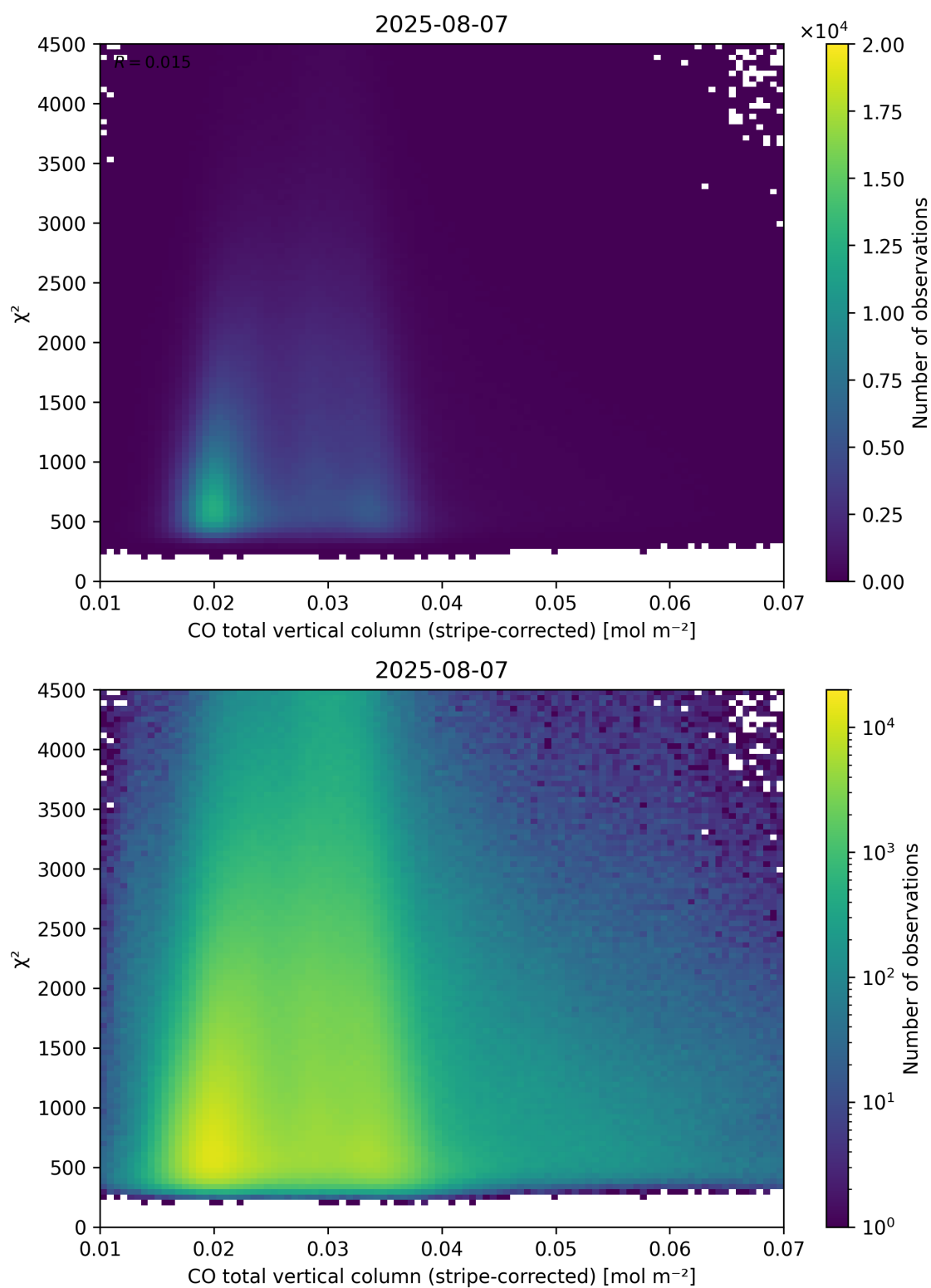
Figure 37: Scatter density plot of “CO total vertical column (stripe-corrected)” against “ \chi^2 ” for 2025-08-06 to 2025-08-08.
