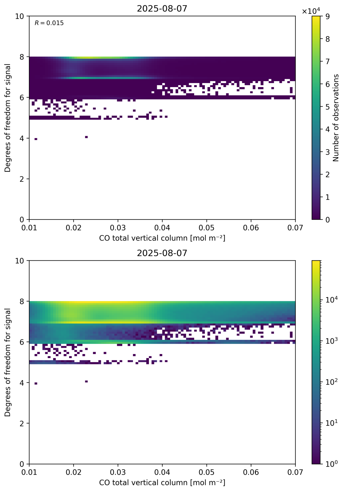
Figure 41: Scatter density plot of “CO total vertical column” against “Degrees of freedom for signal” for 2025-08-06 to 2025-08-08.
