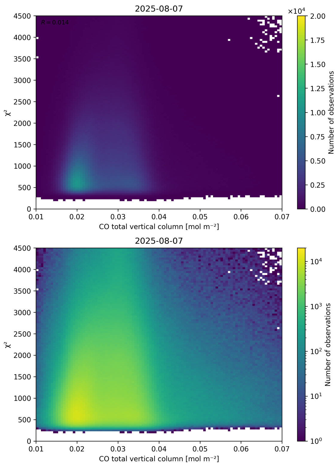
Figure 35: Scatter density plot of “CO total vertical column” against “ \chi^2 ” for 2025-08-06 to 2025-08-08.
