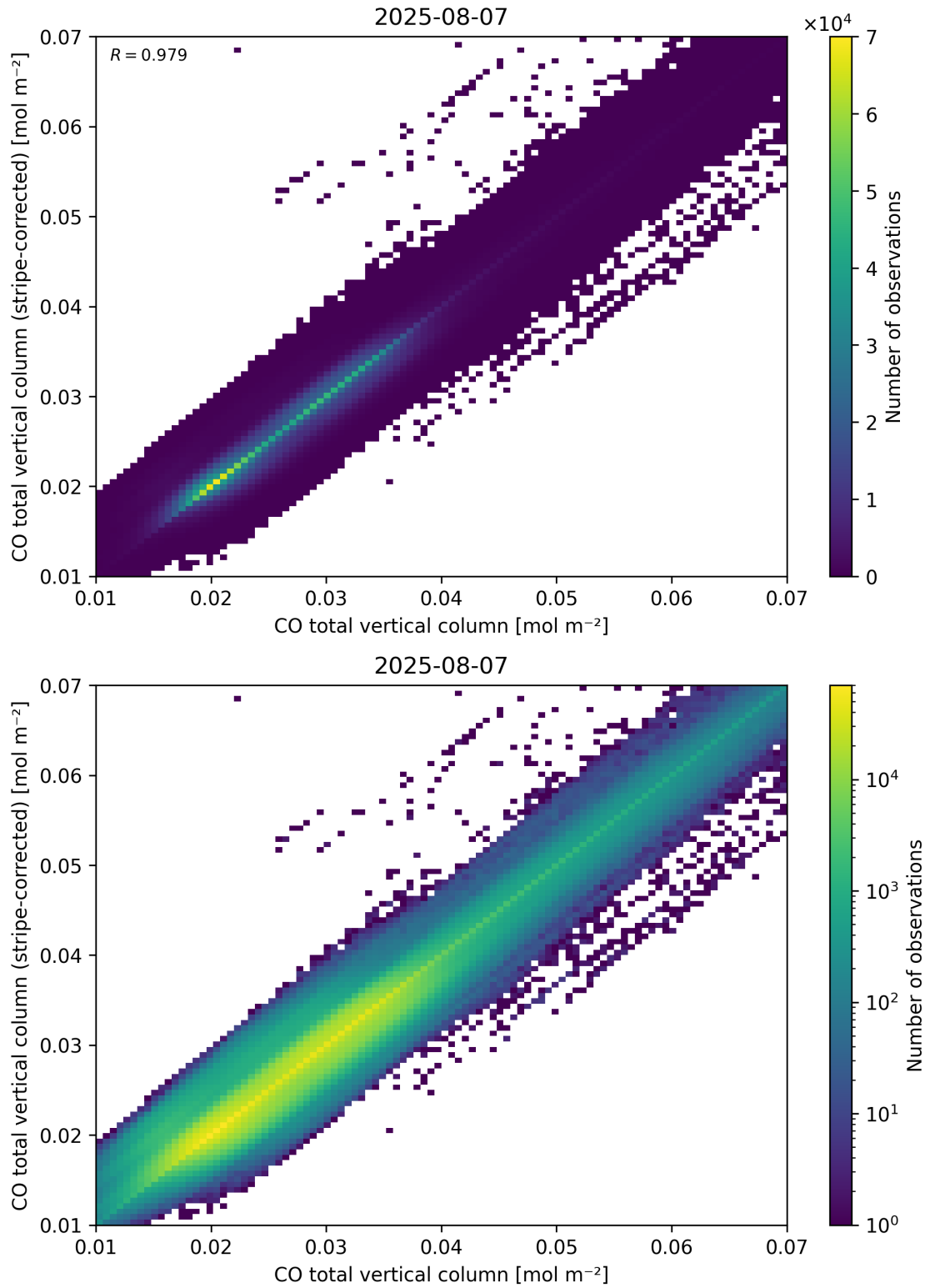
Figure 33: Scatter density plot of “CO total vertical column” against “CO total vertical column (stripe-corrected)” for 2025-08-06 to 2025-08-08.
