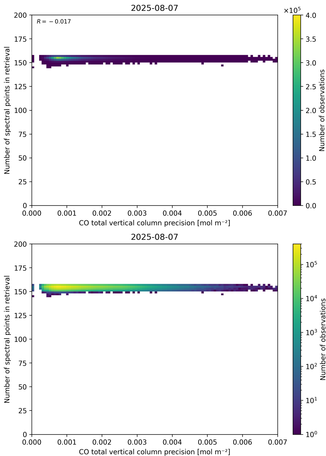
Figure 47: Scatter density plot of “CO total vertical column precision” against “Number of spectral points in retrieval” for 2025-08-06 to 2025-08-08.
