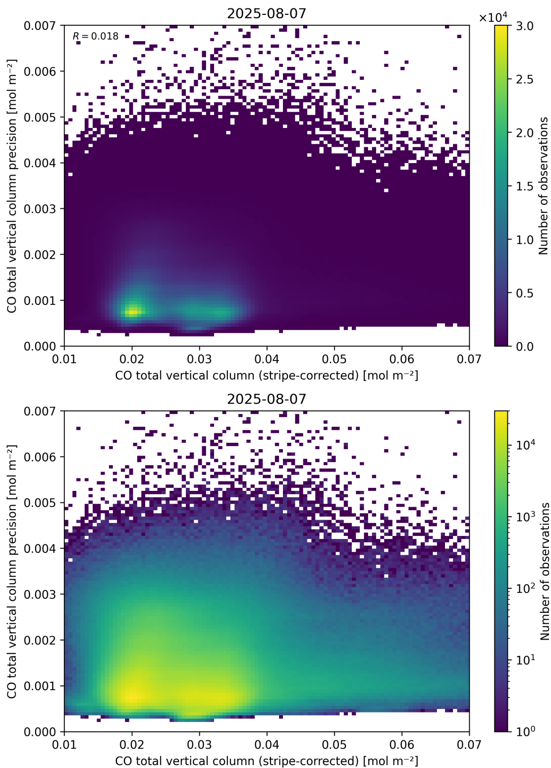
Figure 36: Scatter density plot of “CO total vertical column (stripe-corrected)” against “CO total vertical column precision” for 2025-08-06 to 2025-08-08.
