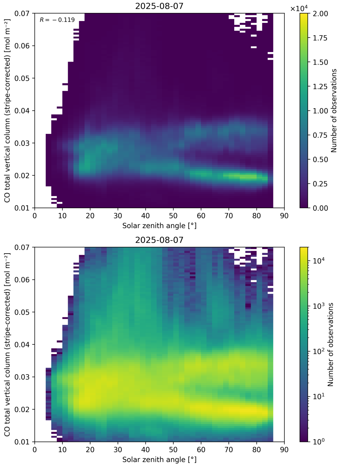
Figure 62: Scatter density plot of “Solar zenith angle” against “CO total vertical column (stripe-corrected)” for 2025-08-06 to 2025-08-08.
