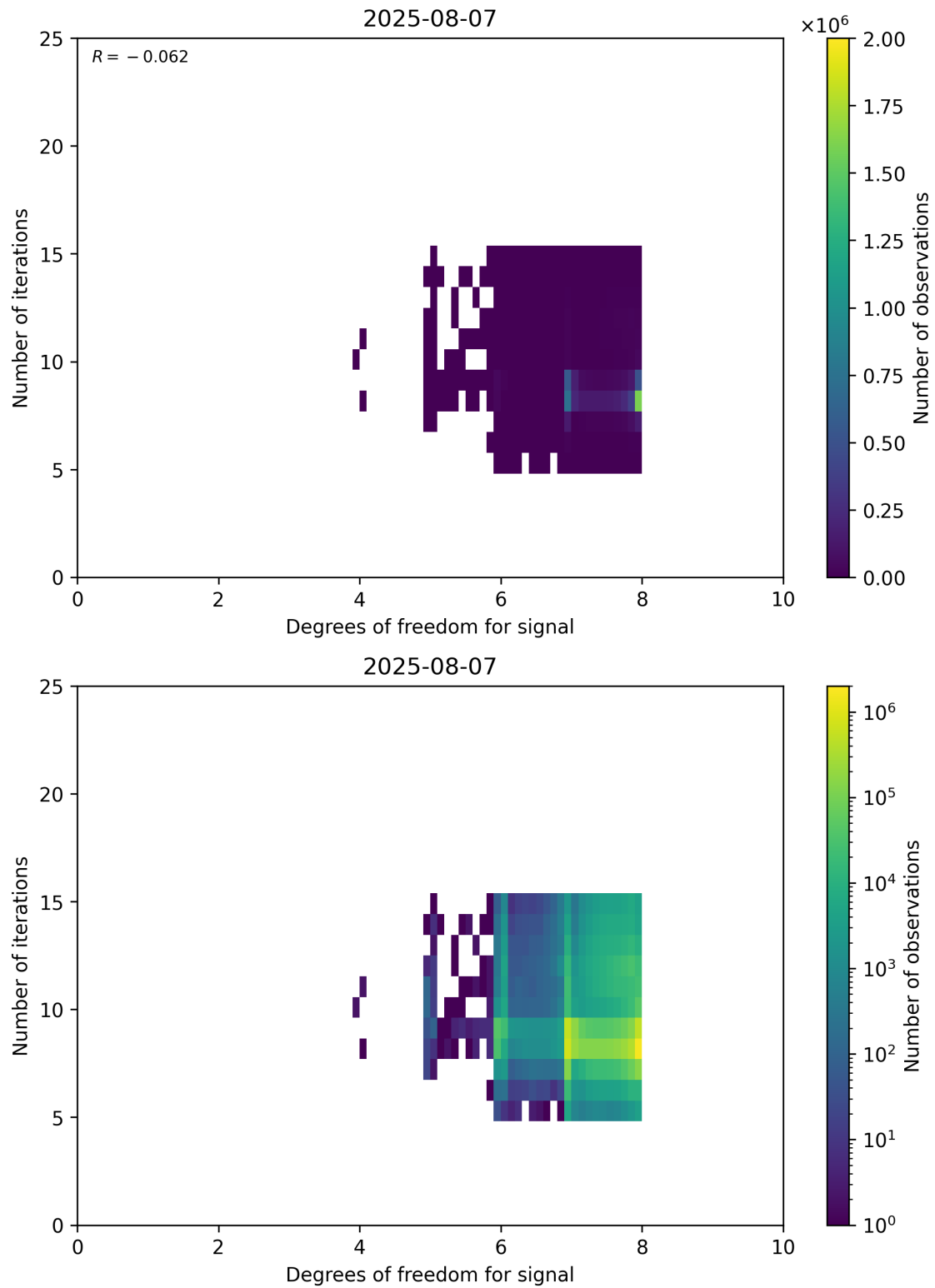
Figure 50: Scatter density plot of “Degrees of freedom for signal” against “Number of iterations” for 2025-08-06 to 2025-08-08.
