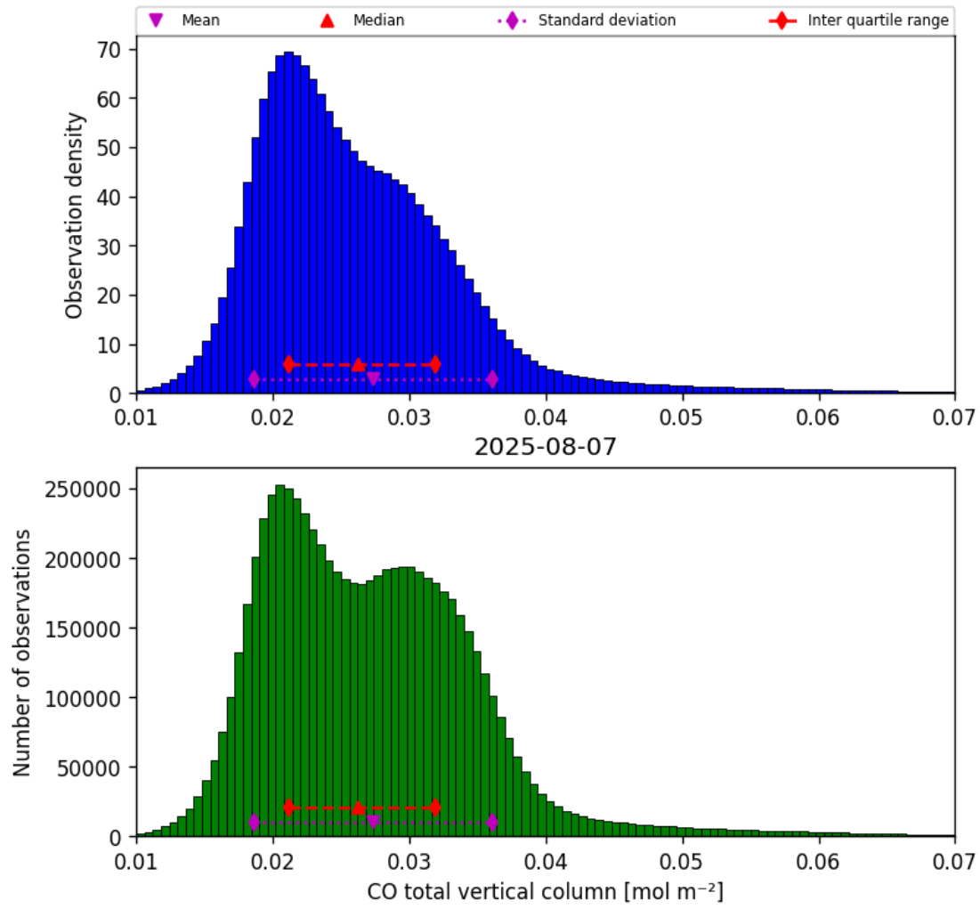
Figure 18: Histogram of “CO total vertical column” for 2025-08-06 to 2025-08-08
