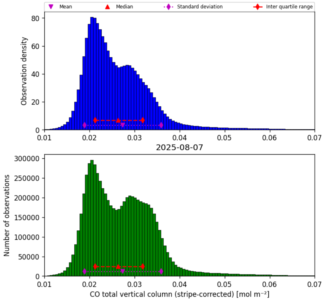
Figure 19: Histogram of “CO total vertical column (stripe-corrected)” for 2025-08-06 to 2025-08-08
