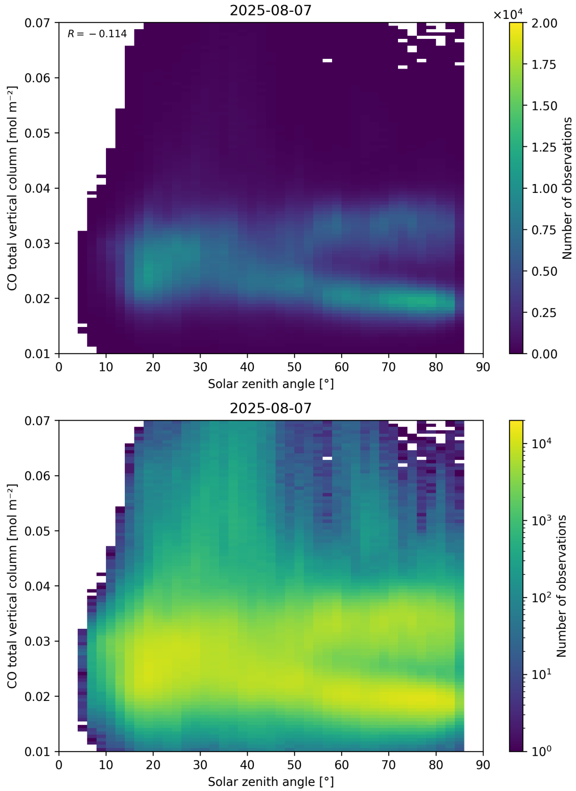
Figure 61: Scatter density plot of “Solar zenith angle” against “CO total vertical column” for 2025-08-06 to 2025-08-08.
