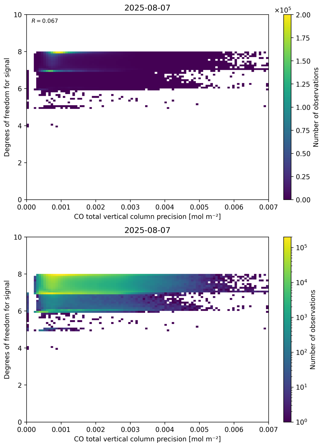
Figure 45: Scatter density plot of “CO total vertical column precision” against “Degrees of freedom for signal” for 2025-08-06 to 2025-08-08.
