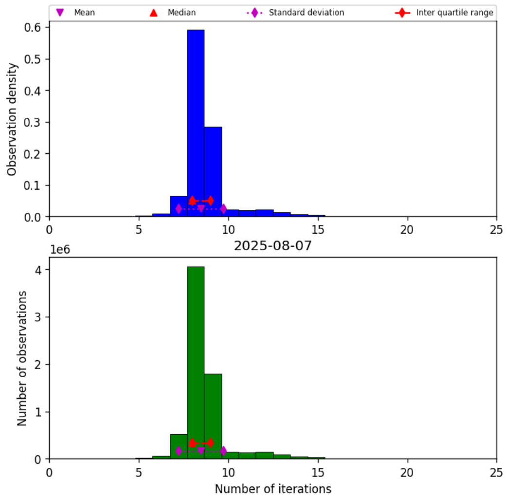
Figure 24: Histogram of “Number of iterations” for 2025-08-06 to 2025-08-08
