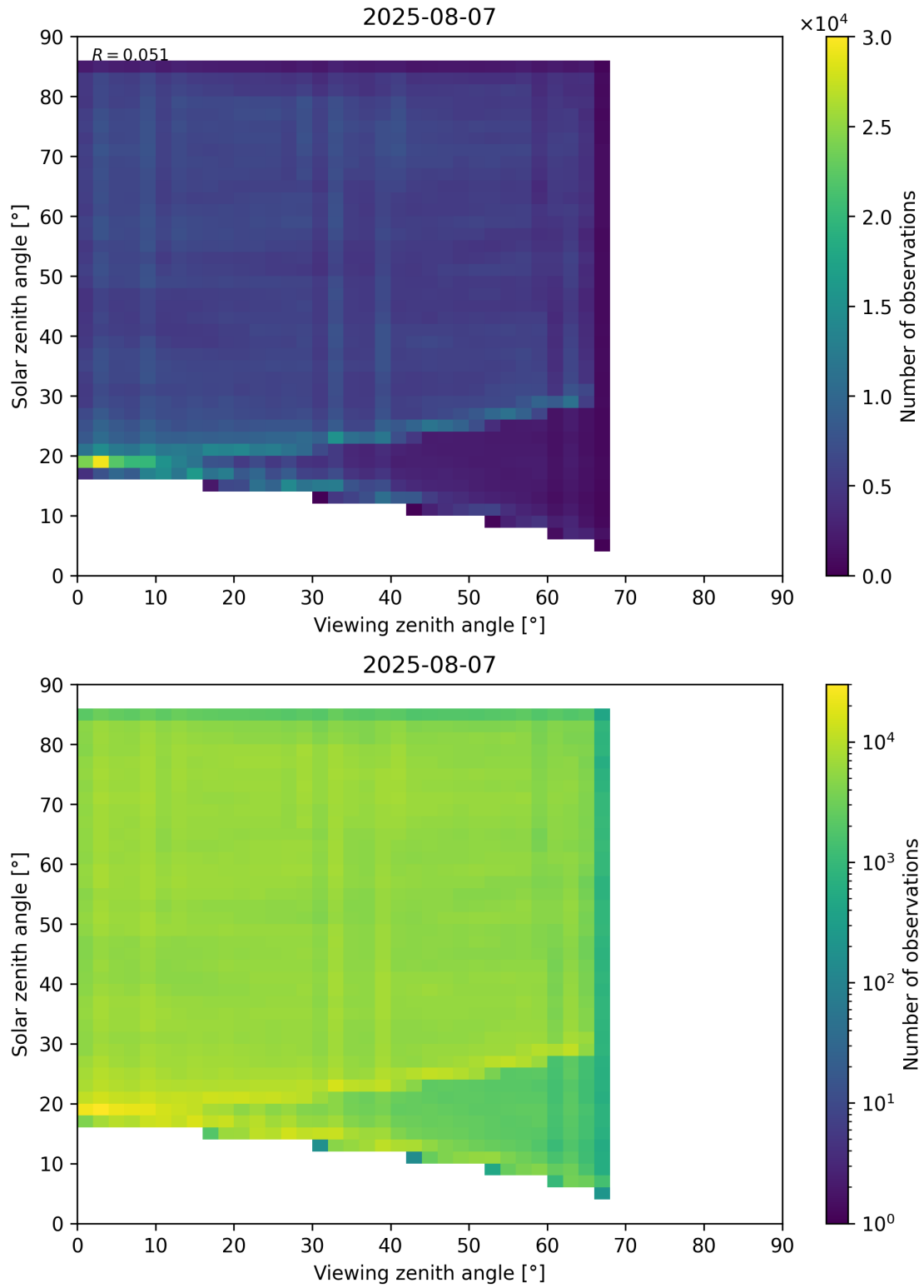
Figure 77: Scatter density plot of “Viewing zenith angle” against “Solar zenith angle” for 2025-08-06 to 2025-08-08.
