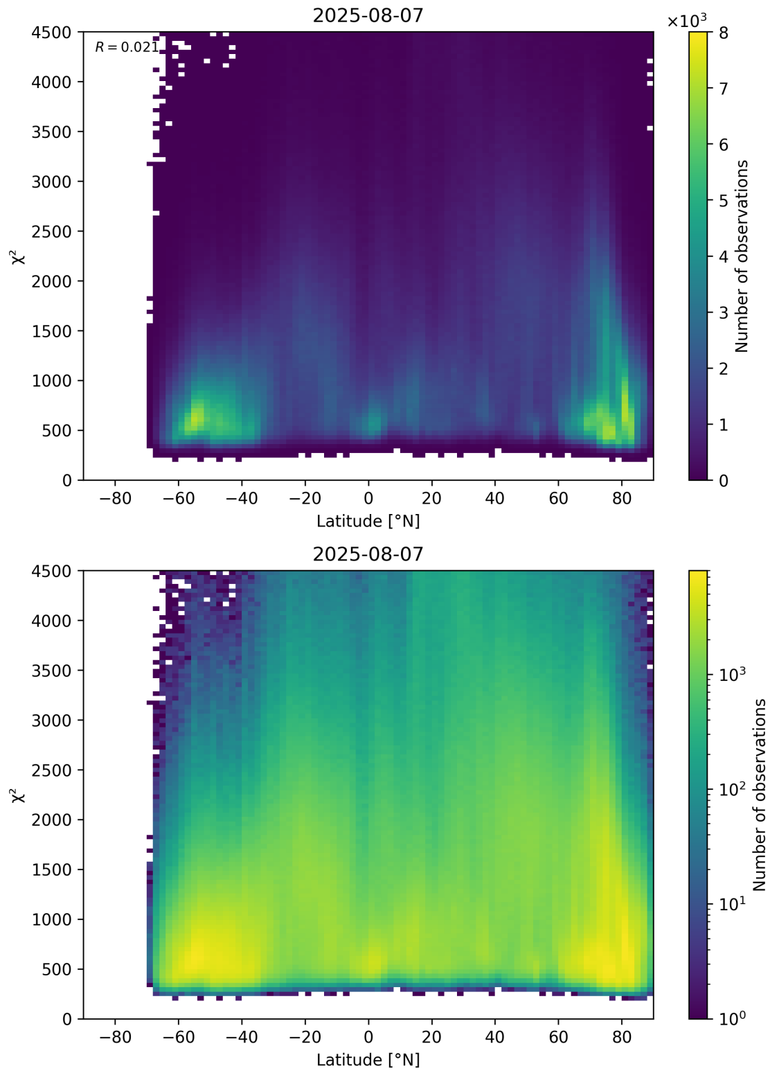
Figure 54: Scatter density plot of “Latitude” against “ \chi^2 ” for 2025-08-06 to 2025-08-08.
