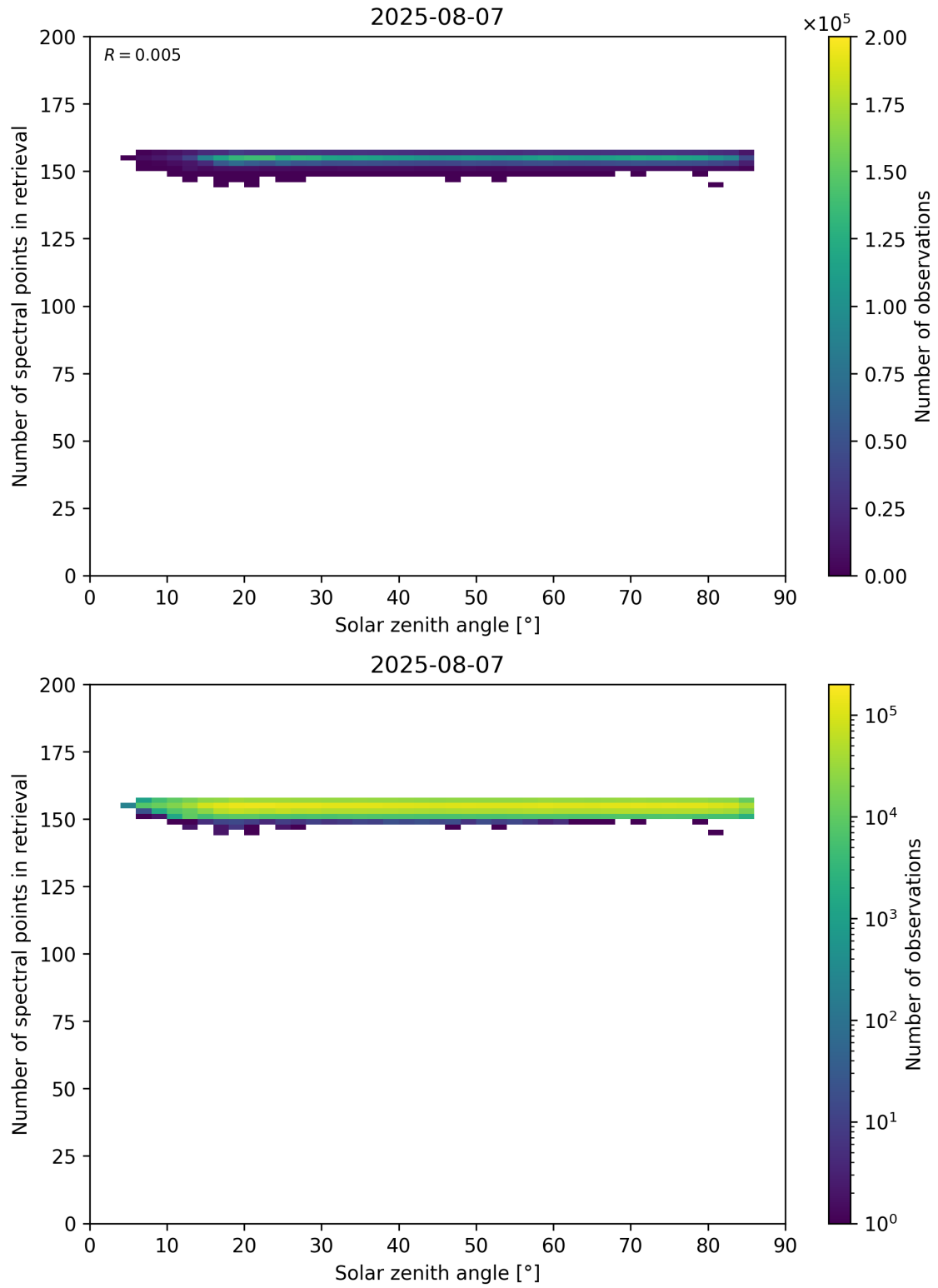
Figure 68: Scatter density plot of “Solar zenith angle” against “Number of spectral points in retrieval” for 2025-08-06 to 2025-08-08.
