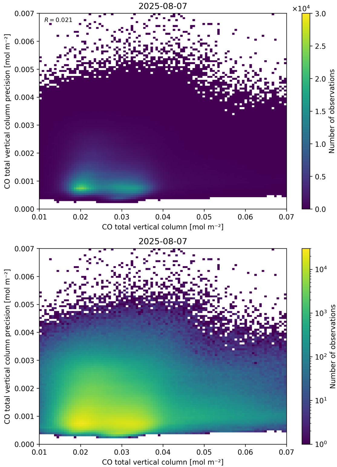
Figure 34: Scatter density plot of “CO total vertical column” against “CO total vertical column precision” for 2025-08-06 to 2025-08-08.
