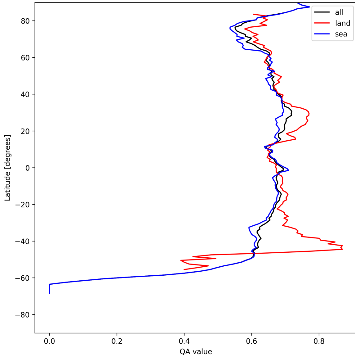
Figure 9: Zonal average of “QA value” for 2025-08-06 to 2025-08-08.
