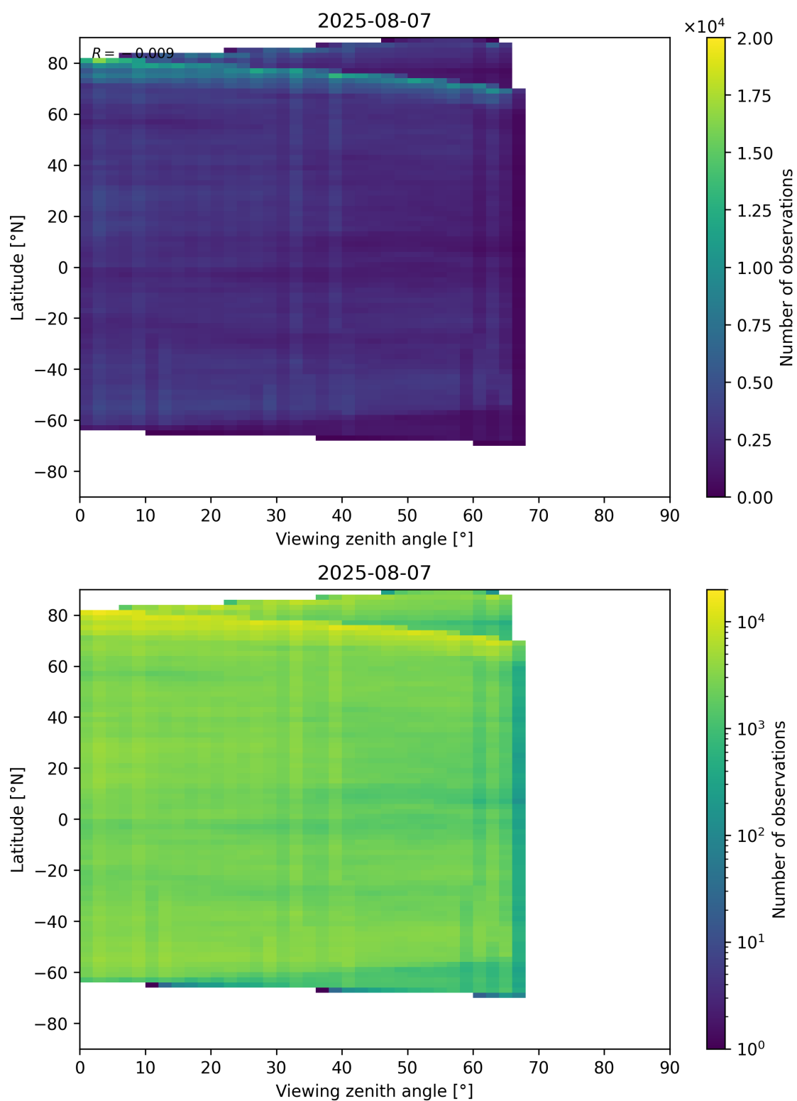
Figure 74: Scatter density plot of “Viewing zenith angle” against “Latitude” for 2025-08-06 to 2025-08-08.
