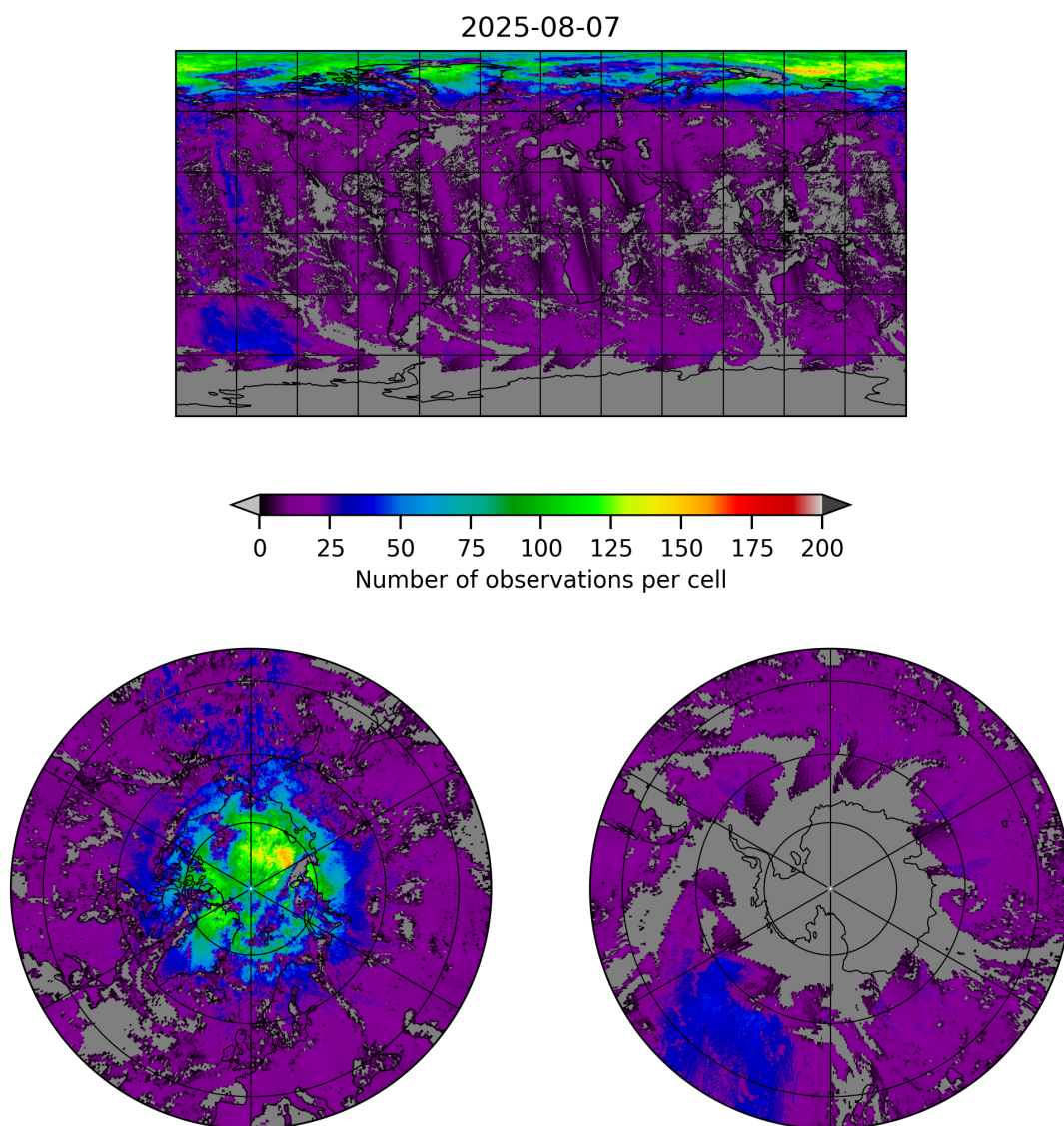
Figure 8: Map of the number of observations for 2025-08-06 to 2025-08-08
