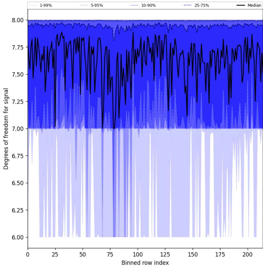
Figure 31: Along track statistics of “Degrees of freedom for signal” for 2025-08-06 to 2025-08-08
