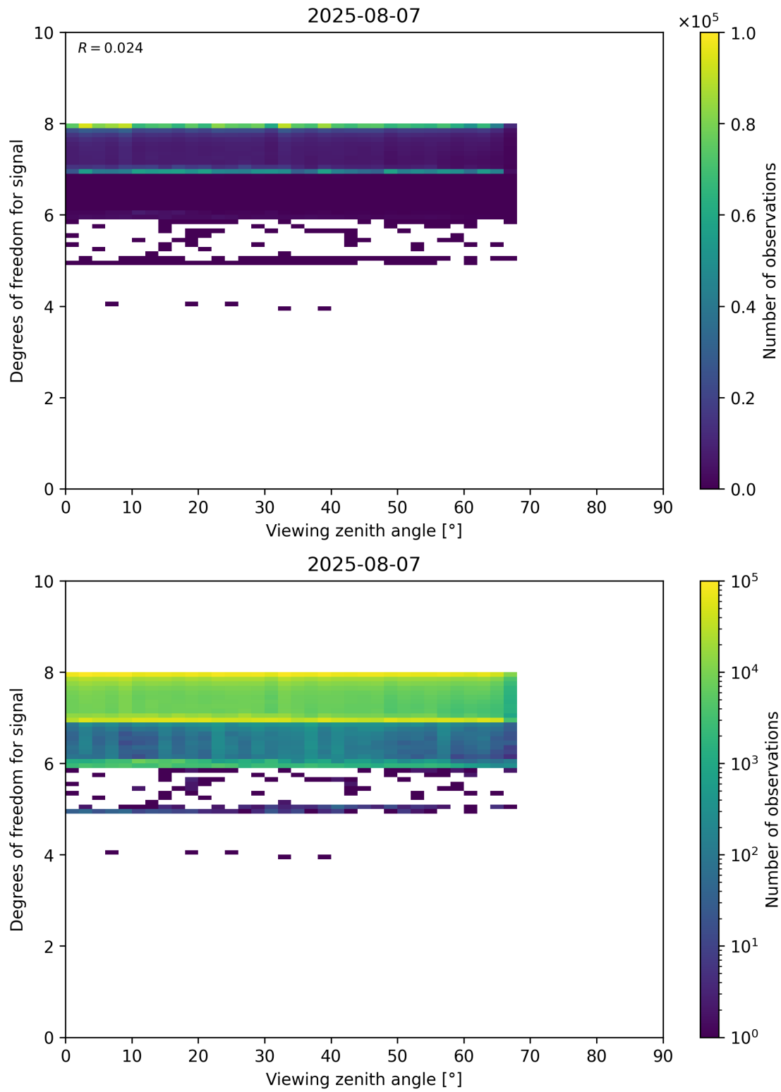
Figure 73: Scatter density plot of “Viewing zenith angle” against “Degrees of freedom for signal” for 2025-08-06 to 2025-08-08.
