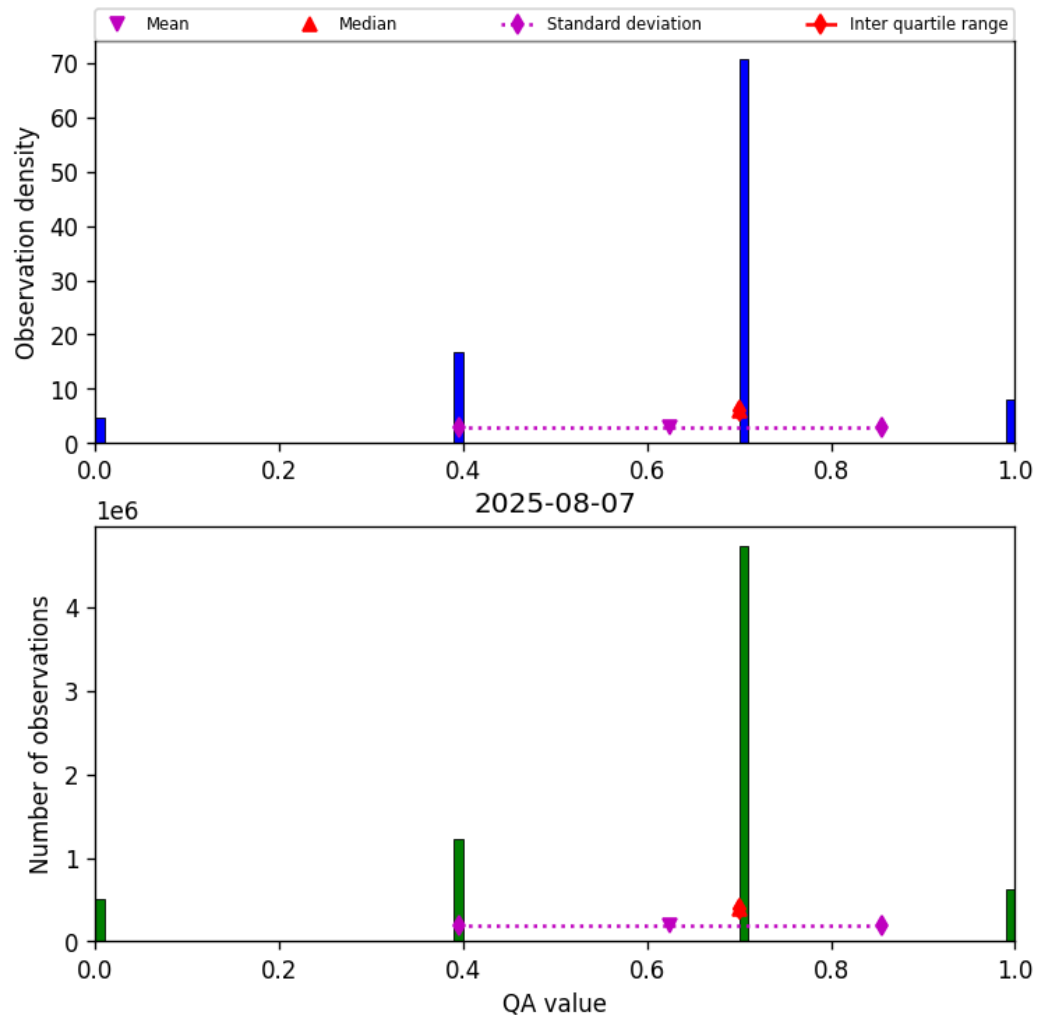
Figure 17: Histogram of “QA value” for 2025-08-06 to 2025-08-08
