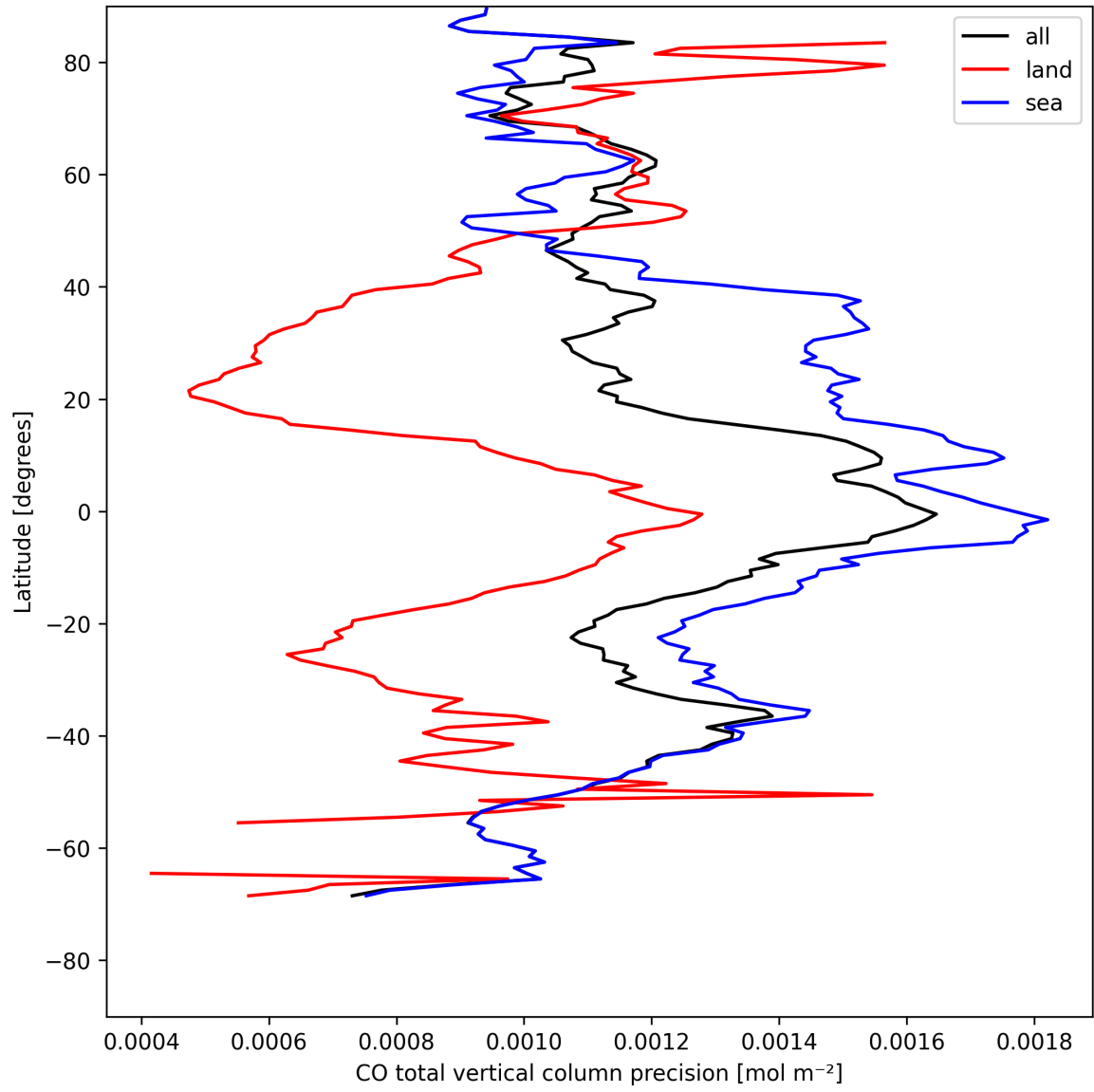
Figure 12: Zonal average of "CO total vertical column precision" for 2025-08-06 to 2025-08-08.
