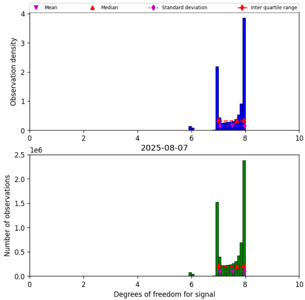
Figure 23: Histogram of “Degrees of freedom for signal” for 2025-08-06 to 2025-08-08
