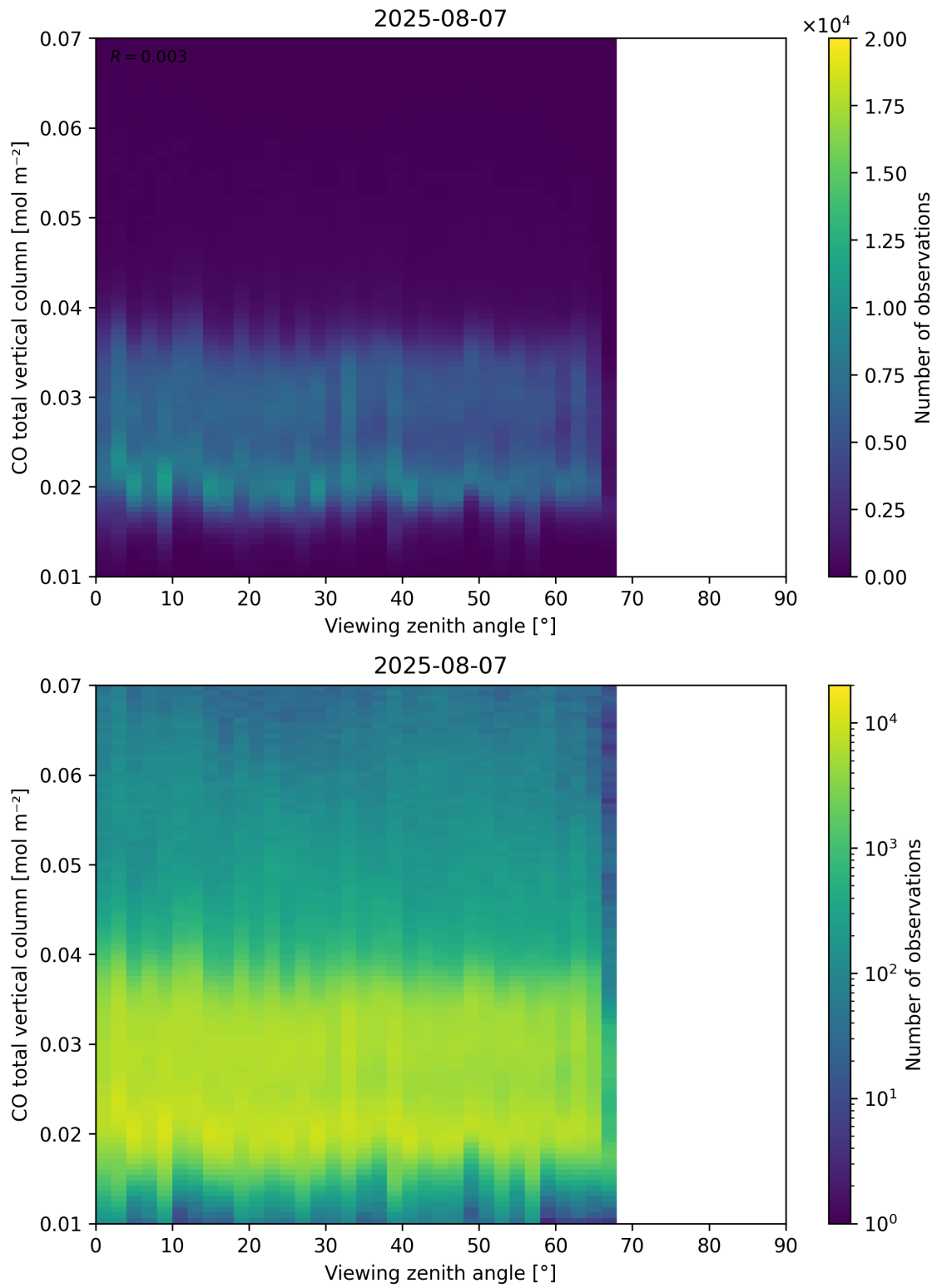
Figure 69: Scatter density plot of “Viewing zenith angle” against “CO total vertical column” for 2025-08-06 to 2025-08-08.
