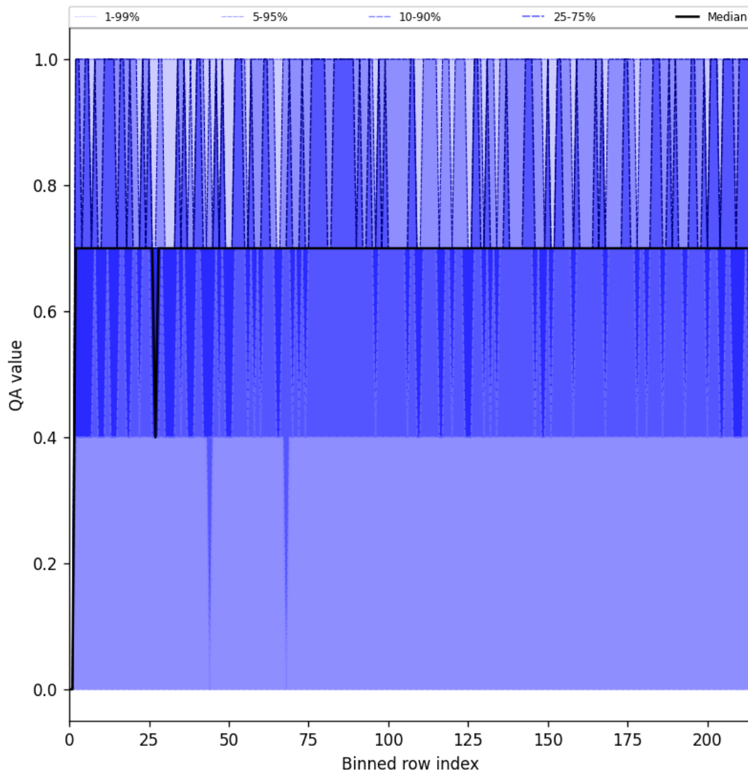
Figure 25: Along track statistics of “QA value” for 2025-08-06 to 2025-08-08
