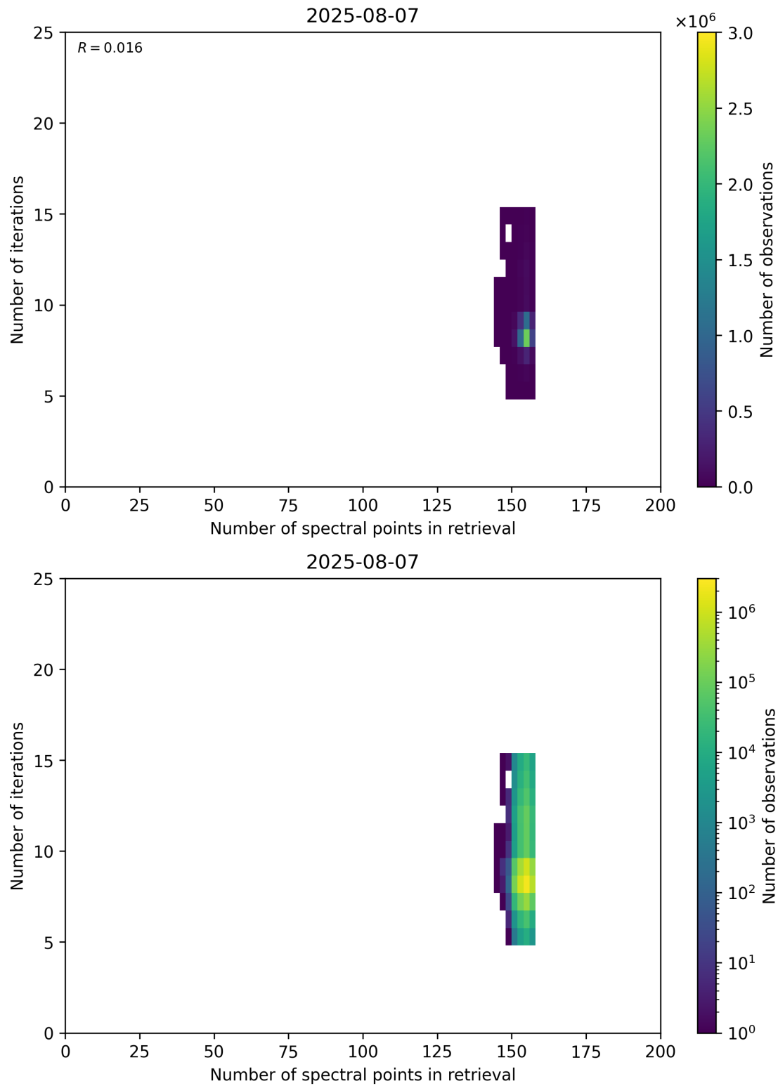
Figure 60: Scatter density plot of “Number of spectral points in retrieval” against “Number of iterations” for 2025-08-06 to 2025-08-08.
