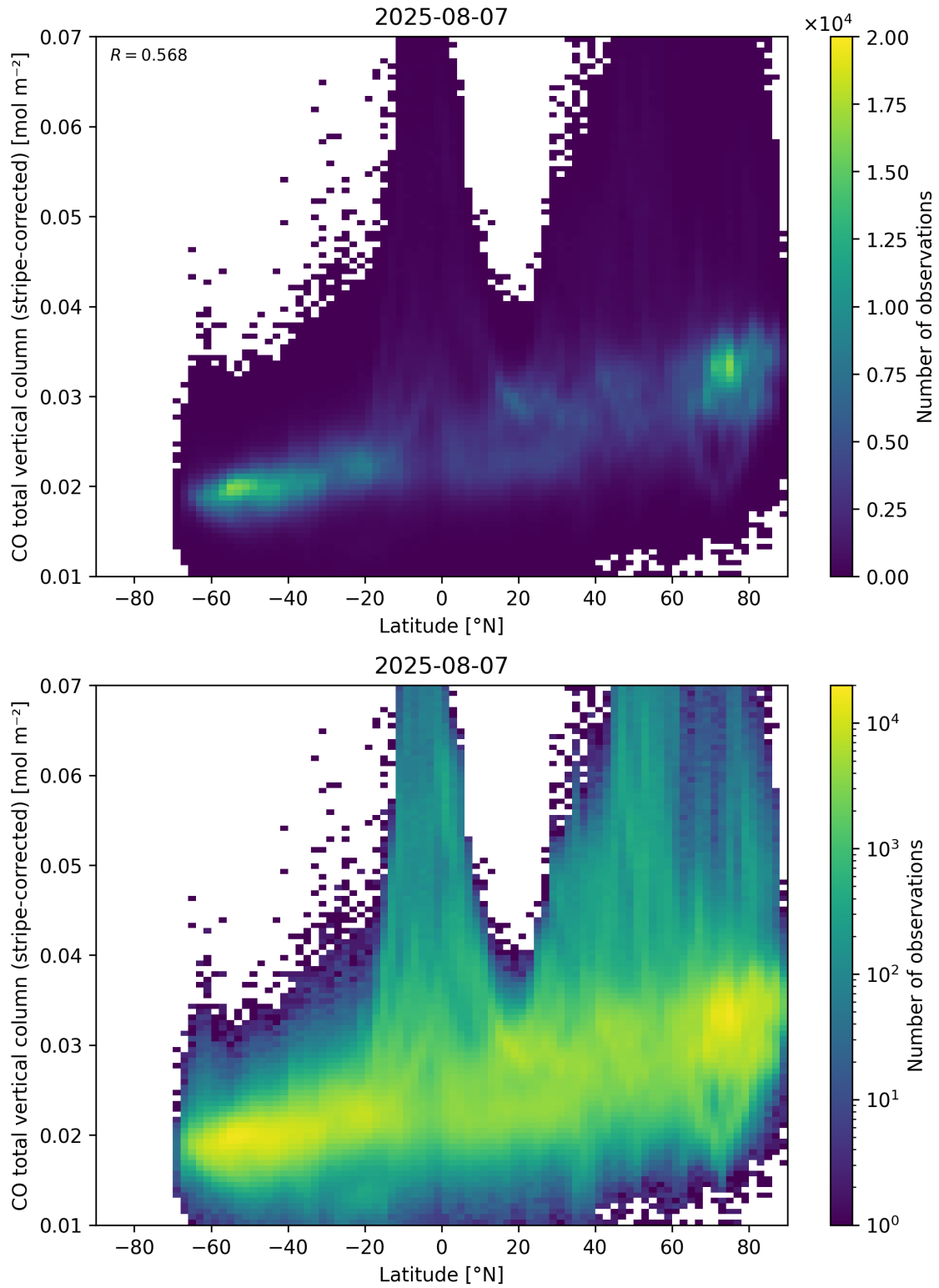
Figure 52: Scatter density plot of “Latitude” against “CO total vertical column (stripe-corrected)” for 2025-08-06 to 2025-08-08.
