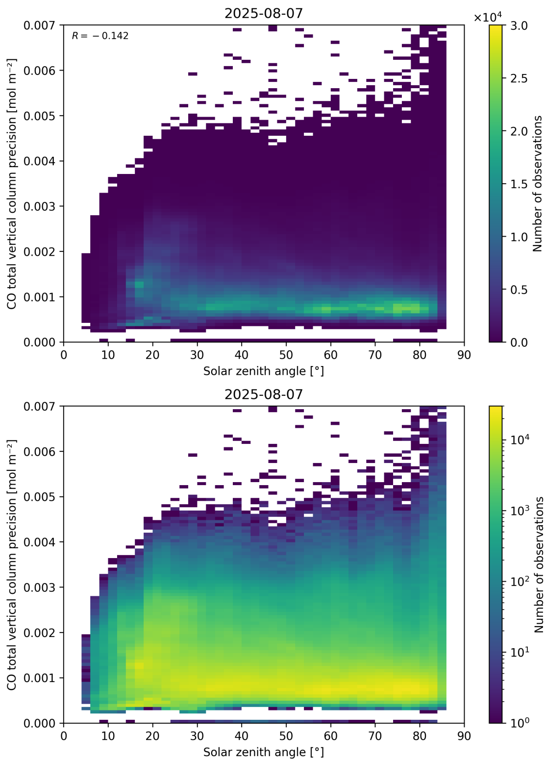
Figure 63: Scatter density plot of “Solar zenith angle” against “CO total vertical column precision” for 2025-08-06 to 2025-08-08.
