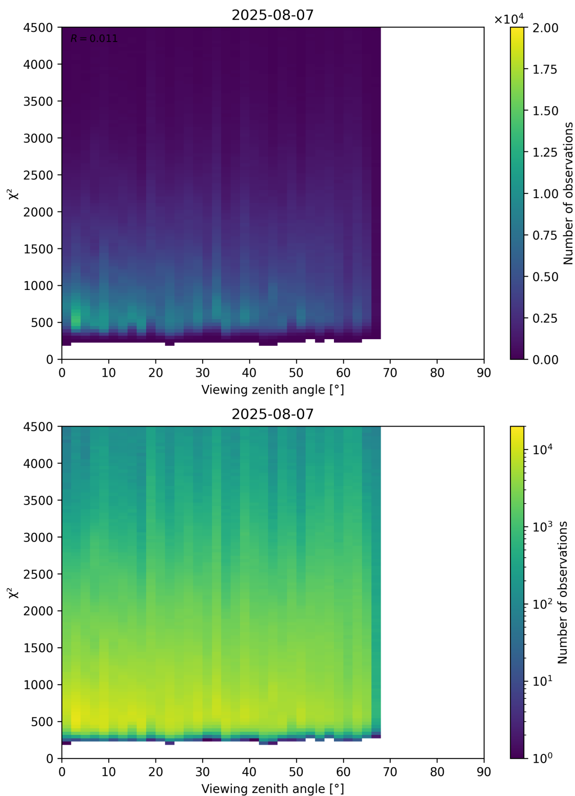
Figure 72: Scatter density plot of “Viewing zenith angle” against “ \chi^2 ” for 2025-08-06 to 2025-08-08.
