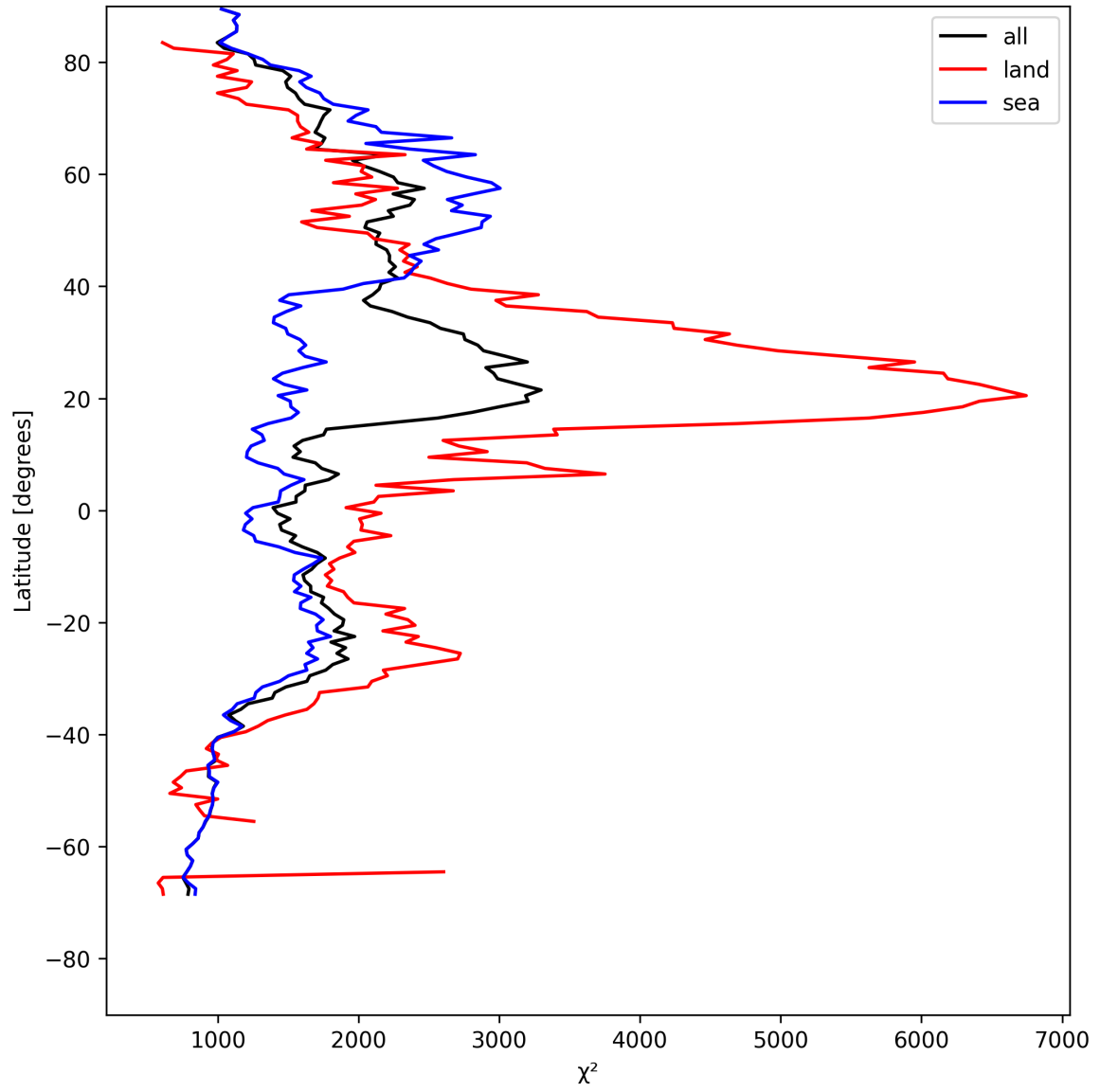
Figure 14: Zonal average of “ \chi^2 ” for 2025-08-06 to 2025-08-08.
