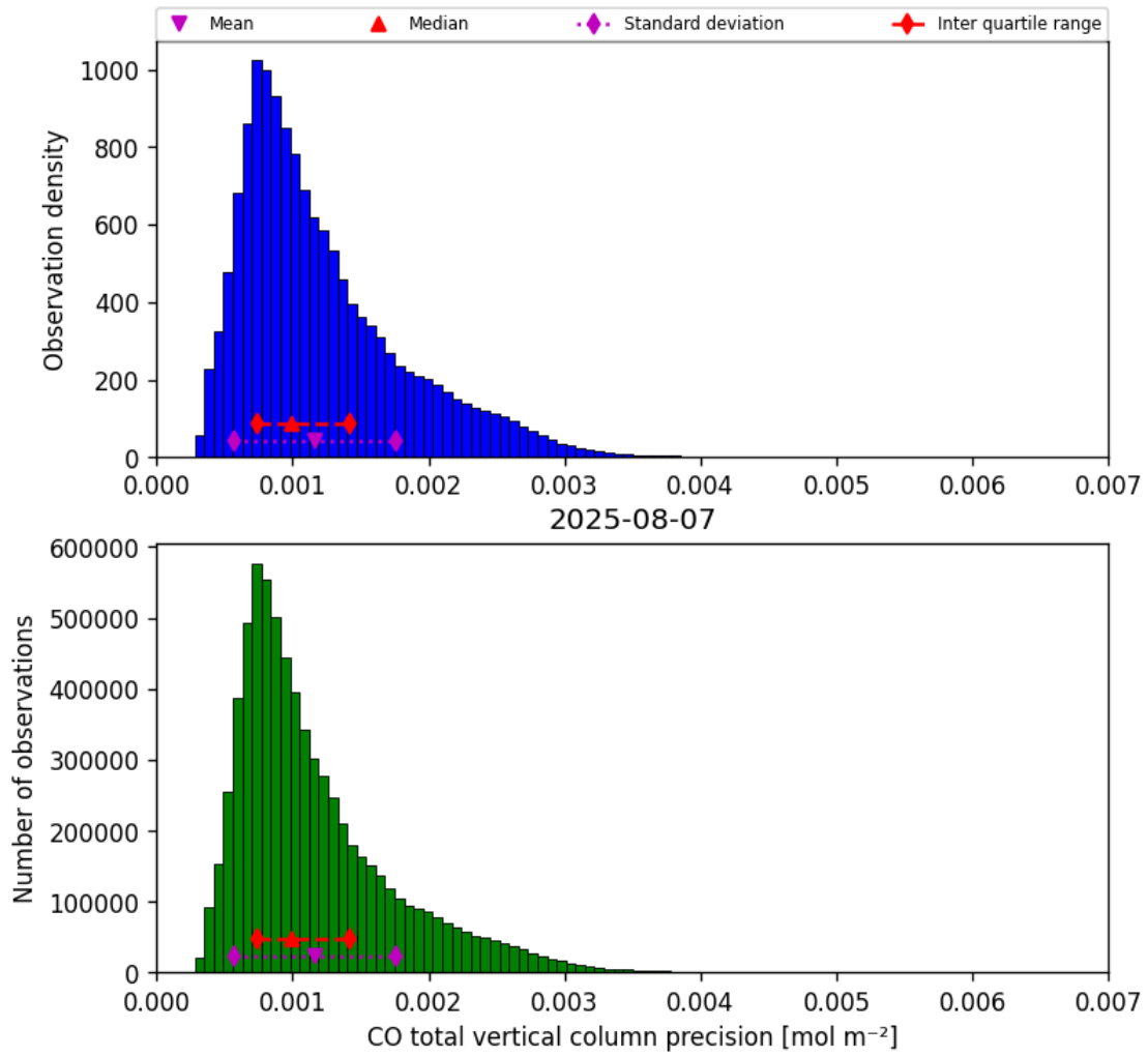
Figure 20: Histogram of “CO total vertical column precision” for 2025-08-06 to 2025-08-08
