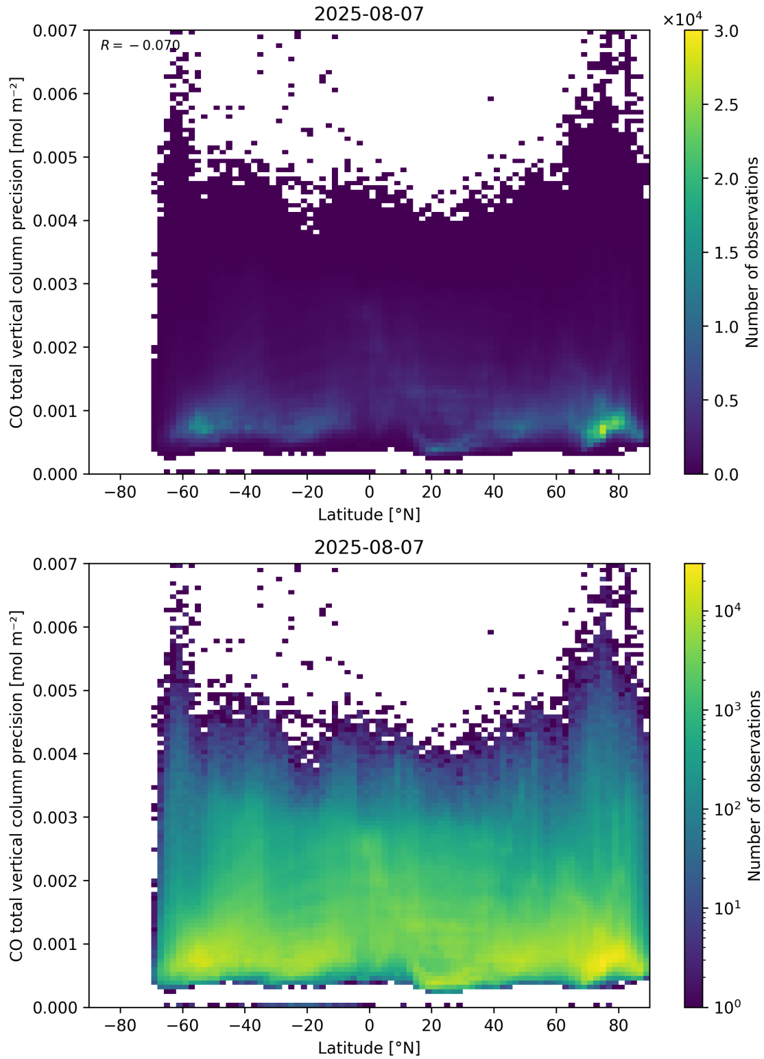
Figure 53: Scatter density plot of “Latitude” against “CO total vertical column precision” for 2025-08-06 to 2025-08-08.
