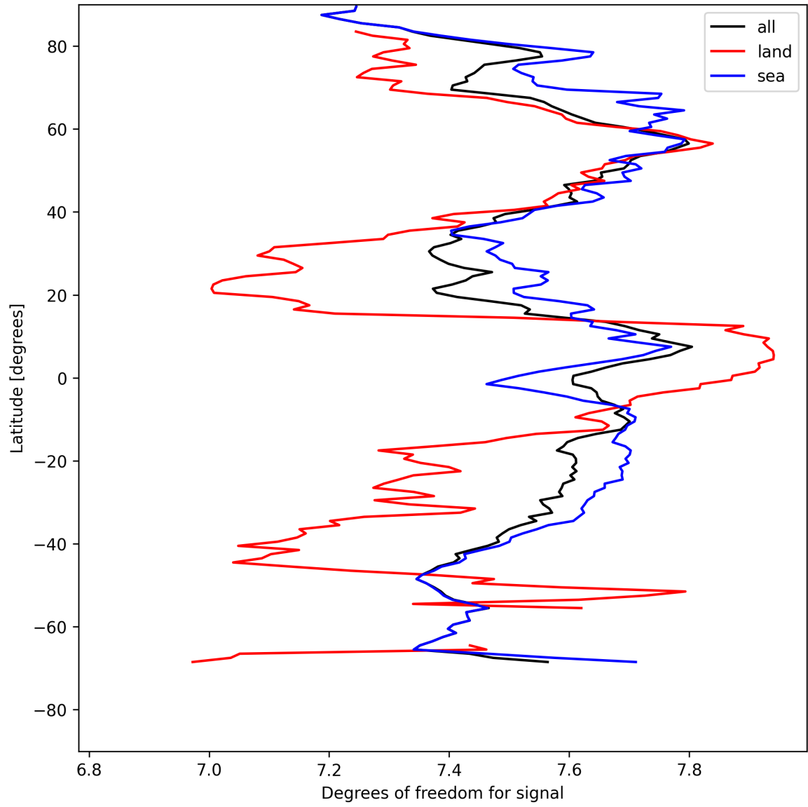
Figure 15: Zonal average of “Degrees of freedom for signal” for 2025-08-06 to 2025-08-08.
