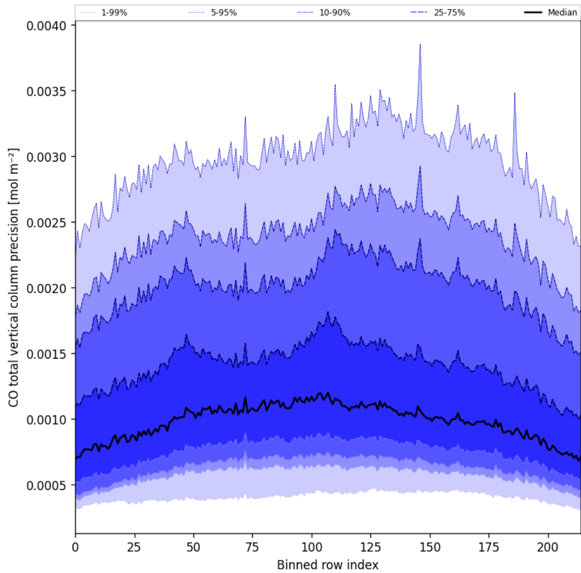
Figure 28: Along track statistics of “CO total vertical column precision” for 2025-08-06 to 2025-08-08
