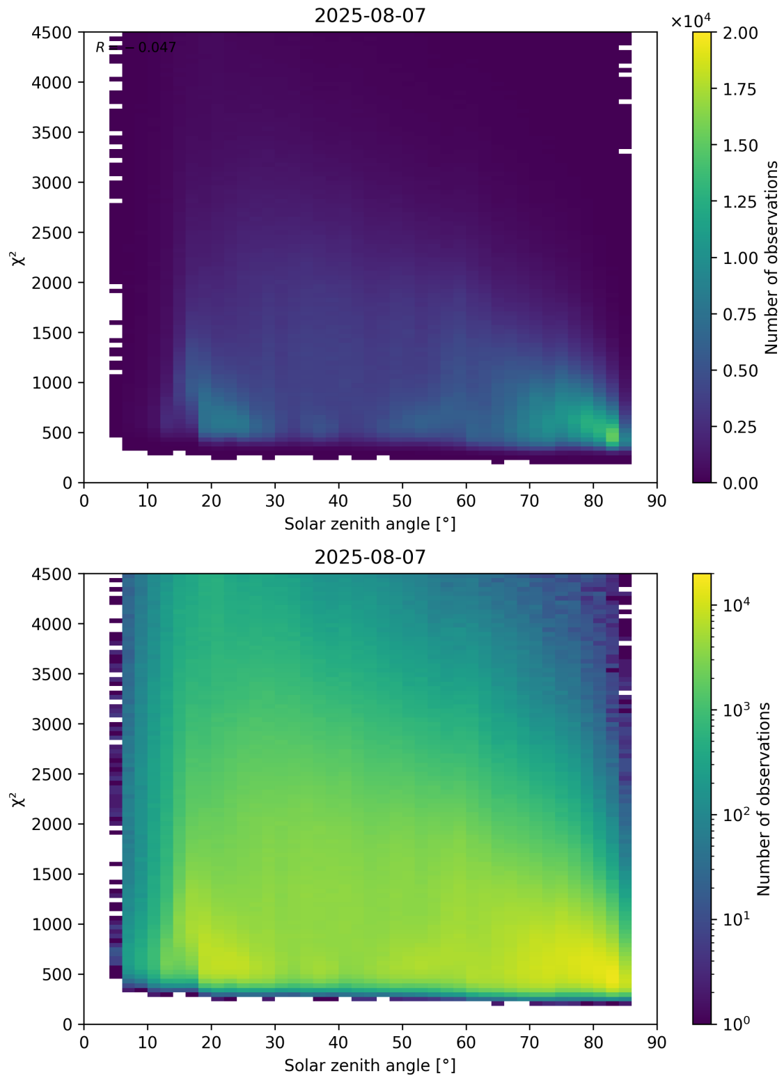
Figure 64: Scatter density plot of “Solar zenith angle” against “ \chi^2 ” for 2025-08-06 to 2025-08-08.
