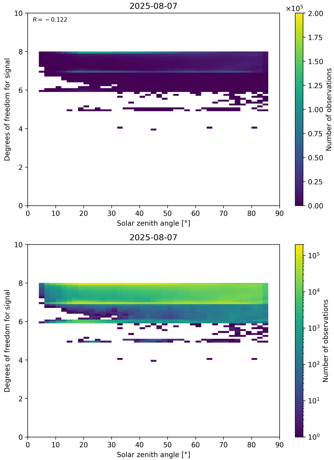
Figure 65: Scatter density plot of “Solar zenith angle” against “Degrees of freedom for signal” for 2025-08-06 to 2025-08-08.
