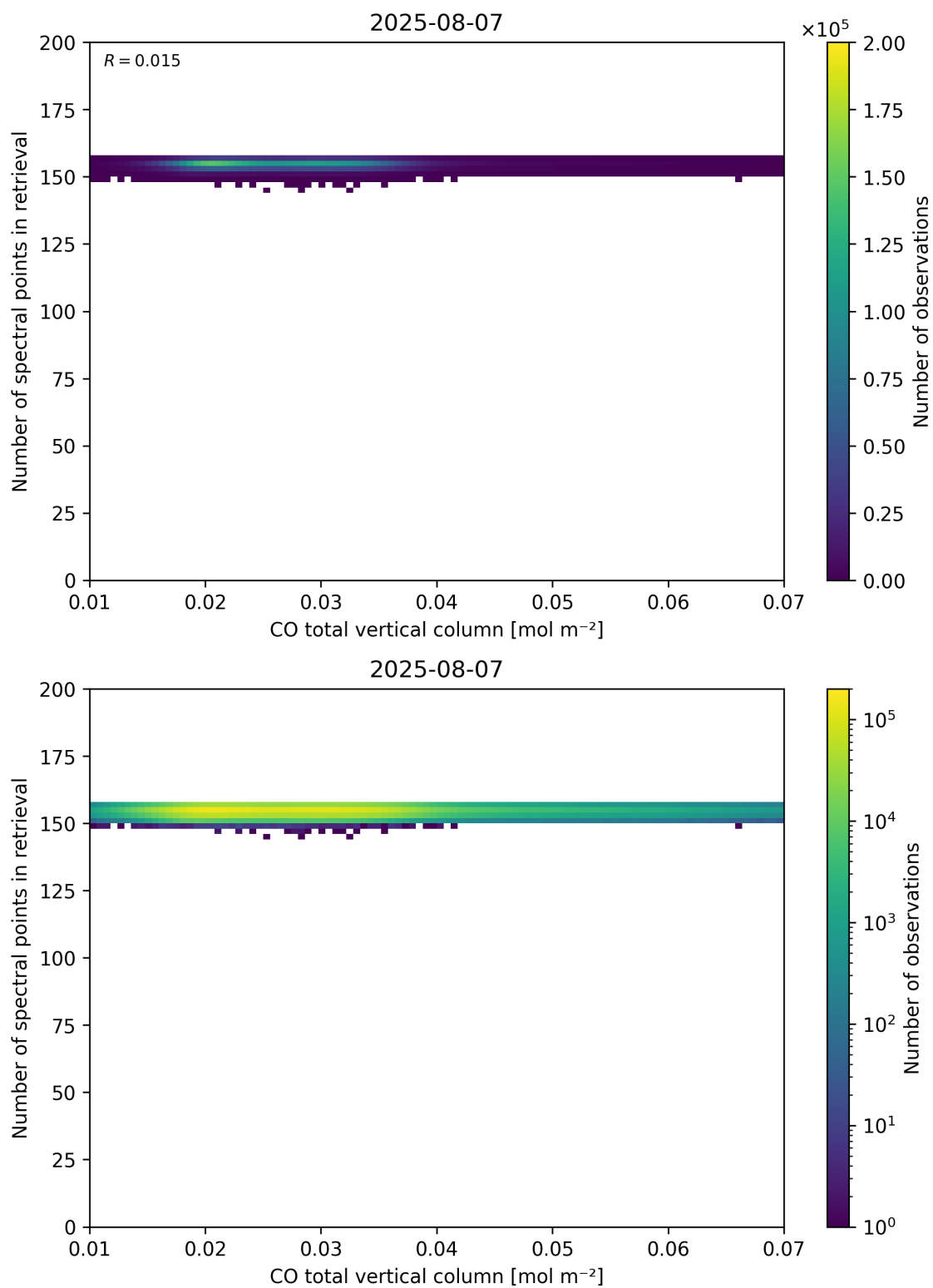
Figure 43: Scatter density plot of “CO total vertical column” against “Number of spectral points in retrieval” for 2025-08-06 to 2025-08-08.
