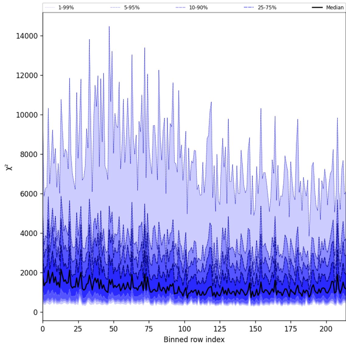
Figure 30: Along track statistics of “ \chi^2 ” for 2025-08-06 to 2025-08-08
