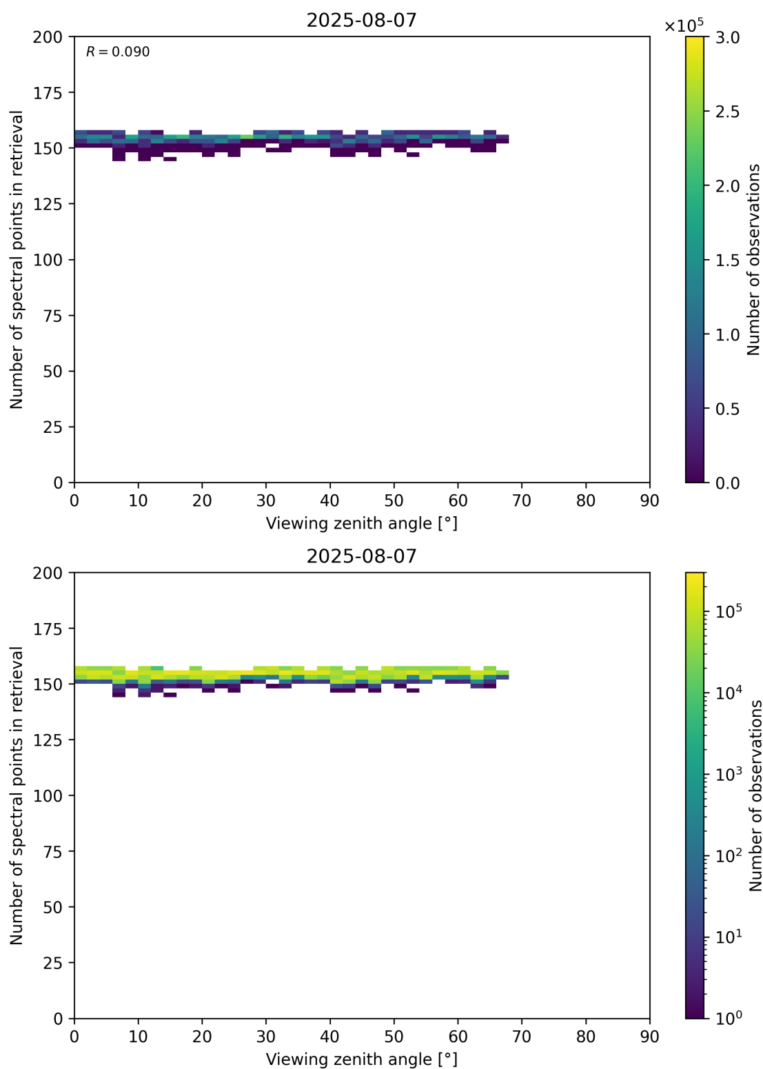
Figure 76: Scatter density plot of “Viewing zenith angle” against “Number of spectral points in retrieval” for 2025-08-06 to 2025-08-08.
