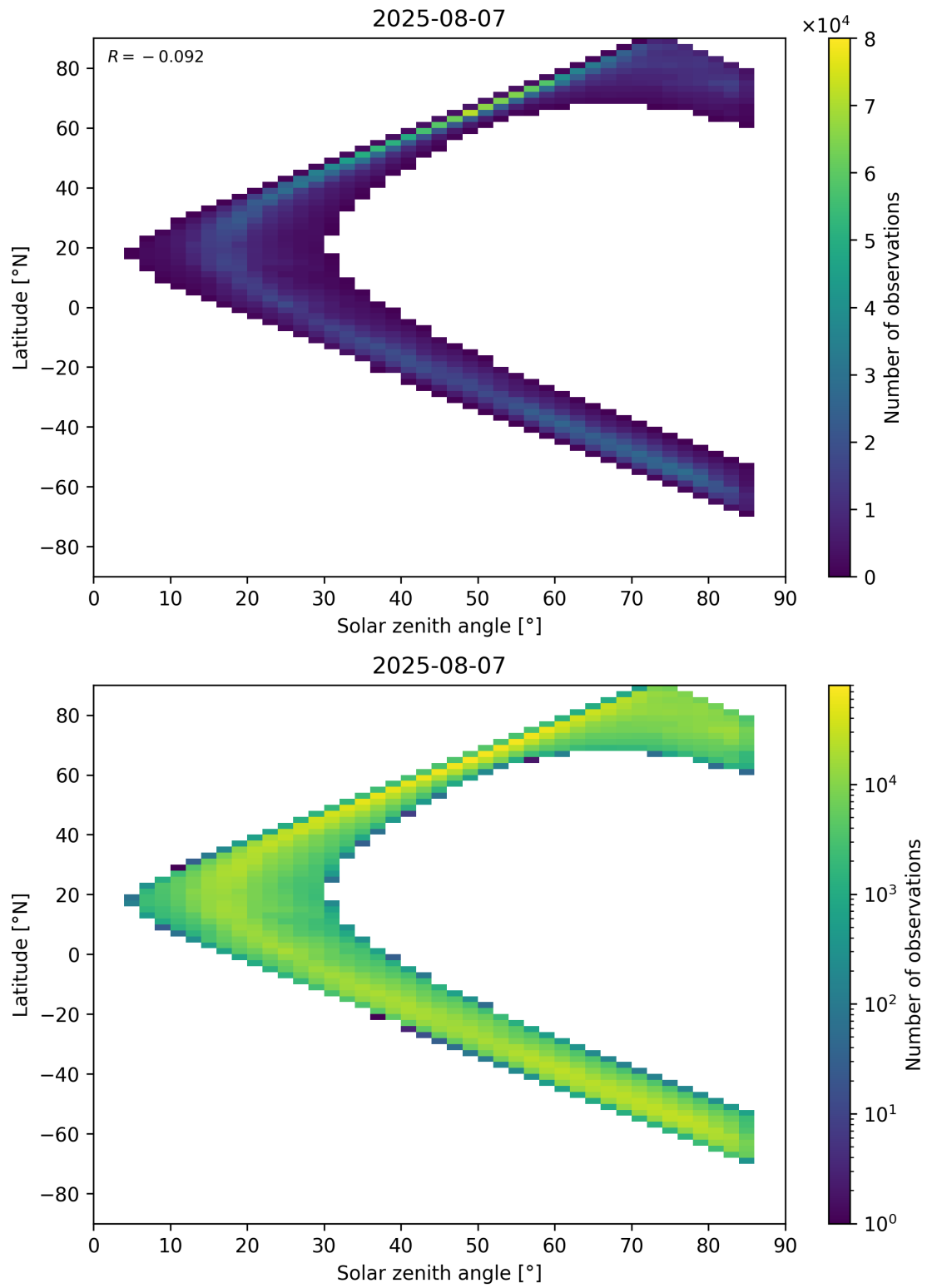
Figure 66: Scatter density plot of “Solar zenith angle” against “Latitude” for 2025-08-06 to 2025-08-08.
