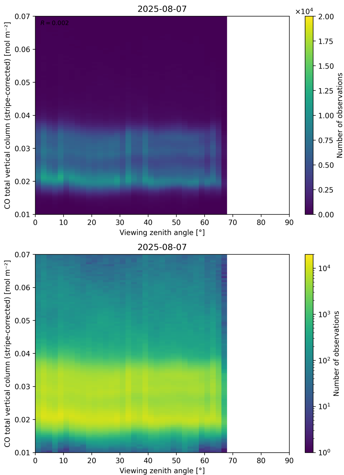
Figure 70: Scatter density plot of “Viewing zenith angle” against “CO total vertical column (stripe-corrected)” for 2025-08-06 to 2025-08-08.
