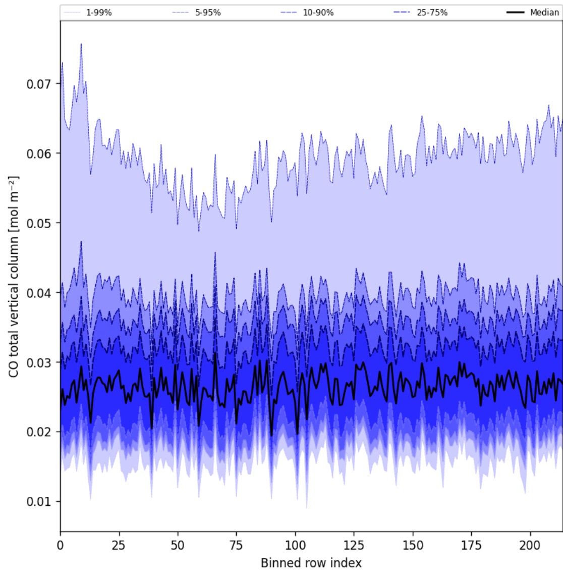
Figure 26: Along track statistics of “CO total vertical column” for 2025-08-06 to 2025-08-08
