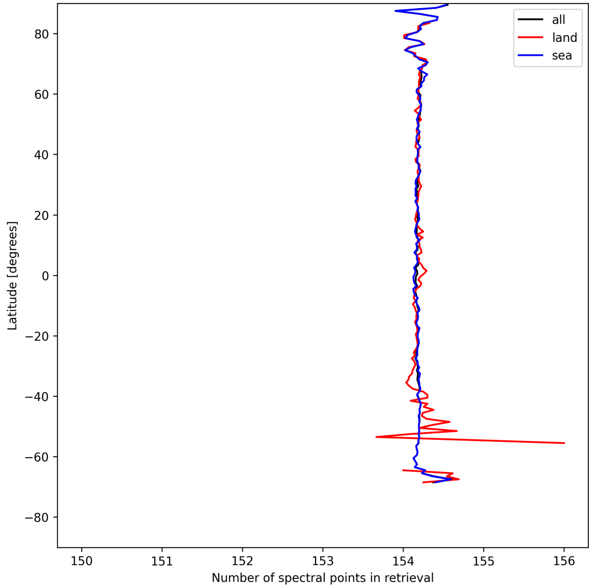
Figure 13: Zonal average of “Number of spectral points in retrieval” for 2025-08-06 to 2025-08-08.
