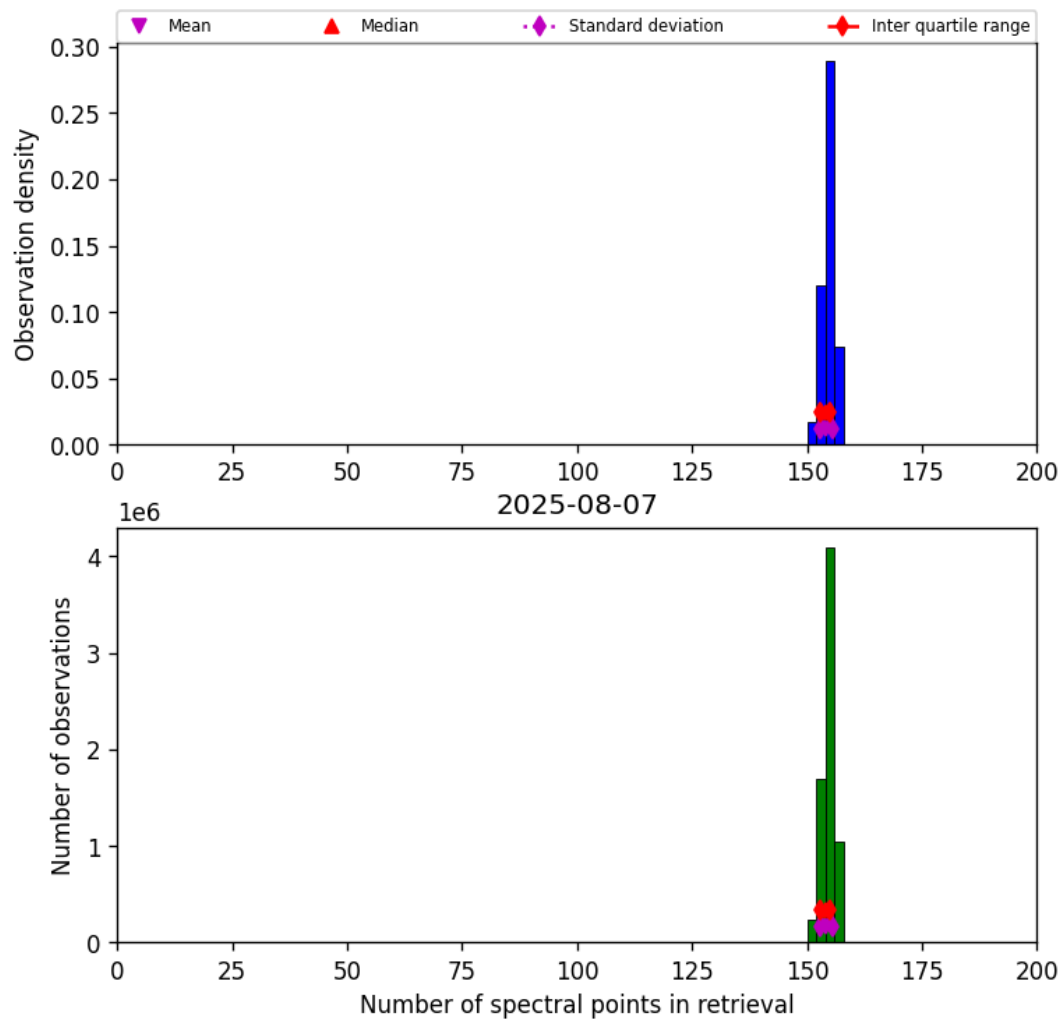
Figure 21: Histogram of “Number of spectral points in retrieval” for 2025-08-06 to 2025-08-08
