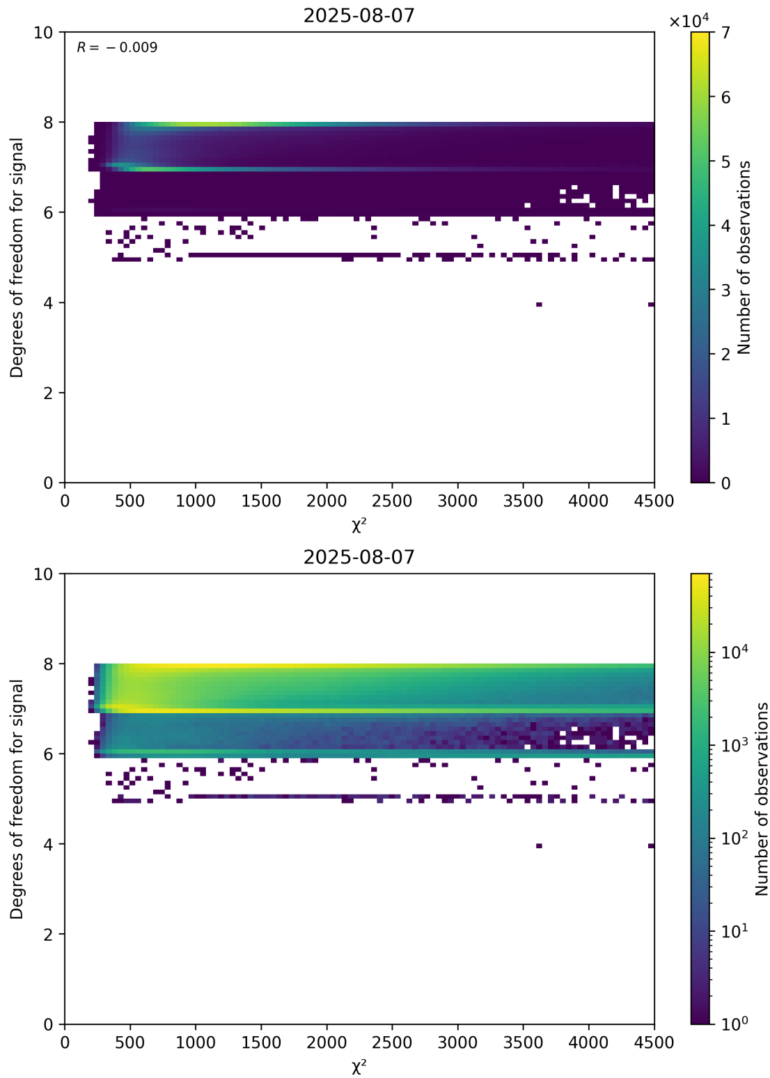
Figure 48: Scatter density plot of “ \chi^2 ” against “Degrees of freedom for signal” for 2025-08-06 to 2025-08-08.
