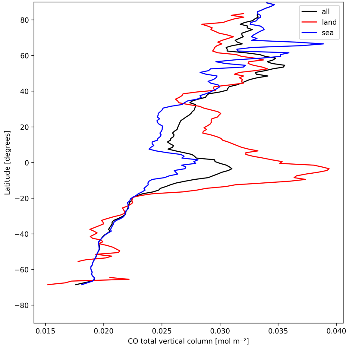
Figure 10: Zonal average of “CO total vertical column” for 2025-08-06 to 2025-08-08.
