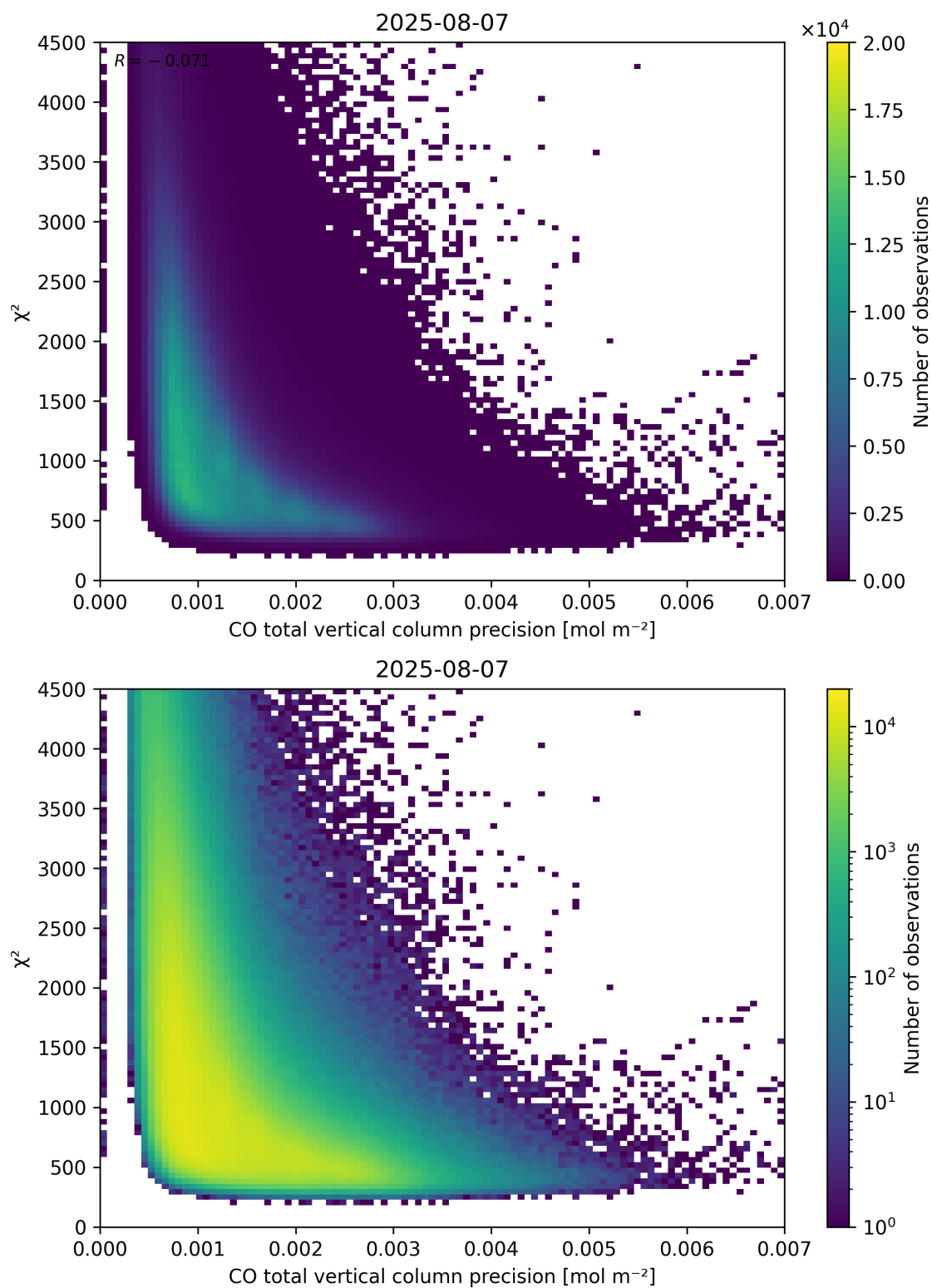
Figure 44: Scatter density plot of “CO total vertical column precision” against “ \chi^2 ” for 2025-08-06 to 2025-08-08.
