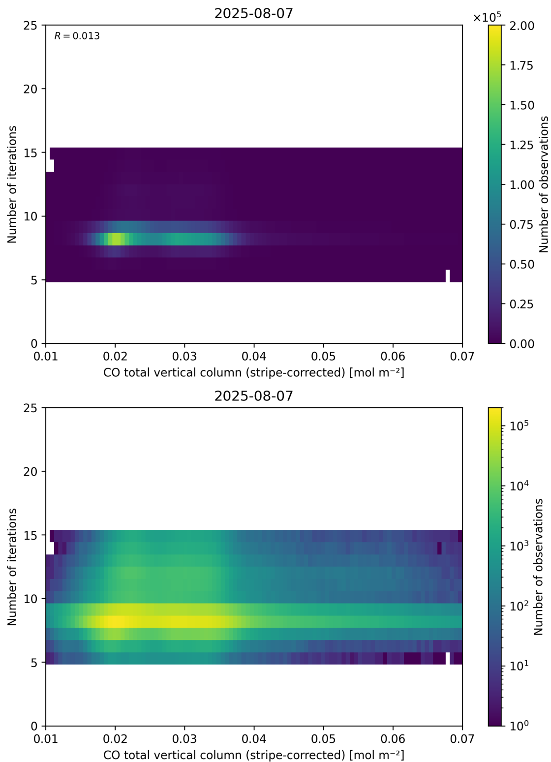
Figure 39: Scatter density plot of “CO total vertical column (stripe-corrected)” against “Number of iterations” for 2025-08-06 to 2025-08-08.
