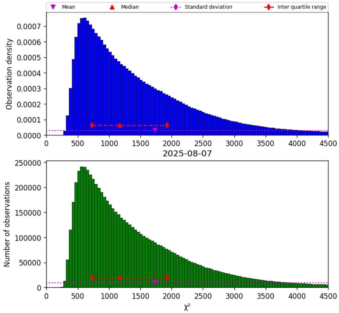
Figure 22: Histogram of “ \chi^2 ” for 2025-08-06 to 2025-08-08
