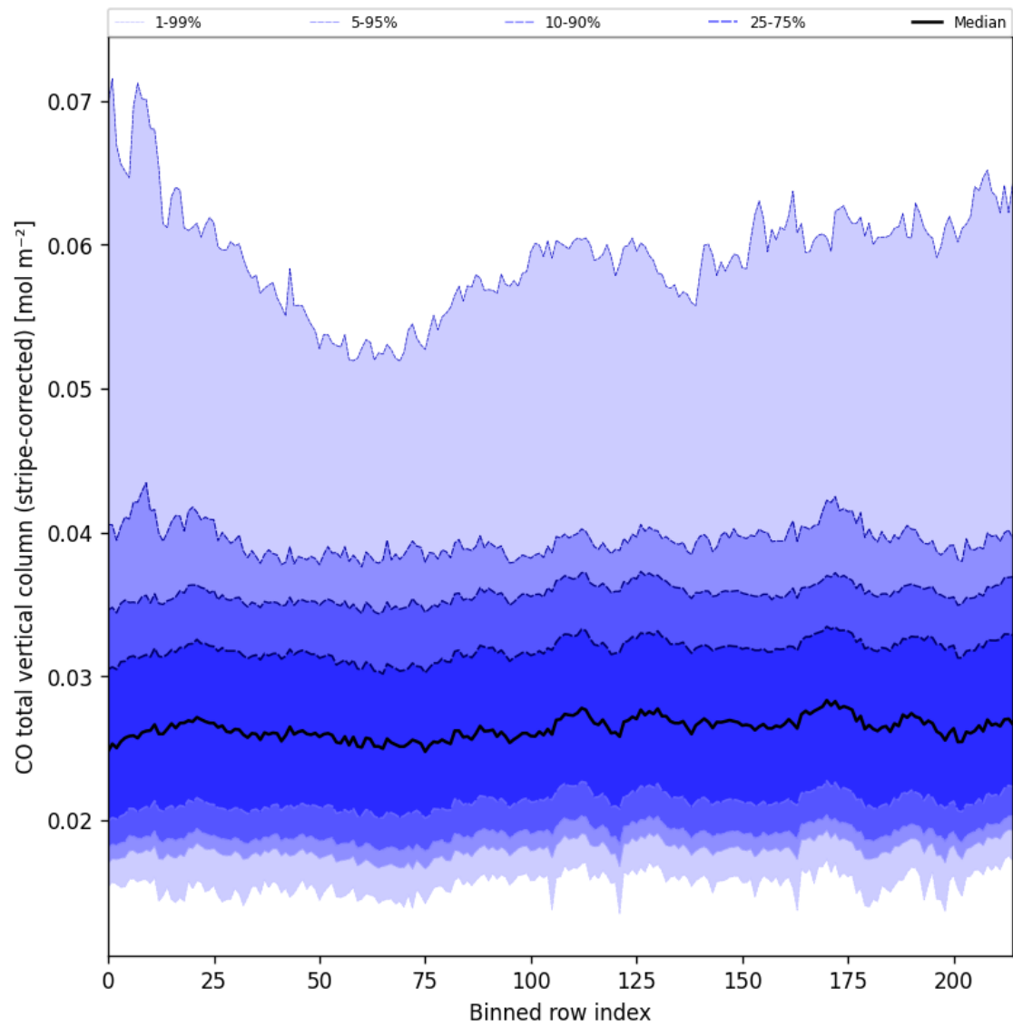
Figure 27: Along track statistics of “CO total vertical column (stripe-corrected)” for 2025-08-06 to 2025-08-08
