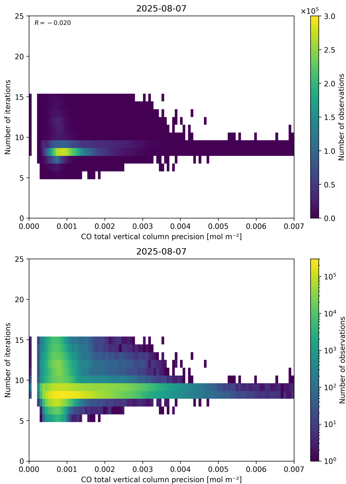
Figure 46: Scatter density plot of “CO total vertical column precision” against “Number of iterations” for 2025-08-06 to 2025-08-08.
