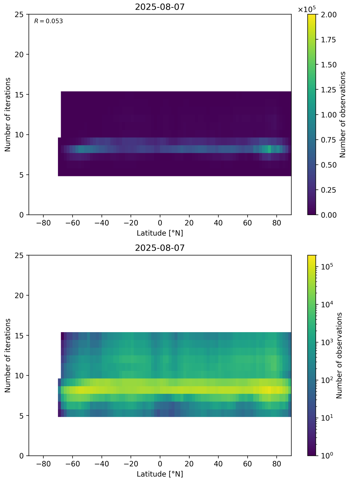
Figure 56: Scatter density plot of “Latitude” against “Number of iterations” for 2025-08-06 to 2025-08-08.
