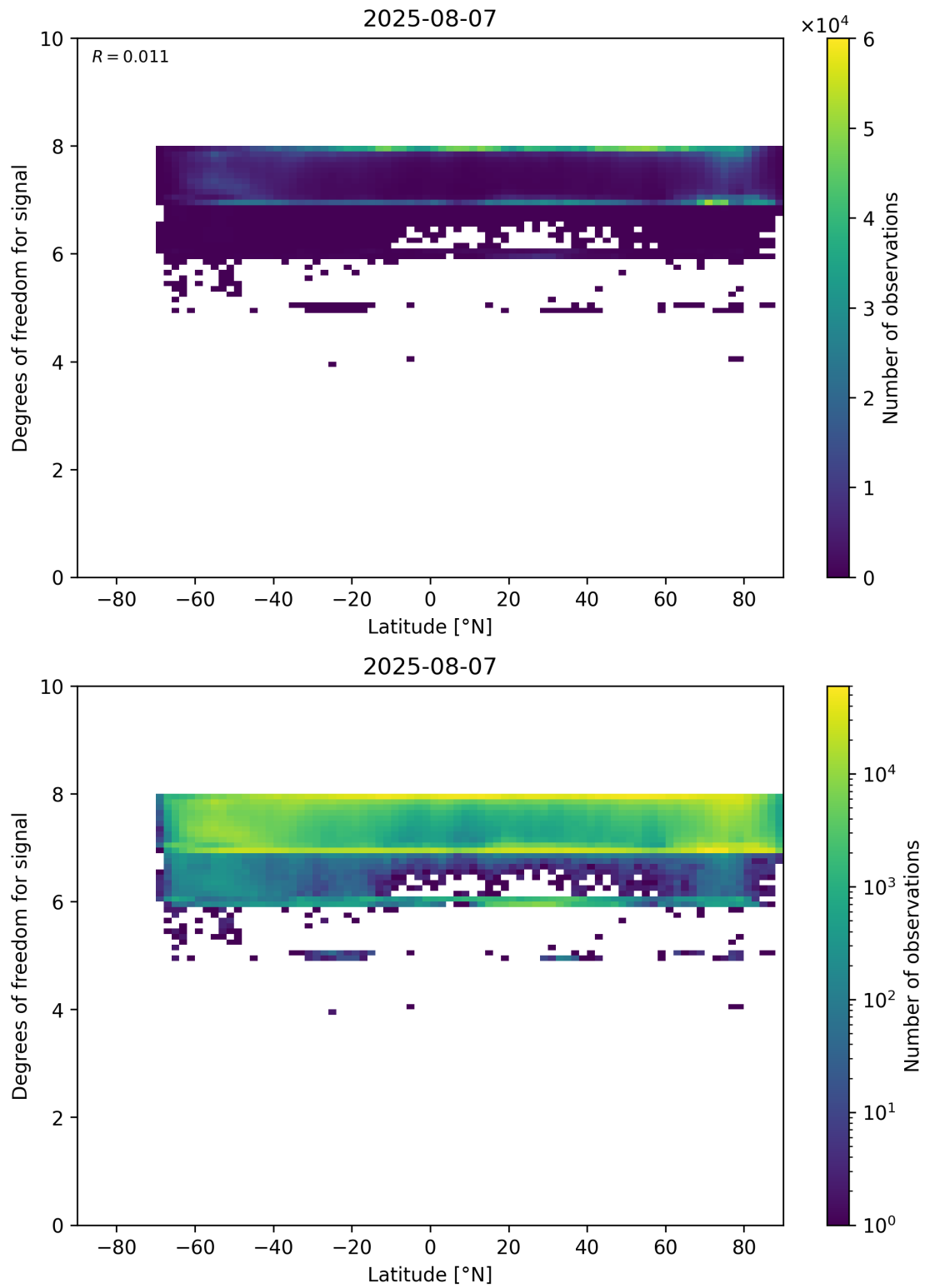
Figure 55: Scatter density plot of “Latitude” against “Degrees of freedom for signal” for 2025-08-06 to 2025-08-08.
