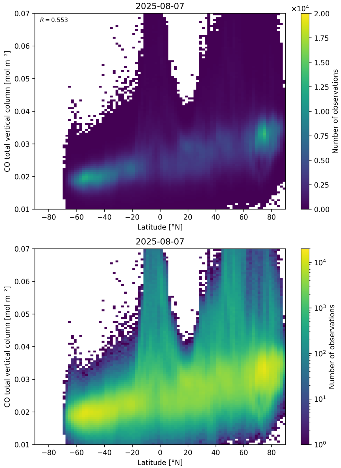
Figure 51: Scatter density plot of “Latitude” against “CO total vertical column” for 2025-08-06 to 2025-08-08.
