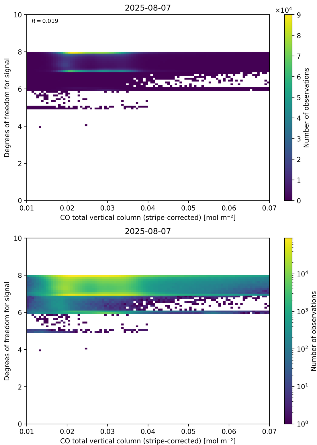
Figure 38: Scatter density plot of “CO total vertical column (stripe-corrected)” against “Degrees of freedom for signal” for 2025-08-06 to 2025-08-08.
