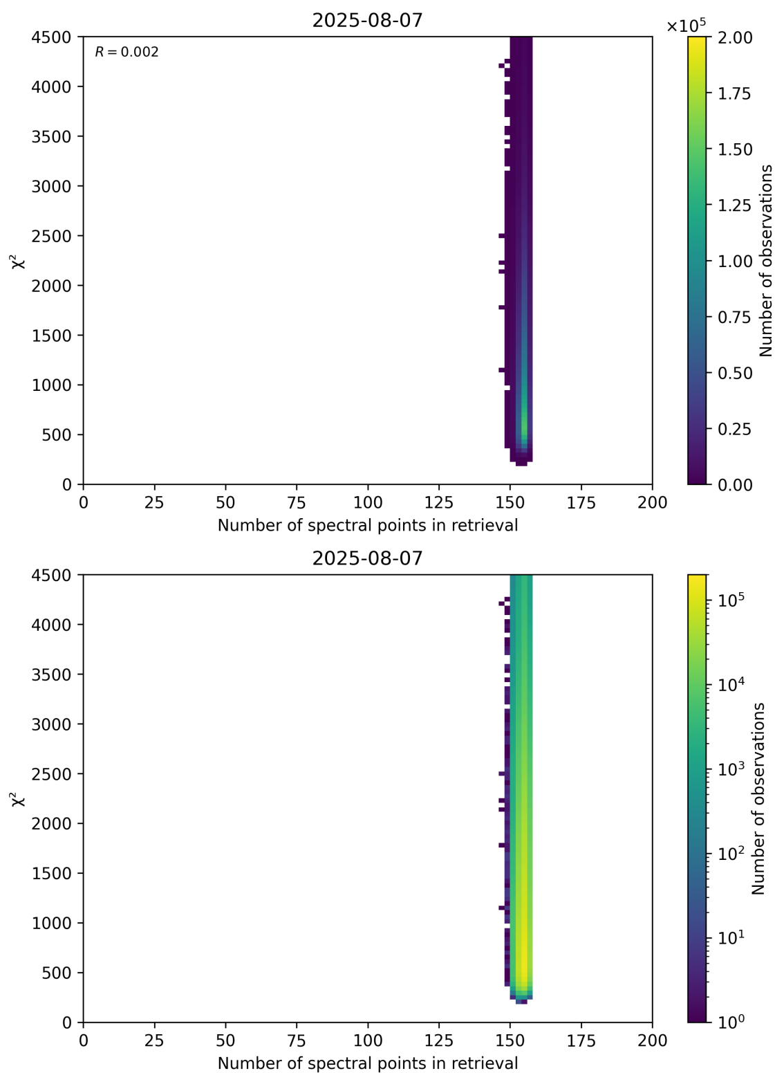
Figure 58: Scatter density plot of “Number of spectral points in retrieval” against “ \chi^2 ” for 2025-08-06 to 2025-08-08.
