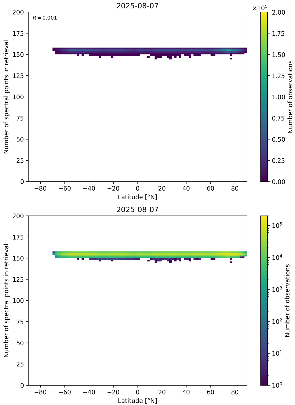
Figure 57: Scatter density plot of “Latitude” against “Number of spectral points in retrieval” for 2025-08-06 to 2025-08-08.
