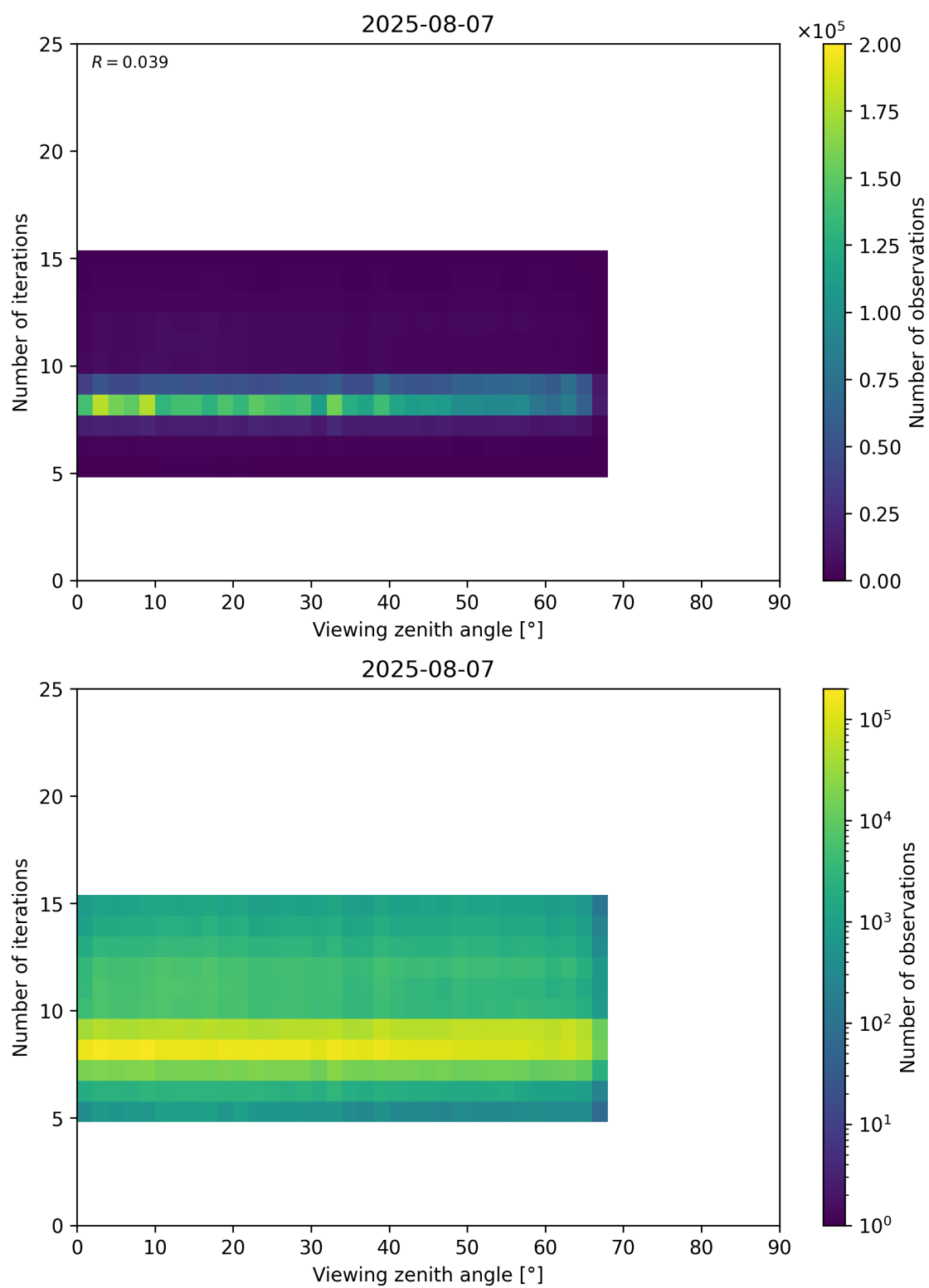
Figure 75: Scatter density plot of “Viewing zenith angle” against “Number of iterations” for 2025-08-06 to 2025-08-08.
