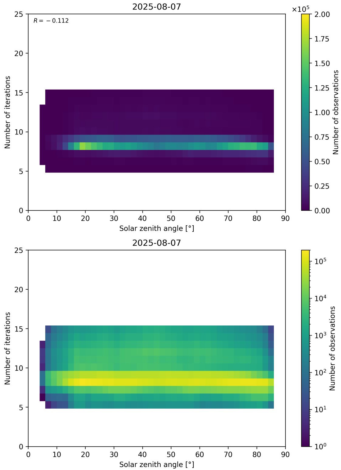
Figure 67: Scatter density plot of “Solar zenith angle” against “Number of iterations” for 2025-08-06 to 2025-08-08.
