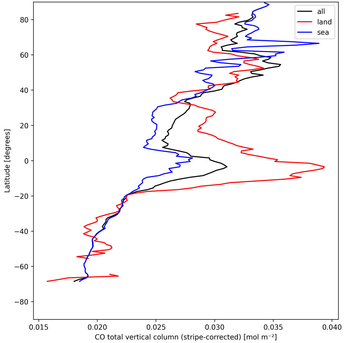
Figure 11: Zonal average of “CO total vertical column (stripe-corrected)” for 2025-08-06 to 2025-08-08.
