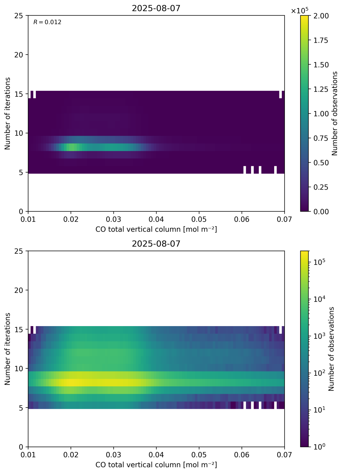
Figure 42: Scatter density plot of “CO total vertical column” against “Number of iterations” for 2025-08-06 to 2025-08-08.
