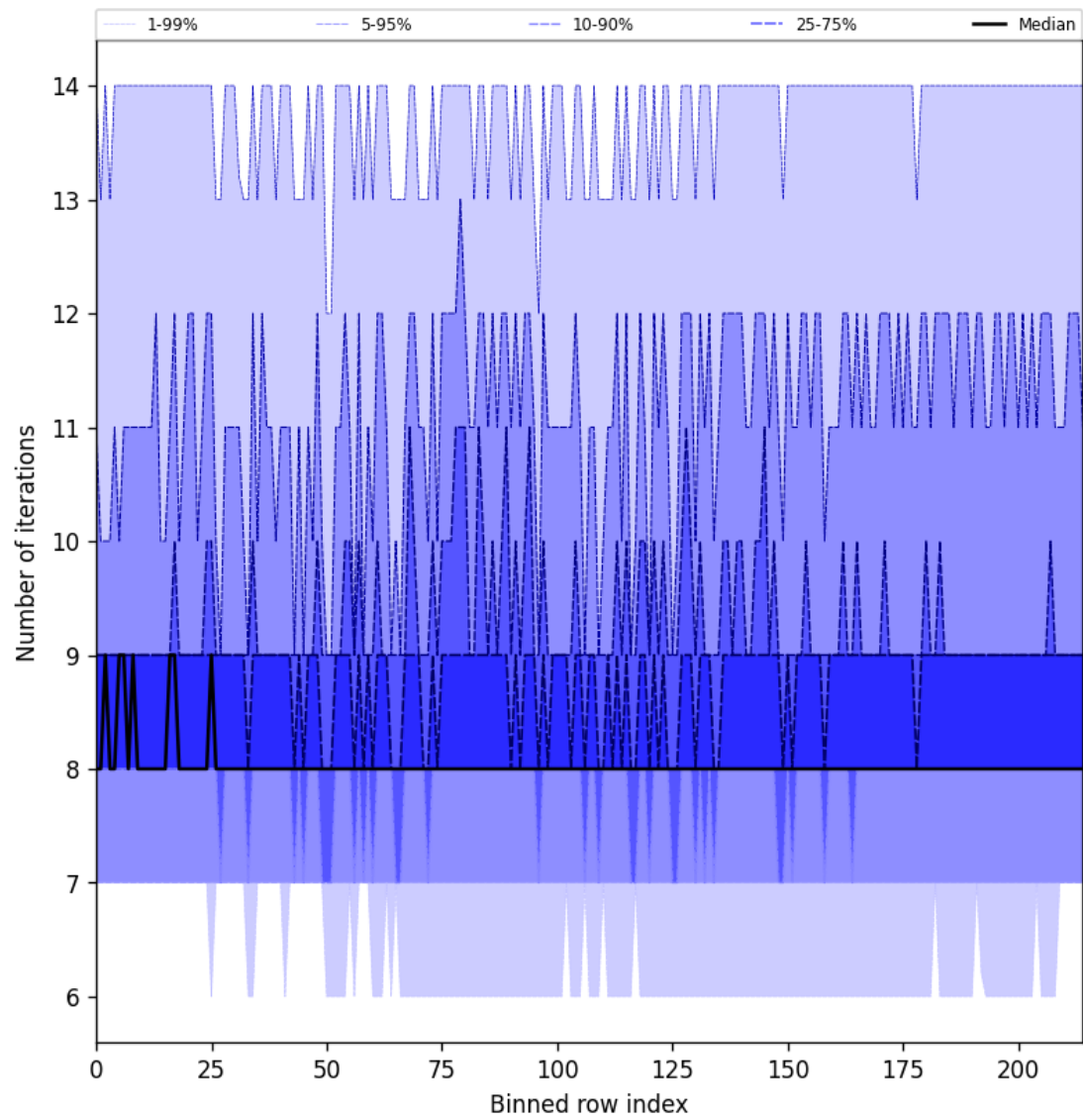
Figure 32: Along track statistics of “Number of iterations” for 2025-08-06 to 2025-08-08
