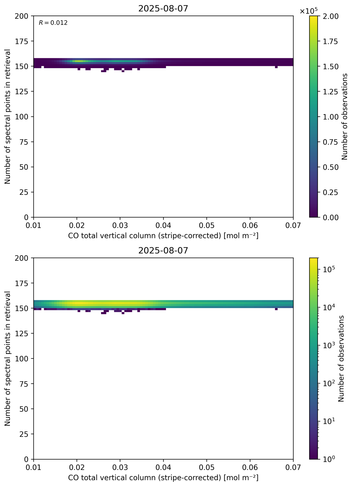
Figure 40: Scatter density plot of “CO total vertical column (stripe-corrected)” against “Number of spectral points in retrieval” for 2025-08-06 to 2025-08-08.
