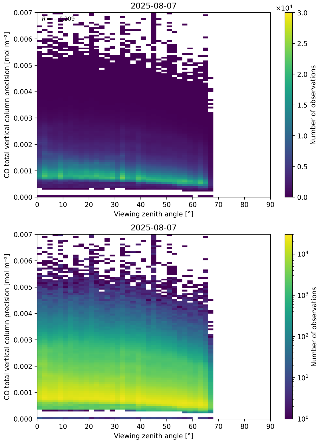
Figure 71: Scatter density plot of “Viewing zenith angle” against “CO total vertical column precision” for 2025-08-06 to 2025-08-08.
