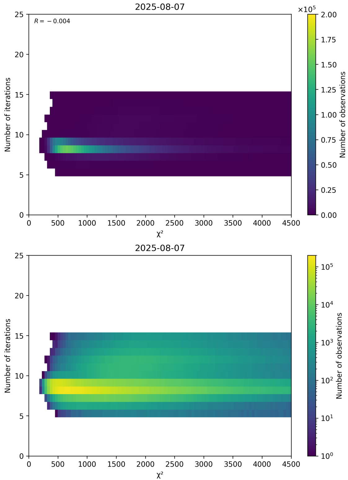
Figure 49: Scatter density plot of “ \chi^2 ” against “Number of iterations” for 2025-08-06 to 2025-08-08.
