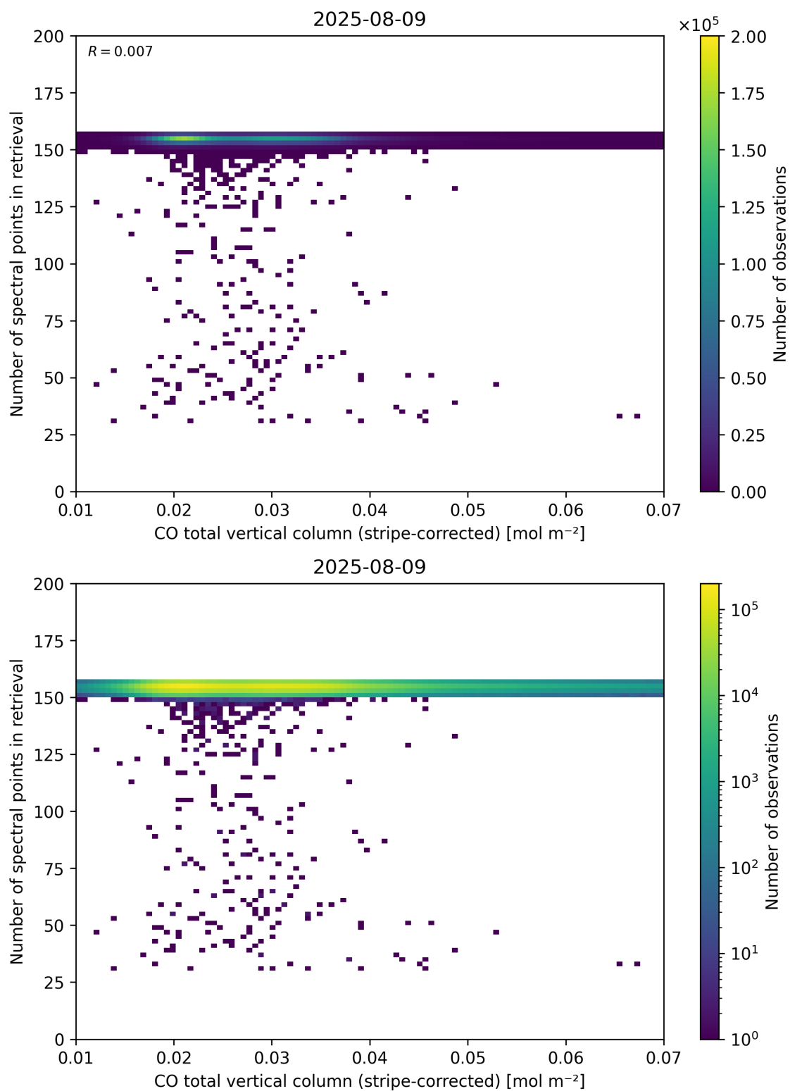
Figure 40: Scatter density plot of “CO total vertical column (stripe-corrected)” against “Number of spectral points in retrieval” for 2025-08-09 to 2025-08-10.
