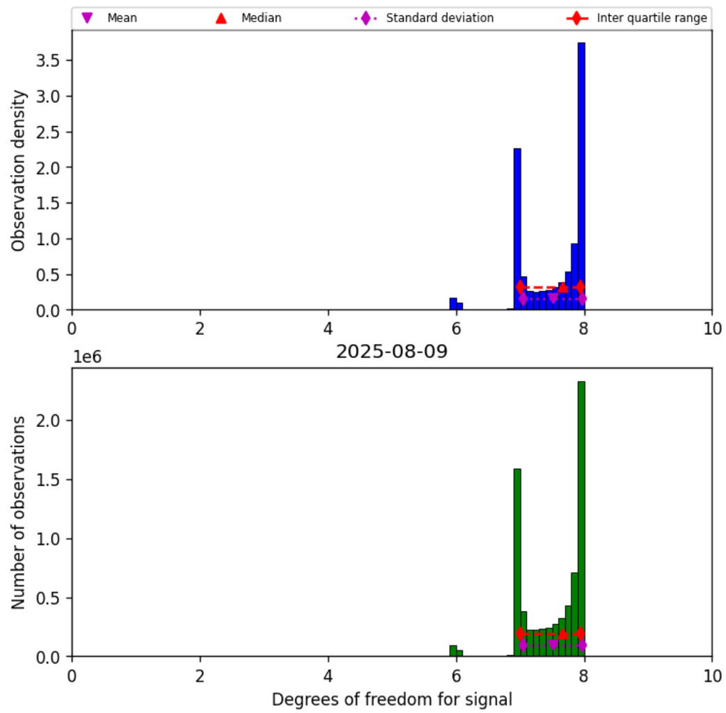
Figure 23: Histogram of “Degrees of freedom for signal” for 2025-08-09 to 2025-08-10
