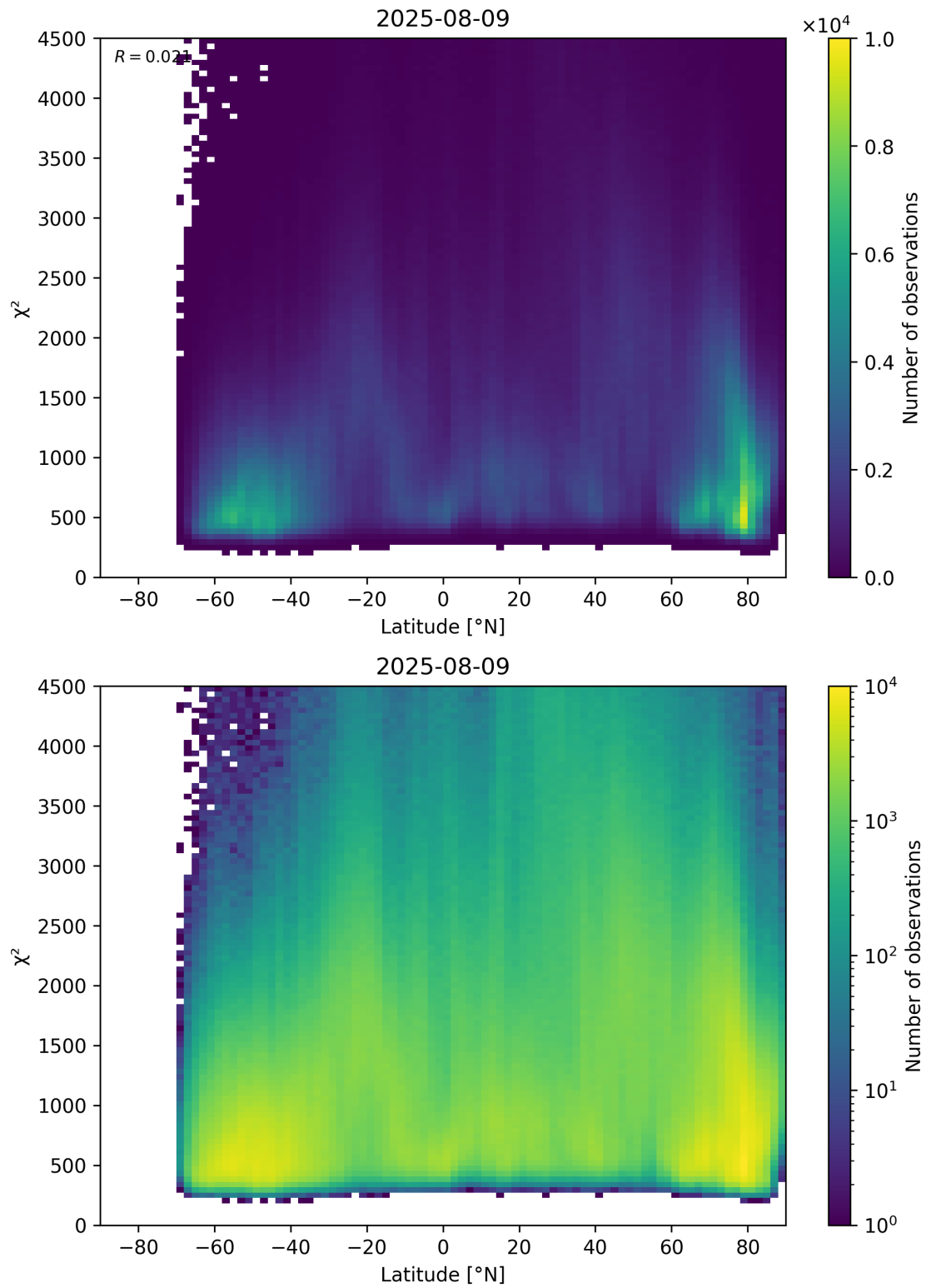
Figure 54: Scatter density plot of “Latitude” against “ \chi^2 ” for 2025-08-09 to 2025-08-10.
