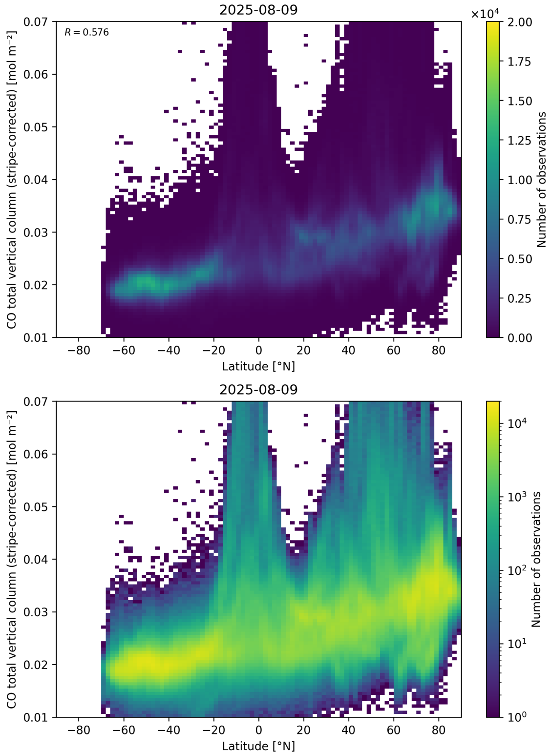
Figure 52: Scatter density plot of “Latitude” against “CO total vertical column (stripe-corrected)” for 2025-08-09 to 2025-08-10.
