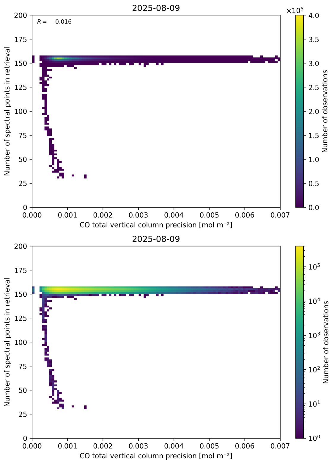
Figure 47: Scatter density plot of “CO total vertical column precision” against “Number of spectral points in retrieval” for 2025-08-09 to 2025-08-10.
