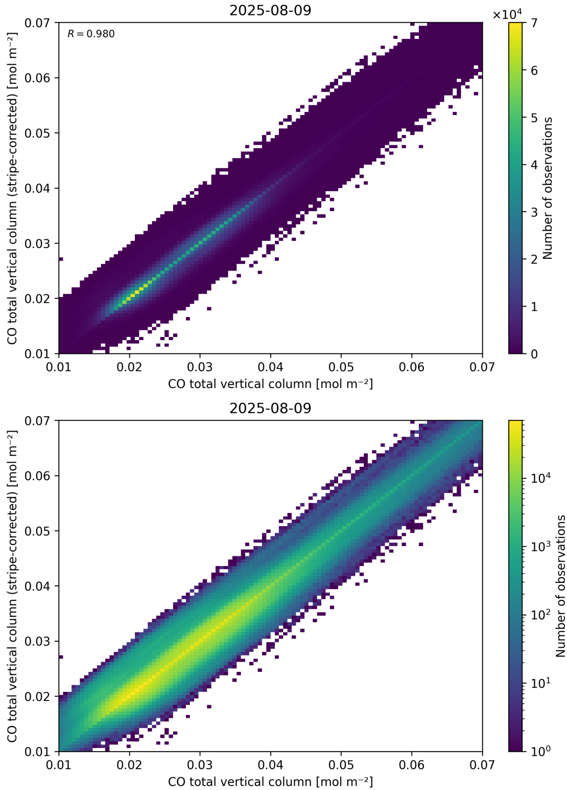
Figure 33: Scatter density plot of “CO total vertical column” against “CO total vertical column (stripe-corrected)” for 2025-08-09 to 2025-08-10.
