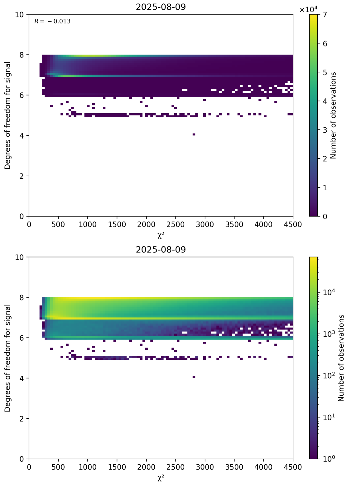
Figure 48: Scatter density plot of “ \chi^2 ” against “Degrees of freedom for signal” for 2025-08-09 to 2025-08-10.
