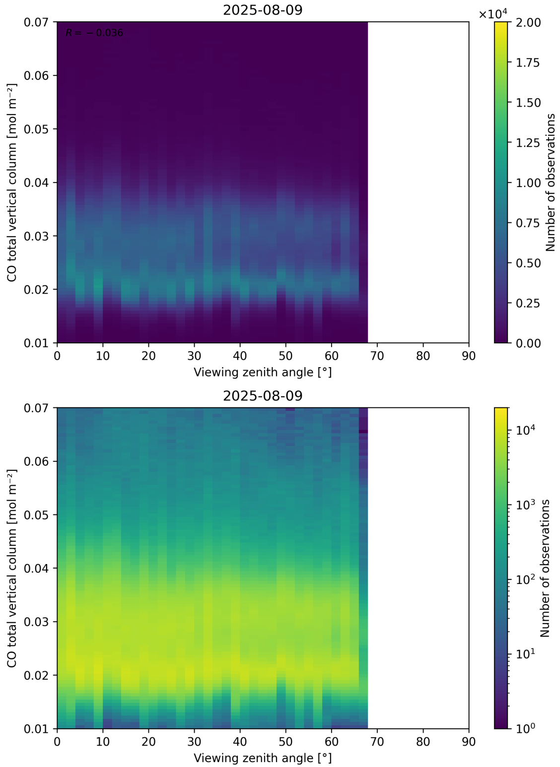
Figure 69: Scatter density plot of “Viewing zenith angle” against “CO total vertical column” for 2025-08-09 to 2025-08-10.
