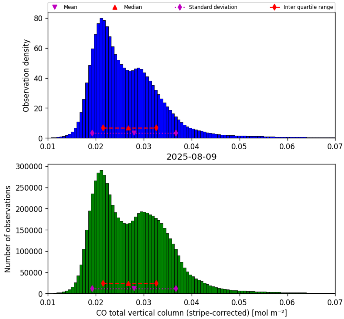
Figure 19: Histogram of “CO total vertical column (stripe-corrected)” for 2025-08-09 to 2025-08-10
