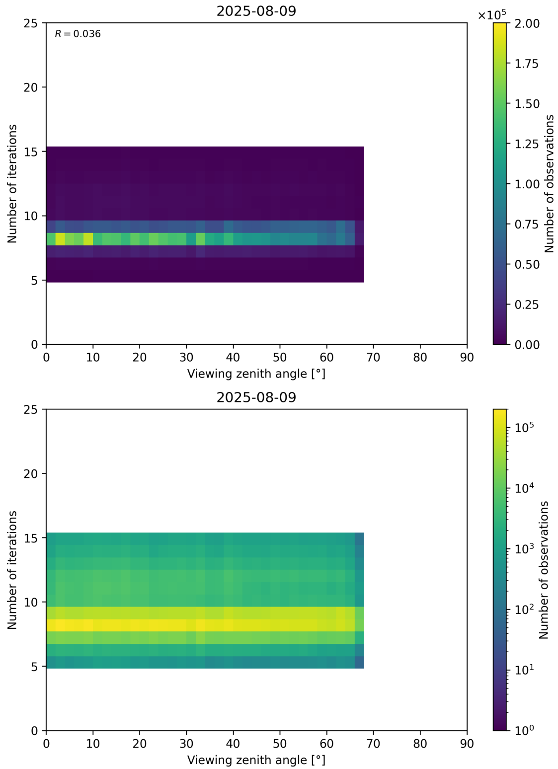
Figure 75: Scatter density plot of “Viewing zenith angle” against “Number of iterations” for 2025-08-09 to 2025-08-10.
