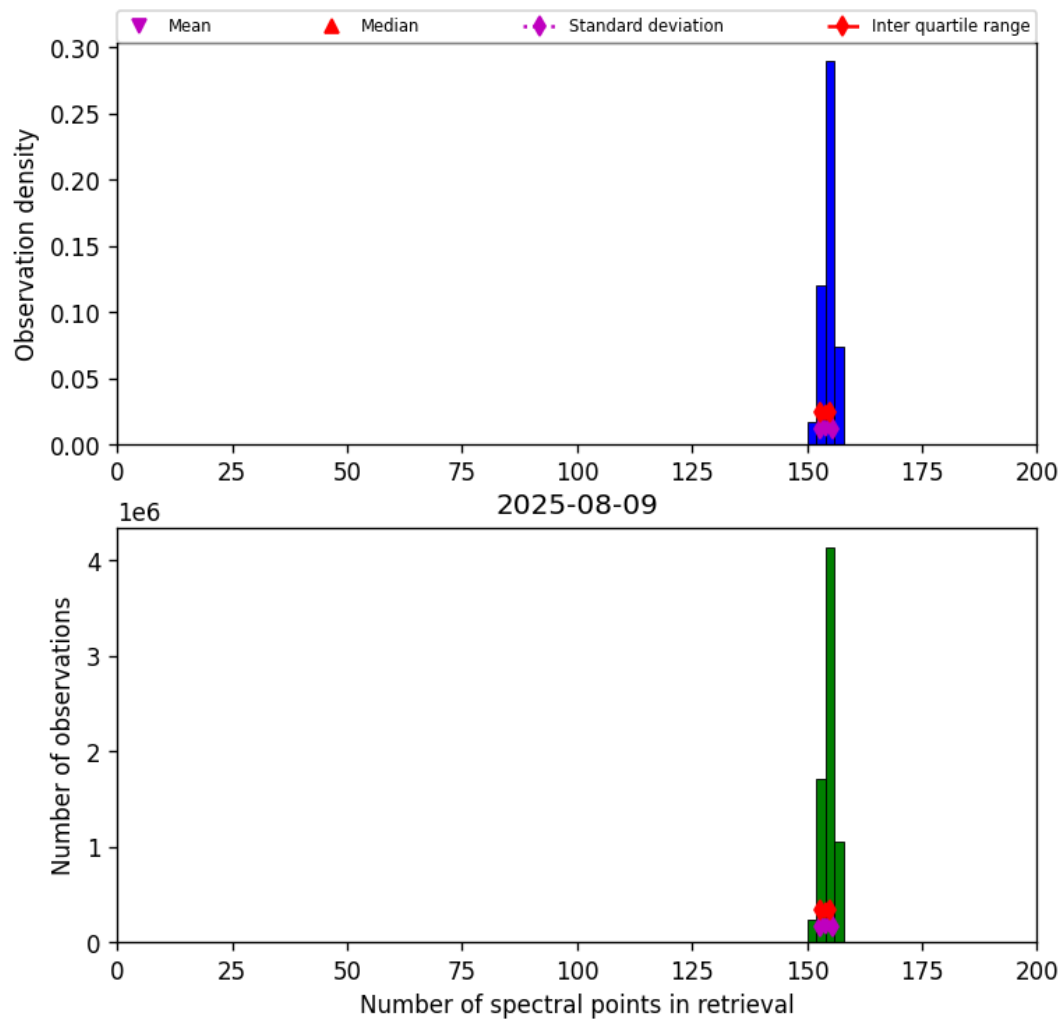
Figure 21: Histogram of “Number of spectral points in retrieval” for 2025-08-09 to 2025-08-10
