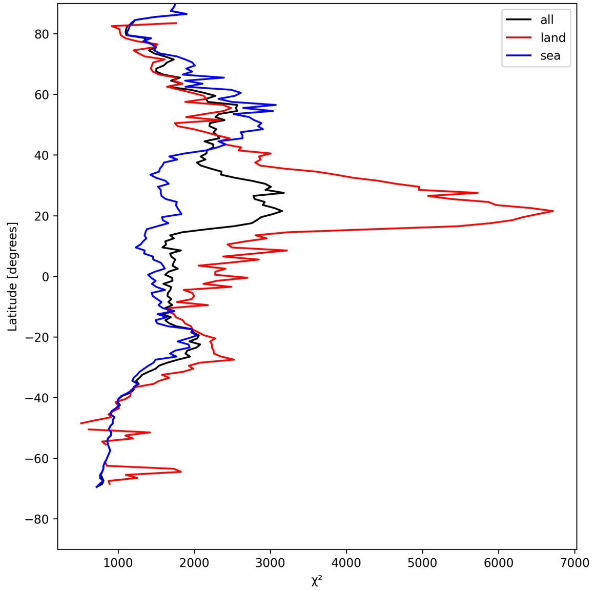
Figure 14: Zonal average of “ \chi^2 ” for 2025-08-09 to 2025-08-10.
