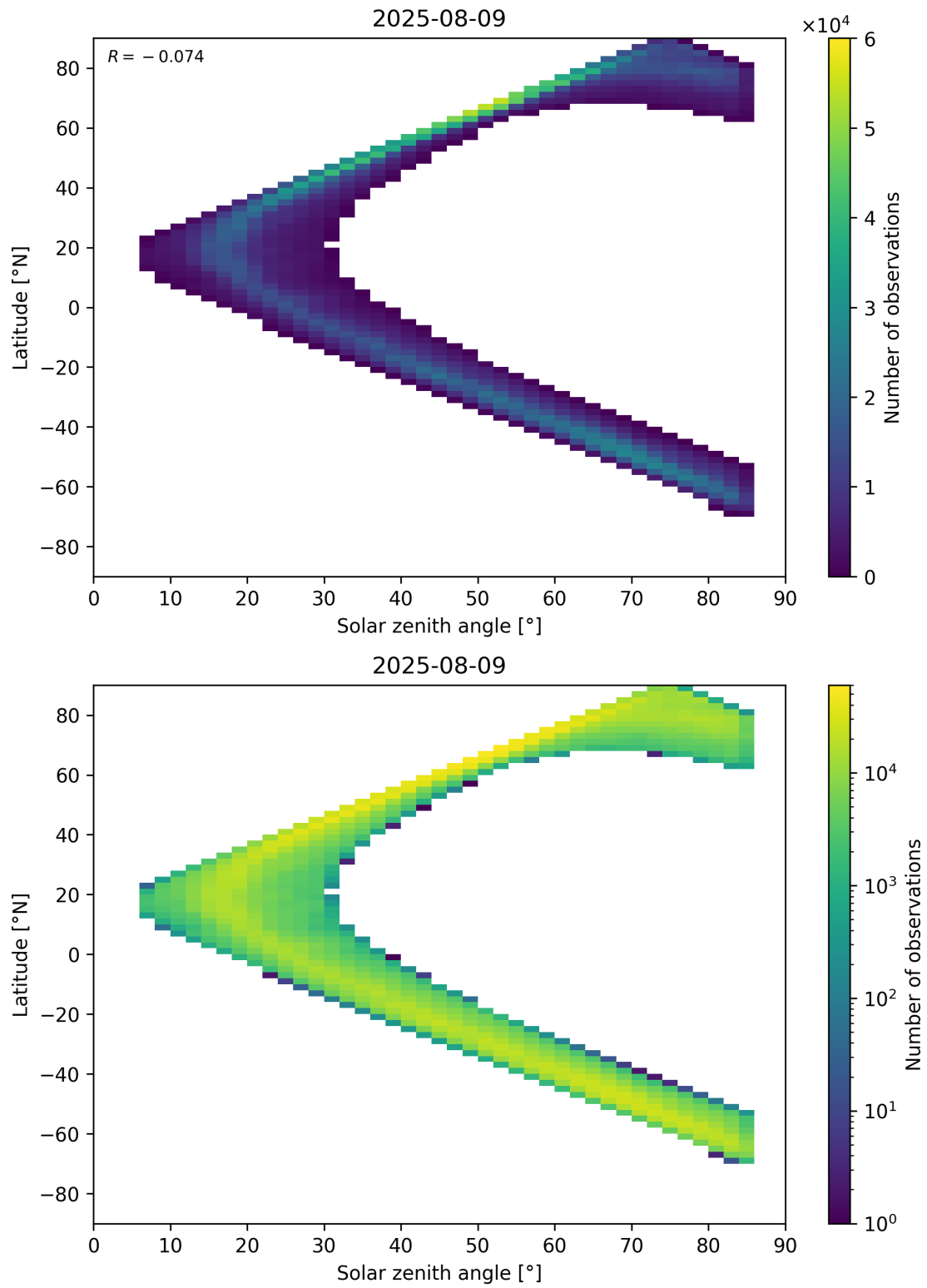
Figure 66: Scatter density plot of “Solar zenith angle” against “Latitude” for 2025-08-09 to 2025-08-10.
