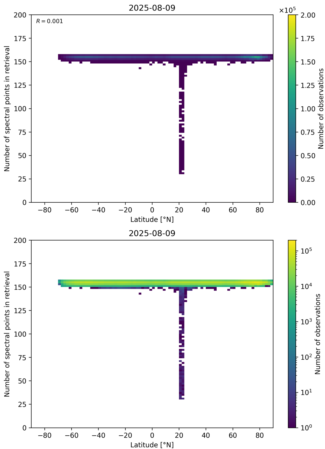
Figure 57: Scatter density plot of “Latitude” against “Number of spectral points in retrieval” for 2025-08-09 to 2025-08-10.
