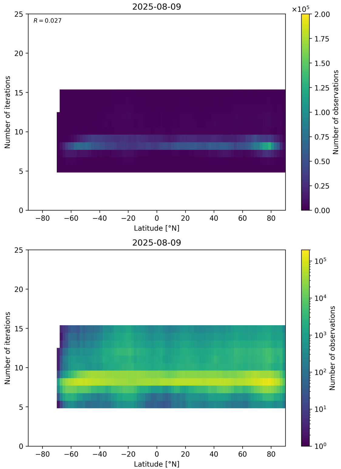
Figure 56: Scatter density plot of “Latitude” against “Number of iterations” for 2025-08-09 to 2025-08-10.
