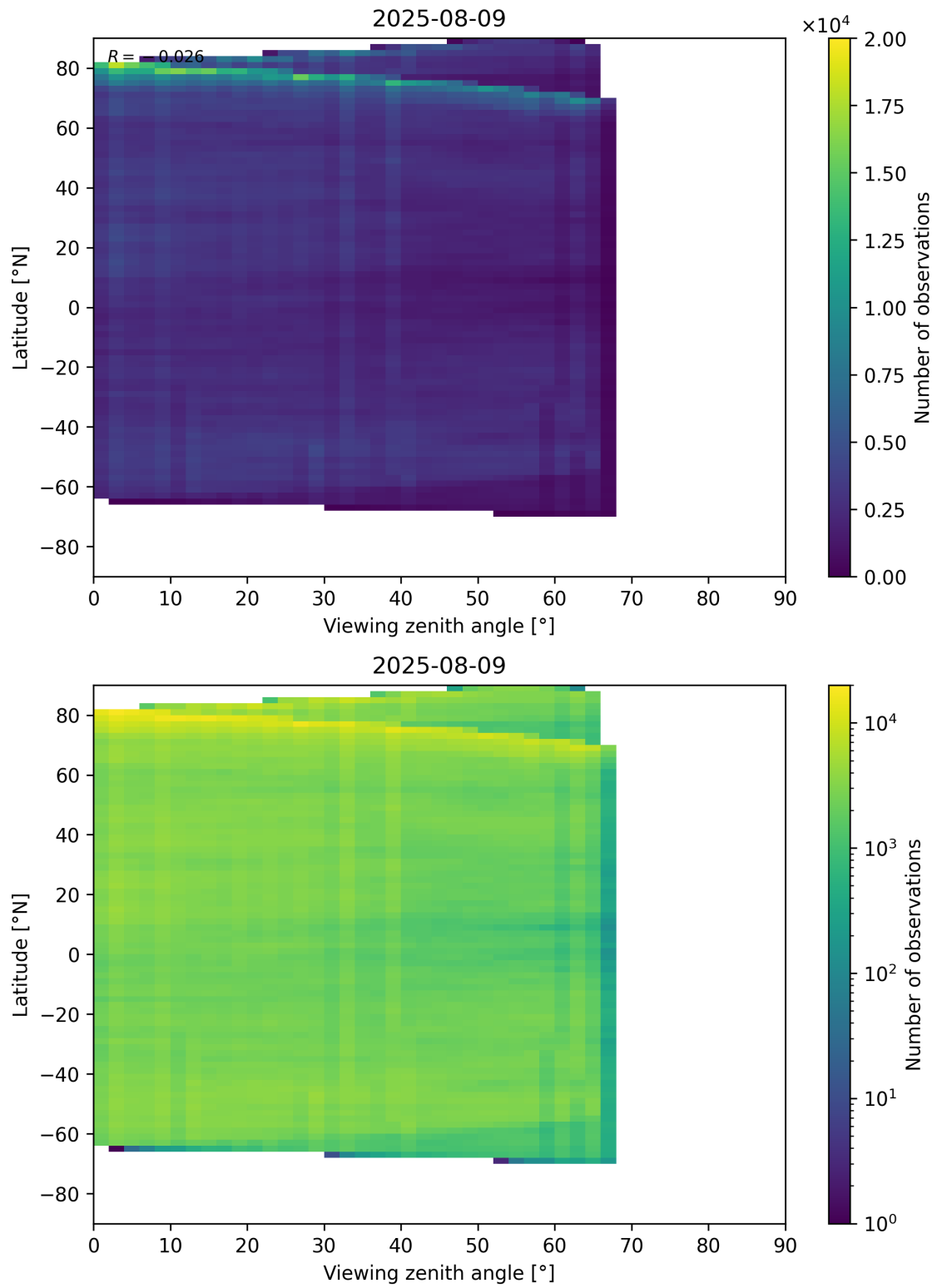
Figure 74: Scatter density plot of “Viewing zenith angle” against “Latitude” for 2025-08-09 to 2025-08-10.
