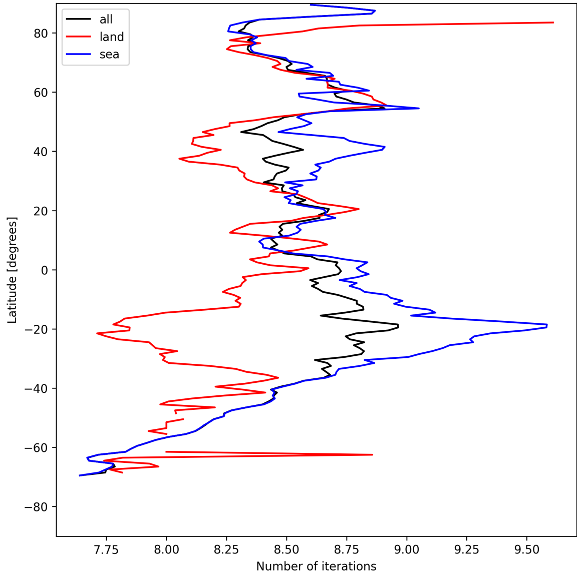
Figure 16: Zonal average of “Number of iterations” for 2025-08-09 to 2025-08-10.
