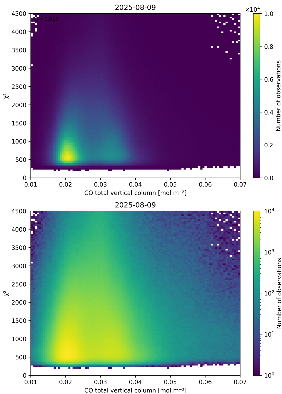
Figure 35: Scatter density plot of “CO total vertical column” against “ \chi^2 ” for 2025-08-09 to 2025-08-10.
