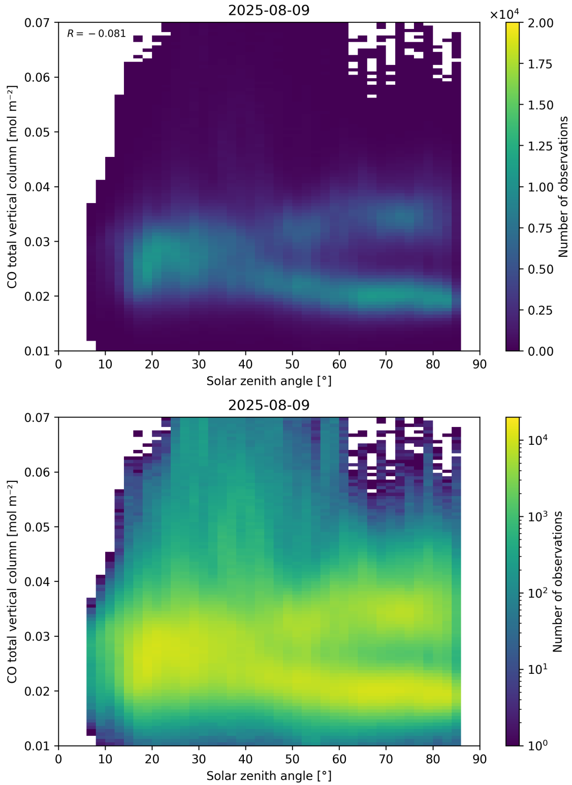
Figure 61: Scatter density plot of “Solar zenith angle” against “CO total vertical column” for 2025-08-09 to 2025-08-10.
