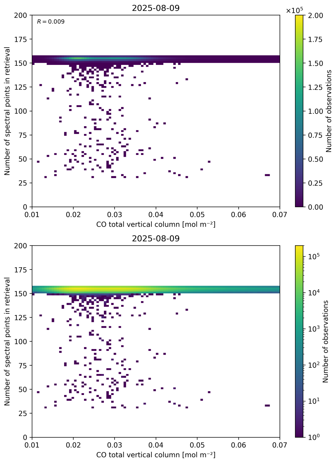
Figure 43: Scatter density plot of “CO total vertical column” against “Number of spectral points in retrieval” for 2025-08-09 to 2025-08-10.
