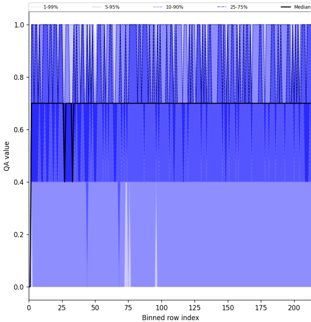
Figure 25: Along track statistics of “QA value” for 2025-08-09 to 2025-08-10
