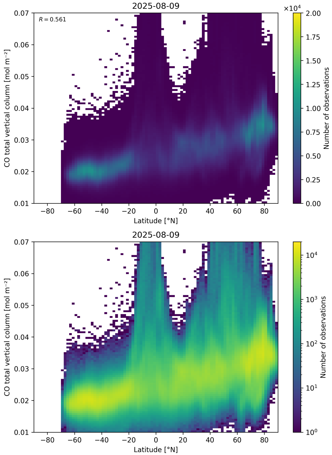
Figure 51: Scatter density plot of “Latitude” against “CO total vertical column” for 2025-08-09 to 2025-08-10.
