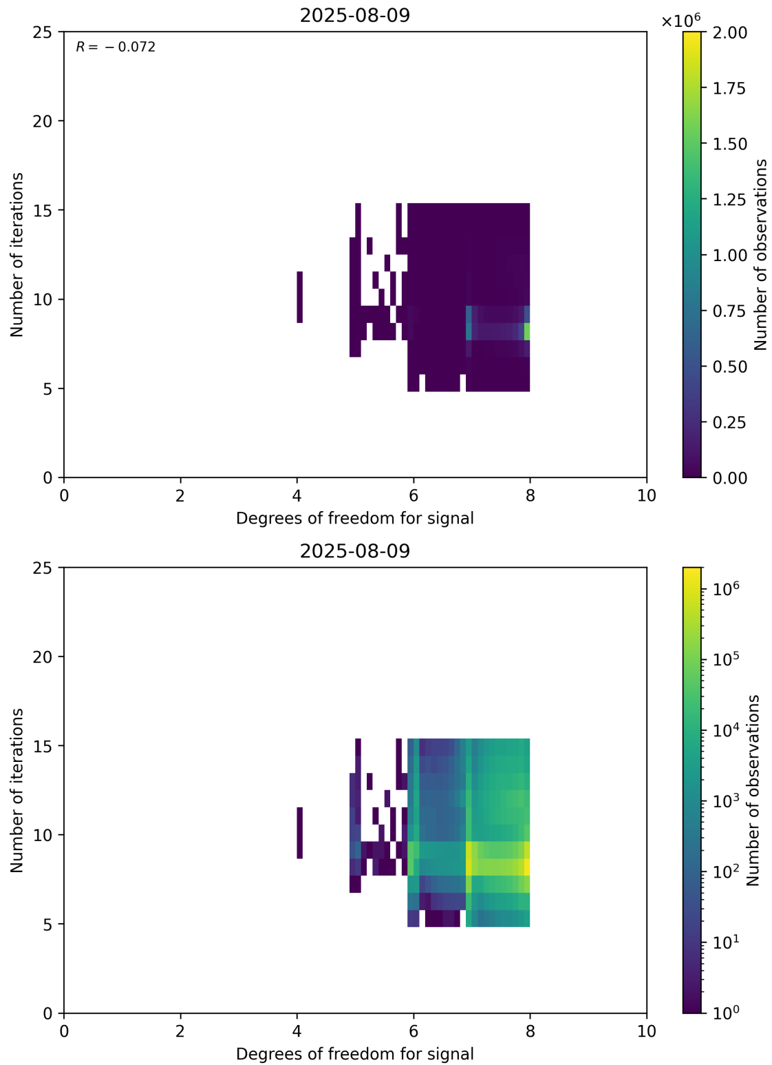
Figure 50: Scatter density plot of “Degrees of freedom for signal” against “Number of iterations” for 2025-08-09 to 2025-08-10.
