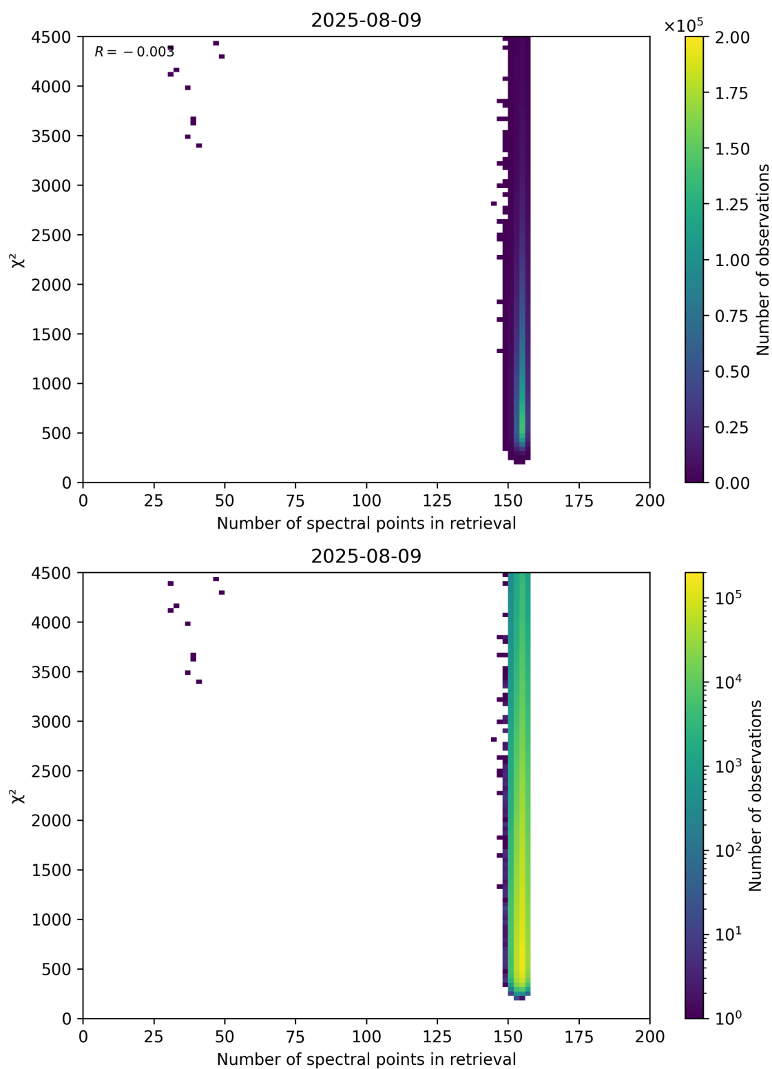
Figure 58: Scatter density plot of “Number of spectral points in retrieval” against “ \chi^2 ” for 2025-08-09 to 2025-08-10.
