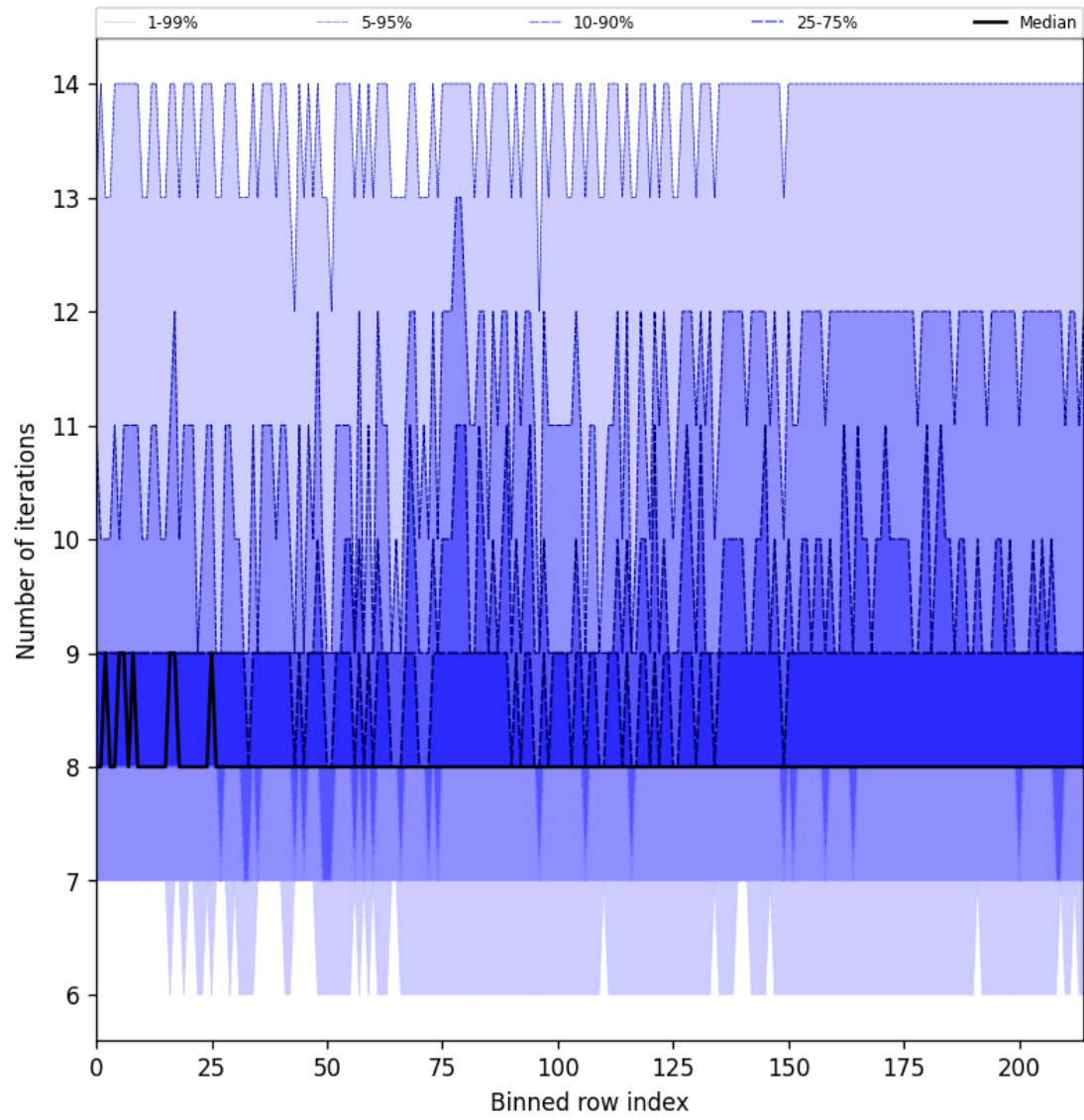
Figure 32: Along track statistics of “Number of iterations” for 2025-08-09 to 2025-08-10
