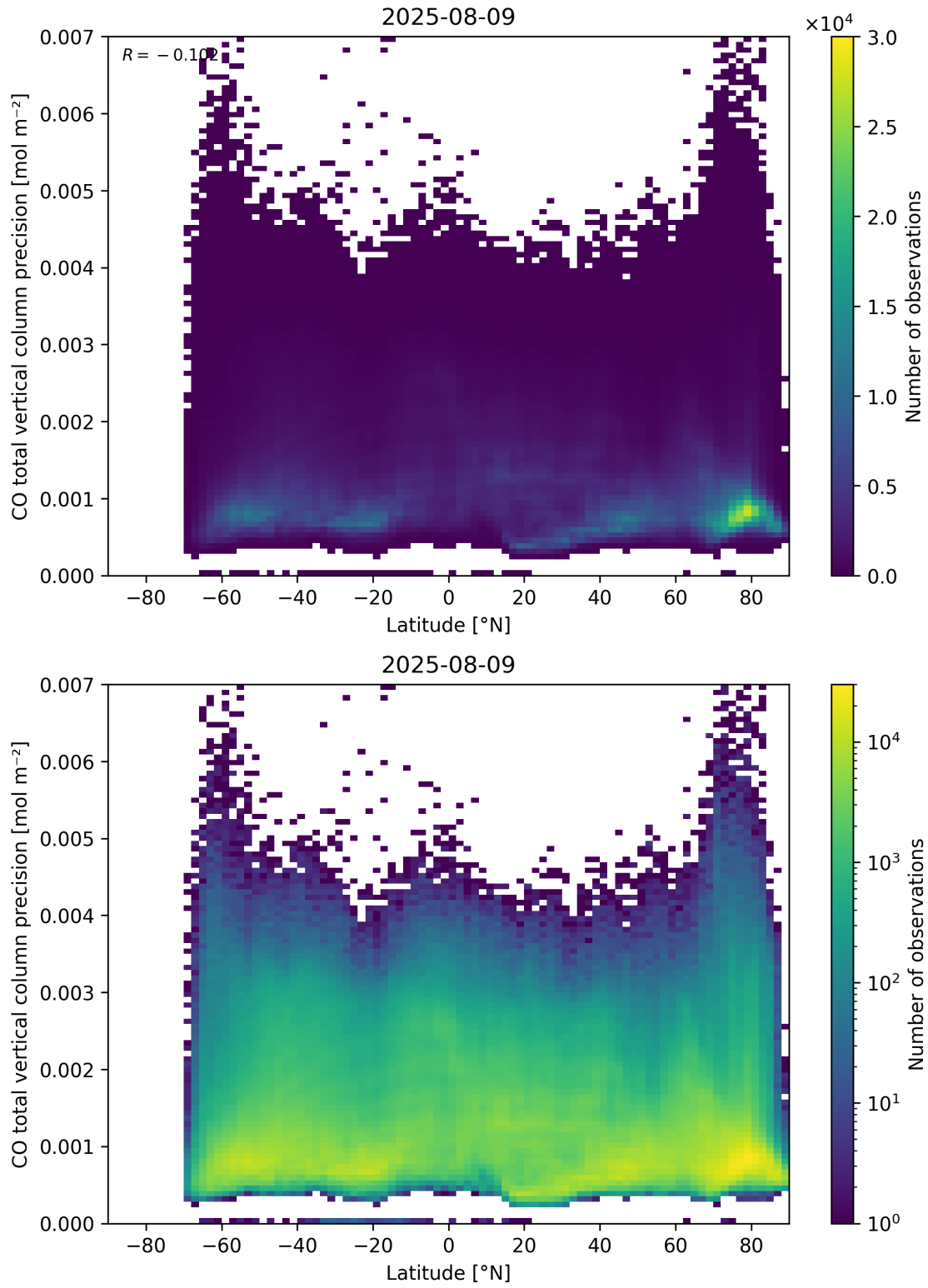
Figure 53: Scatter density plot of “Latitude” against “CO total vertical column precision” for 2025-08-09 to 2025-08-10.
