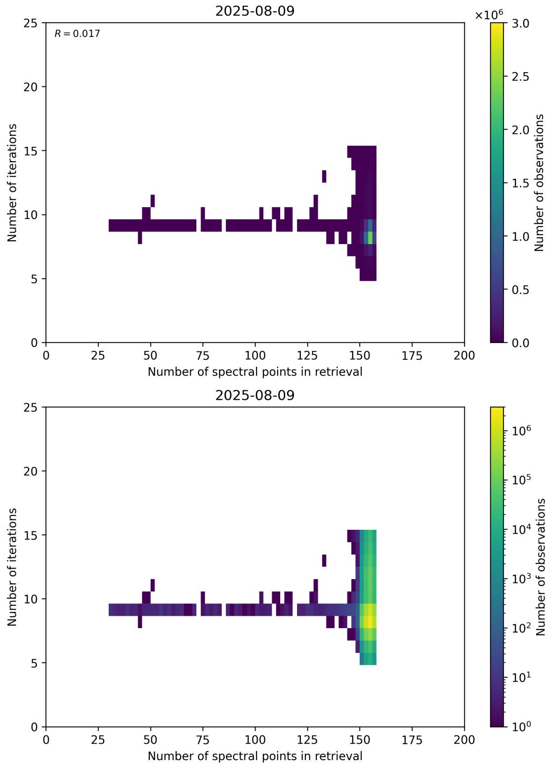
Figure 60: Scatter density plot of “Number of spectral points in retrieval” against “Number of iterations” for 2025-08-09 to 2025-08-10.
