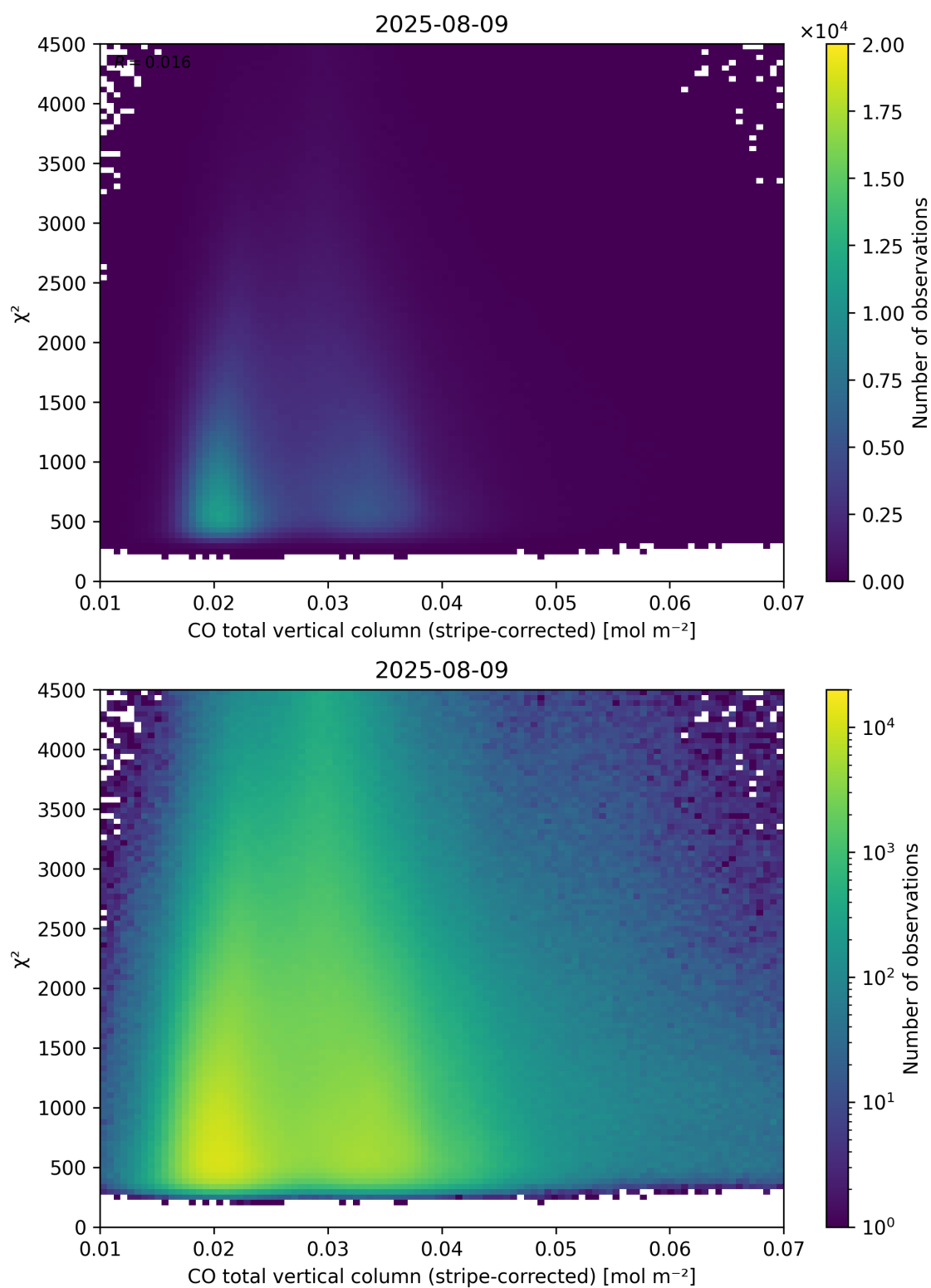
Figure 37: Scatter density plot of “CO total vertical column (stripe-corrected)” against “ \chi^2 ” for 2025-08-09 to 2025-08-10.
