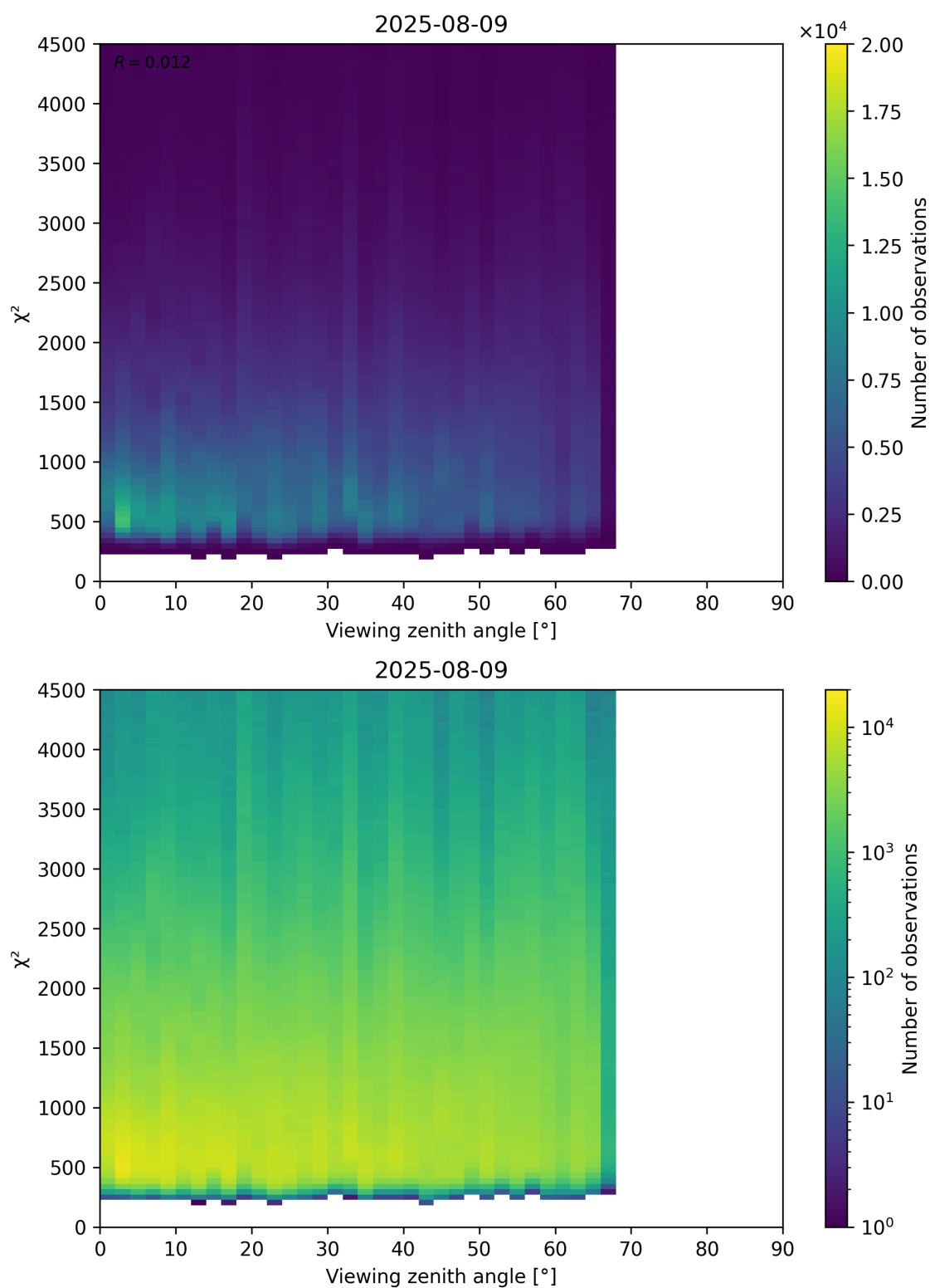
Figure 72: Scatter density plot of “Viewing zenith angle” against “ \chi^2 ” for 2025-08-09 to 2025-08-10.
