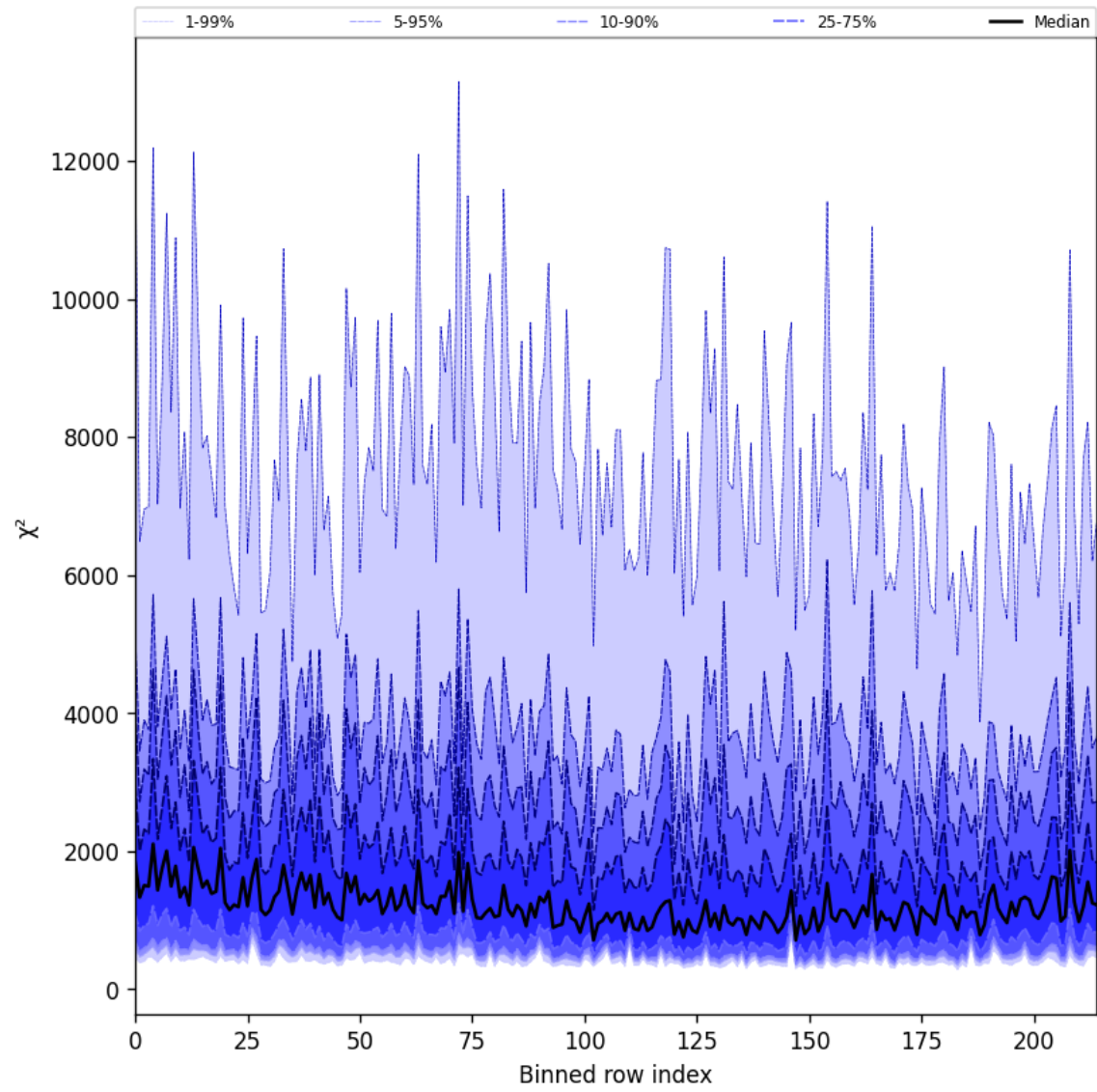
Figure 30: Along track statistics of “ \chi^2 ” for 2025-08-09 to 2025-08-10
