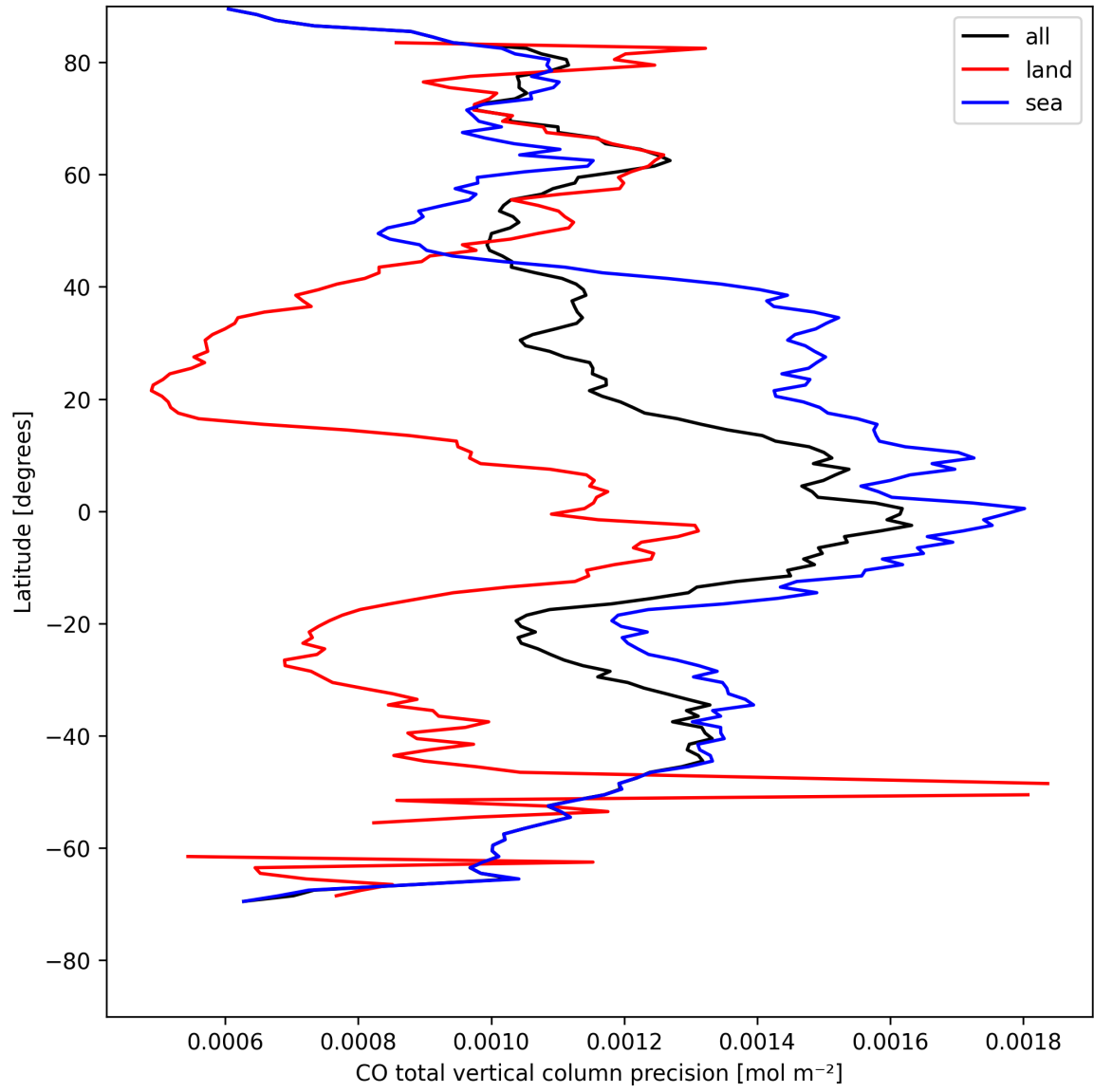
Figure 12: Zonal average of “CO total vertical column precision” for 2025-08-09 to 2025-08-10.
