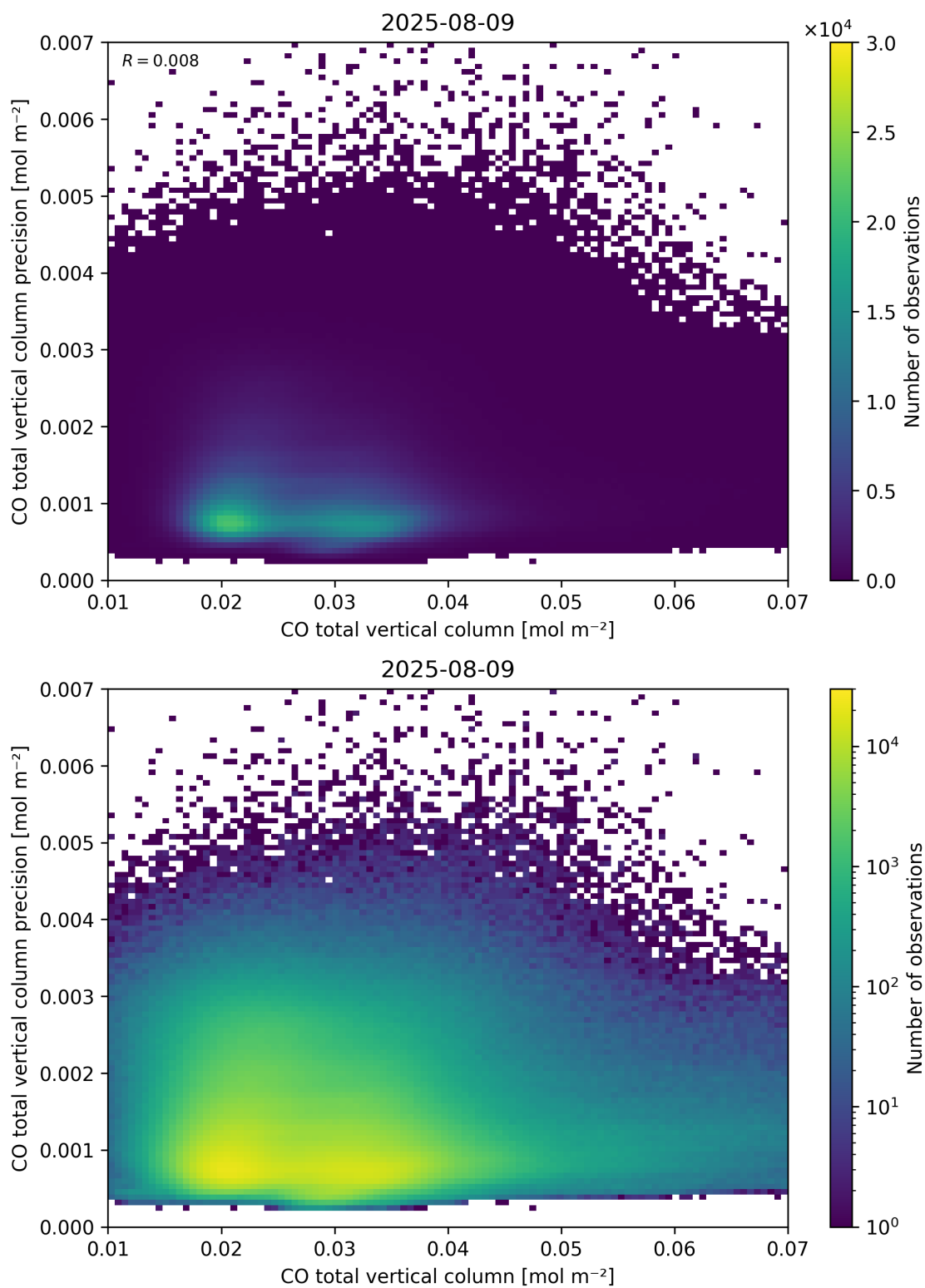
Figure 34: Scatter density plot of “CO total vertical column” against “CO total vertical column precision” for 2025-08-09 to 2025-08-10.
