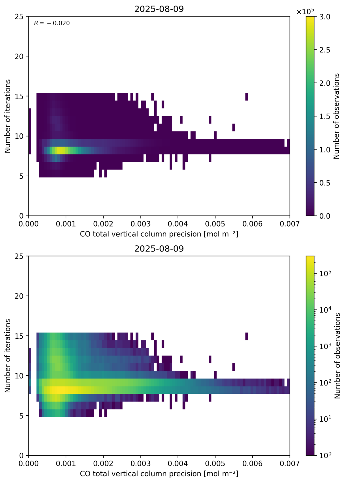
Figure 46: Scatter density plot of “CO total vertical column precision” against “Number of iterations” for 2025-08-09 to 2025-08-10.
