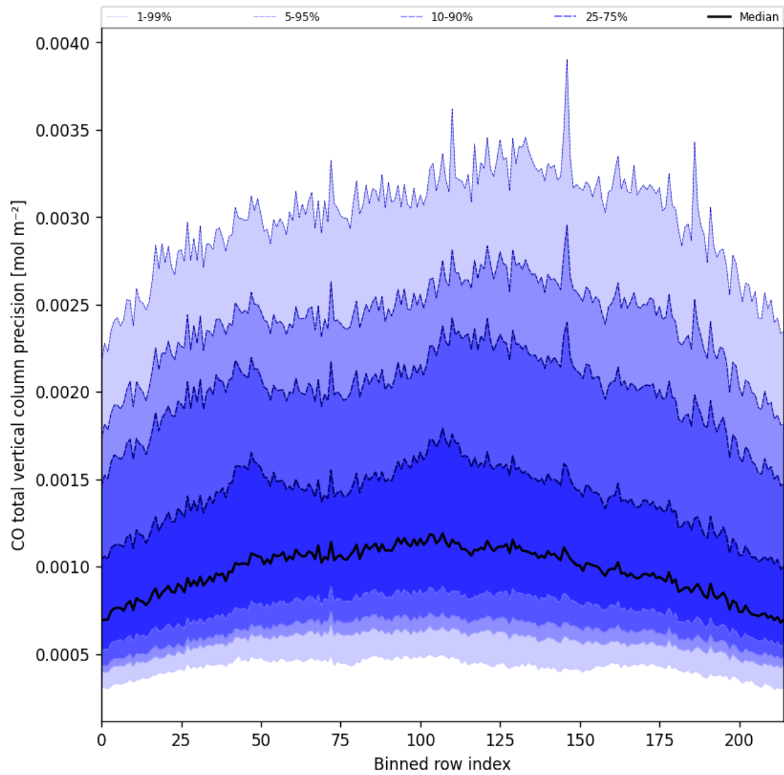
Figure 28: Along track statistics of “CO total vertical column precision” for 2025-08-09 to 2025-08-10
