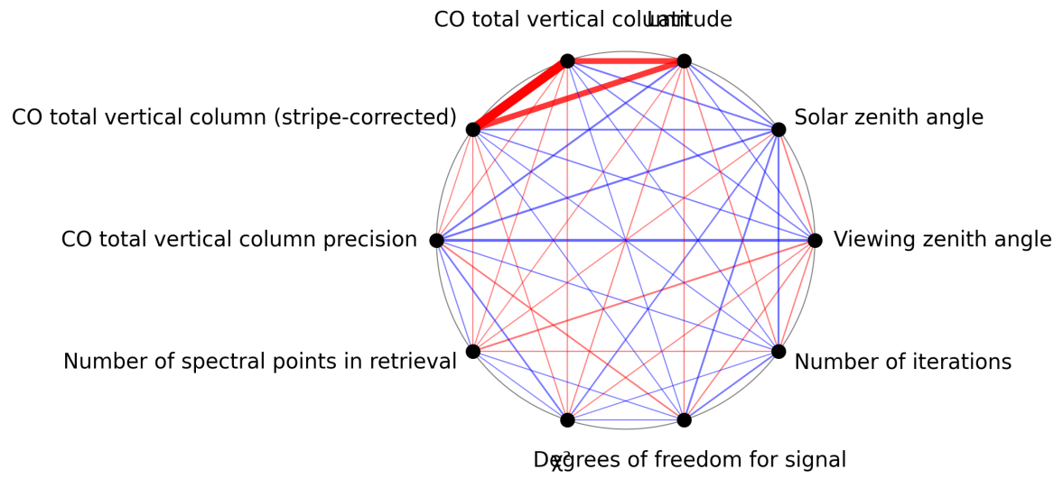
Figure 1: Map of correlation graph for 2025-08-09 to 2025-08-10.
