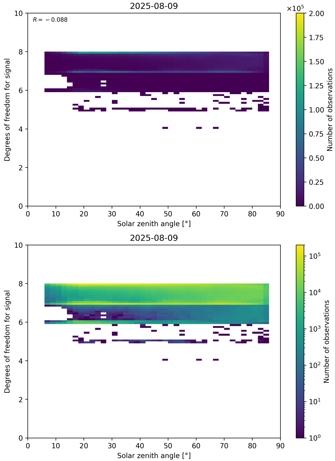
Figure 65: Scatter density plot of “Solar zenith angle” against “Degrees of freedom for signal” for 2025-08-09 to 2025-08-10.
