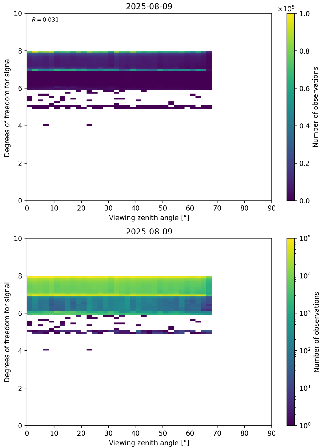
Figure 73: Scatter density plot of “Viewing zenith angle” against “Degrees of freedom for signal” for 2025-08-09 to 2025-08-10.
