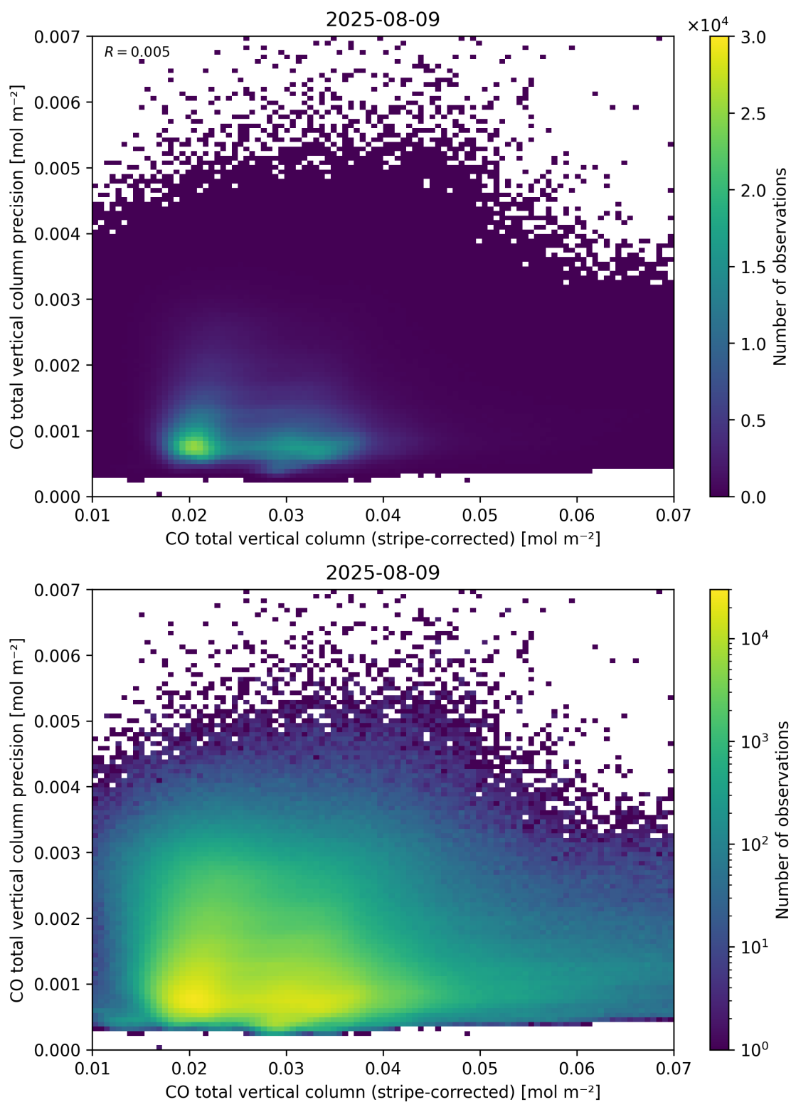
Figure 36: Scatter density plot of “CO total vertical column (stripe-corrected)” against “CO total vertical column precision” for 2025-08-09 to 2025-08-10.
