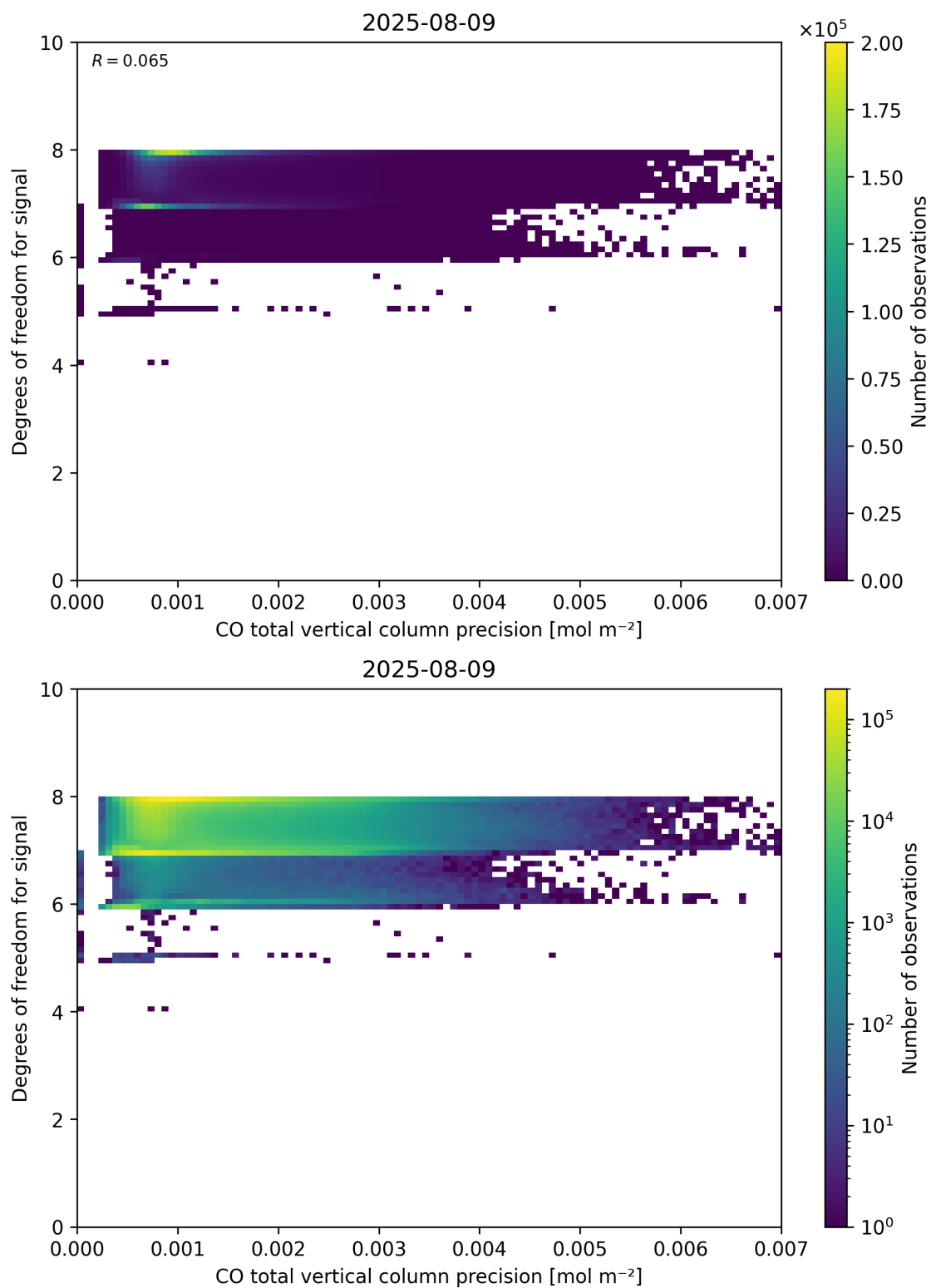
Figure 45: Scatter density plot of “CO total vertical column precision” against “Degrees of freedom for signal” for 2025-08-09 to 2025-08-10.
