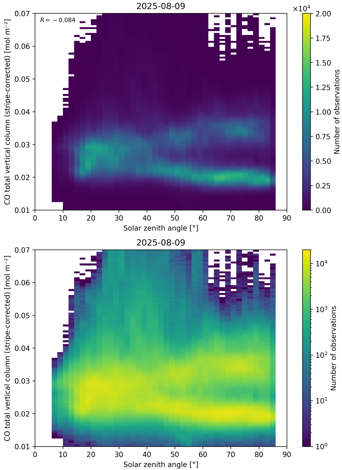
Figure 62: Scatter density plot of “Solar zenith angle” against “CO total vertical column (stripe-corrected)” for 2025-08-09 to 2025-08-10.
