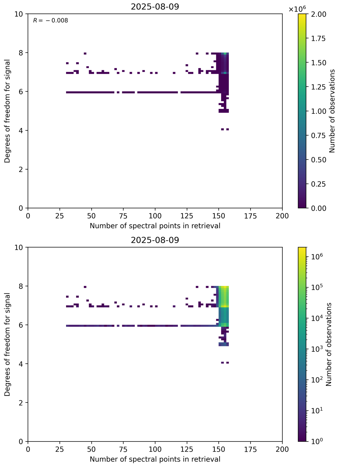
Figure 59: Scatter density plot of “Number of spectral points in retrieval” against “Degrees of freedom for signal” for 2025-08-09 to 2025-08-10.
