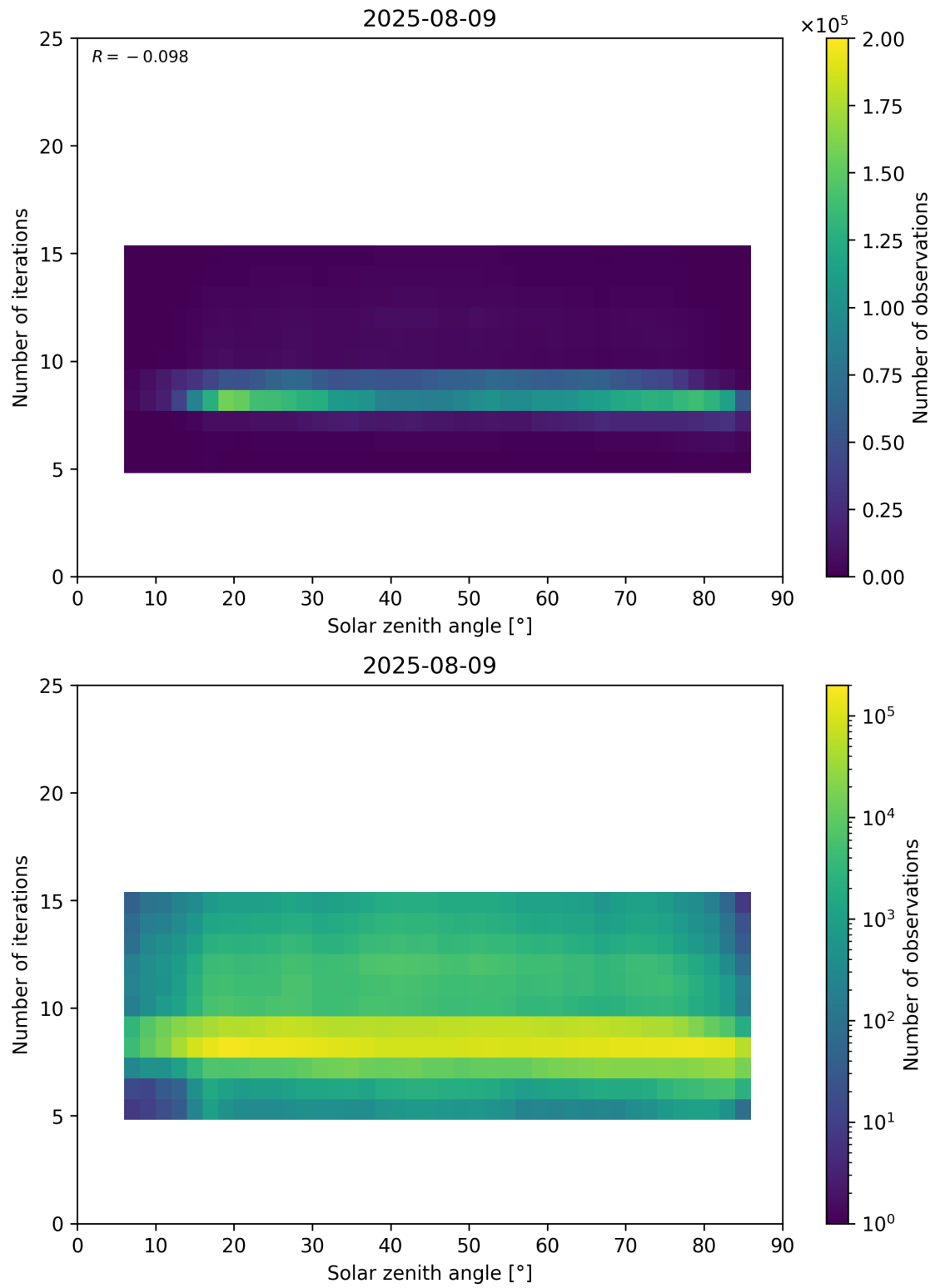
Figure 67: Scatter density plot of “Solar zenith angle” against “Number of iterations” for 2025-08-09 to 2025-08-10.
