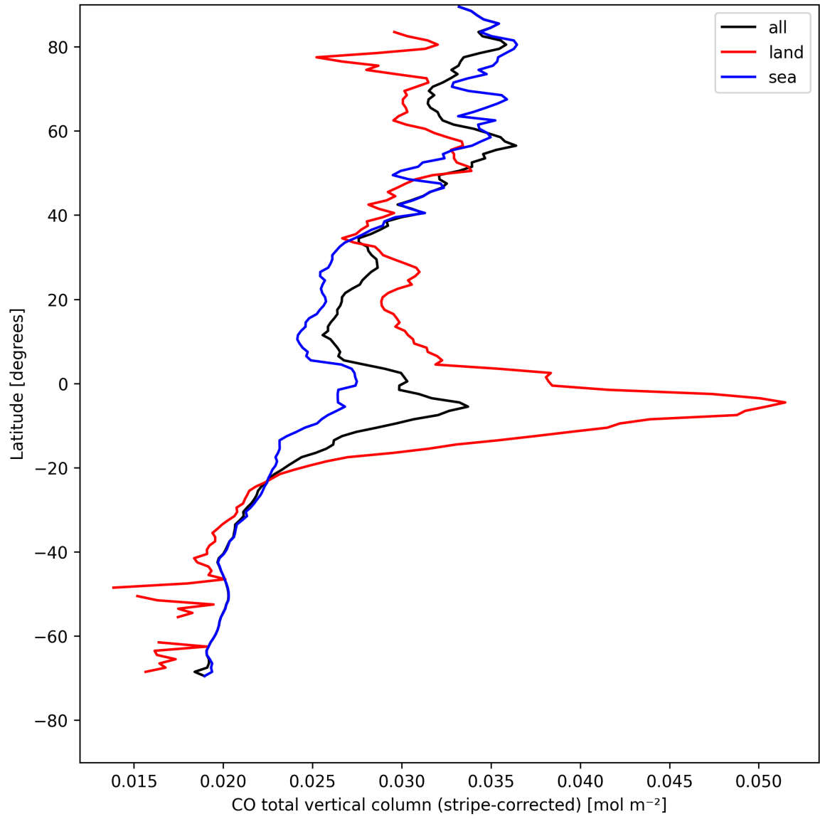
Figure 11: Zonal average of “CO total vertical column (stripe-corrected)” for 2025-08-09 to 2025-08-10.
