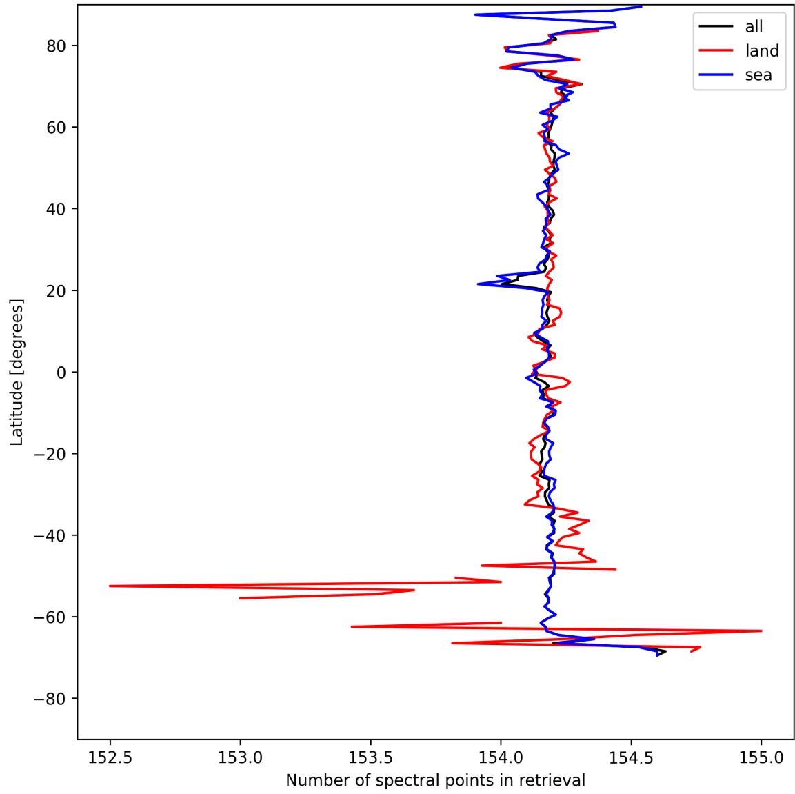
Figure 13: Zonal average of “Number of spectral points in retrieval” for 2025-08-09 to 2025-08-10.
