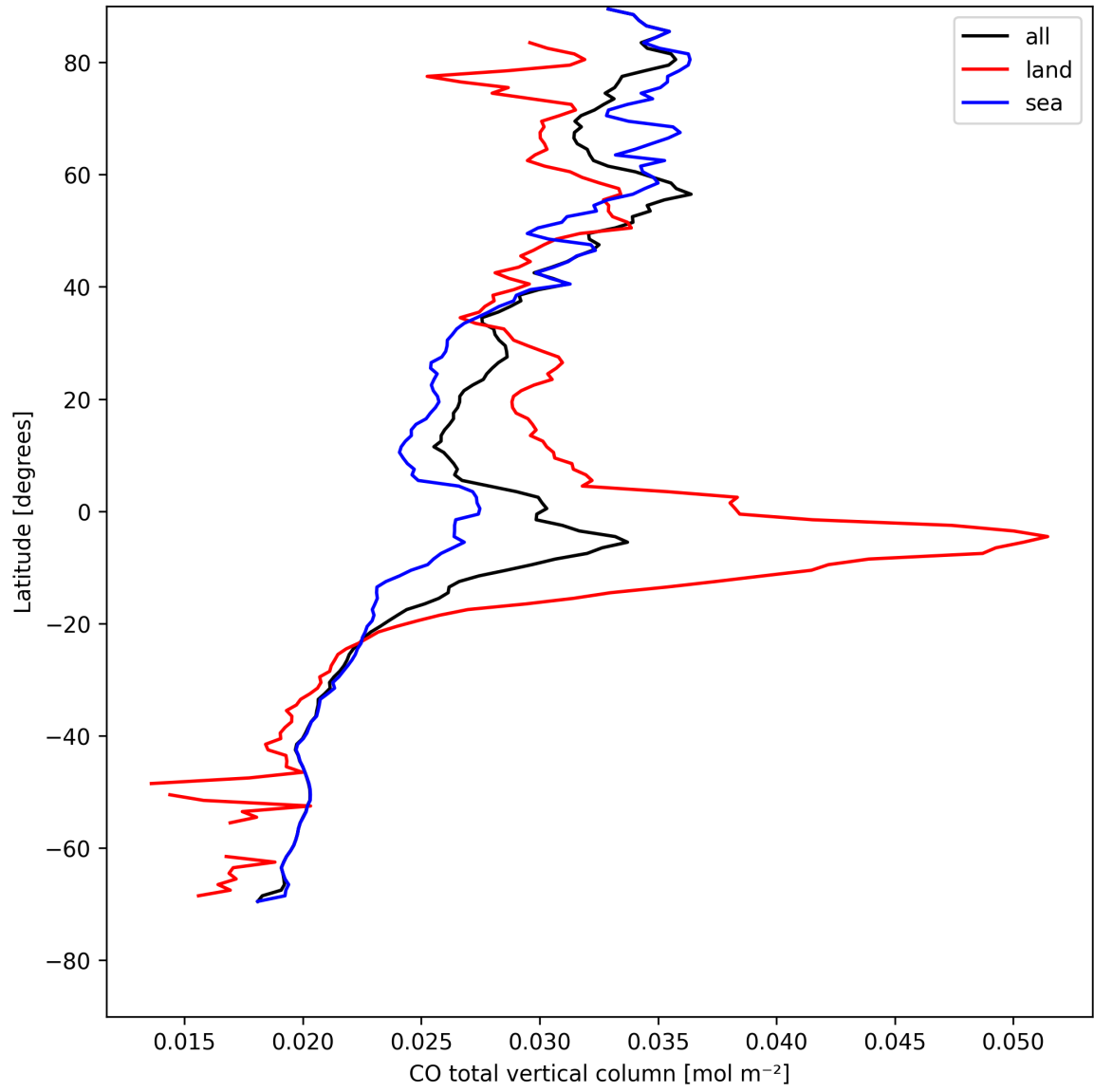
Figure 10: Zonal average of “CO total vertical column” for 2025-08-09 to 2025-08-10.
