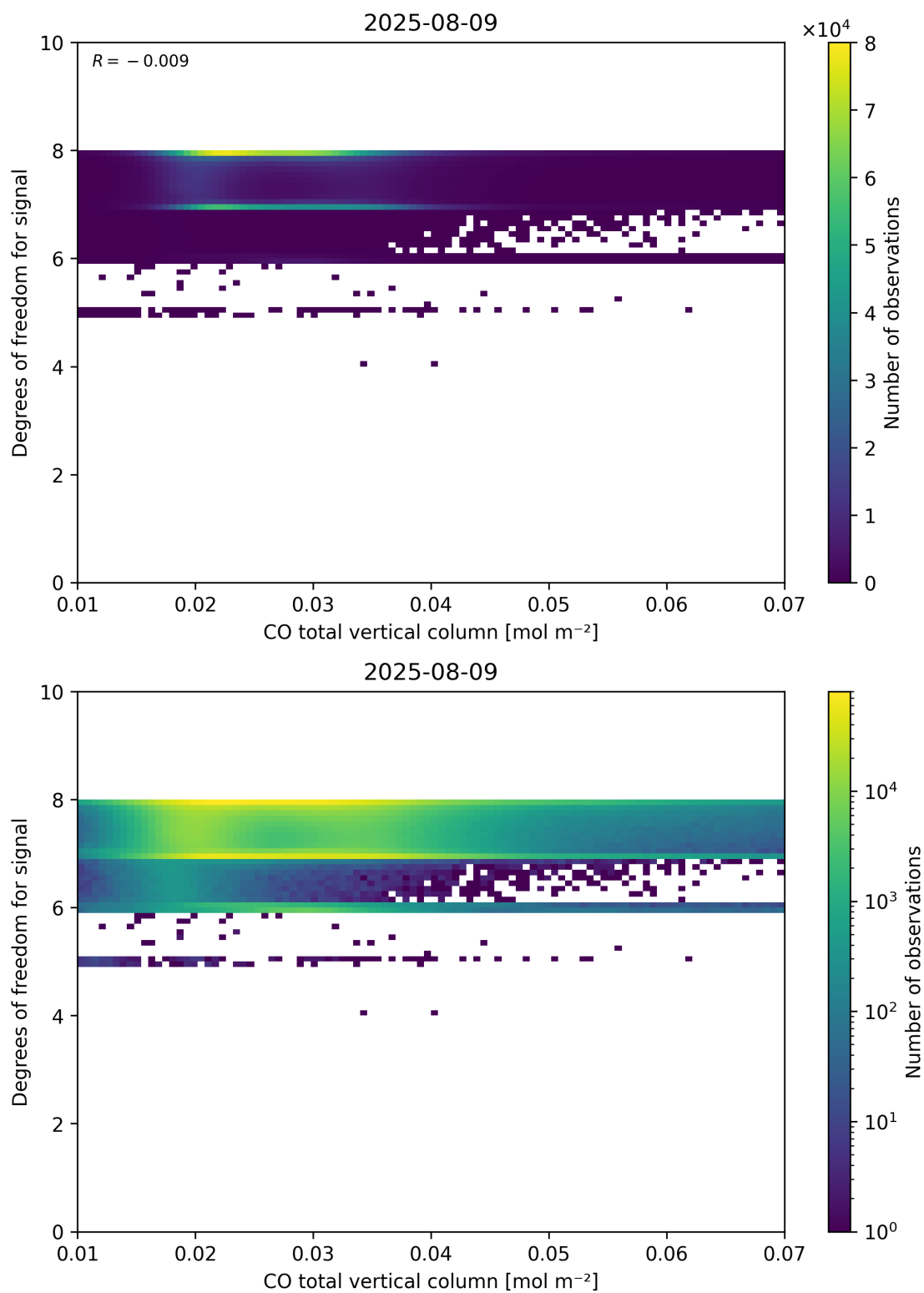
Figure 41: Scatter density plot of “CO total vertical column” against “Degrees of freedom for signal” for 2025-08-09 to 2025-08-10.
