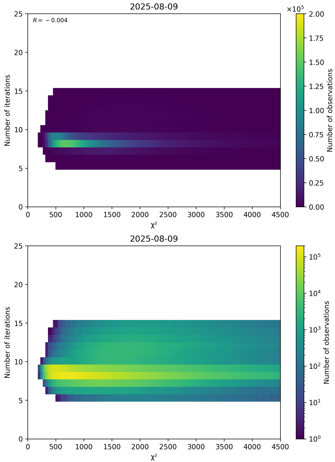
Figure 49: Scatter density plot of “ \chi^2 ” against “Number of iterations” for 2025-08-09 to 2025-08-10.
