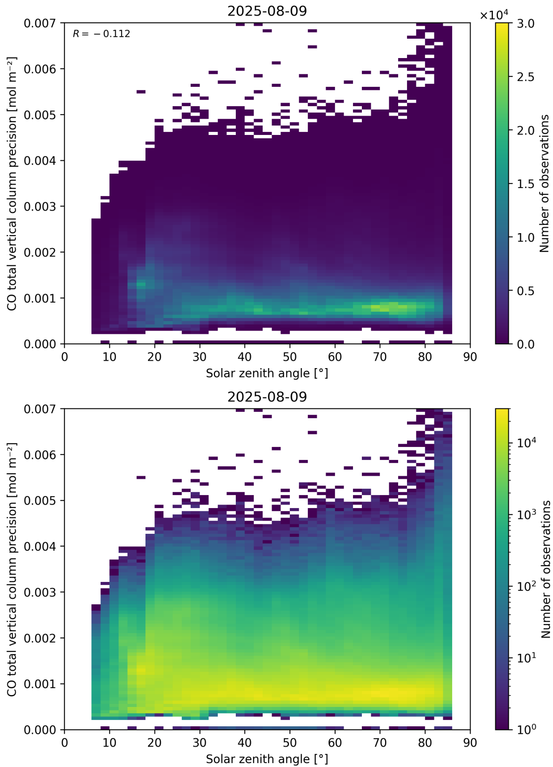
Figure 63: Scatter density plot of “Solar zenith angle” against “CO total vertical column precision” for 2025-08-09 to 2025-08-10.
