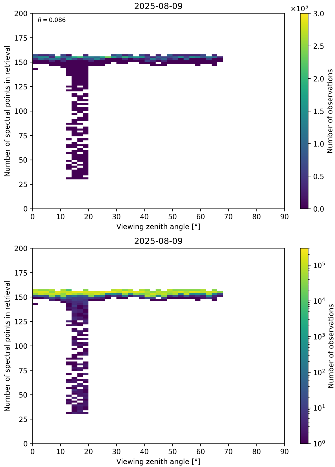
Figure 76: Scatter density plot of “Viewing zenith angle” against “Number of spectral points in retrieval” for 2025-08-09 to 2025-08-10.
