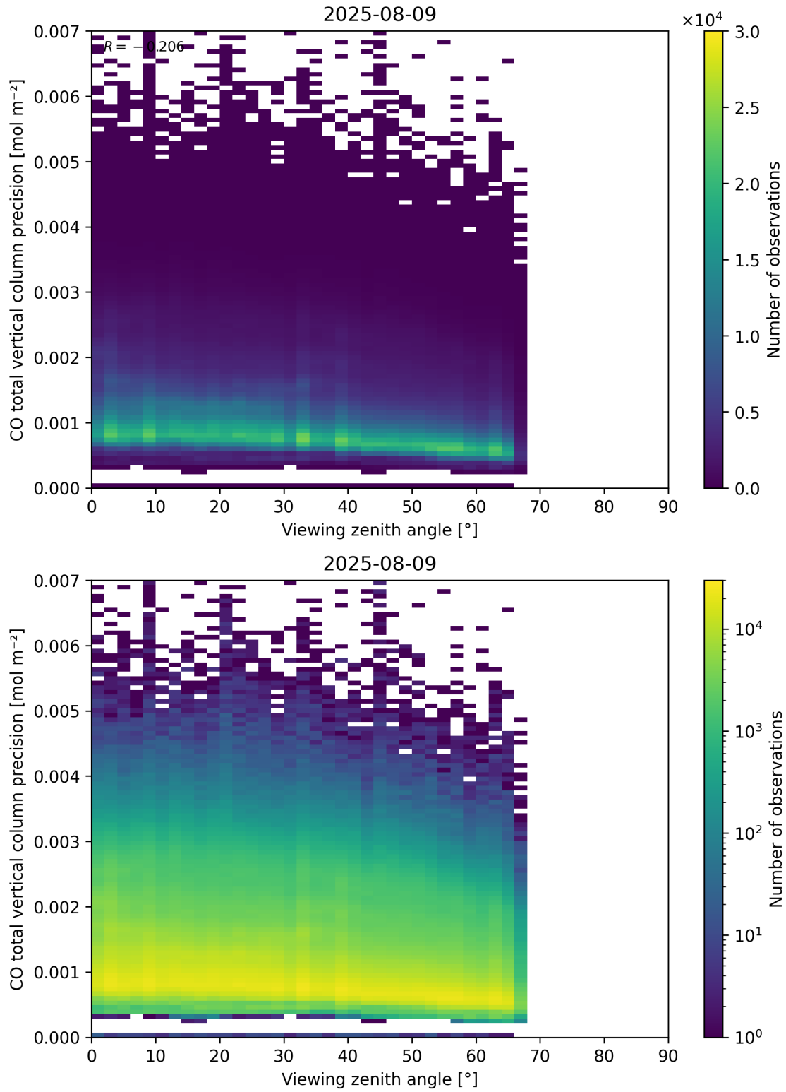
Figure 71: Scatter density plot of “Viewing zenith angle” against “CO total vertical column precision” for 2025-08-09 to 2025-08-10.
