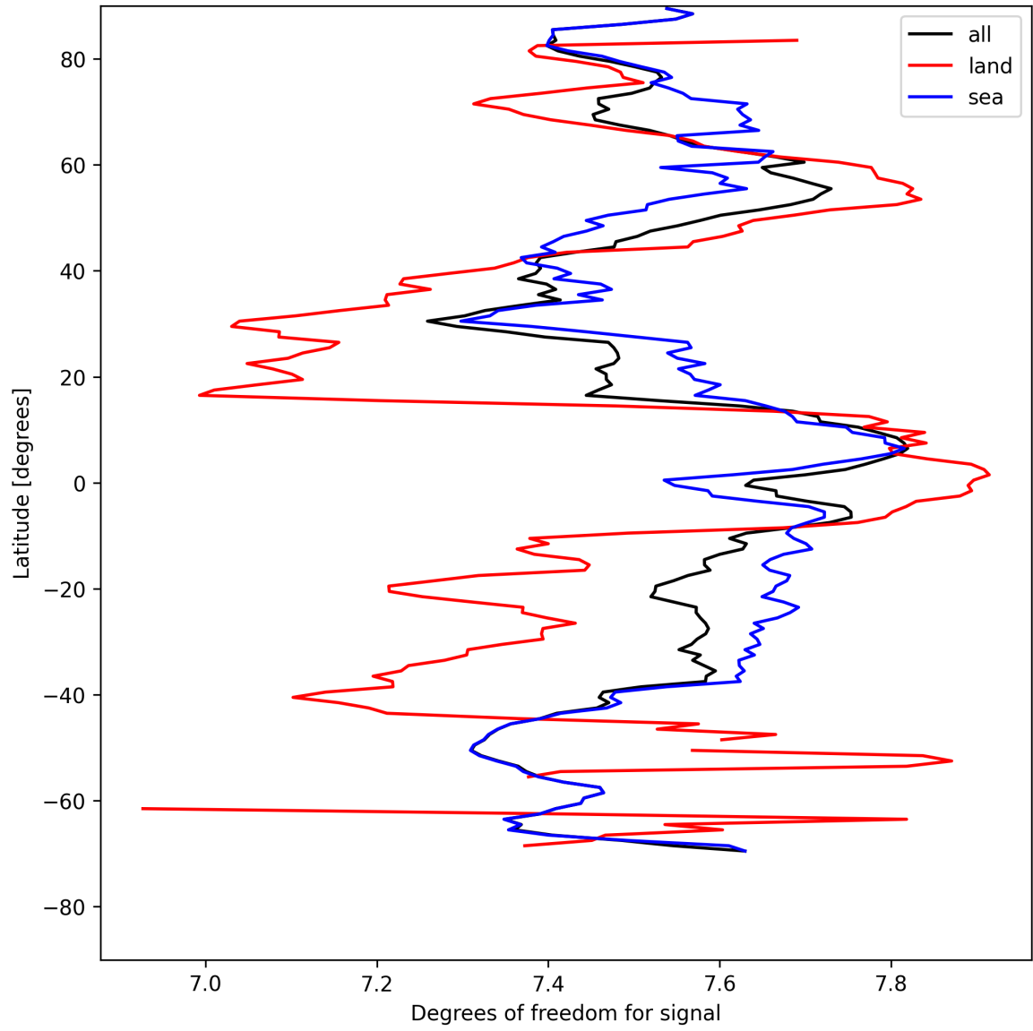
Figure 15: Zonal average of “Degrees of freedom for signal” for 2025-08-09 to 2025-08-10.
