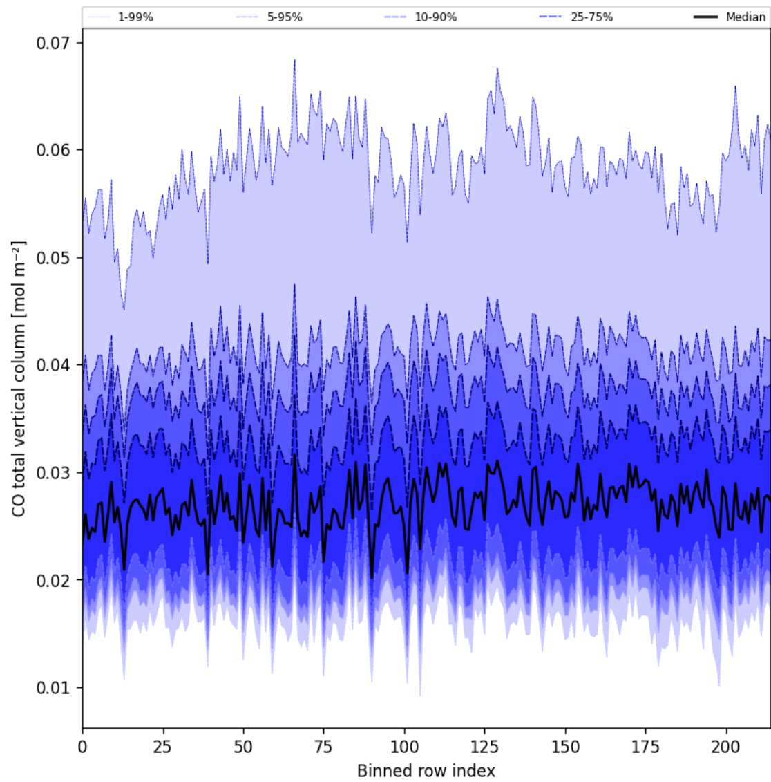
Figure 26: Along track statistics of “CO total vertical column” for 2025-08-09 to 2025-08-10
