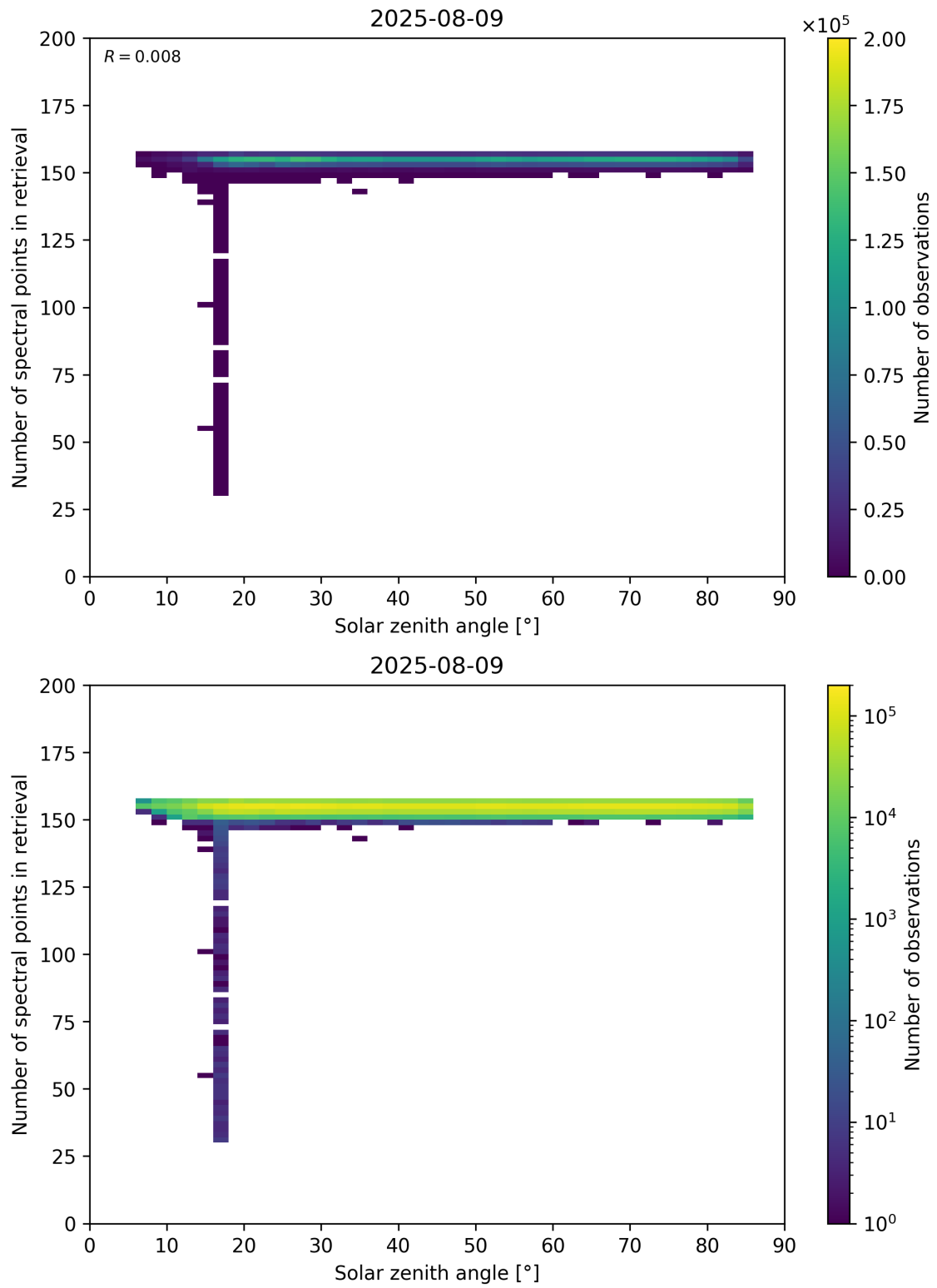
Figure 68: Scatter density plot of “Solar zenith angle” against “Number of spectral points in retrieval” for 2025-08-09 to 2025-08-10.
