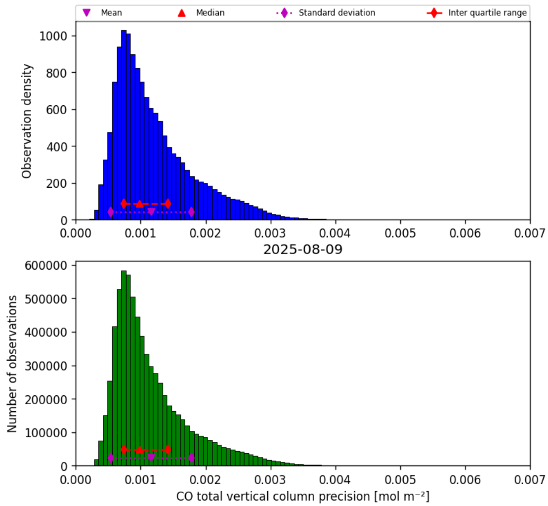
Figure 20: Histogram of “CO total vertical column precision” for 2025-08-09 to 2025-08-10
