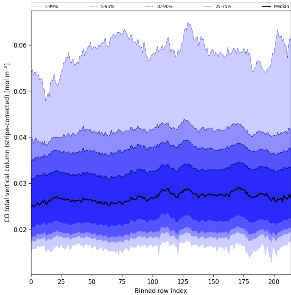
Figure 27: Along track statistics of “CO total vertical column (stripe-corrected)” for 2025-08-09 to 2025-08-10
