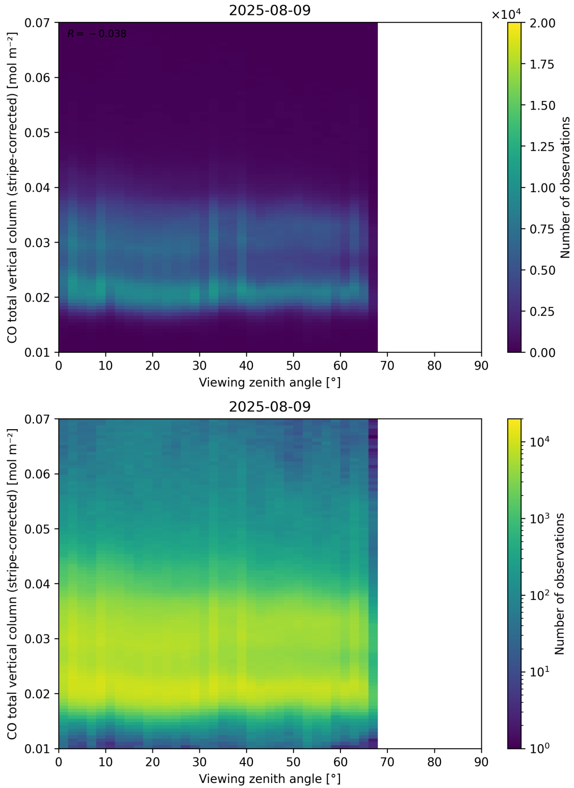
Figure 70: Scatter density plot of “Viewing zenith angle” against “CO total vertical column (stripe-corrected)” for 2025-08-09 to 2025-08-10.
