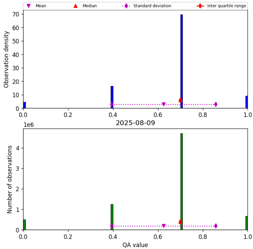
Figure 17: Histogram of “QA value” for 2025-08-09 to 2025-08-10
