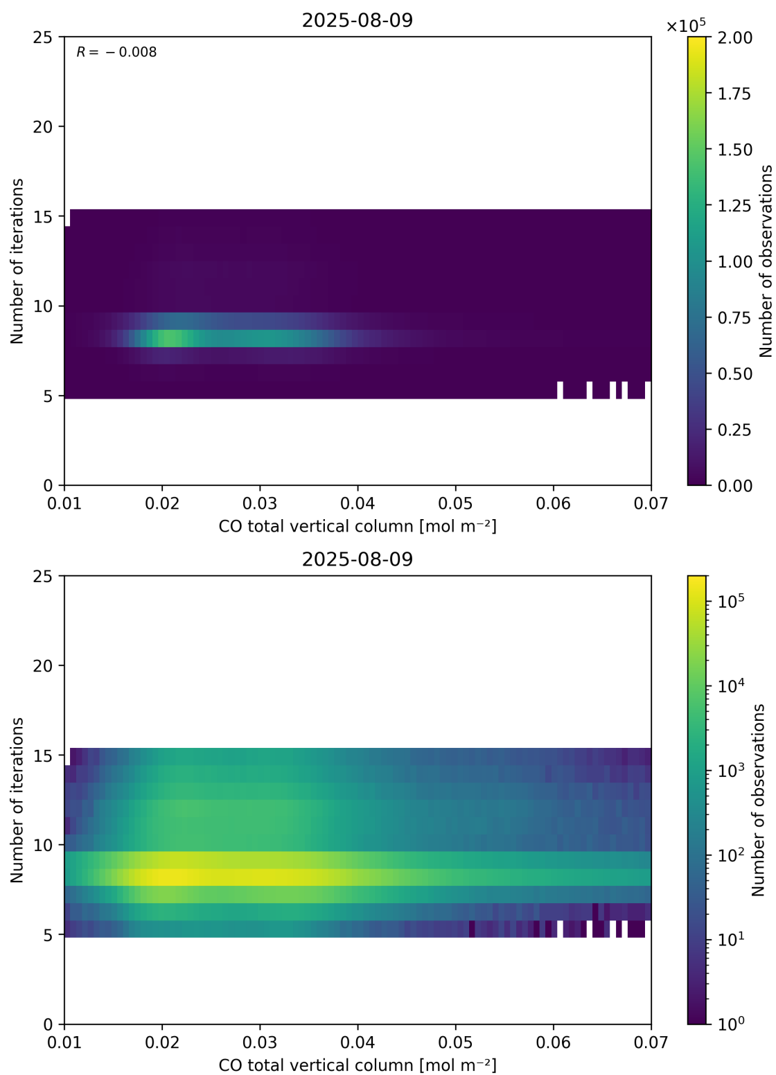
Figure 42: Scatter density plot of “CO total vertical column” against “Number of iterations” for 2025-08-09 to 2025-08-10.
