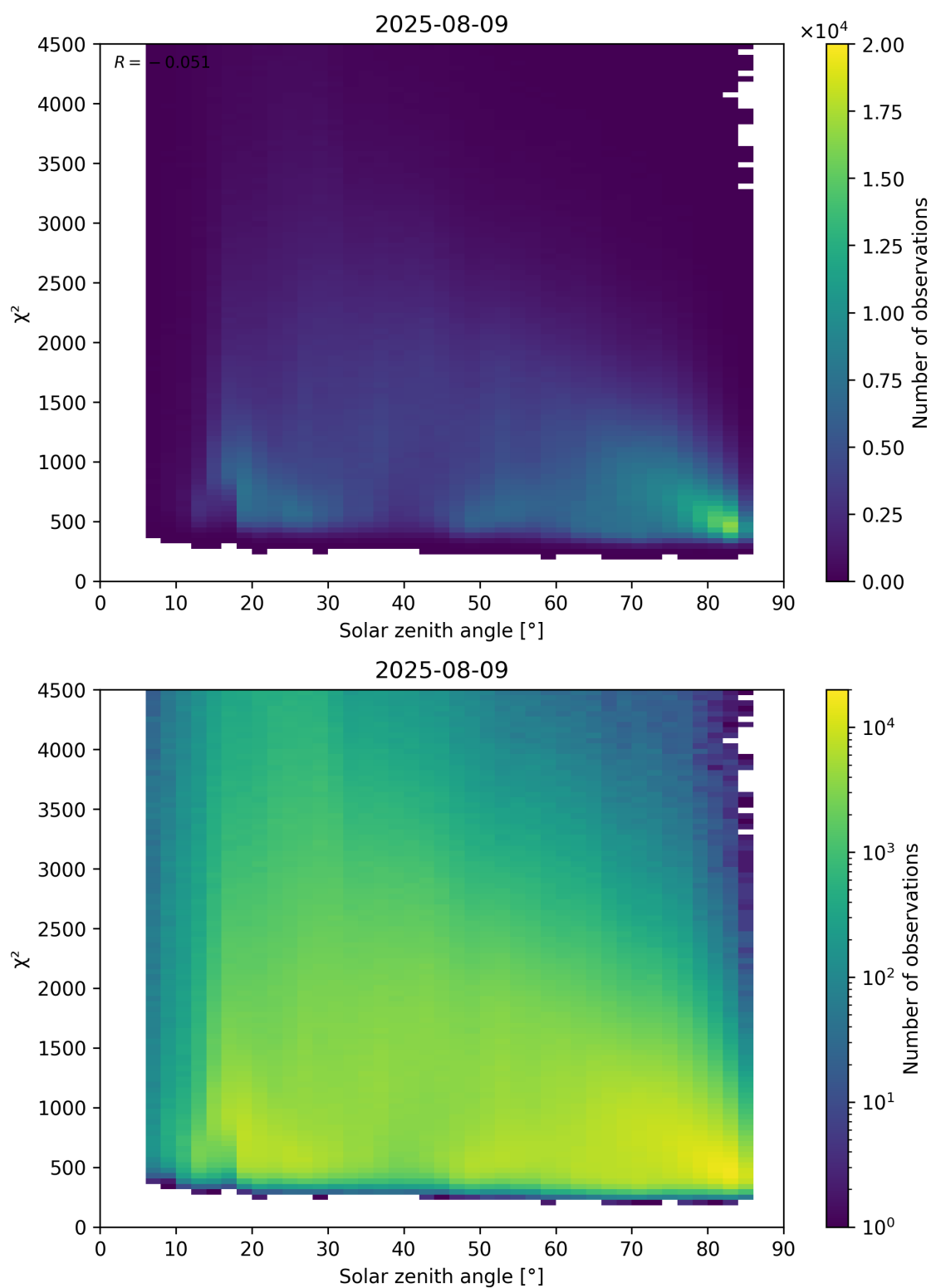
Figure 64: Scatter density plot of “Solar zenith angle” against “ \chi^2 ” for 2025-08-09 to 2025-08-10.
