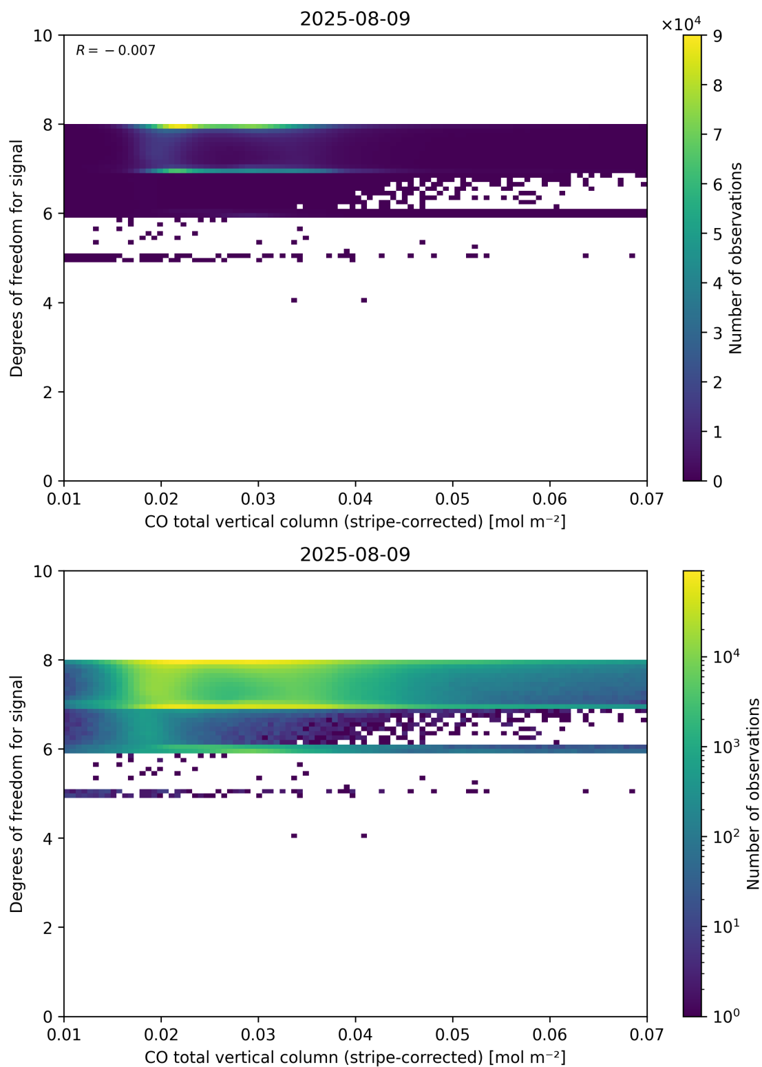
Figure 38: Scatter density plot of “CO total vertical column (stripe-corrected)” against “Degrees of freedom for signal” for 2025-08-09 to 2025-08-10.
