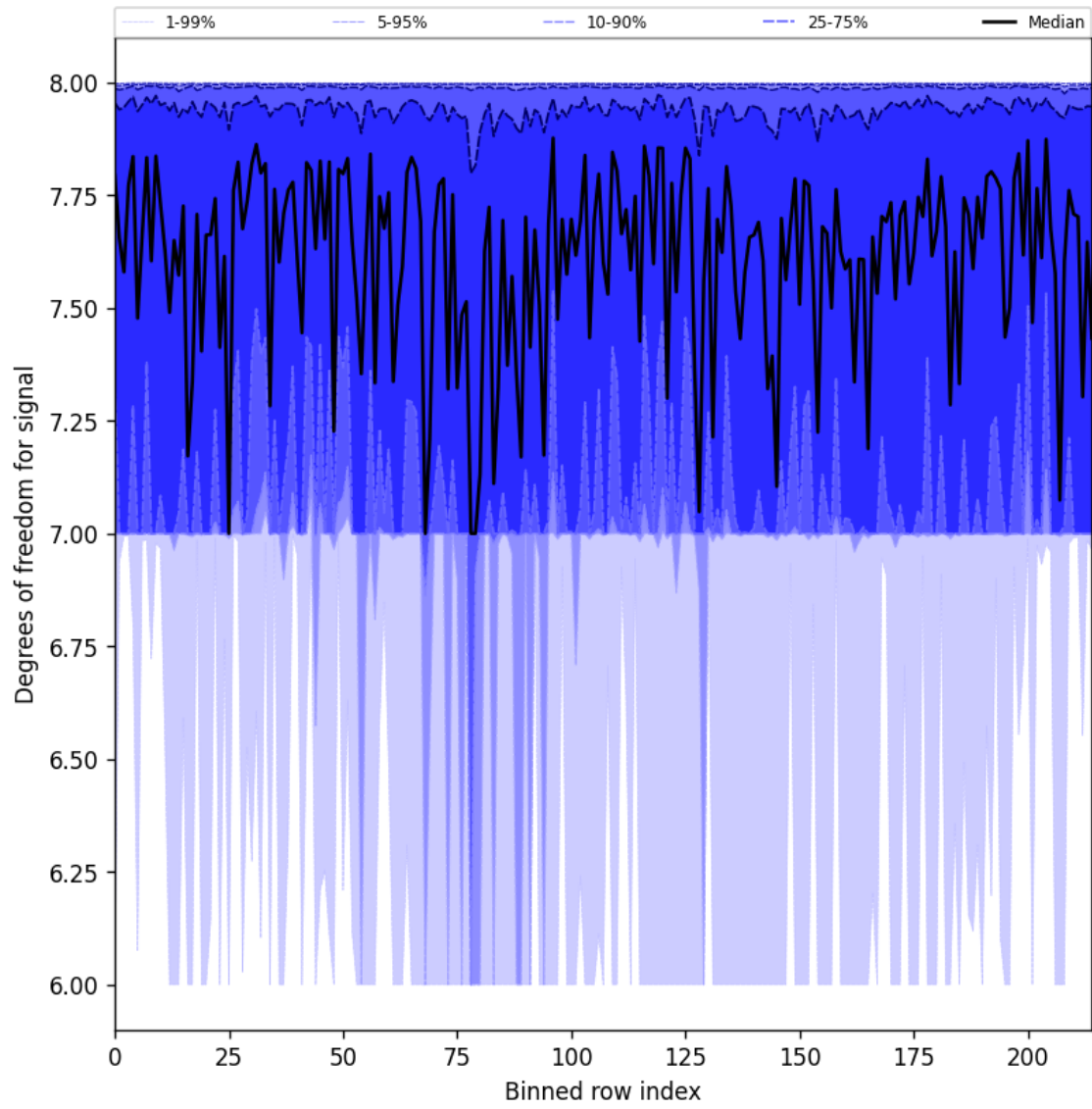
Figure 31: Along track statistics of “Degrees of freedom for signal” for 2025-08-09 to 2025-08-10
