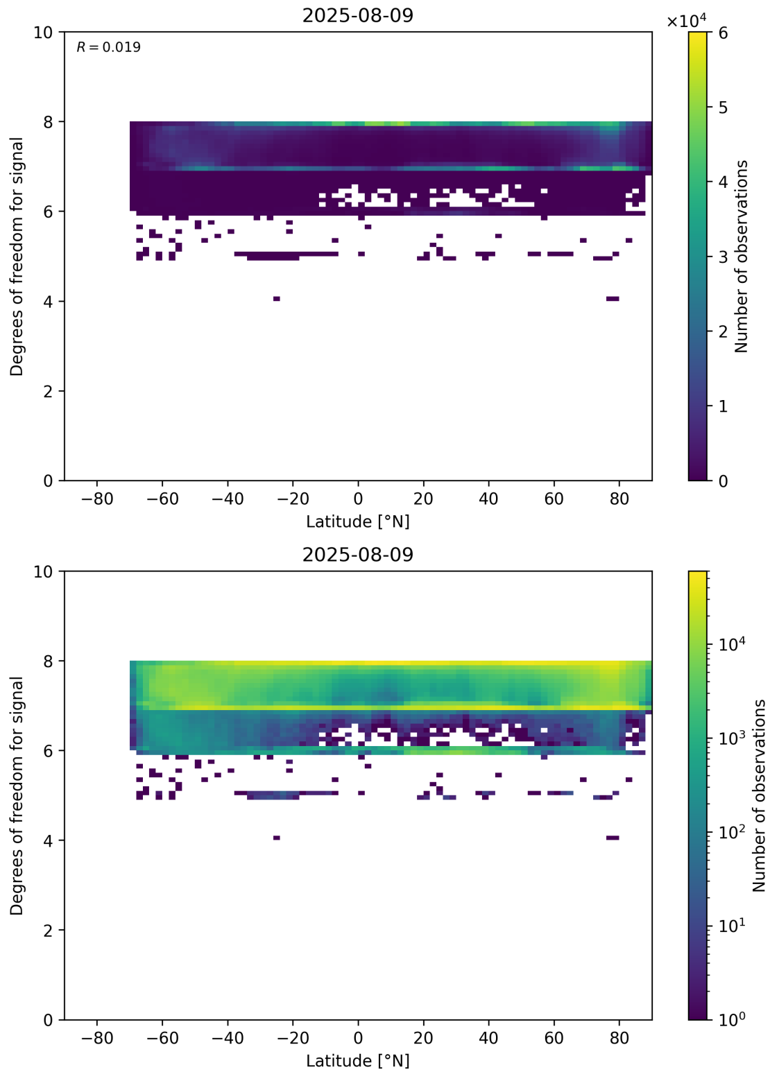
Figure 55: Scatter density plot of “Latitude” against “Degrees of freedom for signal” for 2025-08-09 to 2025-08-10.
