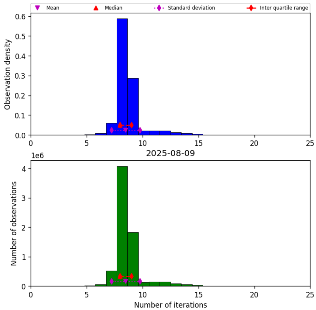
Figure 24: Histogram of “Number of iterations” for 2025-08-09 to 2025-08-10
