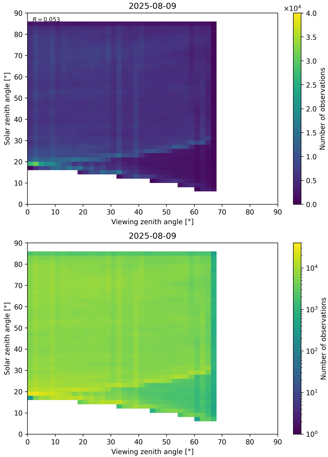
Figure 77: Scatter density plot of “Viewing zenith angle” against “Solar zenith angle” for 2025-08-09 to 2025-08-10.
