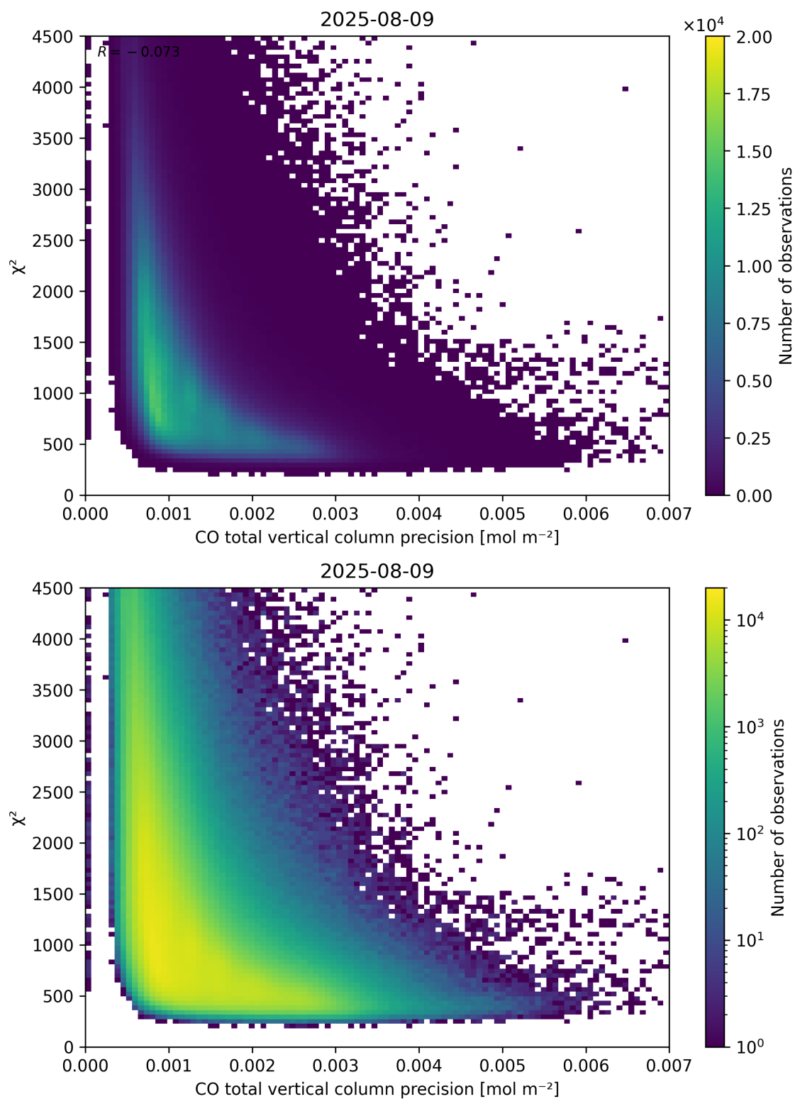
Figure 44: Scatter density plot of “CO total vertical column precision” against “ \chi^2 ” for 2025-08-09 to 2025-08-10.
