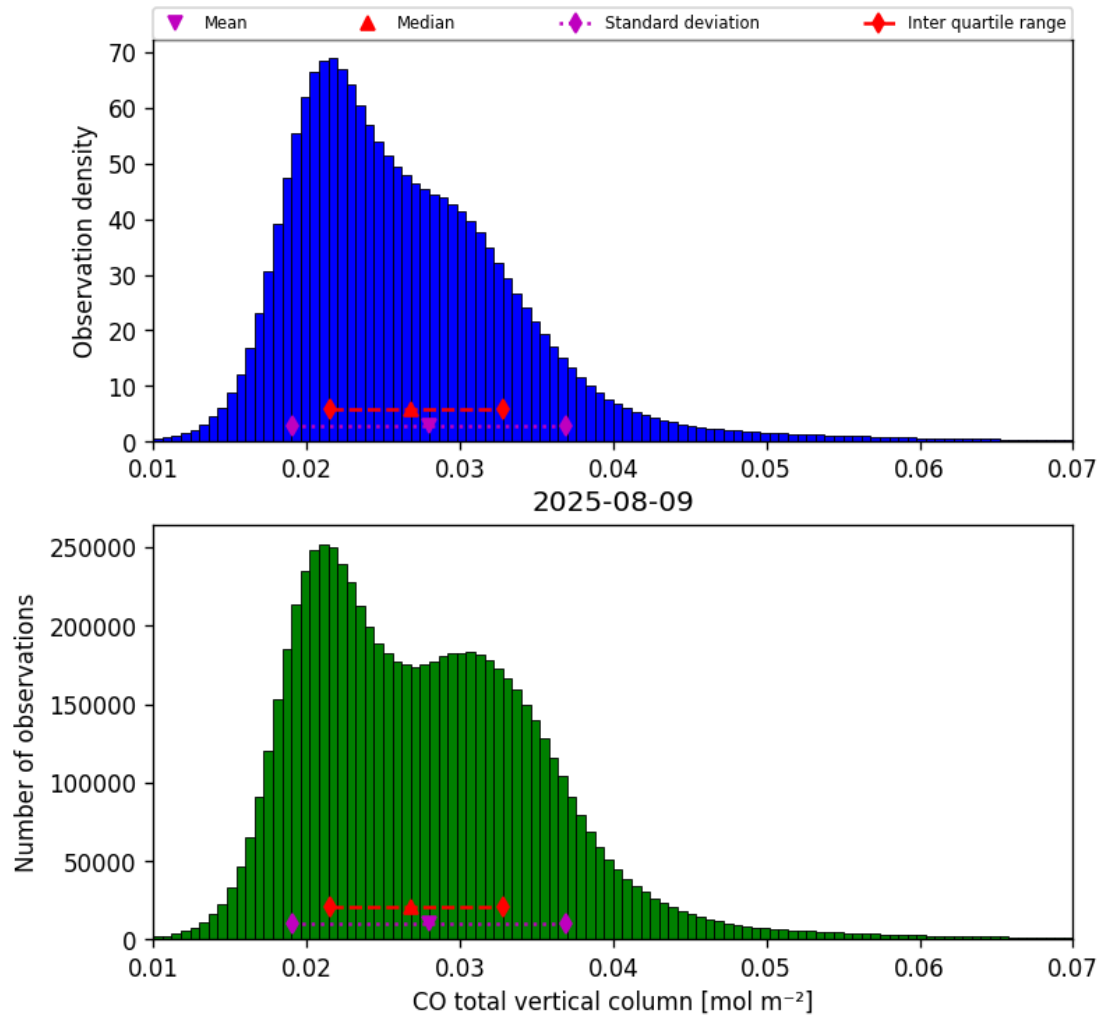
Figure 18: Histogram of “CO total vertical column” for 2025-08-09 to 2025-08-10
