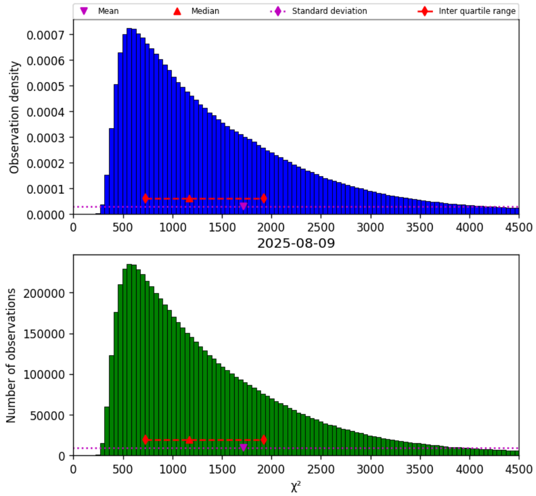
Figure 22: Histogram of “ \chi^2 ” for 2025-08-09 to 2025-08-10
