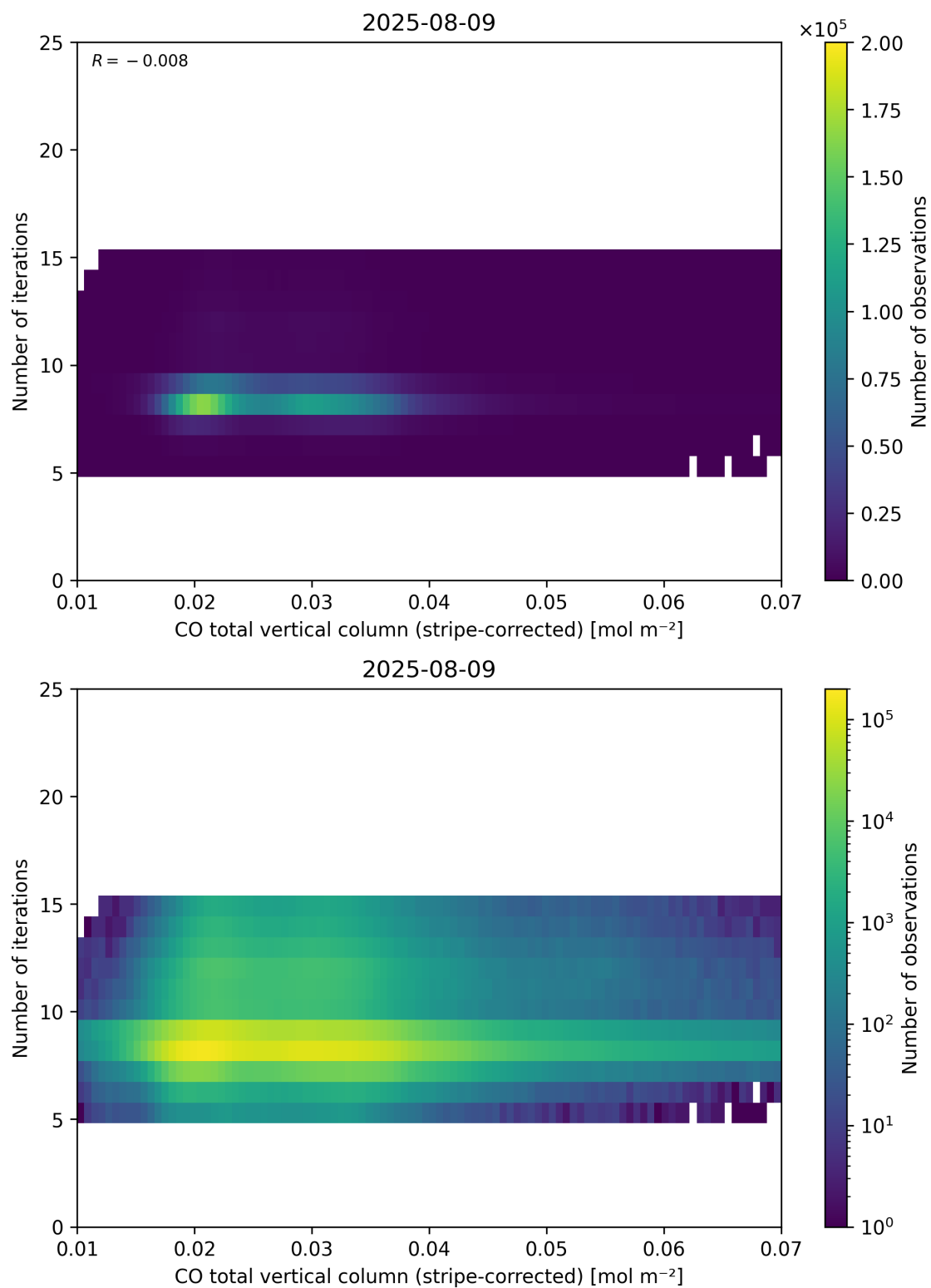
Figure 39: Scatter density plot of “CO total vertical column (stripe-corrected)” against “Number of iterations” for 2025-08-09 to 2025-08-10.
