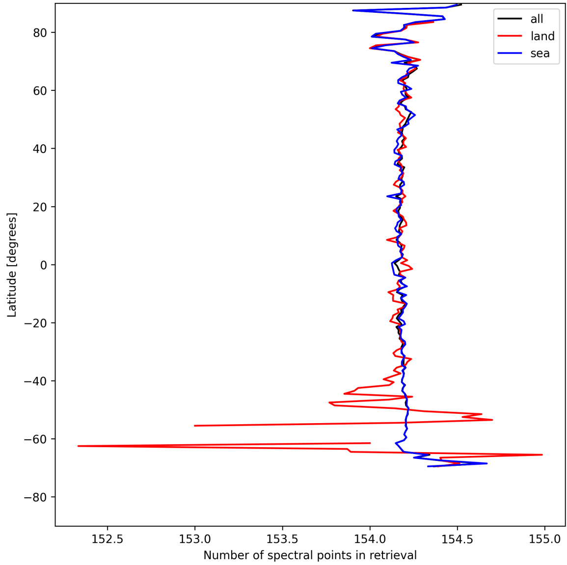
Figure 13: Zonal average of “Number of spectral points in retrieval” for 2025-08-09 to 2025-08-11.
