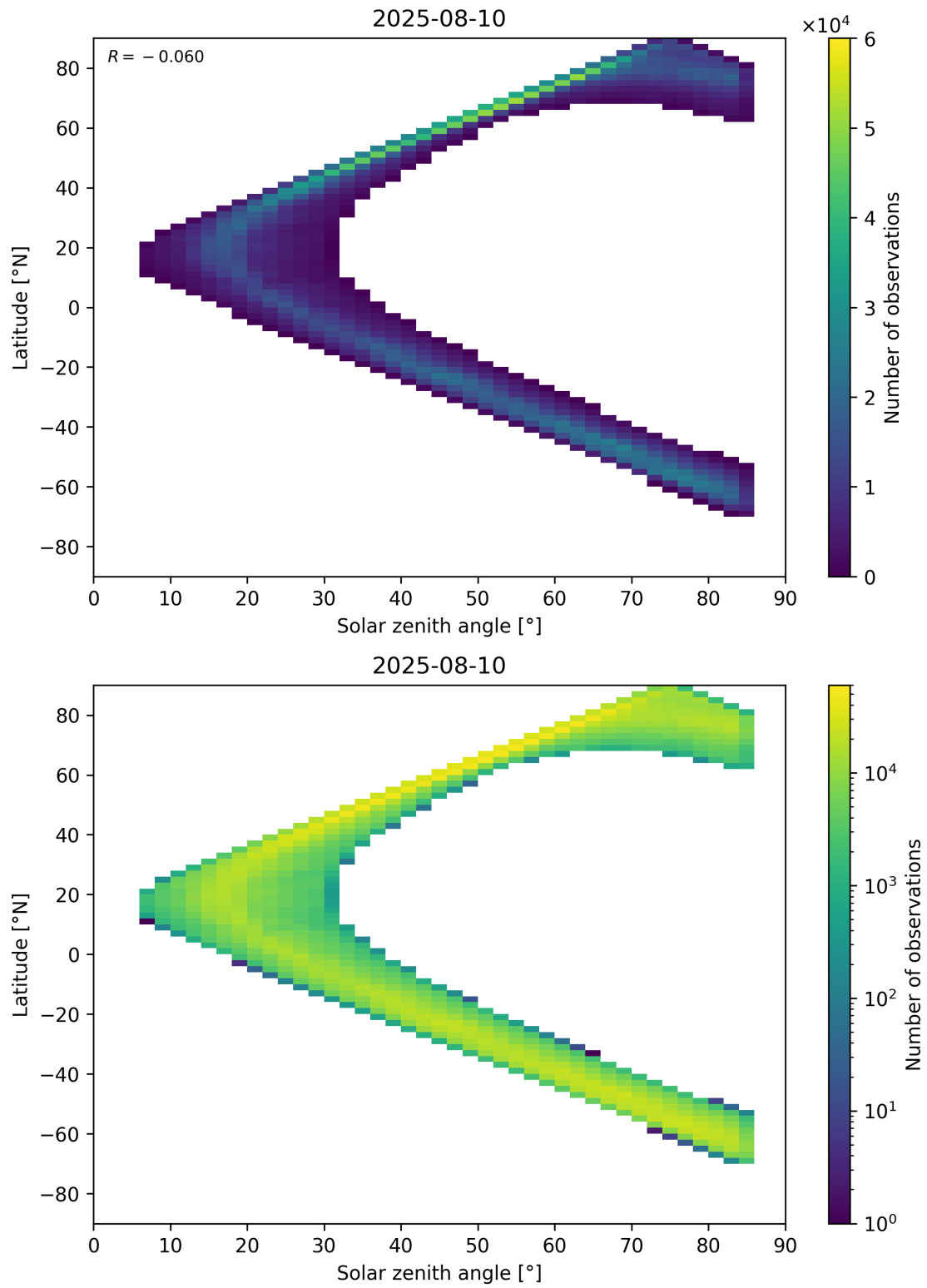
Figure 66: Scatter density plot of “Solar zenith angle” against “Latitude” for 2025-08-09 to 2025-08-11.
