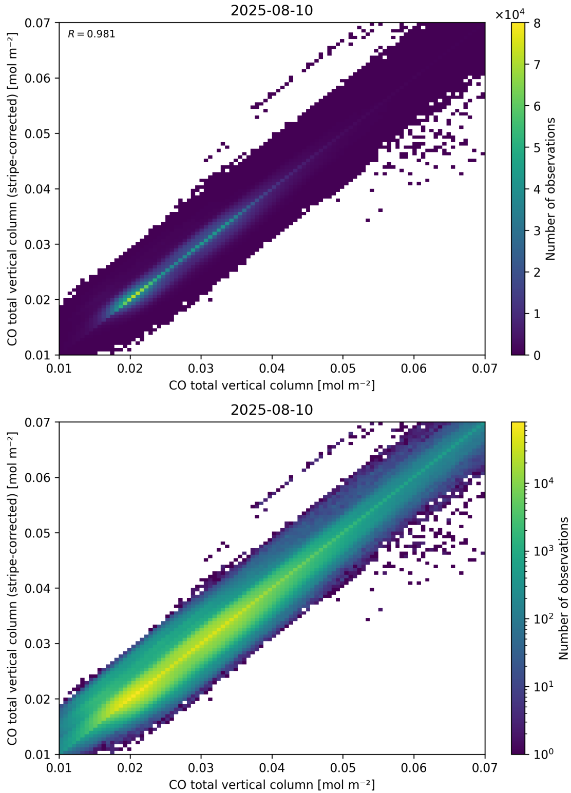
Figure 33: Scatter density plot of “CO total vertical column” against “CO total vertical column (stripe-corrected)” for 2025-08-09 to 2025-08-11.
