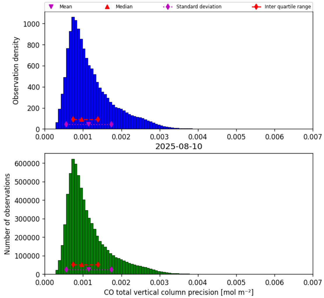
Figure 20: Histogram of “CO total vertical column precision” for 2025-08-09 to 2025-08-11
