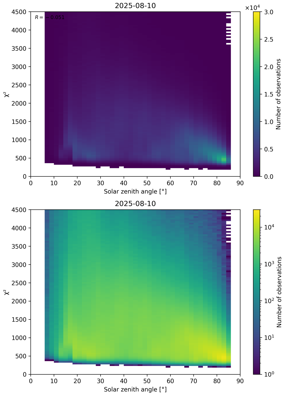
Figure 64: Scatter density plot of “Solar zenith angle” against “ \chi^2 ” for 2025-08-09 to 2025-08-11.
