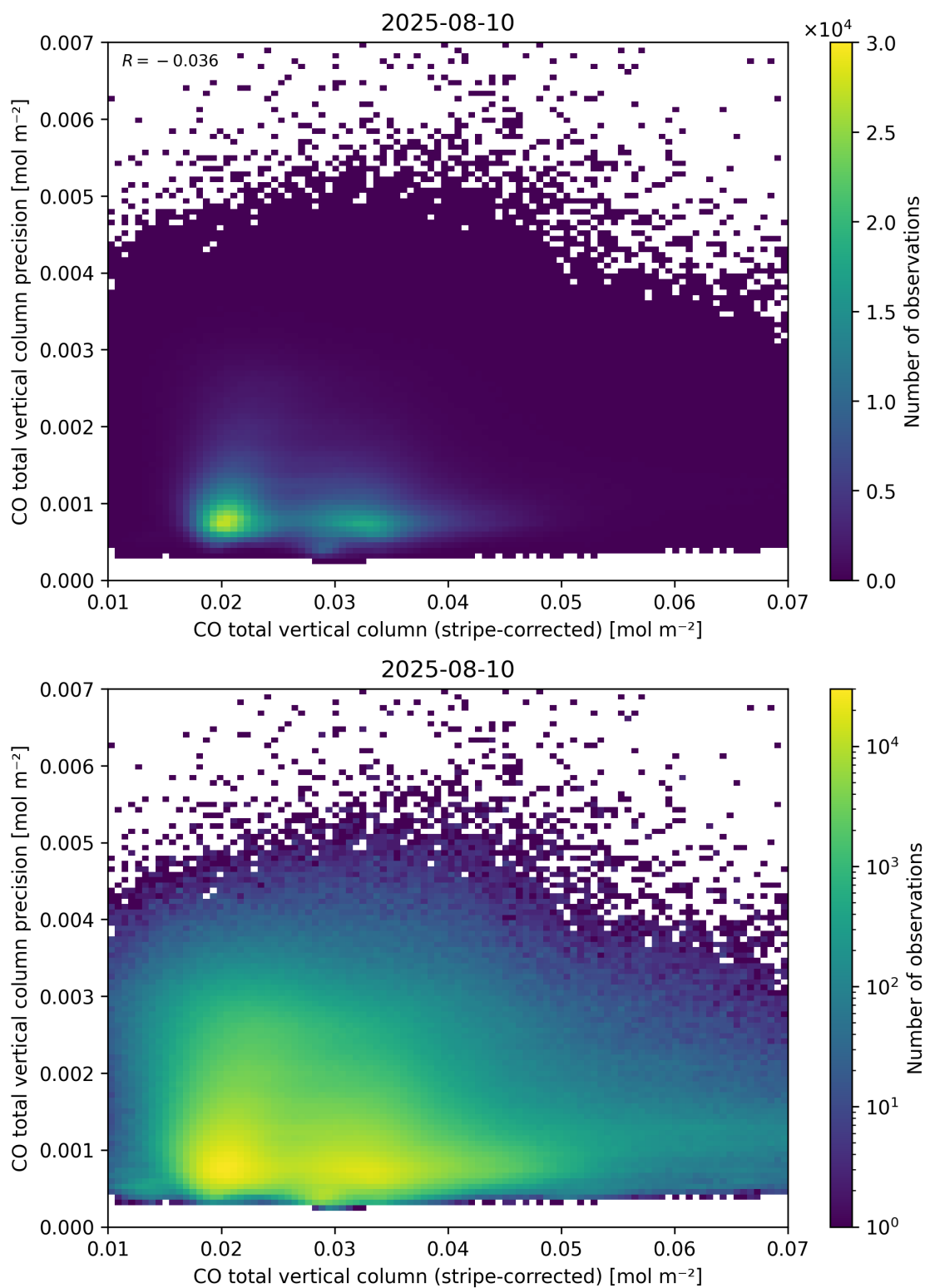
Figure 36: Scatter density plot of “CO total vertical column (stripe-corrected)” against “CO total vertical column precision” for 2025-08-09 to 2025-08-11.
