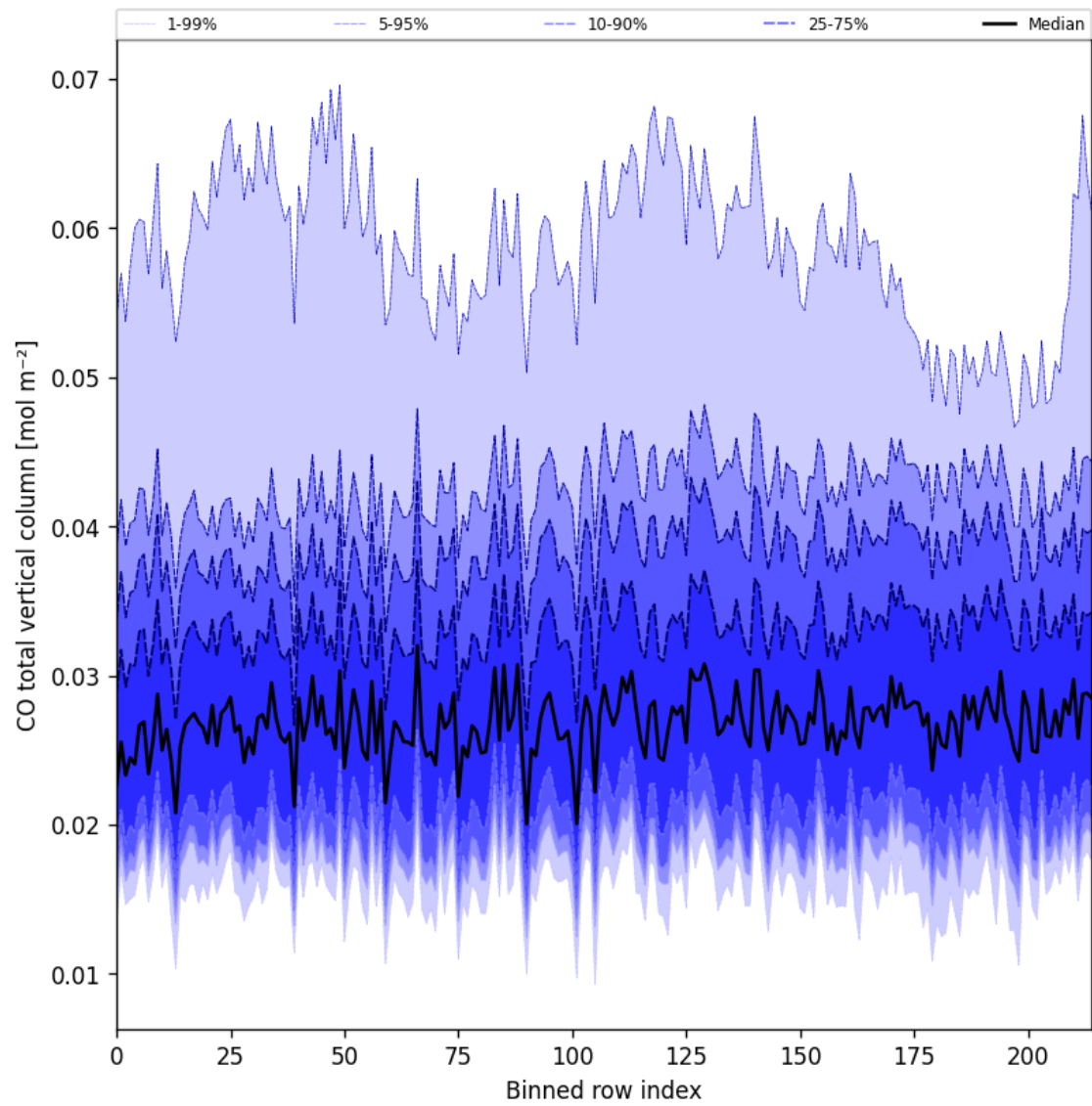
Figure 26: Along track statistics of “CO total vertical column” for 2025-08-09 to 2025-08-11
