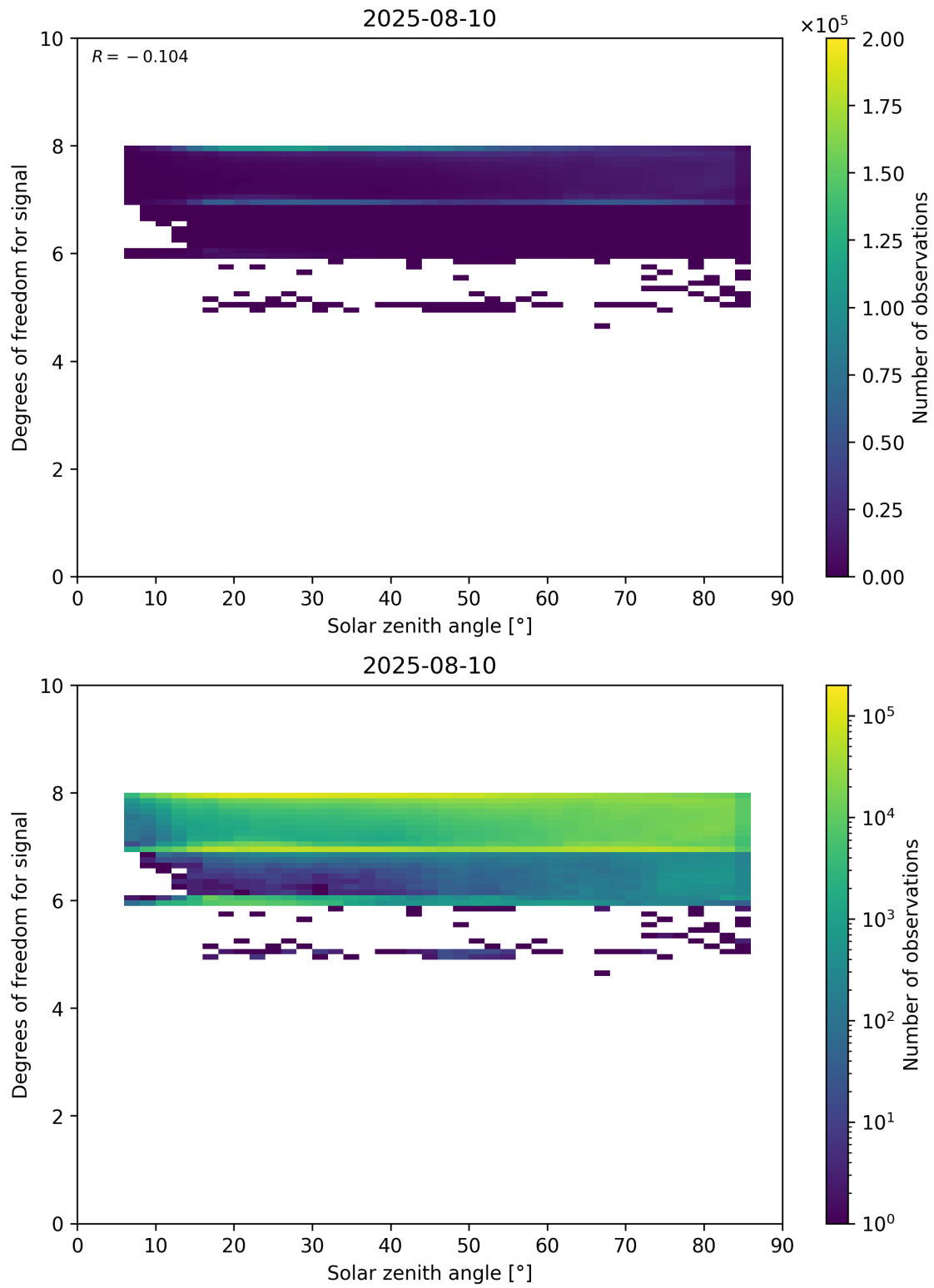
Figure 65: Scatter density plot of “Solar zenith angle” against “Degrees of freedom for signal” for 2025-08-09 to 2025-08-11.
