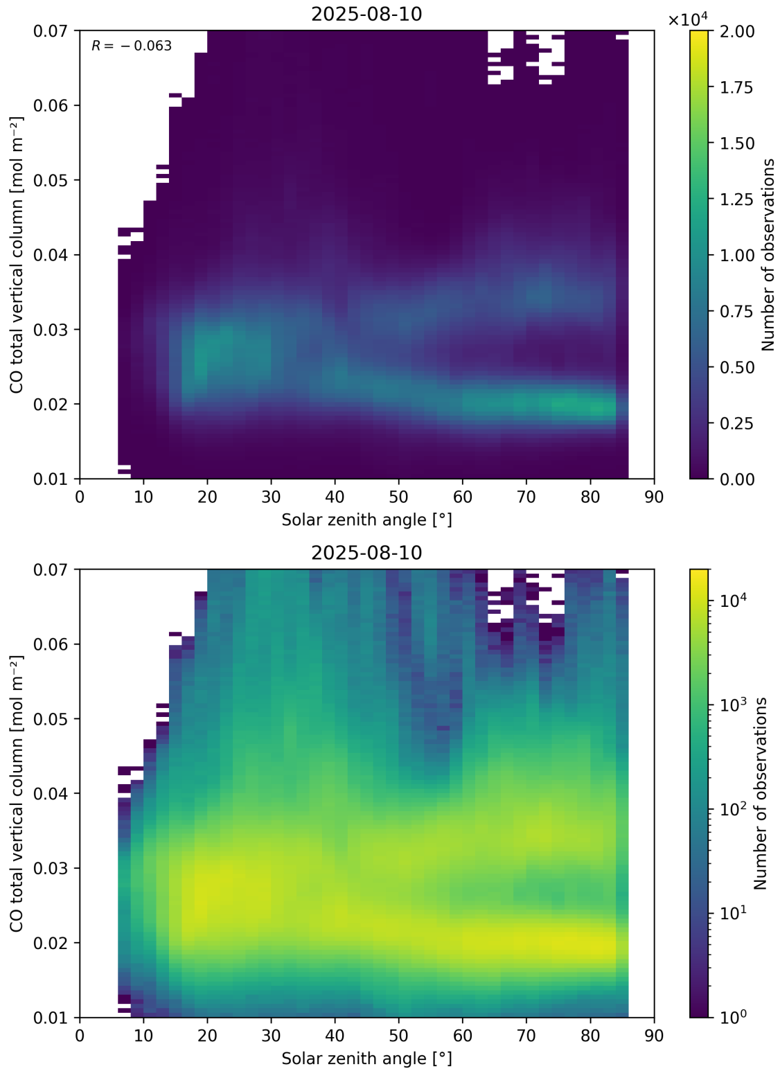
Figure 61: Scatter density plot of “Solar zenith angle” against “CO total vertical column” for 2025-08-09 to 2025-08-11.
