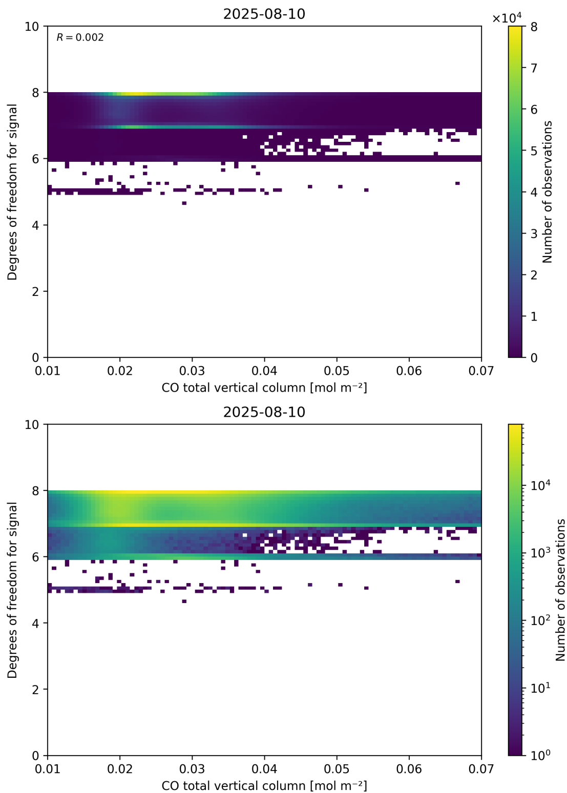
Figure 41: Scatter density plot of “CO total vertical column” against “Degrees of freedom for signal” for 2025-08-09 to 2025-08-11.
