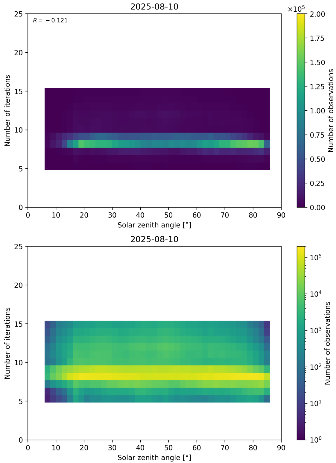
Figure 67: Scatter density plot of “Solar zenith angle” against “Number of iterations” for 2025-08-09 to 2025-08-11.
