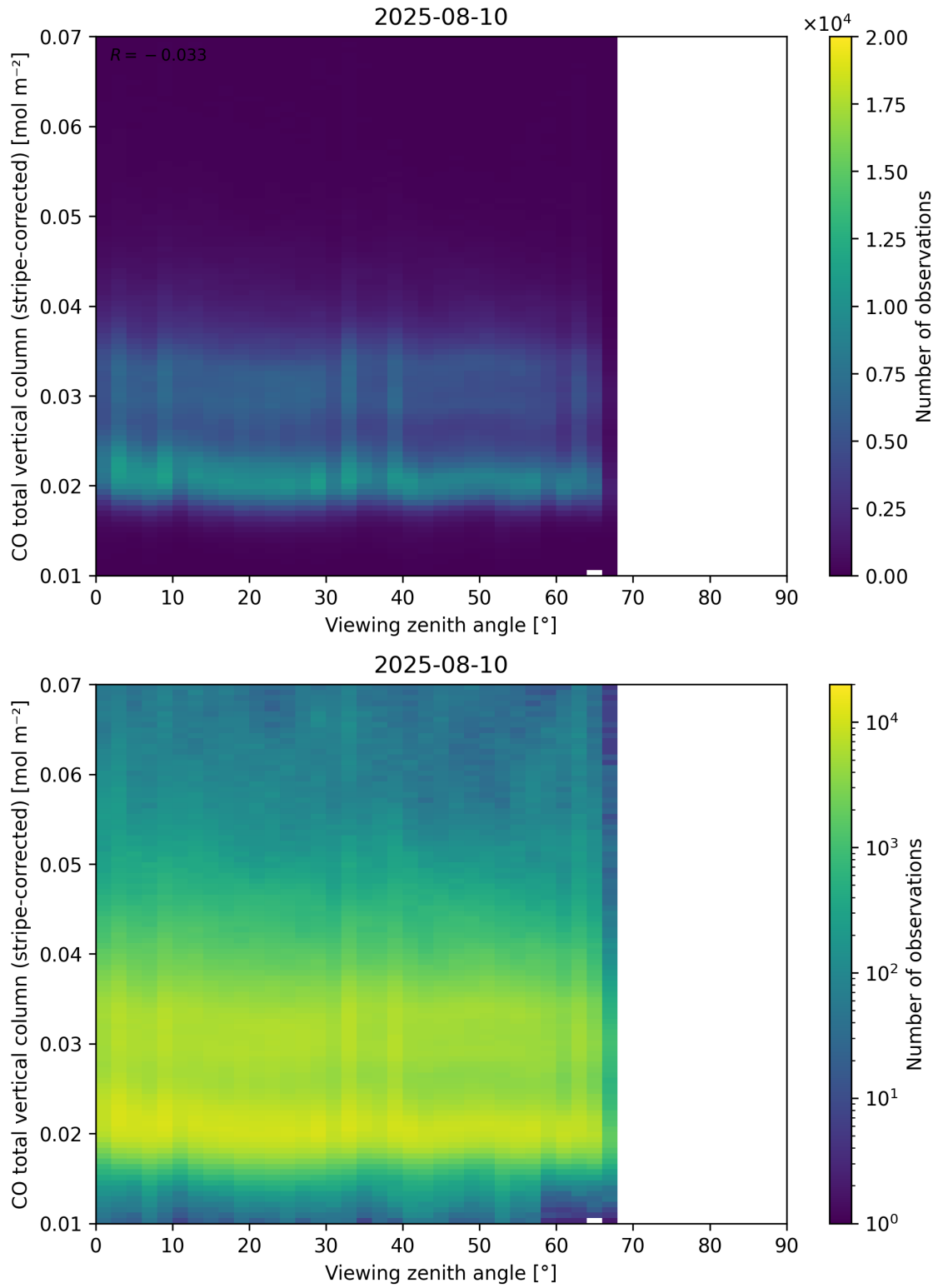
Figure 70: Scatter density plot of “Viewing zenith angle” against “CO total vertical column (stripe-corrected)” for 2025-08-09 to 2025-08-11.
