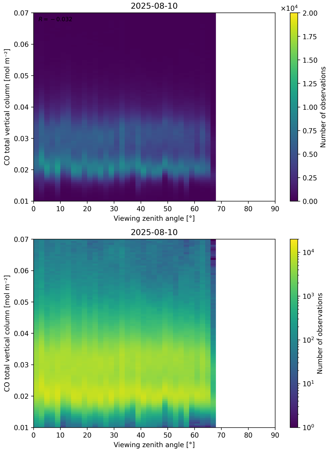
Figure 69: Scatter density plot of “Viewing zenith angle” against “CO total vertical column” for 2025-08-09 to 2025-08-11.
