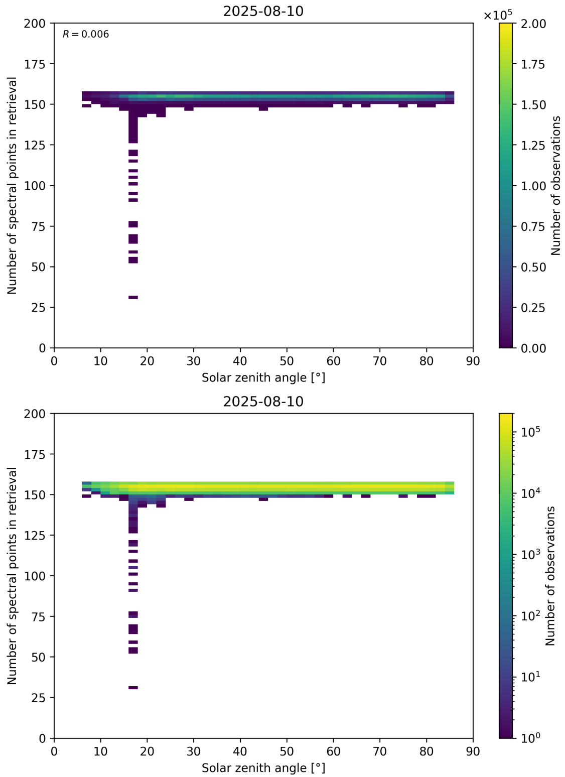
Figure 68: Scatter density plot of “Solar zenith angle” against “Number of spectral points in retrieval” for 2025-08-09 to 2025-08-11.
