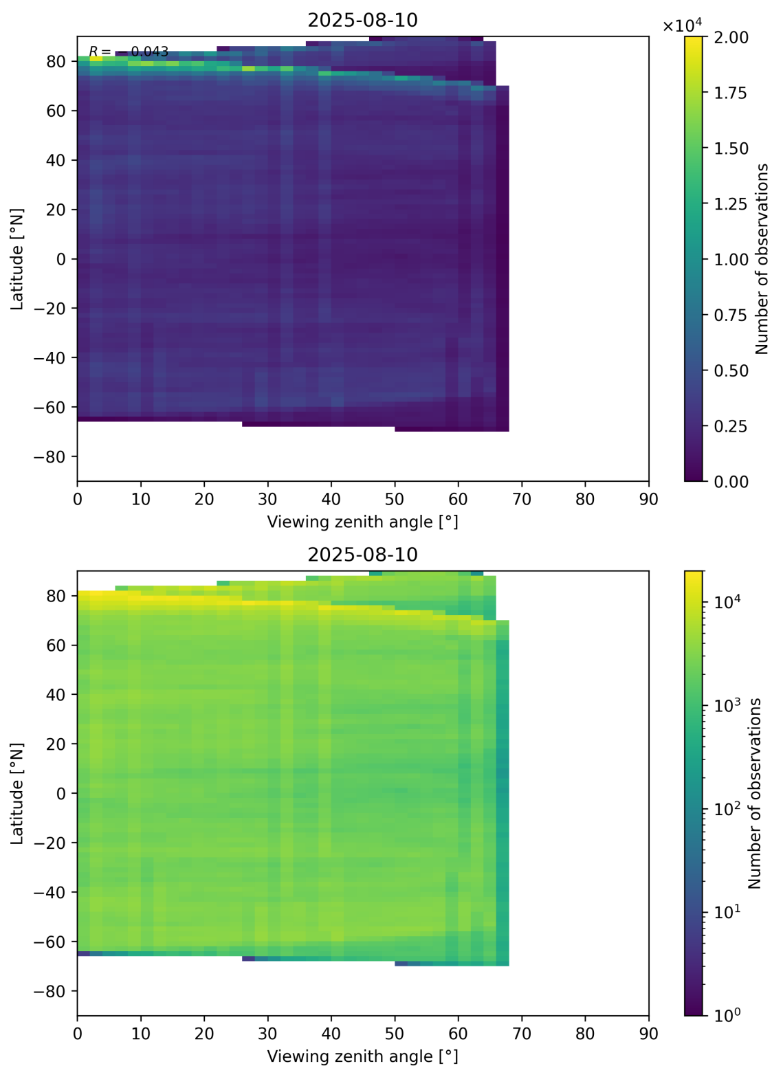
Figure 74: Scatter density plot of “Viewing zenith angle” against “Latitude” for 2025-08-09 to 2025-08-11.
