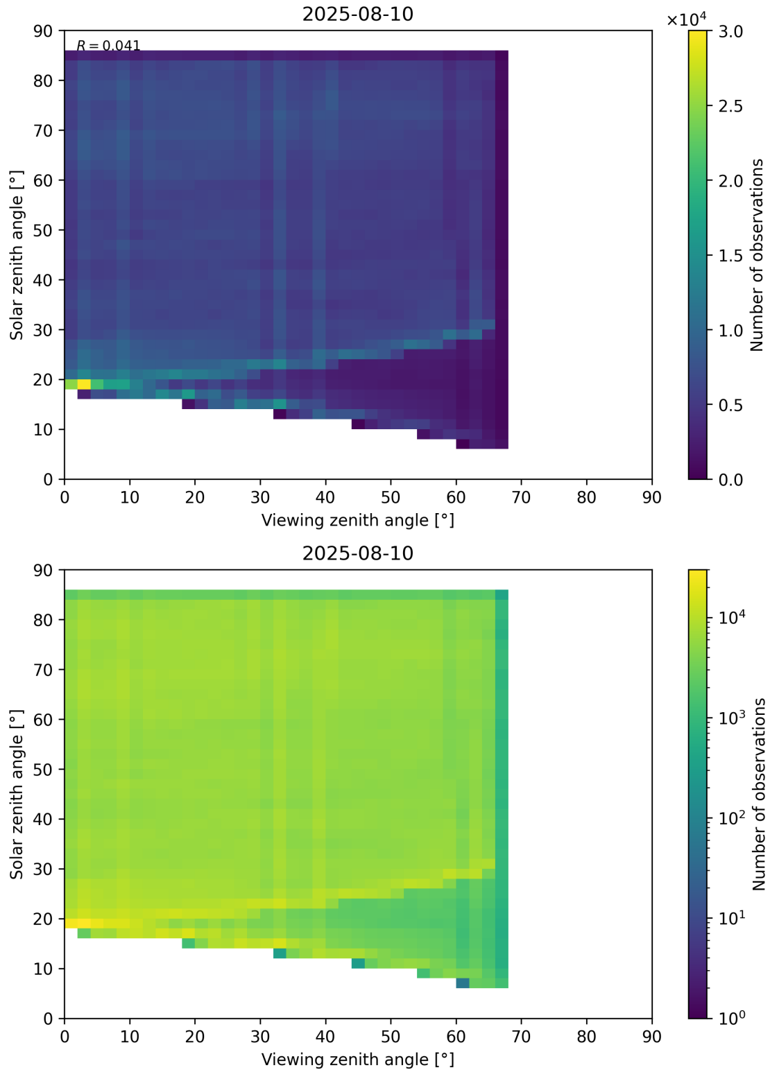
Figure 77: Scatter density plot of “Viewing zenith angle” against “Solar zenith angle” for 2025-08-09 to 2025-08-11.
