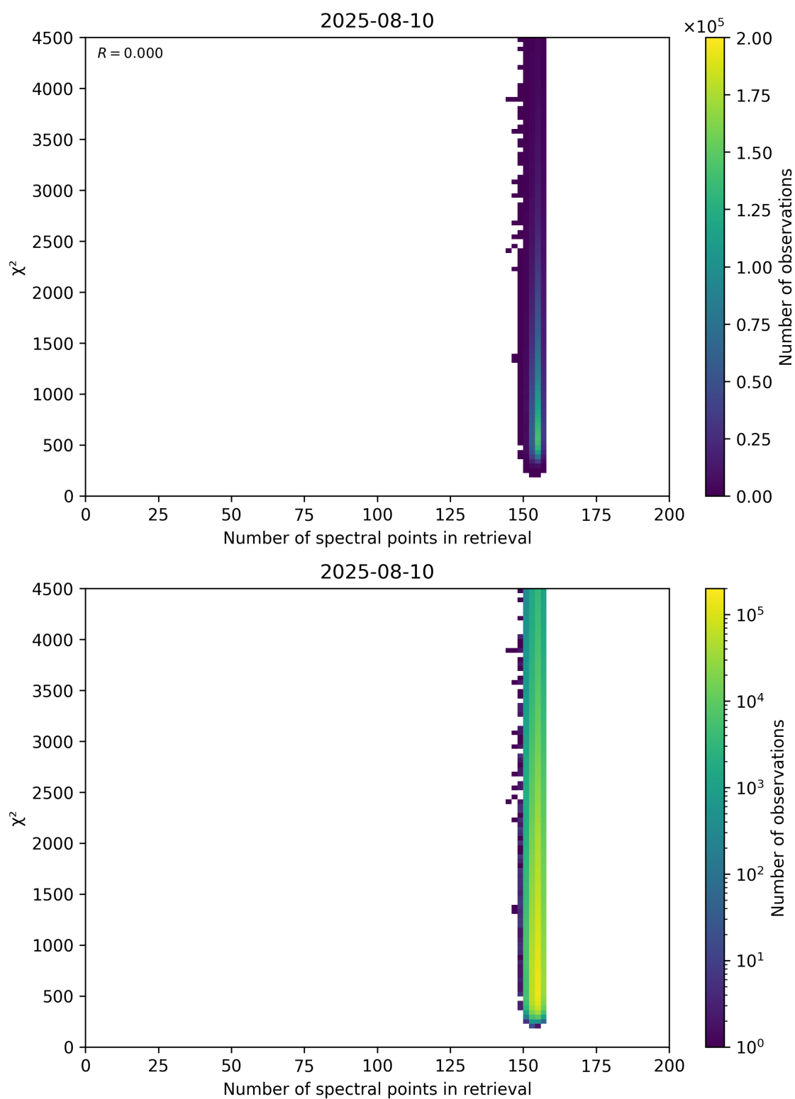
Figure 58: Scatter density plot of “Number of spectral points in retrieval” against “ \chi^2 ” for 2025-08-09 to 2025-08-11.
