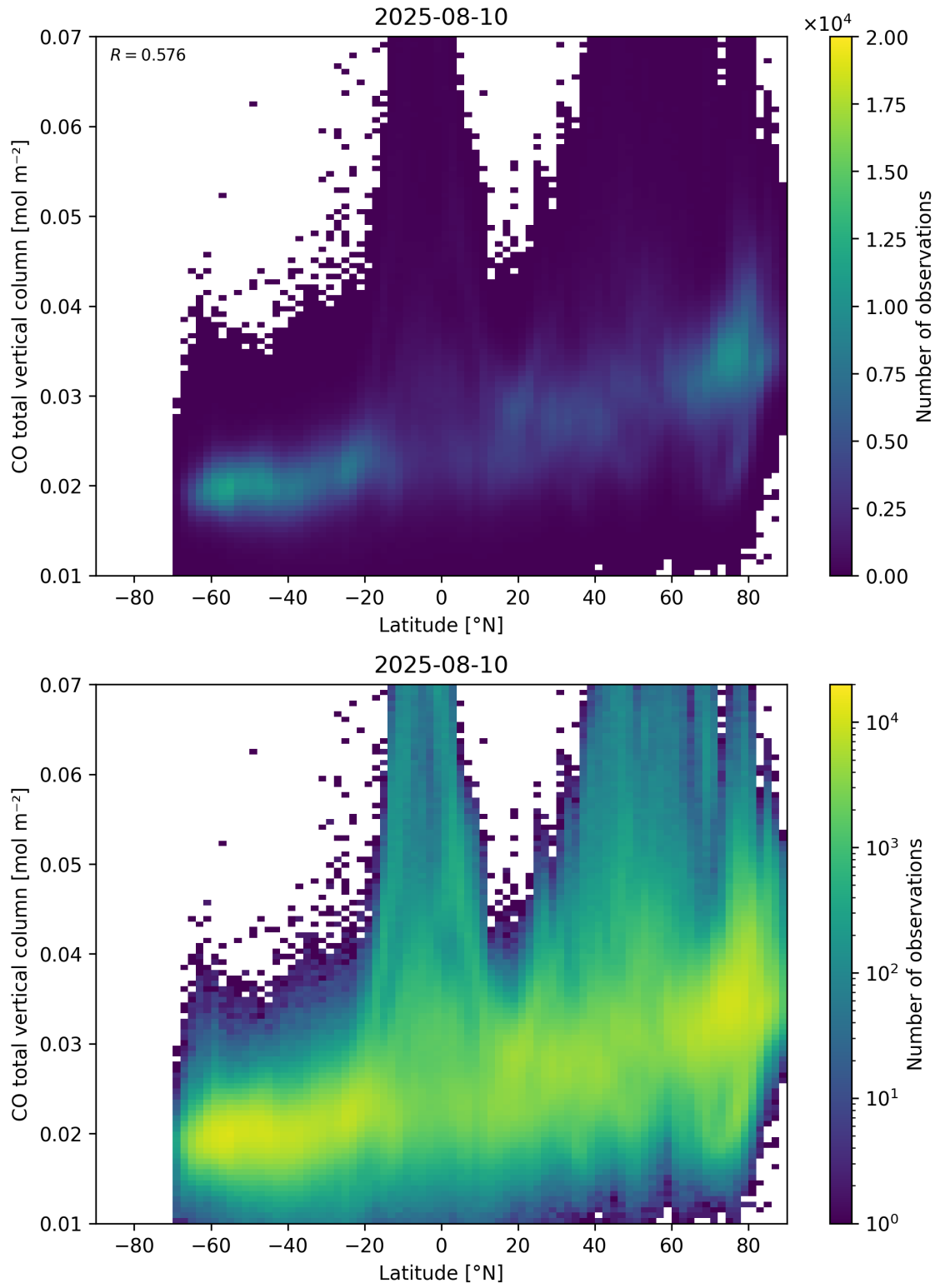
Figure 51: Scatter density plot of “Latitude” against “CO total vertical column” for 2025-08-09 to 2025-08-11.
