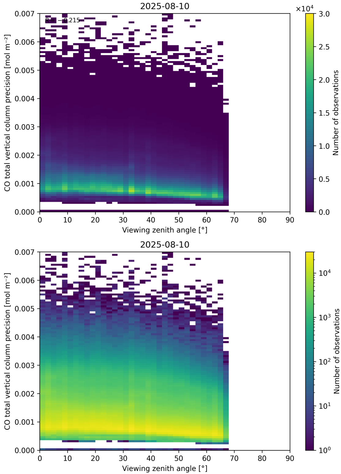
Figure 71: Scatter density plot of “Viewing zenith angle” against “CO total vertical column precision” for 2025-08-09 to 2025-08-11.
