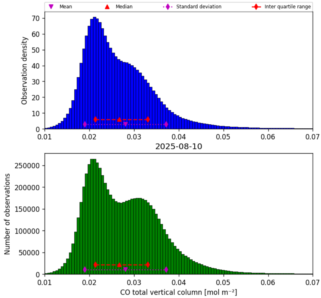
Figure 18: Histogram of “CO total vertical column” for 2025-08-09 to 2025-08-11
