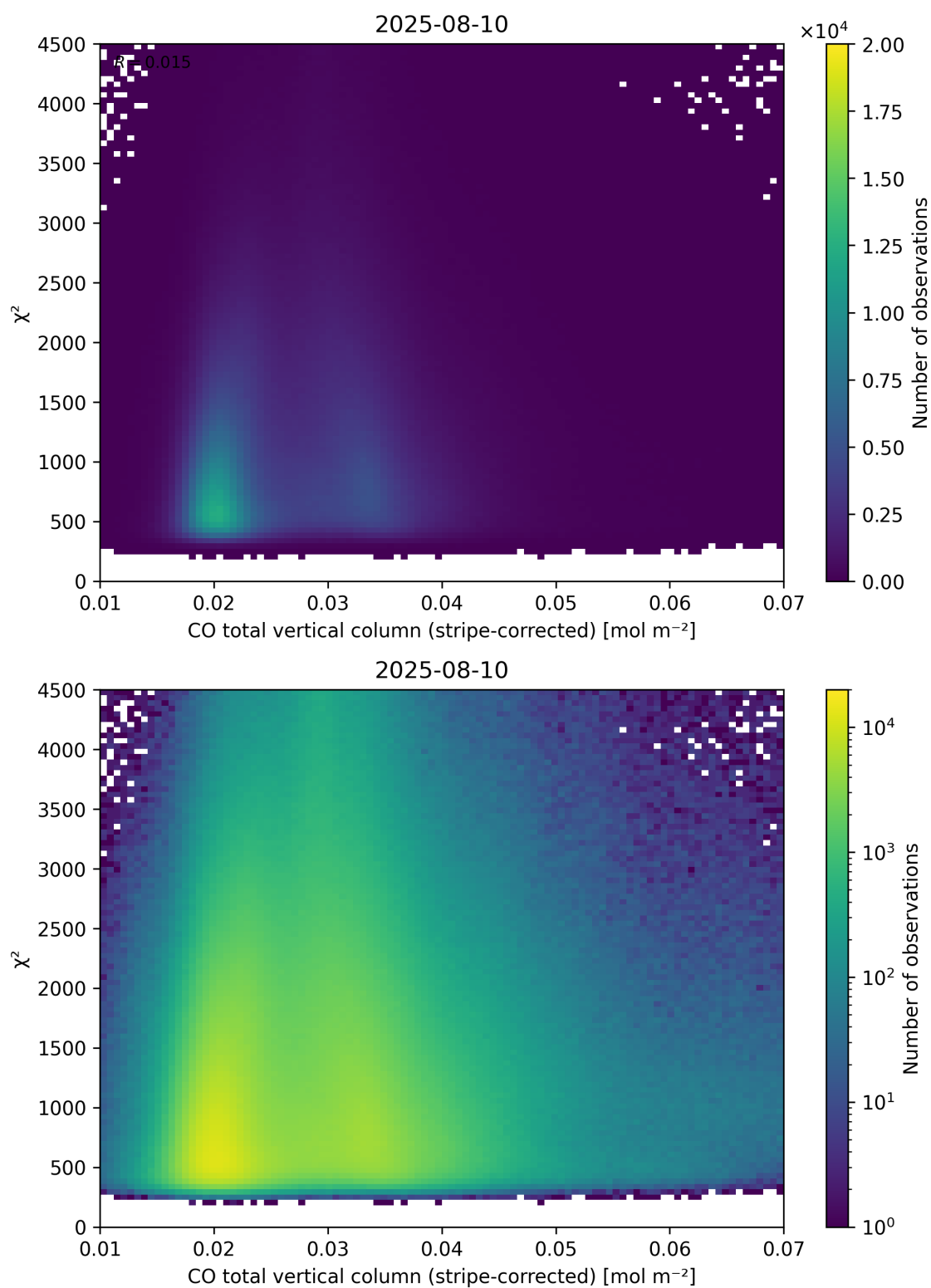
Figure 37: Scatter density plot of “CO total vertical column (stripe-corrected)” against “ \chi^2 ” for 2025-08-09 to 2025-08-11.
