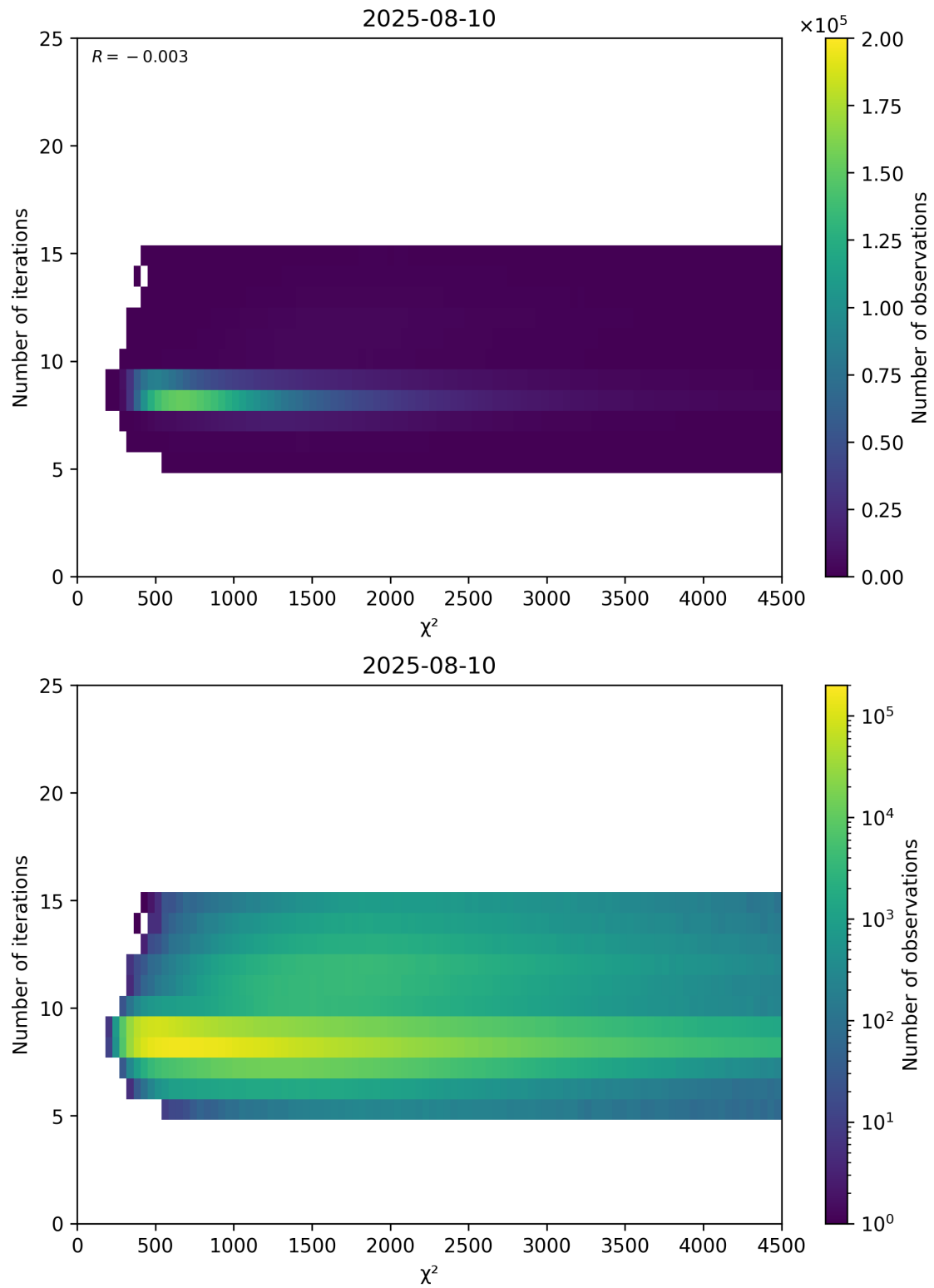
Figure 49: Scatter density plot of “ \chi^2 ” against “Number of iterations” for 2025-08-09 to 2025-08-11.
