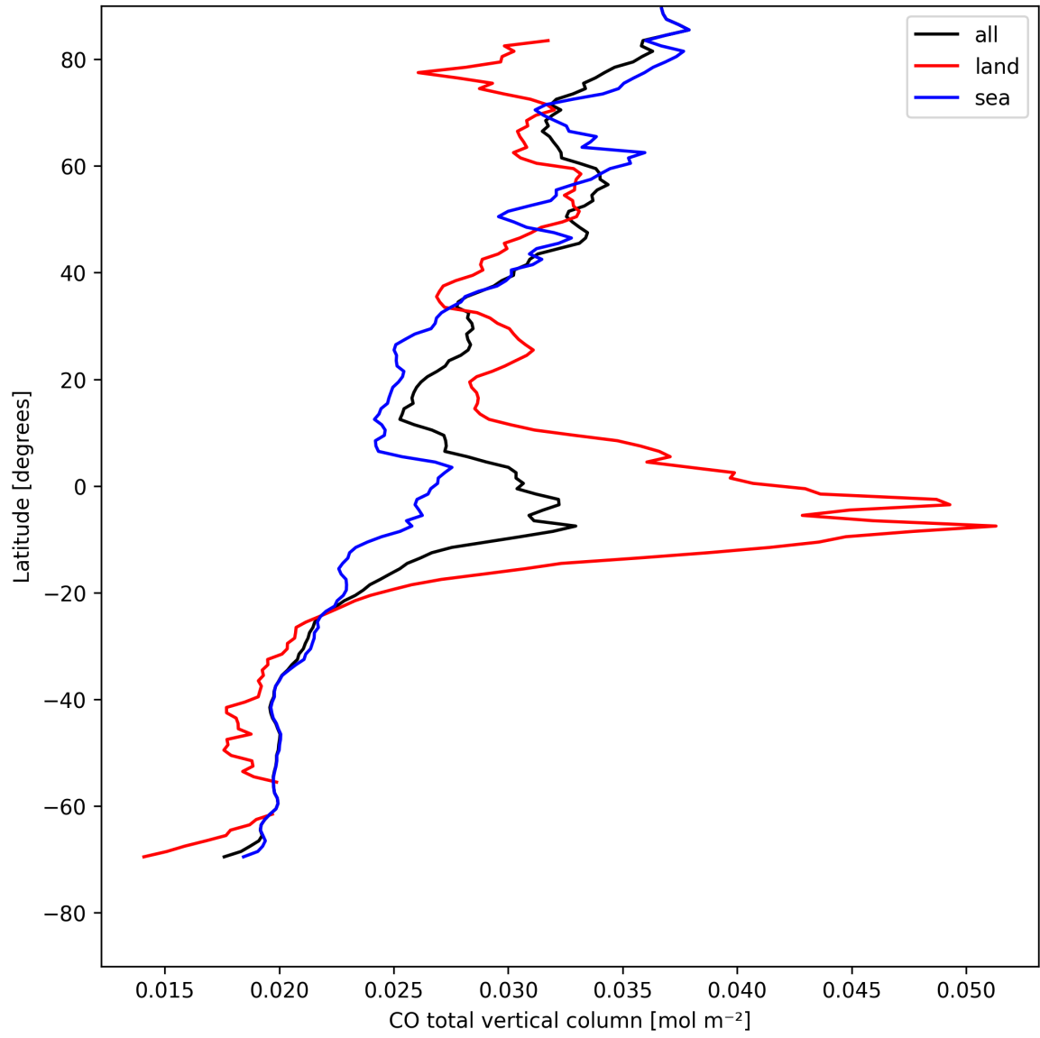
Figure 10: Zonal average of “CO total vertical column” for 2025-08-09 to 2025-08-11.
