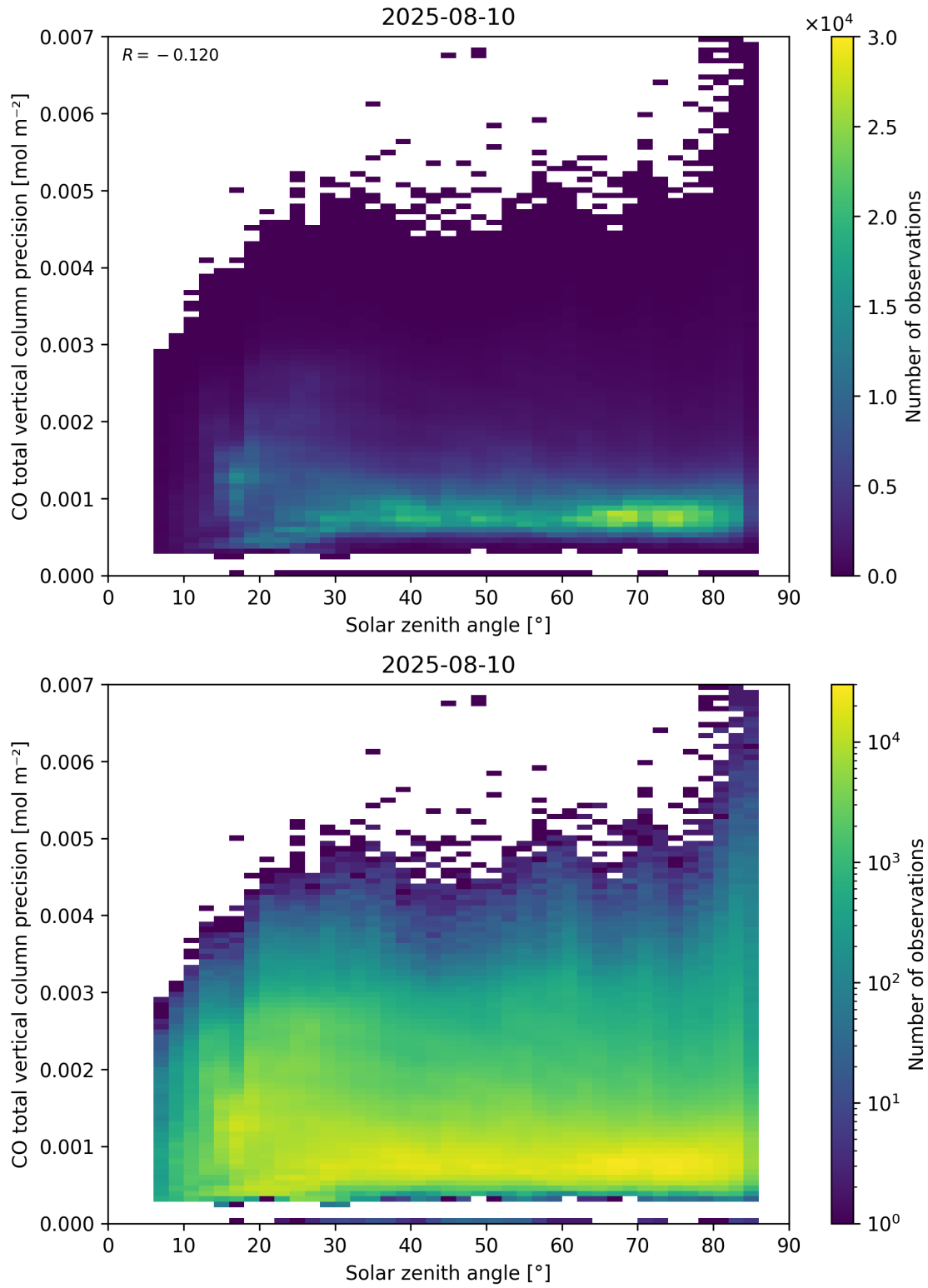
Figure 63: Scatter density plot of “Solar zenith angle” against “CO total vertical column precision” for 2025-08-09 to 2025-08-11.
