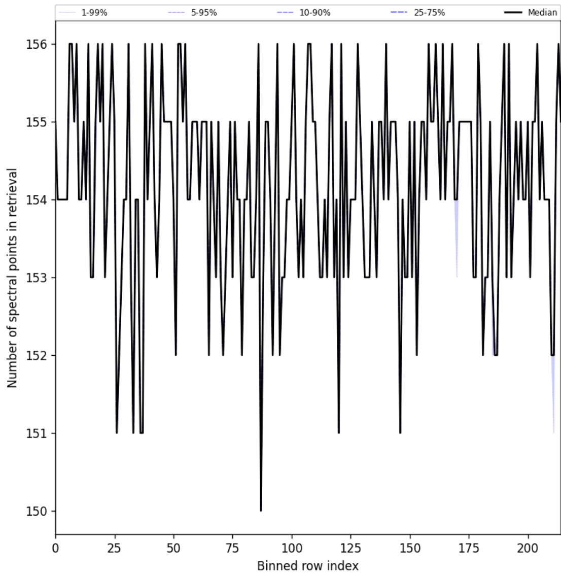
Figure 29: Along track statistics of “Number of spectral points in retrieval” for 2025-08-09 to 2025-08-11
