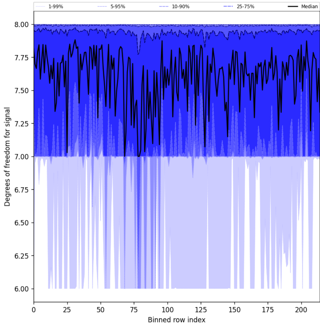
Figure 31: Along track statistics of “Degrees of freedom for signal” for 2025-08-09 to 2025-08-11
