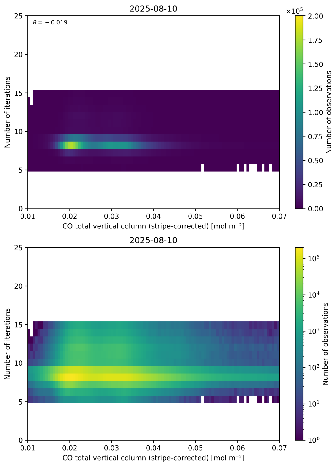
Figure 39: Scatter density plot of “CO total vertical column (stripe-corrected)” against “Number of iterations” for 2025-08-09 to 2025-08-11.
