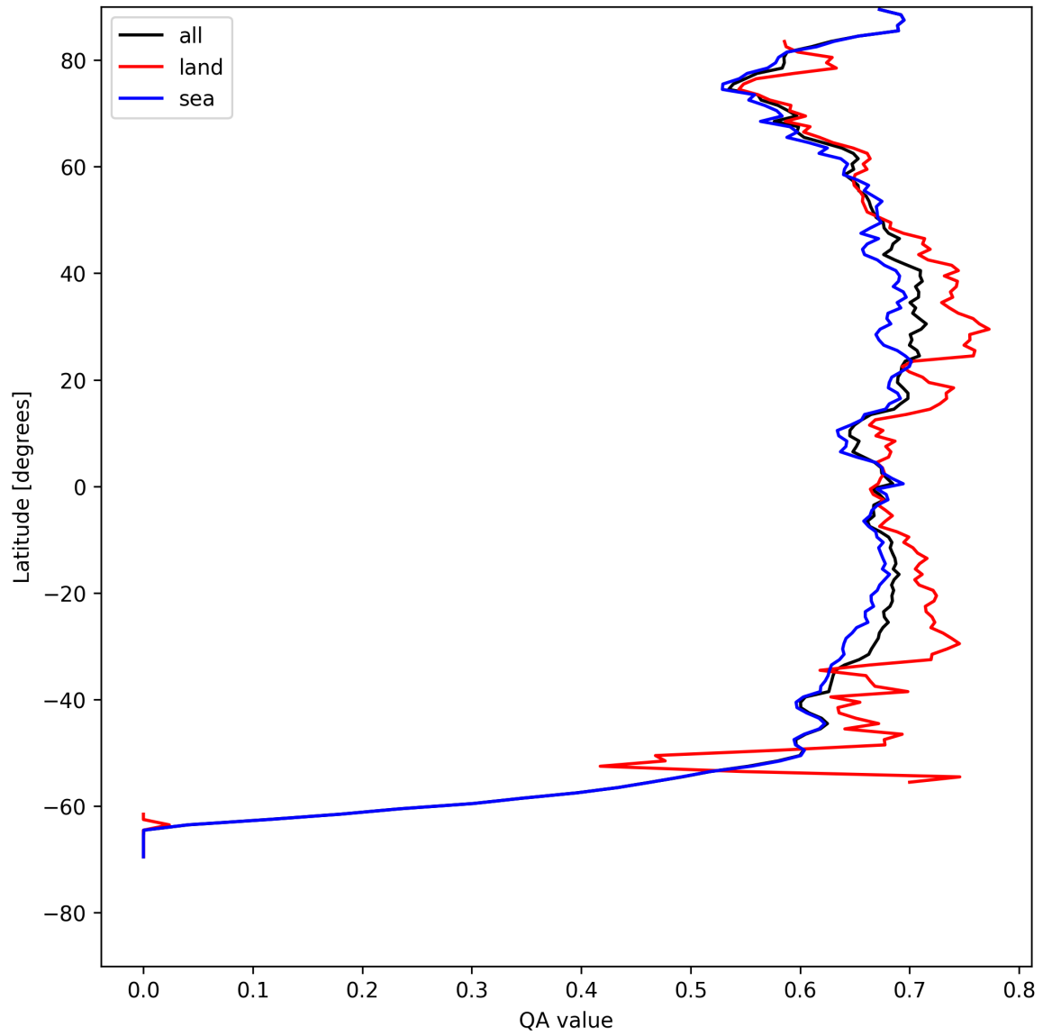
Figure 9: Zonal average of “QA value” for 2025-08-09 to 2025-08-11.
