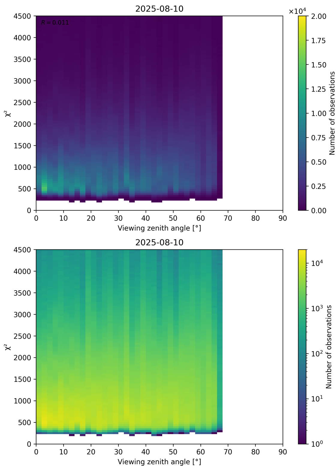
Figure 72: Scatter density plot of “Viewing zenith angle” against “ \chi^2 ” for 2025-08-09 to 2025-08-11.
