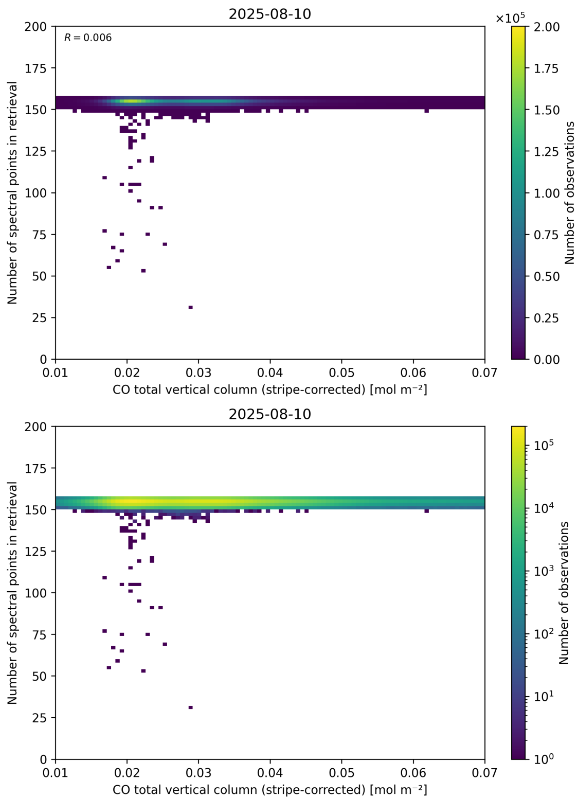
Figure 40: Scatter density plot of “CO total vertical column (stripe-corrected)” against “Number of spectral points in retrieval” for 2025-08-09 to 2025-08-11.
