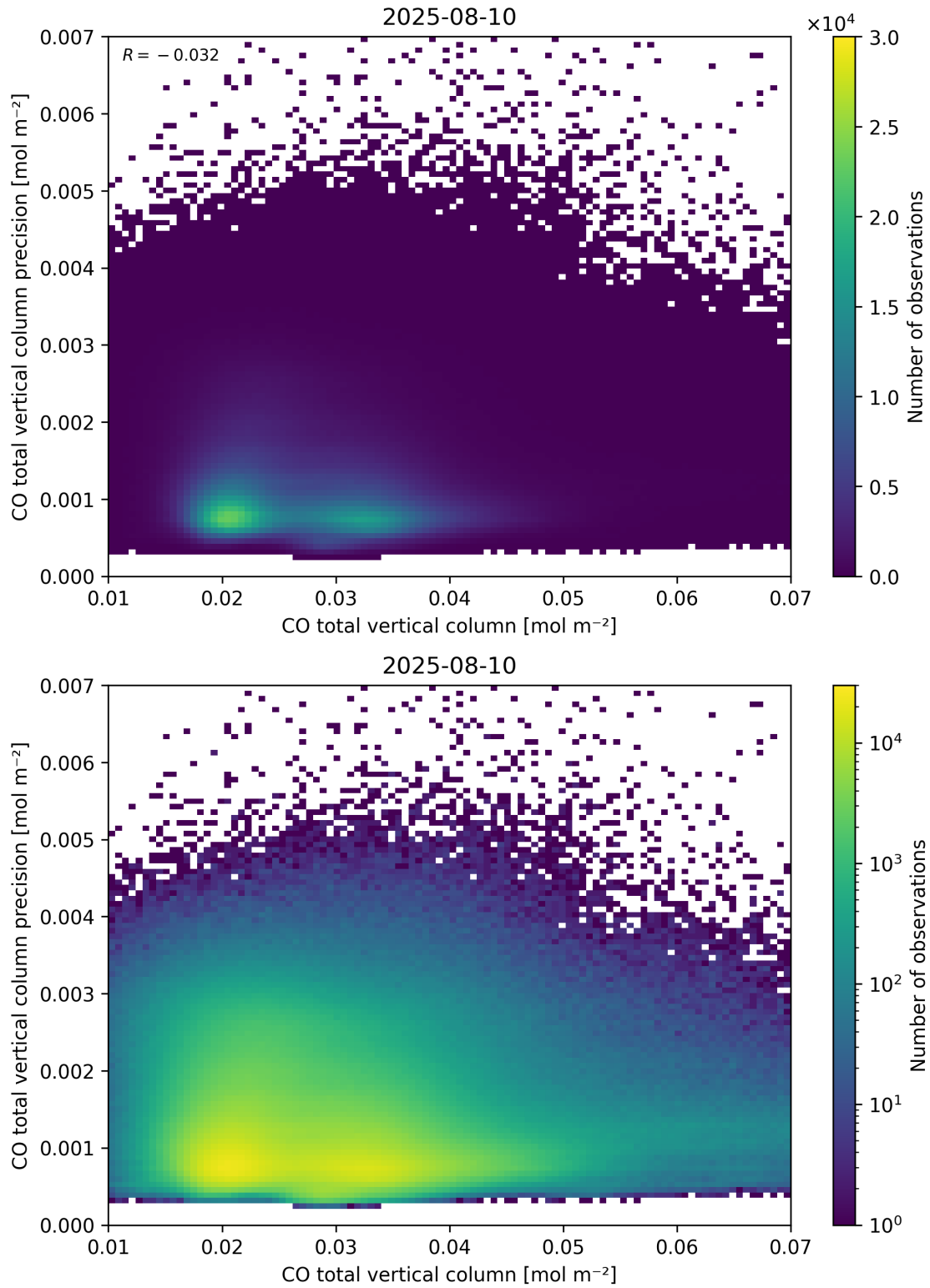
Figure 34: Scatter density plot of “CO total vertical column” against “CO total vertical column precision” for 2025-08-09 to 2025-08-11.
