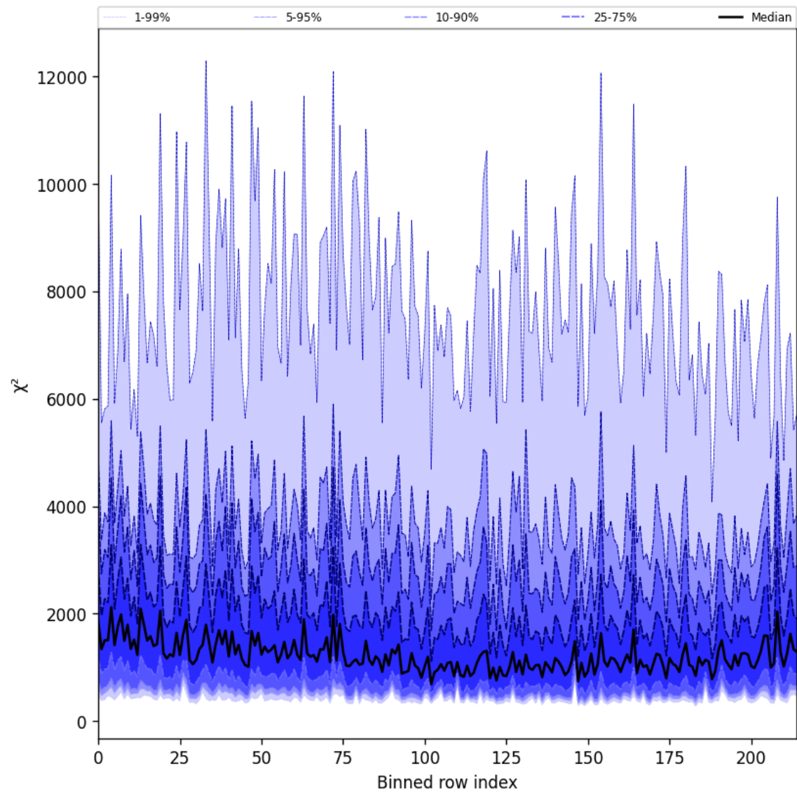
Figure 30: Along track statistics of “ \chi^2 ” for 2025-08-09 to 2025-08-11
