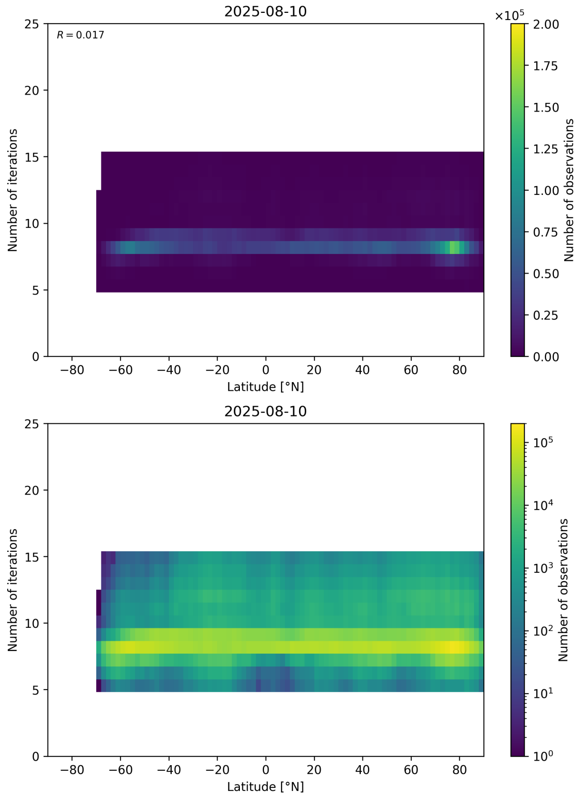
Figure 56: Scatter density plot of “Latitude” against “Number of iterations” for 2025-08-09 to 2025-08-11.
