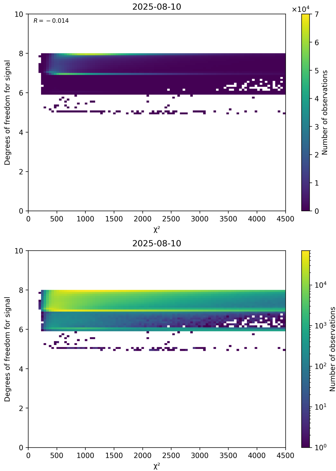
Figure 48: Scatter density plot of " \chi^2 " against "Degrees of freedom for signal" for 2025-08-09 to 2025-08-11.
