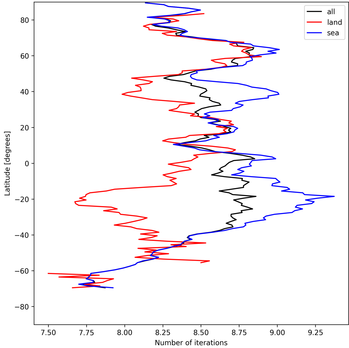
Figure 16: Zonal average of “Number of iterations” for 2025-08-09 to 2025-08-11.
