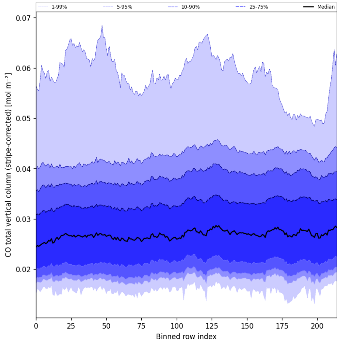
Figure 27: Along track statistics of “CO total vertical column (stripe-corrected)” for 2025-08-09 to 2025-08-11
