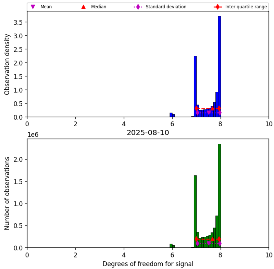
Figure 23: Histogram of “Degrees of freedom for signal” for 2025-08-09 to 2025-08-11
