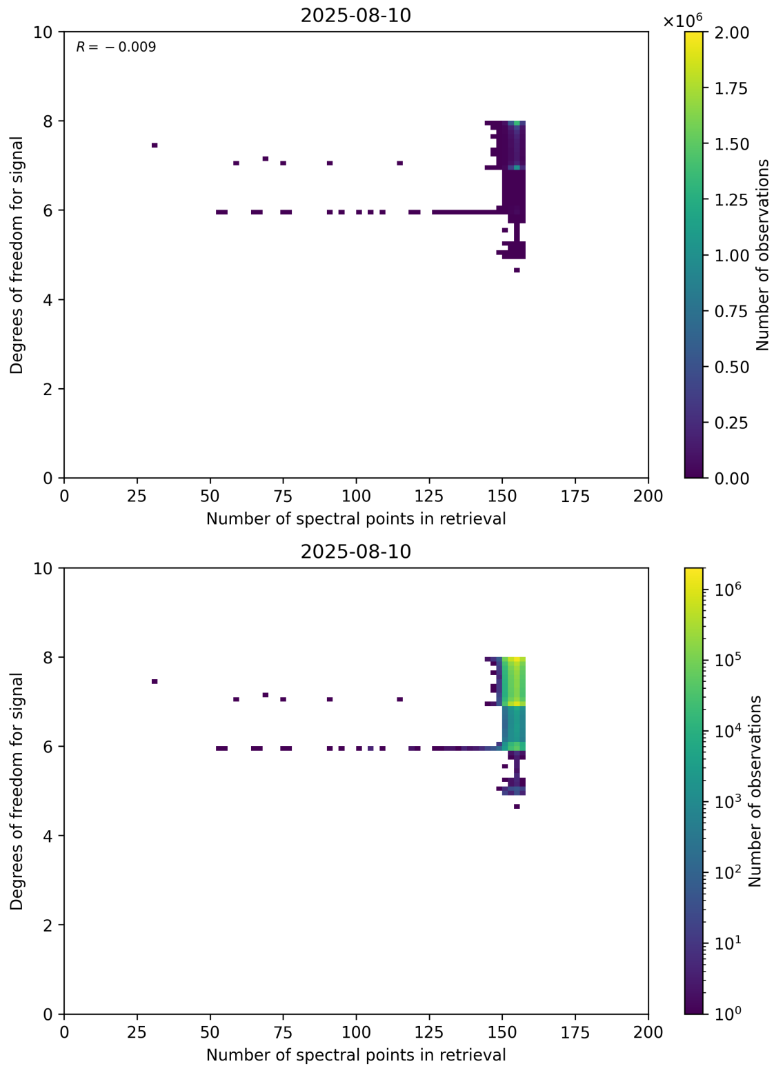
Figure 59: Scatter density plot of “Number of spectral points in retrieval” against “Degrees of freedom for signal” for 2025-08-09 to 2025-08-11.
