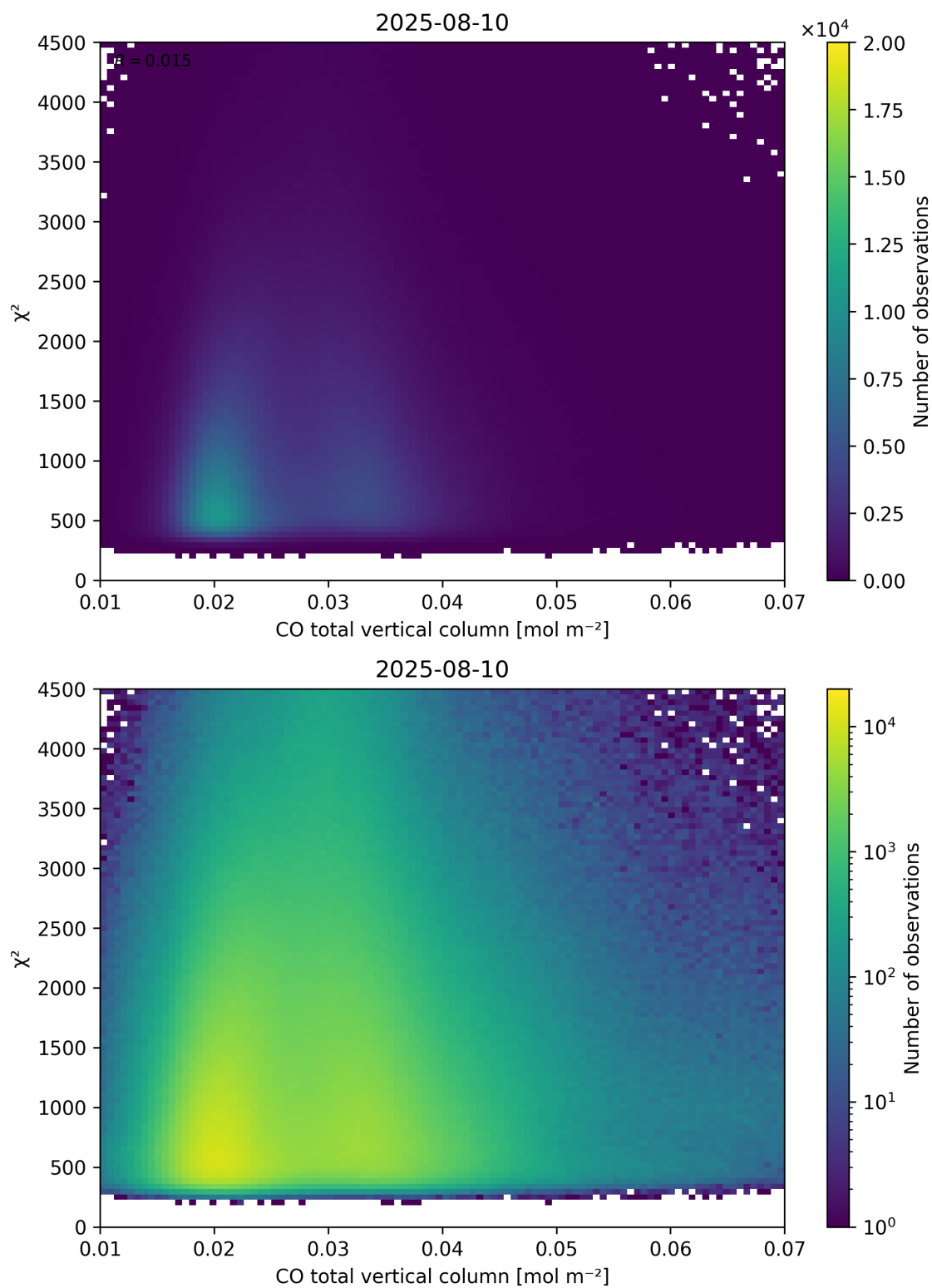
Figure 35: Scatter density plot of “CO total vertical column” against “ \chi^2 ” for 2025-08-09 to 2025-08-11.
