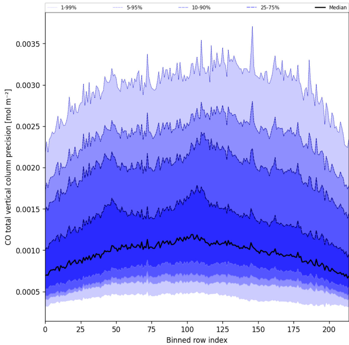
Figure 28: Along track statistics of “CO total vertical column precision” for 2025-08-09 to 2025-08-11
