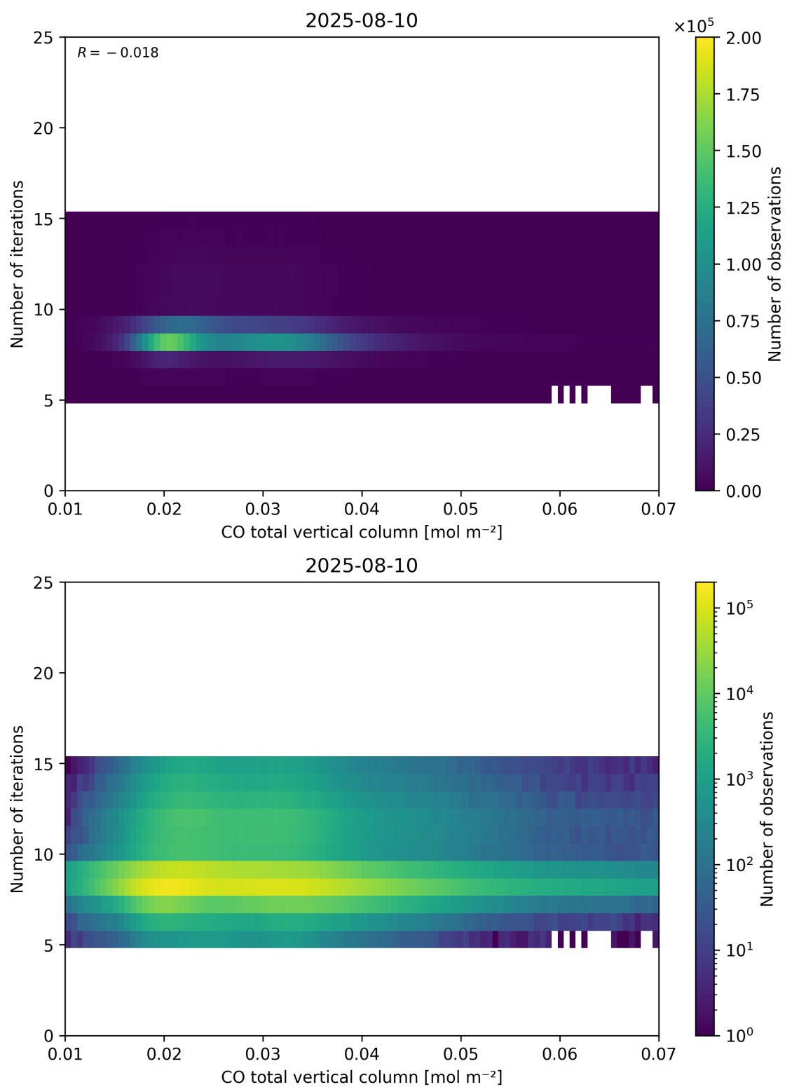
Figure 42: Scatter density plot of “CO total vertical column” against “Number of iterations” for 2025-08-09 to 2025-08-11.
