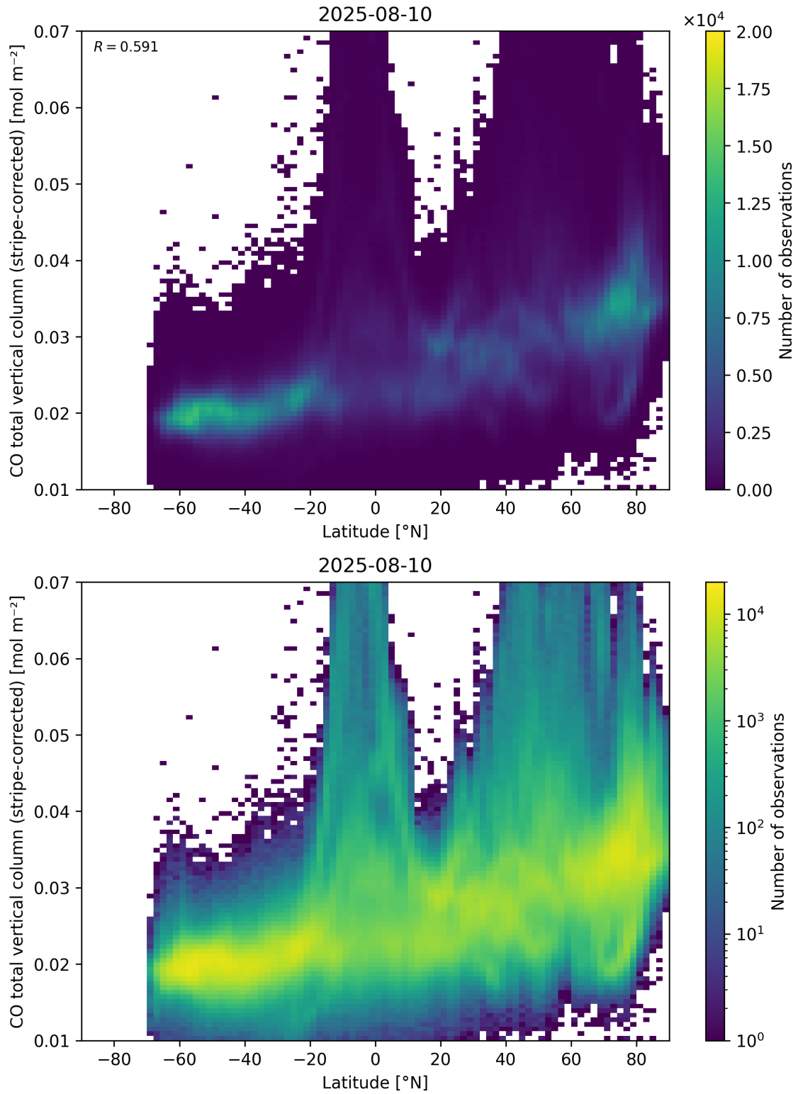
Figure 52: Scatter density plot of “Latitude” against “CO total vertical column (stripe-corrected)” for 2025-08-09 to 2025-08-11.
