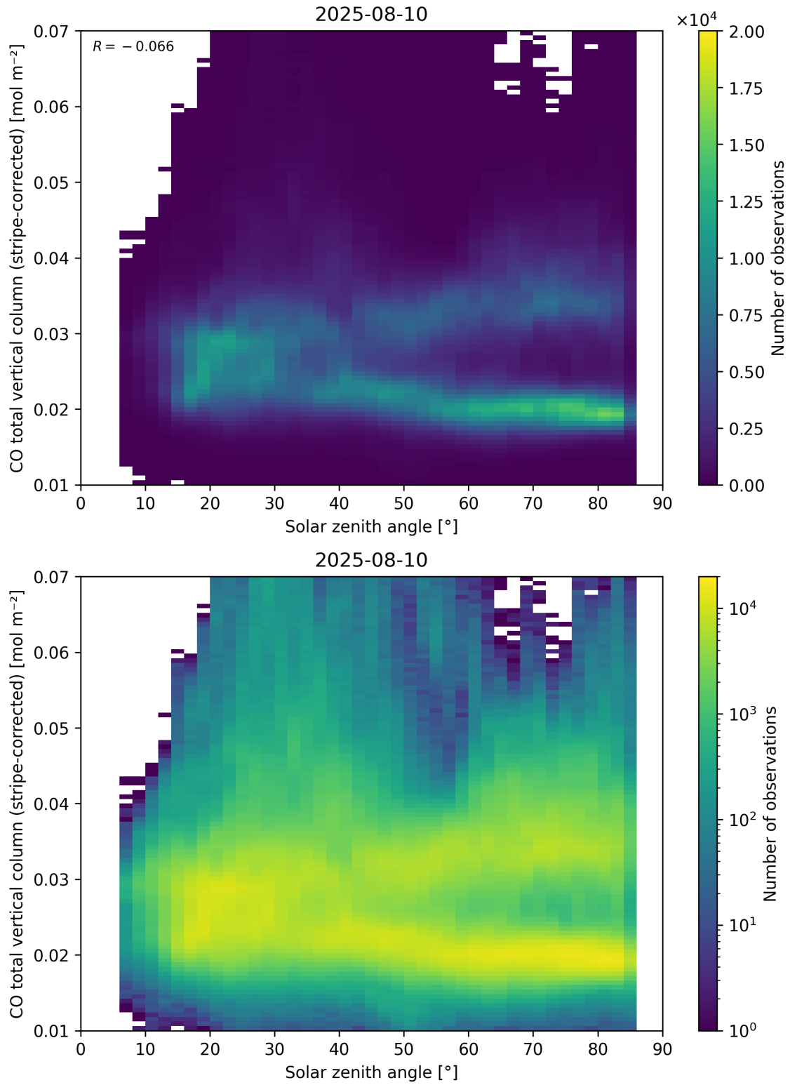
Figure 62: Scatter density plot of “Solar zenith angle” against “CO total vertical column (stripe-corrected)” for 2025-08-09 to 2025-08-11.
