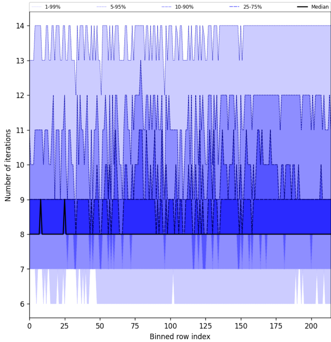
Figure 32: Along track statistics of “Number of iterations” for 2025-08-09 to 2025-08-11
