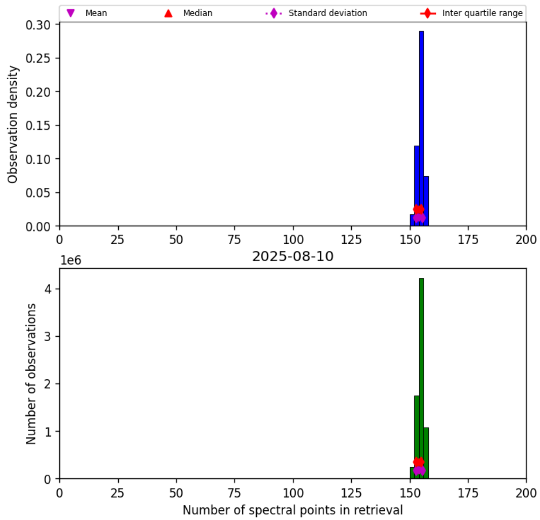
Figure 21: Histogram of “Number of spectral points in retrieval” for 2025-08-09 to 2025-08-11
