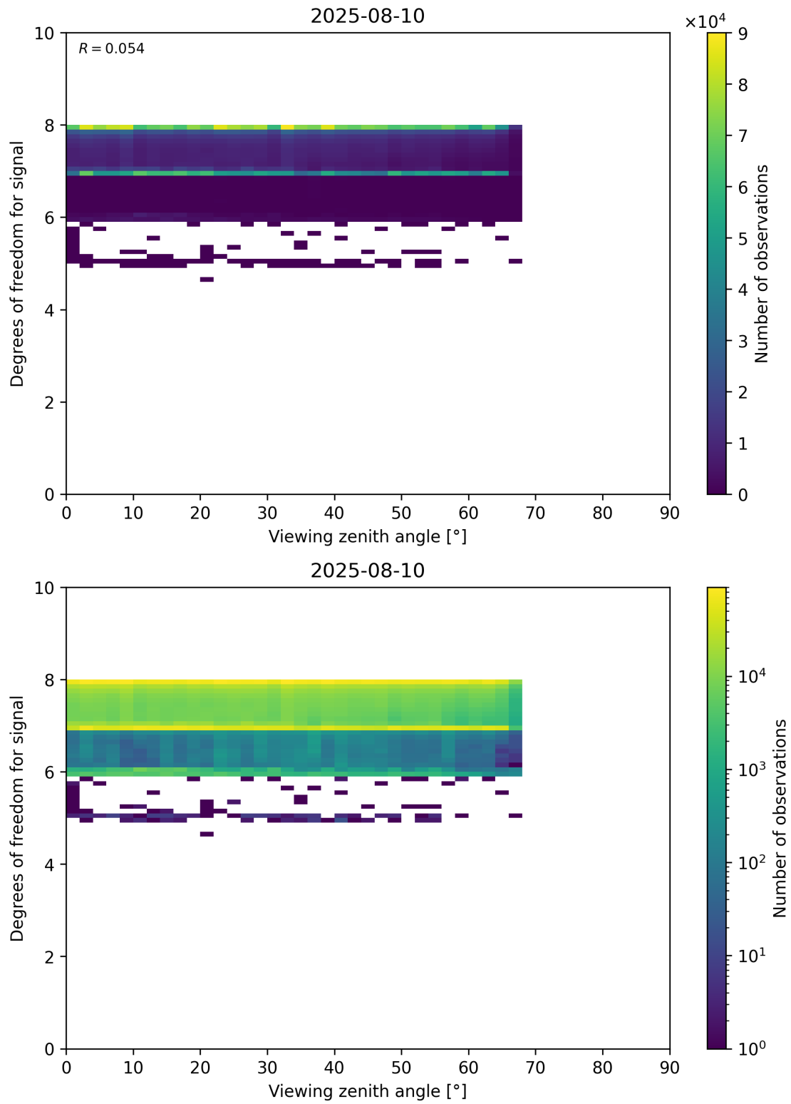
Figure 73: Scatter density plot of “Viewing zenith angle” against “Degrees of freedom for signal” for 2025-08-09 to 2025-08-11.
