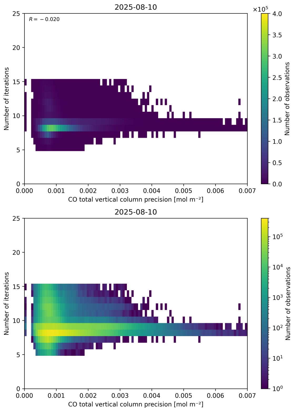
Figure 46: Scatter density plot of “CO total vertical column precision” against “Number of iterations” for 2025-08-09 to 2025-08-11.
