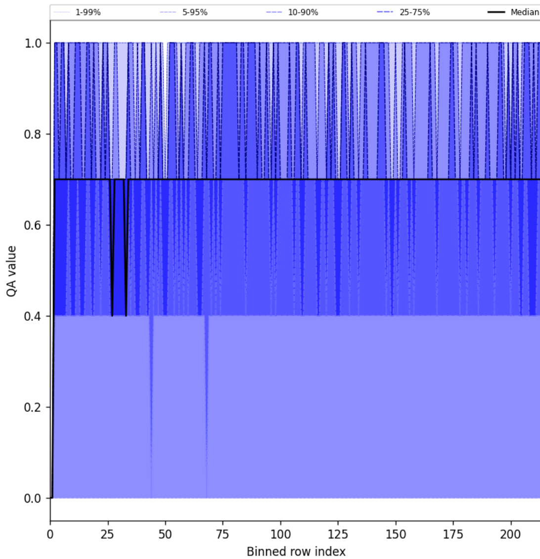
Figure 25: Along track statistics of “QA value” for 2025-08-09 to 2025-08-11
