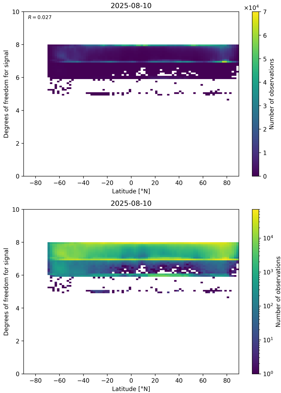
Figure 55: Scatter density plot of “Latitude” against “Degrees of freedom for signal” for 2025-08-09 to 2025-08-11.
