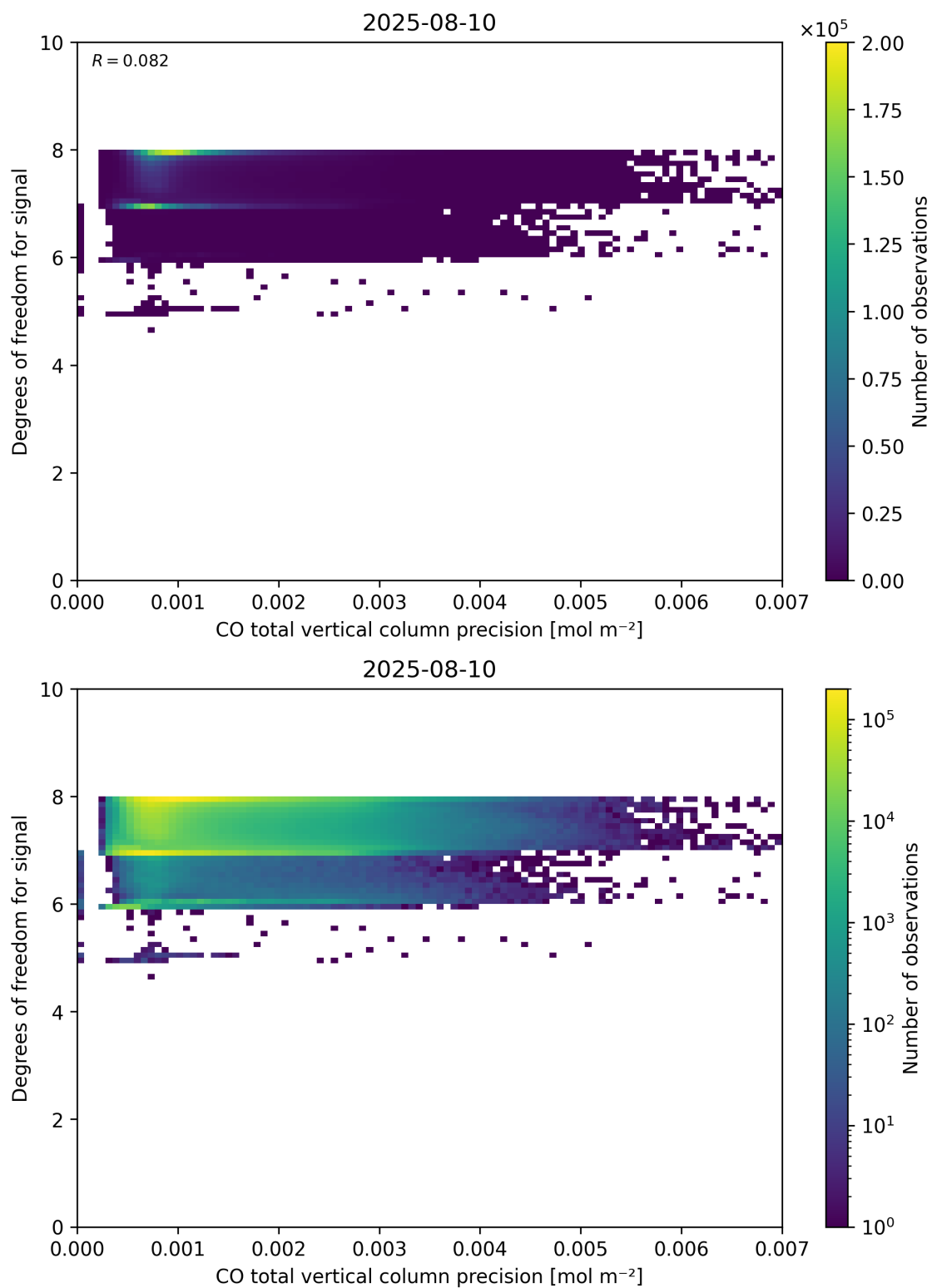
Figure 45: Scatter density plot of “CO total vertical column precision” against “Degrees of freedom for signal” for 2025-08-09 to 2025-08-11.
