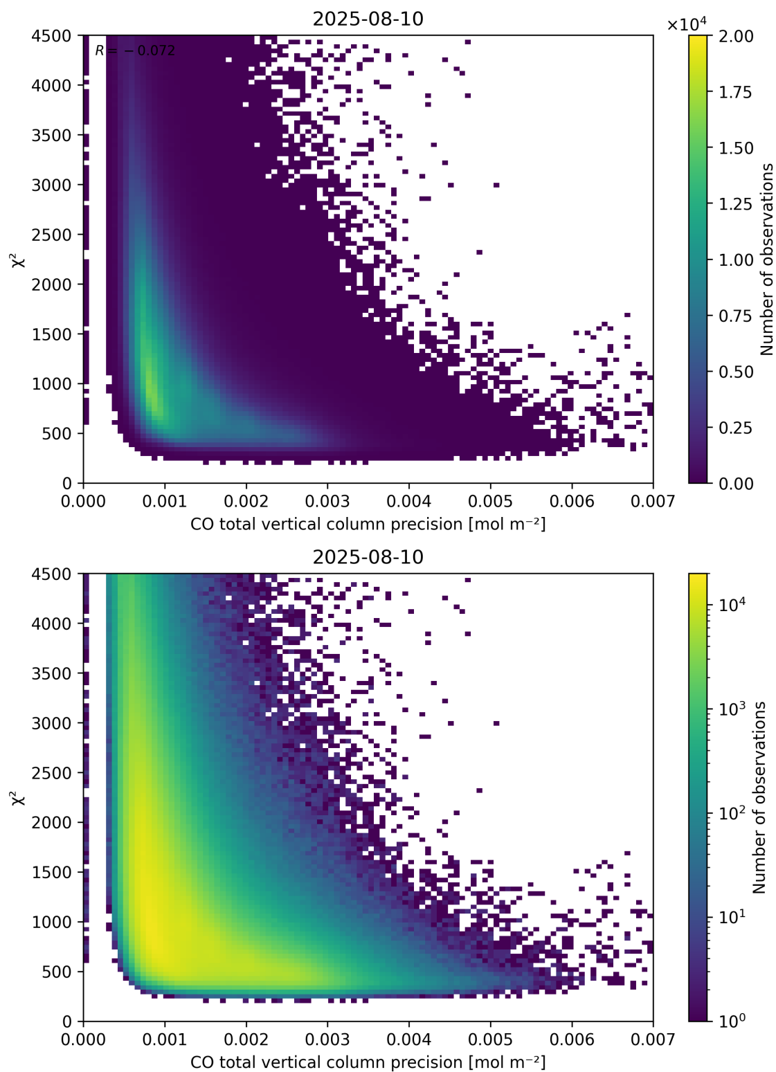
Figure 44: Scatter density plot of “CO total vertical column precision” against “ \chi^2 ” for 2025-08-09 to 2025-08-11.
