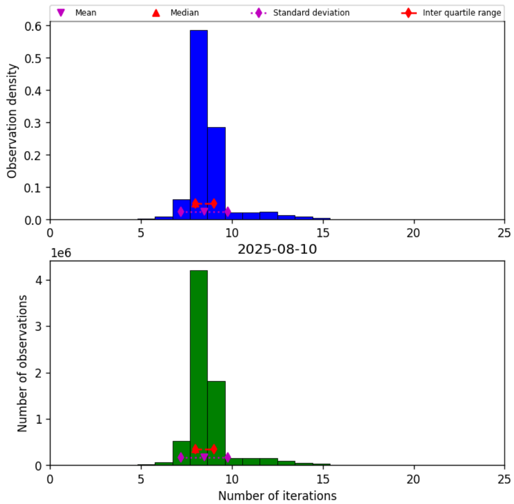
Figure 24: Histogram of “Number of iterations” for 2025-08-09 to 2025-08-11
