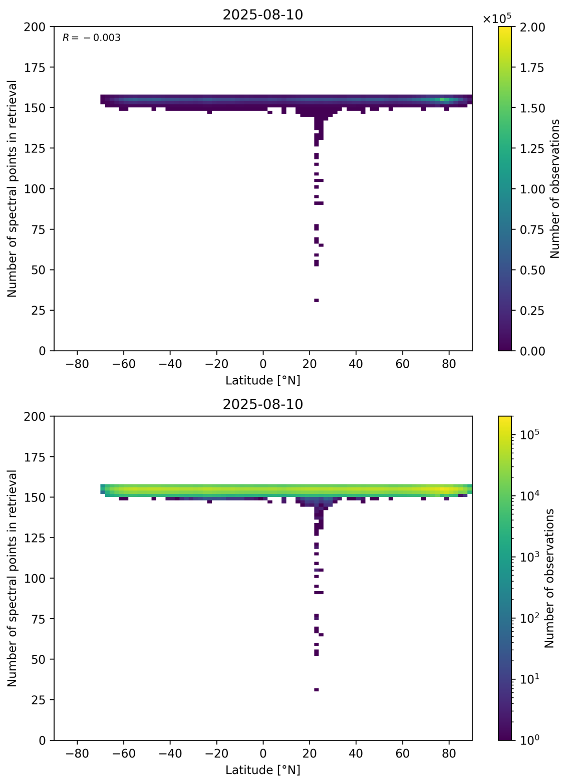
Figure 57: Scatter density plot of “Latitude” against “Number of spectral points in retrieval” for 2025-08-09 to 2025-08-11.
