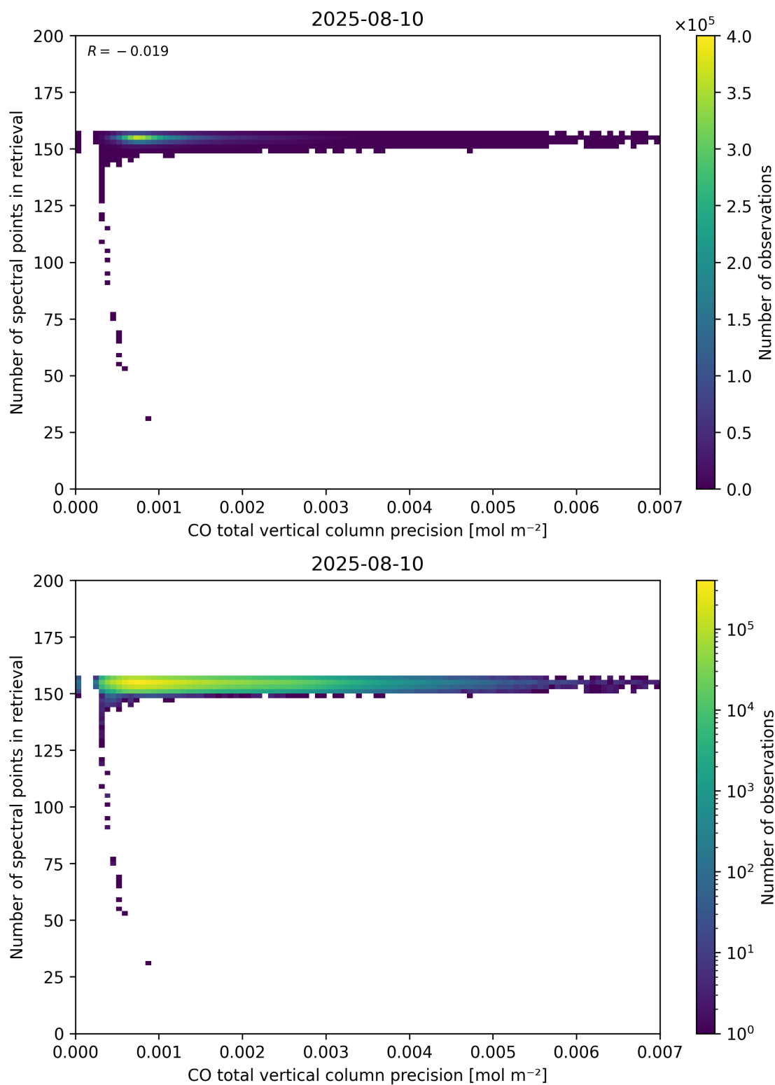
Figure 47: Scatter density plot of “CO total vertical column precision” against “Number of spectral points in retrieval” for 2025-08-09 to 2025-08-11.
