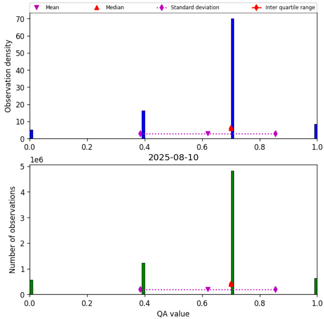
Figure 17: Histogram of “QA value” for 2025-08-09 to 2025-08-11
