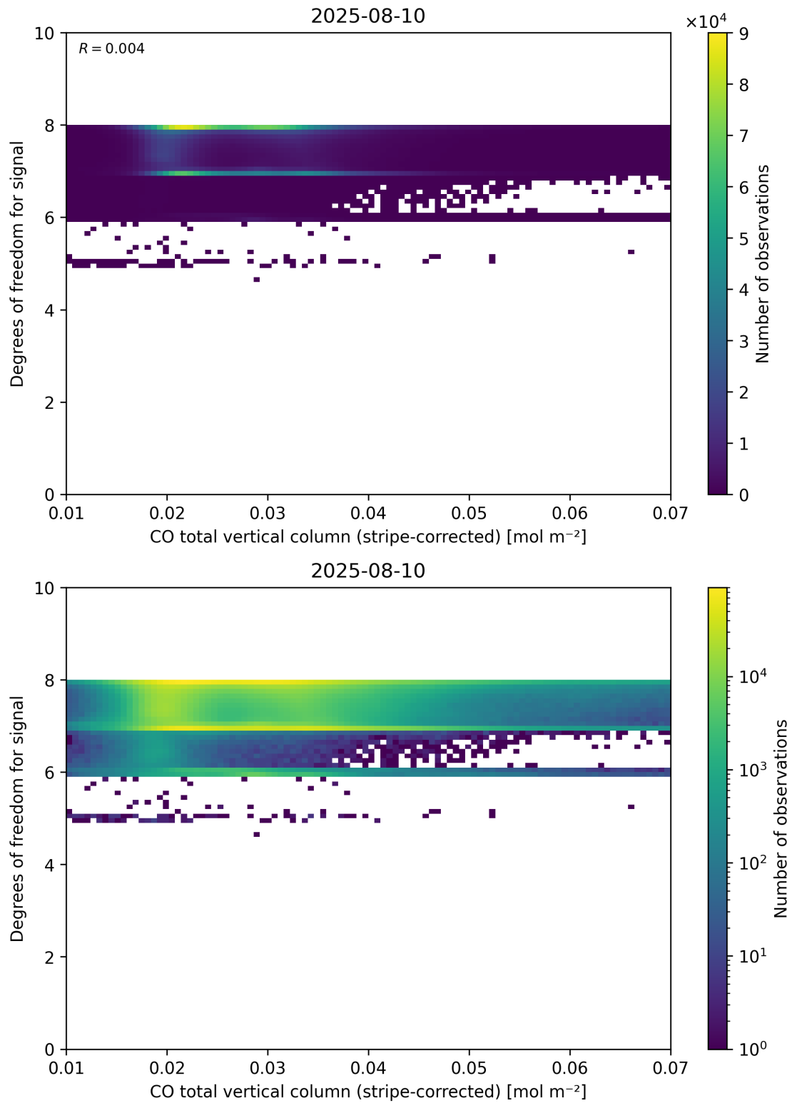
Figure 38: Scatter density plot of “CO total vertical column (stripe-corrected)” against “Degrees of freedom for signal” for 2025-08-09 to 2025-08-11.
