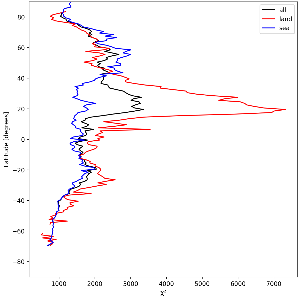
Figure 14: Zonal average of “ \chi^2 ” for 2025-08-09 to 2025-08-11.
