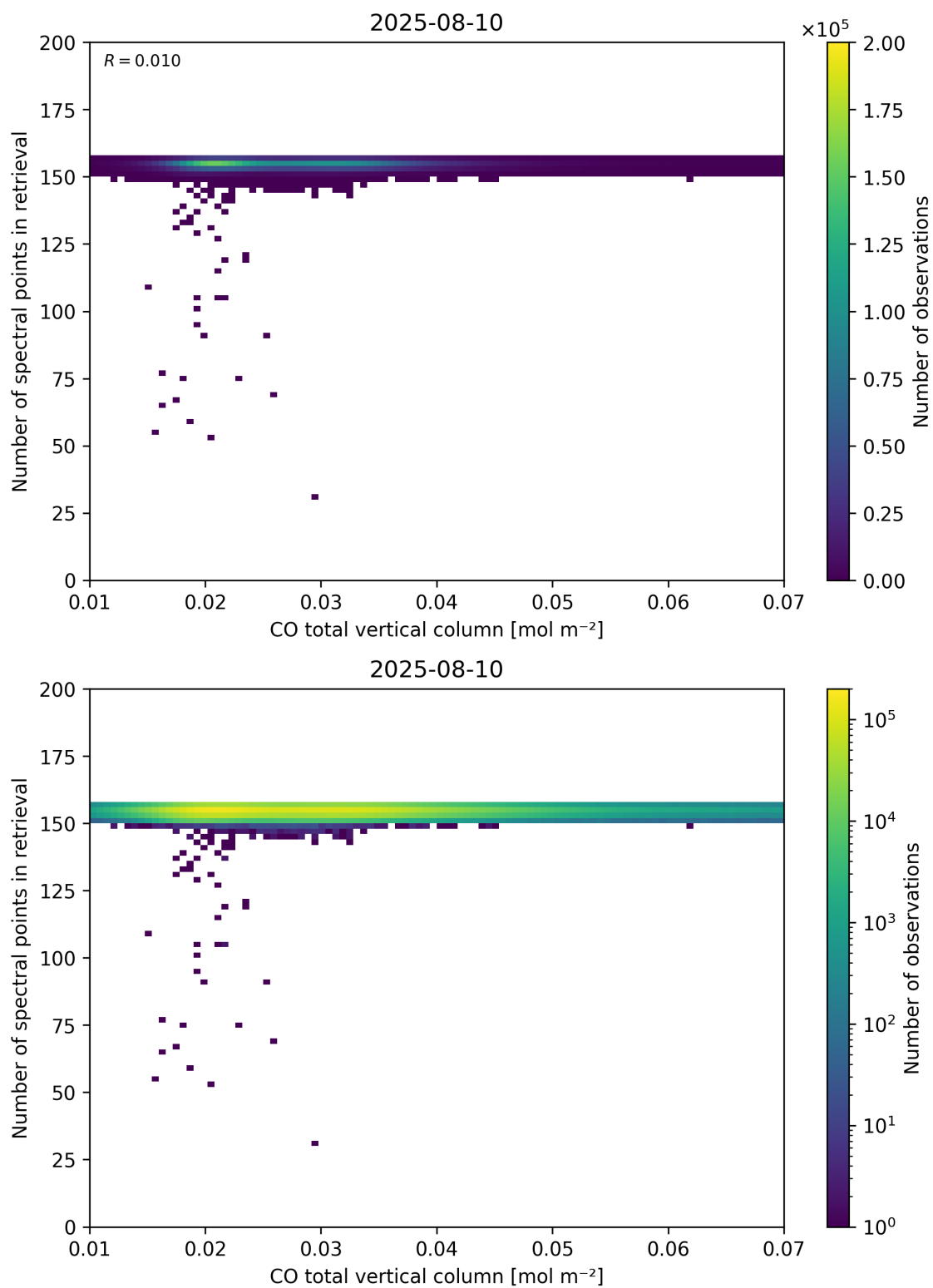
Figure 43: Scatter density plot of “CO total vertical column” against “Number of spectral points in retrieval” for 2025-08-09 to 2025-08-11.
