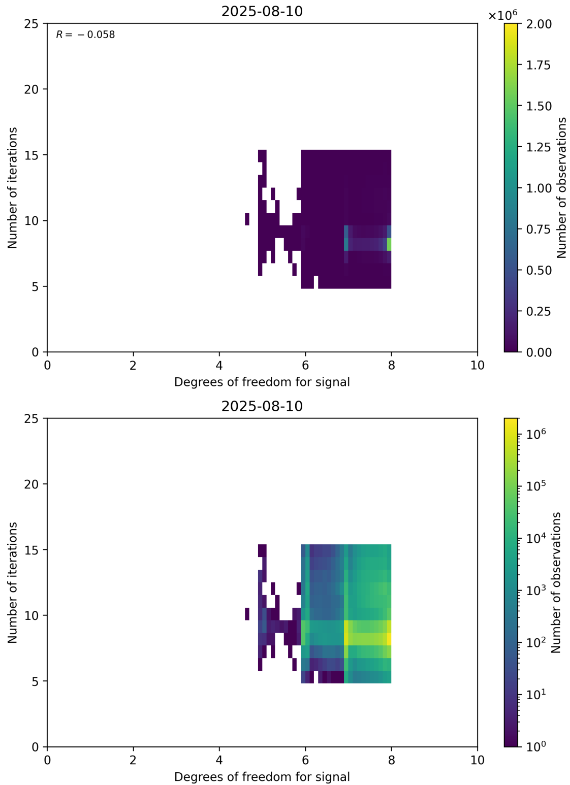
Figure 50: Scatter density plot of “Degrees of freedom for signal” against “Number of iterations” for 2025-08-09 to 2025-08-11.
