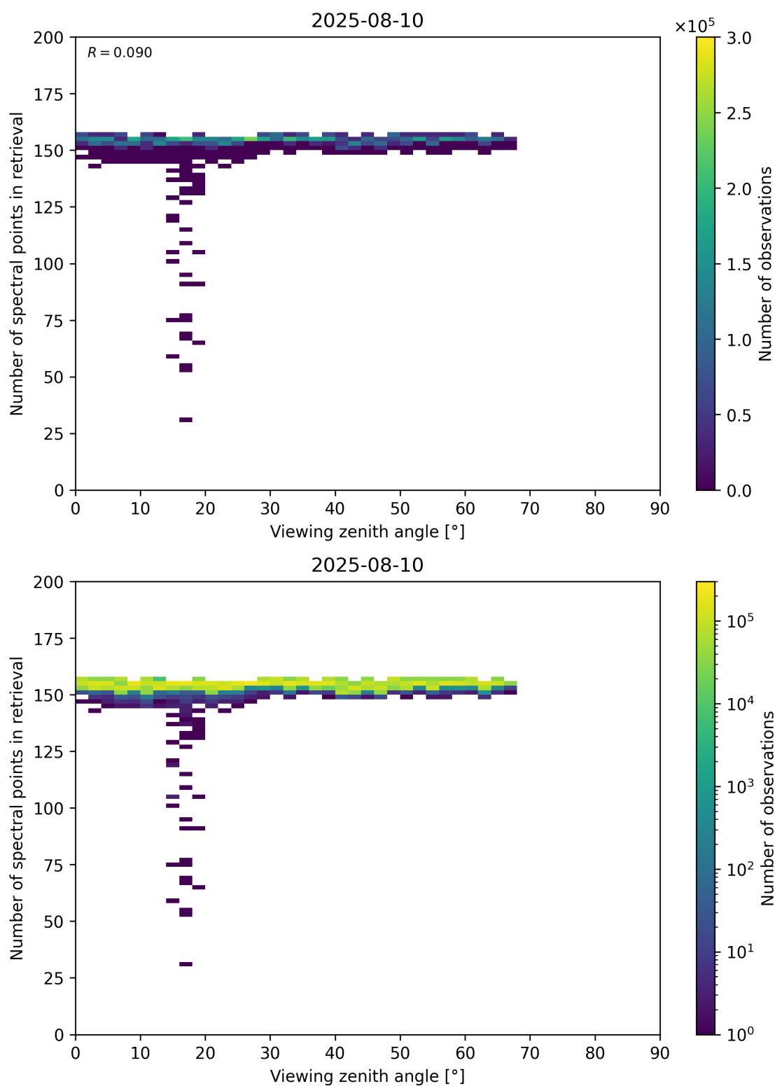
Figure 76: Scatter density plot of “Viewing zenith angle” against “Number of spectral points in retrieval” for 2025-08-09 to 2025-08-11.
