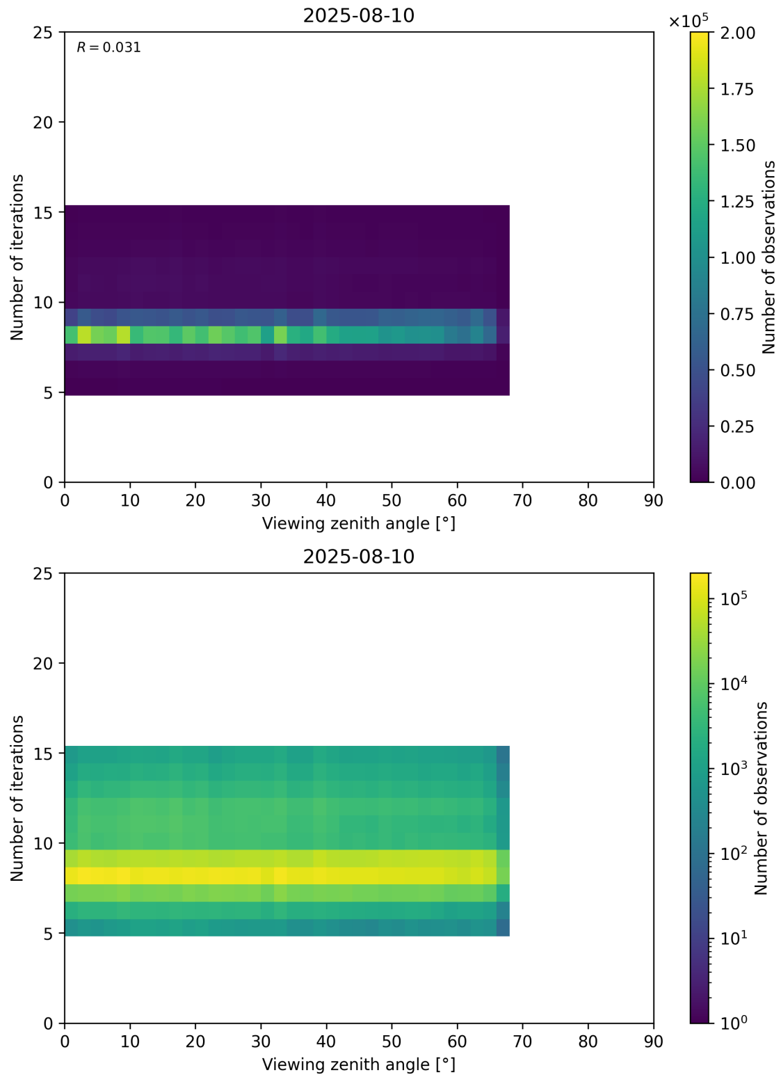
Figure 75: Scatter density plot of “Viewing zenith angle” against “Number of iterations” for 2025-08-09 to 2025-08-11.
