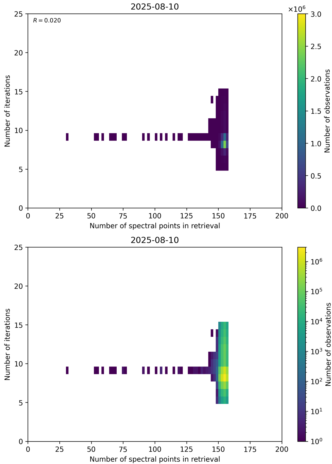
Figure 60: Scatter density plot of “Number of spectral points in retrieval” against “Number of iterations” for 2025-08-09 to 2025-08-11.
