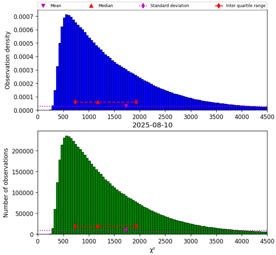
Figure 22: Histogram of “ \chi^2 ” for 2025-08-09 to 2025-08-11
