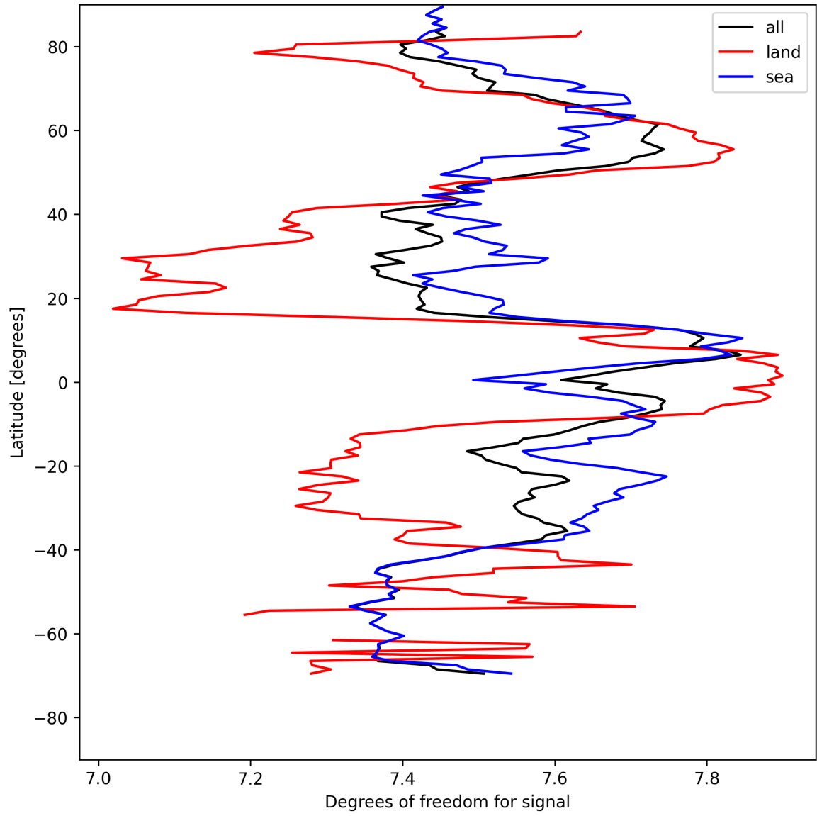
Figure 15: Zonal average of “Degrees of freedom for signal” for 2025-08-09 to 2025-08-11.
