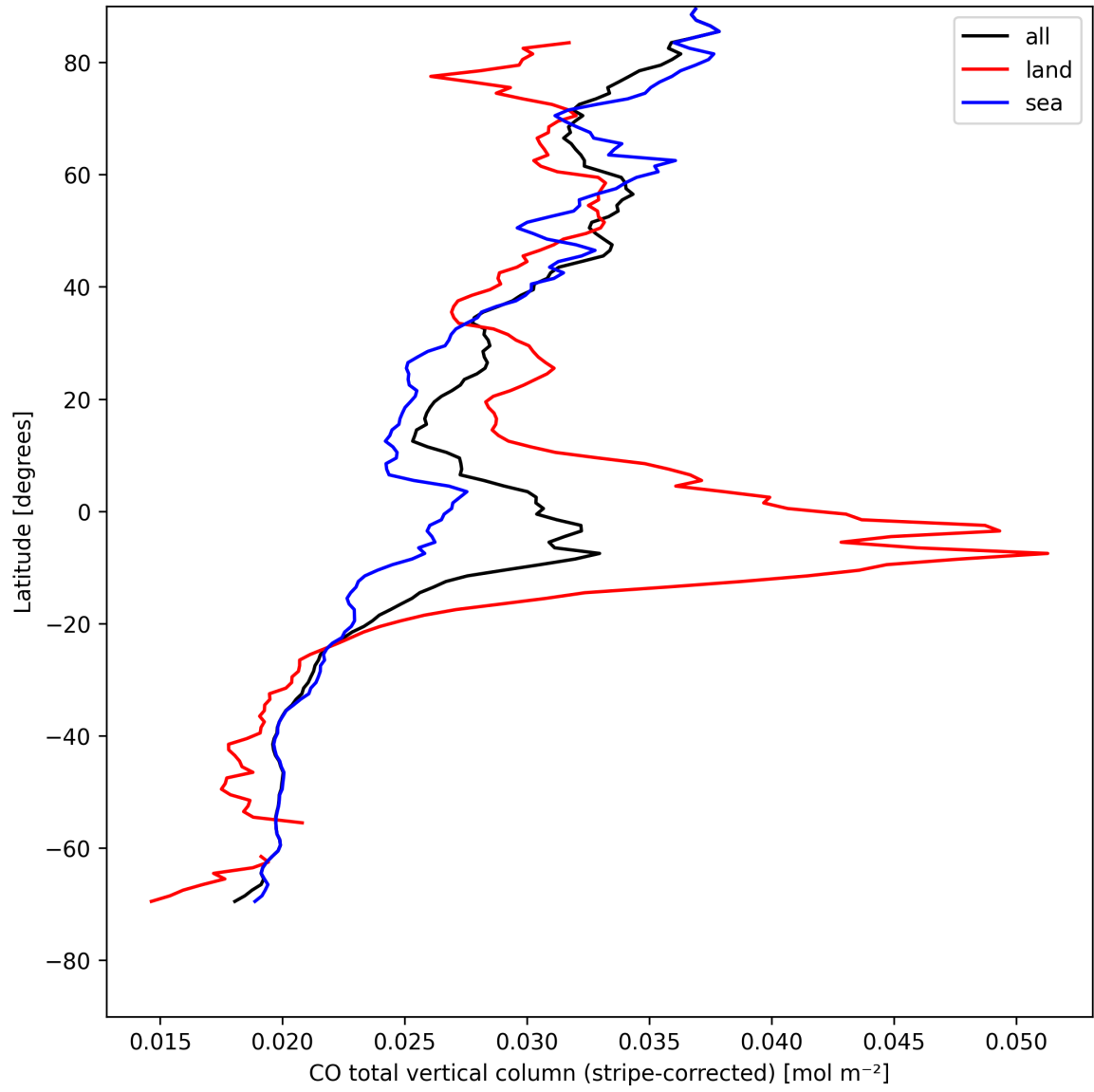
Figure 11: Zonal average of “CO total vertical column (stripe-corrected)” for 2025-08-09 to 2025-08-11.
