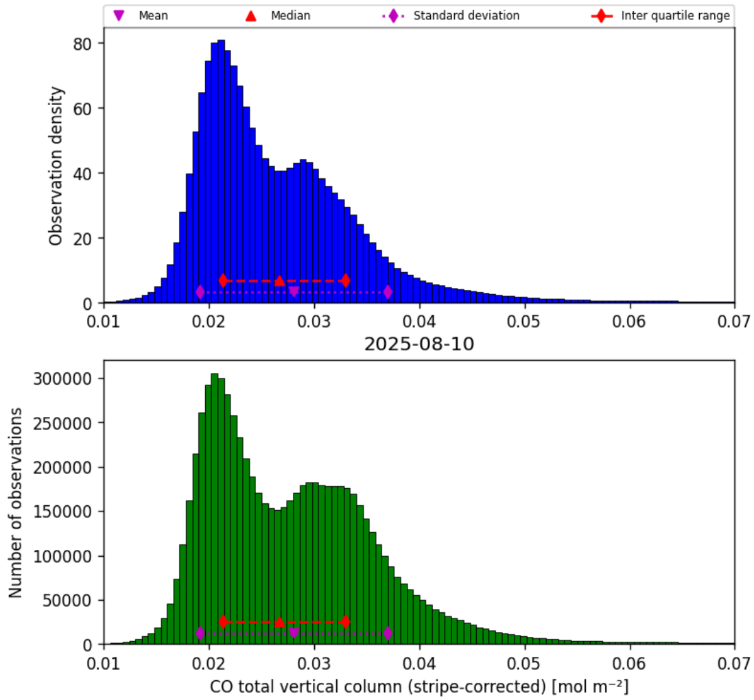
Figure 19: Histogram of “CO total vertical column (stripe-corrected)” for 2025-08-09 to 2025-08-11
