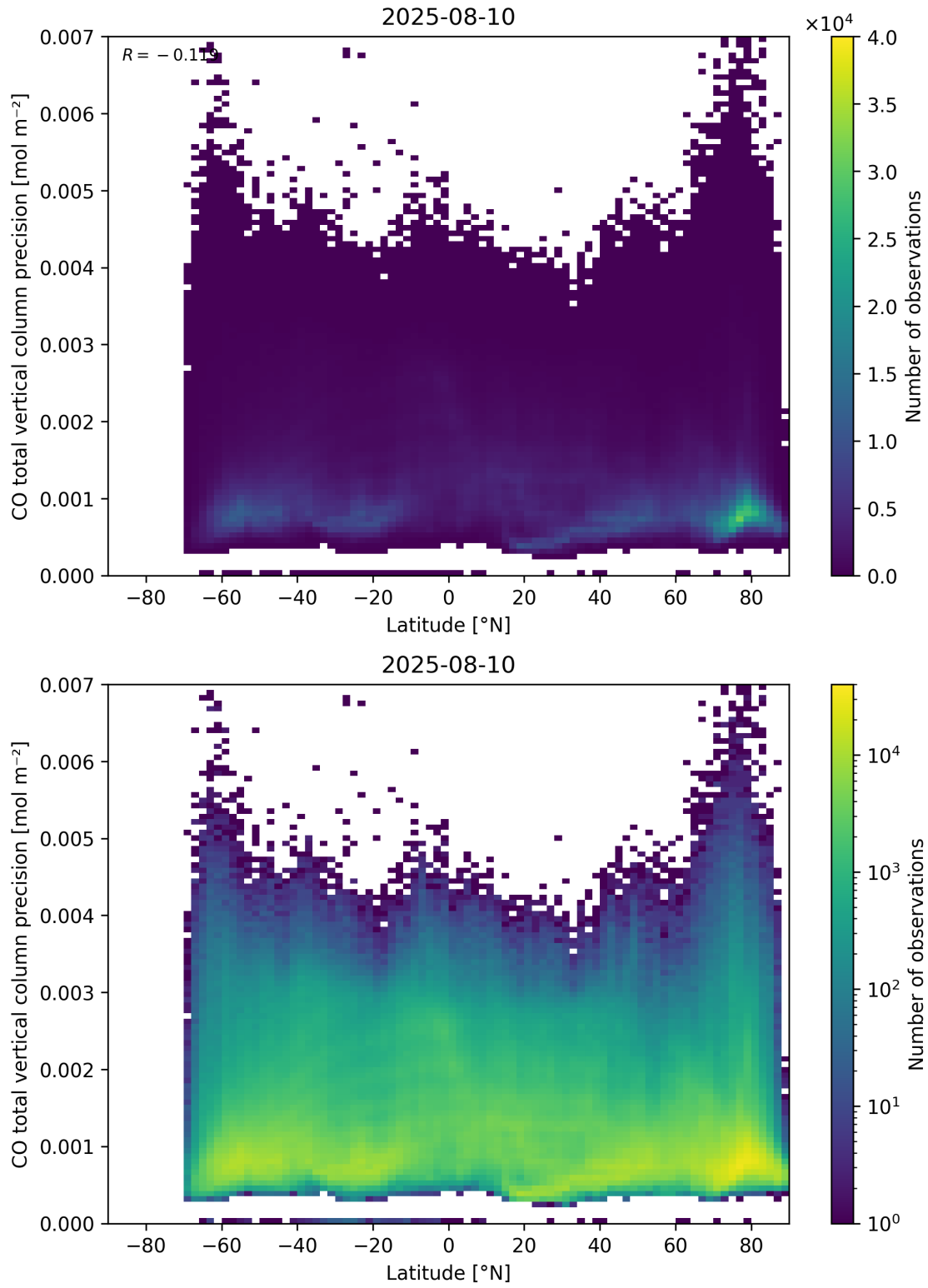
Figure 53: Scatter density plot of “Latitude” against “CO total vertical column precision” for 2025-08-09 to 2025-08-11.
