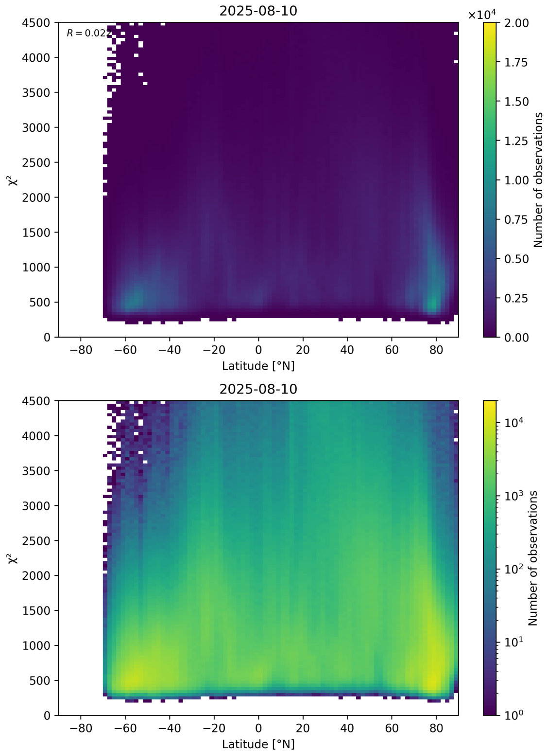
Figure 54: Scatter density plot of “Latitude” against “ \chi^2 ” for 2025-08-09 to 2025-08-11.
