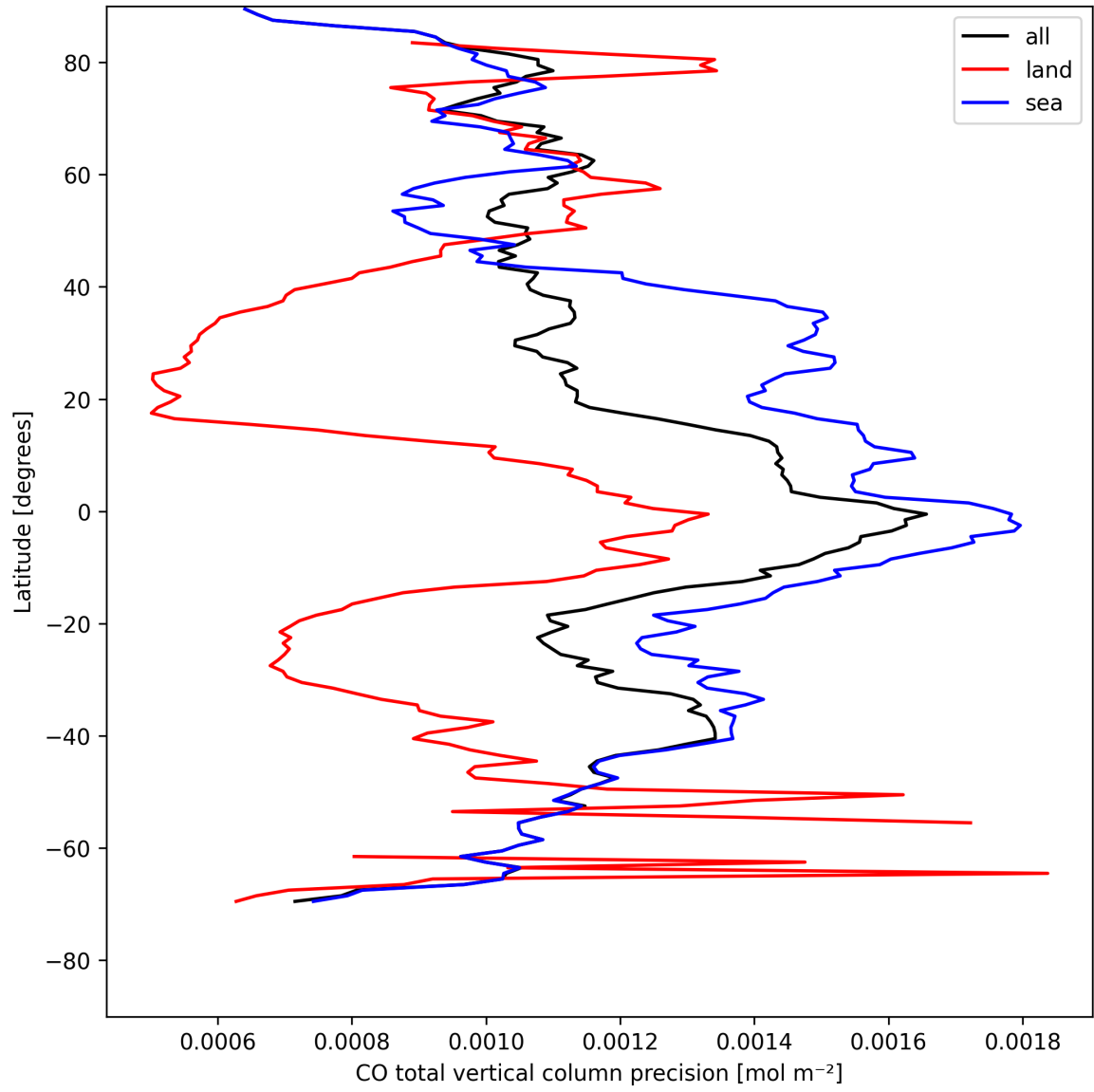
Figure 12: Zonal average of “CO total vertical column precision” for 2025-08-09 to 2025-08-11.
