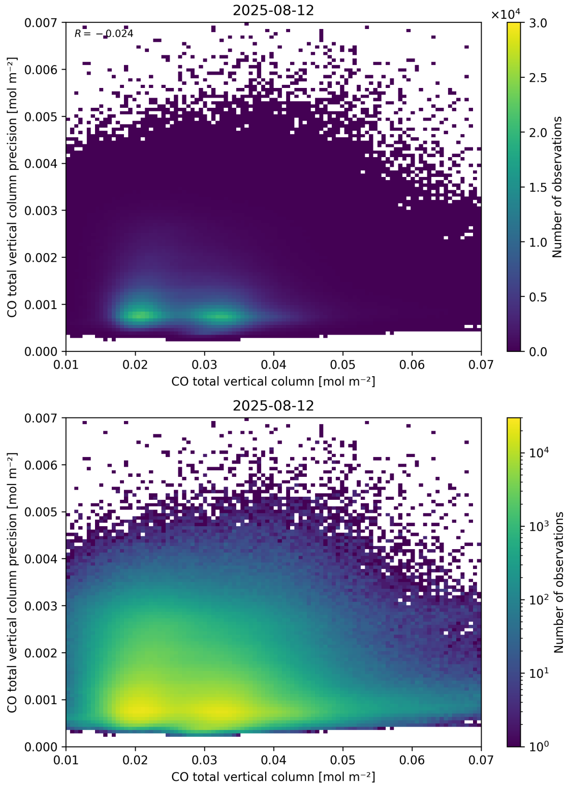
Figure 34: Scatter density plot of “CO total vertical column” against “CO total vertical column precision” for 2025-08-11 to 2025-08-13.
