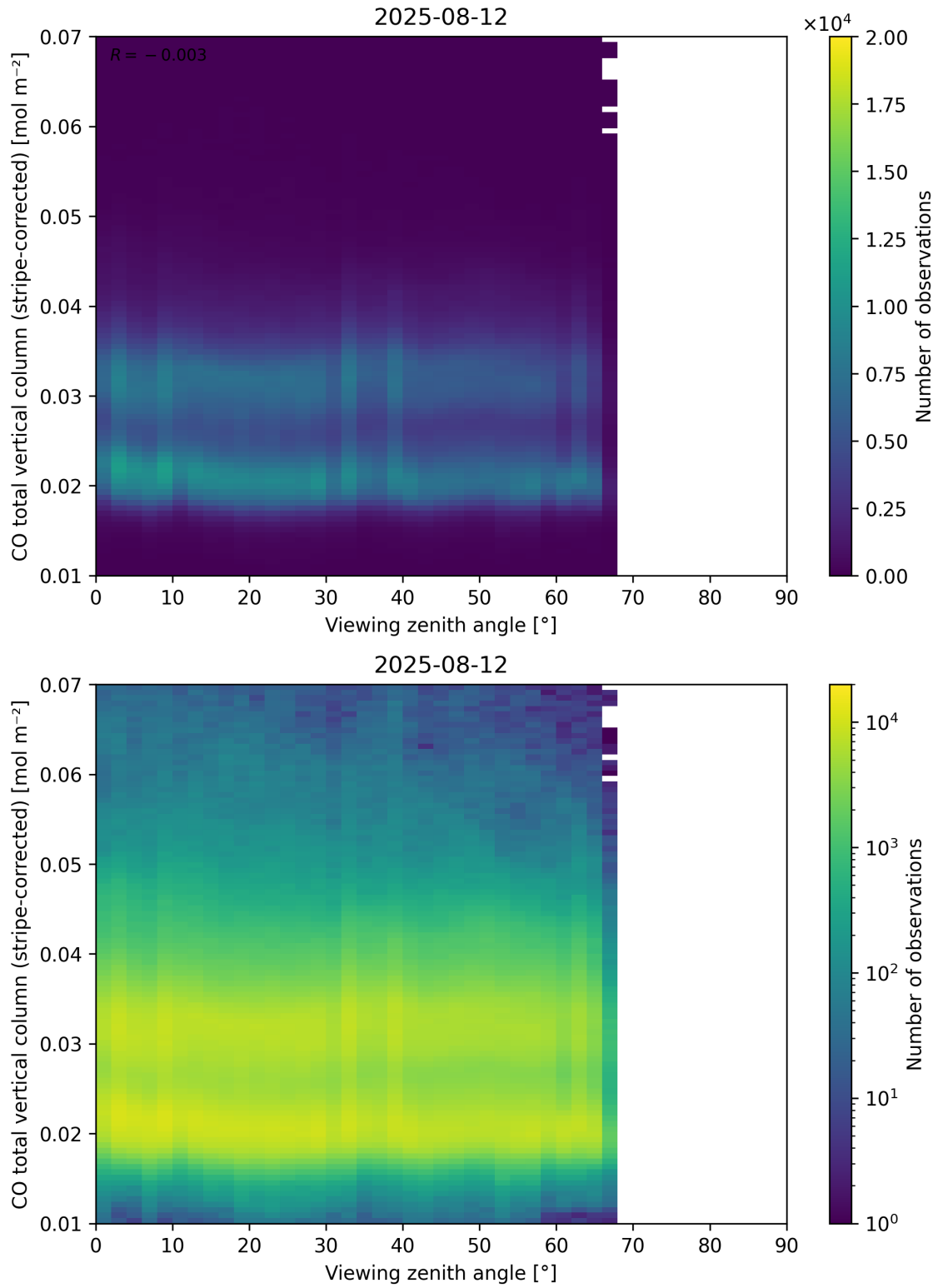
Figure 70: Scatter density plot of “Viewing zenith angle” against “CO total vertical column (stripe-corrected)” for 2025-08-11 to 2025-08-13.
