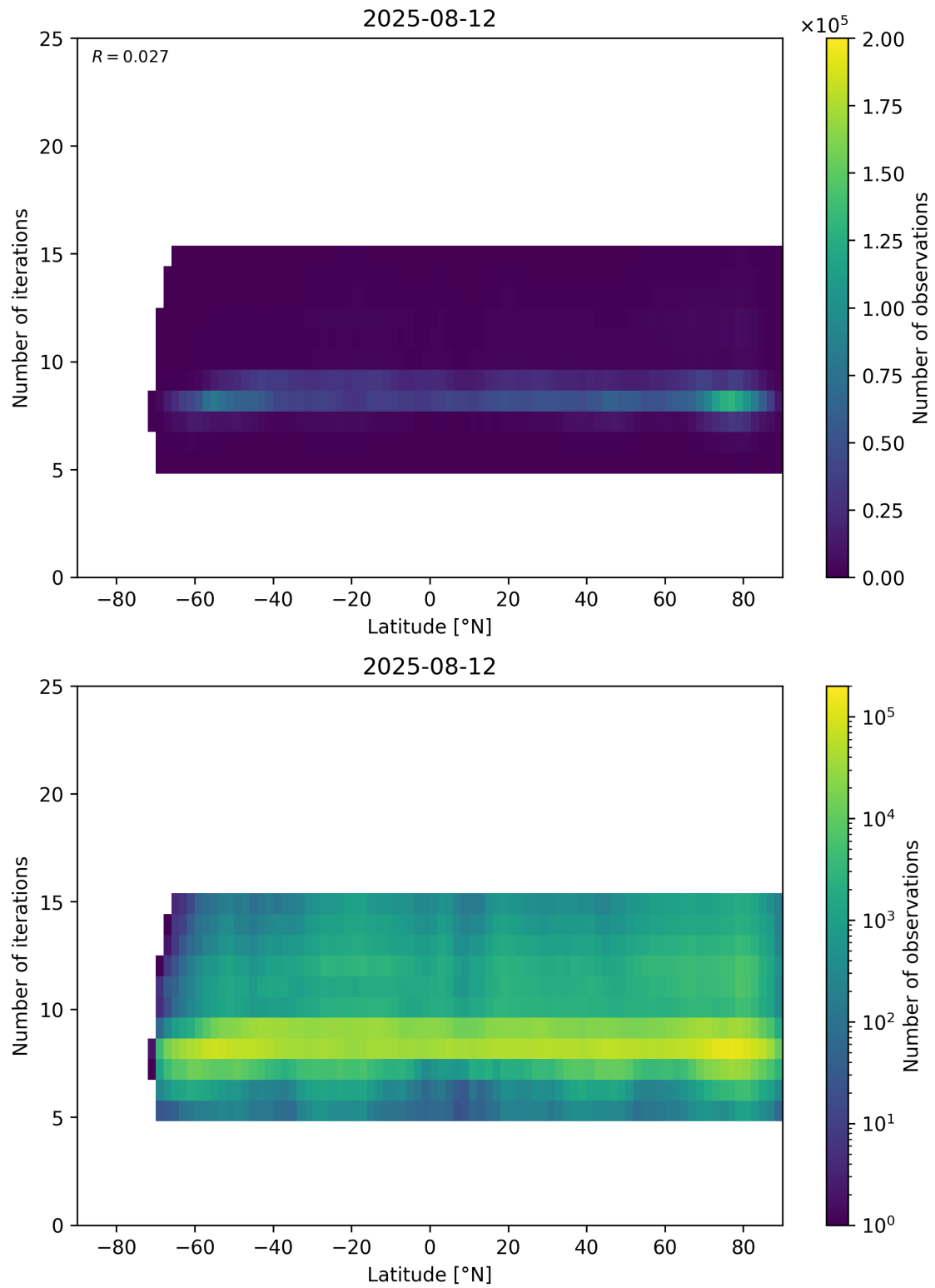
Figure 56: Scatter density plot of “Latitude” against “Number of iterations” for 2025-08-11 to 2025-08-13.
