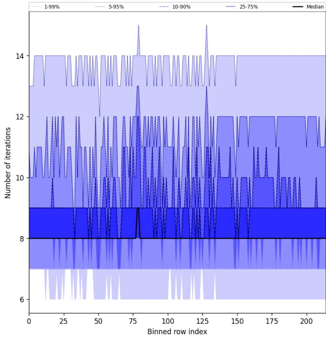
Figure 32: Along track statistics of “Number of iterations” for 2025-08-11 to 2025-08-13
