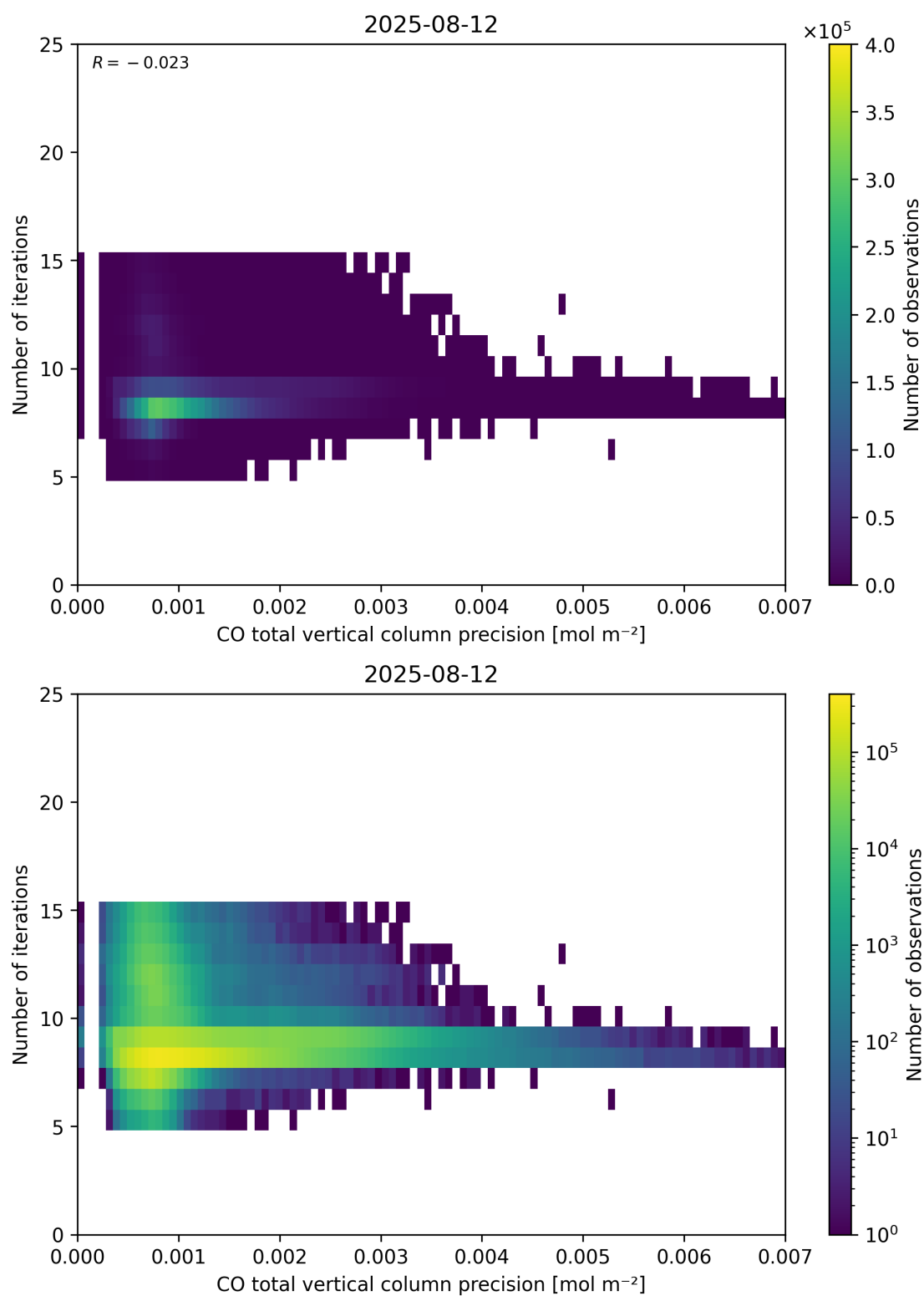
Figure 46: Scatter density plot of “CO total vertical column precision” against “Number of iterations” for 2025-08-11 to 2025-08-13.
