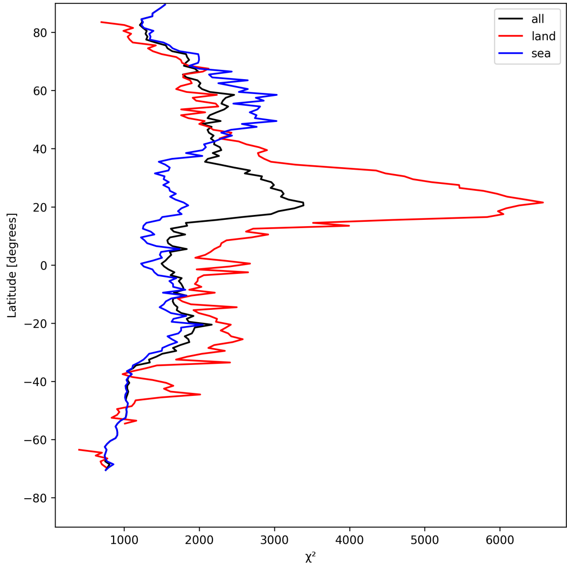
Figure 14: Zonal average of “ \chi^2 ” for 2025-08-11 to 2025-08-13.
