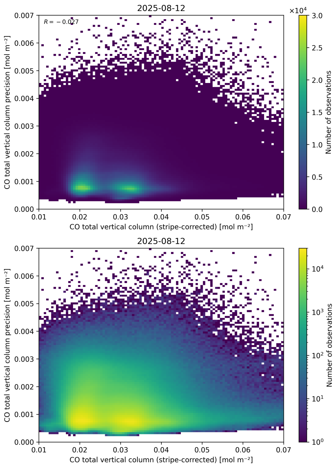
Figure 36: Scatter density plot of “CO total vertical column (stripe-corrected)” against “CO total vertical column precision” for 2025-08-11 to 2025-08-13.
