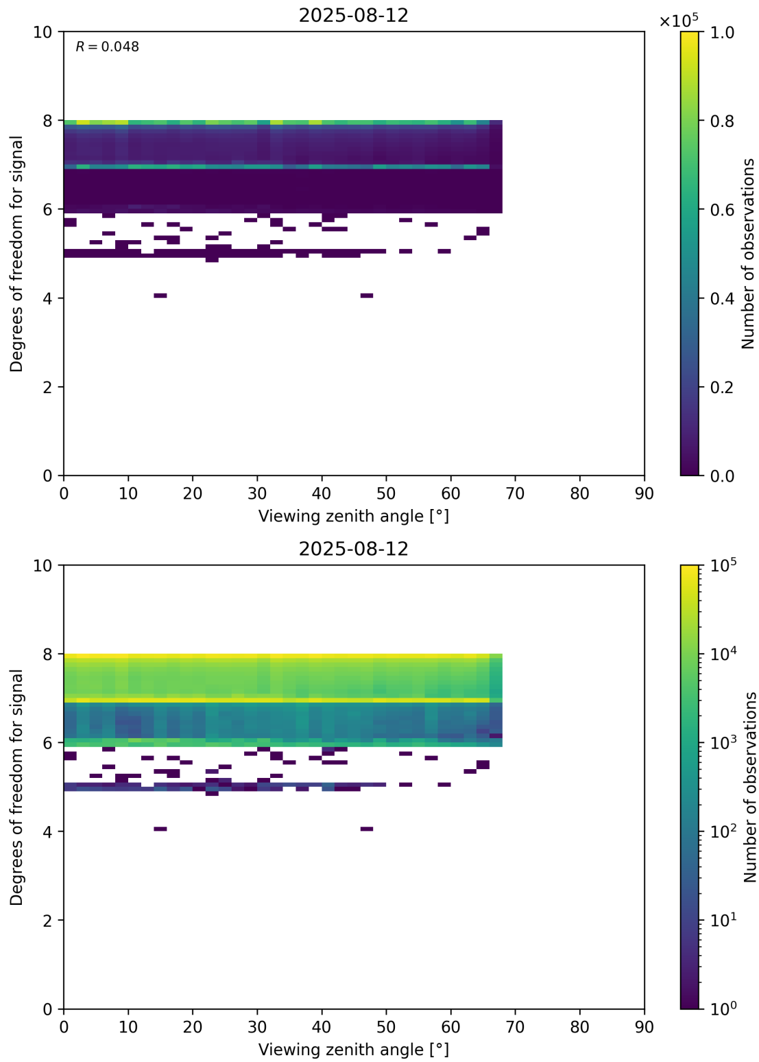
Figure 73: Scatter density plot of “Viewing zenith angle” against “Degrees of freedom for signal” for 2025-08-11 to 2025-08-13.
