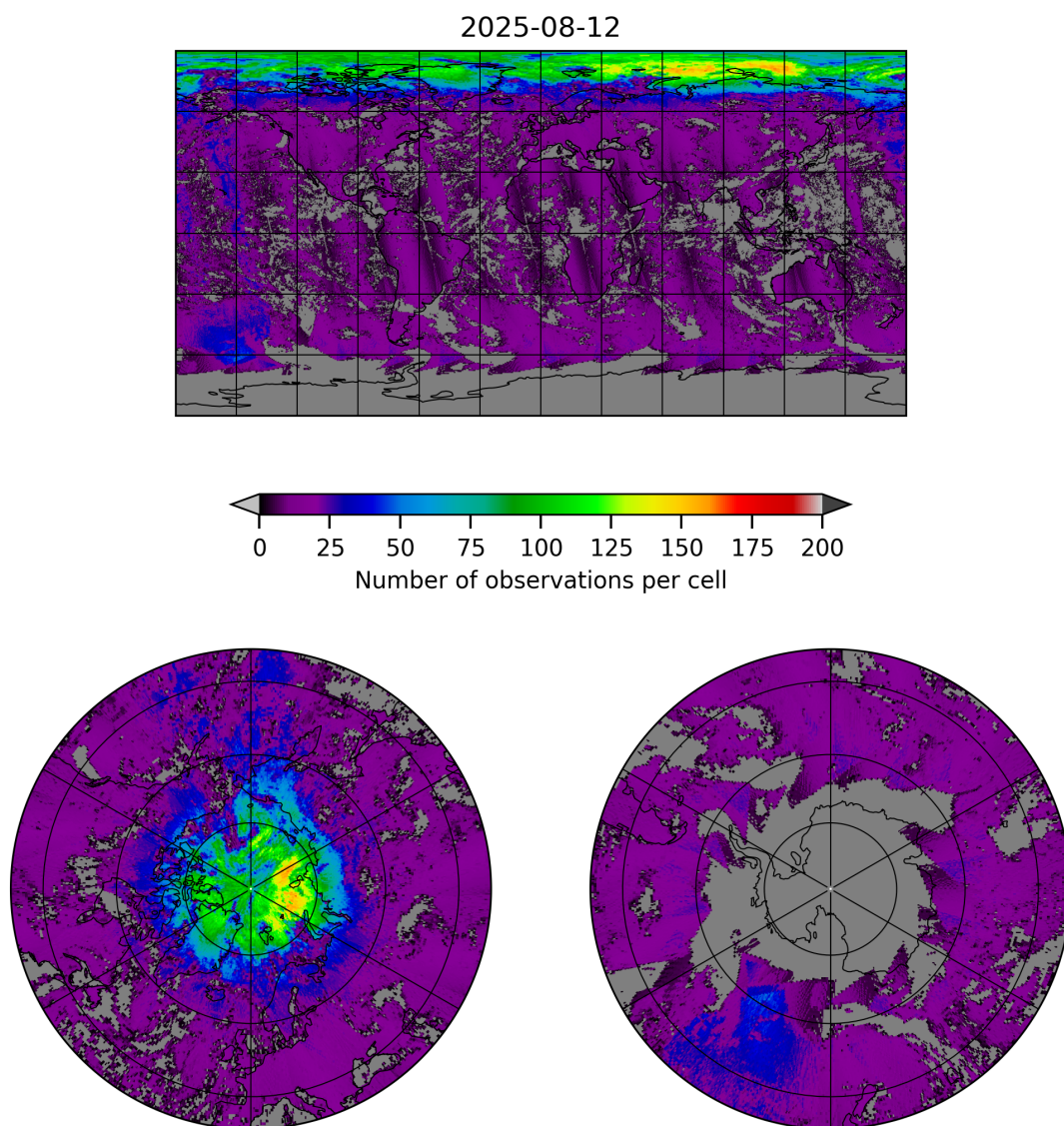
Figure 8: Map of the number of observations for 2025-08-11 to 2025-08-13
