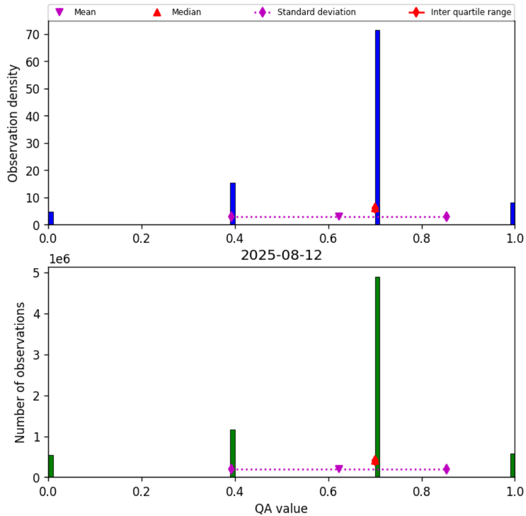
Figure 17: Histogram of “QA value” for 2025-08-11 to 2025-08-13
