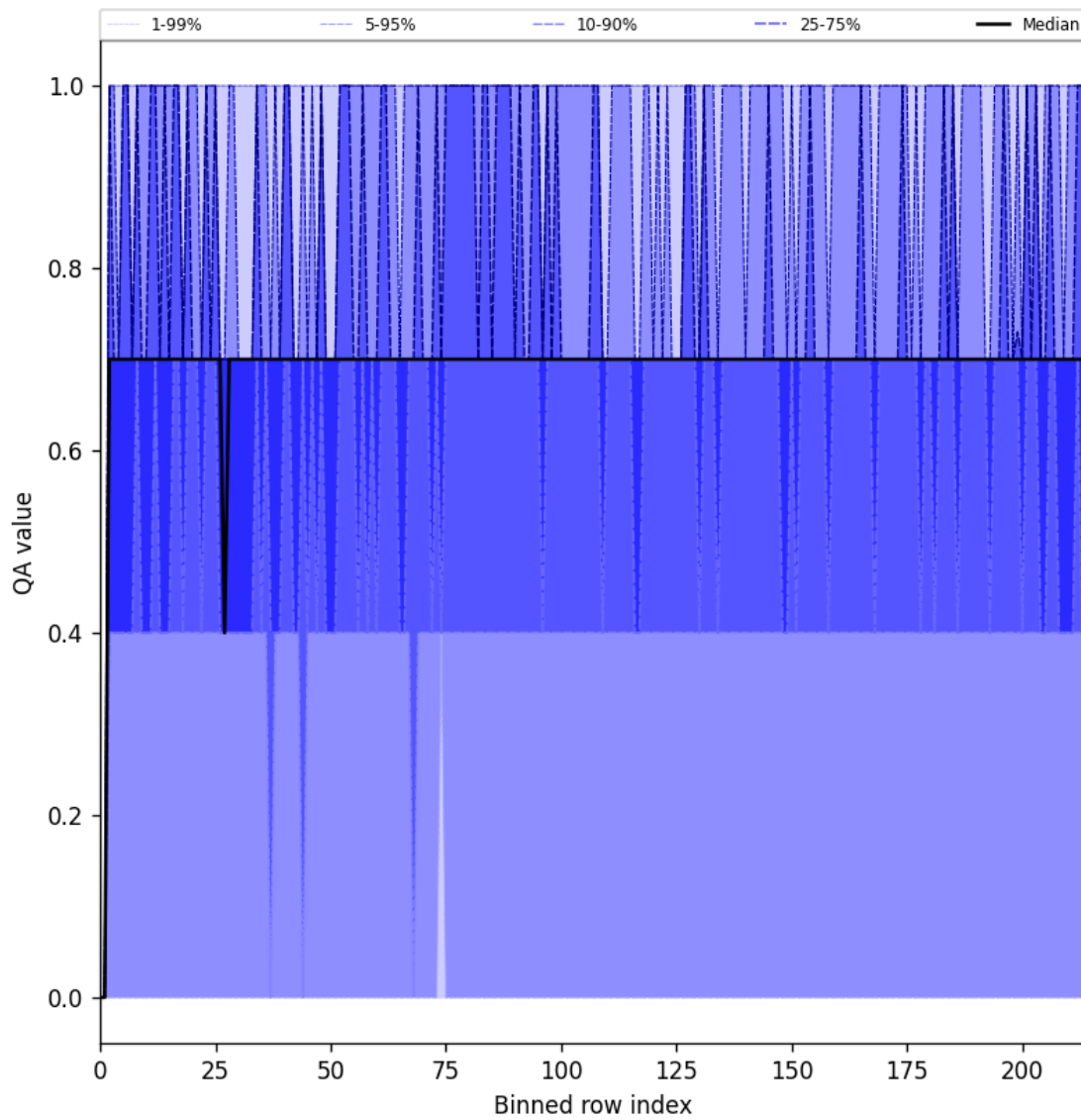
Figure 25: Along track statistics of “QA value” for 2025-08-11 to 2025-08-13
