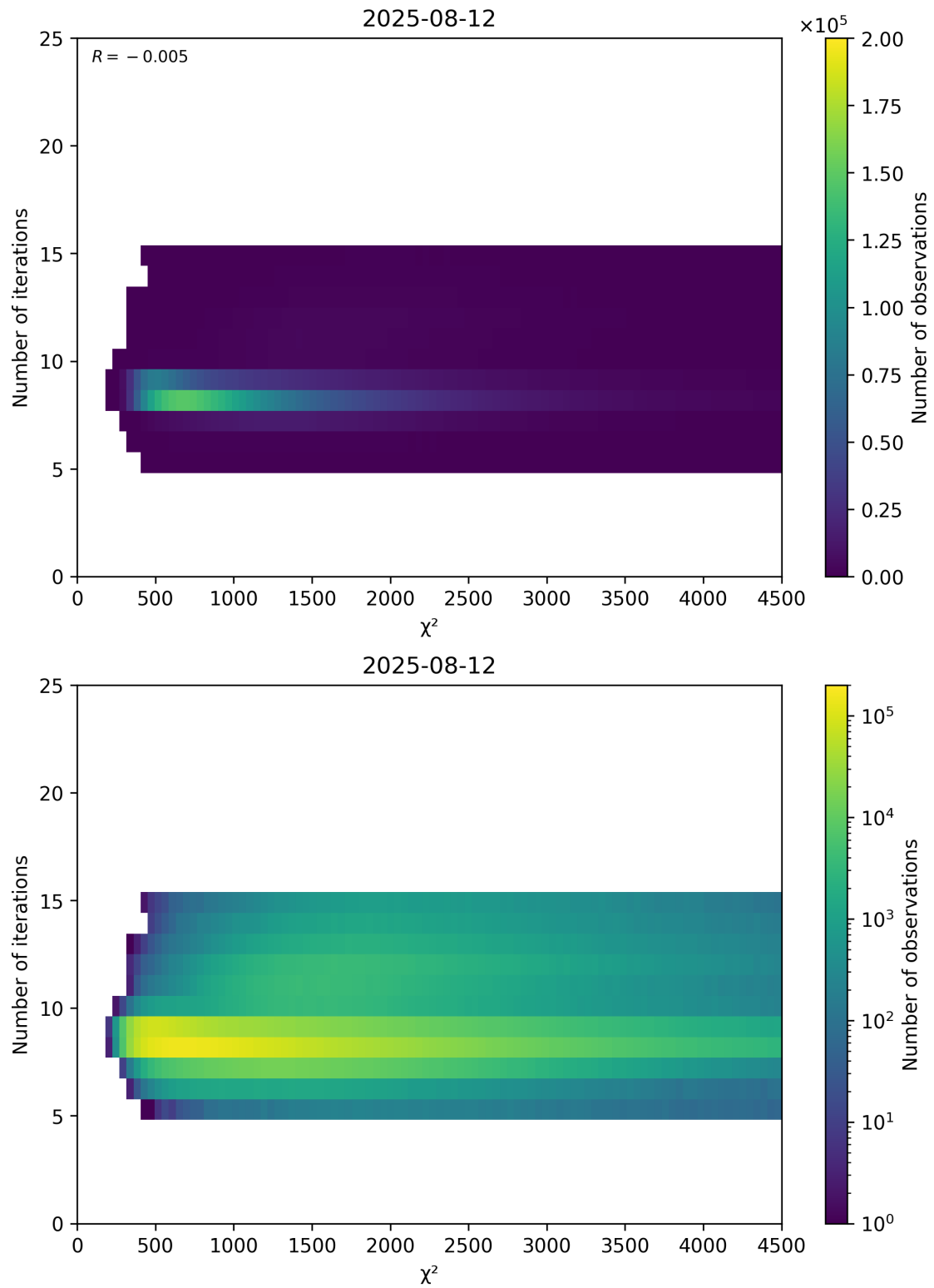
Figure 49: Scatter density plot of “ \chi^2 ” against “Number of iterations” for 2025-08-11 to 2025-08-13.
