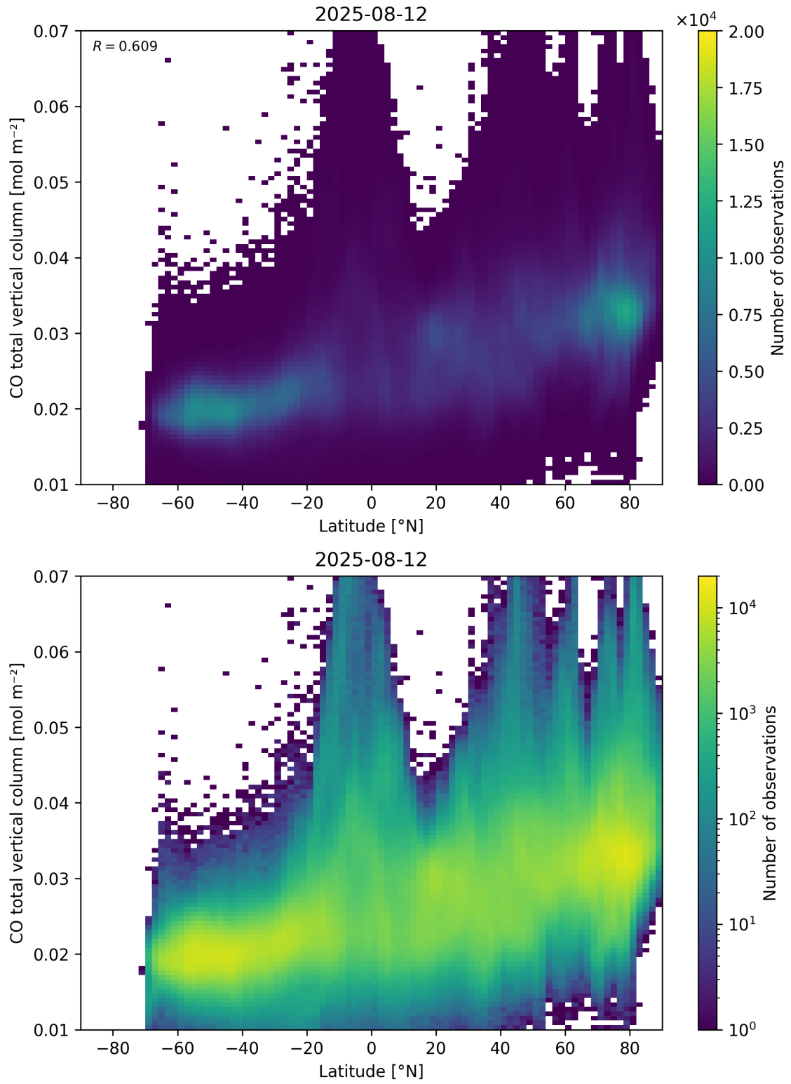
Figure 51: Scatter density plot of “Latitude” against “CO total vertical column” for 2025-08-11 to 2025-08-13.
