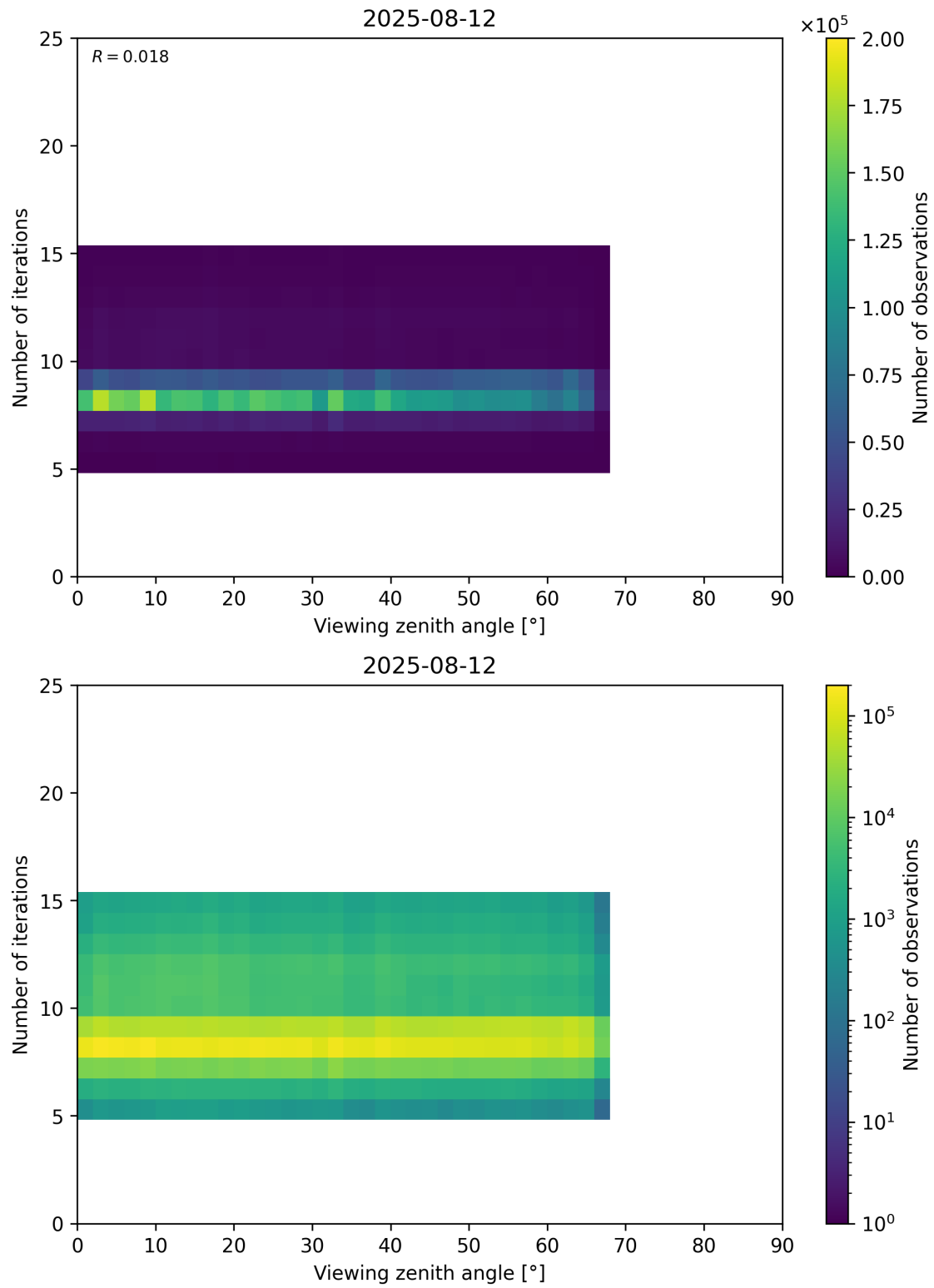
Figure 75: Scatter density plot of “Viewing zenith angle” against “Number of iterations” for 2025-08-11 to 2025-08-13.
