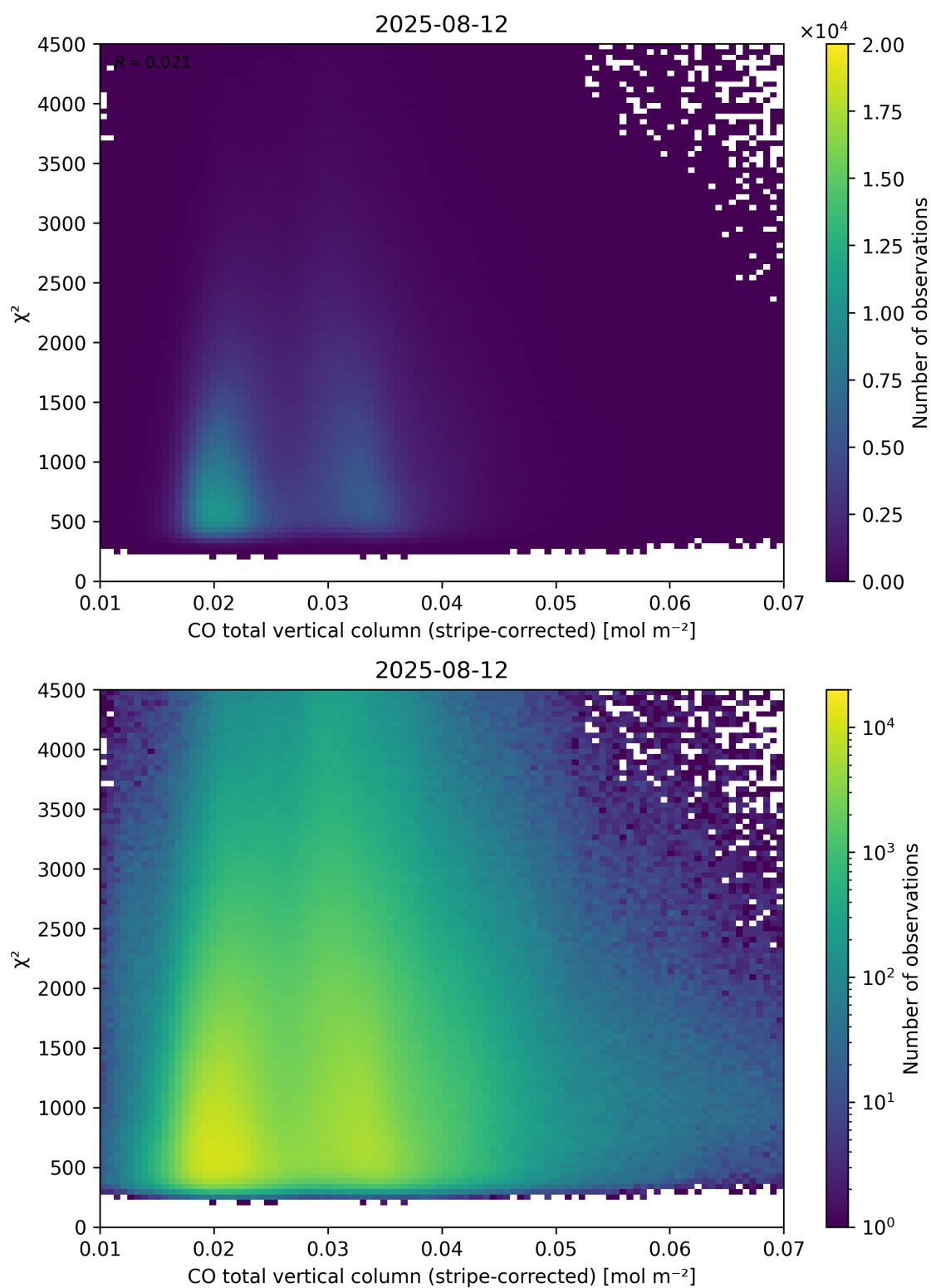
Figure 37: Scatter density plot of “CO total vertical column (stripe-corrected)” against “ \chi^2 ” for 2025-08-11 to 2025-08-13.
