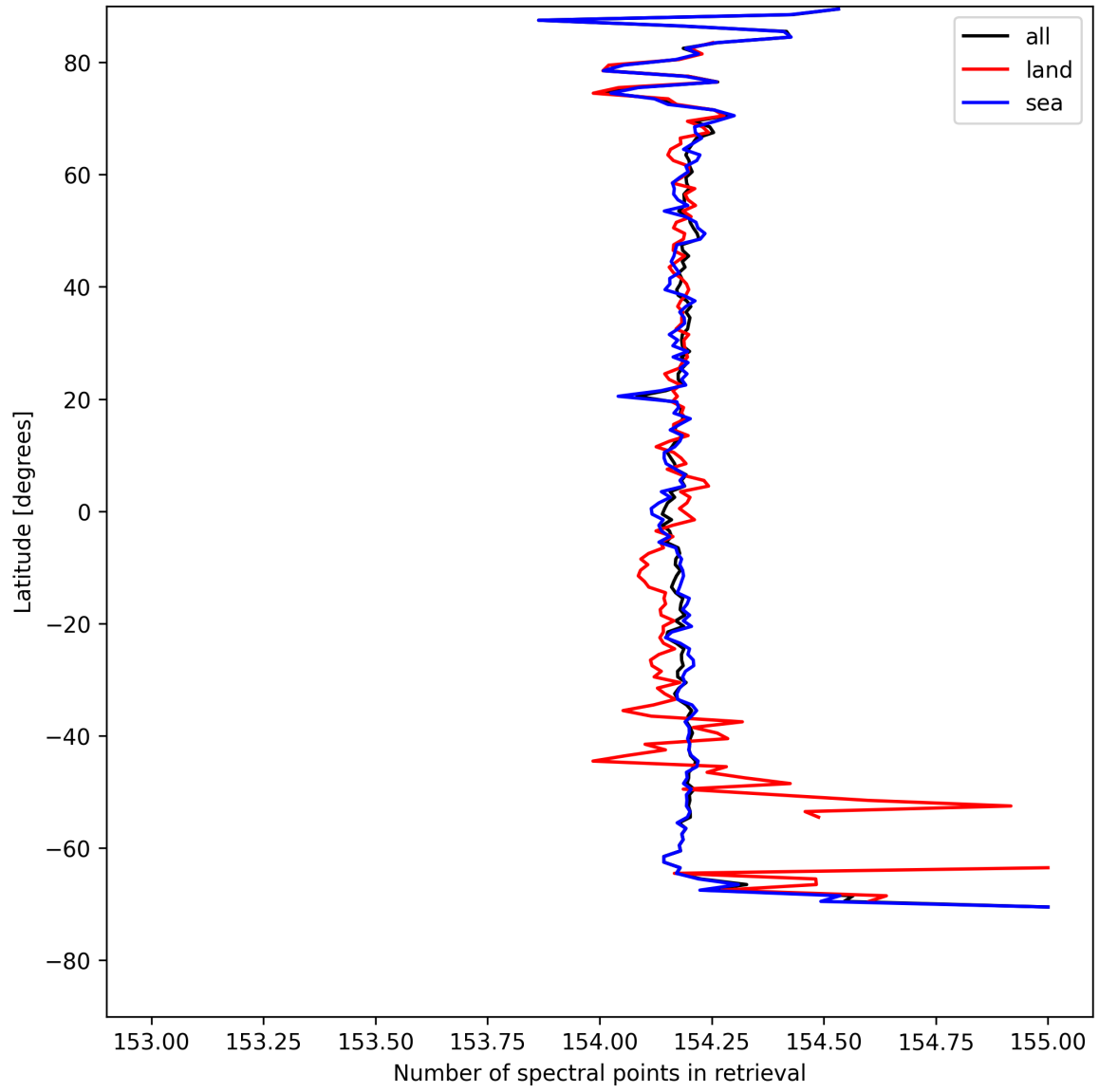
Figure 13: Zonal average of “Number of spectral points in retrieval” for 2025-08-11 to 2025-08-13.
