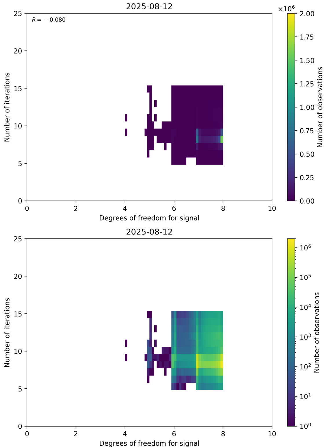
Figure 50: Scatter density plot of “Degrees of freedom for signal” against “Number of iterations” for 2025-08-11 to 2025-08-13.
