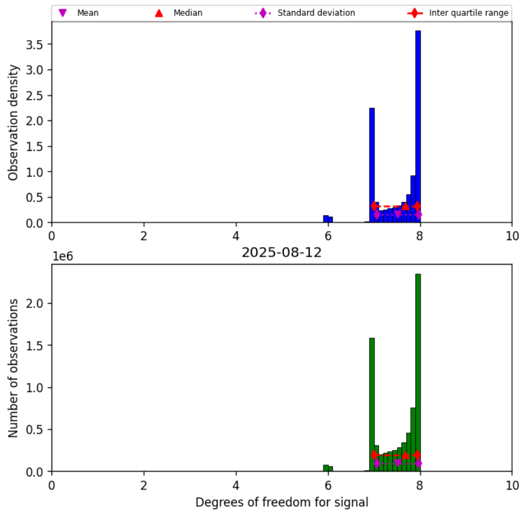
Figure 23: Histogram of “Degrees of freedom for signal” for 2025-08-11 to 2025-08-13
