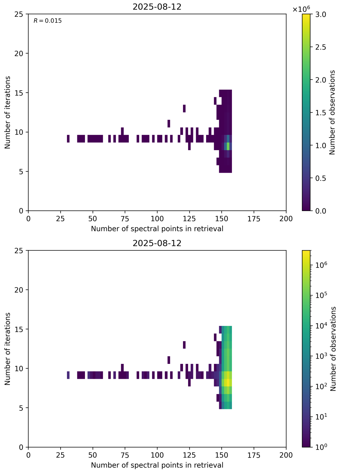
Figure 60: Scatter density plot of “Number of spectral points in retrieval” against “Number of iterations” for 2025-08-11 to 2025-08-13.
