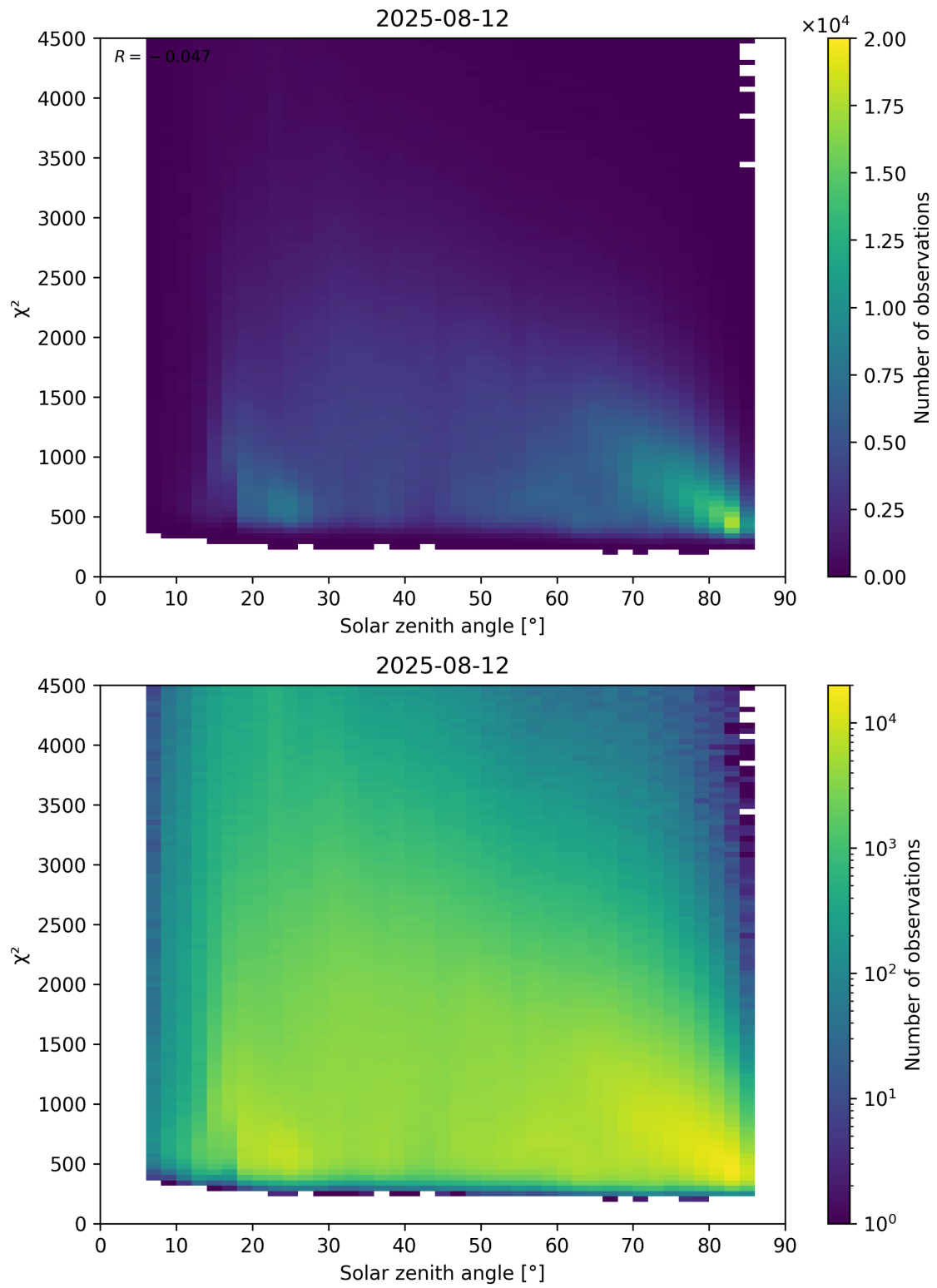
Figure 64: Scatter density plot of “Solar zenith angle” against “ \chi^2 ” for 2025-08-11 to 2025-08-13.
