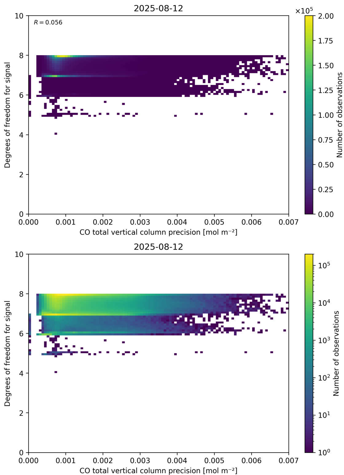
Figure 45: Scatter density plot of “CO total vertical column precision” against “Degrees of freedom for signal” for 2025-08-11 to 2025-08-13.
