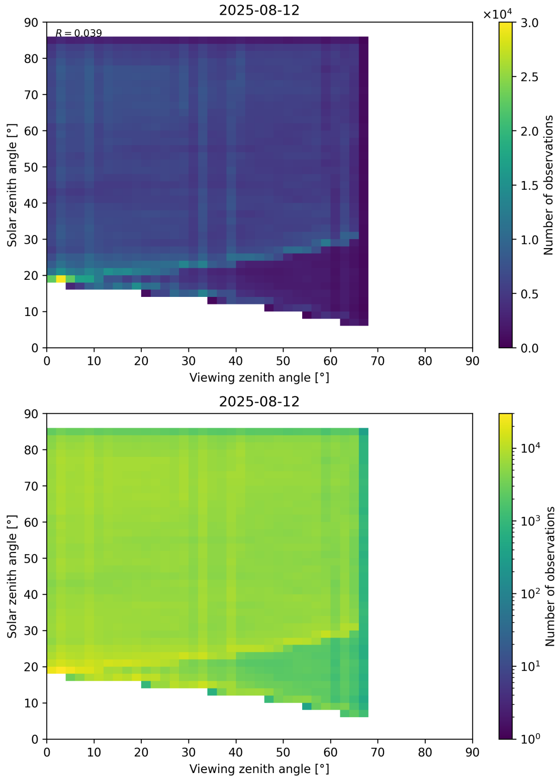
Figure 77: Scatter density plot of “Viewing zenith angle” against “Solar zenith angle” for 2025-08-11 to 2025-08-13.
