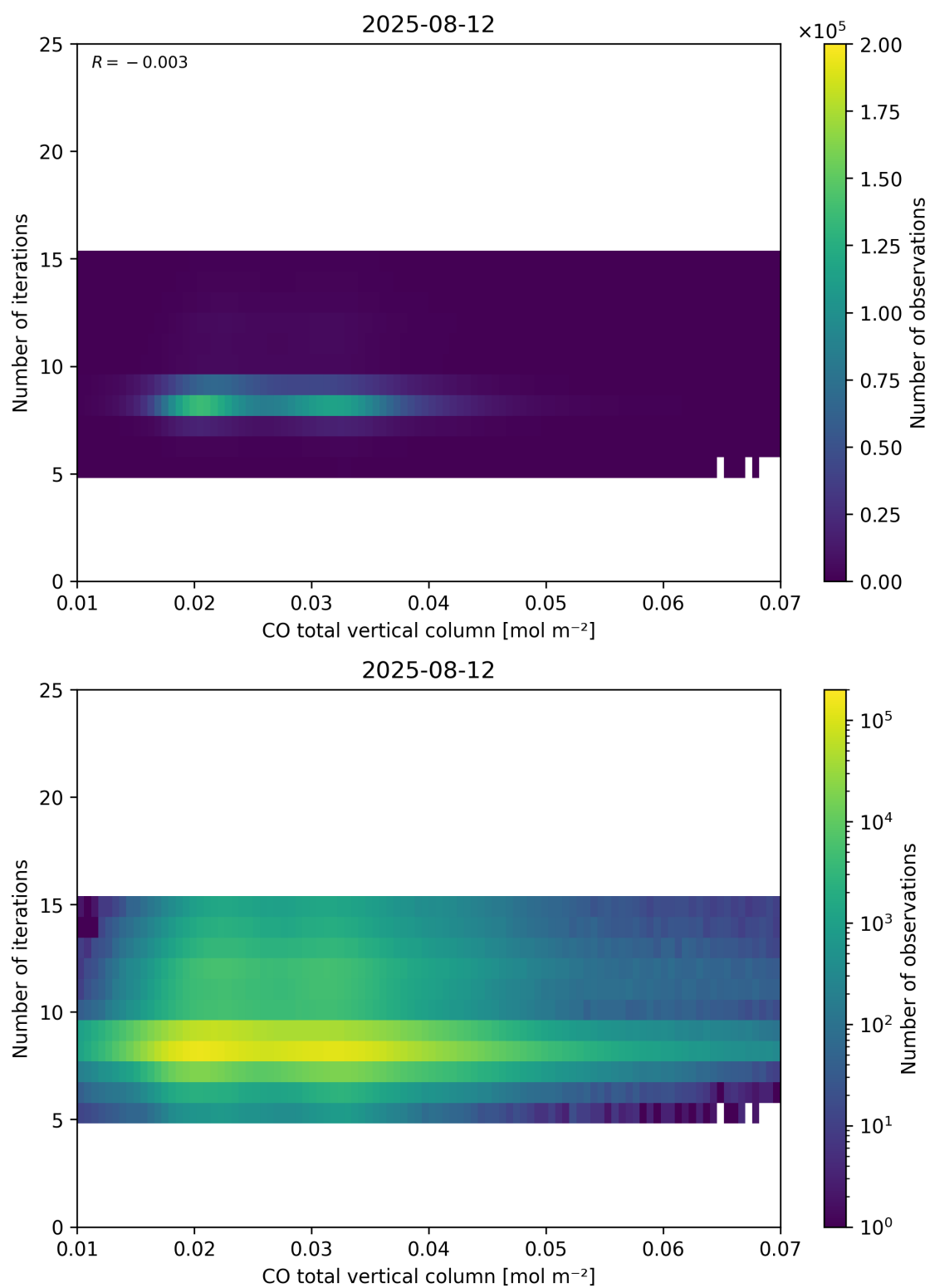
Figure 42: Scatter density plot of “CO total vertical column” against “Number of iterations” for 2025-08-11 to 2025-08-13.
