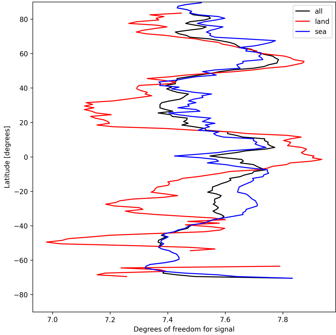
Figure 15: Zonal average of “Degrees of freedom for signal” for 2025-08-11 to 2025-08-13.
