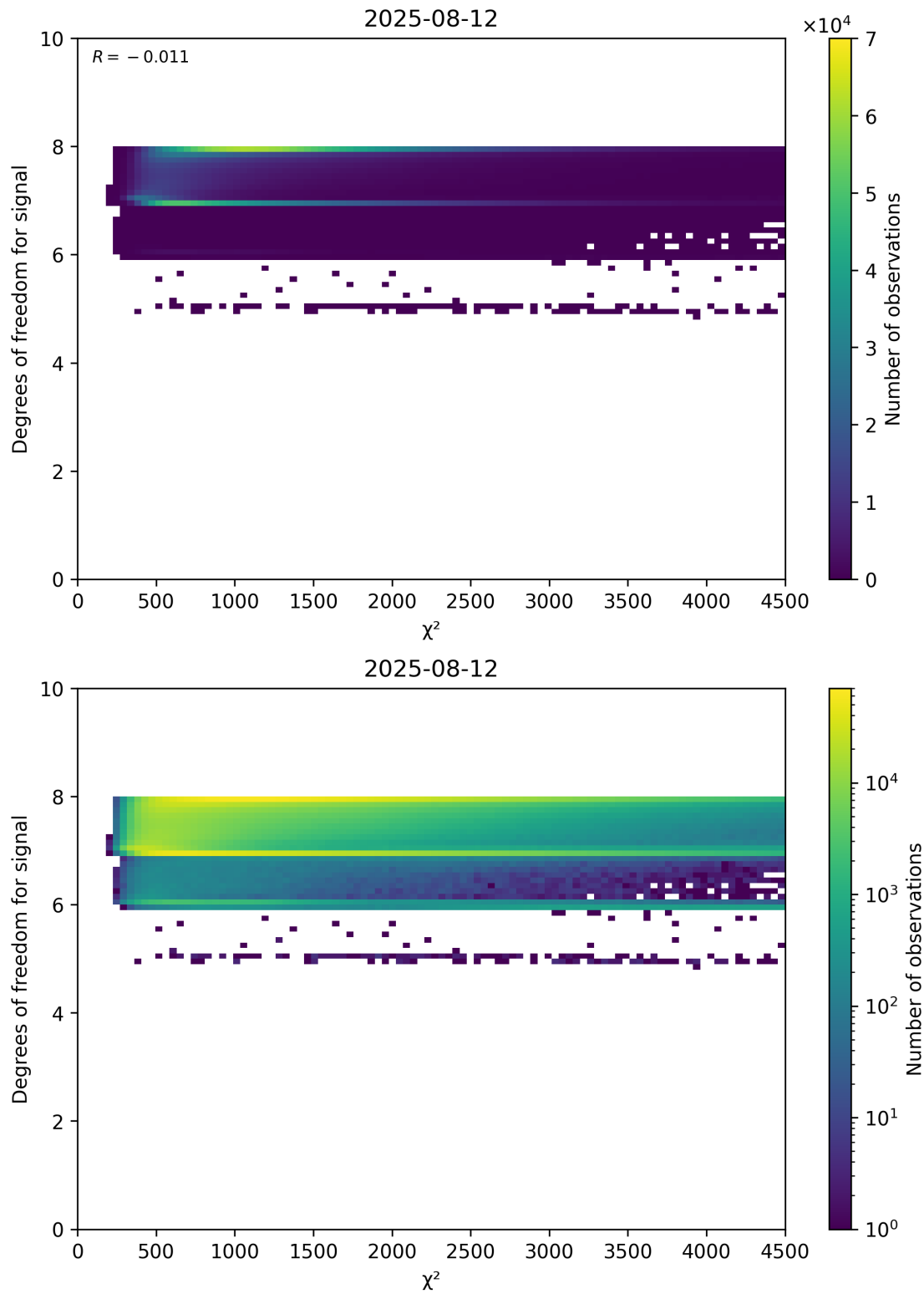
Figure 48: Scatter density plot of “ \chi^2 ” against “Degrees of freedom for signal” for 2025-08-11 to 2025-08-13.
