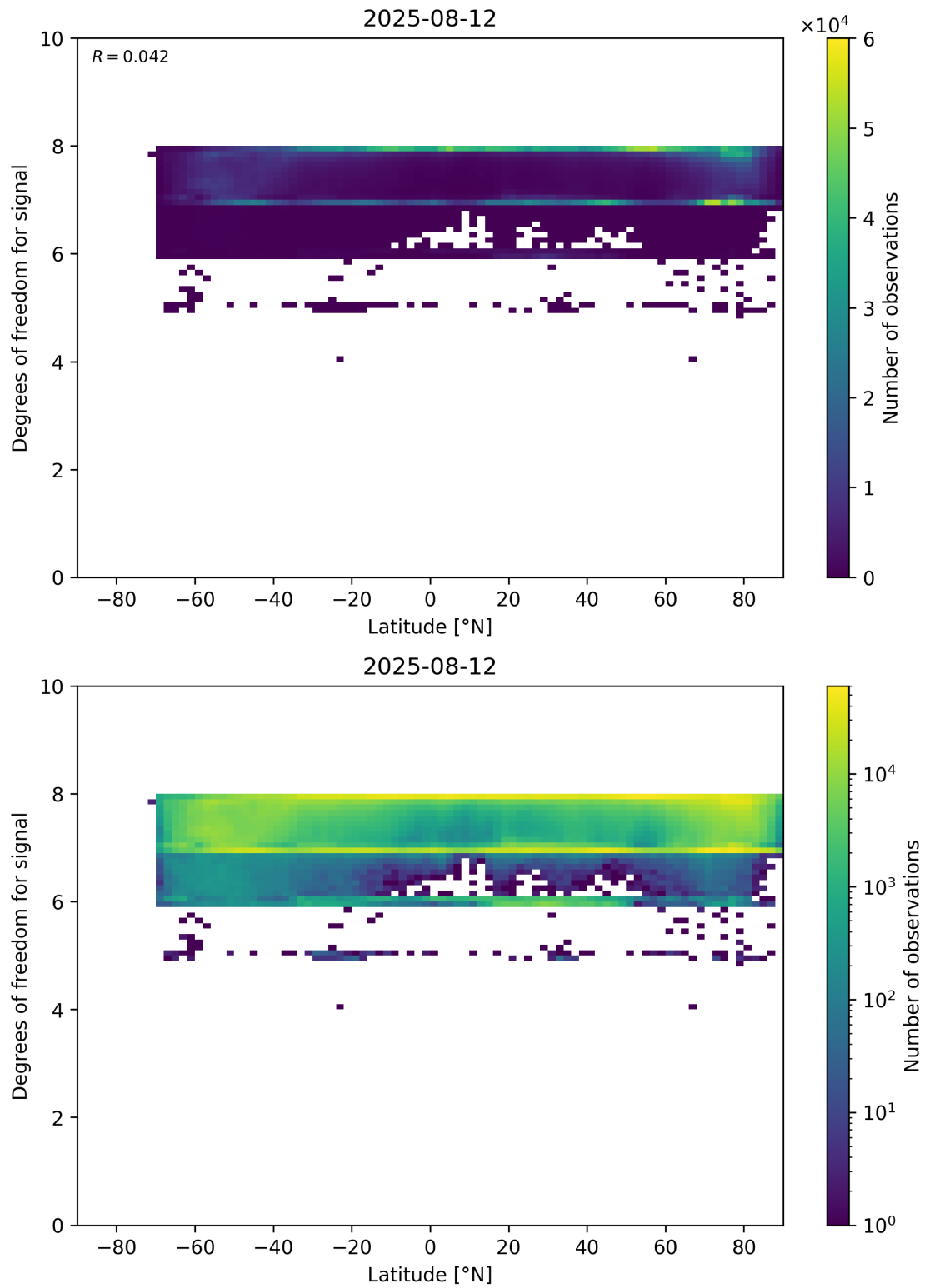
Figure 55: Scatter density plot of “Latitude” against “Degrees of freedom for signal” for 2025-08-11 to 2025-08-13.
