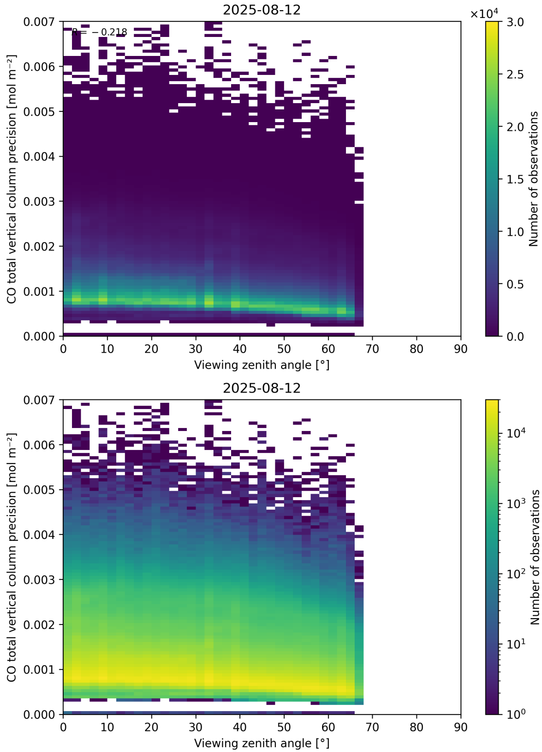
Figure 71: Scatter density plot of “Viewing zenith angle” against “CO total vertical column precision” for 2025-08-11 to 2025-08-13.
