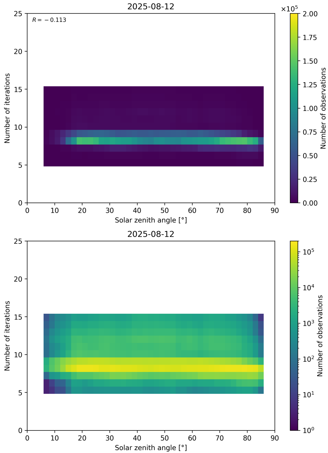
Figure 67: Scatter density plot of “Solar zenith angle” against “Number of iterations” for 2025-08-11 to 2025-08-13.
