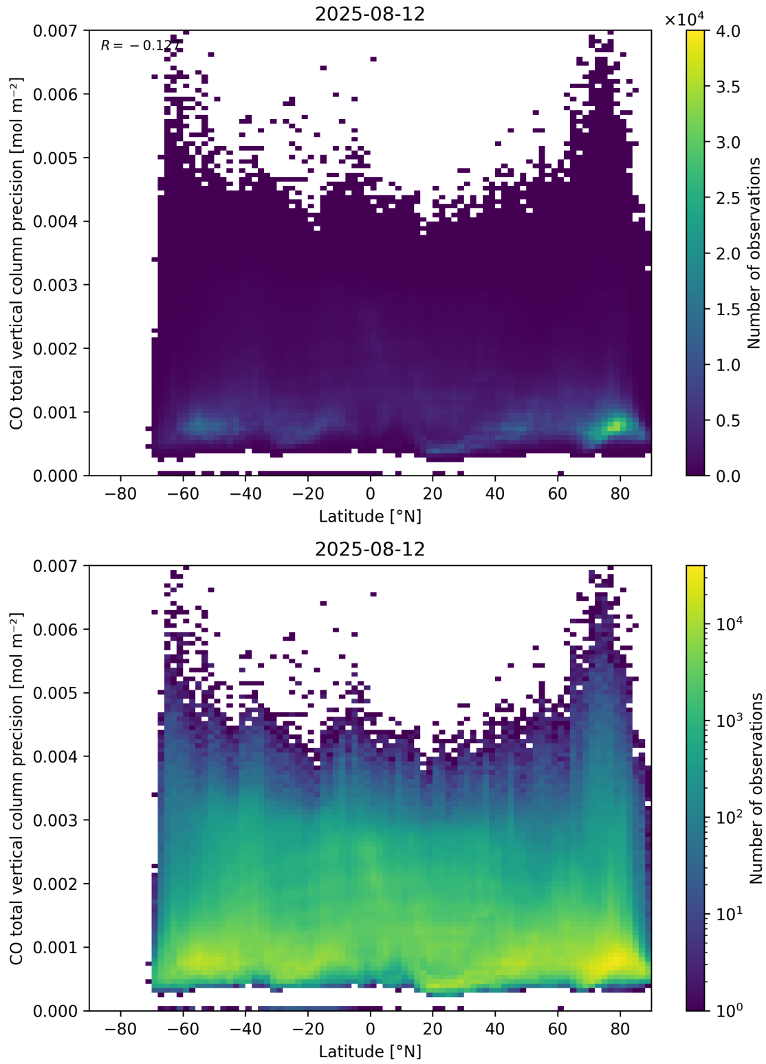
Figure 53: Scatter density plot of “Latitude” against “CO total vertical column precision” for 2025-08-11 to 2025-08-13.
