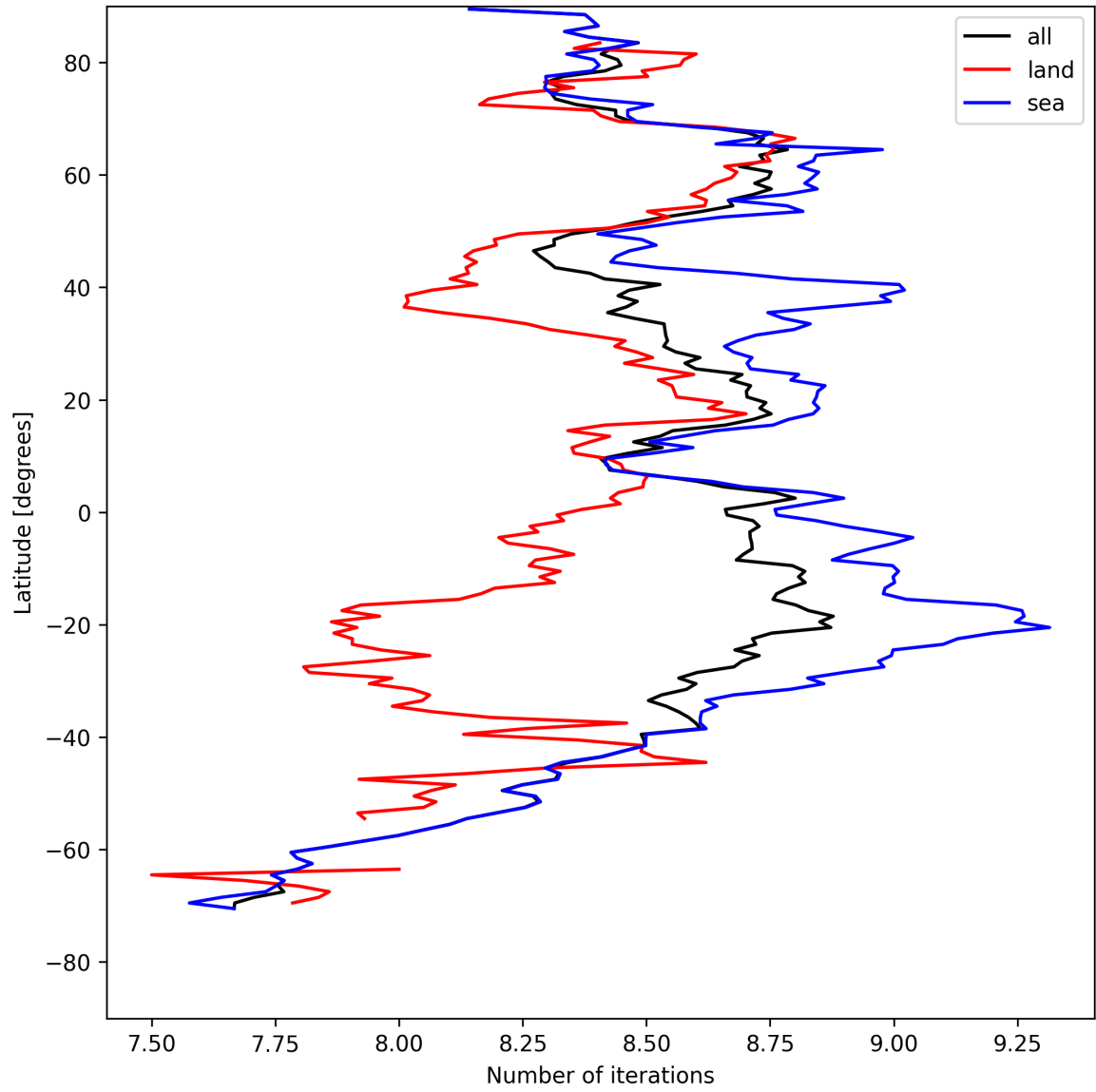
Figure 16: Zonal average of “Number of iterations” for 2025-08-11 to 2025-08-13.
