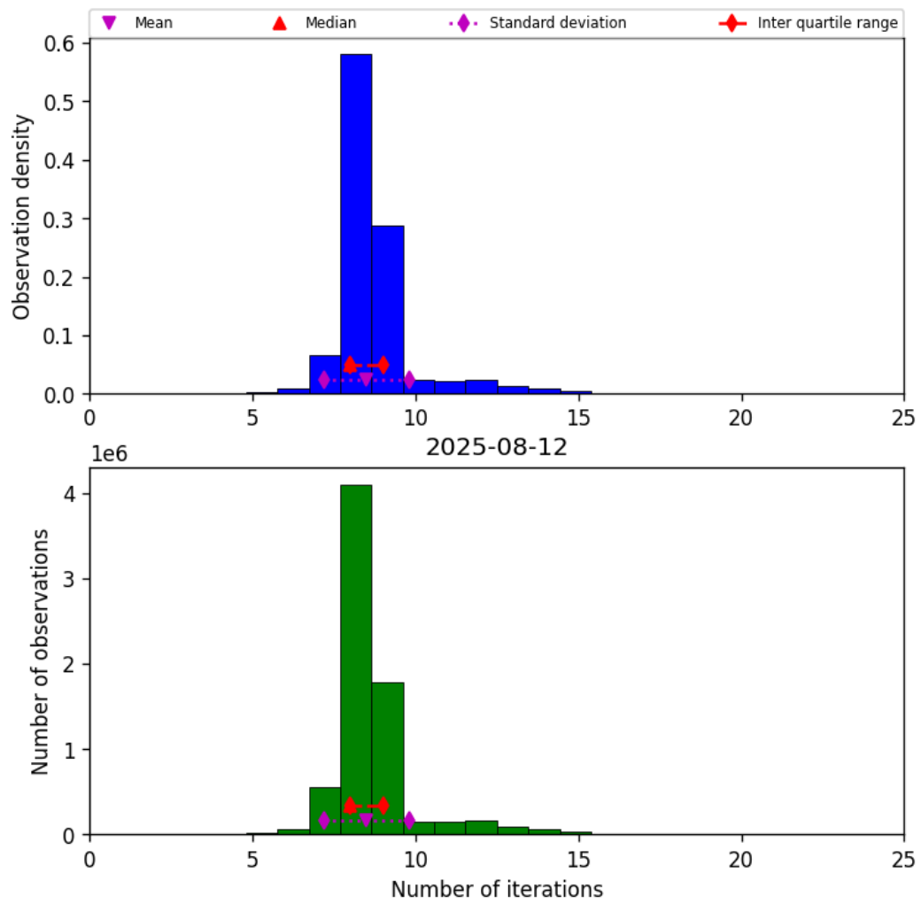
Figure 24: Histogram of “Number of iterations” for 2025-08-11 to 2025-08-13
