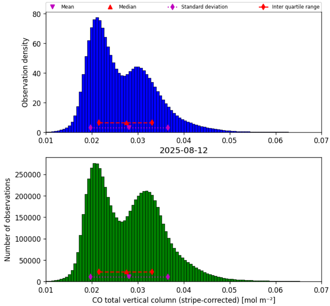
Figure 19: Histogram of “CO total vertical column (stripe-corrected)” for 2025-08-11 to 2025-08-13
