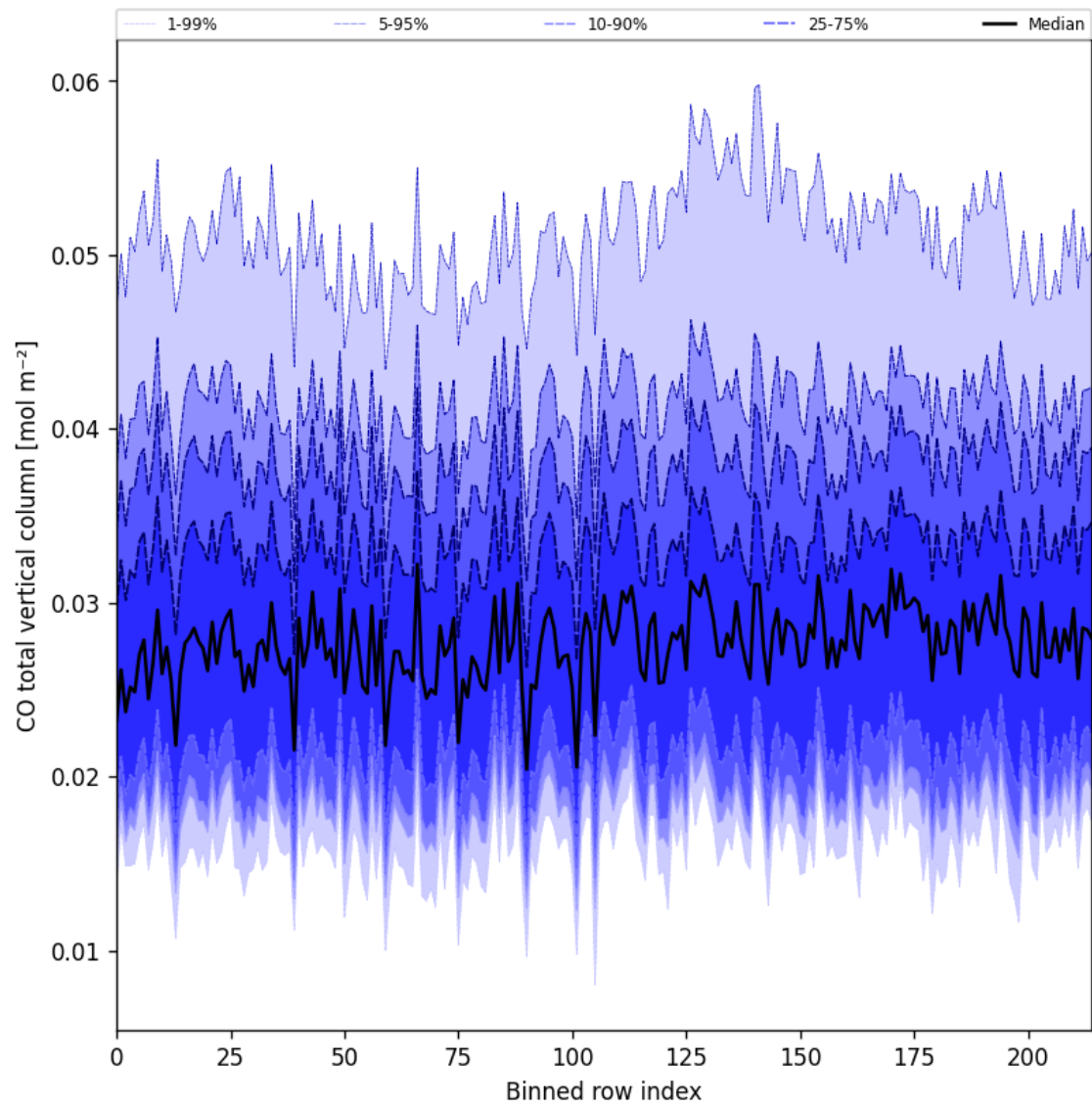
Figure 26: Along track statistics of “CO total vertical column” for 2025-08-11 to 2025-08-13
