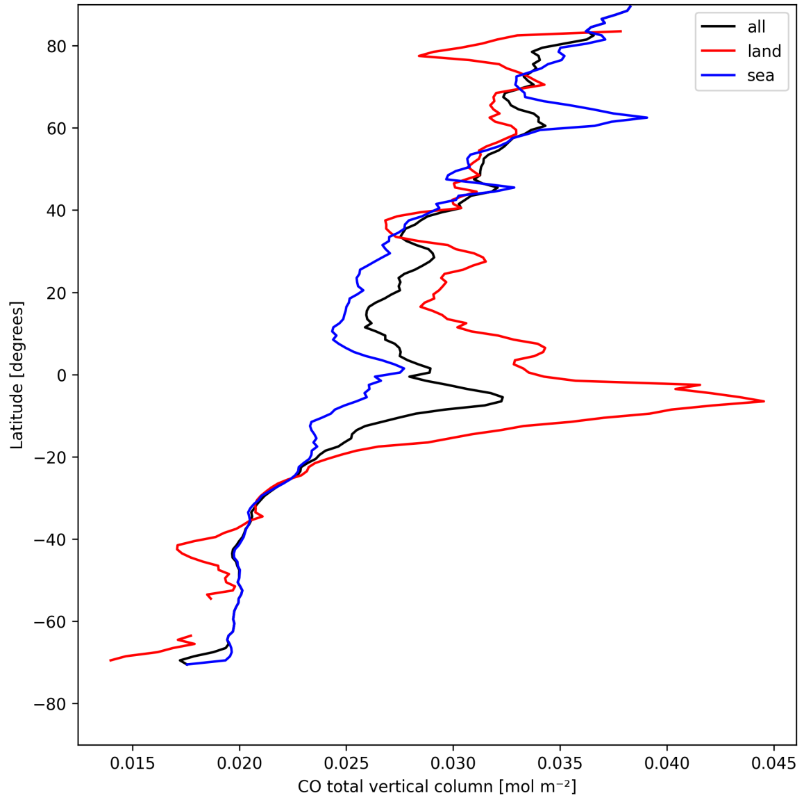
Figure 10: Zonal average of “CO total vertical column” for 2025-08-11 to 2025-08-13.
