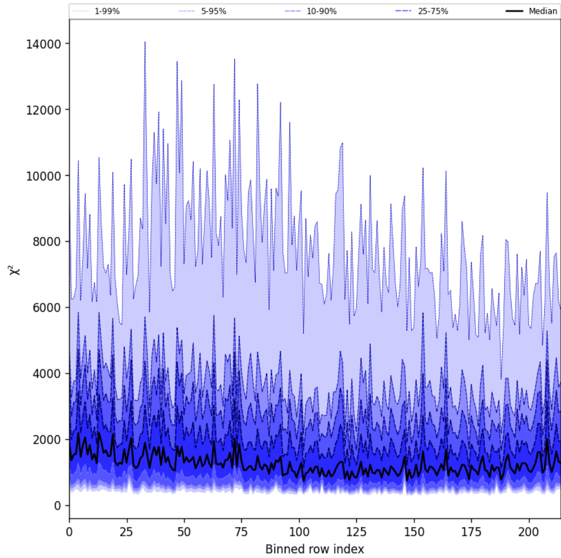
Figure 30: Along track statistics of “ \chi^2 ” for 2025-08-11 to 2025-08-13
