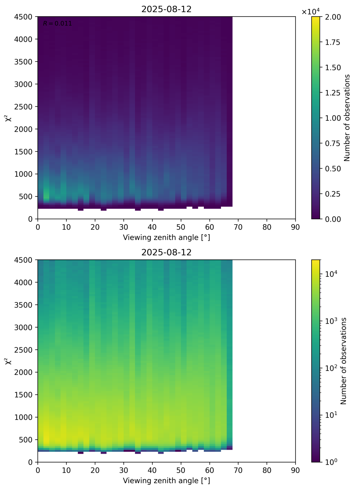
Figure 72: Scatter density plot of “Viewing zenith angle” against “ \chi^2 ” for 2025-08-11 to 2025-08-13.
