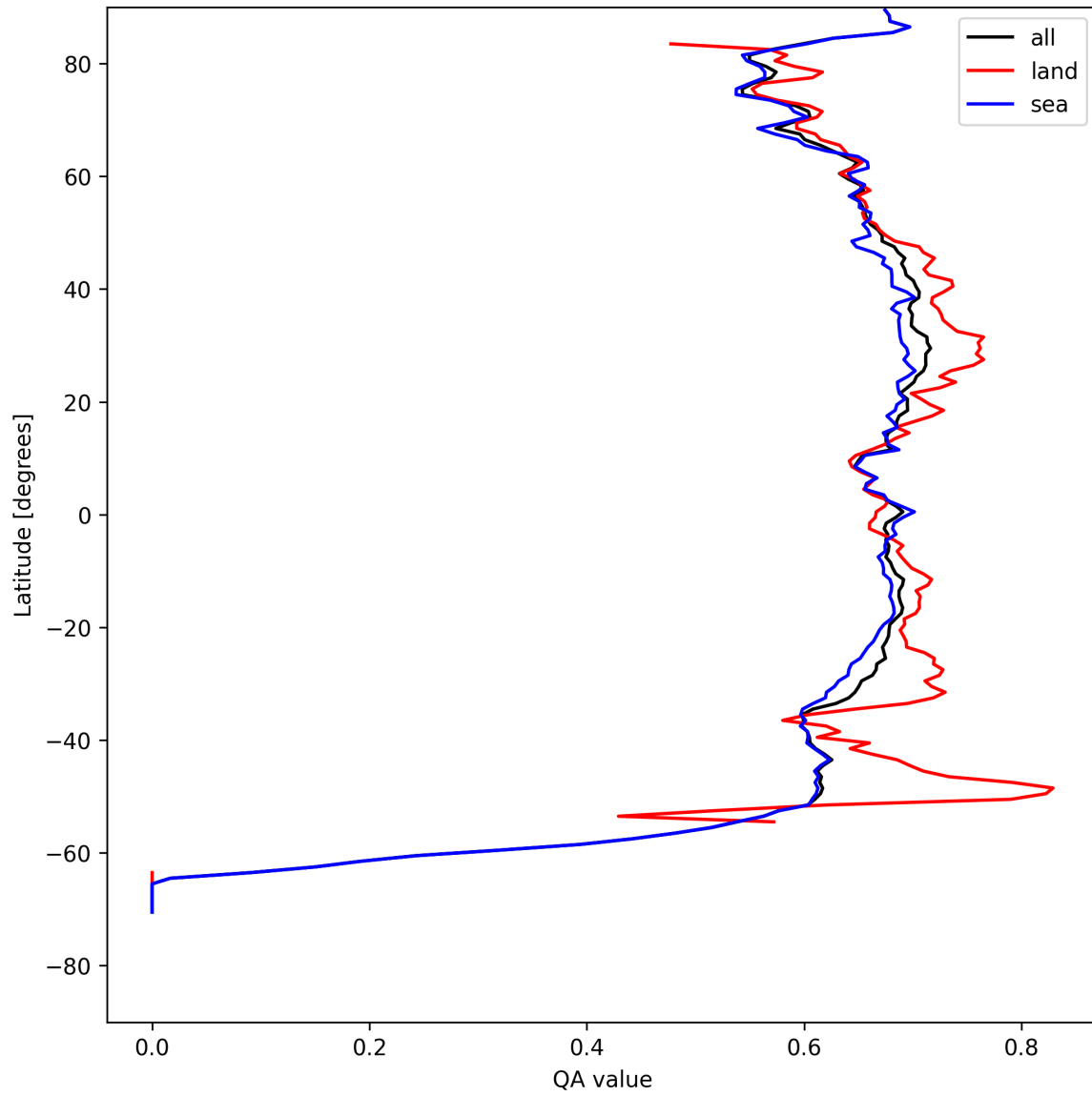
Figure 9: Zonal average of “QA value” for 2025-08-11 to 2025-08-13.
