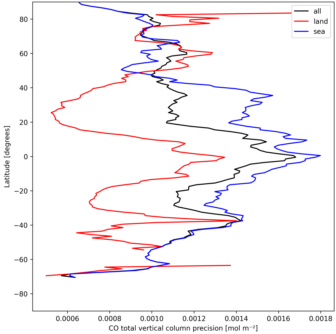
Figure 12: Zonal average of "CO total vertical column precision" for 2025-08-11 to 2025-08-13.
