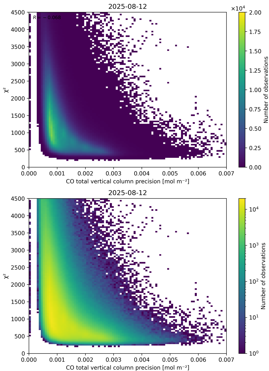
Figure 44: Scatter density plot of “CO total vertical column precision” against “ \chi^2 ” for 2025-08-11 to 2025-08-13.
