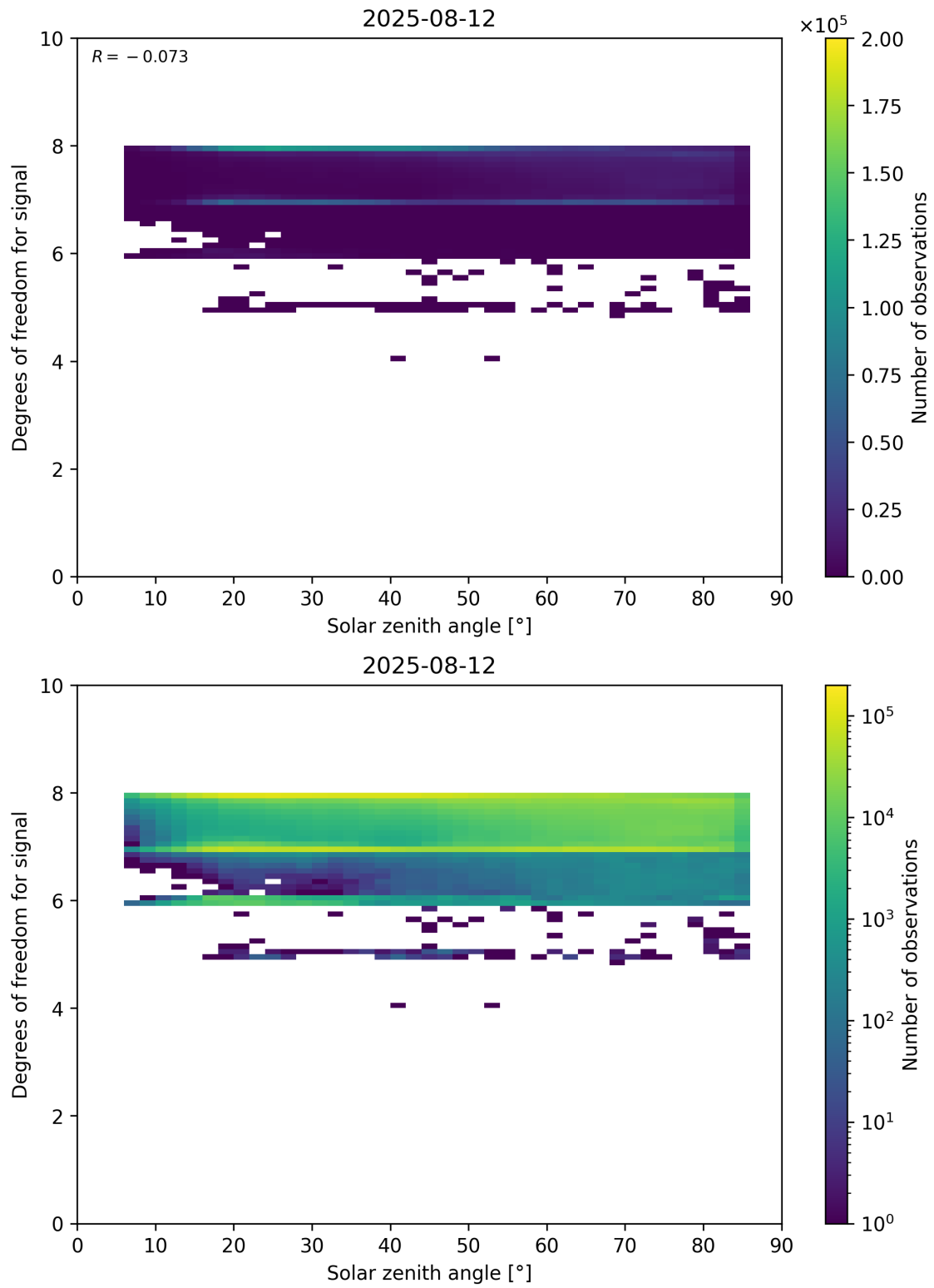
Figure 65: Scatter density plot of “Solar zenith angle” against “Degrees of freedom for signal” for 2025-08-11 to 2025-08-13.
