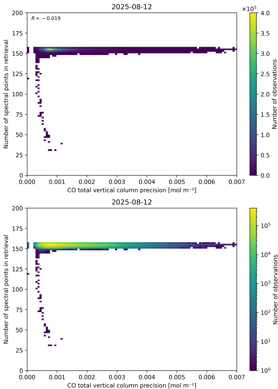
Figure 47: Scatter density plot of “CO total vertical column precision” against “Number of spectral points in retrieval” for 2025-08-11 to 2025-08-13.
