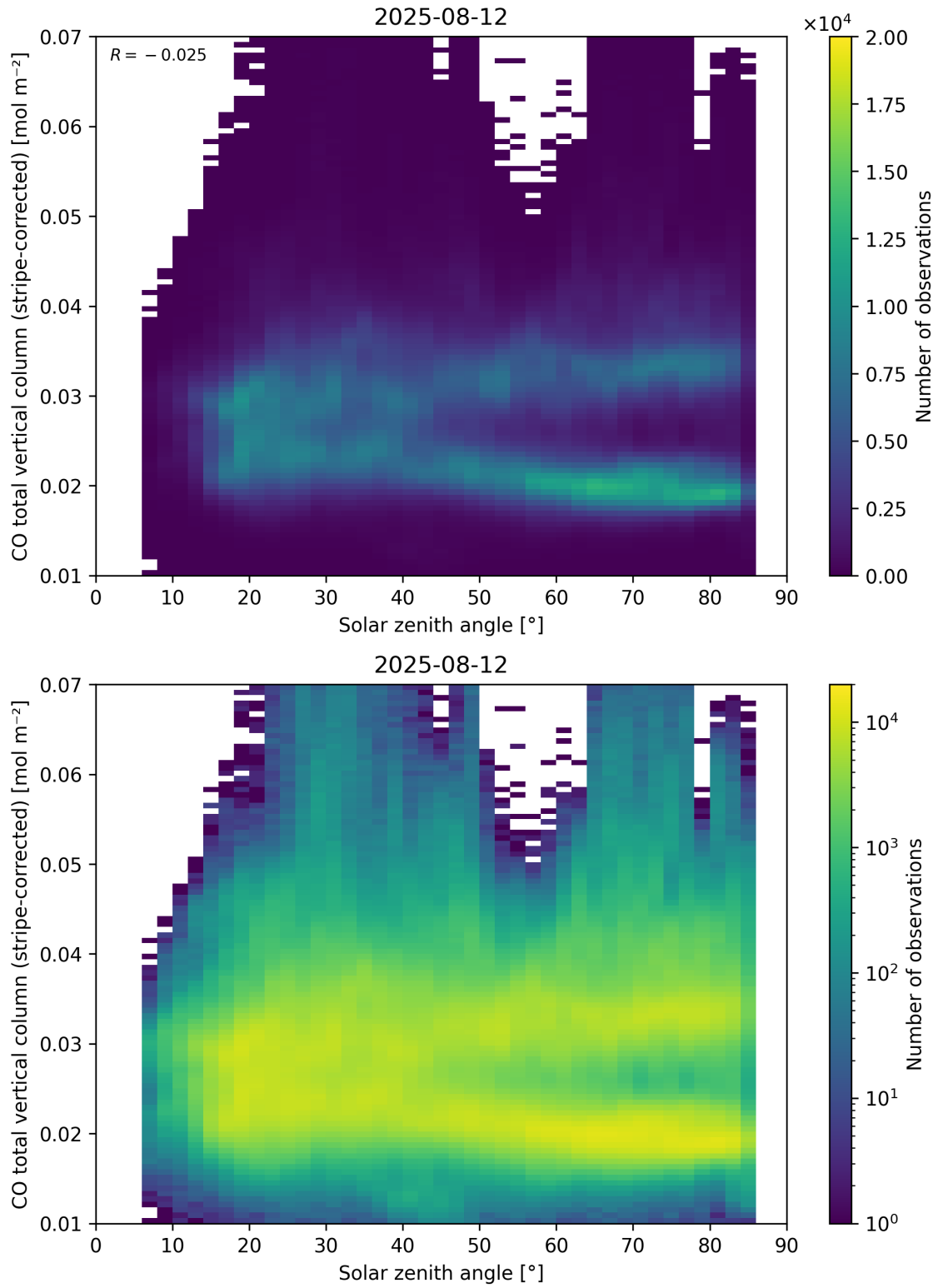
Figure 62: Scatter density plot of “Solar zenith angle” against “CO total vertical column (stripe-corrected)” for 2025-08-11 to 2025-08-13.
