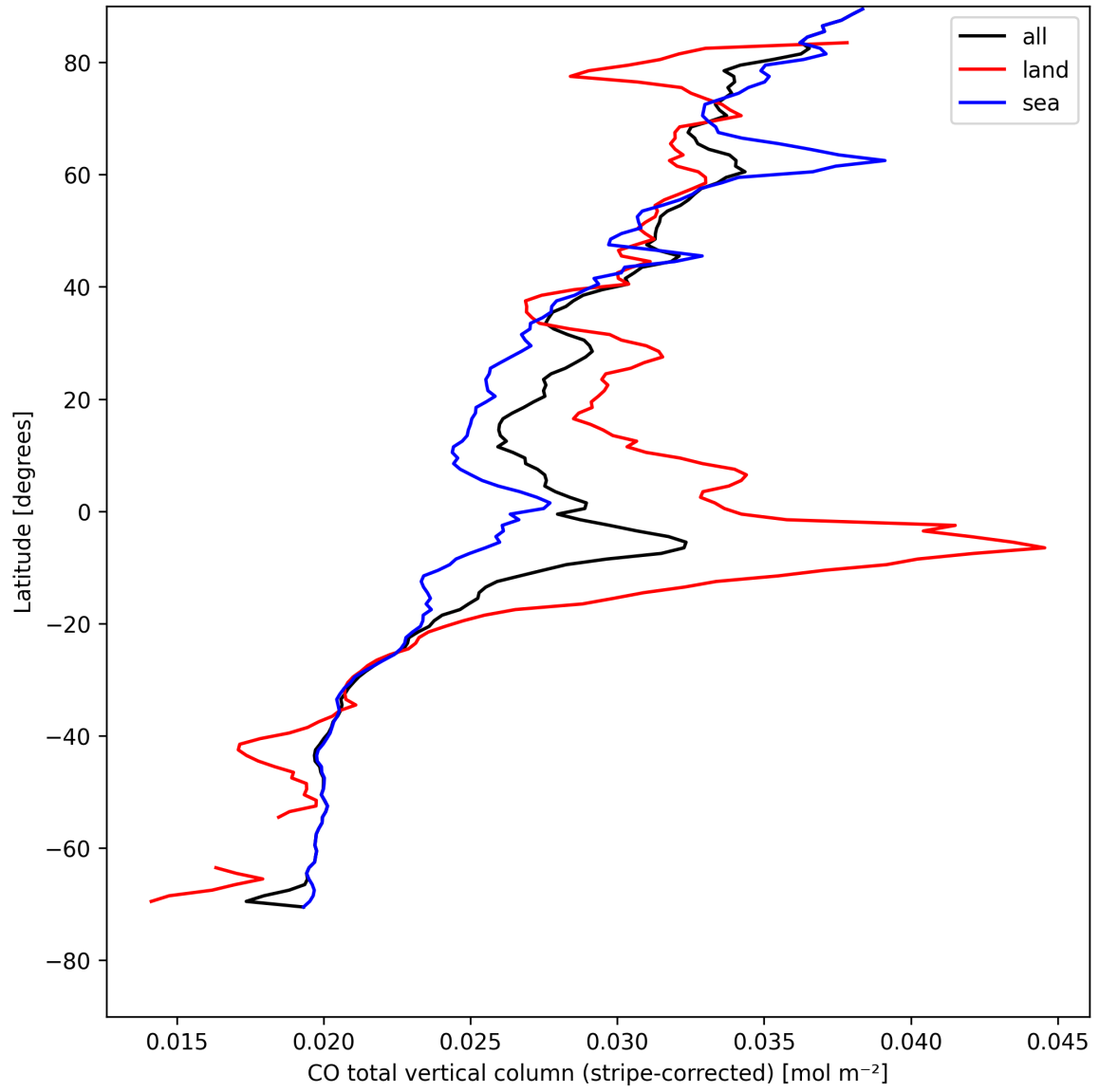
Figure 11: Zonal average of “CO total vertical column (stripe-corrected)” for 2025-08-11 to 2025-08-13.
