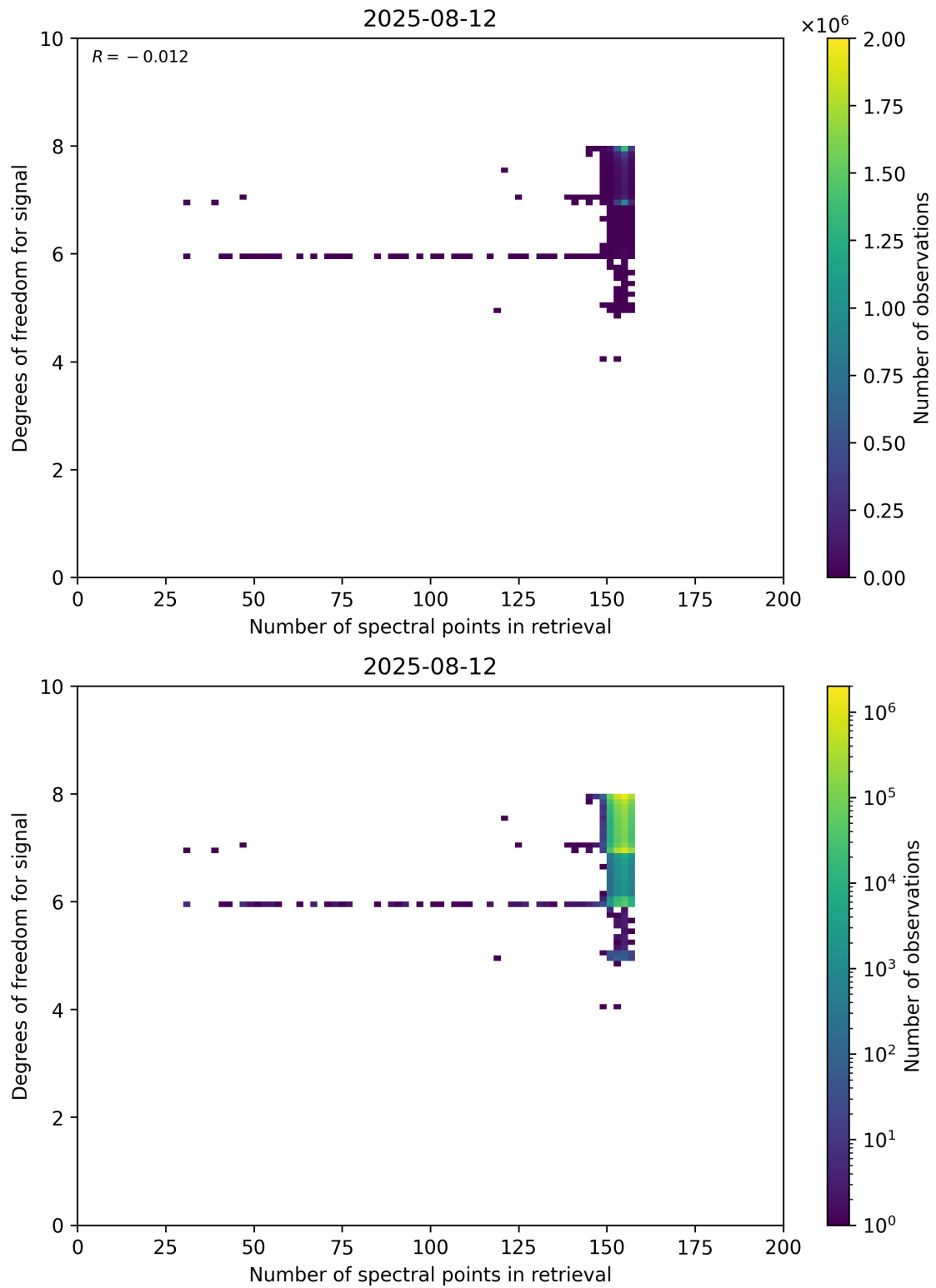
Figure 59: Scatter density plot of “Number of spectral points in retrieval” against “Degrees of freedom for signal” for 2025-08-11 to 2025-08-13.
