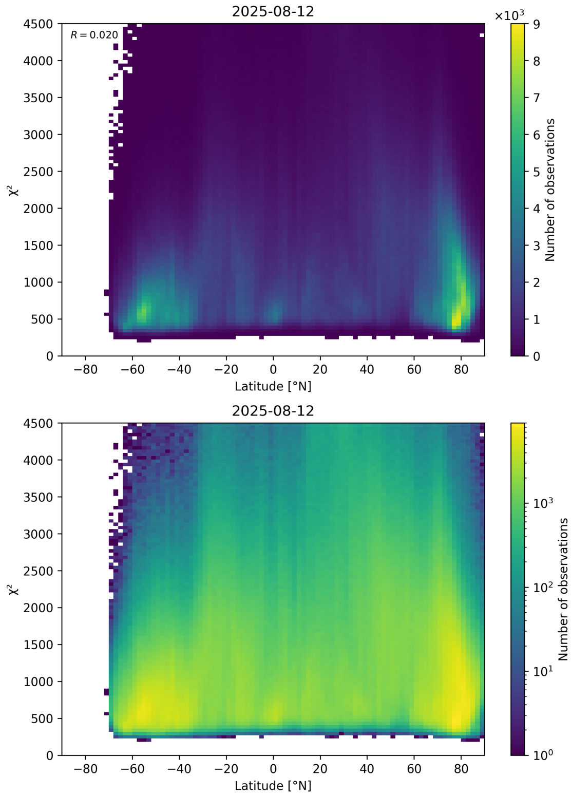
Figure 54: Scatter density plot of “Latitude” against “ \chi^2 ” for 2025-08-11 to 2025-08-13.
