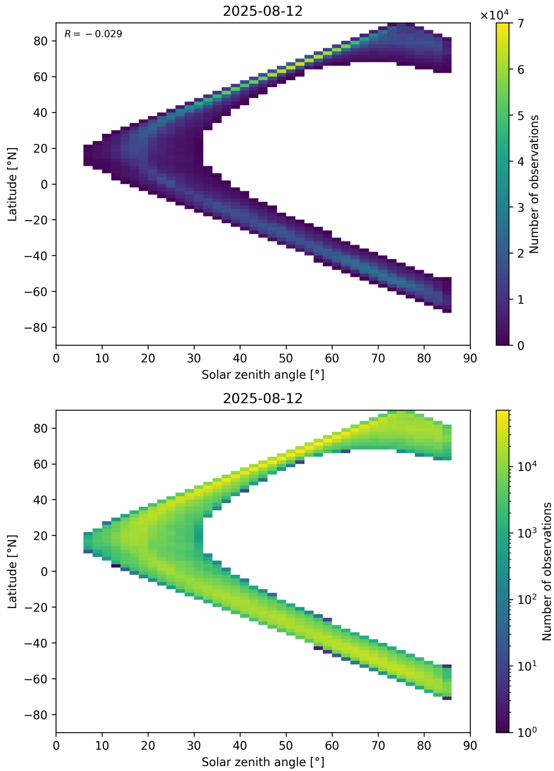
Figure 66: Scatter density plot of “Solar zenith angle” against “Latitude” for 2025-08-11 to 2025-08-13.
