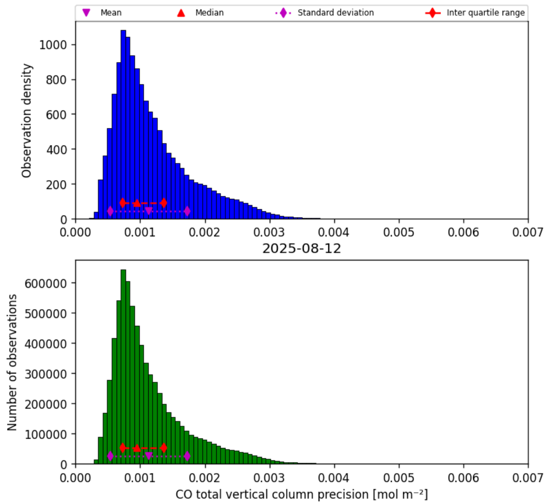
Figure 20: Histogram of “CO total vertical column precision” for 2025-08-11 to 2025-08-13
