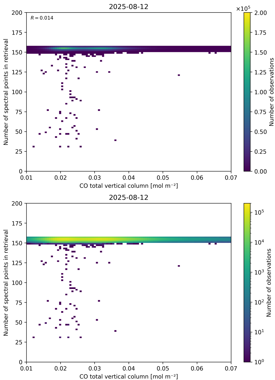
Figure 43: Scatter density plot of “CO total vertical column” against “Number of spectral points in retrieval” for 2025-08-11 to 2025-08-13.
