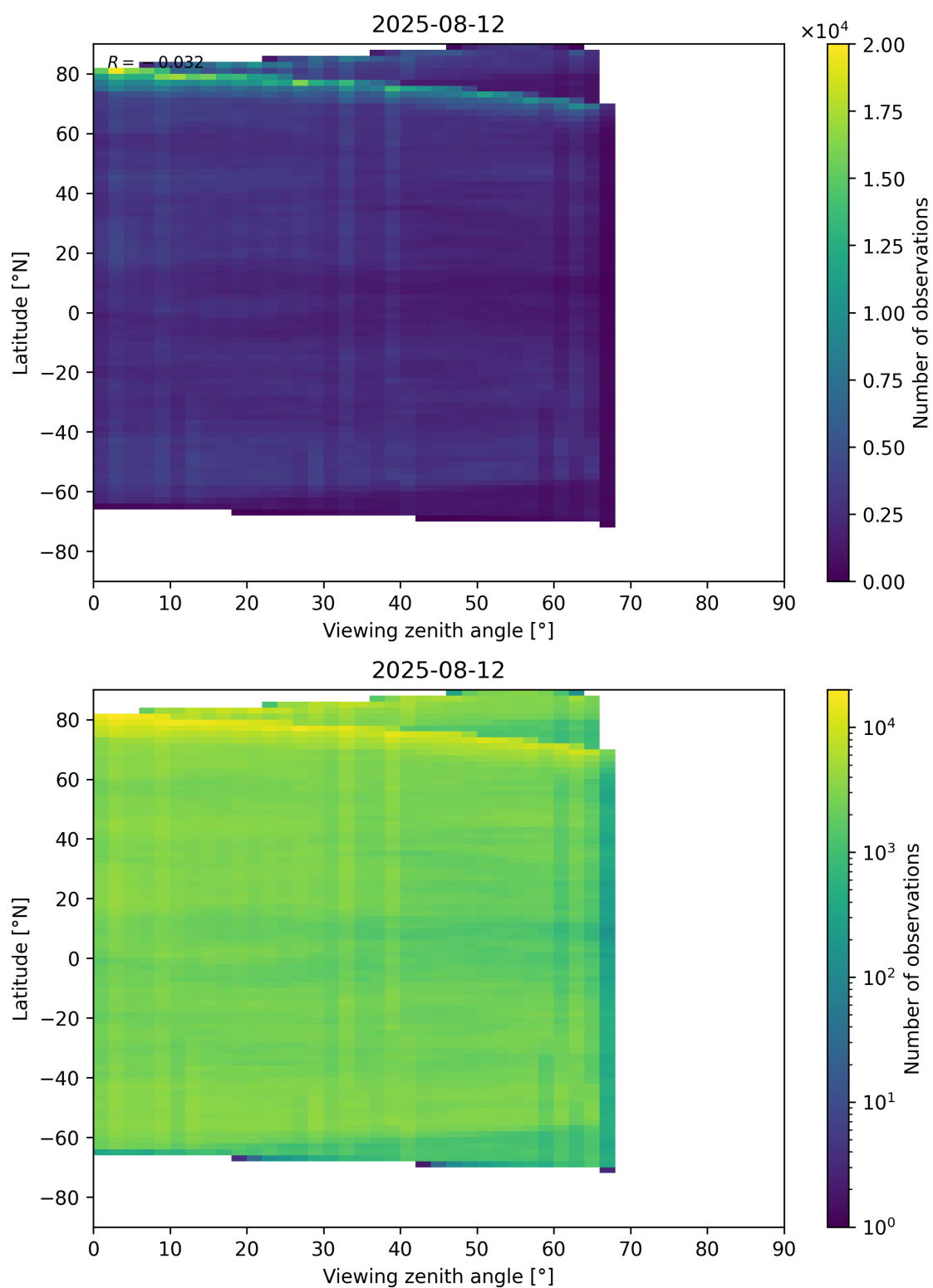
Figure 74: Scatter density plot of “Viewing zenith angle” against “Latitude” for 2025-08-11 to 2025-08-13.
