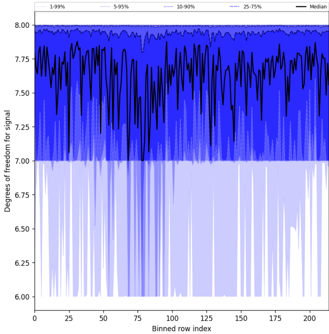
Figure 31: Along track statistics of “Degrees of freedom for signal” for 2025-08-11 to 2025-08-13
