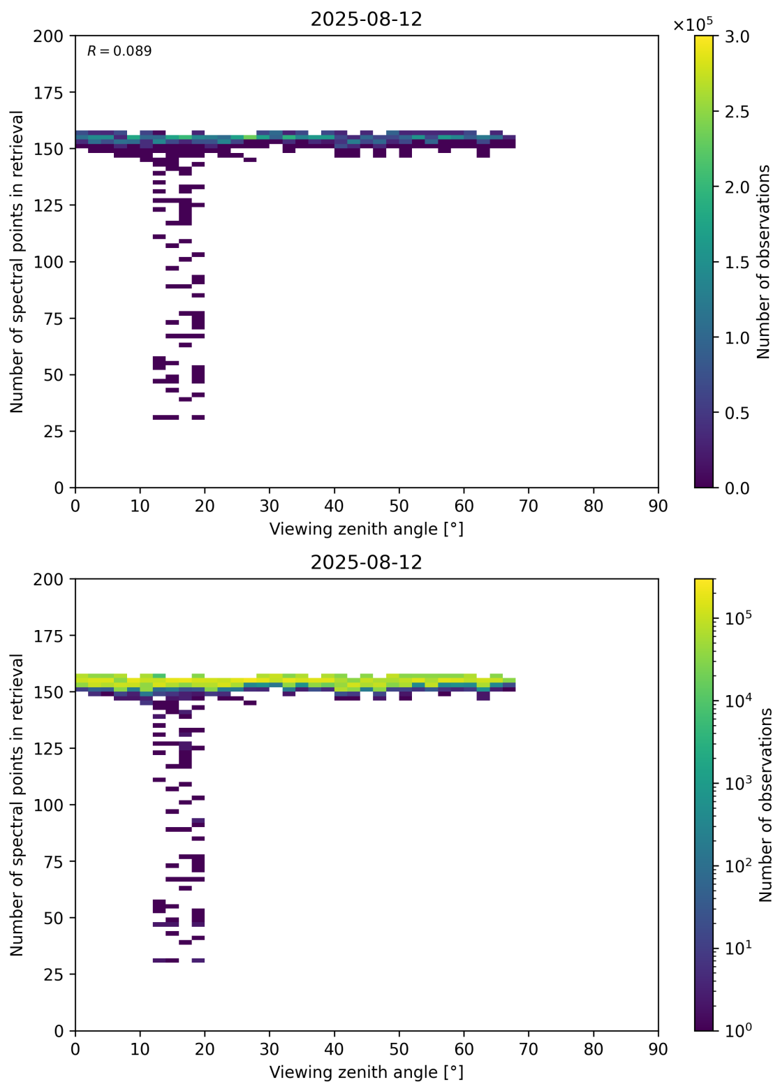
Figure 76: Scatter density plot of “Viewing zenith angle” against “Number of spectral points in retrieval” for 2025-08-11 to 2025-08-13.
