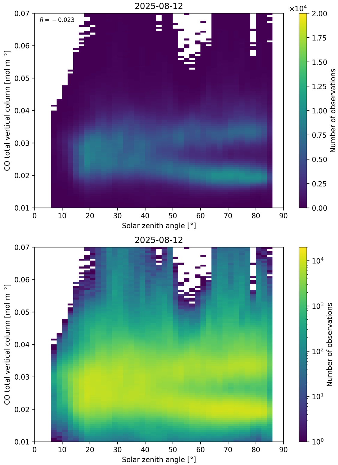
Figure 61: Scatter density plot of “Solar zenith angle” against “CO total vertical column” for 2025-08-11 to 2025-08-13.
