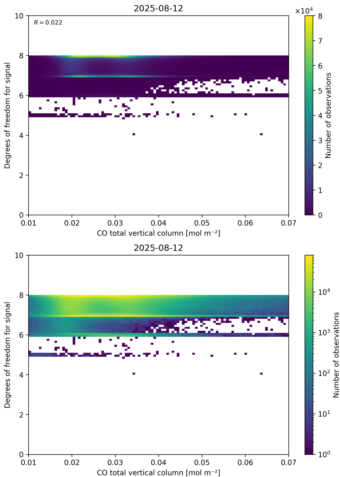
Figure 41: Scatter density plot of “CO total vertical column” against “Degrees of freedom for signal” for 2025-08-11 to 2025-08-13.
