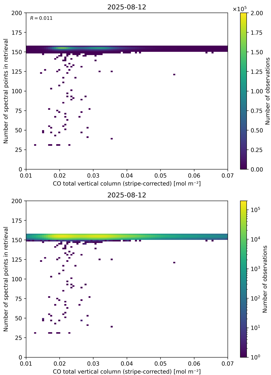
Figure 40: Scatter density plot of “CO total vertical column (stripe-corrected)” against “Number of spectral points in retrieval” for 2025-08-11 to 2025-08-13.
