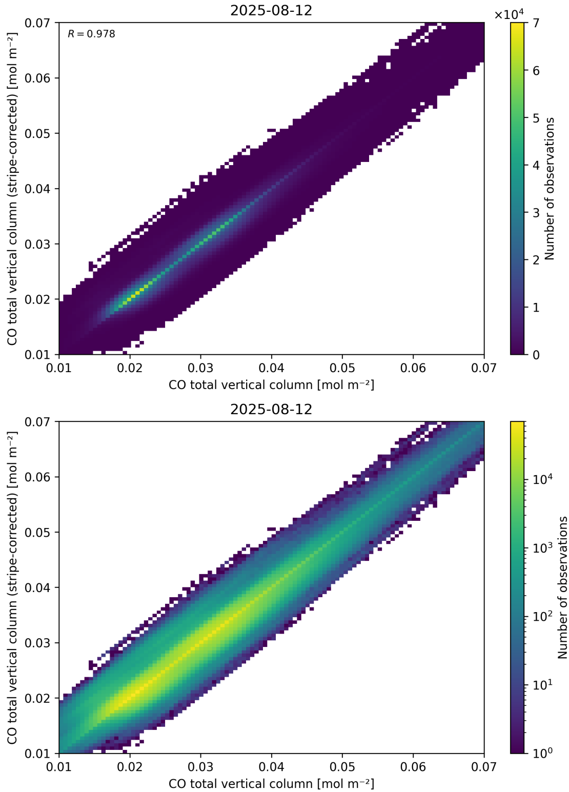
Figure 33: Scatter density plot of “CO total vertical column” against “CO total vertical column (stripe-corrected)” for 2025-08-11 to 2025-08-13.
