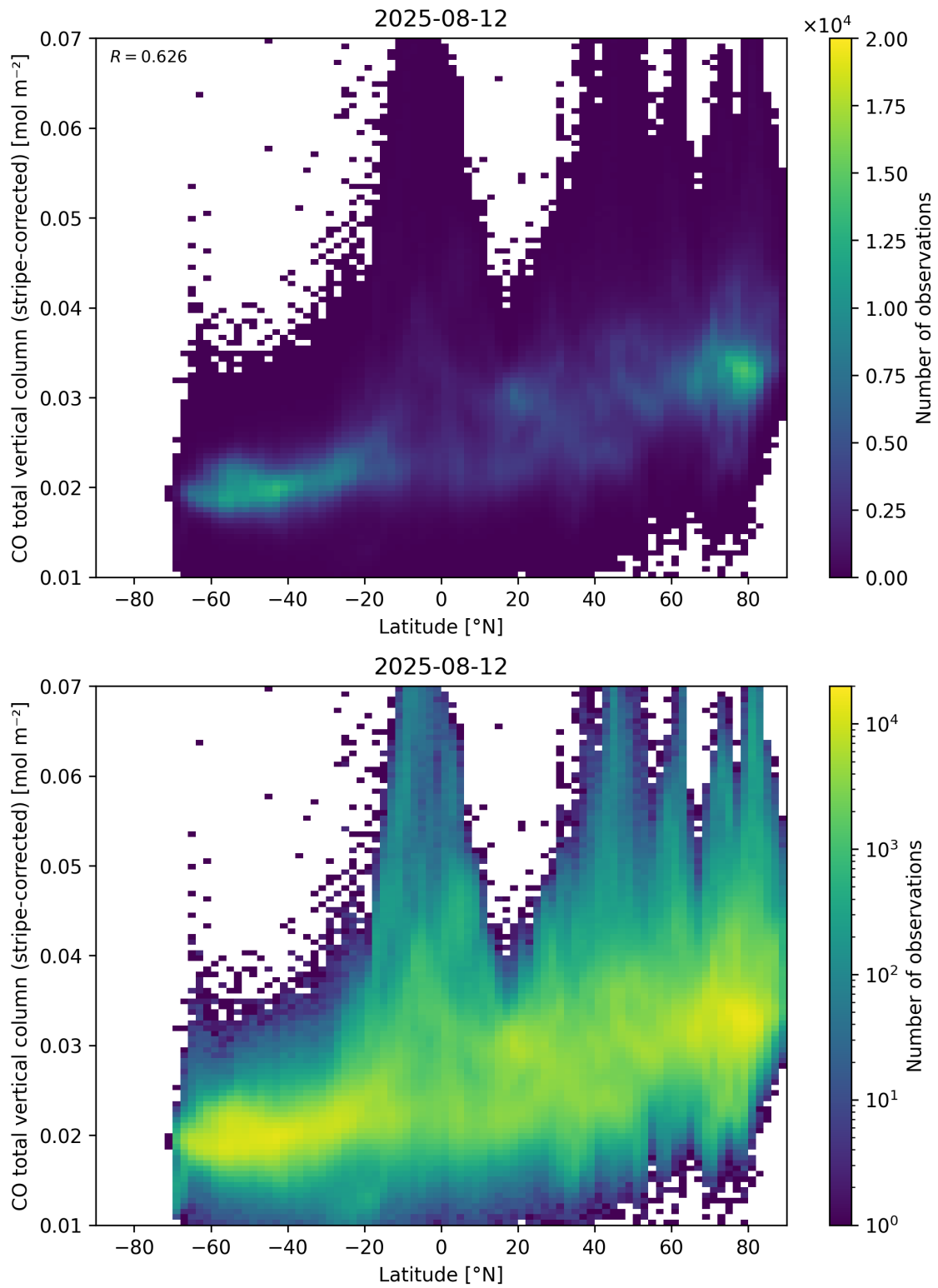
Figure 52: Scatter density plot of “Latitude” against “CO total vertical column (stripe-corrected)” for 2025-08-11 to 2025-08-13.
