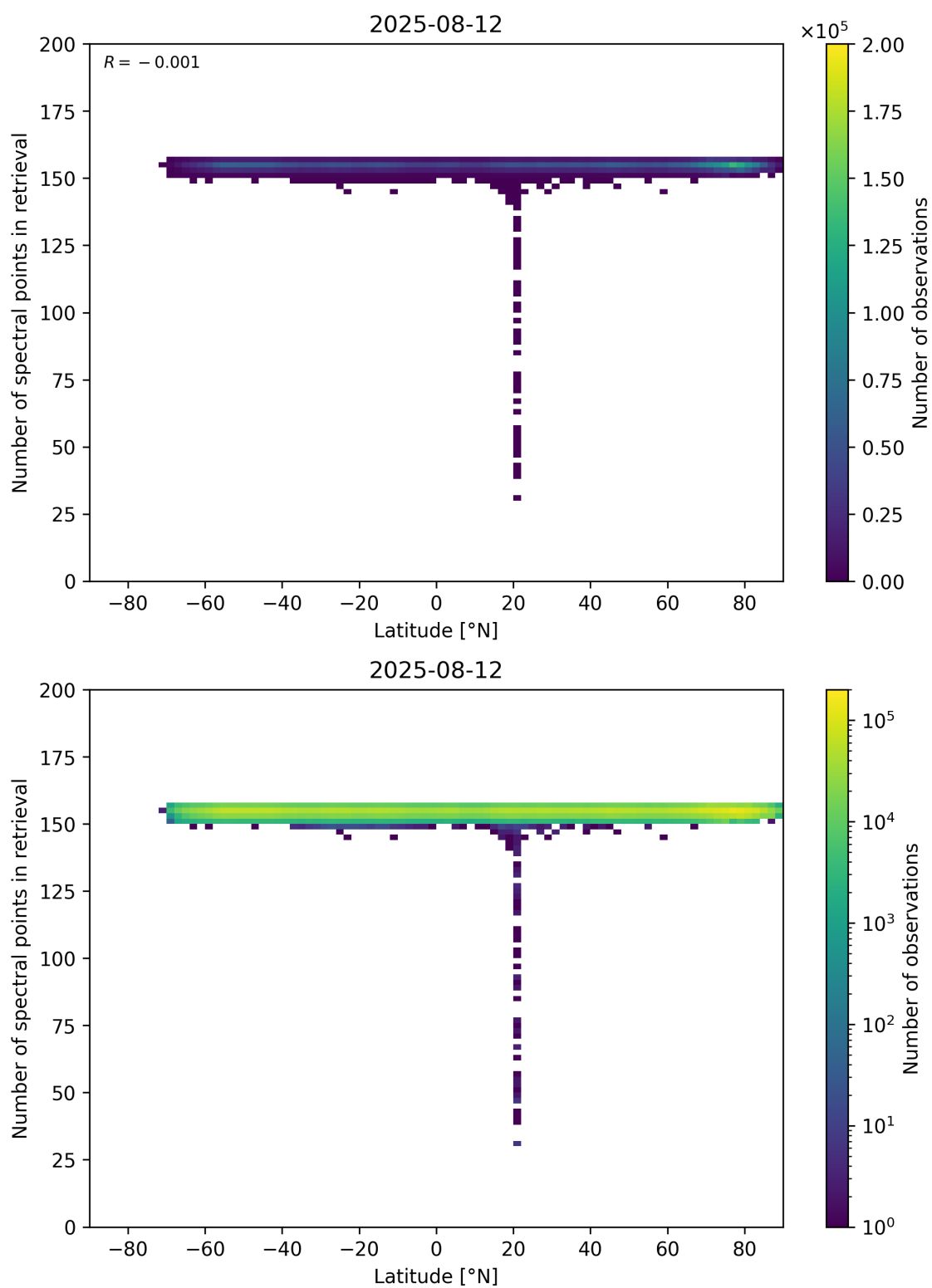
Figure 57: Scatter density plot of “Latitude” against “Number of spectral points in retrieval” for 2025-08-11 to 2025-08-13.
