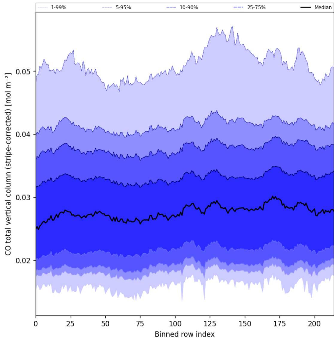
Figure 27: Along track statistics of “CO total vertical column (stripe-corrected)” for 2025-08-11 to 2025-08-13
