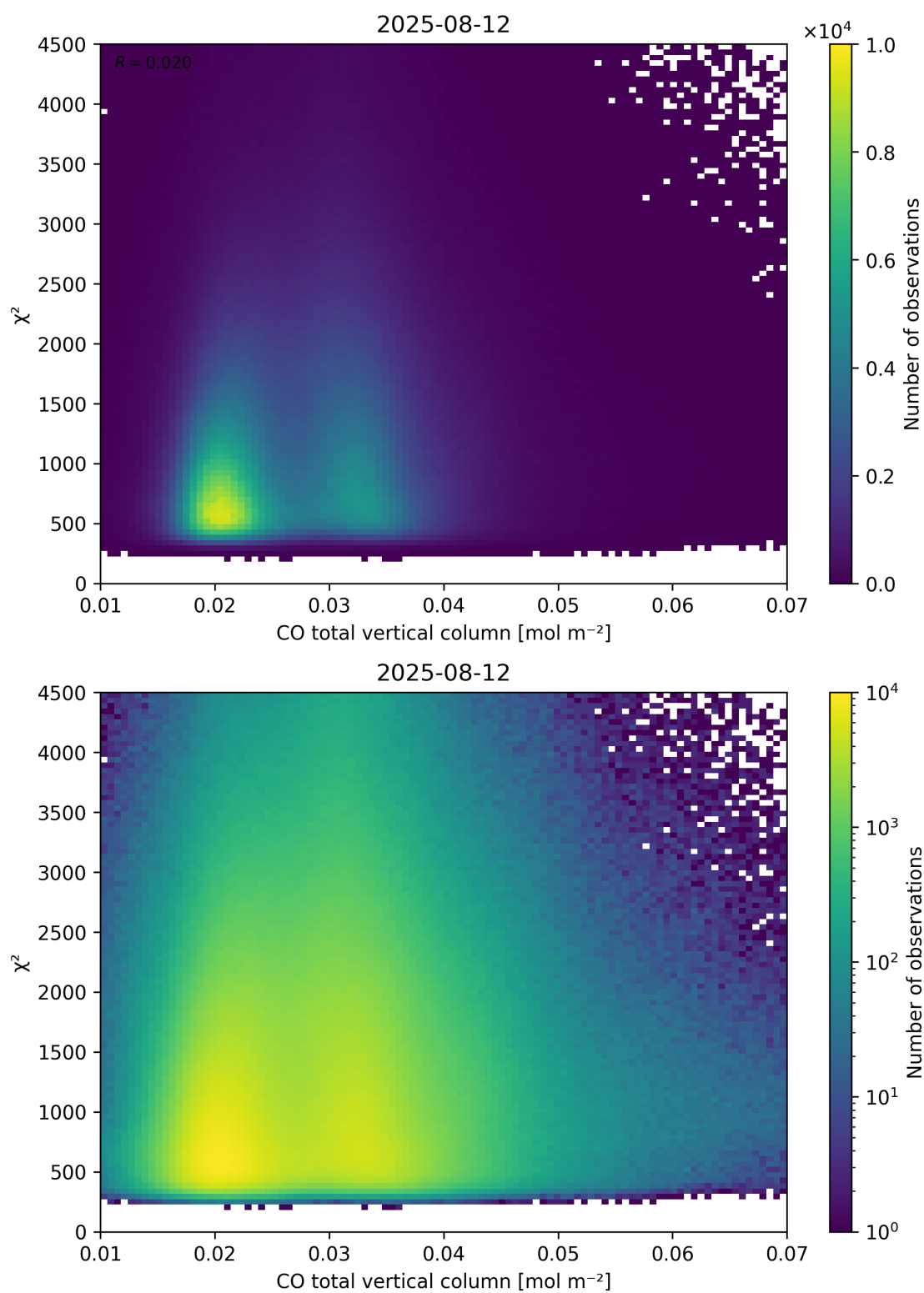
Figure 35: Scatter density plot of “CO total vertical column” against “ \chi^2 ” for 2025-08-11 to 2025-08-13.
