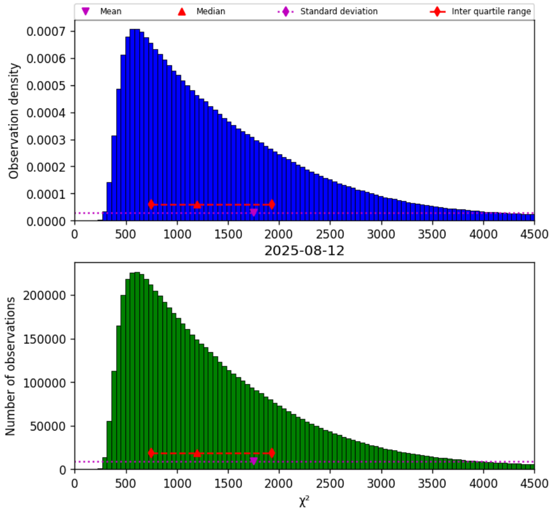
Figure 22: Histogram of “ \chi^2 ” for 2025-08-11 to 2025-08-13
