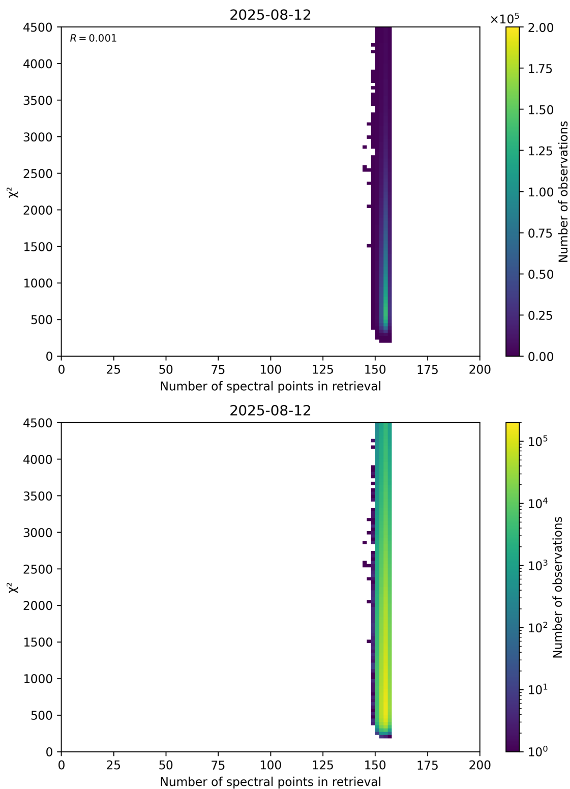
Figure 58: Scatter density plot of “Number of spectral points in retrieval” against “ \chi^2 ” for 2025-08-11 to 2025-08-13.
