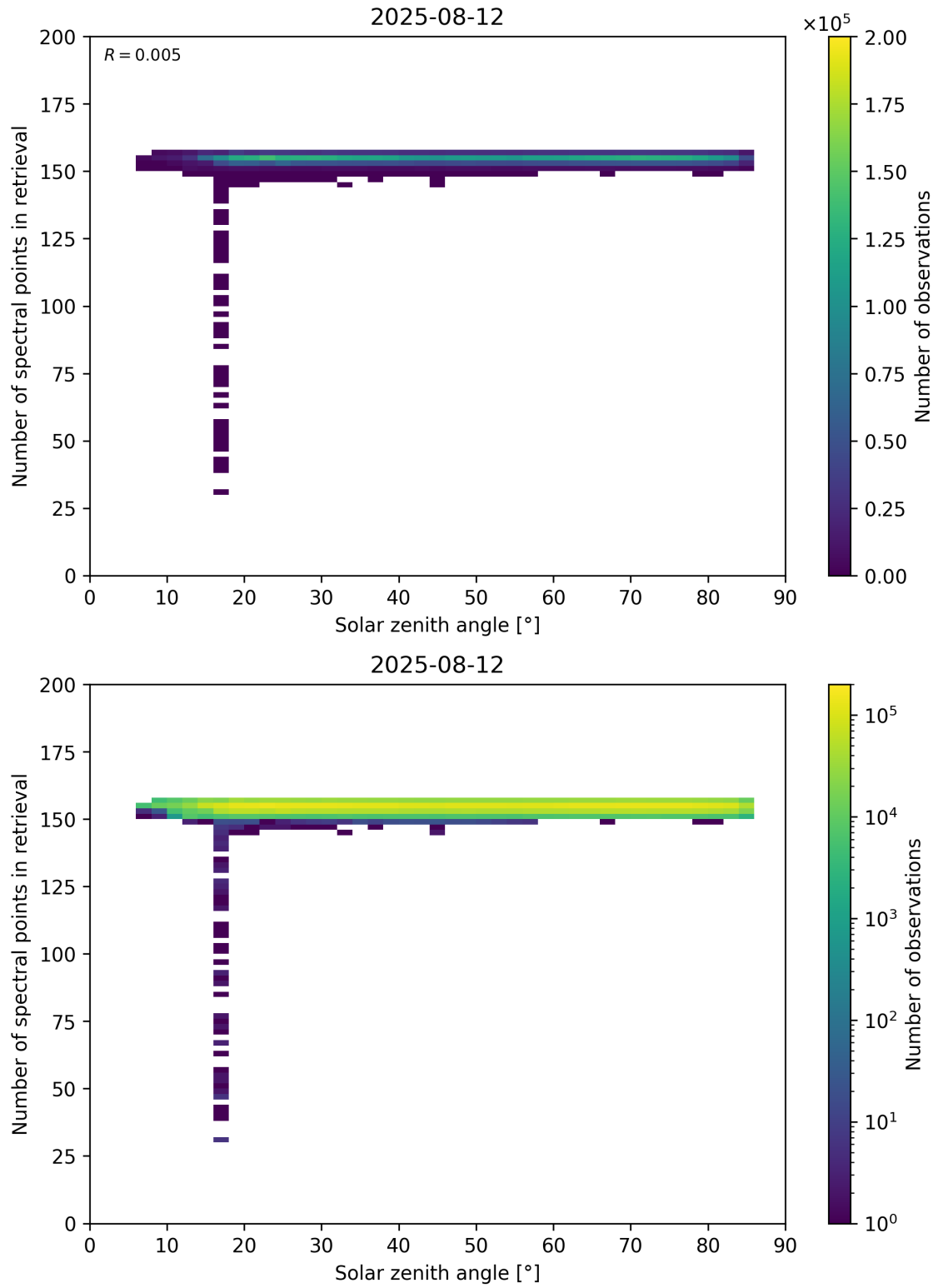
Figure 68: Scatter density plot of “Solar zenith angle” against “Number of spectral points in retrieval” for 2025-08-11 to 2025-08-13.
