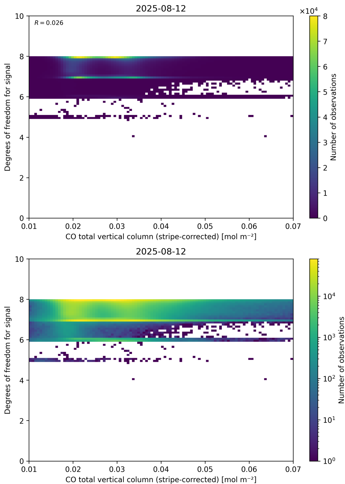
Figure 38: Scatter density plot of “CO total vertical column (stripe-corrected)” against “Degrees of freedom for signal” for 2025-08-11 to 2025-08-13.
