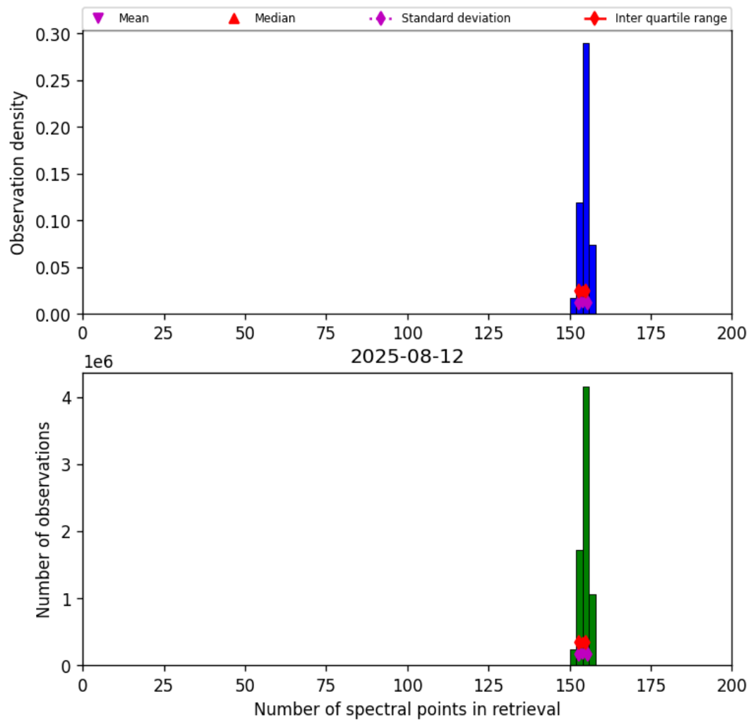
Figure 21: Histogram of “Number of spectral points in retrieval” for 2025-08-11 to 2025-08-13
