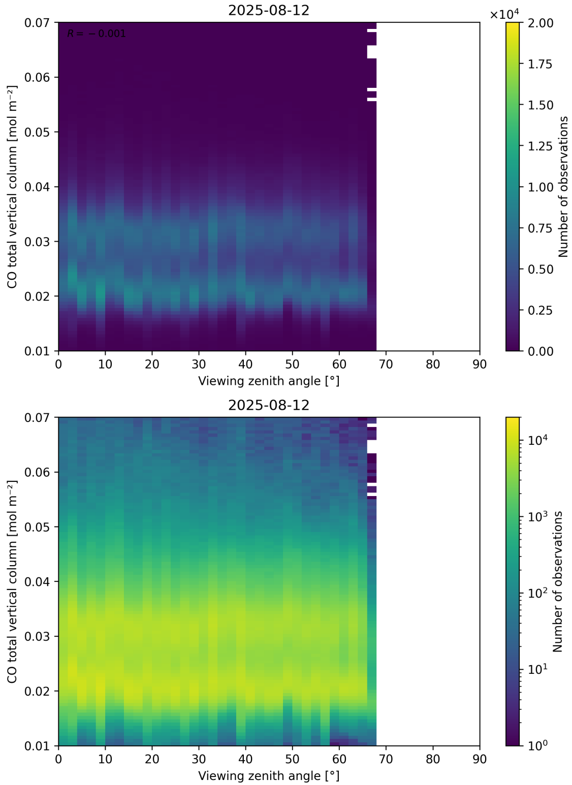
Figure 69: Scatter density plot of “Viewing zenith angle” against “CO total vertical column” for 2025-08-11 to 2025-08-13.
