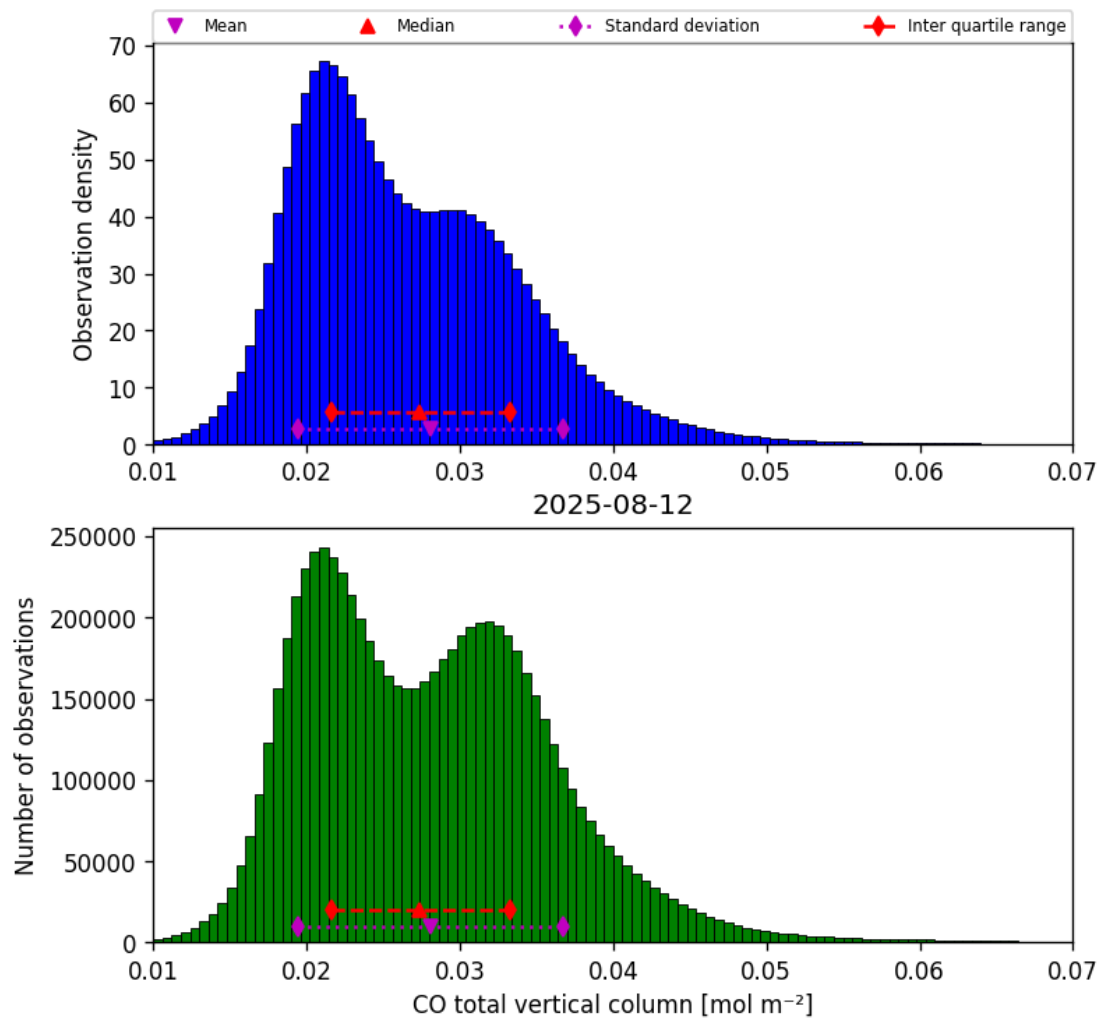
Figure 18: Histogram of “CO total vertical column” for 2025-08-11 to 2025-08-13
