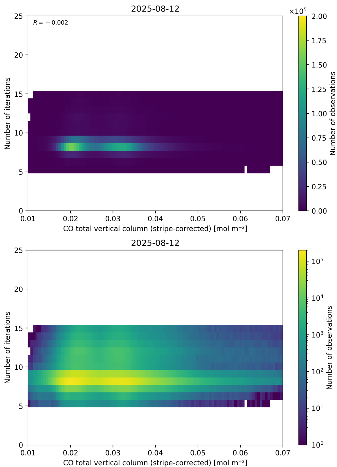
Figure 39: Scatter density plot of “CO total vertical column (stripe-corrected)” against “Number of iterations” for 2025-08-11 to 2025-08-13.
