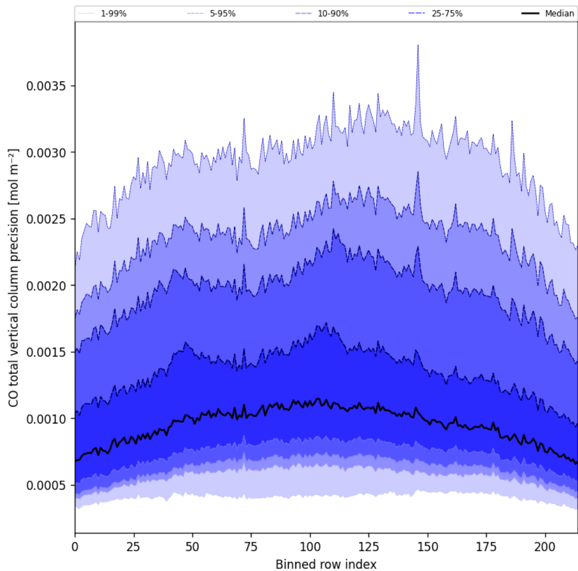
Figure 28: Along track statistics of “CO total vertical column precision” for 2025-08-11 to 2025-08-13
