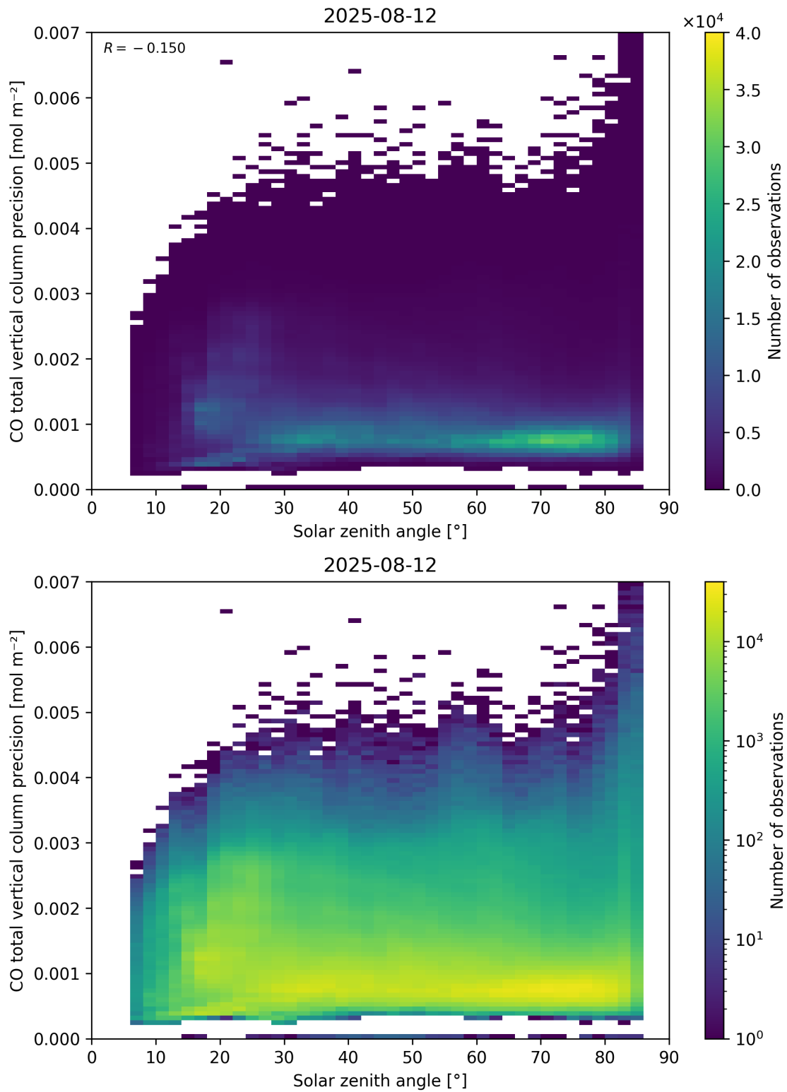
Figure 63: Scatter density plot of “Solar zenith angle” against “CO total vertical column precision” for 2025-08-11 to 2025-08-13.
