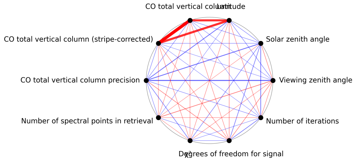
Figure 1: Map of correlation graph for 2025-08-11 to 2025-08-13.
