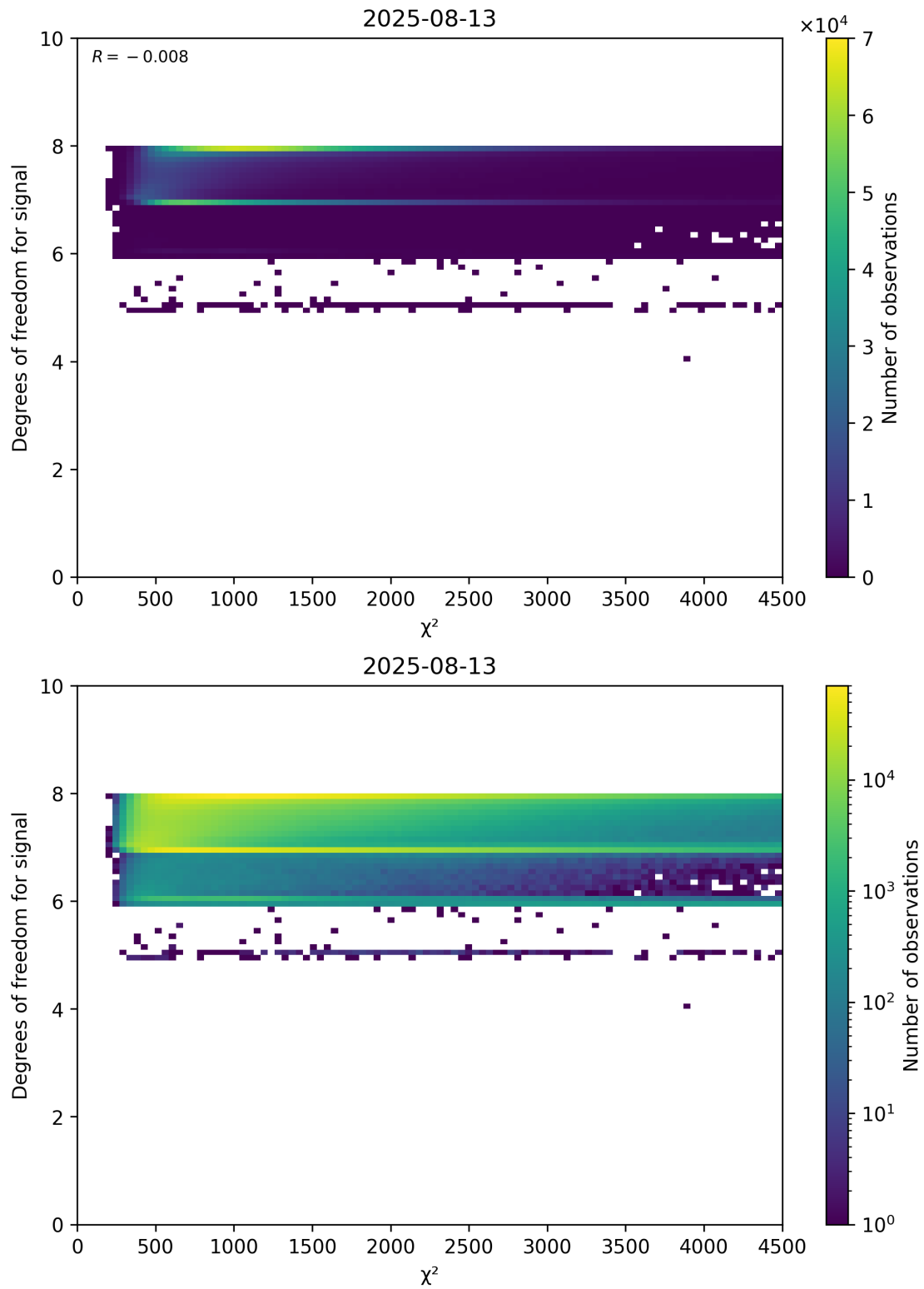
Figure 48: Scatter density plot of " \chi^2 " against "Degrees of freedom for signal" for 2025-08-12 to 2025-08-14.
