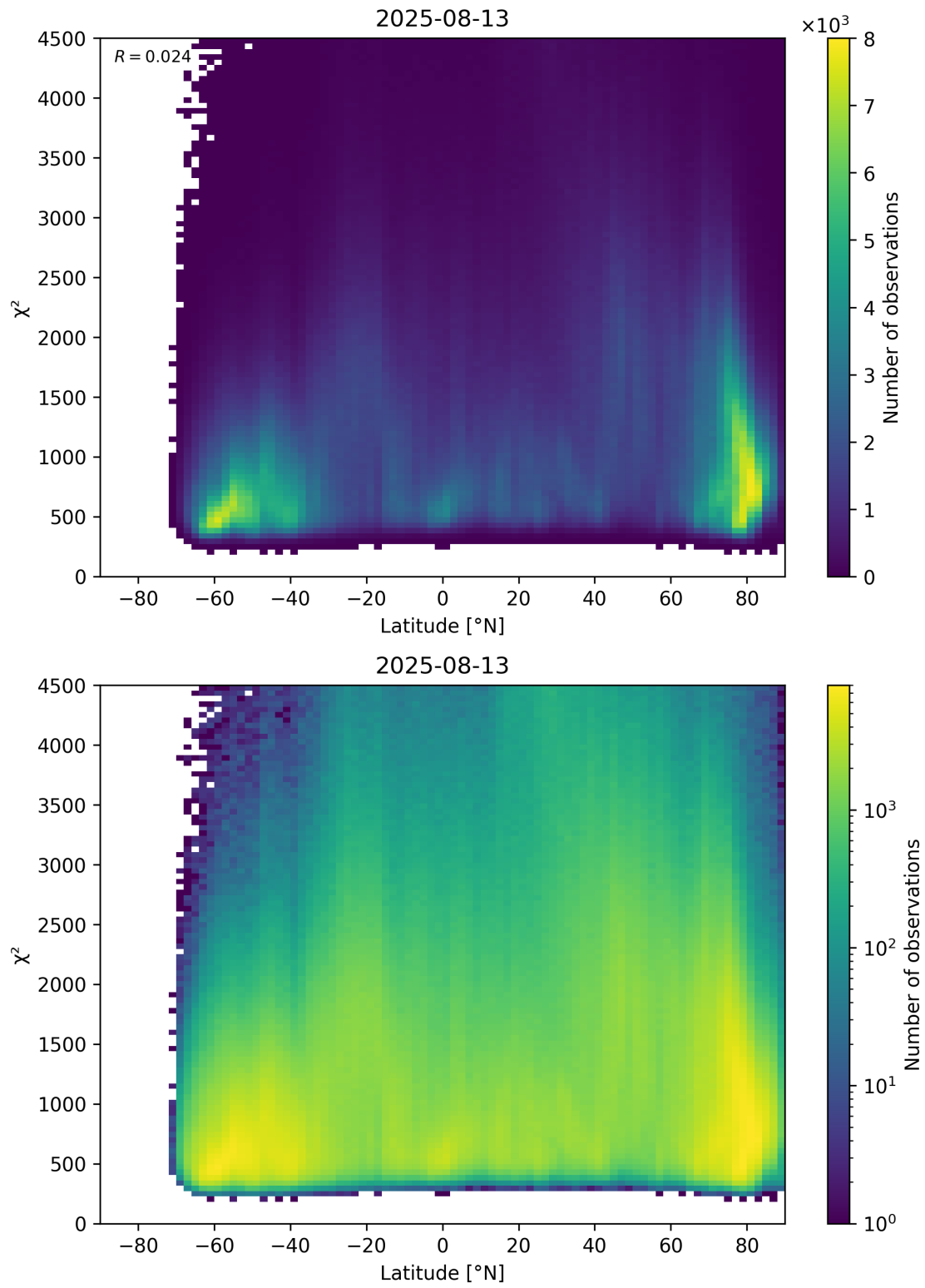
Figure 54: Scatter density plot of “Latitude” against “ \chi^2 ” for 2025-08-12 to 2025-08-14.
