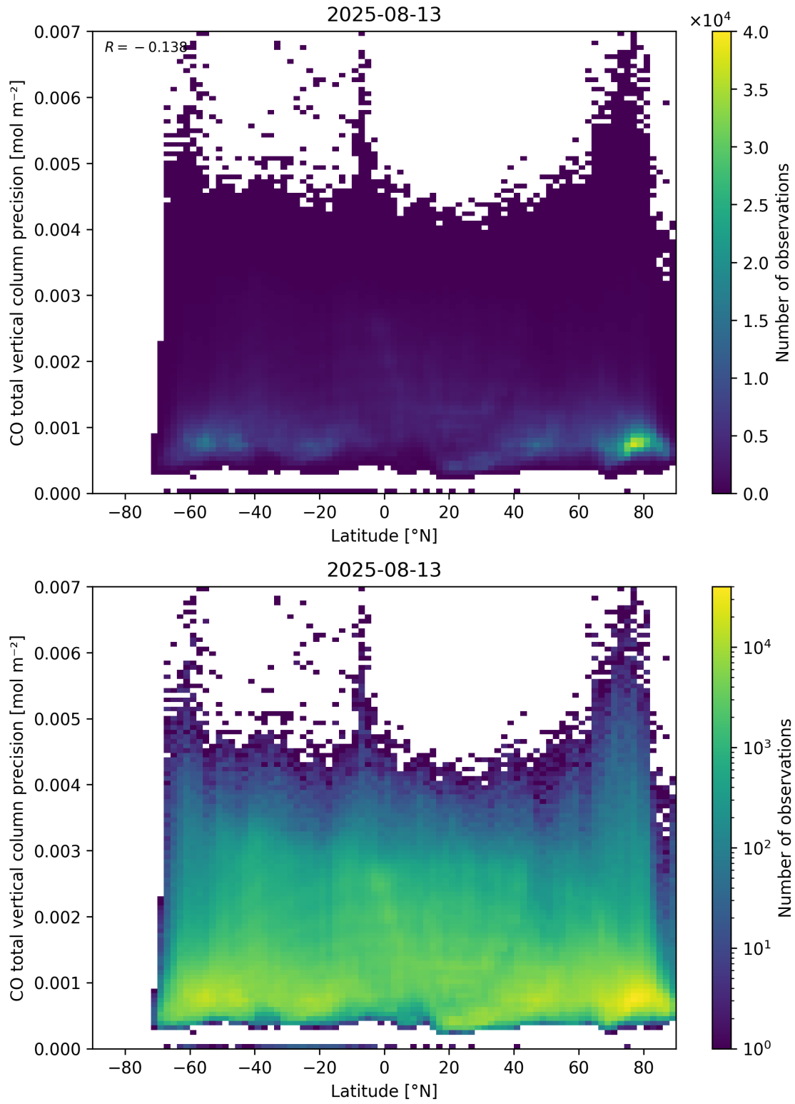
Figure 53: Scatter density plot of “Latitude” against “CO total vertical column precision” for 2025-08-12 to 2025-08-14.
