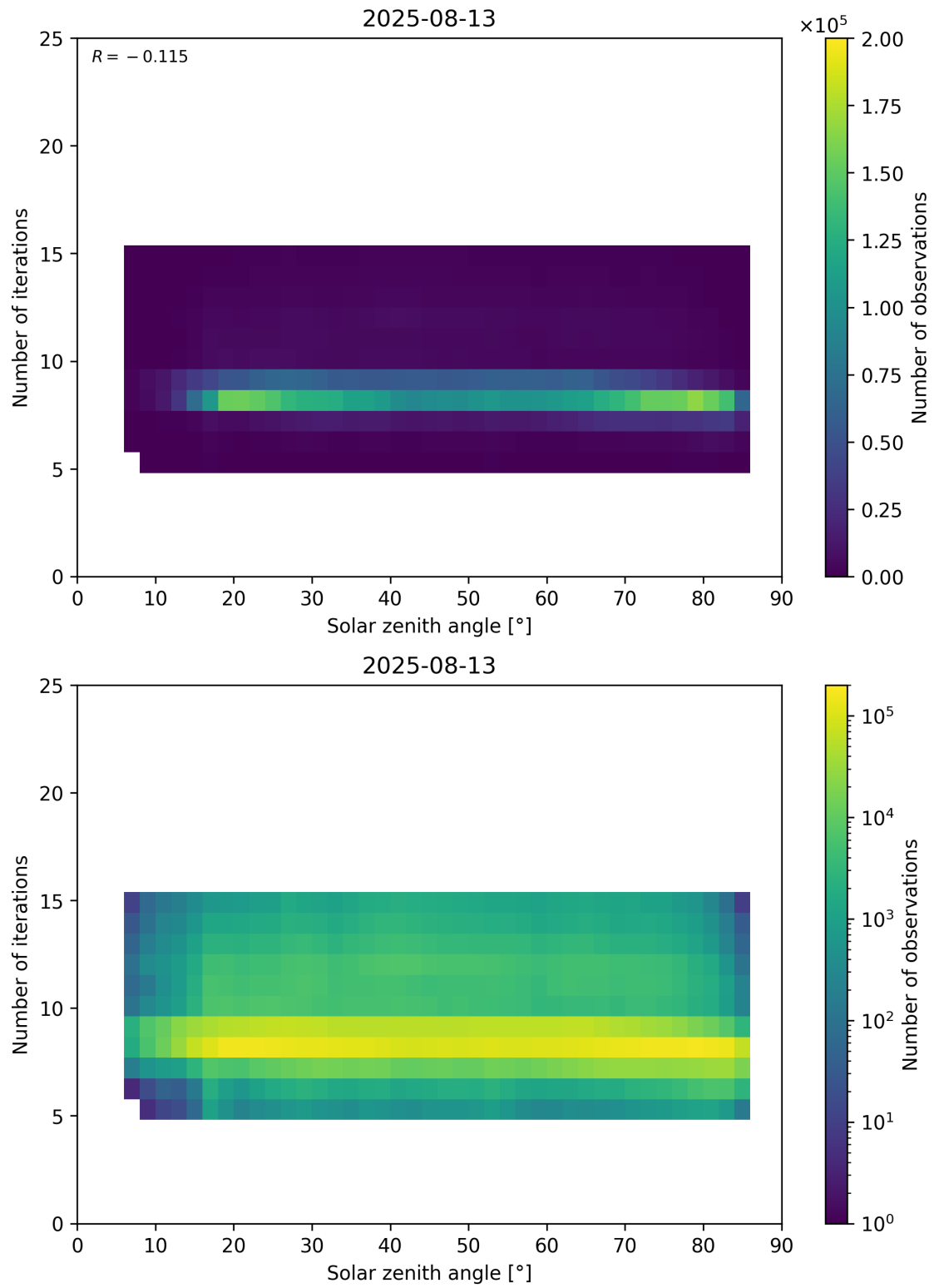
Figure 67: Scatter density plot of “Solar zenith angle” against “Number of iterations” for 2025-08-12 to 2025-08-14.
