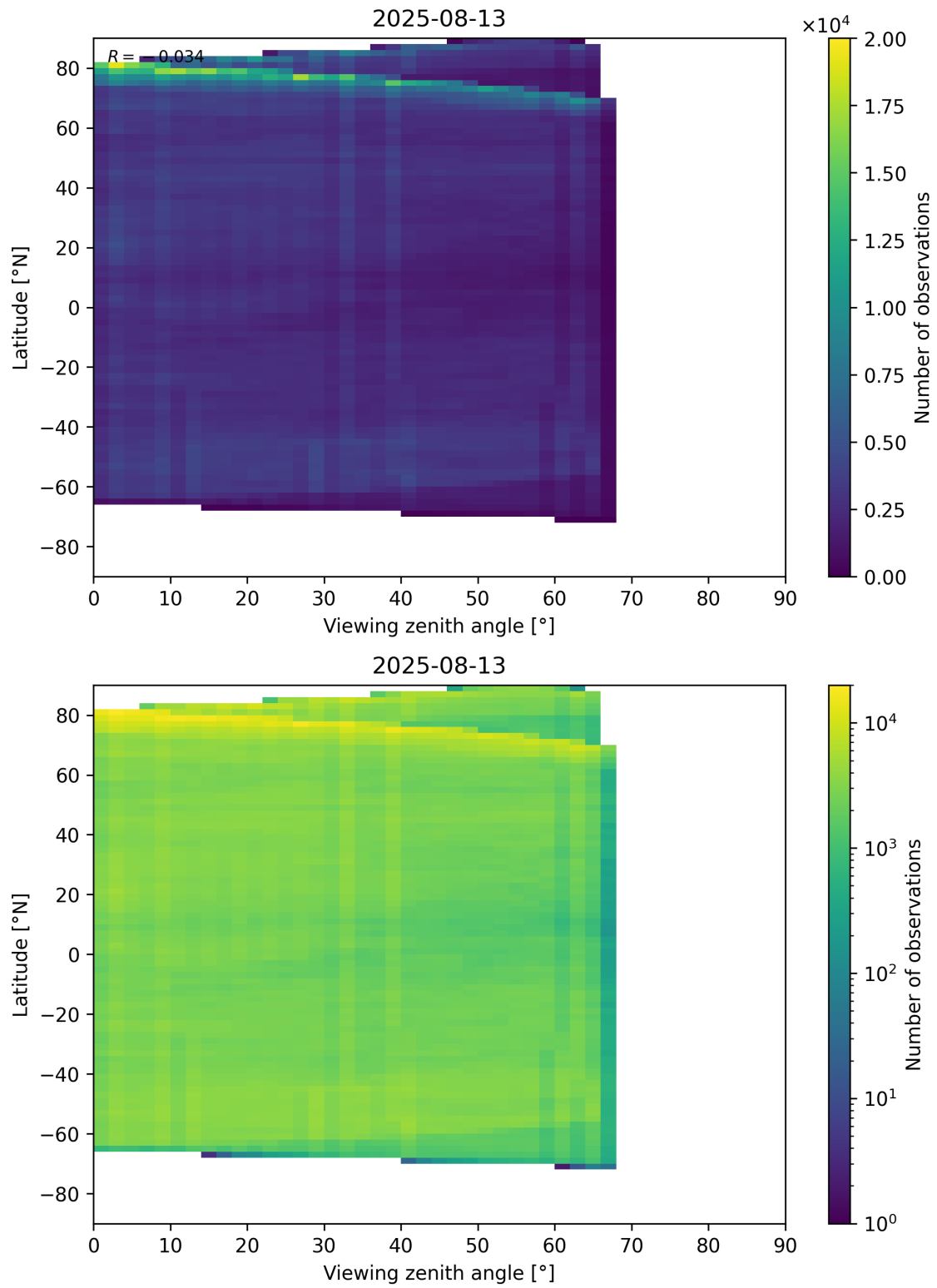
Figure 74: Scatter density plot of “Viewing zenith angle” against “Latitude” for 2025-08-12 to 2025-08-14.
