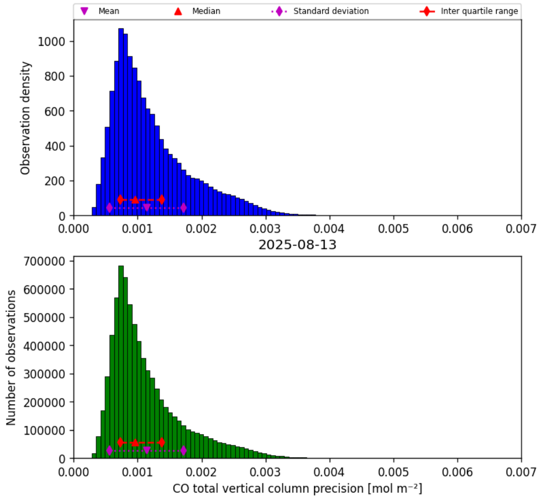
Figure 20: Histogram of “CO total vertical column precision” for 2025-08-12 to 2025-08-14
