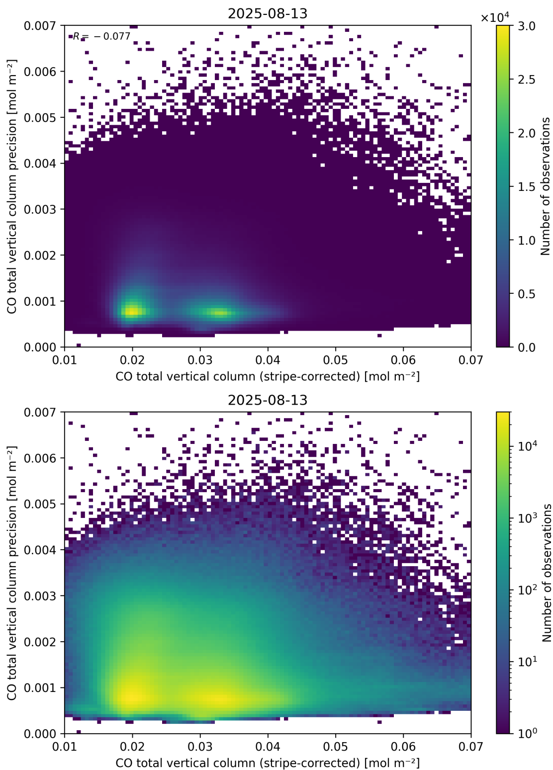
Figure 36: Scatter density plot of “CO total vertical column (stripe-corrected)” against “CO total vertical column precision” for 2025-08-12 to 2025-08-14.
