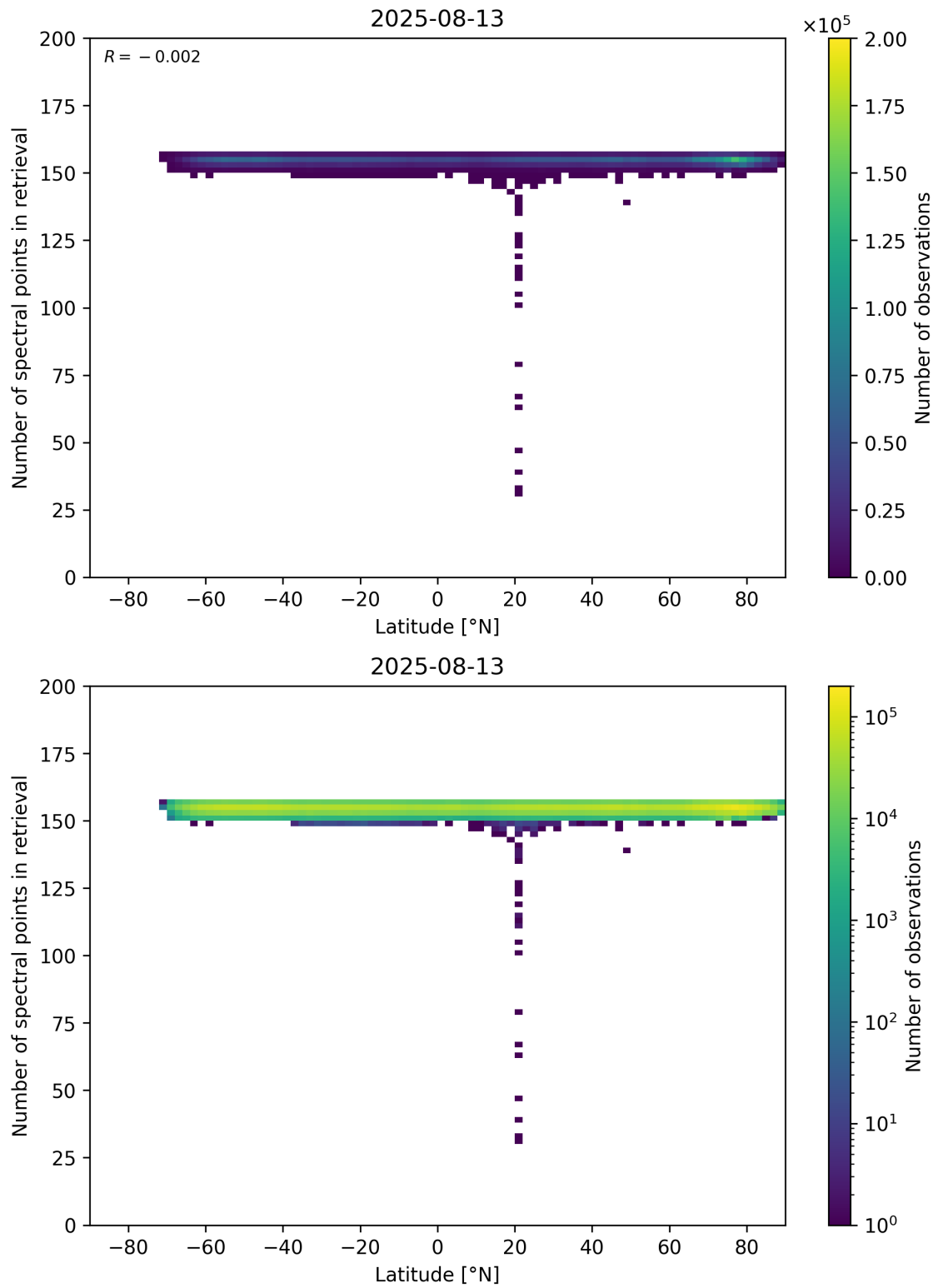
Figure 57: Scatter density plot of “Latitude” against “Number of spectral points in retrieval” for 2025-08-12 to 2025-08-14.
