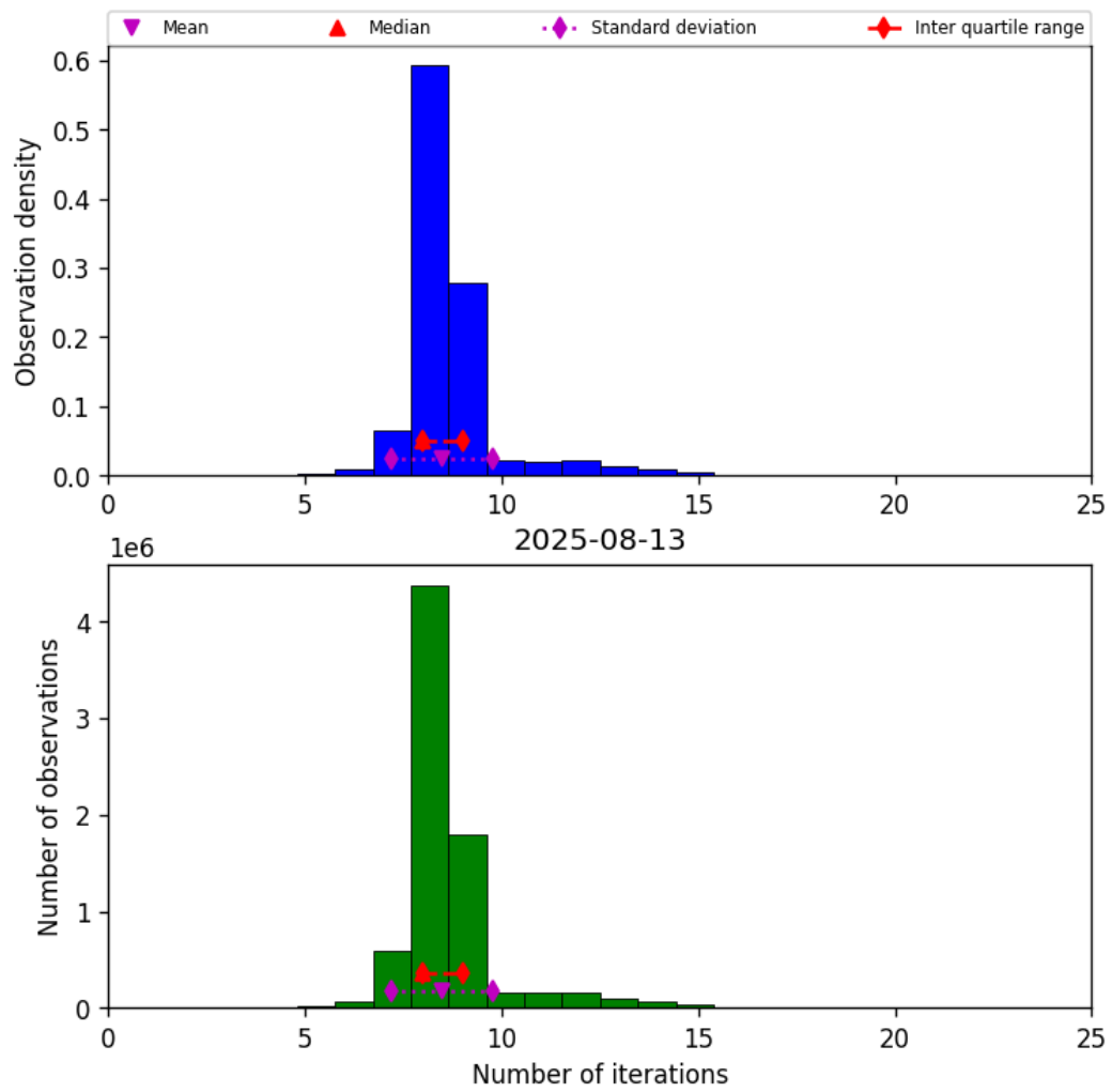
Figure 24: Histogram of “Number of iterations” for 2025-08-12 to 2025-08-14
