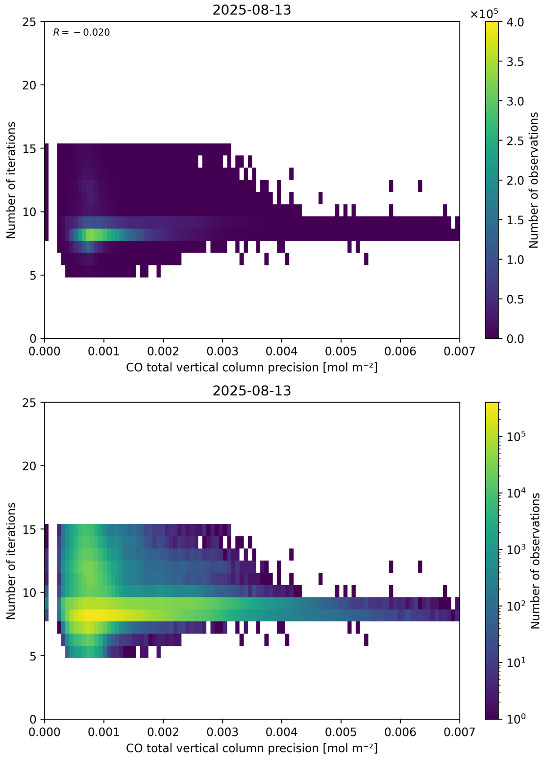
Figure 46: Scatter density plot of “CO total vertical column precision” against “Number of iterations” for 2025-08-12 to 2025-08-14.
