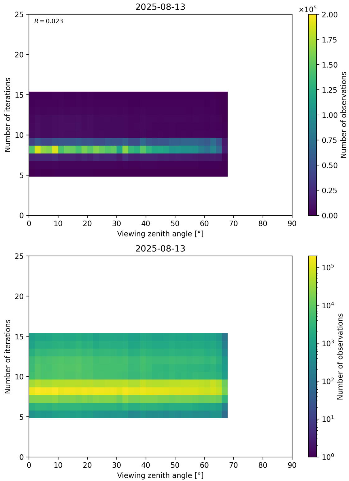
Figure 75: Scatter density plot of “Viewing zenith angle” against “Number of iterations” for 2025-08-12 to 2025-08-14.
