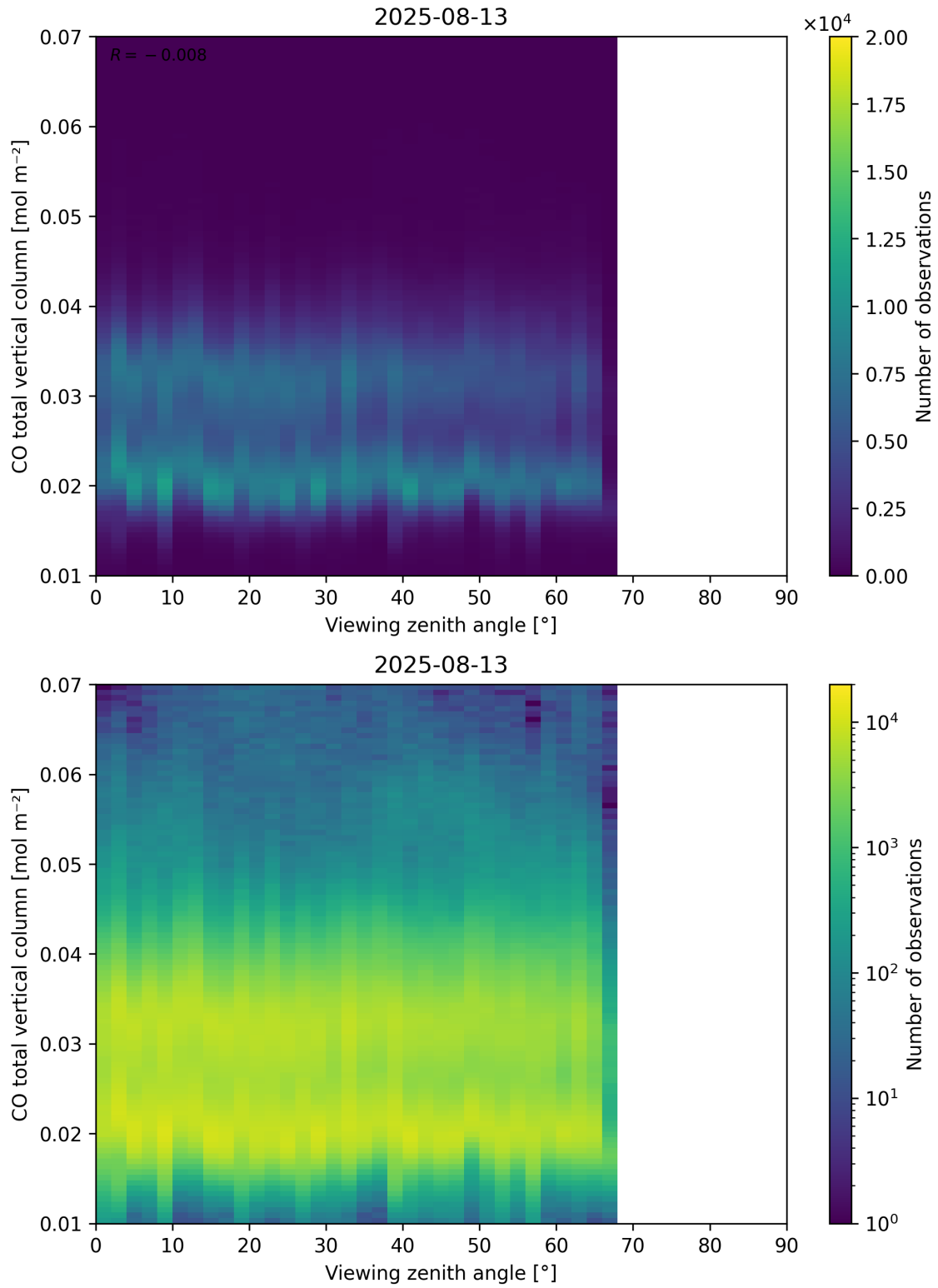
Figure 69: Scatter density plot of “Viewing zenith angle” against “CO total vertical column” for 2025-08-12 to 2025-08-14.
