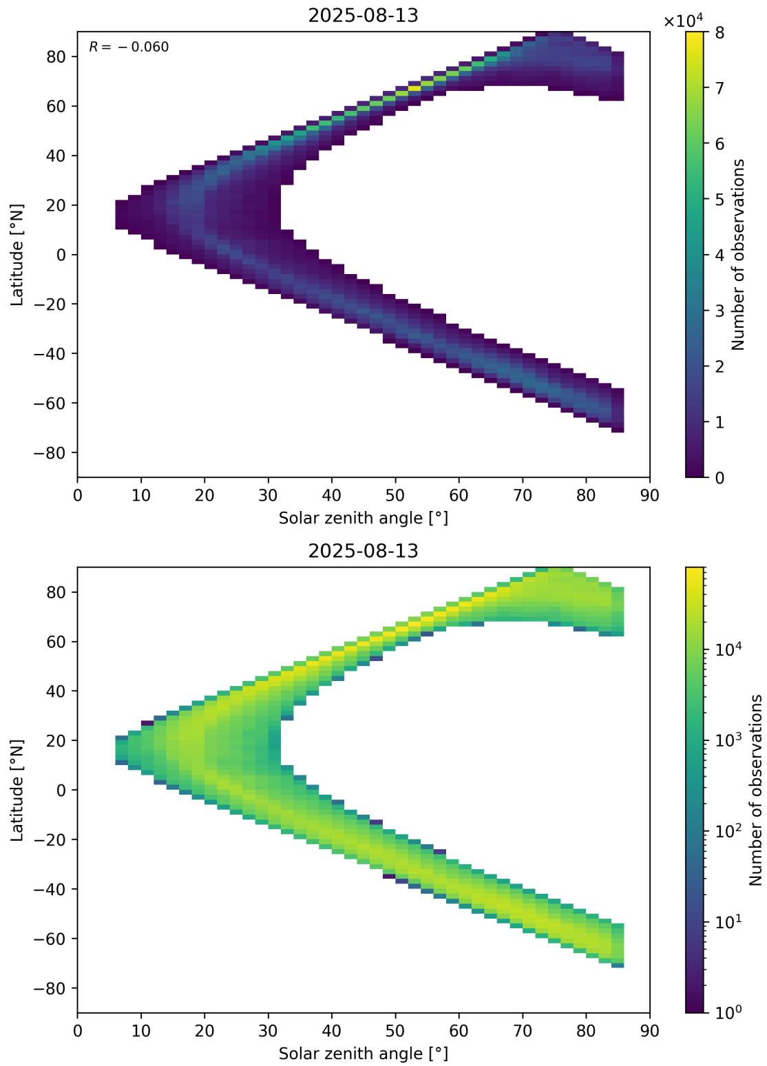
Figure 66: Scatter density plot of “Solar zenith angle” against “Latitude” for 2025-08-12 to 2025-08-14.
