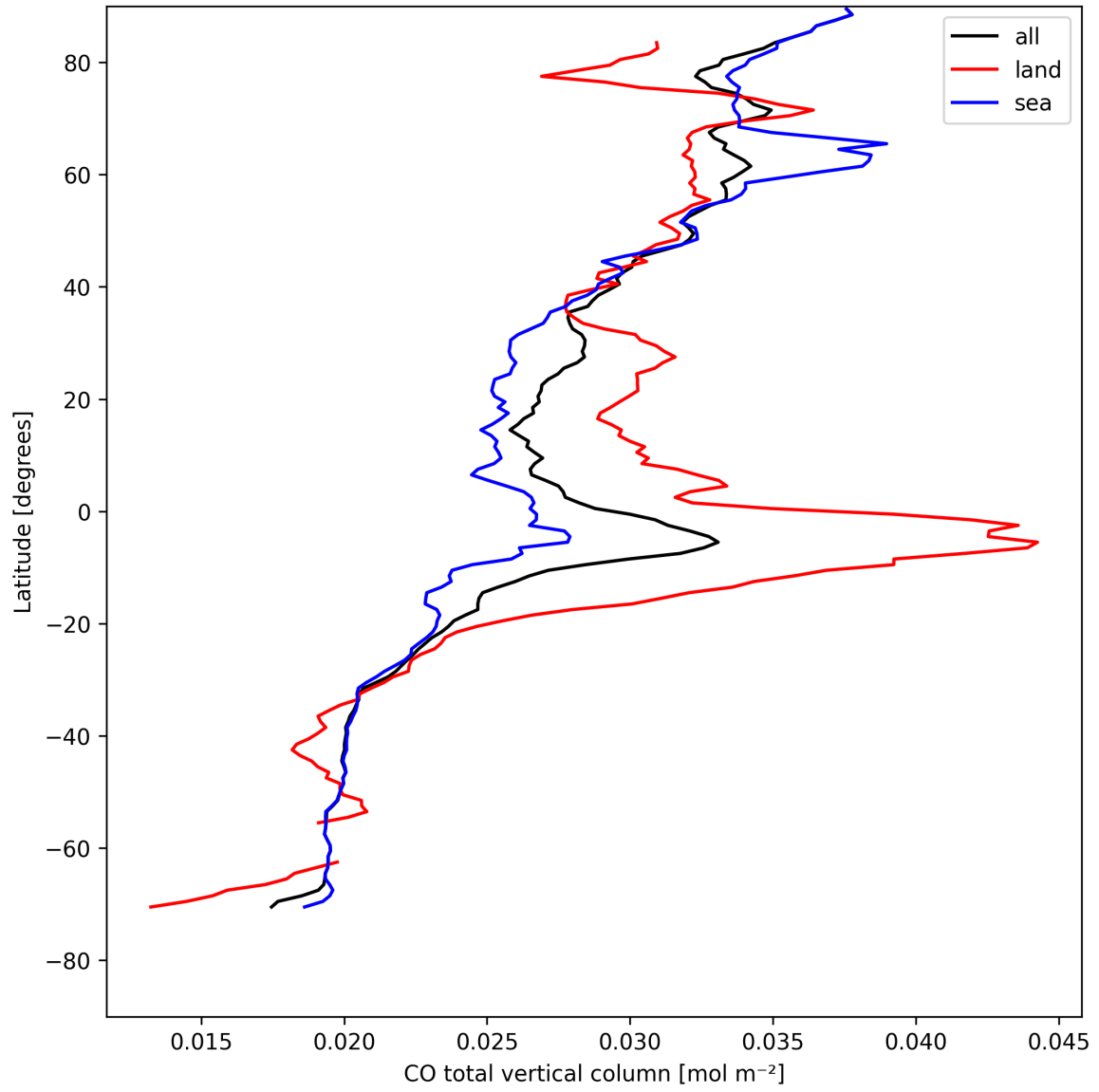
Figure 10: Zonal average of “CO total vertical column” for 2025-08-12 to 2025-08-14.
