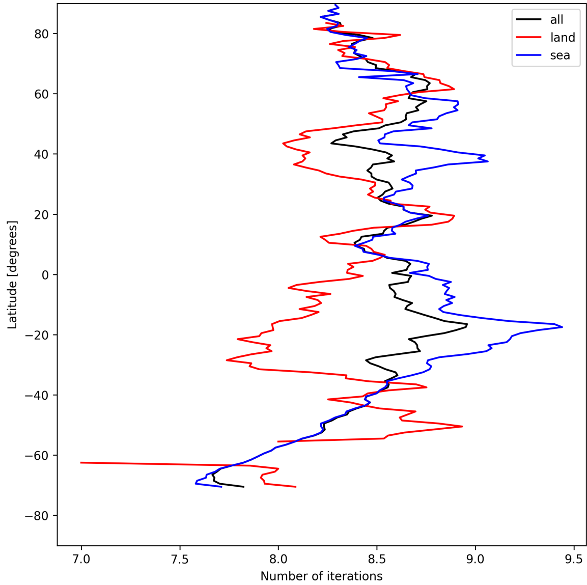
Figure 16: Zonal average of “Number of iterations” for 2025-08-12 to 2025-08-14.
