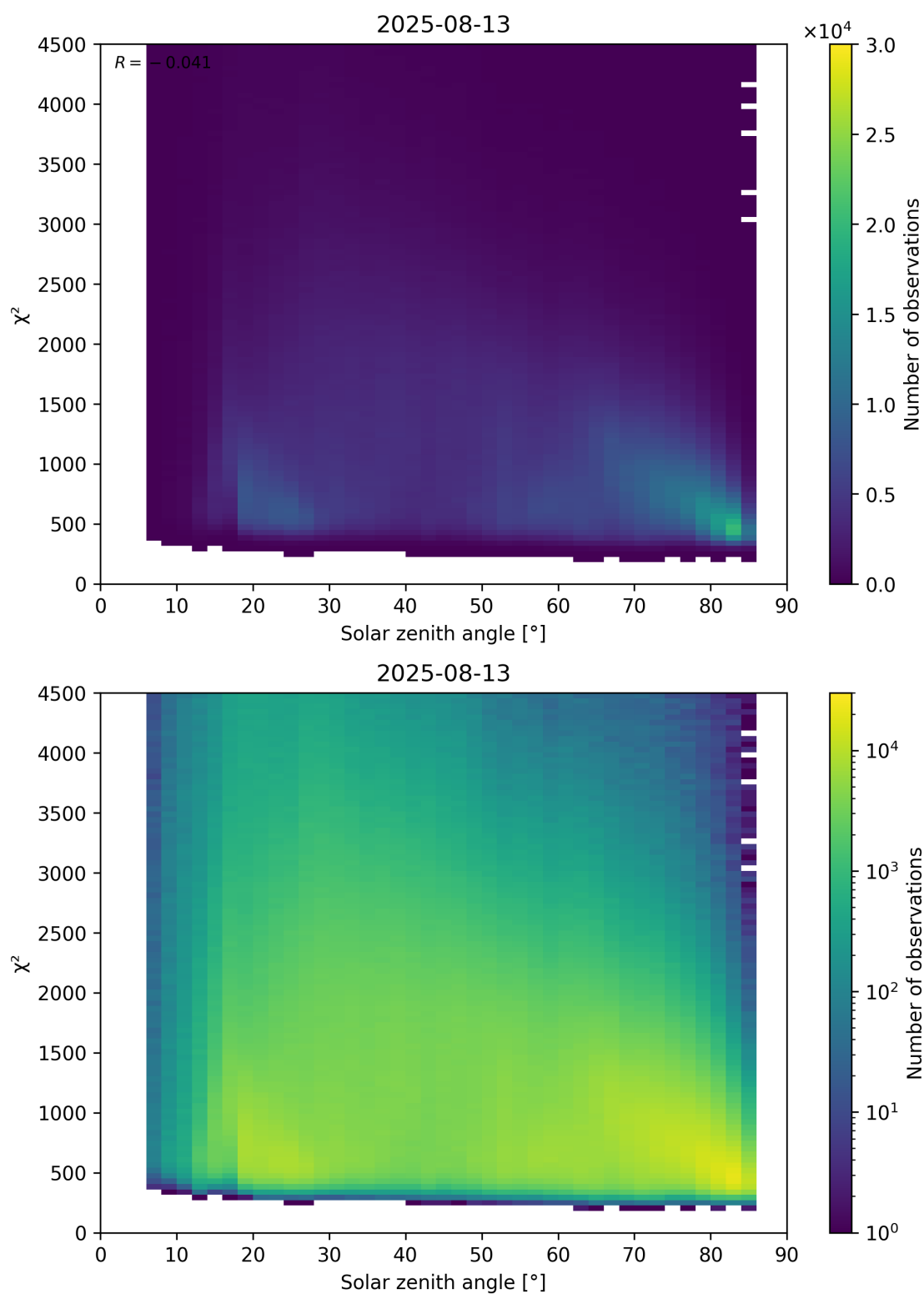
Figure 64: Scatter density plot of “Solar zenith angle” against “ \chi^2 ” for 2025-08-12 to 2025-08-14.
