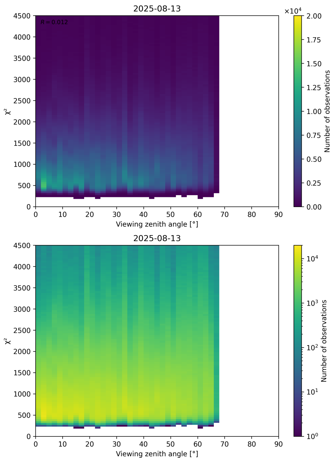
Figure 72: Scatter density plot of “Viewing zenith angle” against “ \chi^2 ” for 2025-08-12 to 2025-08-14.
