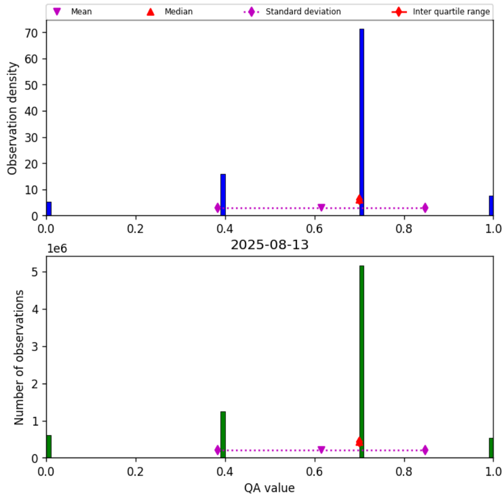
Figure 17: Histogram of “QA value” for 2025-08-12 to 2025-08-14
