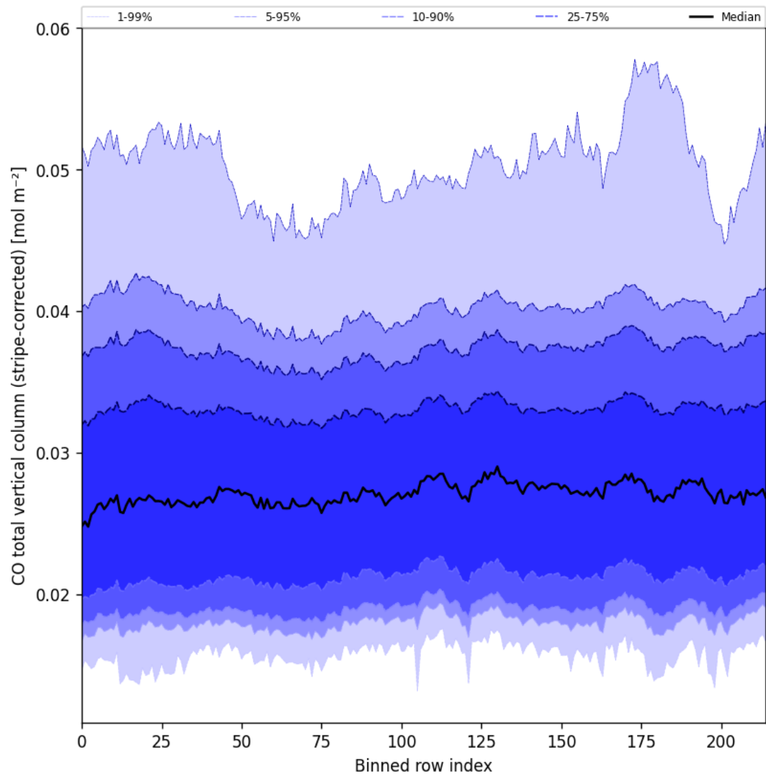
Figure 27: Along track statistics of “CO total vertical column (stripe-corrected)” for 2025-08-12 to 2025-08-14
