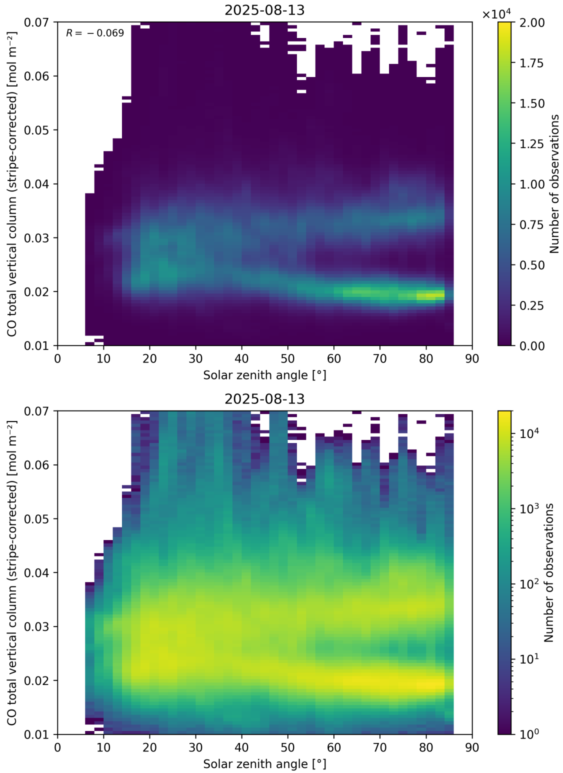
Figure 62: Scatter density plot of “Solar zenith angle” against “CO total vertical column (stripe-corrected)” for 2025-08-12 to 2025-08-14.
