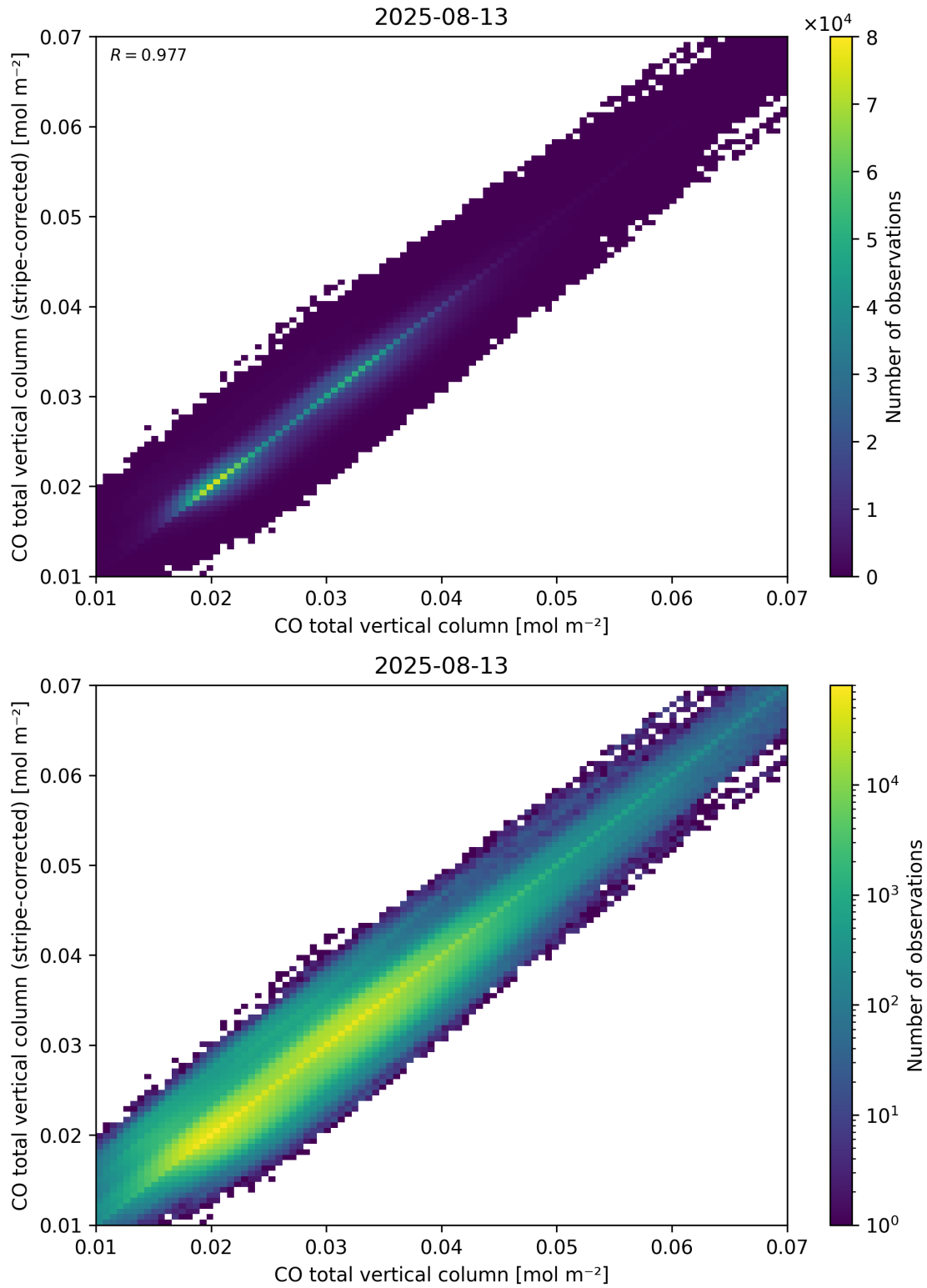
Figure 33: Scatter density plot of “CO total vertical column” against “CO total vertical column (stripe-corrected)” for 2025-08-12 to 2025-08-14.
