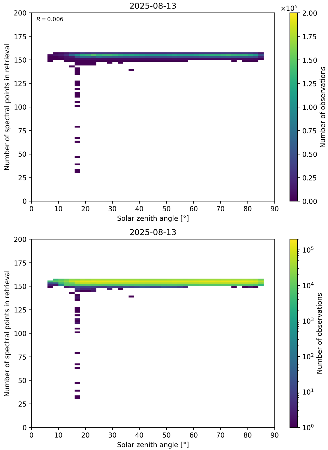
Figure 68: Scatter density plot of “Solar zenith angle” against “Number of spectral points in retrieval” for 2025-08-12 to 2025-08-14.
