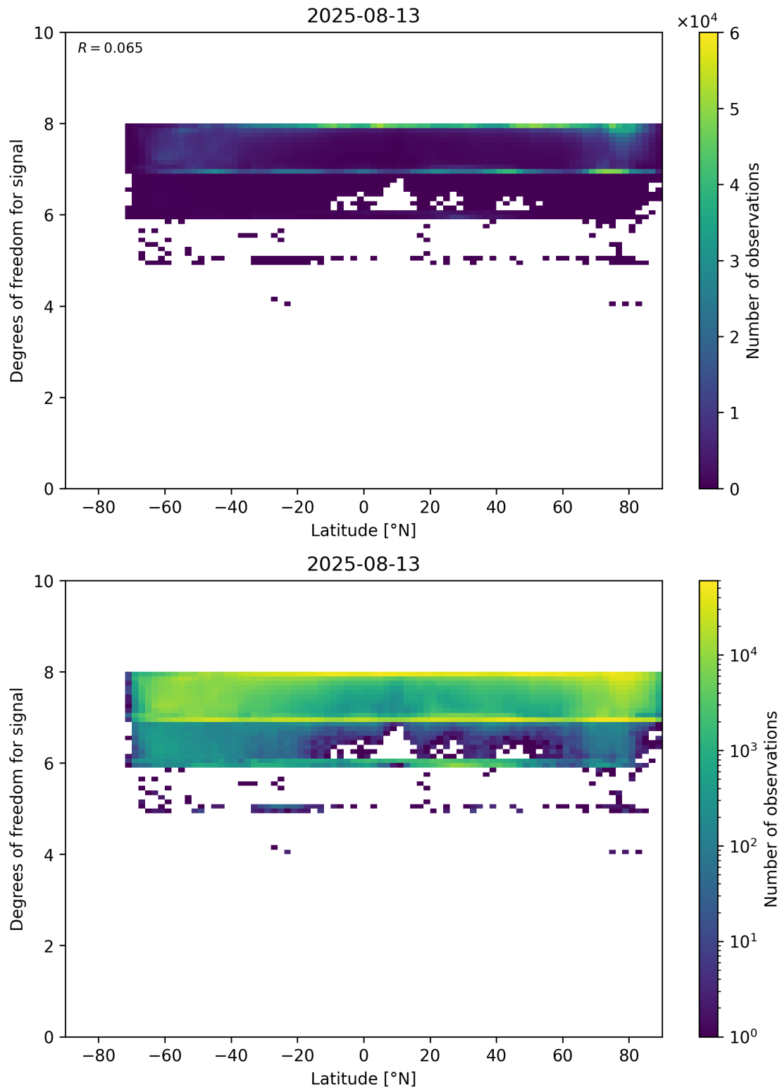
Figure 55: Scatter density plot of “Latitude” against “Degrees of freedom for signal” for 2025-08-12 to 2025-08-14.
