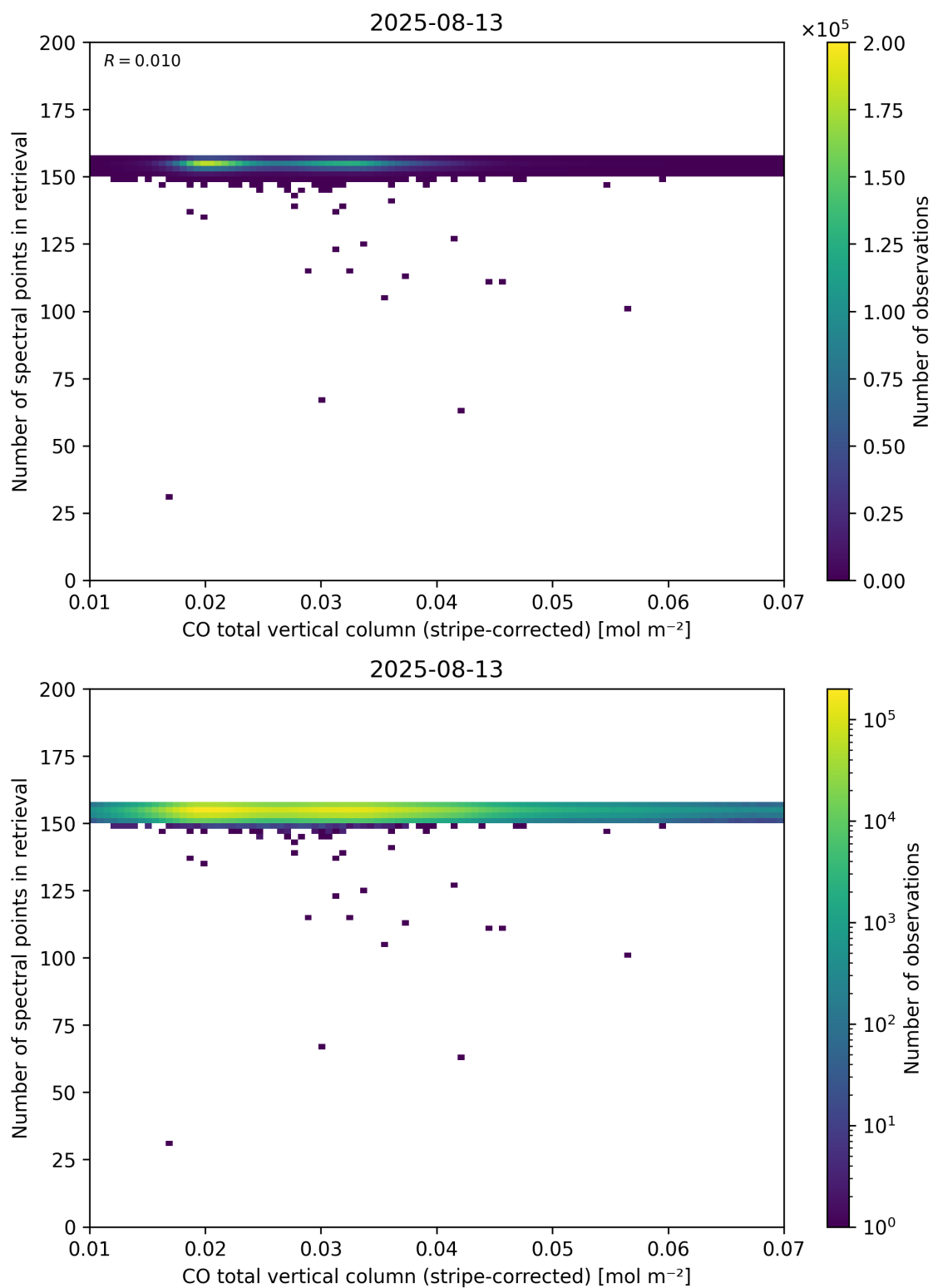
Figure 40: Scatter density plot of “CO total vertical column (stripe-corrected)” against “Number of spectral points in retrieval” for 2025-08-12 to 2025-08-14.
