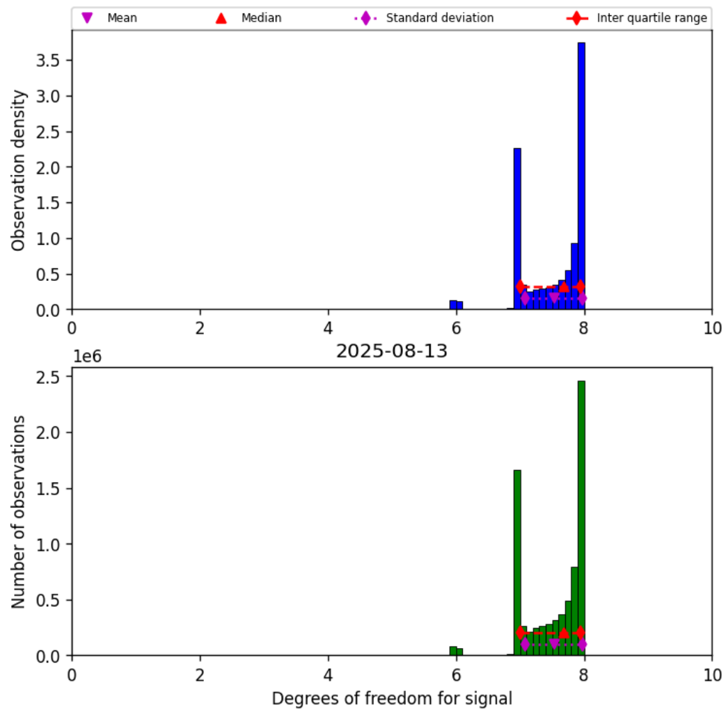
Figure 23: Histogram of “Degrees of freedom for signal” for 2025-08-12 to 2025-08-14
