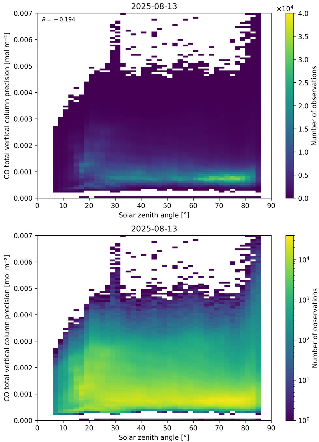
Figure 63: Scatter density plot of “Solar zenith angle” against “CO total vertical column precision” for 2025-08-12 to 2025-08-14.
