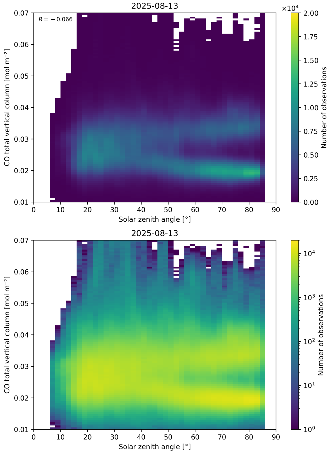
Figure 61: Scatter density plot of “Solar zenith angle” against “CO total vertical column” for 2025-08-12 to 2025-08-14.
