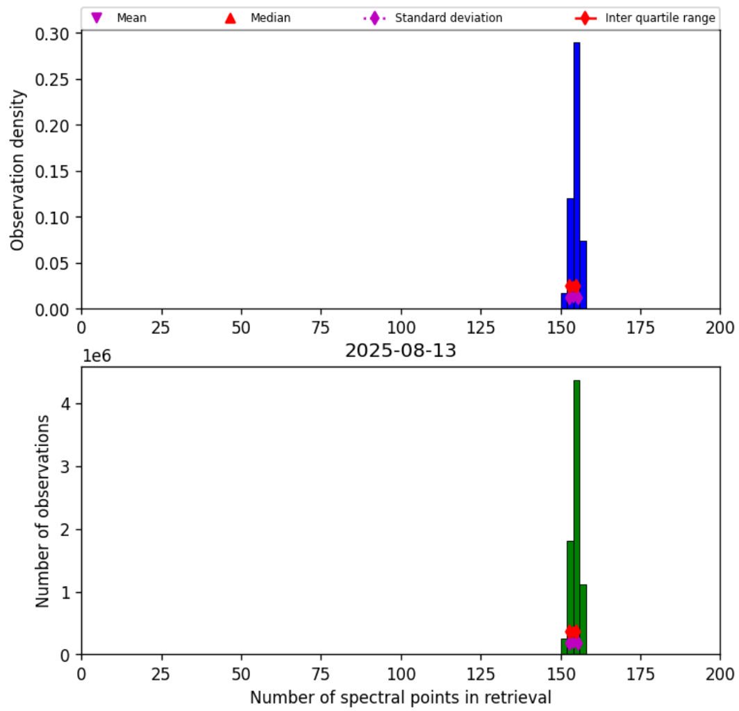
Figure 21: Histogram of “Number of spectral points in retrieval” for 2025-08-12 to 2025-08-14
