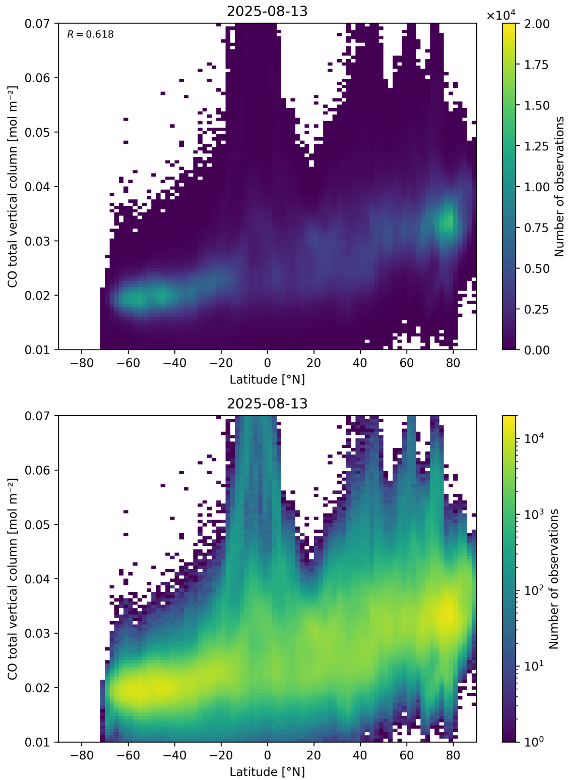
Figure 51: Scatter density plot of “Latitude” against “CO total vertical column” for 2025-08-12 to 2025-08-14.
