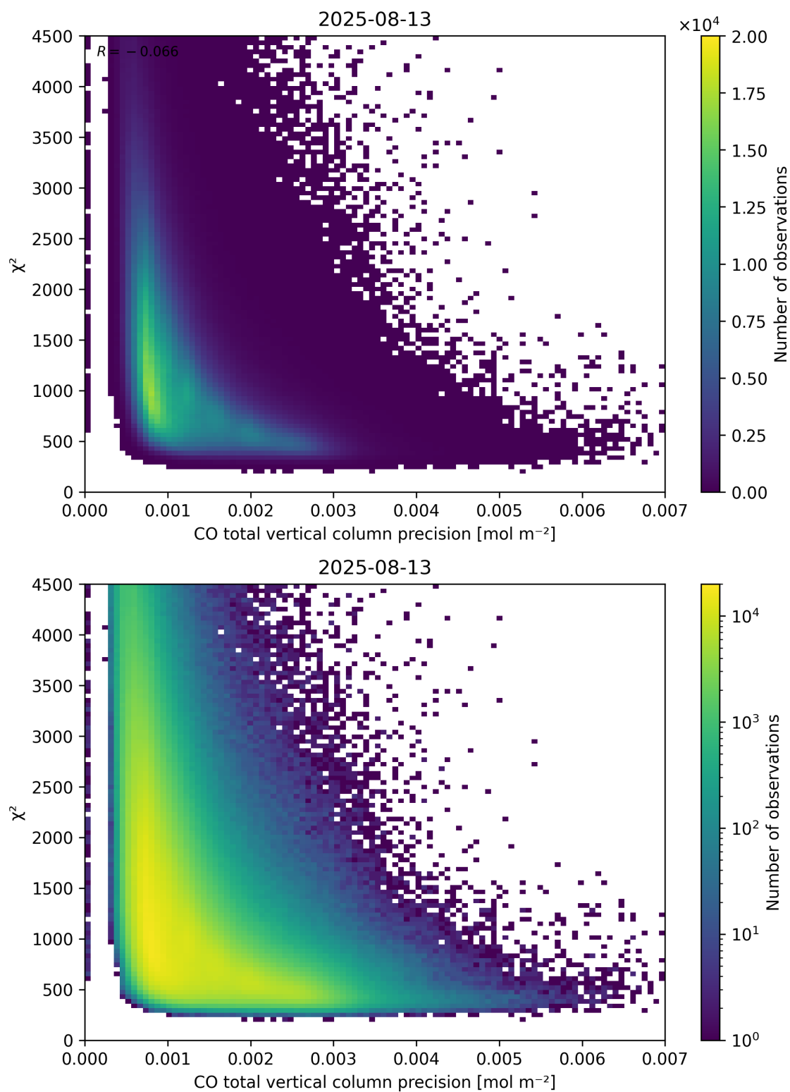
Figure 44: Scatter density plot of “CO total vertical column precision” against “ \chi^2 ” for 2025-08-12 to 2025-08-14.
