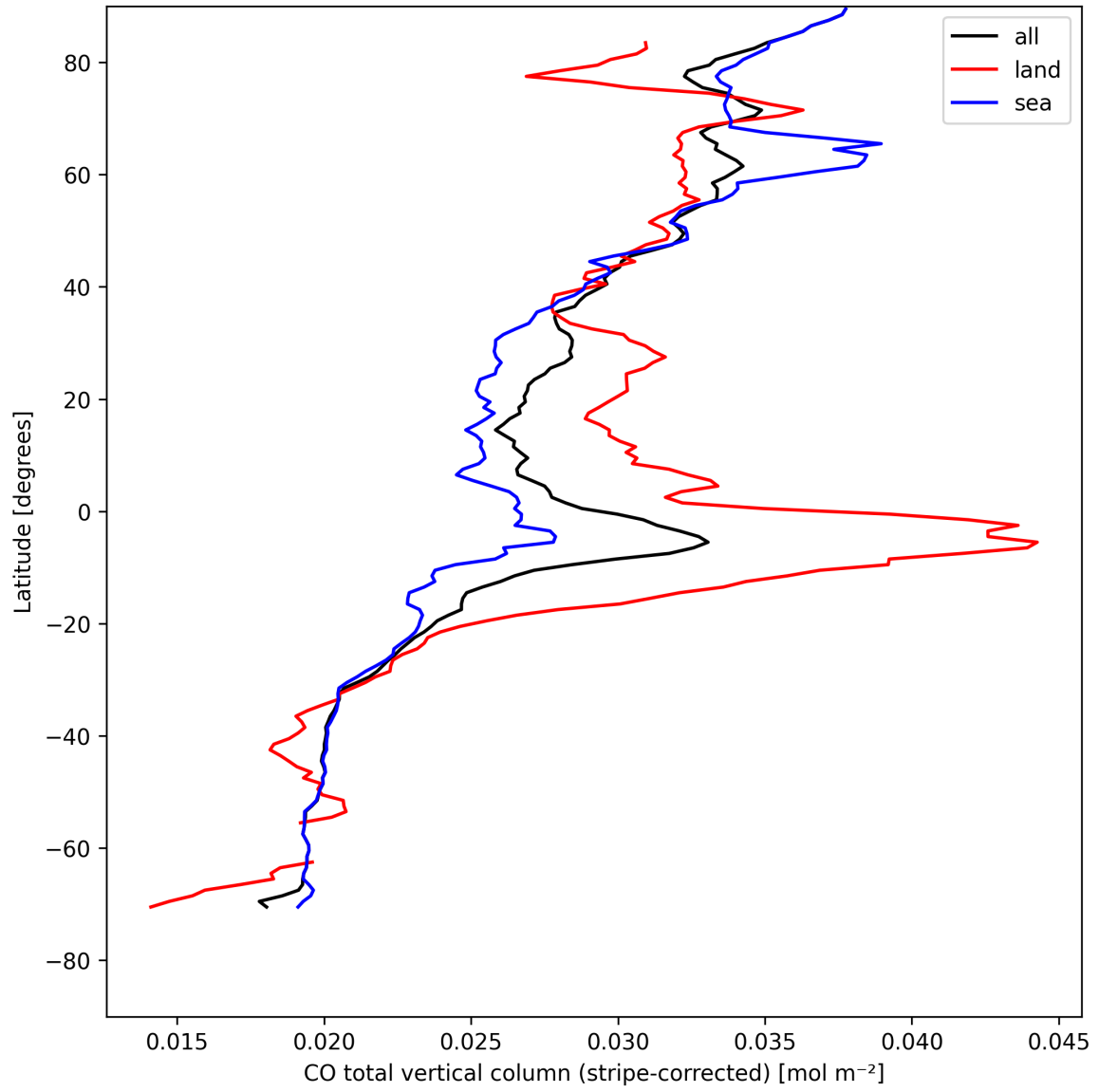
Figure 11: Zonal average of “CO total vertical column (stripe-corrected)” for 2025-08-12 to 2025-08-14.
