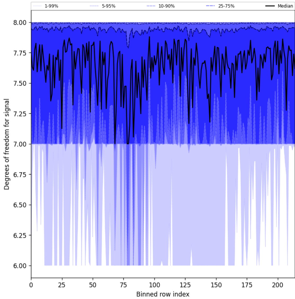
Figure 31: Along track statistics of “Degrees of freedom for signal” for 2025-08-12 to 2025-08-14
