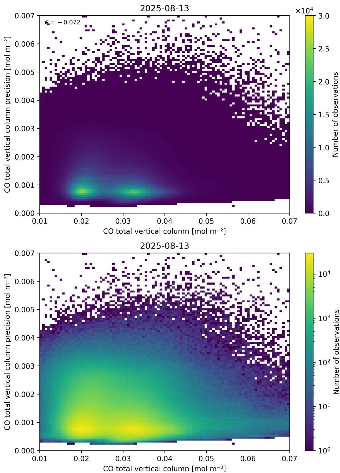
Figure 34: Scatter density plot of “CO total vertical column” against “CO total vertical column precision” for 2025-08-12 to 2025-08-14.
