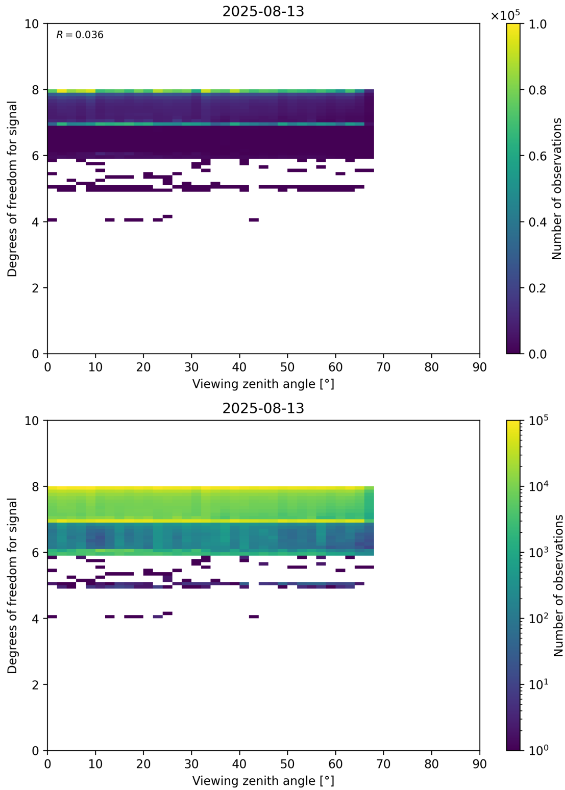
Figure 73: Scatter density plot of “Viewing zenith angle” against “Degrees of freedom for signal” for 2025-08-12 to 2025-08-14.
