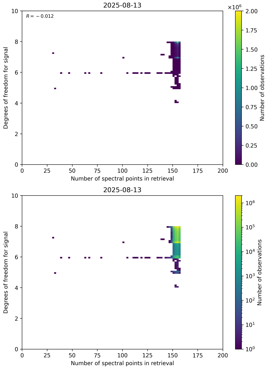
Figure 59: Scatter density plot of “Number of spectral points in retrieval” against “Degrees of freedom for signal” for 2025-08-12 to 2025-08-14.
