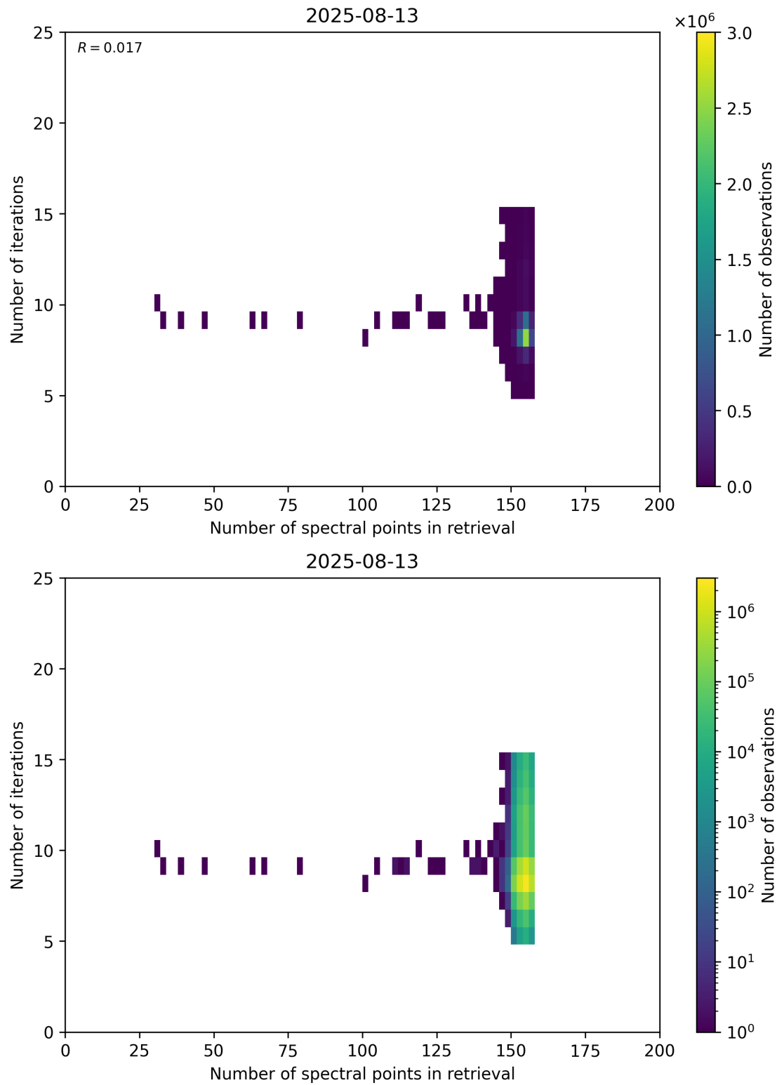
Figure 60: Scatter density plot of “Number of spectral points in retrieval” against “Number of iterations” for 2025-08-12 to 2025-08-14.
