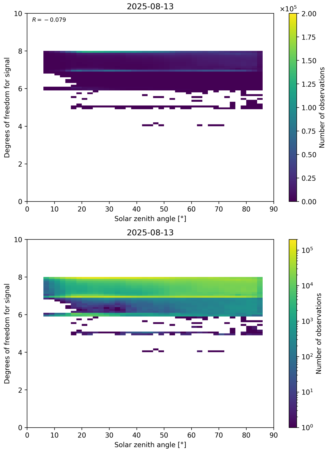
Figure 65: Scatter density plot of “Solar zenith angle” against “Degrees of freedom for signal” for 2025-08-12 to 2025-08-14.
