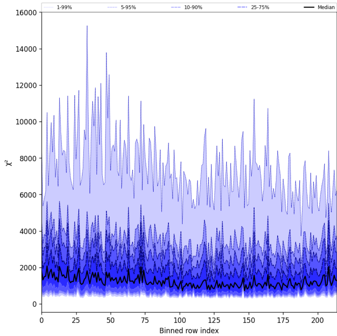
Figure 30: Along track statistics of “ \chi^2 ” for 2025-08-12 to 2025-08-14
