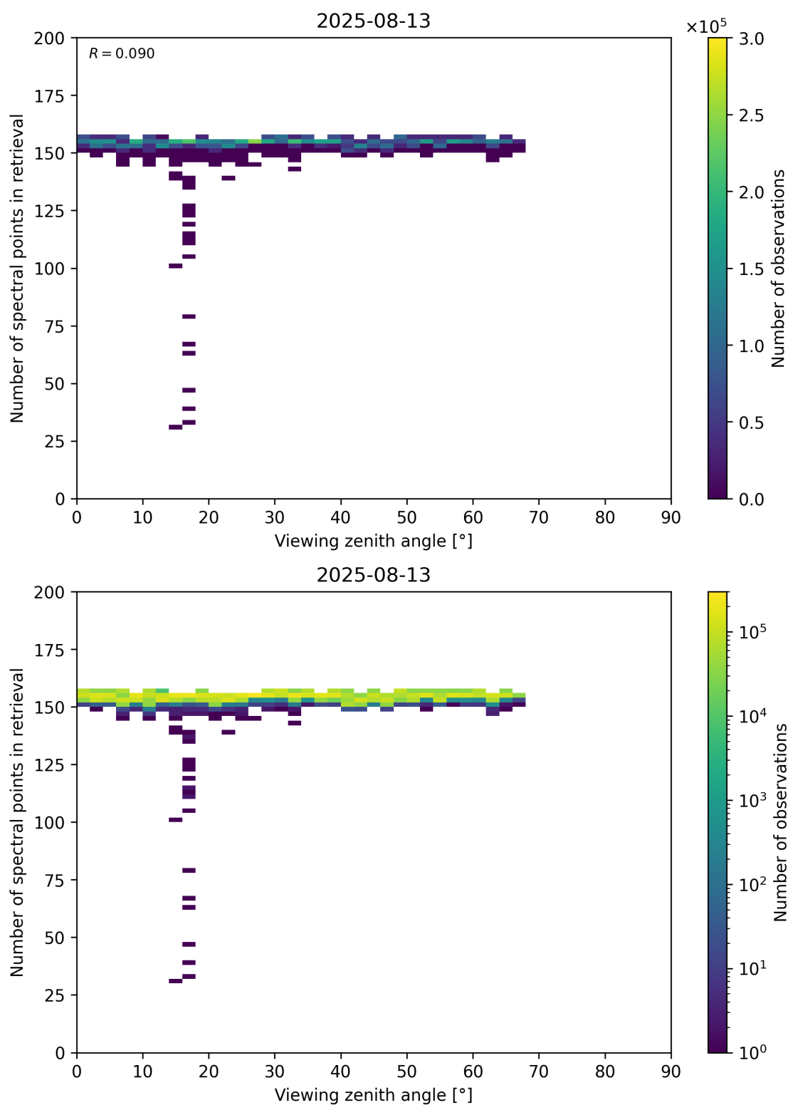
Figure 76: Scatter density plot of “Viewing zenith angle” against “Number of spectral points in retrieval” for 2025-08-12 to 2025-08-14.
