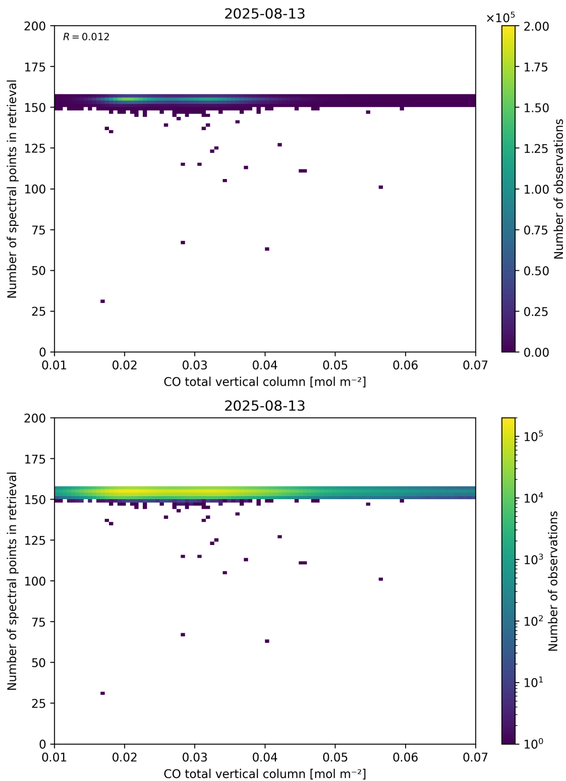
Figure 43: Scatter density plot of “CO total vertical column” against “Number of spectral points in retrieval” for 2025-08-12 to 2025-08-14.
