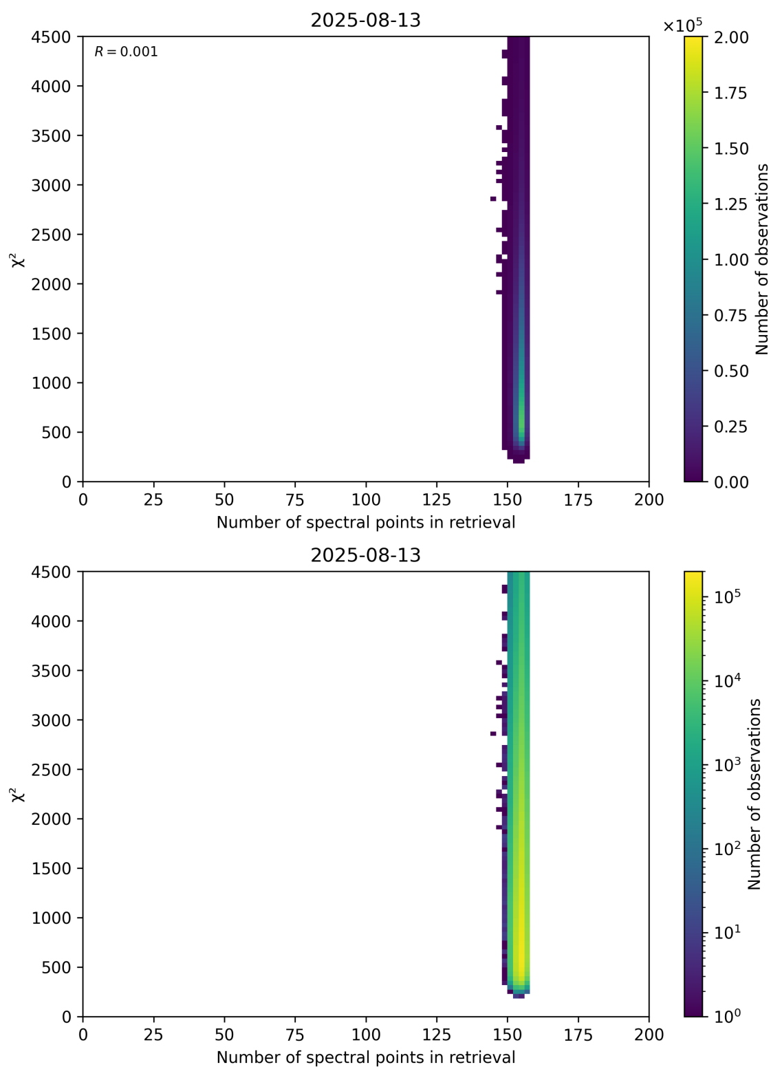
Figure 58: Scatter density plot of “Number of spectral points in retrieval” against “ \chi^2 ” for 2025-08-12 to 2025-08-14.
