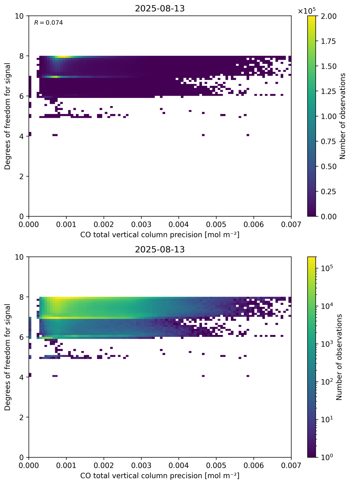
Figure 45: Scatter density plot of “CO total vertical column precision” against “Degrees of freedom for signal” for 2025-08-12 to 2025-08-14.
