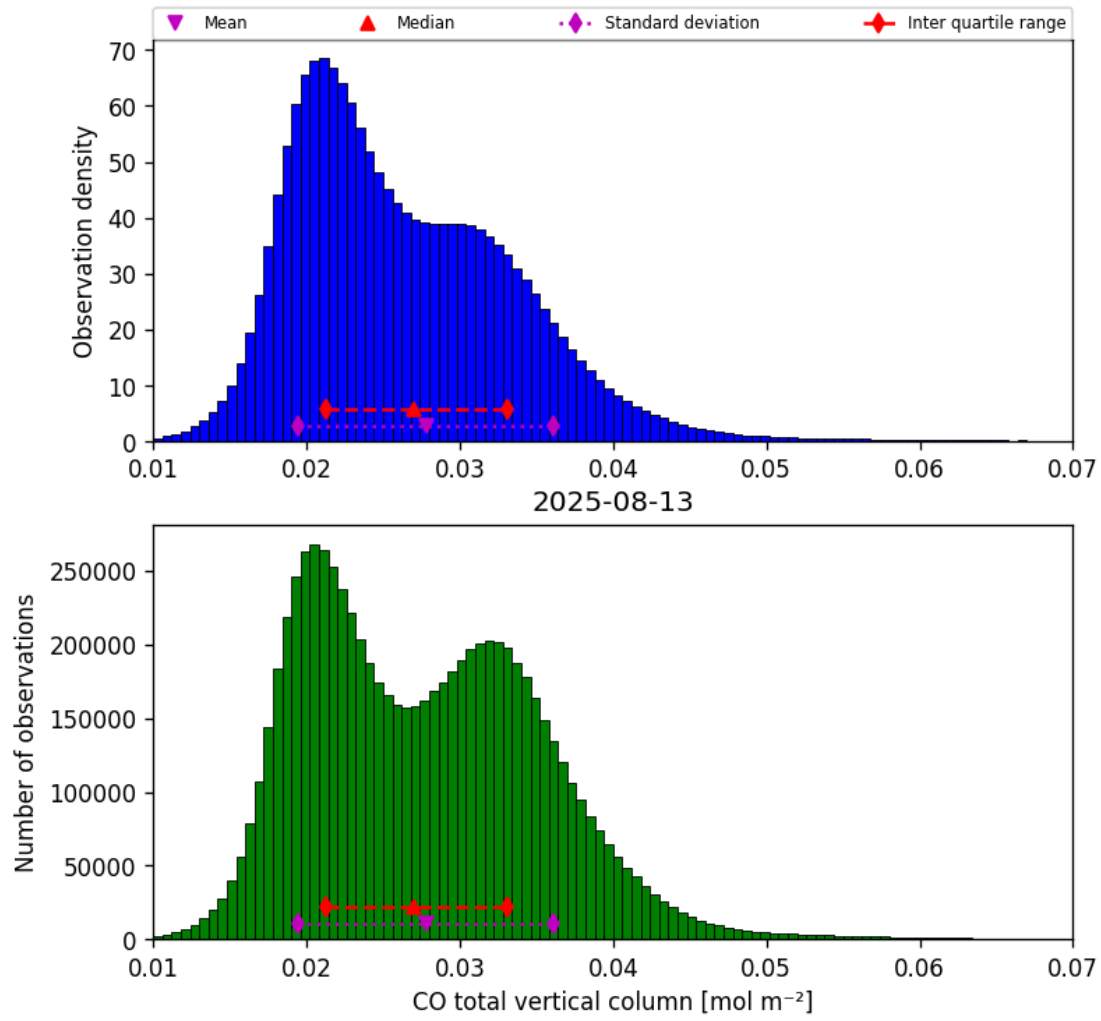
Figure 18: Histogram of “CO total vertical column” for 2025-08-12 to 2025-08-14
