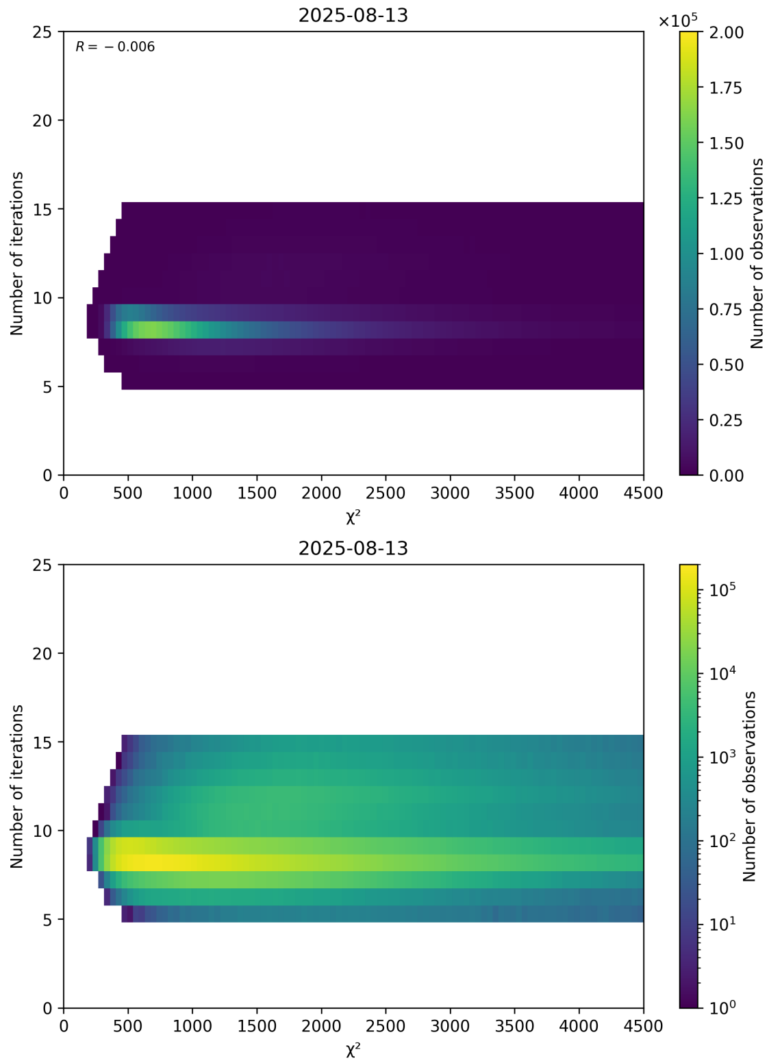
Figure 49: Scatter density plot of “ \chi^2 ” against “Number of iterations” for 2025-08-12 to 2025-08-14.
