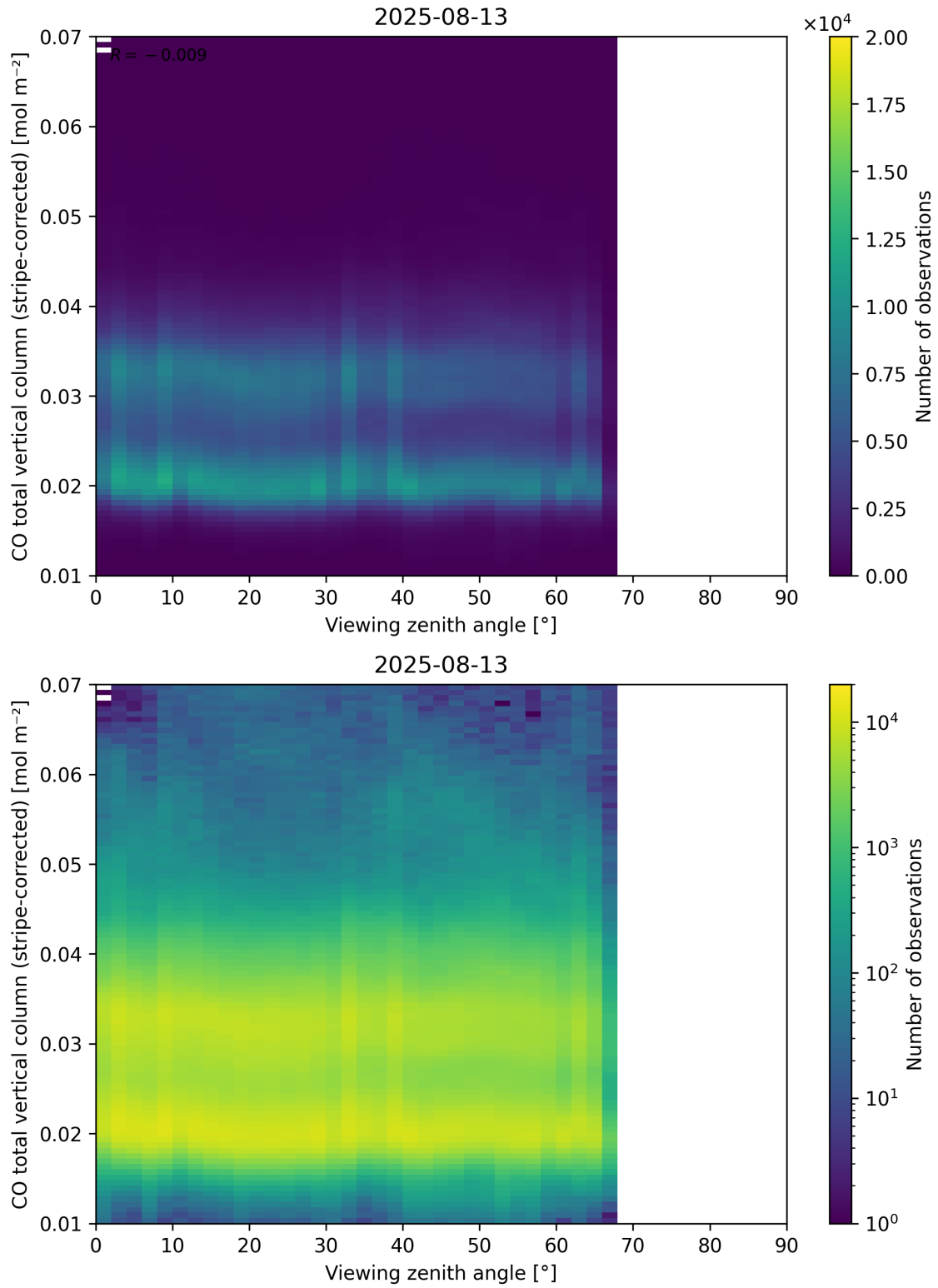
Figure 70: Scatter density plot of “Viewing zenith angle” against “CO total vertical column (stripe-corrected)” for 2025-08-12 to 2025-08-14.
