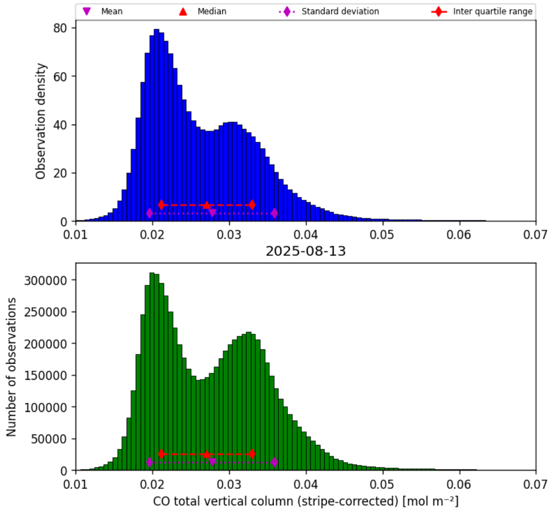
Figure 19: Histogram of “CO total vertical column (stripe-corrected)” for 2025-08-12 to 2025-08-14
