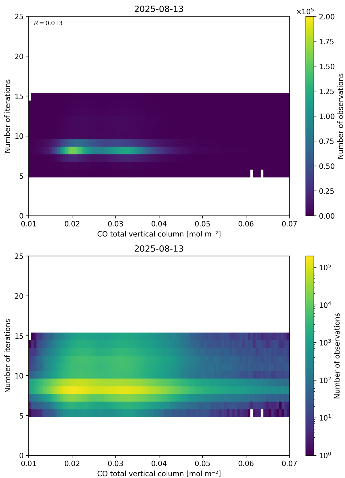
Figure 42: Scatter density plot of “CO total vertical column” against “Number of iterations” for 2025-08-12 to 2025-08-14.
