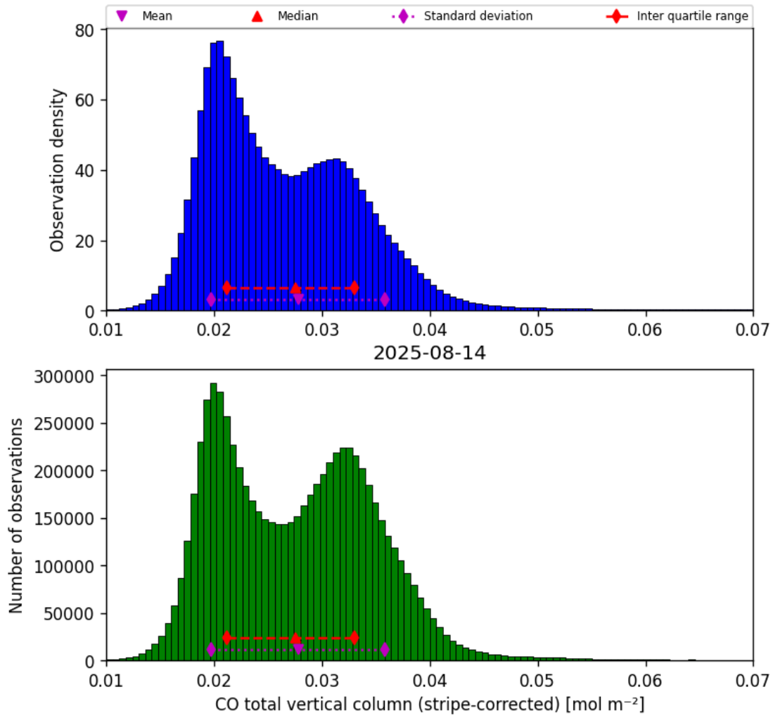
Figure 19: Histogram of “CO total vertical column (stripe-corrected)” for 2025-08-14 to 2025-08-15
