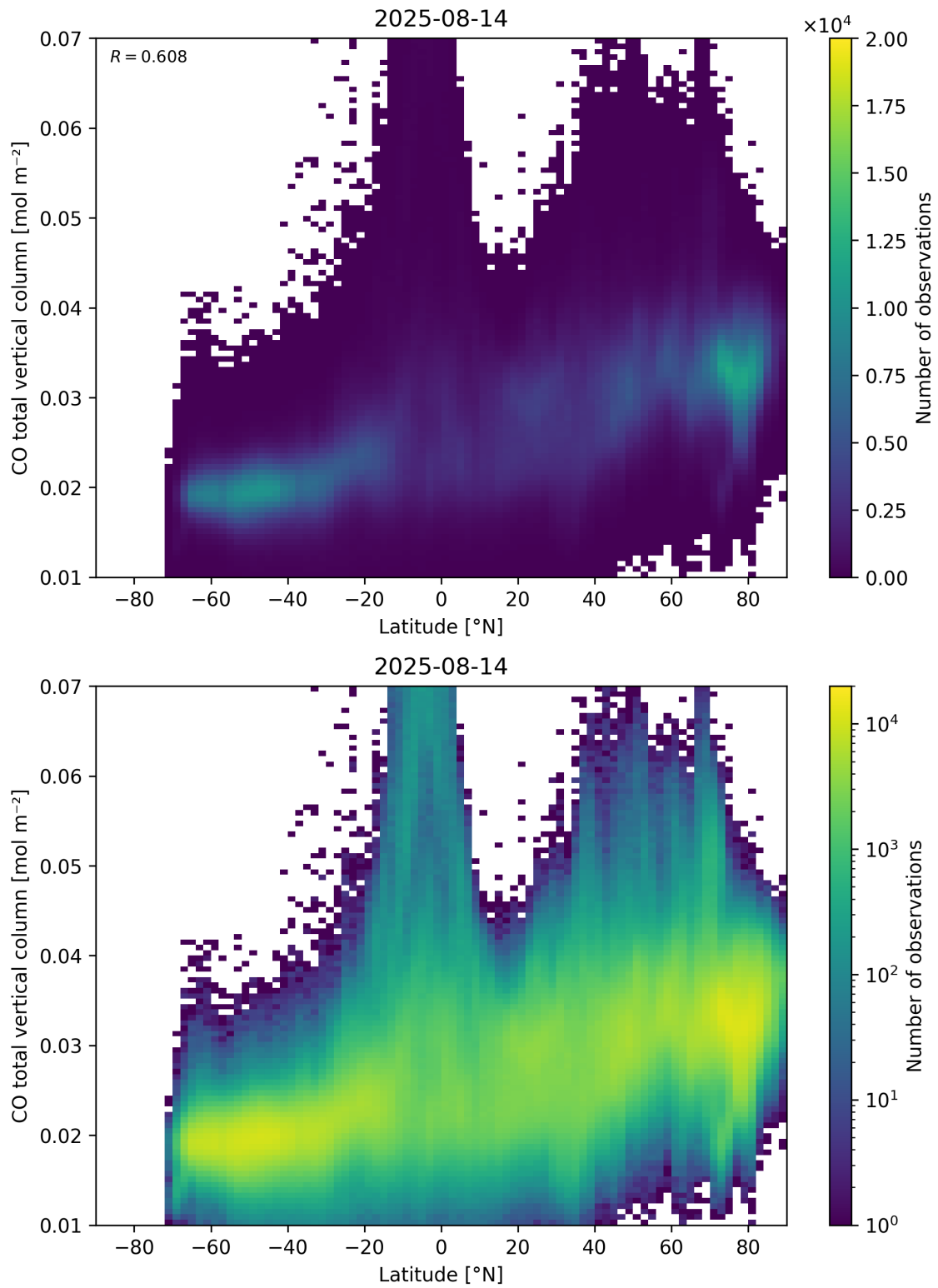
Figure 51: Scatter density plot of “Latitude” against “CO total vertical column” for 2025-08-14 to 2025-08-15.
