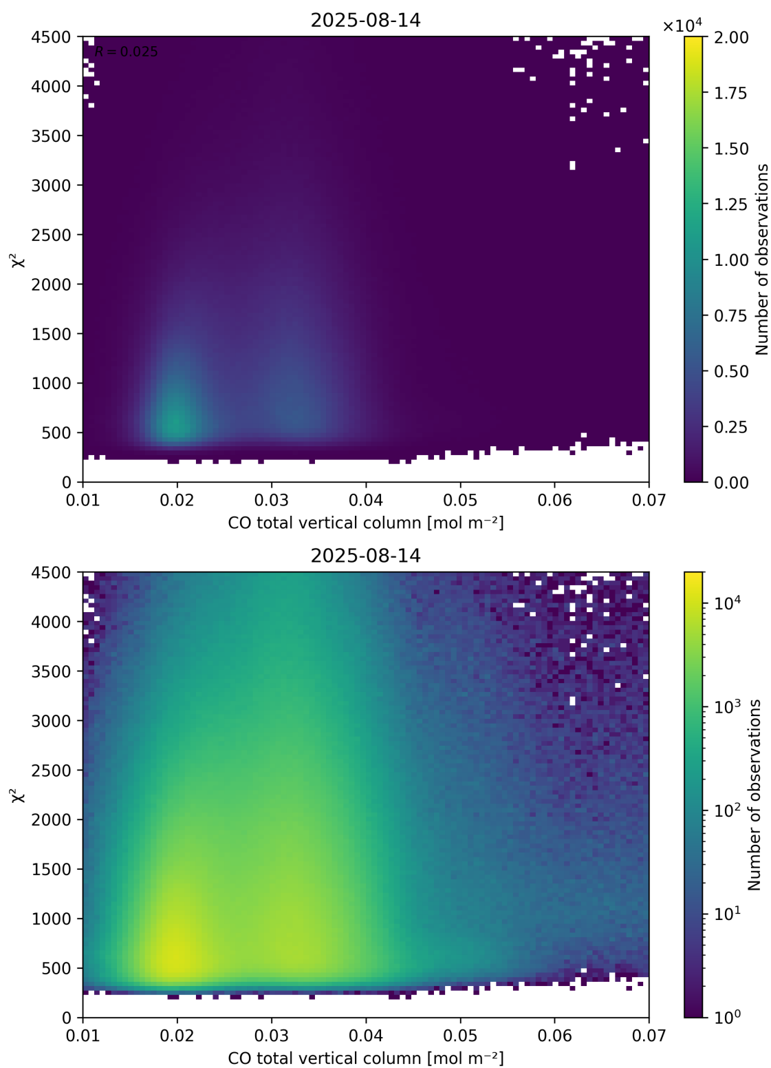
Figure 35: Scatter density plot of “CO total vertical column” against “ \chi^2 ” for 2025-08-14 to 2025-08-15.
