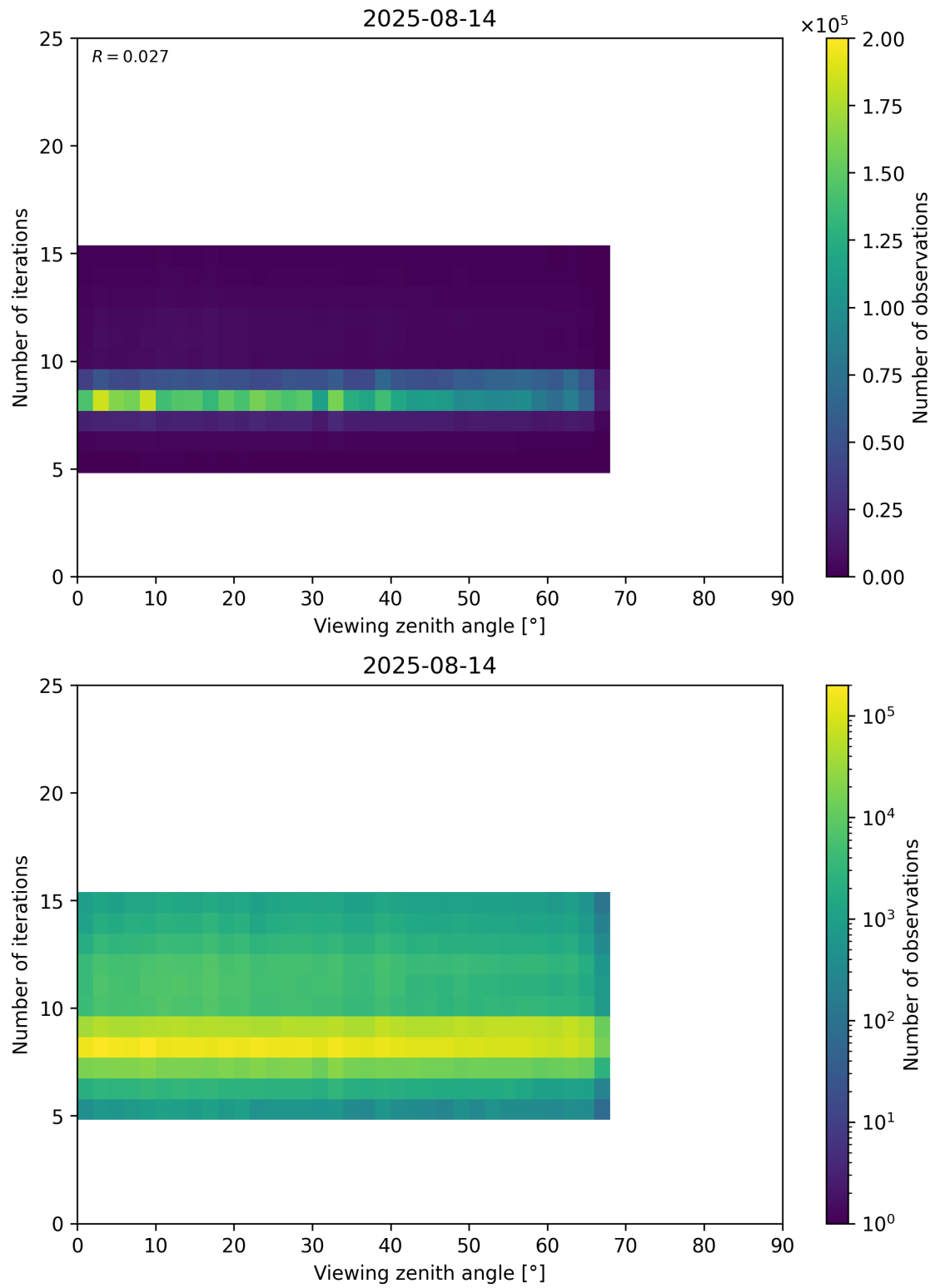
Figure 75: Scatter density plot of “Viewing zenith angle” against “Number of iterations” for 2025-08-14 to 2025-08-15.
