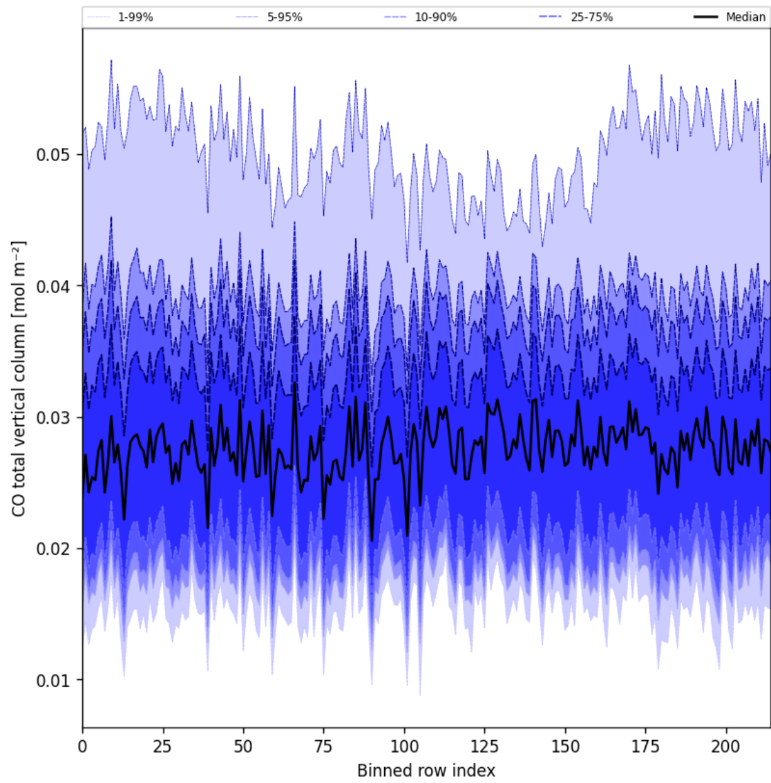
Figure 26: Along track statistics of “CO total vertical column” for 2025-08-14 to 2025-08-15
