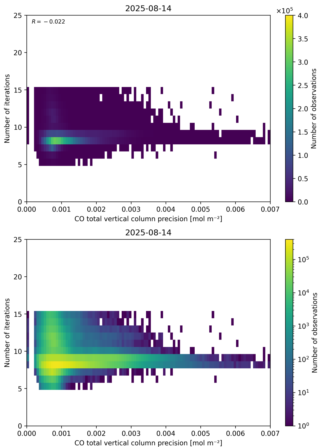
Figure 46: Scatter density plot of “CO total vertical column precision” against “Number of iterations” for 2025-08-14 to 2025-08-15.
