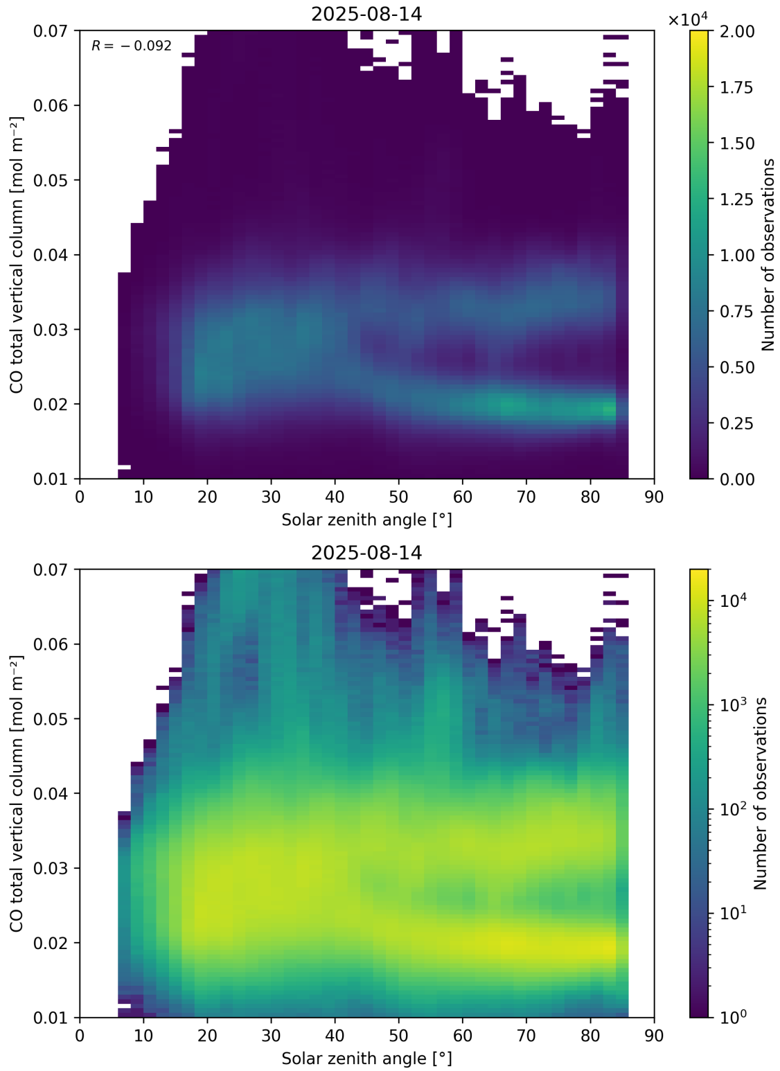
Figure 61: Scatter density plot of “Solar zenith angle” against “CO total vertical column” for 2025-08-14 to 2025-08-15.
