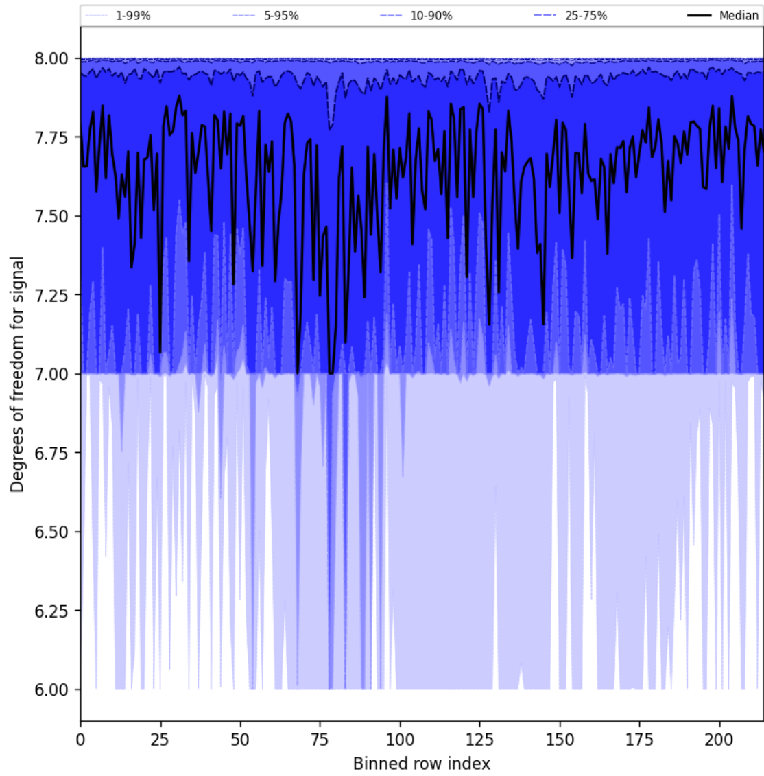
Figure 31: Along track statistics of “Degrees of freedom for signal” for 2025-08-14 to 2025-08-15
