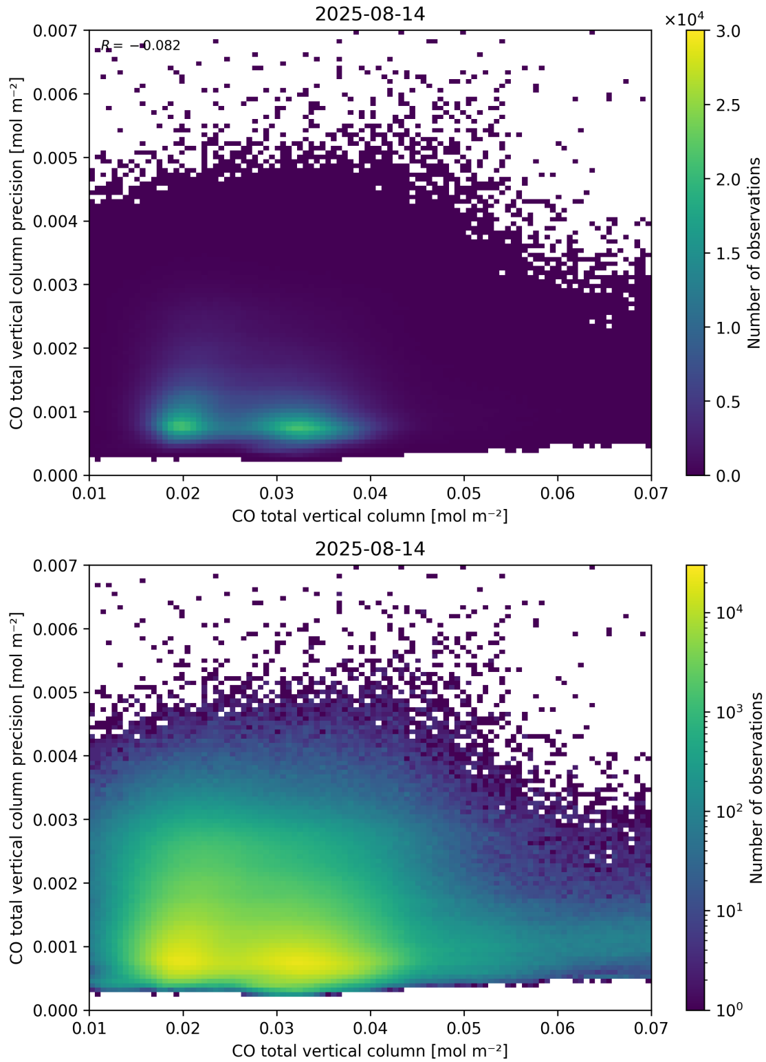
Figure 34: Scatter density plot of “CO total vertical column” against “CO total vertical column precision” for 2025-08-14 to 2025-08-15.
