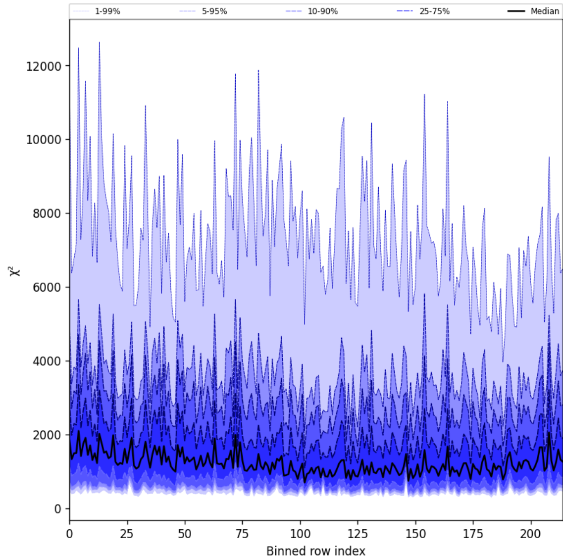
Figure 30: Along track statistics of “ \chi^2 ” for 2025-08-14 to 2025-08-15
