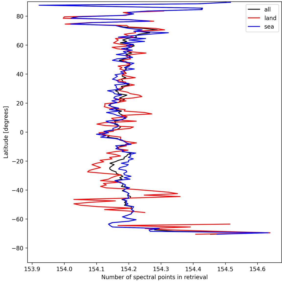
Figure 13: Zonal average of “Number of spectral points in retrieval” for 2025-08-14 to 2025-08-15.
