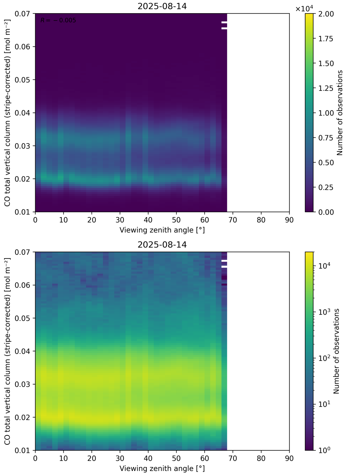
Figure 70: Scatter density plot of “Viewing zenith angle” against “CO total vertical column (stripe-corrected)” for 2025-08-14 to 2025-08-15.
