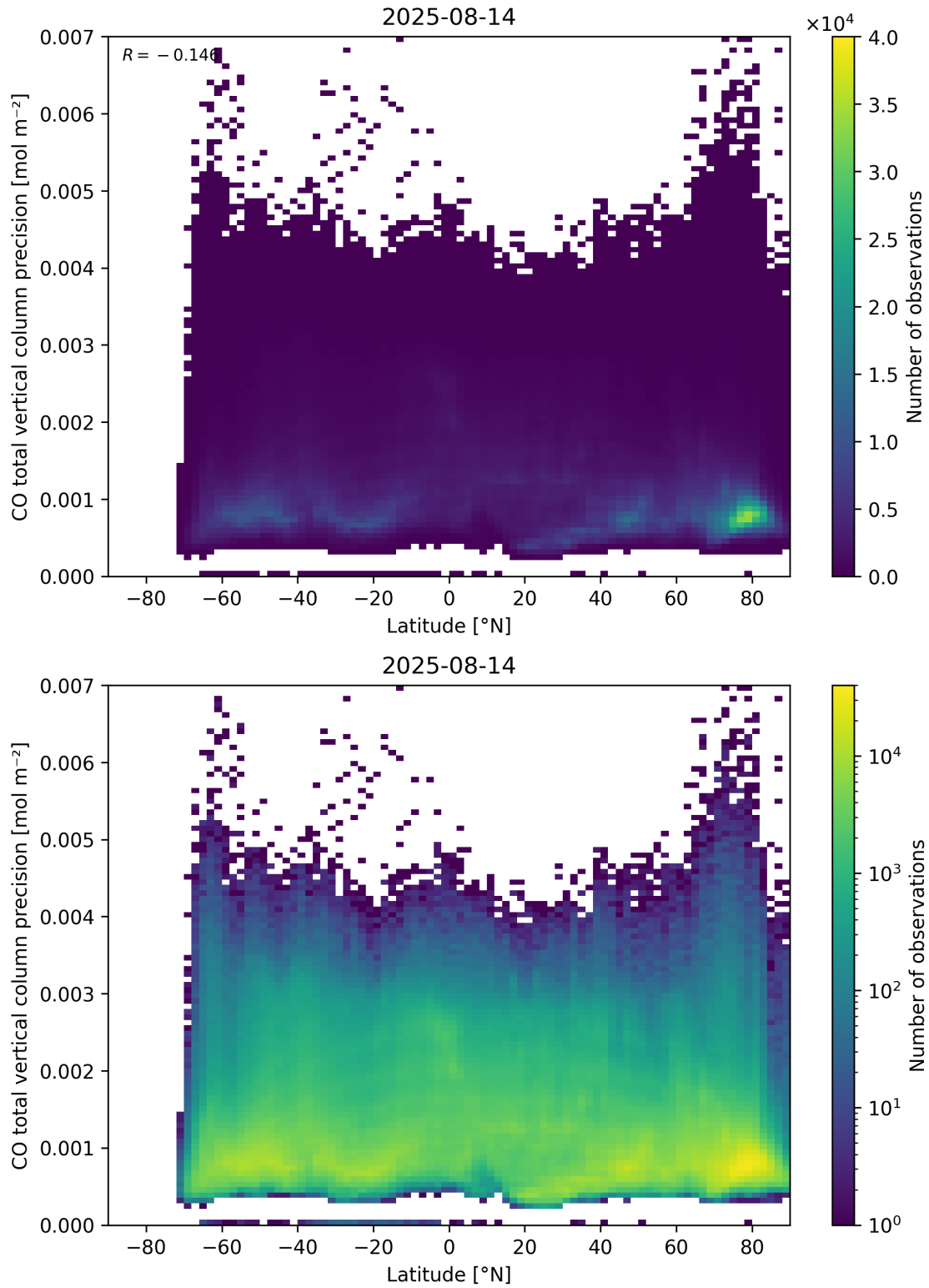
Figure 53: Scatter density plot of “Latitude” against “CO total vertical column precision” for 2025-08-14 to 2025-08-15.
