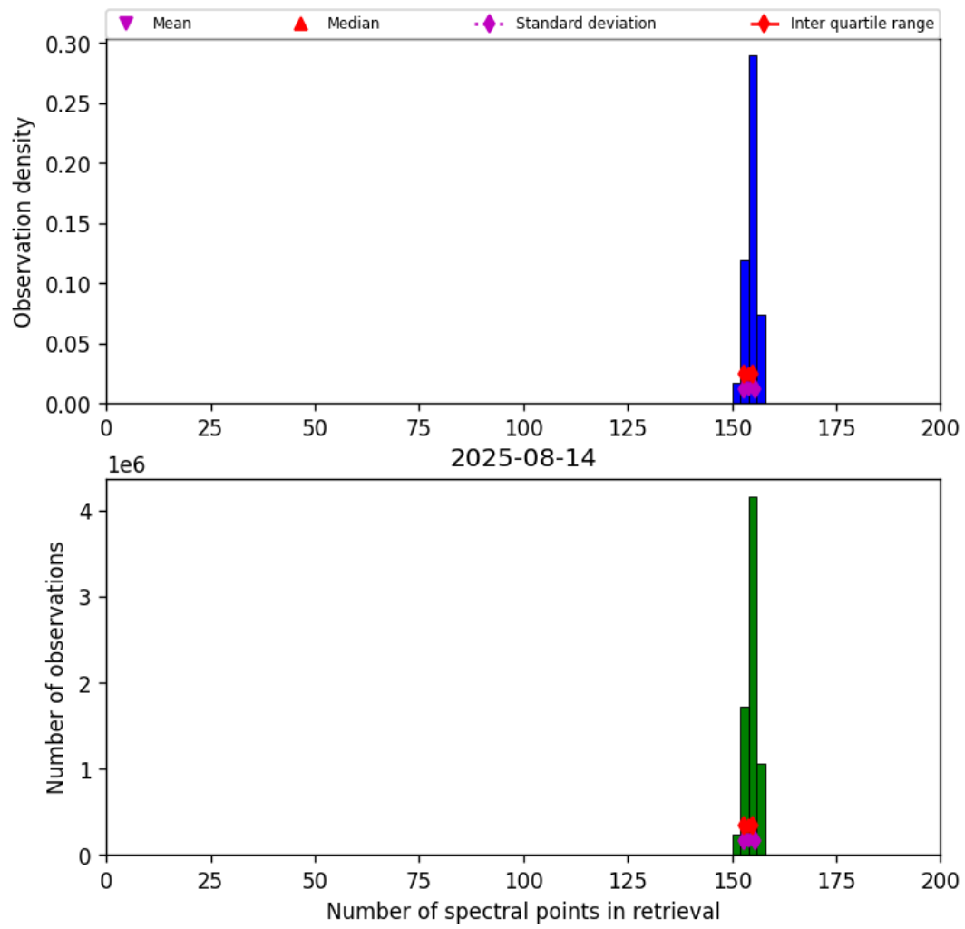
Figure 21: Histogram of “Number of spectral points in retrieval” for 2025-08-14 to 2025-08-15
