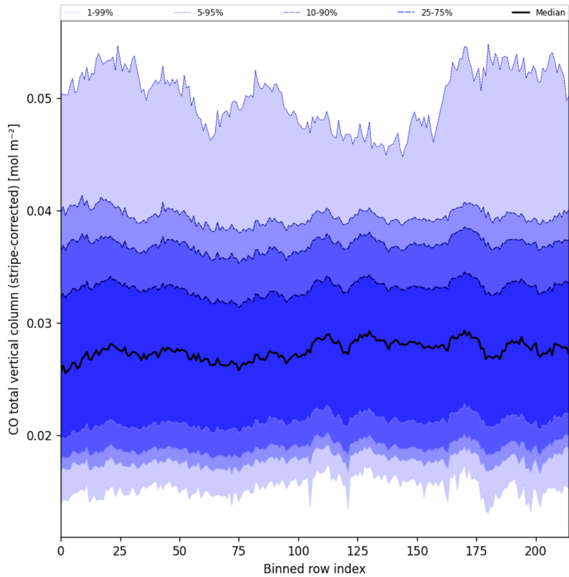
Figure 27: Along track statistics of “CO total vertical column (stripe-corrected)” for 2025-08-14 to 2025-08-15
