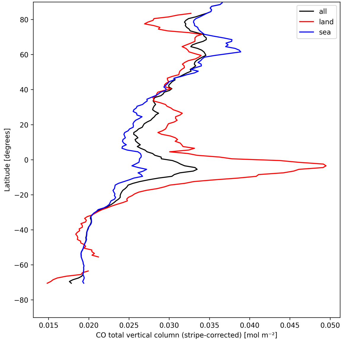
Figure 11: Zonal average of “CO total vertical column (stripe-corrected)” for 2025-08-14 to 2025-08-15.
