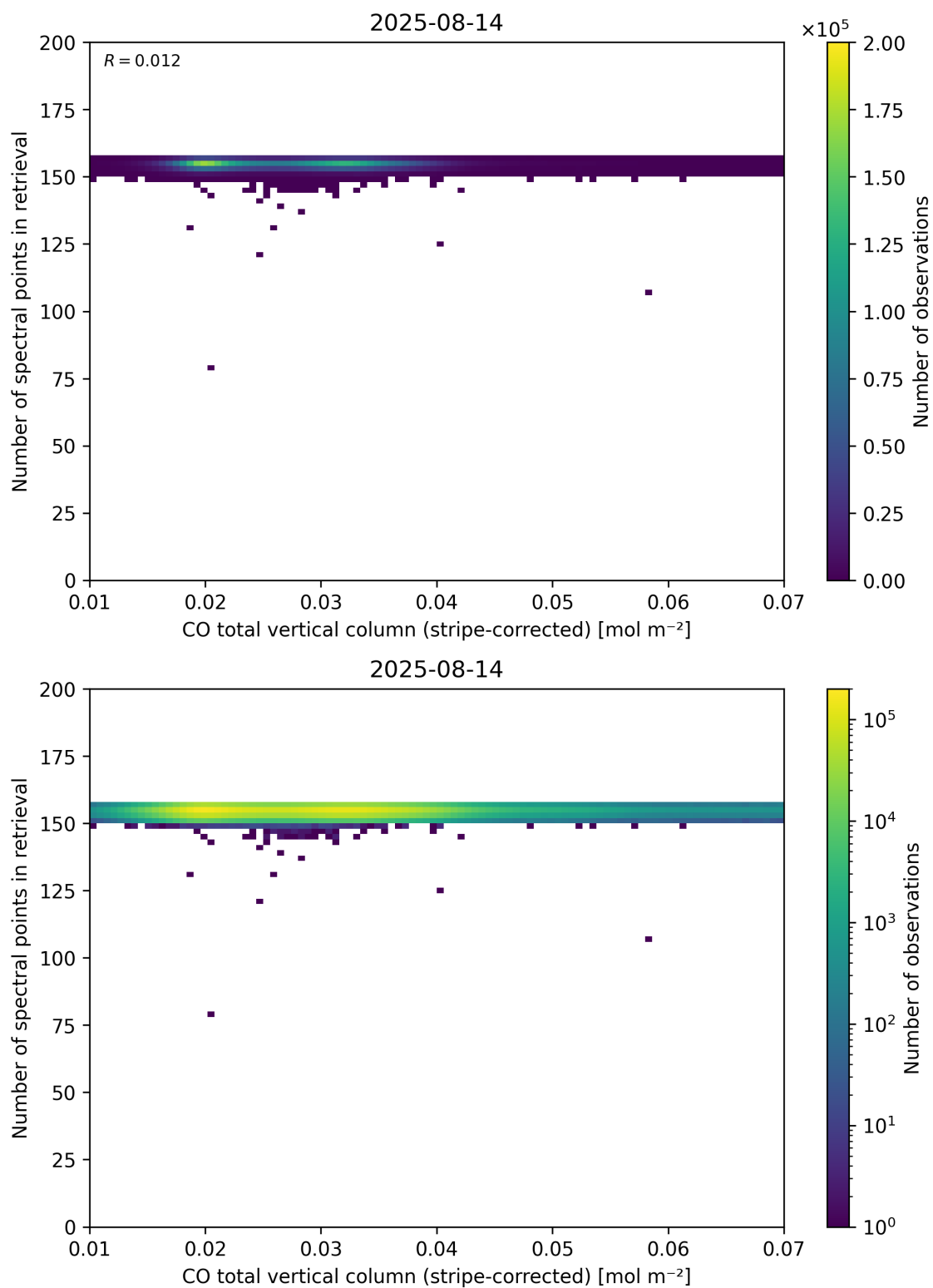
Figure 40: Scatter density plot of “CO total vertical column (stripe-corrected)” against “Number of spectral points in retrieval” for 2025-08-14 to 2025-08-15.
