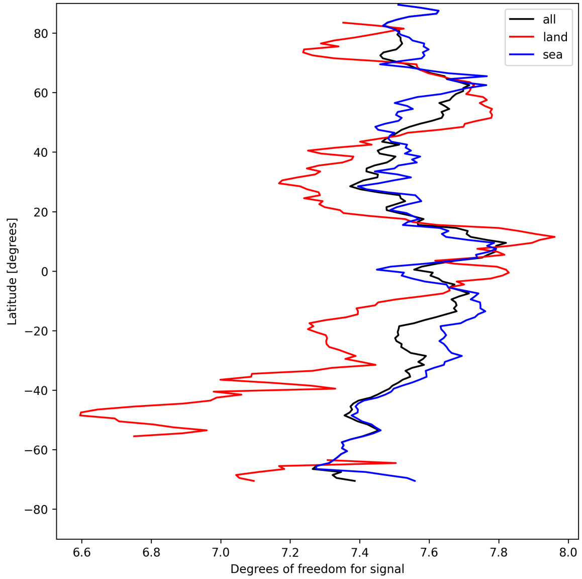
Figure 15: Zonal average of “Degrees of freedom for signal” for 2025-08-14 to 2025-08-15.
