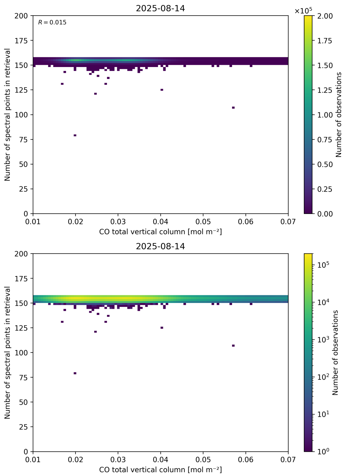
Figure 43: Scatter density plot of “CO total vertical column” against “Number of spectral points in retrieval” for 2025-08-14 to 2025-08-15.
