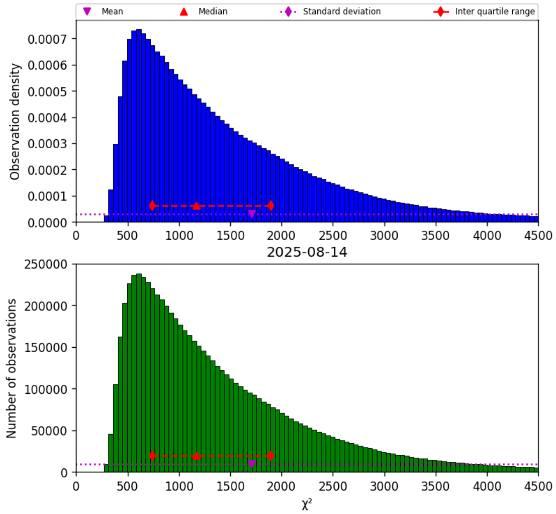
Figure 22: Histogram of “ \chi^2 ” for 2025-08-14 to 2025-08-15
