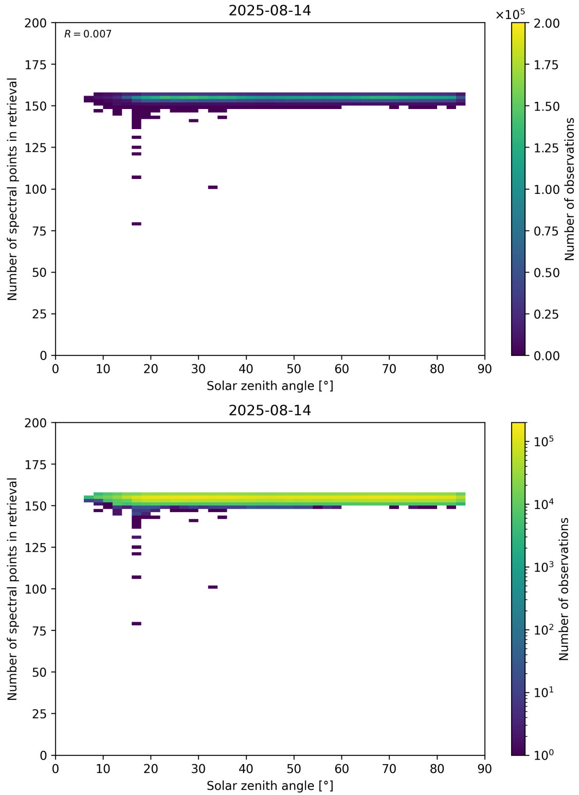
Figure 68: Scatter density plot of “Solar zenith angle” against “Number of spectral points in retrieval” for 2025-08-14 to 2025-08-15.
