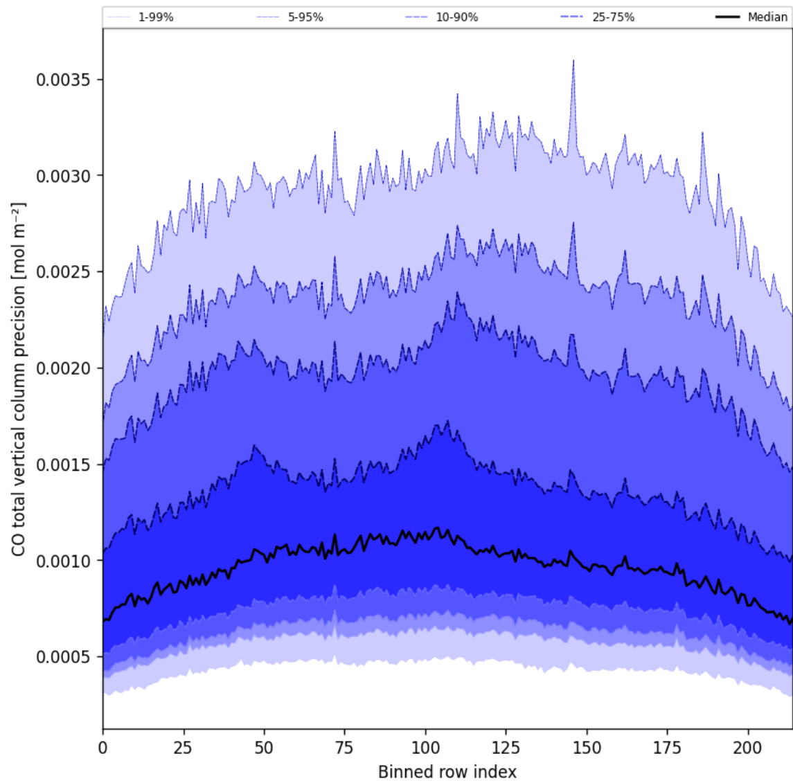
Figure 28: Along track statistics of “CO total vertical column precision” for 2025-08-14 to 2025-08-15
