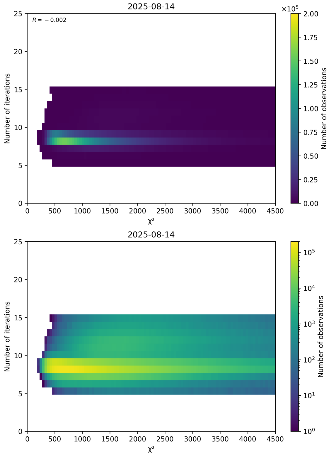
Figure 49: Scatter density plot of “ \chi^2 ” against “Number of iterations” for 2025-08-14 to 2025-08-15.
