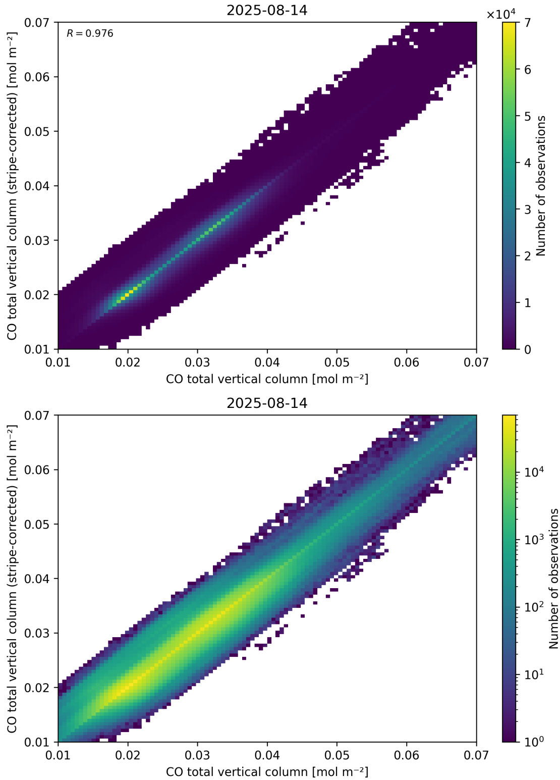
Figure 33: Scatter density plot of “CO total vertical column” against “CO total vertical column (stripe-corrected)” for 2025-08-14 to 2025-08-15.
