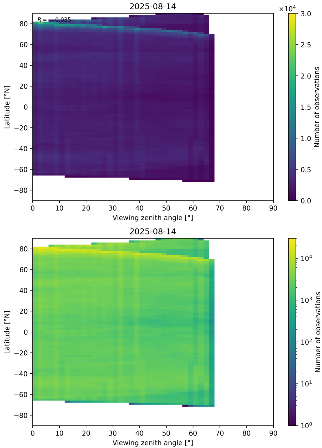
Figure 74: Scatter density plot of “Viewing zenith angle” against “Latitude” for 2025-08-14 to 2025-08-15.
