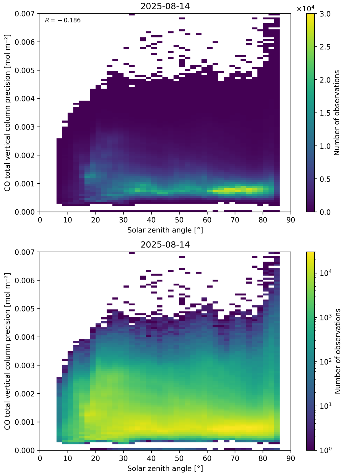
Figure 63: Scatter density plot of “Solar zenith angle” against “CO total vertical column precision” for 2025-08-14 to 2025-08-15.
