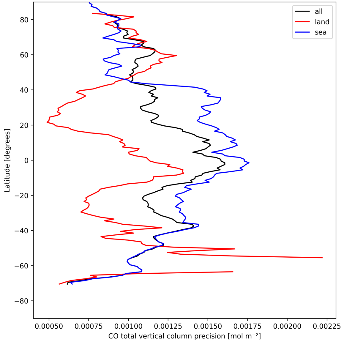
Figure 12: Zonal average of “CO total vertical column precision” for 2025-08-14 to 2025-08-15.
