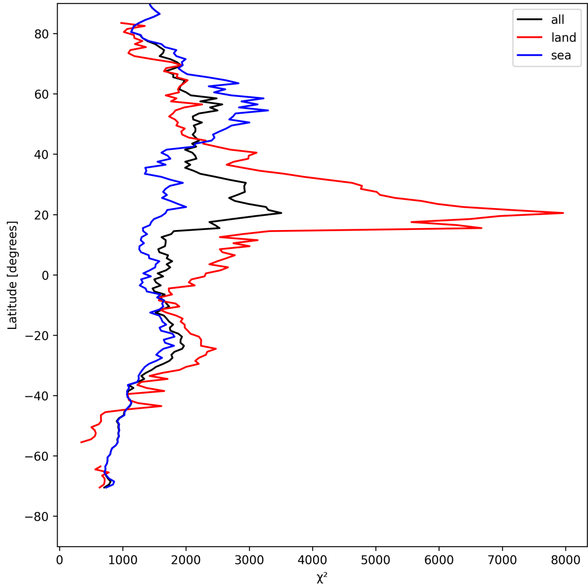
Figure 14: Zonal average of “ \chi^2 ” for 2025-08-14 to 2025-08-15.
