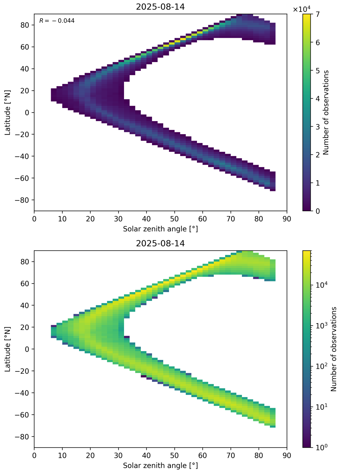
Figure 66: Scatter density plot of “Solar zenith angle” against “Latitude” for 2025-08-14 to 2025-08-15.
