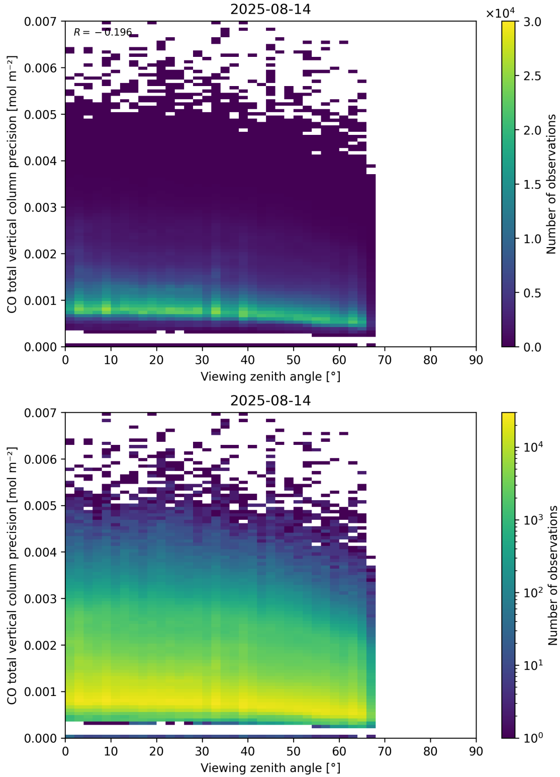
Figure 71: Scatter density plot of “Viewing zenith angle” against “CO total vertical column precision” for 2025-08-14 to 2025-08-15.
