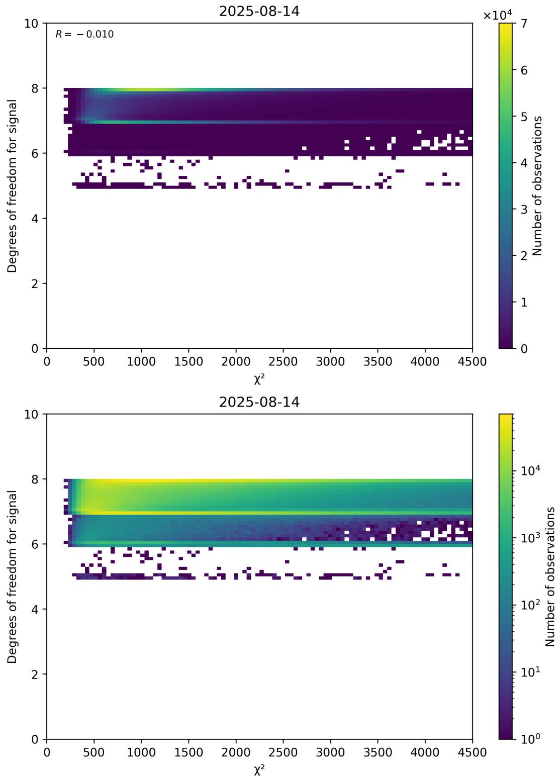
Figure 48: Scatter density plot of " \chi^2 " against "Degrees of freedom for signal" for 2025-08-14 to 2025-08-15.
