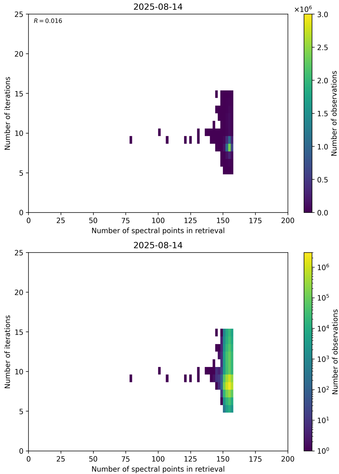
Figure 60: Scatter density plot of “Number of spectral points in retrieval” against “Number of iterations” for 2025-08-14 to 2025-08-15.
