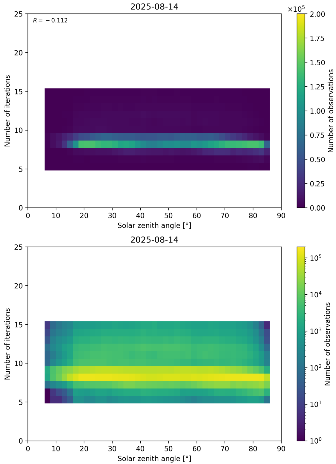
Figure 67: Scatter density plot of “Solar zenith angle” against “Number of iterations” for 2025-08-14 to 2025-08-15.
