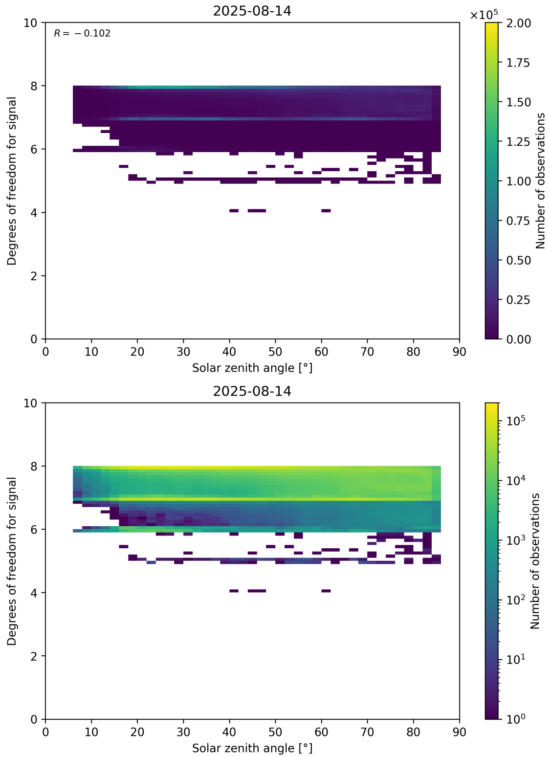
Figure 65: Scatter density plot of “Solar zenith angle” against “Degrees of freedom for signal” for 2025-08-14 to 2025-08-15.
