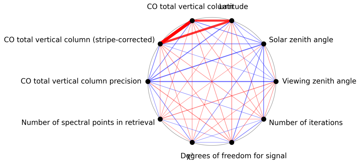
Figure 1: Map of correlation graph for 2025-08-14 to 2025-08-15.
