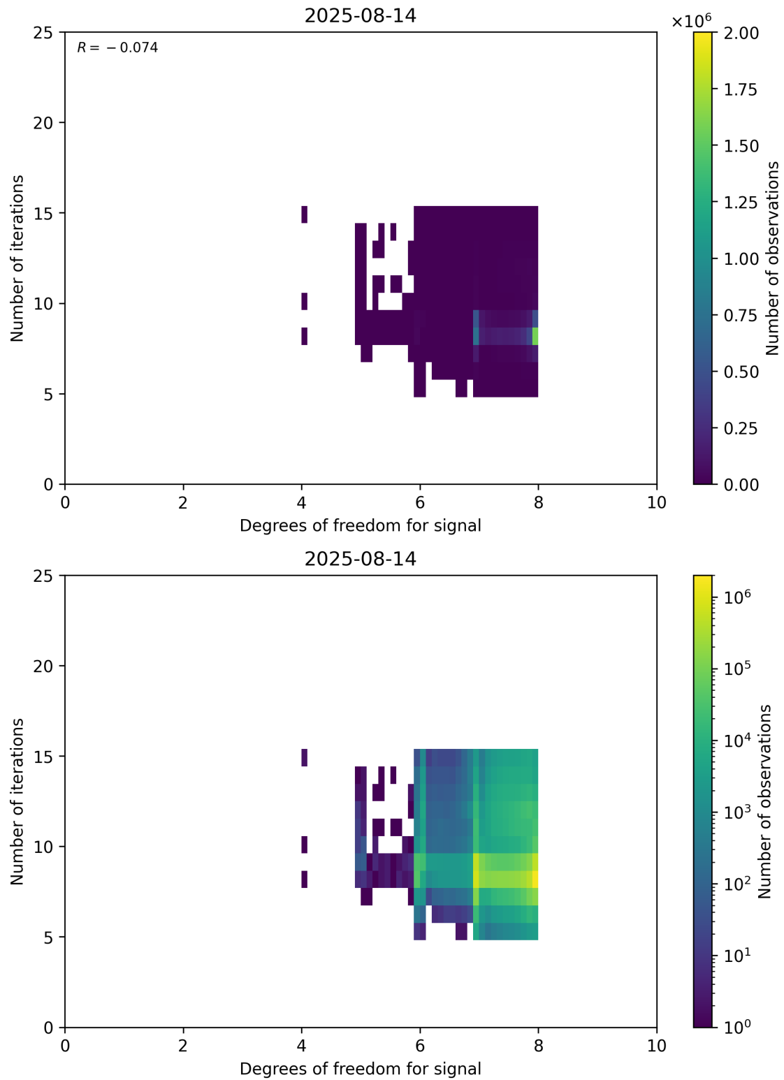
Figure 50: Scatter density plot of “Degrees of freedom for signal” against “Number of iterations” for 2025-08-14 to 2025-08-15.
