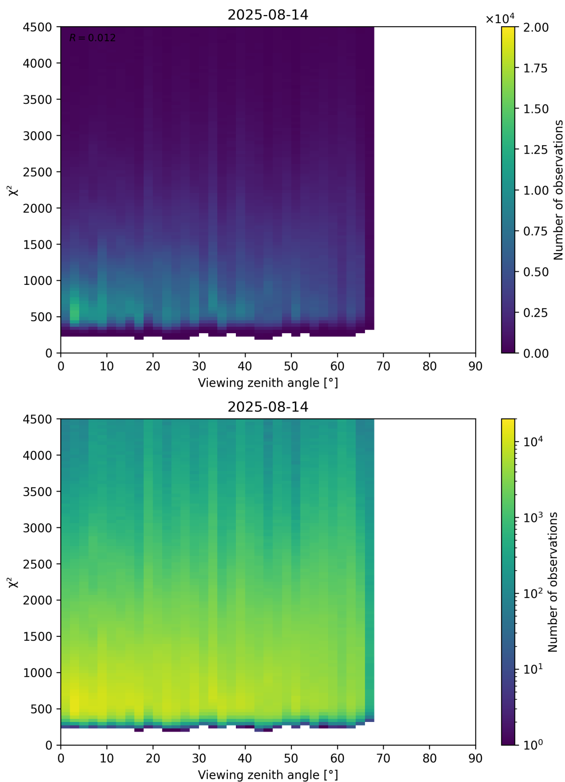
Figure 72: Scatter density plot of “Viewing zenith angle” against “ \chi^2 ” for 2025-08-14 to 2025-08-15.
