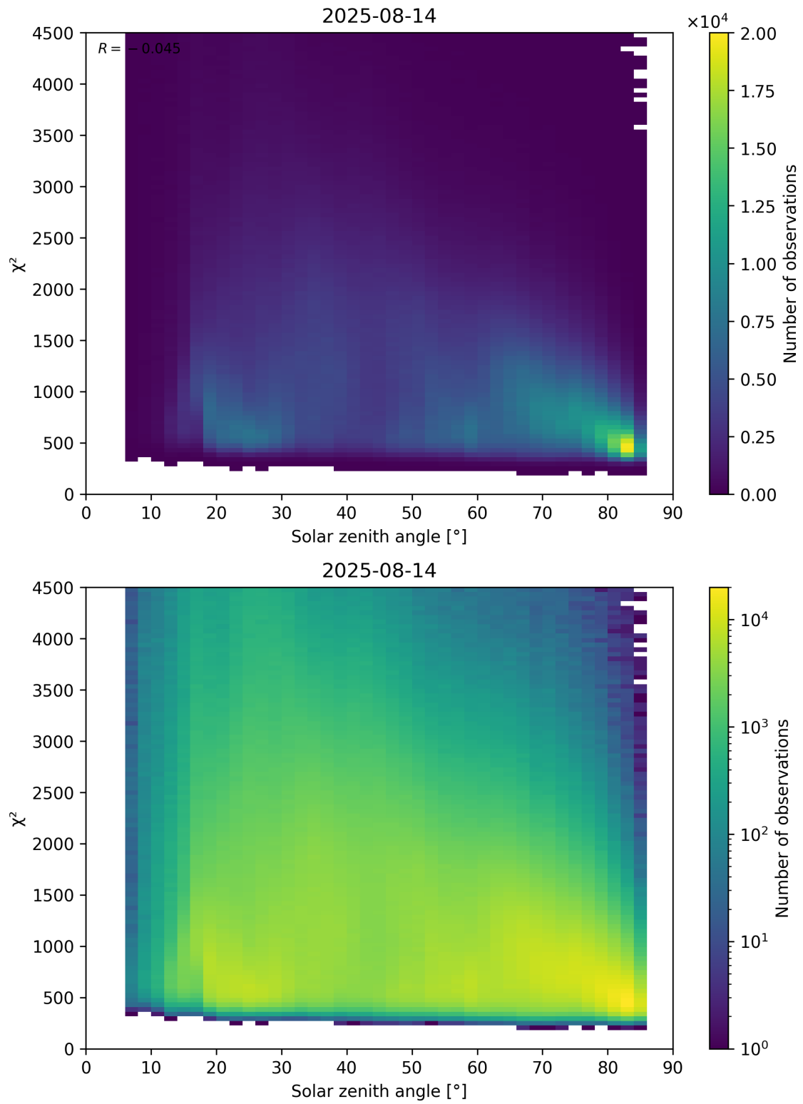
Figure 64: Scatter density plot of “Solar zenith angle” against “ \chi^2 ” for 2025-08-14 to 2025-08-15.
