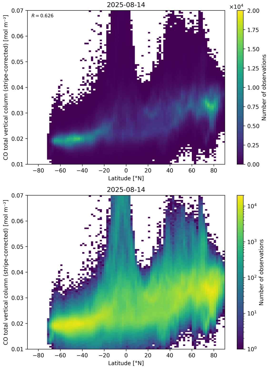
Figure 52: Scatter density plot of “Latitude” against “CO total vertical column (stripe-corrected)” for 2025-08-14 to 2025-08-15.
