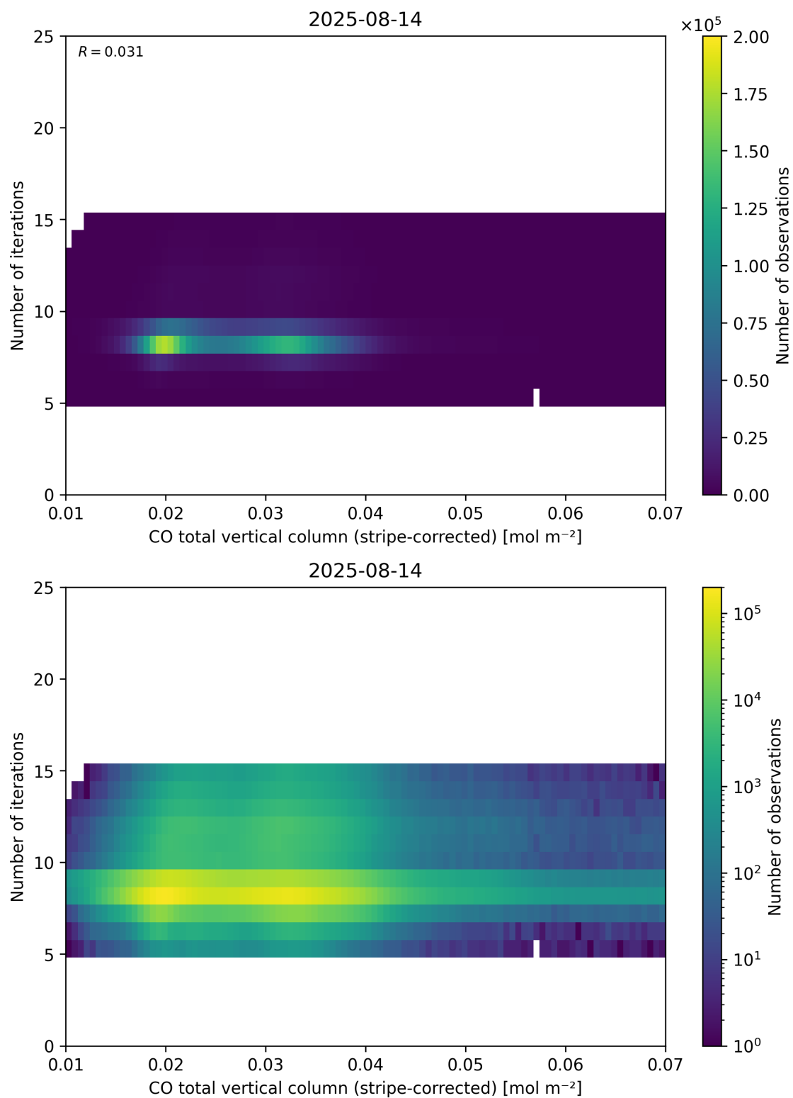
Figure 39: Scatter density plot of “CO total vertical column (stripe-corrected)” against “Number of iterations” for 2025-08-14 to 2025-08-15.
