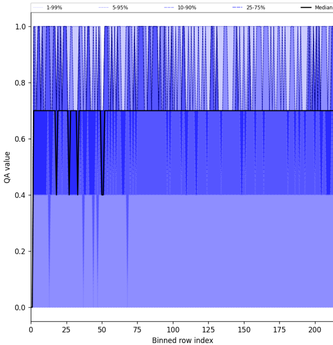
Figure 25: Along track statistics of “QA value” for 2025-08-14 to 2025-08-15
