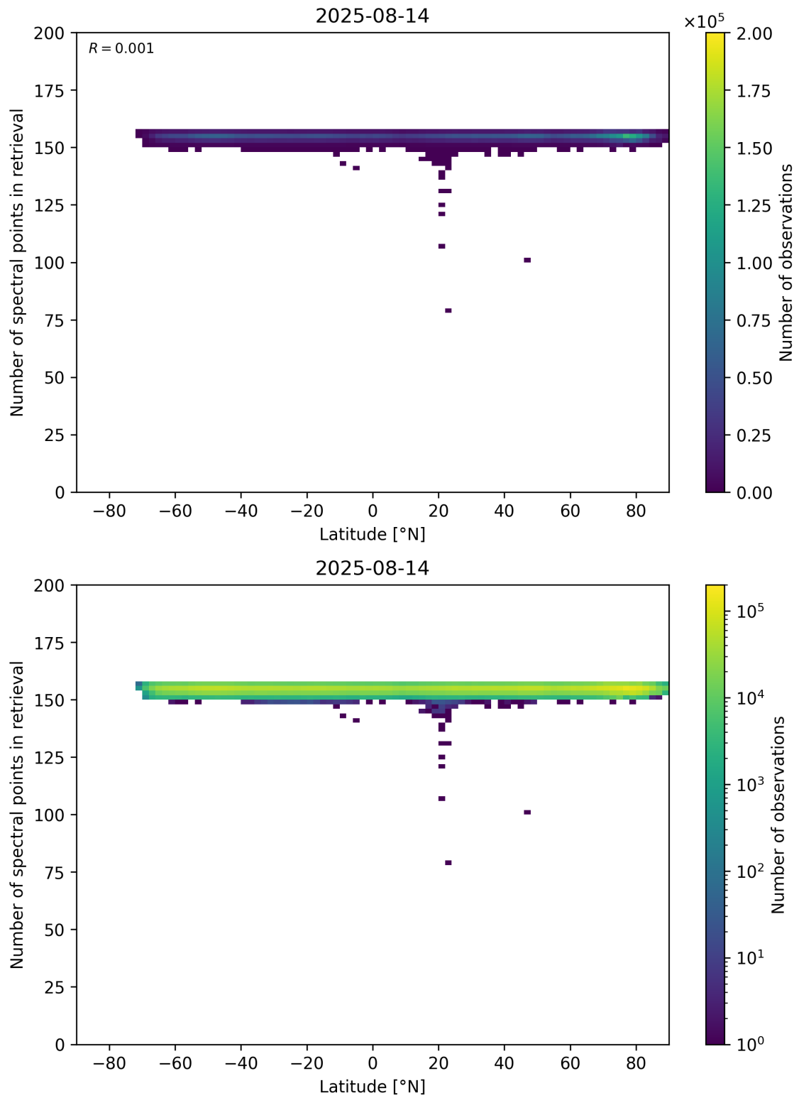
Figure 57: Scatter density plot of “Latitude” against “Number of spectral points in retrieval” for 2025-08-14 to 2025-08-15.
