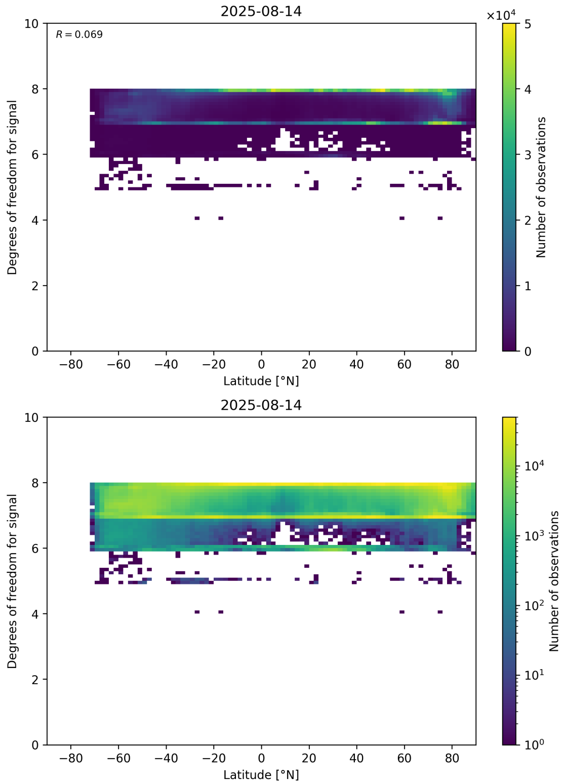
Figure 55: Scatter density plot of “Latitude” against “Degrees of freedom for signal” for 2025-08-14 to 2025-08-15.
