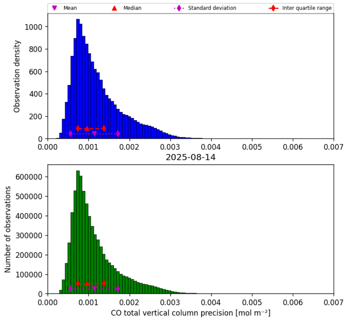
Figure 20: Histogram of “CO total vertical column precision” for 2025-08-14 to 2025-08-15
