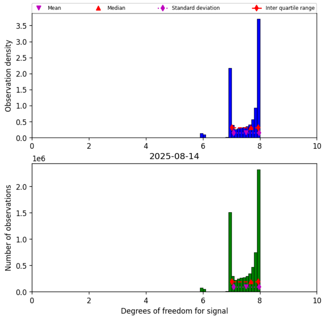
Figure 23: Histogram of “Degrees of freedom for signal” for 2025-08-14 to 2025-08-15
