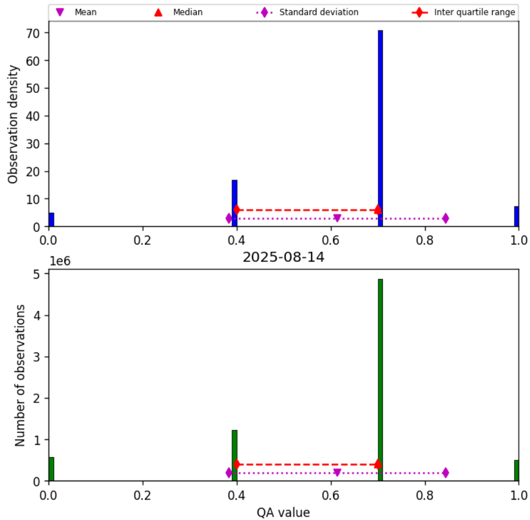
Figure 17: Histogram of “QA value” for 2025-08-14 to 2025-08-15
