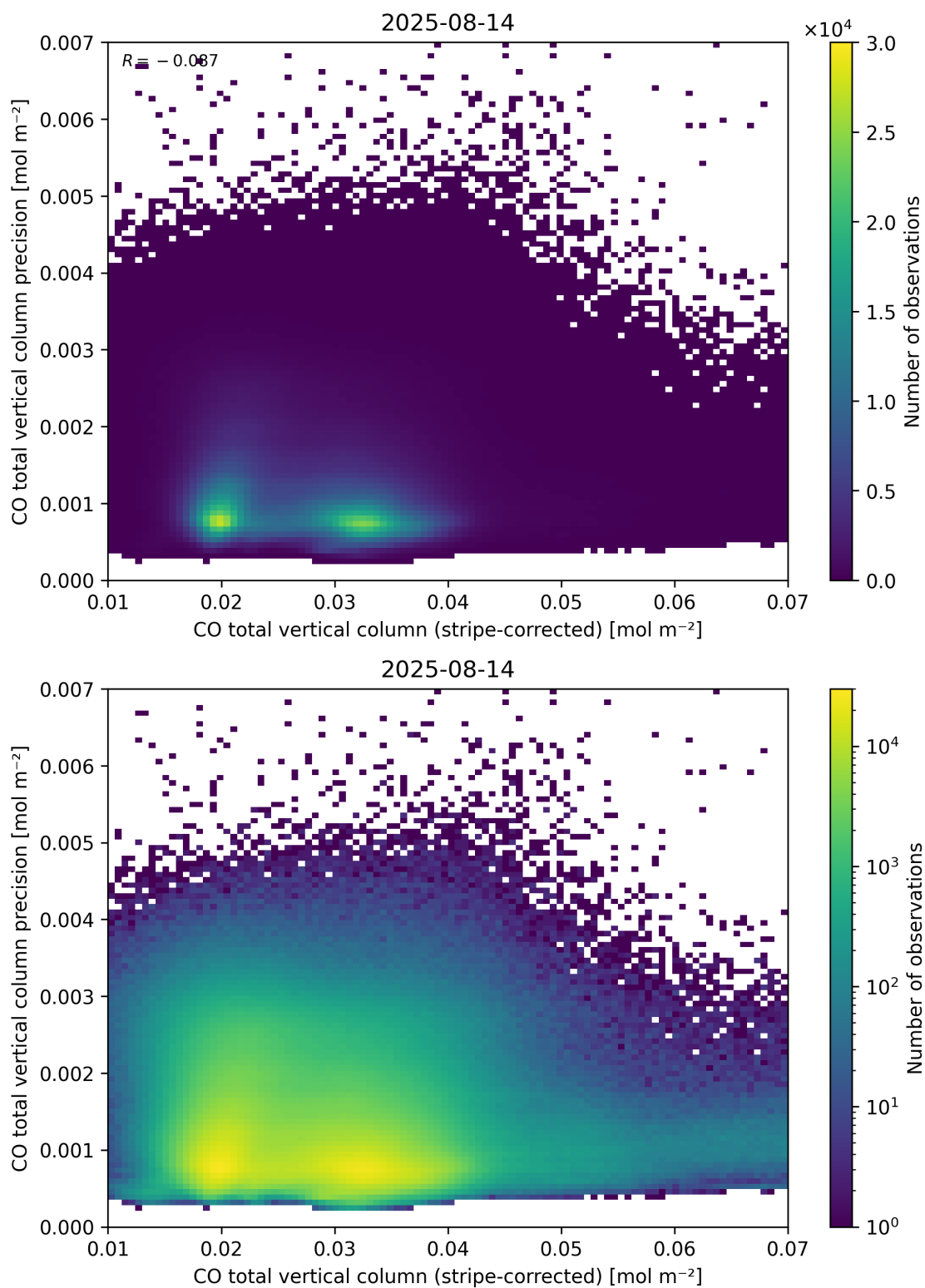
Figure 36: Scatter density plot of “CO total vertical column (stripe-corrected)” against “CO total vertical column precision” for 2025-08-14 to 2025-08-15.
