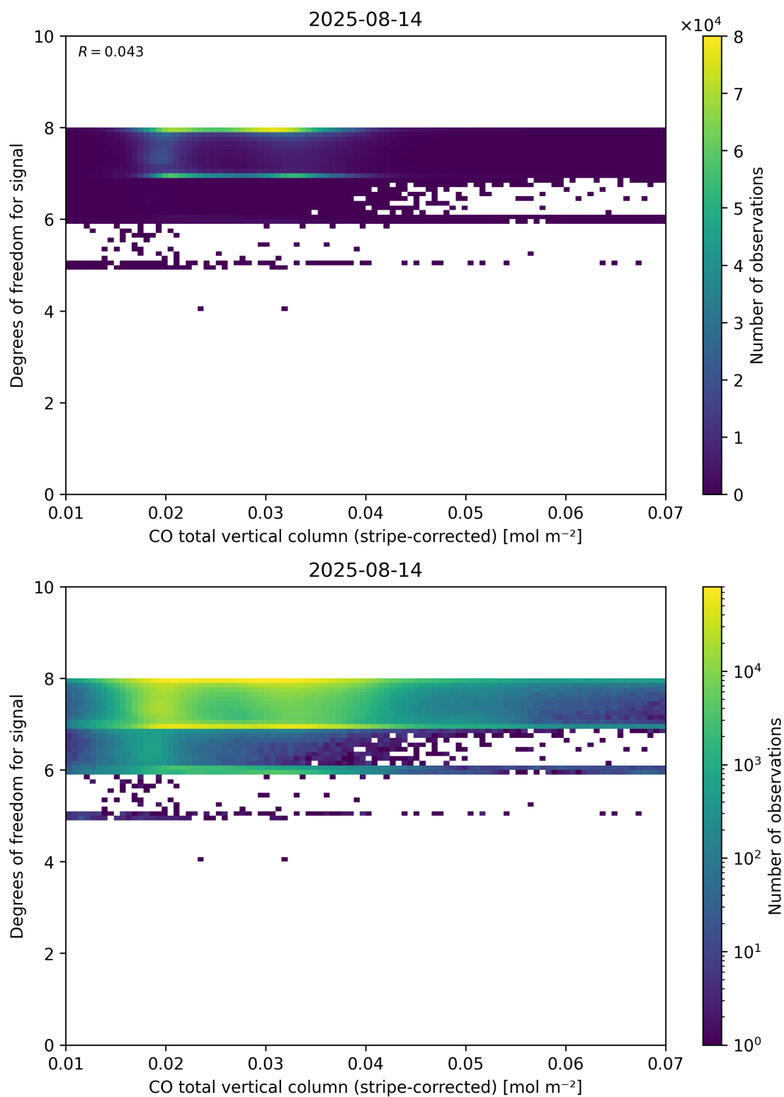
Figure 38: Scatter density plot of “CO total vertical column (stripe-corrected)” against “Degrees of freedom for signal” for 2025-08-14 to 2025-08-15.
