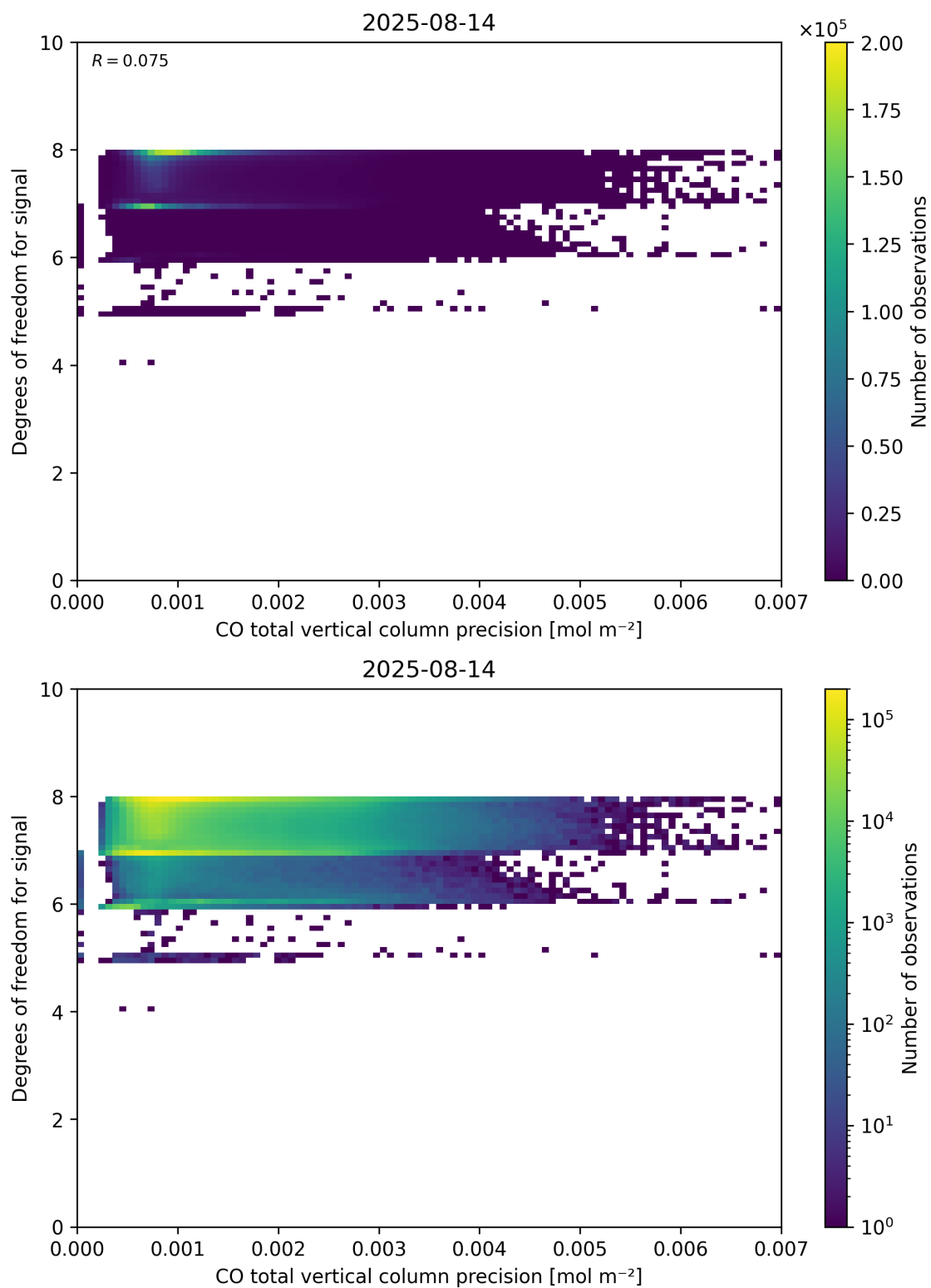
Figure 45: Scatter density plot of “CO total vertical column precision” against “Degrees of freedom for signal” for 2025-08-14 to 2025-08-15.
