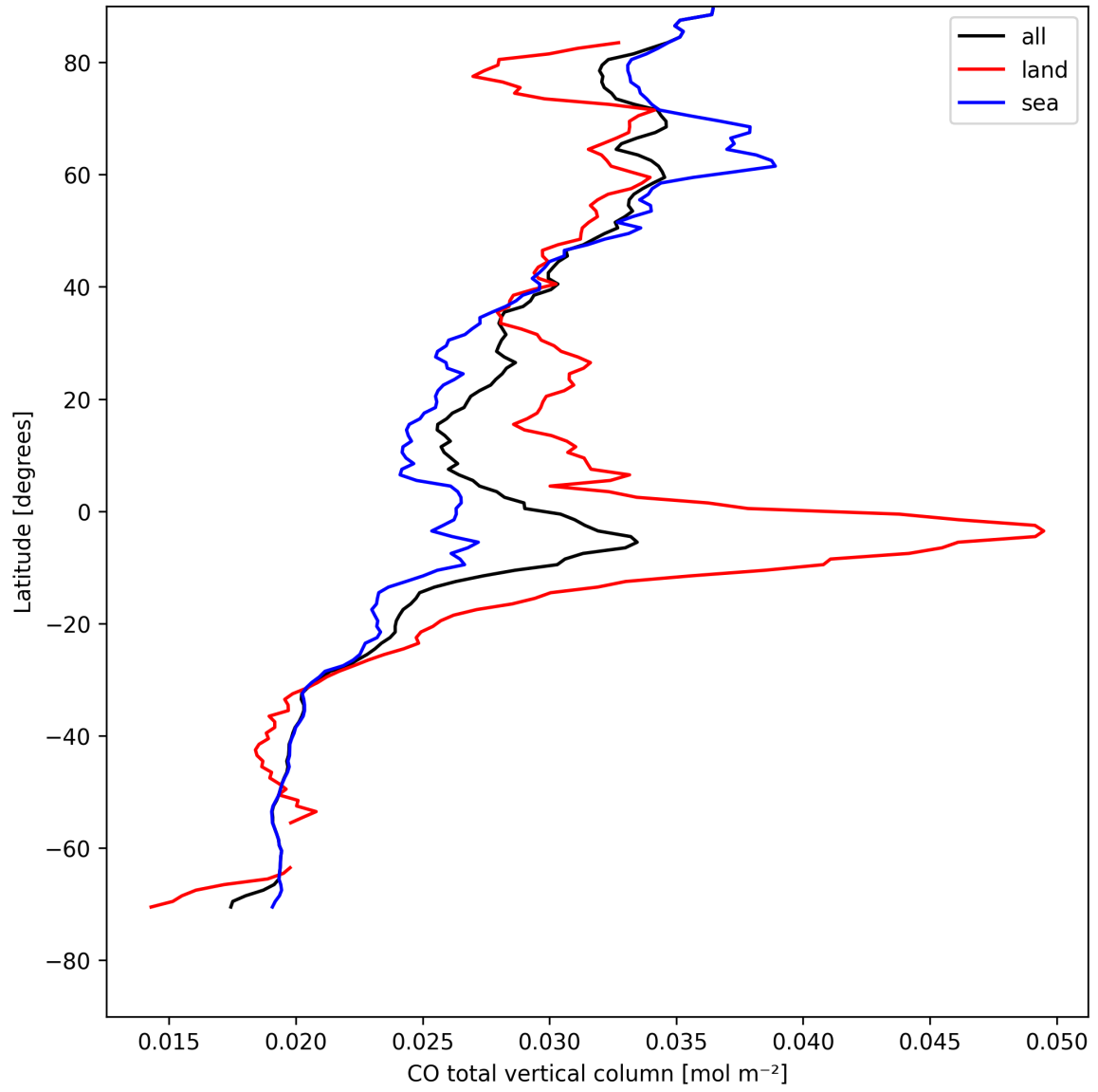
Figure 10: Zonal average of “CO total vertical column” for 2025-08-14 to 2025-08-15.
