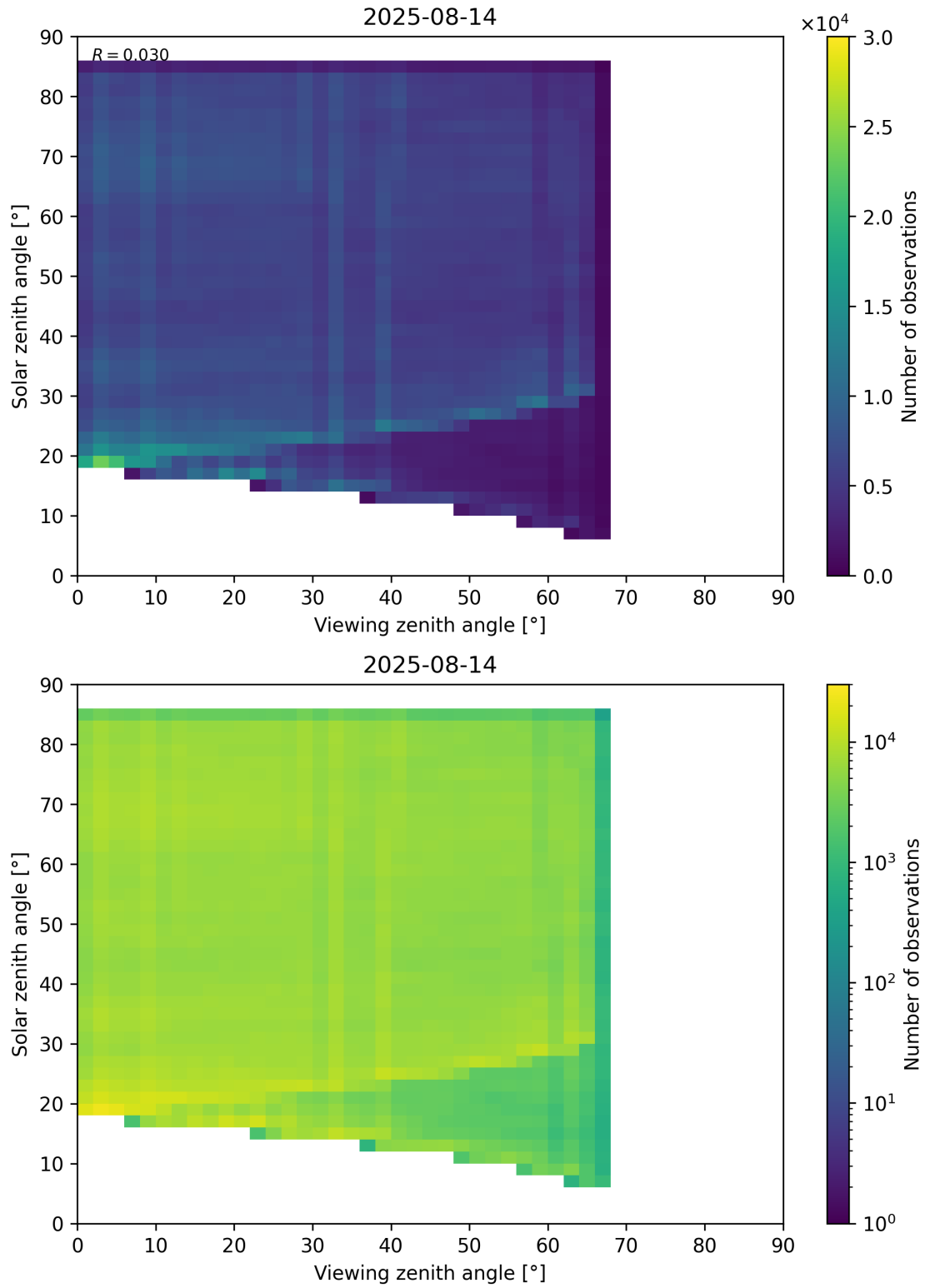
Figure 77: Scatter density plot of “Viewing zenith angle” against “Solar zenith angle” for 2025-08-14 to 2025-08-15.
