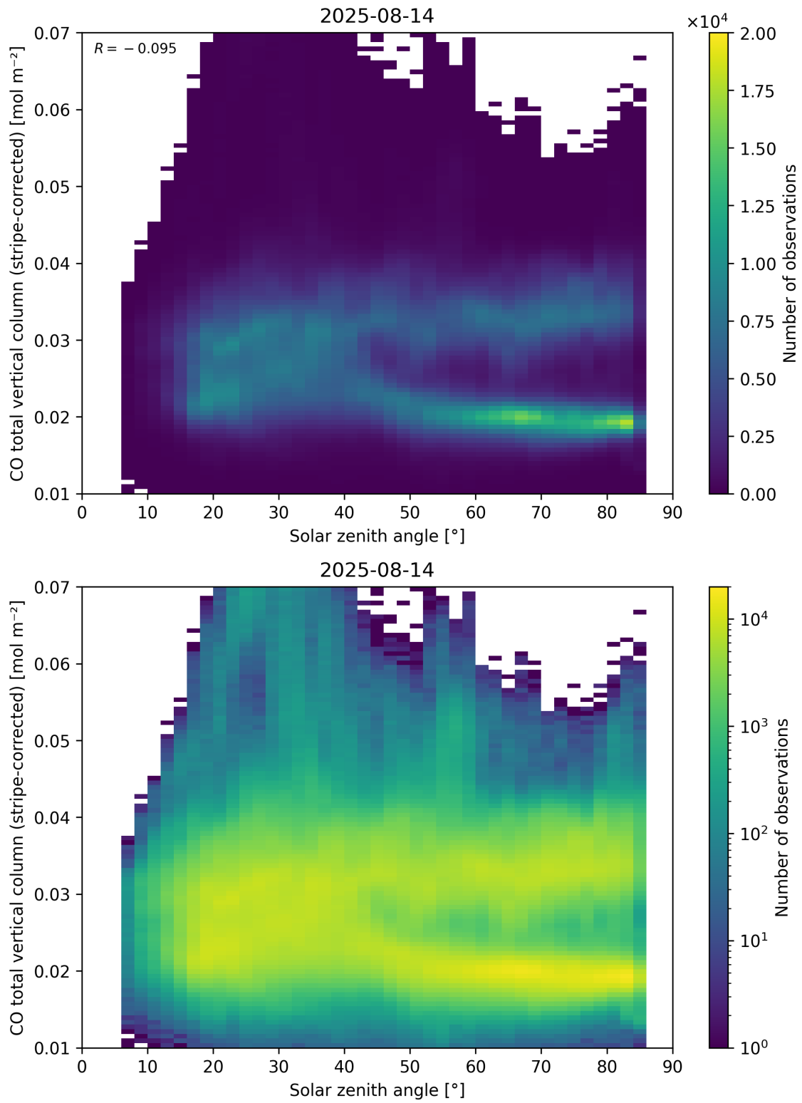
Figure 62: Scatter density plot of “Solar zenith angle” against “CO total vertical column (stripe-corrected)” for 2025-08-14 to 2025-08-15.
