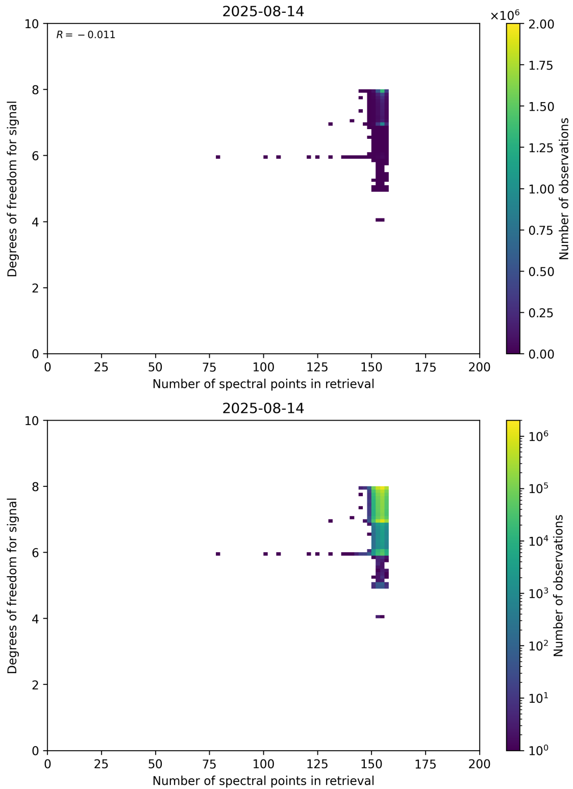
Figure 59: Scatter density plot of “Number of spectral points in retrieval” against “Degrees of freedom for signal” for 2025-08-14 to 2025-08-15.
