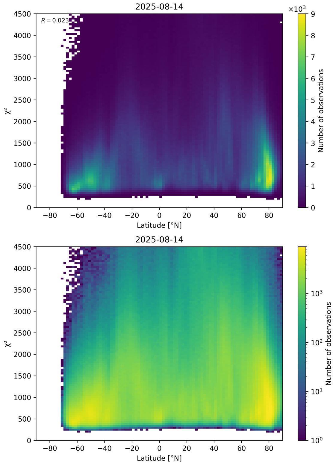
Figure 54: Scatter density plot of “Latitude” against “ \chi^2 ” for 2025-08-14 to 2025-08-15.
