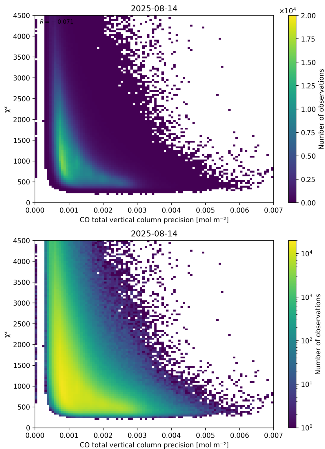
Figure 44: Scatter density plot of “CO total vertical column precision” against “ \chi^2 ” for 2025-08-14 to 2025-08-15.
