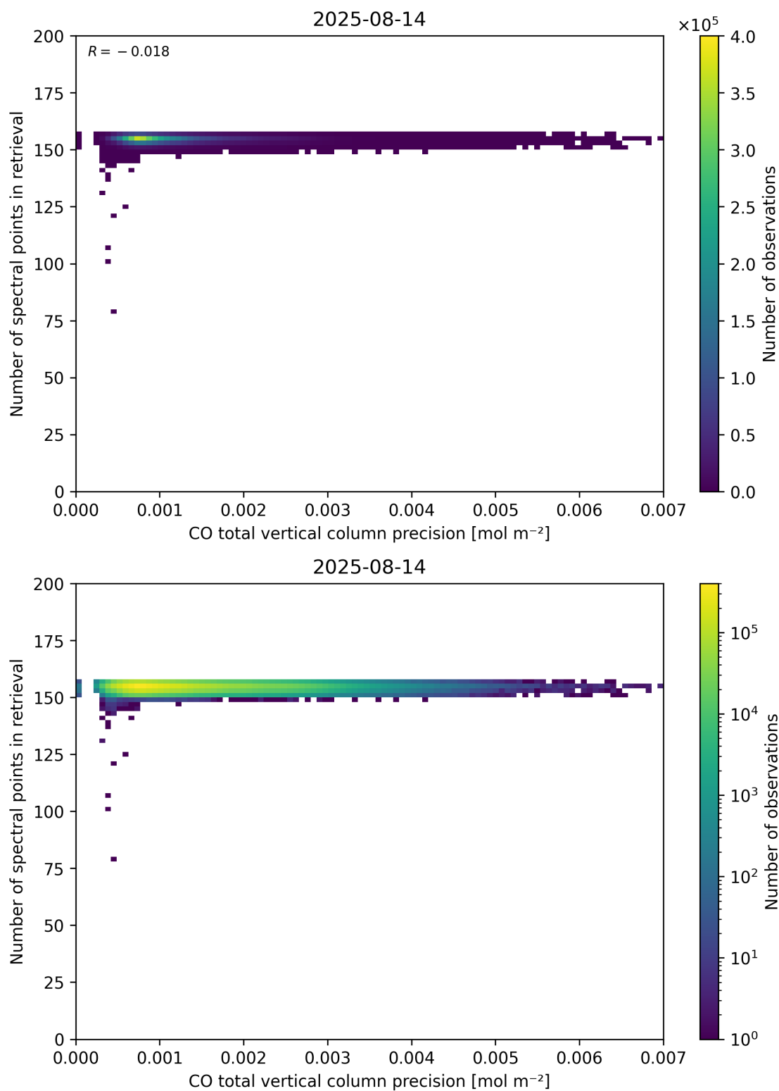
Figure 47: Scatter density plot of “CO total vertical column precision” against “Number of spectral points in retrieval” for 2025-08-14 to 2025-08-15.
