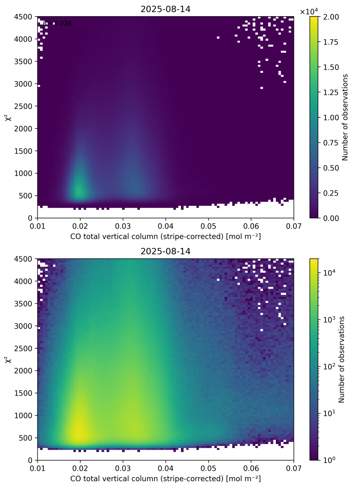
Figure 37: Scatter density plot of “CO total vertical column (stripe-corrected)” against “ \chi^2 ” for 2025-08-14 to 2025-08-15.
