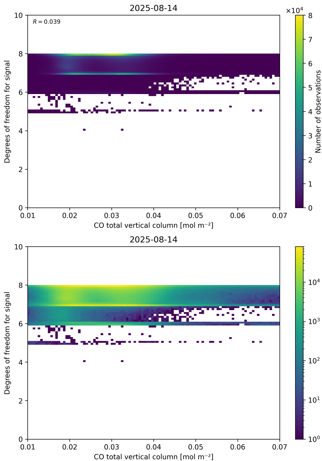
Figure 41: Scatter density plot of “CO total vertical column” against “Degrees of freedom for signal” for 2025-08-14 to 2025-08-15.
