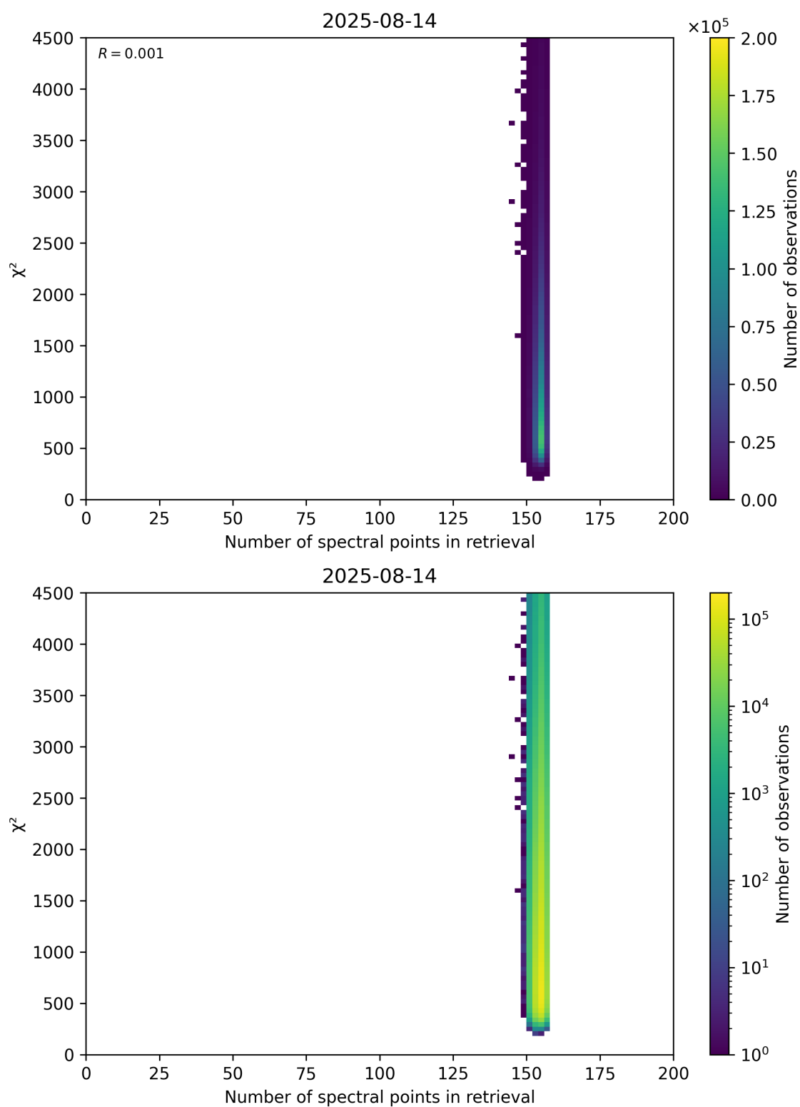
Figure 58: Scatter density plot of “Number of spectral points in retrieval” against “ \chi^2 ” for 2025-08-14 to 2025-08-15.
