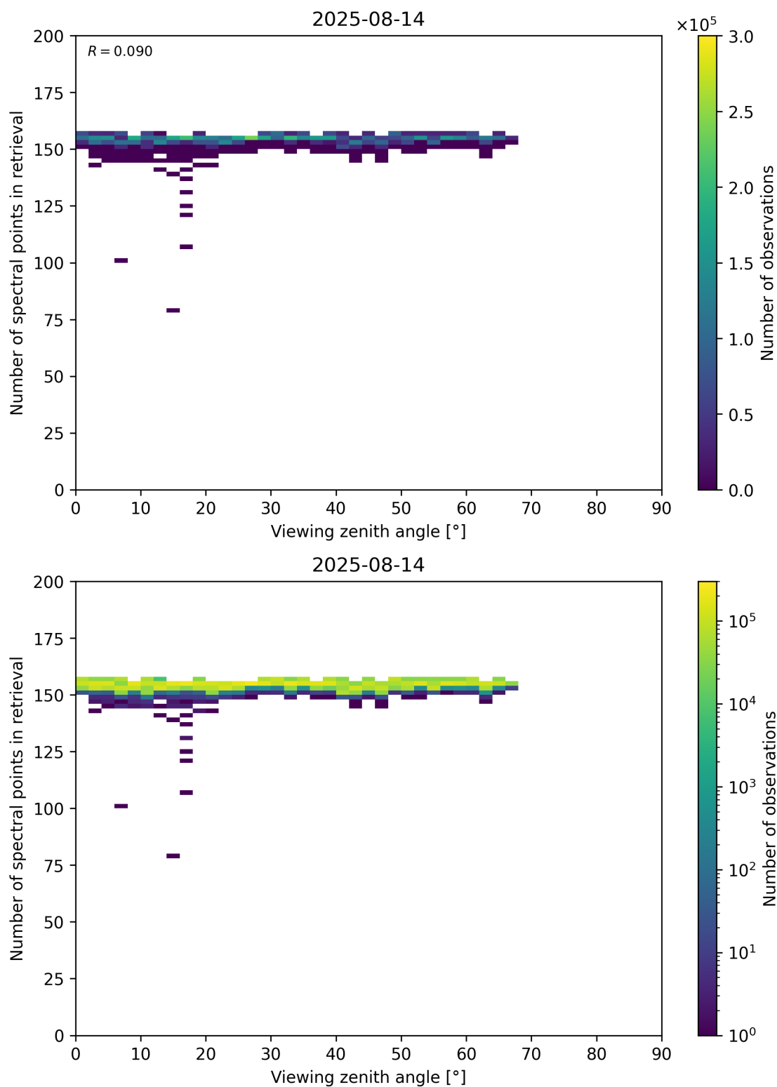
Figure 76: Scatter density plot of “Viewing zenith angle” against “Number of spectral points in retrieval” for 2025-08-14 to 2025-08-15.
