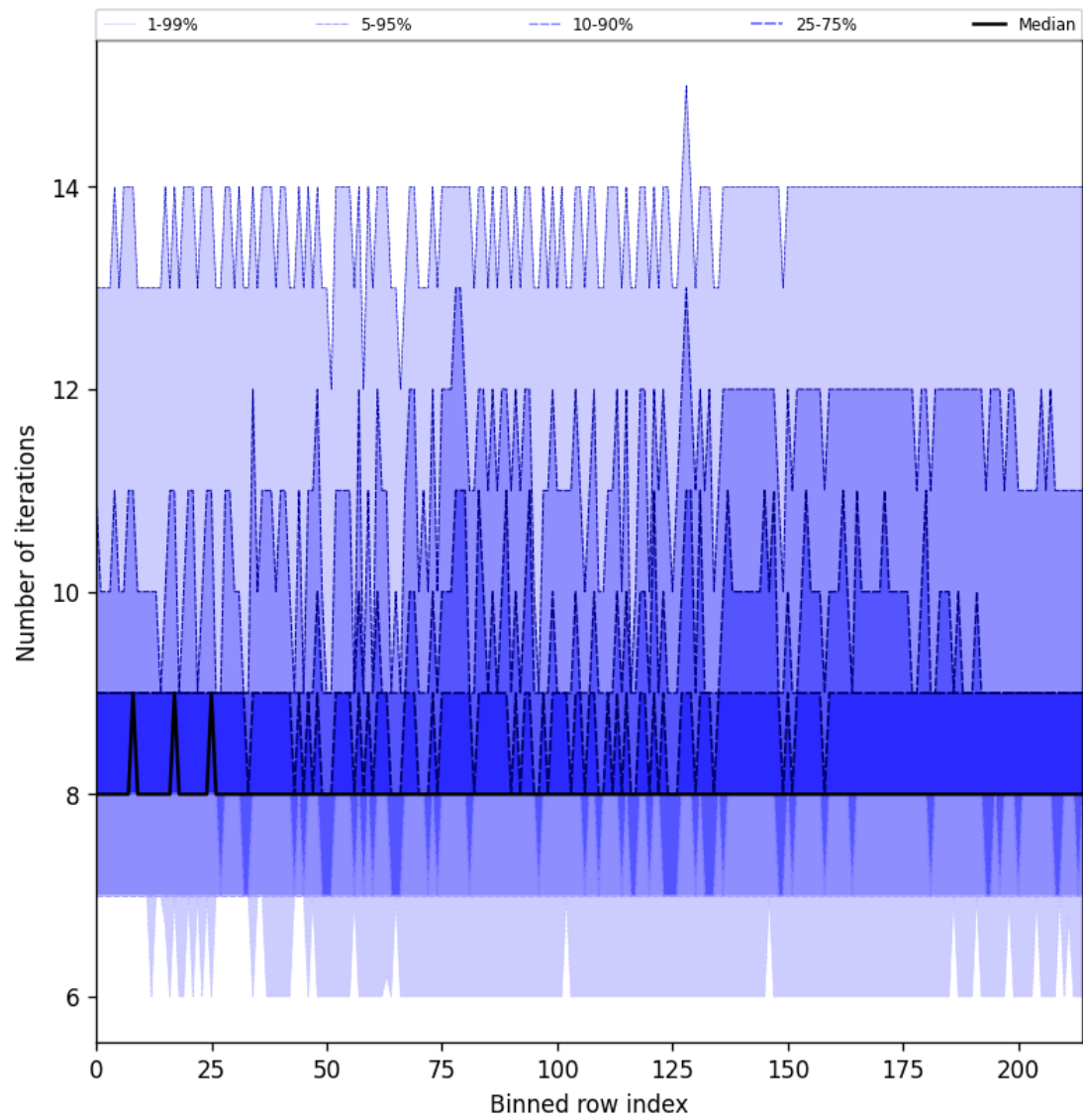
Figure 32: Along track statistics of “Number of iterations” for 2025-08-14 to 2025-08-15
