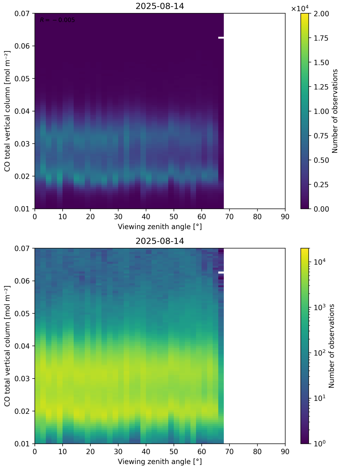
Figure 69: Scatter density plot of “Viewing zenith angle” against “CO total vertical column” for 2025-08-14 to 2025-08-15.
