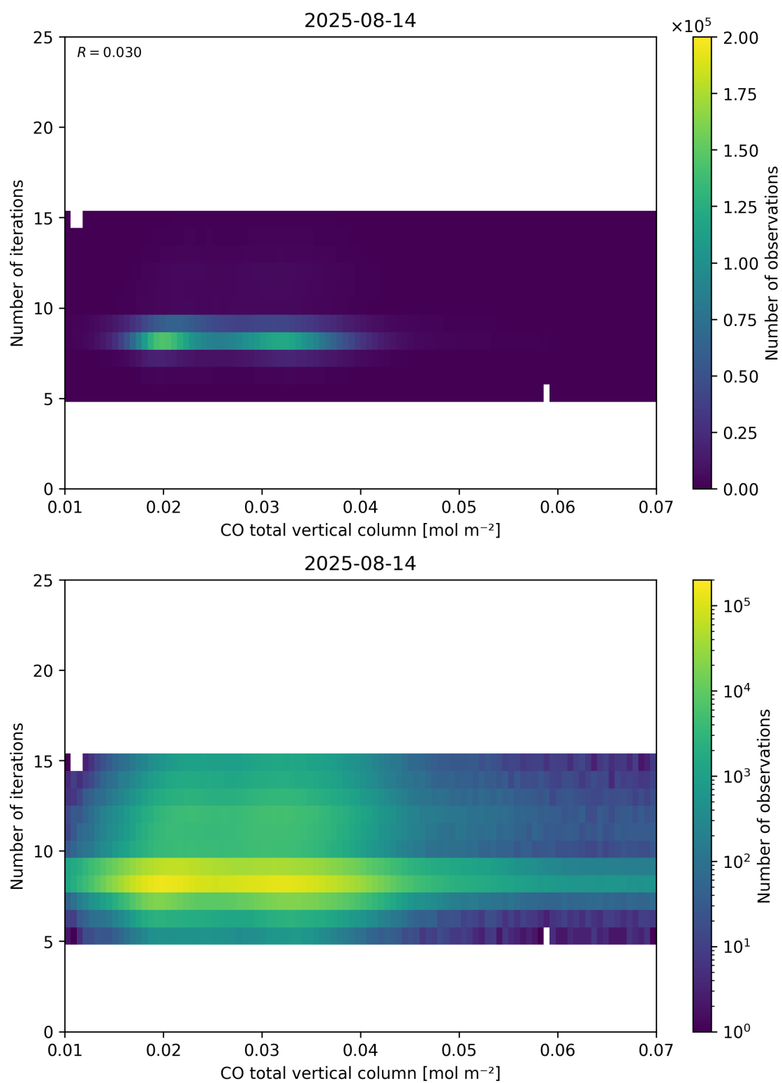
Figure 42: Scatter density plot of “CO total vertical column” against “Number of iterations” for 2025-08-14 to 2025-08-15.
