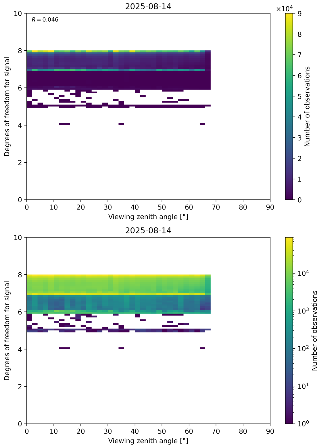
Figure 73: Scatter density plot of “Viewing zenith angle” against “Degrees of freedom for signal” for 2025-08-14 to 2025-08-15.
