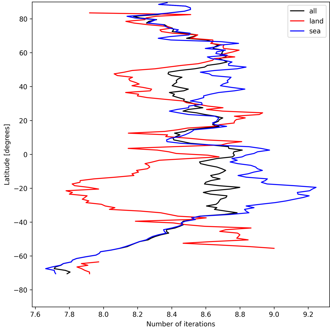
Figure 16: Zonal average of “Number of iterations” for 2025-08-14 to 2025-08-15.
