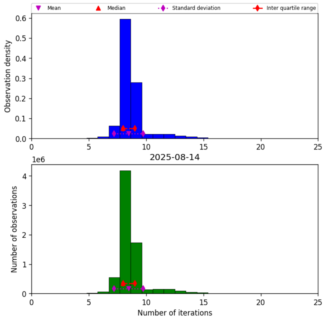
Figure 24: Histogram of “Number of iterations” for 2025-08-14 to 2025-08-15
