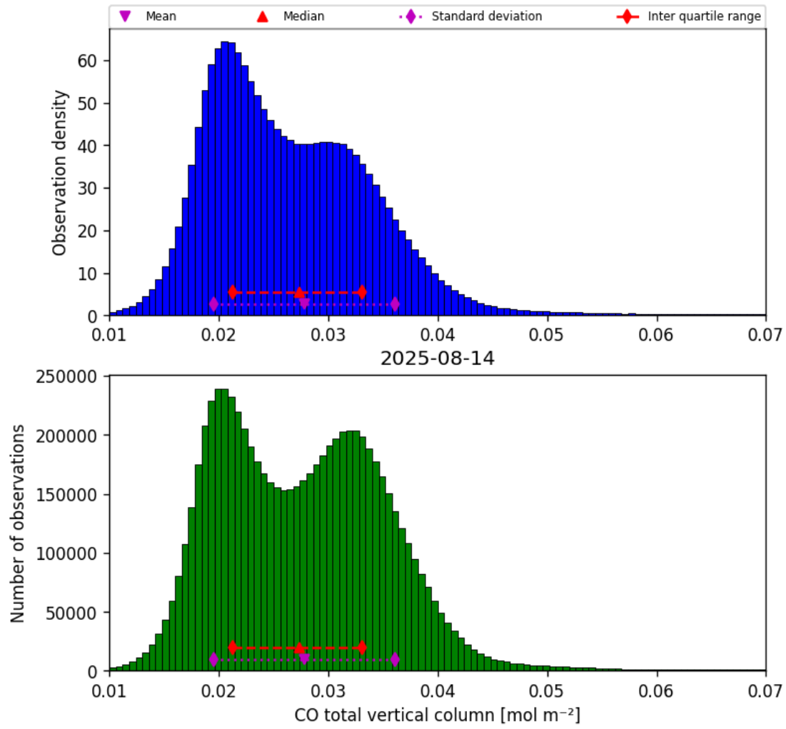
Figure 18: Histogram of “CO total vertical column” for 2025-08-14 to 2025-08-15
