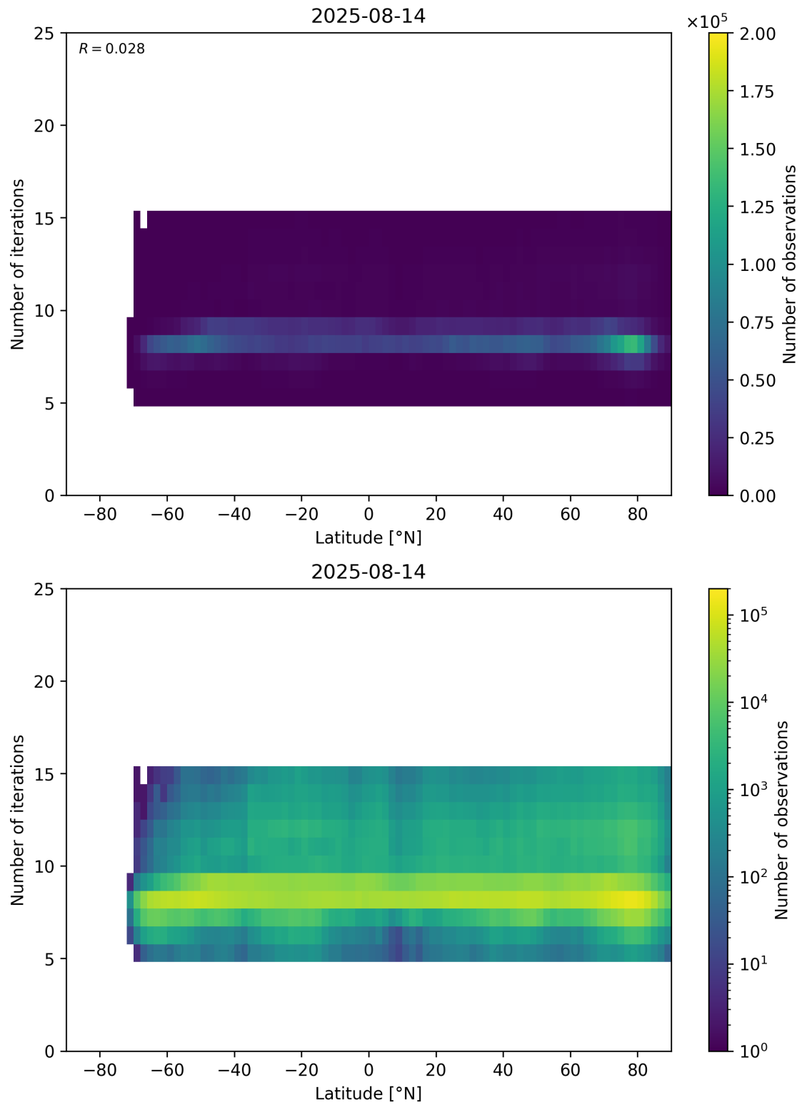
Figure 56: Scatter density plot of “Latitude” against “Number of iterations” for 2025-08-14 to 2025-08-15.
