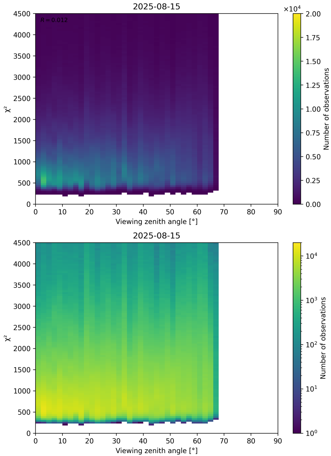
Figure 72: Scatter density plot of “Viewing zenith angle” against “ \chi^2 ” for 2025-08-14 to 2025-08-16.
