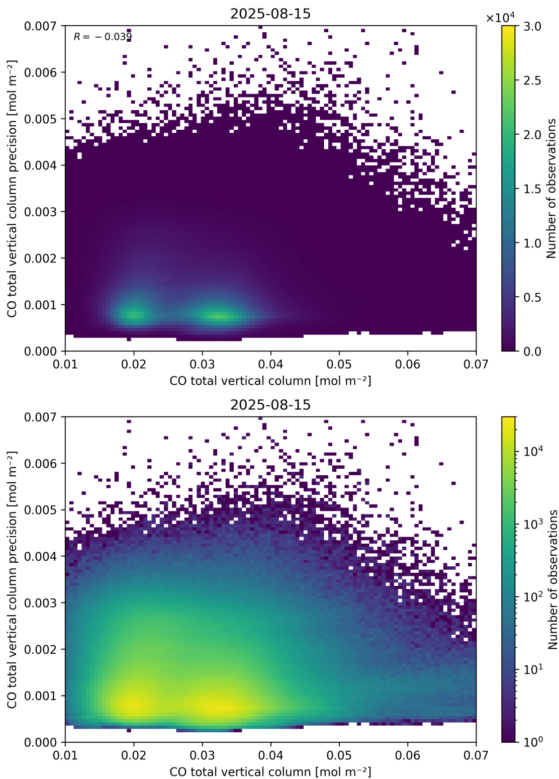
Figure 34: Scatter density plot of “CO total vertical column” against “CO total vertical column precision” for 2025-08-14 to 2025-08-16.
