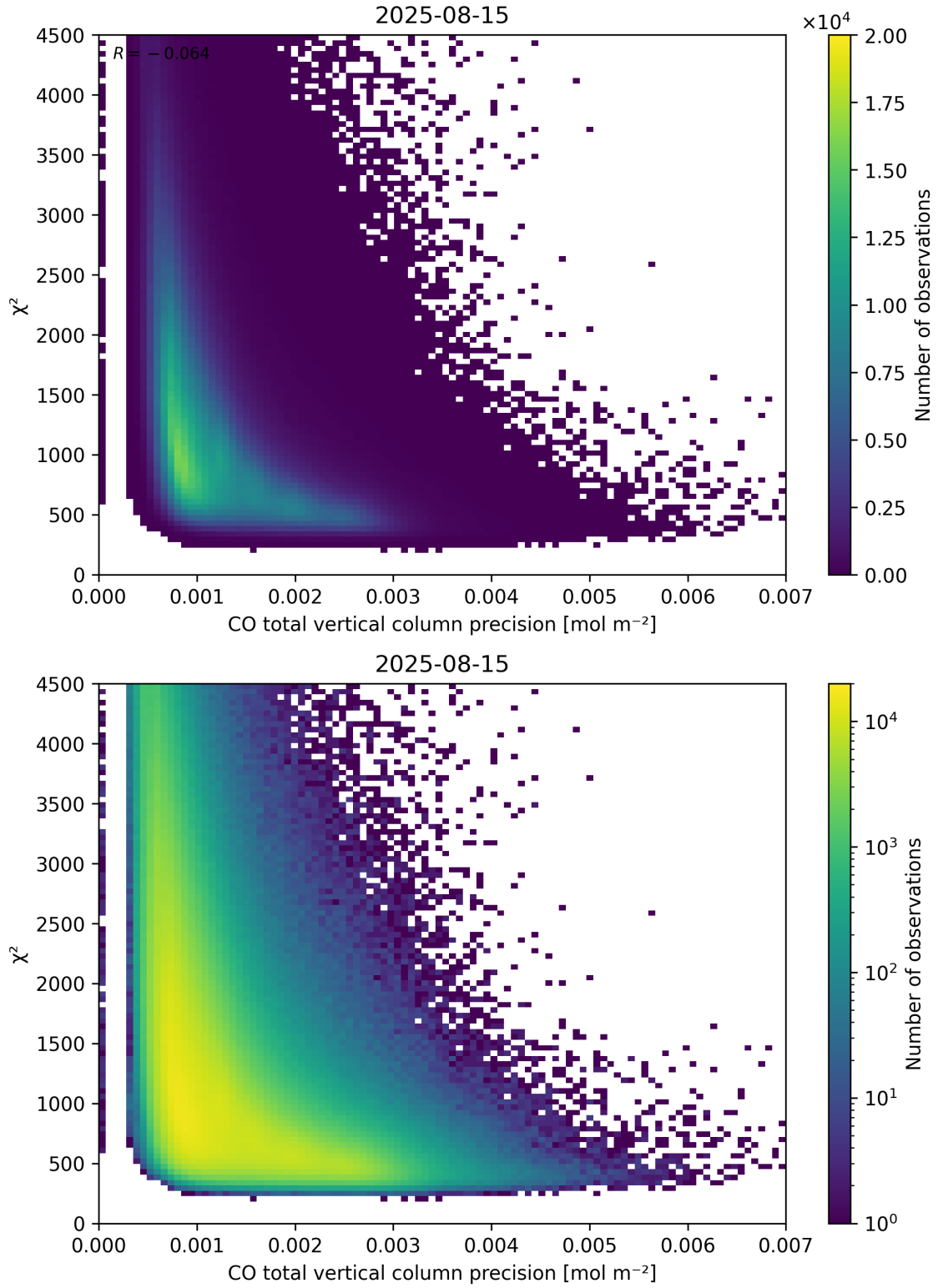
Figure 44: Scatter density plot of “CO total vertical column precision” against “ \chi^2 ” for 2025-08-14 to 2025-08-16.
