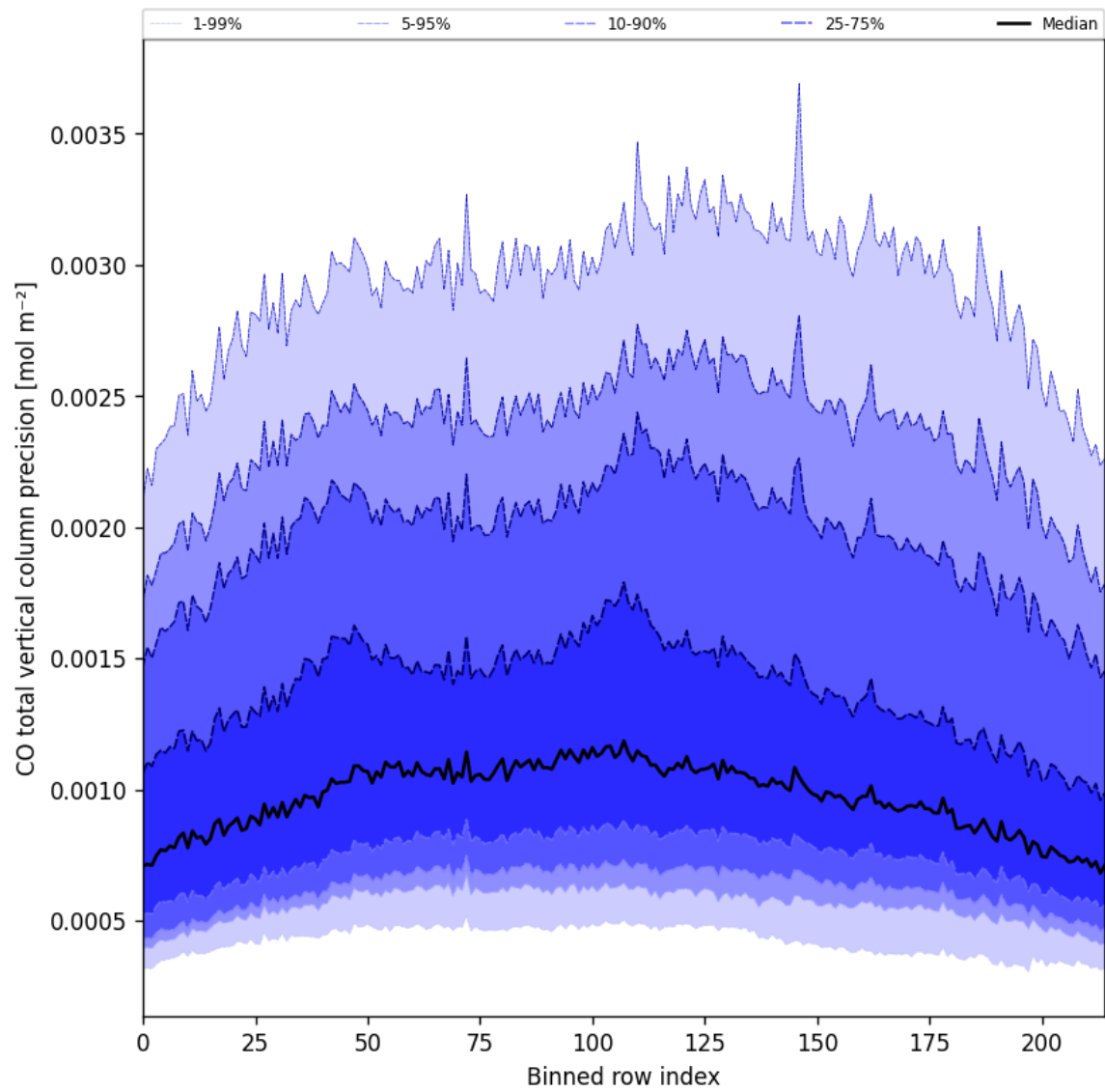
Figure 28: Along track statistics of “CO total vertical column precision” for 2025-08-14 to 2025-08-16
