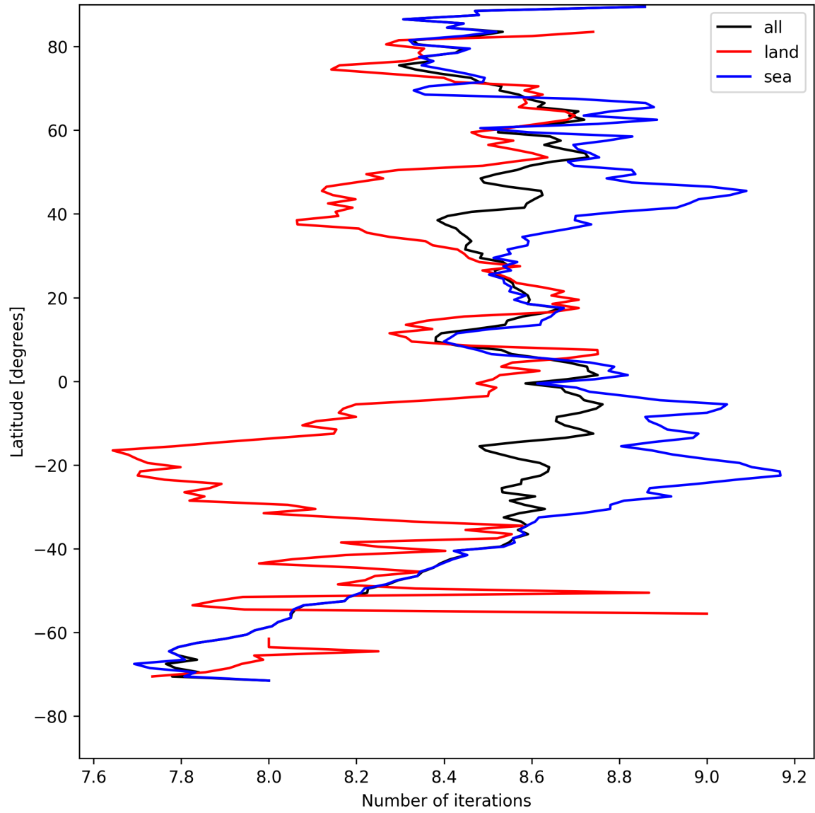
Figure 16: Zonal average of “Number of iterations” for 2025-08-14 to 2025-08-16.
