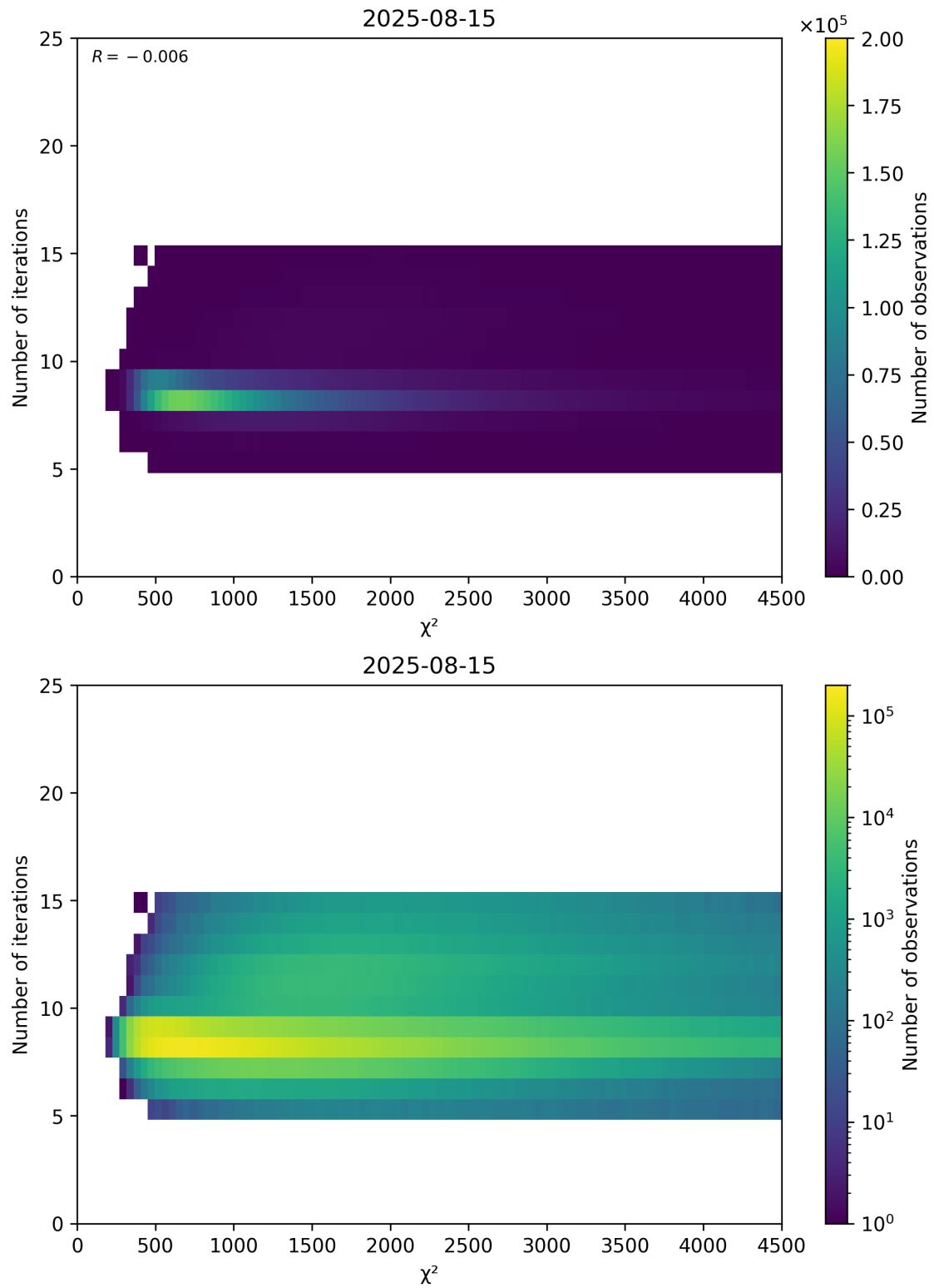
Figure 49: Scatter density plot of “ \chi^2 ” against “Number of iterations” for 2025-08-14 to 2025-08-16.
