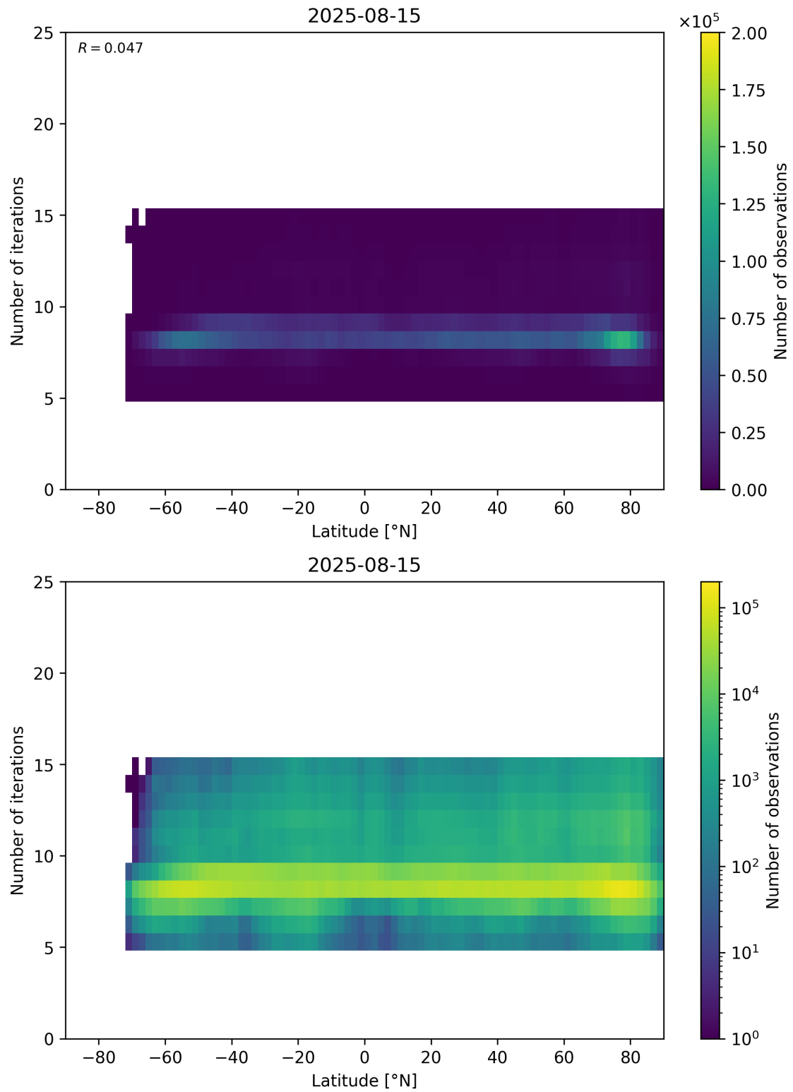
Figure 56: Scatter density plot of “Latitude” against “Number of iterations” for 2025-08-14 to 2025-08-16.
