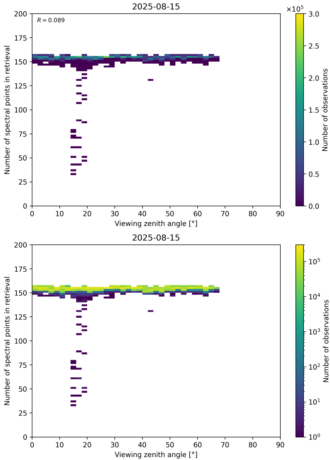
Figure 76: Scatter density plot of “Viewing zenith angle” against “Number of spectral points in retrieval” for 2025-08-14 to 2025-08-16.
