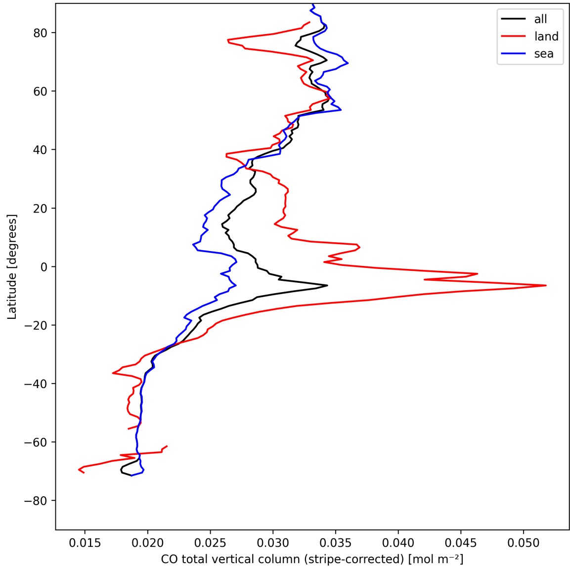
Figure 11: Zonal average of “CO total vertical column (stripe-corrected)” for 2025-08-14 to 2025-08-16.
