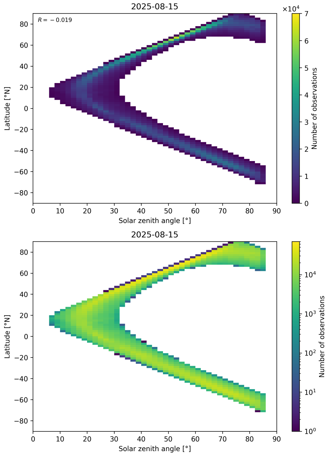
Figure 66: Scatter density plot of “Solar zenith angle” against “Latitude” for 2025-08-14 to 2025-08-16.
