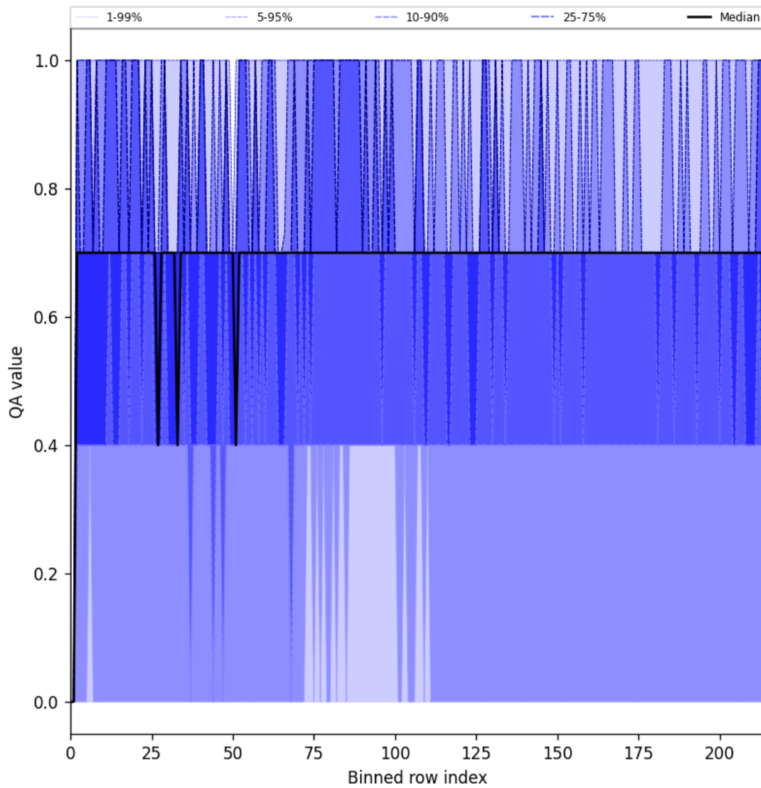
Figure 25: Along track statistics of “QA value” for 2025-08-14 to 2025-08-16
