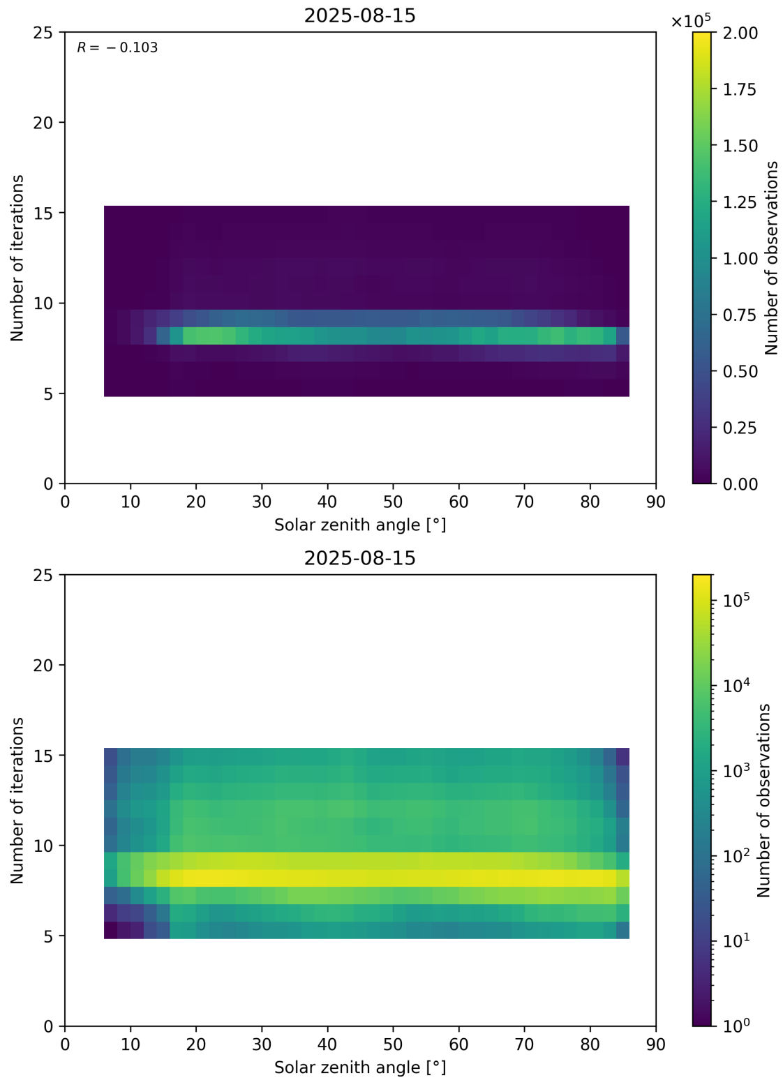
Figure 67: Scatter density plot of “Solar zenith angle” against “Number of iterations” for 2025-08-14 to 2025-08-16.
