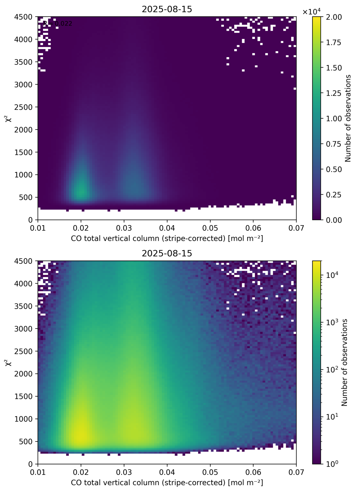
Figure 37: Scatter density plot of “CO total vertical column (stripe-corrected)” against “ \chi^2 ” for 2025-08-14 to 2025-08-16.
