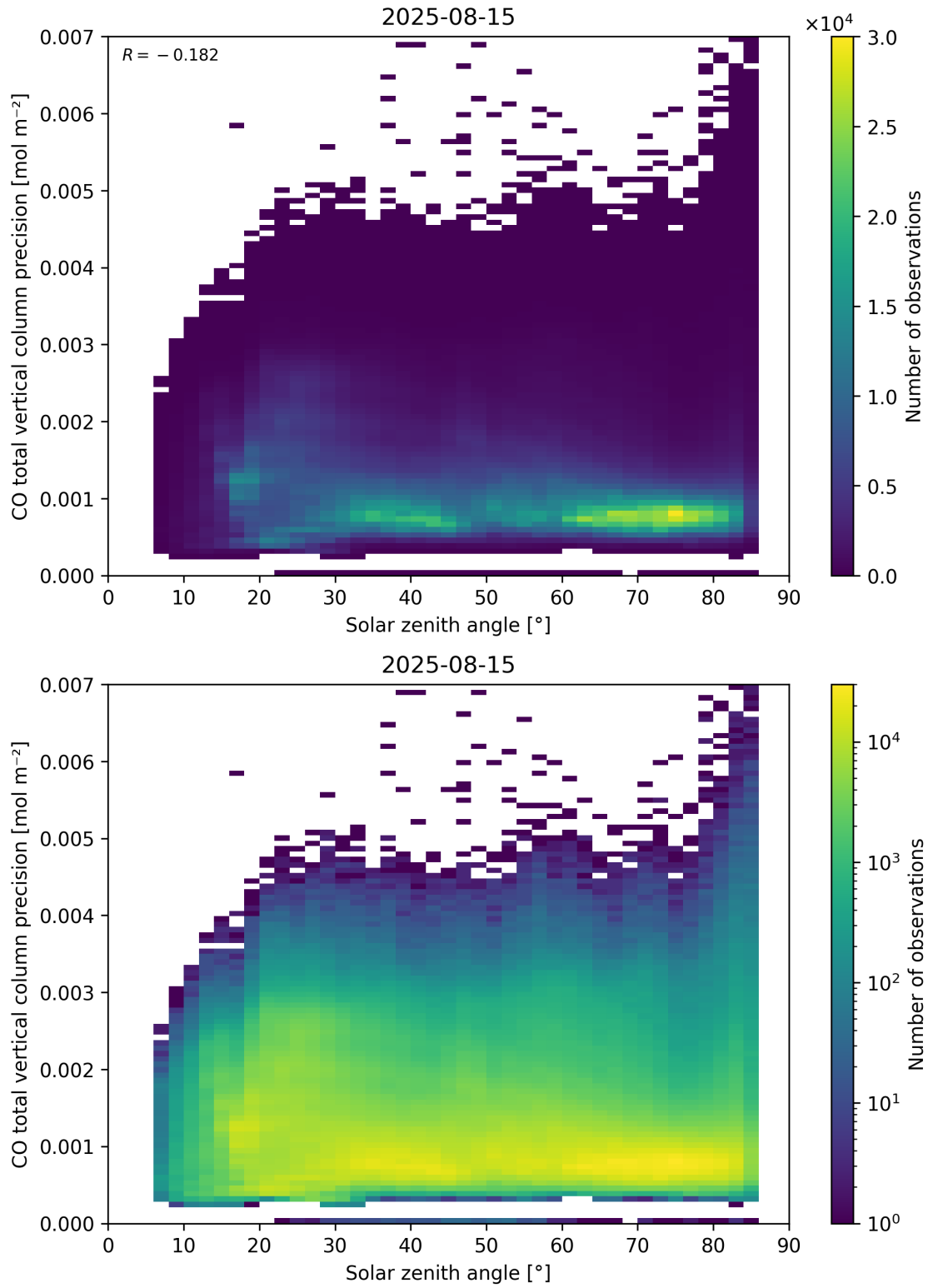
Figure 63: Scatter density plot of “Solar zenith angle” against “CO total vertical column precision” for 2025-08-14 to 2025-08-16.
