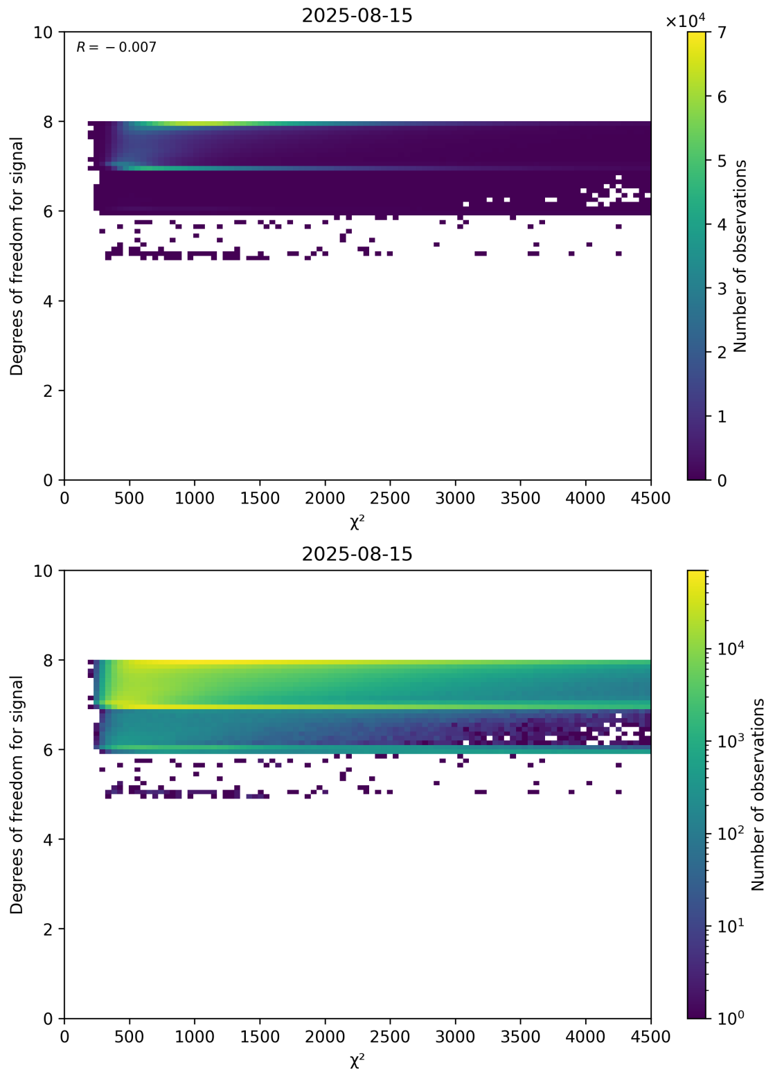
Figure 48: Scatter density plot of " \chi^2 " against "Degrees of freedom for signal" for 2025-08-14 to 2025-08-16.
