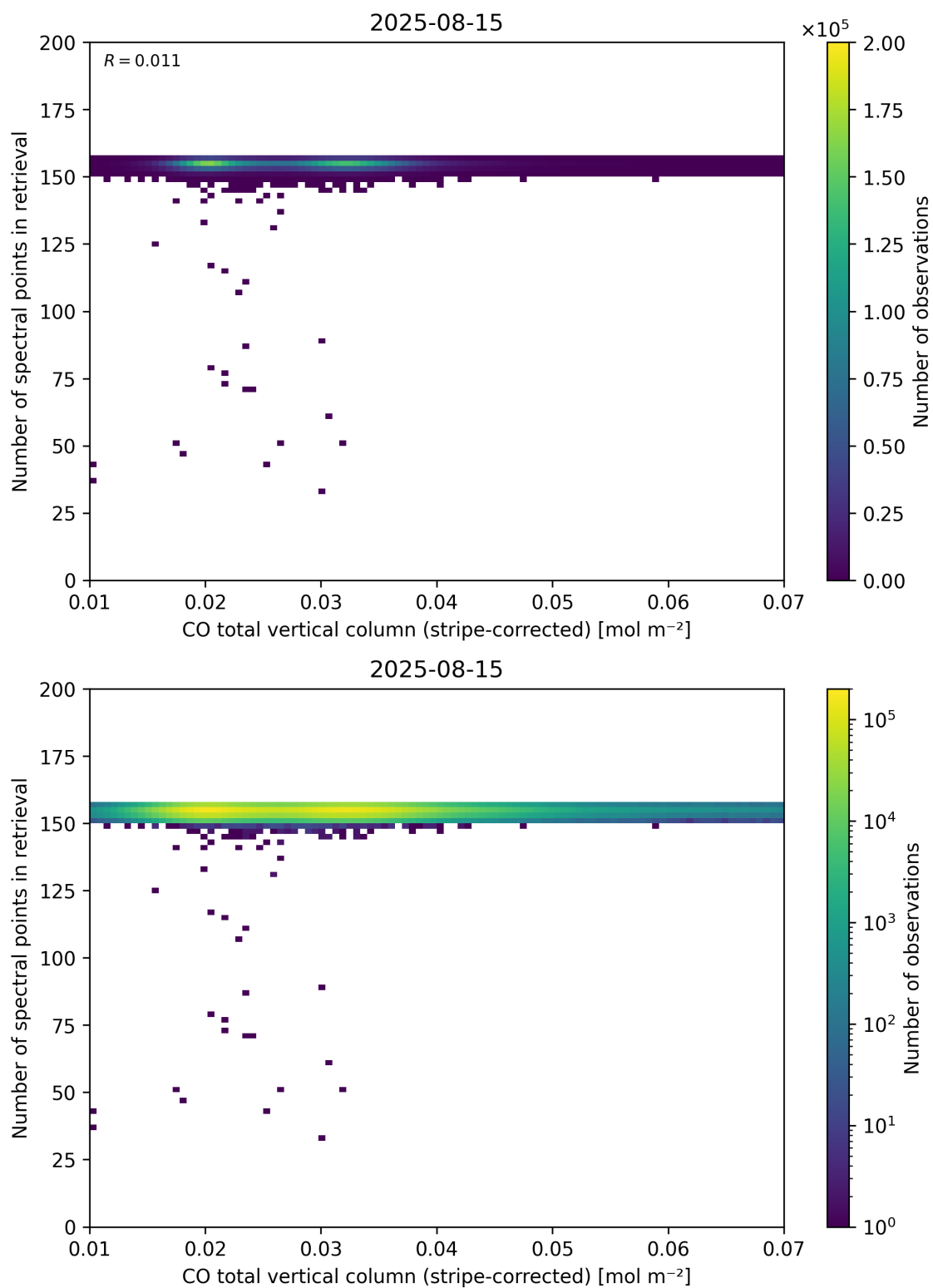
Figure 40: Scatter density plot of “CO total vertical column (stripe-corrected)” against “Number of spectral points in retrieval” for 2025-08-14 to 2025-08-16.
