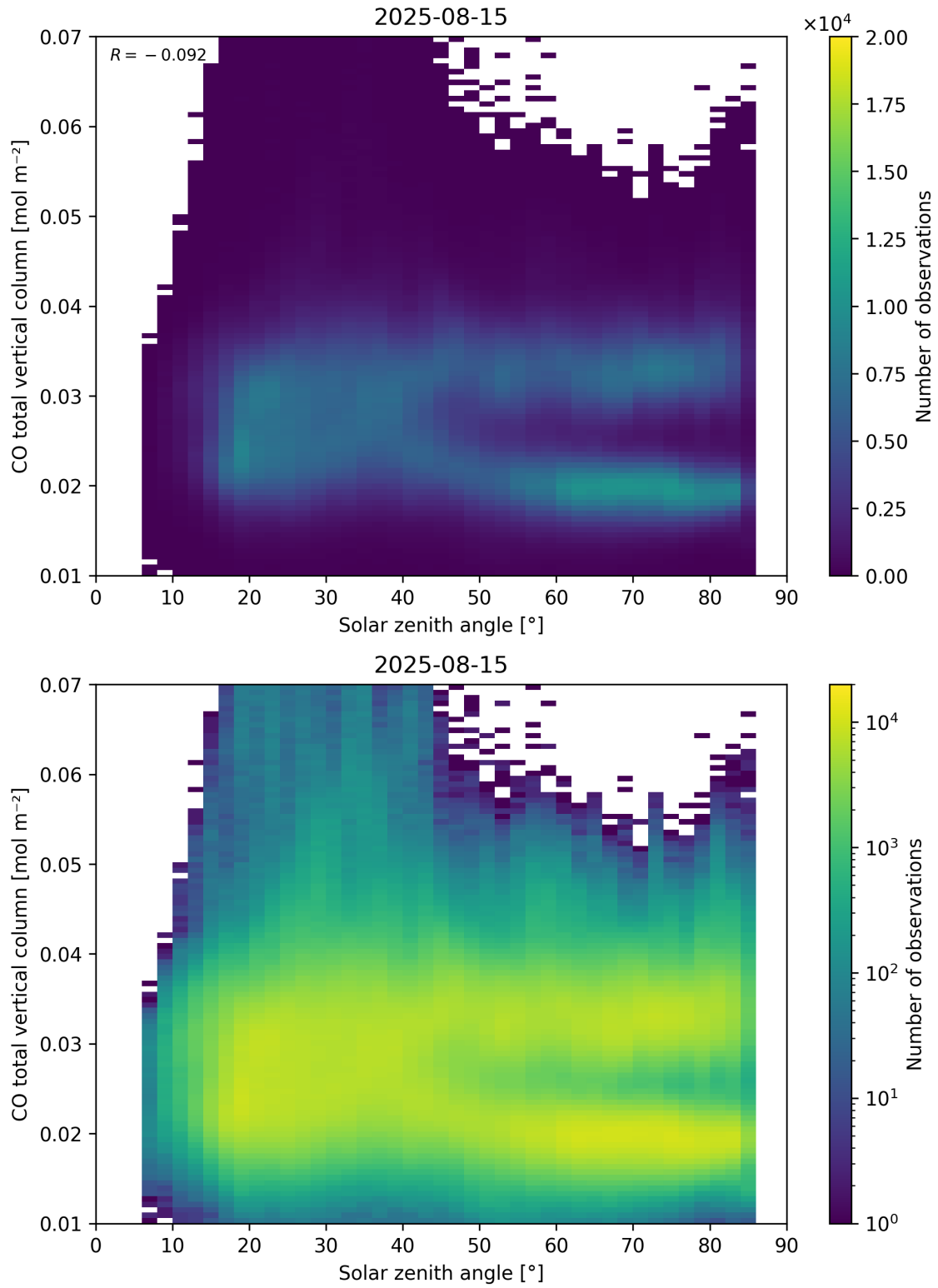
Figure 61: Scatter density plot of “Solar zenith angle” against “CO total vertical column” for 2025-08-14 to 2025-08-16.
