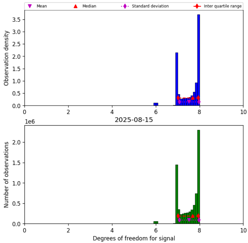
Figure 23: Histogram of “Degrees of freedom for signal” for 2025-08-14 to 2025-08-16
