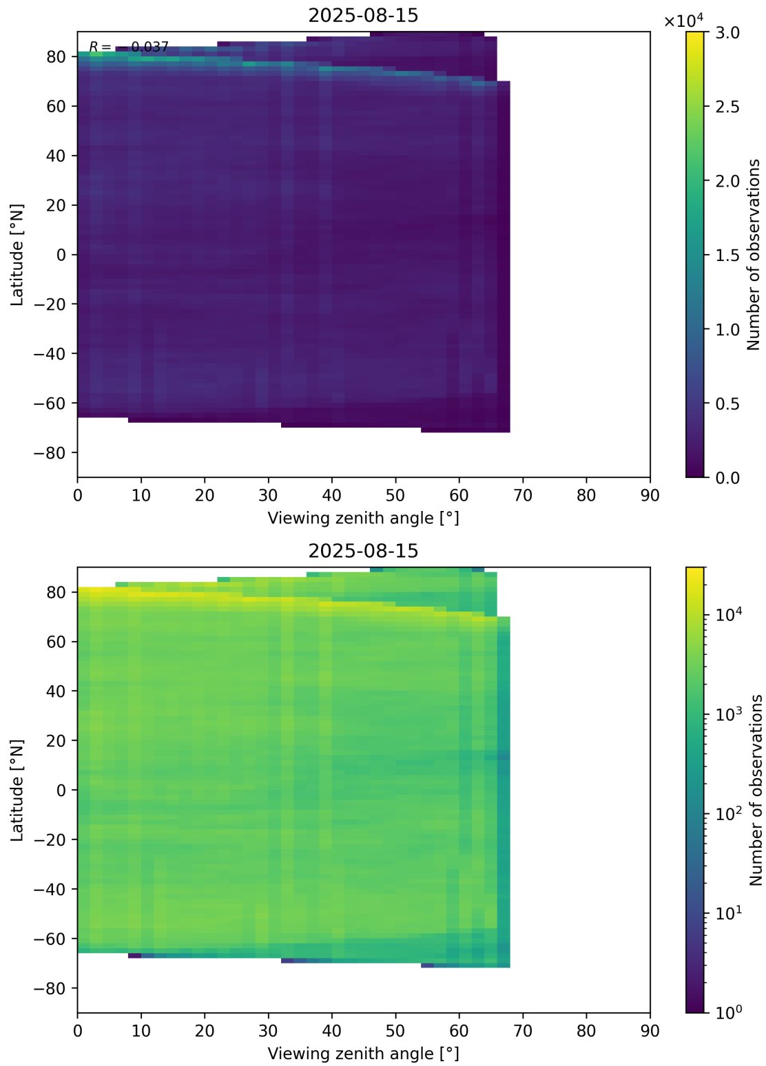
Figure 74: Scatter density plot of “Viewing zenith angle” against “Latitude” for 2025-08-14 to 2025-08-16.
