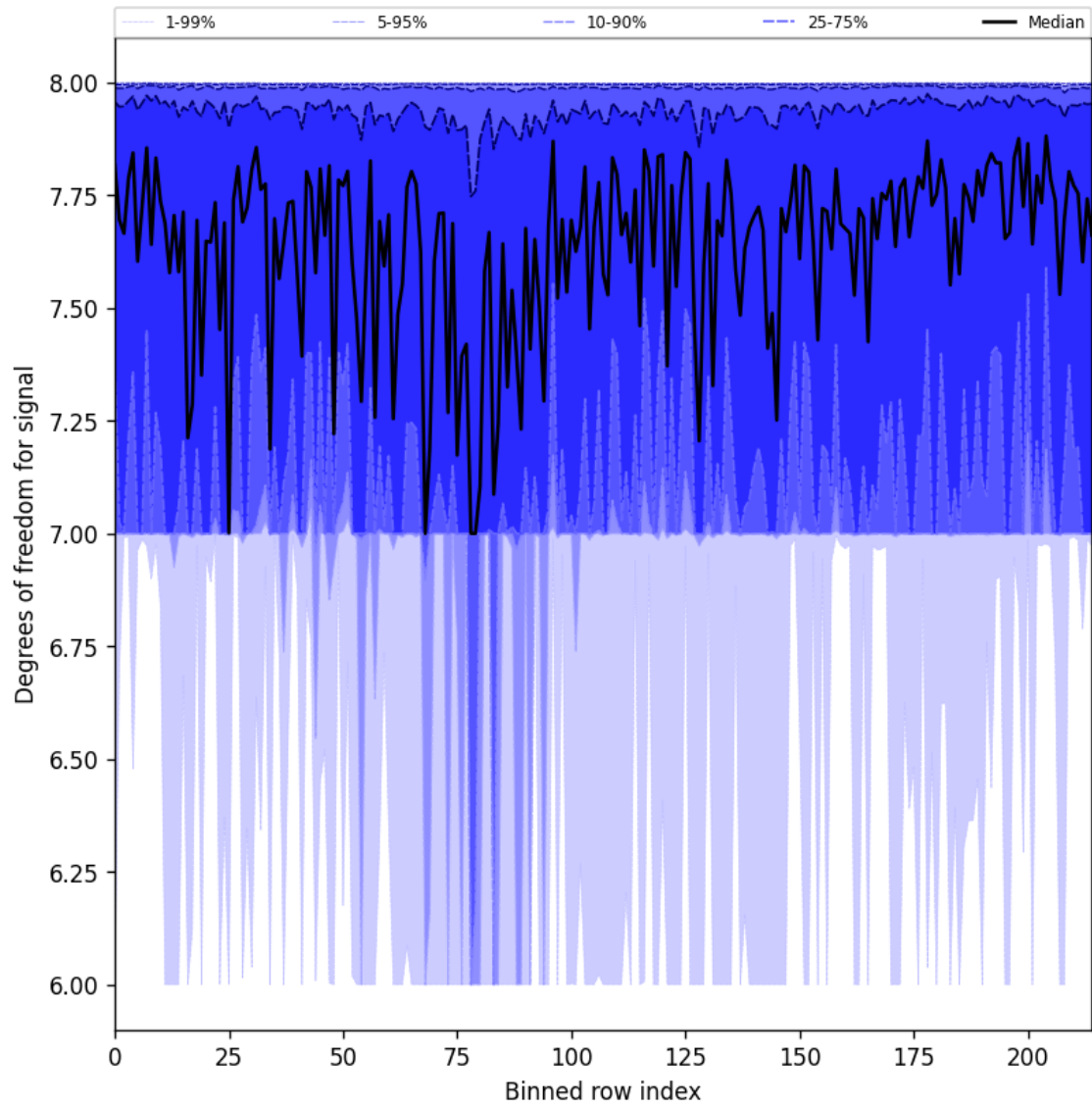
Figure 31: Along track statistics of “Degrees of freedom for signal” for 2025-08-14 to 2025-08-16
