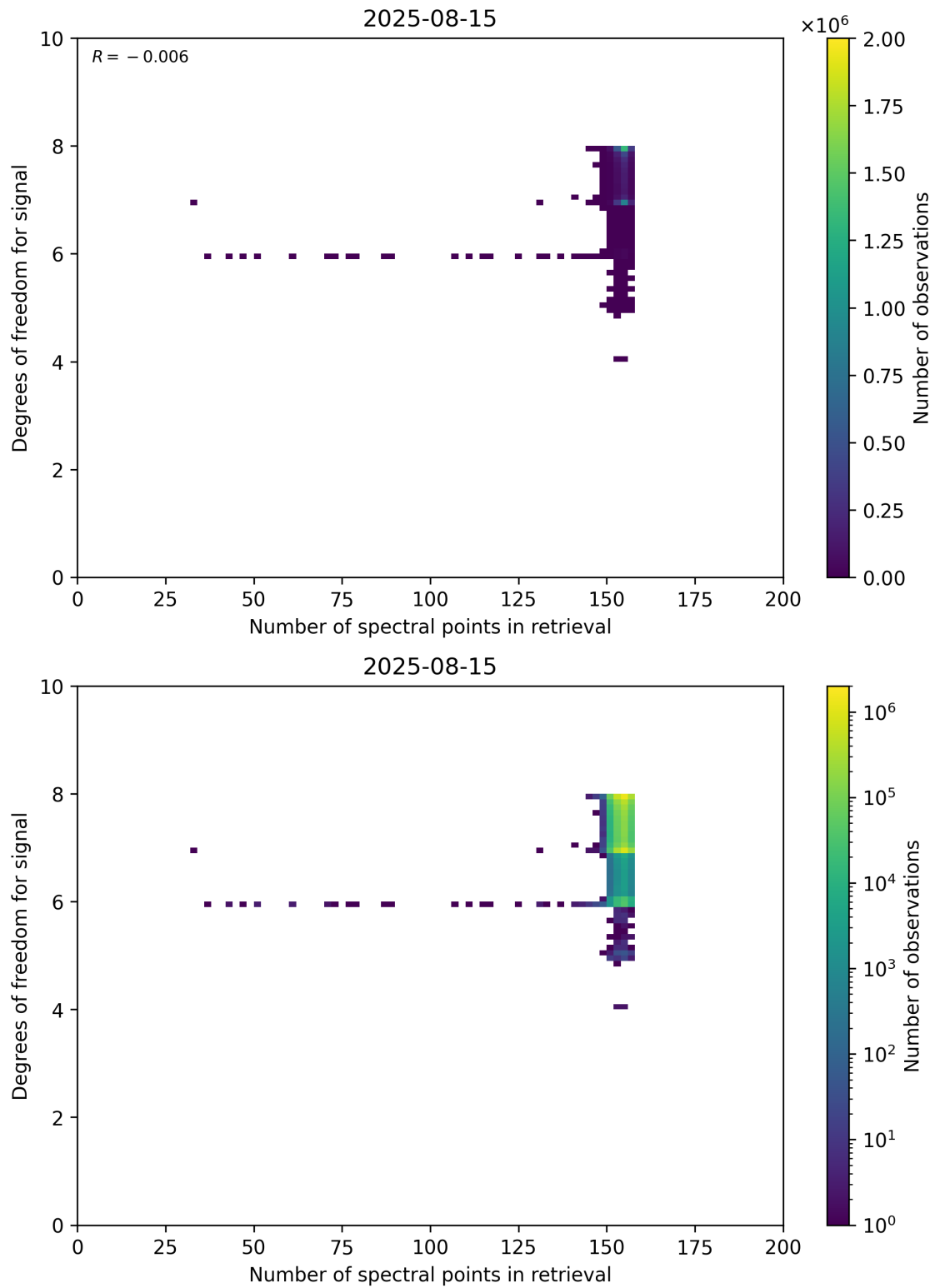
Figure 59: Scatter density plot of “Number of spectral points in retrieval” against “Degrees of freedom for signal” for 2025-08-14 to 2025-08-16.
