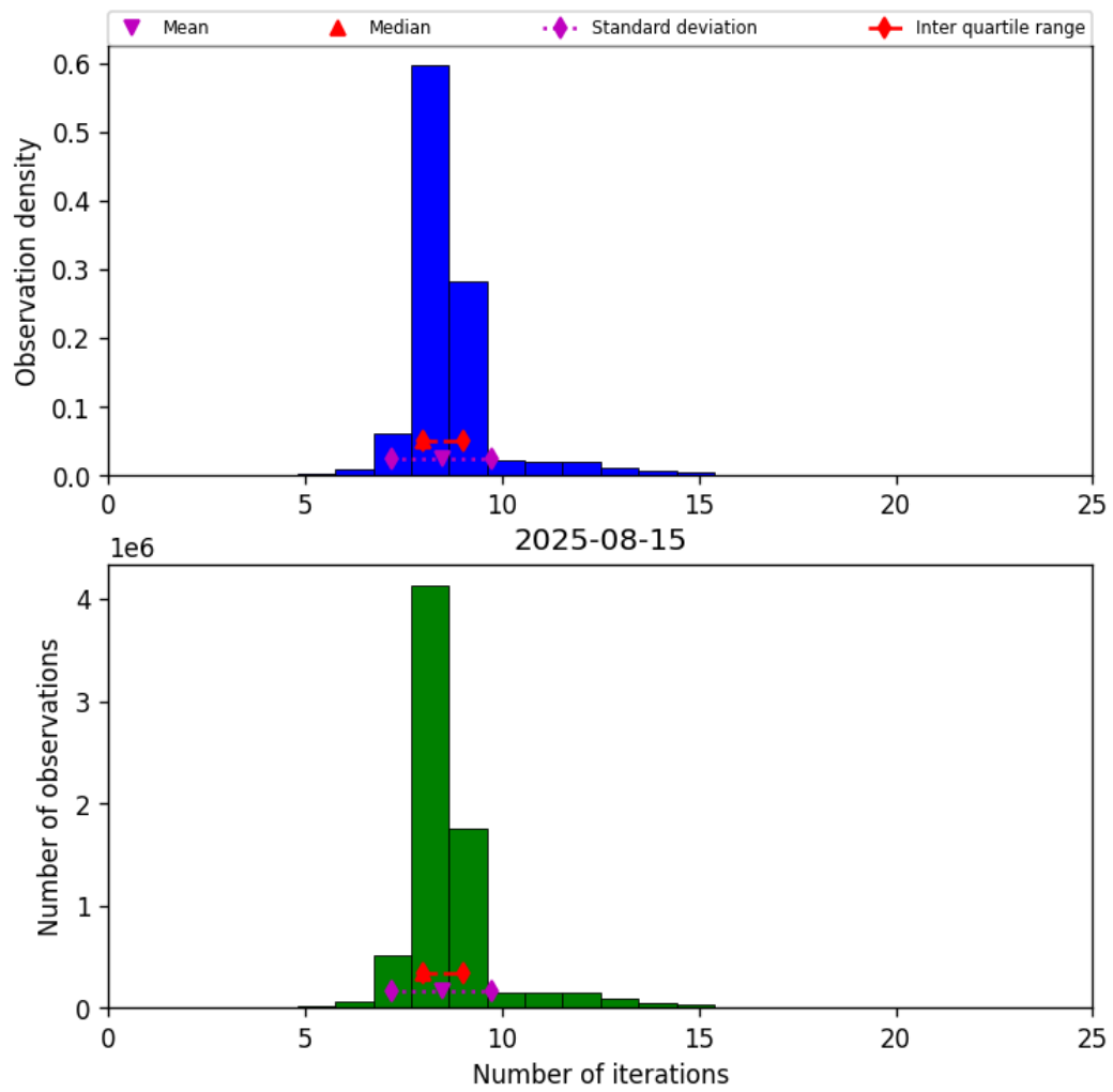
Figure 24: Histogram of “Number of iterations” for 2025-08-14 to 2025-08-16
