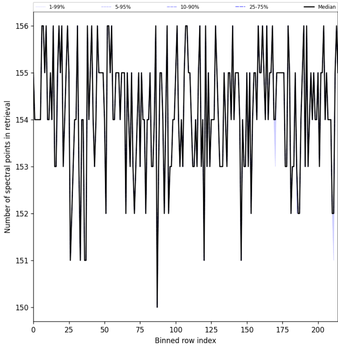
Figure 29: Along track statistics of “Number of spectral points in retrieval” for 2025-08-14 to 2025-08-16
