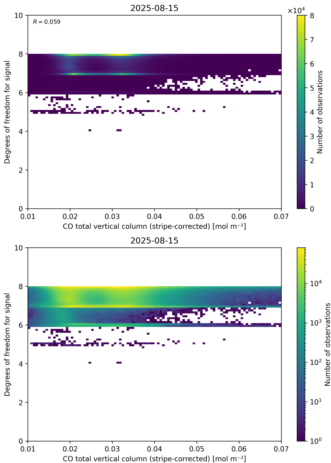
Figure 38: Scatter density plot of “CO total vertical column (stripe-corrected)” against “Degrees of freedom for signal” for 2025-08-14 to 2025-08-16.
