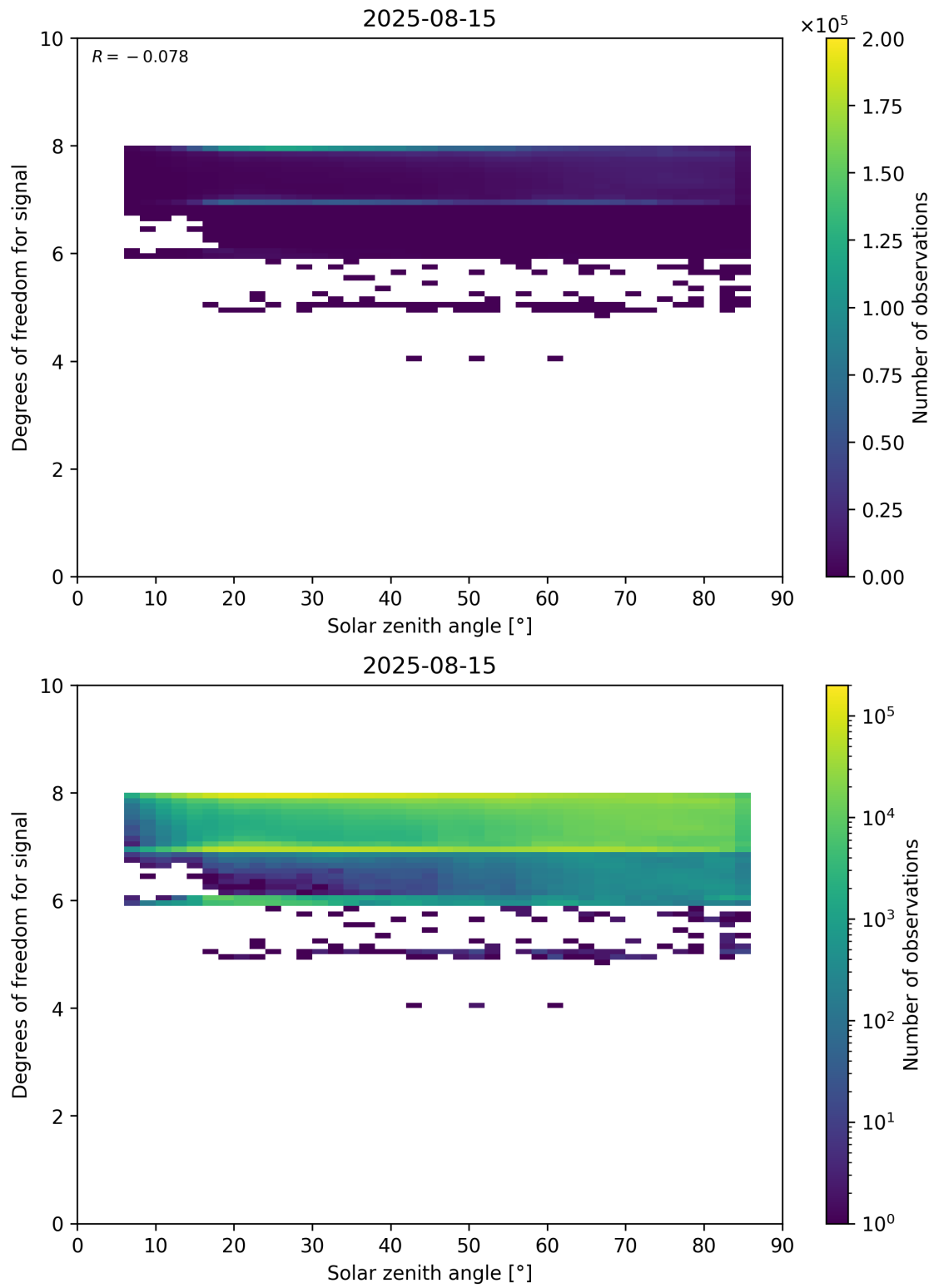
Figure 65: Scatter density plot of “Solar zenith angle” against “Degrees of freedom for signal” for 2025-08-14 to 2025-08-16.
