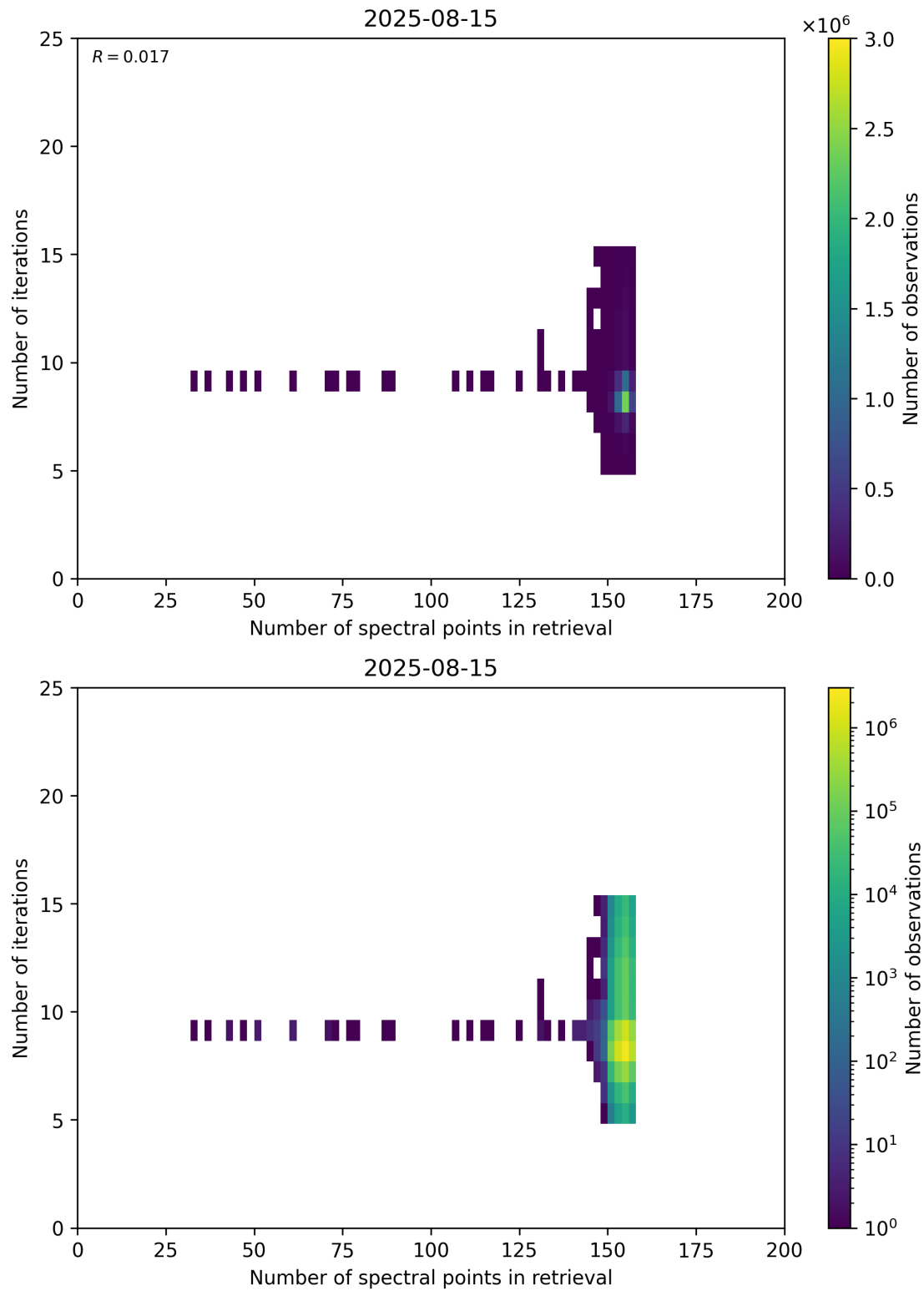
Figure 60: Scatter density plot of “Number of spectral points in retrieval” against “Number of iterations” for 2025-08-14 to 2025-08-16.
