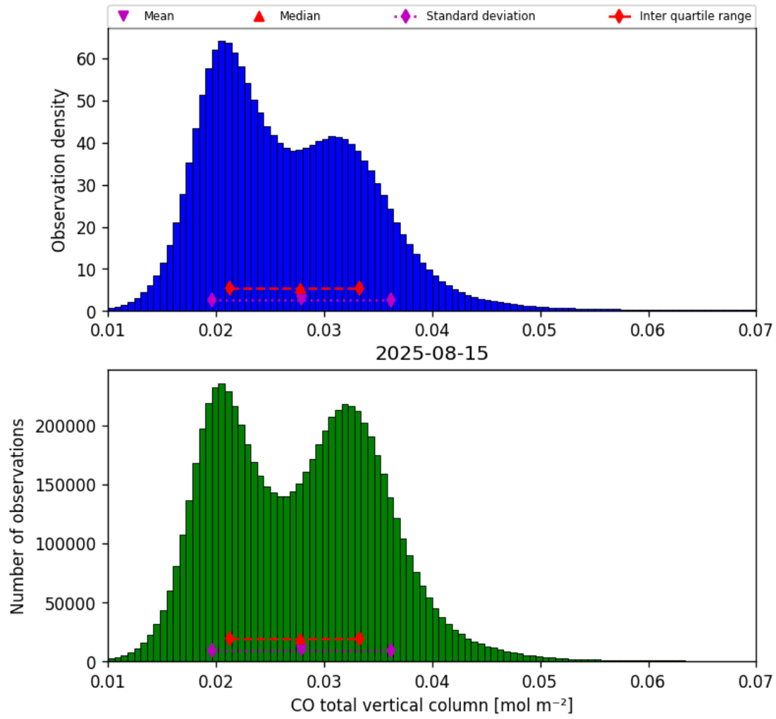
Figure 18: Histogram of “CO total vertical column” for 2025-08-14 to 2025-08-16
