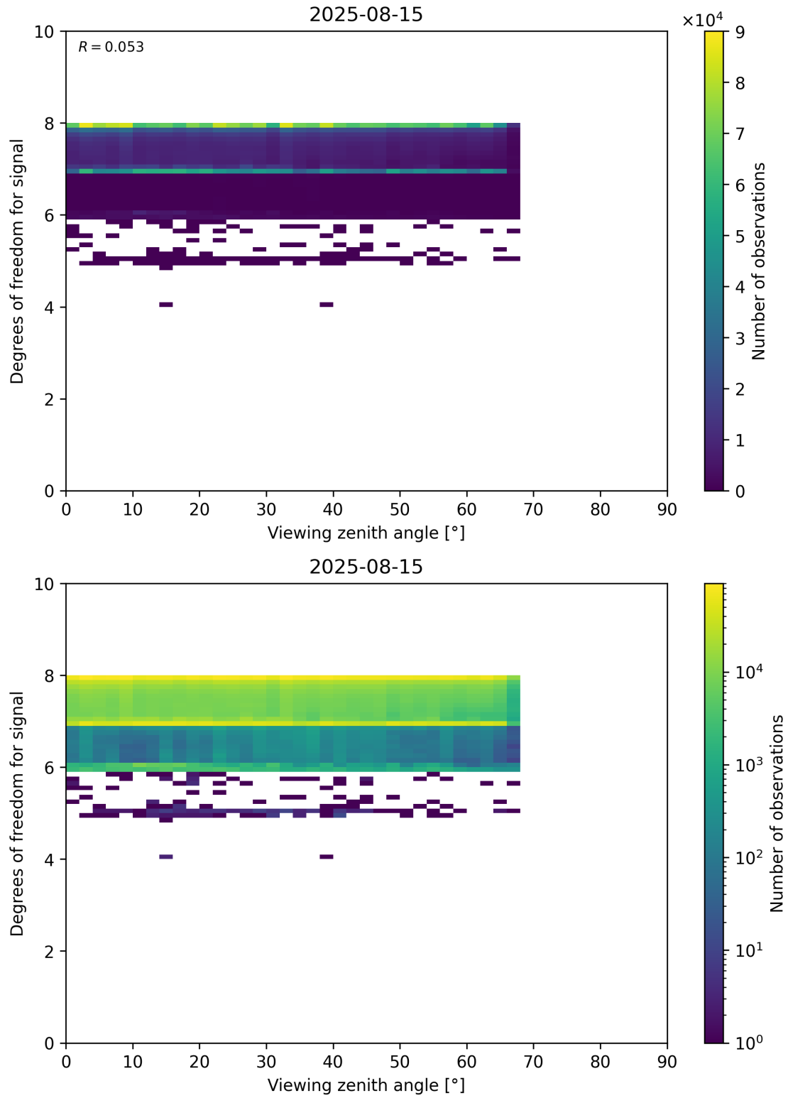
Figure 73: Scatter density plot of “Viewing zenith angle” against “Degrees of freedom for signal” for 2025-08-14 to 2025-08-16.
