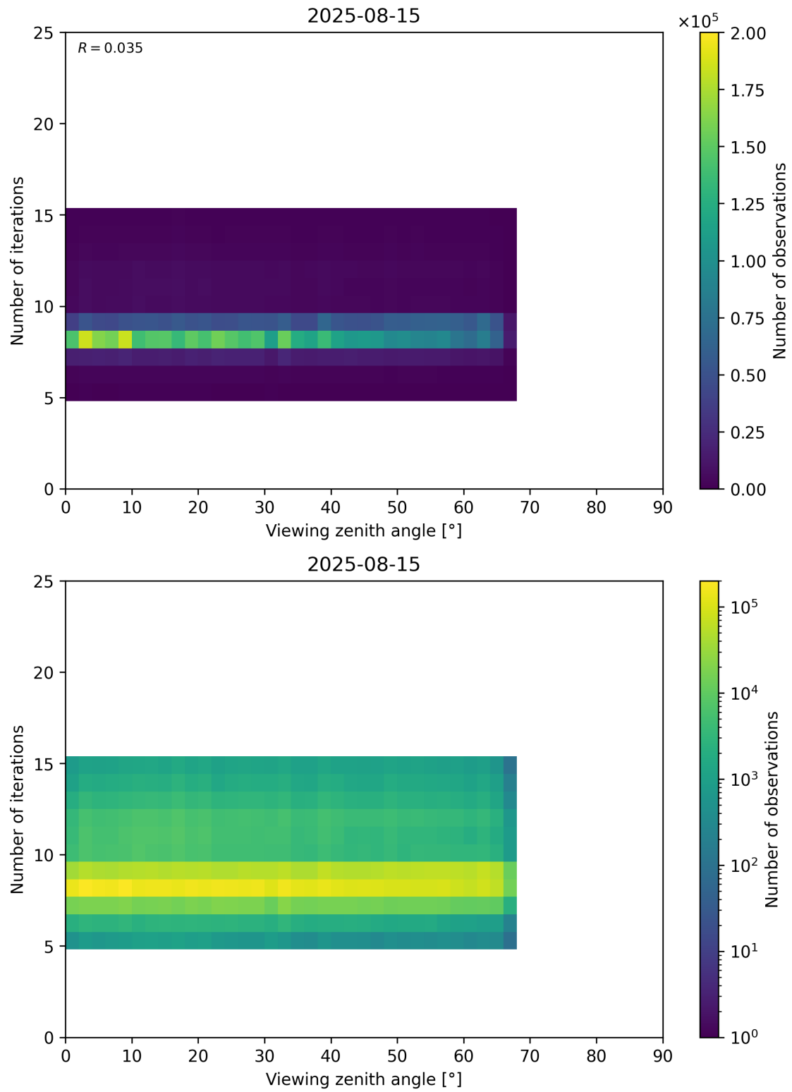
Figure 75: Scatter density plot of “Viewing zenith angle” against “Number of iterations” for 2025-08-14 to 2025-08-16.
