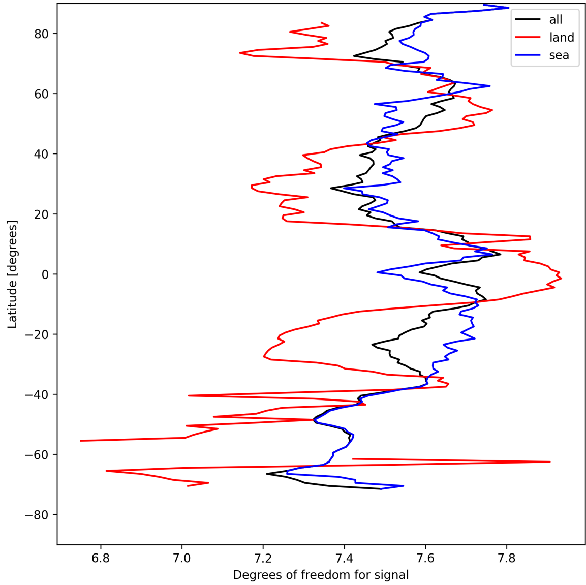
Figure 15: Zonal average of “Degrees of freedom for signal” for 2025-08-14 to 2025-08-16.
