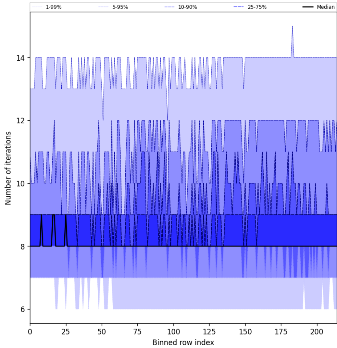
Figure 32: Along track statistics of “Number of iterations” for 2025-08-14 to 2025-08-16
