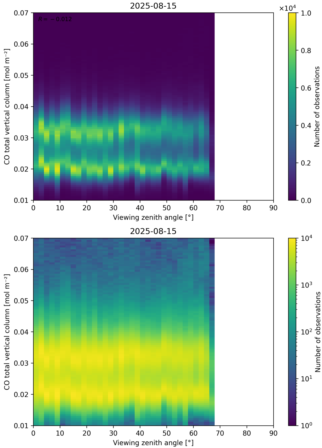
Figure 69: Scatter density plot of “Viewing zenith angle” against “CO total vertical column” for 2025-08-14 to 2025-08-16.
