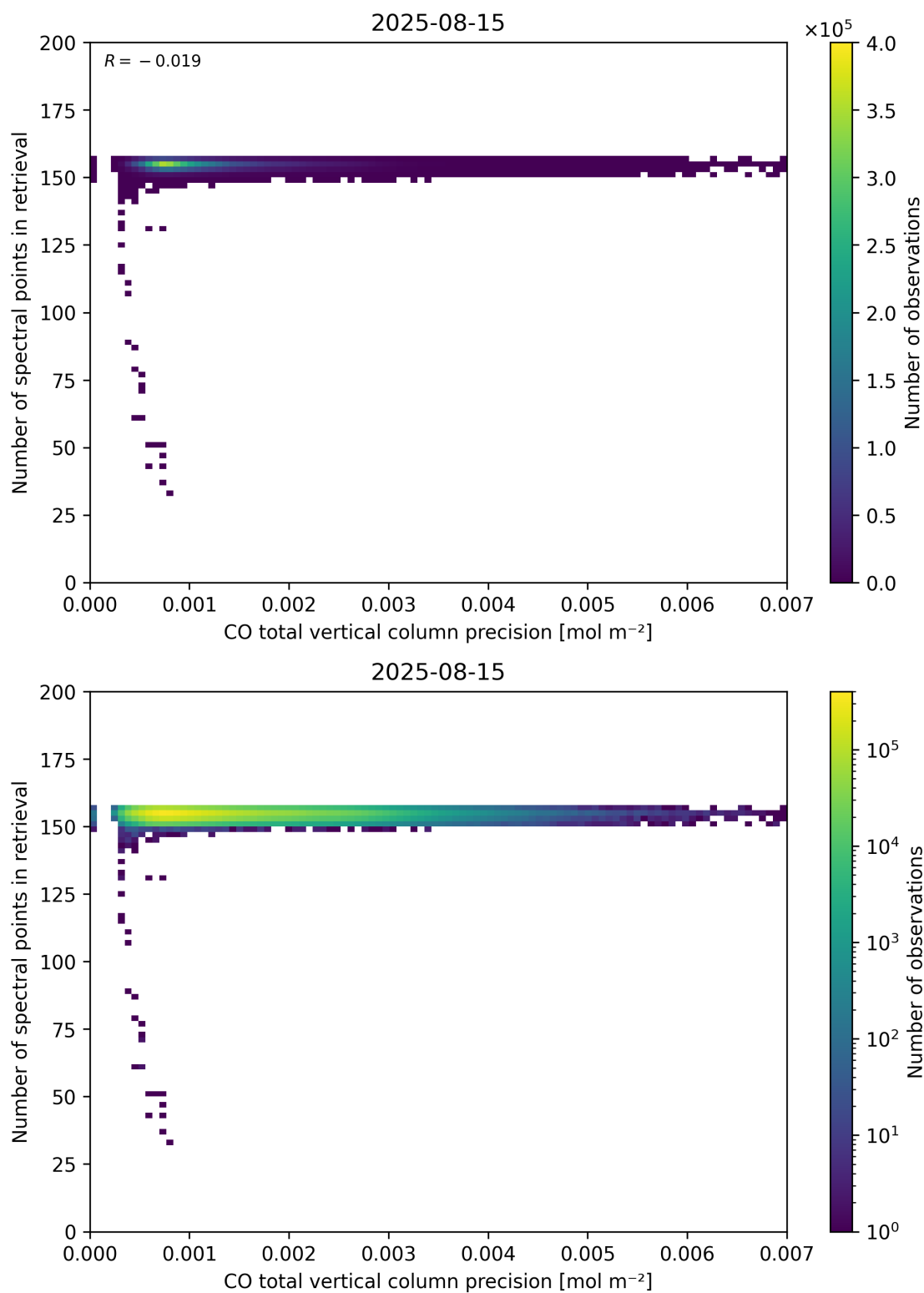
Figure 47: Scatter density plot of “CO total vertical column precision” against “Number of spectral points in retrieval” for 2025-08-14 to 2025-08-16.
