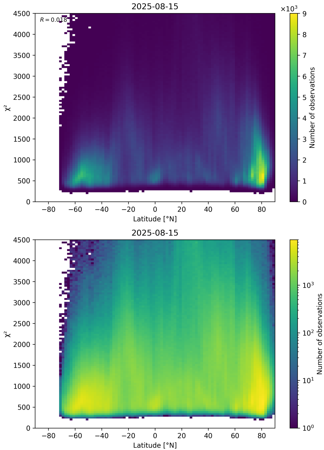
Figure 54: Scatter density plot of “Latitude” against “ \chi^2 ” for 2025-08-14 to 2025-08-16.
