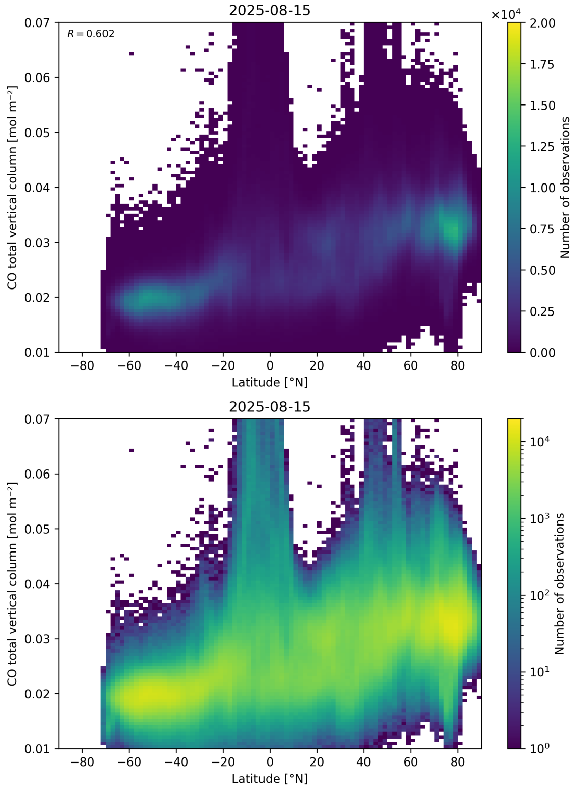
Figure 51: Scatter density plot of “Latitude” against “CO total vertical column” for 2025-08-14 to 2025-08-16.
