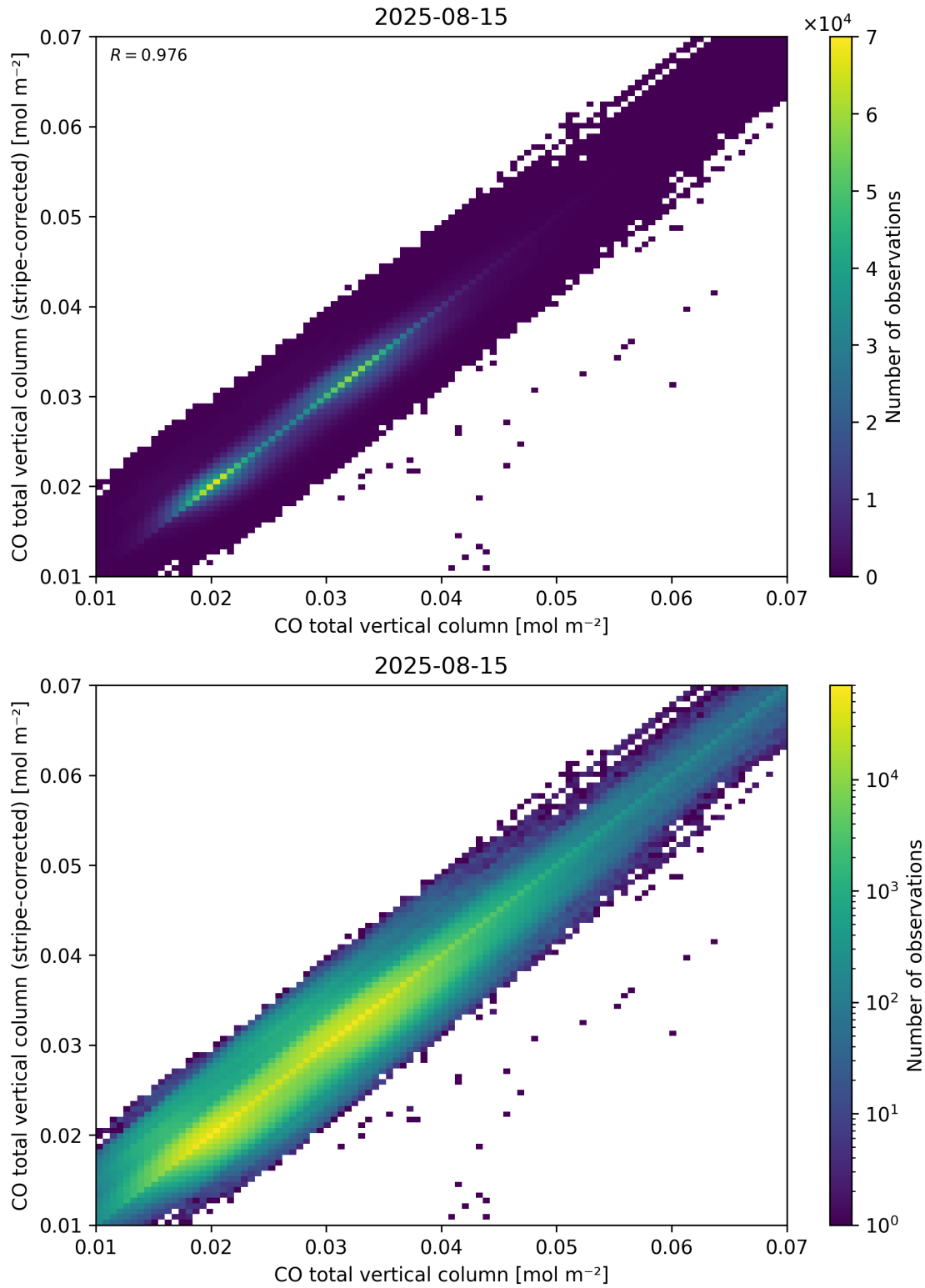
Figure 33: Scatter density plot of “CO total vertical column” against “CO total vertical column (stripe-corrected)” for 2025-08-14 to 2025-08-16.
