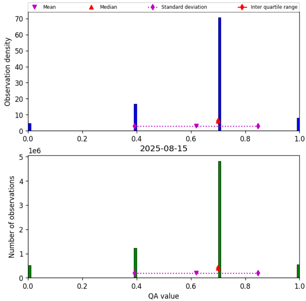
Figure 17: Histogram of “QA value” for 2025-08-14 to 2025-08-16
