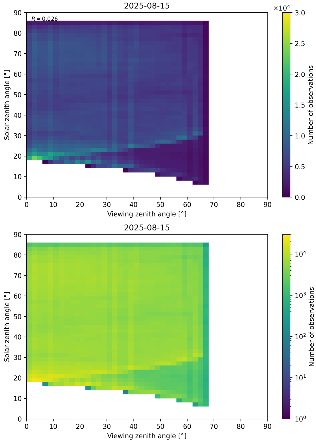
Figure 77: Scatter density plot of “Viewing zenith angle” against “Solar zenith angle” for 2025-08-14 to 2025-08-16.
