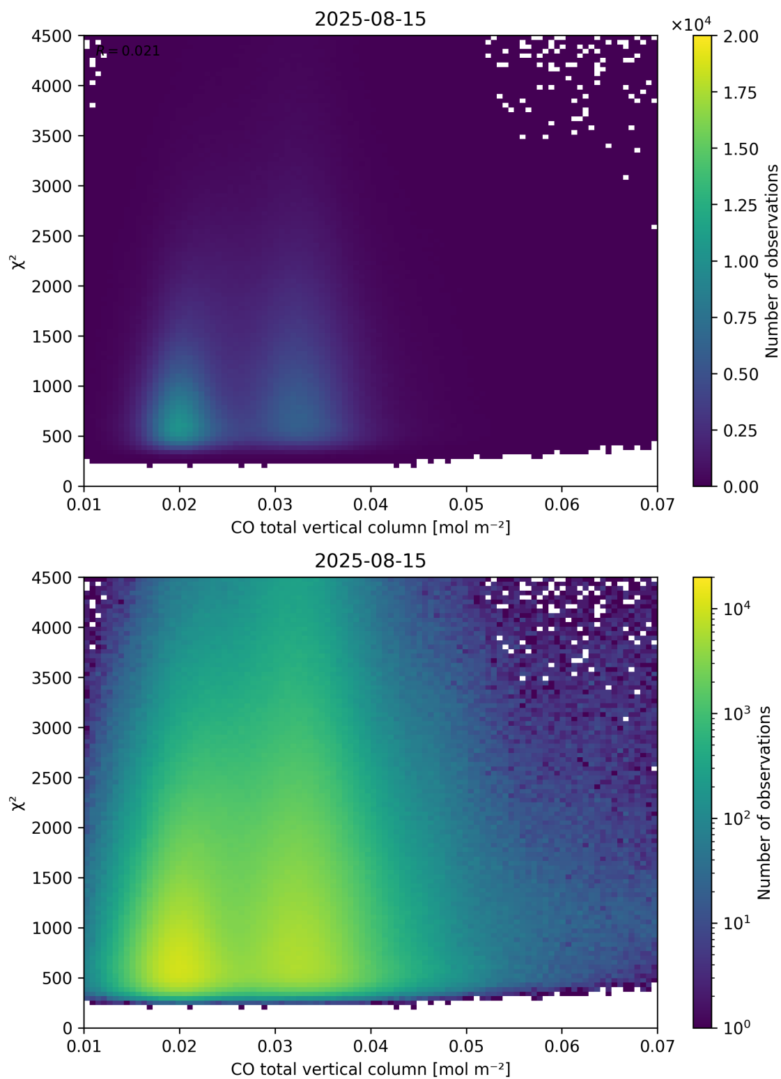
Figure 35: Scatter density plot of “CO total vertical column” against “ \chi^2 ” for 2025-08-14 to 2025-08-16.
