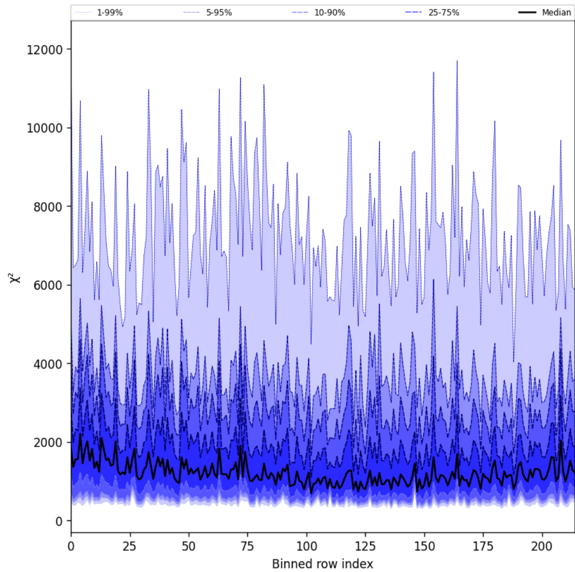
Figure 30: Along track statistics of “ \chi^2 ” for 2025-08-14 to 2025-08-16
