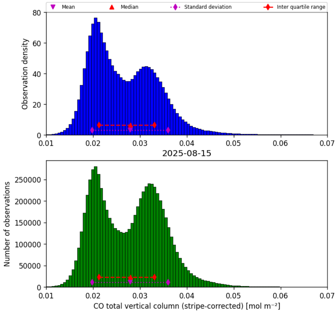
Figure 19: Histogram of “CO total vertical column (stripe-corrected)” for 2025-08-14 to 2025-08-16
