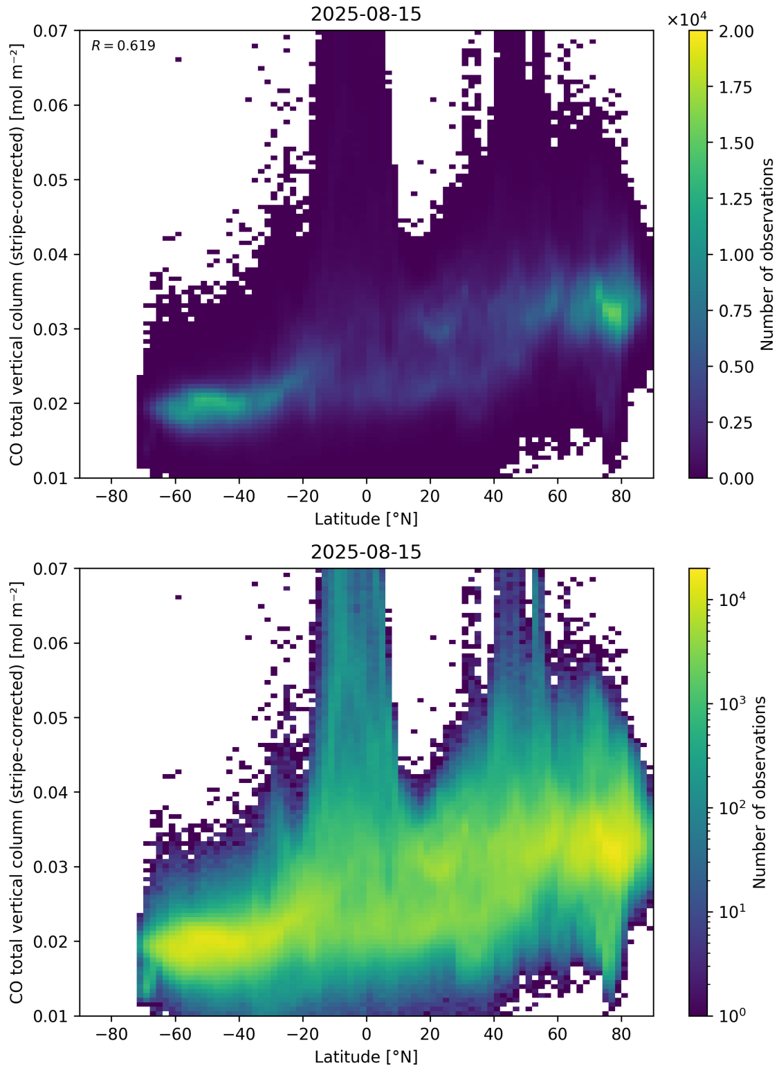
Figure 52: Scatter density plot of “Latitude” against “CO total vertical column (stripe-corrected)” for 2025-08-14 to 2025-08-16.
