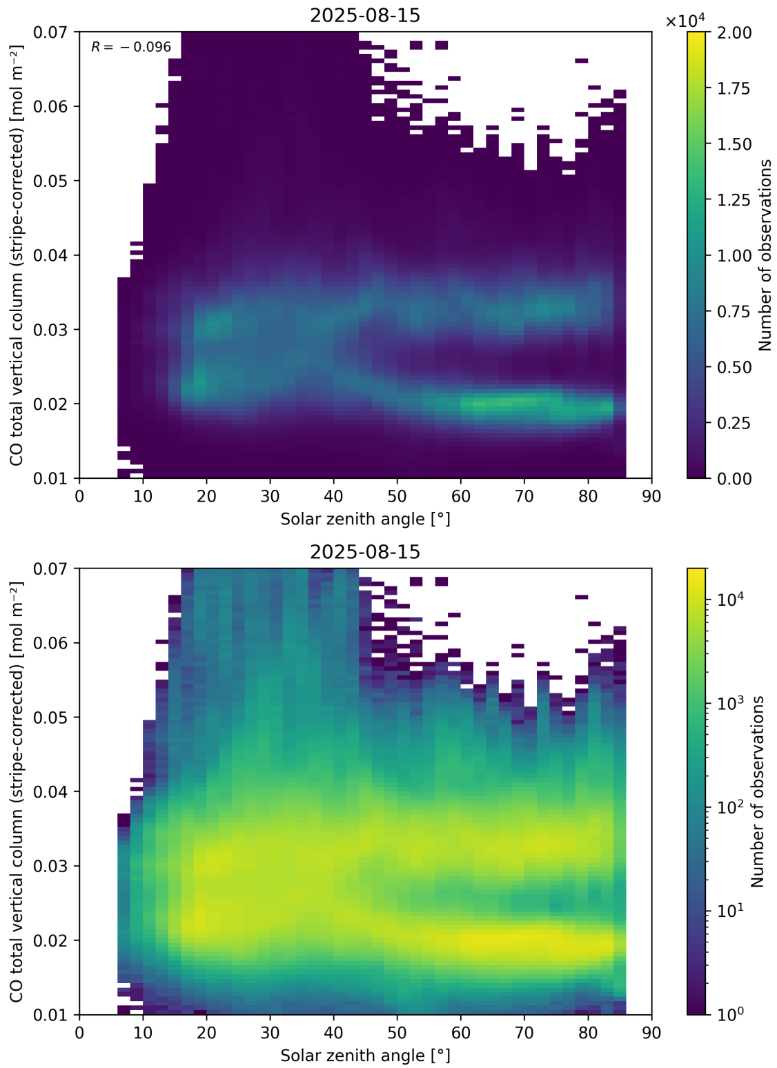
Figure 62: Scatter density plot of “Solar zenith angle” against “CO total vertical column (stripe-corrected)” for 2025-08-14 to 2025-08-16.
