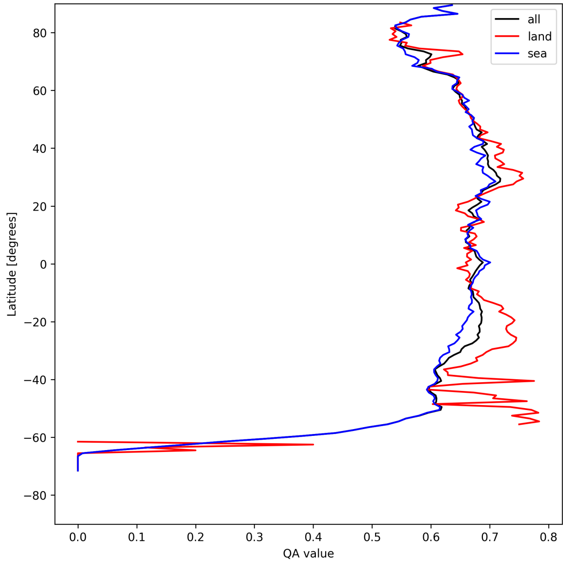
Figure 9: Zonal average of “QA value” for 2025-08-14 to 2025-08-16.
