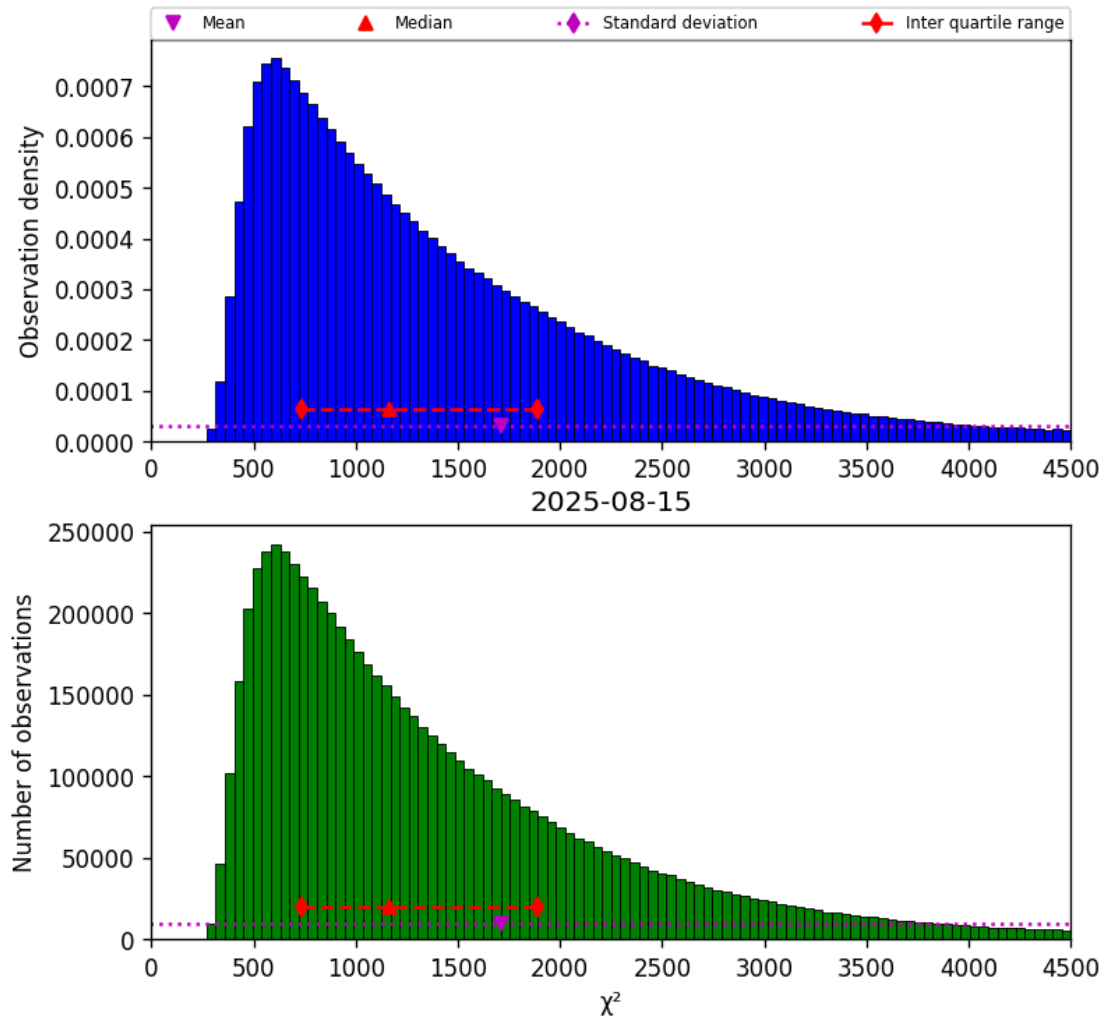
Figure 22: Histogram of “ \chi^2 ” for 2025-08-14 to 2025-08-16
