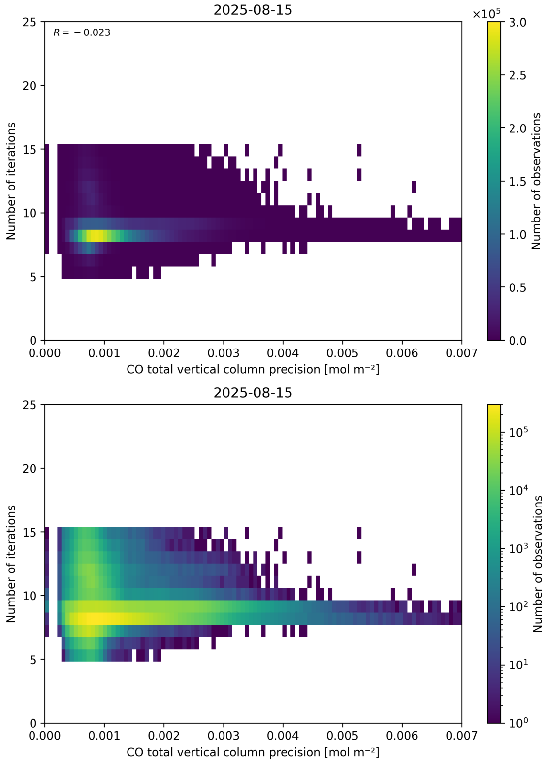
Figure 46: Scatter density plot of “CO total vertical column precision” against “Number of iterations” for 2025-08-14 to 2025-08-16.
