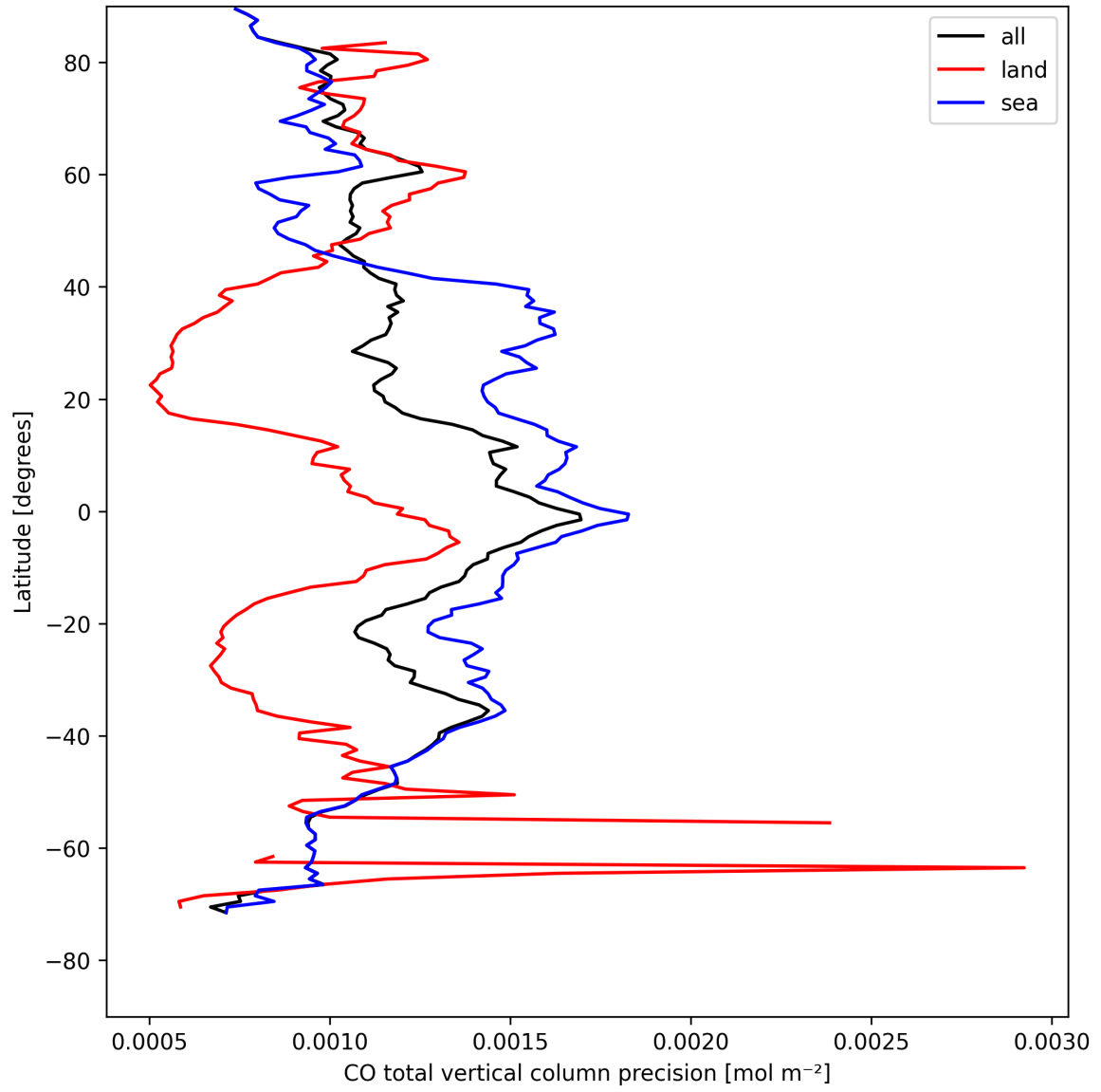
Figure 12: Zonal average of “CO total vertical column precision” for 2025-08-14 to 2025-08-16.
