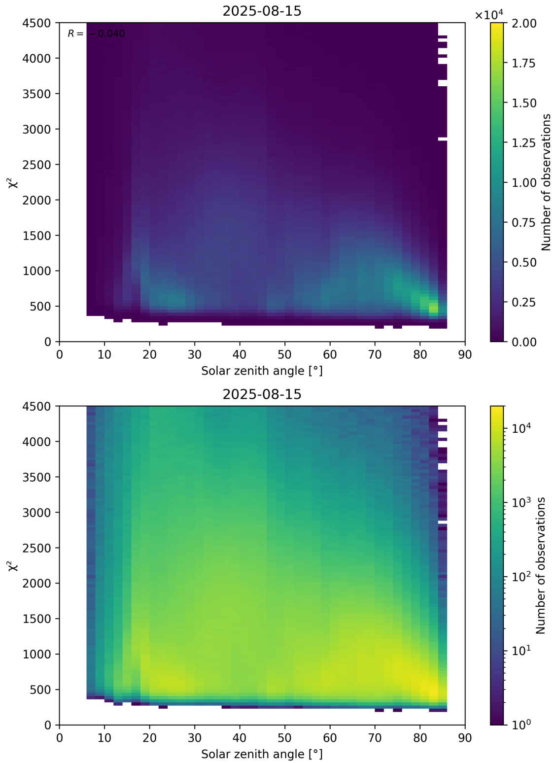
Figure 64: Scatter density plot of “Solar zenith angle” against “ \chi^2 ” for 2025-08-14 to 2025-08-16.
