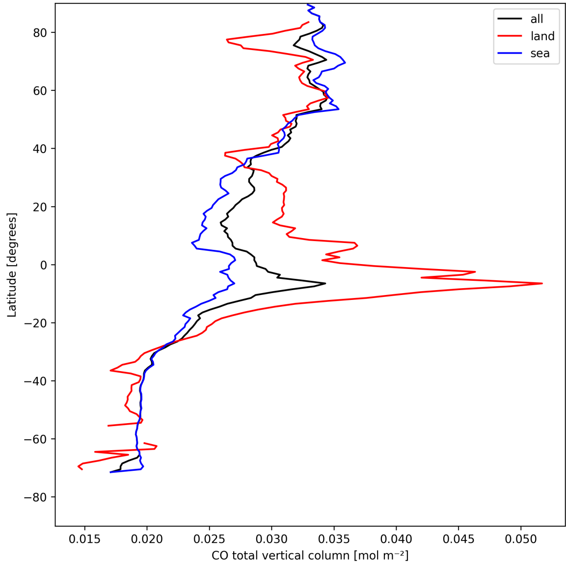
Figure 10: Zonal average of “CO total vertical column” for 2025-08-14 to 2025-08-16.
