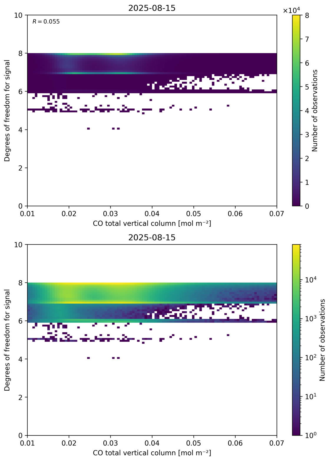
Figure 41: Scatter density plot of “CO total vertical column” against “Degrees of freedom for signal” for 2025-08-14 to 2025-08-16.
