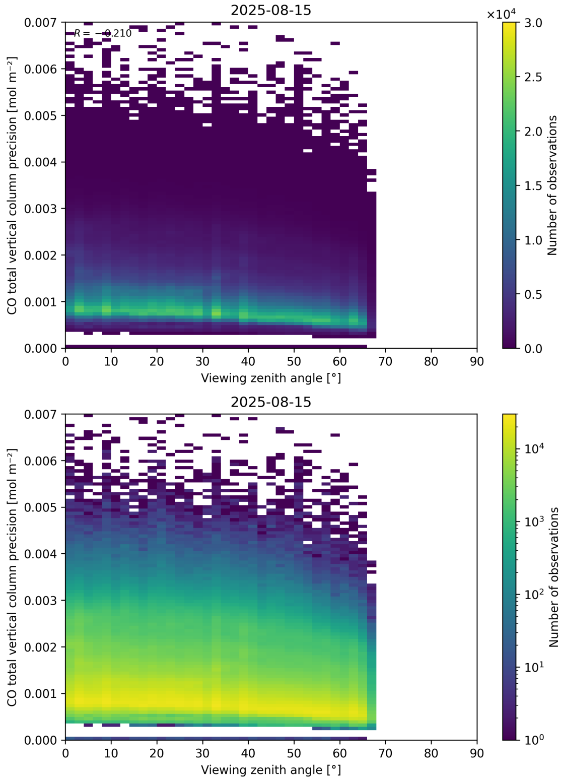
Figure 71: Scatter density plot of “Viewing zenith angle” against “CO total vertical column precision” for 2025-08-14 to 2025-08-16.
