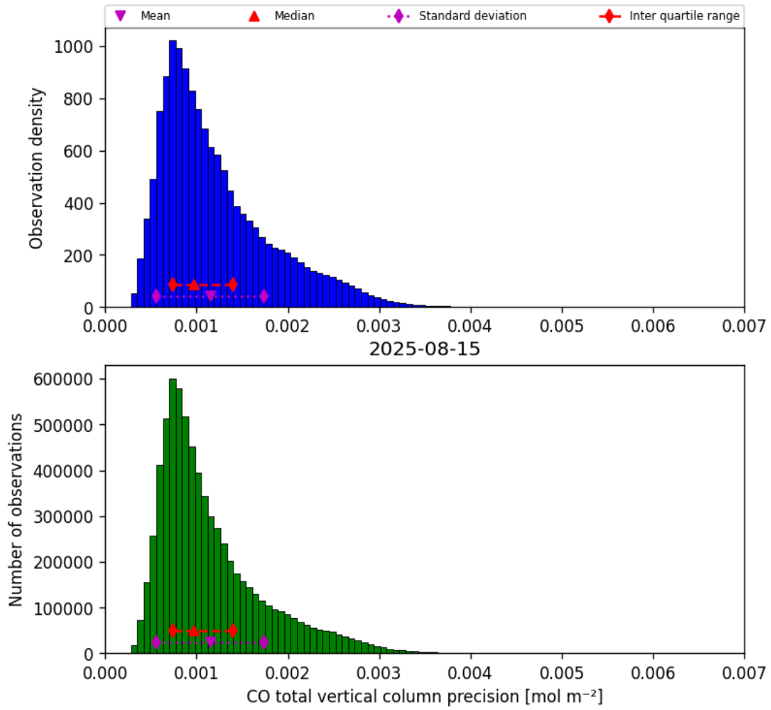
Figure 20: Histogram of “CO total vertical column precision” for 2025-08-14 to 2025-08-16
