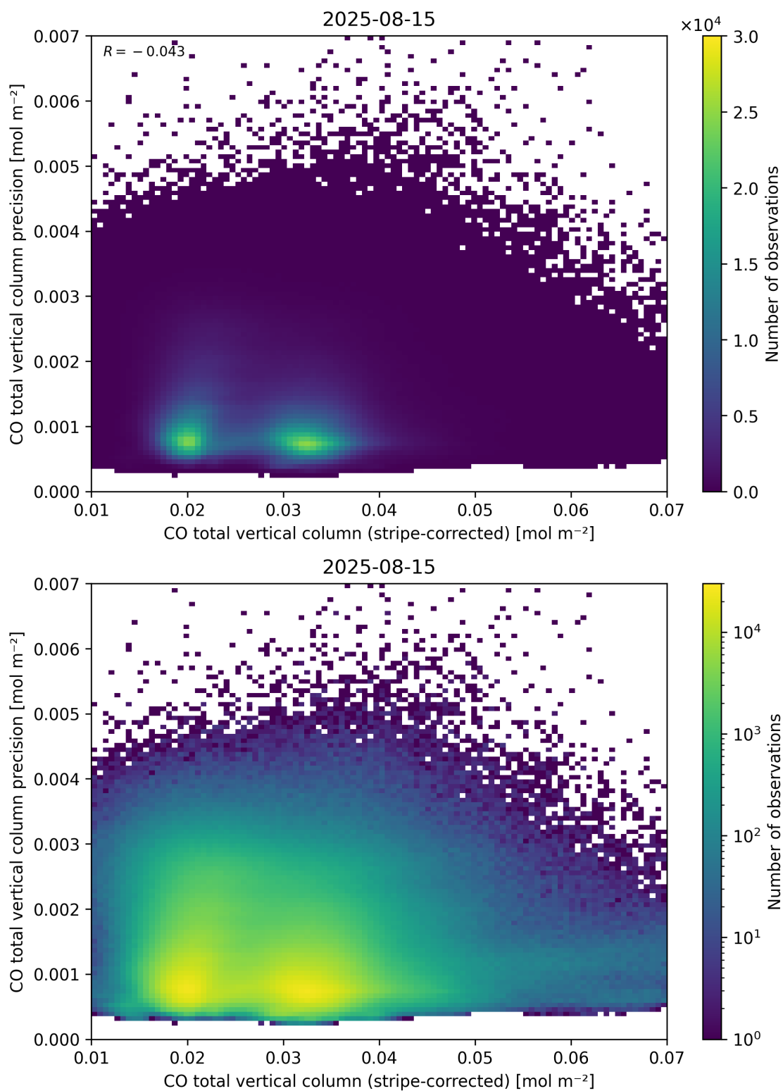
Figure 36: Scatter density plot of “CO total vertical column (stripe-corrected)” against “CO total vertical column precision” for 2025-08-14 to 2025-08-16.
