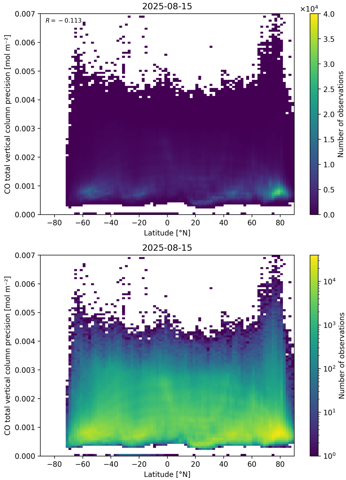
Figure 53: Scatter density plot of “Latitude” against “CO total vertical column precision” for 2025-08-14 to 2025-08-16.
