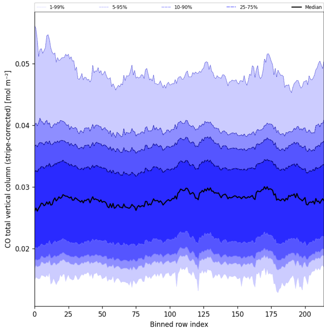
Figure 27: Along track statistics of “CO total vertical column (stripe-corrected)” for 2025-08-14 to 2025-08-16
