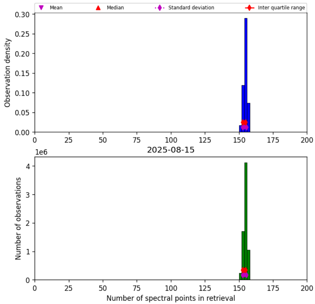
Figure 21: Histogram of “Number of spectral points in retrieval” for 2025-08-14 to 2025-08-16
