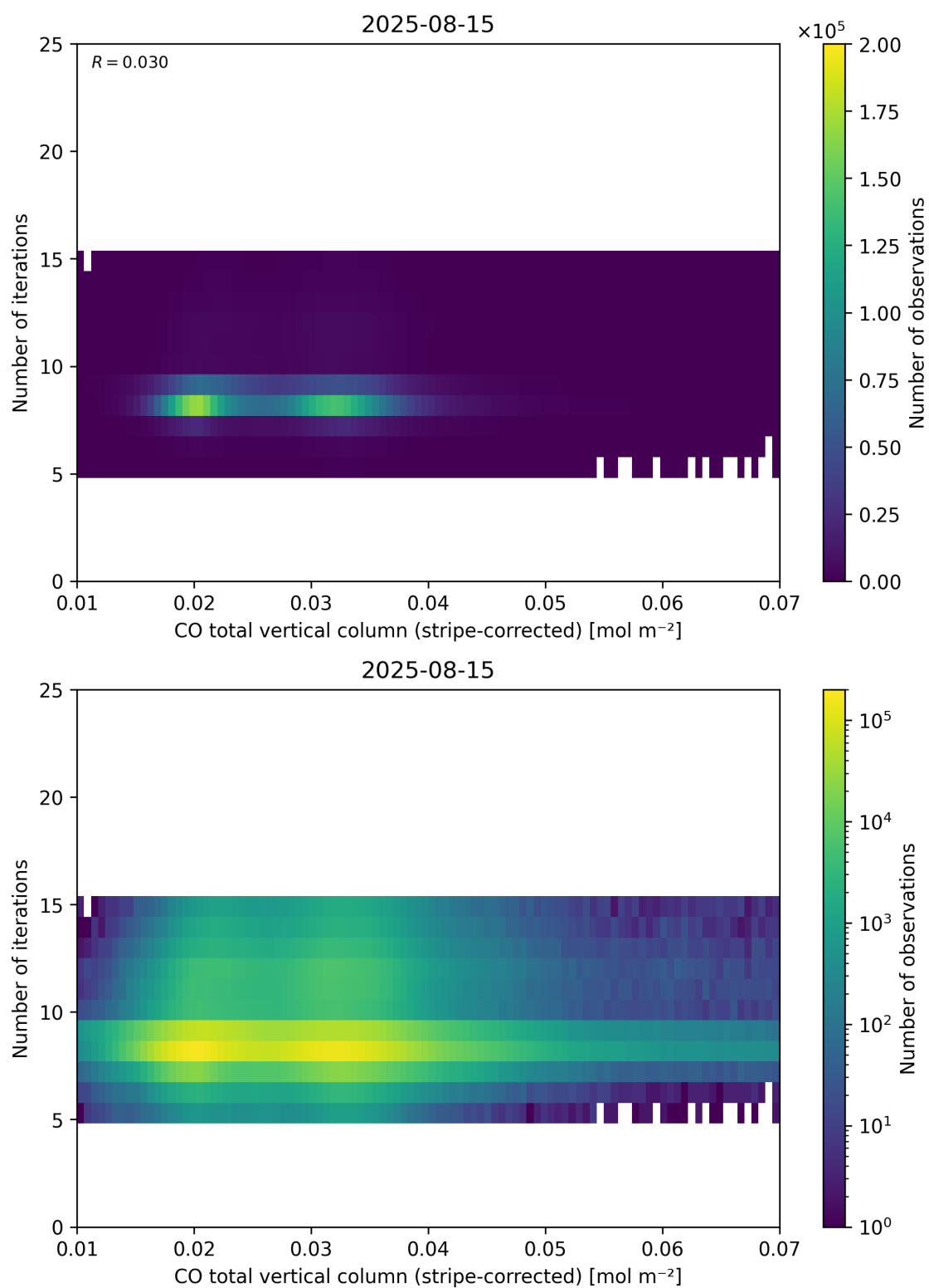
Figure 39: Scatter density plot of “CO total vertical column (stripe-corrected)” against “Number of iterations” for 2025-08-14 to 2025-08-16.
