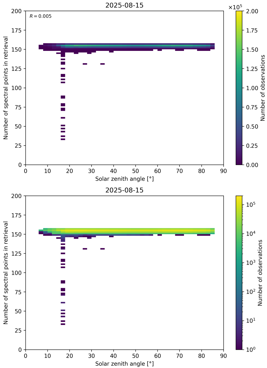
Figure 68: Scatter density plot of “Solar zenith angle” against “Number of spectral points in retrieval” for 2025-08-14 to 2025-08-16.
