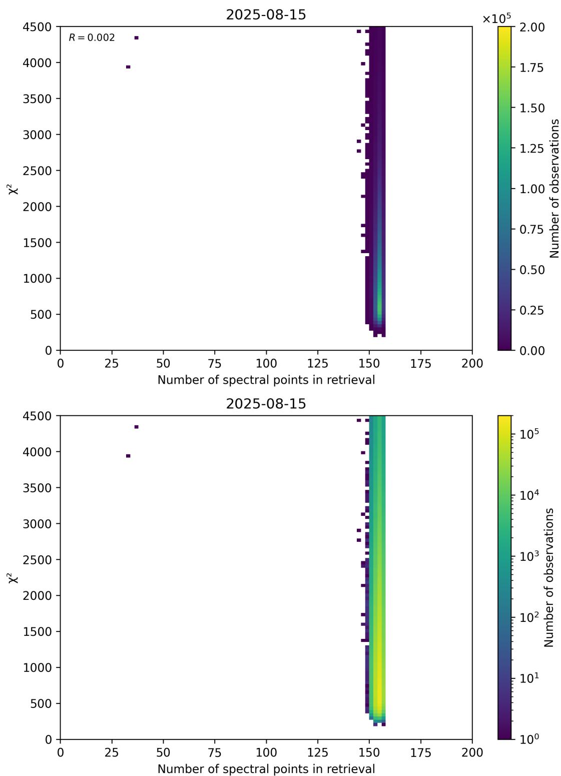
Figure 58: Scatter density plot of “Number of spectral points in retrieval” against “ \chi^2 ” for 2025-08-14 to 2025-08-16.
