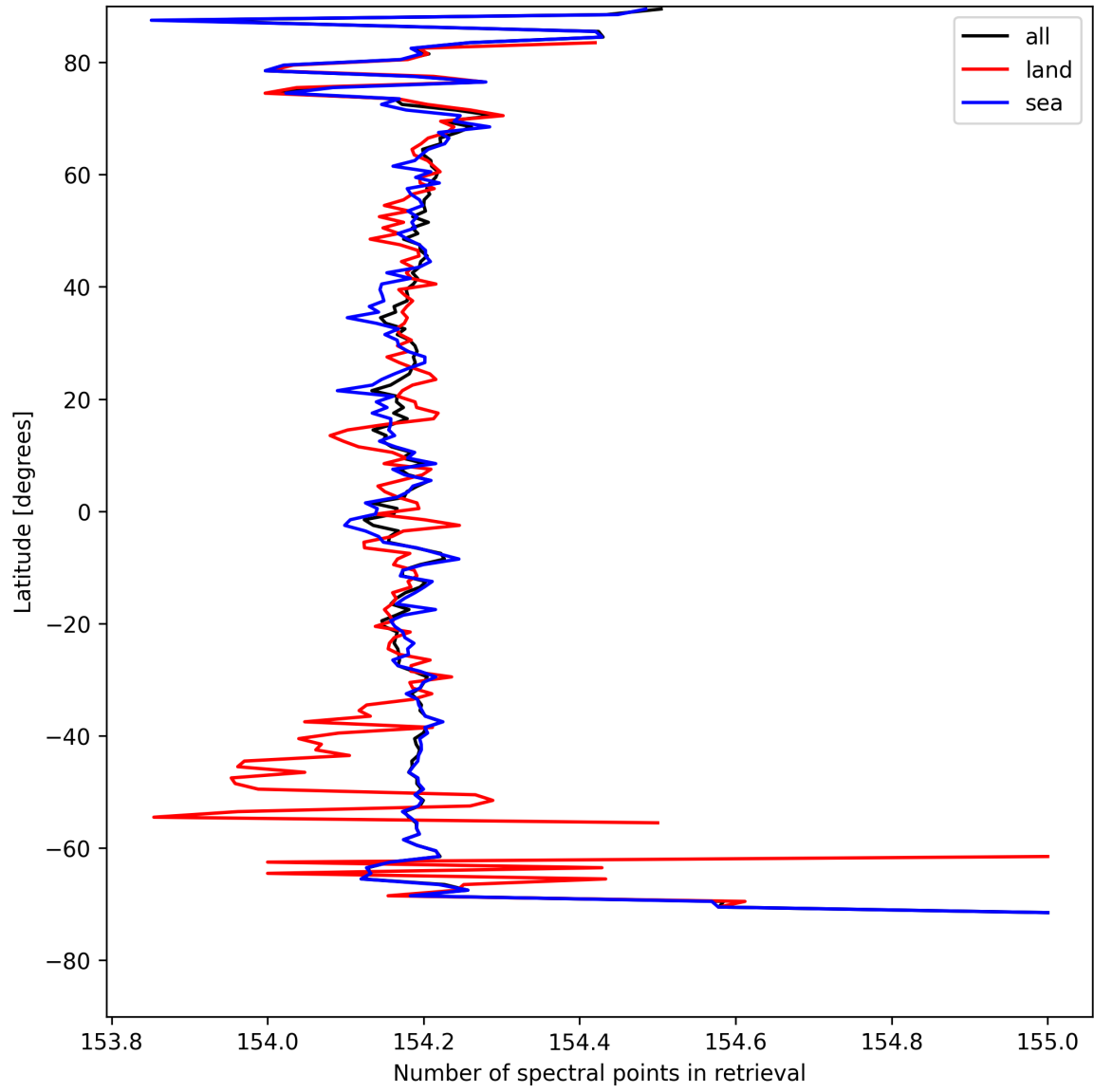
Figure 13: Zonal average of “Number of spectral points in retrieval” for 2025-08-14 to 2025-08-16.
