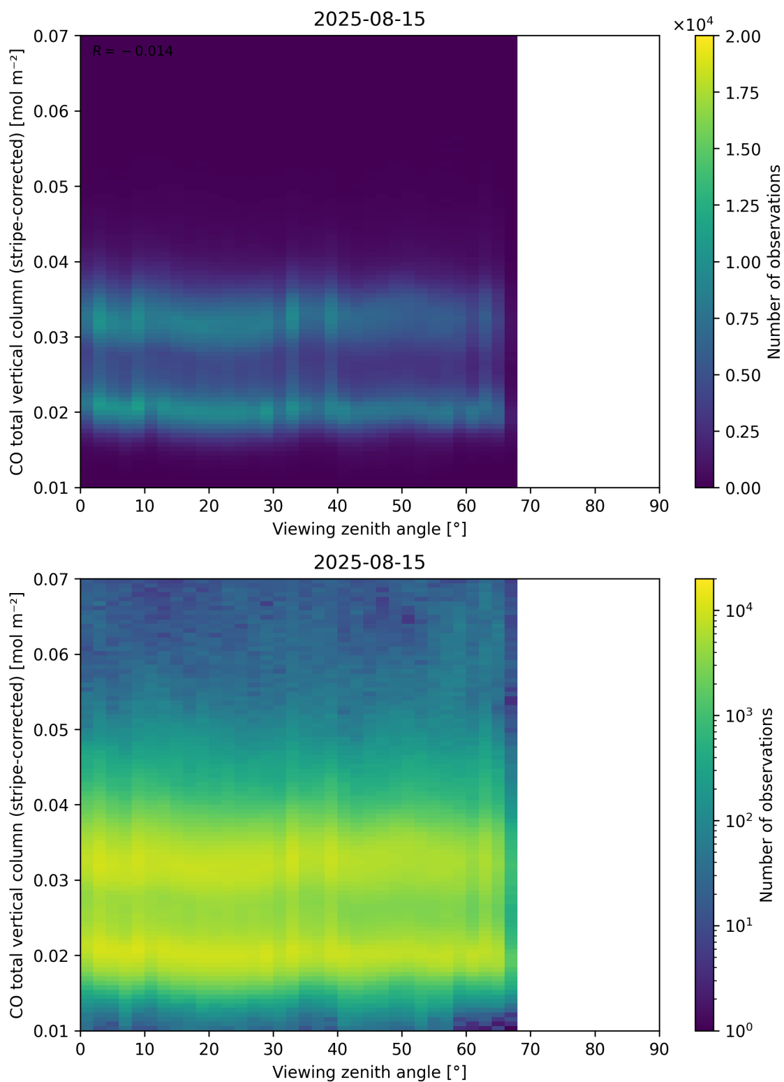
Figure 70: Scatter density plot of “Viewing zenith angle” against “CO total vertical column (stripe-corrected)” for 2025-08-14 to 2025-08-16.
