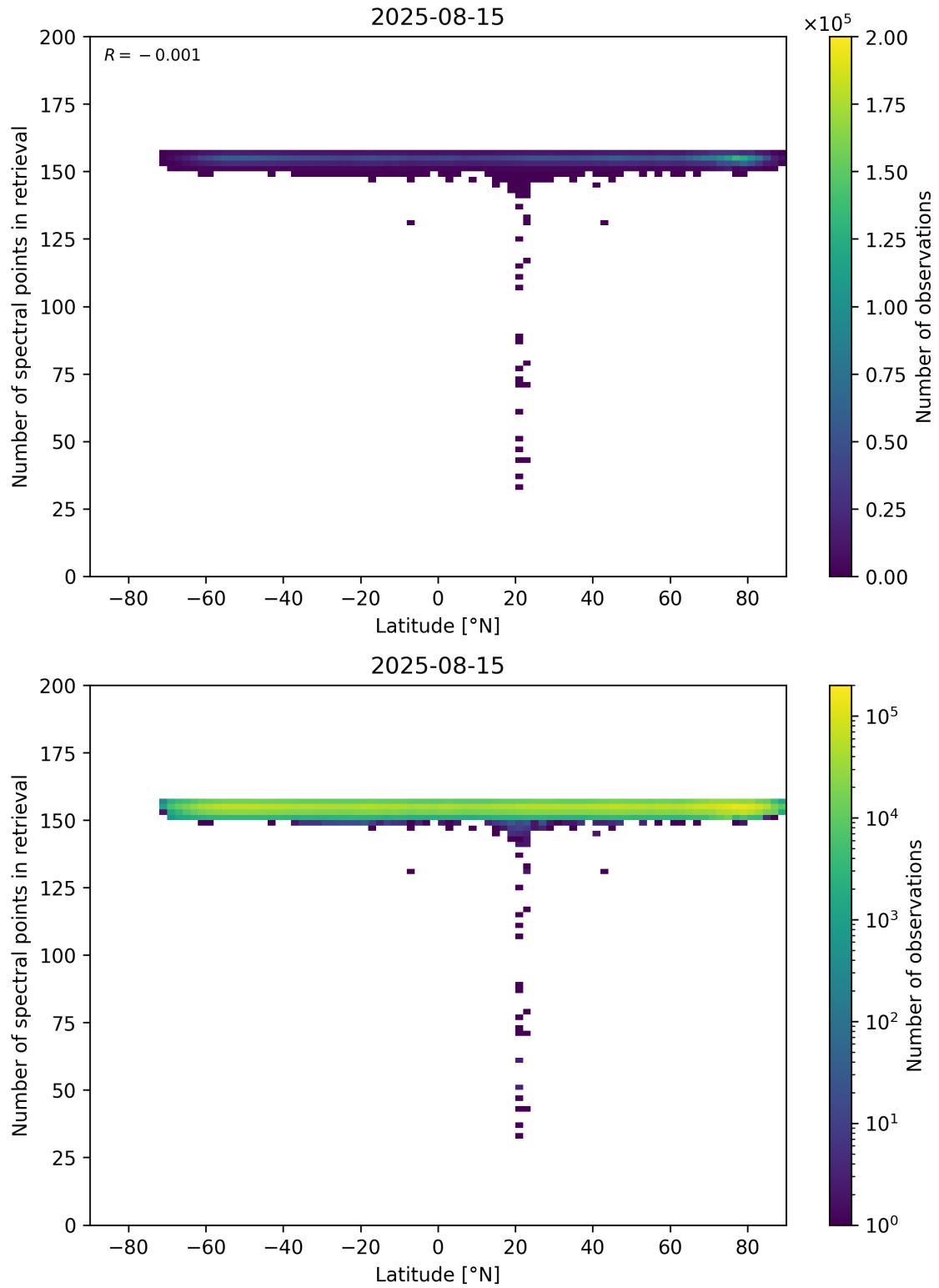
Figure 57: Scatter density plot of “Latitude” against “Number of spectral points in retrieval” for 2025-08-14 to 2025-08-16.
