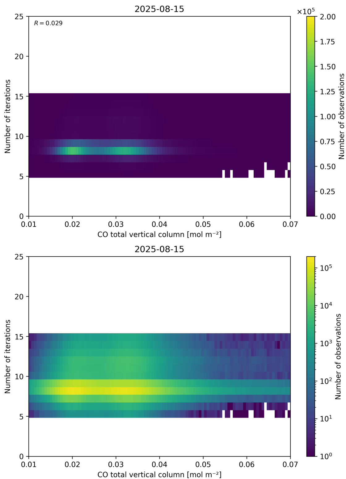
Figure 42: Scatter density plot of “CO total vertical column” against “Number of iterations” for 2025-08-14 to 2025-08-16.
