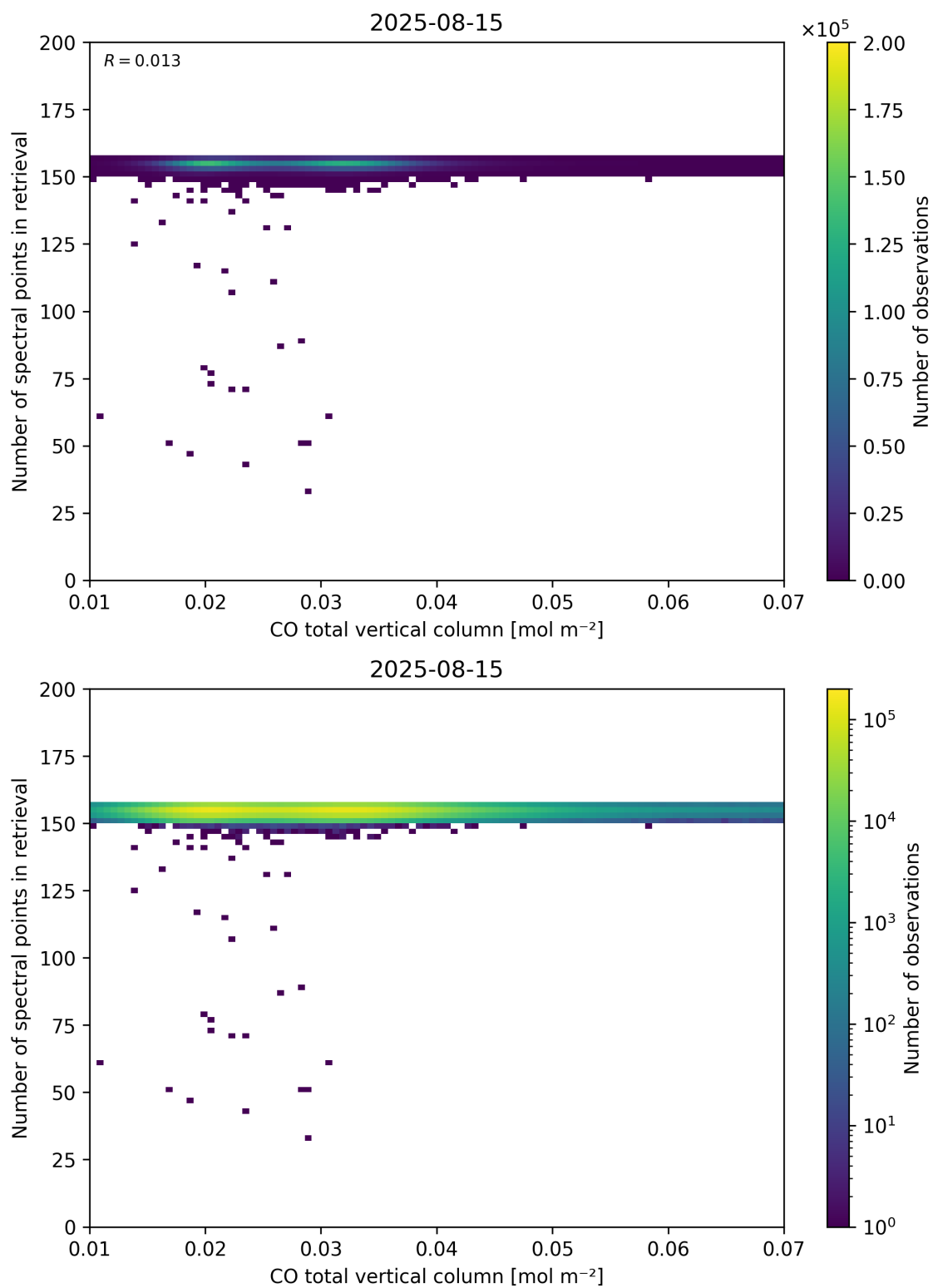
Figure 43: Scatter density plot of “CO total vertical column” against “Number of spectral points in retrieval” for 2025-08-14 to 2025-08-16.
