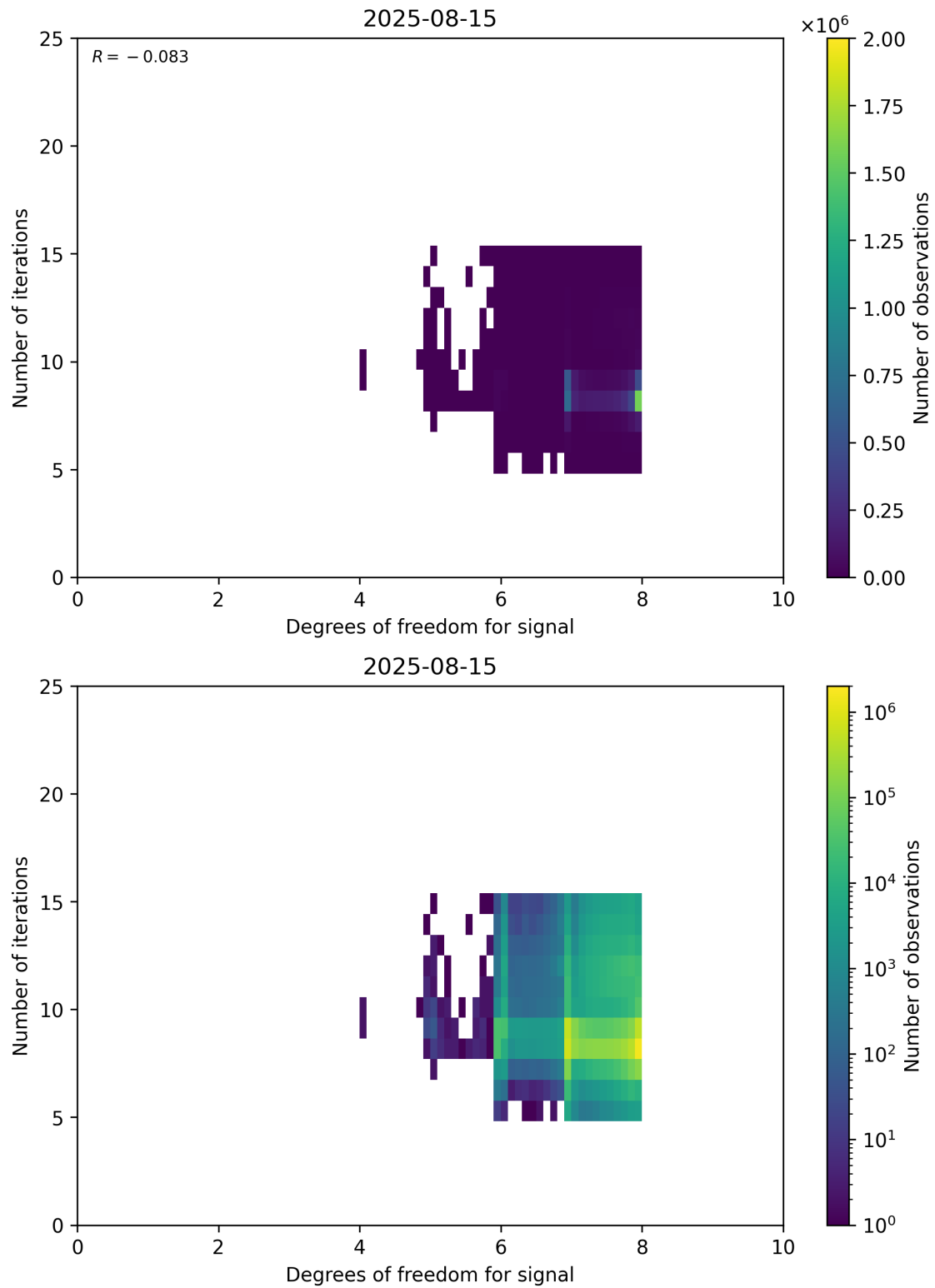
Figure 50: Scatter density plot of “Degrees of freedom for signal” against “Number of iterations” for 2025-08-14 to 2025-08-16.
