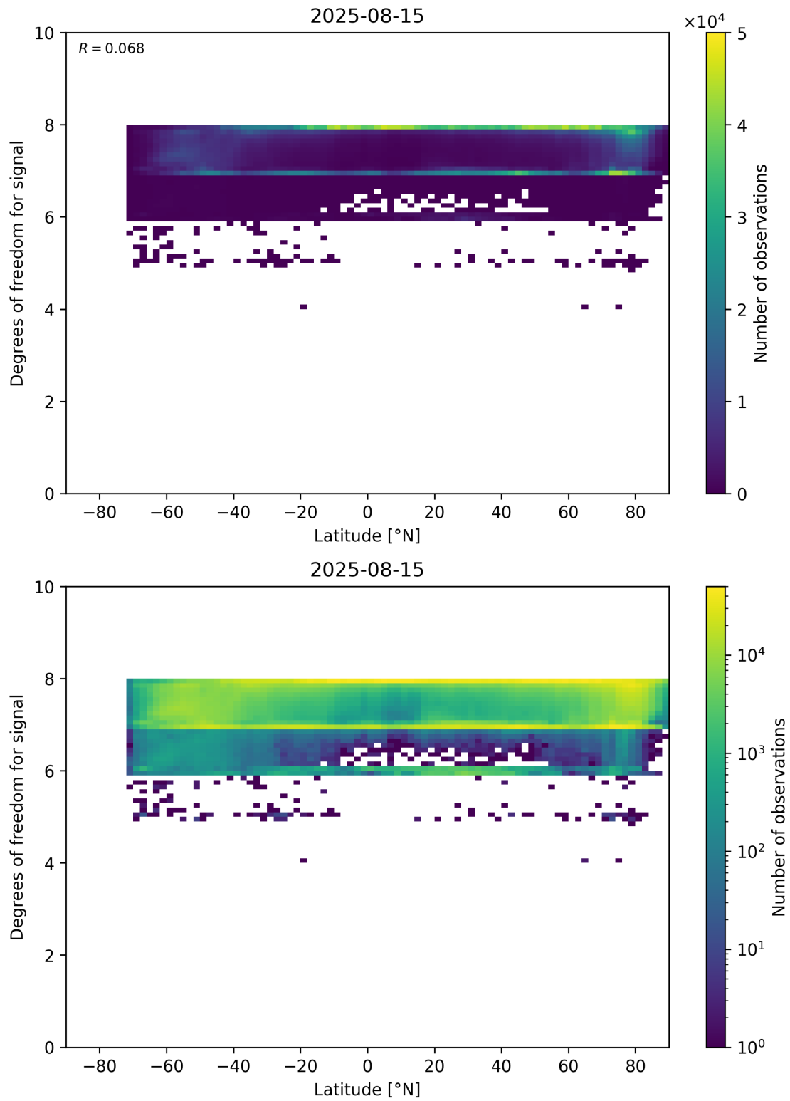
Figure 55: Scatter density plot of “Latitude” against “Degrees of freedom for signal” for 2025-08-14 to 2025-08-16.
