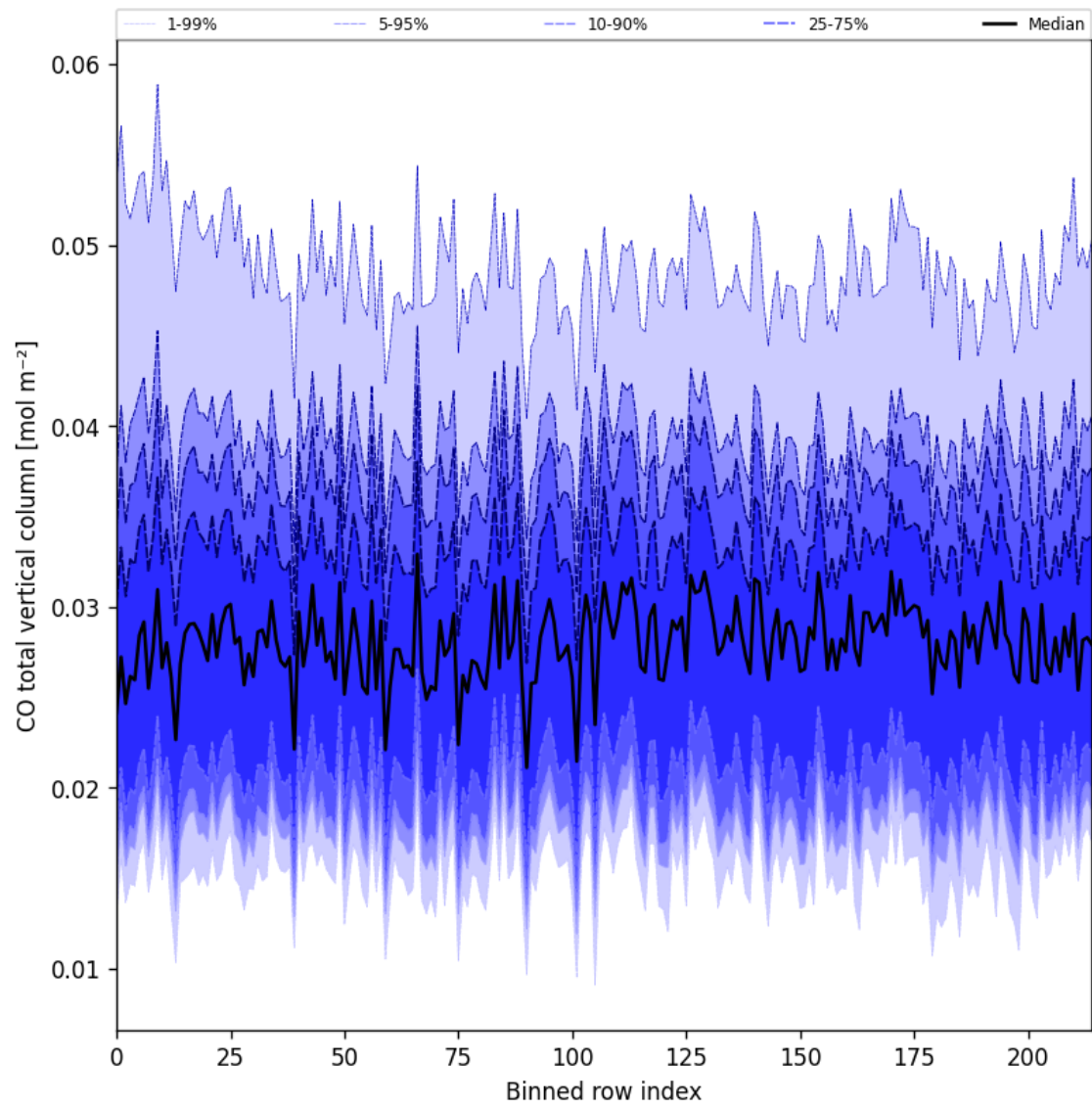
Figure 26: Along track statistics of “CO total vertical column” for 2025-08-14 to 2025-08-16
