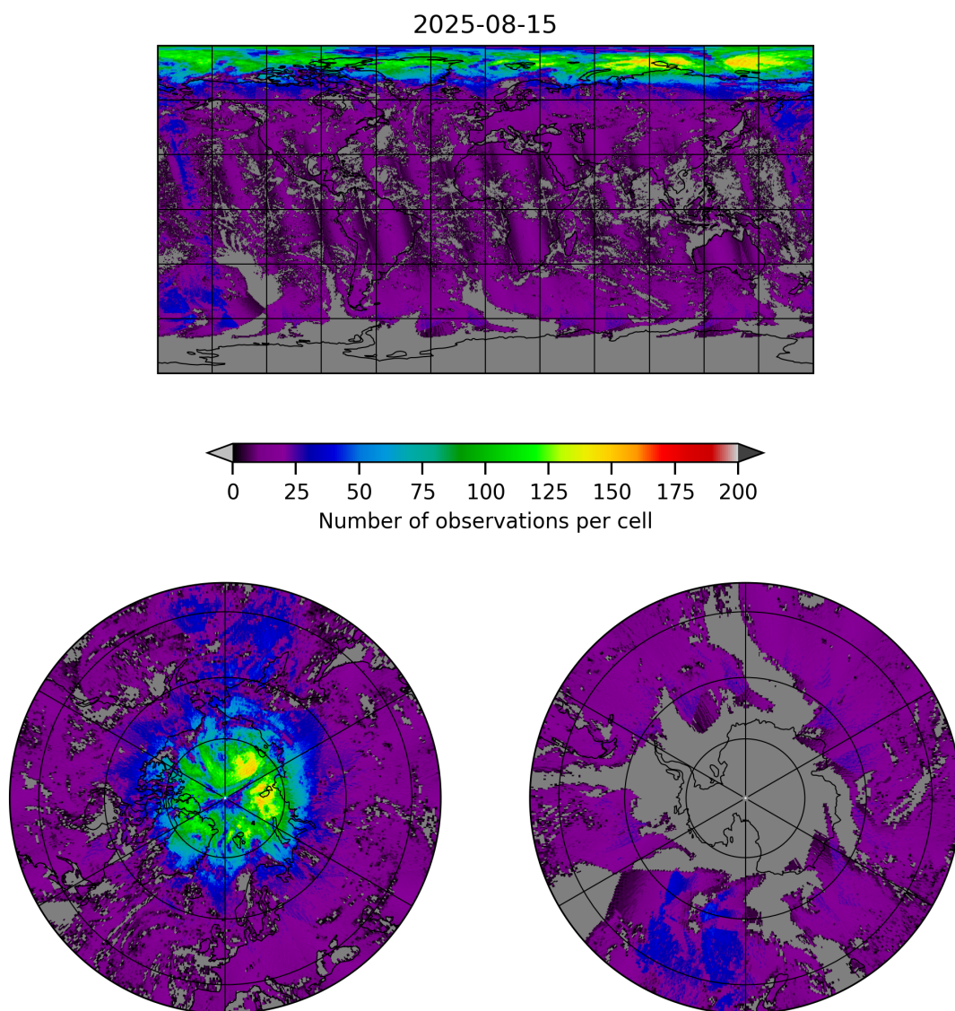
Figure 8: Map of the number of observations for 2025-08-14 to 2025-08-16
