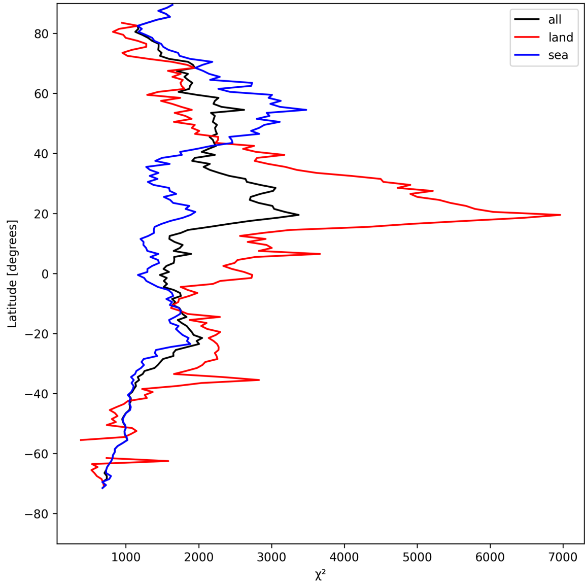
Figure 14: Zonal average of “ \chi^2 ” for 2025-08-14 to 2025-08-16.
