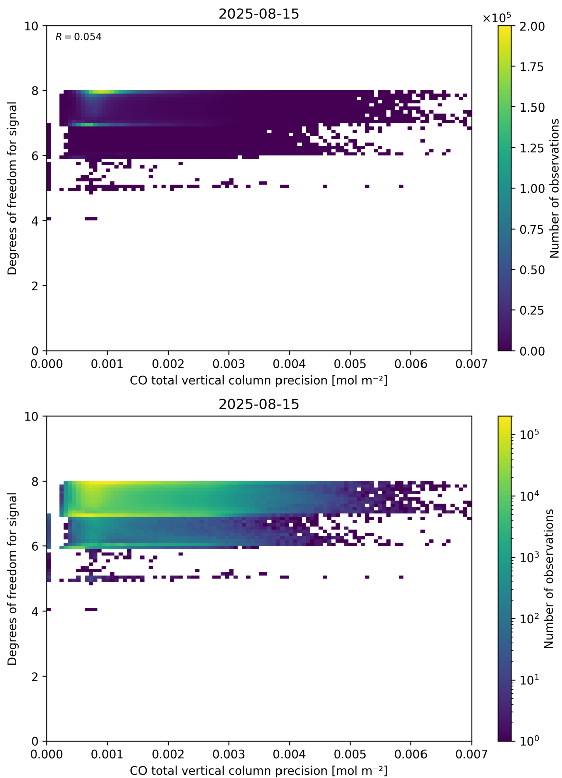
Figure 45: Scatter density plot of “CO total vertical column precision” against “Degrees of freedom for signal” for 2025-08-14 to 2025-08-16.
