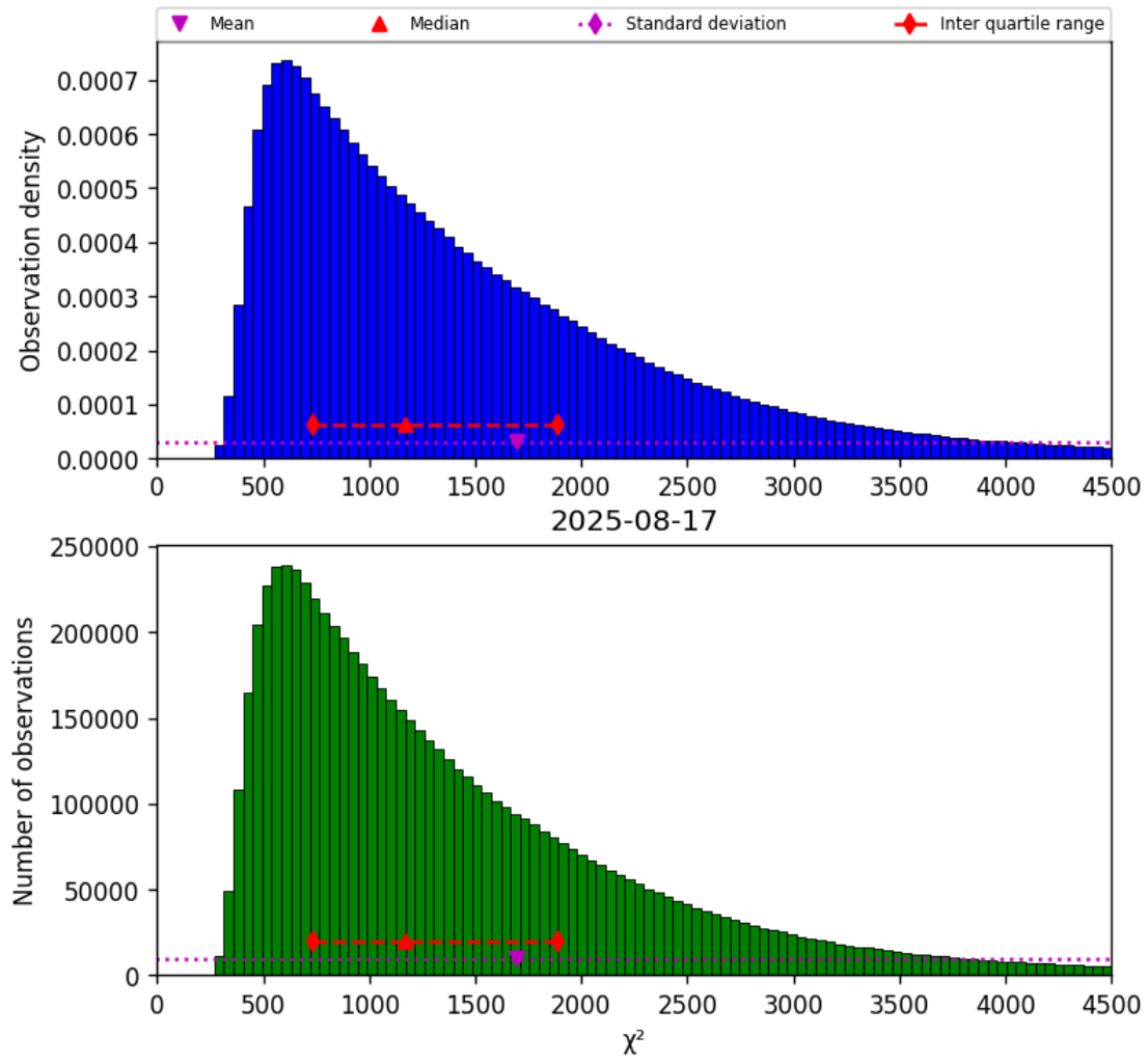
Figure 22: Histogram of “ \chi^2 ” for 2025-08-16 to 2025-08-18
