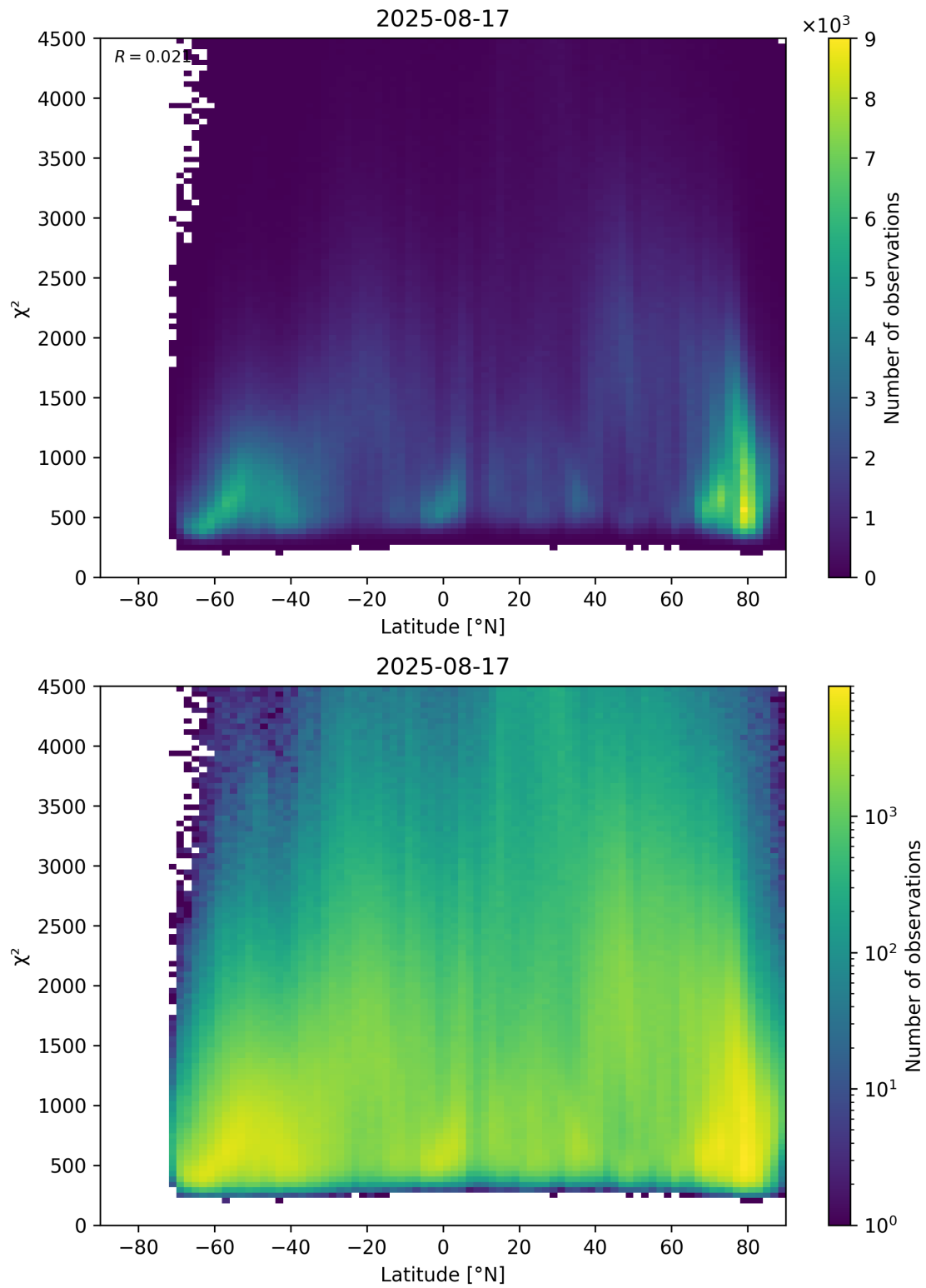
Figure 54: Scatter density plot of “Latitude” against “ \chi^2 ” for 2025-08-16 to 2025-08-18.
