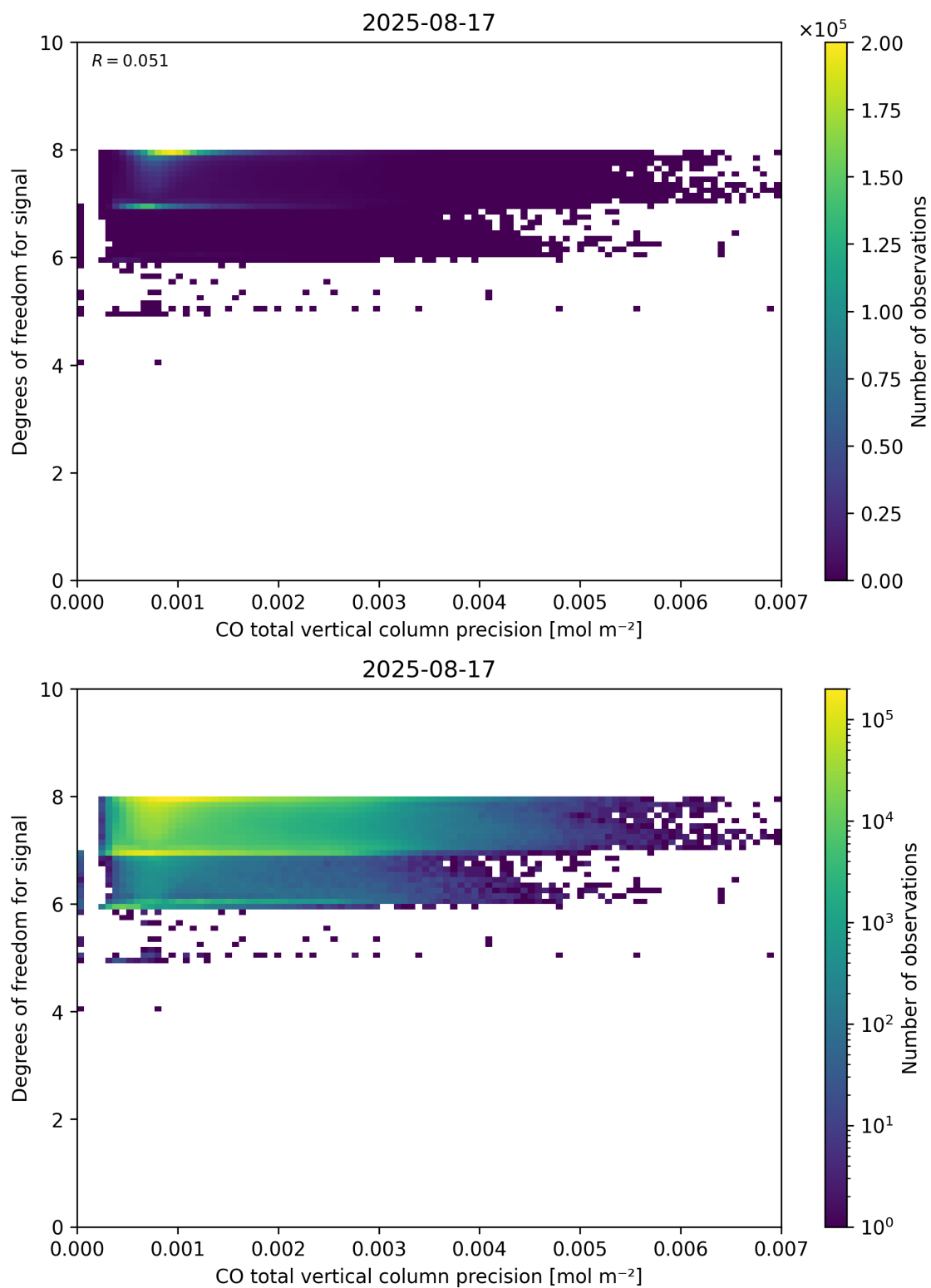
Figure 45: Scatter density plot of “CO total vertical column precision” against “Degrees of freedom for signal” for 2025-08-16 to 2025-08-18.
