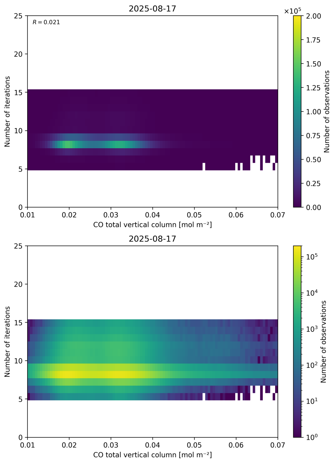
Figure 42: Scatter density plot of “CO total vertical column” against “Number of iterations” for 2025-08-16 to 2025-08-18.
