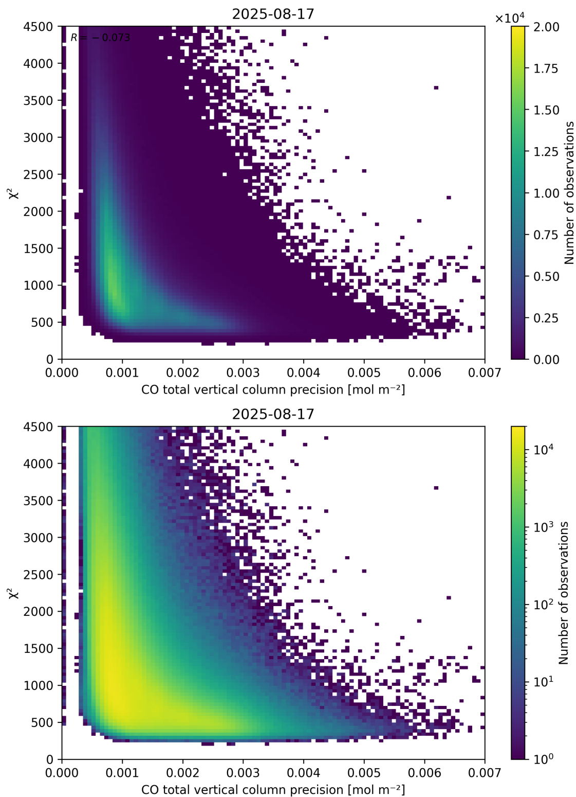
Figure 44: Scatter density plot of “CO total vertical column precision” against “ \chi^2 ” for 2025-08-16 to 2025-08-18.
