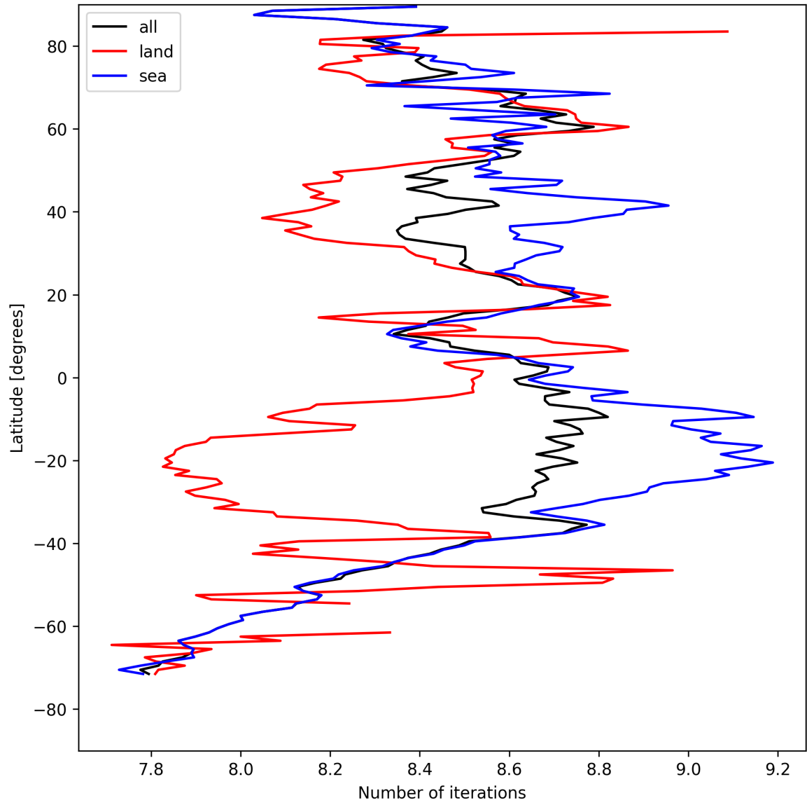
Figure 16: Zonal average of “Number of iterations” for 2025-08-16 to 2025-08-18.
