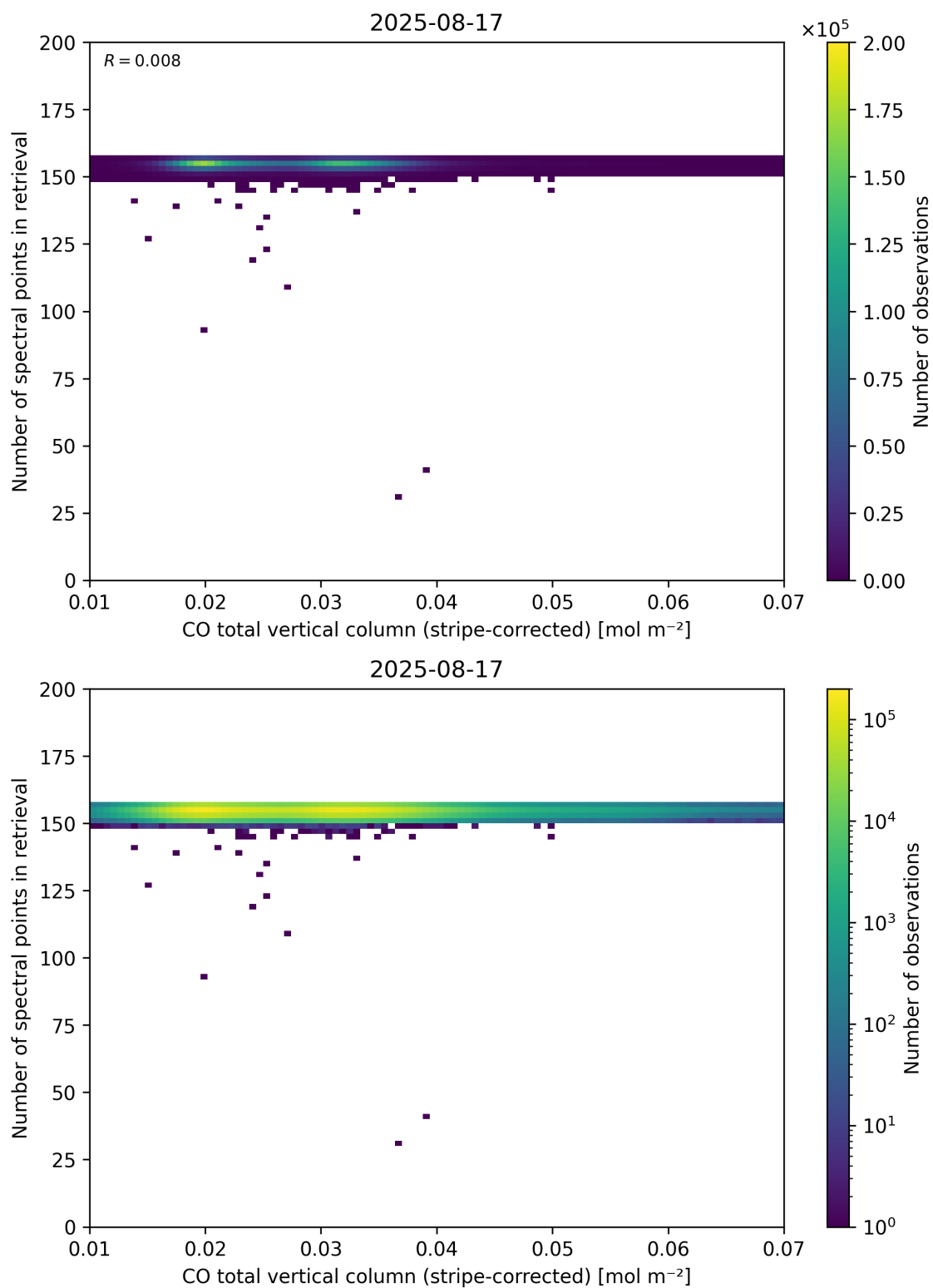
Figure 40: Scatter density plot of “CO total vertical column (stripe-corrected)” against “Number of spectral points in retrieval” for 2025-08-16 to 2025-08-18.
