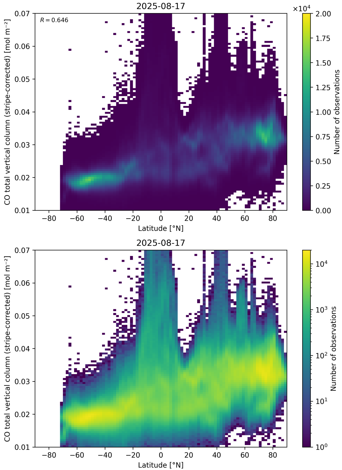
Figure 52: Scatter density plot of “Latitude” against “CO total vertical column (stripe-corrected)” for 2025-08-16 to 2025-08-18.
