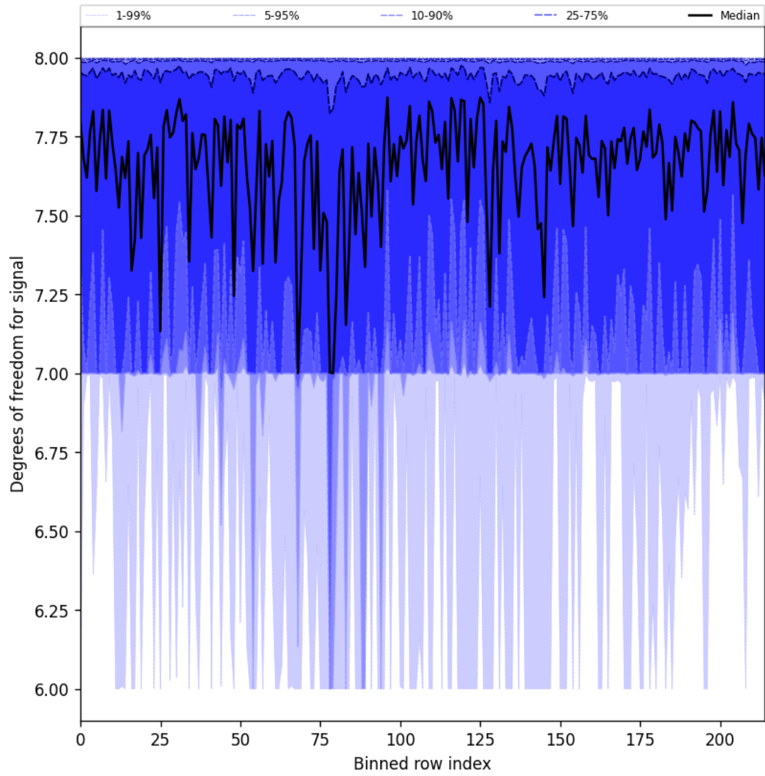
Figure 31: Along track statistics of “Degrees of freedom for signal” for 2025-08-16 to 2025-08-18
