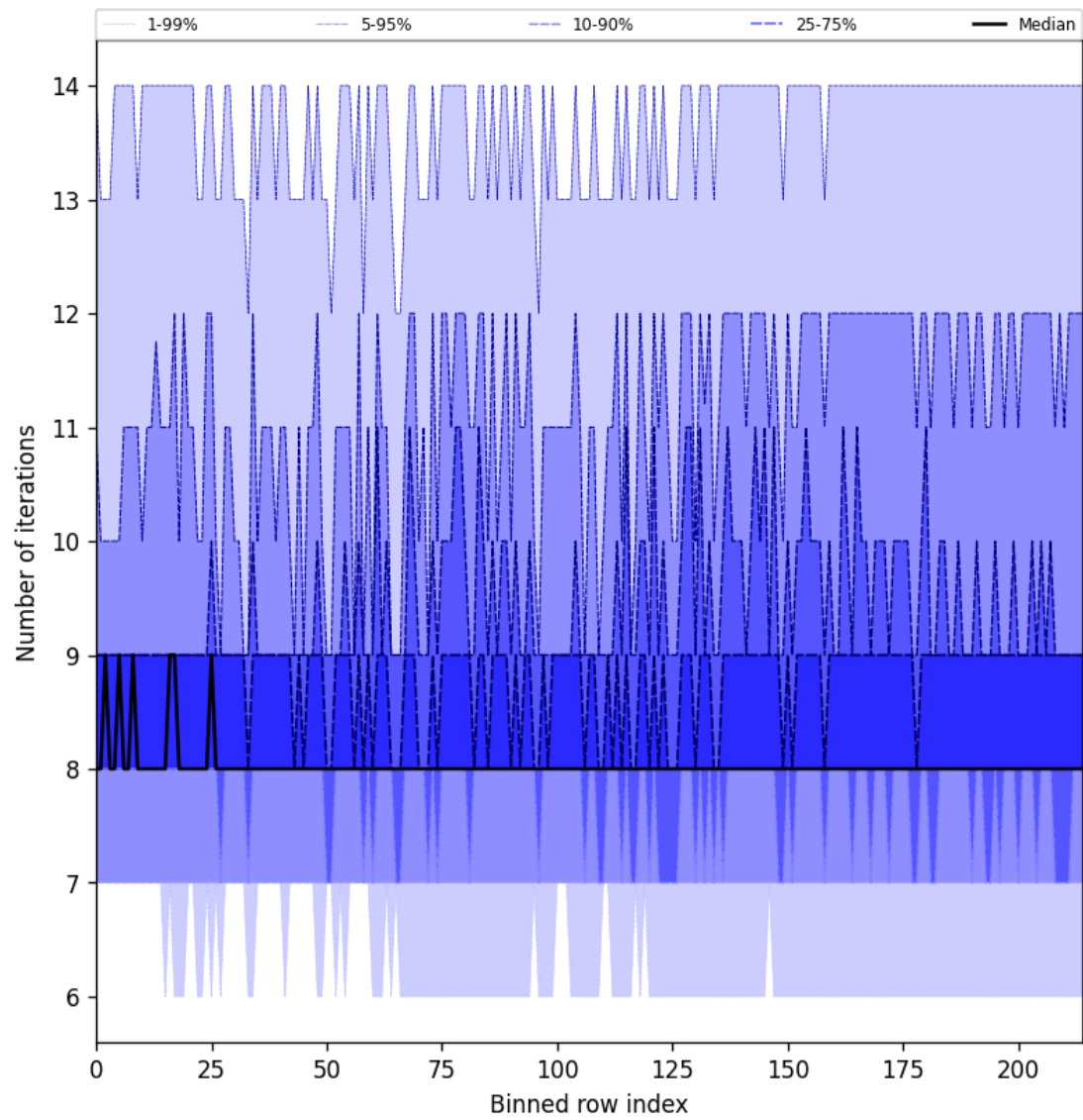
Figure 32: Along track statistics of “Number of iterations” for 2025-08-16 to 2025-08-18
