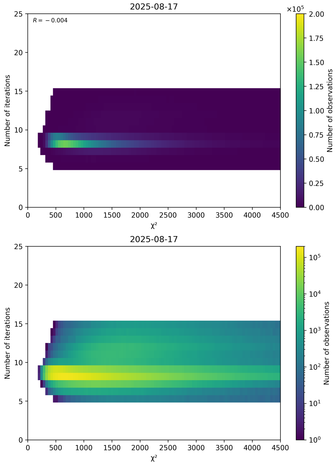
Figure 49: Scatter density plot of “ \chi^2 ” against “Number of iterations” for 2025-08-16 to 2025-08-18.
