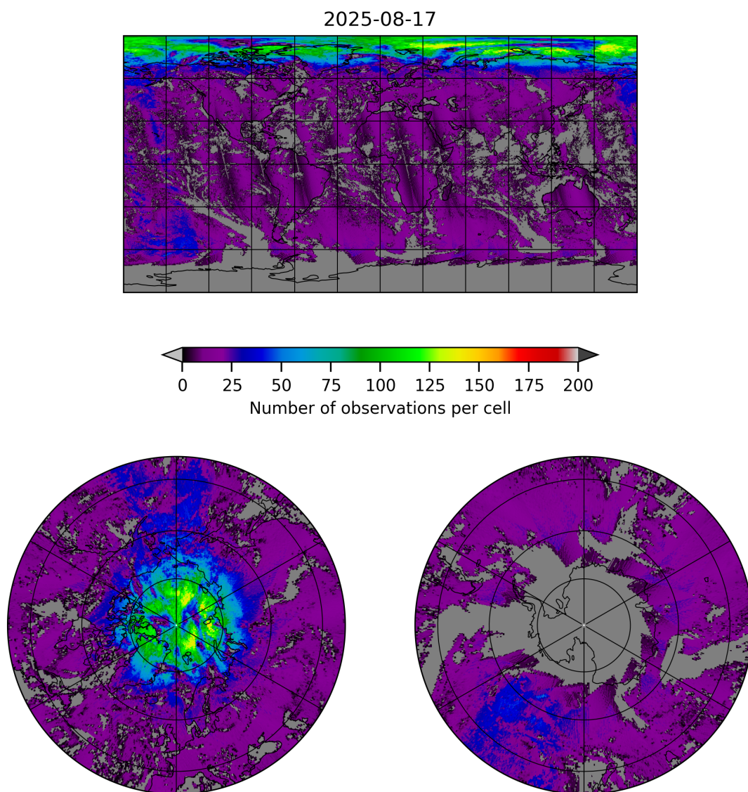
Figure 8: Map of the number of observations for 2025-08-16 to 2025-08-18
