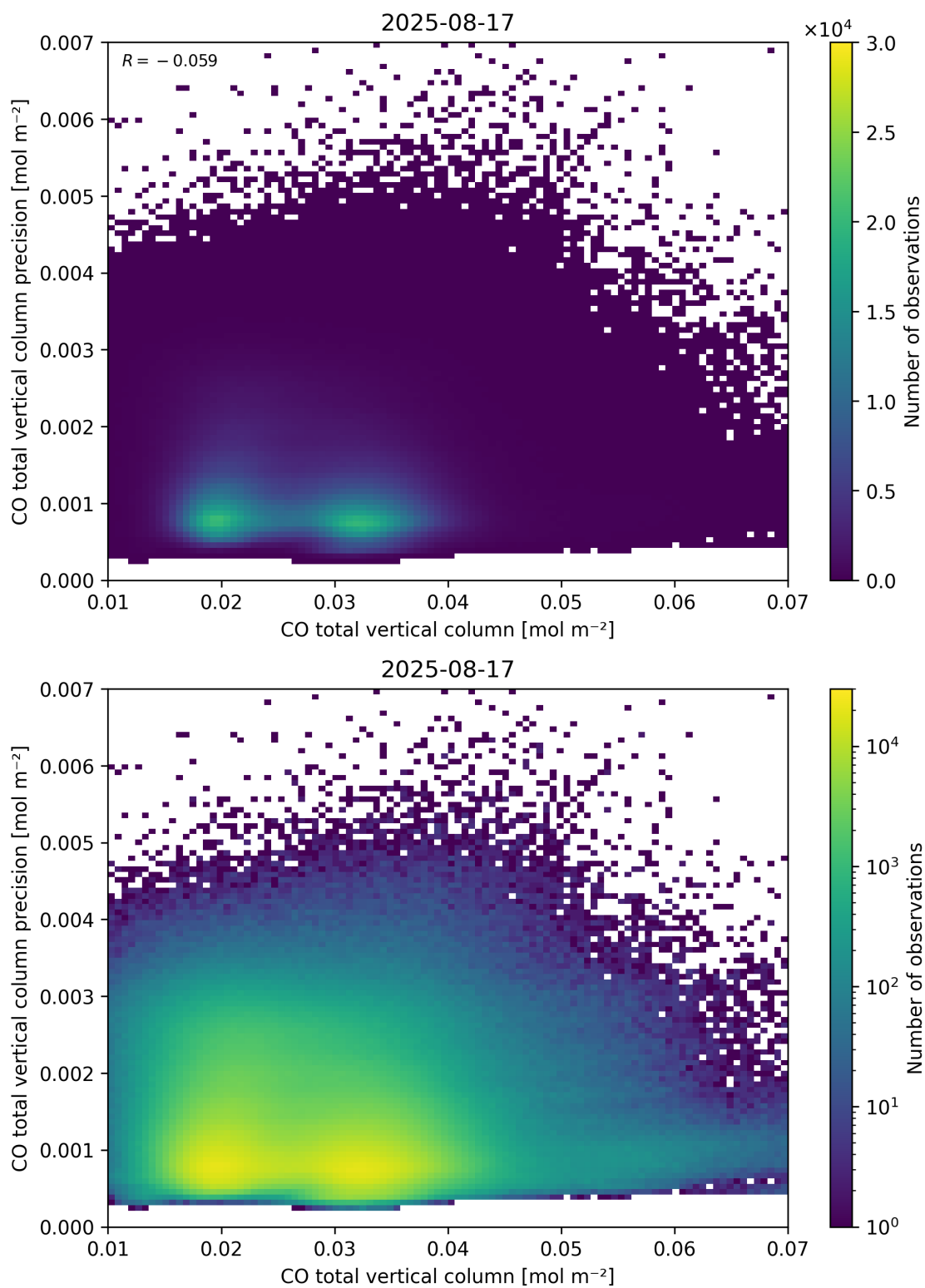
Figure 34: Scatter density plot of “CO total vertical column” against “CO total vertical column precision” for 2025-08-16 to 2025-08-18.
