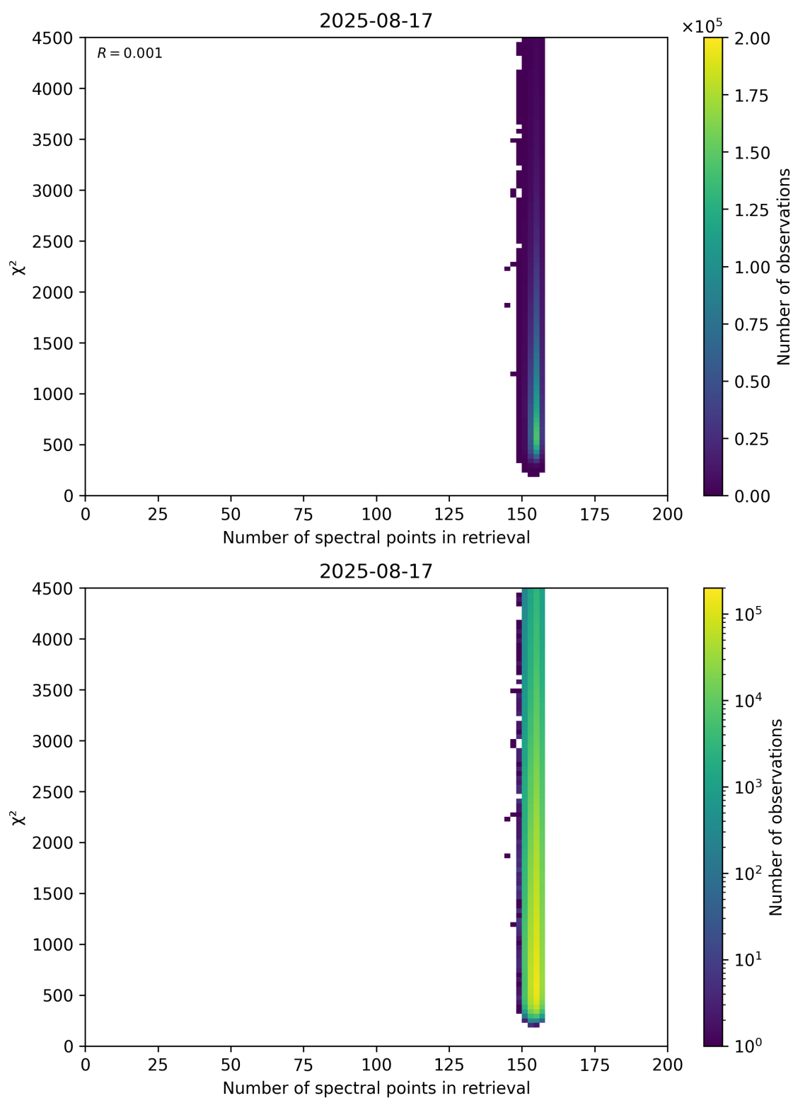
Figure 58: Scatter density plot of “Number of spectral points in retrieval” against “ \chi^2 ” for 2025-08-16 to 2025-08-18.
