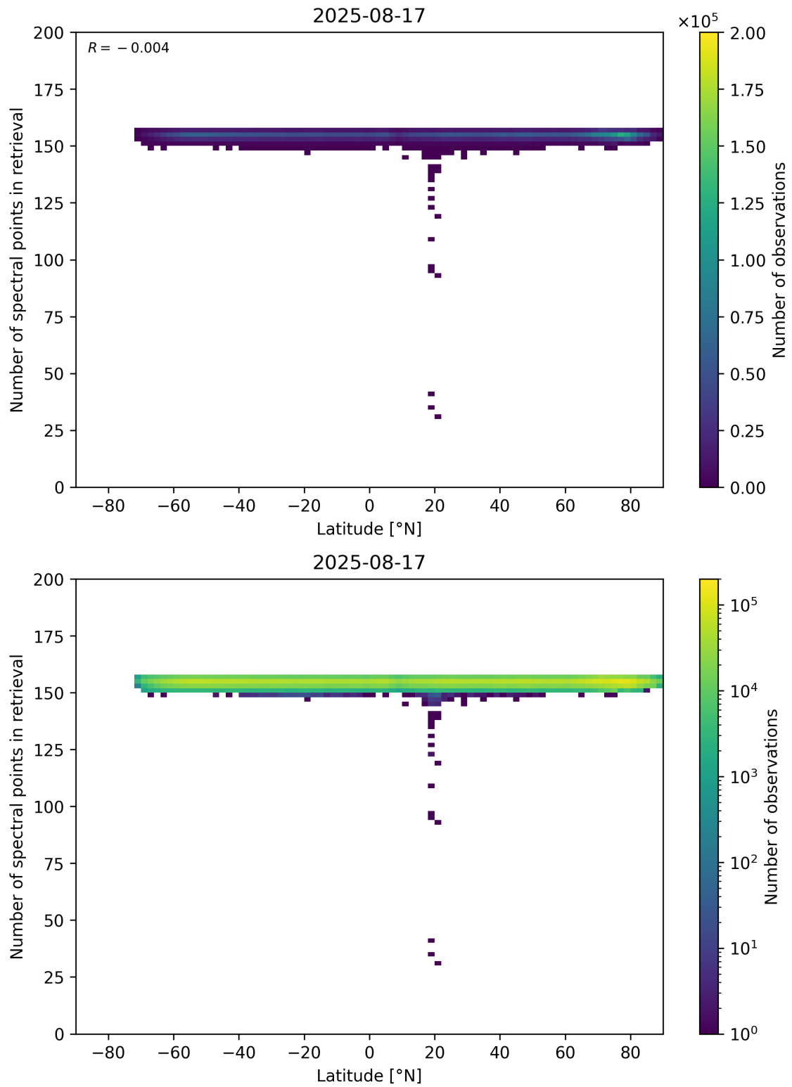
Figure 57: Scatter density plot of “Latitude” against “Number of spectral points in retrieval” for 2025-08-16 to 2025-08-18.
