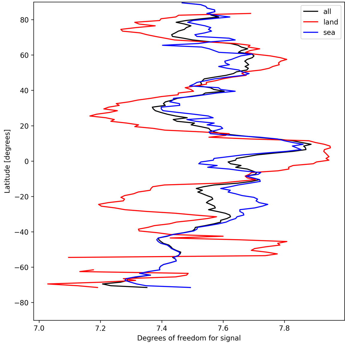
Figure 15: Zonal average of “Degrees of freedom for signal” for 2025-08-16 to 2025-08-18.
