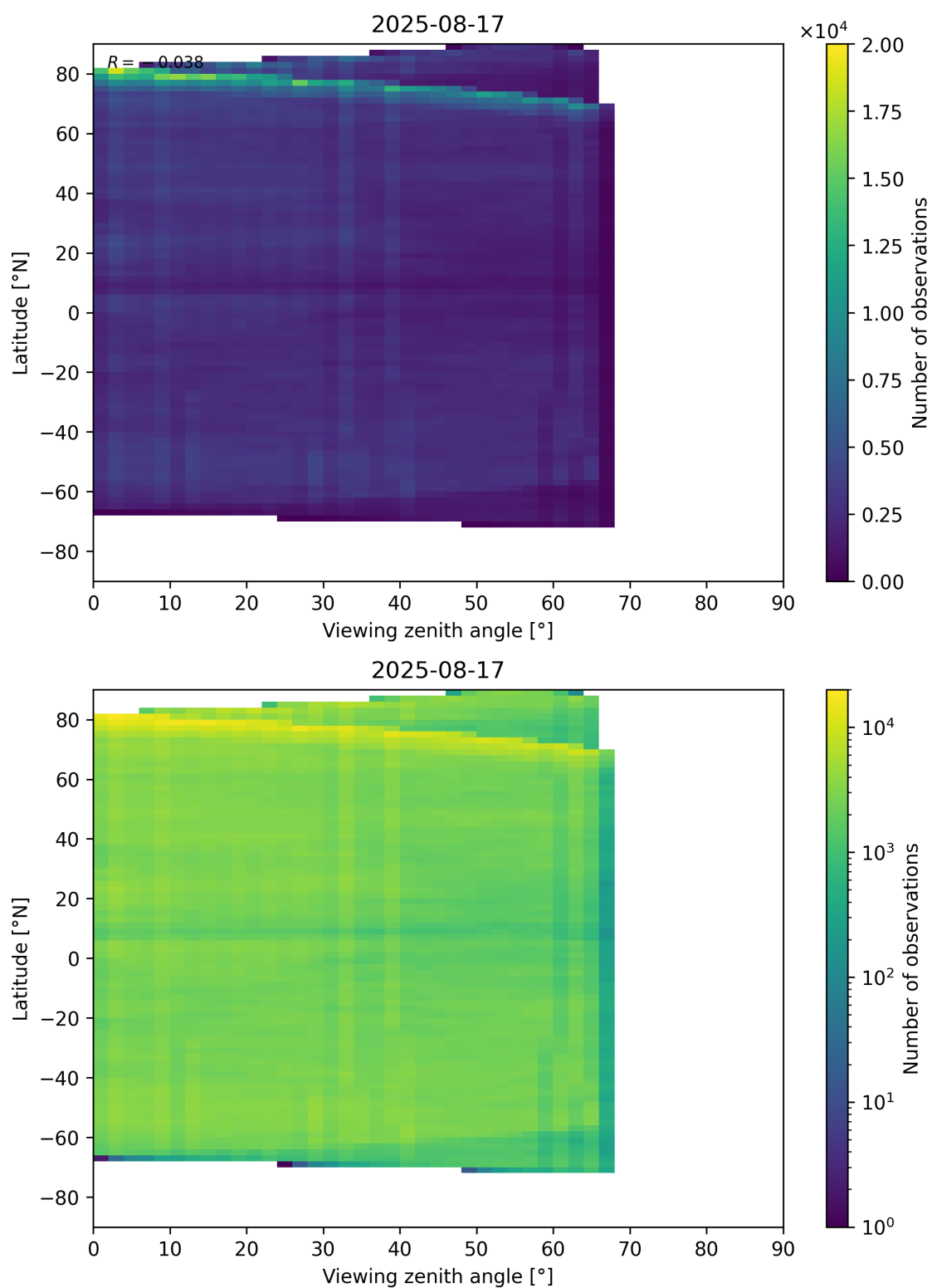
Figure 74: Scatter density plot of “Viewing zenith angle” against “Latitude” for 2025-08-16 to 2025-08-18.
