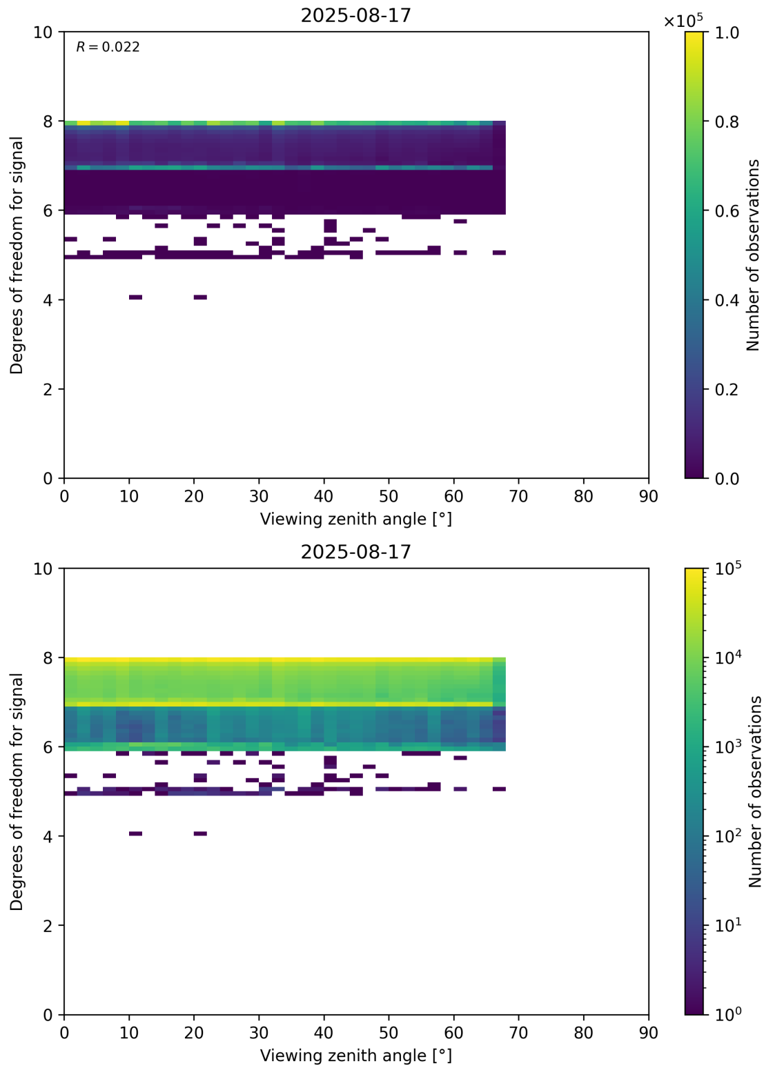
Figure 73: Scatter density plot of “Viewing zenith angle” against “Degrees of freedom for signal” for 2025-08-16 to 2025-08-18.
