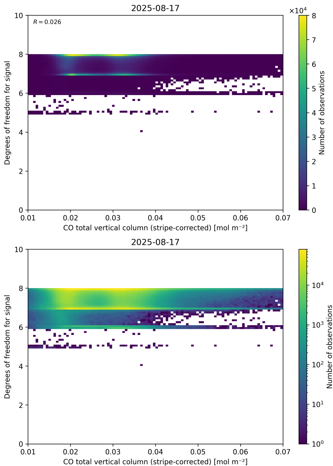
Figure 38: Scatter density plot of “CO total vertical column (stripe-corrected)” against “Degrees of freedom for signal” for 2025-08-16 to 2025-08-18.
