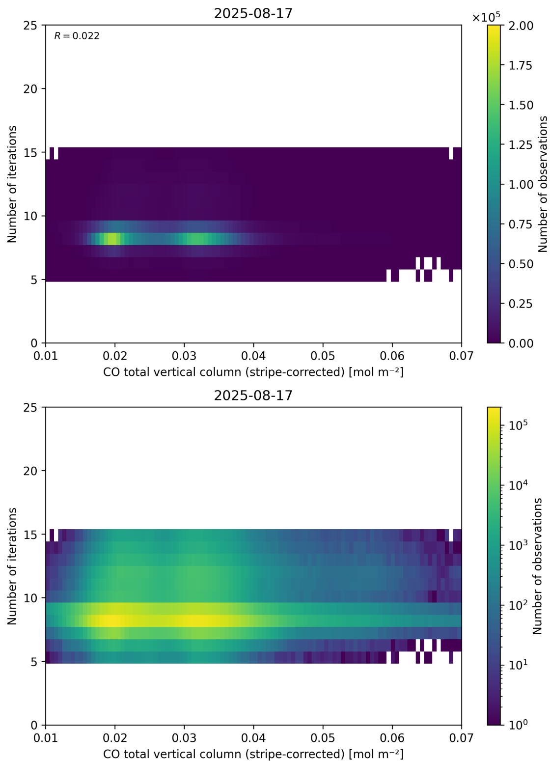
Figure 39: Scatter density plot of “CO total vertical column (stripe-corrected)” against “Number of iterations” for 2025-08-16 to 2025-08-18.
