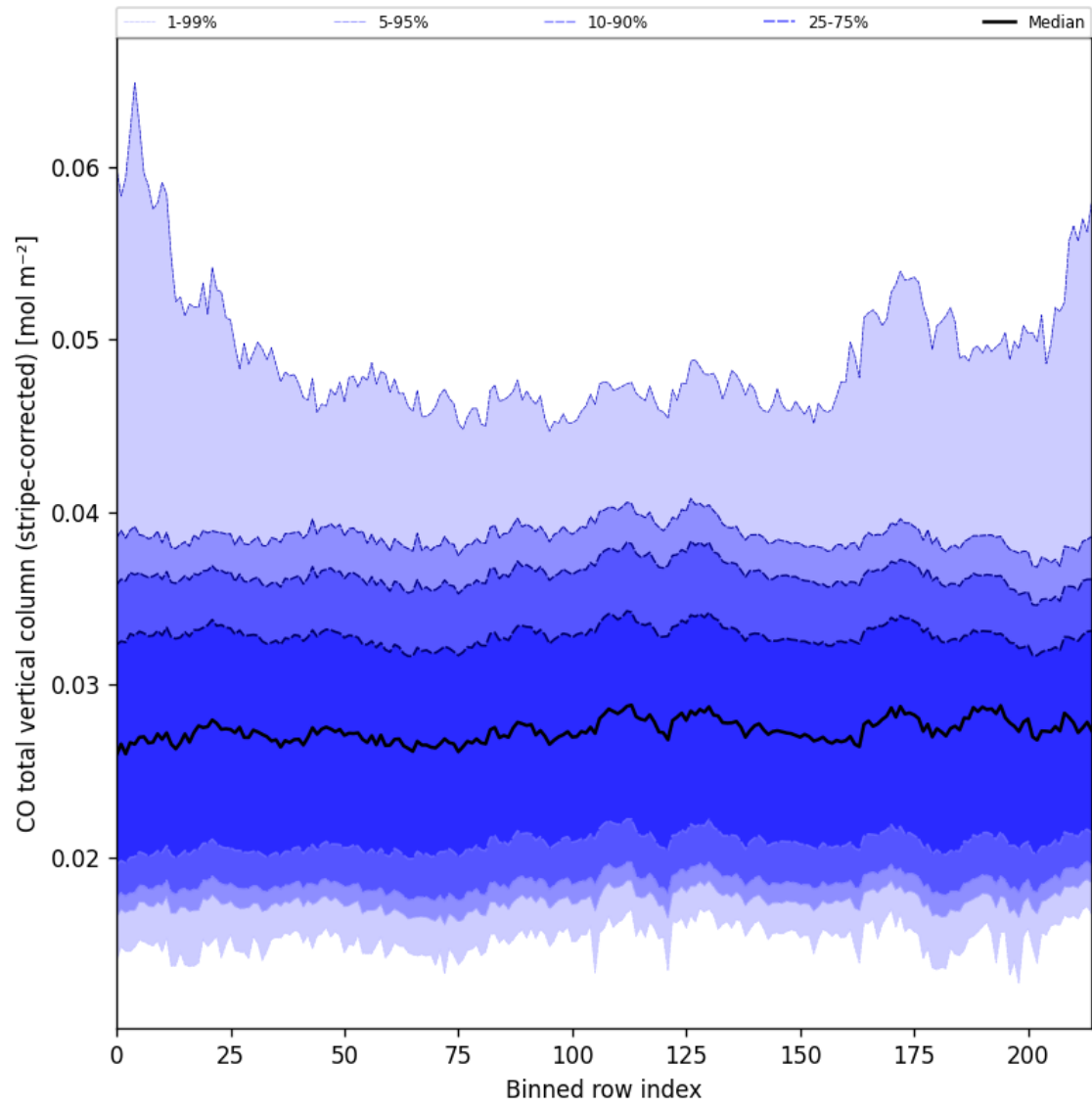
Figure 27: Along track statistics of “CO total vertical column (stripe-corrected)” for 2025-08-16 to 2025-08-18
