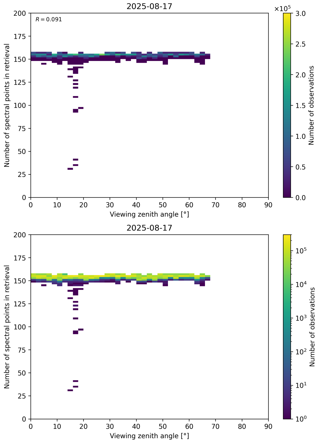
Figure 76: Scatter density plot of “Viewing zenith angle” against “Number of spectral points in retrieval” for 2025-08-16 to 2025-08-18.
