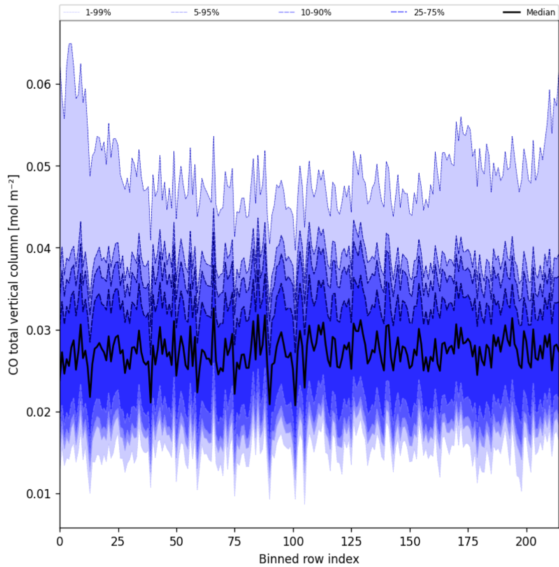
Figure 26: Along track statistics of “CO total vertical column” for 2025-08-16 to 2025-08-18
