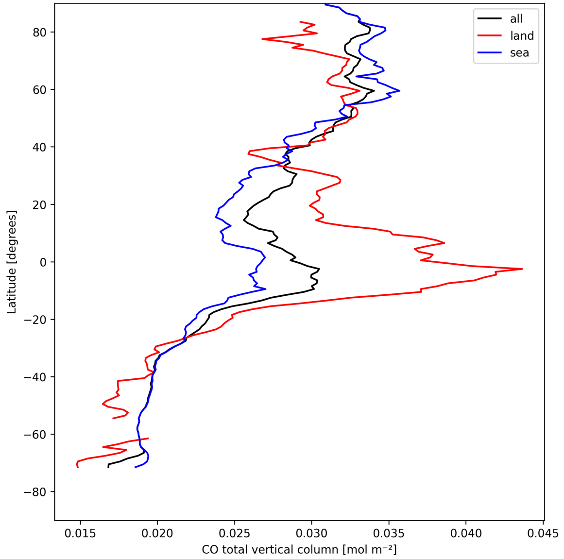
Figure 10: Zonal average of “CO total vertical column” for 2025-08-16 to 2025-08-18.
