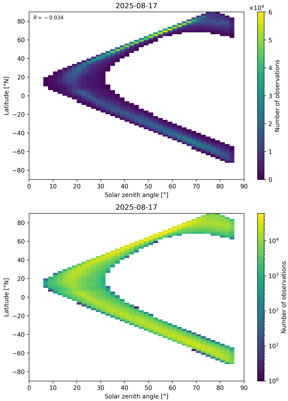
Figure 66: Scatter density plot of “Solar zenith angle” against “Latitude” for 2025-08-16 to 2025-08-18.
