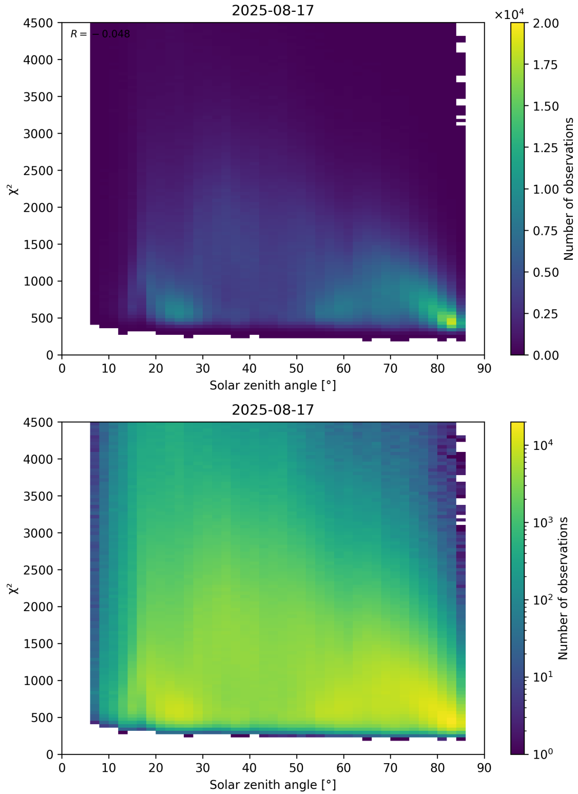
Figure 64: Scatter density plot of “Solar zenith angle” against “ \chi^2 ” for 2025-08-16 to 2025-08-18.
