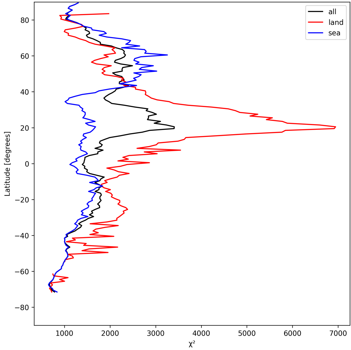
Figure 14: Zonal average of “ \chi^2 ” for 2025-08-16 to 2025-08-18.
