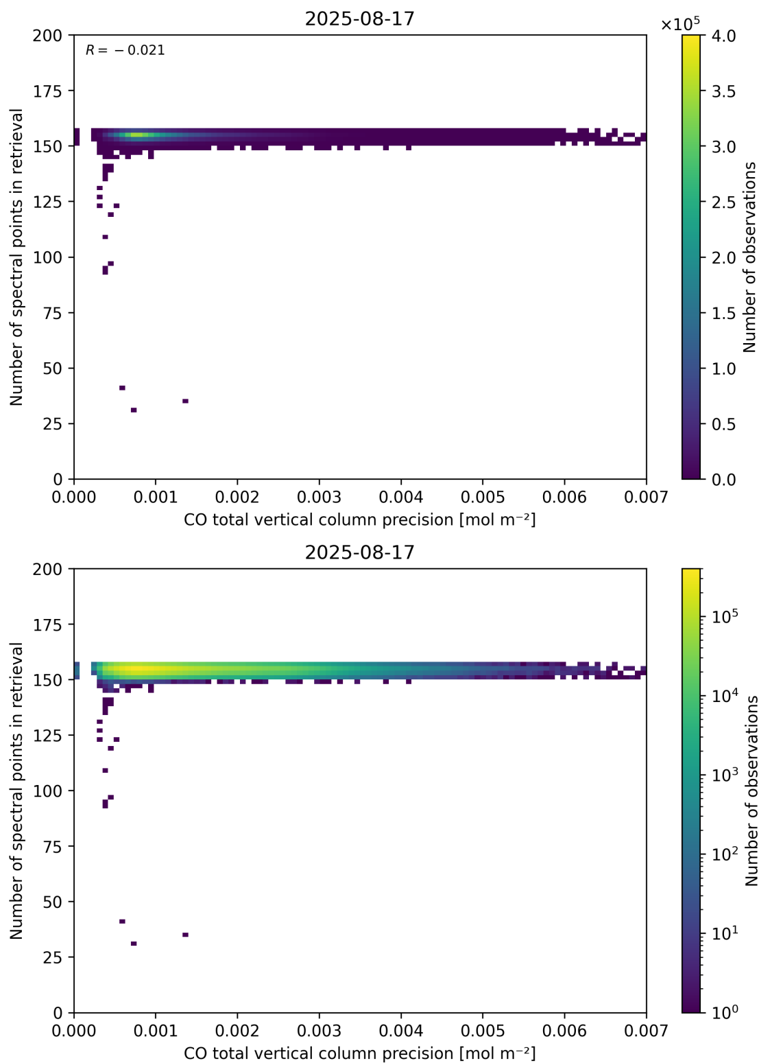
Figure 47: Scatter density plot of “CO total vertical column precision” against “Number of spectral points in retrieval” for 2025-08-16 to 2025-08-18.
