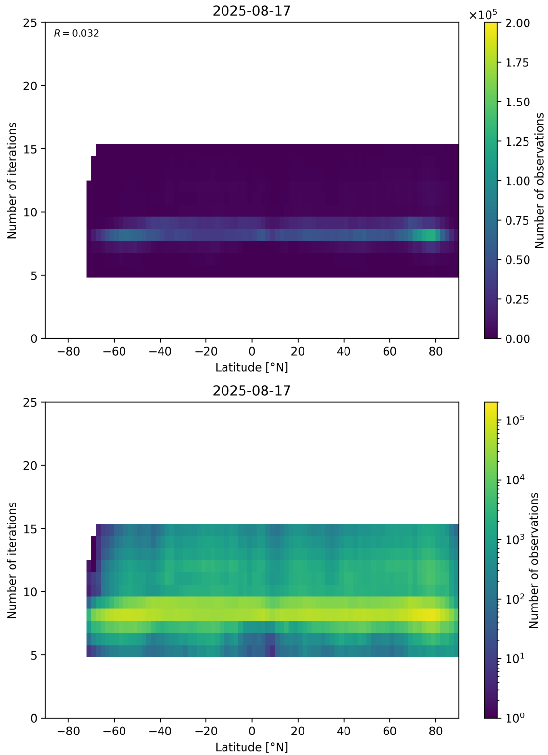
Figure 56: Scatter density plot of “Latitude” against “Number of iterations” for 2025-08-16 to 2025-08-18.
