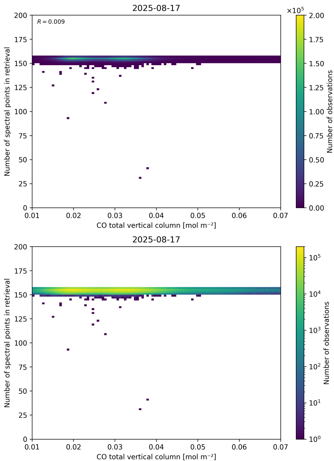
Figure 43: Scatter density plot of “CO total vertical column” against “Number of spectral points in retrieval” for 2025-08-16 to 2025-08-18.
