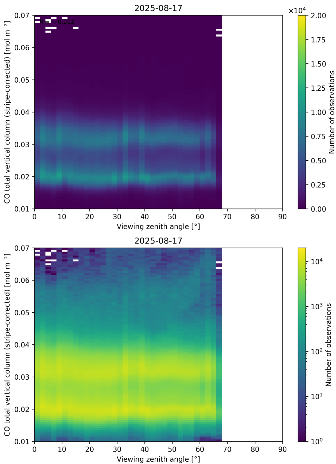
Figure 70: Scatter density plot of “Viewing zenith angle” against “CO total vertical column (stripe-corrected)” for 2025-08-16 to 2025-08-18.
