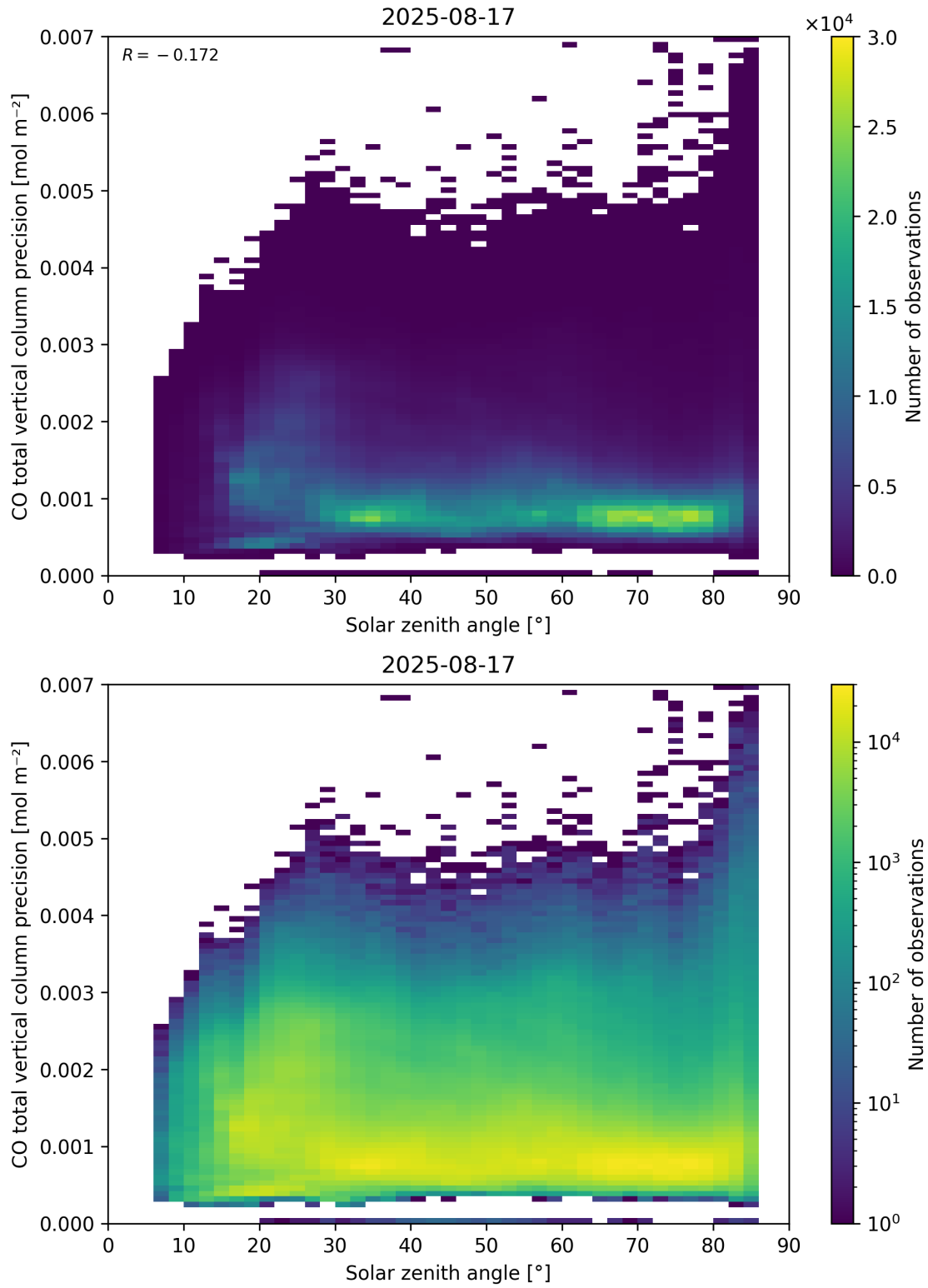
Figure 63: Scatter density plot of “Solar zenith angle” against “CO total vertical column precision” for 2025-08-16 to 2025-08-18.
