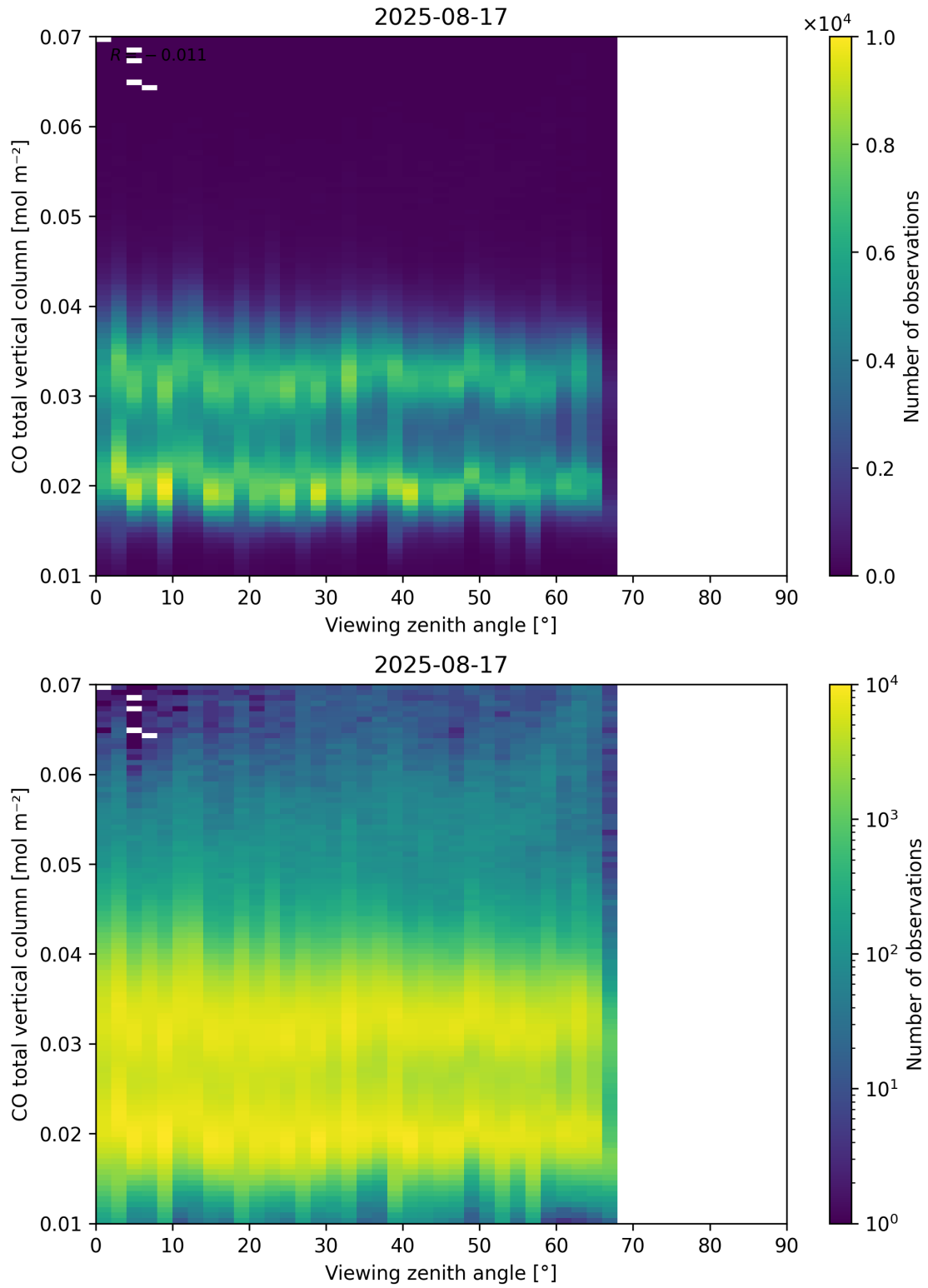
Figure 69: Scatter density plot of “Viewing zenith angle” against “CO total vertical column” for 2025-08-16 to 2025-08-18.
