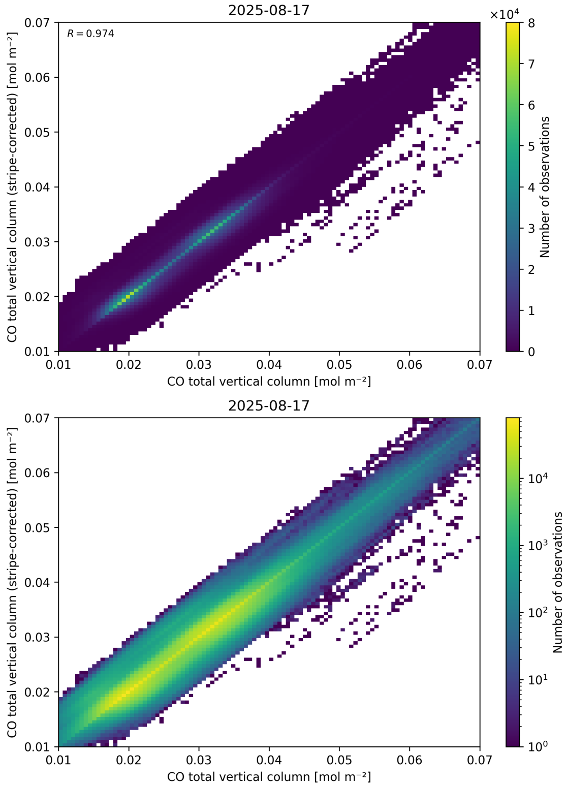
Figure 33: Scatter density plot of “CO total vertical column” against “CO total vertical column (stripe-corrected)” for 2025-08-16 to 2025-08-18.
