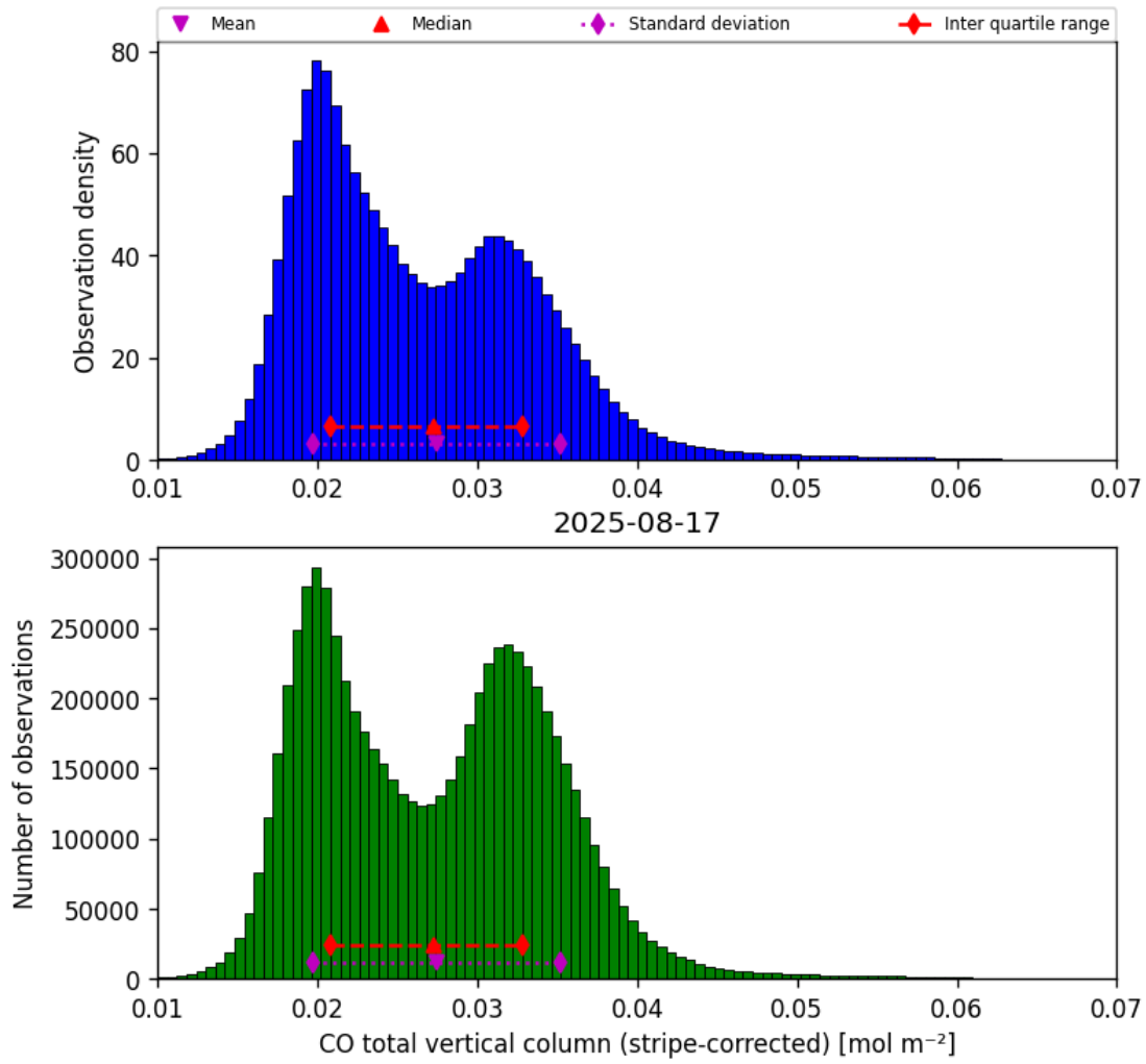
Figure 19: Histogram of “CO total vertical column (stripe-corrected)” for 2025-08-16 to 2025-08-18
