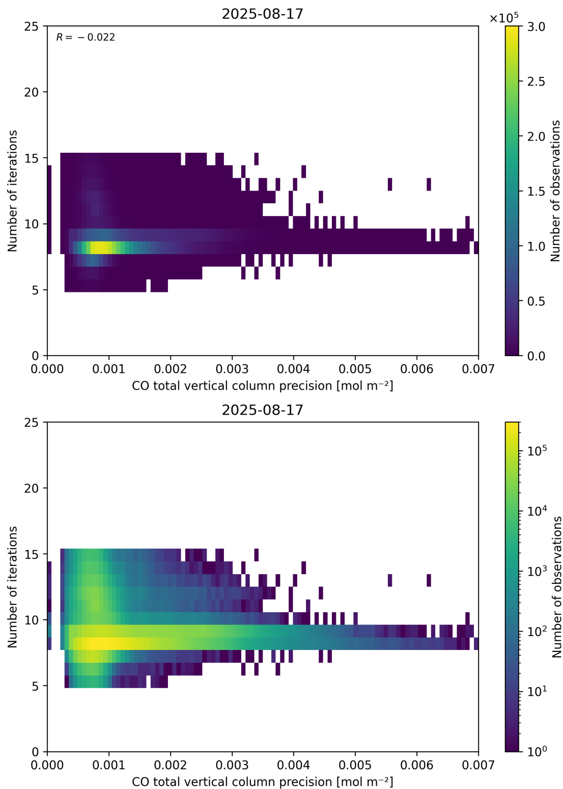
Figure 46: Scatter density plot of “CO total vertical column precision” against “Number of iterations” for 2025-08-16 to 2025-08-18.
