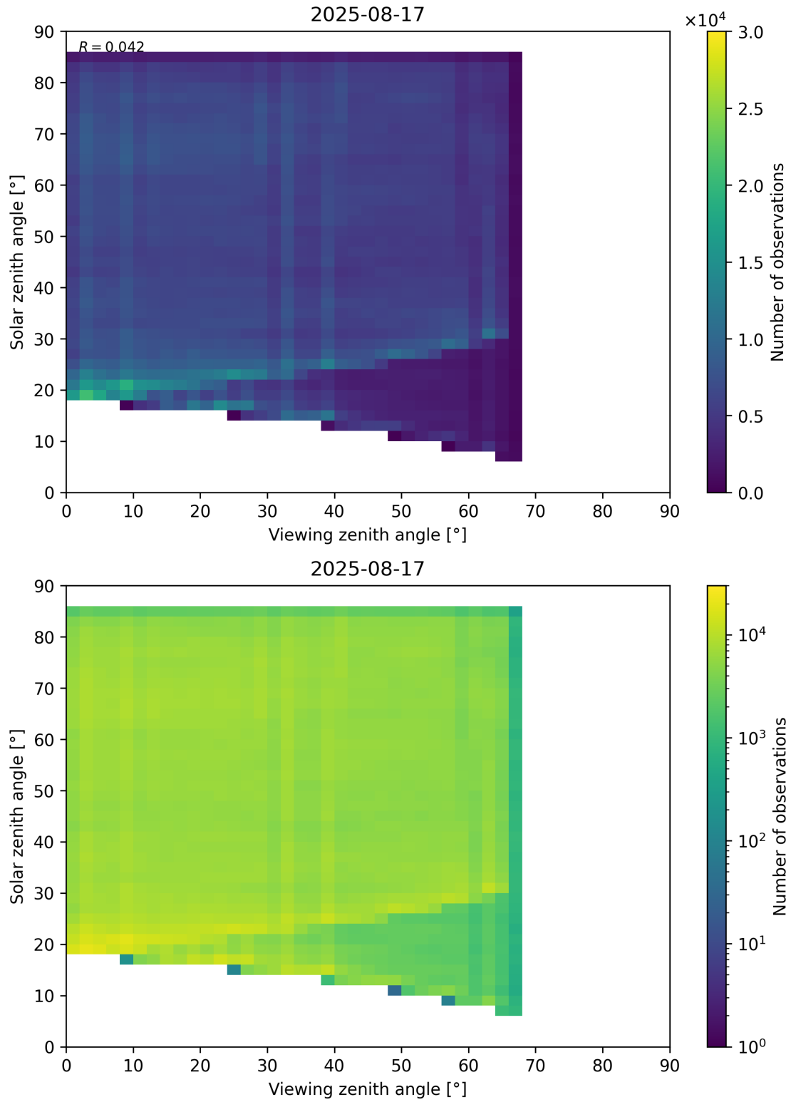
Figure 77: Scatter density plot of “Viewing zenith angle” against “Solar zenith angle” for 2025-08-16 to 2025-08-18.
