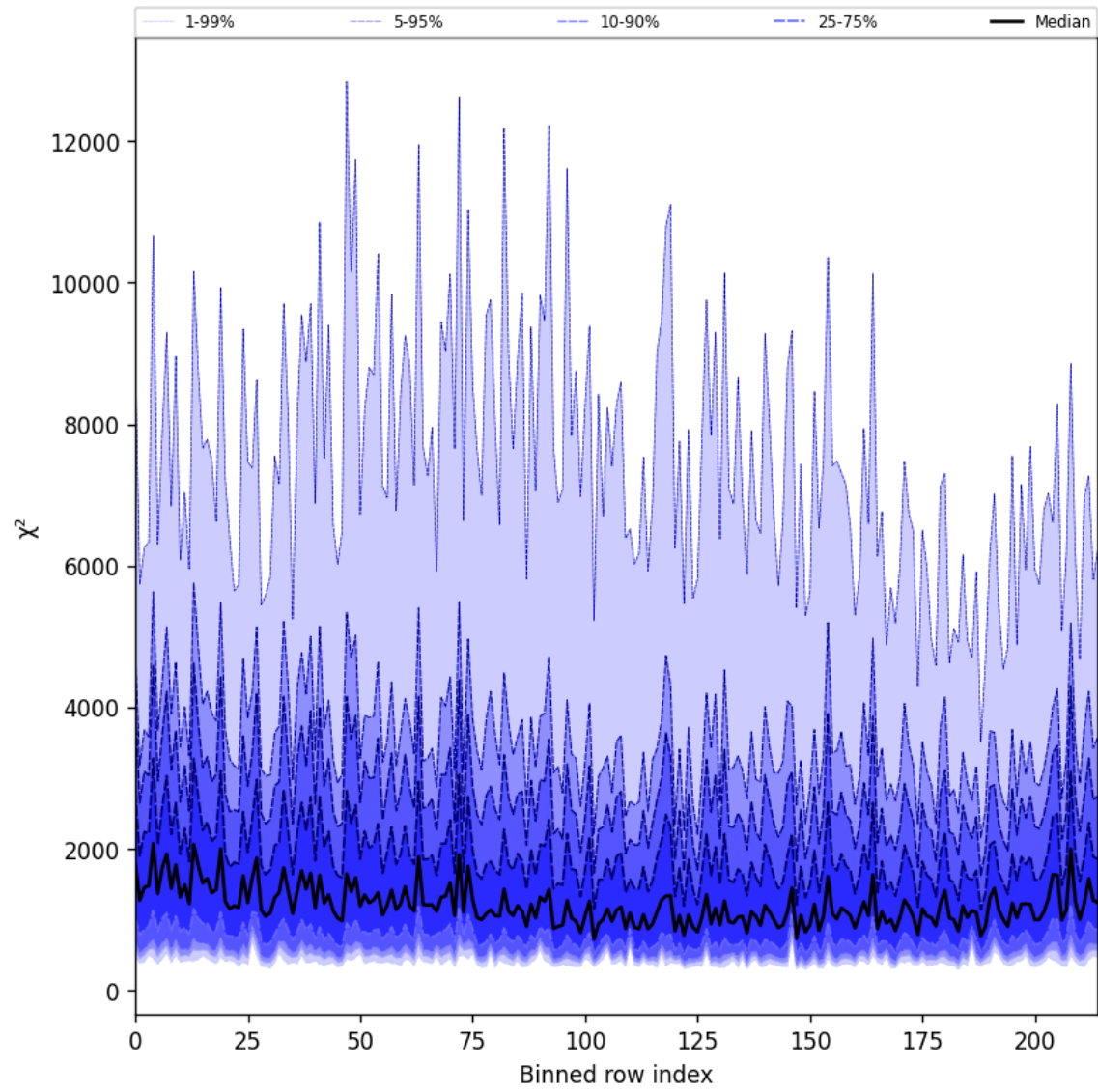
Figure 30: Along track statistics of “ \chi^2 ” for 2025-08-16 to 2025-08-18
