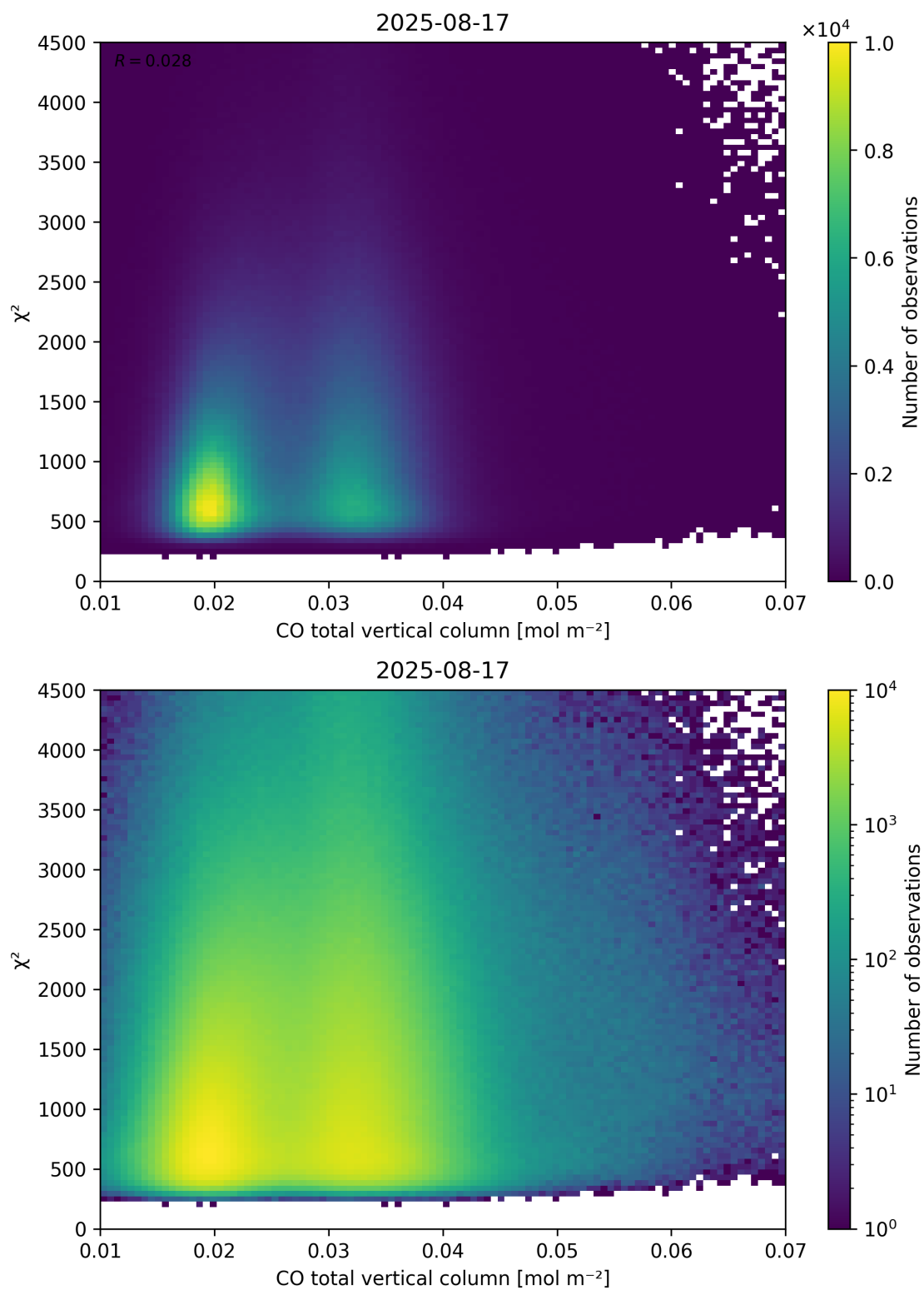
Figure 35: Scatter density plot of “CO total vertical column” against “ \chi^2 ” for 2025-08-16 to 2025-08-18.
