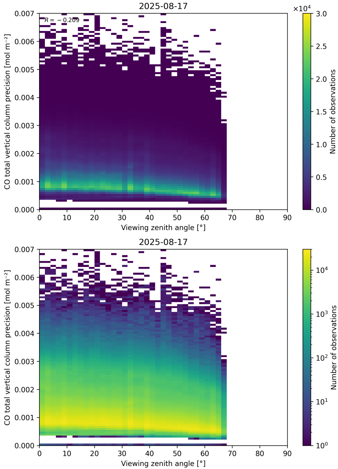
Figure 71: Scatter density plot of “Viewing zenith angle” against “CO total vertical column precision” for 2025-08-16 to 2025-08-18.
