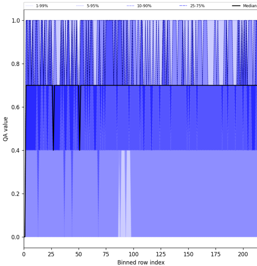
Figure 25: Along track statistics of “QA value” for 2025-08-16 to 2025-08-18
