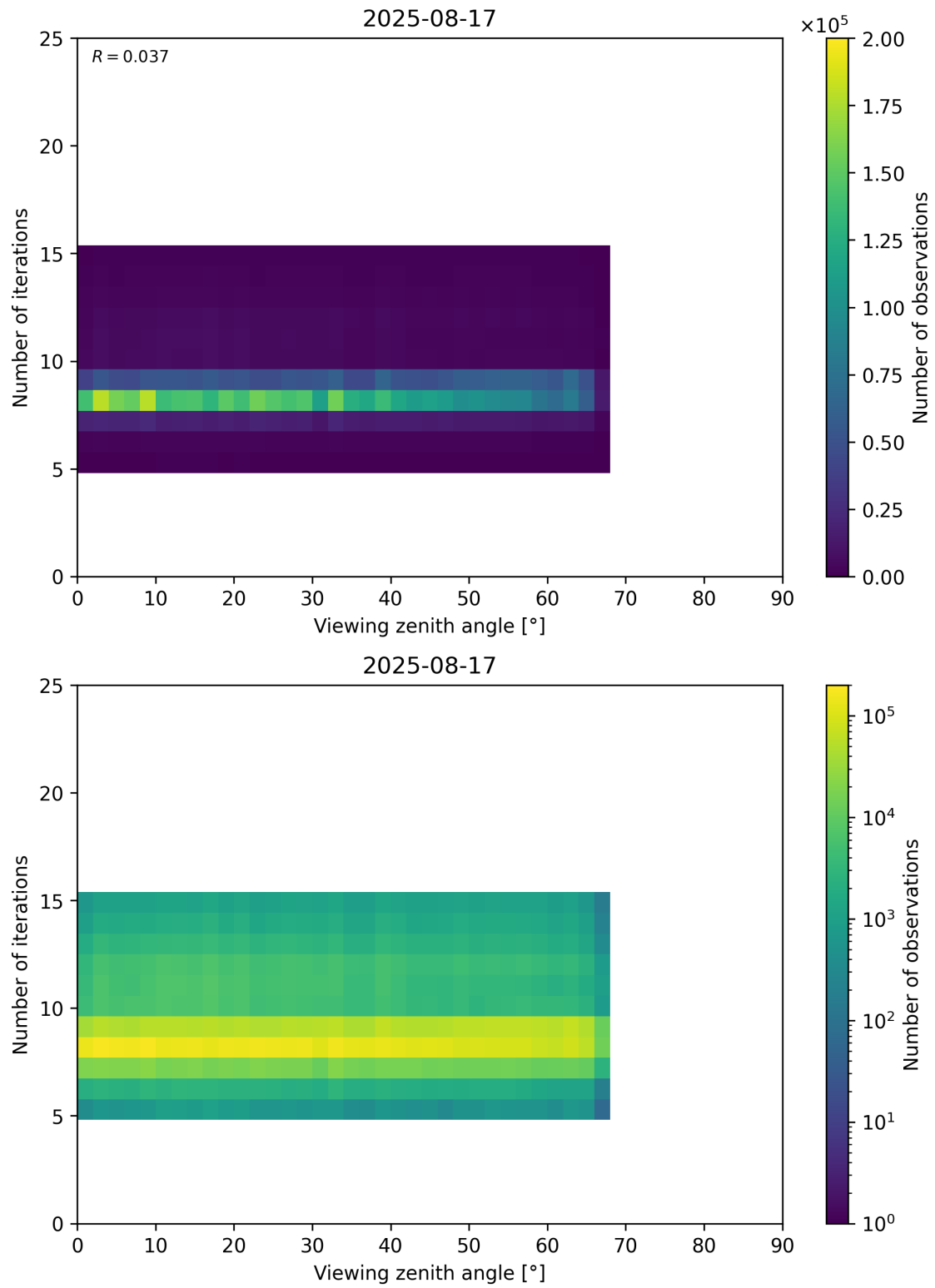
Figure 75: Scatter density plot of “Viewing zenith angle” against “Number of iterations” for 2025-08-16 to 2025-08-18.
