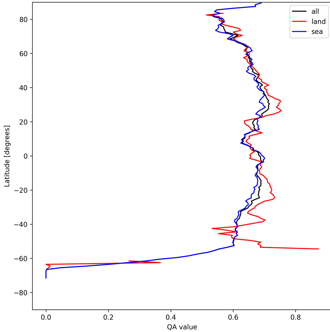
Figure 9: Zonal average of “QA value” for 2025-08-16 to 2025-08-18.
