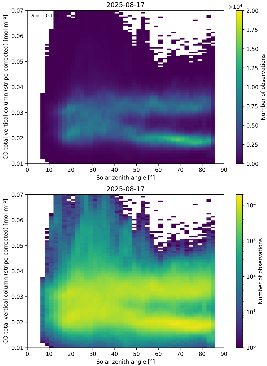
Figure 62: Scatter density plot of “Solar zenith angle” against “CO total vertical column (stripe-corrected)” for 2025-08-16 to 2025-08-18.
