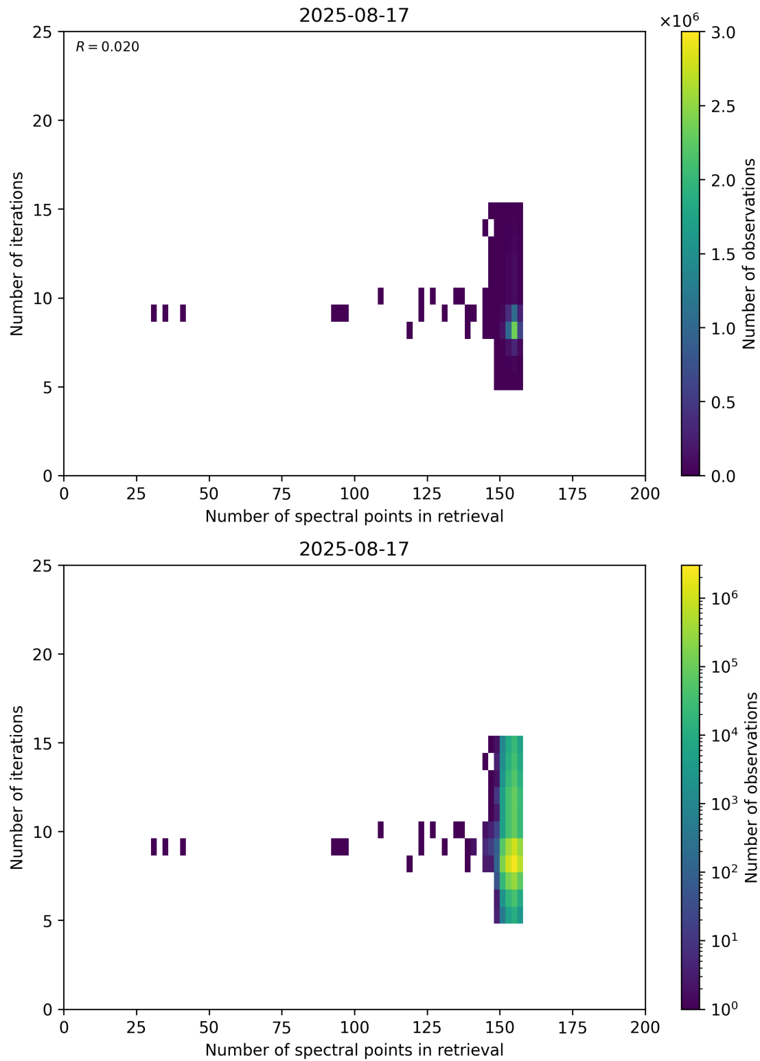
Figure 60: Scatter density plot of “Number of spectral points in retrieval” against “Number of iterations” for 2025-08-16 to 2025-08-18.
