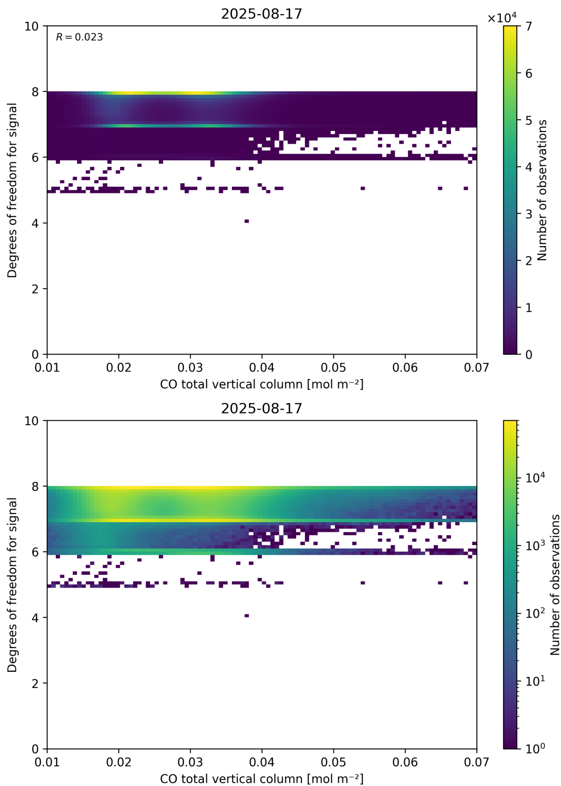
Figure 41: Scatter density plot of “CO total vertical column” against “Degrees of freedom for signal” for 2025-08-16 to 2025-08-18.
