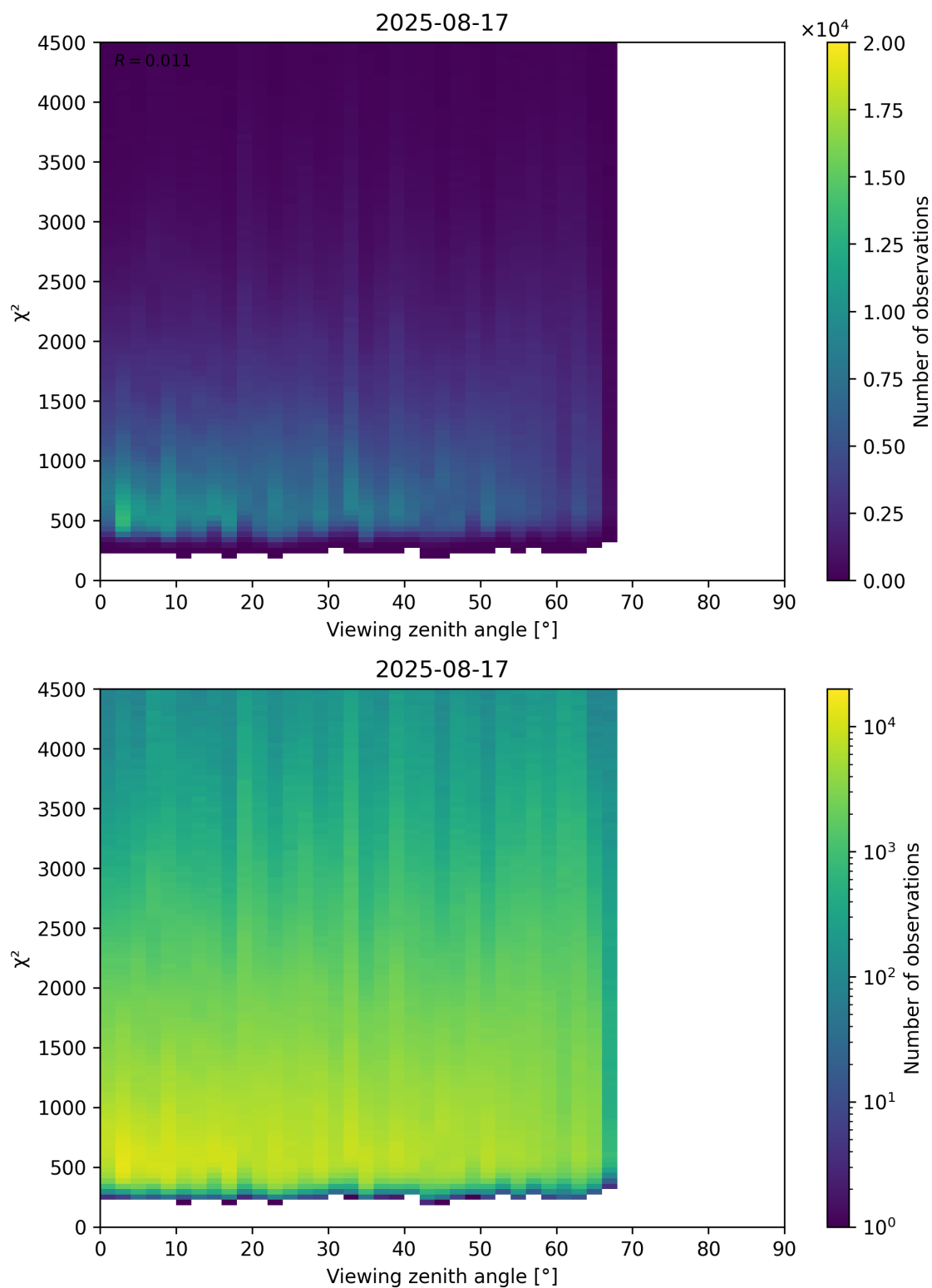
Figure 72: Scatter density plot of “Viewing zenith angle” against “ \chi^2 ” for 2025-08-16 to 2025-08-18.
