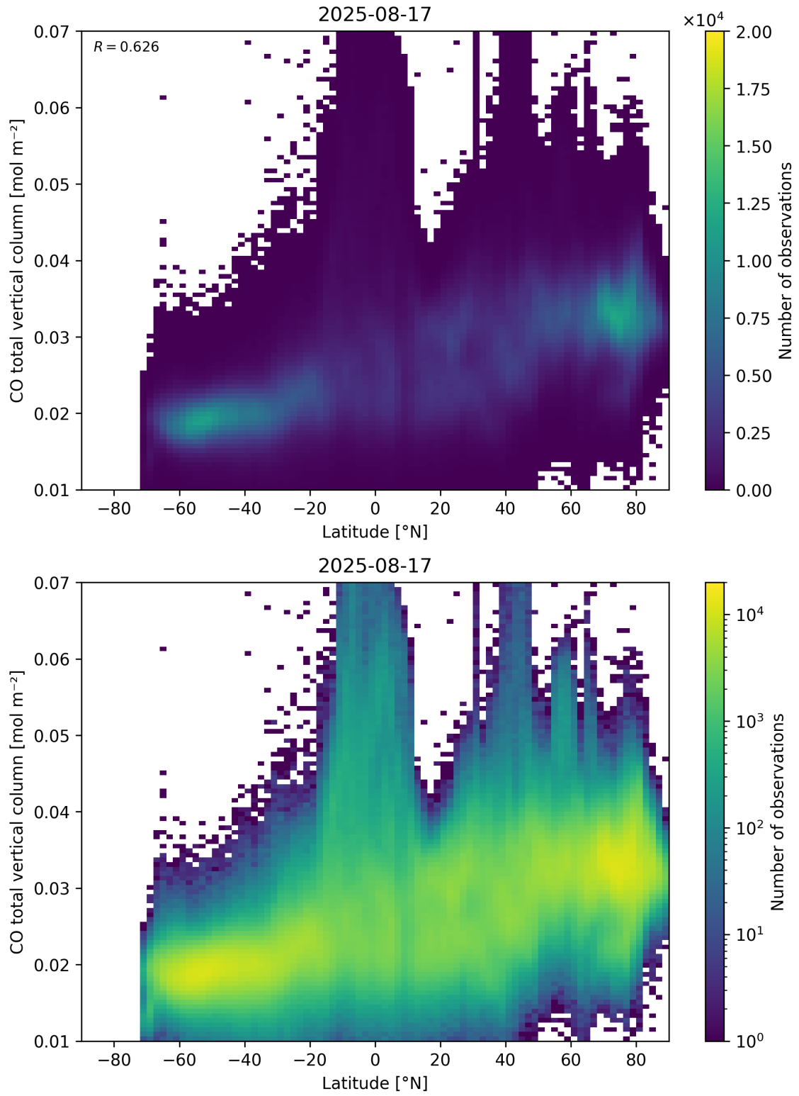
Figure 51: Scatter density plot of “Latitude” against “CO total vertical column” for 2025-08-16 to 2025-08-18.
