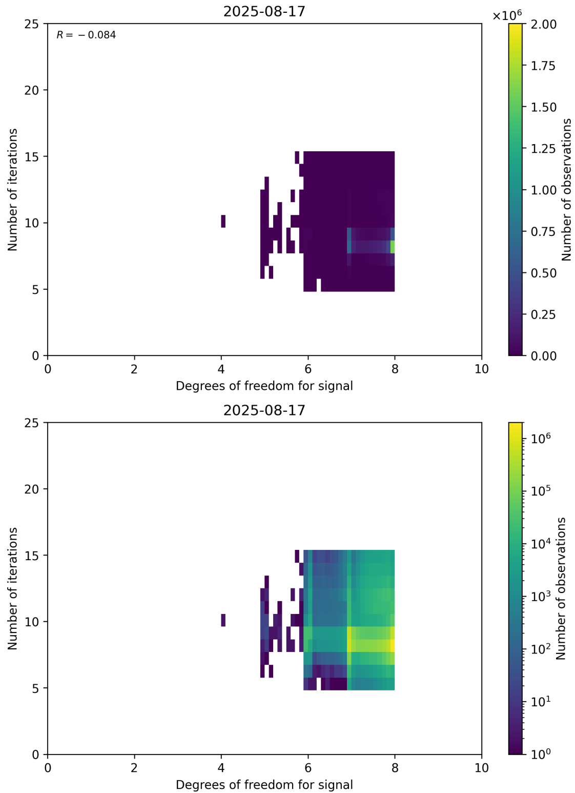
Figure 50: Scatter density plot of “Degrees of freedom for signal” against “Number of iterations” for 2025-08-16 to 2025-08-18.
