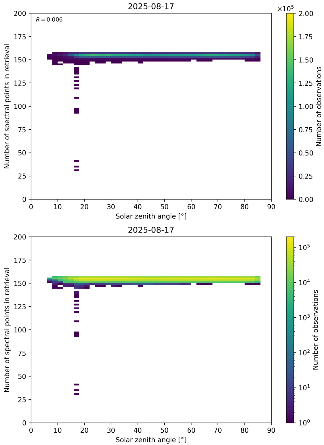
Figure 68: Scatter density plot of “Solar zenith angle” against “Number of spectral points in retrieval” for 2025-08-16 to 2025-08-18.
