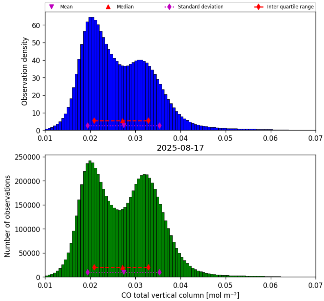
Figure 18: Histogram of “CO total vertical column” for 2025-08-16 to 2025-08-18
