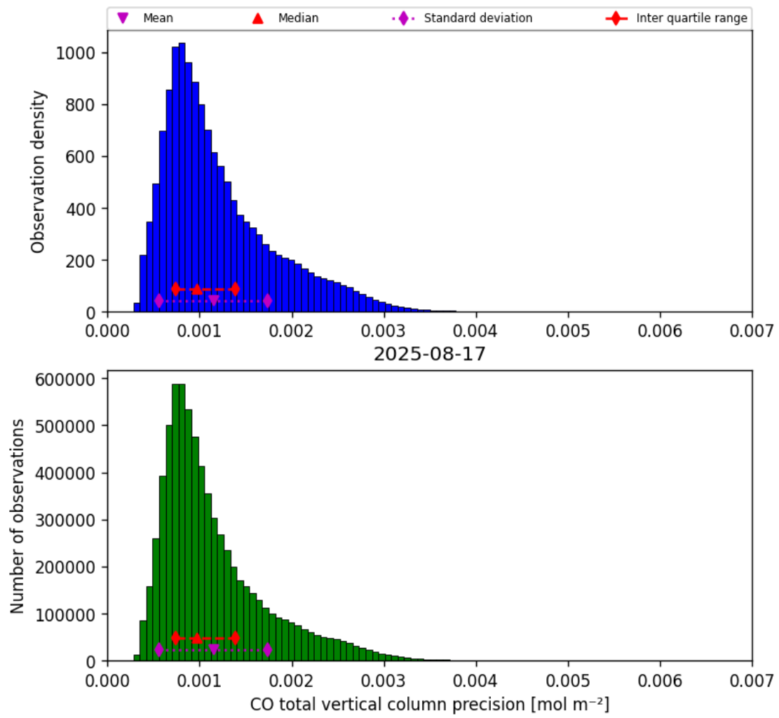
Figure 20: Histogram of “CO total vertical column precision” for 2025-08-16 to 2025-08-18
