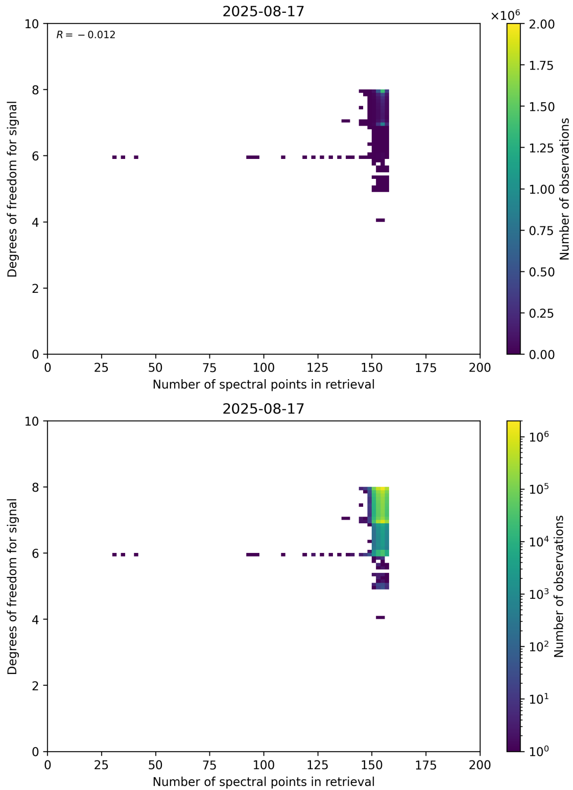
Figure 59: Scatter density plot of “Number of spectral points in retrieval” against “Degrees of freedom for signal” for 2025-08-16 to 2025-08-18.
