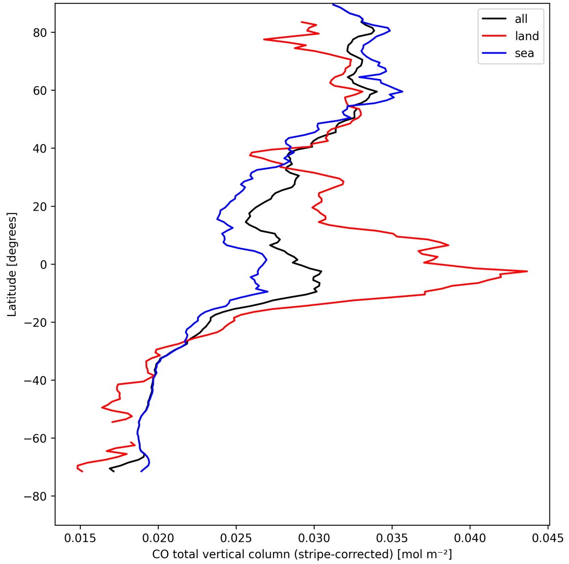
Figure 11: Zonal average of “CO total vertical column (stripe-corrected)” for 2025-08-16 to 2025-08-18.
