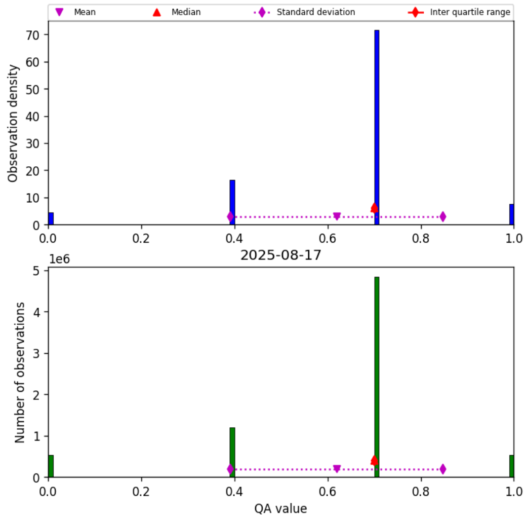
Figure 17: Histogram of “QA value” for 2025-08-16 to 2025-08-18
