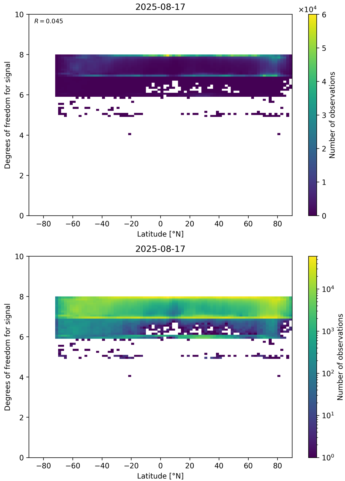
Figure 55: Scatter density plot of “Latitude” against “Degrees of freedom for signal” for 2025-08-16 to 2025-08-18.
