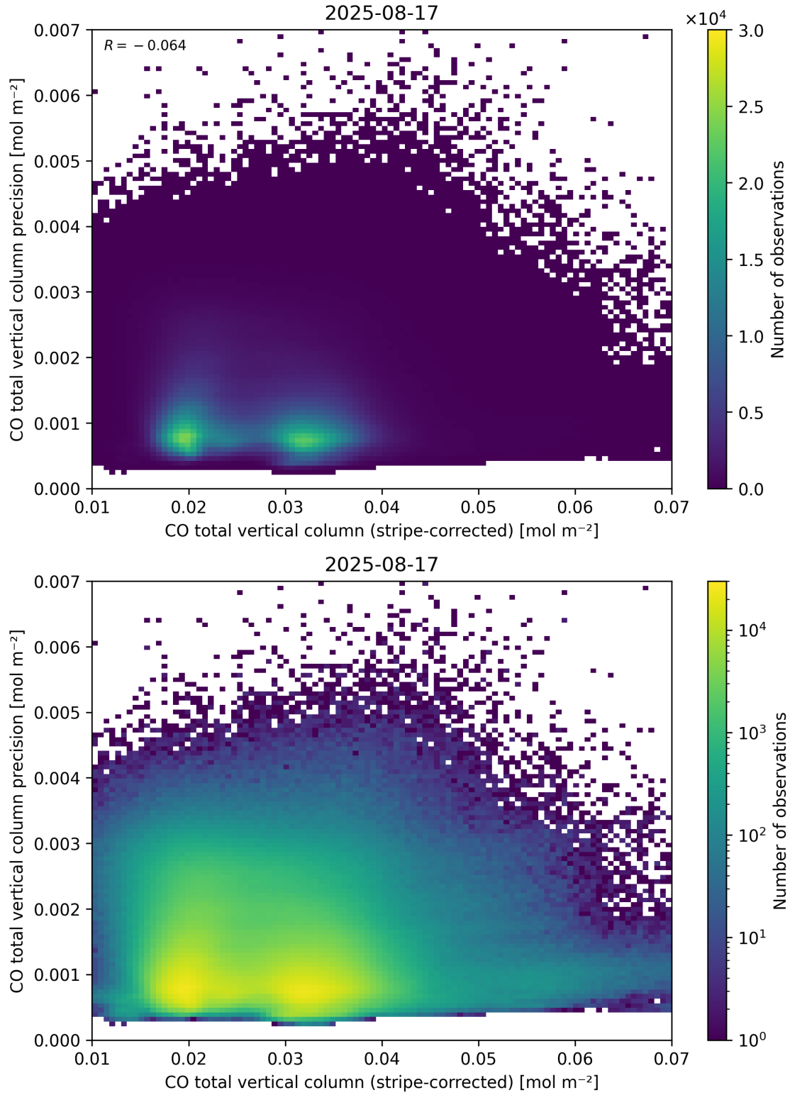
Figure 36: Scatter density plot of “CO total vertical column (stripe-corrected)” against “CO total vertical column precision” for 2025-08-16 to 2025-08-18.
