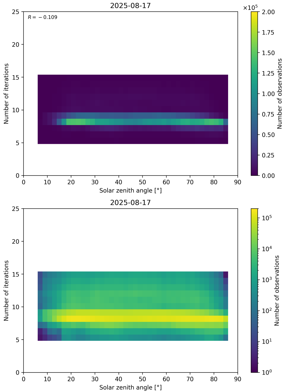
Figure 67: Scatter density plot of “Solar zenith angle” against “Number of iterations” for 2025-08-16 to 2025-08-18.
