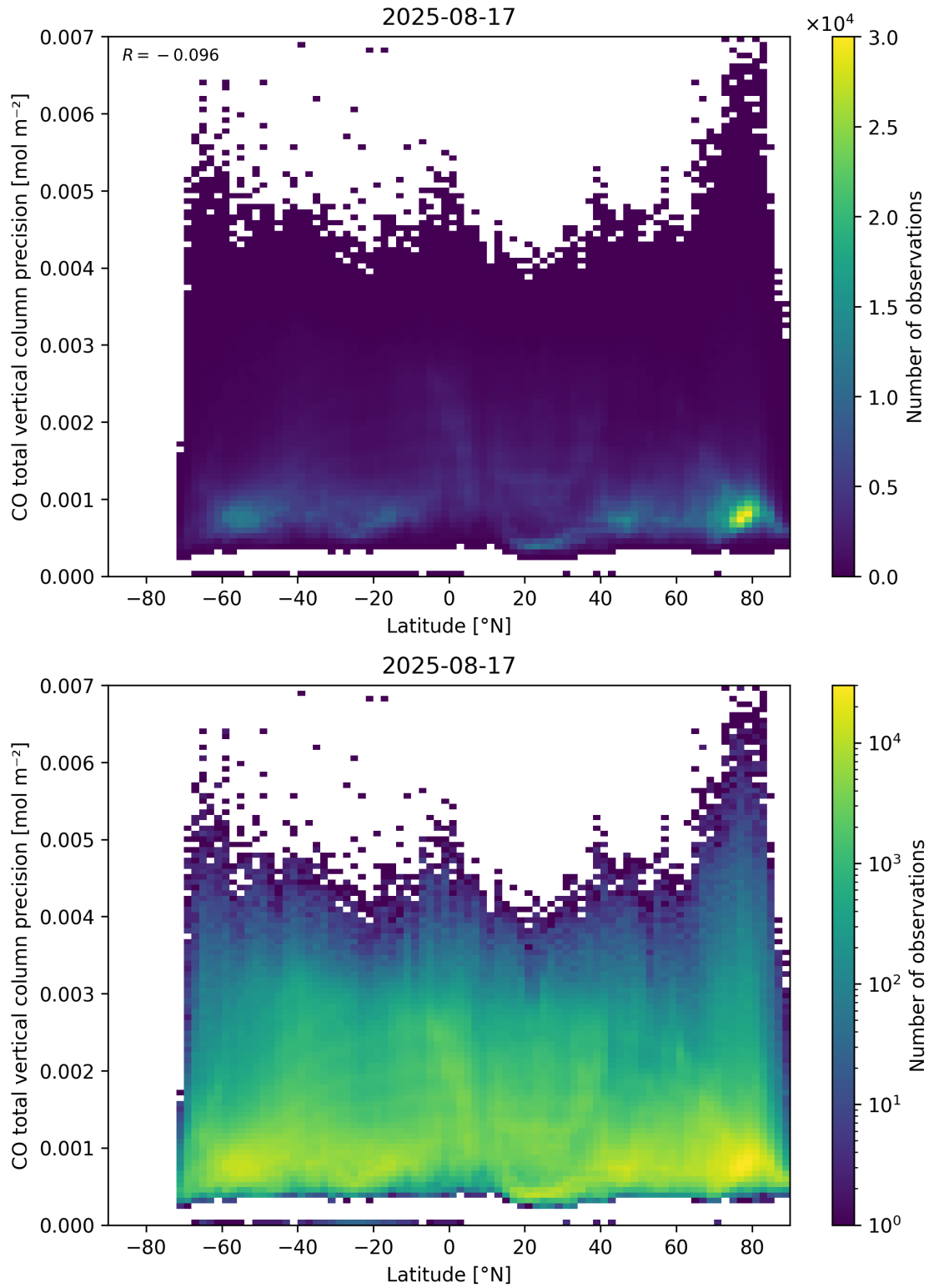
Figure 53: Scatter density plot of “Latitude” against “CO total vertical column precision” for 2025-08-16 to 2025-08-18.
