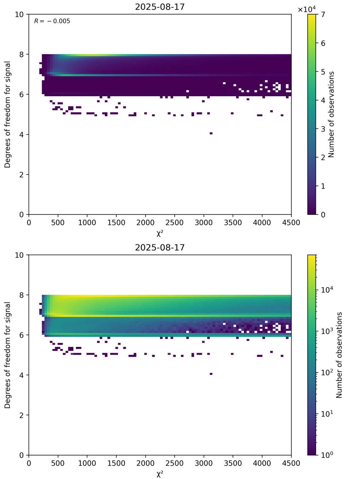
Figure 48: Scatter density plot of “ \chi^2 ” against “Degrees of freedom for signal” for 2025-08-16 to 2025-08-18.
