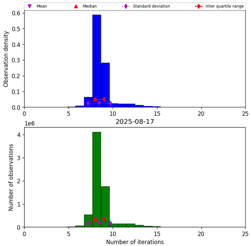
Figure 24: Histogram of “Number of iterations” for 2025-08-16 to 2025-08-18
