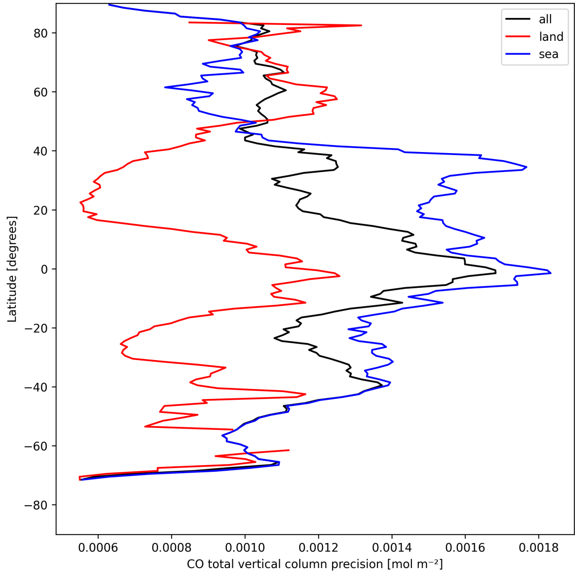
Figure 12: Zonal average of “CO total vertical column precision” for 2025-08-16 to 2025-08-18.
