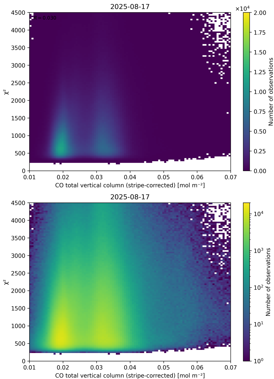
Figure 37: Scatter density plot of “CO total vertical column (stripe-corrected)” against “ \chi^2 ” for 2025-08-16 to 2025-08-18.
