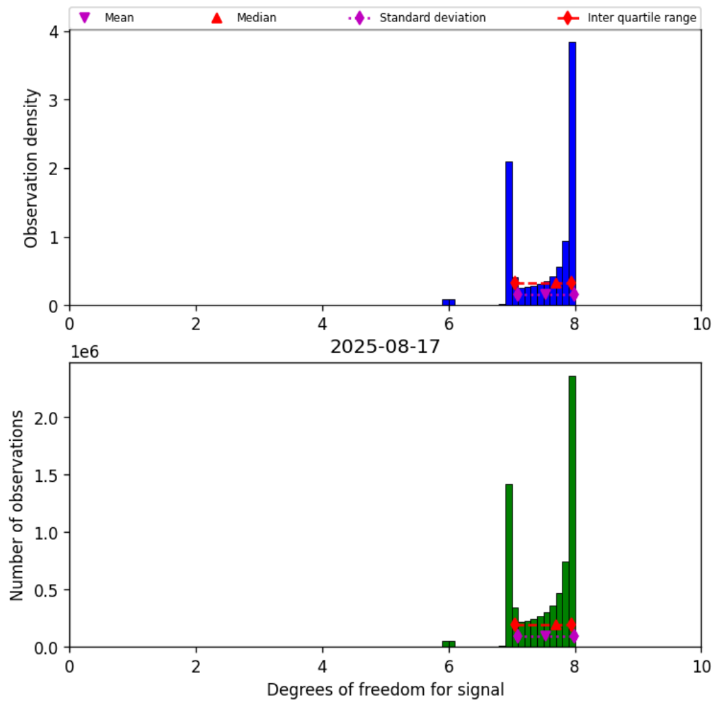
Figure 23: Histogram of “Degrees of freedom for signal” for 2025-08-16 to 2025-08-18
