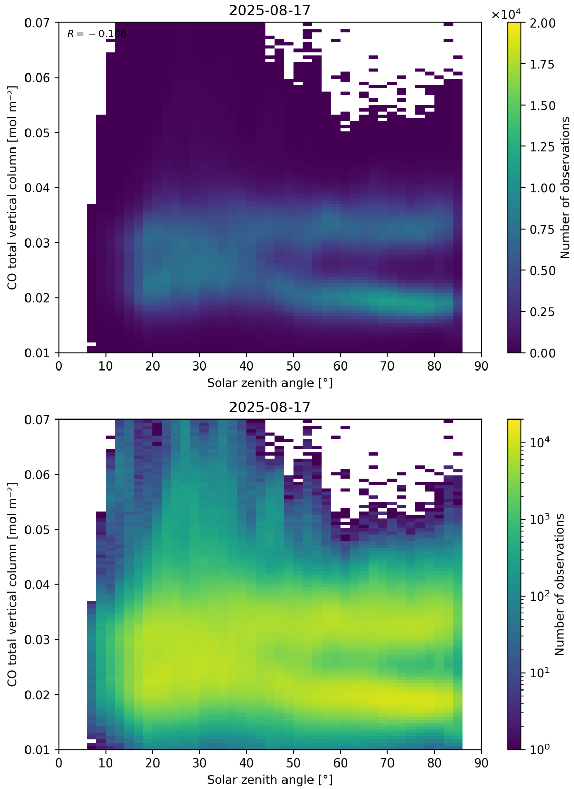
Figure 61: Scatter density plot of “Solar zenith angle” against “CO total vertical column” for 2025-08-16 to 2025-08-18.
