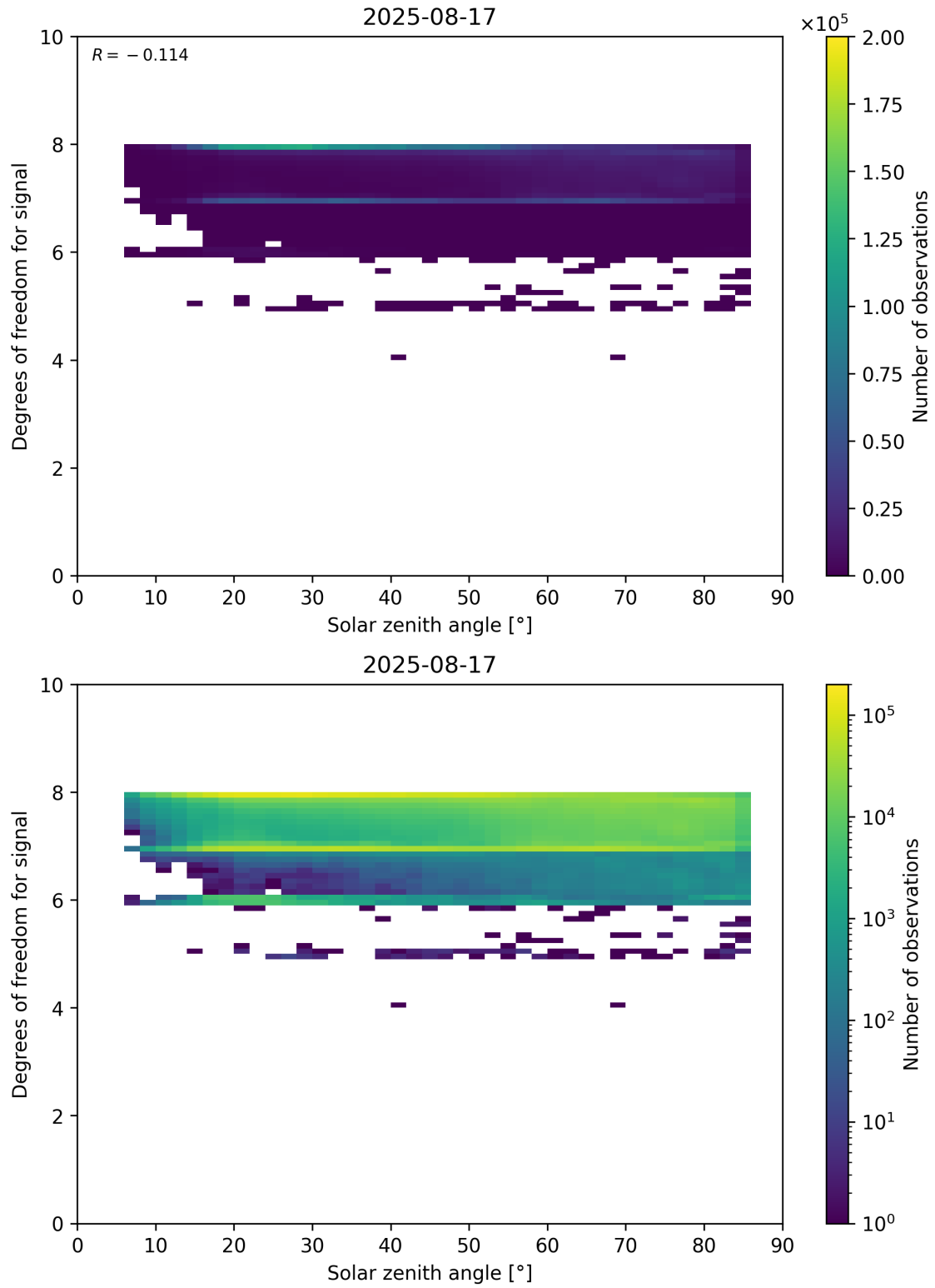
Figure 65: Scatter density plot of “Solar zenith angle” against “Degrees of freedom for signal” for 2025-08-16 to 2025-08-18.
