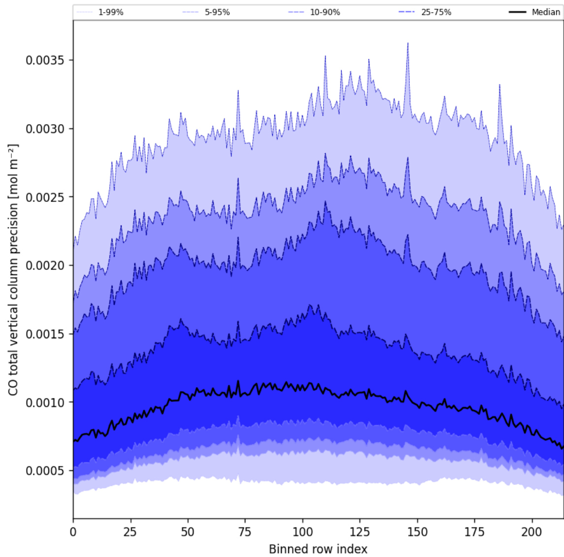
Figure 28: Along track statistics of “CO total vertical column precision” for 2025-08-16 to 2025-08-18
