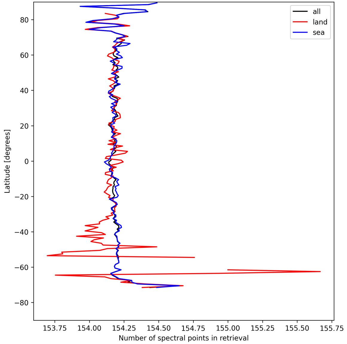
Figure 13: Zonal average of “Number of spectral points in retrieval” for 2025-08-16 to 2025-08-18.
