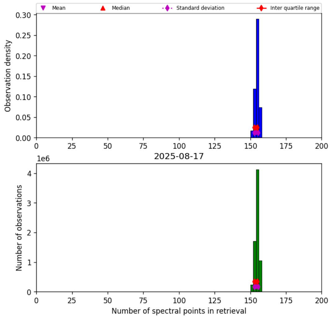
Figure 21: Histogram of “Number of spectral points in retrieval” for 2025-08-16 to 2025-08-18
