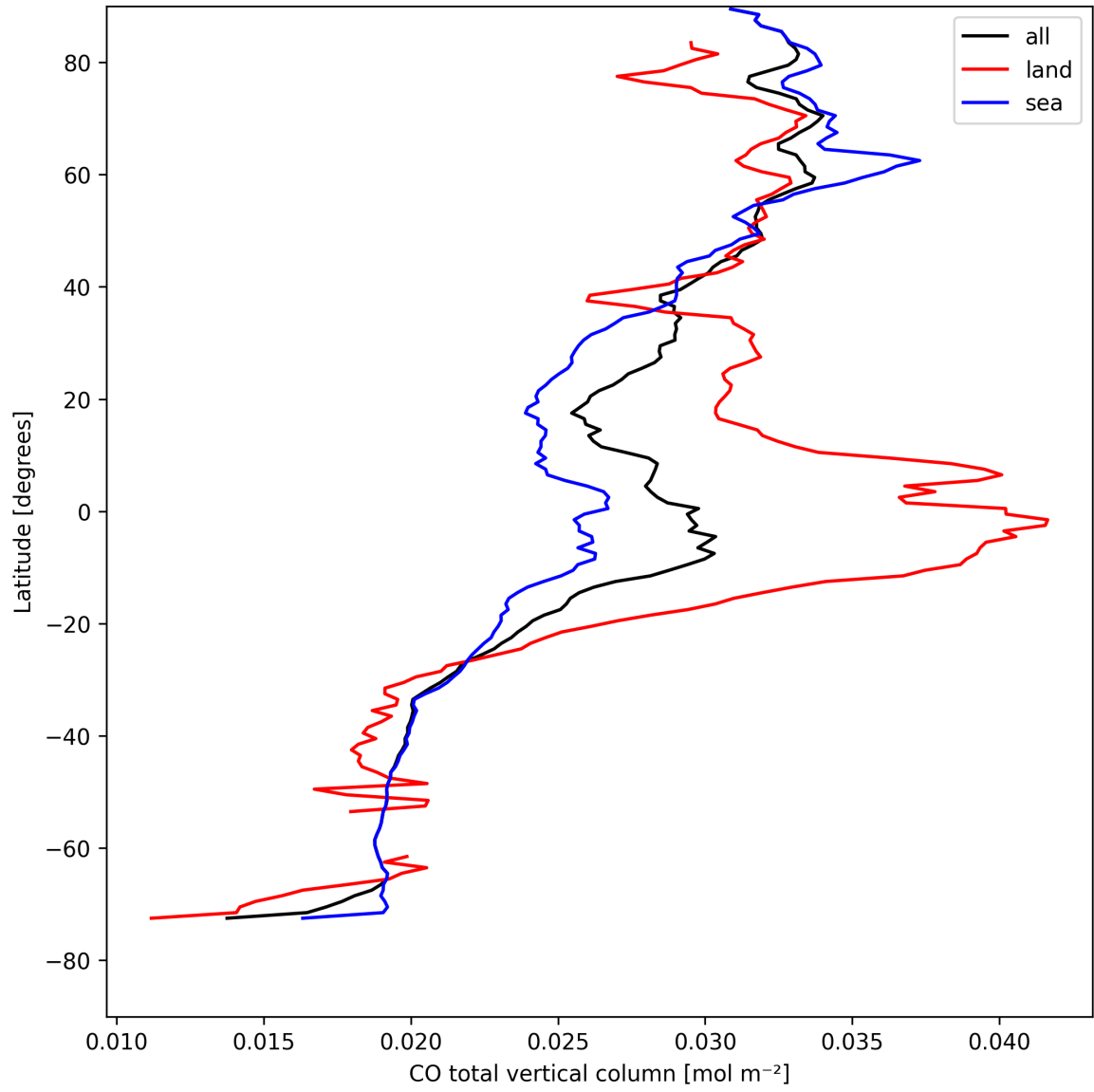
Figure 10: Zonal average of “CO total vertical column” for 2025-08-17 to 2025-08-19.
