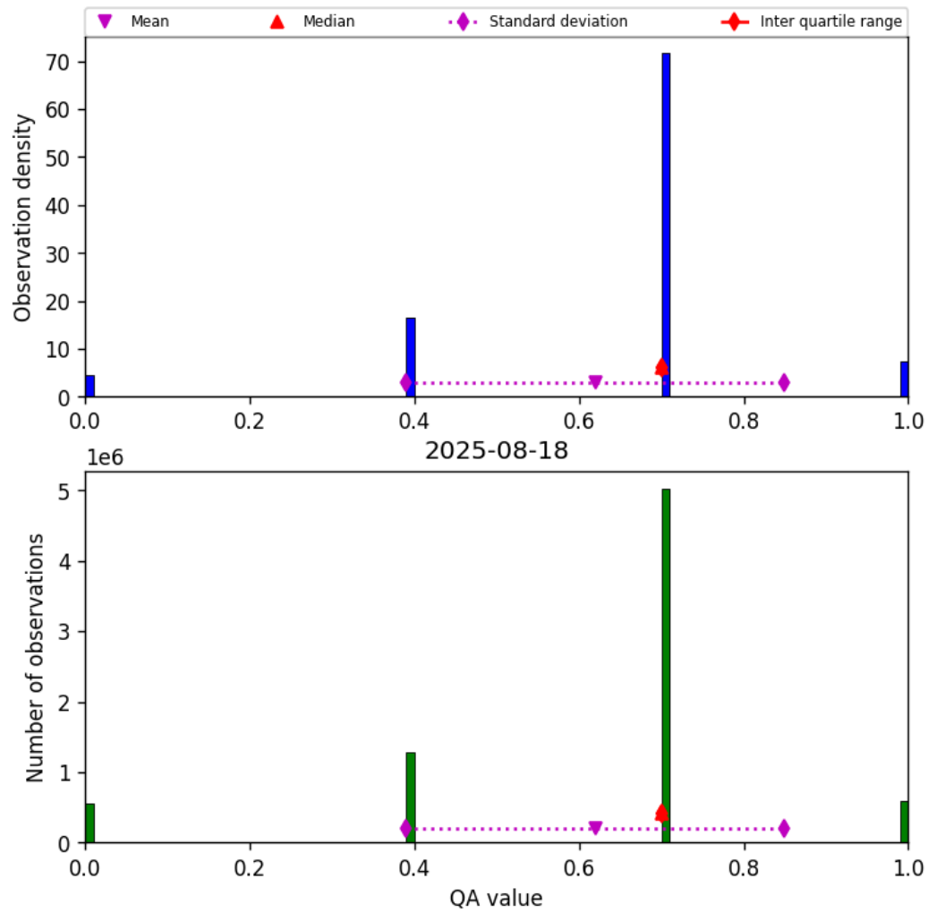
Figure 17: Histogram of “QA value” for 2025-08-17 to 2025-08-19
