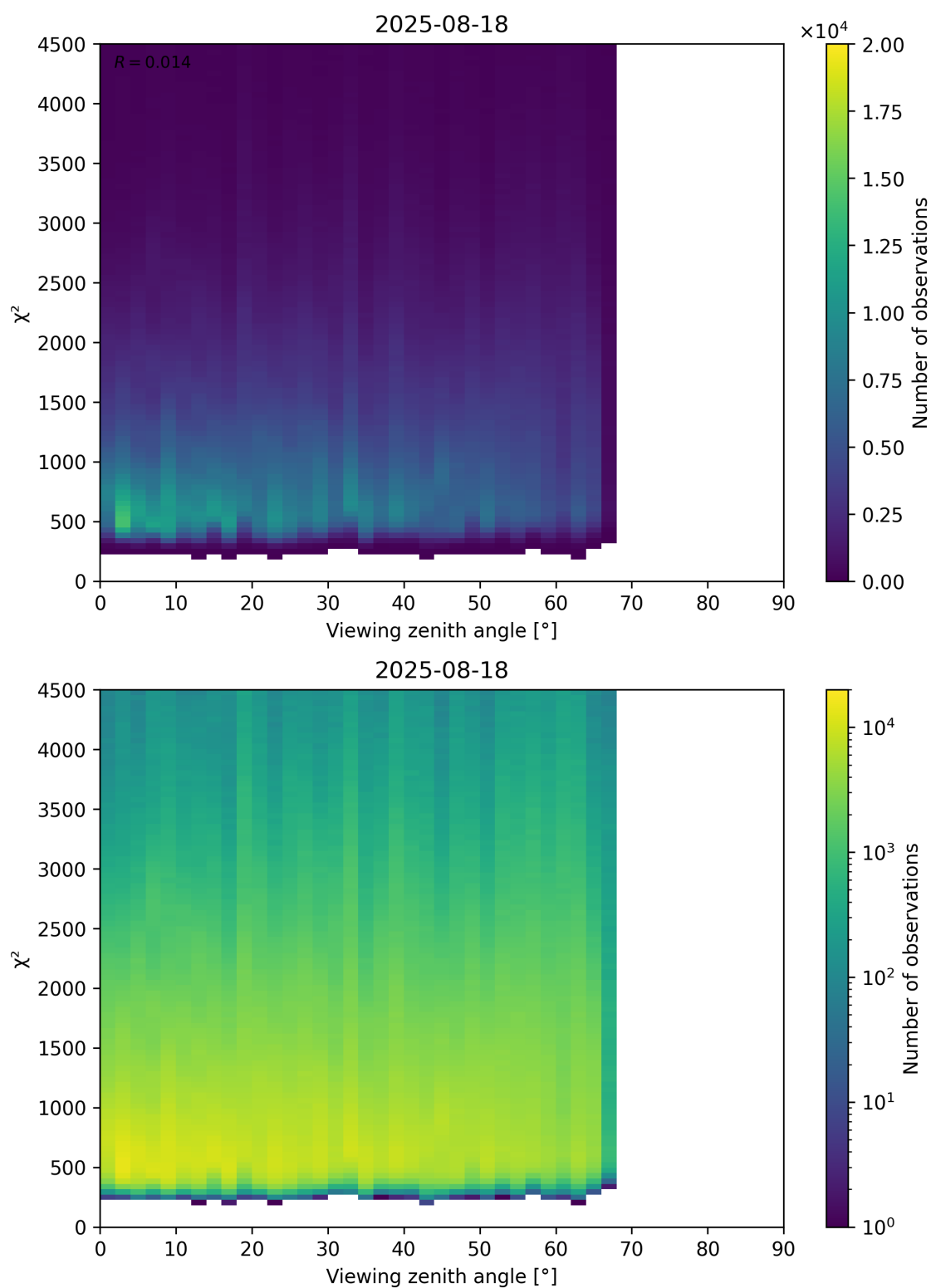
Figure 72: Scatter density plot of “Viewing zenith angle” against “ \chi^2 ” for 2025-08-17 to 2025-08-19.
