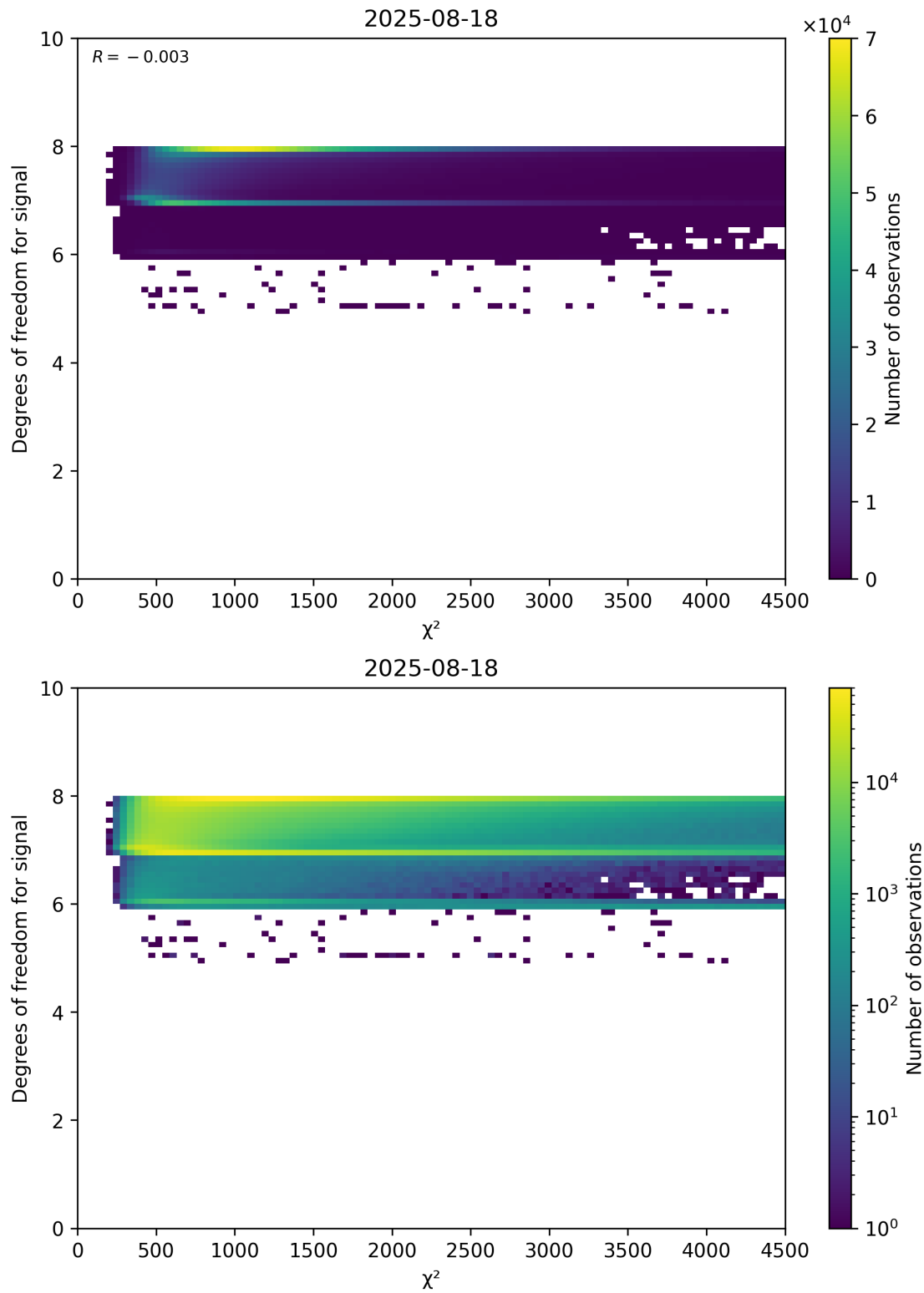
Figure 48: Scatter density plot of “ \chi^2 ” against “Degrees of freedom for signal” for 2025-08-17 to 2025-08-19.
