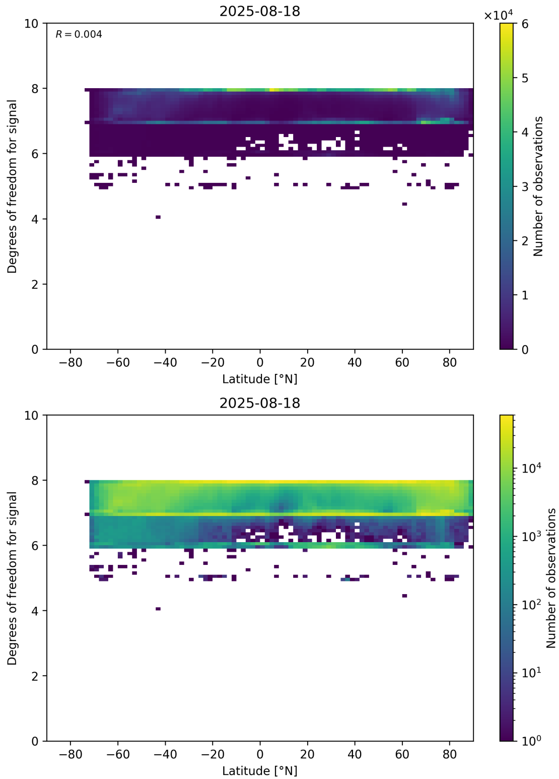
Figure 55: Scatter density plot of “Latitude” against “Degrees of freedom for signal” for 2025-08-17 to 2025-08-19.
