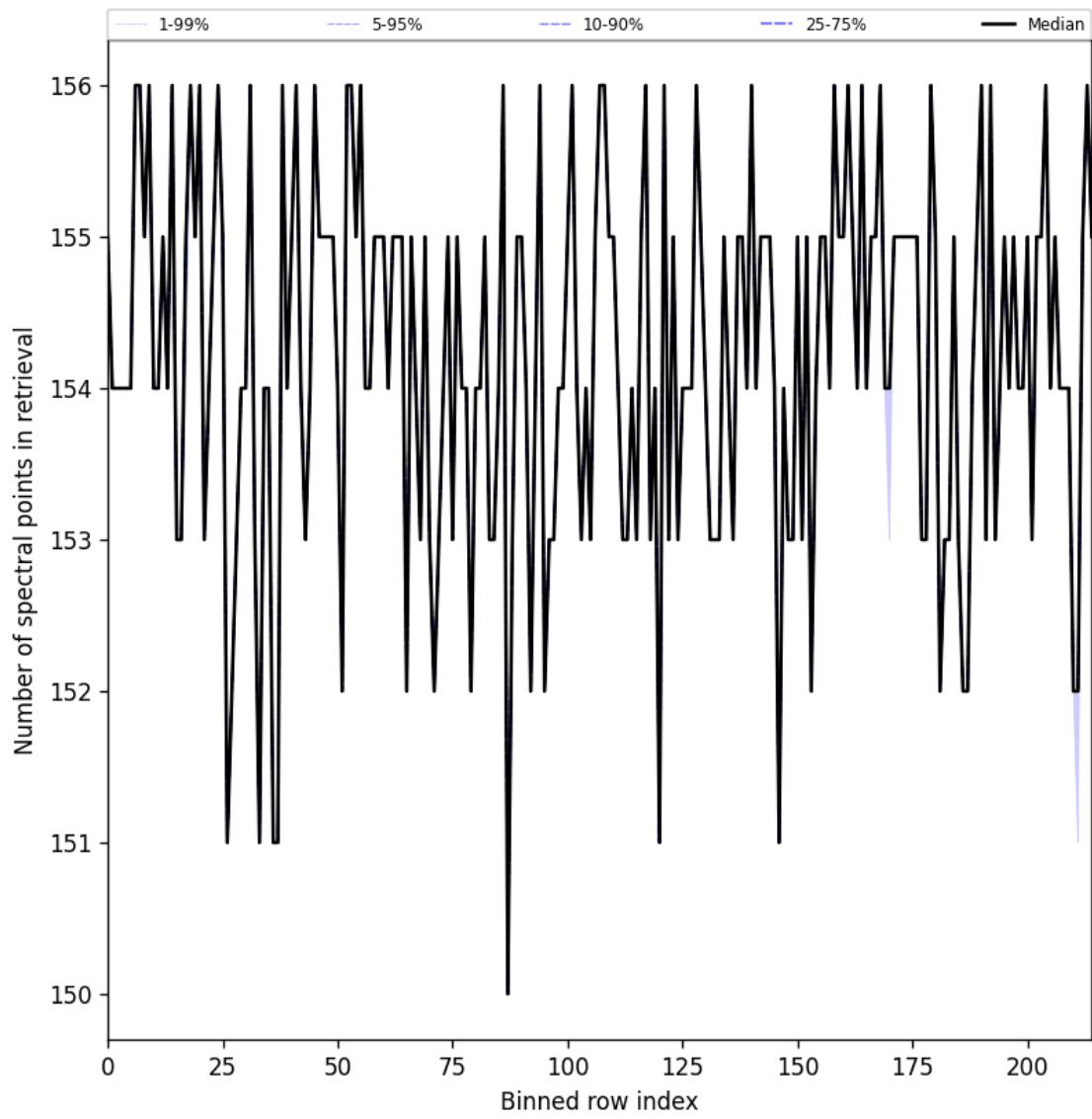
Figure 29: Along track statistics of “Number of spectral points in retrieval” for 2025-08-17 to 2025-08-19
