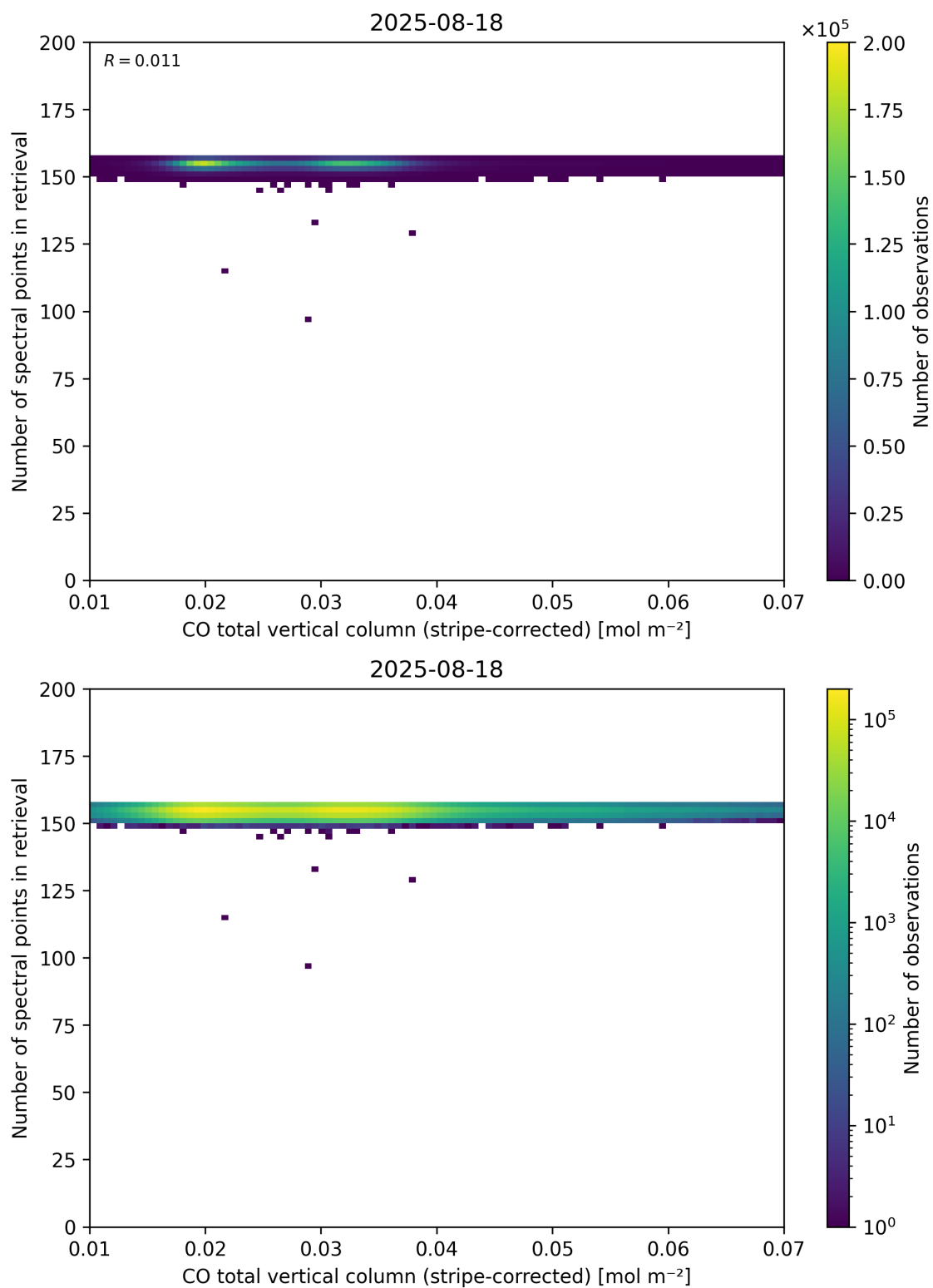
Figure 40: Scatter density plot of “CO total vertical column (stripe-corrected)” against “Number of spectral points in retrieval” for 2025-08-17 to 2025-08-19.
