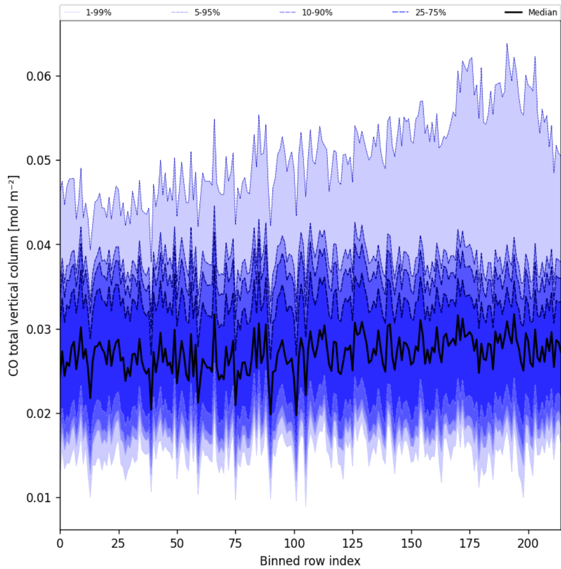
Figure 26: Along track statistics of “CO total vertical column” for 2025-08-17 to 2025-08-19
