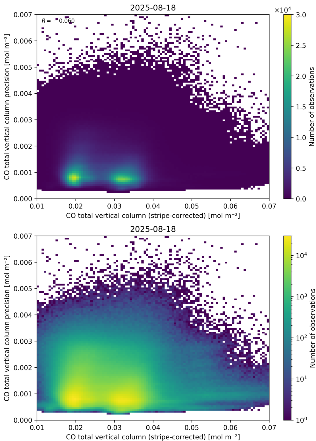
Figure 36: Scatter density plot of “CO total vertical column (stripe-corrected)” against “CO total vertical column precision” for 2025-08-17 to 2025-08-19.
