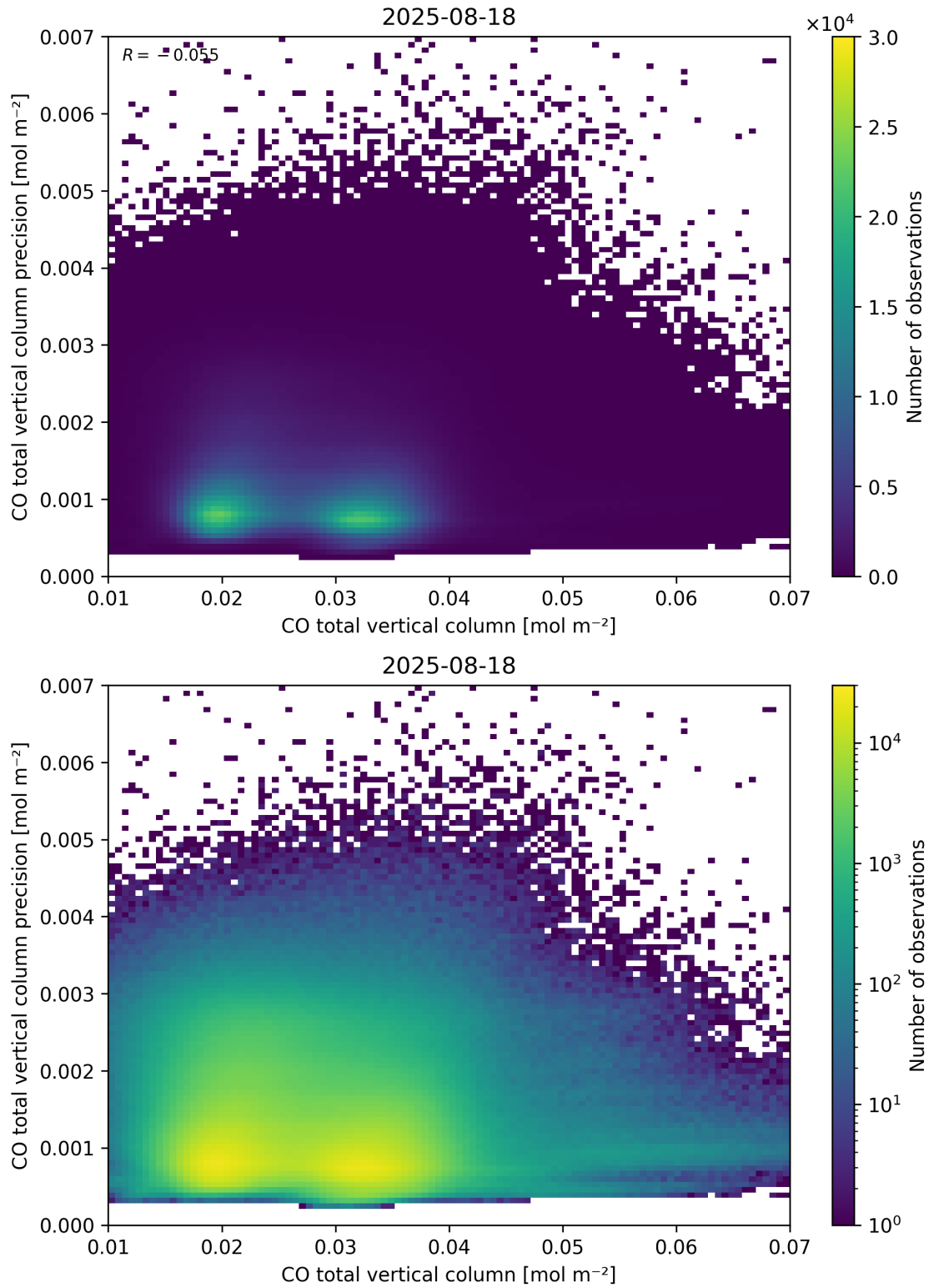
Figure 34: Scatter density plot of “CO total vertical column” against “CO total vertical column precision” for 2025-08-17 to 2025-08-19.
