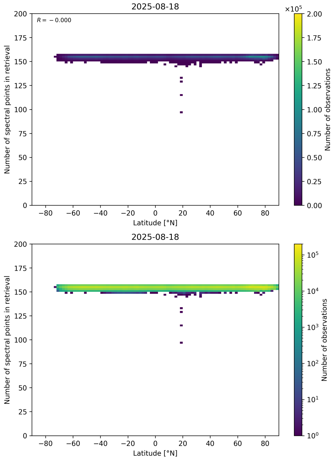
Figure 57: Scatter density plot of “Latitude” against “Number of spectral points in retrieval” for 2025-08-17 to 2025-08-19.
