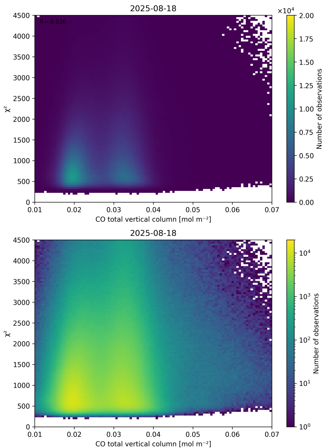
Figure 35: Scatter density plot of “CO total vertical column” against “ \chi^2 ” for 2025-08-17 to 2025-08-19.
