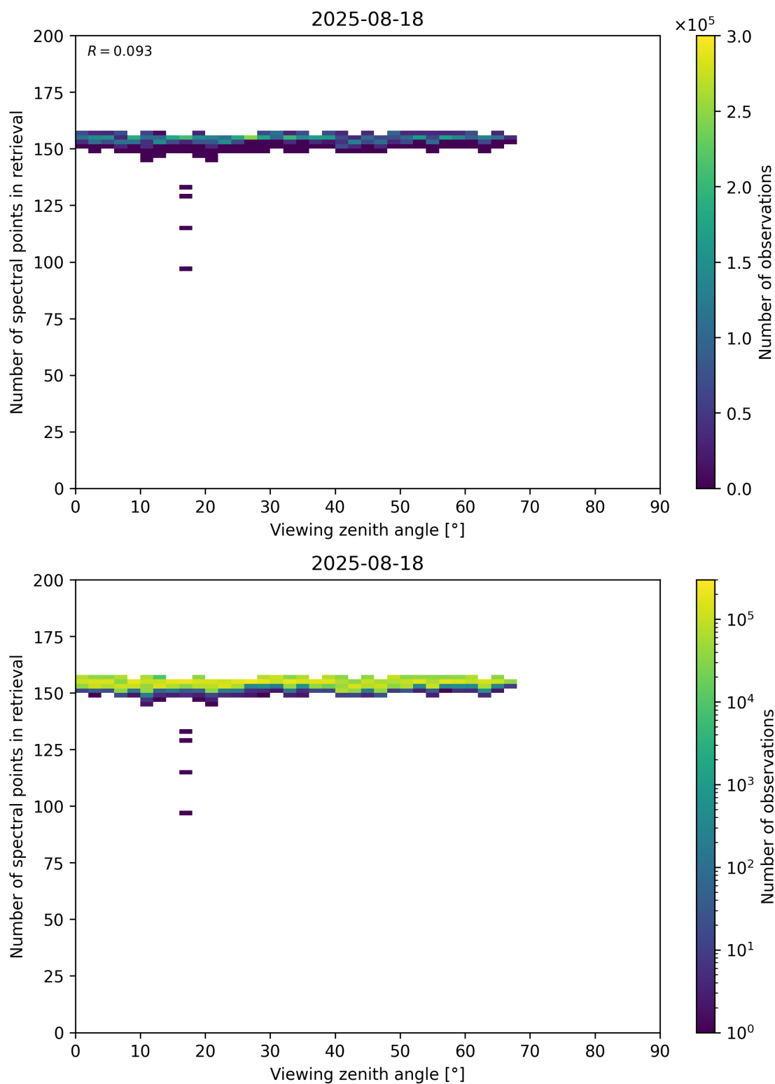
Figure 76: Scatter density plot of “Viewing zenith angle” against “Number of spectral points in retrieval” for 2025-08-17 to 2025-08-19.
