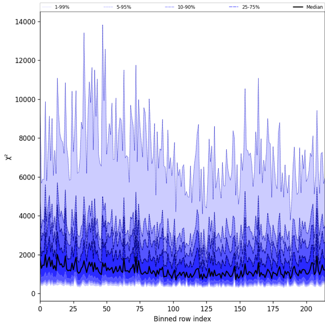
Figure 30: Along track statistics of “ \chi^2 ” for 2025-08-17 to 2025-08-19
