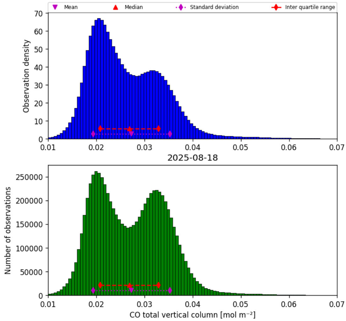
Figure 18: Histogram of “CO total vertical column” for 2025-08-17 to 2025-08-19
