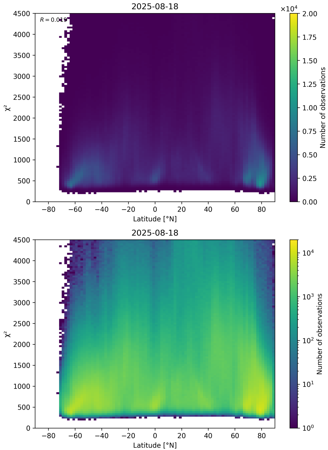
Figure 54: Scatter density plot of “Latitude” against “ \chi^2 ” for 2025-08-17 to 2025-08-19.
