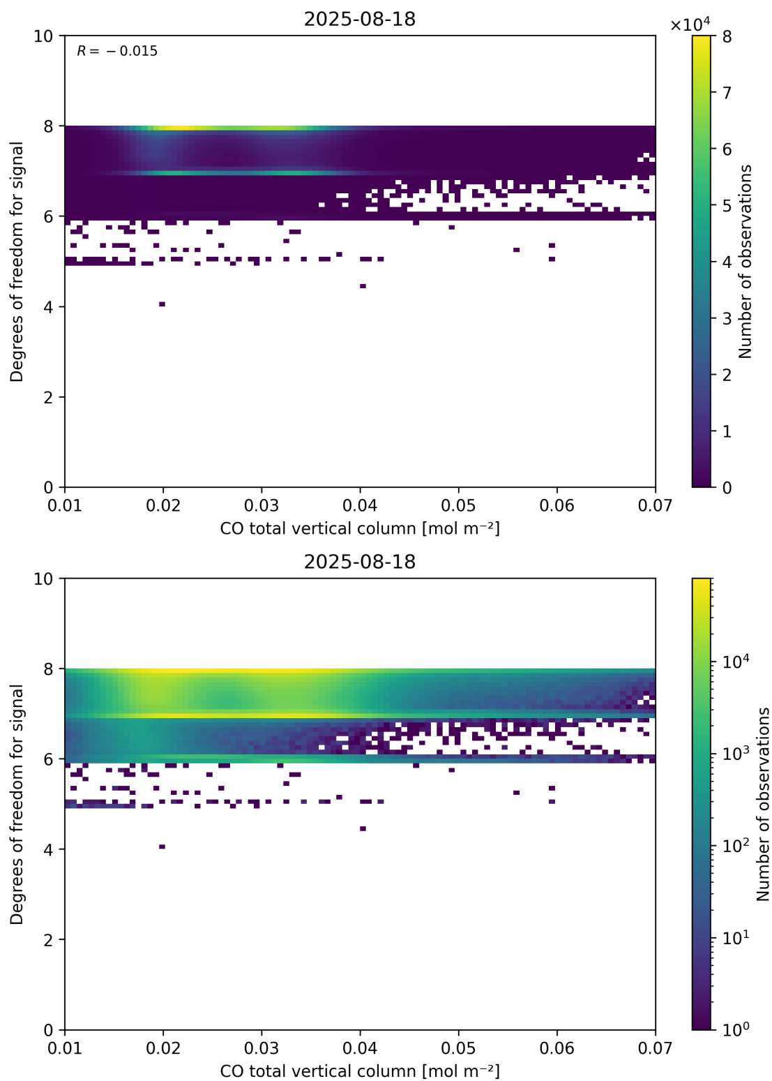
Figure 41: Scatter density plot of “CO total vertical column” against “Degrees of freedom for signal” for 2025-08-17 to 2025-08-19.
