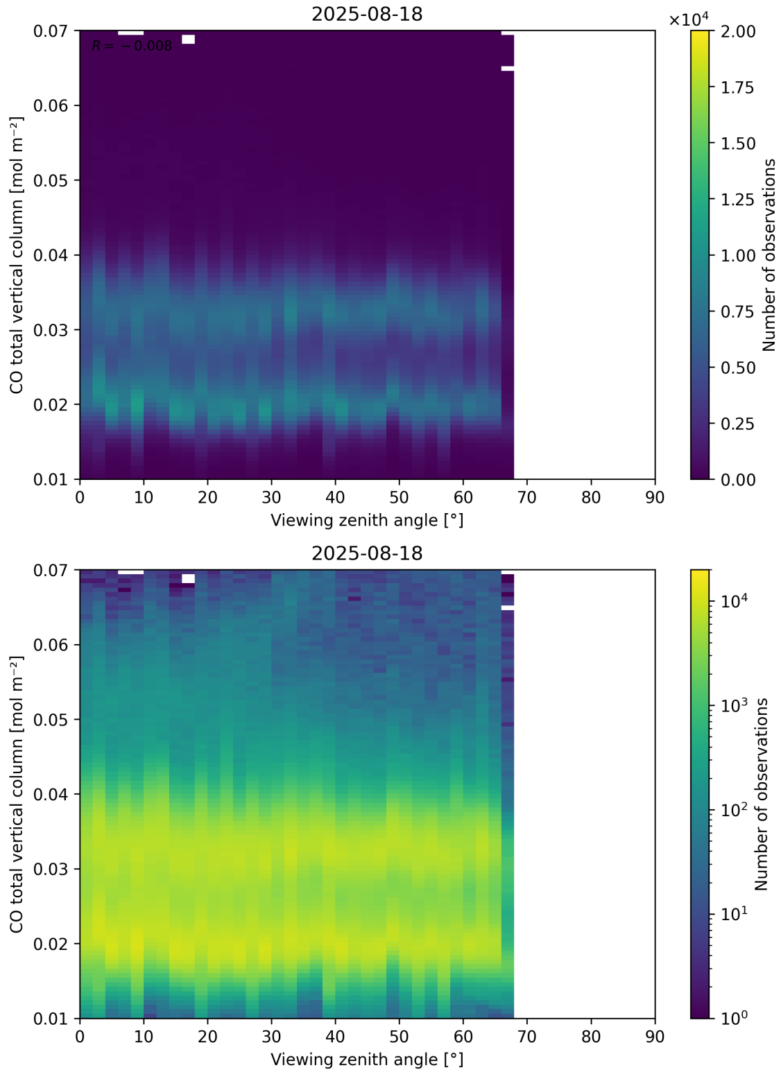
Figure 69: Scatter density plot of “Viewing zenith angle” against “CO total vertical column” for 2025-08-17 to 2025-08-19.
