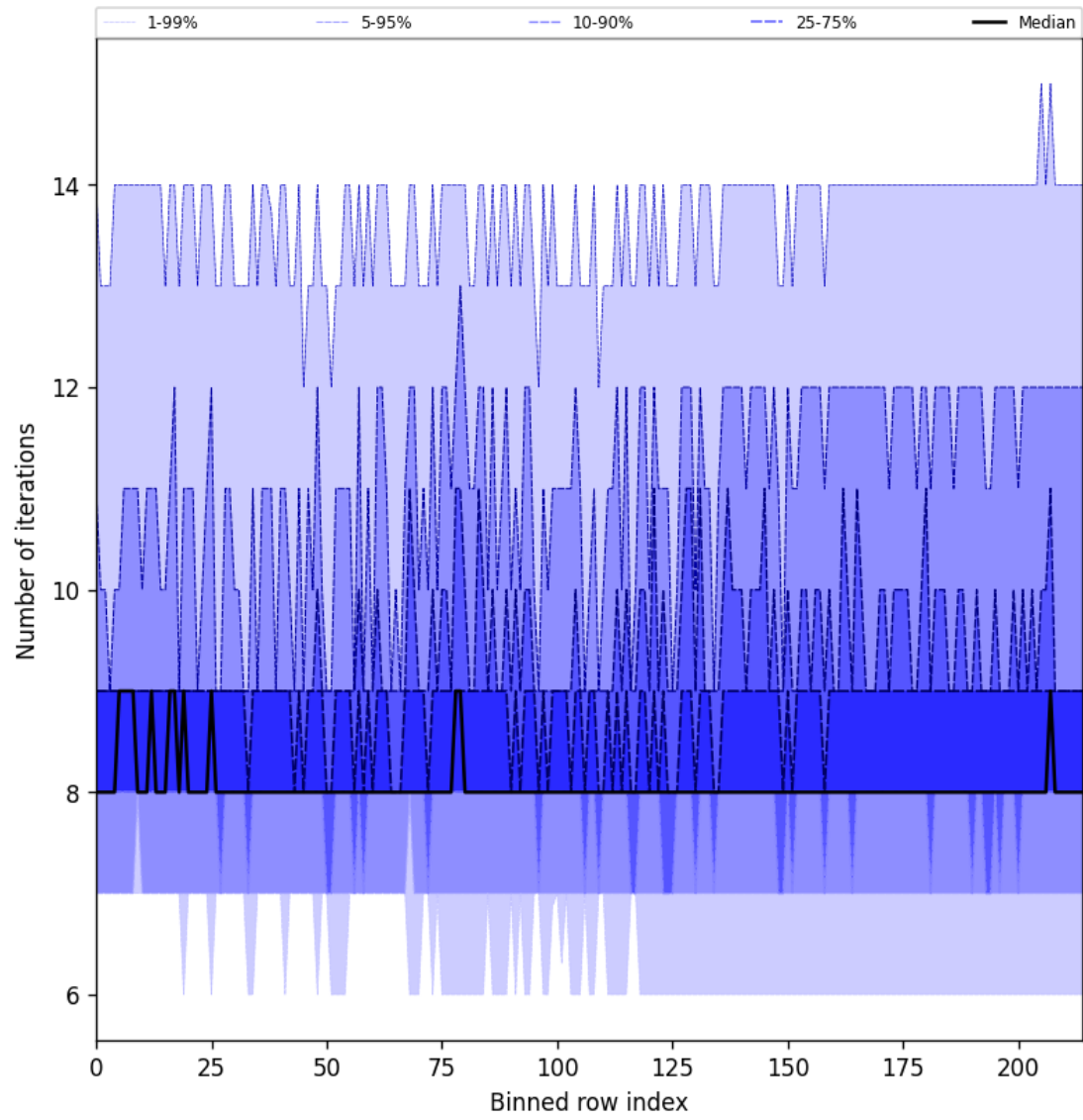
Figure 32: Along track statistics of “Number of iterations” for 2025-08-17 to 2025-08-19
