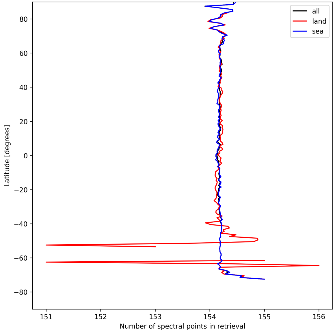
Figure 13: Zonal average of “Number of spectral points in retrieval” for 2025-08-17 to 2025-08-19.
