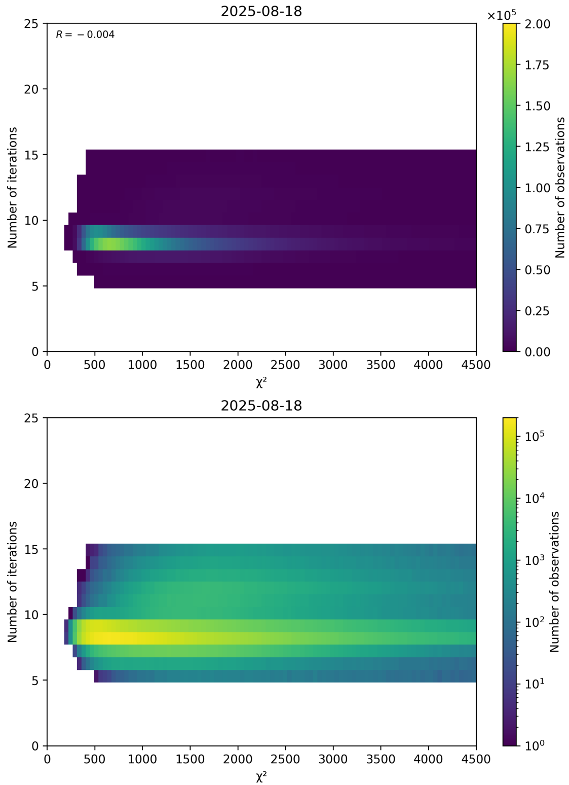
Figure 49: Scatter density plot of “ \chi^2 ” against “Number of iterations” for 2025-08-17 to 2025-08-19.
