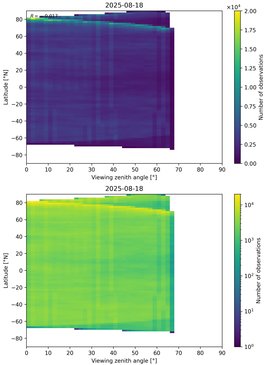
Figure 74: Scatter density plot of “Viewing zenith angle” against “Latitude” for 2025-08-17 to 2025-08-19.
