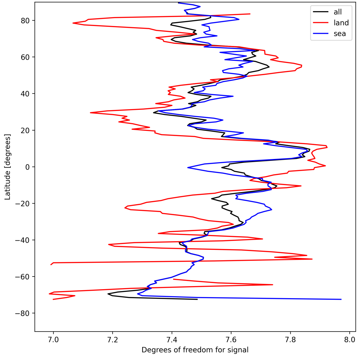
Figure 15: Zonal average of “Degrees of freedom for signal” for 2025-08-17 to 2025-08-19.
