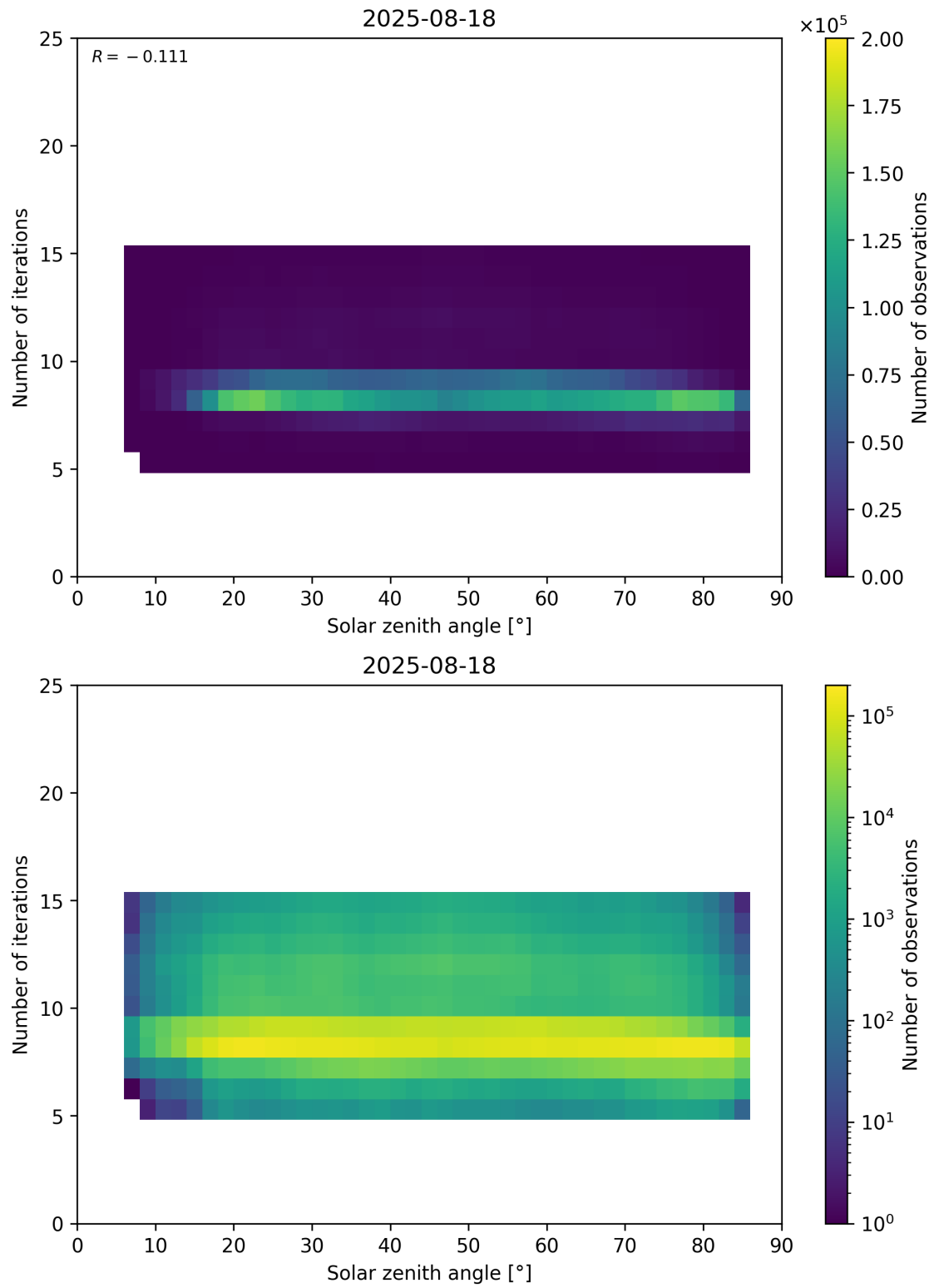
Figure 67: Scatter density plot of “Solar zenith angle” against “Number of iterations” for 2025-08-17 to 2025-08-19.
