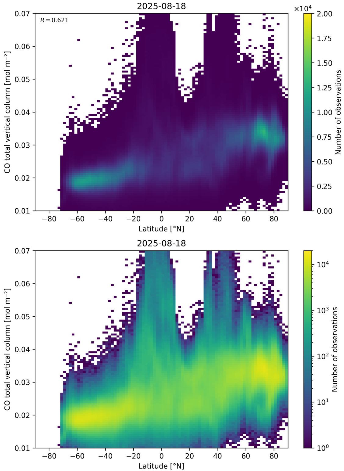
Figure 51: Scatter density plot of “Latitude” against “CO total vertical column” for 2025-08-17 to 2025-08-19.
