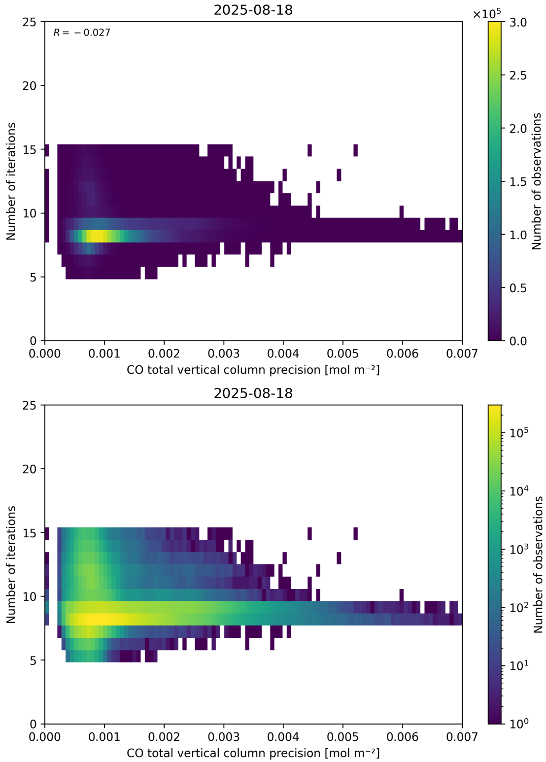
Figure 46: Scatter density plot of “CO total vertical column precision” against “Number of iterations” for 2025-08-17 to 2025-08-19.
