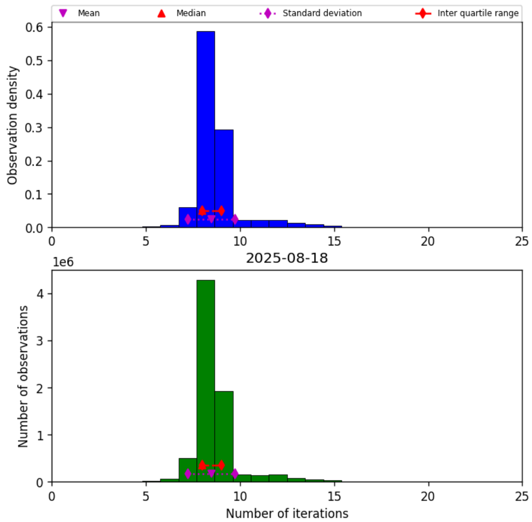
Figure 24: Histogram of “Number of iterations” for 2025-08-17 to 2025-08-19
