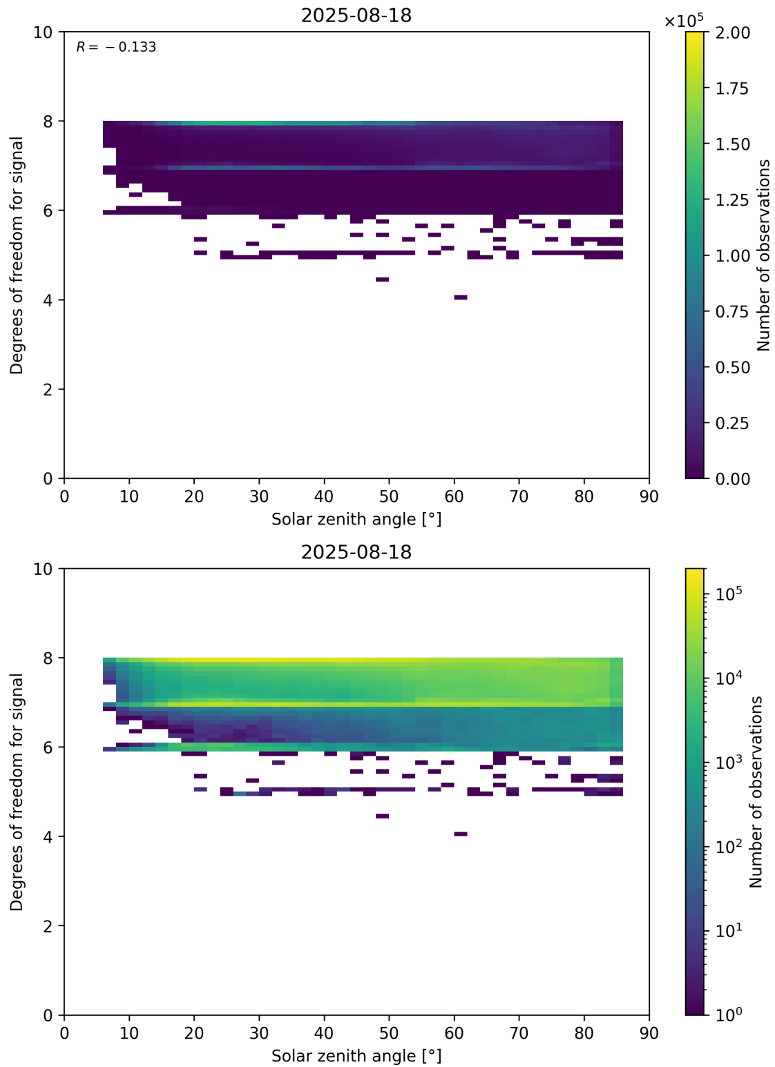
Figure 65: Scatter density plot of “Solar zenith angle” against “Degrees of freedom for signal” for 2025-08-17 to 2025-08-19.
