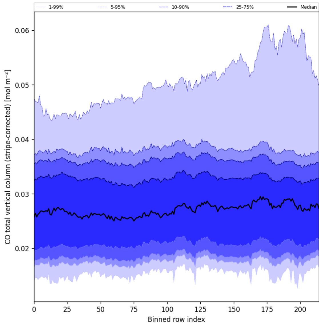
Figure 27: Along track statistics of “CO total vertical column (stripe-corrected)” for 2025-08-17 to 2025-08-19
