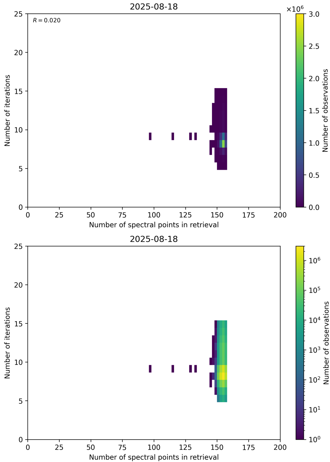
Figure 60: Scatter density plot of “Number of spectral points in retrieval” against “Number of iterations” for 2025-08-17 to 2025-08-19.
