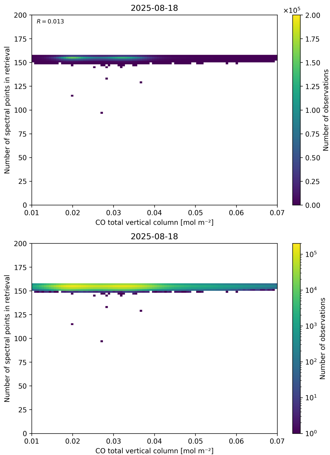
Figure 43: Scatter density plot of “CO total vertical column” against “Number of spectral points in retrieval” for 2025-08-17 to 2025-08-19.
