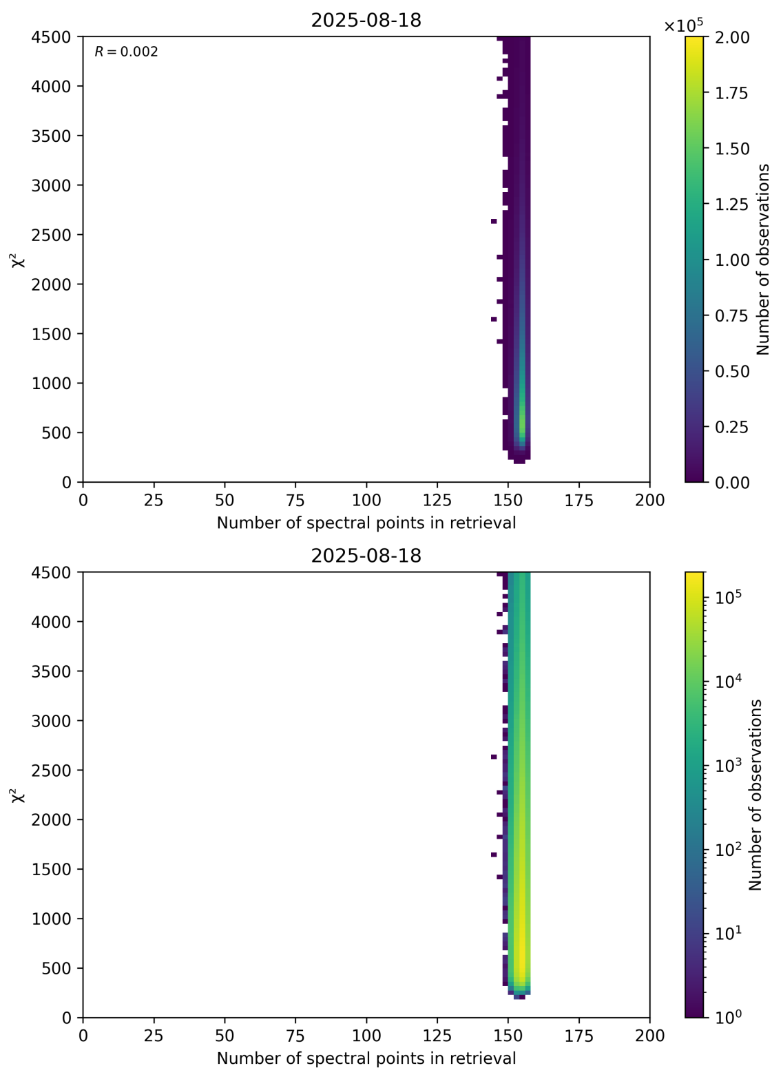
Figure 58: Scatter density plot of “Number of spectral points in retrieval” against “ \chi^2 ” for 2025-08-17 to 2025-08-19.
