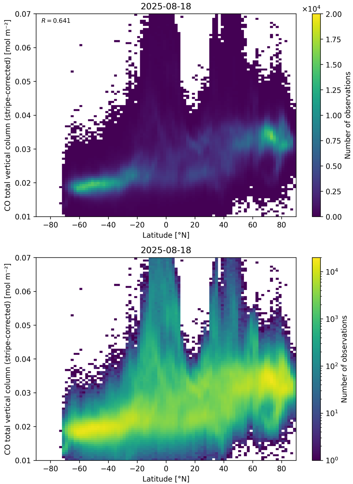
Figure 52: Scatter density plot of “Latitude” against “CO total vertical column (stripe-corrected)” for 2025-08-17 to 2025-08-19.
