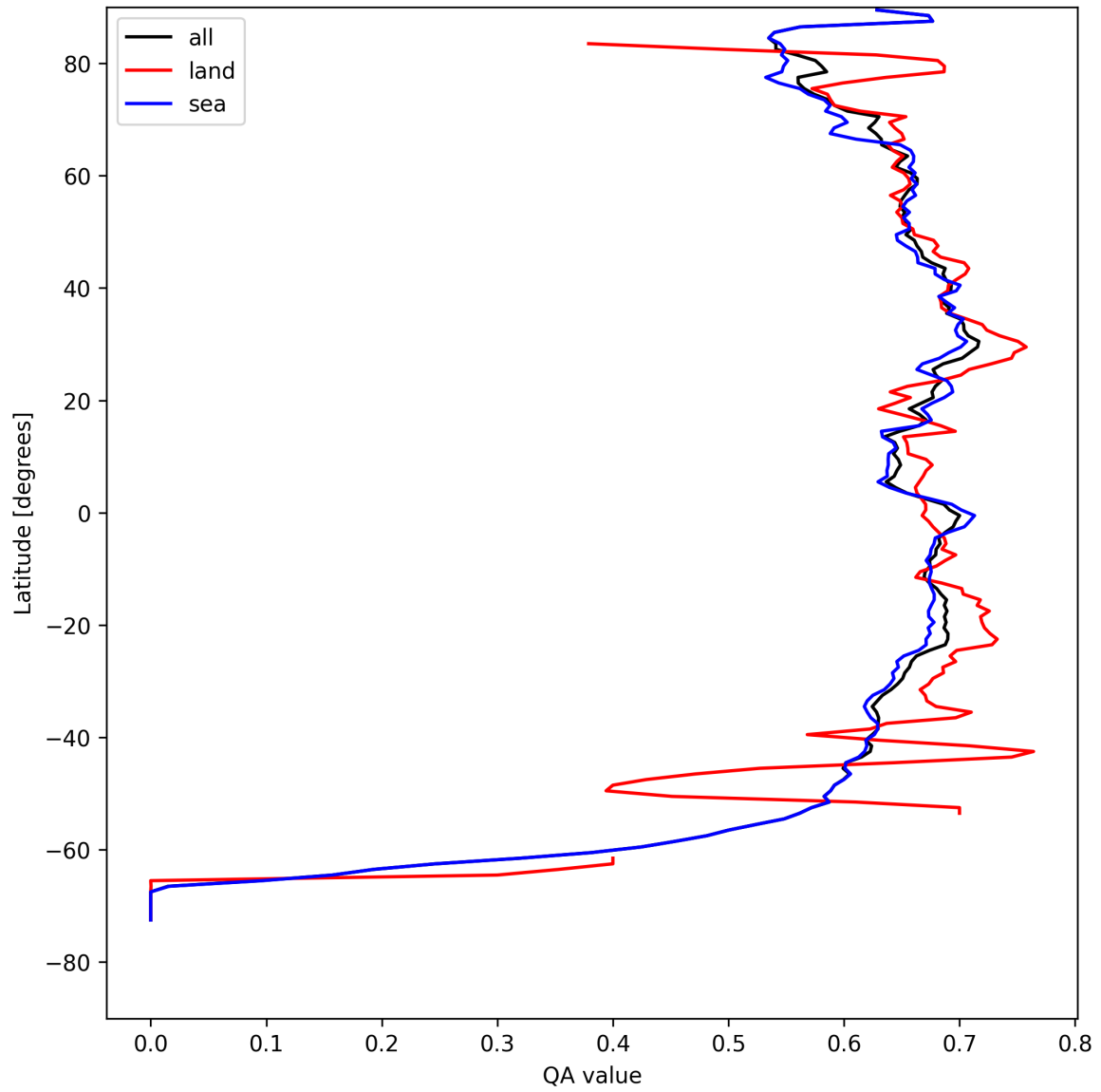
Figure 9: Zonal average of “QA value” for 2025-08-17 to 2025-08-19.
