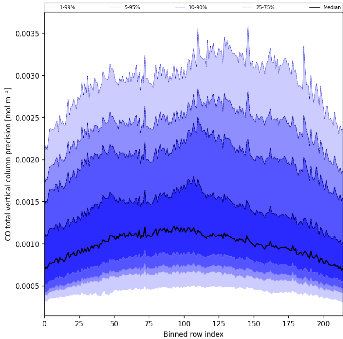
Figure 28: Along track statistics of “CO total vertical column precision” for 2025-08-17 to 2025-08-19
