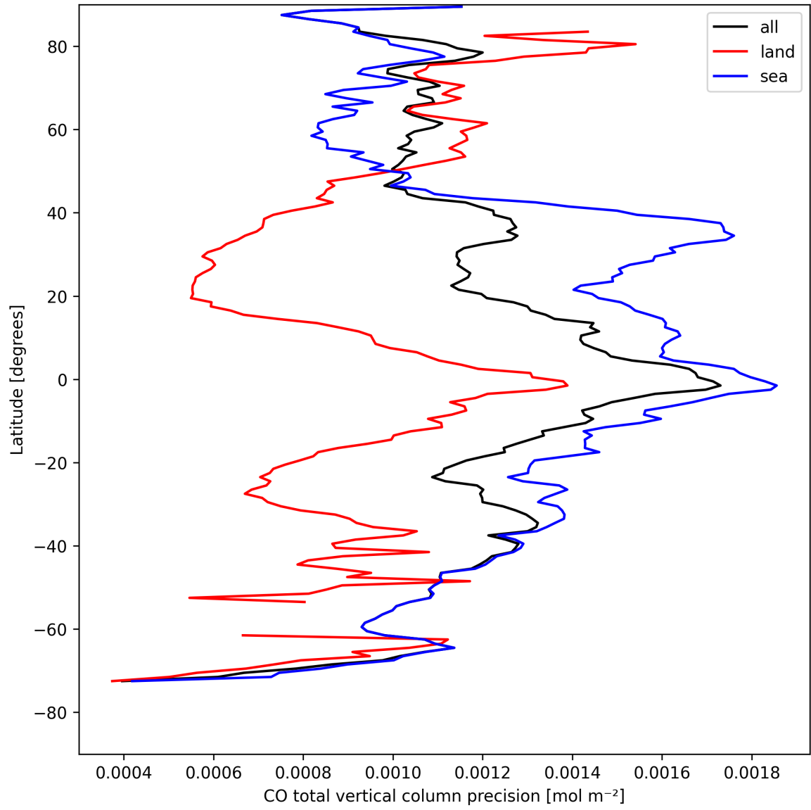
Figure 12: Zonal average of "CO total vertical column precision" for 2025-08-17 to 2025-08-19.
