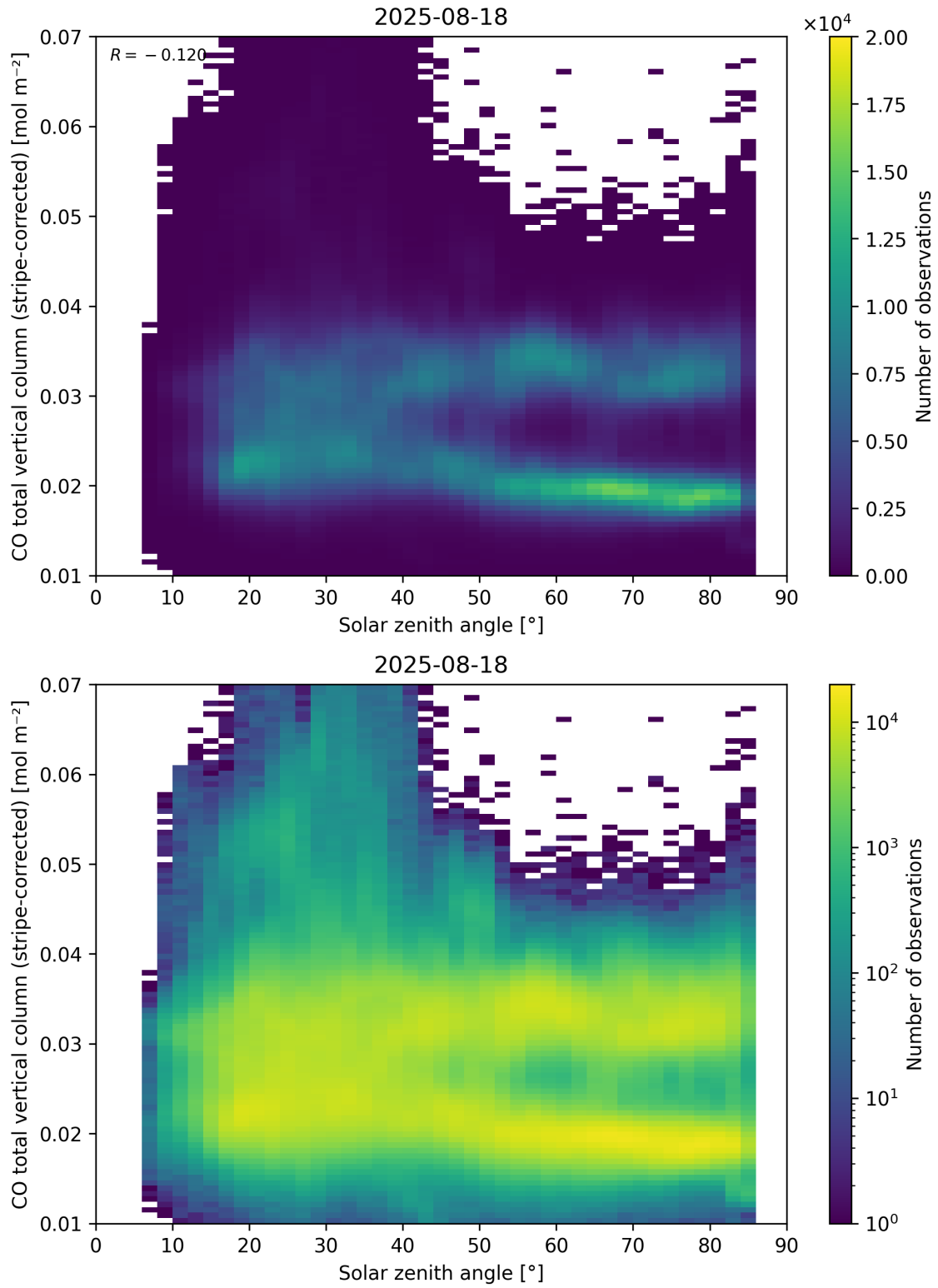
Figure 62: Scatter density plot of “Solar zenith angle” against “CO total vertical column (stripe-corrected)” for 2025-08-17 to 2025-08-19.
