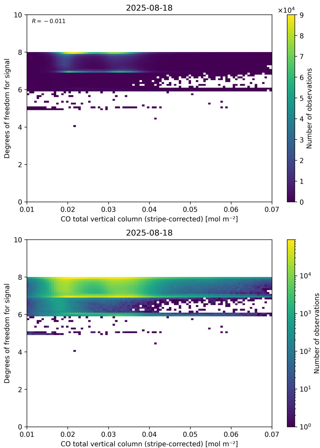
Figure 38: Scatter density plot of “CO total vertical column (stripe-corrected)” against “Degrees of freedom for signal” for 2025-08-17 to 2025-08-19.
