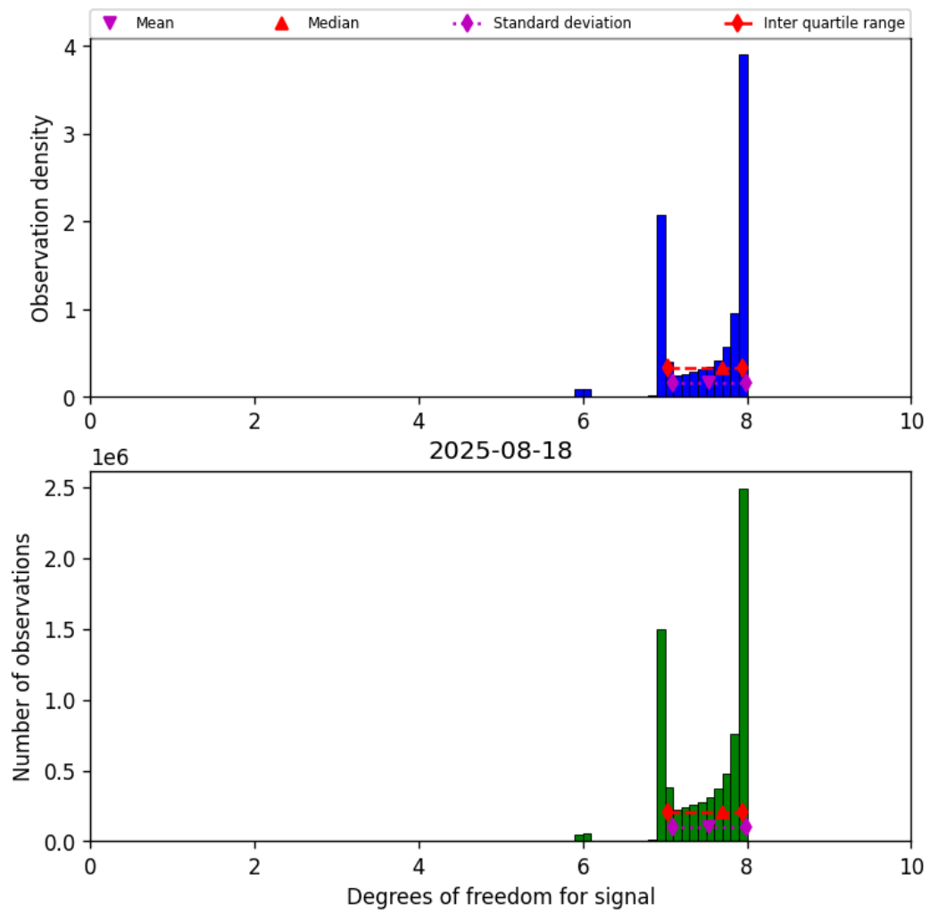
Figure 23: Histogram of “Degrees of freedom for signal” for 2025-08-17 to 2025-08-19
