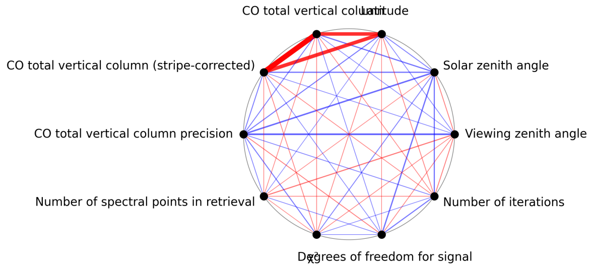
Figure 1: Map of correlation graph for 2025-08-17 to 2025-08-19.
