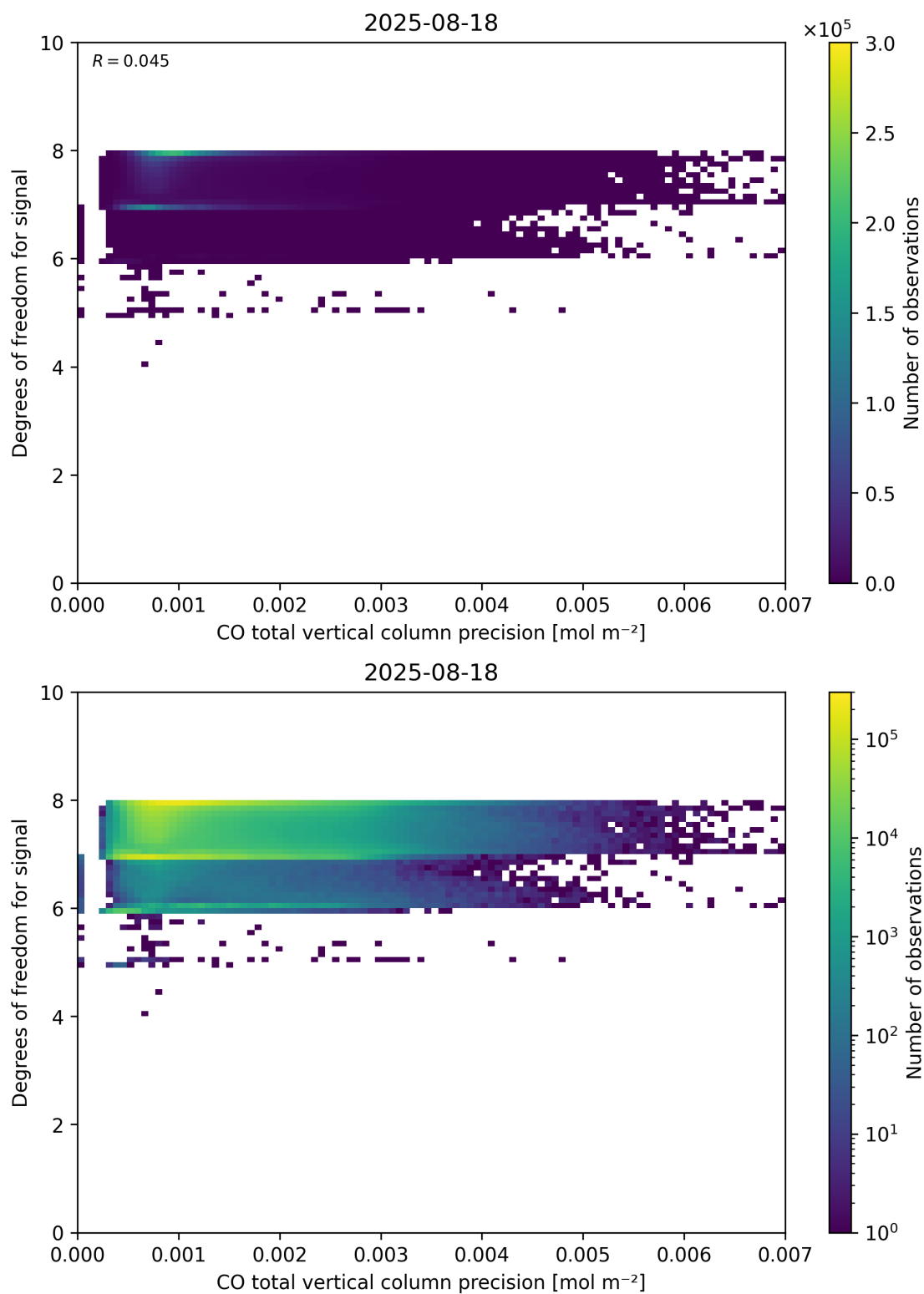
Figure 45: Scatter density plot of “CO total vertical column precision” against “Degrees of freedom for signal” for 2025-08-17 to 2025-08-19.
