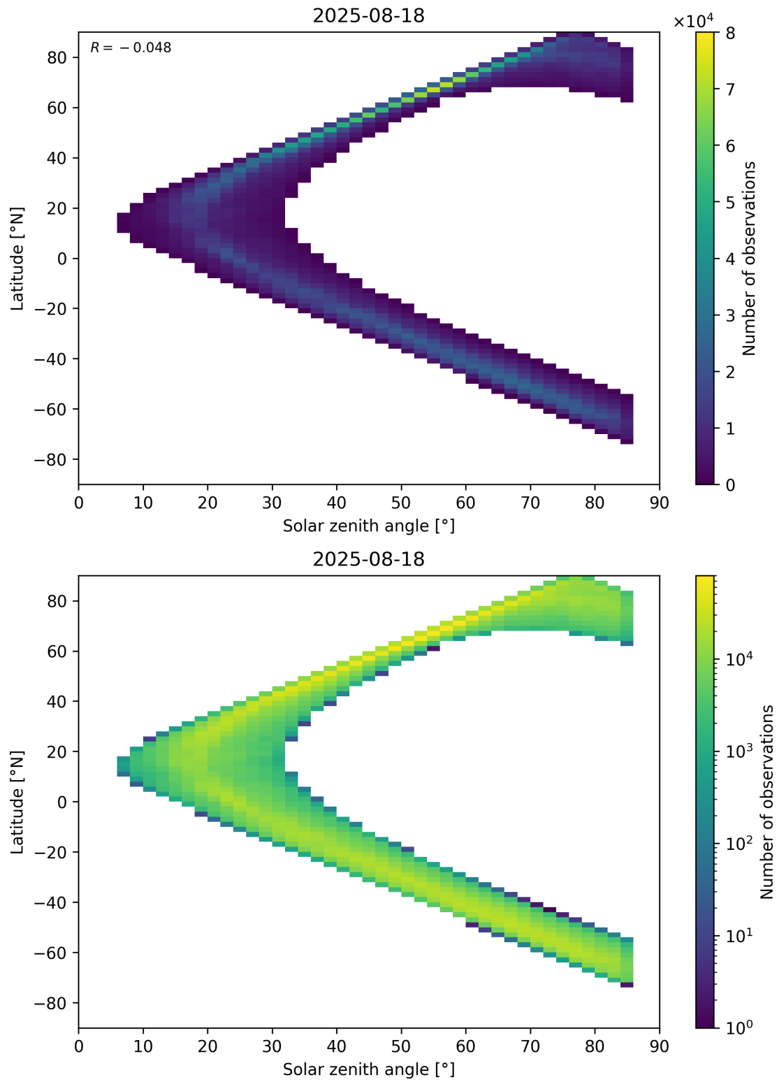
Figure 66: Scatter density plot of “Solar zenith angle” against “Latitude” for 2025-08-17 to 2025-08-19.
