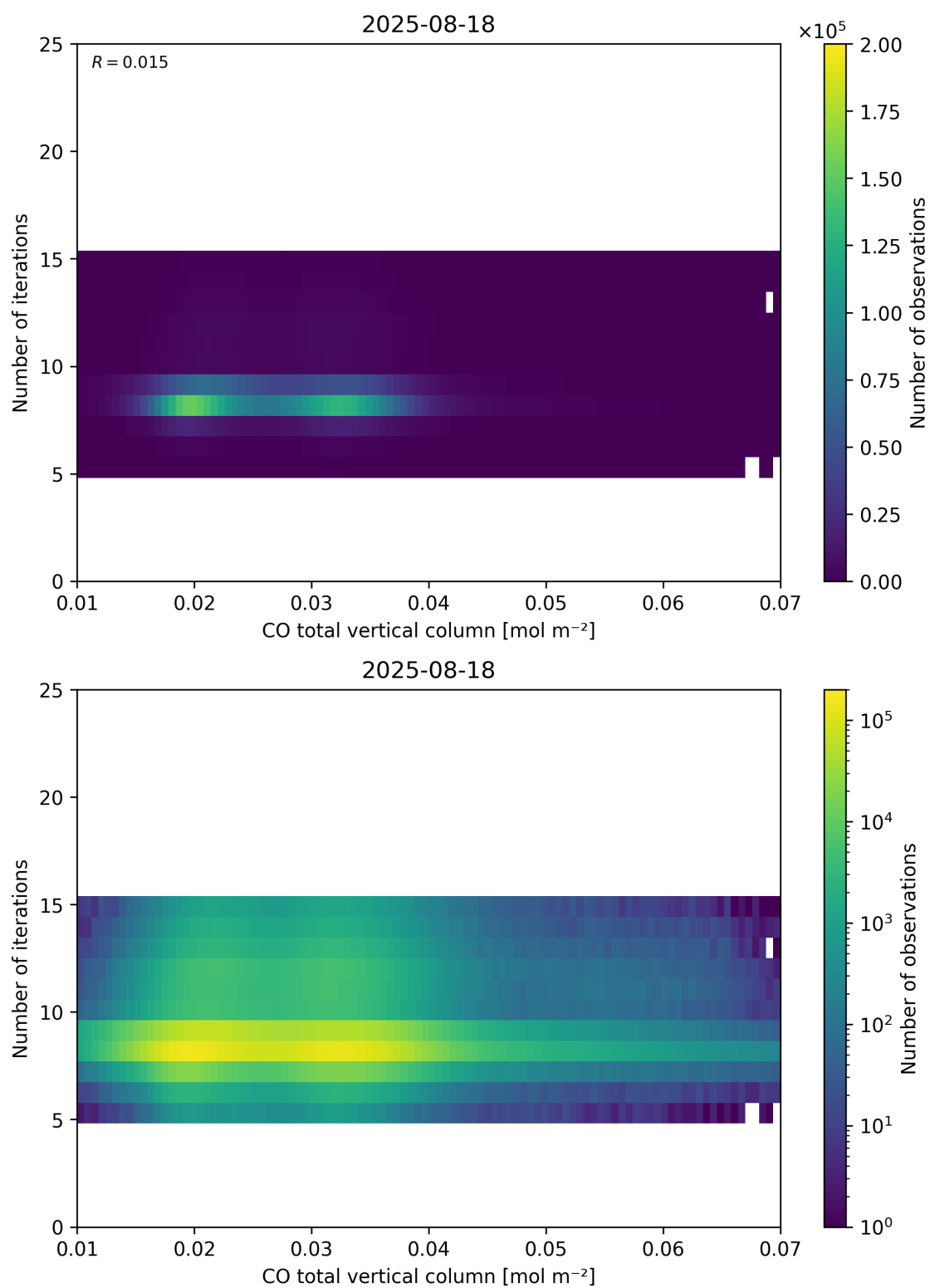
Figure 42: Scatter density plot of “CO total vertical column” against “Number of iterations” for 2025-08-17 to 2025-08-19.
