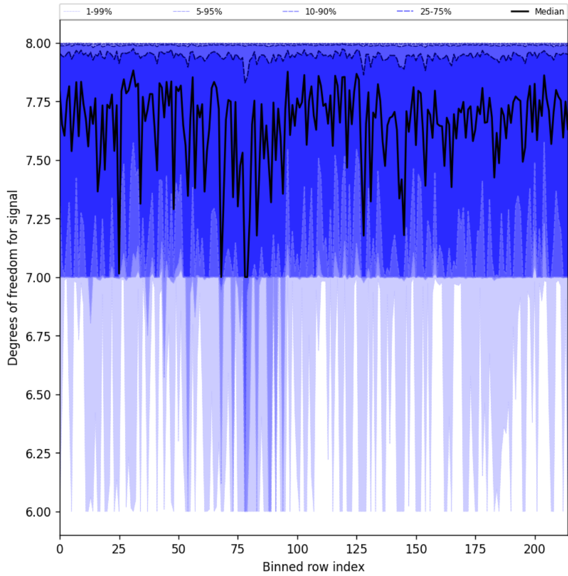
Figure 31: Along track statistics of “Degrees of freedom for signal” for 2025-08-17 to 2025-08-19
