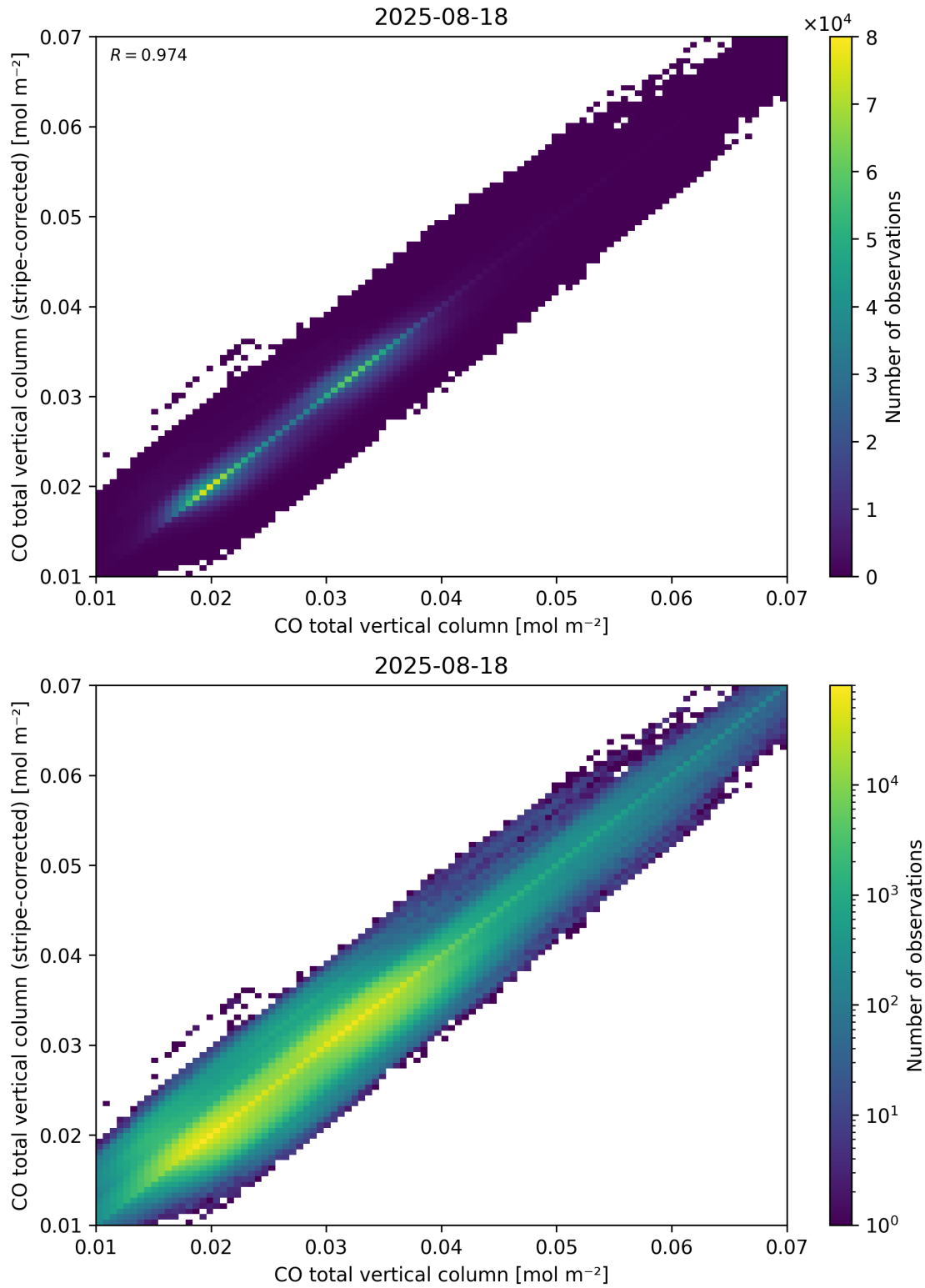
Figure 33: Scatter density plot of “CO total vertical column” against “CO total vertical column (stripe-corrected)” for 2025-08-17 to 2025-08-19.
