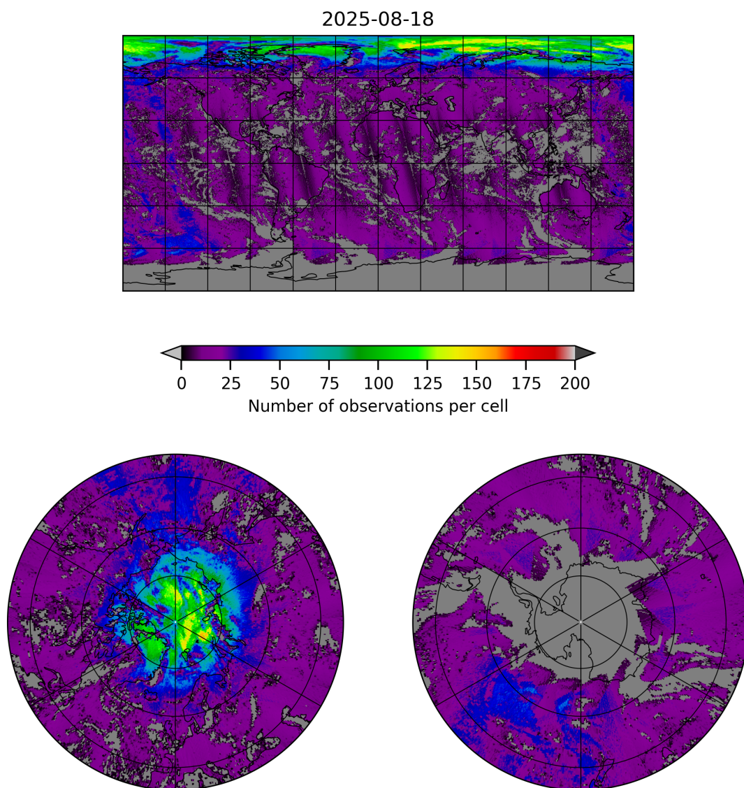
Figure 8: Map of the number of observations for 2025-08-17 to 2025-08-19
