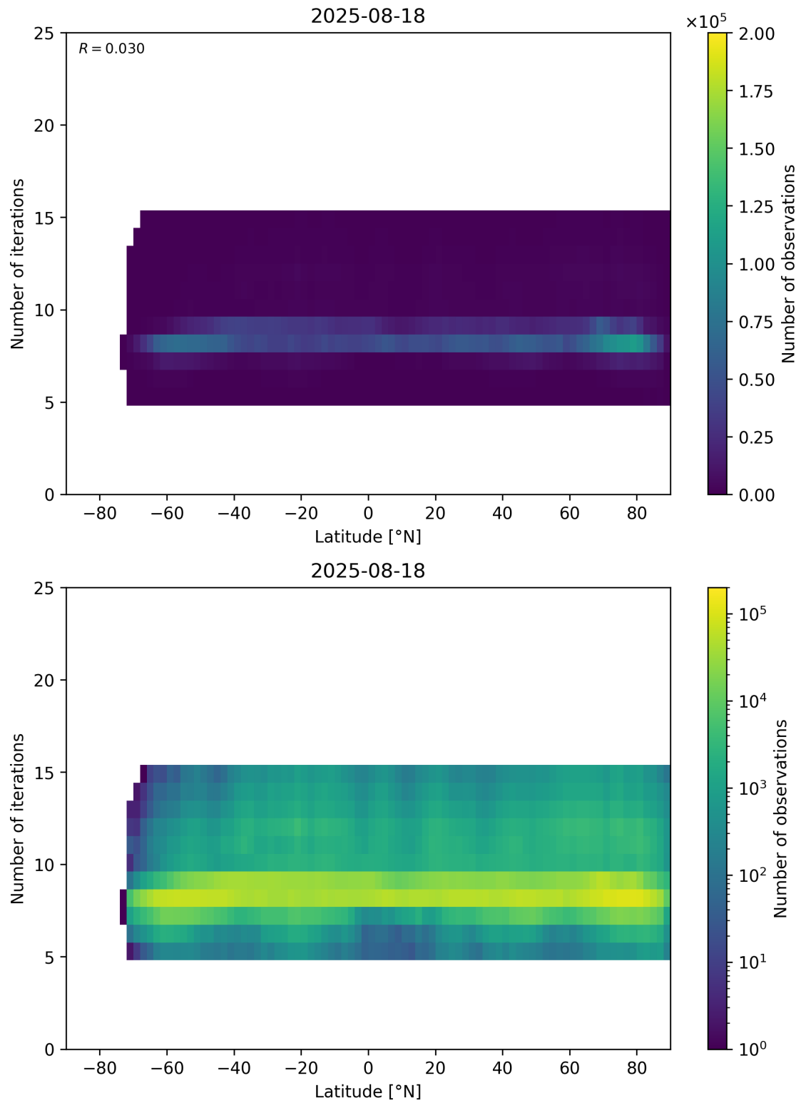
Figure 56: Scatter density plot of “Latitude” against “Number of iterations” for 2025-08-17 to 2025-08-19.
