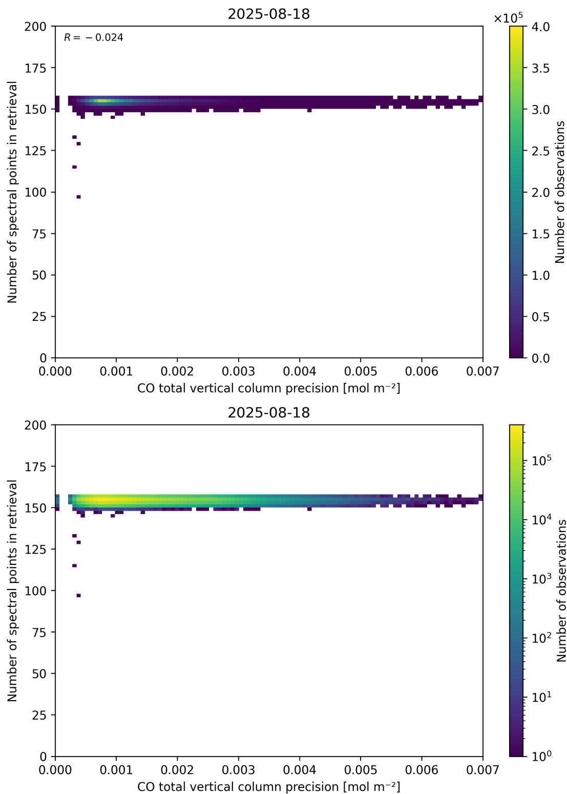
Figure 47: Scatter density plot of “CO total vertical column precision” against “Number of spectral points in retrieval” for 2025-08-17 to 2025-08-19.
