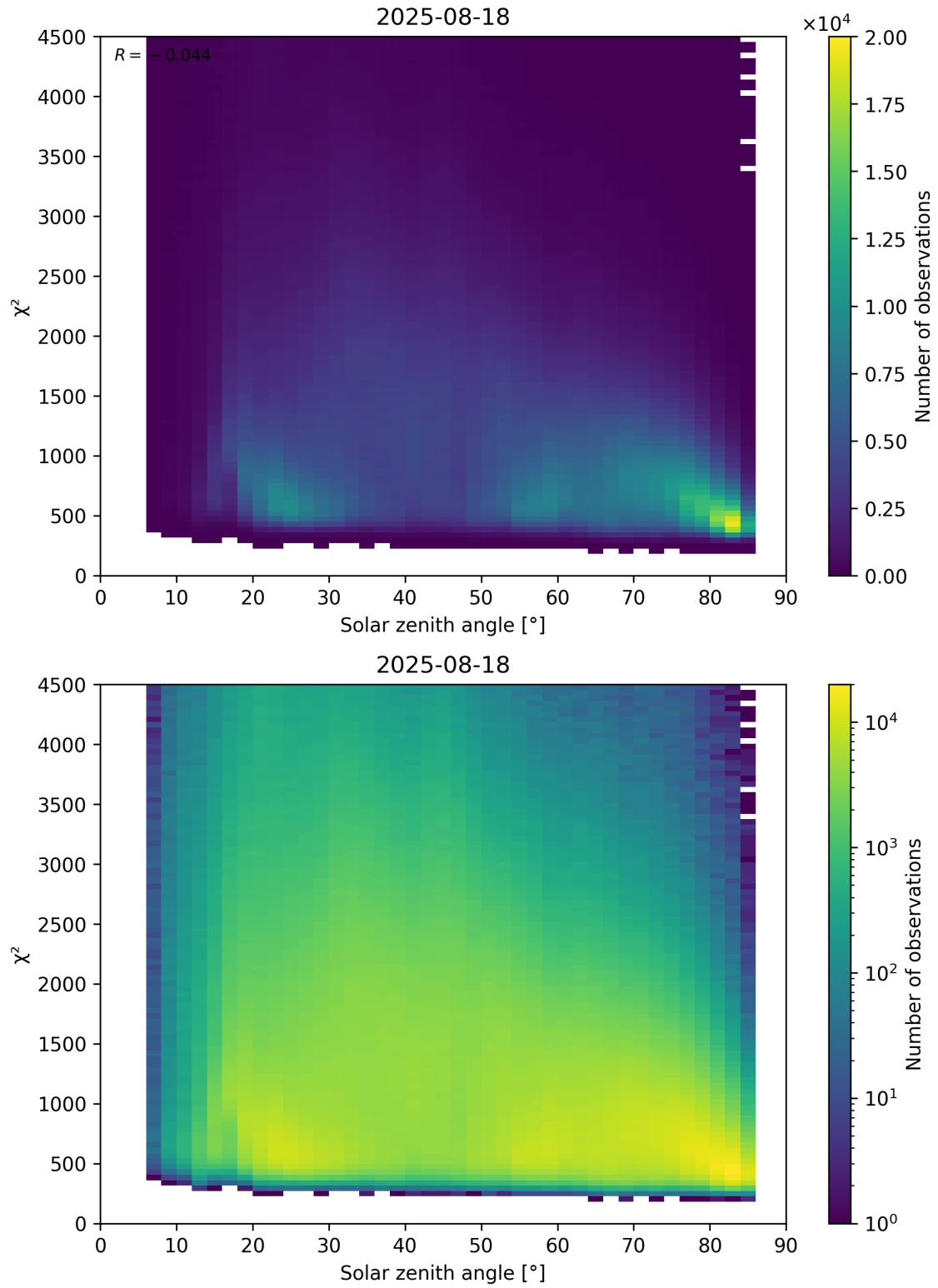
Figure 64: Scatter density plot of “Solar zenith angle” against “ \chi^2 ” for 2025-08-17 to 2025-08-19.
