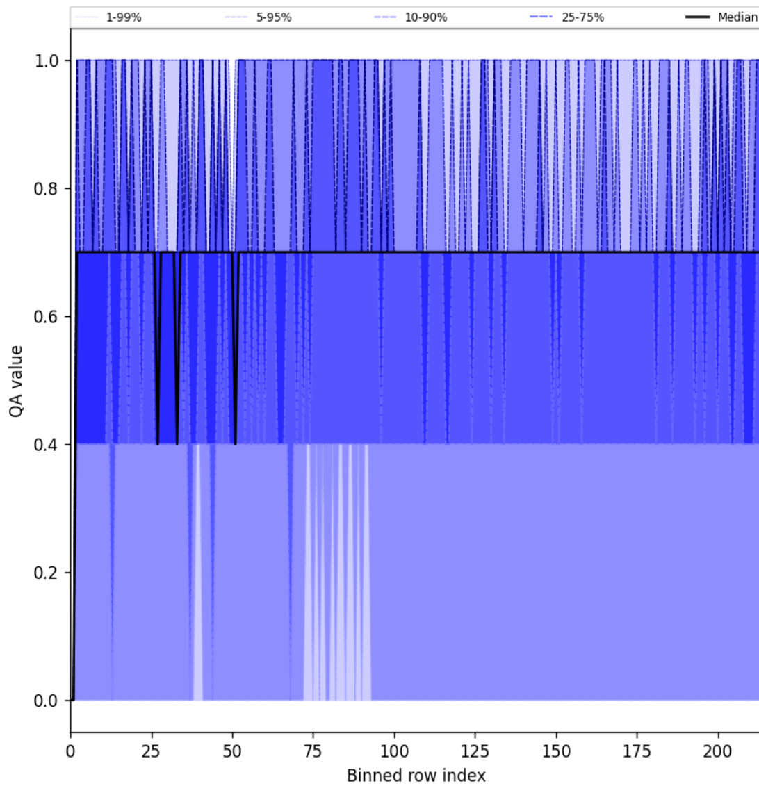
Figure 25: Along track statistics of “QA value” for 2025-08-17 to 2025-08-19
