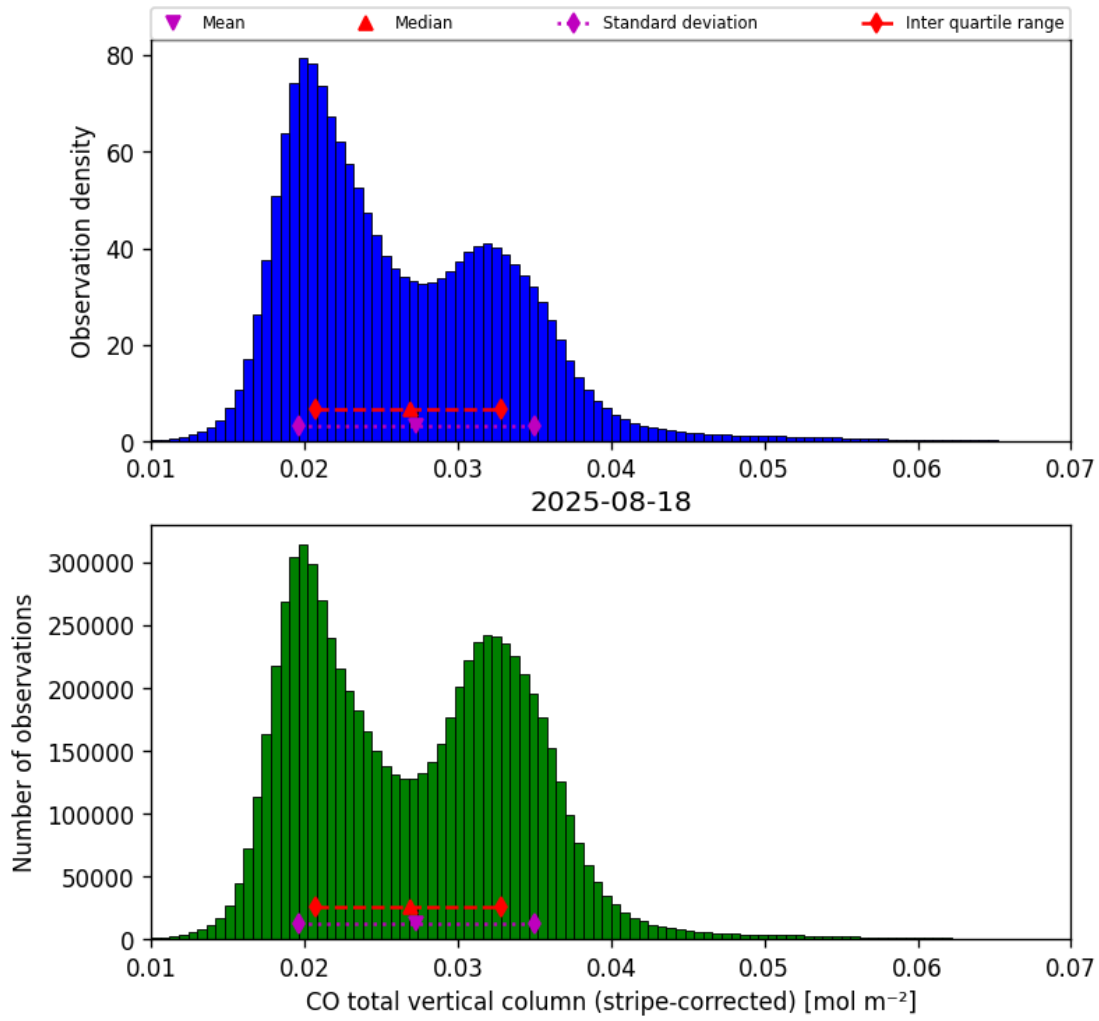
Figure 19: Histogram of “CO total vertical column (stripe-corrected)” for 2025-08-17 to 2025-08-19
