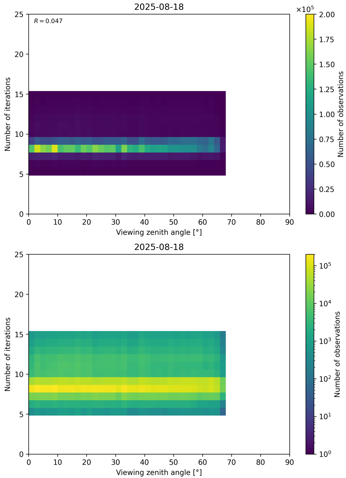
Figure 75: Scatter density plot of “Viewing zenith angle” against “Number of iterations” for 2025-08-17 to 2025-08-19.
