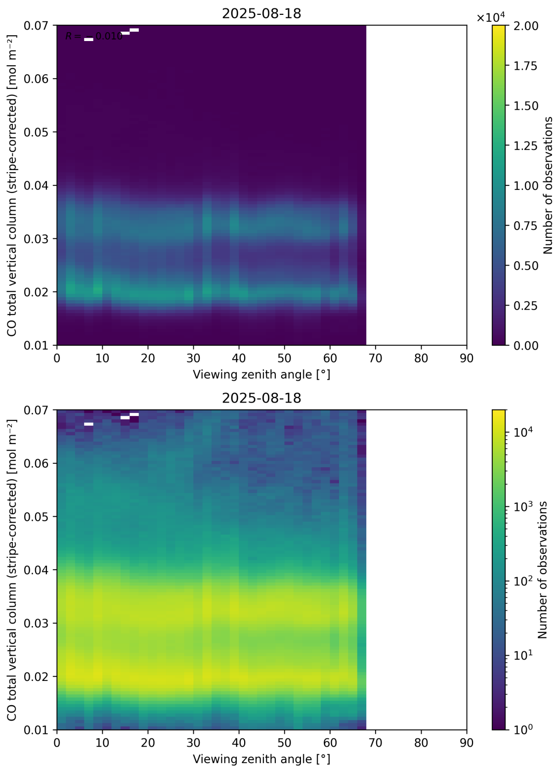
Figure 70: Scatter density plot of “Viewing zenith angle” against “CO total vertical column (stripe-corrected)” for 2025-08-17 to 2025-08-19.
