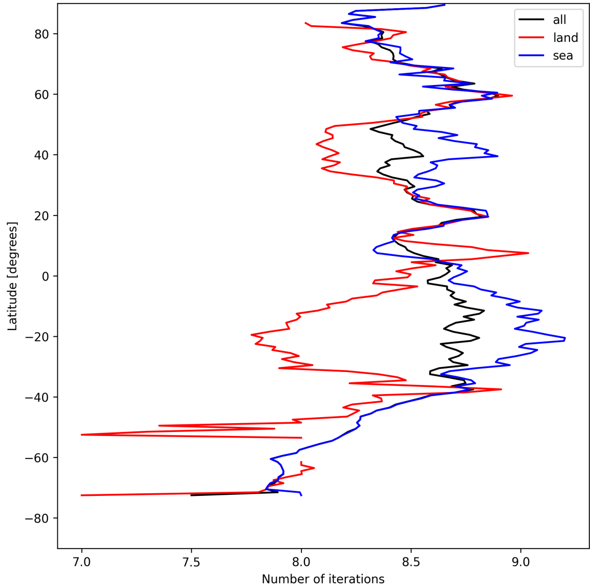
Figure 16: Zonal average of “Number of iterations” for 2025-08-17 to 2025-08-19.
