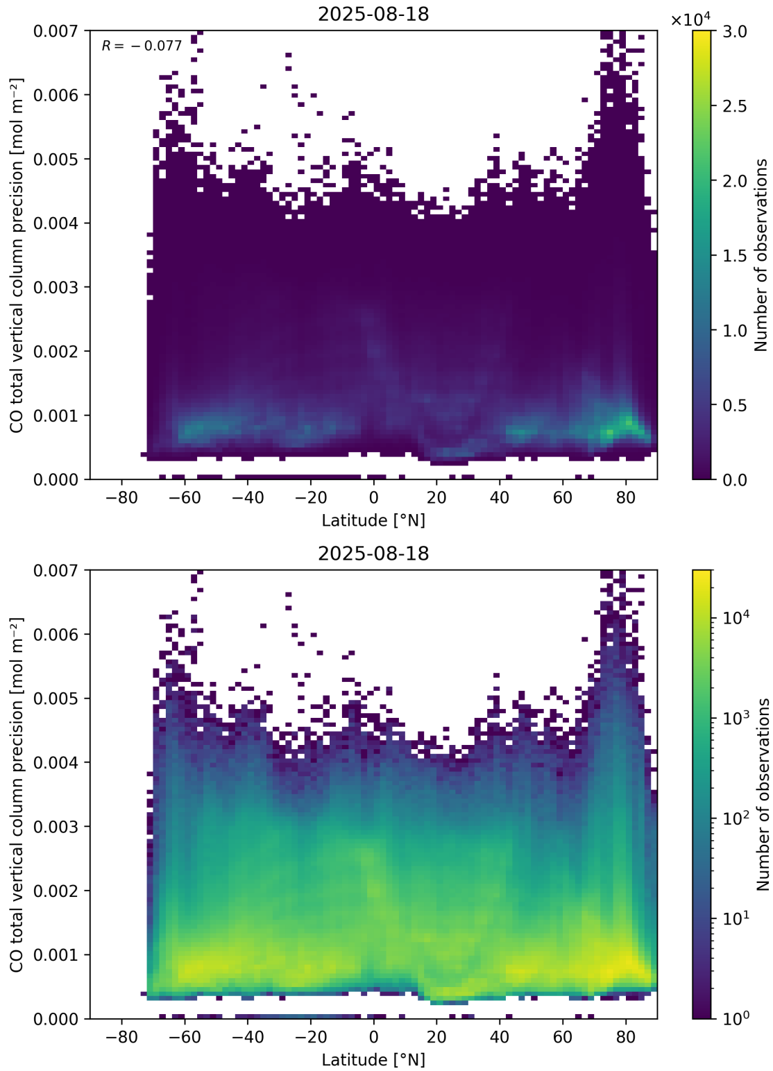
Figure 53: Scatter density plot of “Latitude” against “CO total vertical column precision” for 2025-08-17 to 2025-08-19.
