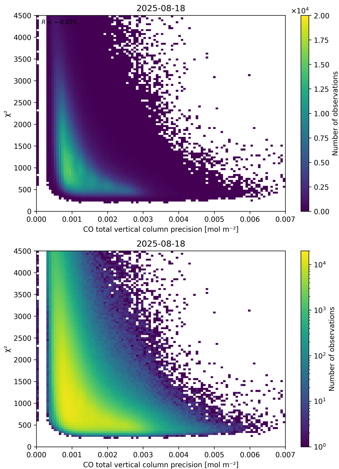
Figure 44: Scatter density plot of “CO total vertical column precision” against “ \chi^2 ” for 2025-08-17 to 2025-08-19.
