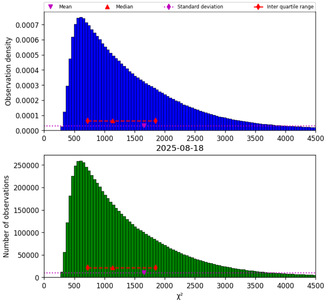
Figure 22: Histogram of “ \chi^2 ” for 2025-08-17 to 2025-08-19
