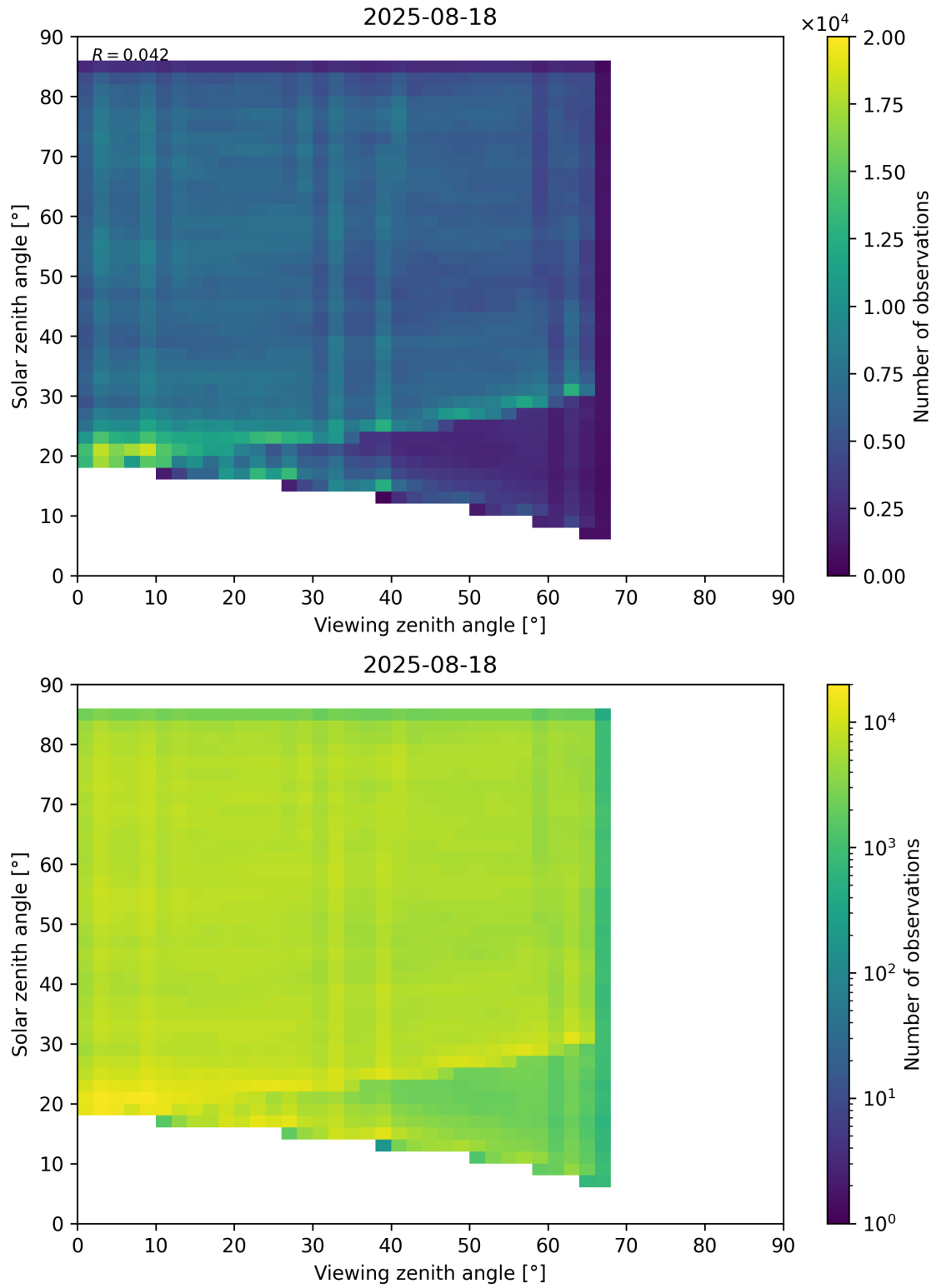
Figure 77: Scatter density plot of “Viewing zenith angle” against “Solar zenith angle” for 2025-08-17 to 2025-08-19.
