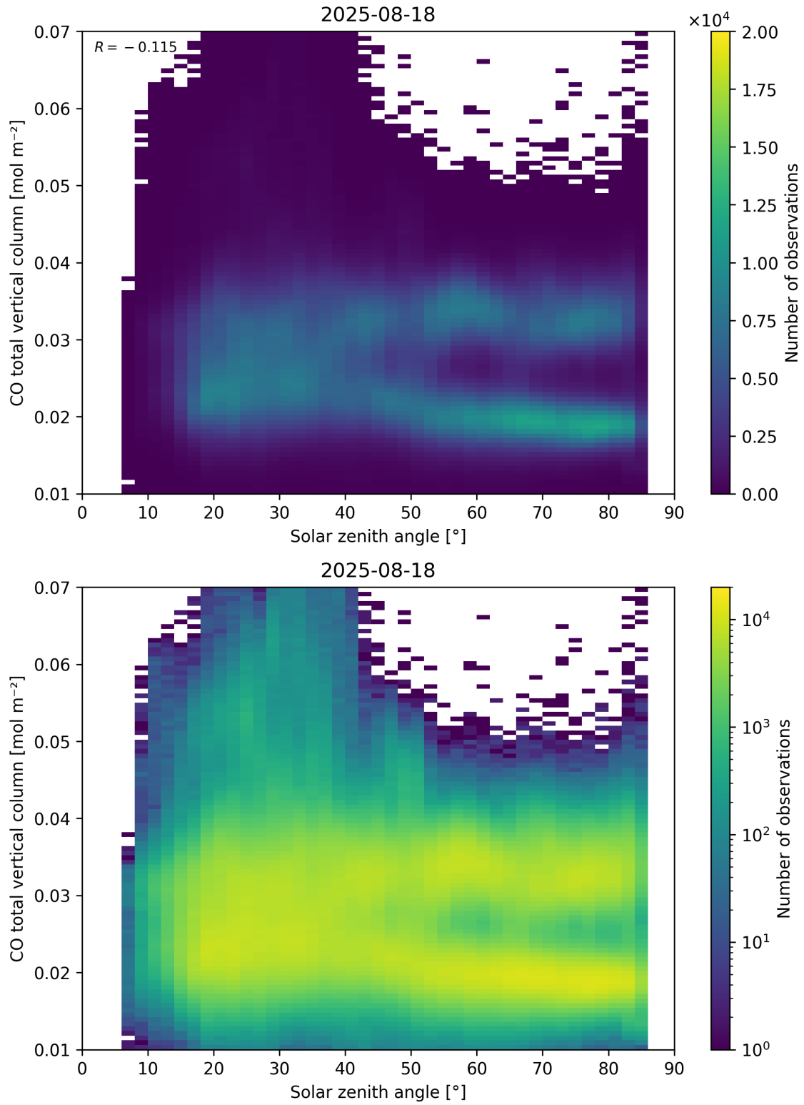
Figure 61: Scatter density plot of “Solar zenith angle” against “CO total vertical column” for 2025-08-17 to 2025-08-19.
