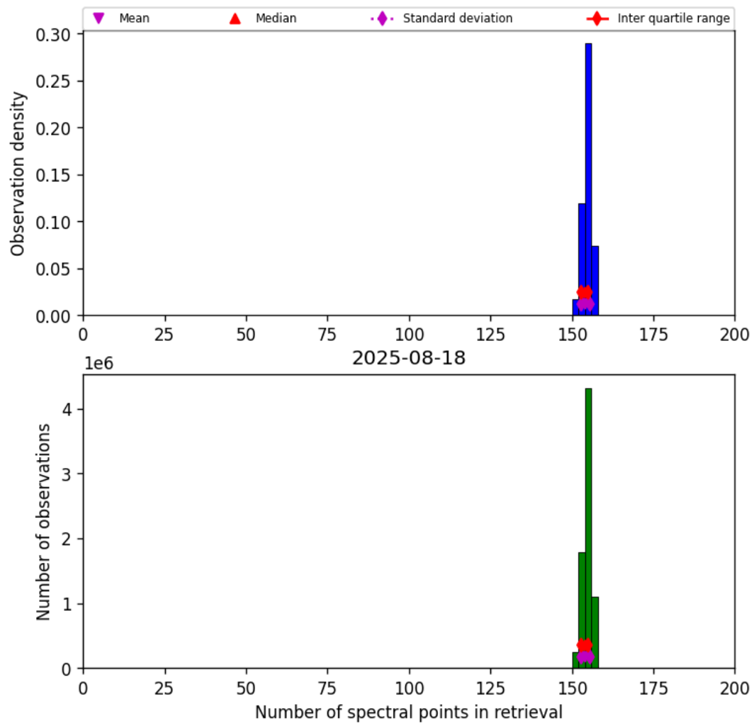
Figure 21: Histogram of “Number of spectral points in retrieval” for 2025-08-17 to 2025-08-19
