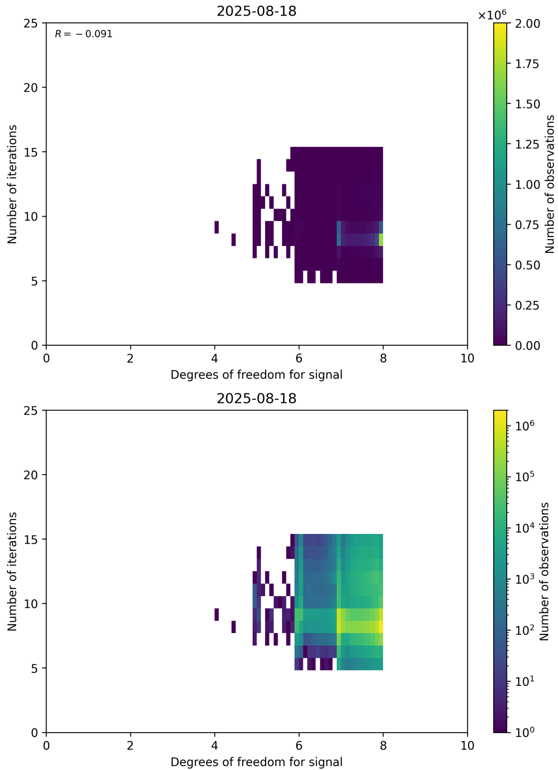
Figure 50: Scatter density plot of “Degrees of freedom for signal” against “Number of iterations” for 2025-08-17 to 2025-08-19.
