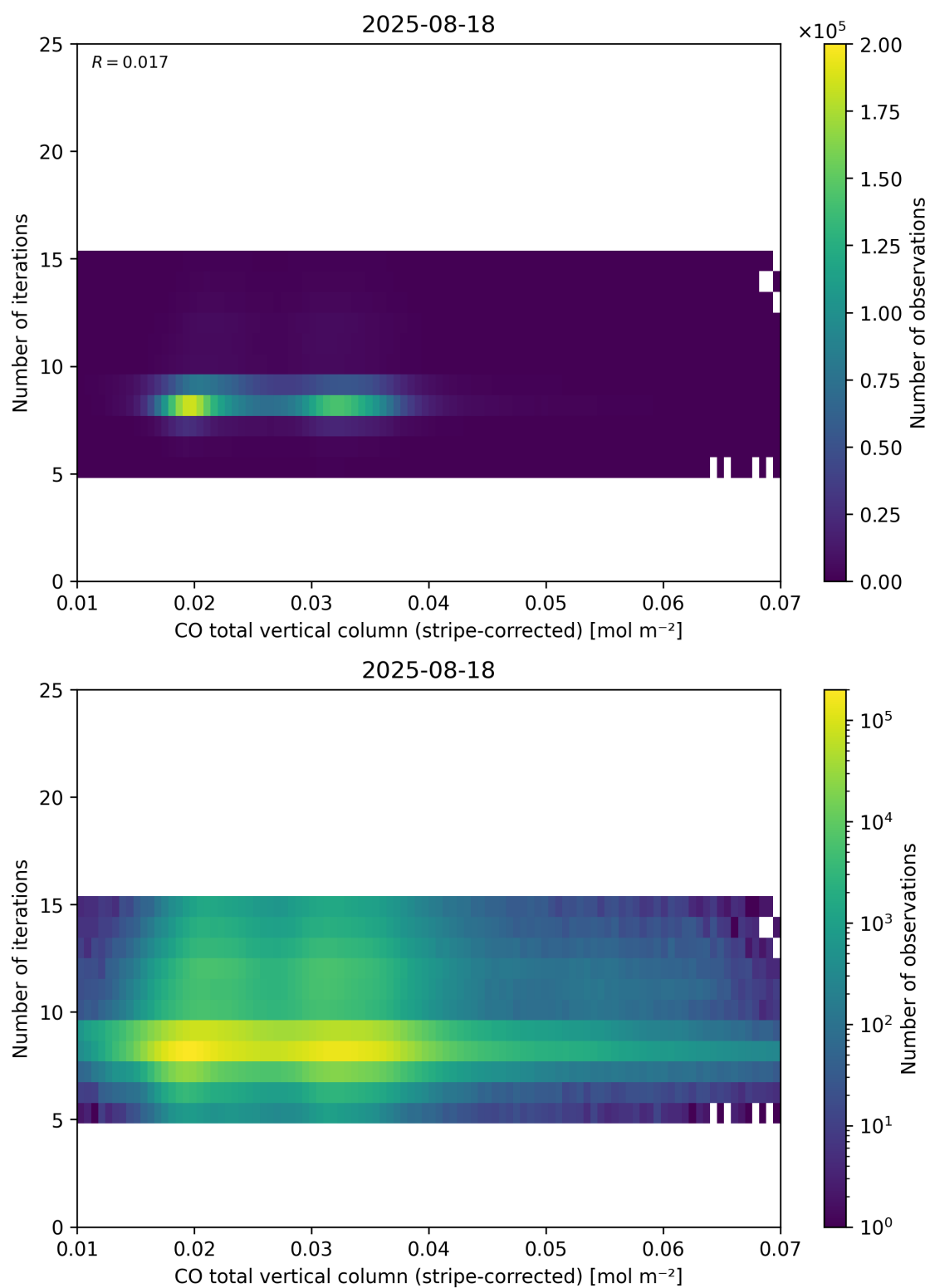
Figure 39: Scatter density plot of “CO total vertical column (stripe-corrected)” against “Number of iterations” for 2025-08-17 to 2025-08-19.
