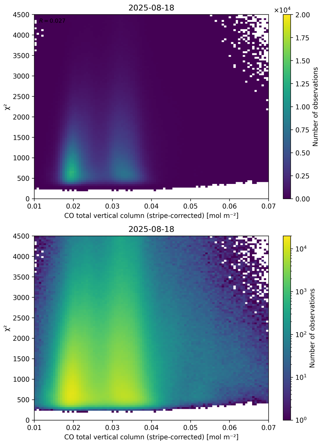
Figure 37: Scatter density plot of “CO total vertical column (stripe-corrected)” against “ \chi^2 ” for 2025-08-17 to 2025-08-19.
