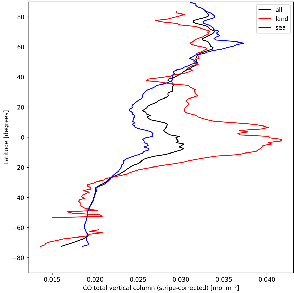
Figure 11: Zonal average of “CO total vertical column (stripe-corrected)” for 2025-08-17 to 2025-08-19.
