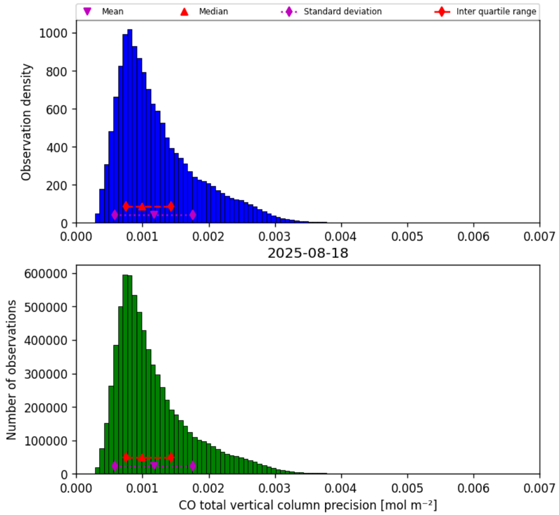
Figure 20: Histogram of “CO total vertical column precision” for 2025-08-17 to 2025-08-19
