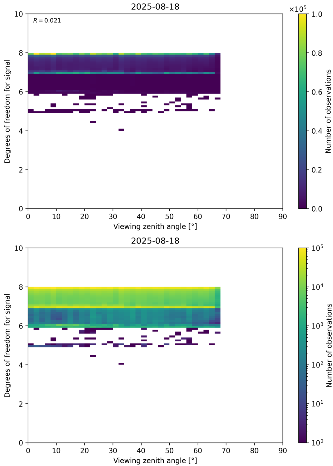
Figure 73: Scatter density plot of “Viewing zenith angle” against “Degrees of freedom for signal” for 2025-08-17 to 2025-08-19.
