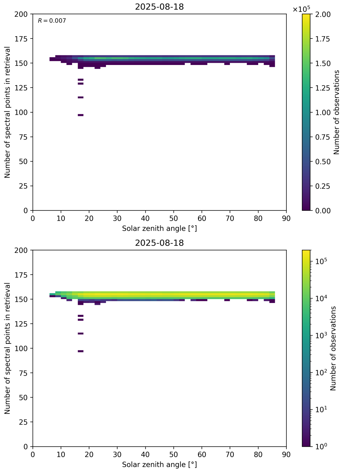
Figure 68: Scatter density plot of “Solar zenith angle” against “Number of spectral points in retrieval” for 2025-08-17 to 2025-08-19.
