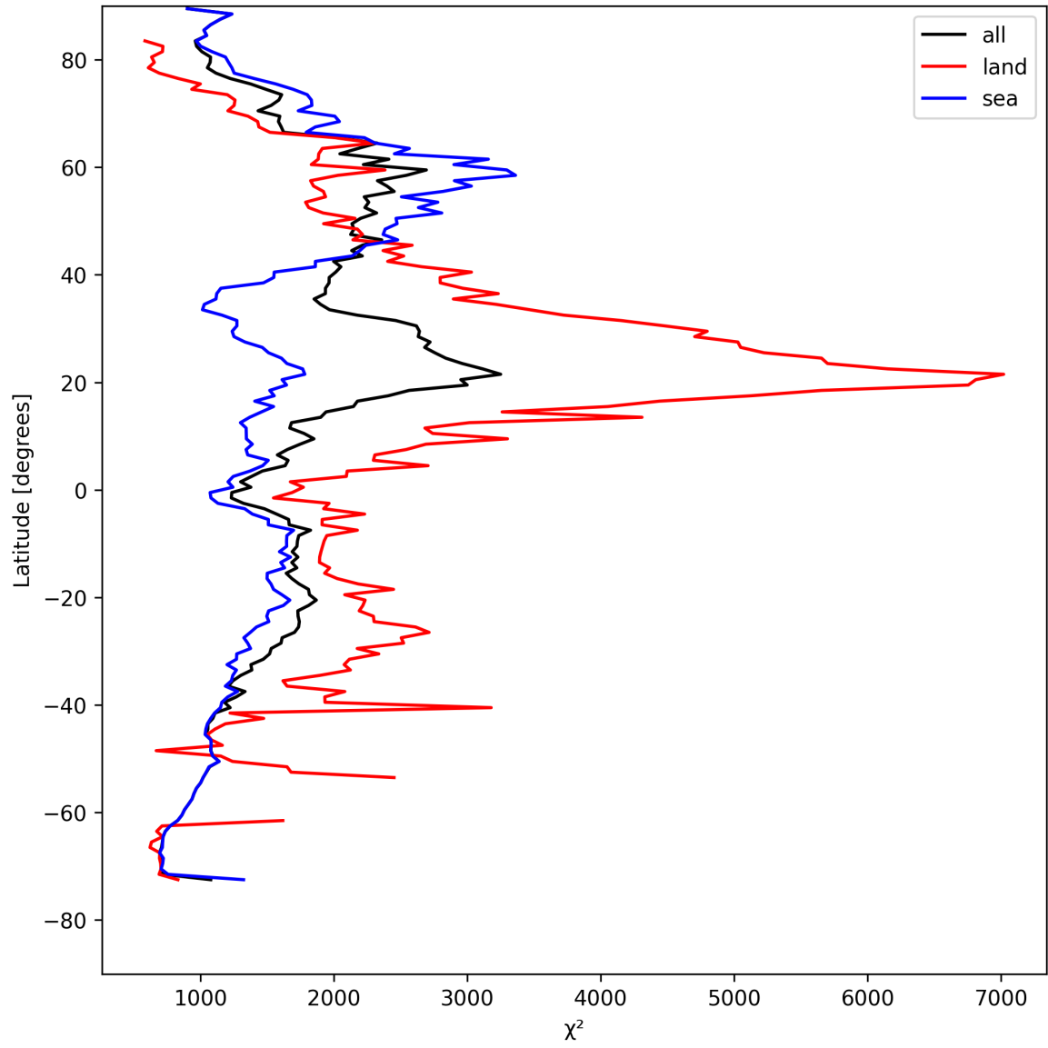
Figure 14: Zonal average of “ \chi^2 ” for 2025-08-17 to 2025-08-19.
