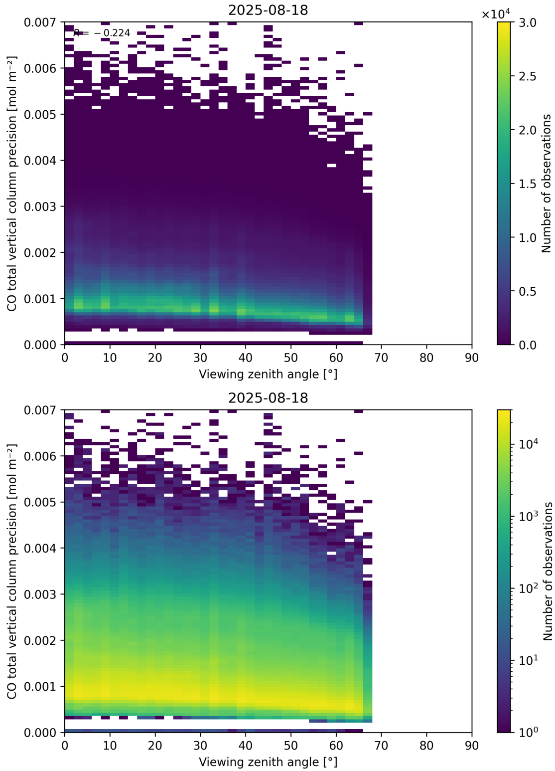
Figure 71: Scatter density plot of “Viewing zenith angle” against “CO total vertical column precision” for 2025-08-17 to 2025-08-19.
