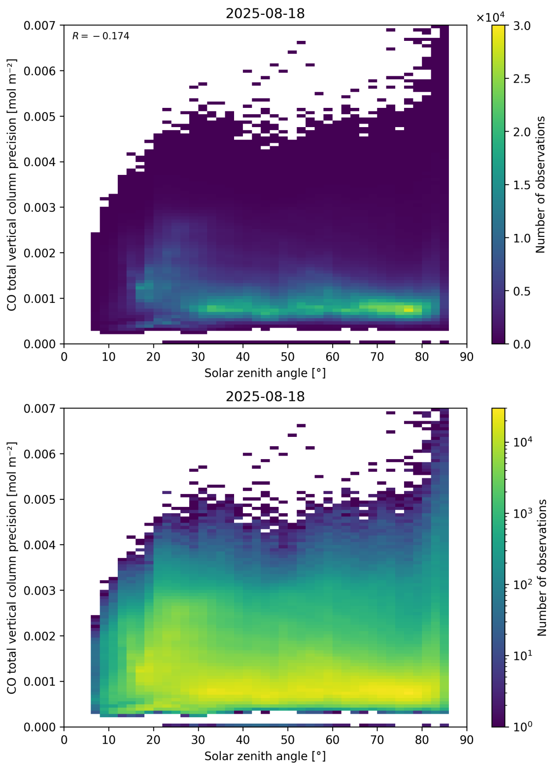
Figure 63: Scatter density plot of “Solar zenith angle” against “CO total vertical column precision” for 2025-08-17 to 2025-08-19.
