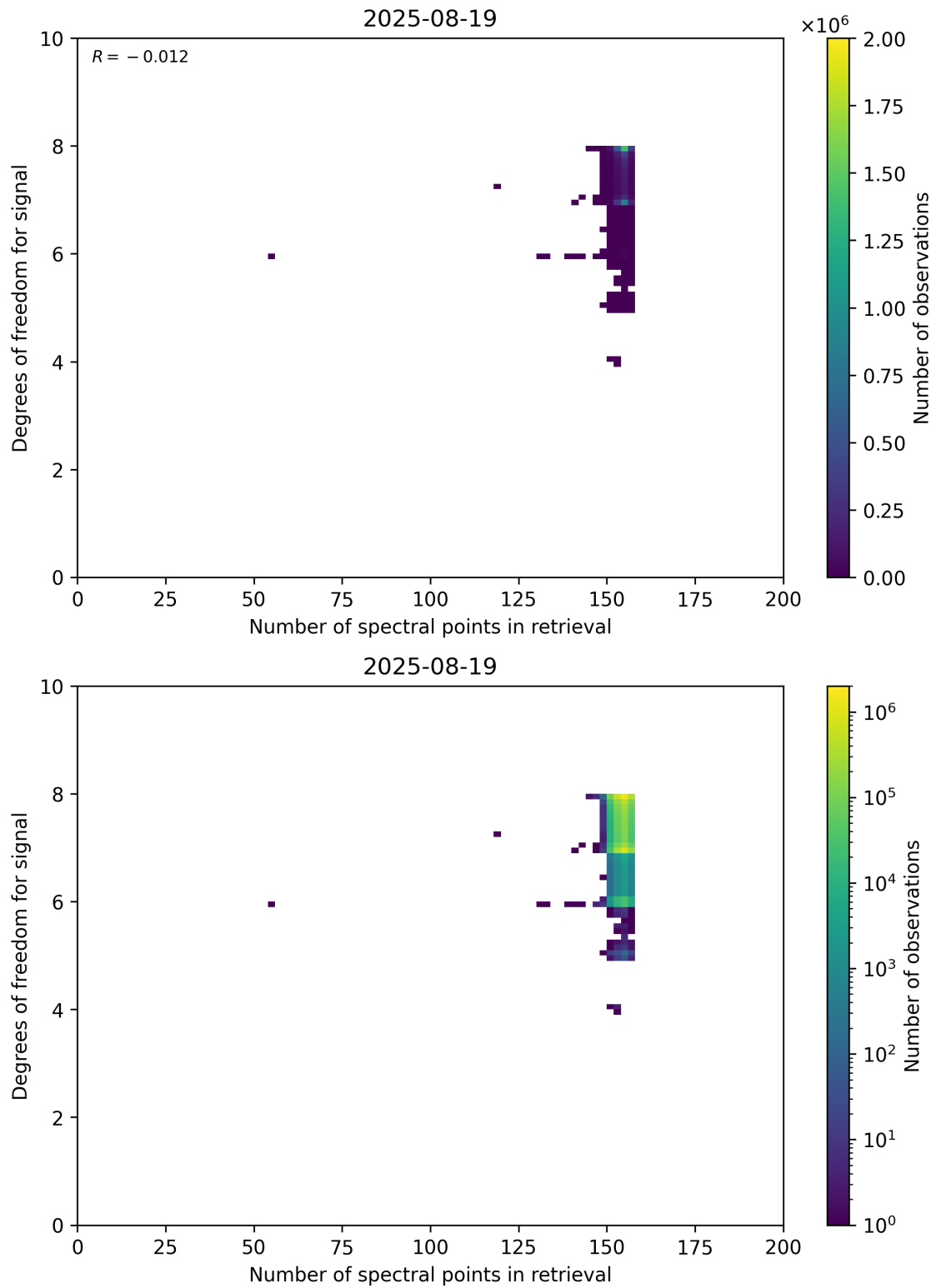
Figure 59: Scatter density plot of “Number of spectral points in retrieval” against “Degrees of freedom for signal” for 2025-08-19 to 2025-08-20.
