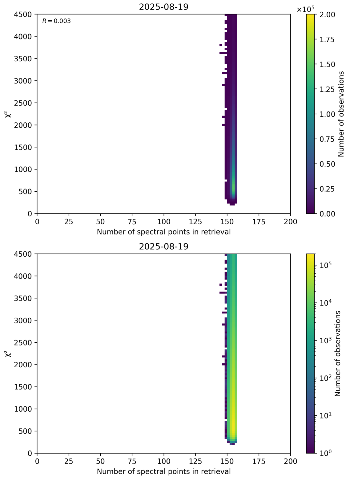
Figure 58: Scatter density plot of “Number of spectral points in retrieval” against “ \chi^2 ” for 2025-08-19 to 2025-08-20.
