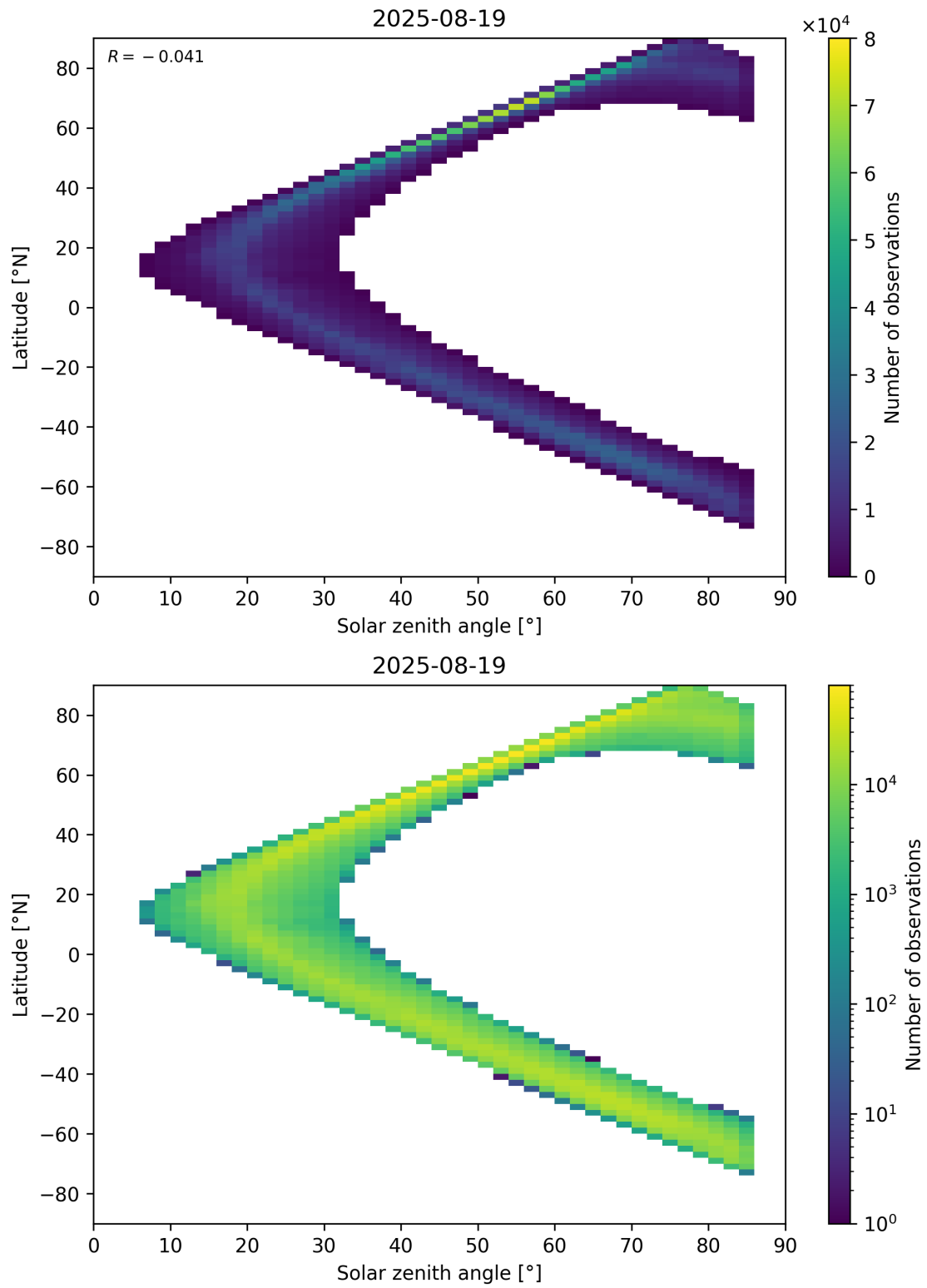
Figure 66: Scatter density plot of “Solar zenith angle” against “Latitude” for 2025-08-19 to 2025-08-20.
