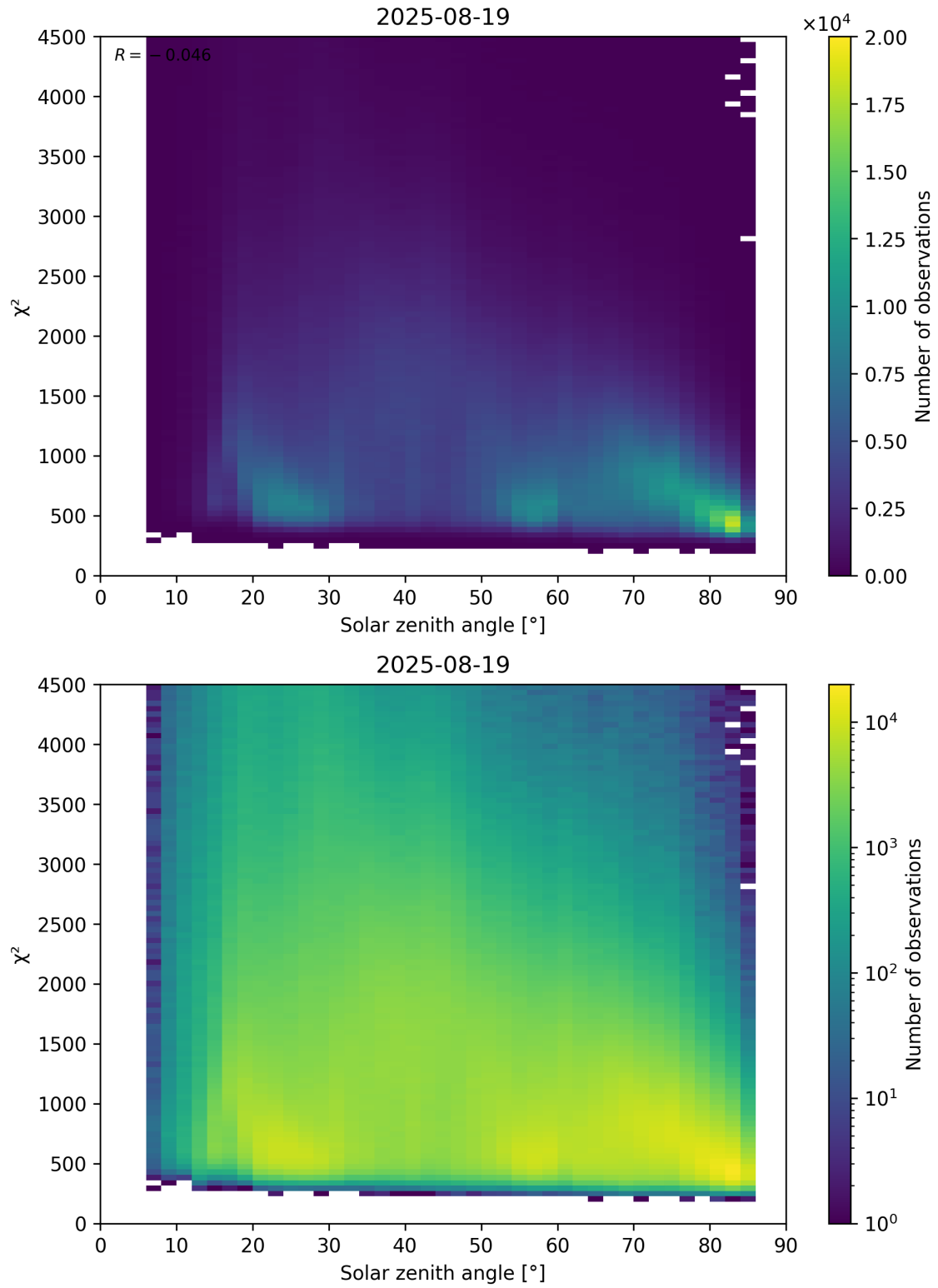
Figure 64: Scatter density plot of “Solar zenith angle” against “ \chi^2 ” for 2025-08-19 to 2025-08-20.
