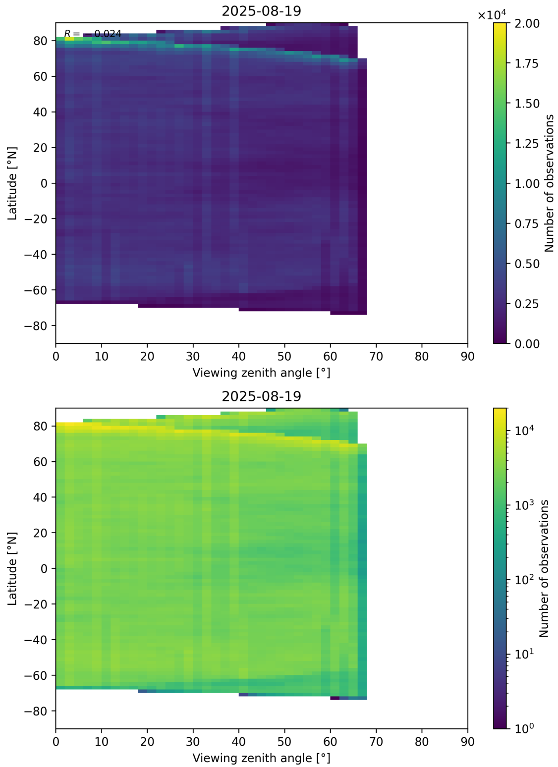
Figure 74: Scatter density plot of “Viewing zenith angle” against “Latitude” for 2025-08-19 to 2025-08-20.
