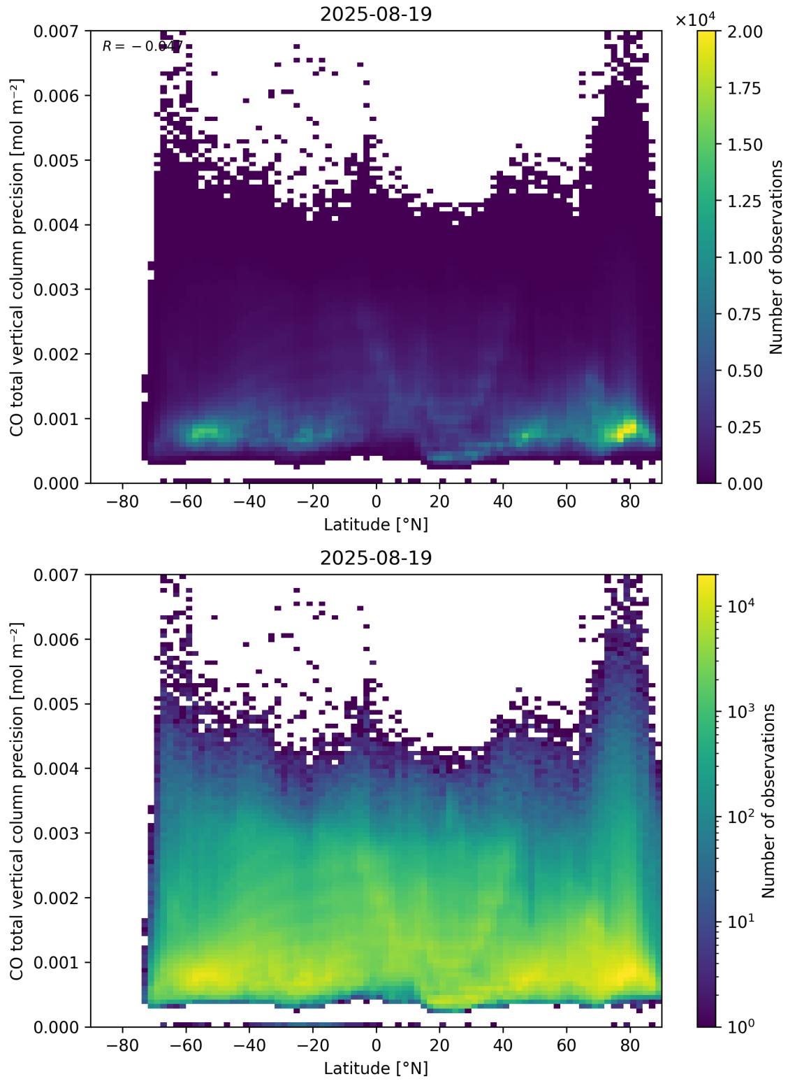
Figure 53: Scatter density plot of “Latitude” against “CO total vertical column precision” for 2025-08-19 to 2025-08-20.
