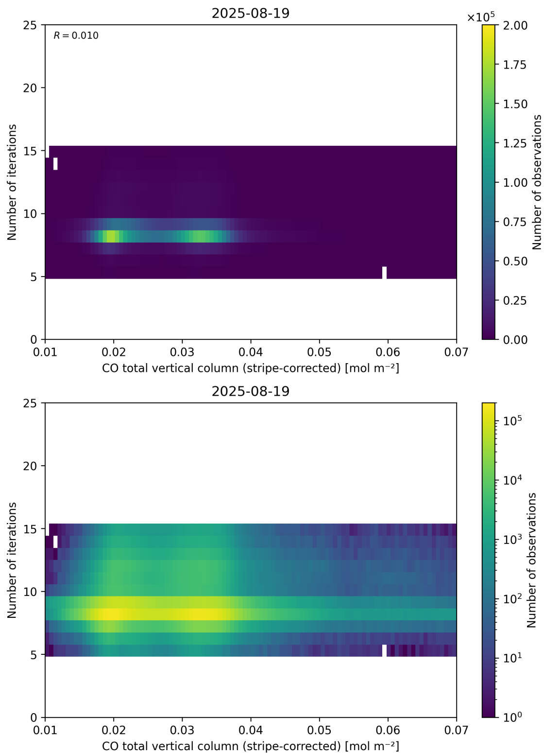
Figure 39: Scatter density plot of “CO total vertical column (stripe-corrected)” against “Number of iterations” for 2025-08-19 to 2025-08-20.
