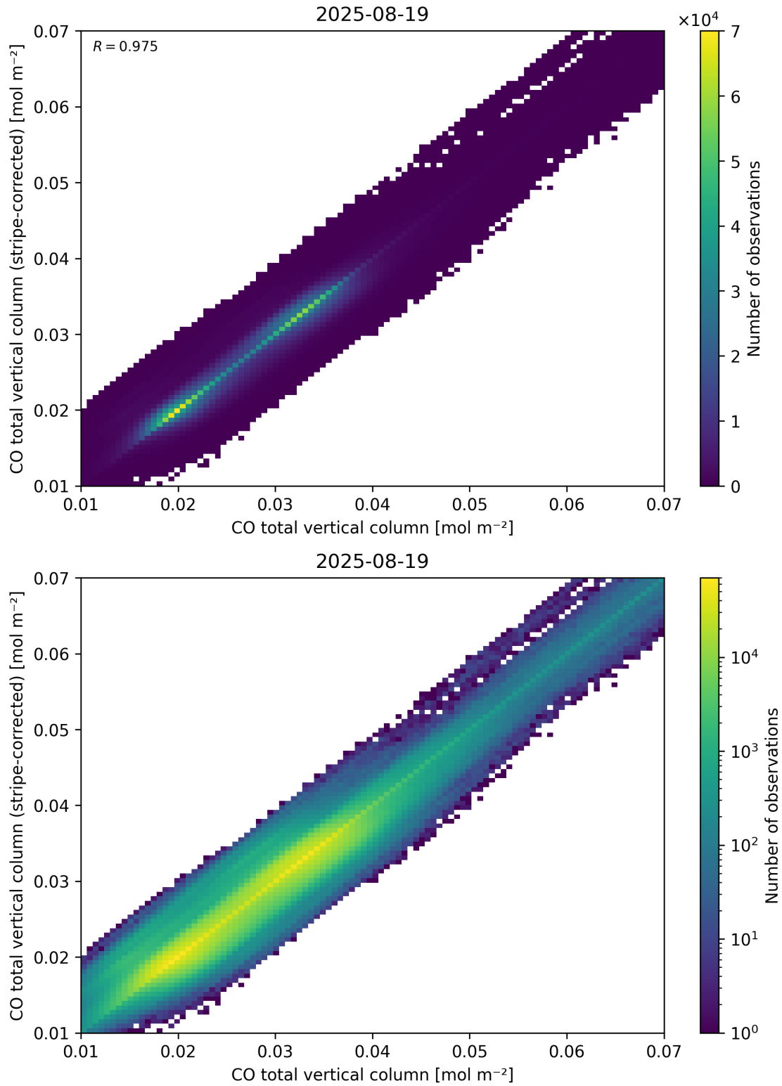
Figure 33: Scatter density plot of “CO total vertical column” against “CO total vertical column (stripe-corrected)” for 2025-08-19 to 2025-08-20.
