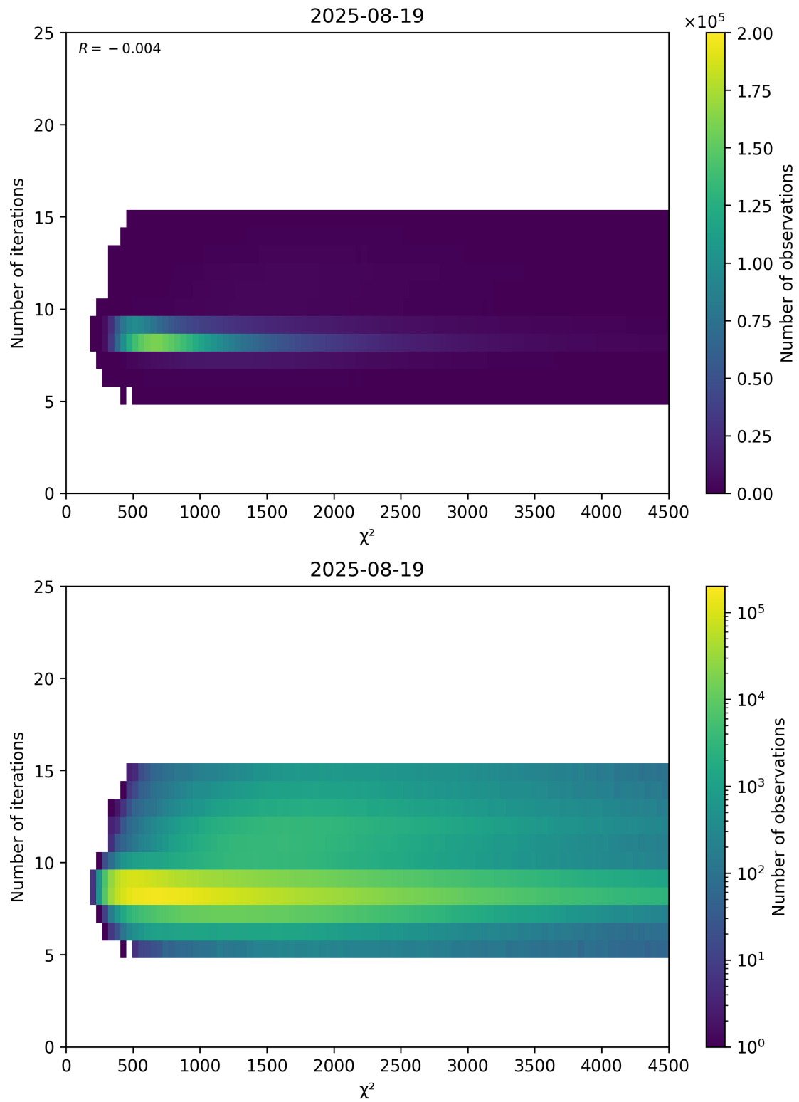
Figure 49: Scatter density plot of “ \chi^2 ” against “Number of iterations” for 2025-08-19 to 2025-08-20.
