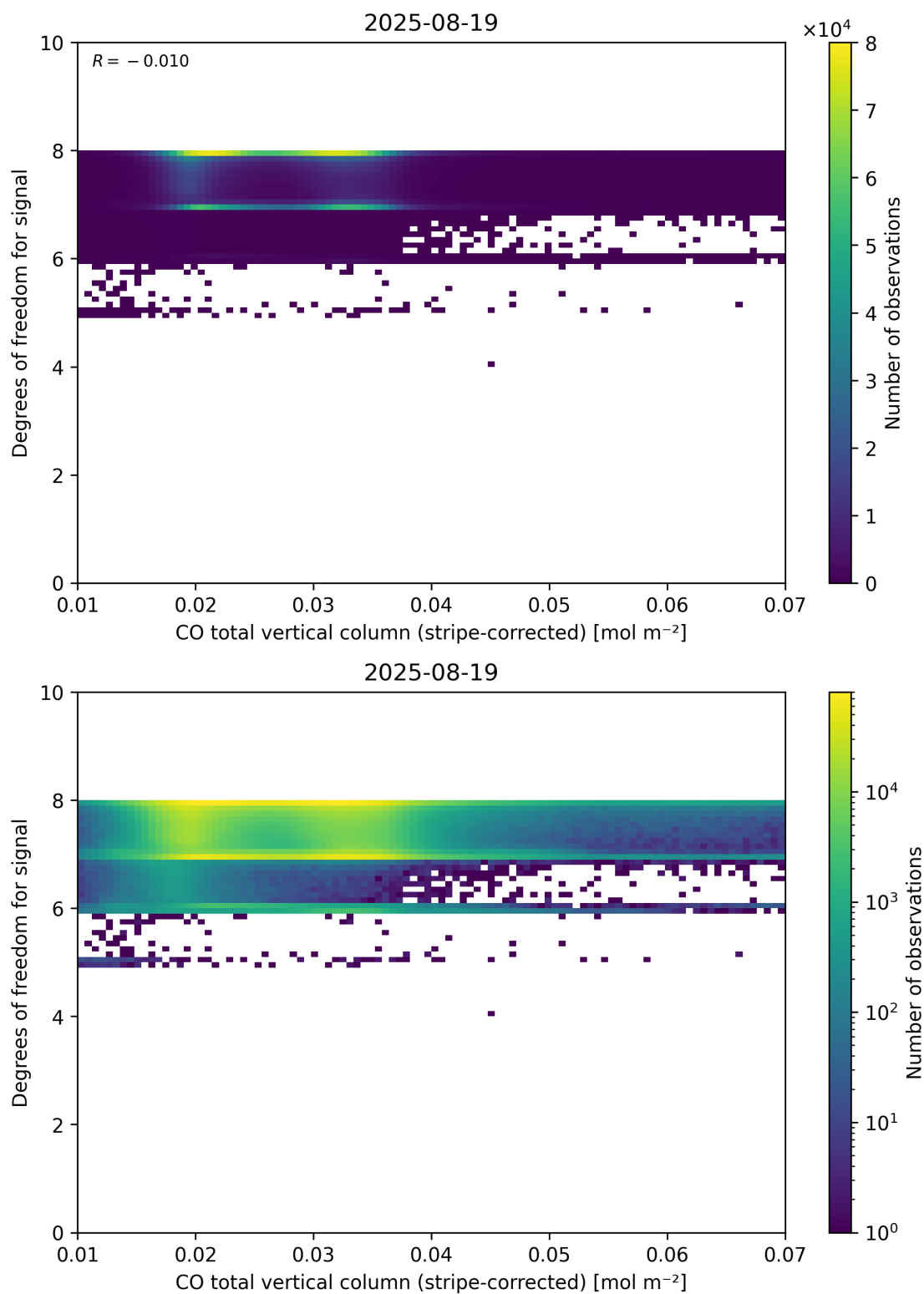
Figure 38: Scatter density plot of “CO total vertical column (stripe-corrected)” against “Degrees of freedom for signal” for 2025-08-19 to 2025-08-20.
