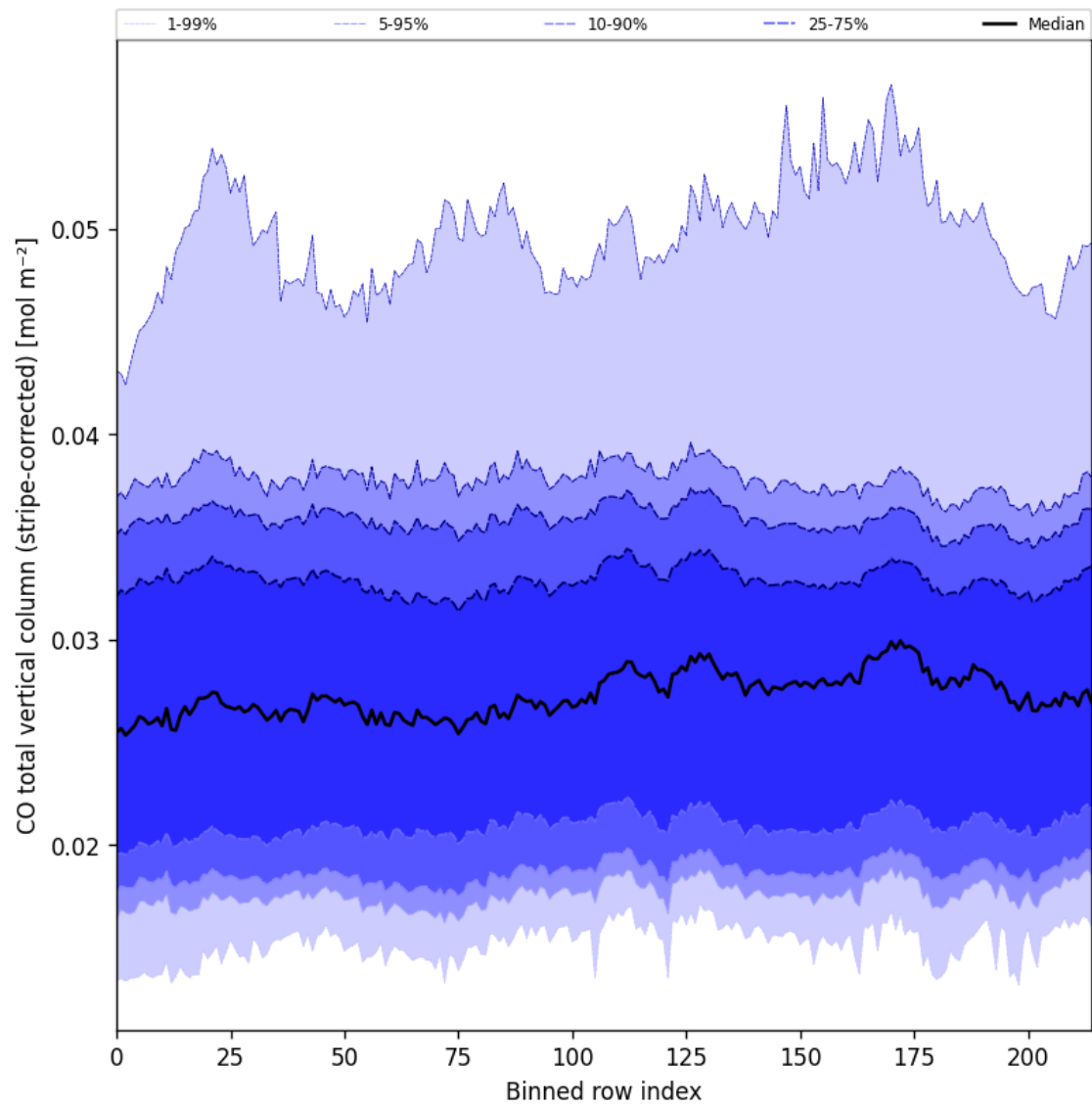
Figure 27: Along track statistics of “CO total vertical column (stripe-corrected)” for 2025-08-19 to 2025-08-20
