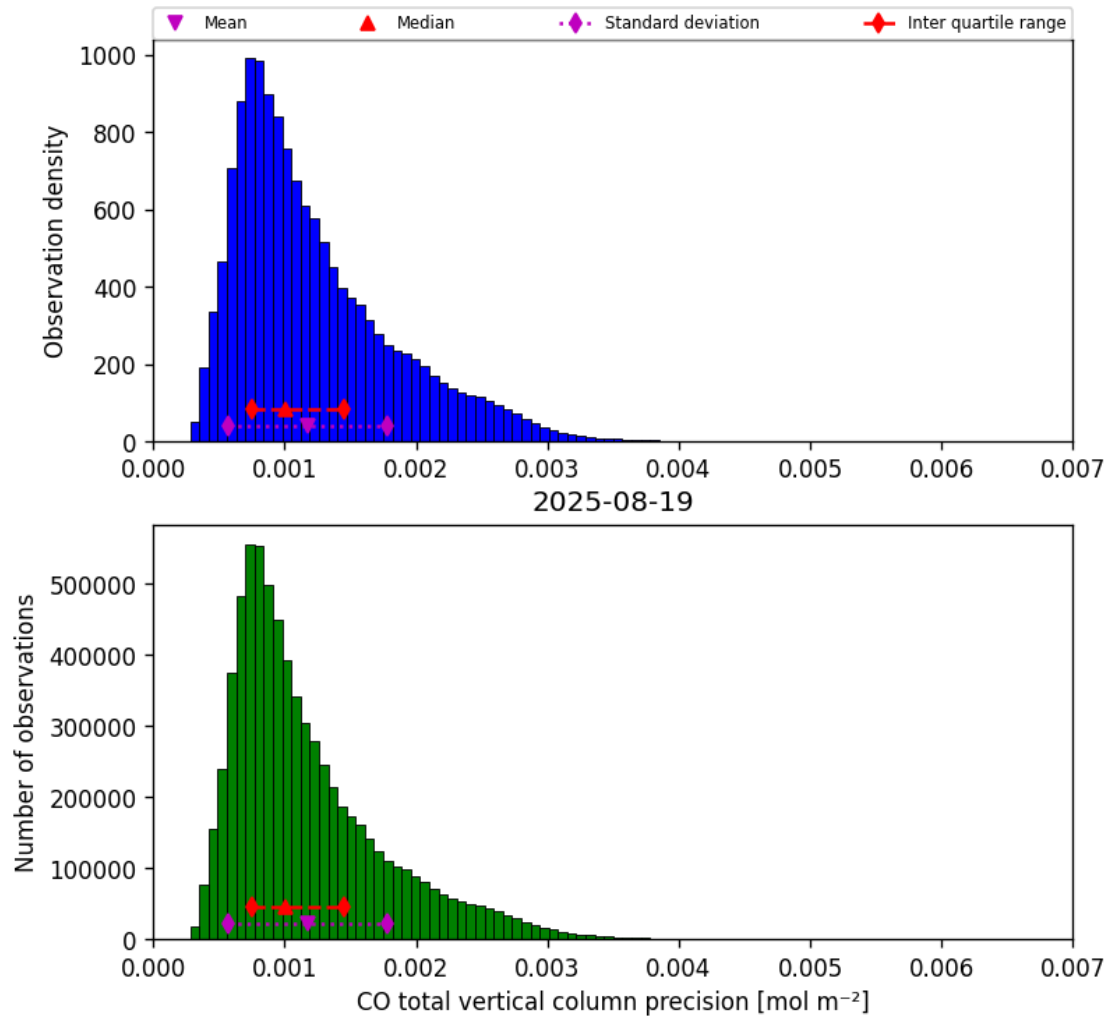
Figure 20: Histogram of “CO total vertical column precision” for 2025-08-19 to 2025-08-20
