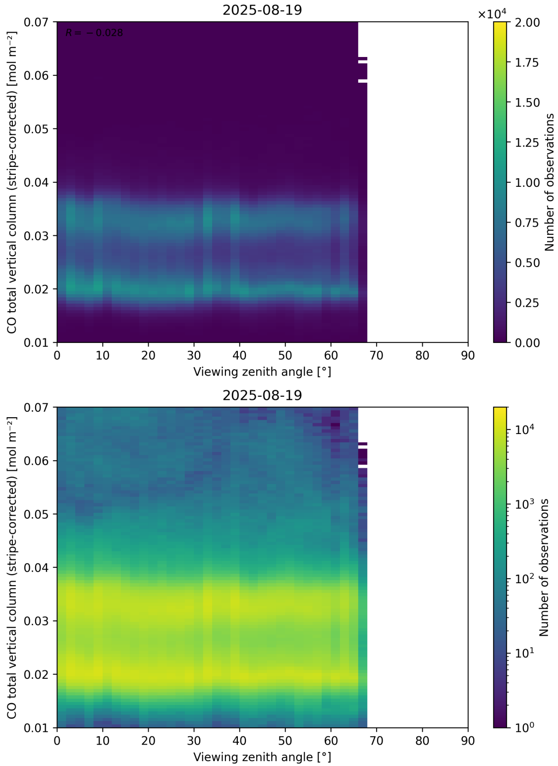
Figure 70: Scatter density plot of “Viewing zenith angle” against “CO total vertical column (stripe-corrected)” for 2025-08-19 to 2025-08-20.
