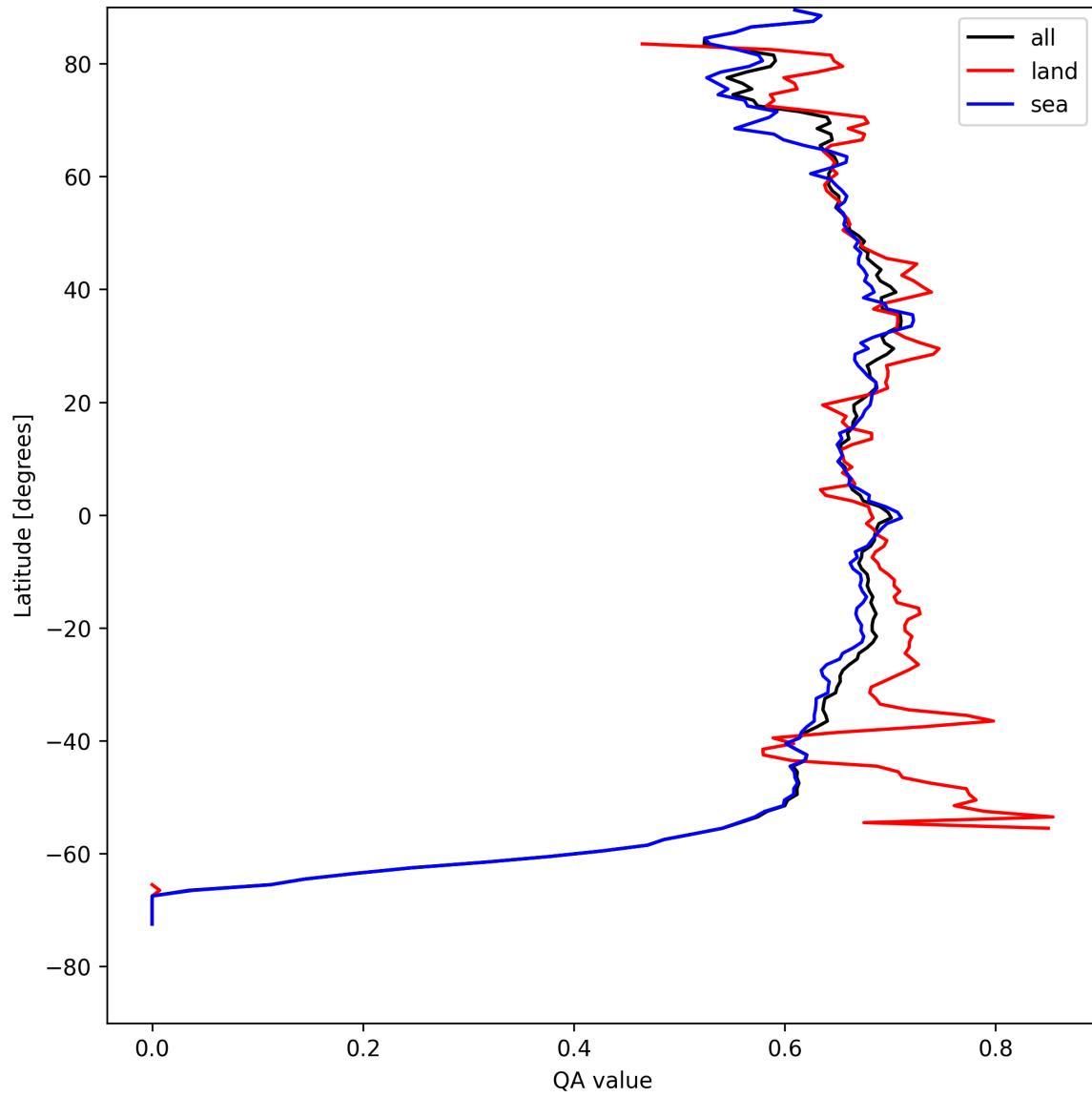
Figure 9: Zonal average of “QA value” for 2025-08-19 to 2025-08-20.
