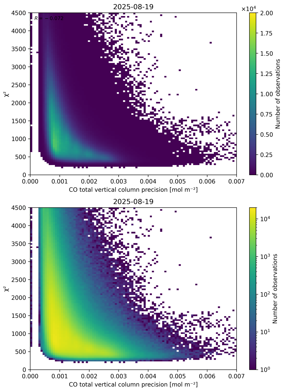
Figure 44: Scatter density plot of “CO total vertical column precision” against “ \chi^2 ” for 2025-08-19 to 2025-08-20.
