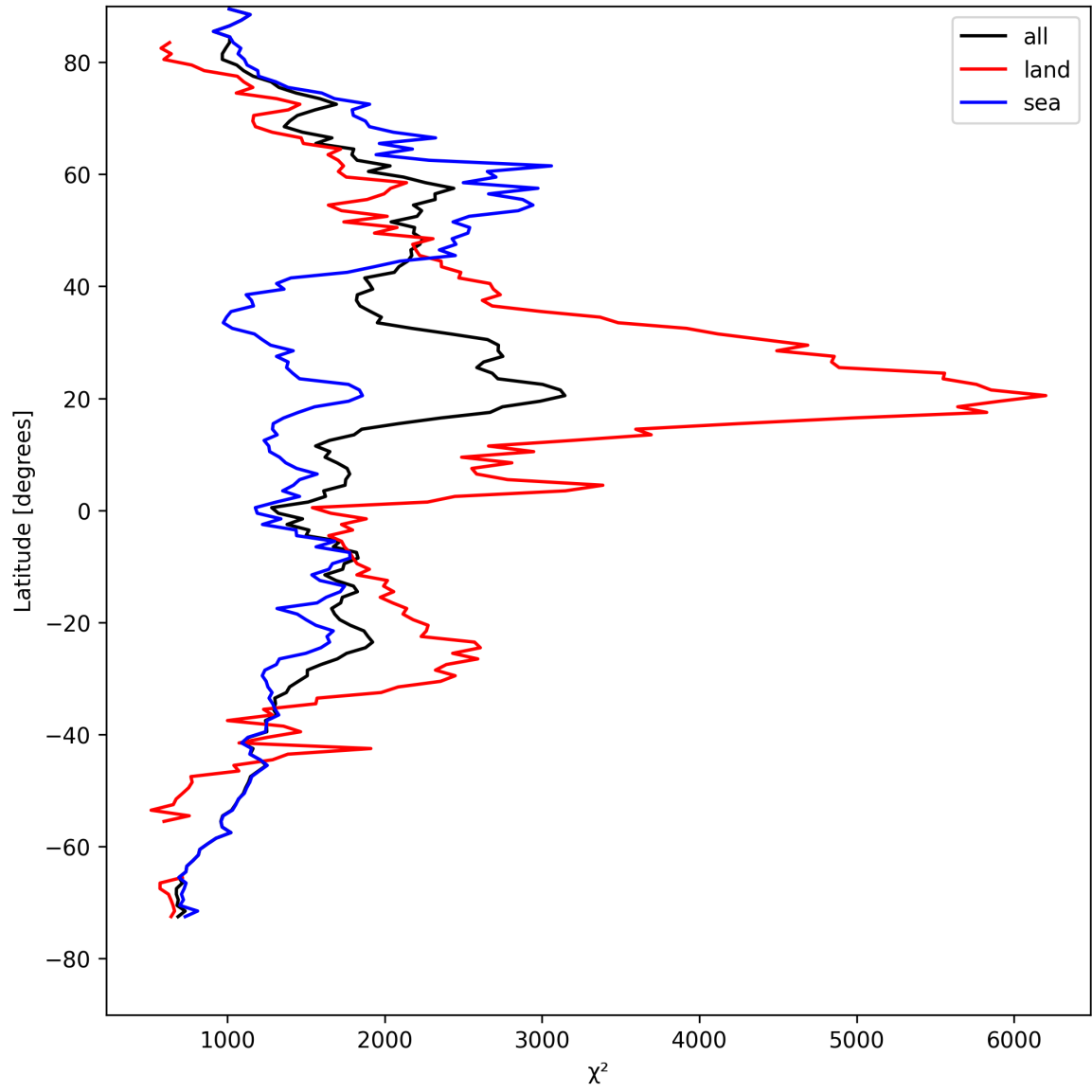
Figure 14: Zonal average of “ \chi^2 ” for 2025-08-19 to 2025-08-20.
