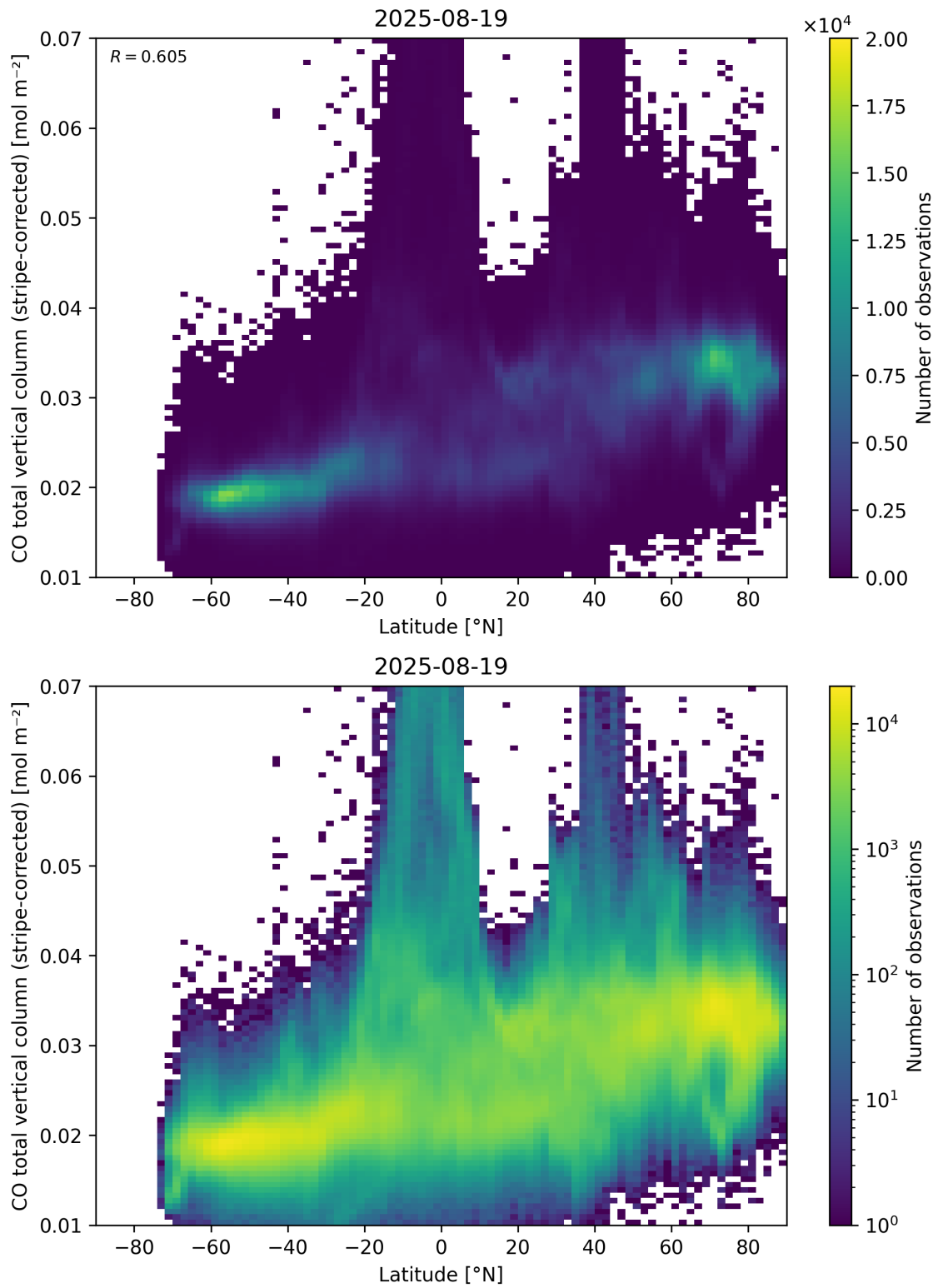
Figure 52: Scatter density plot of “Latitude” against “CO total vertical column (stripe-corrected)” for 2025-08-19 to 2025-08-20.
