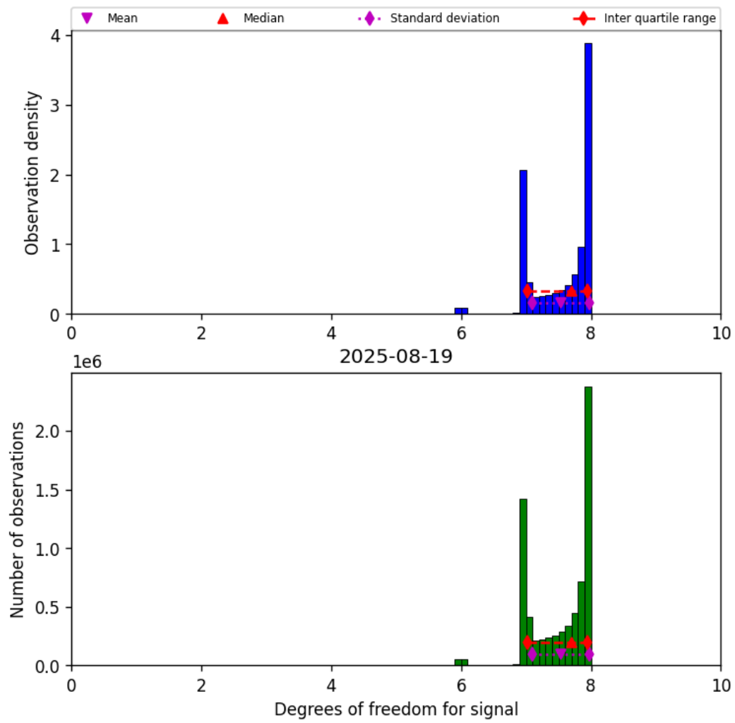
Figure 23: Histogram of “Degrees of freedom for signal” for 2025-08-19 to 2025-08-20
