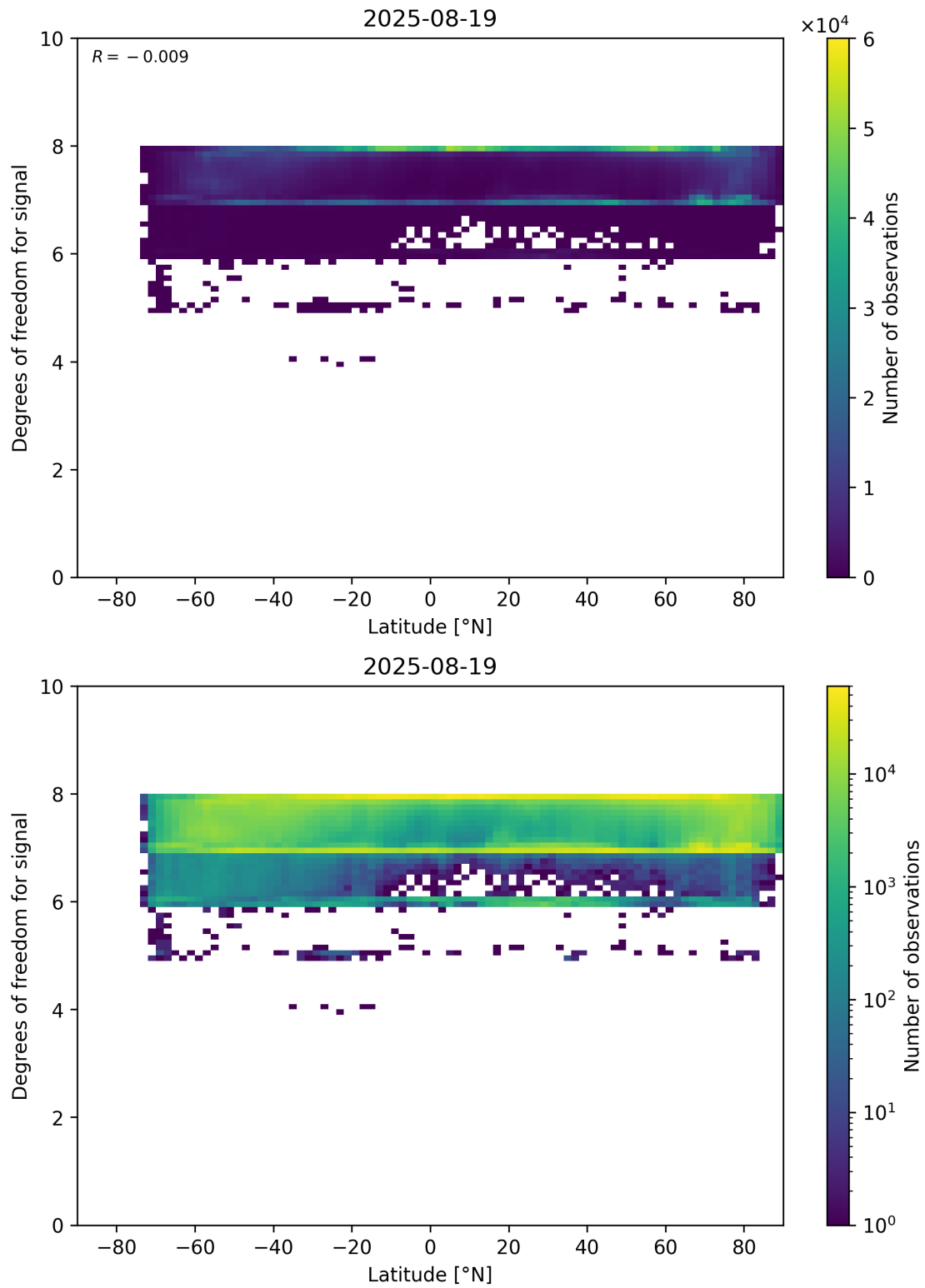
Figure 55: Scatter density plot of “Latitude” against “Degrees of freedom for signal” for 2025-08-19 to 2025-08-20.
