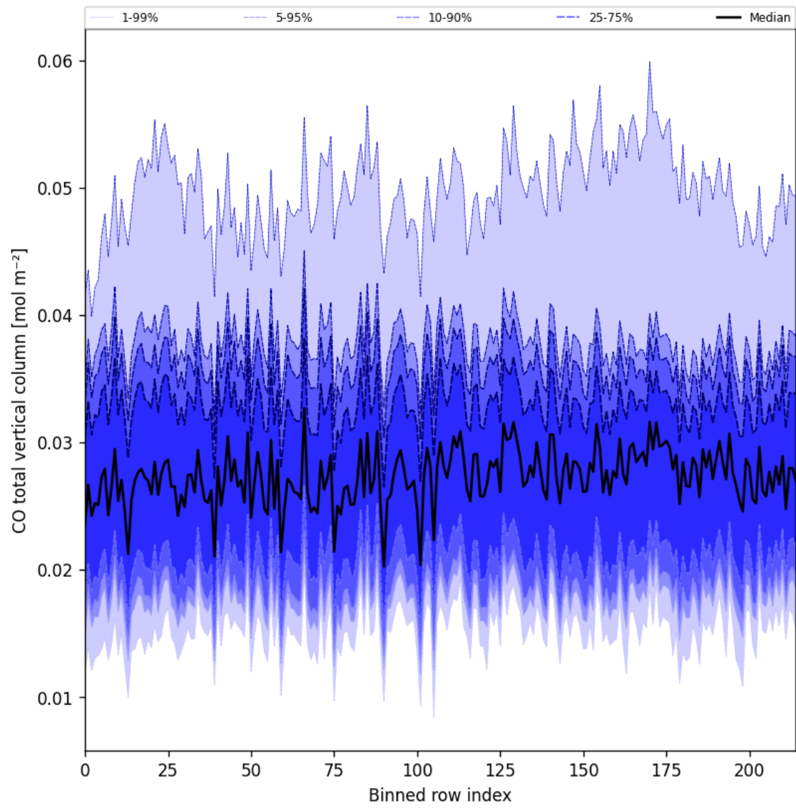
Figure 26: Along track statistics of “CO total vertical column” for 2025-08-19 to 2025-08-20
