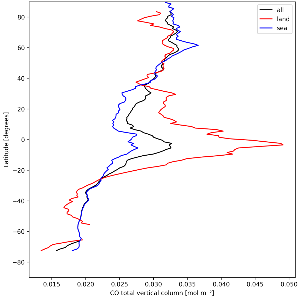
Figure 10: Zonal average of “CO total vertical column” for 2025-08-19 to 2025-08-20.
