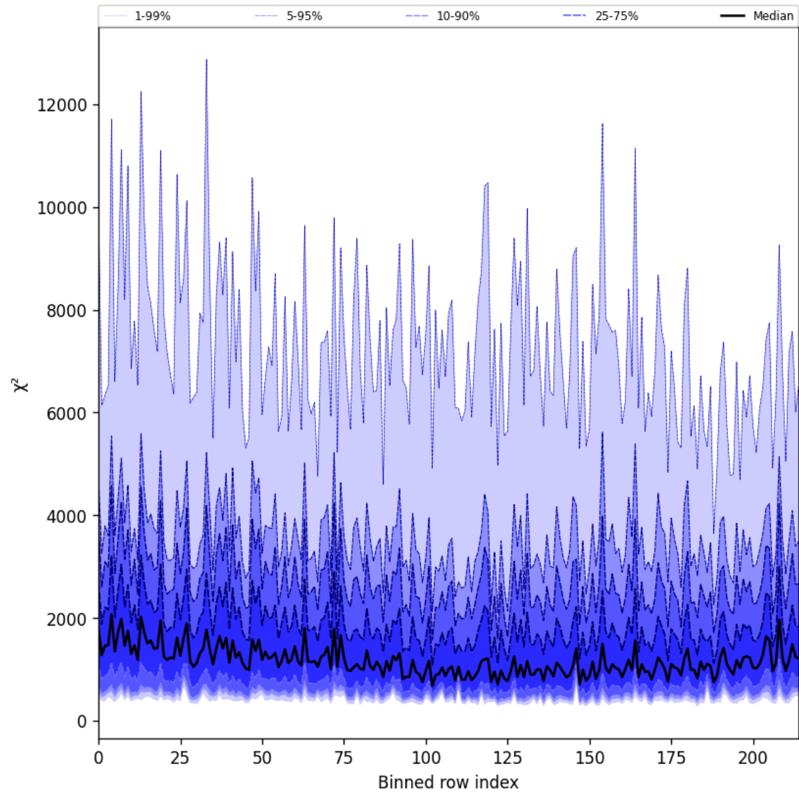
Figure 30: Along track statistics of “ \chi^2 ” for 2025-08-19 to 2025-08-20
