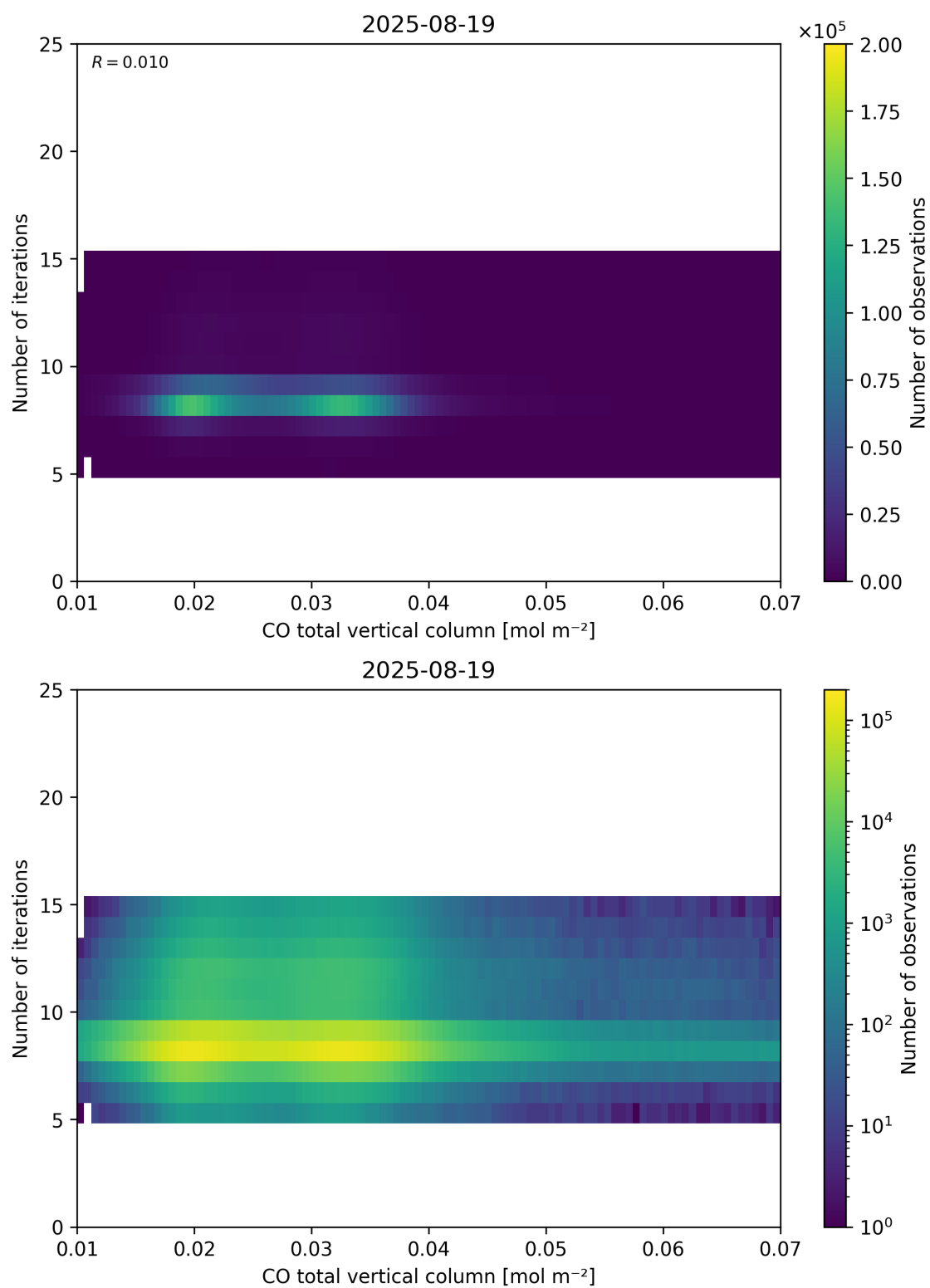
Figure 42: Scatter density plot of “CO total vertical column” against “Number of iterations” for 2025-08-19 to 2025-08-20.
