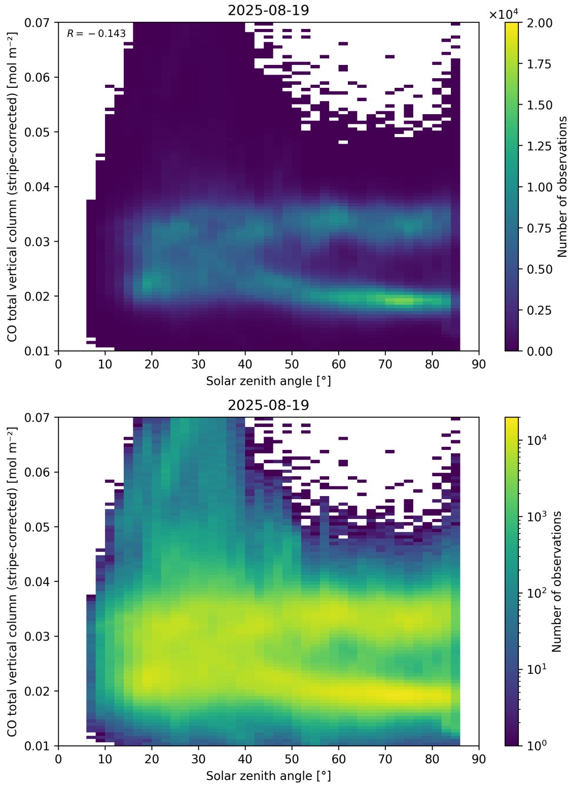
Figure 62: Scatter density plot of “Solar zenith angle” against “CO total vertical column (stripe-corrected)” for 2025-08-19 to 2025-08-20.
