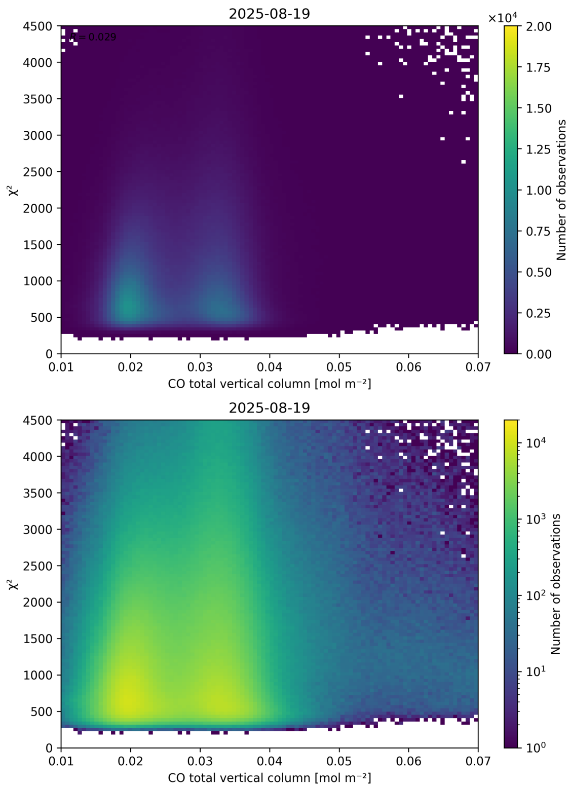
Figure 35: Scatter density plot of “CO total vertical column” against “ \chi^2 ” for 2025-08-19 to 2025-08-20.
