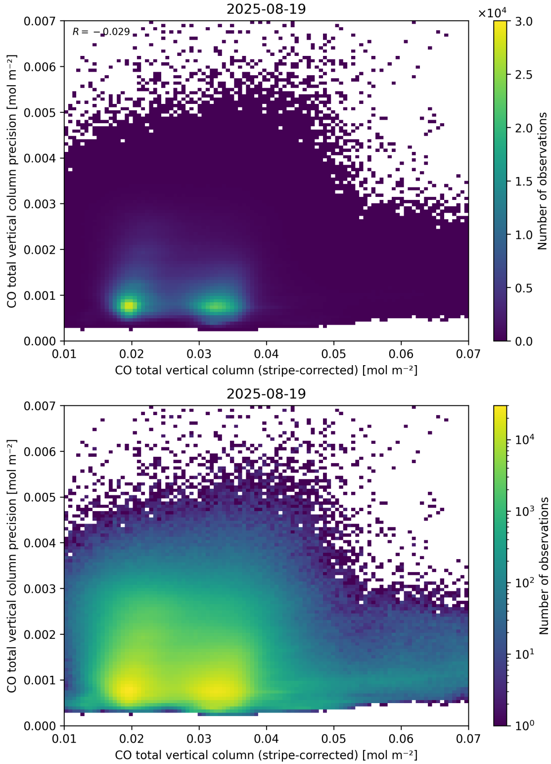
Figure 36: Scatter density plot of “CO total vertical column (stripe-corrected)” against “CO total vertical column precision” for 2025-08-19 to 2025-08-20.
