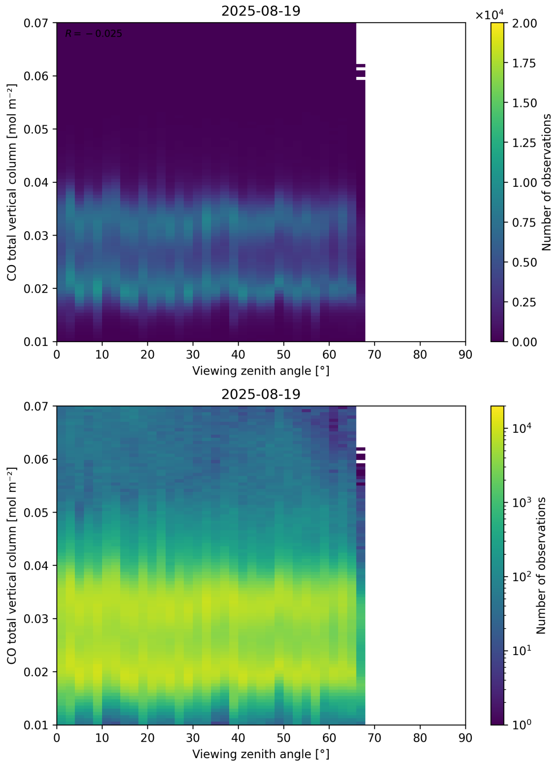
Figure 69: Scatter density plot of “Viewing zenith angle” against “CO total vertical column” for 2025-08-19 to 2025-08-20.
