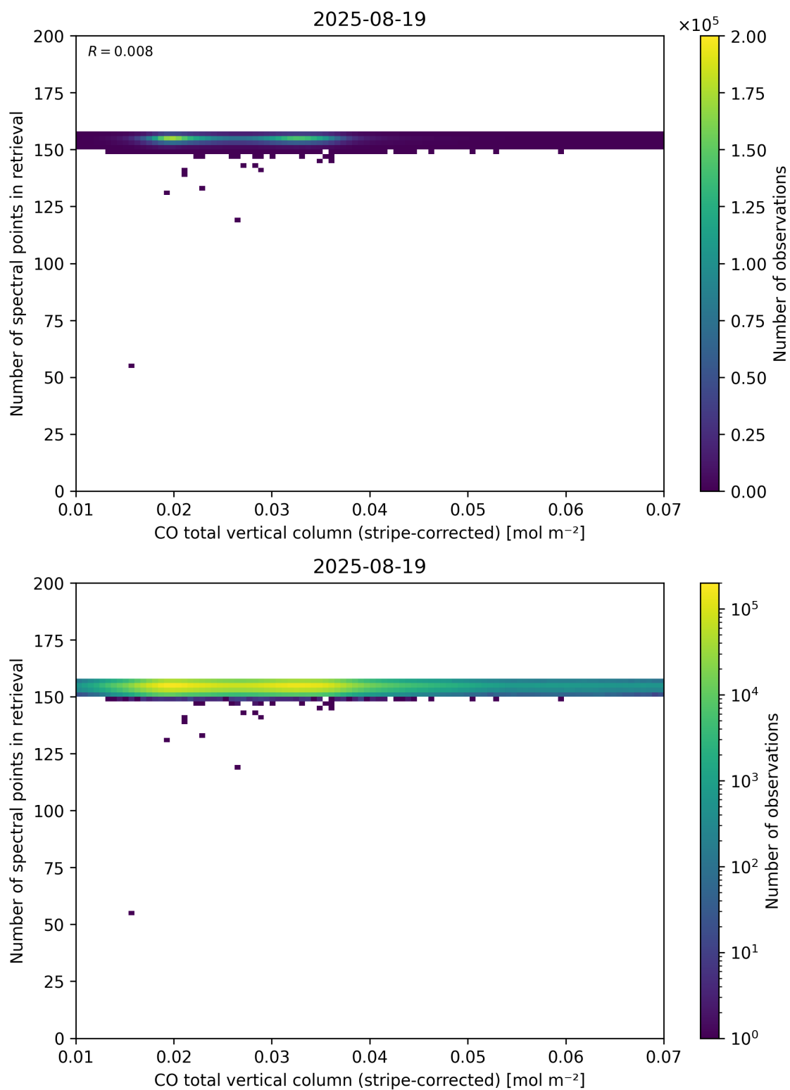
Figure 40: Scatter density plot of “CO total vertical column (stripe-corrected)” against “Number of spectral points in retrieval” for 2025-08-19 to 2025-08-20.
