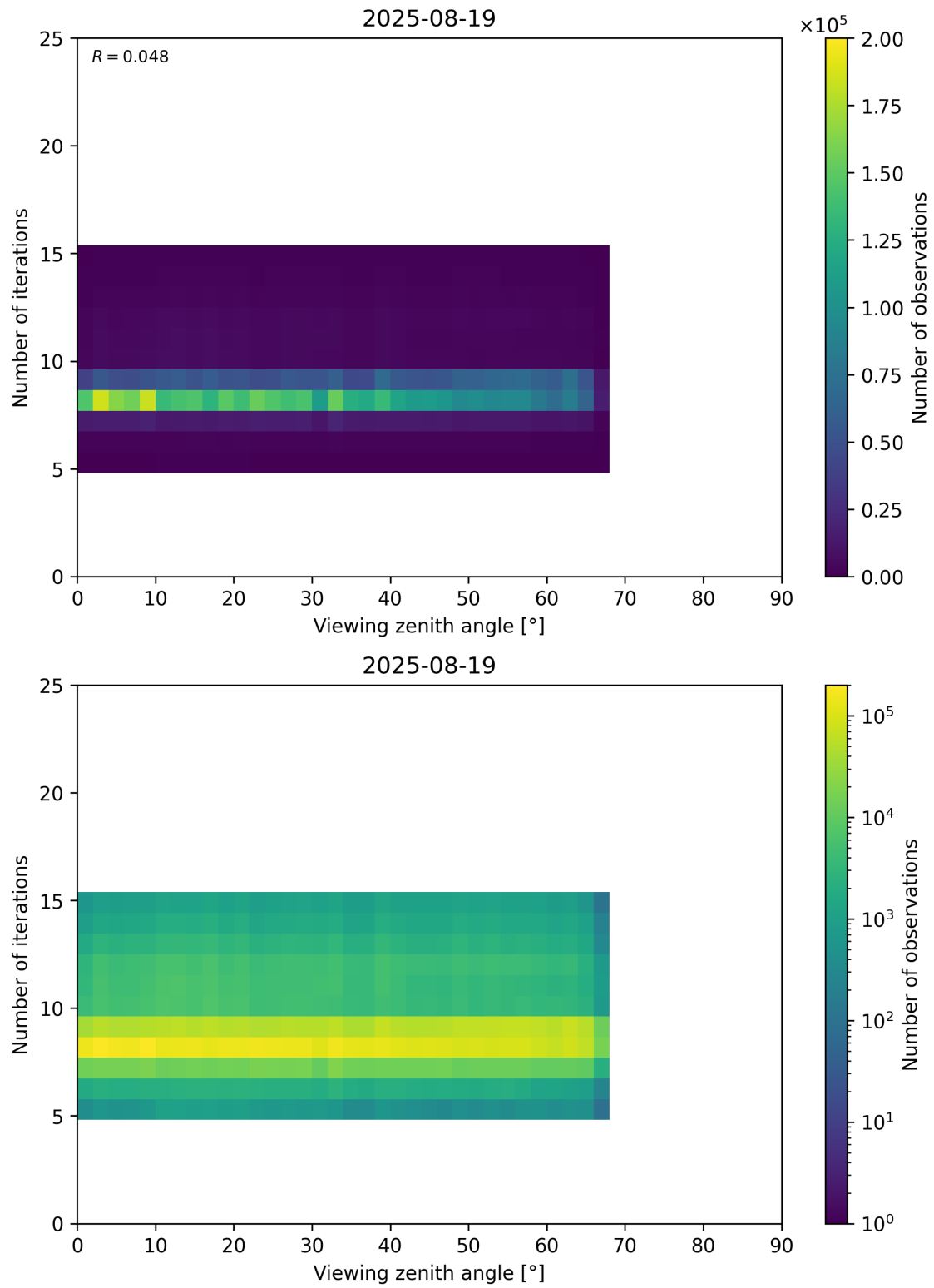
Figure 75: Scatter density plot of “Viewing zenith angle” against “Number of iterations” for 2025-08-19 to 2025-08-20.
