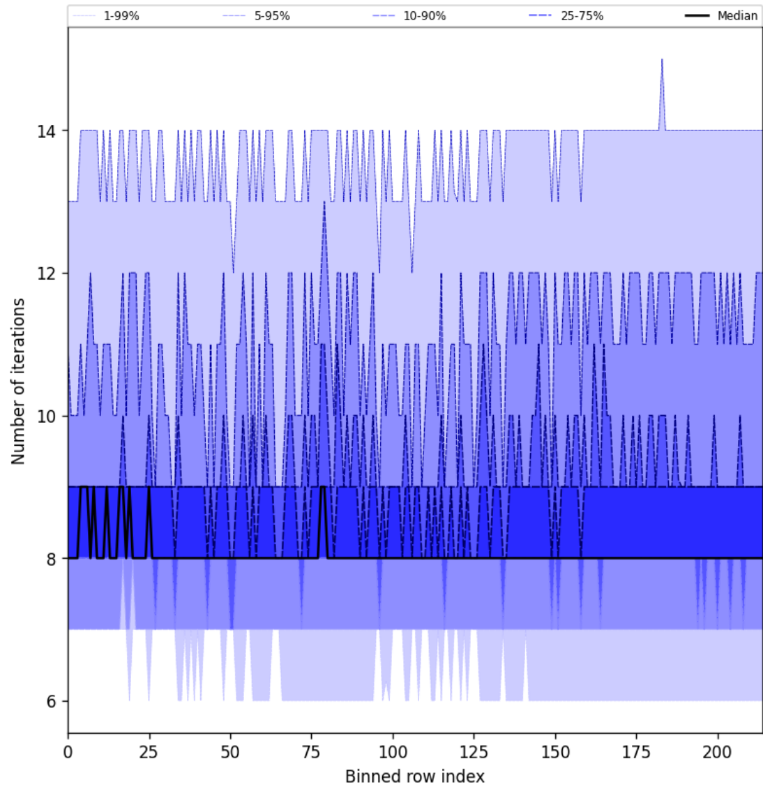
Figure 32: Along track statistics of “Number of iterations” for 2025-08-19 to 2025-08-20
