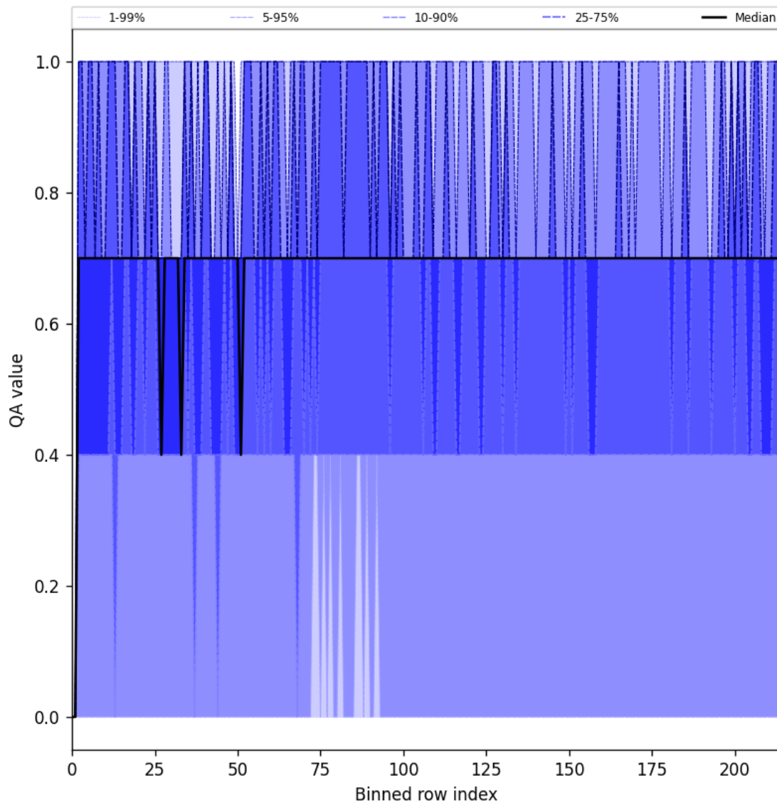
Figure 25: Along track statistics of “QA value” for 2025-08-19 to 2025-08-20
