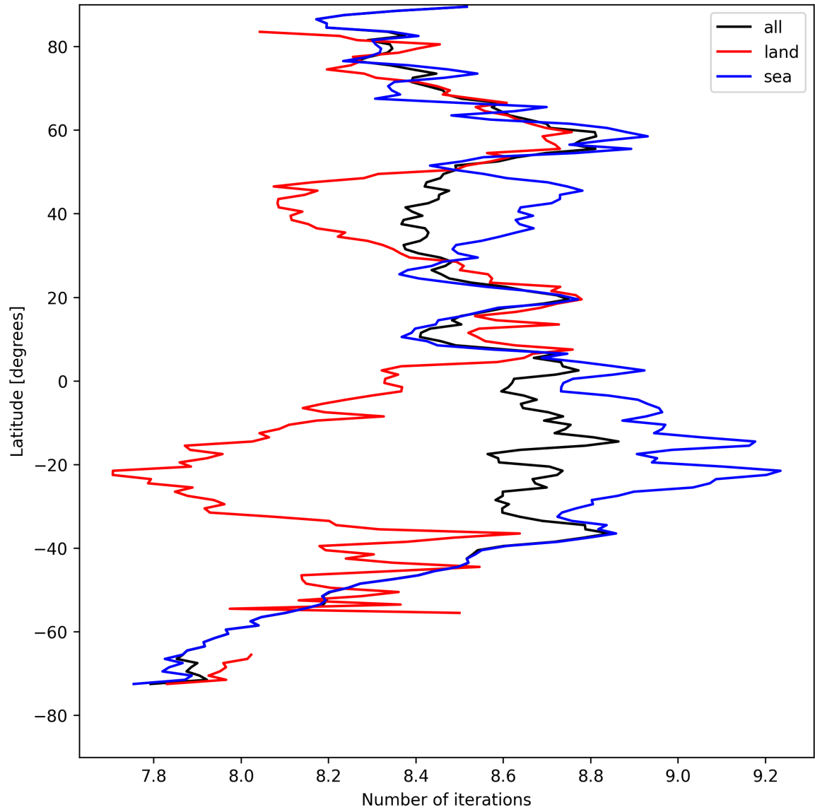
Figure 16: Zonal average of “Number of iterations” for 2025-08-19 to 2025-08-20.
