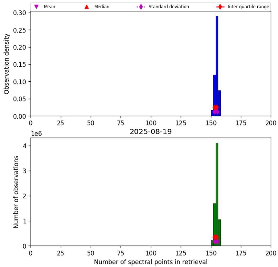
Figure 21: Histogram of “Number of spectral points in retrieval” for 2025-08-19 to 2025-08-20
