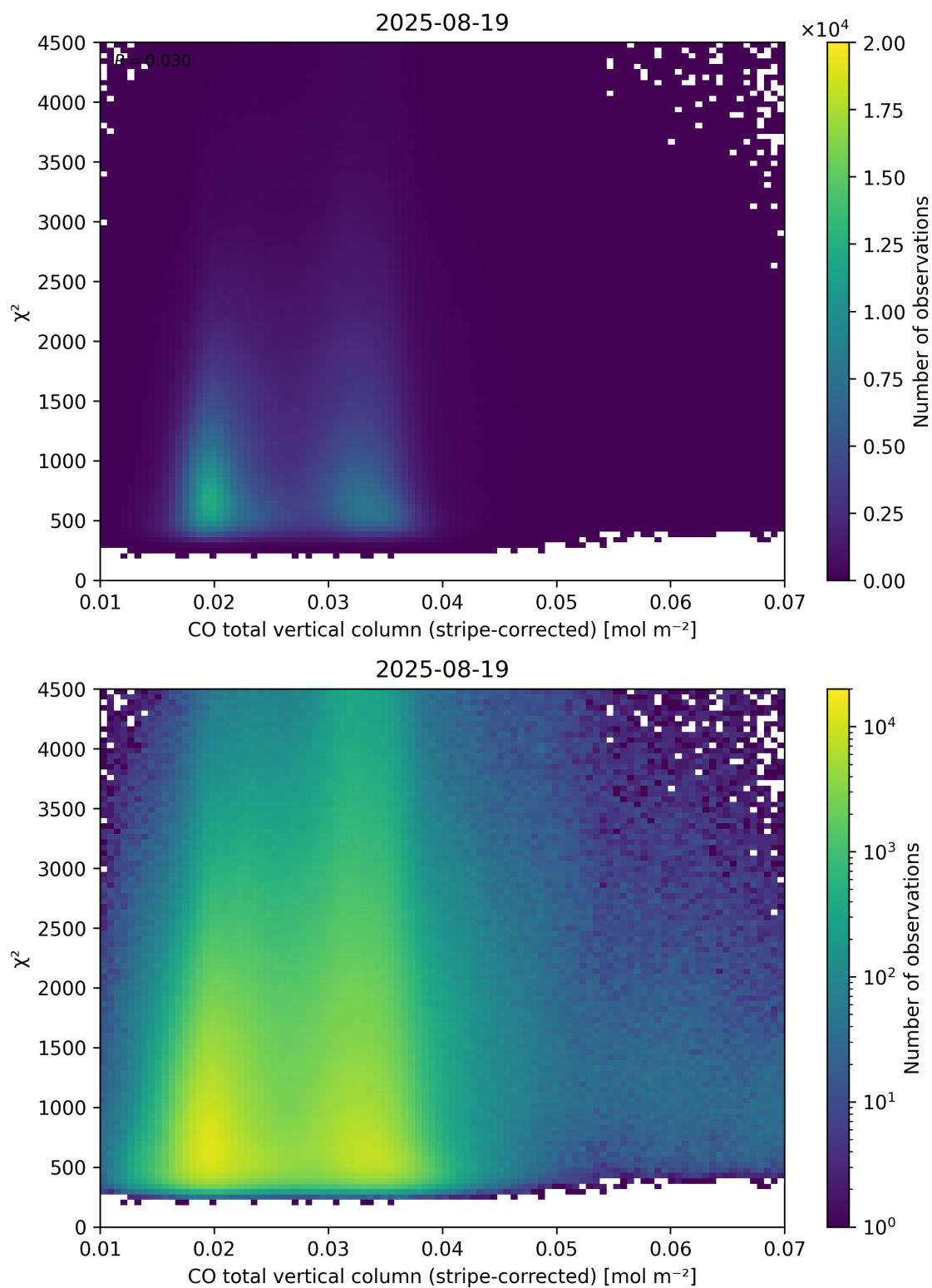
Figure 37: Scatter density plot of “CO total vertical column (stripe-corrected)” against “ \chi^2 ” for 2025-08-19 to 2025-08-20.
