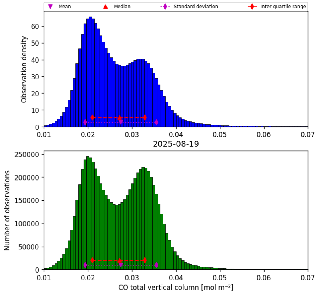
Figure 18: Histogram of “CO total vertical column” for 2025-08-19 to 2025-08-20
