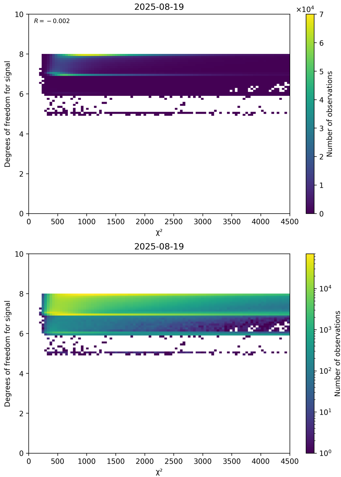
Figure 48: Scatter density plot of “ \chi^2 ” against “Degrees of freedom for signal” for 2025-08-19 to 2025-08-20.
