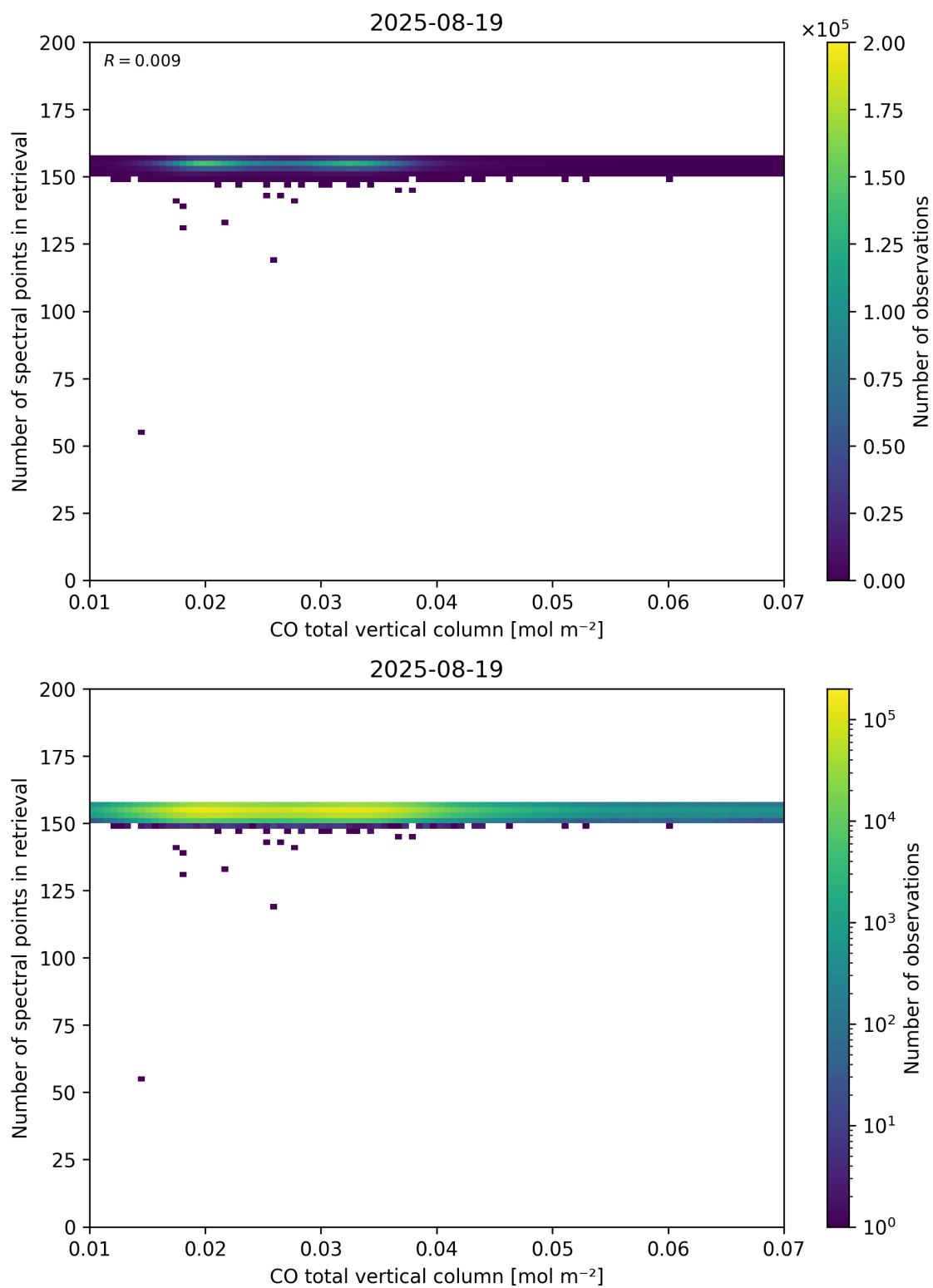
Figure 43: Scatter density plot of “CO total vertical column” against “Number of spectral points in retrieval” for 2025-08-19 to 2025-08-20.
