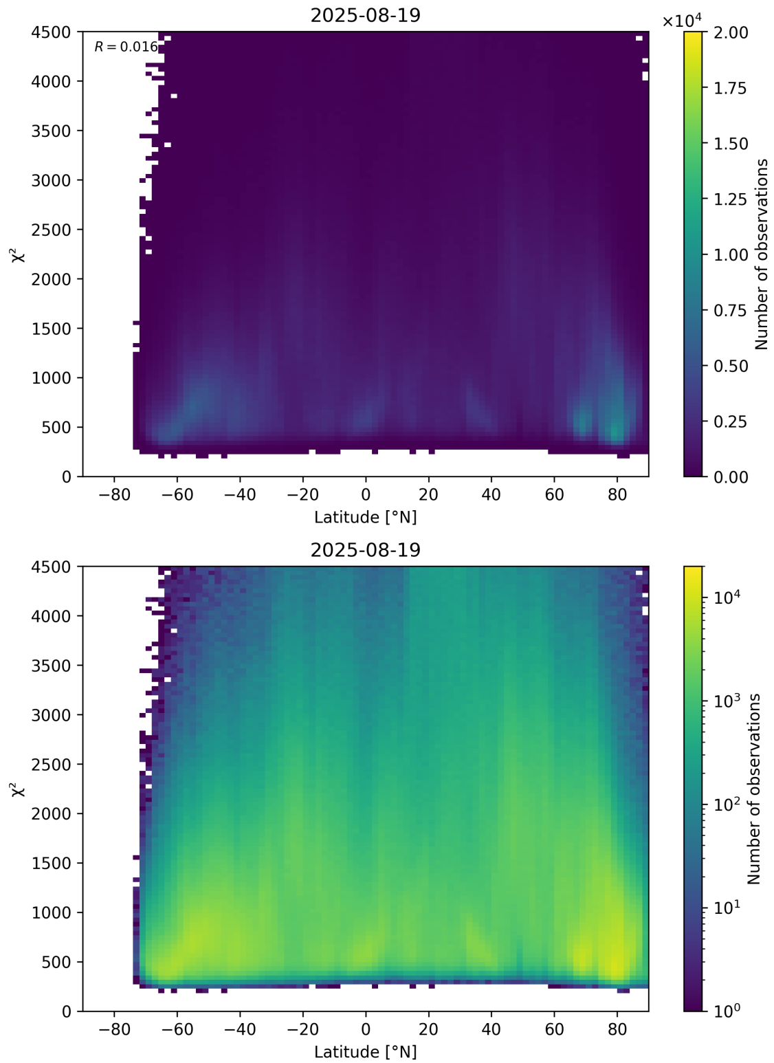
Figure 54: Scatter density plot of “Latitude” against “ \chi^2 ” for 2025-08-19 to 2025-08-20.
