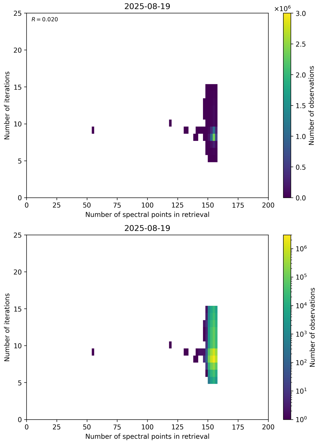
Figure 60: Scatter density plot of “Number of spectral points in retrieval” against “Number of iterations” for 2025-08-19 to 2025-08-20.
