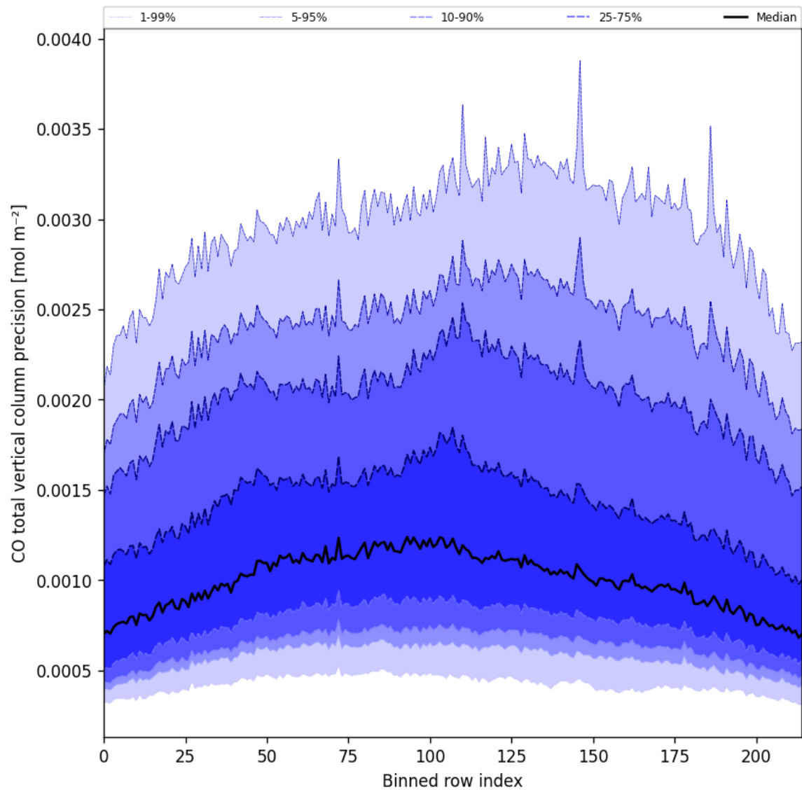
Figure 28: Along track statistics of “CO total vertical column precision” for 2025-08-19 to 2025-08-20
