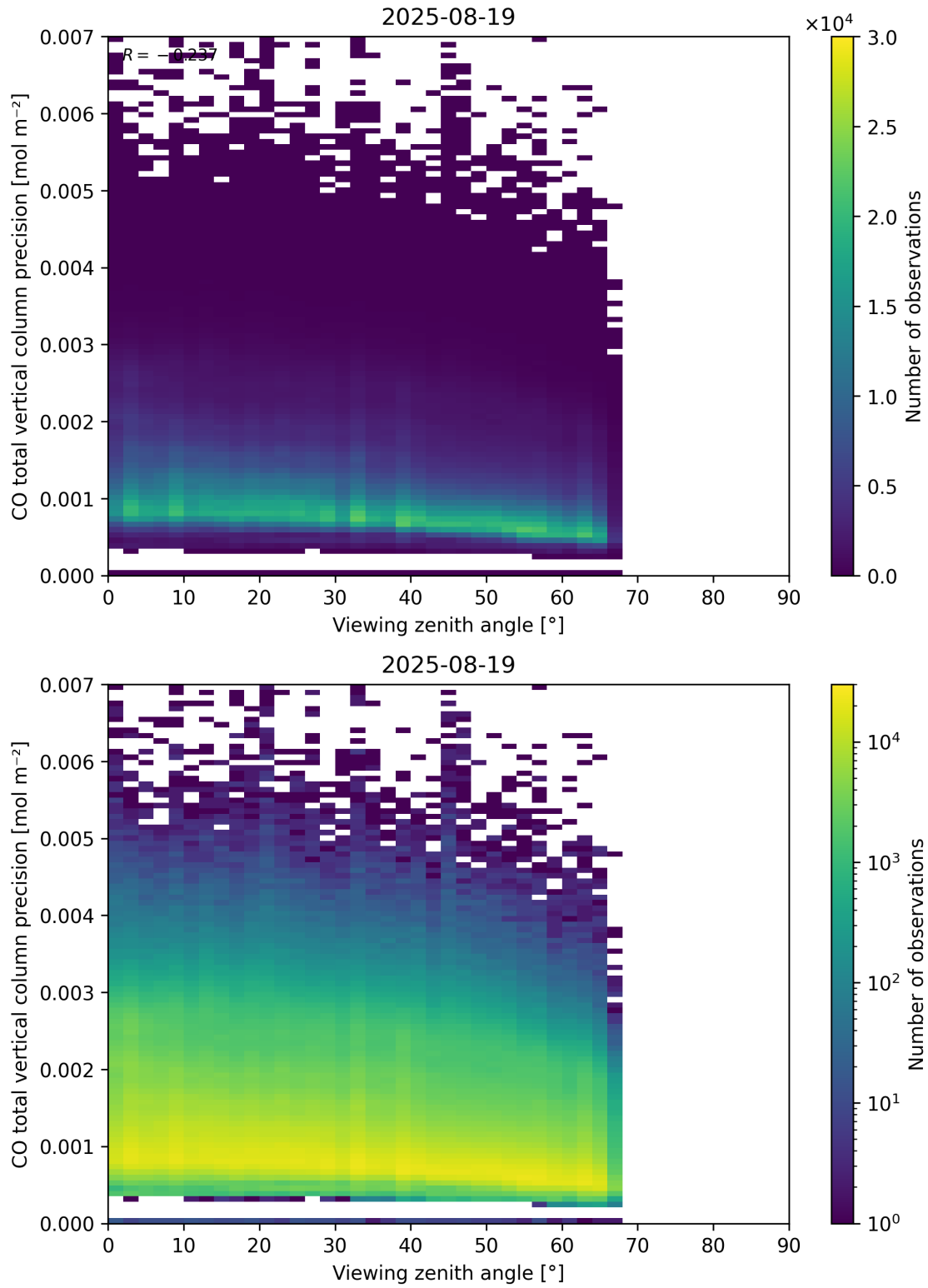
Figure 71: Scatter density plot of “Viewing zenith angle” against “CO total vertical column precision” for 2025-08-19 to 2025-08-20.
