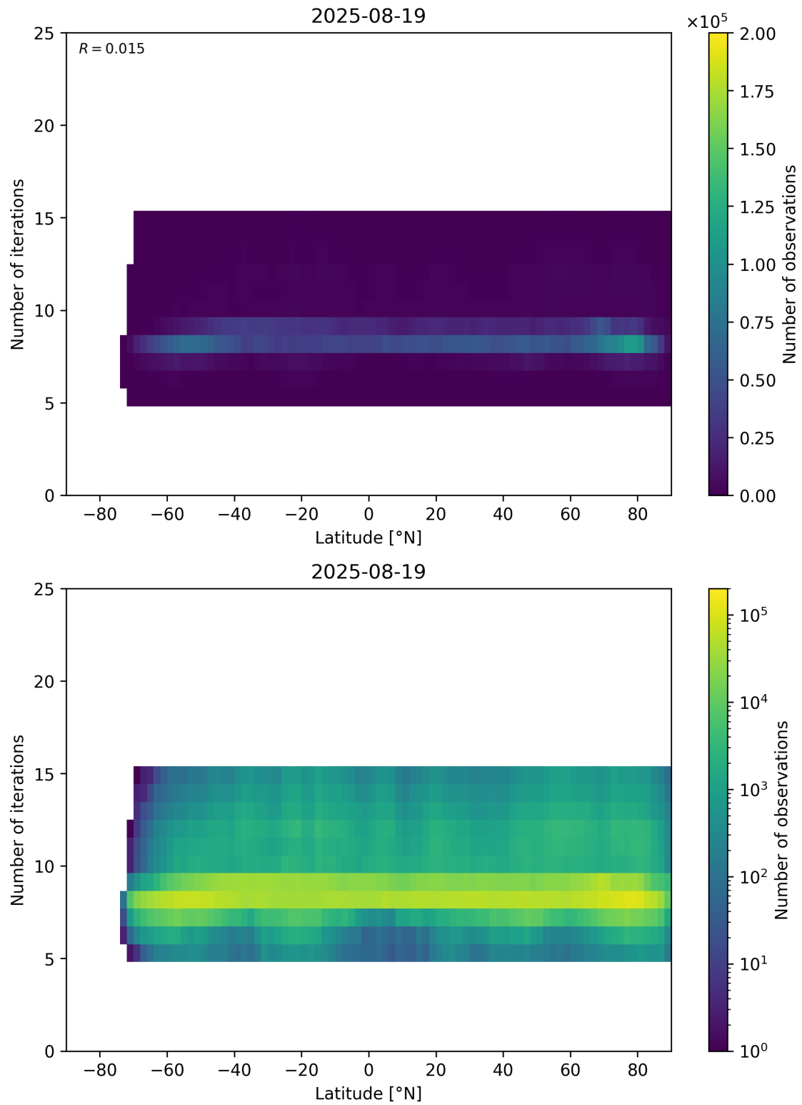
Figure 56: Scatter density plot of “Latitude” against “Number of iterations” for 2025-08-19 to 2025-08-20.
