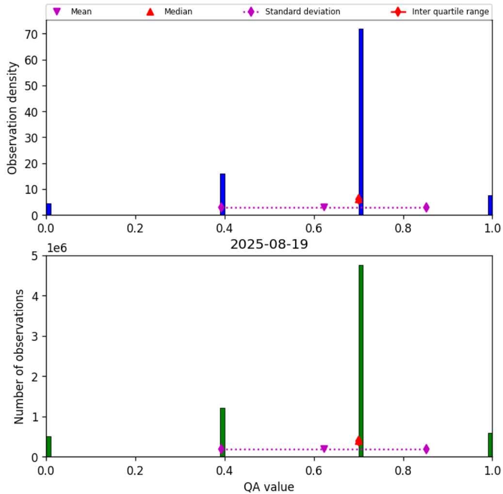
Figure 17: Histogram of “QA value” for 2025-08-19 to 2025-08-20
