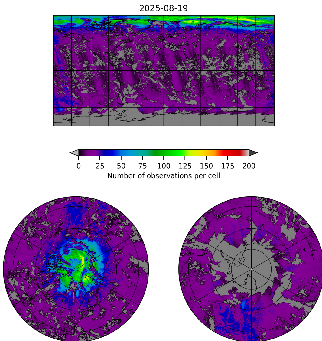
Figure 8: Map of the number of observations for 2025-08-19 to 2025-08-20
