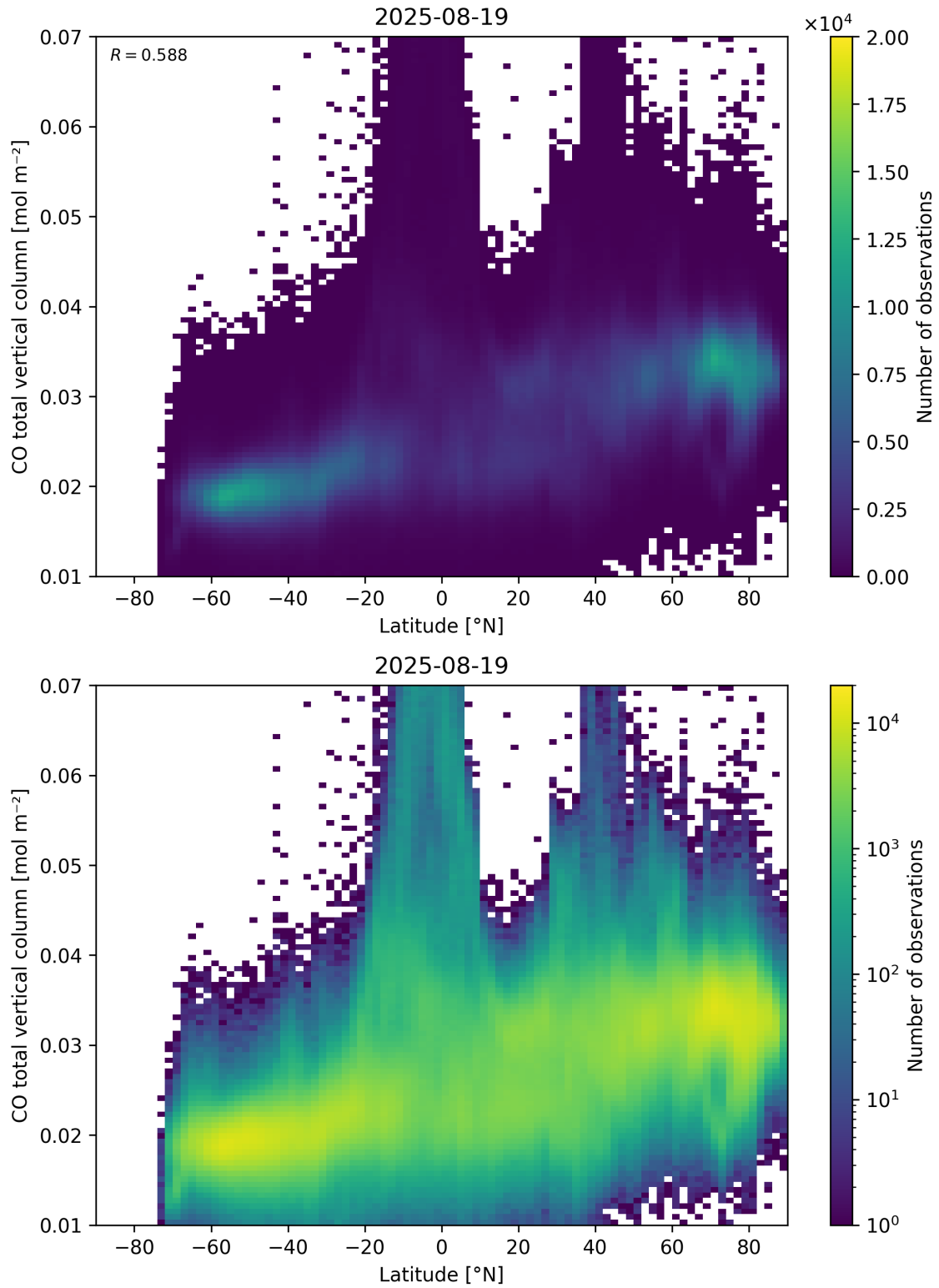
Figure 51: Scatter density plot of “Latitude” against “CO total vertical column” for 2025-08-19 to 2025-08-20.
