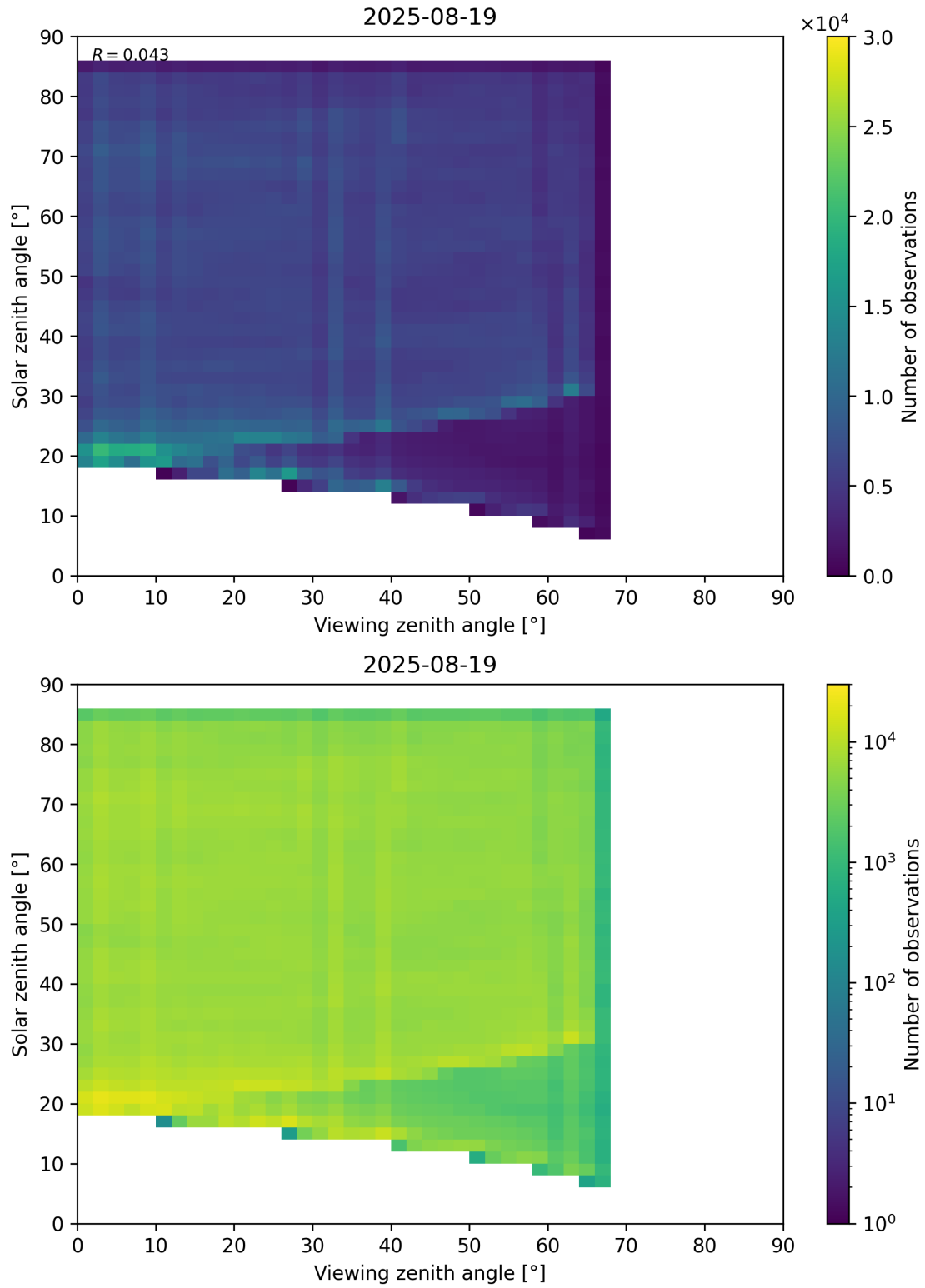
Figure 77: Scatter density plot of “Viewing zenith angle” against “Solar zenith angle” for 2025-08-19 to 2025-08-20.
