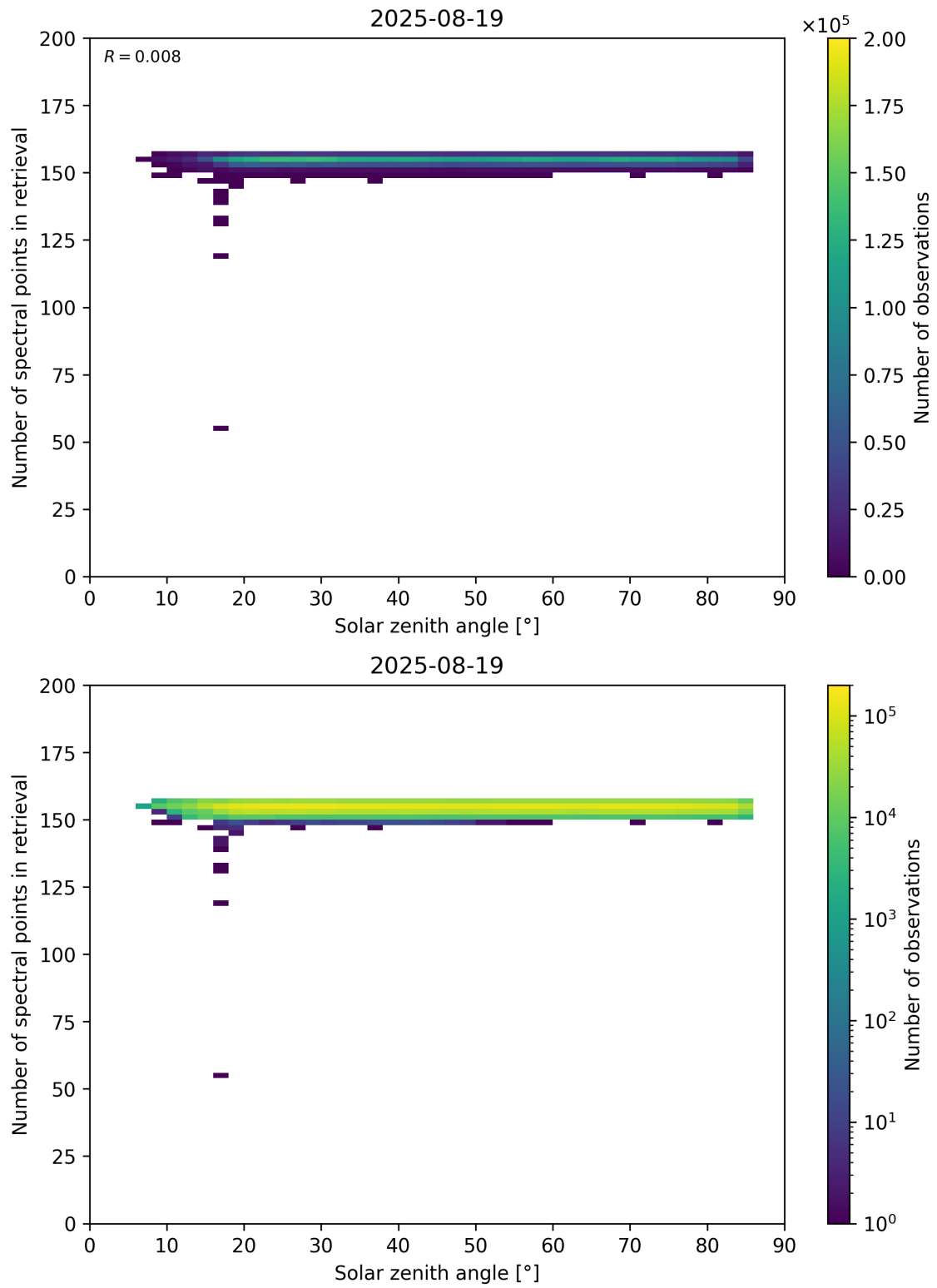
Figure 68: Scatter density plot of “Solar zenith angle” against “Number of spectral points in retrieval” for 2025-08-19 to 2025-08-20.
