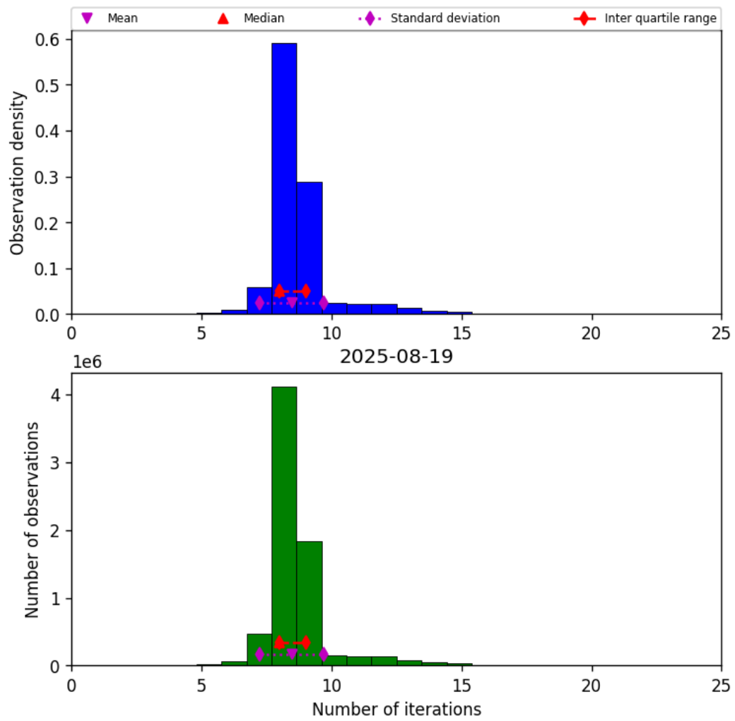
Figure 24: Histogram of “Number of iterations” for 2025-08-19 to 2025-08-20
