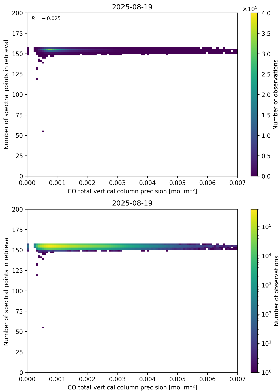
Figure 47: Scatter density plot of “CO total vertical column precision” against “Number of spectral points in retrieval” for 2025-08-19 to 2025-08-20.
