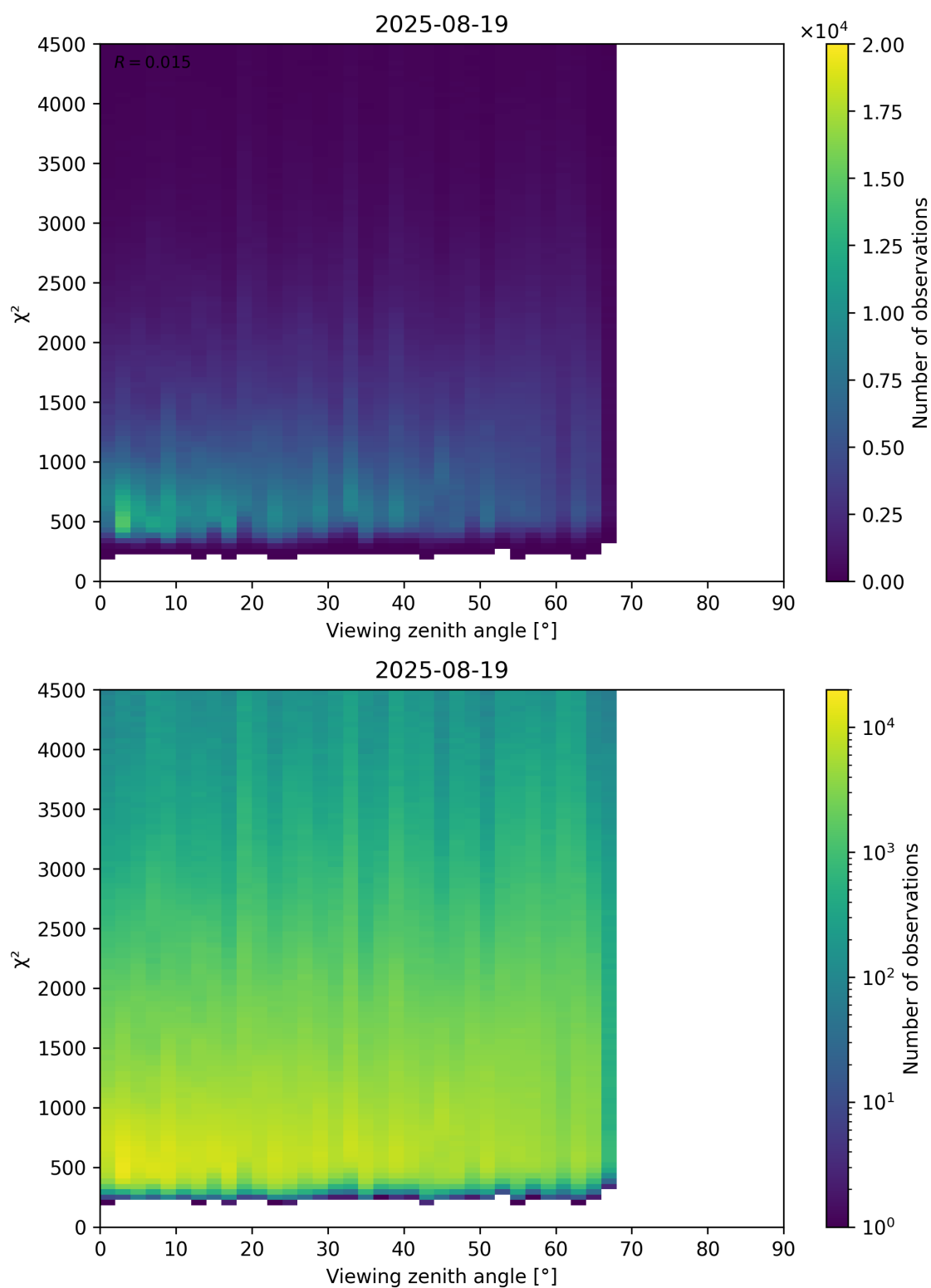
Figure 72: Scatter density plot of “Viewing zenith angle” against “ \chi^2 ” for 2025-08-19 to 2025-08-20.
