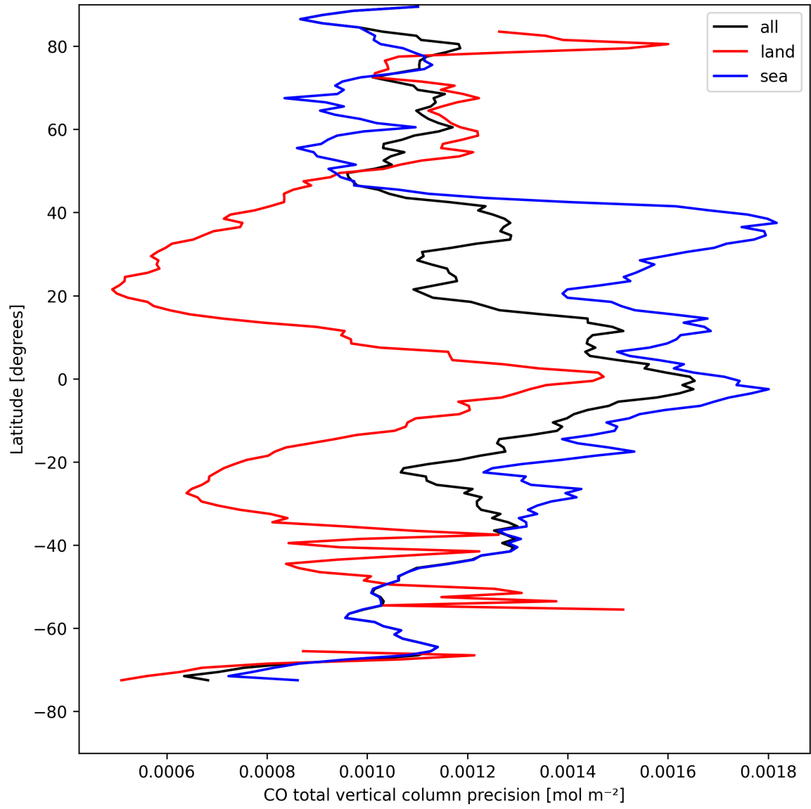
Figure 12: Zonal average of “CO total vertical column precision” for 2025-08-19 to 2025-08-20.
