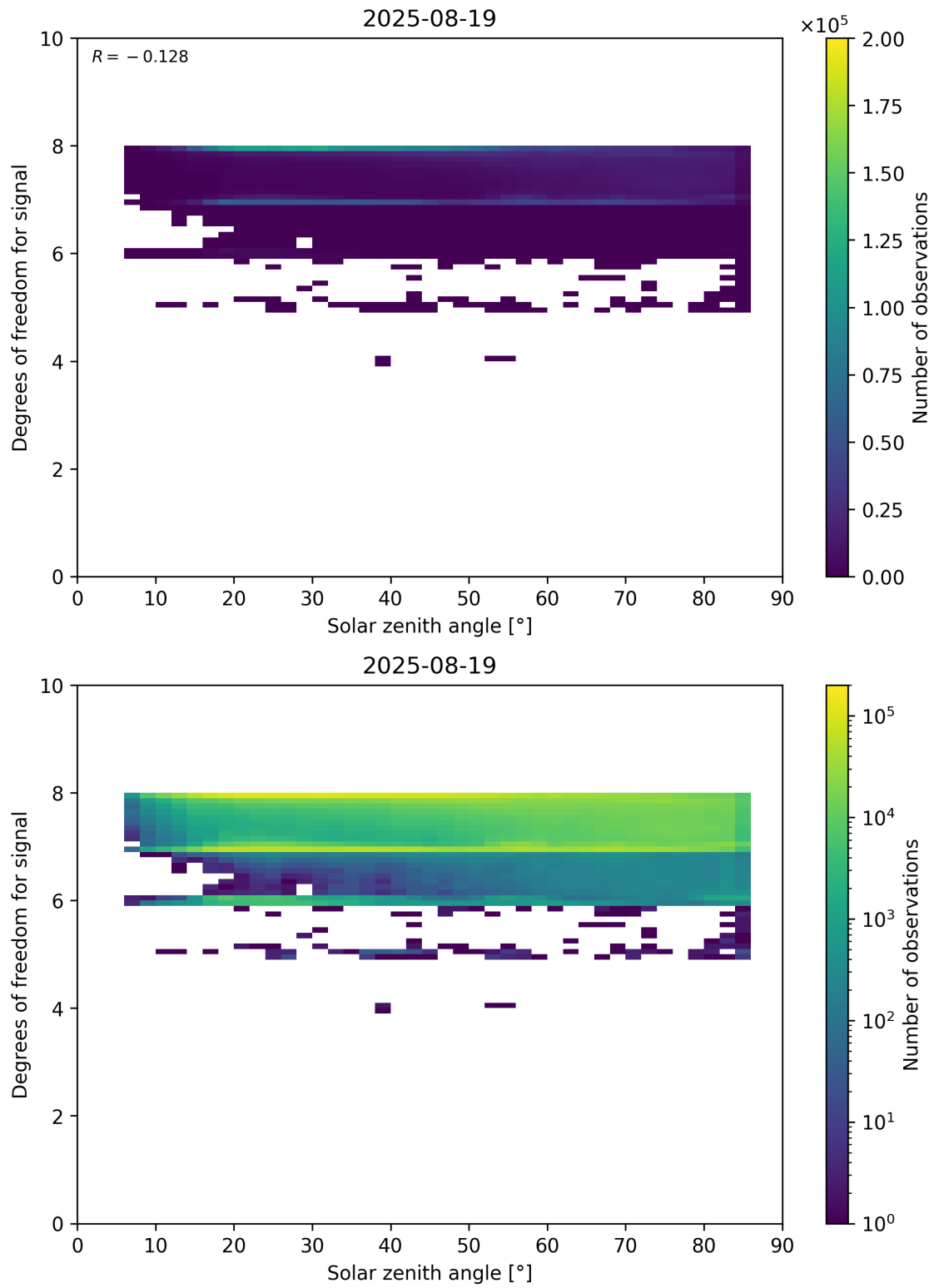
Figure 65: Scatter density plot of “Solar zenith angle” against “Degrees of freedom for signal” for 2025-08-19 to 2025-08-20.
