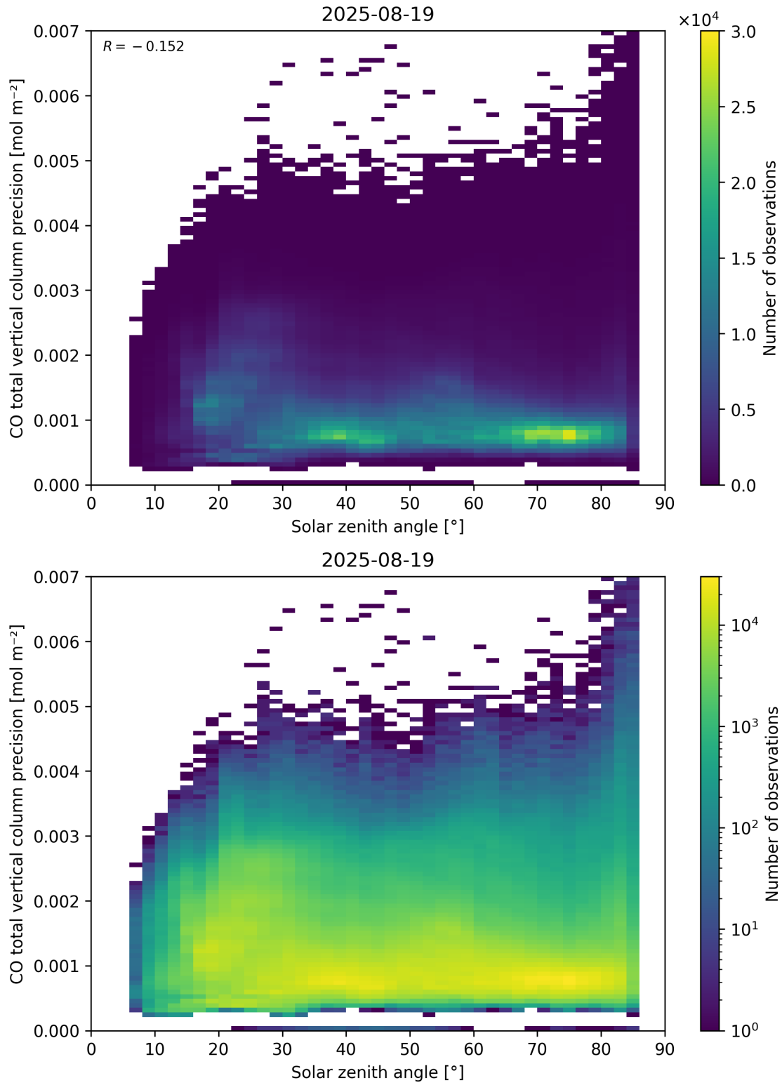
Figure 63: Scatter density plot of “Solar zenith angle” against “CO total vertical column precision” for 2025-08-19 to 2025-08-20.
