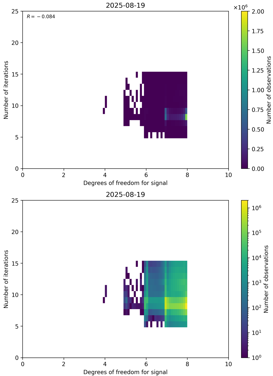
Figure 50: Scatter density plot of “Degrees of freedom for signal” against “Number of iterations” for 2025-08-19 to 2025-08-20.
