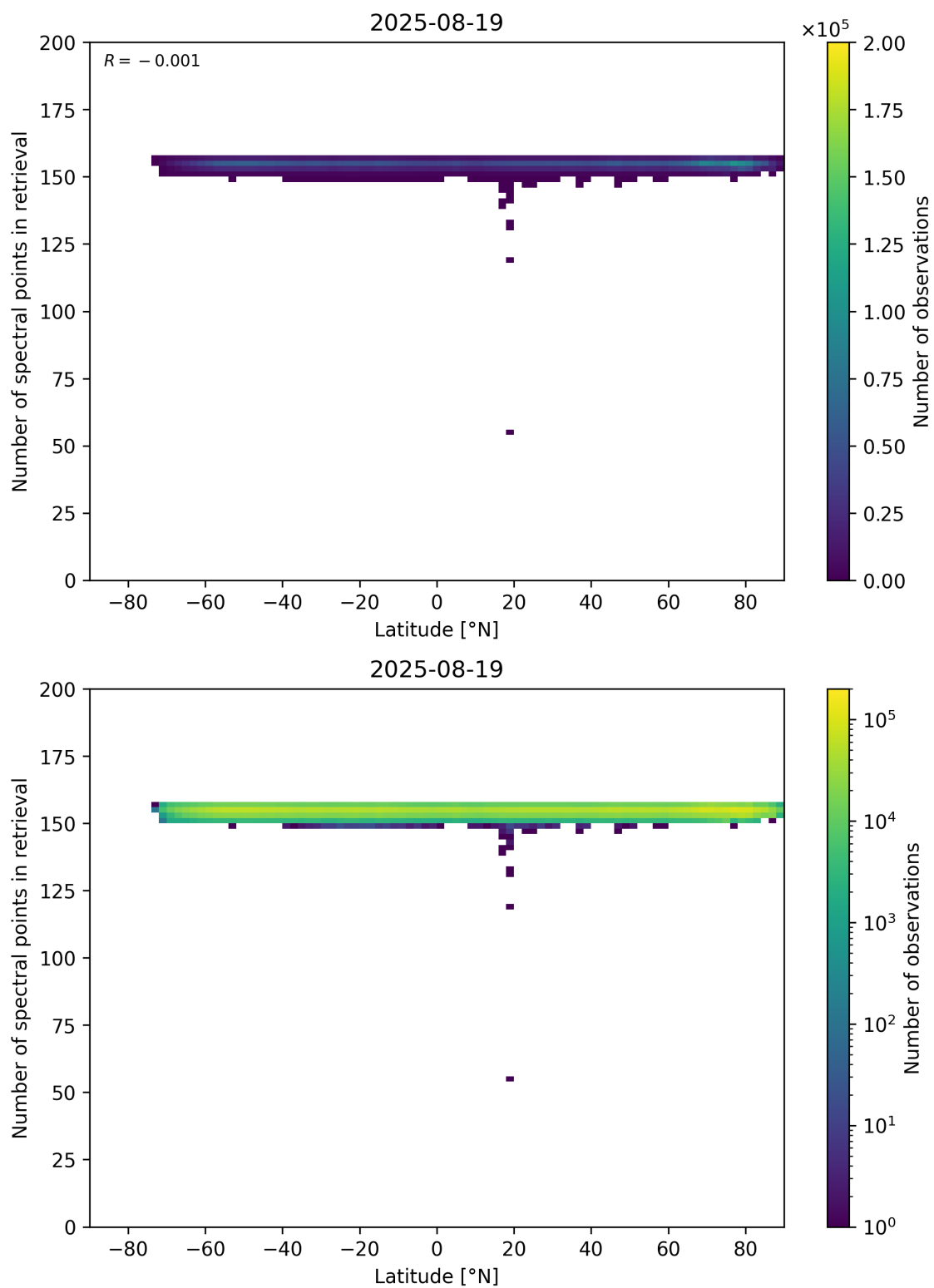
Figure 57: Scatter density plot of “Latitude” against “Number of spectral points in retrieval” for 2025-08-19 to 2025-08-20.
