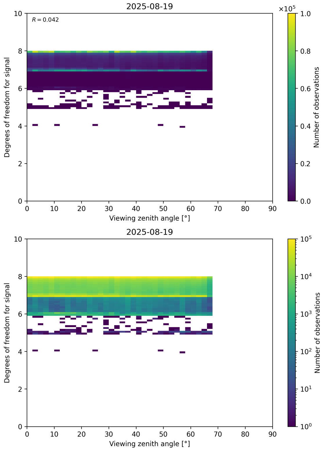
Figure 73: Scatter density plot of “Viewing zenith angle” against “Degrees of freedom for signal” for 2025-08-19 to 2025-08-20.
