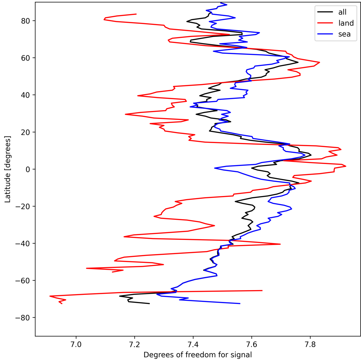
Figure 15: Zonal average of “Degrees of freedom for signal” for 2025-08-19 to 2025-08-20.
