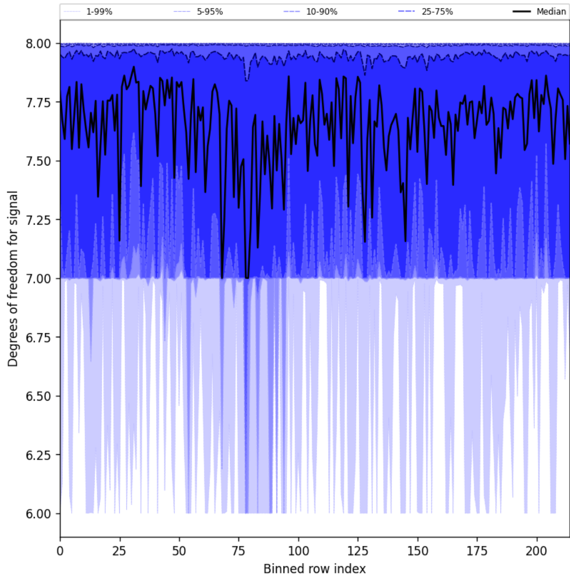
Figure 31: Along track statistics of “Degrees of freedom for signal” for 2025-08-19 to 2025-08-20
