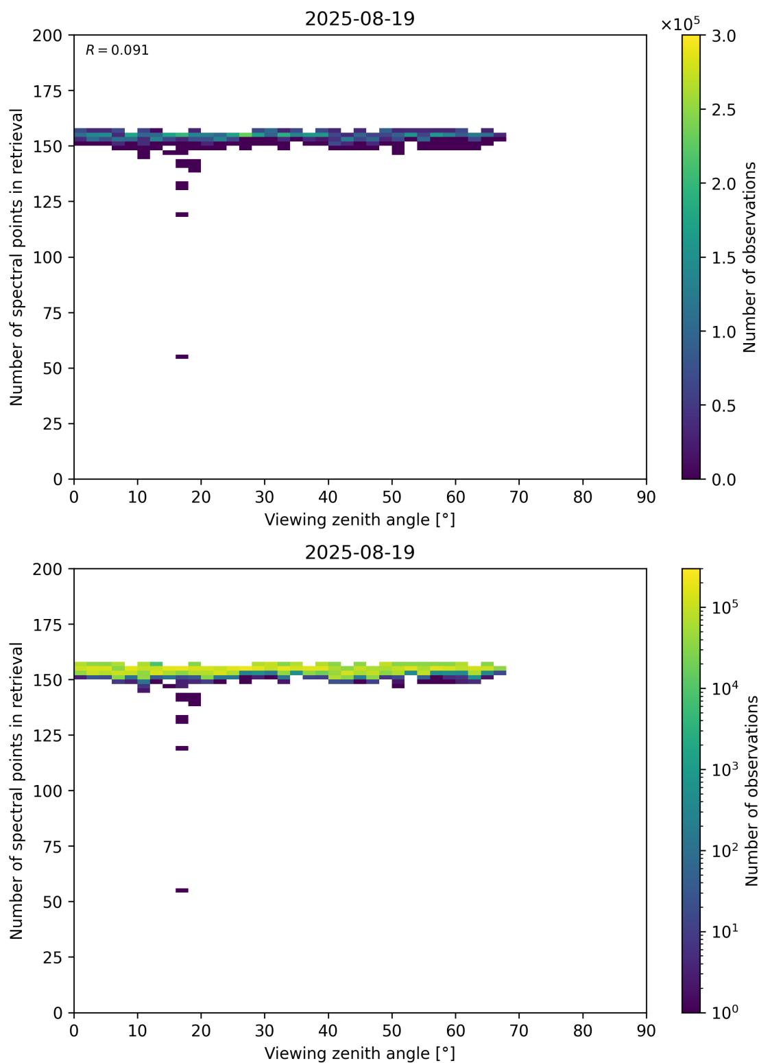
Figure 76: Scatter density plot of “Viewing zenith angle” against “Number of spectral points in retrieval” for 2025-08-19 to 2025-08-20.
