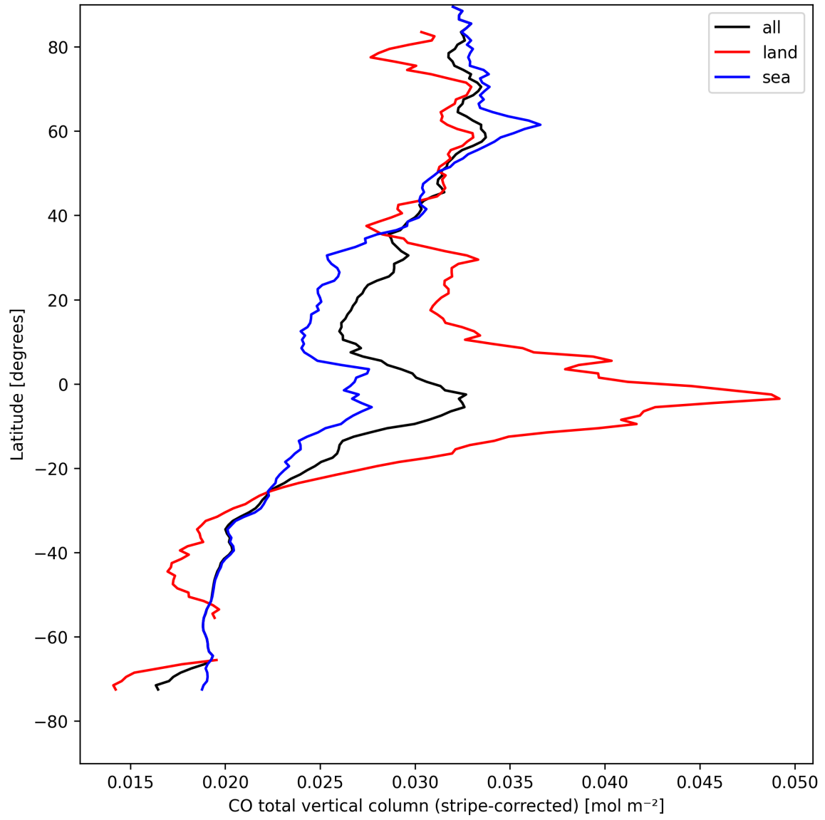
Figure 11: Zonal average of “CO total vertical column (stripe-corrected)” for 2025-08-19 to 2025-08-20.
