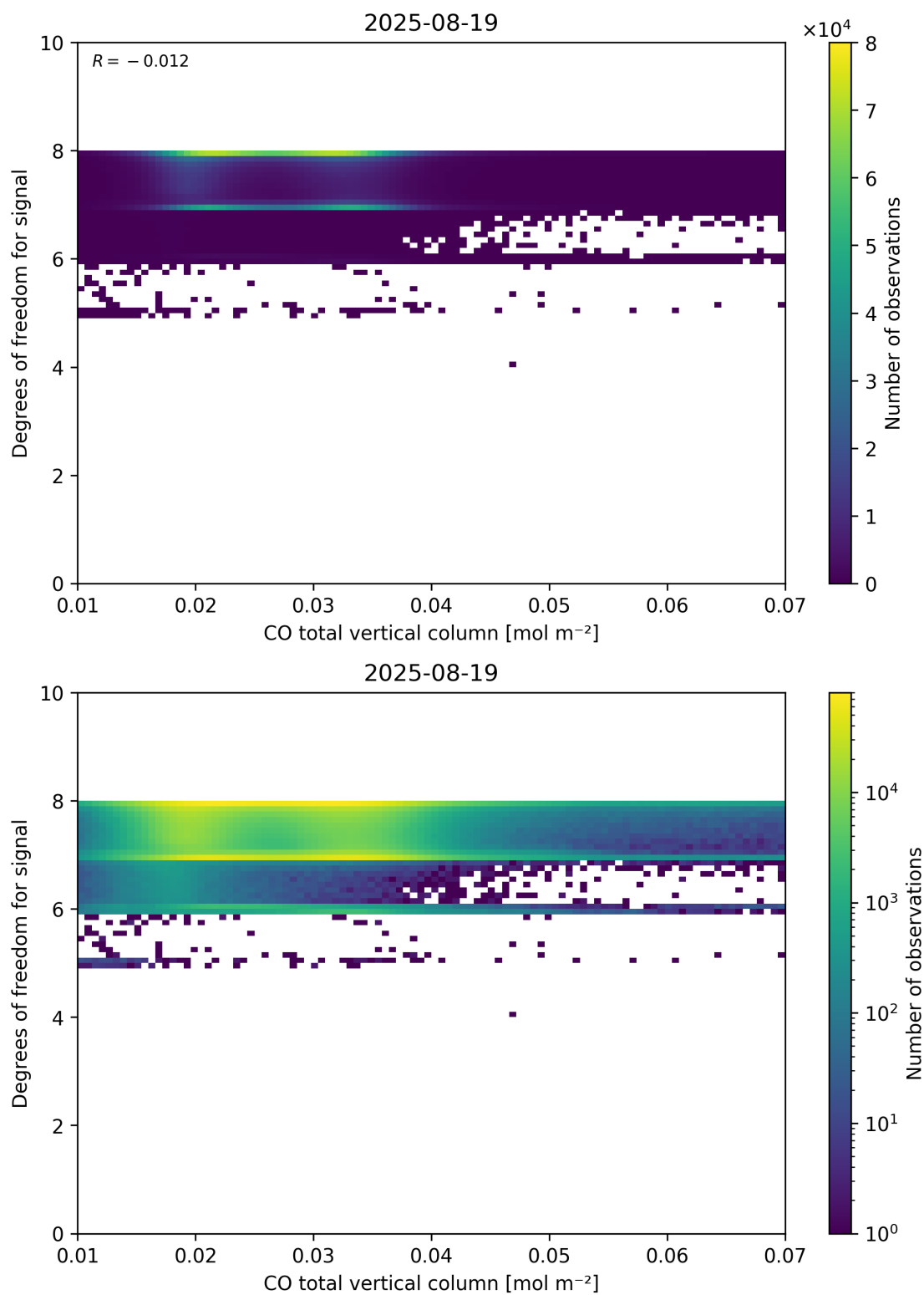
Figure 41: Scatter density plot of “CO total vertical column” against “Degrees of freedom for signal” for 2025-08-19 to 2025-08-20.
