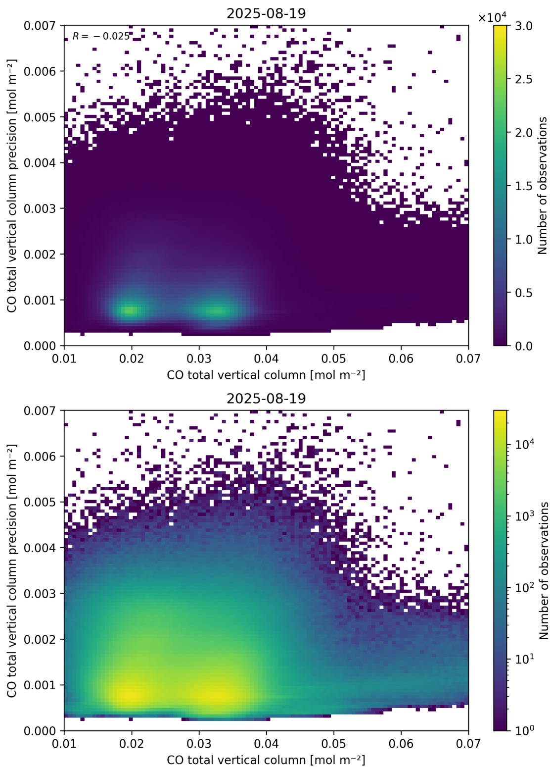
Figure 34: Scatter density plot of “CO total vertical column” against “CO total vertical column precision” for 2025-08-19 to 2025-08-20.
