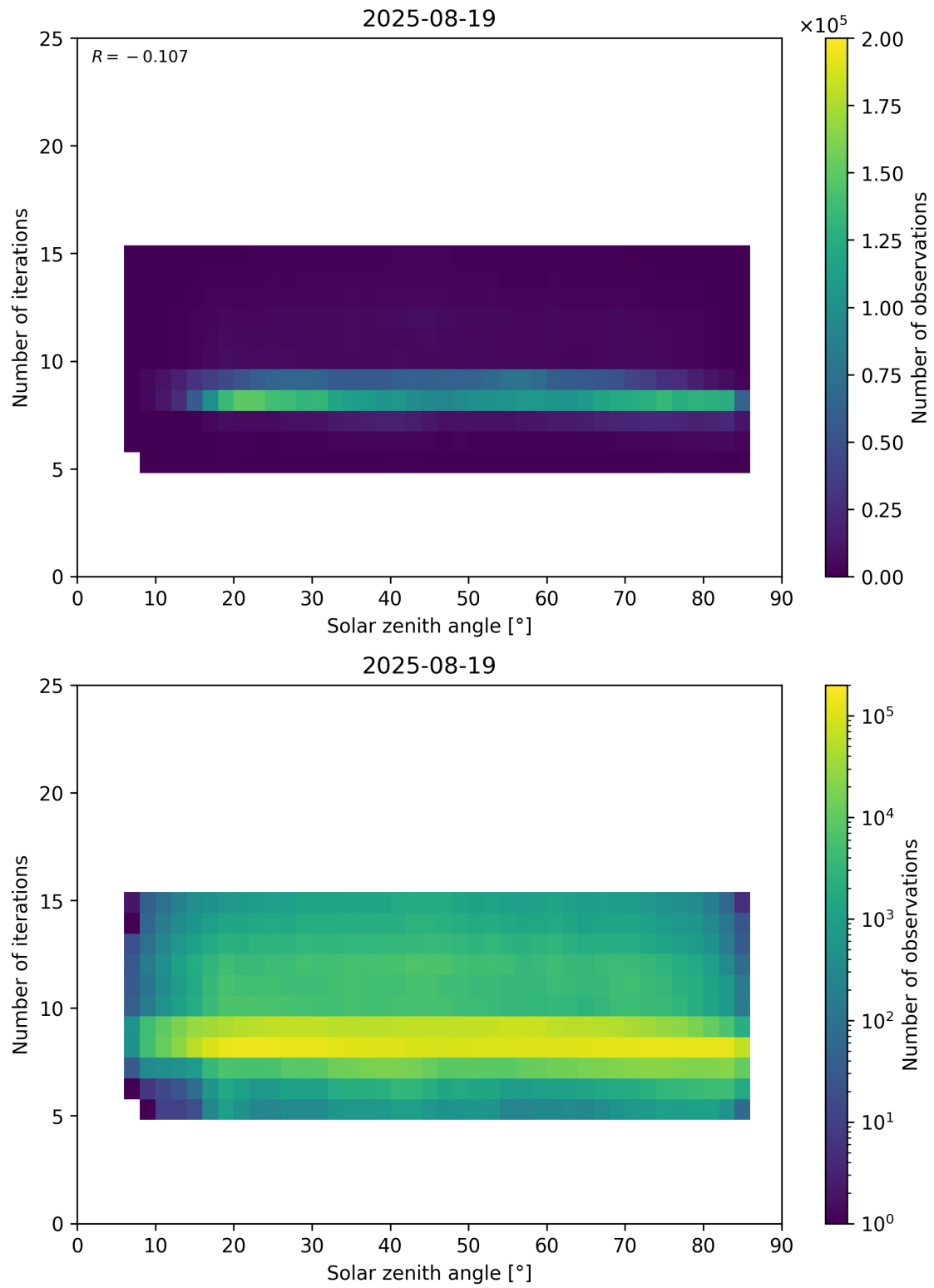
Figure 67: Scatter density plot of “Solar zenith angle” against “Number of iterations” for 2025-08-19 to 2025-08-20.
