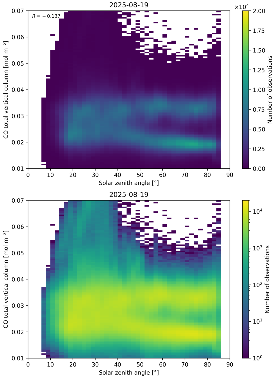
Figure 61: Scatter density plot of “Solar zenith angle” against “CO total vertical column” for 2025-08-19 to 2025-08-20.
