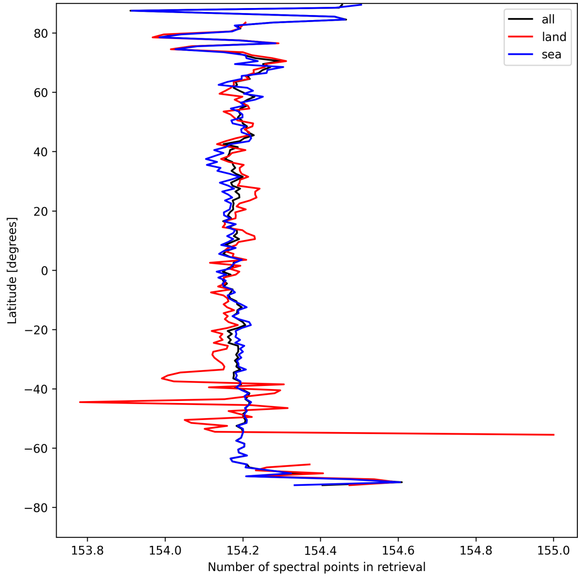
Figure 13: Zonal average of “Number of spectral points in retrieval” for 2025-08-19 to 2025-08-20.
