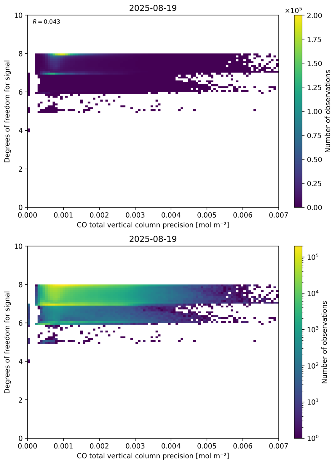
Figure 45: Scatter density plot of “CO total vertical column precision” against “Degrees of freedom for signal” for 2025-08-19 to 2025-08-20.
