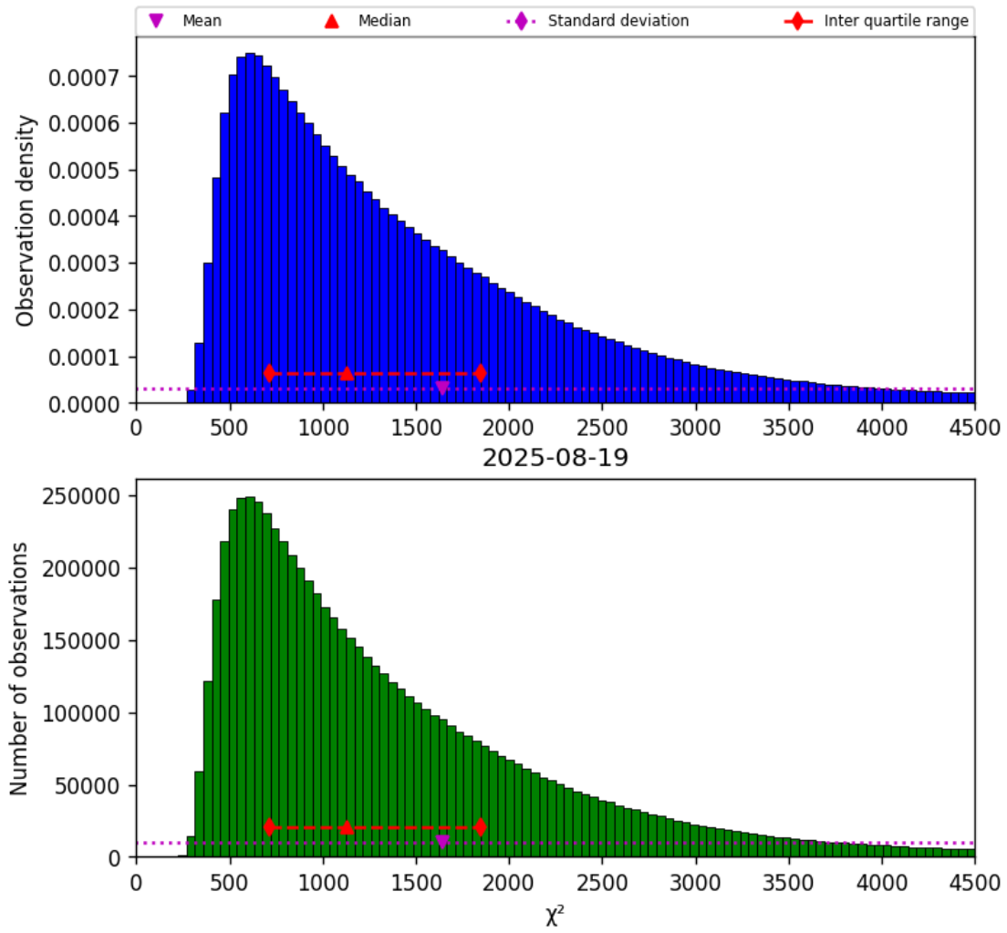
Figure 22: Histogram of “ \chi^2 ” for 2025-08-19 to 2025-08-20
