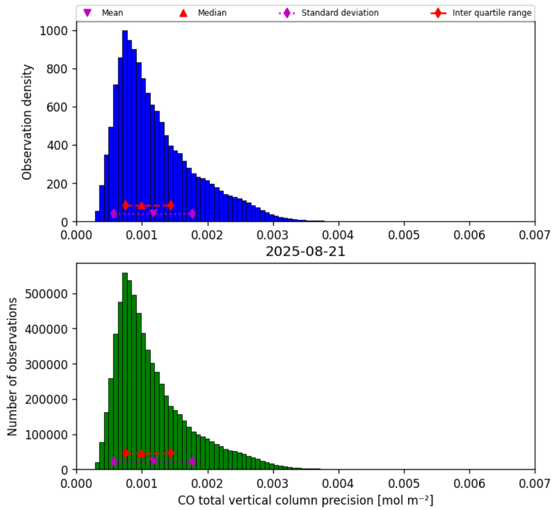
Figure 20: Histogram of “CO total vertical column precision” for 2025-08-20 to 2025-08-22
