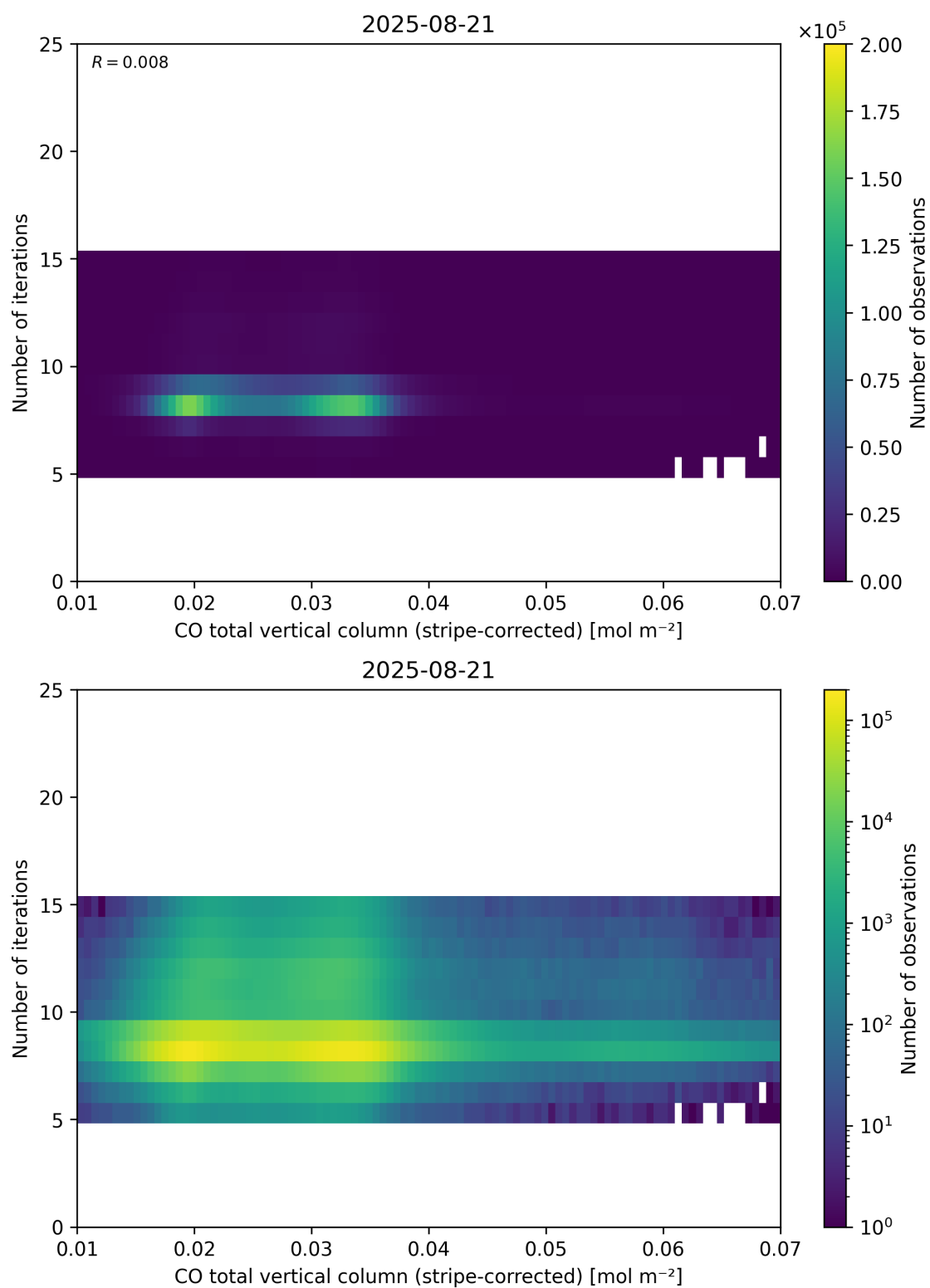
Figure 39: Scatter density plot of “CO total vertical column (stripe-corrected)” against “Number of iterations” for 2025-08-20 to 2025-08-22.
