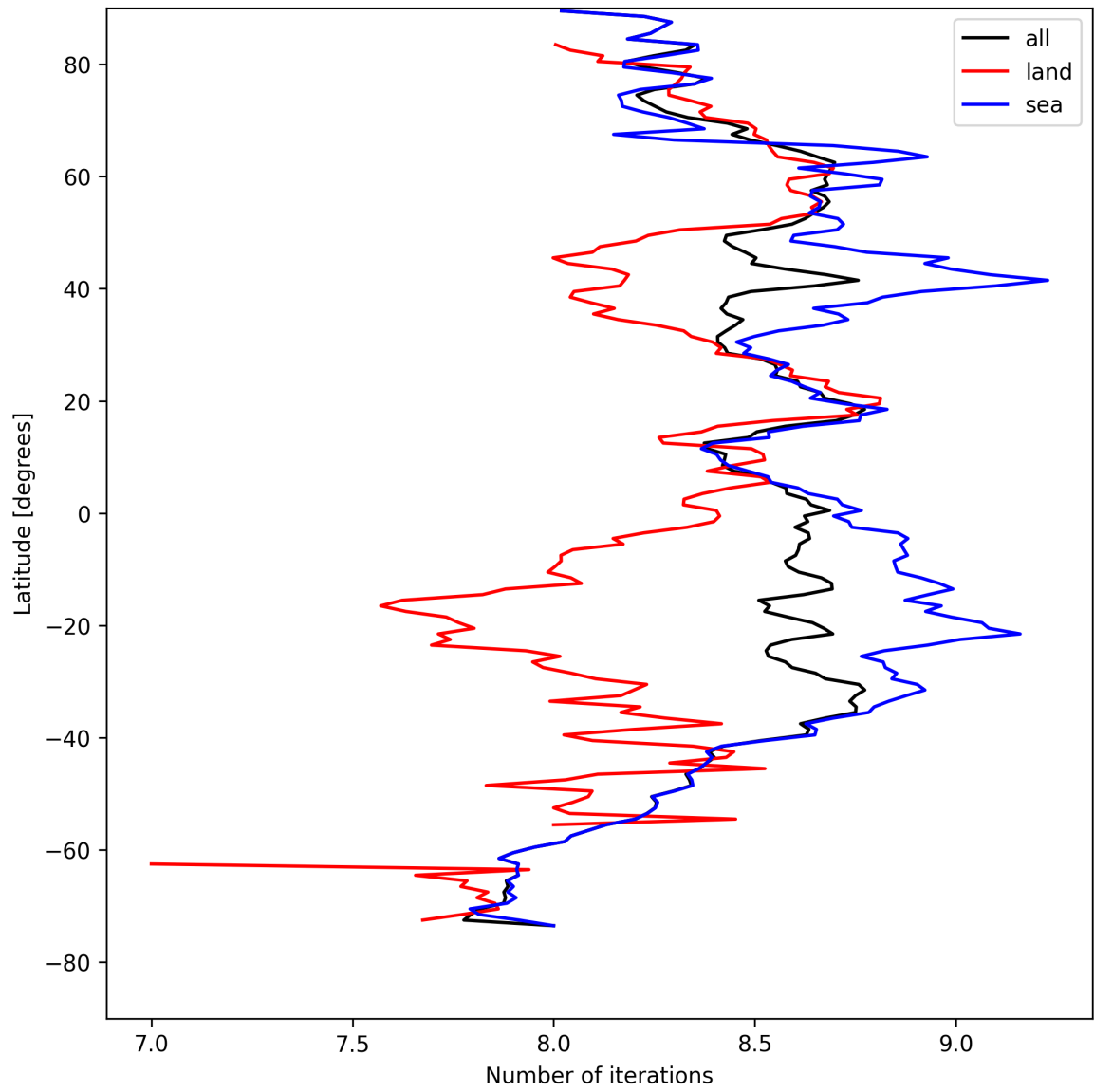
Figure 16: Zonal average of “Number of iterations” for 2025-08-20 to 2025-08-22.
