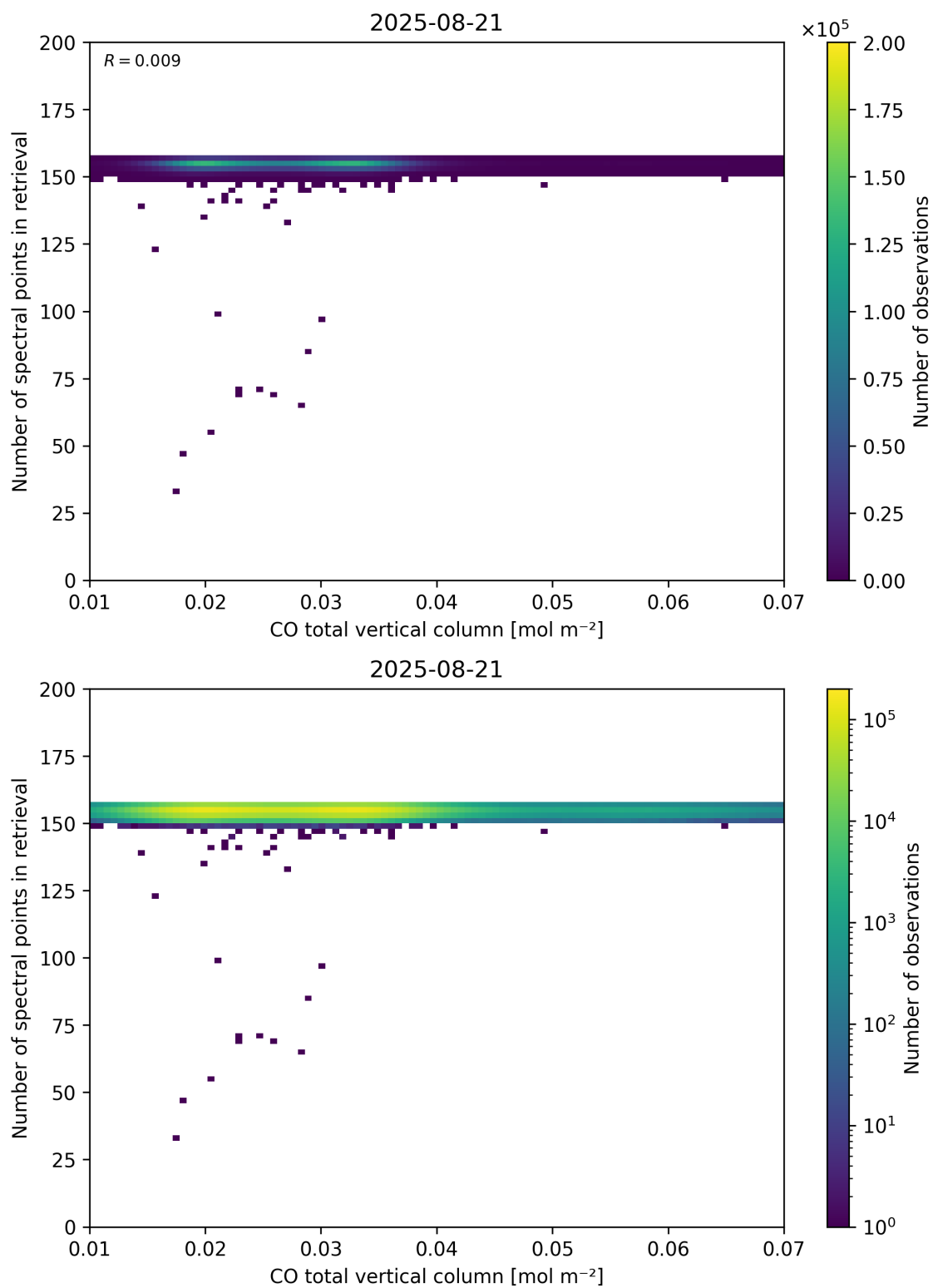
Figure 43: Scatter density plot of “CO total vertical column” against “Number of spectral points in retrieval” for 2025-08-20 to 2025-08-22.
