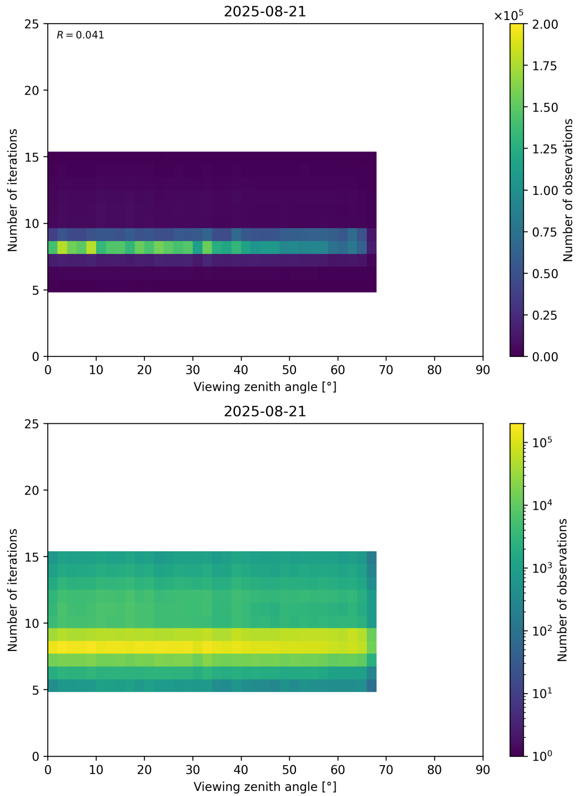
Figure 75: Scatter density plot of “Viewing zenith angle” against “Number of iterations” for 2025-08-20 to 2025-08-22.
