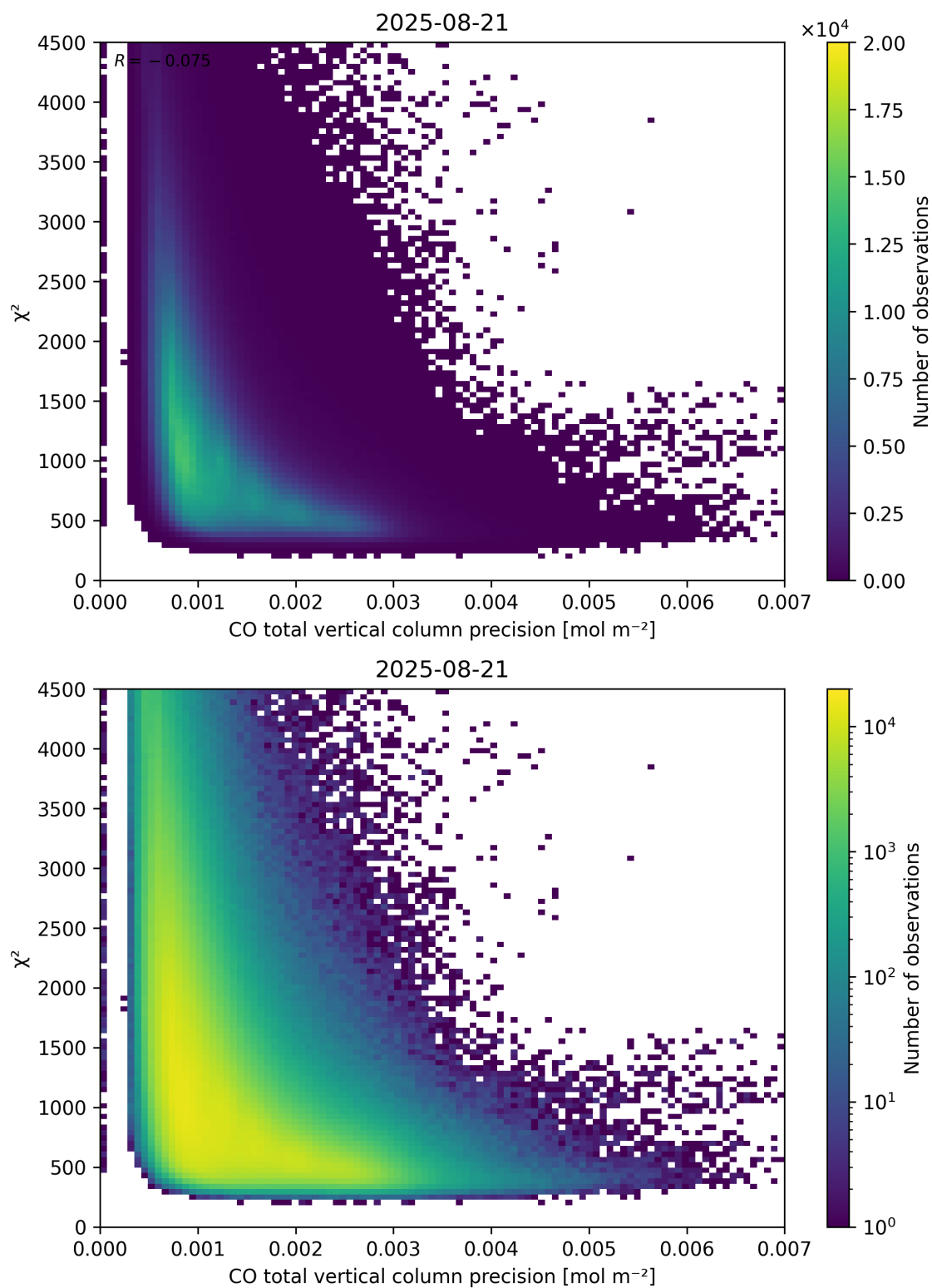
Figure 44: Scatter density plot of “CO total vertical column precision” against “ \chi^2 ” for 2025-08-20 to 2025-08-22.
