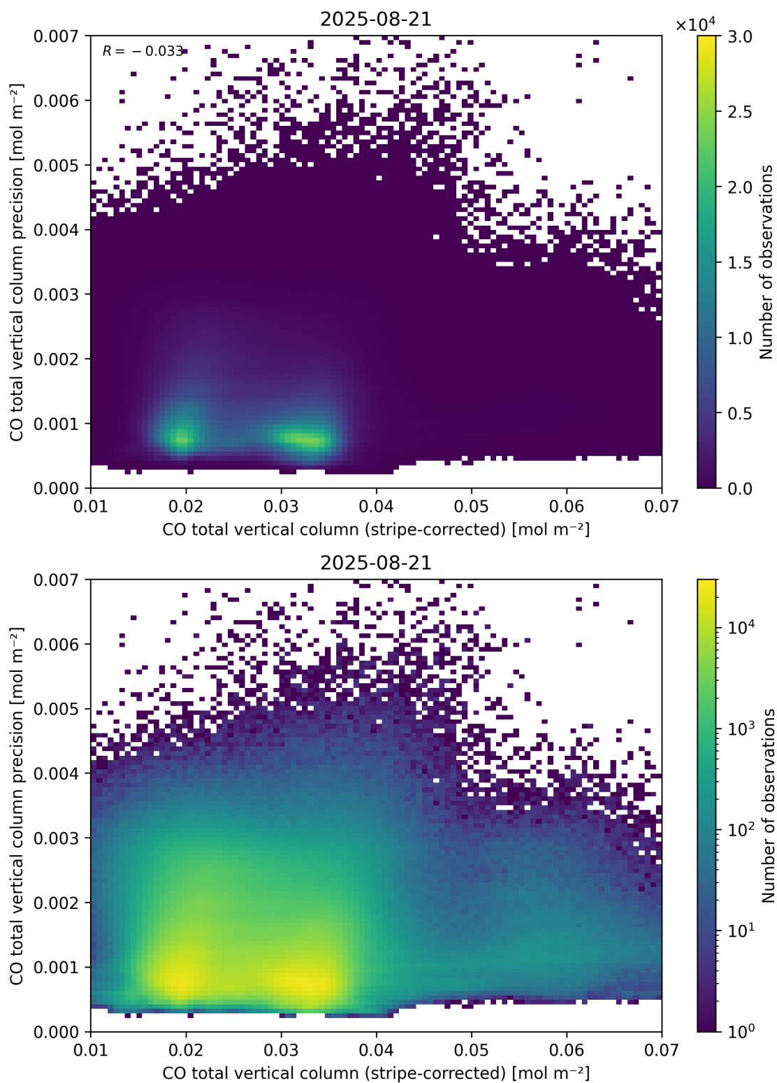
Figure 36: Scatter density plot of “CO total vertical column (stripe-corrected)” against “CO total vertical column precision” for 2025-08-20 to 2025-08-22.
