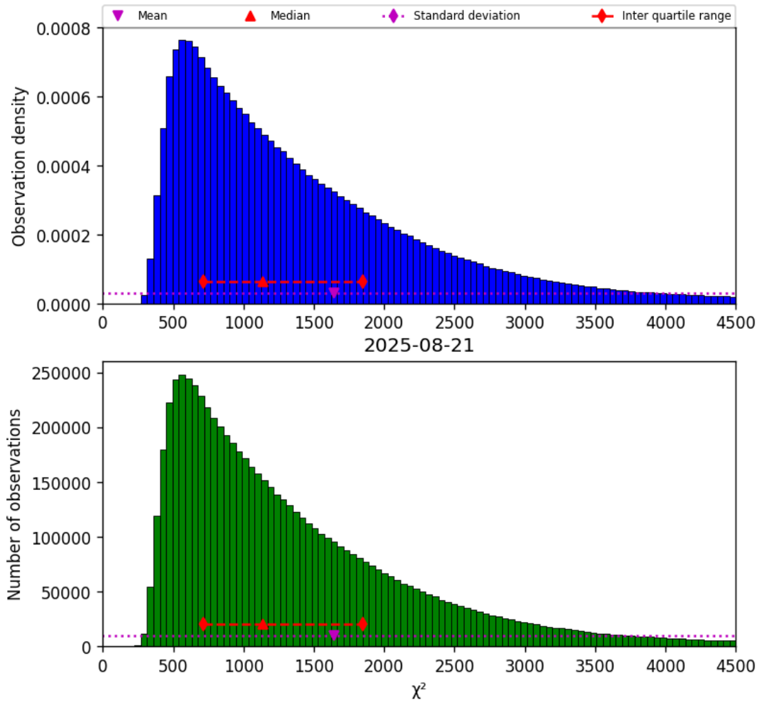
Figure 22: Histogram of “ \chi^2 ” for 2025-08-20 to 2025-08-22
