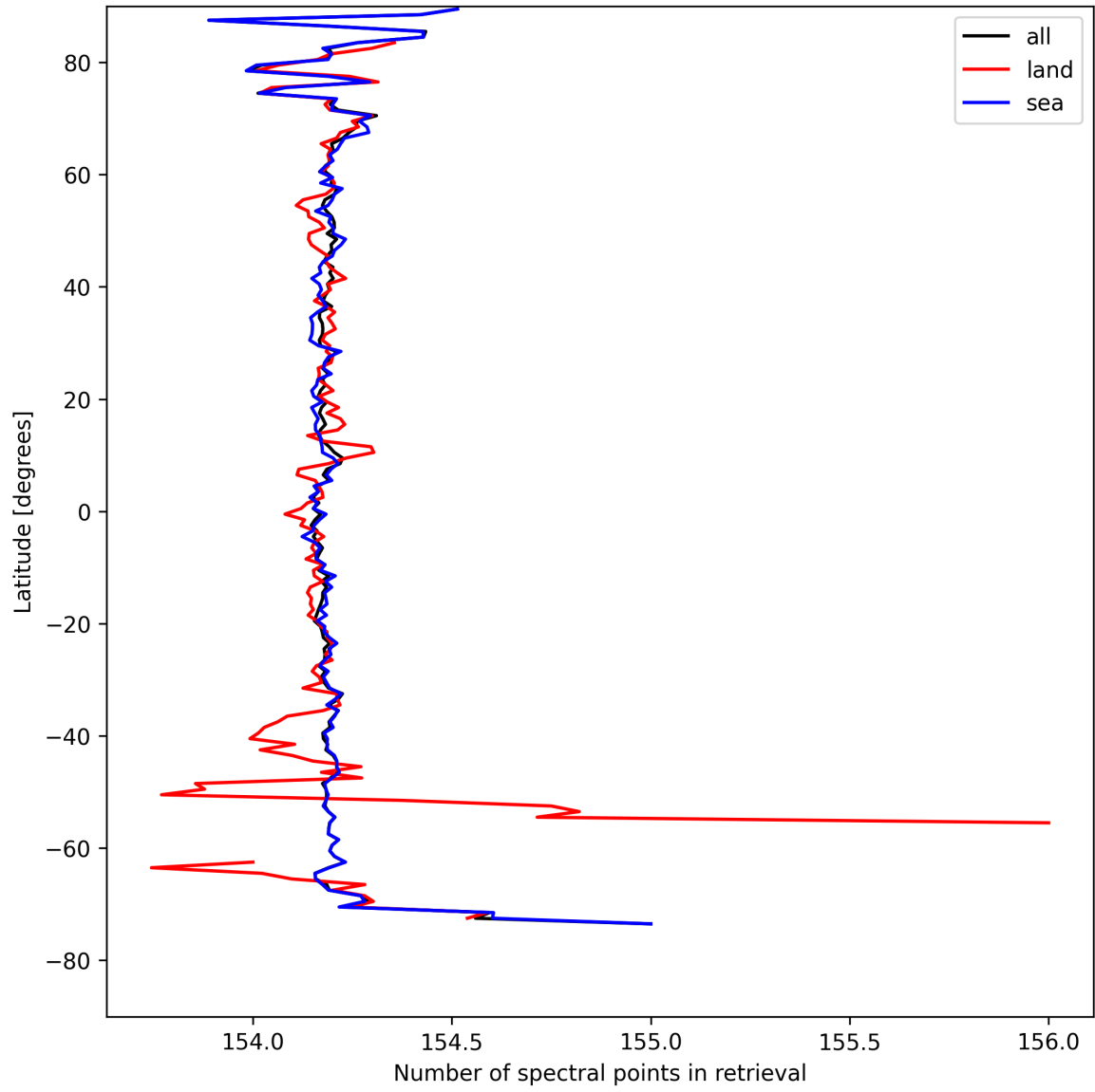
Figure 13: Zonal average of “Number of spectral points in retrieval” for 2025-08-20 to 2025-08-22.
