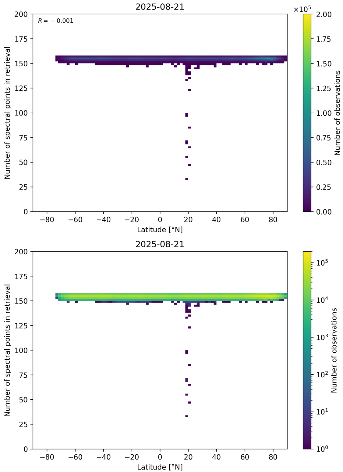
Figure 57: Scatter density plot of “Latitude” against “Number of spectral points in retrieval” for 2025-08-20 to 2025-08-22.
