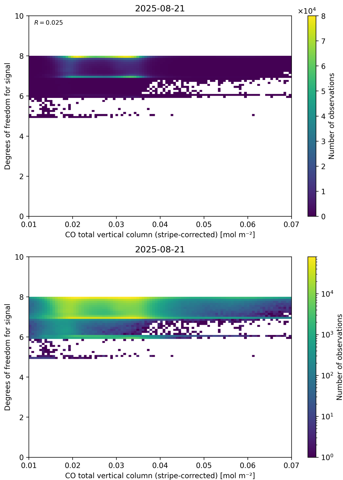
Figure 38: Scatter density plot of “CO total vertical column (stripe-corrected)” against “Degrees of freedom for signal” for 2025-08-20 to 2025-08-22.
