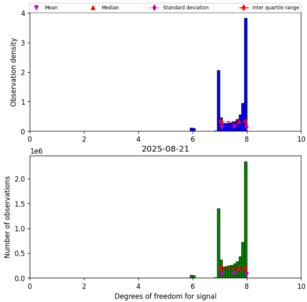
Figure 23: Histogram of “Degrees of freedom for signal” for 2025-08-20 to 2025-08-22
