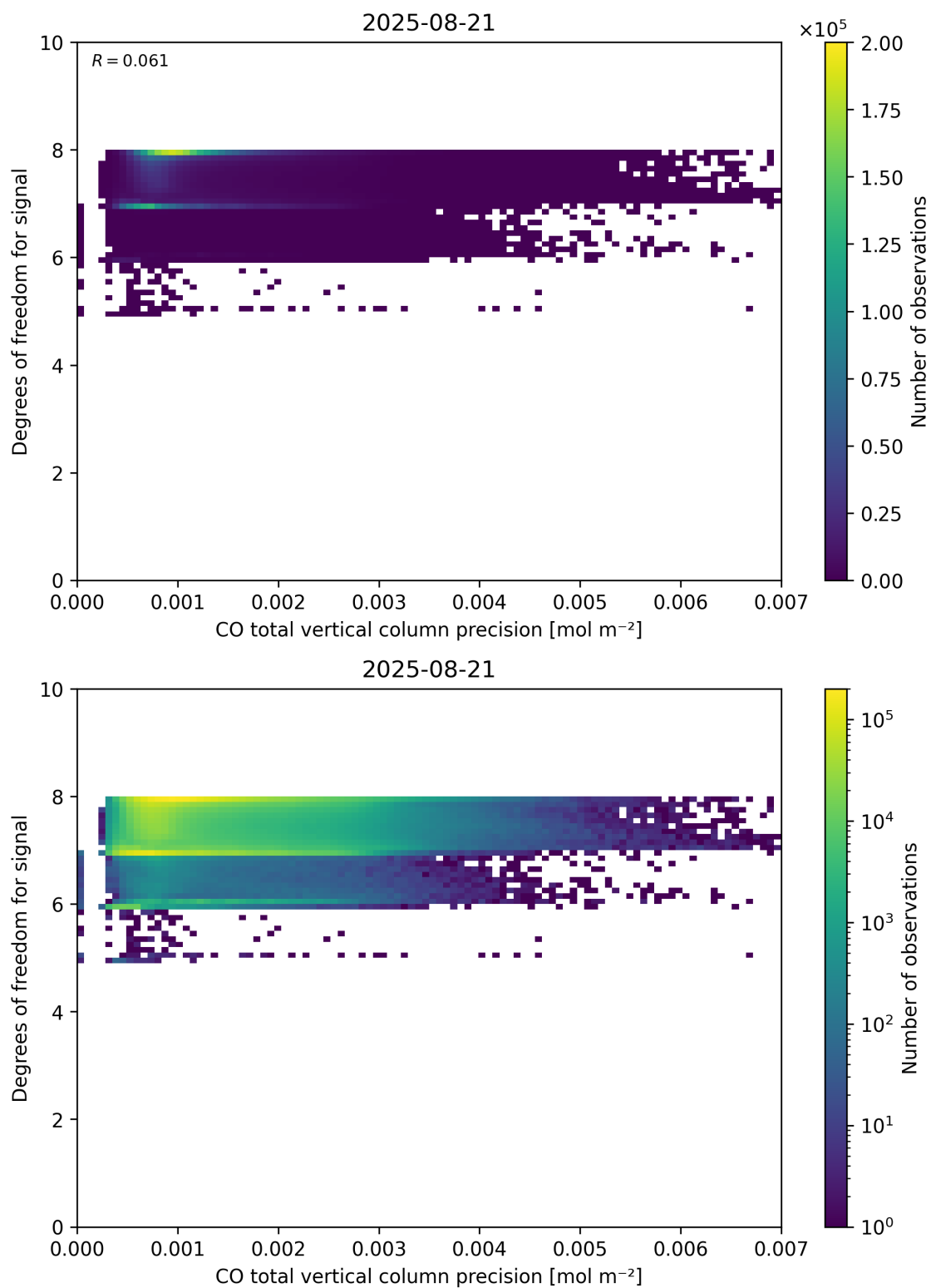
Figure 45: Scatter density plot of “CO total vertical column precision” against “Degrees of freedom for signal” for 2025-08-20 to 2025-08-22.
