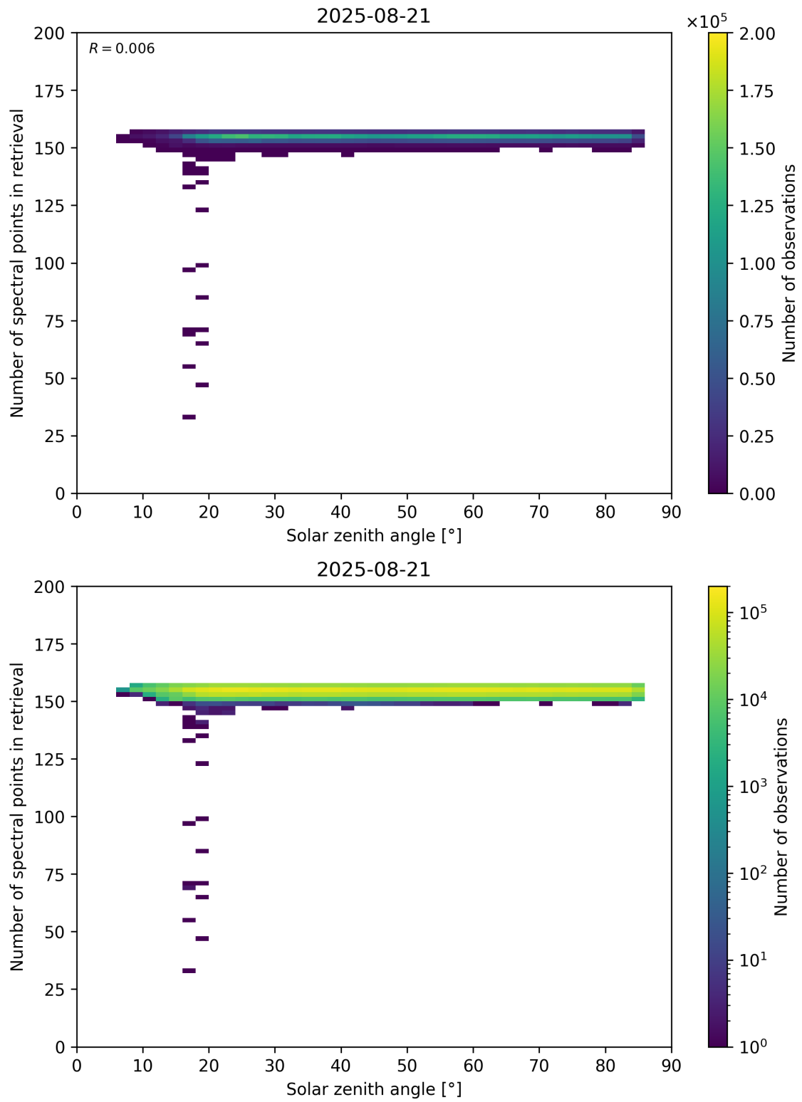
Figure 68: Scatter density plot of “Solar zenith angle” against “Number of spectral points in retrieval” for 2025-08-20 to 2025-08-22.
