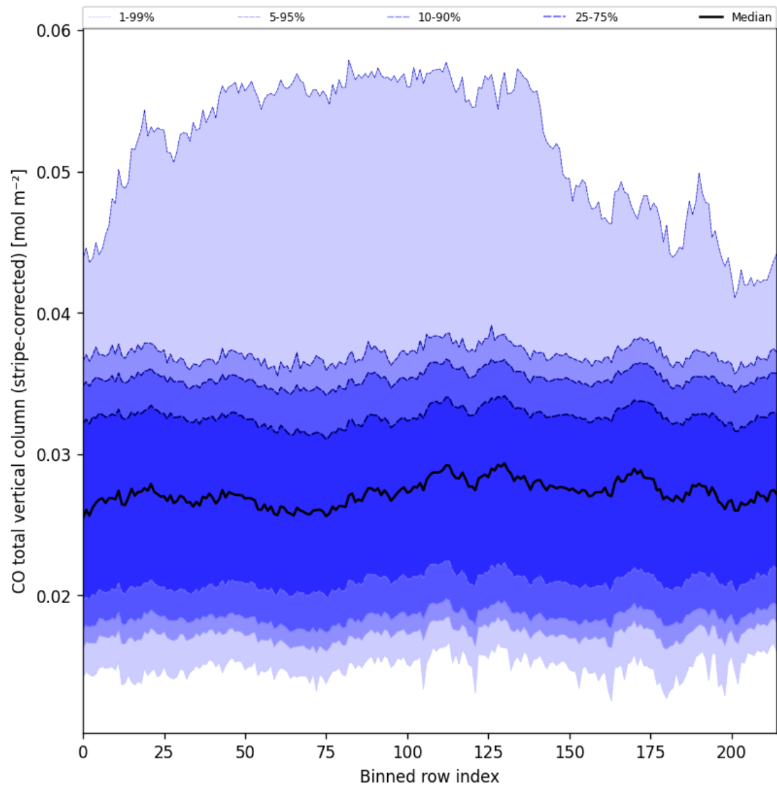
Figure 27: Along track statistics of “CO total vertical column (stripe-corrected)” for 2025-08-20 to 2025-08-22
