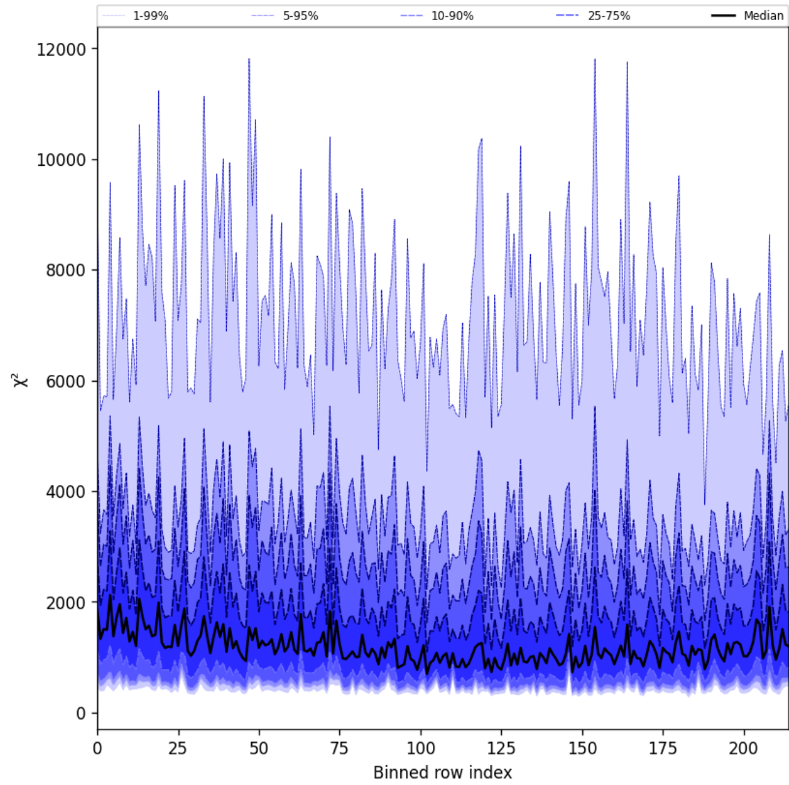
Figure 30: Along track statistics of “ \chi^2 ” for 2025-08-20 to 2025-08-22
