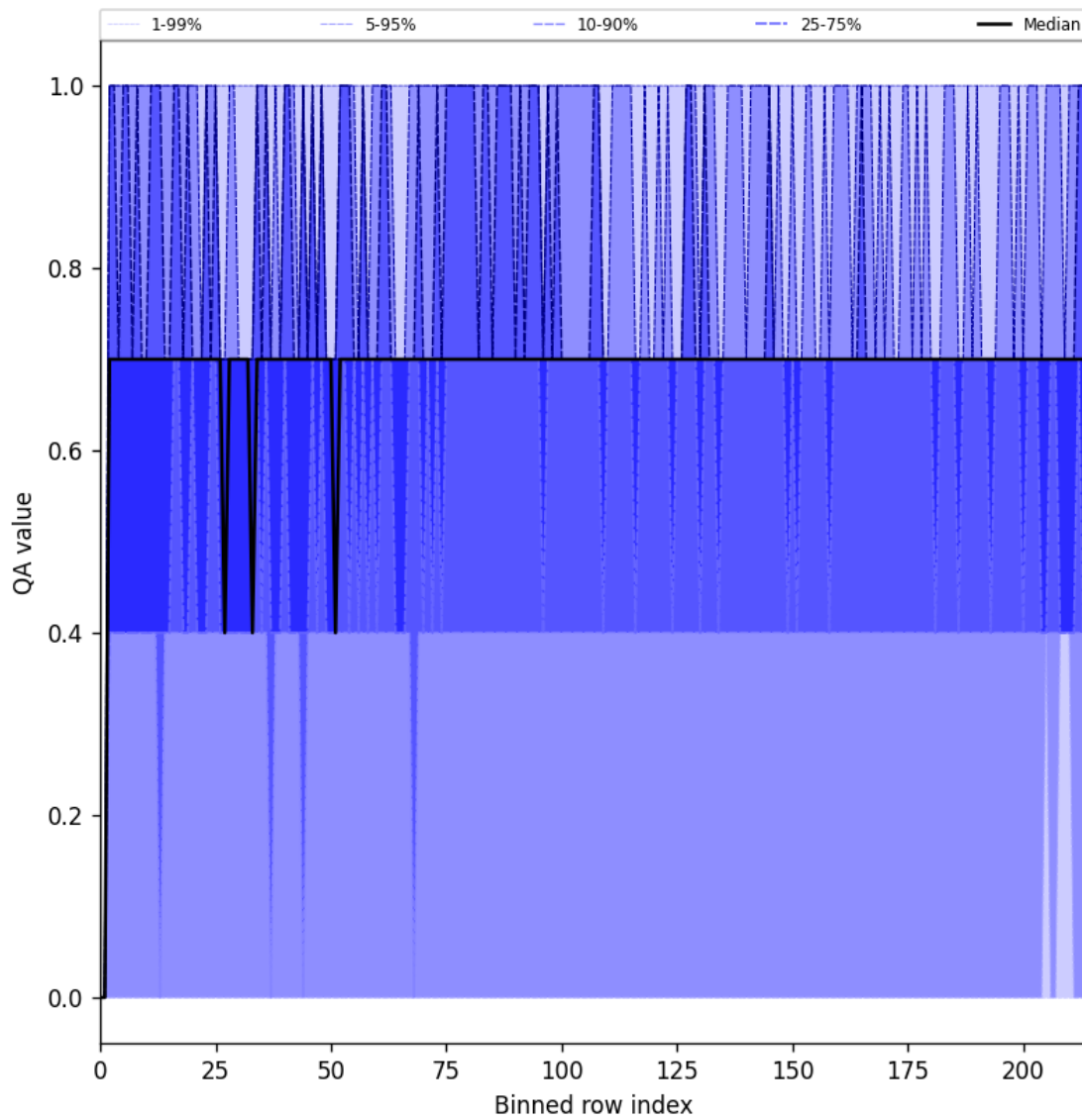
Figure 25: Along track statistics of “QA value” for 2025-08-20 to 2025-08-22
