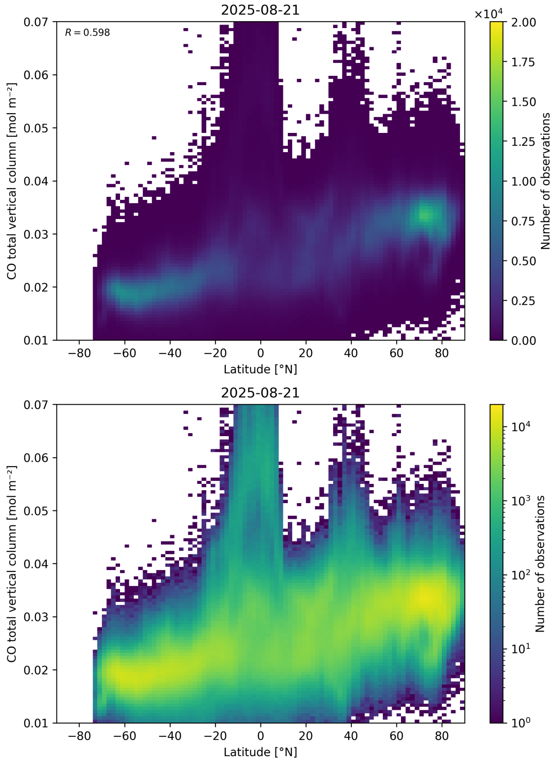
Figure 51: Scatter density plot of “Latitude” against “CO total vertical column” for 2025-08-20 to 2025-08-22.
