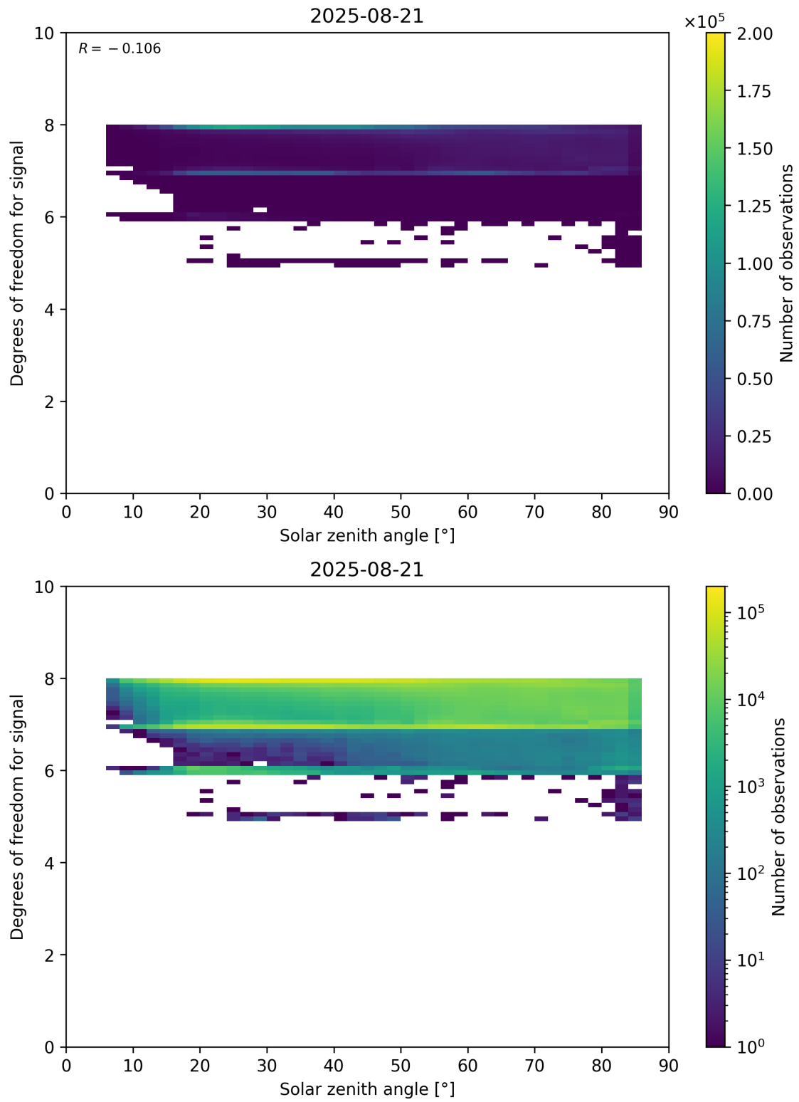
Figure 65: Scatter density plot of “Solar zenith angle” against “Degrees of freedom for signal” for 2025-08-20 to 2025-08-22.
