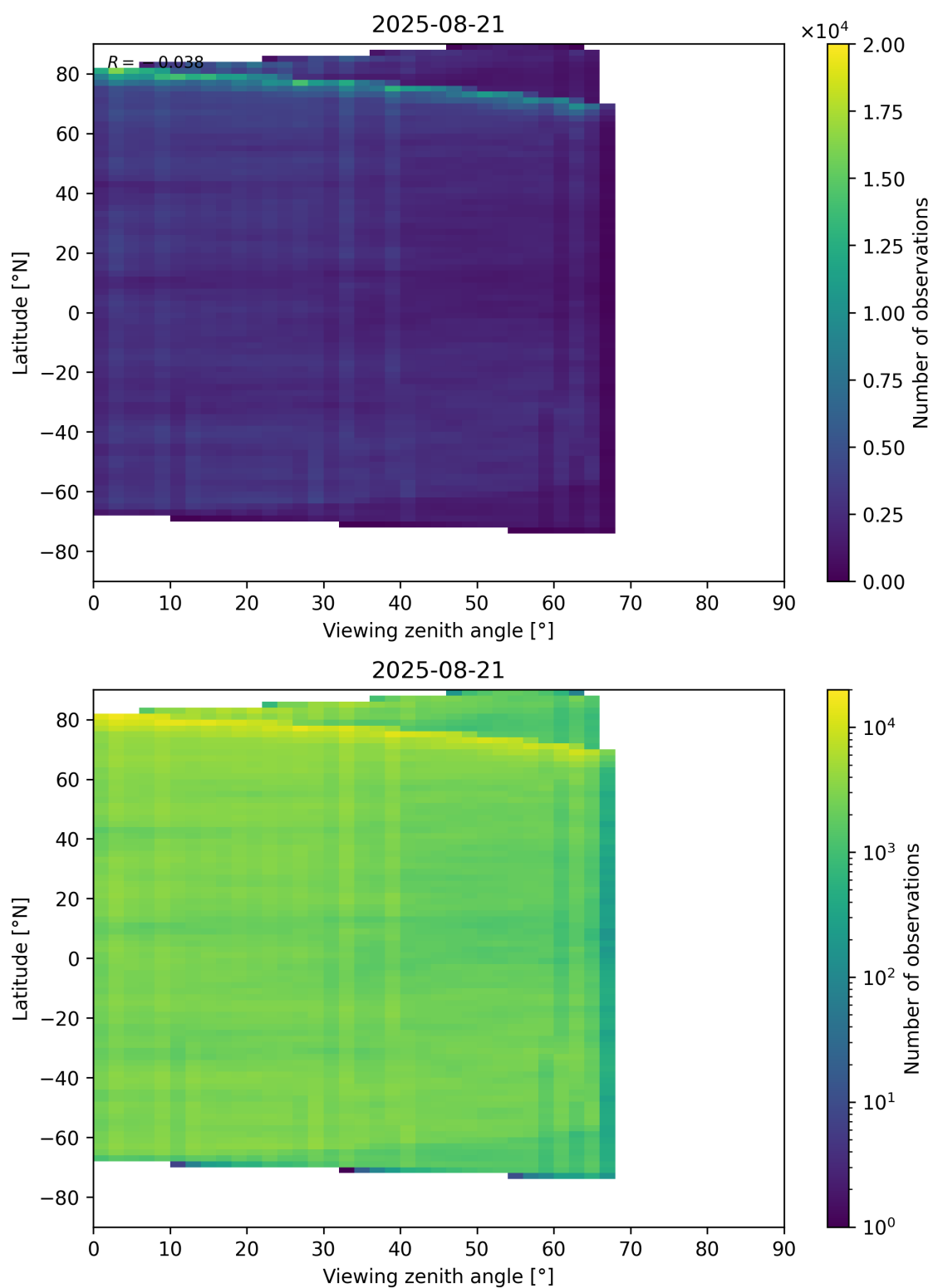
Figure 74: Scatter density plot of “Viewing zenith angle” against “Latitude” for 2025-08-20 to 2025-08-22.
