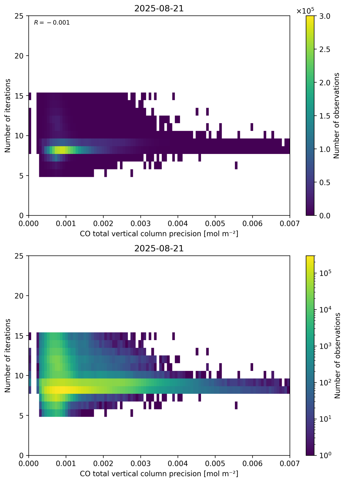
Figure 46: Scatter density plot of “CO total vertical column precision” against “Number of iterations” for 2025-08-20 to 2025-08-22.
