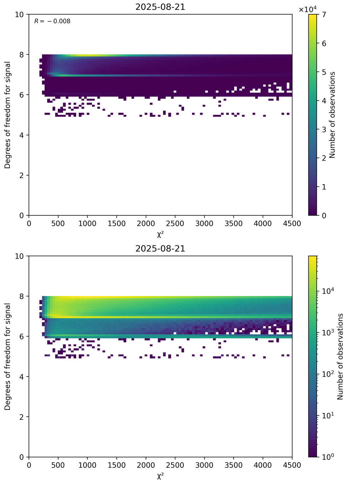
Figure 48: Scatter density plot of “ \chi^2 ” against “Degrees of freedom for signal” for 2025-08-20 to 2025-08-22.
