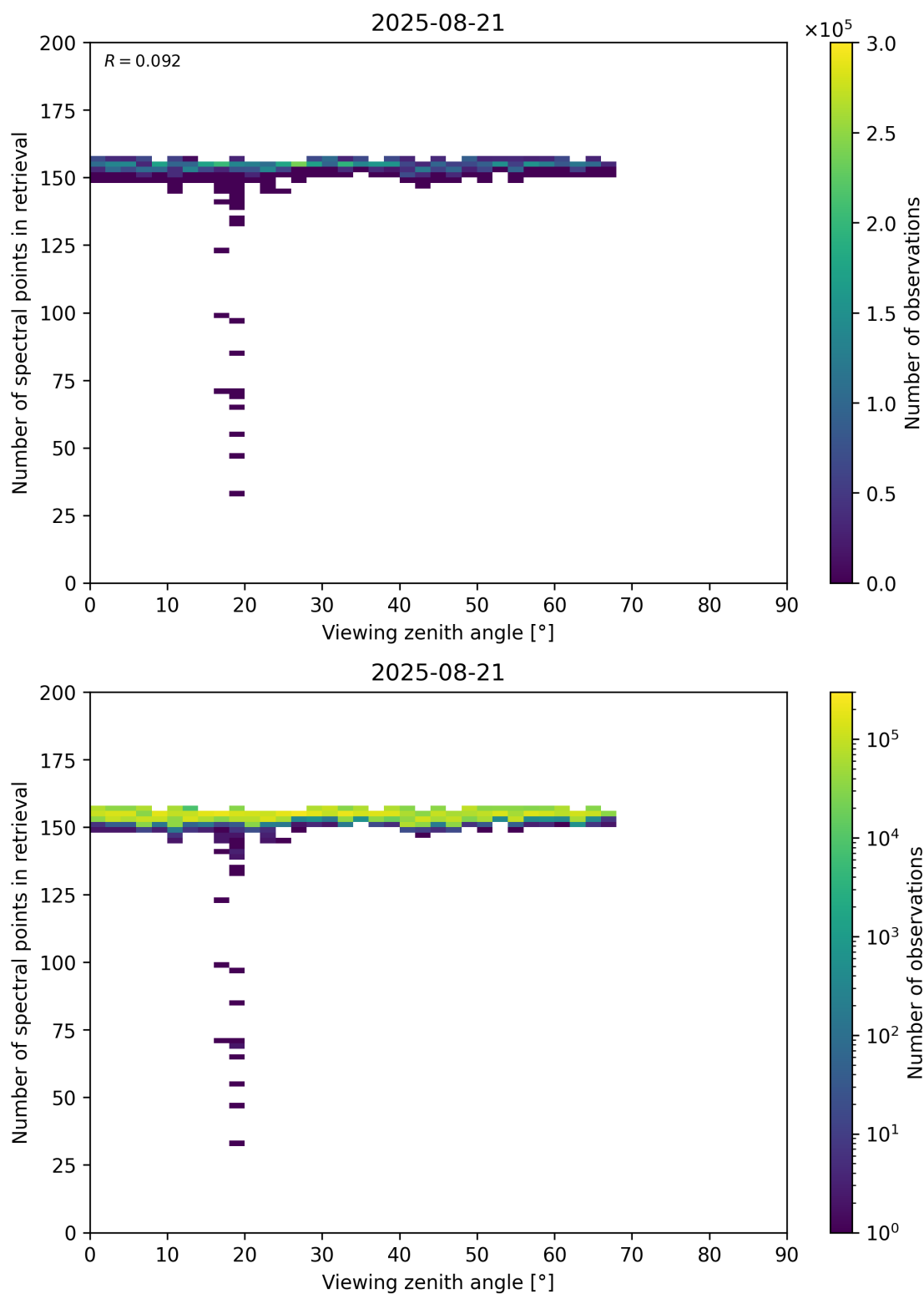
Figure 76: Scatter density plot of “Viewing zenith angle” against “Number of spectral points in retrieval” for 2025-08-20 to 2025-08-22.
