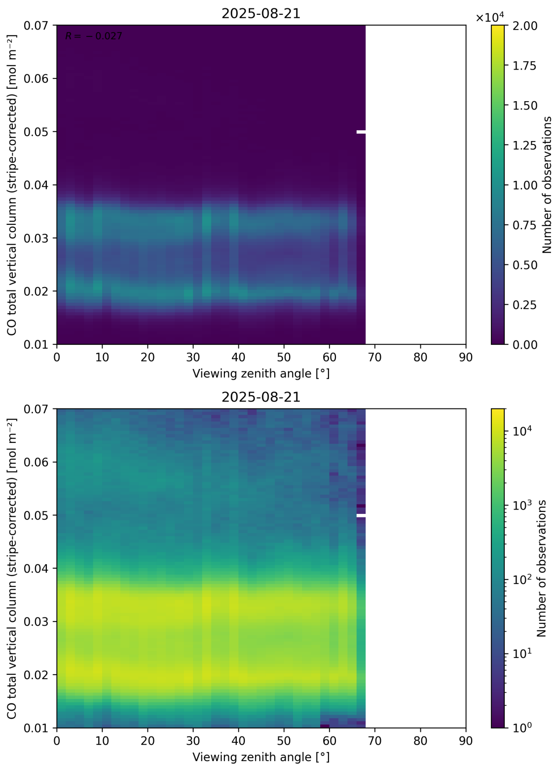
Figure 70: Scatter density plot of “Viewing zenith angle” against “CO total vertical column (stripe-corrected)” for 2025-08-20 to 2025-08-22.
