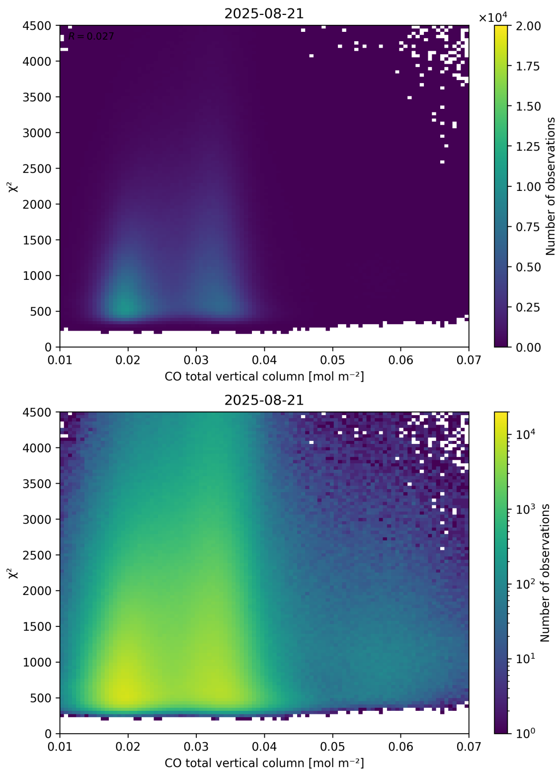
Figure 35: Scatter density plot of “CO total vertical column” against “ \chi^2 ” for 2025-08-20 to 2025-08-22.
