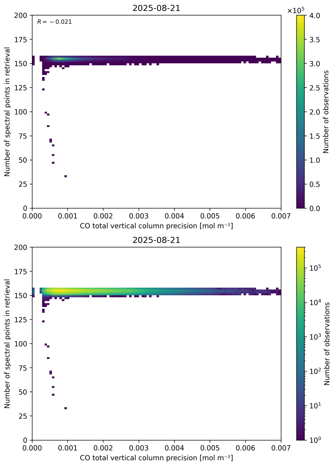
Figure 47: Scatter density plot of “CO total vertical column precision” against “Number of spectral points in retrieval” for 2025-08-20 to 2025-08-22.
