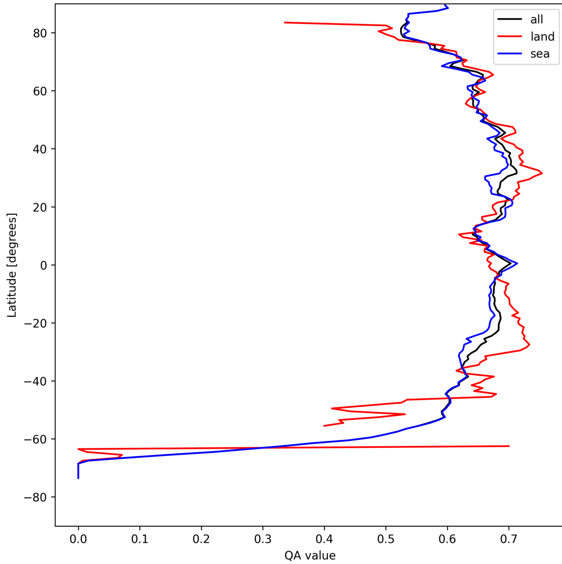
Figure 9: Zonal average of “QA value” for 2025-08-20 to 2025-08-22.
