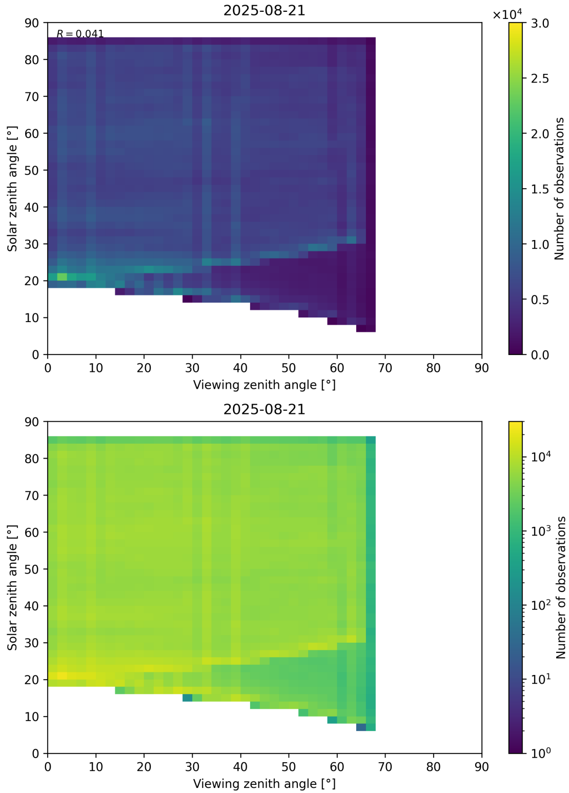
Figure 77: Scatter density plot of “Viewing zenith angle” against “Solar zenith angle” for 2025-08-20 to 2025-08-22.
