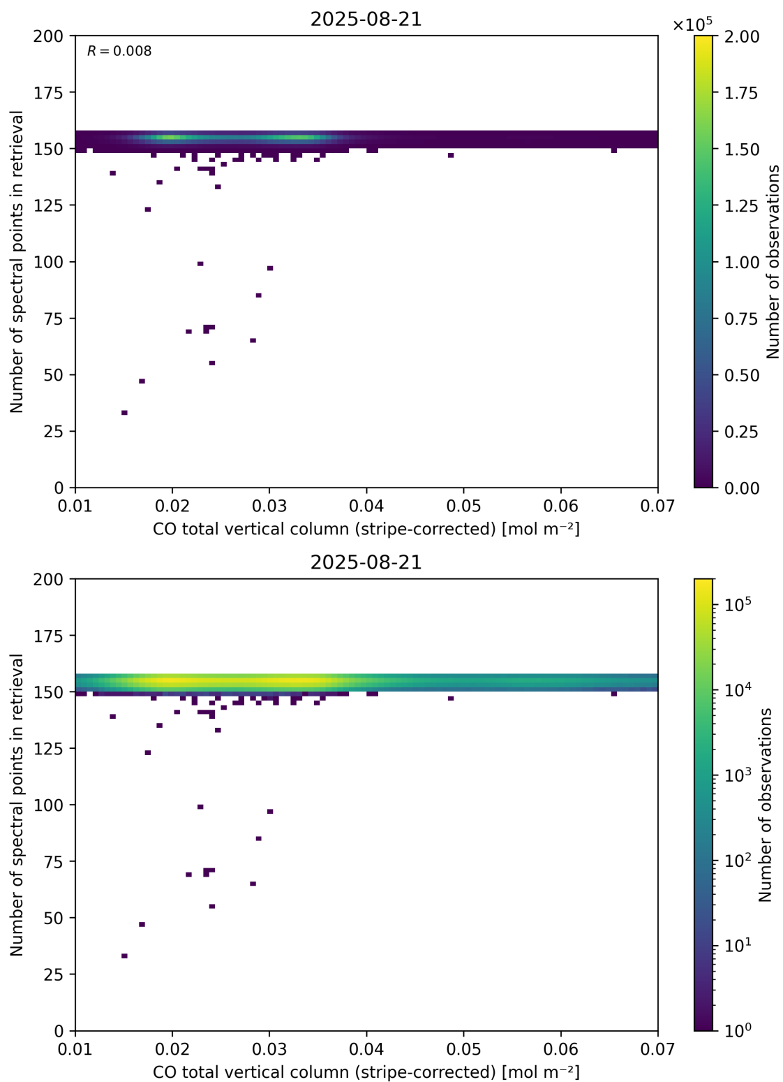
Figure 40: Scatter density plot of “CO total vertical column (stripe-corrected)” against “Number of spectral points in retrieval” for 2025-08-20 to 2025-08-22.
