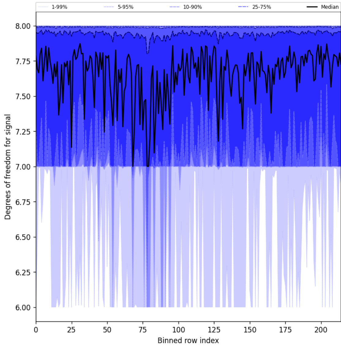
Figure 31: Along track statistics of “Degrees of freedom for signal” for 2025-08-20 to 2025-08-22
