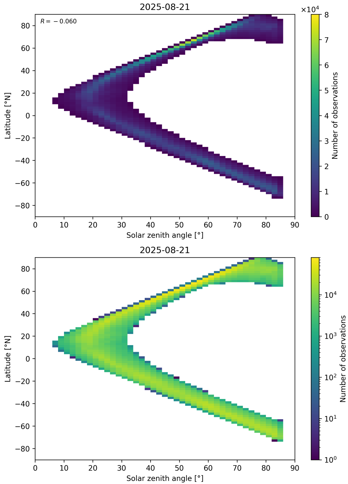
Figure 66: Scatter density plot of “Solar zenith angle” against “Latitude” for 2025-08-20 to 2025-08-22.
