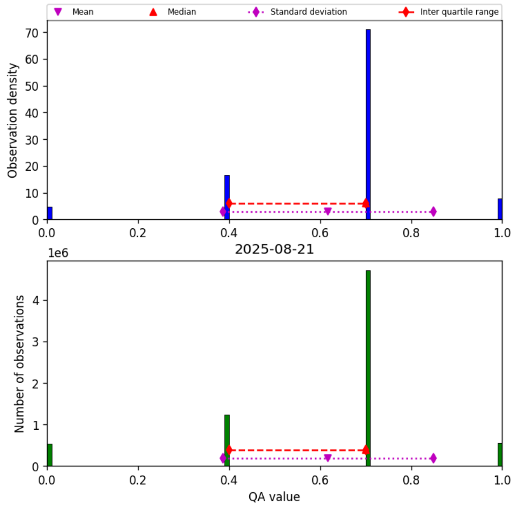
Figure 17: Histogram of “QA value” for 2025-08-20 to 2025-08-22
