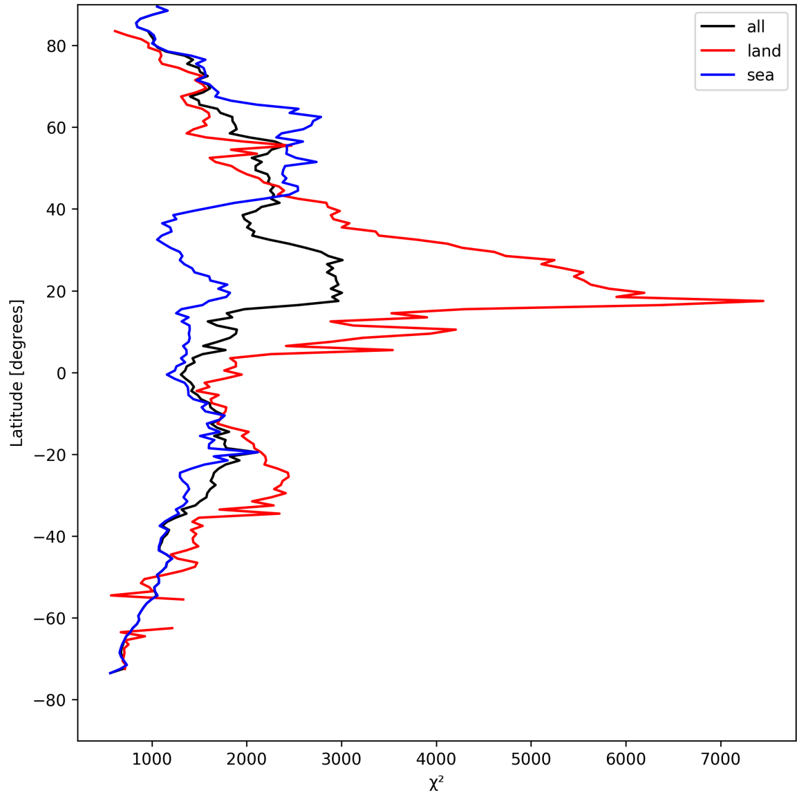
Figure 14: Zonal average of “ \chi^2 ” for 2025-08-20 to 2025-08-22.
