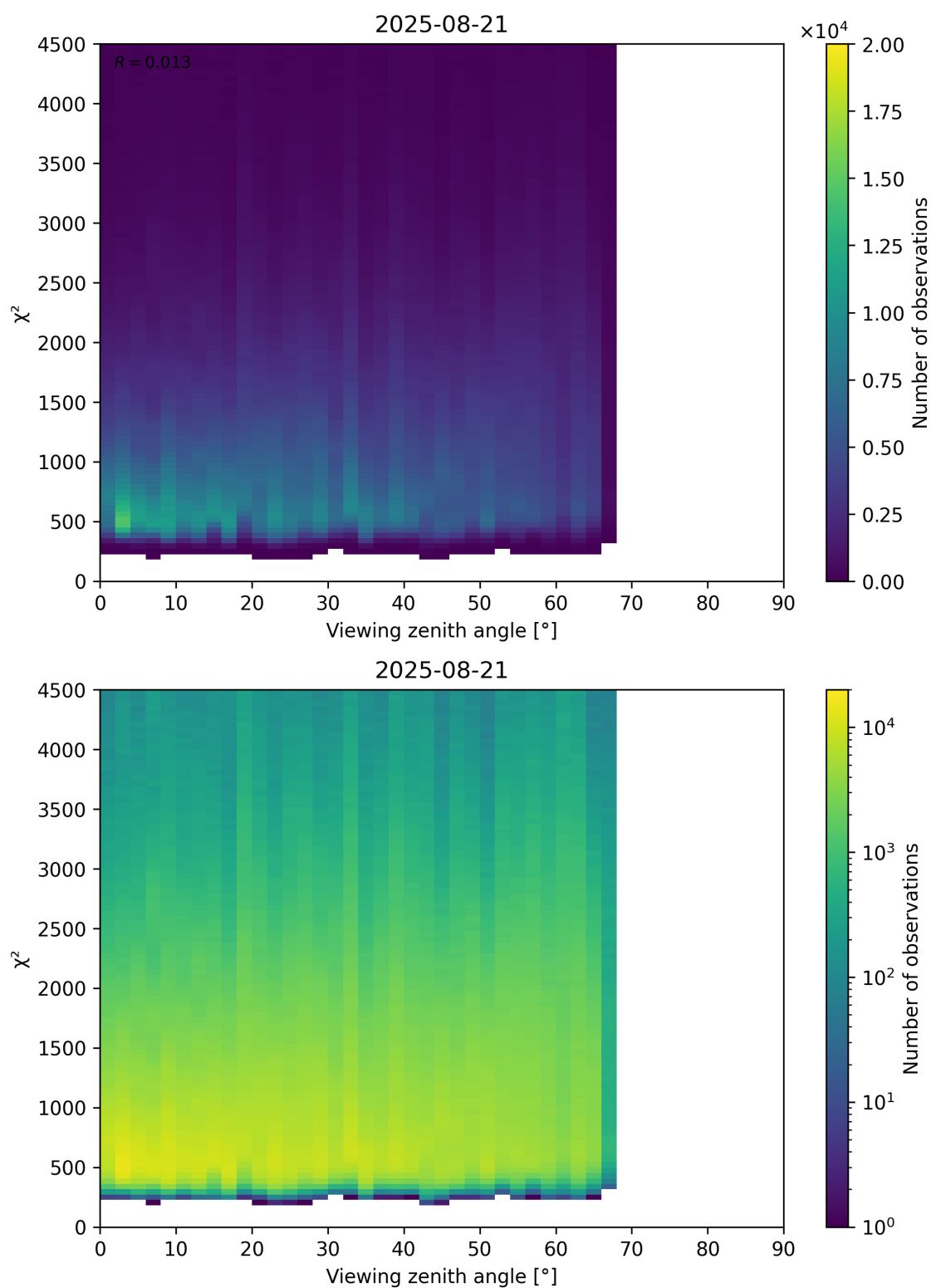
Figure 72: Scatter density plot of “Viewing zenith angle” against “ \chi^2 ” for 2025-08-20 to 2025-08-22.
