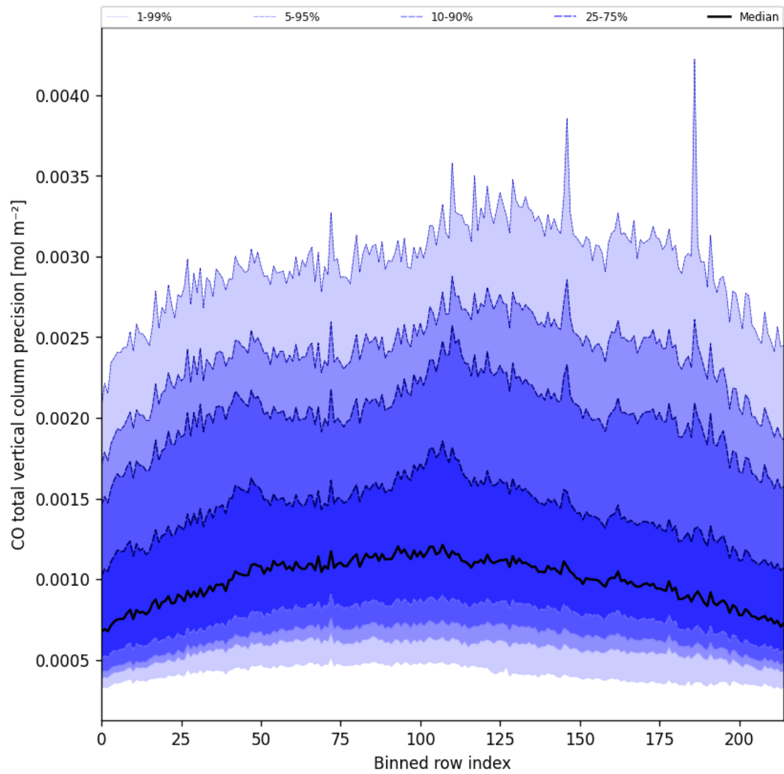
Figure 28: Along track statistics of “CO total vertical column precision” for 2025-08-20 to 2025-08-22
