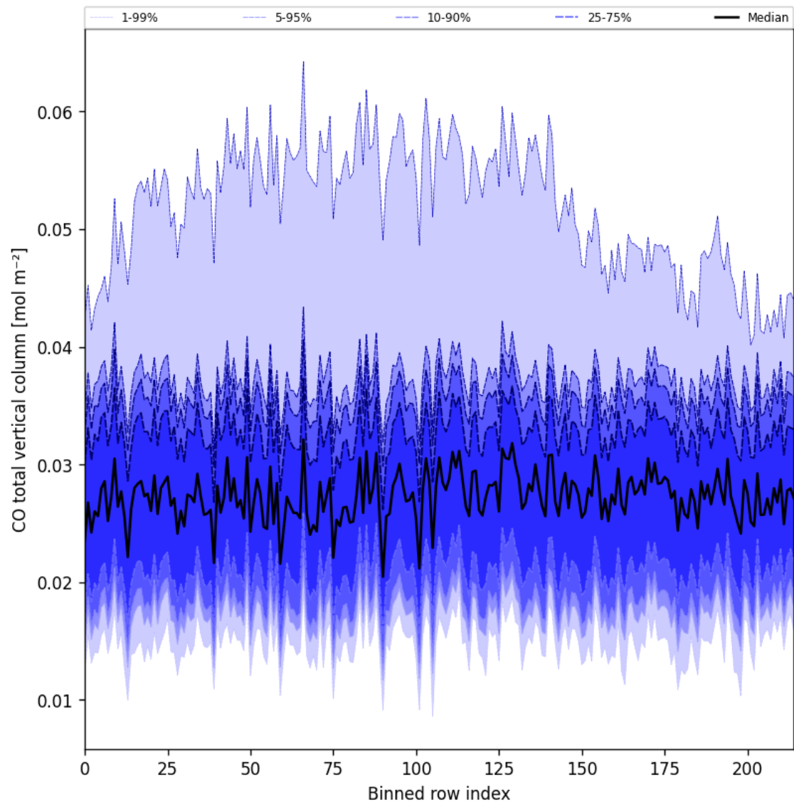
Figure 26: Along track statistics of “CO total vertical column” for 2025-08-20 to 2025-08-22
