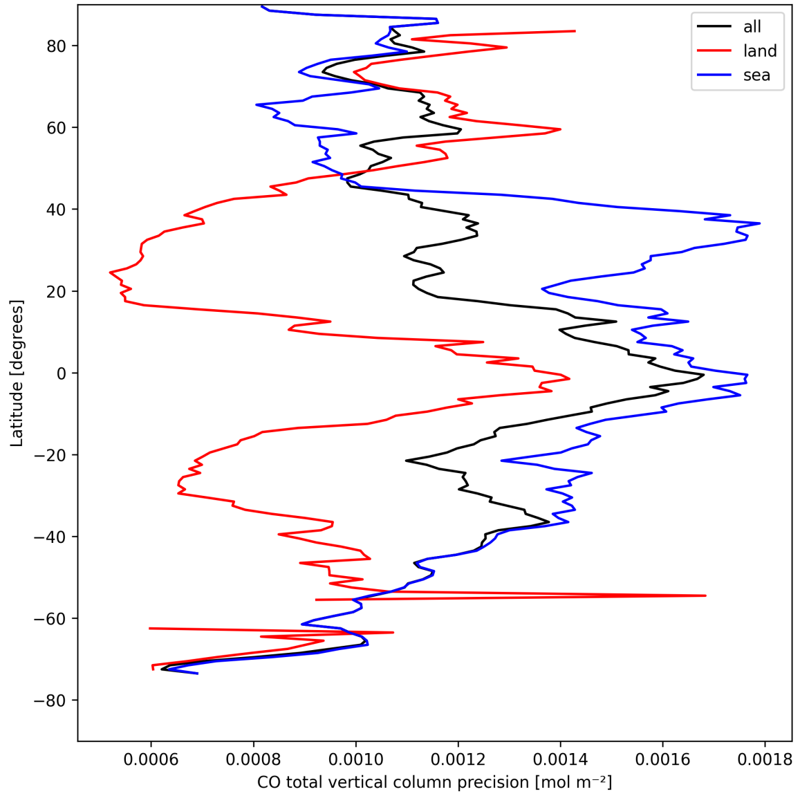
Figure 12: Zonal average of "CO total vertical column precision" for 2025-08-20 to 2025-08-22.
