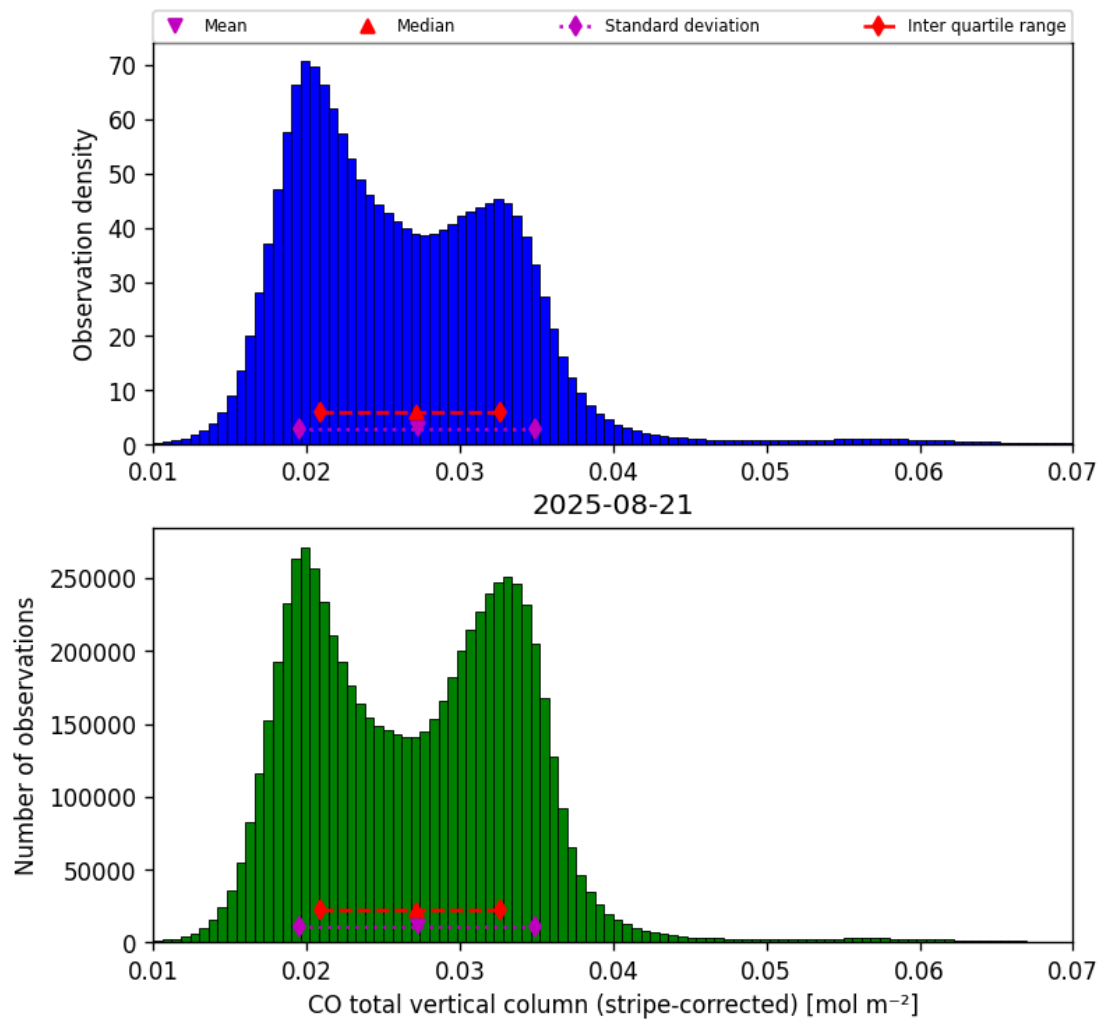
Figure 19: Histogram of “CO total vertical column (stripe-corrected)” for 2025-08-20 to 2025-08-22
