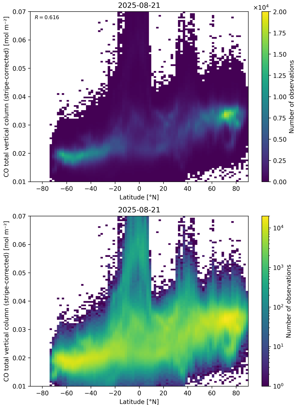
Figure 52: Scatter density plot of “Latitude” against “CO total vertical column (stripe-corrected)” for 2025-08-20 to 2025-08-22.
