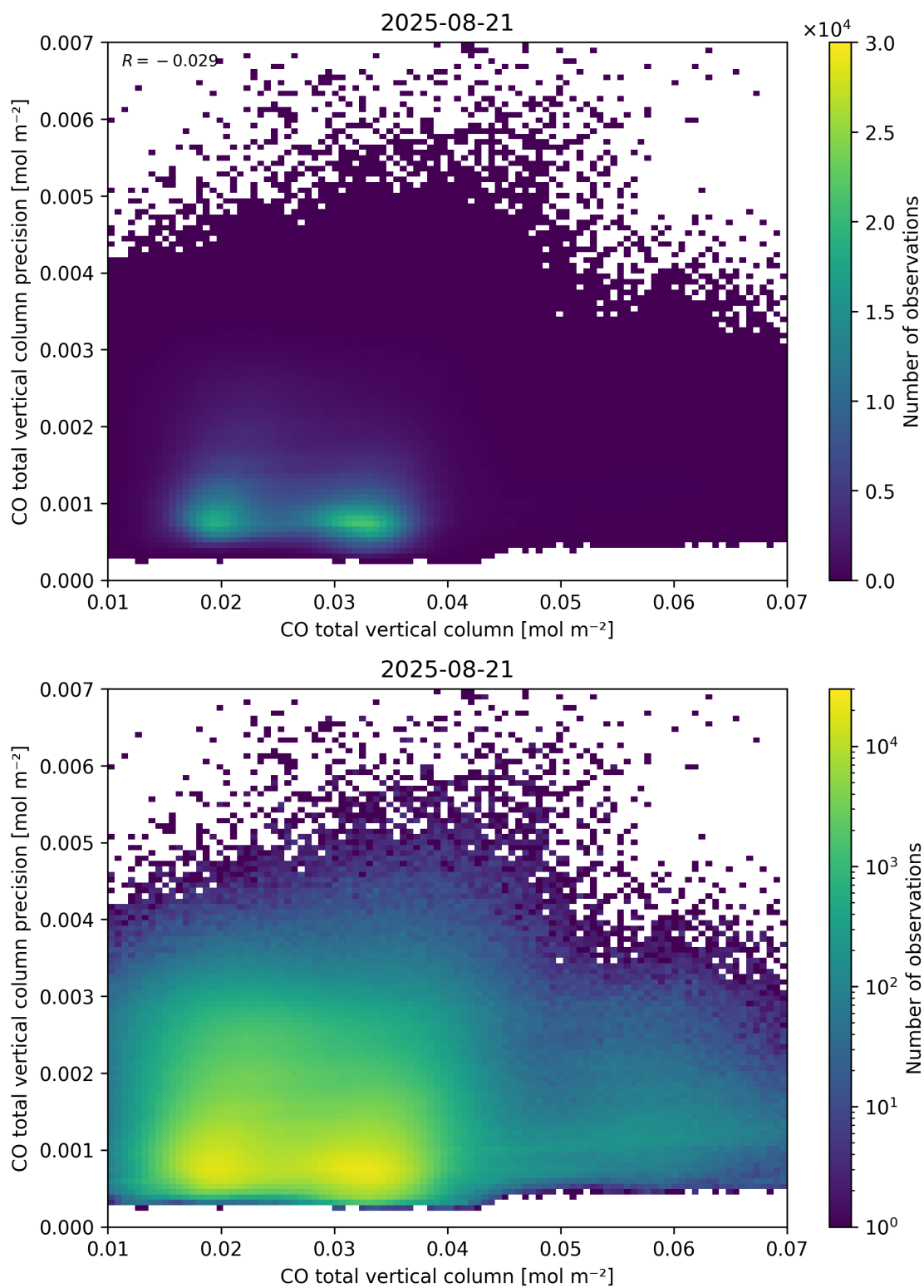
Figure 34: Scatter density plot of “CO total vertical column” against “CO total vertical column precision” for 2025-08-20 to 2025-08-22.
