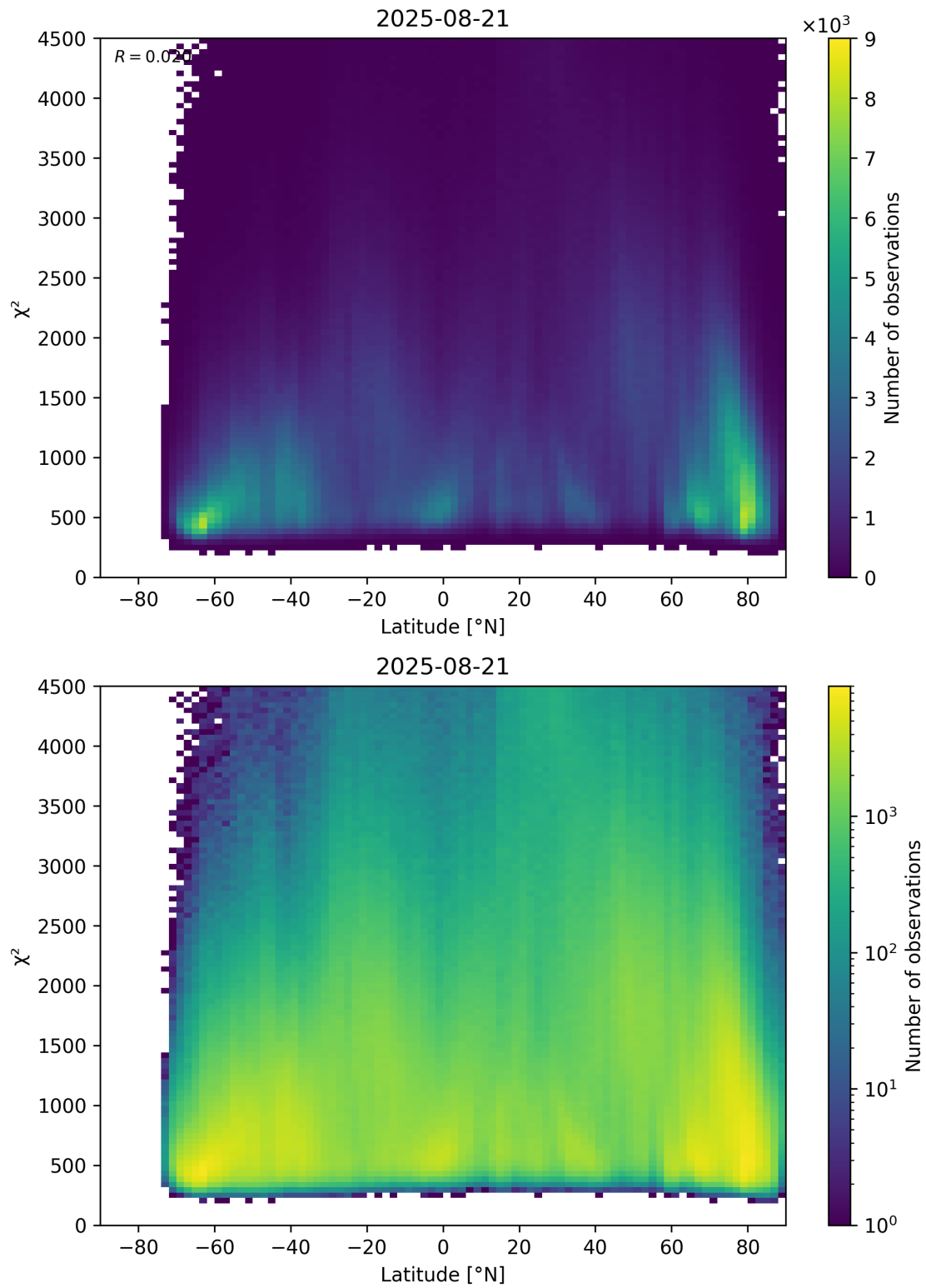
Figure 54: Scatter density plot of “Latitude” against “ \chi^2 ” for 2025-08-20 to 2025-08-22.
