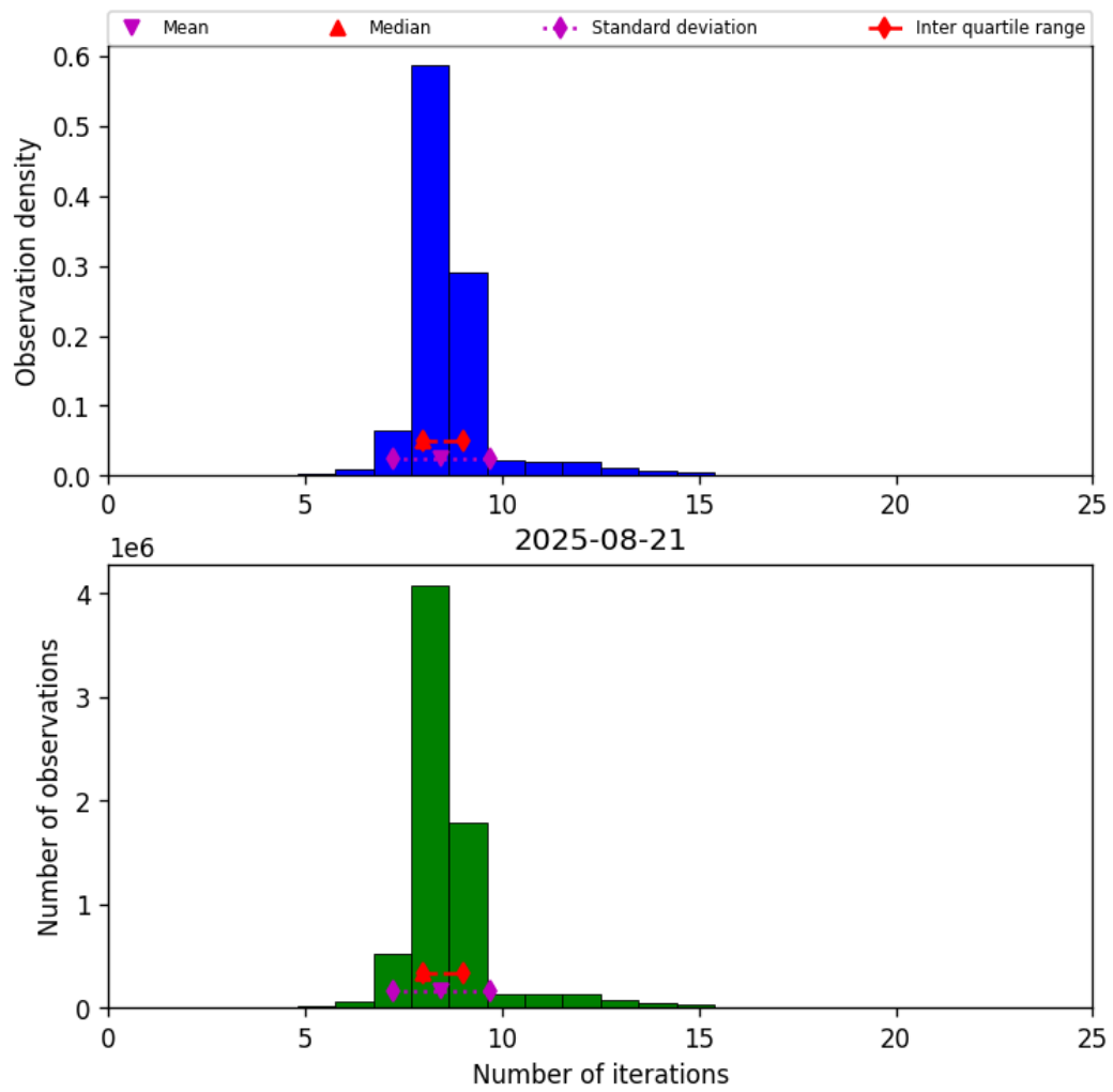
Figure 24: Histogram of “Number of iterations” for 2025-08-20 to 2025-08-22
