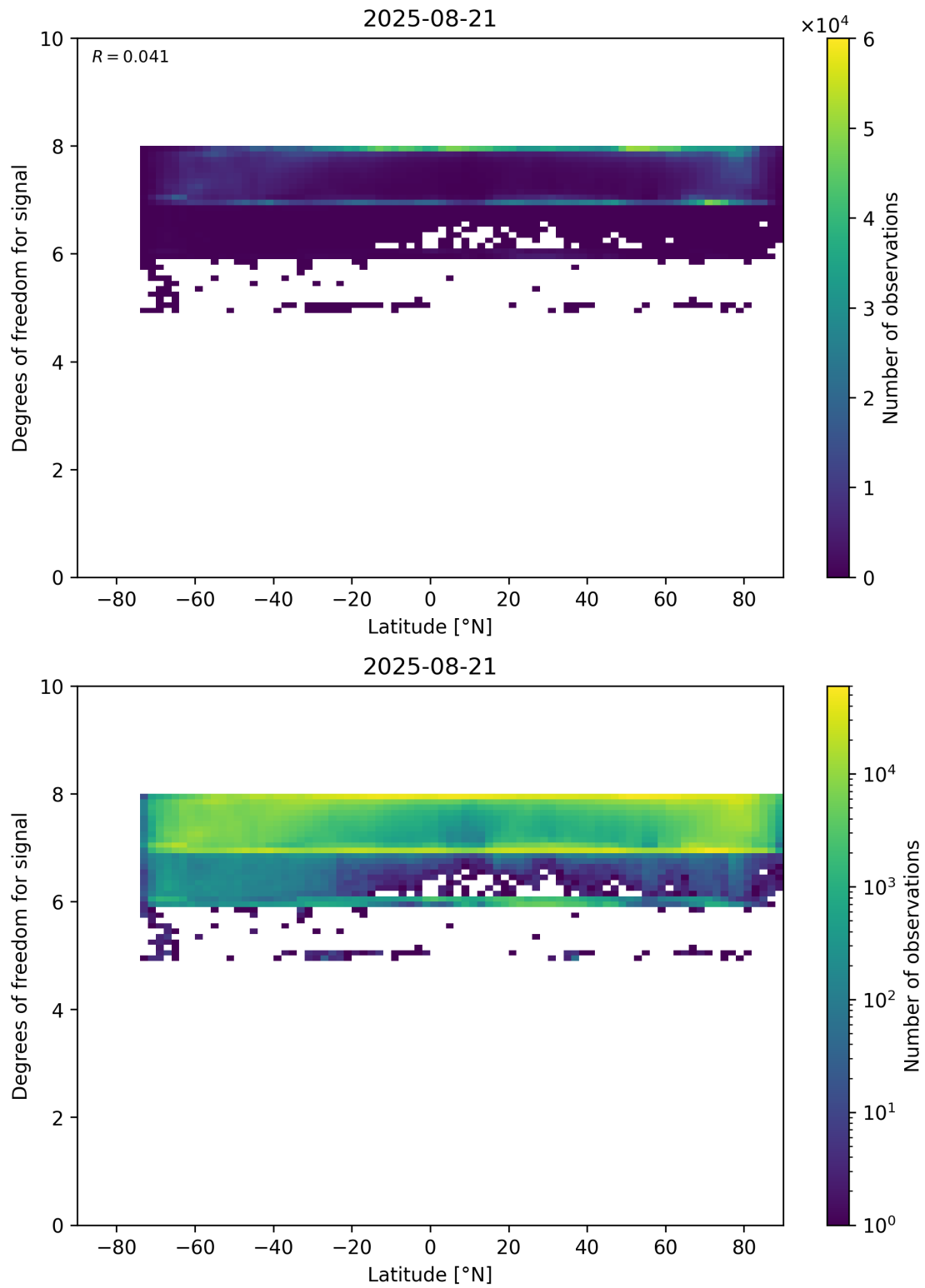
Figure 55: Scatter density plot of “Latitude” against “Degrees of freedom for signal” for 2025-08-20 to 2025-08-22.
