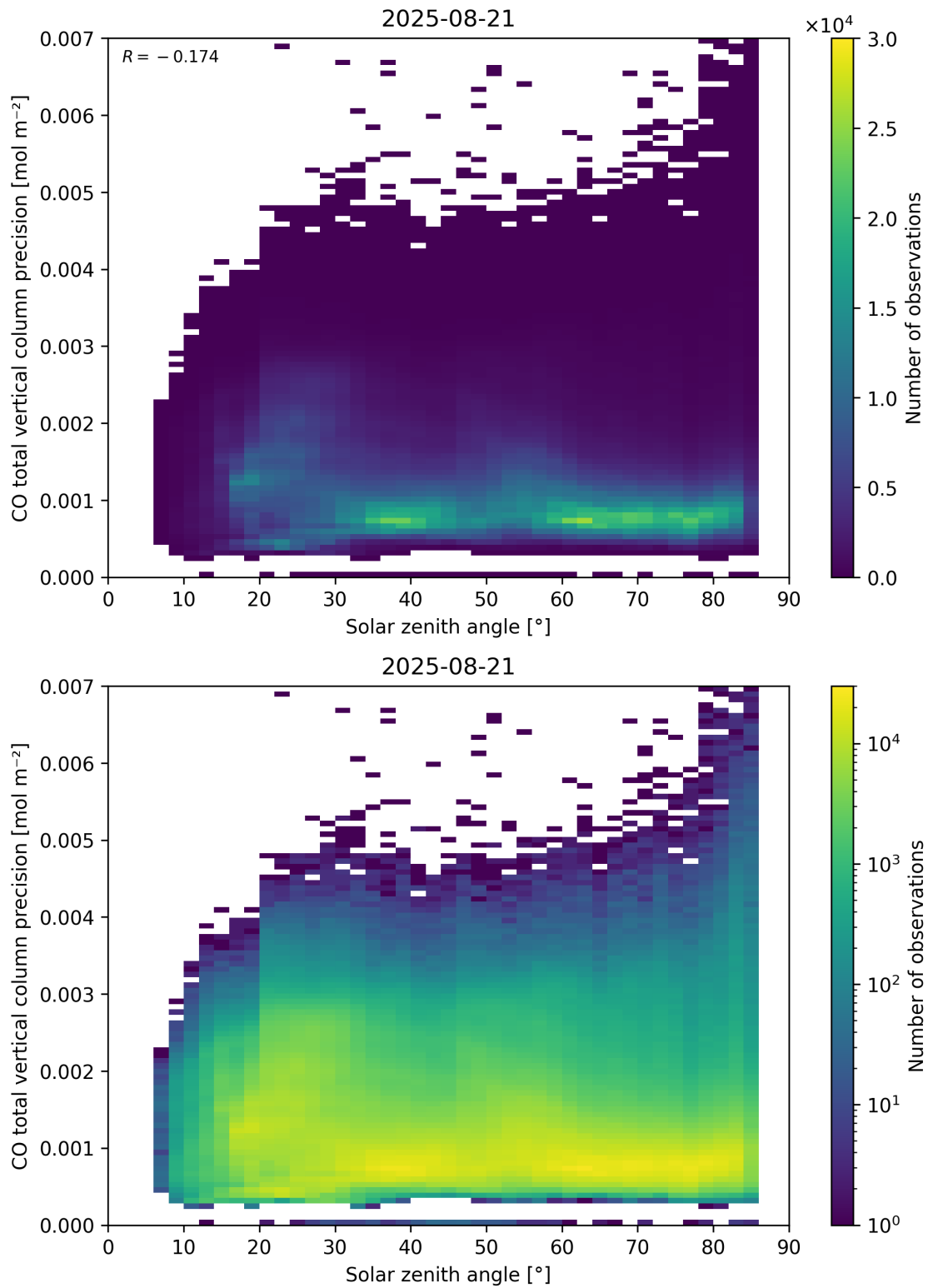
Figure 63: Scatter density plot of “Solar zenith angle” against “CO total vertical column precision” for 2025-08-20 to 2025-08-22.
