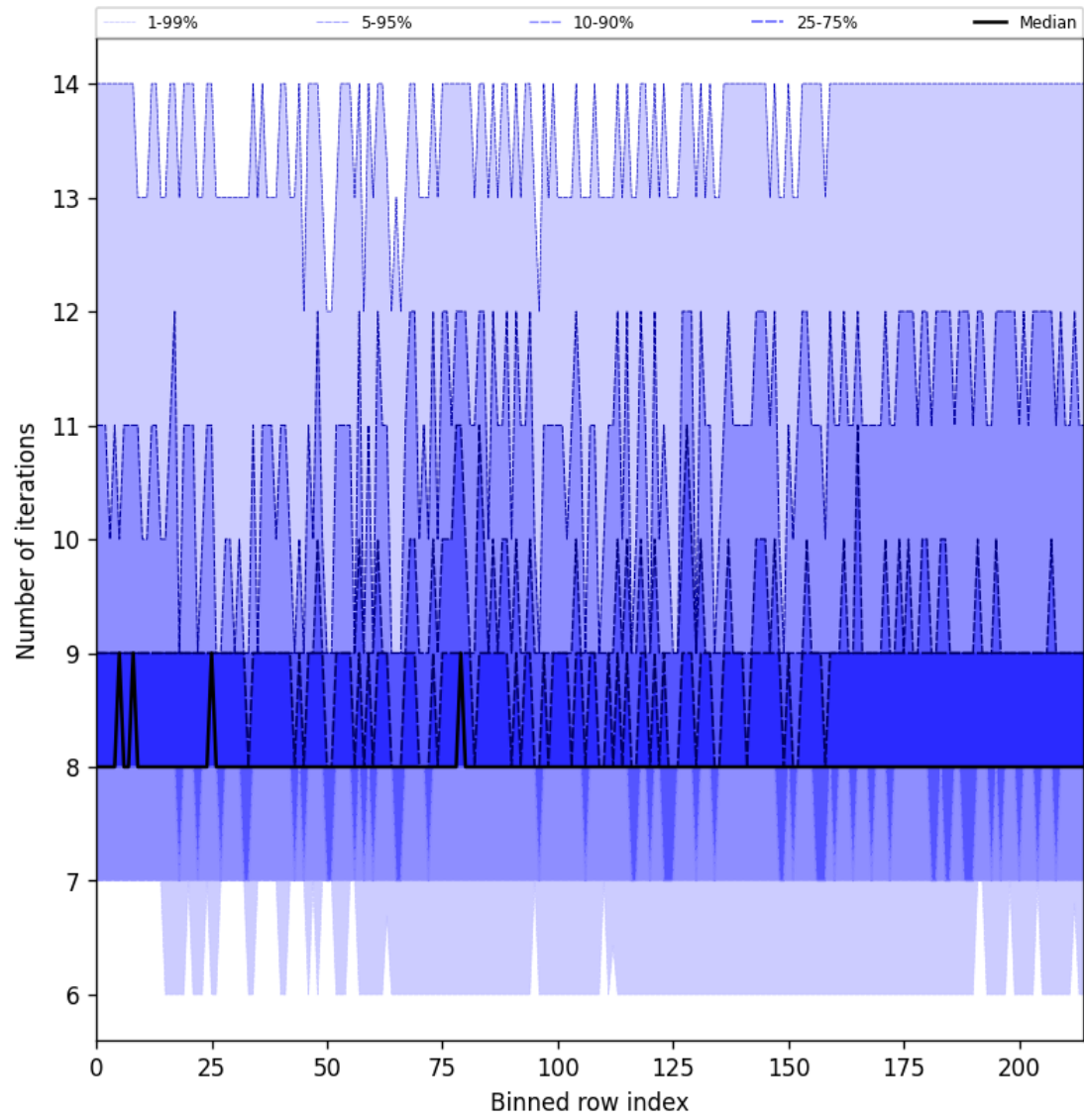
Figure 32: Along track statistics of “Number of iterations” for 2025-08-20 to 2025-08-22
