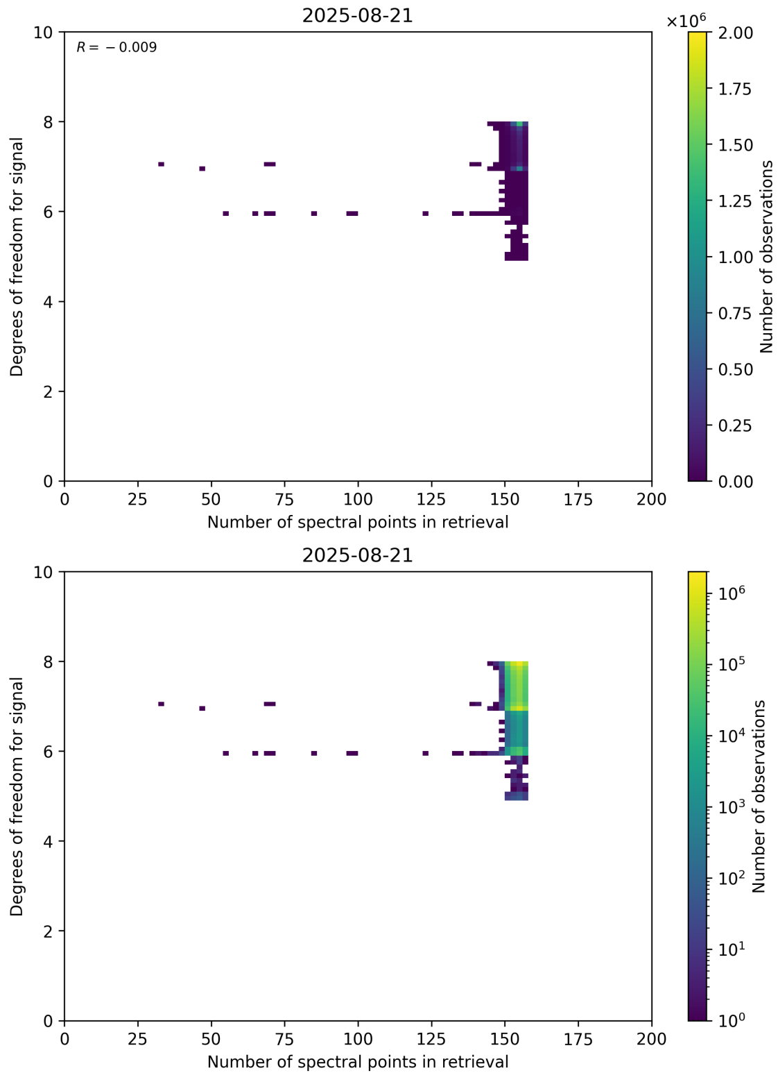
Figure 59: Scatter density plot of “Number of spectral points in retrieval” against “Degrees of freedom for signal” for 2025-08-20 to 2025-08-22.
