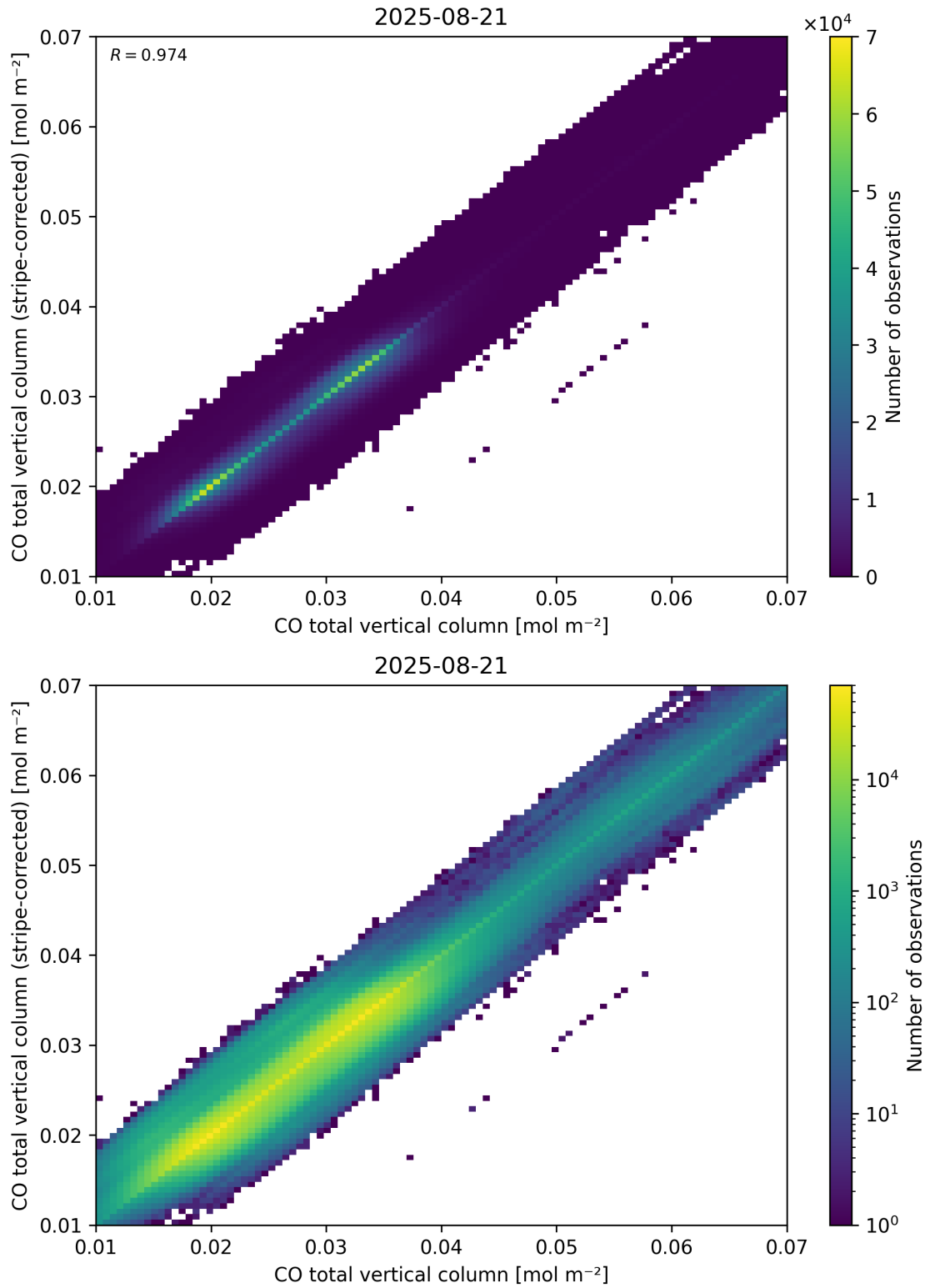
Figure 33: Scatter density plot of “CO total vertical column” against “CO total vertical column (stripe-corrected)” for 2025-08-20 to 2025-08-22.
