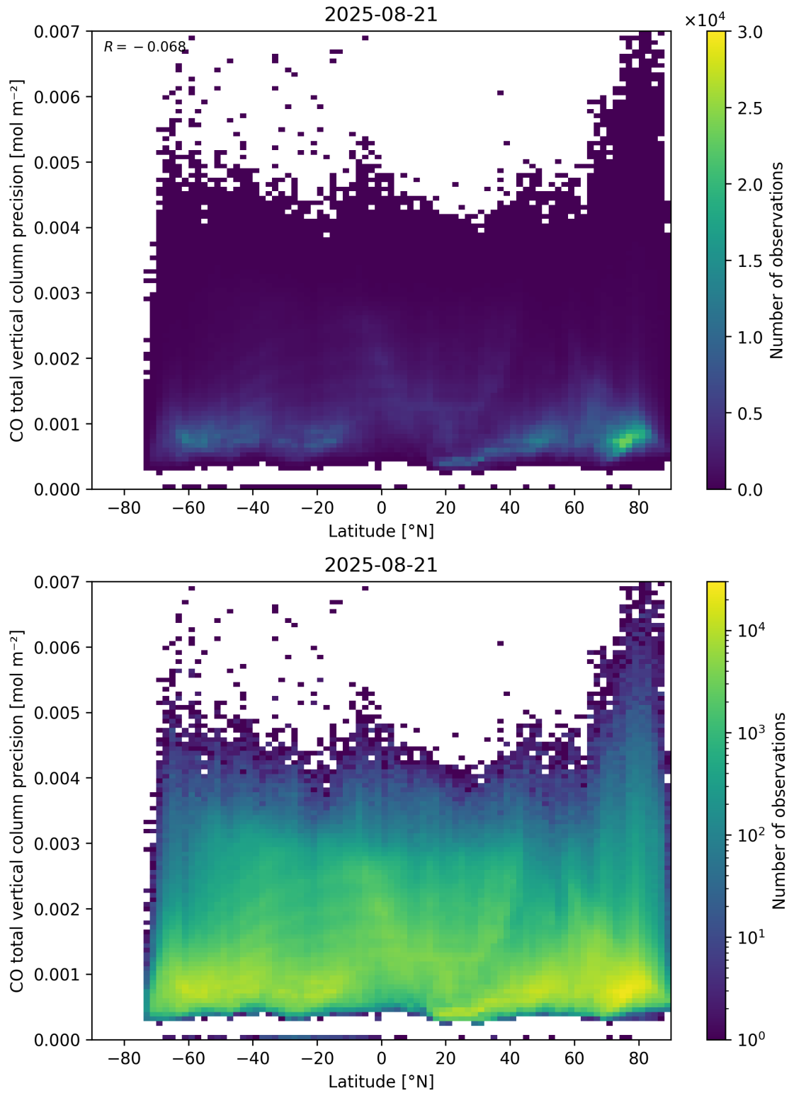
Figure 53: Scatter density plot of “Latitude” against “CO total vertical column precision” for 2025-08-20 to 2025-08-22.
