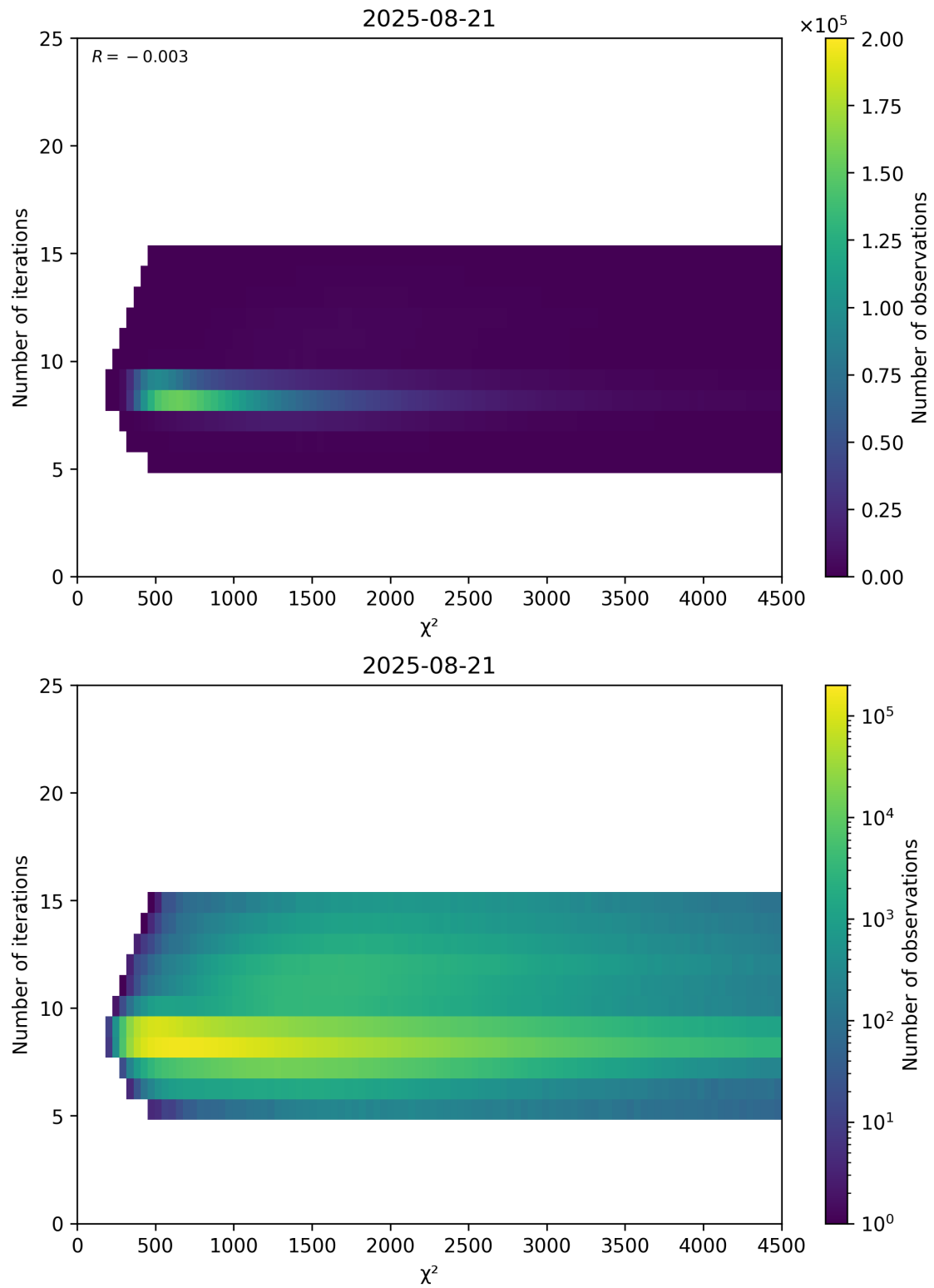
Figure 49: Scatter density plot of “ \chi^2 ” against “Number of iterations” for 2025-08-20 to 2025-08-22.
