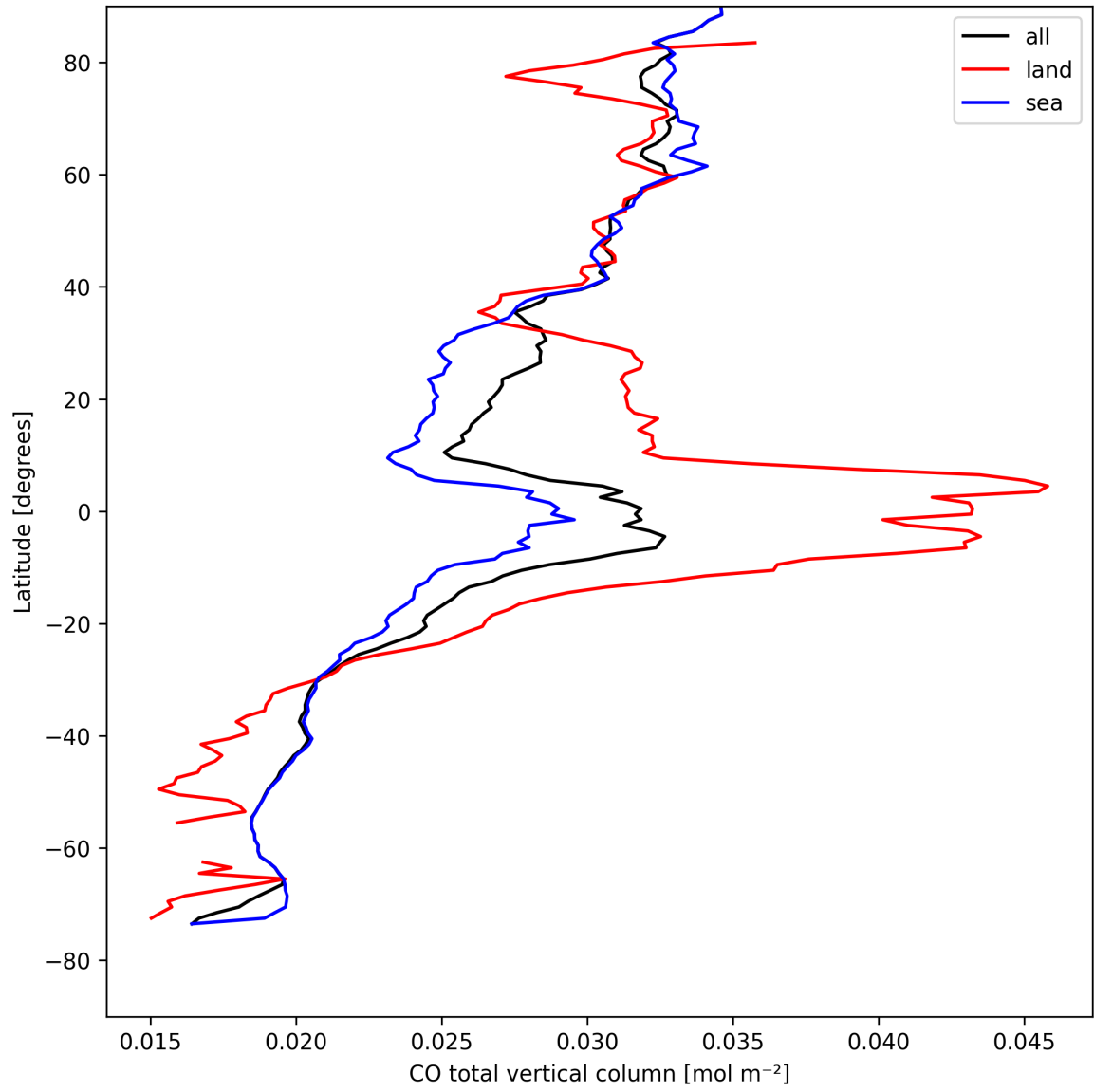
Figure 10: Zonal average of “CO total vertical column” for 2025-08-20 to 2025-08-22.
