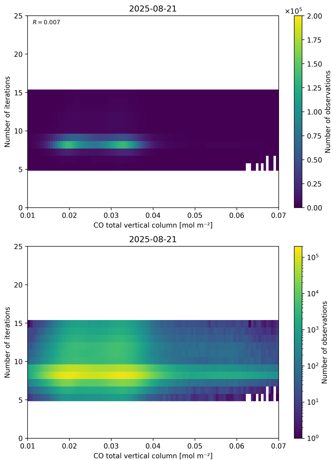
Figure 42: Scatter density plot of “CO total vertical column” against “Number of iterations” for 2025-08-20 to 2025-08-22.
