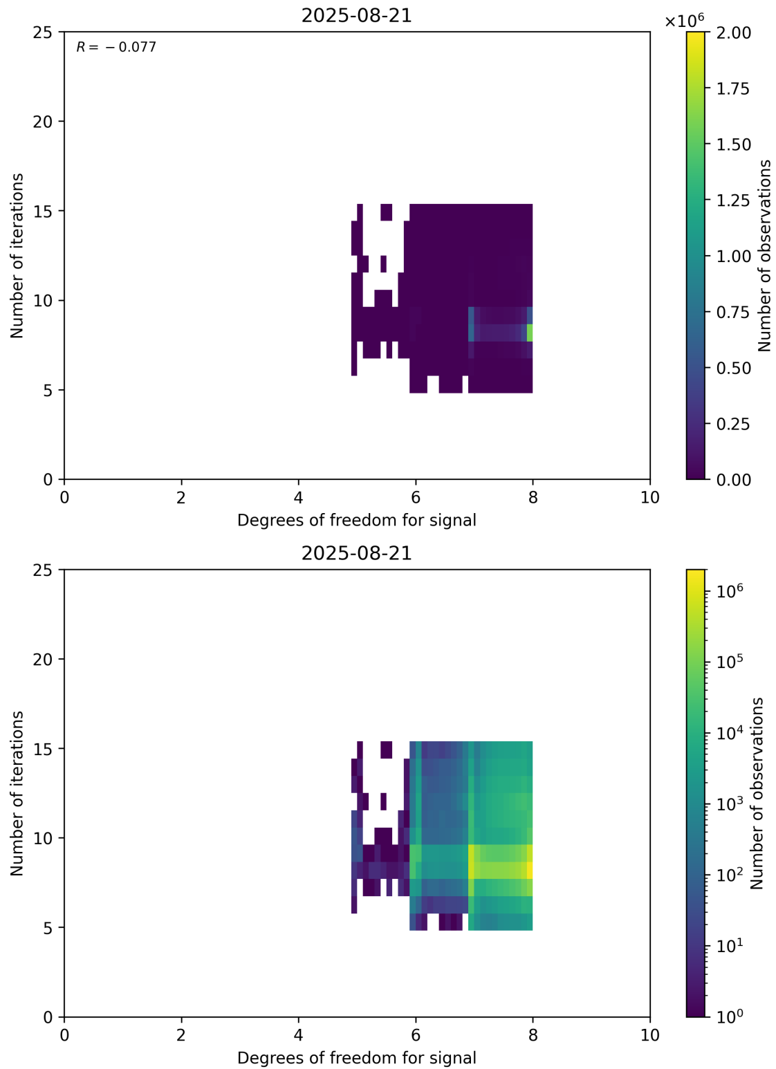
Figure 50: Scatter density plot of “Degrees of freedom for signal” against “Number of iterations” for 2025-08-20 to 2025-08-22.
