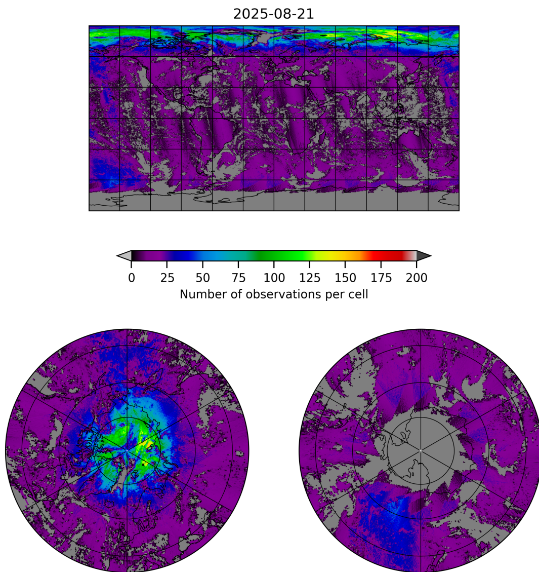
Figure 8: Map of the number of observations for 2025-08-20 to 2025-08-22
