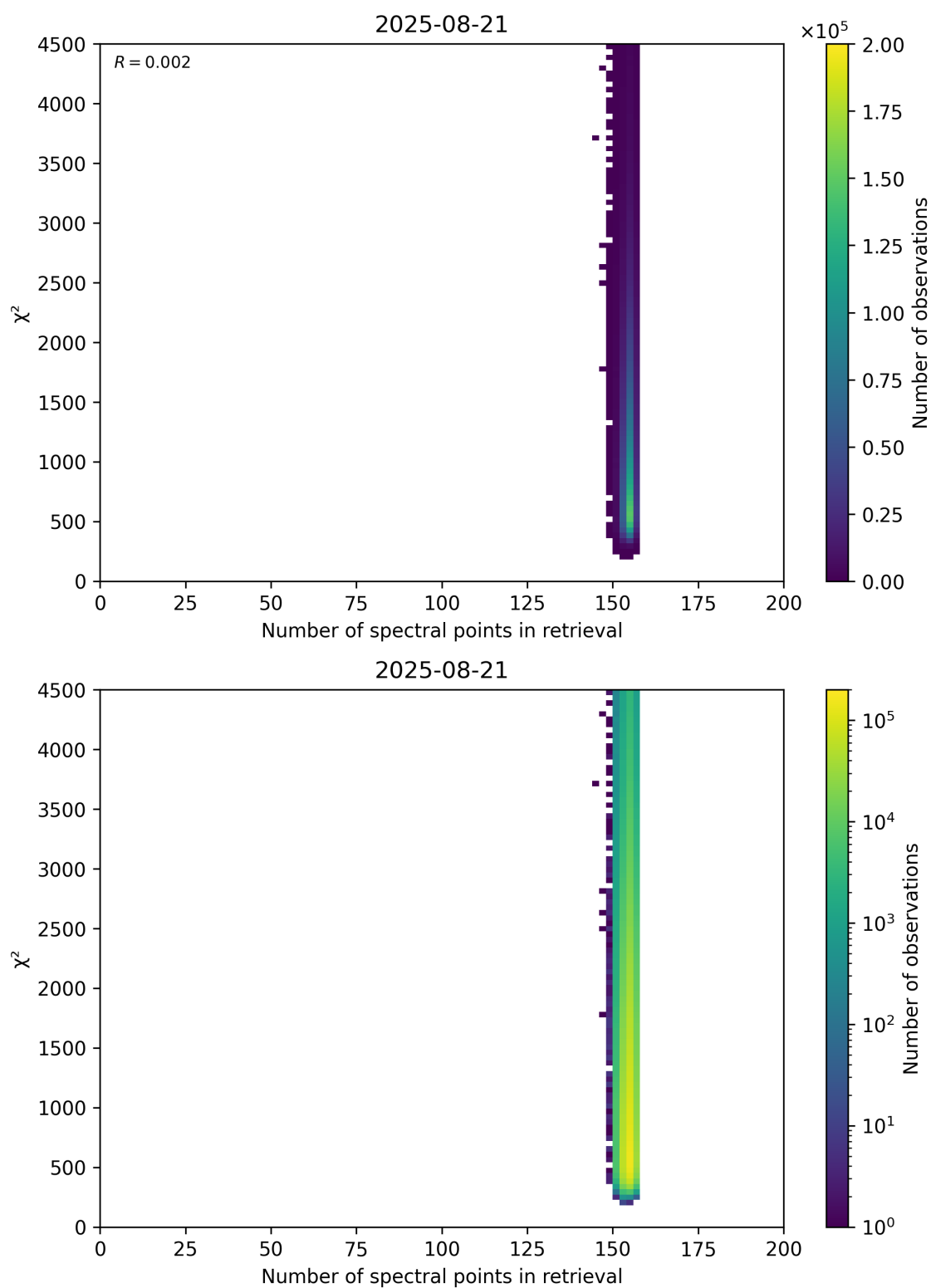
Figure 58: Scatter density plot of “Number of spectral points in retrieval” against “ \chi^2 ” for 2025-08-20 to 2025-08-22.
