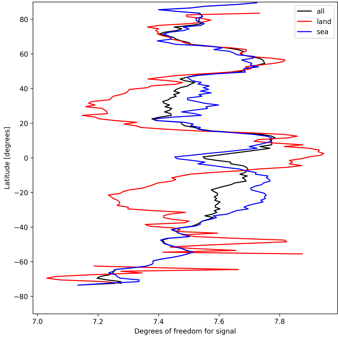
Figure 15: Zonal average of “Degrees of freedom for signal” for 2025-08-20 to 2025-08-22.
