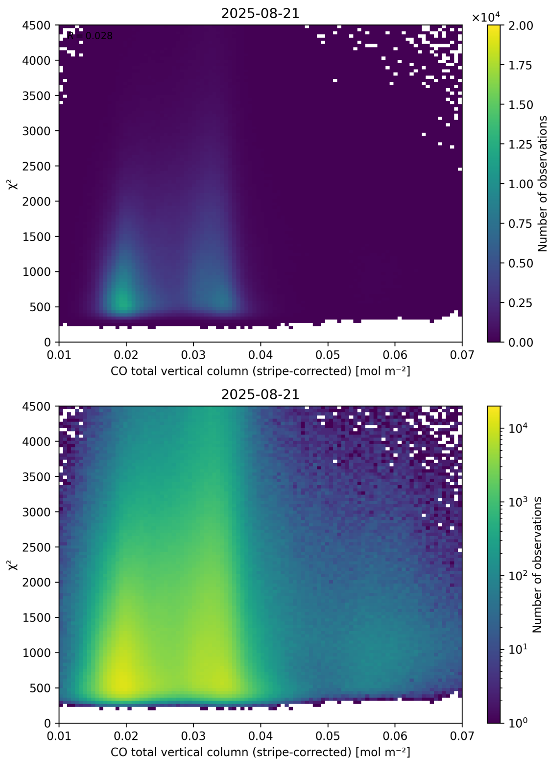
Figure 37: Scatter density plot of “CO total vertical column (stripe-corrected)” against “ \chi^2 ” for 2025-08-20 to 2025-08-22.
