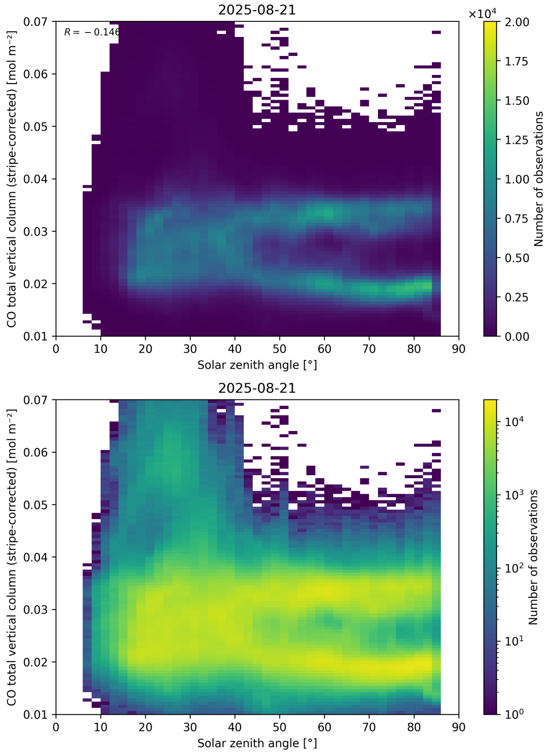
Figure 62: Scatter density plot of “Solar zenith angle” against “CO total vertical column (stripe-corrected)” for 2025-08-20 to 2025-08-22.
