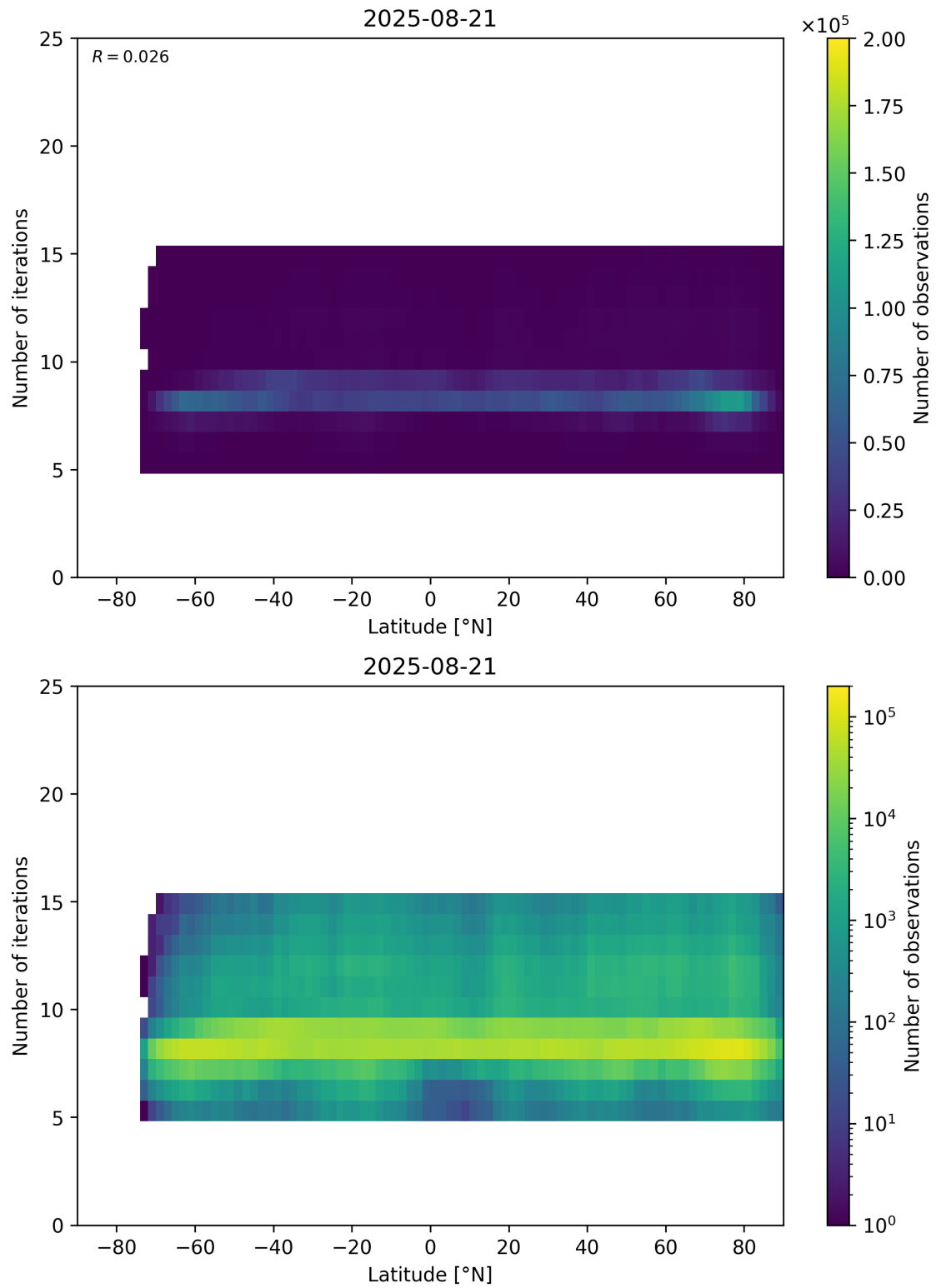
Figure 56: Scatter density plot of “Latitude” against “Number of iterations” for 2025-08-20 to 2025-08-22.
