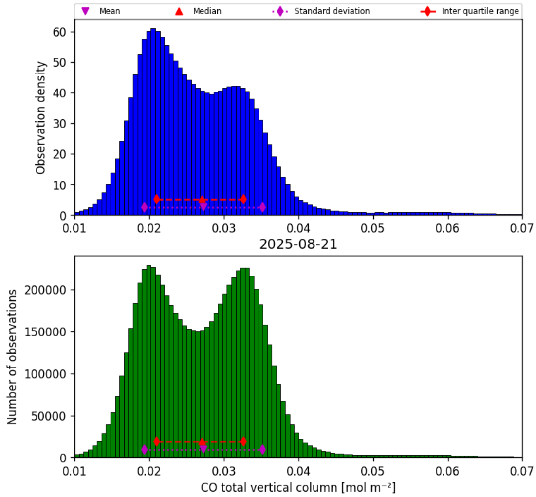
Figure 18: Histogram of “CO total vertical column” for 2025-08-20 to 2025-08-22
