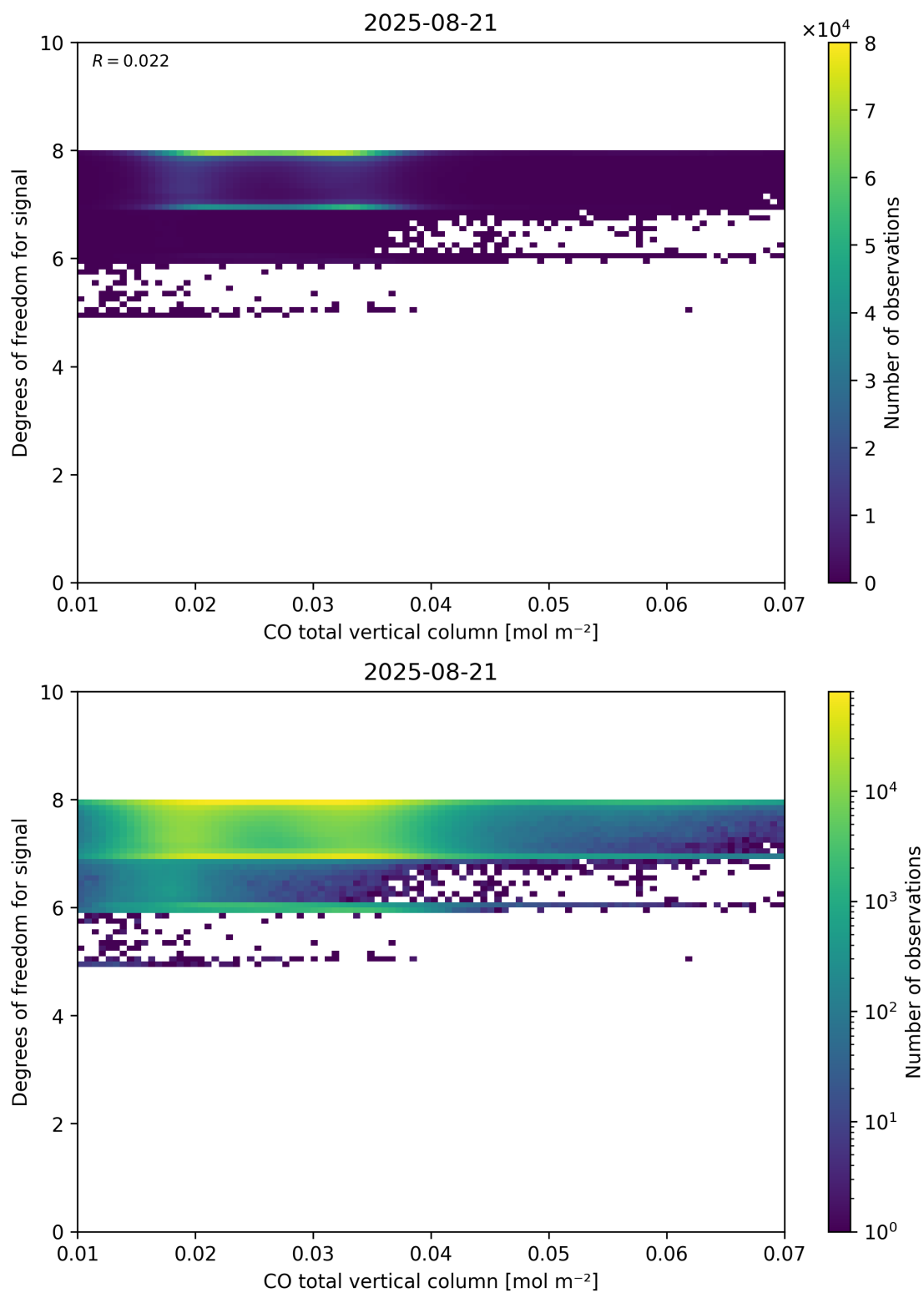
Figure 41: Scatter density plot of “CO total vertical column” against “Degrees of freedom for signal” for 2025-08-20 to 2025-08-22.
