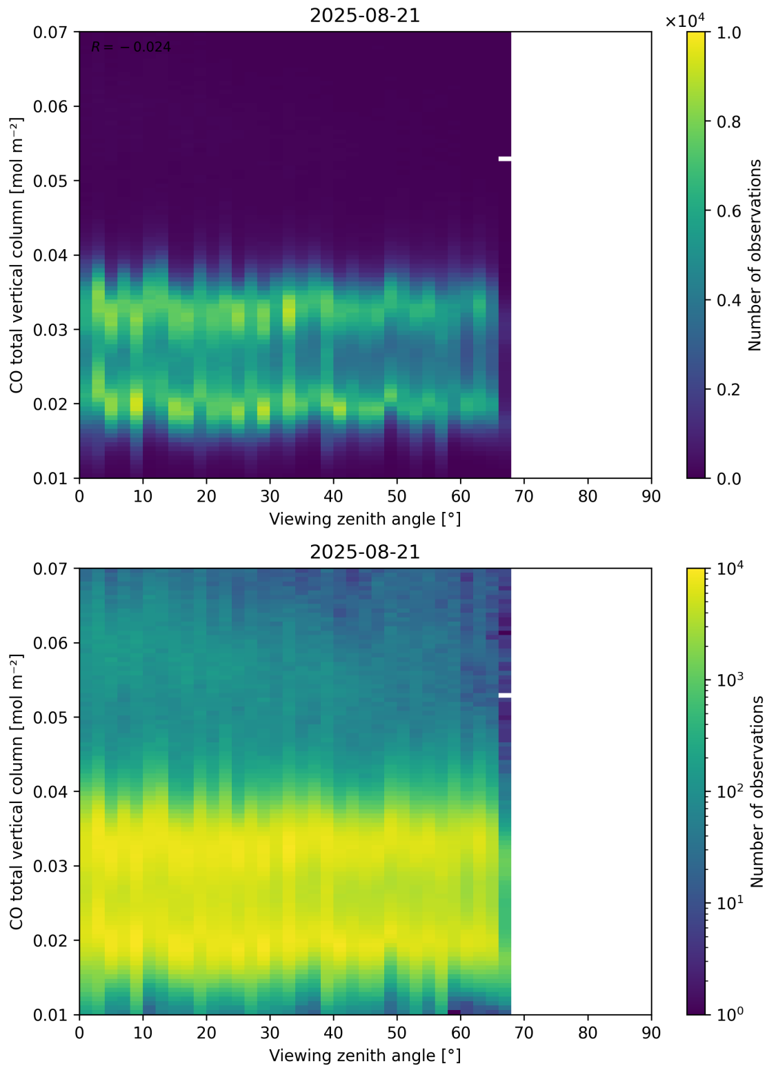
Figure 69: Scatter density plot of “Viewing zenith angle” against “CO total vertical column” for 2025-08-20 to 2025-08-22.
