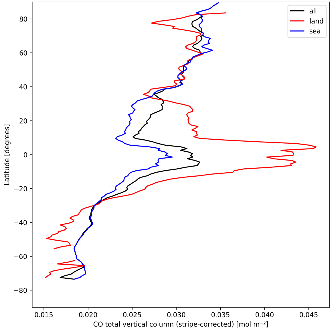
Figure 11: Zonal average of “CO total vertical column (stripe-corrected)” for 2025-08-20 to 2025-08-22.
