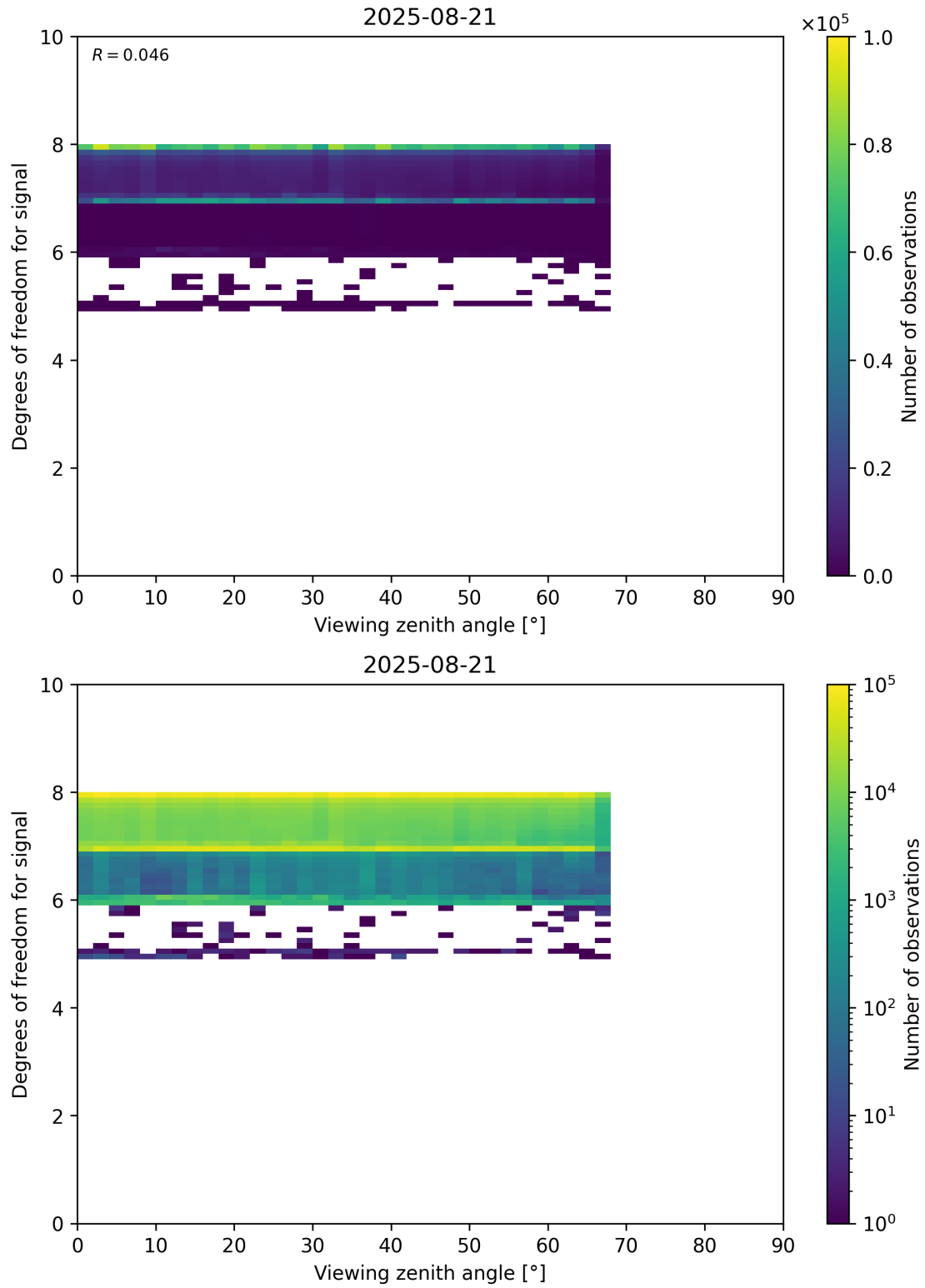
Figure 73: Scatter density plot of “Viewing zenith angle” against “Degrees of freedom for signal” for 2025-08-20 to 2025-08-22.
