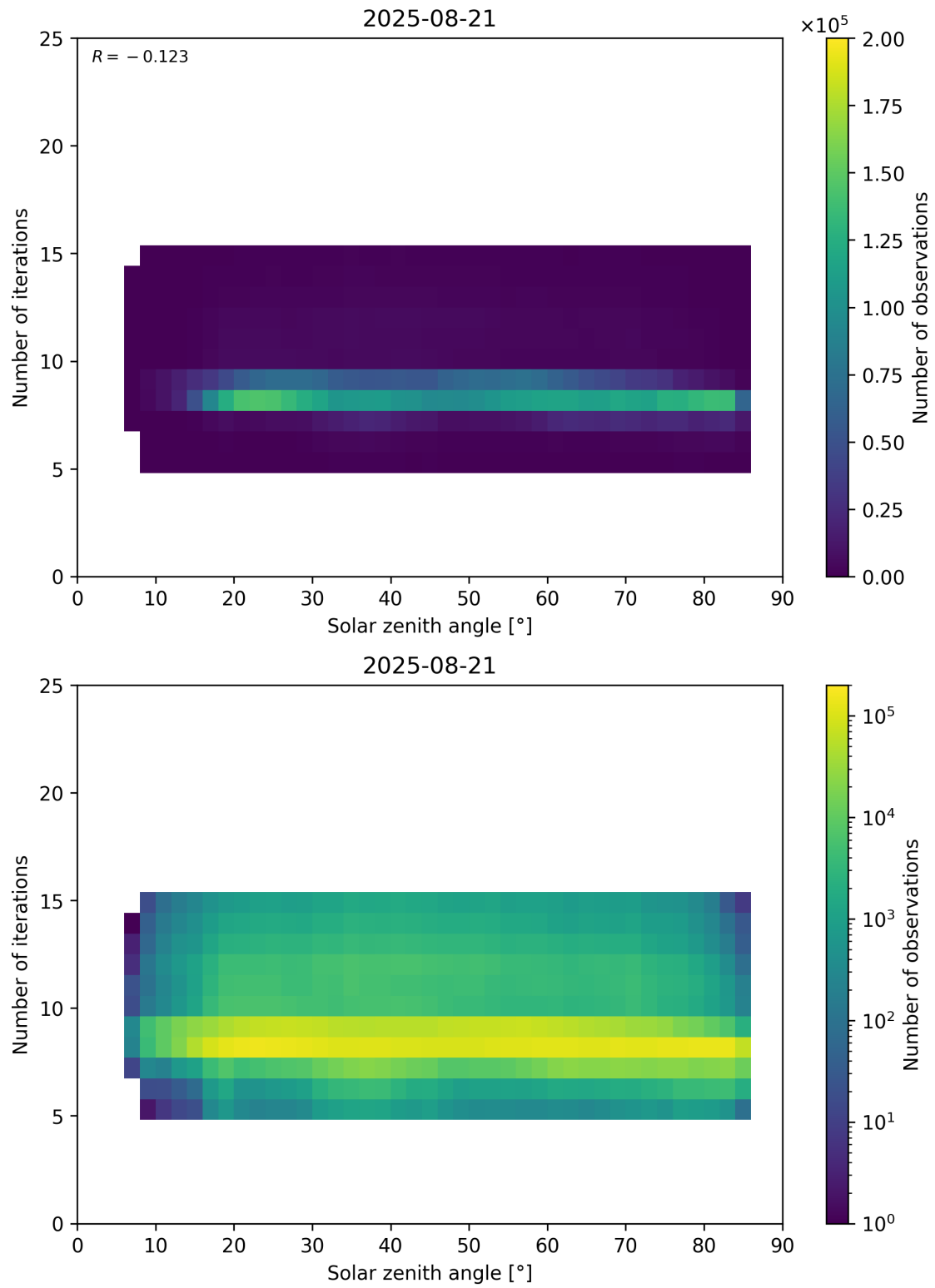
Figure 67: Scatter density plot of “Solar zenith angle” against “Number of iterations” for 2025-08-20 to 2025-08-22.
