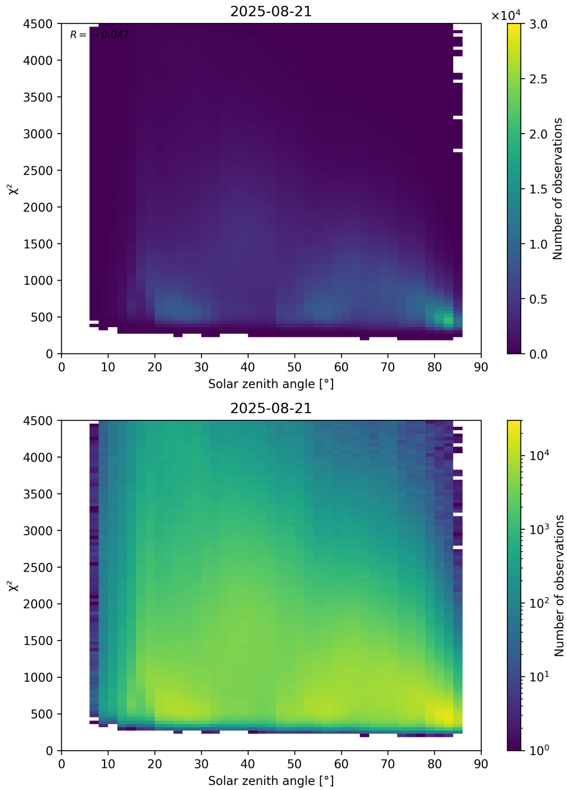
Figure 64: Scatter density plot of “Solar zenith angle” against “ \chi^2 ” for 2025-08-20 to 2025-08-22.
