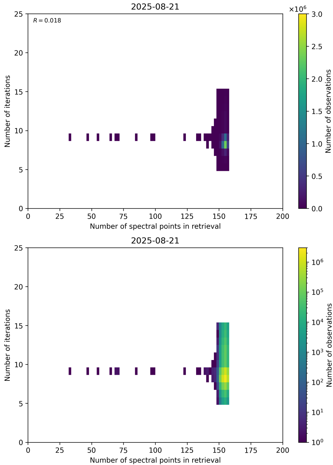
Figure 60: Scatter density plot of “Number of spectral points in retrieval” against “Number of iterations” for 2025-08-20 to 2025-08-22.
