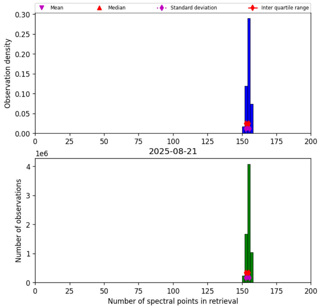
Figure 21: Histogram of “Number of spectral points in retrieval” for 2025-08-20 to 2025-08-22
