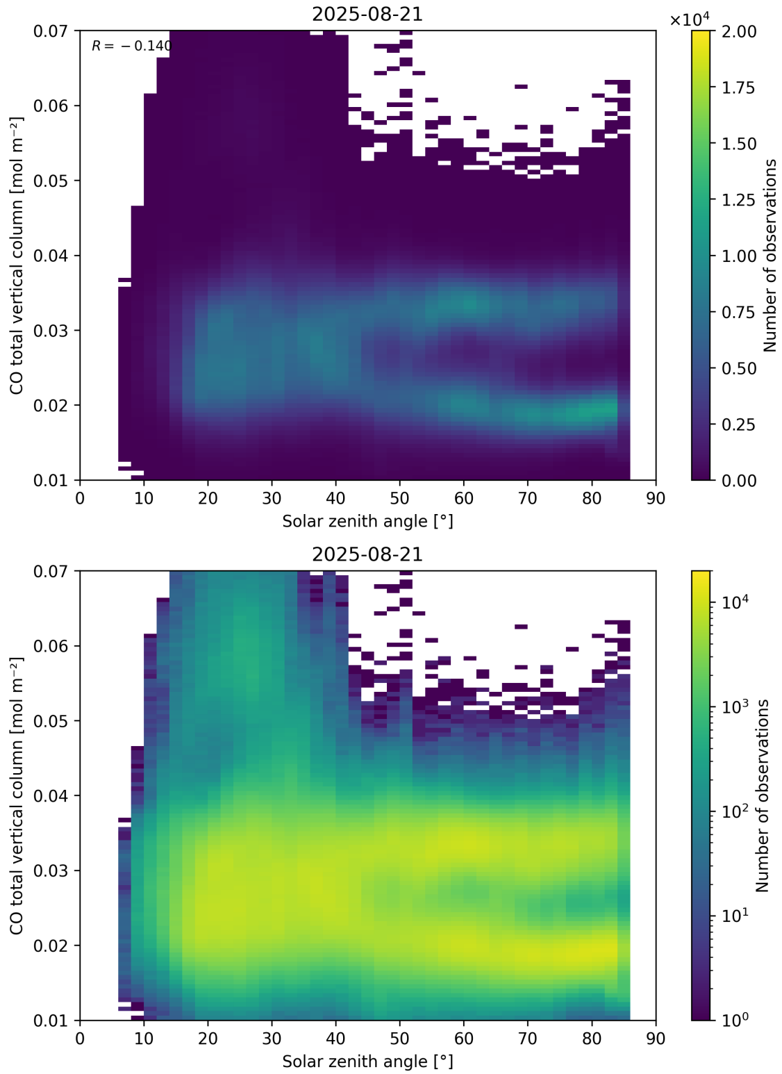
Figure 61: Scatter density plot of “Solar zenith angle” against “CO total vertical column” for 2025-08-20 to 2025-08-22.
