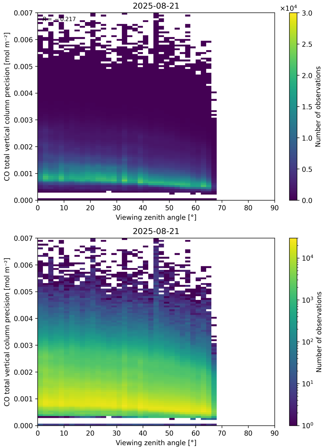
Figure 71: Scatter density plot of “Viewing zenith angle” against “CO total vertical column precision” for 2025-08-20 to 2025-08-22.
