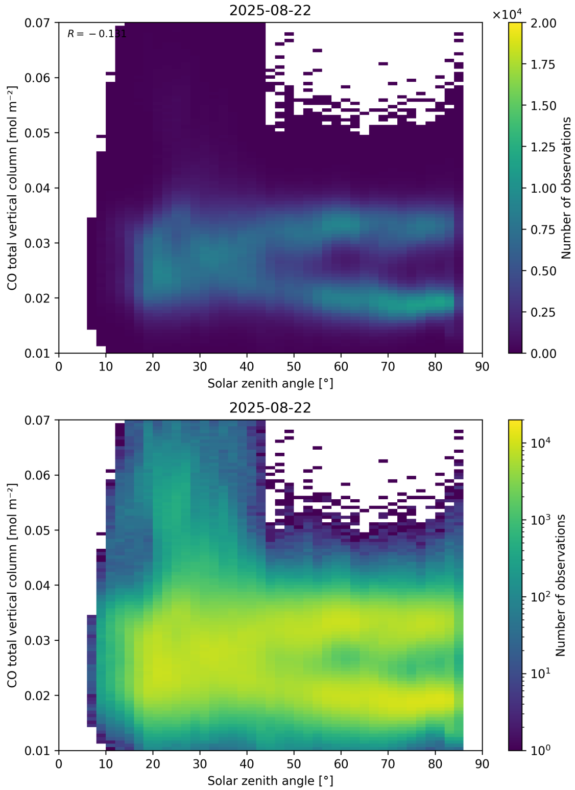
Figure 61: Scatter density plot of “Solar zenith angle” against “CO total vertical column” for 2025-08-21 to 2025-08-23.
