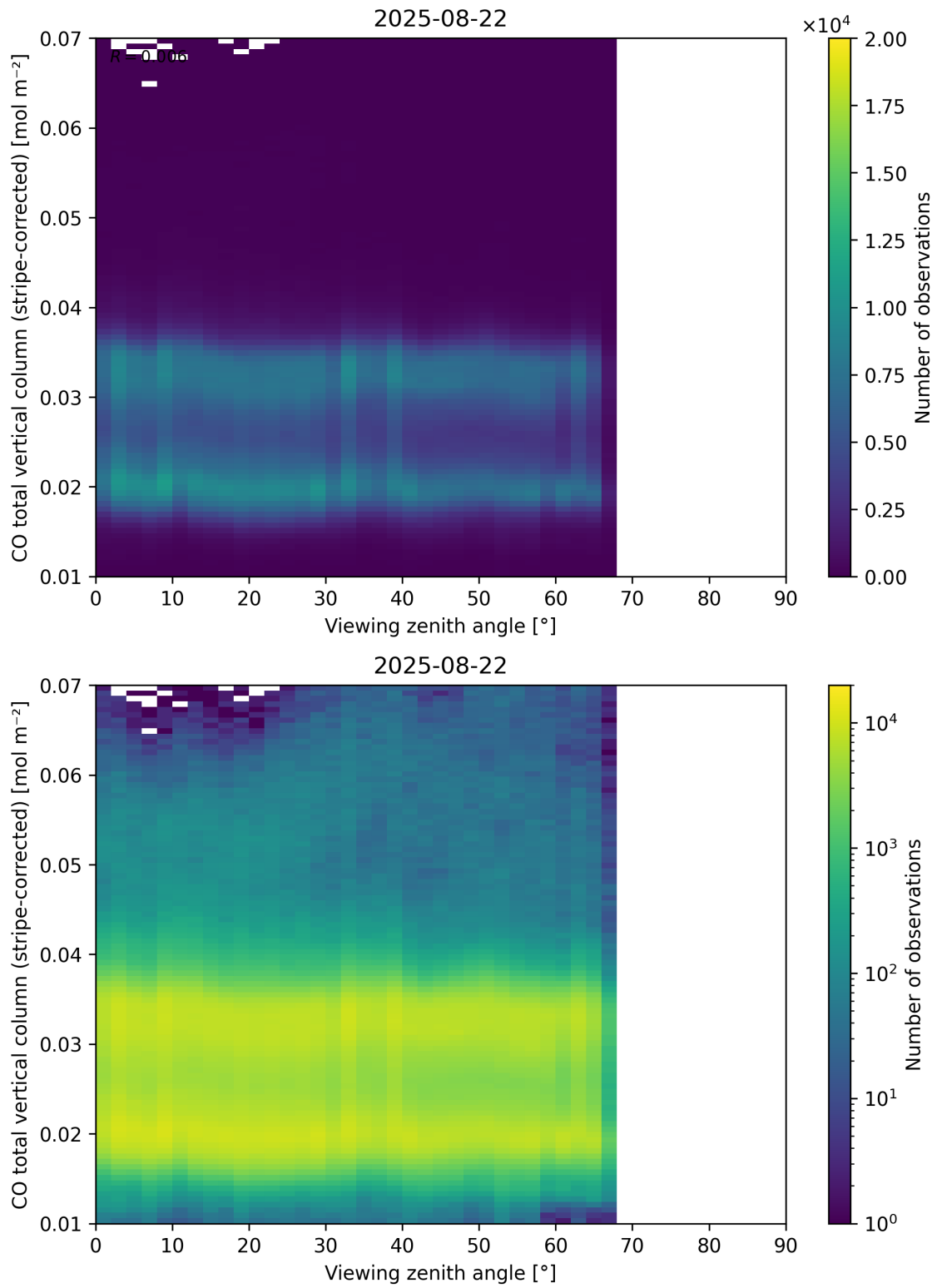
Figure 70: Scatter density plot of “Viewing zenith angle” against “CO total vertical column (stripe-corrected)” for 2025-08-21 to 2025-08-23.
