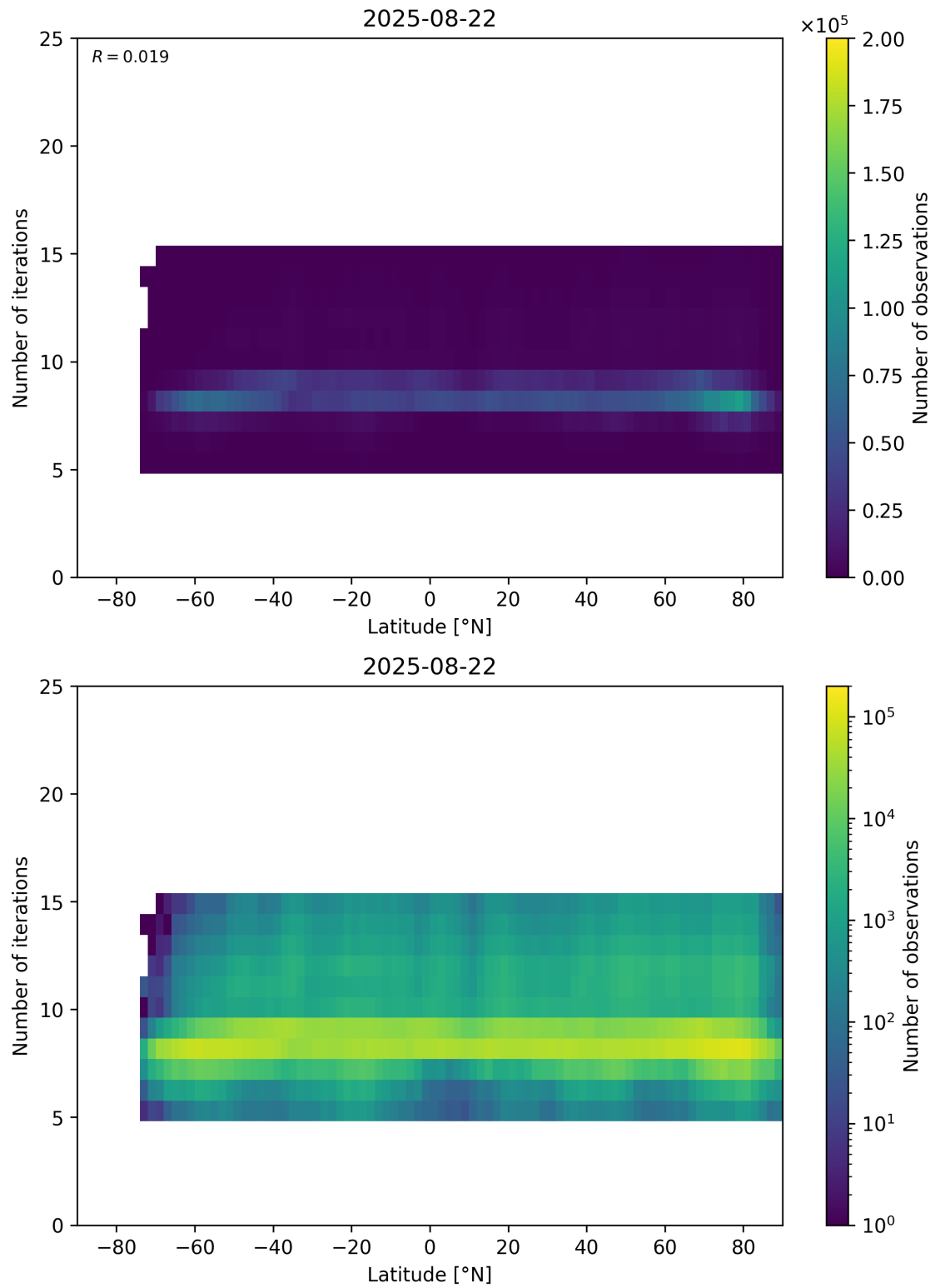
Figure 56: Scatter density plot of “Latitude” against “Number of iterations” for 2025-08-21 to 2025-08-23.
