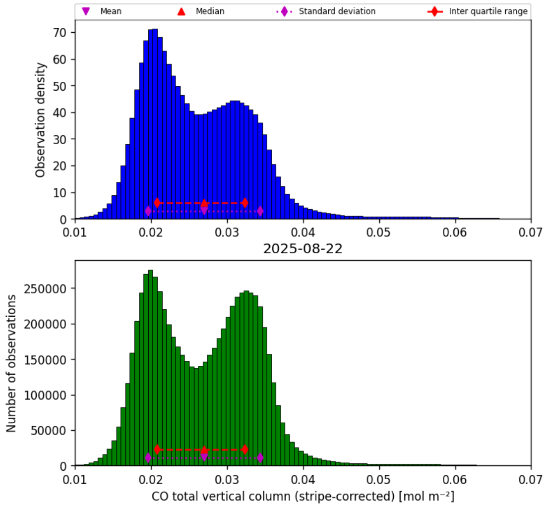
Figure 19: Histogram of “CO total vertical column (stripe-corrected)” for 2025-08-21 to 2025-08-23
