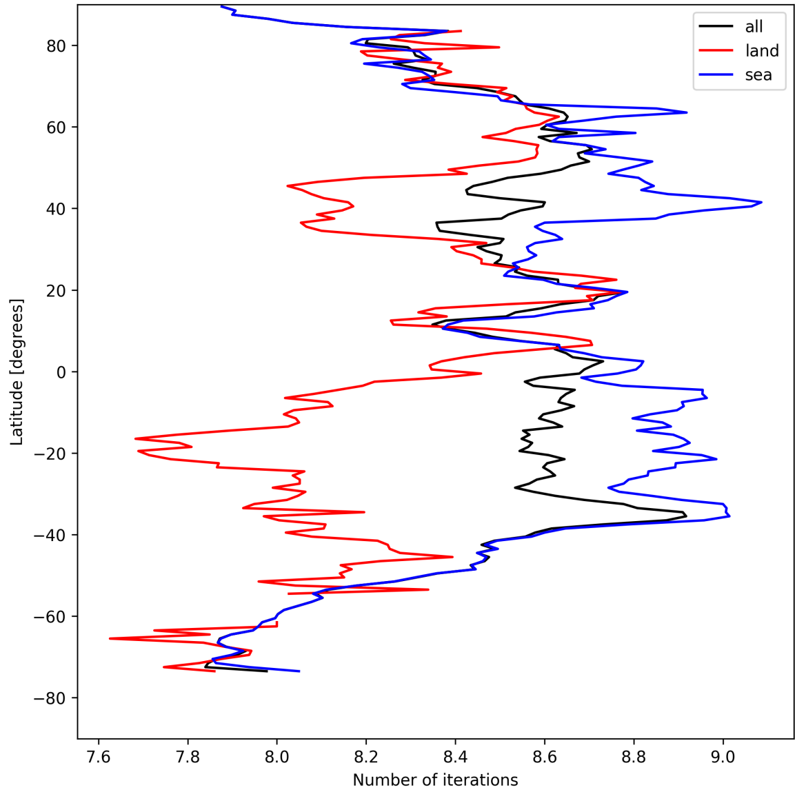
Figure 16: Zonal average of “Number of iterations” for 2025-08-21 to 2025-08-23.
