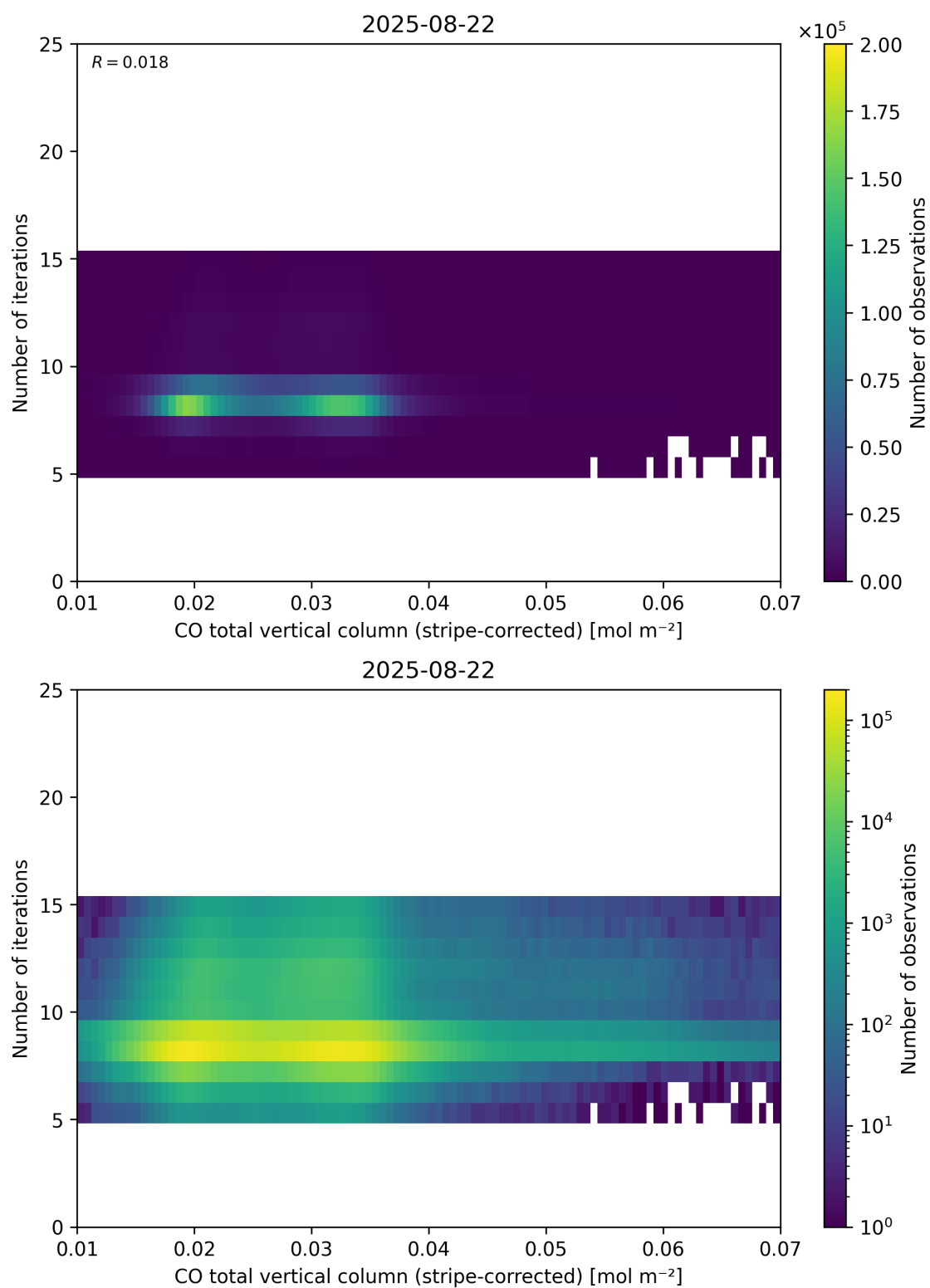
Figure 39: Scatter density plot of “CO total vertical column (stripe-corrected)” against “Number of iterations” for 2025-08-21 to 2025-08-23.
