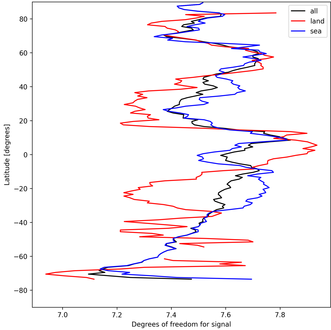
Figure 15: Zonal average of “Degrees of freedom for signal” for 2025-08-21 to 2025-08-23.
