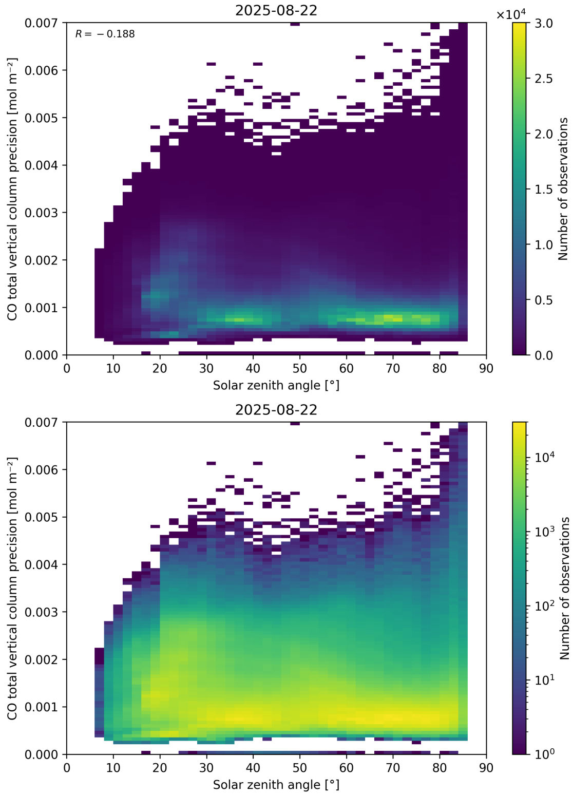
Figure 63: Scatter density plot of “Solar zenith angle” against “CO total vertical column precision” for 2025-08-21 to 2025-08-23.
