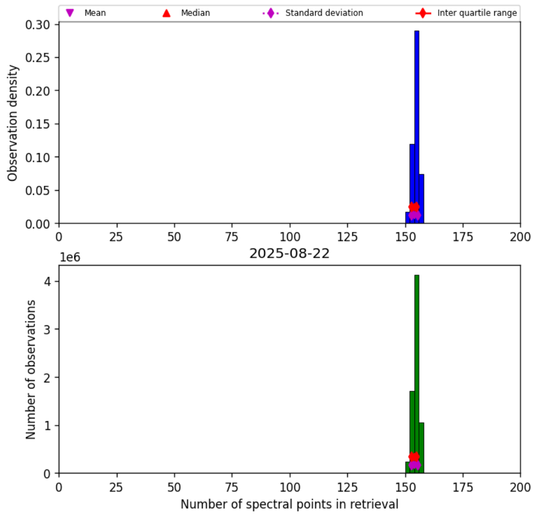
Figure 21: Histogram of “Number of spectral points in retrieval” for 2025-08-21 to 2025-08-23
