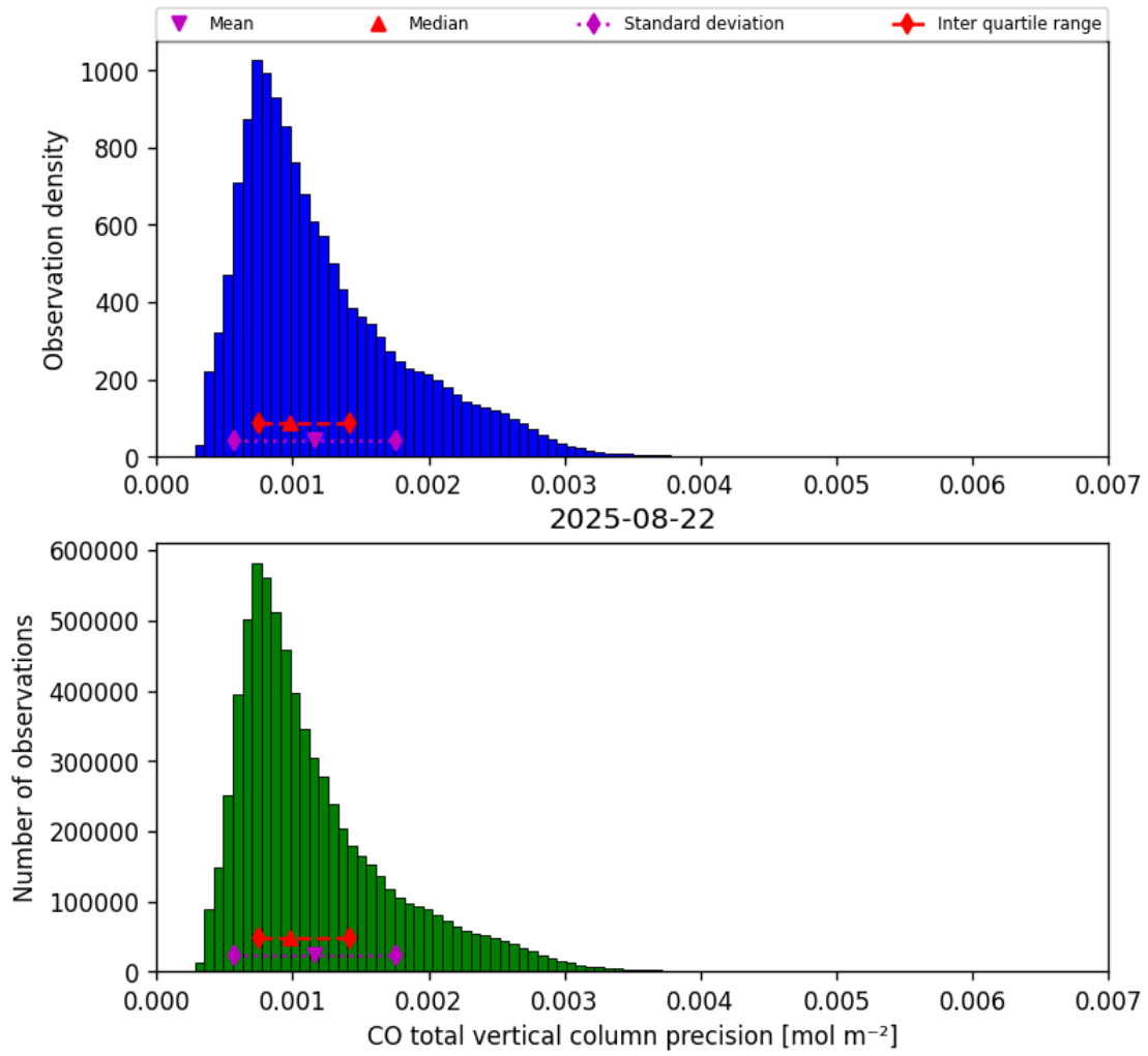
Figure 20: Histogram of “CO total vertical column precision” for 2025-08-21 to 2025-08-23
