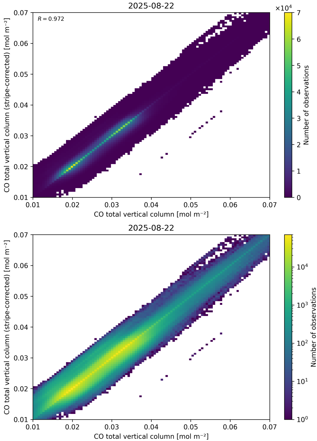
Figure 33: Scatter density plot of “CO total vertical column” against “CO total vertical column (stripe-corrected)” for 2025-08-21 to 2025-08-23.
