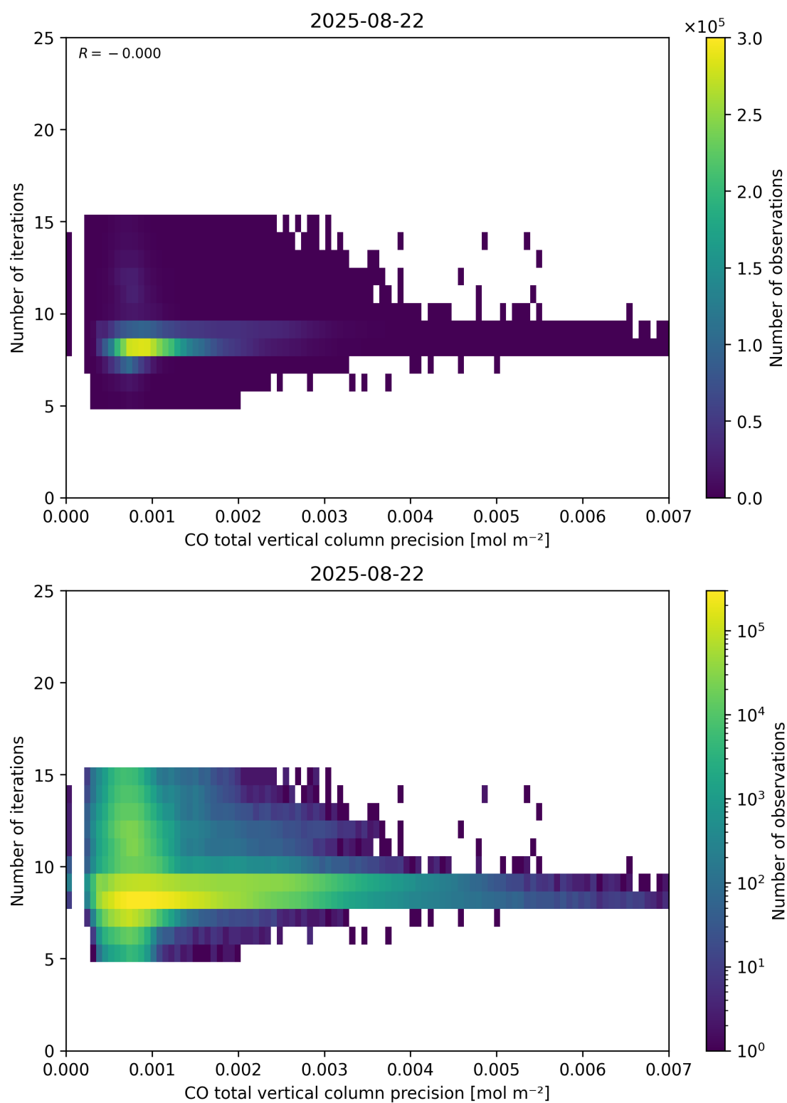
Figure 46: Scatter density plot of “CO total vertical column precision” against “Number of iterations” for 2025-08-21 to 2025-08-23.
