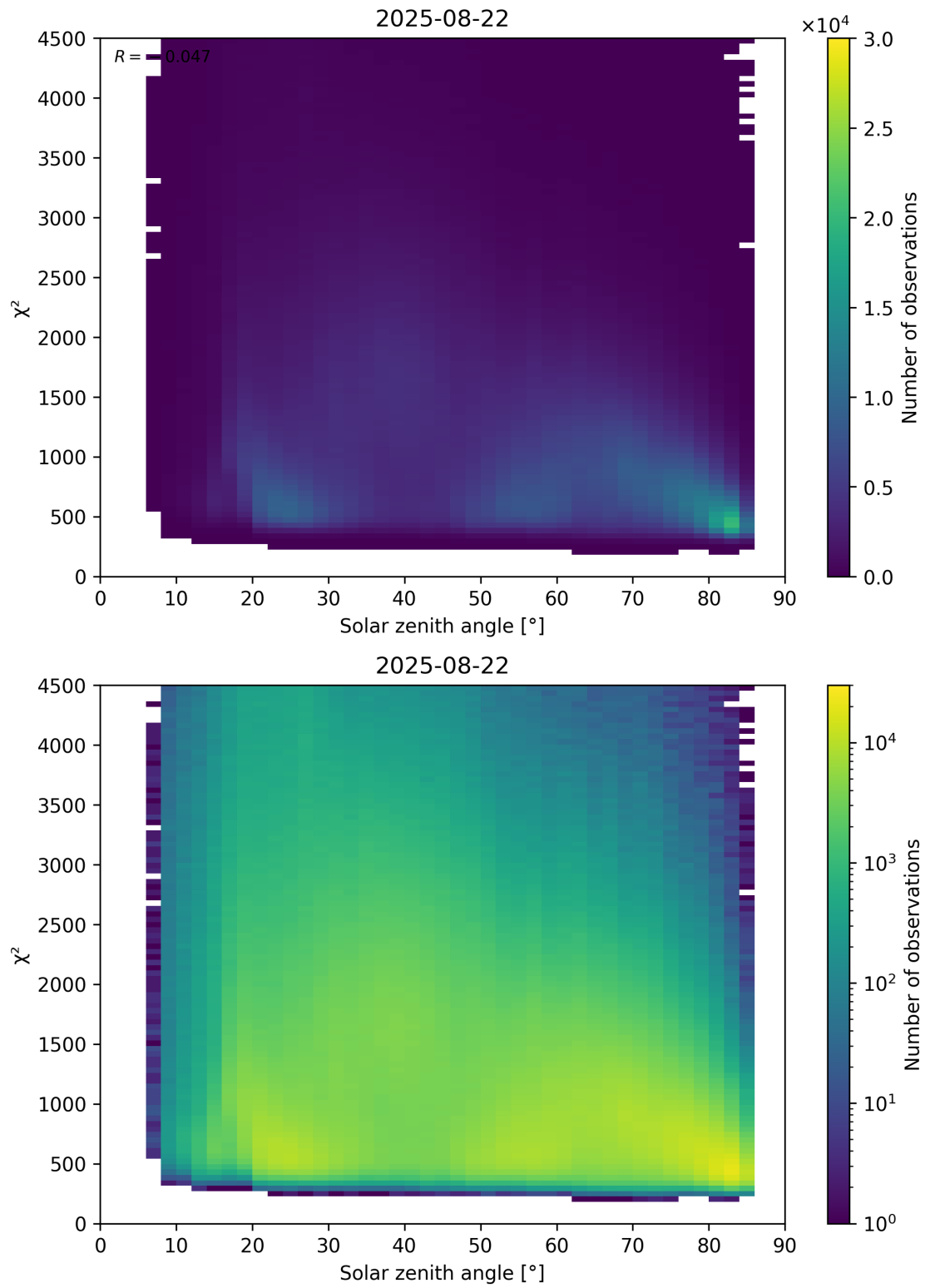
Figure 64: Scatter density plot of “Solar zenith angle” against “ \chi^2 ” for 2025-08-21 to 2025-08-23.
