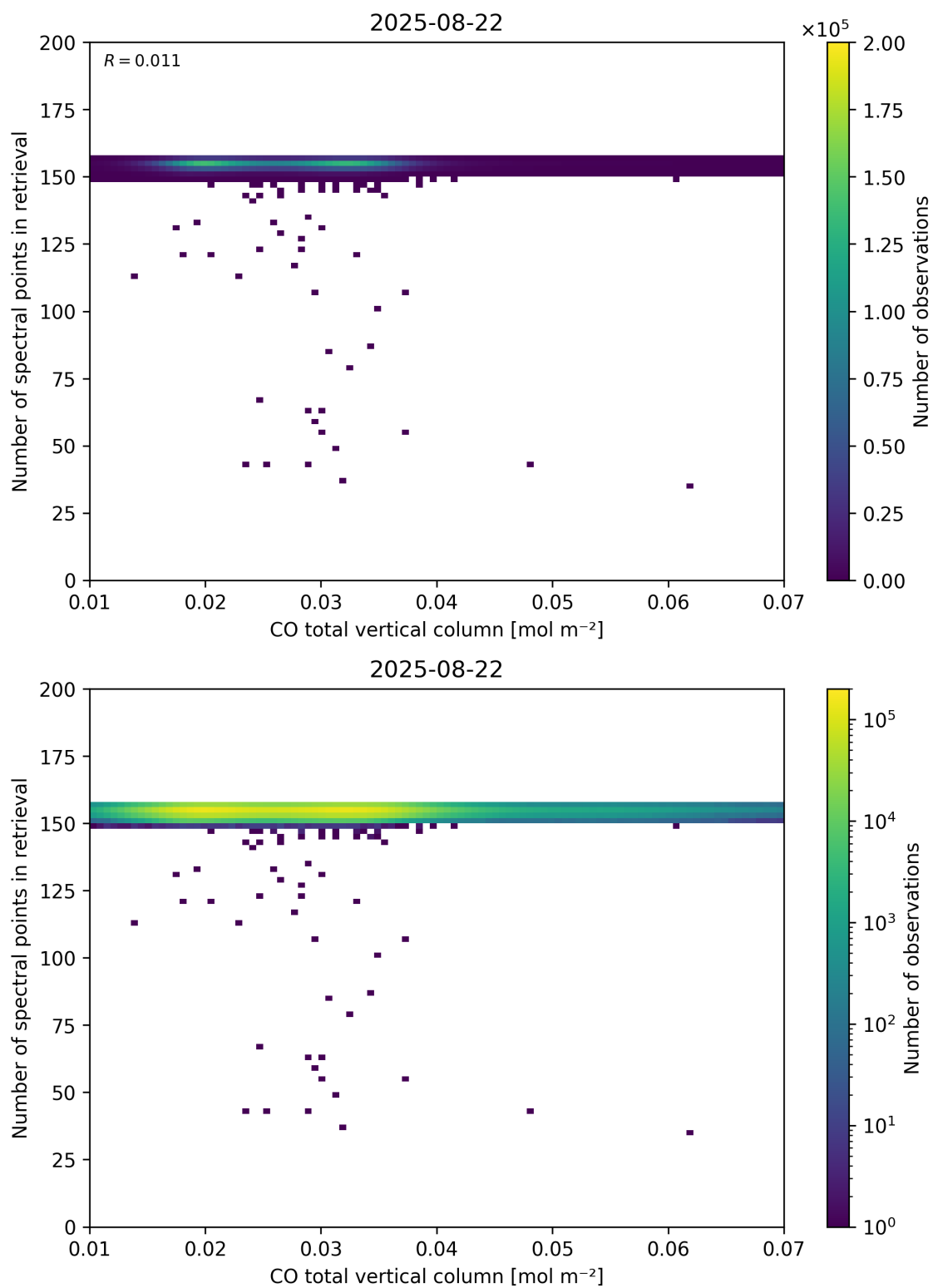
Figure 43: Scatter density plot of “CO total vertical column” against “Number of spectral points in retrieval” for 2025-08-21 to 2025-08-23.
