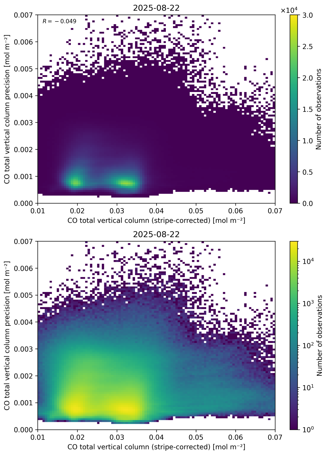
Figure 36: Scatter density plot of “CO total vertical column (stripe-corrected)” against “CO total vertical column precision” for 2025-08-21 to 2025-08-23.
