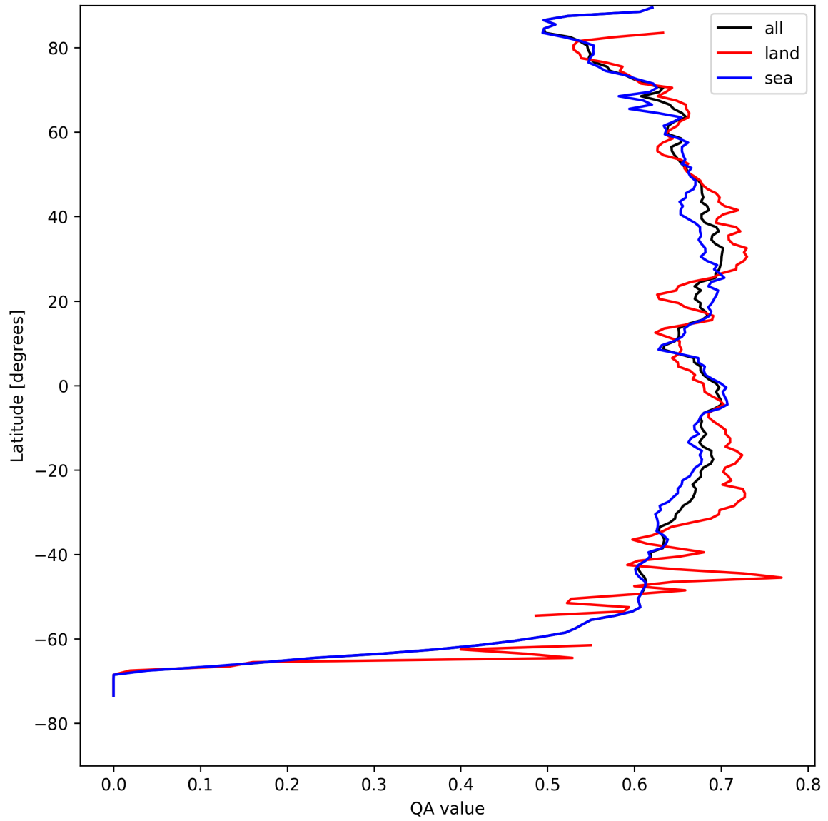
Figure 9: Zonal average of “QA value” for 2025-08-21 to 2025-08-23.
