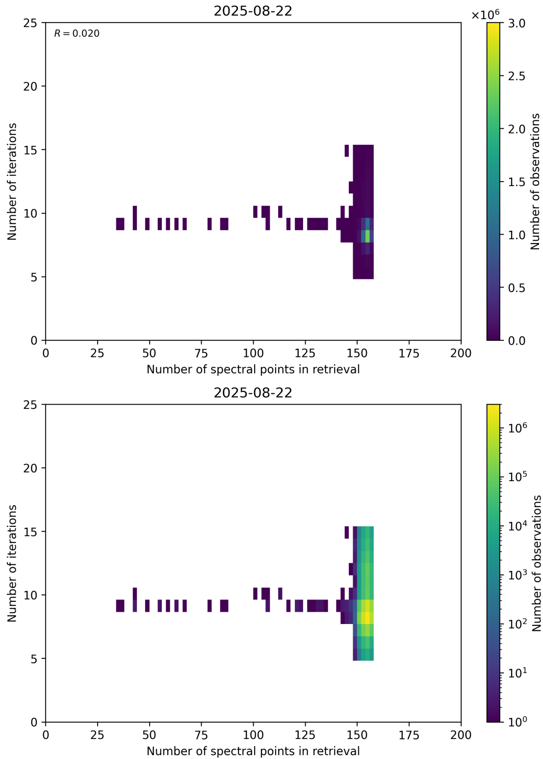
Figure 60: Scatter density plot of “Number of spectral points in retrieval” against “Number of iterations” for 2025-08-21 to 2025-08-23.
