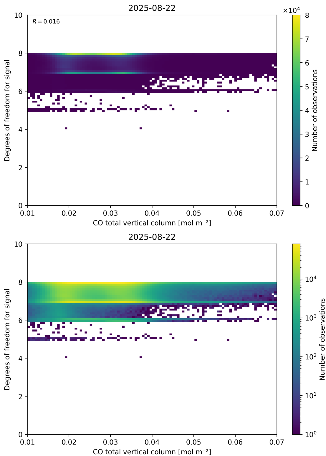
Figure 41: Scatter density plot of “CO total vertical column” against “Degrees of freedom for signal” for 2025-08-21 to 2025-08-23.
