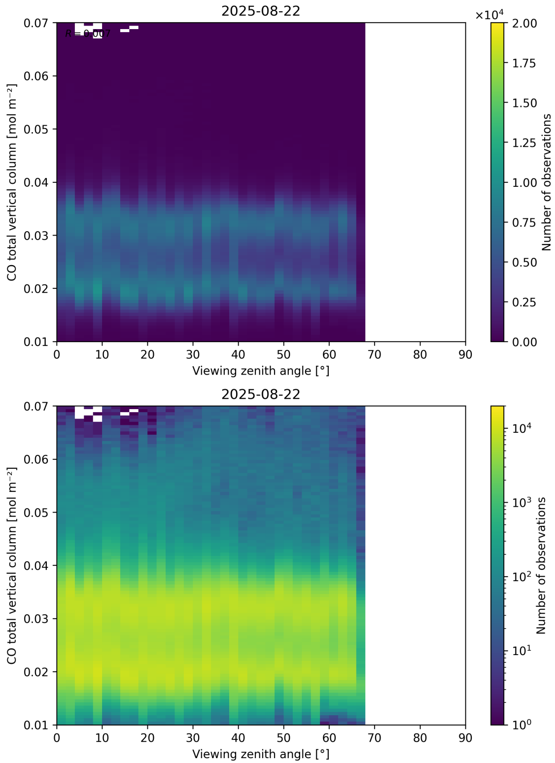
Figure 69: Scatter density plot of “Viewing zenith angle” against “CO total vertical column” for 2025-08-21 to 2025-08-23.
