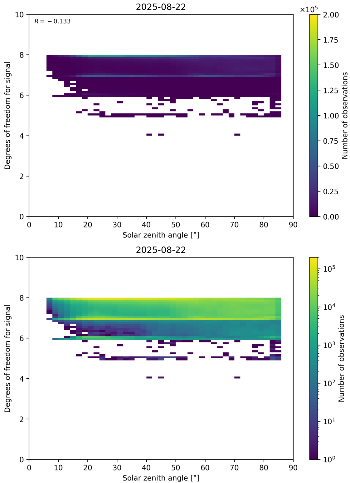
Figure 65: Scatter density plot of “Solar zenith angle” against “Degrees of freedom for signal” for 2025-08-21 to 2025-08-23.
