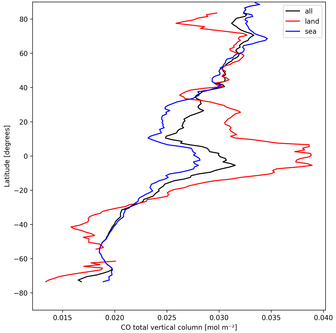
Figure 10: Zonal average of “CO total vertical column” for 2025-08-21 to 2025-08-23.
