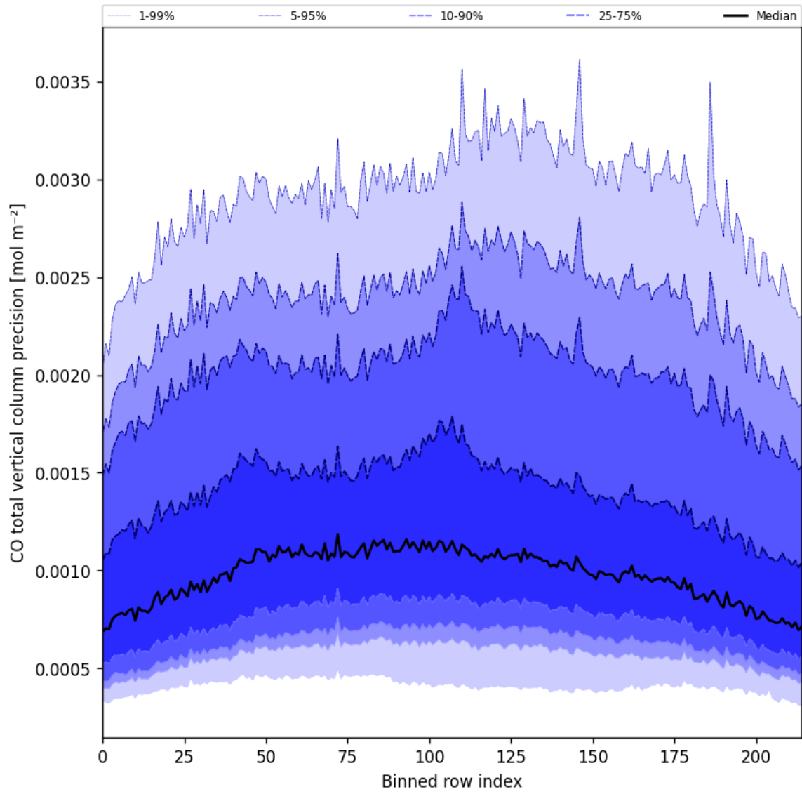
Figure 28: Along track statistics of “CO total vertical column precision” for 2025-08-21 to 2025-08-23
