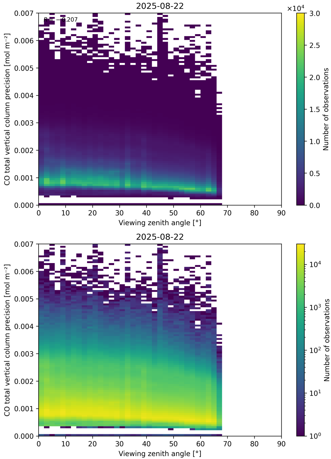
Figure 71: Scatter density plot of “Viewing zenith angle” against “CO total vertical column precision” for 2025-08-21 to 2025-08-23.
