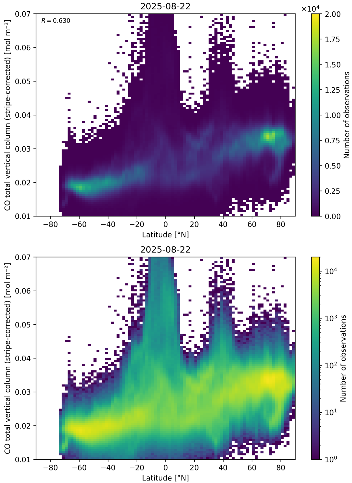
Figure 52: Scatter density plot of “Latitude” against “CO total vertical column (stripe-corrected)” for 2025-08-21 to 2025-08-23.
