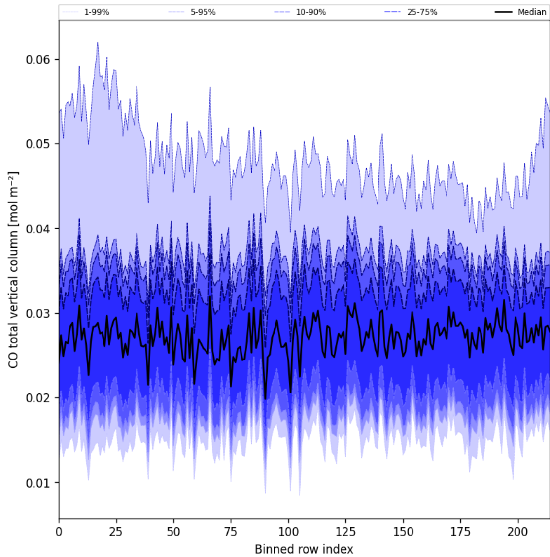
Figure 26: Along track statistics of “CO total vertical column” for 2025-08-21 to 2025-08-23
