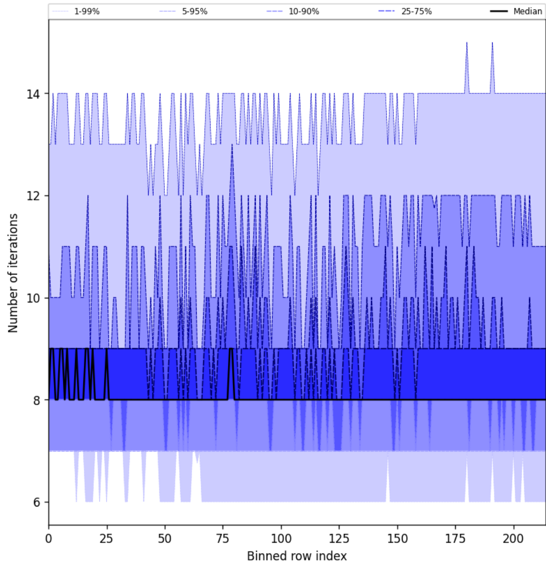
Figure 32: Along track statistics of “Number of iterations” for 2025-08-21 to 2025-08-23
