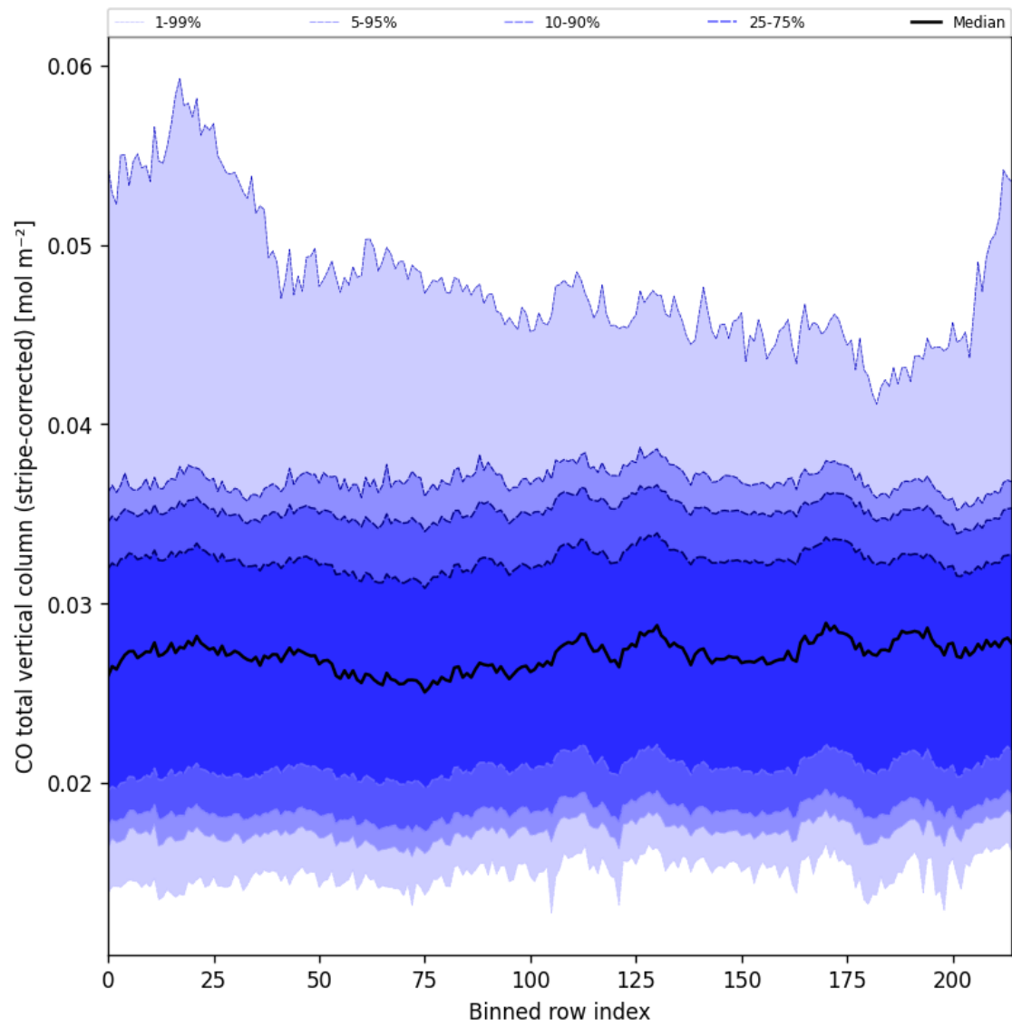
Figure 27: Along track statistics of “CO total vertical column (stripe-corrected)” for 2025-08-21 to 2025-08-23
