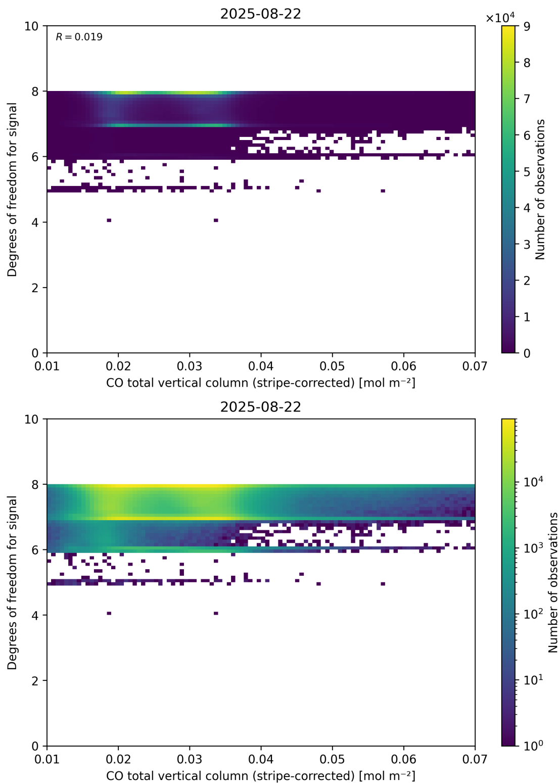
Figure 38: Scatter density plot of “CO total vertical column (stripe-corrected)” against “Degrees of freedom for signal” for 2025-08-21 to 2025-08-23.
