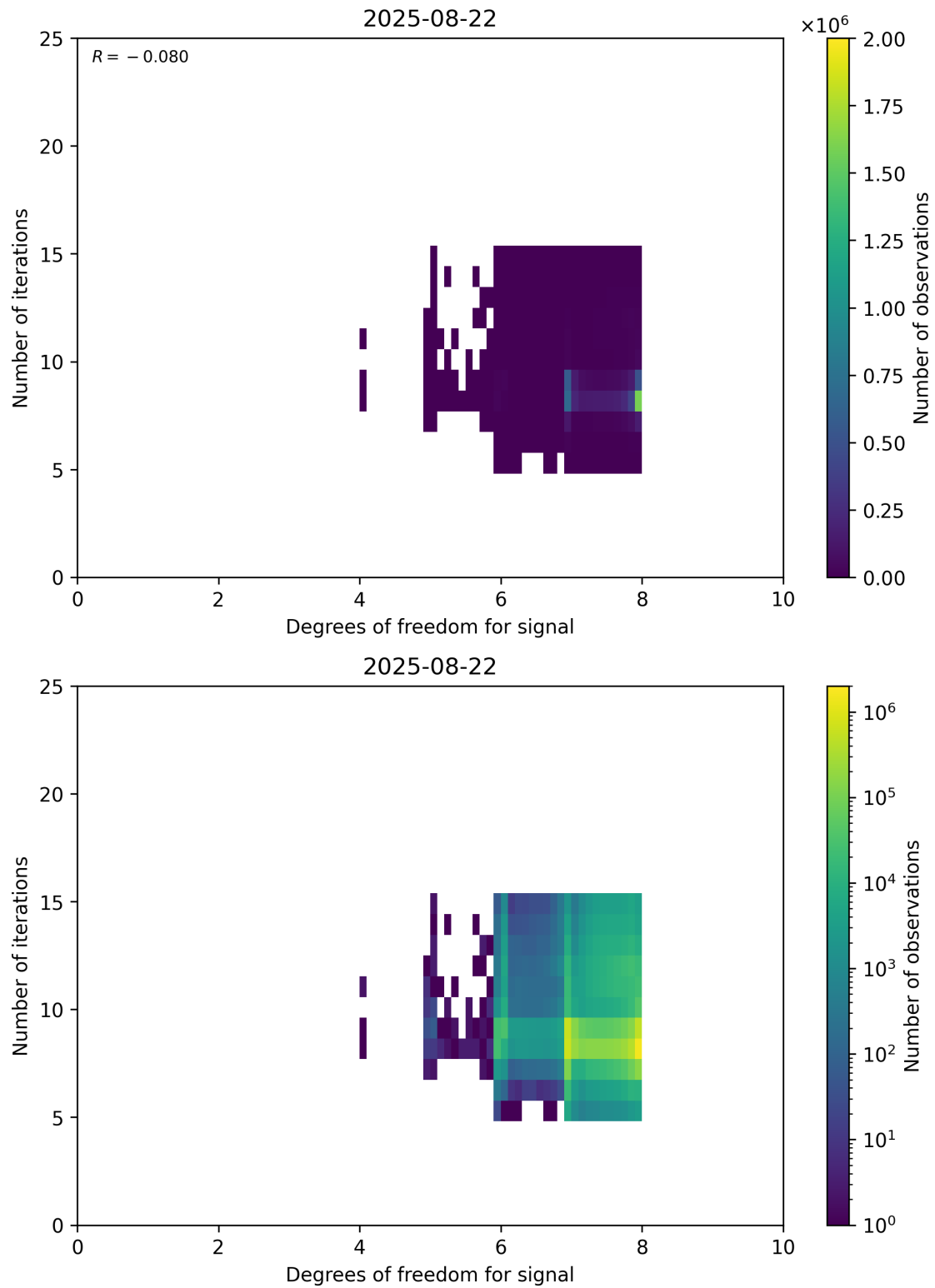
Figure 50: Scatter density plot of “Degrees of freedom for signal” against “Number of iterations” for 2025-08-21 to 2025-08-23.
