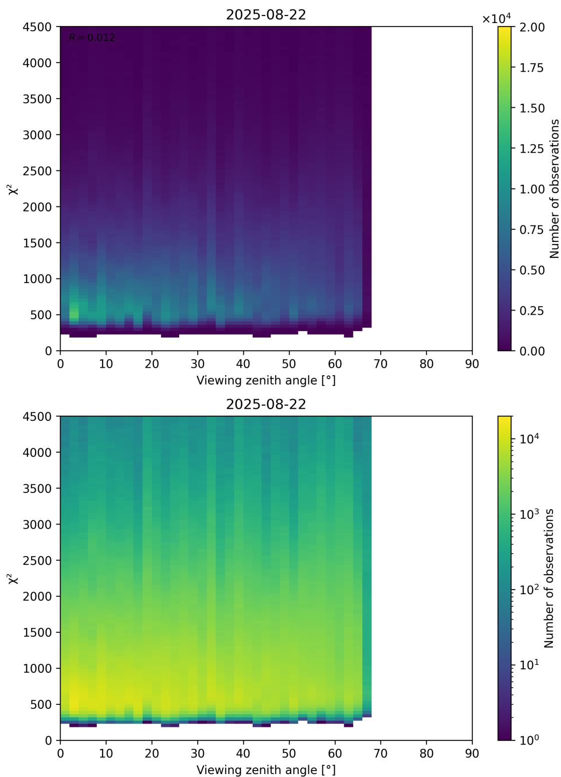
Figure 72: Scatter density plot of “Viewing zenith angle” against “ \chi^2 ” for 2025-08-21 to 2025-08-23.
