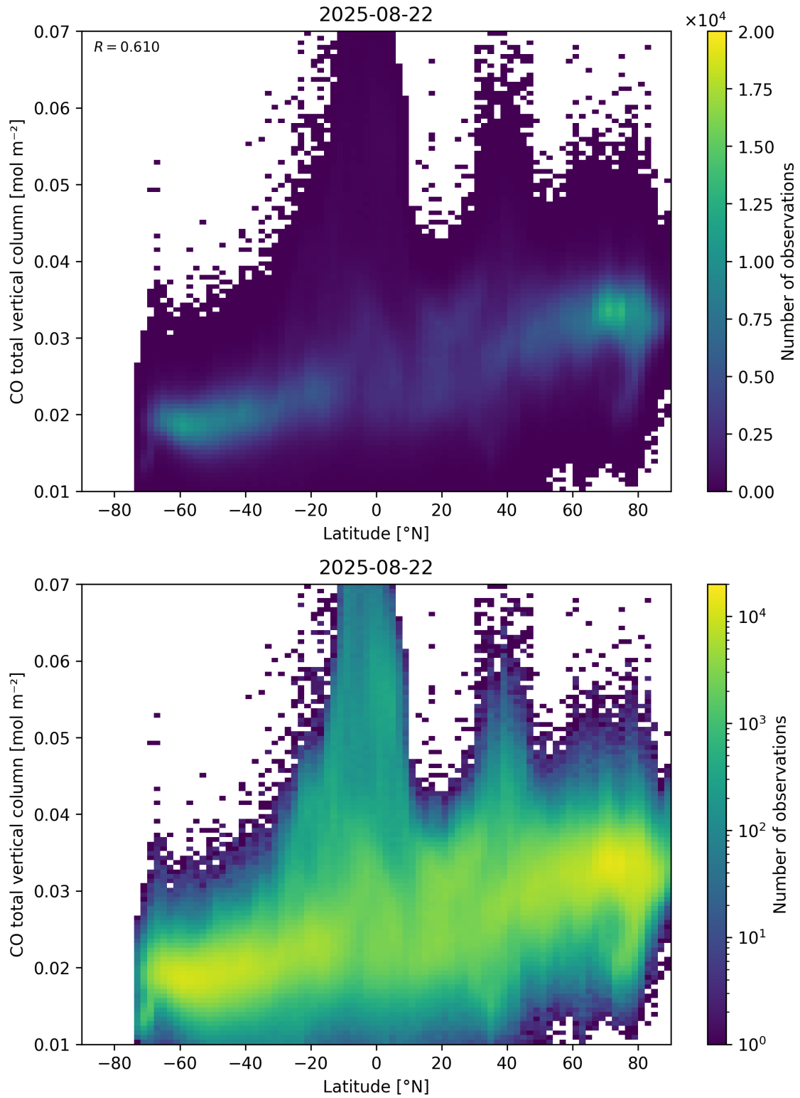
Figure 51: Scatter density plot of “Latitude” against “CO total vertical column” for 2025-08-21 to 2025-08-23.
