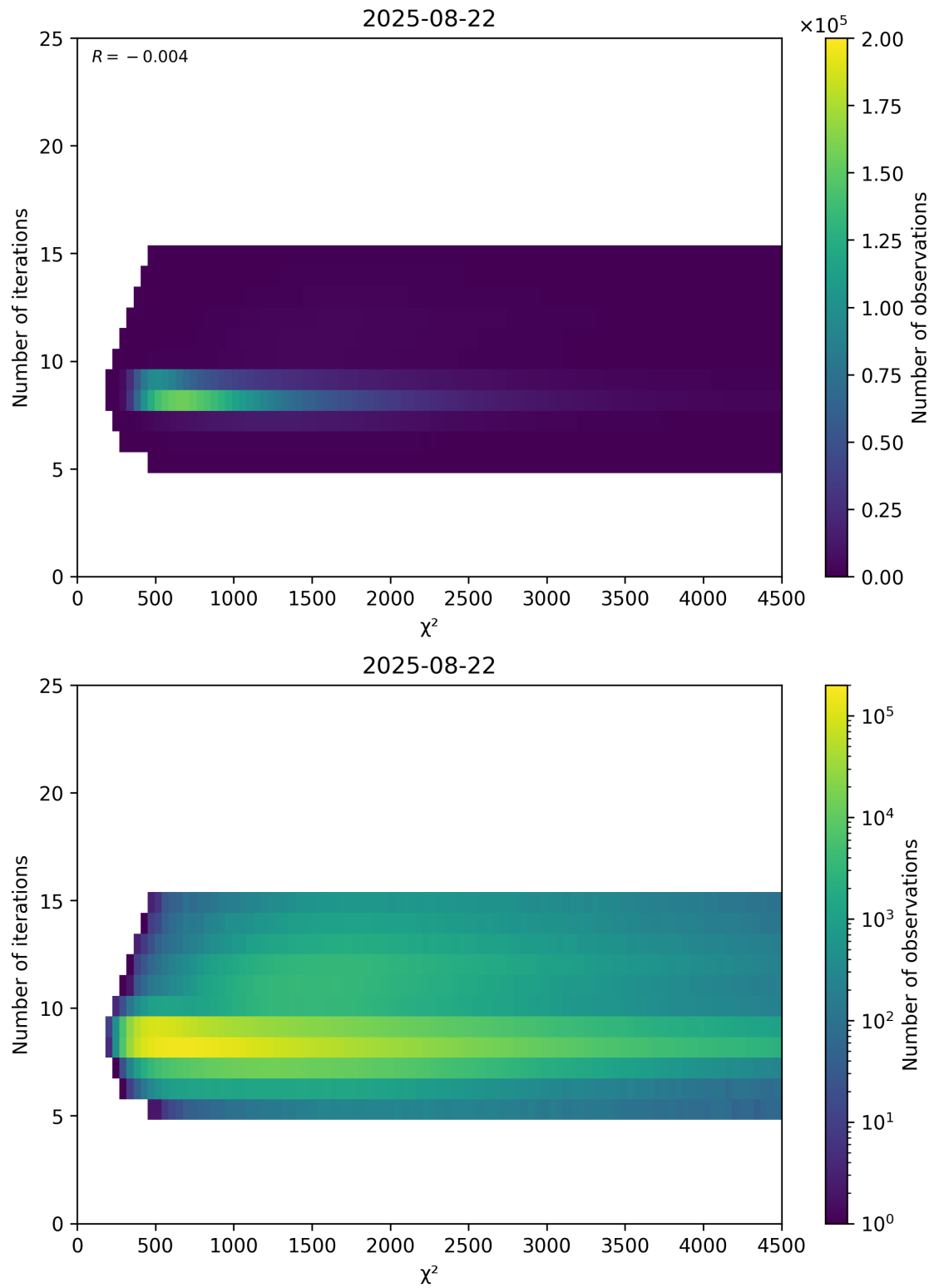
Figure 49: Scatter density plot of “ \chi^2 ” against “Number of iterations” for 2025-08-21 to 2025-08-23.
