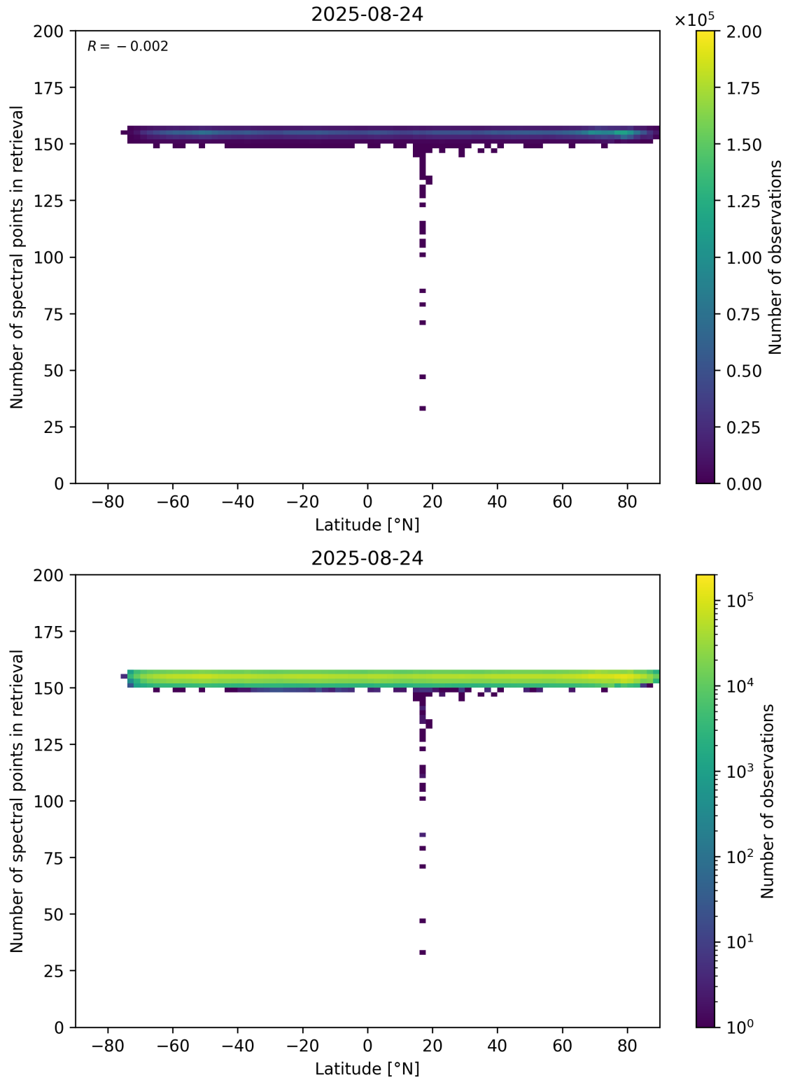
Figure 57: Scatter density plot of “Latitude” against “Number of spectral points in retrieval” for 2025-08-23 to 2025-08-25.
