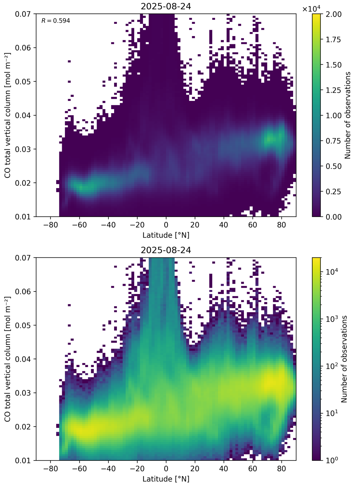
Figure 51: Scatter density plot of “Latitude” against “CO total vertical column” for 2025-08-23 to 2025-08-25.
