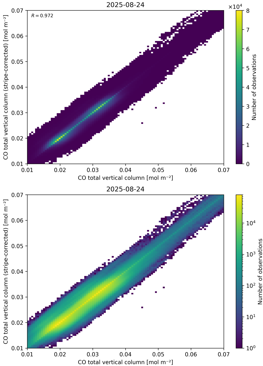
Figure 33: Scatter density plot of “CO total vertical column” against “CO total vertical column (stripe-corrected)” for 2025-08-23 to 2025-08-25.
