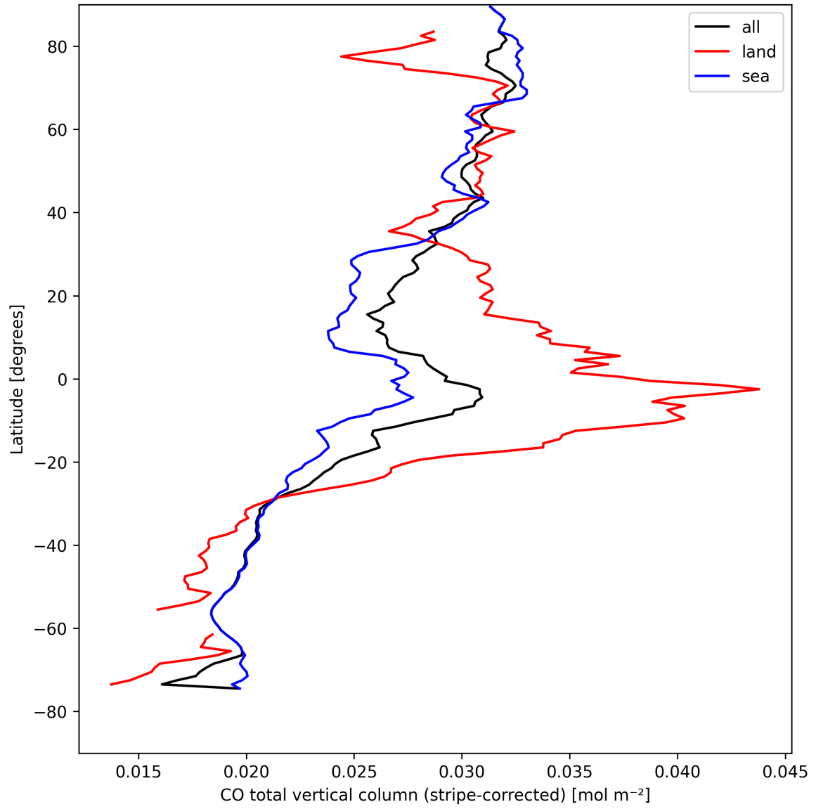
Figure 11: Zonal average of “CO total vertical column (stripe-corrected)” for 2025-08-23 to 2025-08-25.
