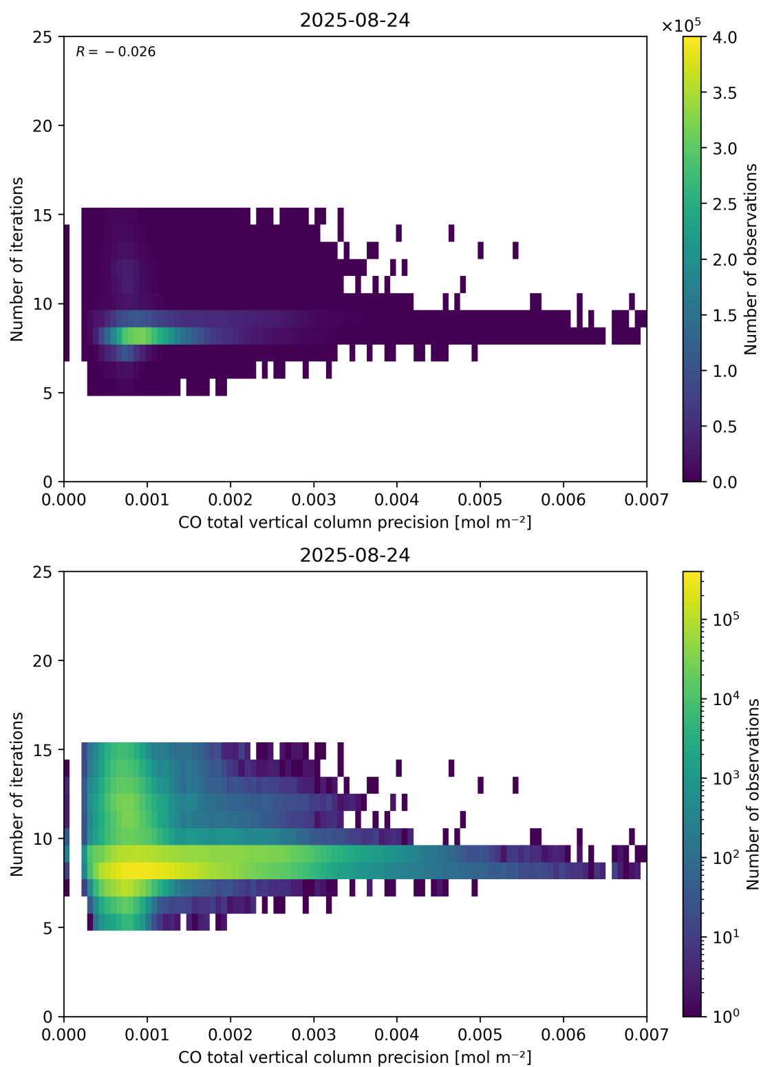
Figure 46: Scatter density plot of “CO total vertical column precision” against “Number of iterations” for 2025-08-23 to 2025-08-25.
