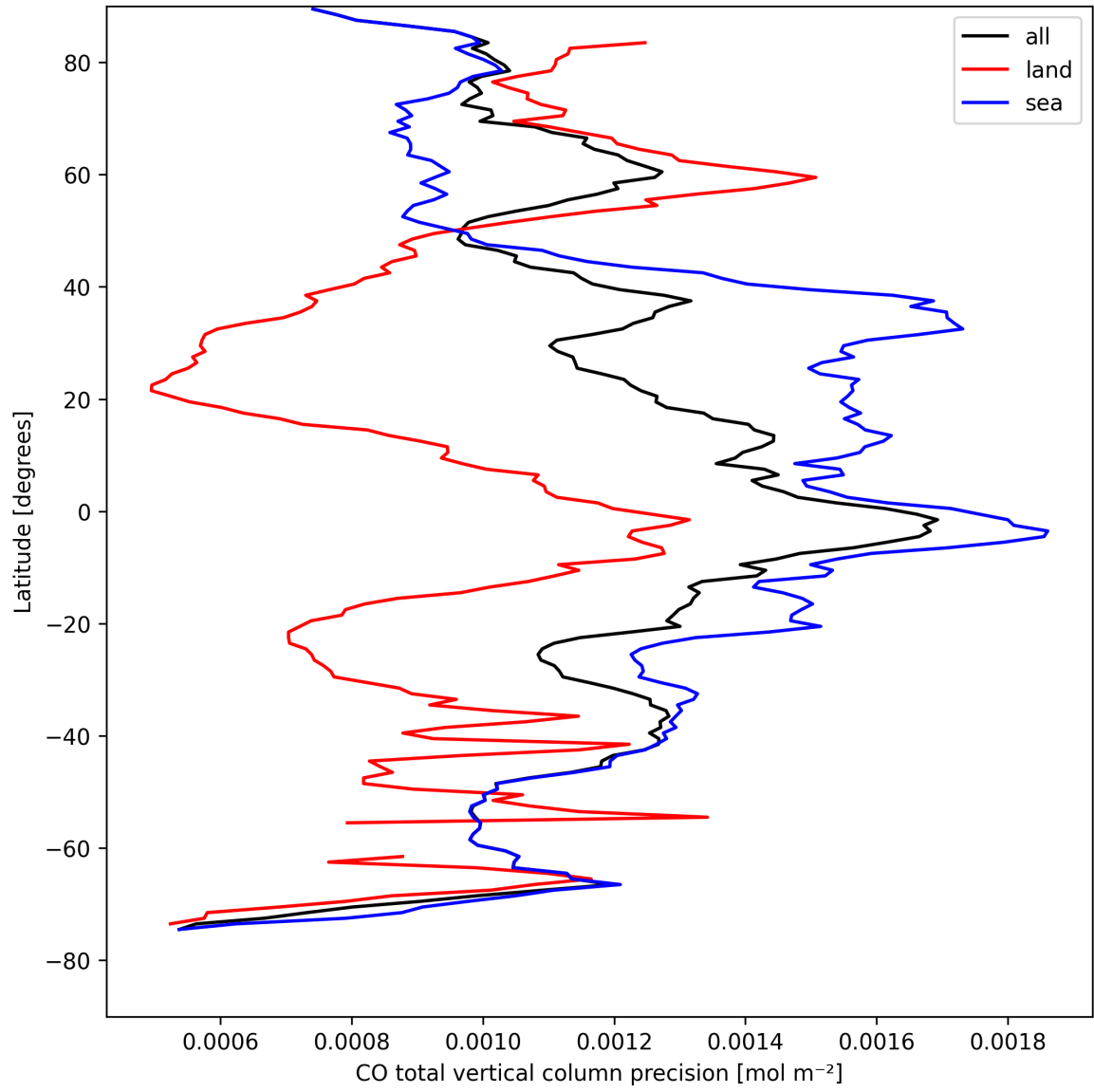
Figure 12: Zonal average of “CO total vertical column precision” for 2025-08-23 to 2025-08-25.
