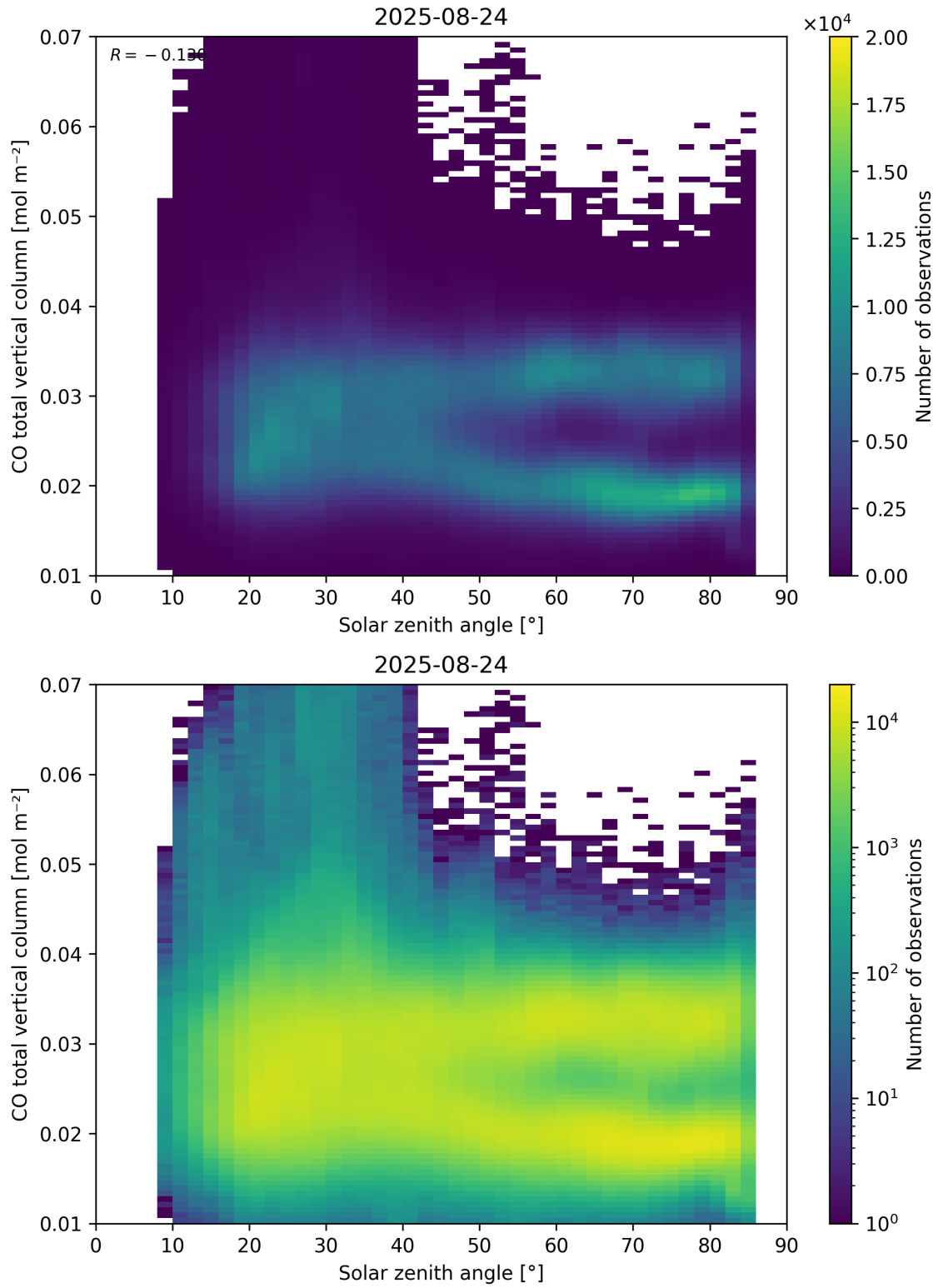
Figure 61: Scatter density plot of “Solar zenith angle” against “CO total vertical column” for 2025-08-23 to 2025-08-25.
