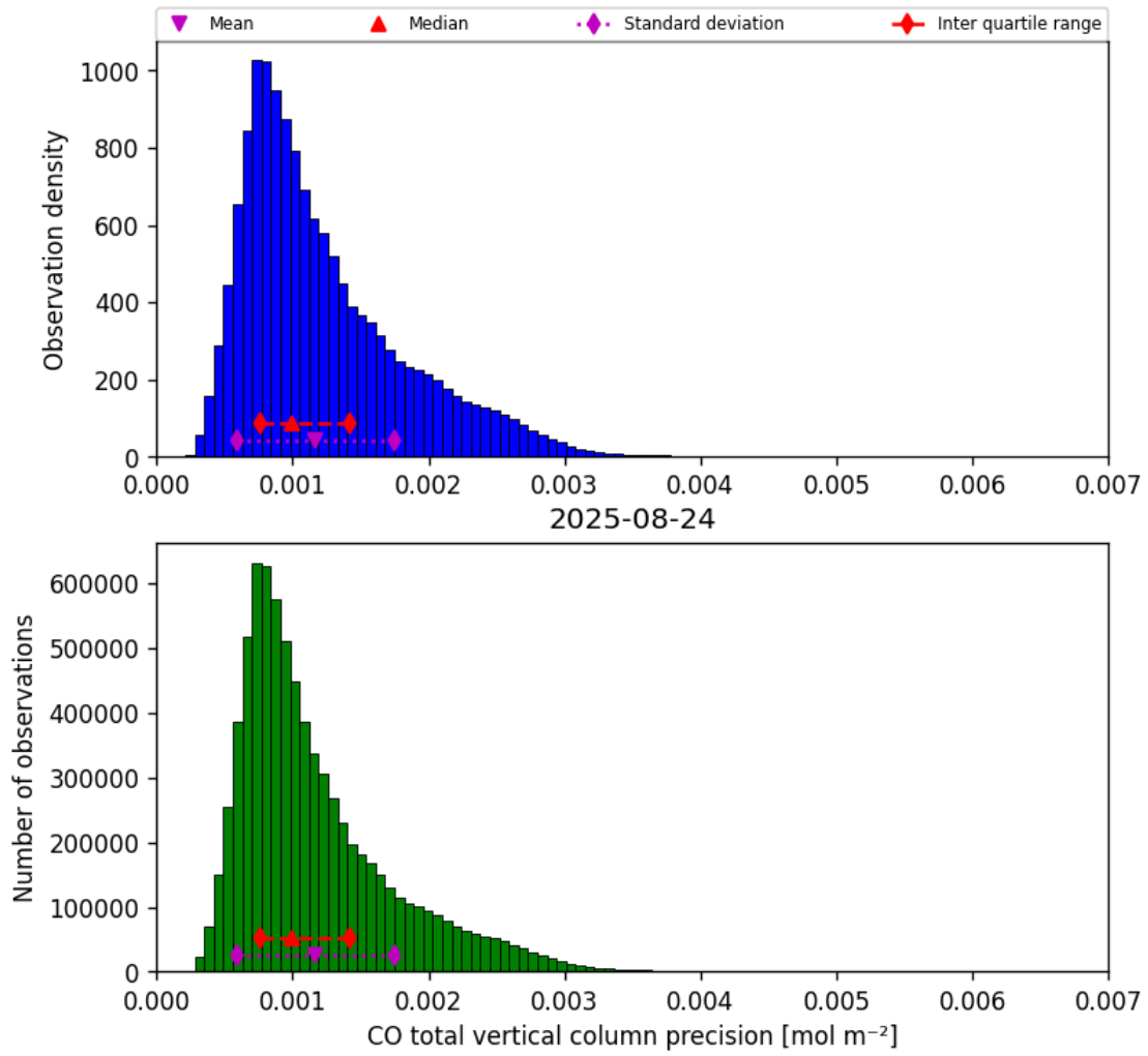
Figure 20: Histogram of “CO total vertical column precision” for 2025-08-23 to 2025-08-25
