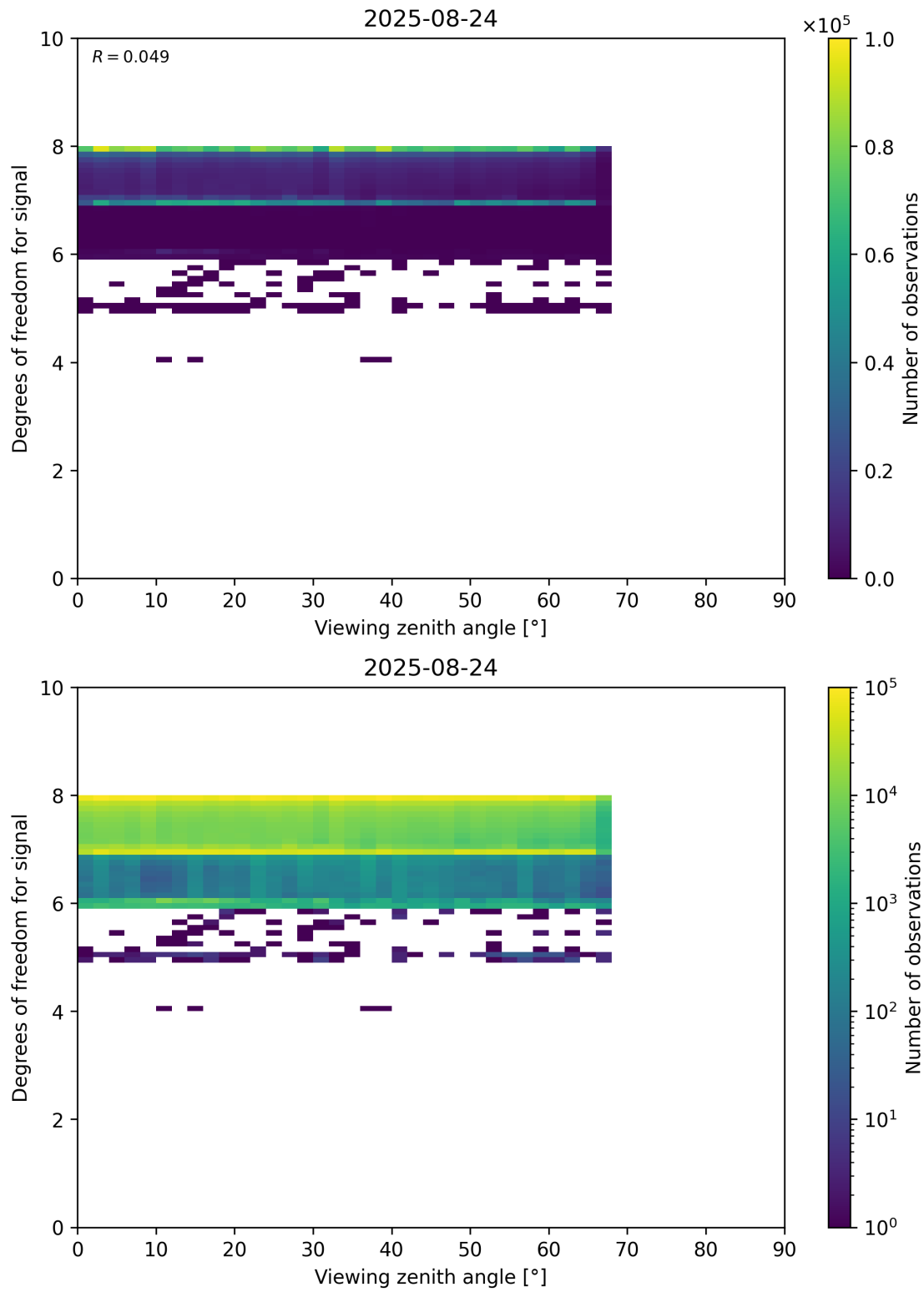
Figure 73: Scatter density plot of “Viewing zenith angle” against “Degrees of freedom for signal” for 2025-08-23 to 2025-08-25.
