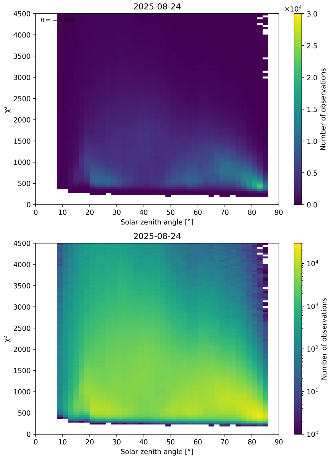
Figure 64: Scatter density plot of “Solar zenith angle” against “ \chi^2 ” for 2025-08-23 to 2025-08-25.
