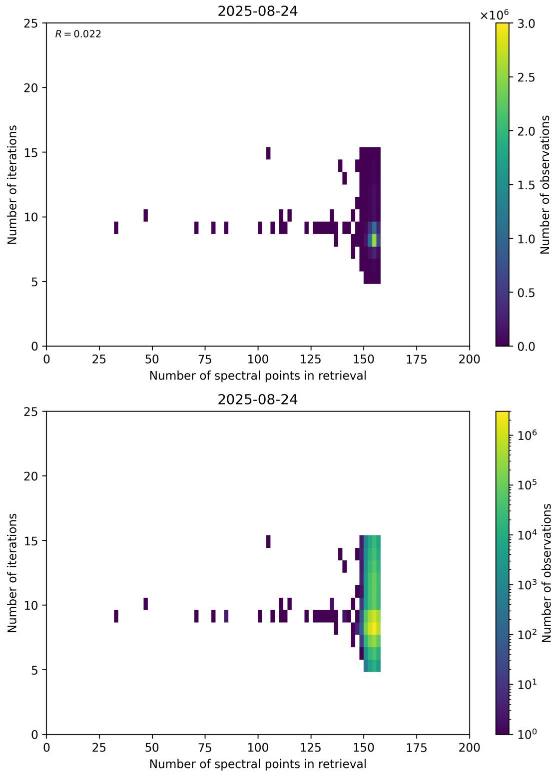
Figure 60: Scatter density plot of “Number of spectral points in retrieval” against “Number of iterations” for 2025-08-23 to 2025-08-25.
