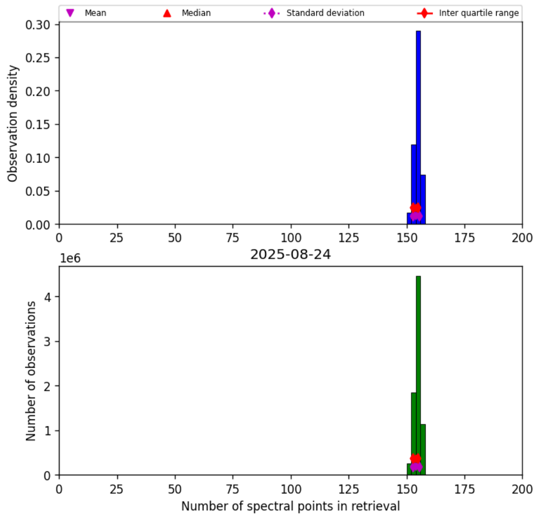
Figure 21: Histogram of “Number of spectral points in retrieval” for 2025-08-23 to 2025-08-25
