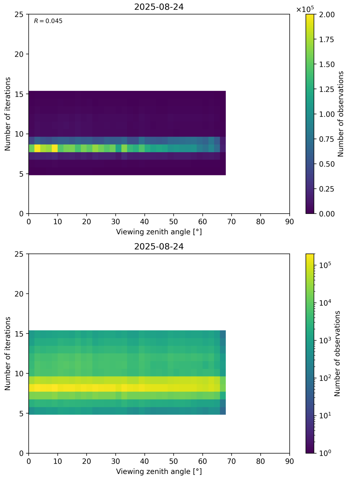
Figure 75: Scatter density plot of “Viewing zenith angle” against “Number of iterations” for 2025-08-23 to 2025-08-25.
