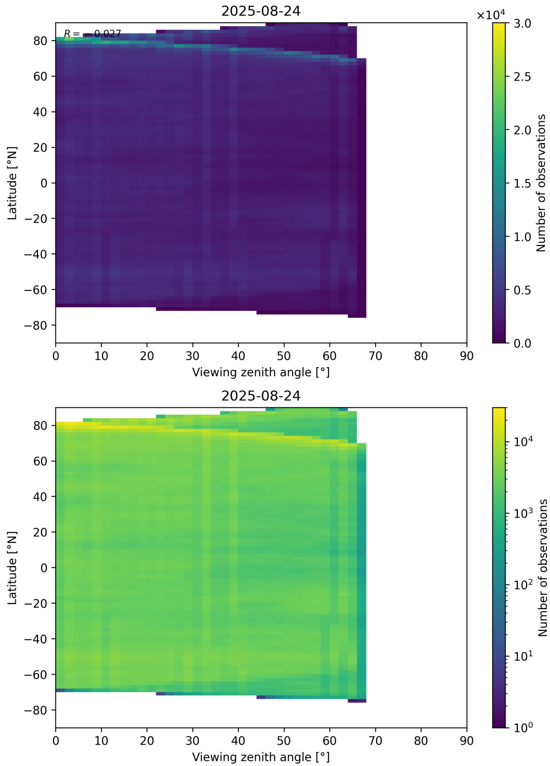
Figure 74: Scatter density plot of “Viewing zenith angle” against “Latitude” for 2025-08-23 to 2025-08-25.
