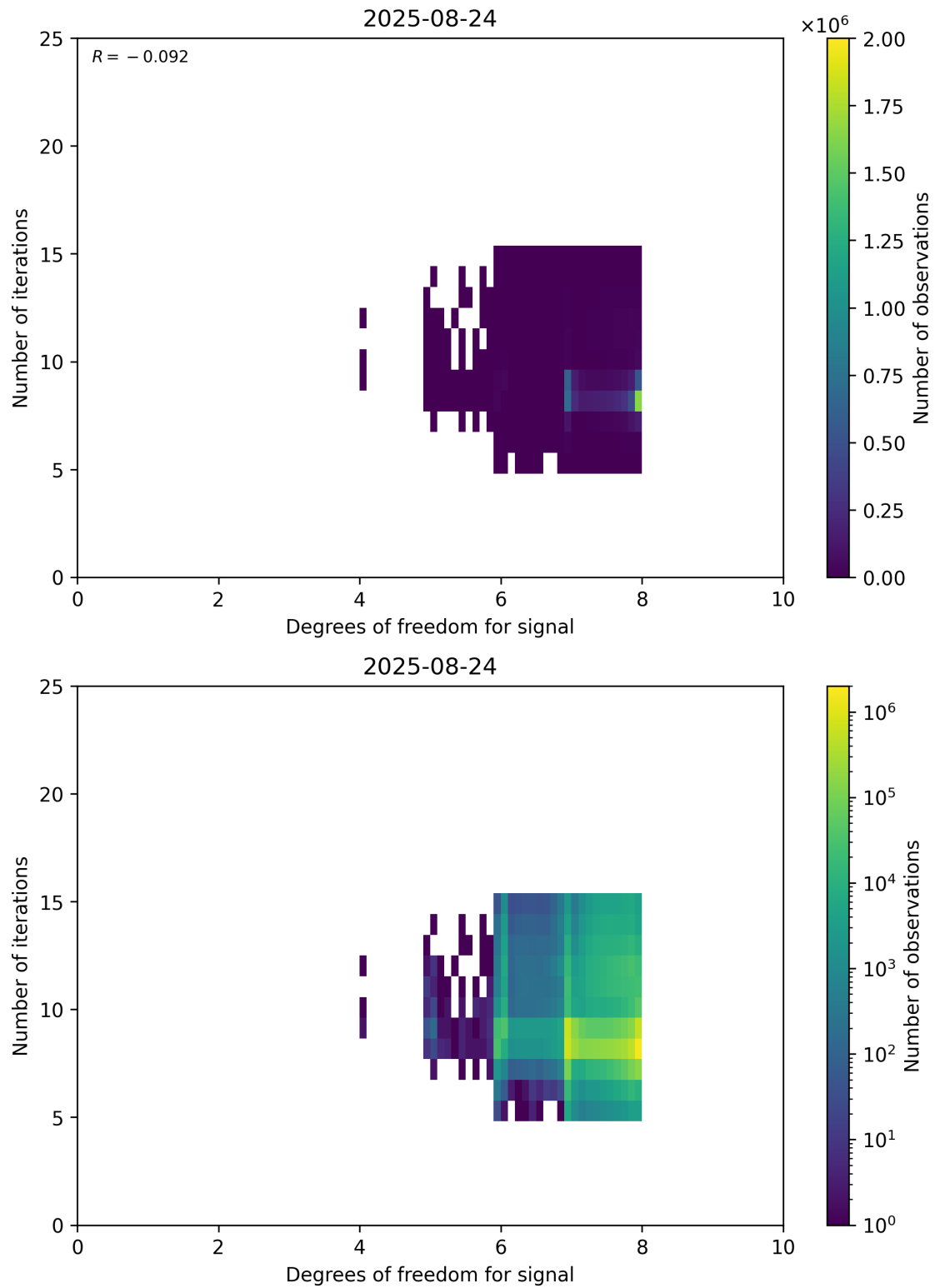
Figure 50: Scatter density plot of “Degrees of freedom for signal” against “Number of iterations” for 2025-08-23 to 2025-08-25.
