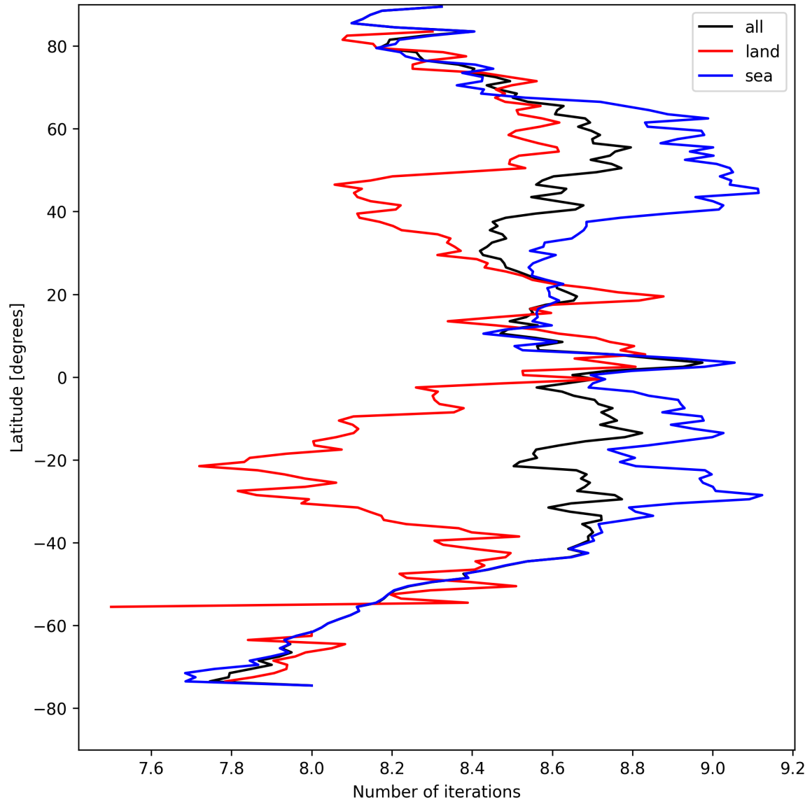
Figure 16: Zonal average of “Number of iterations” for 2025-08-23 to 2025-08-25.
