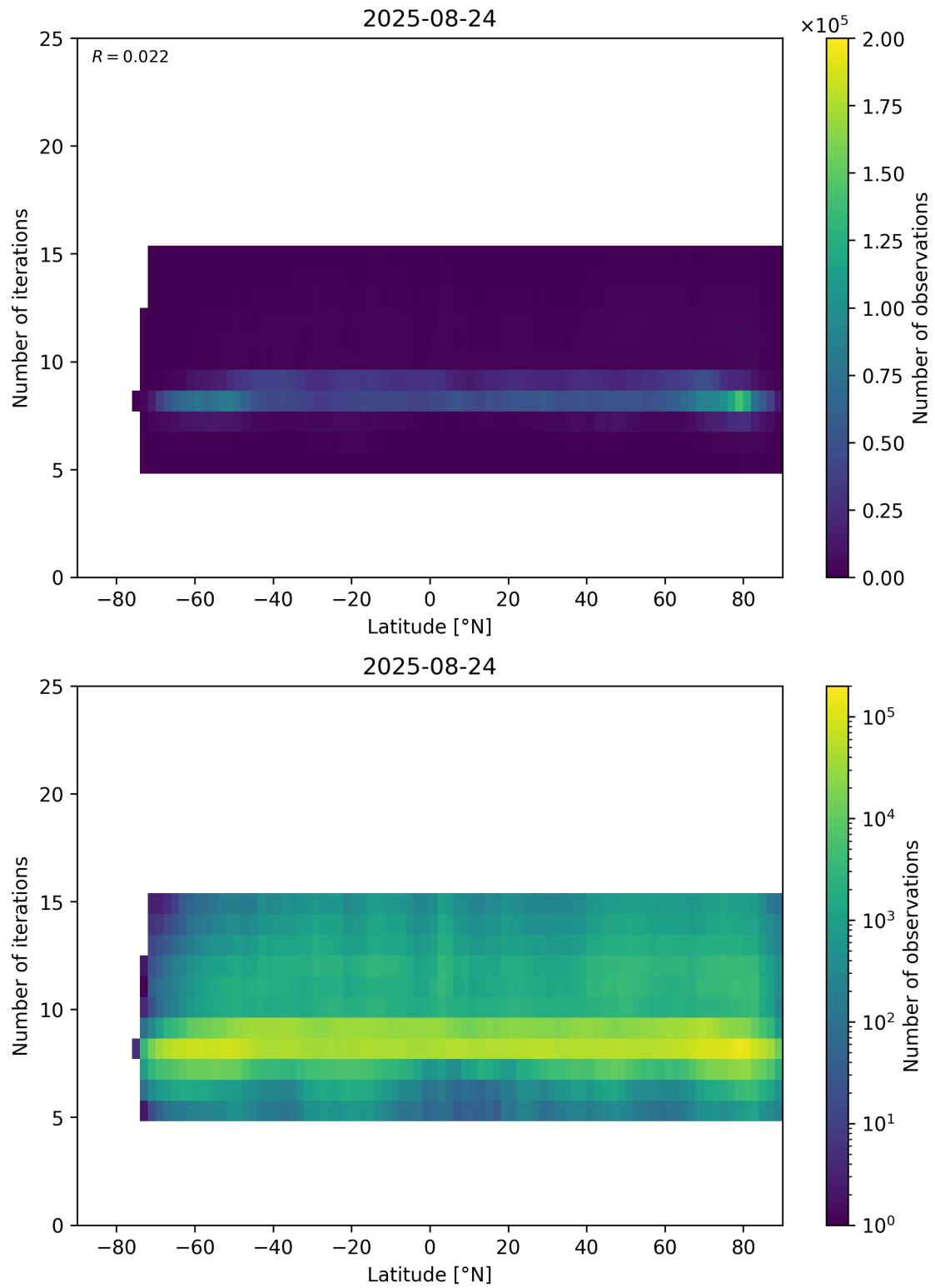
Figure 56: Scatter density plot of “Latitude” against “Number of iterations” for 2025-08-23 to 2025-08-25.
