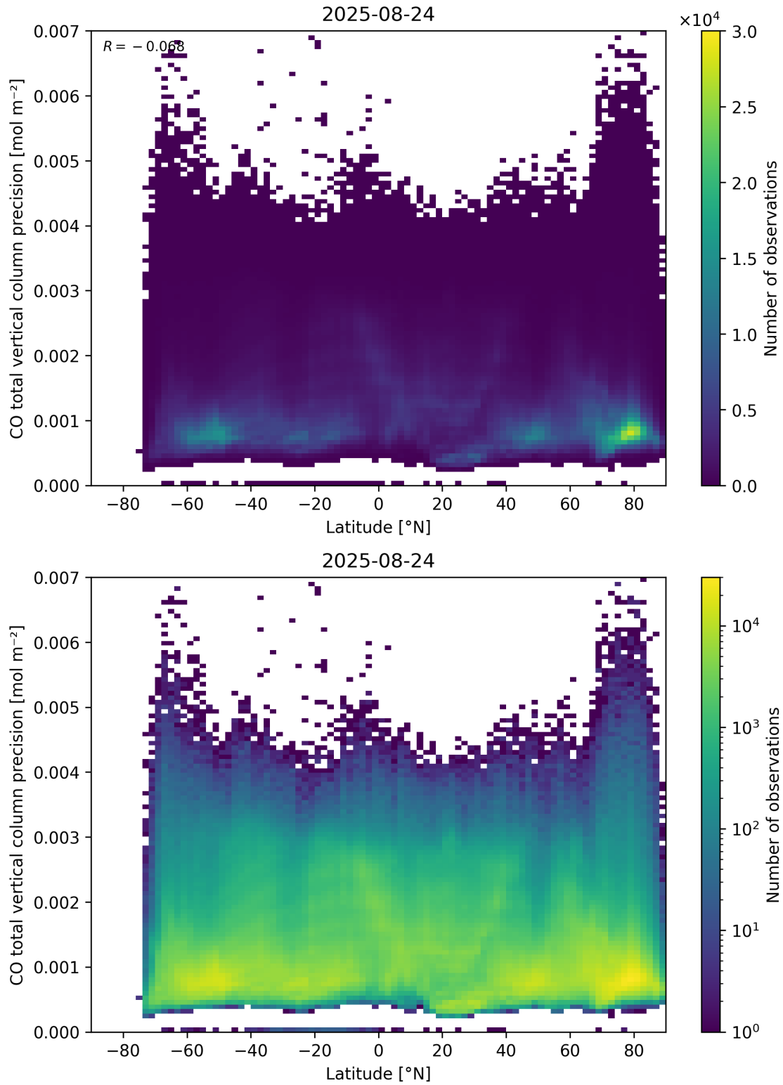
Figure 53: Scatter density plot of “Latitude” against “CO total vertical column precision” for 2025-08-23 to 2025-08-25.
