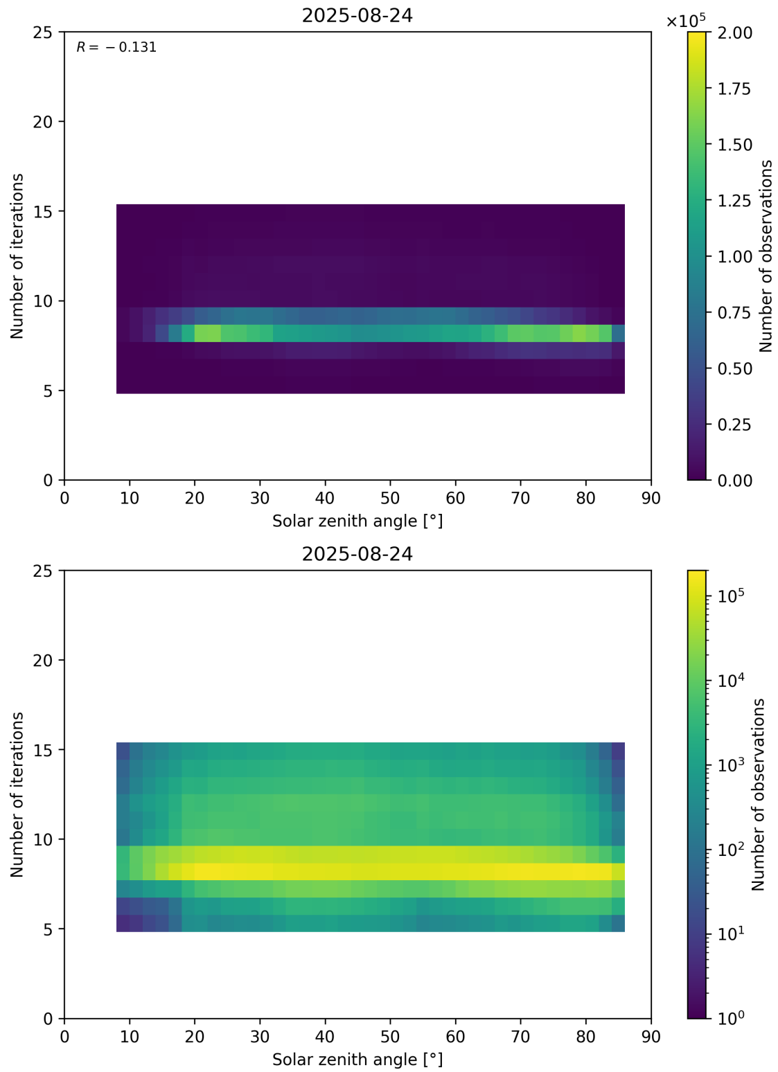
Figure 67: Scatter density plot of “Solar zenith angle” against “Number of iterations” for 2025-08-23 to 2025-08-25.
