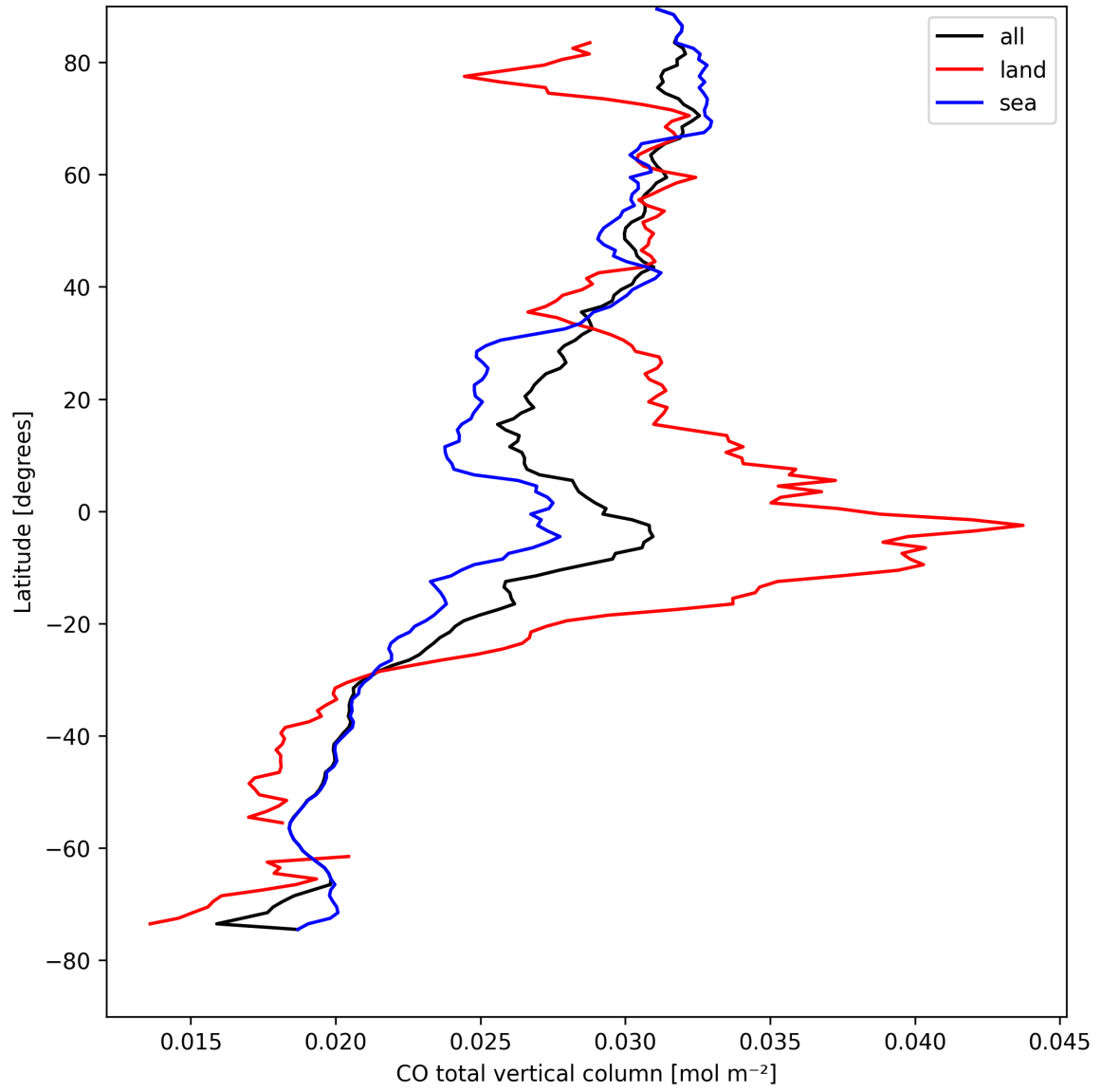
Figure 10: Zonal average of “CO total vertical column” for 2025-08-23 to 2025-08-25.
