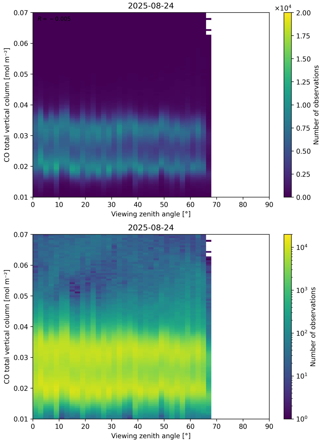
Figure 69: Scatter density plot of “Viewing zenith angle” against “CO total vertical column” for 2025-08-23 to 2025-08-25.
