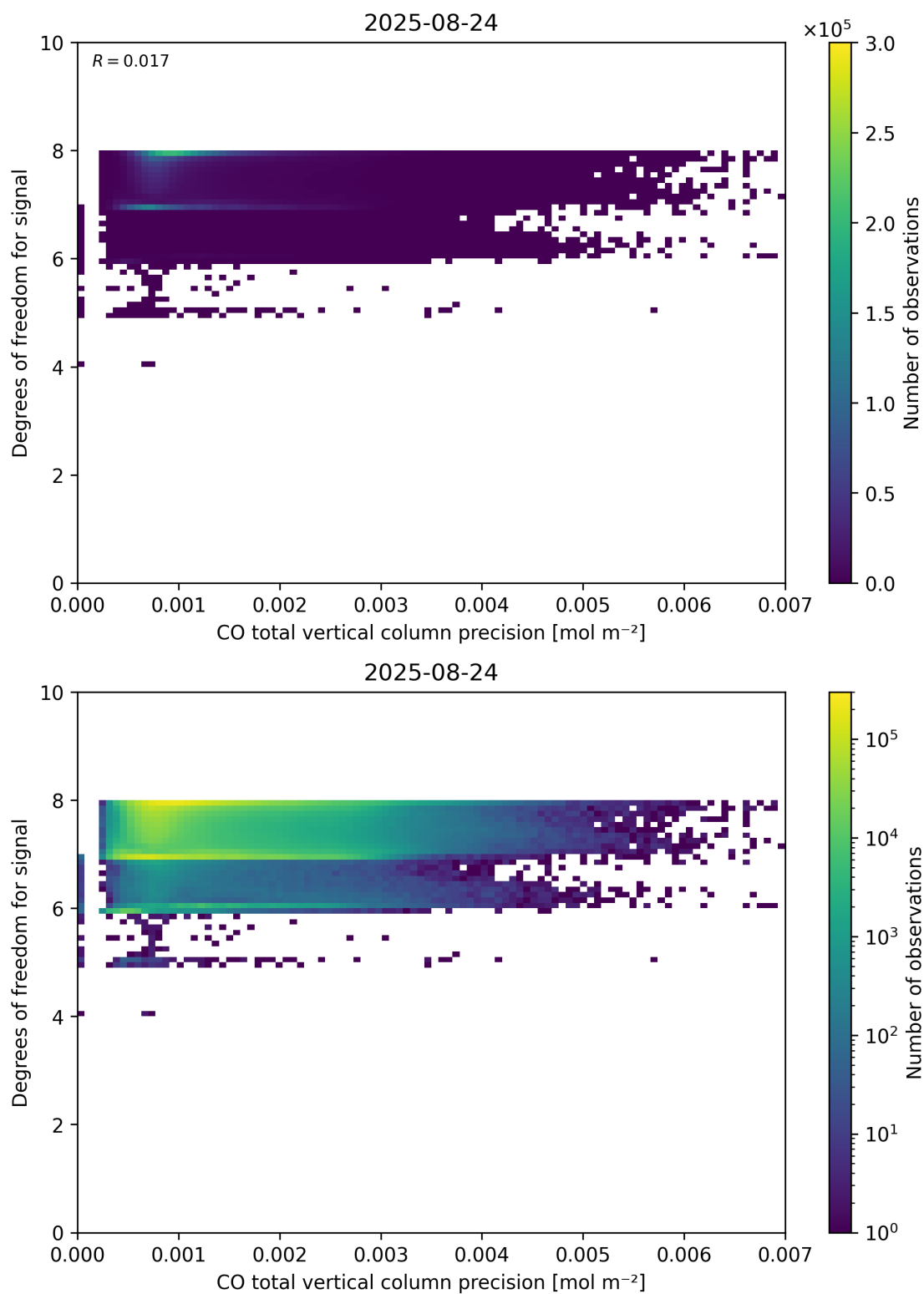
Figure 45: Scatter density plot of “CO total vertical column precision” against “Degrees of freedom for signal” for 2025-08-23 to 2025-08-25.
