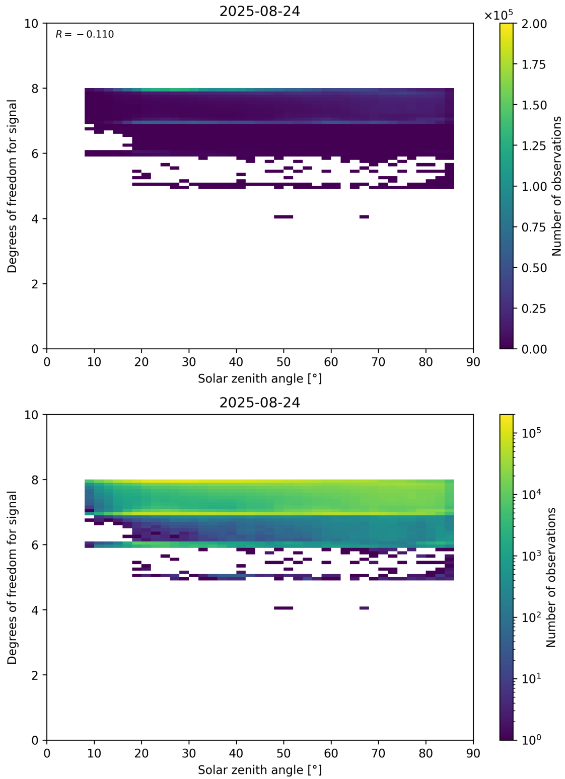
Figure 65: Scatter density plot of “Solar zenith angle” against “Degrees of freedom for signal” for 2025-08-23 to 2025-08-25.
