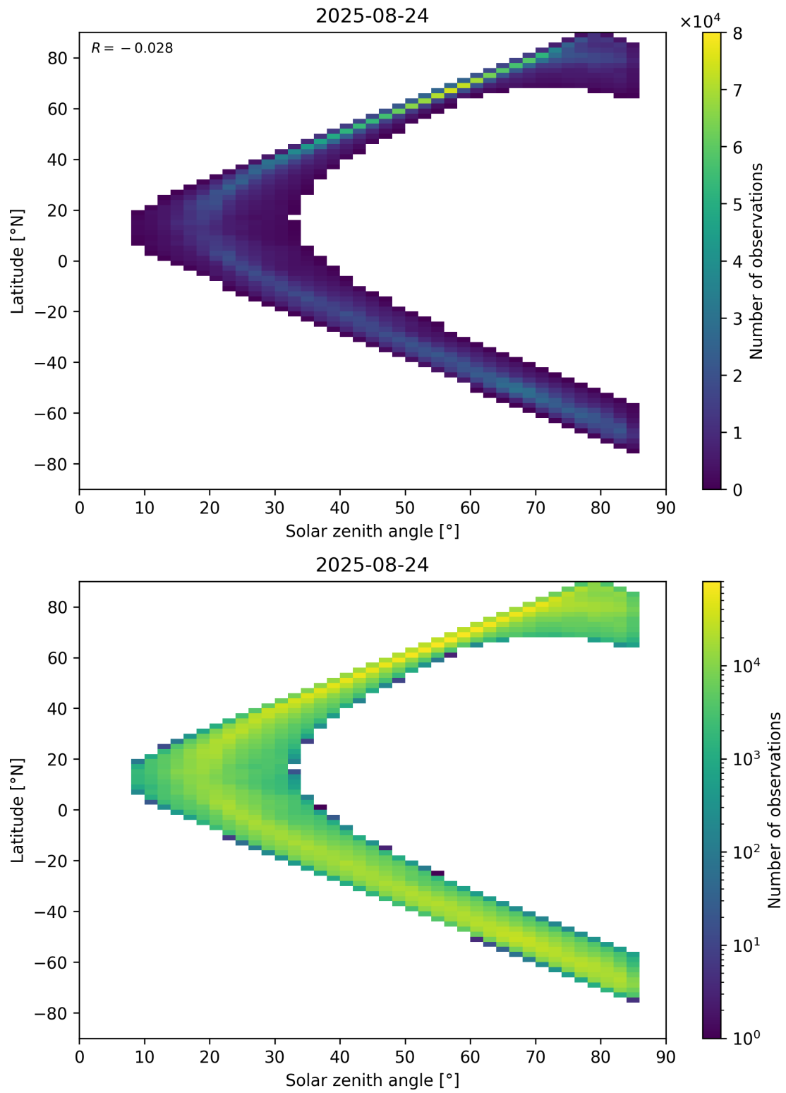
Figure 66: Scatter density plot of “Solar zenith angle” against “Latitude” for 2025-08-23 to 2025-08-25.
