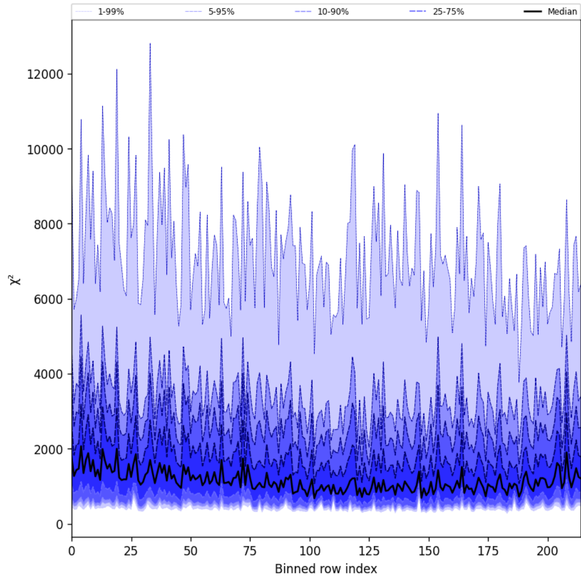
Figure 30: Along track statistics of “ \chi^2 ” for 2025-08-23 to 2025-08-25
