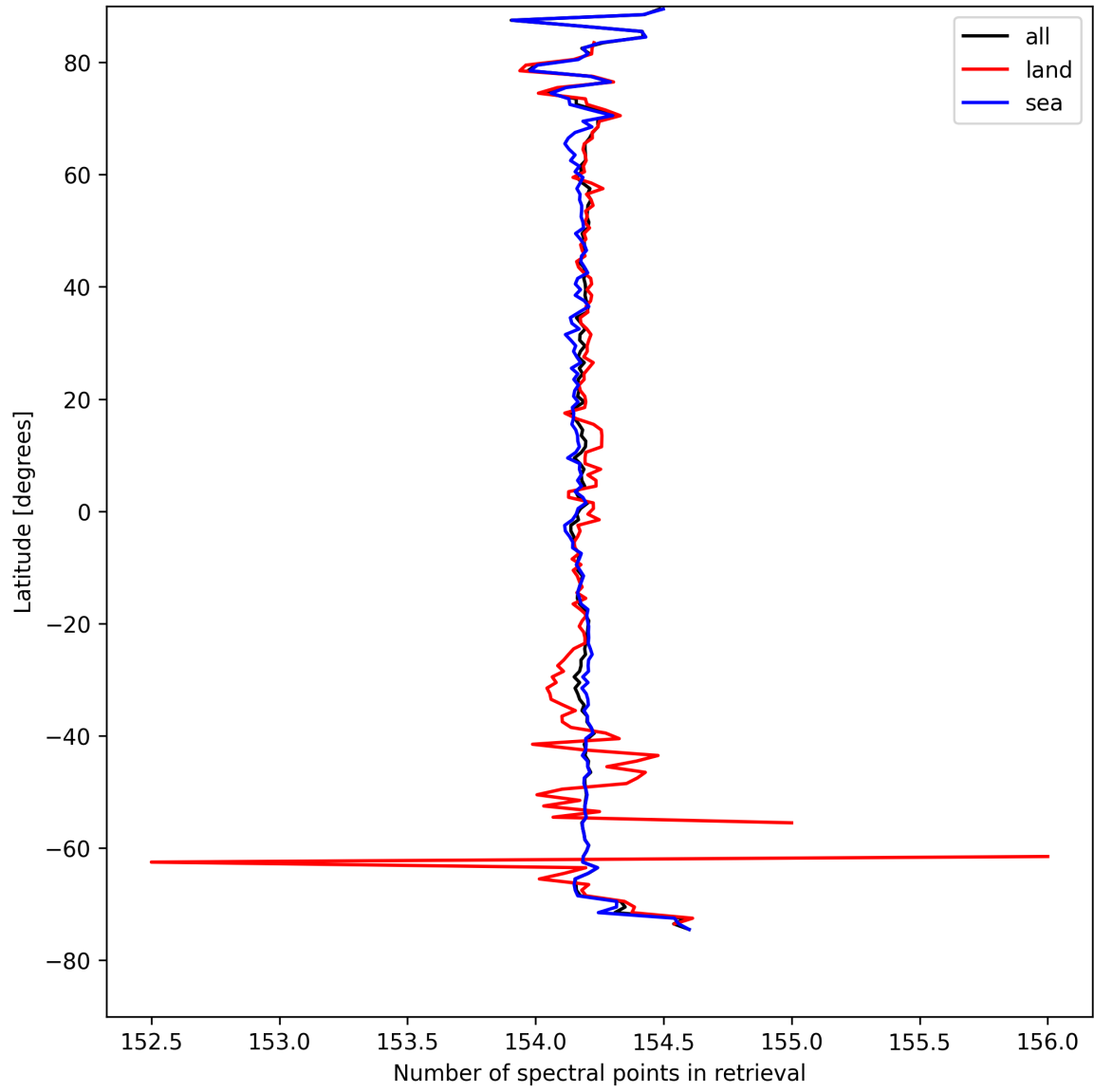
Figure 13: Zonal average of “Number of spectral points in retrieval” for 2025-08-23 to 2025-08-25.
