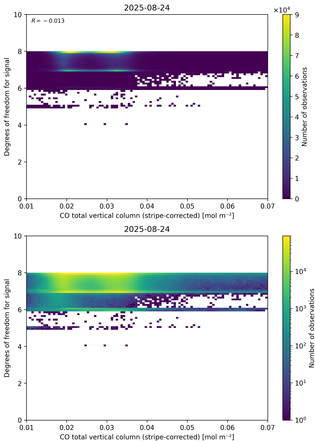
Figure 38: Scatter density plot of “CO total vertical column (stripe-corrected)” against “Degrees of freedom for signal” for 2025-08-23 to 2025-08-25.
