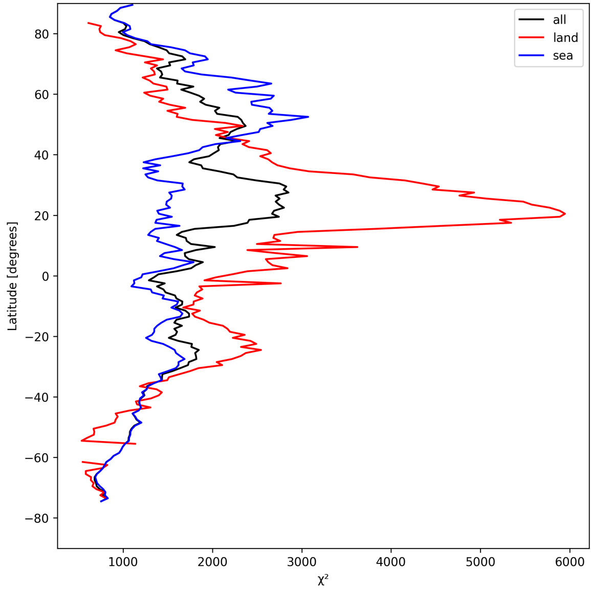
Figure 14: Zonal average of “ \chi^2 ” for 2025-08-23 to 2025-08-25.
