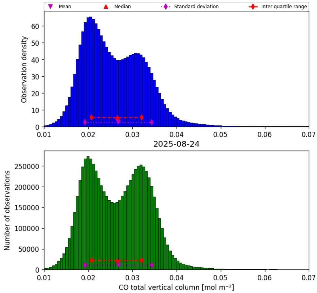
Figure 18: Histogram of “CO total vertical column” for 2025-08-23 to 2025-08-25
