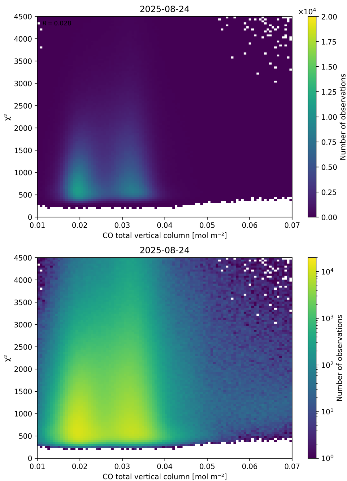
Figure 35: Scatter density plot of “CO total vertical column” against “ \chi^2 ” for 2025-08-23 to 2025-08-25.
