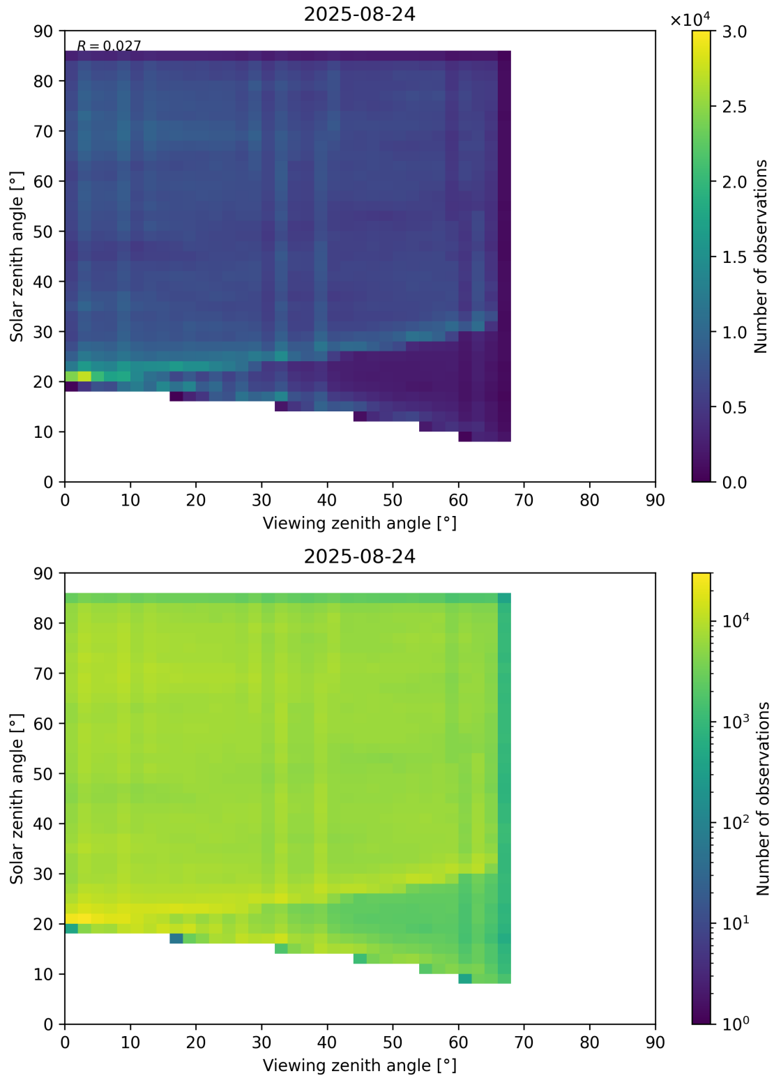
Figure 77: Scatter density plot of “Viewing zenith angle” against “Solar zenith angle” for 2025-08-23 to 2025-08-25.
