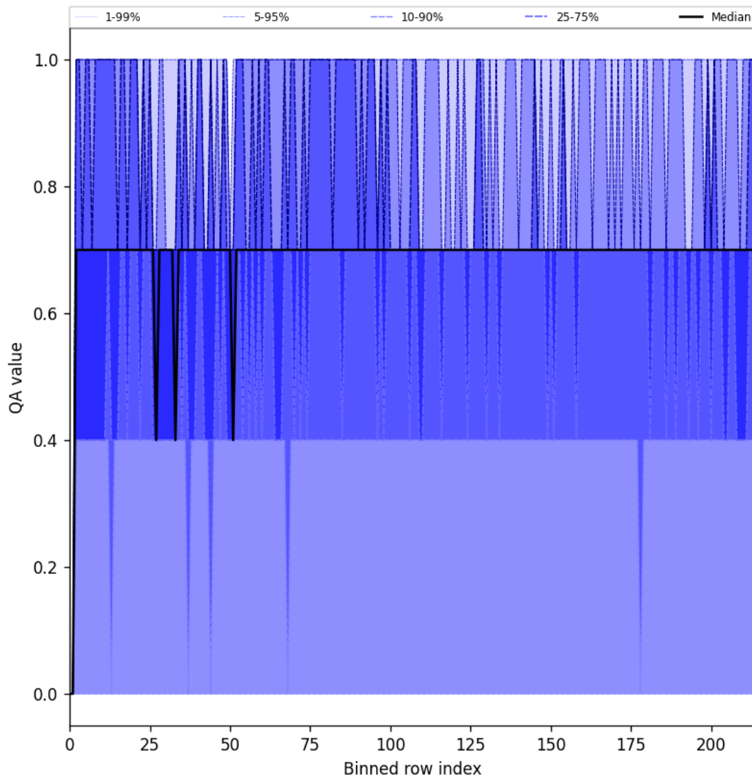
Figure 25: Along track statistics of “QA value” for 2025-08-23 to 2025-08-25
