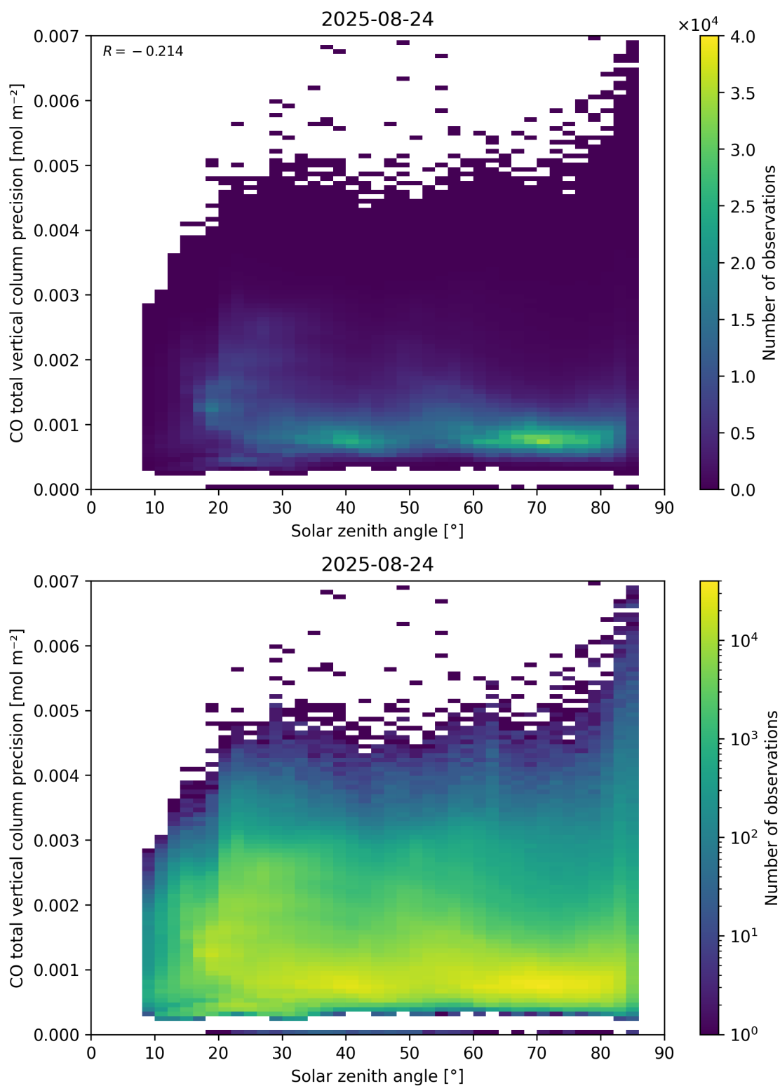
Figure 63: Scatter density plot of “Solar zenith angle” against “CO total vertical column precision” for 2025-08-23 to 2025-08-25.
