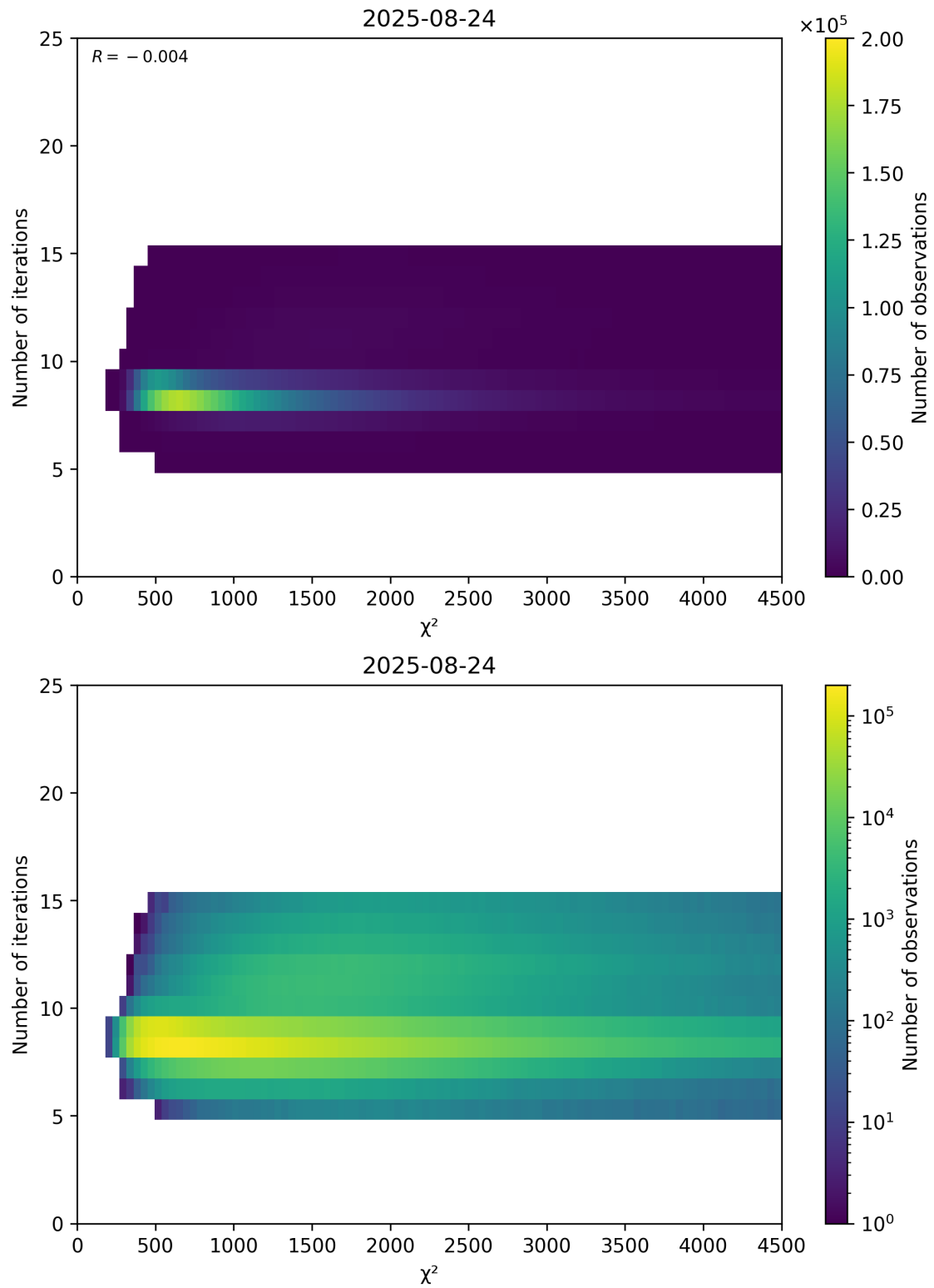
Figure 49: Scatter density plot of “ \chi^2 ” against “Number of iterations” for 2025-08-23 to 2025-08-25.
