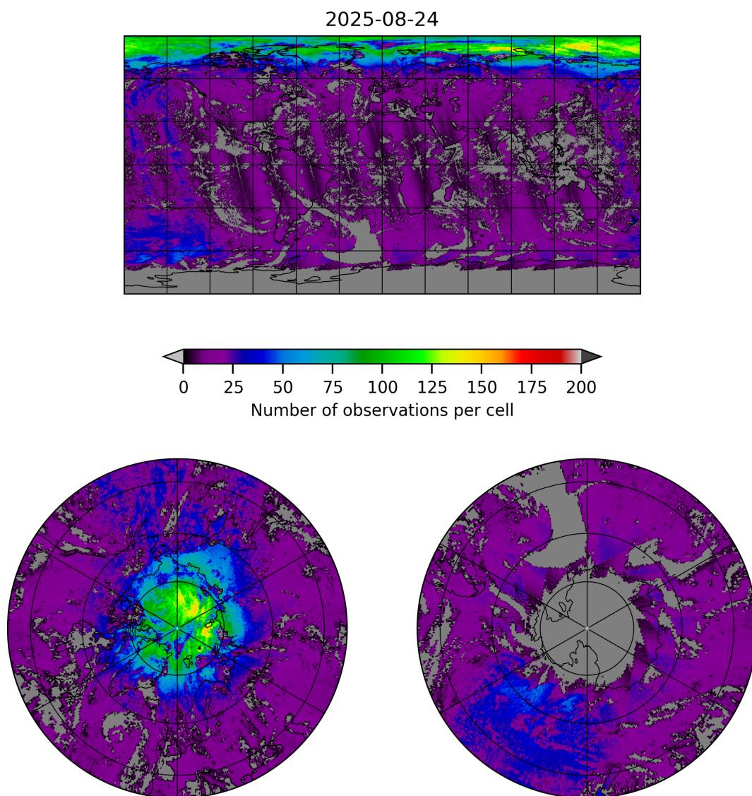
Figure 8: Map of the number of observations for 2025-08-23 to 2025-08-25
