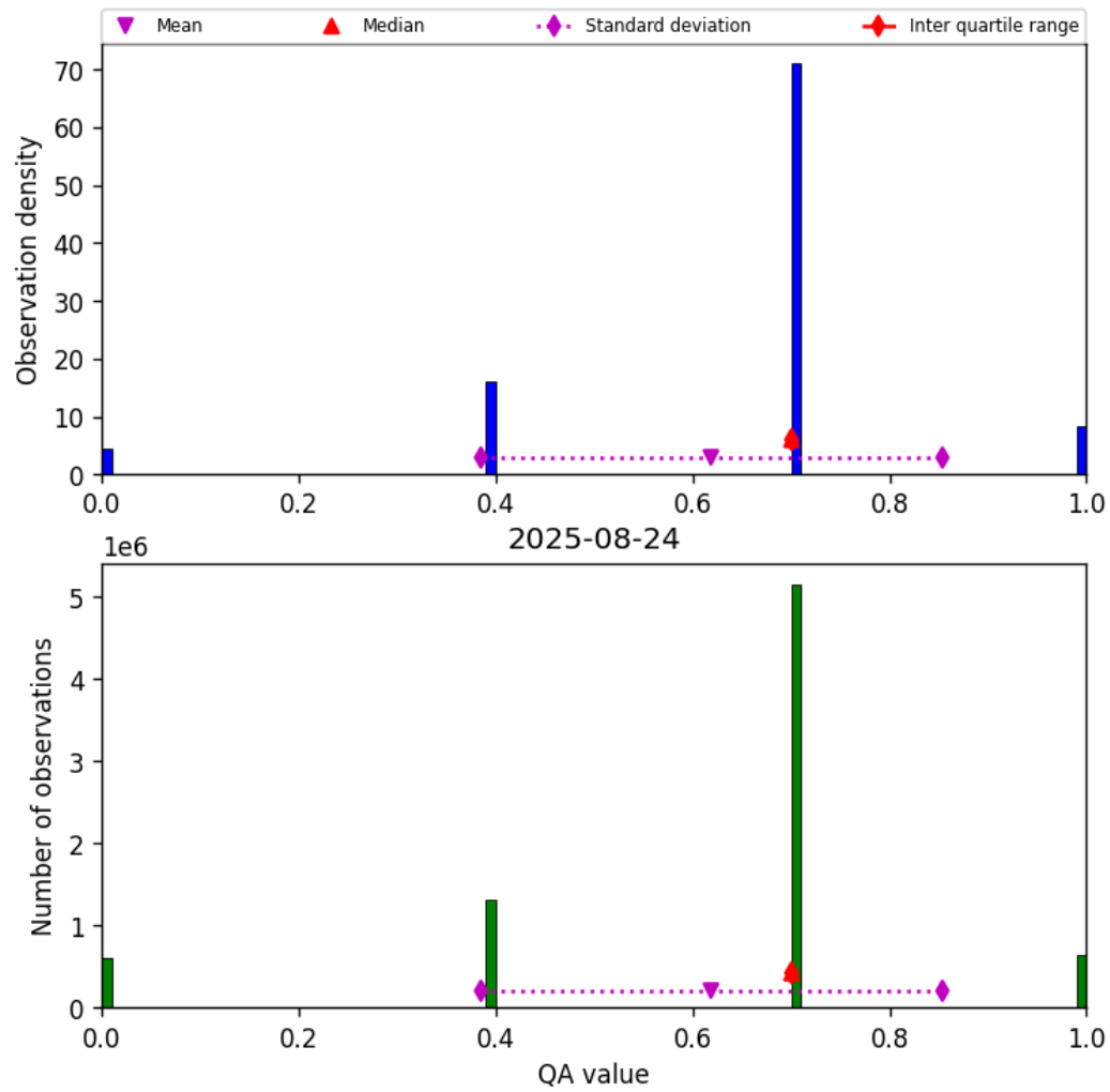
Figure 17: Histogram of “QA value” for 2025-08-23 to 2025-08-25
