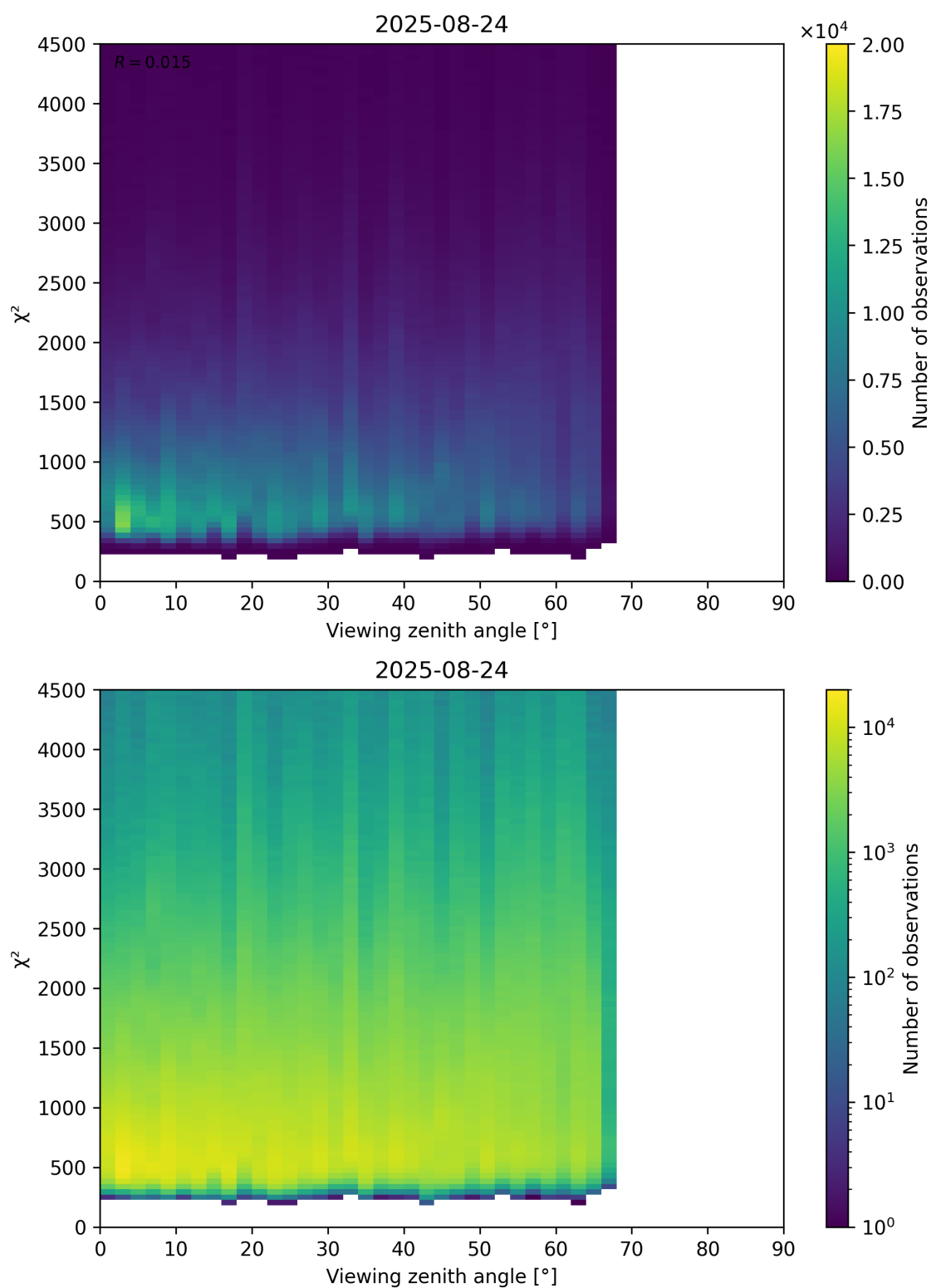
Figure 72: Scatter density plot of “Viewing zenith angle” against “ \chi^2 ” for 2025-08-23 to 2025-08-25.
