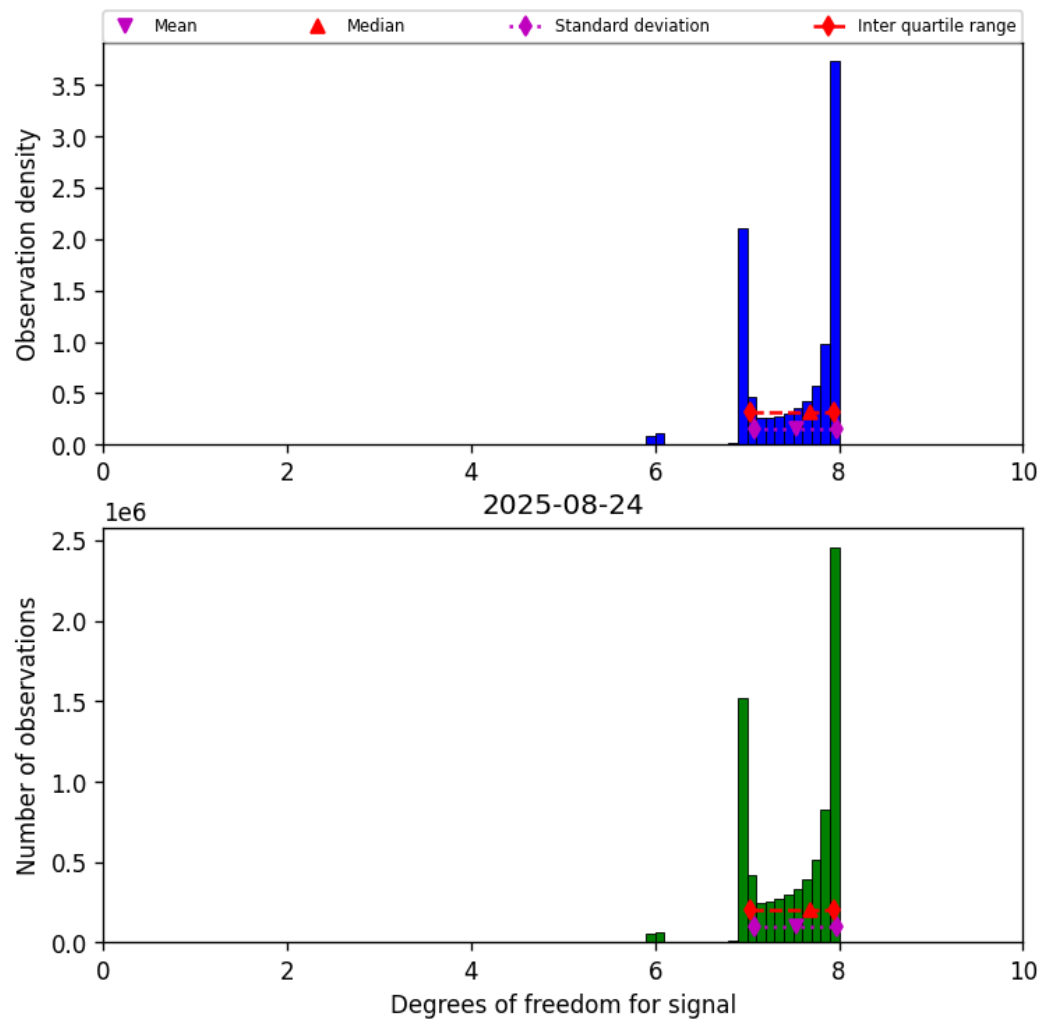
Figure 23: Histogram of “Degrees of freedom for signal” for 2025-08-23 to 2025-08-25
