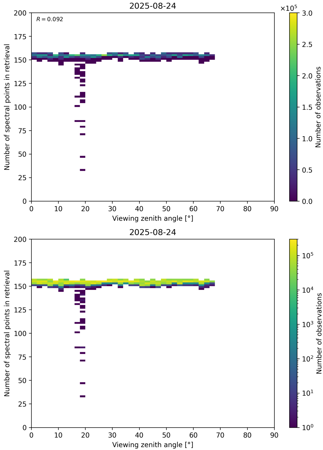
Figure 76: Scatter density plot of “Viewing zenith angle” against “Number of spectral points in retrieval” for 2025-08-23 to 2025-08-25.
