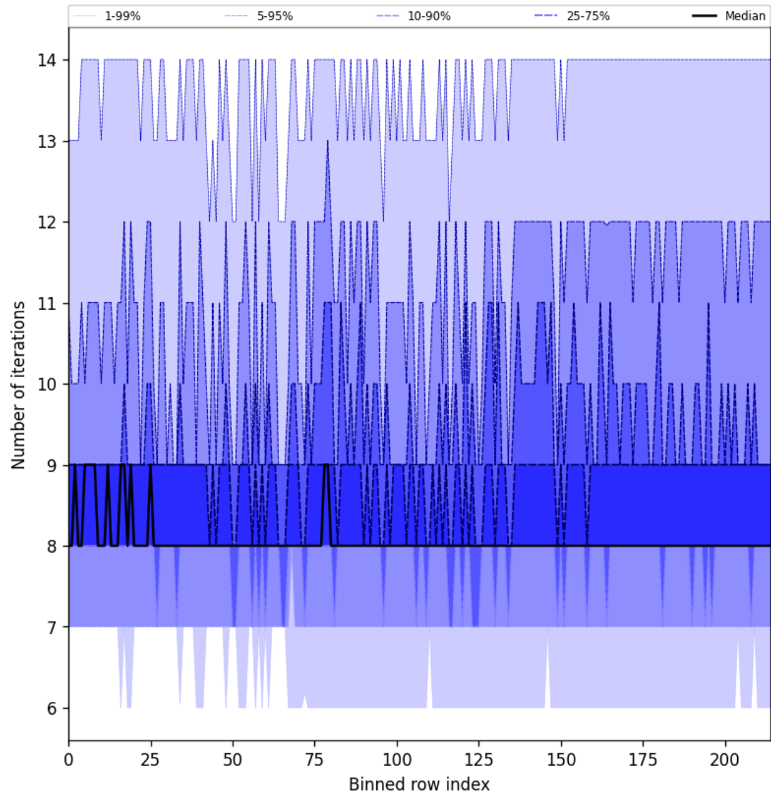
Figure 32: Along track statistics of “Number of iterations” for 2025-08-23 to 2025-08-25
