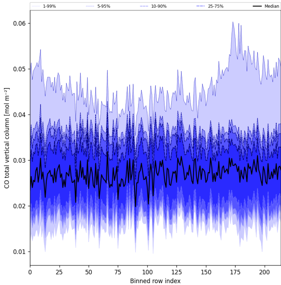
Figure 26: Along track statistics of “CO total vertical column” for 2025-08-23 to 2025-08-25
