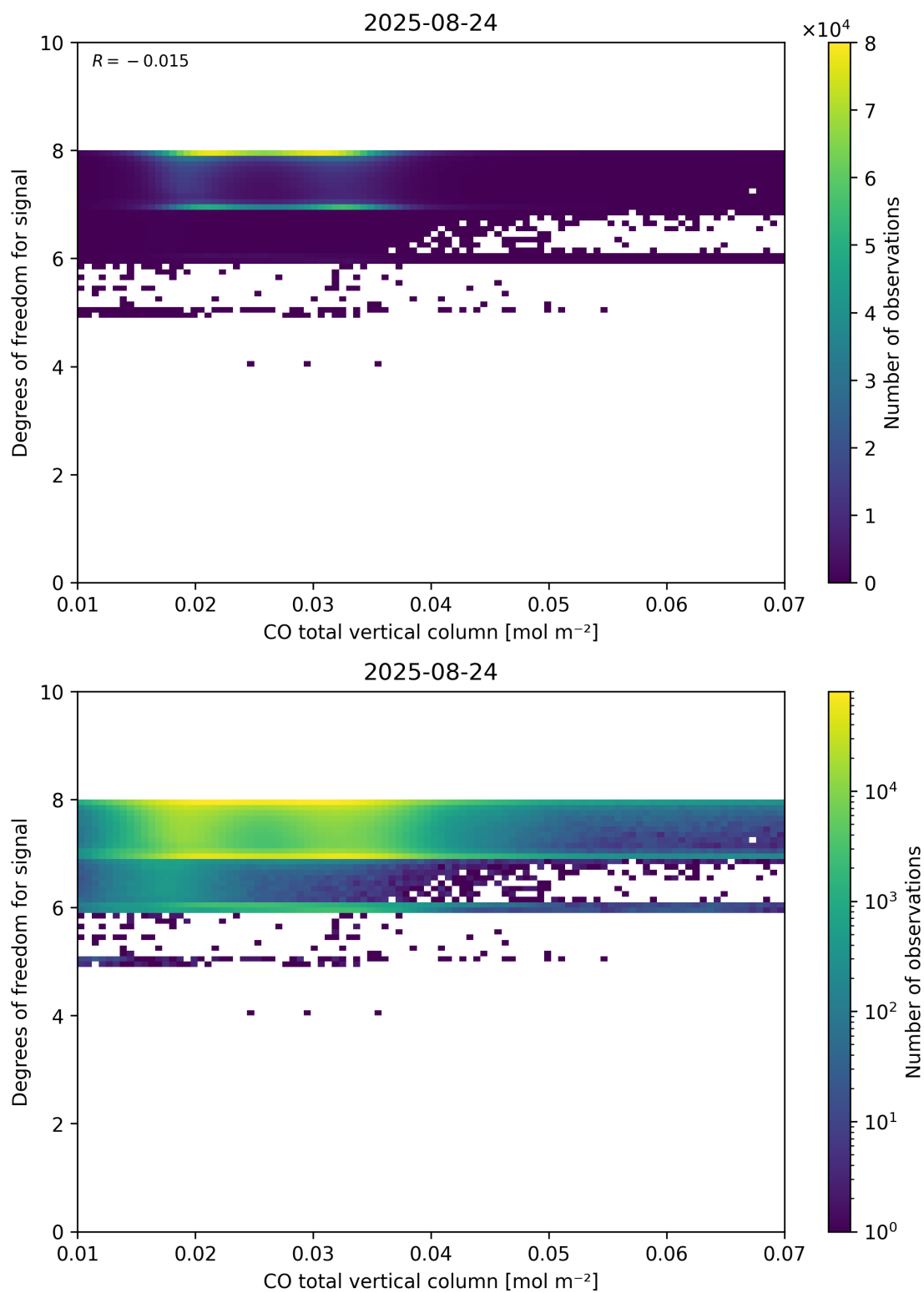
Figure 41: Scatter density plot of “CO total vertical column” against “Degrees of freedom for signal” for 2025-08-23 to 2025-08-25.
