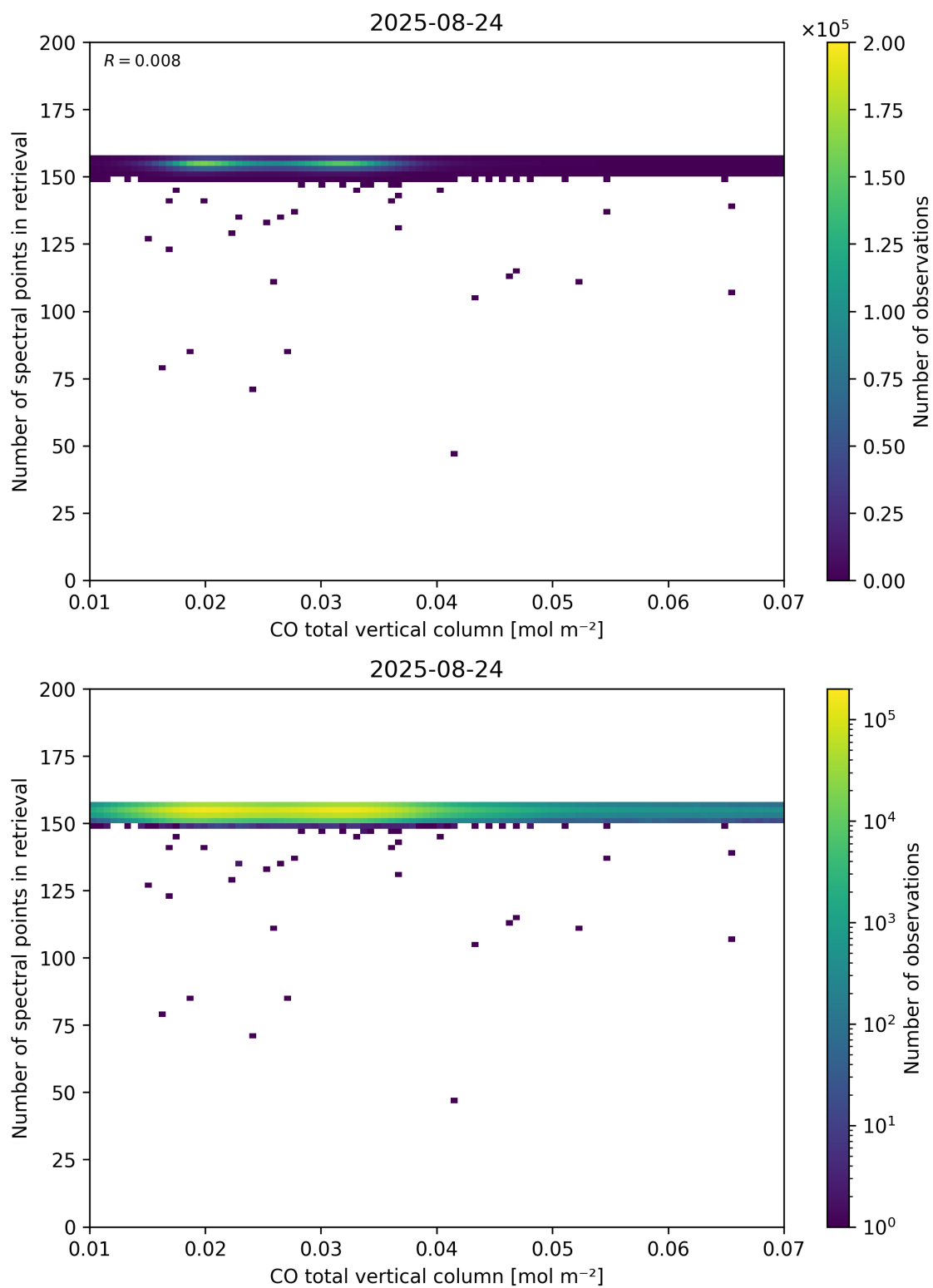
Figure 43: Scatter density plot of “CO total vertical column” against “Number of spectral points in retrieval” for 2025-08-23 to 2025-08-25.
