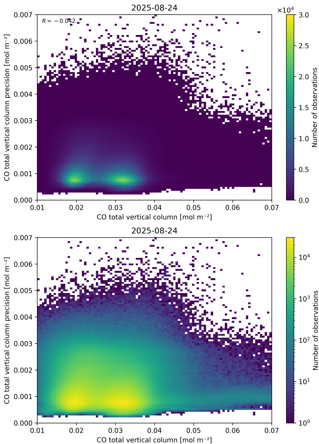
Figure 34: Scatter density plot of “CO total vertical column” against “CO total vertical column precision” for 2025-08-23 to 2025-08-25.
