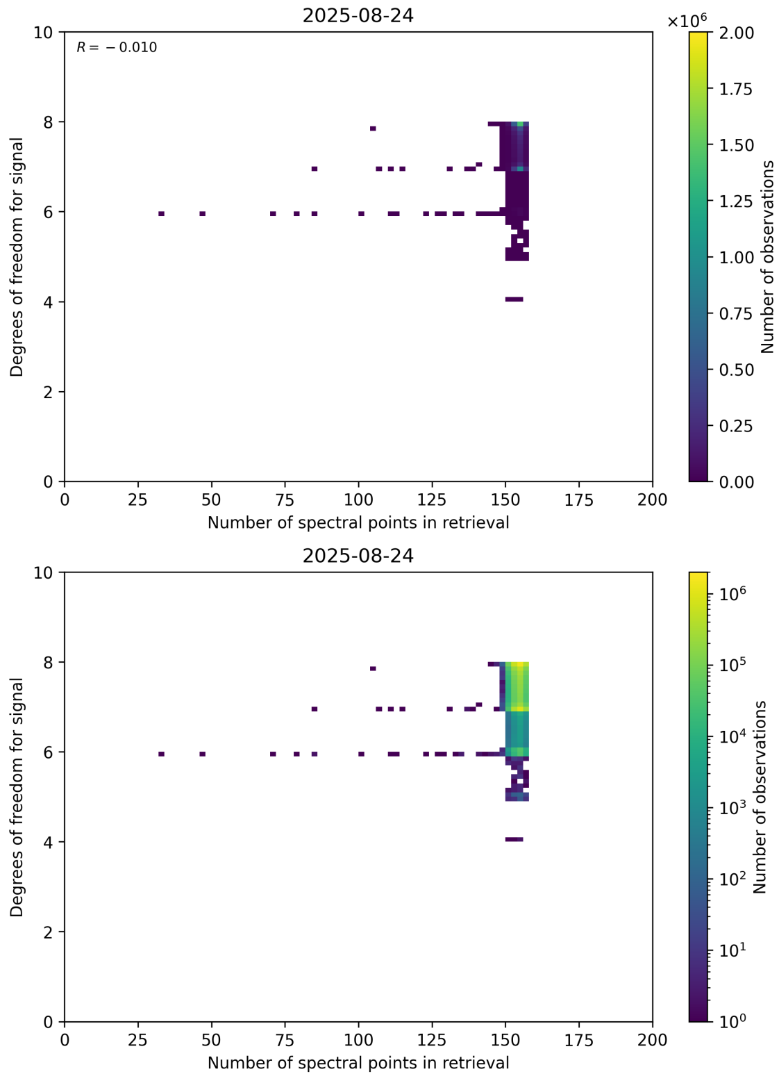
Figure 59: Scatter density plot of “Number of spectral points in retrieval” against “Degrees of freedom for signal” for 2025-08-23 to 2025-08-25.
