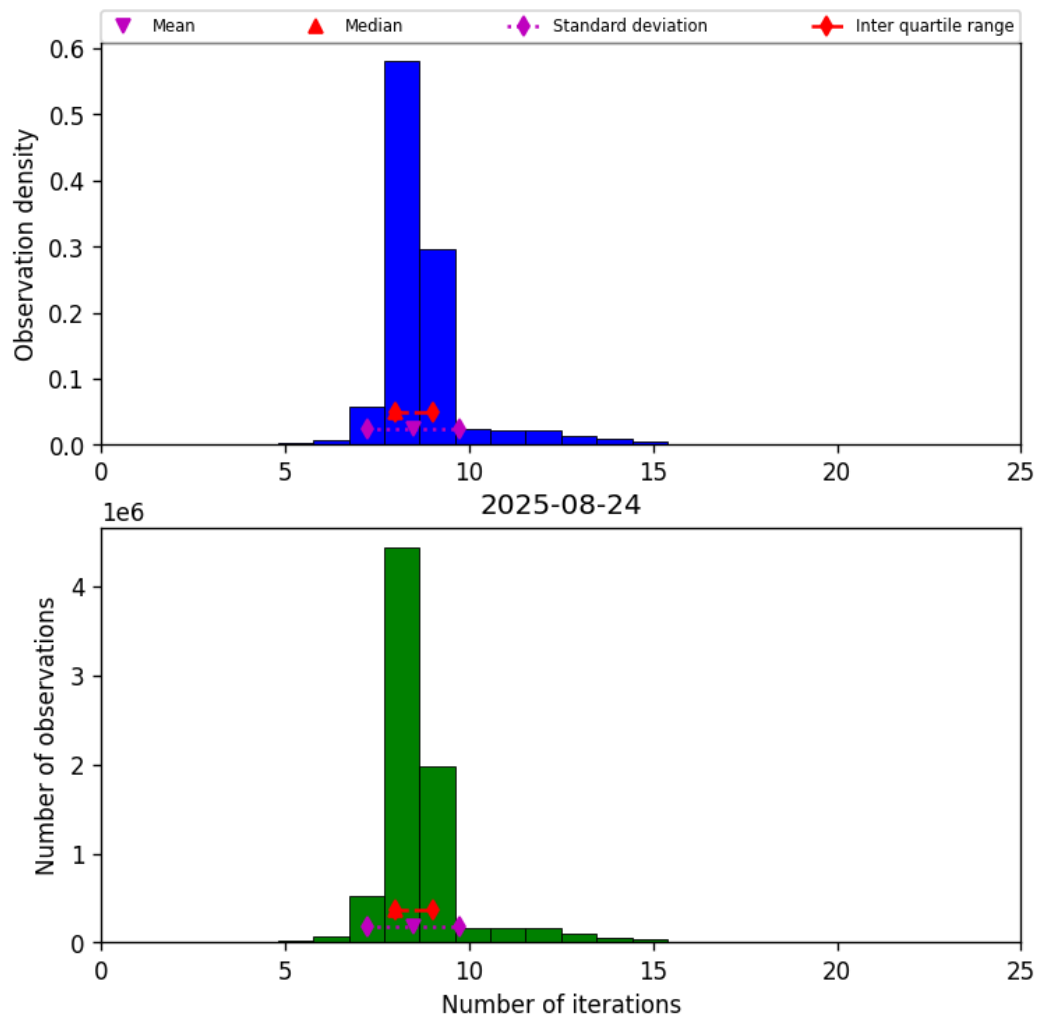
Figure 24: Histogram of “Number of iterations” for 2025-08-23 to 2025-08-25
