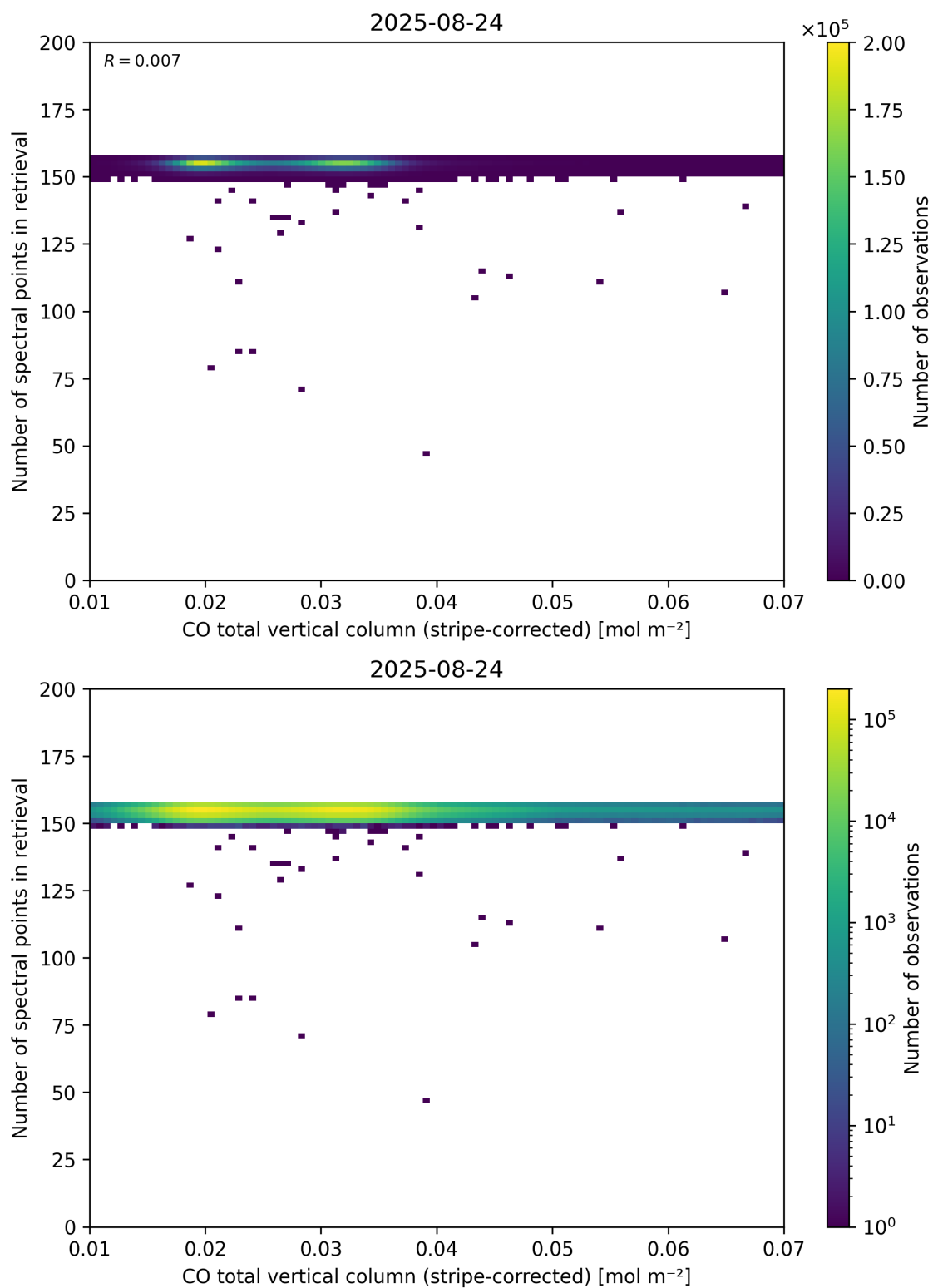
Figure 40: Scatter density plot of “CO total vertical column (stripe-corrected)” against “Number of spectral points in retrieval” for 2025-08-23 to 2025-08-25.
