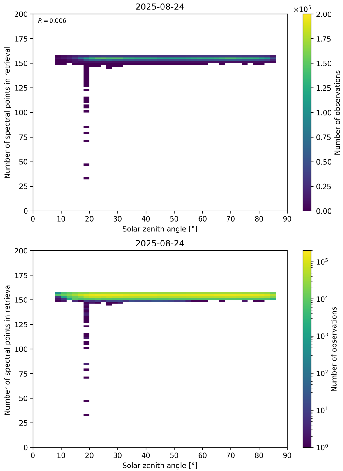
Figure 68: Scatter density plot of “Solar zenith angle” against “Number of spectral points in retrieval” for 2025-08-23 to 2025-08-25.
