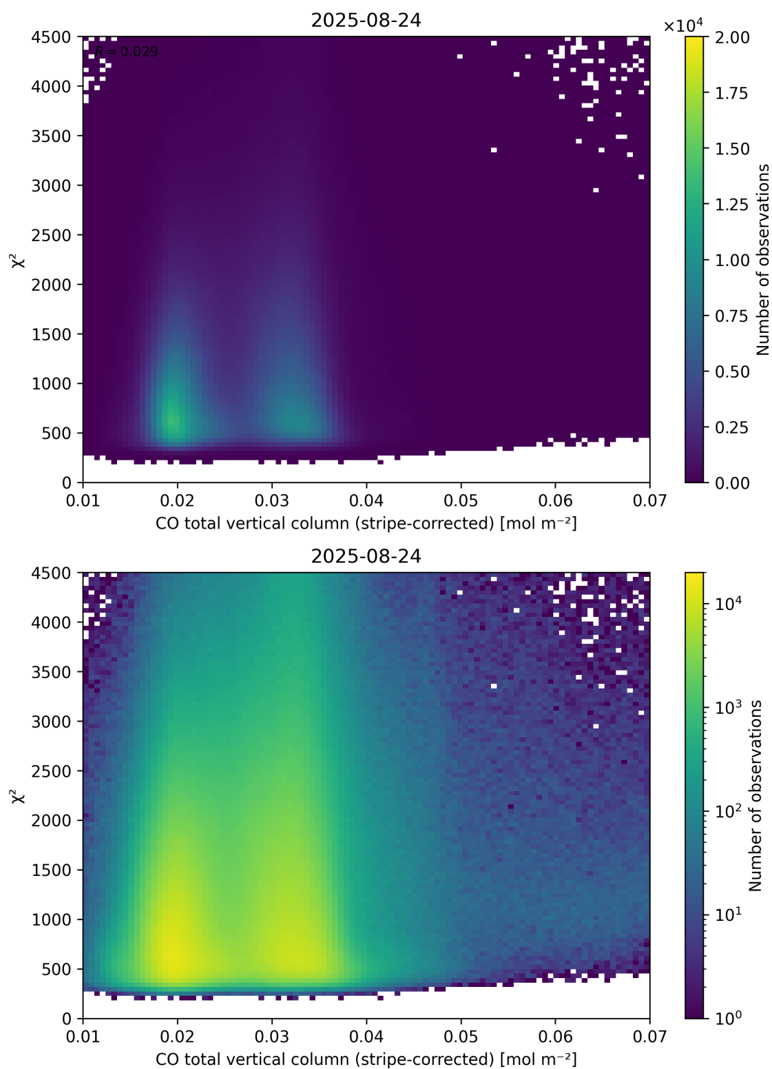
Figure 37: Scatter density plot of “CO total vertical column (stripe-corrected)” against “ \chi^2 ” for 2025-08-23 to 2025-08-25.
