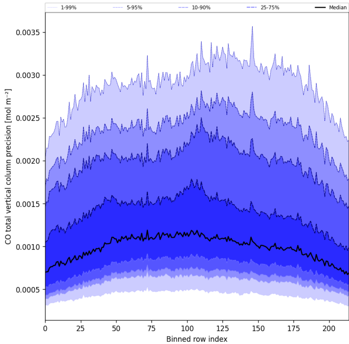
Figure 28: Along track statistics of “CO total vertical column precision” for 2025-08-23 to 2025-08-25
