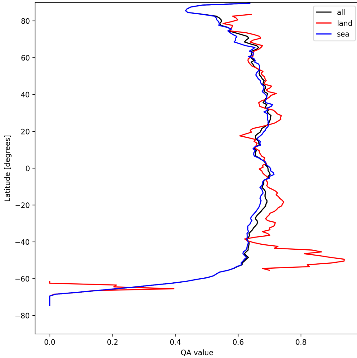
Figure 9: Zonal average of “QA value” for 2025-08-23 to 2025-08-25.
