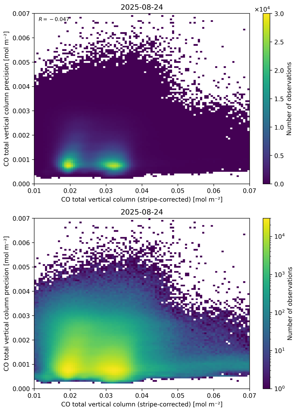
Figure 36: Scatter density plot of “CO total vertical column (stripe-corrected)” against “CO total vertical column precision” for 2025-08-23 to 2025-08-25.
