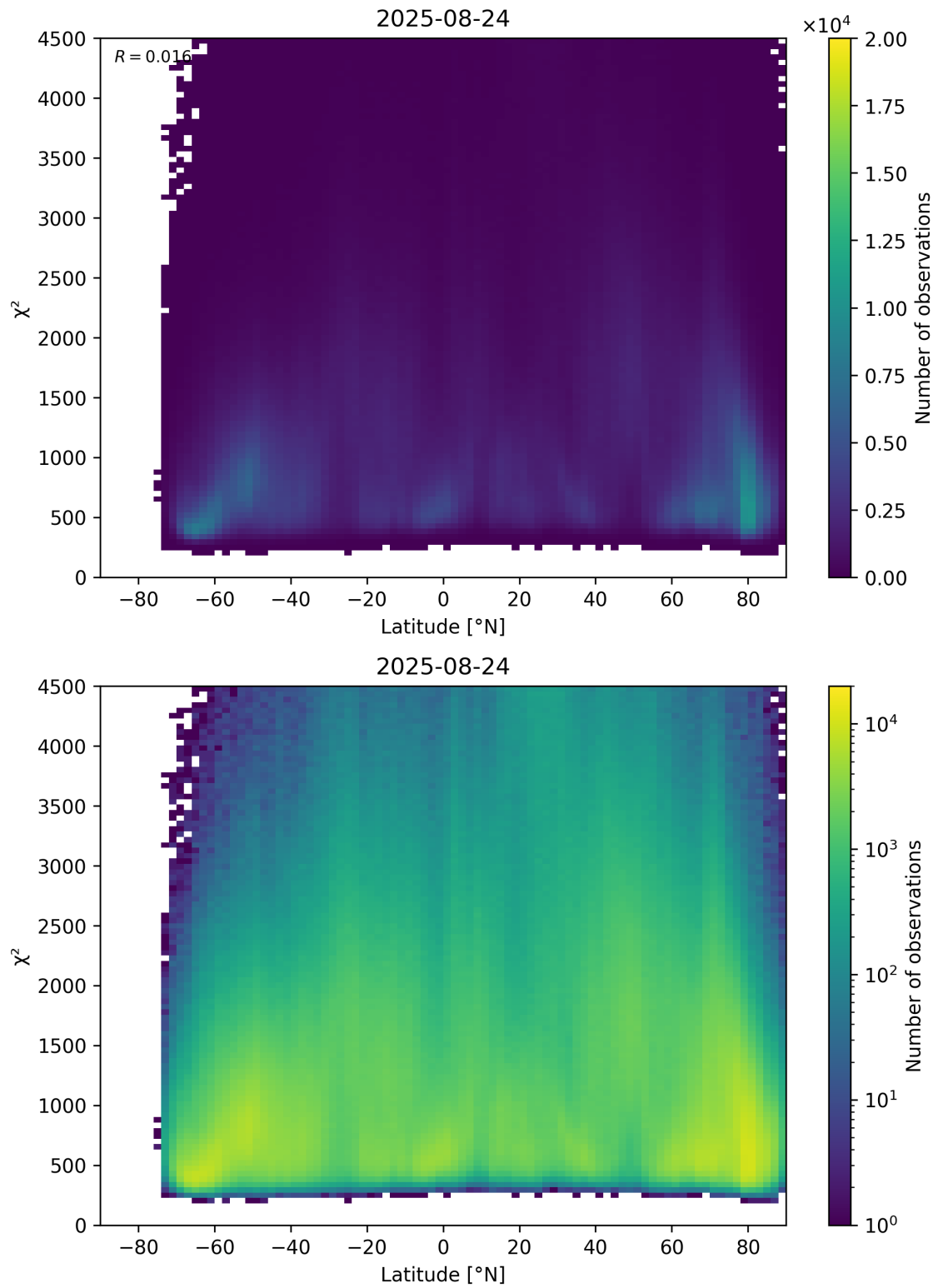
Figure 54: Scatter density plot of “Latitude” against “ \chi^2 ” for 2025-08-23 to 2025-08-25.
