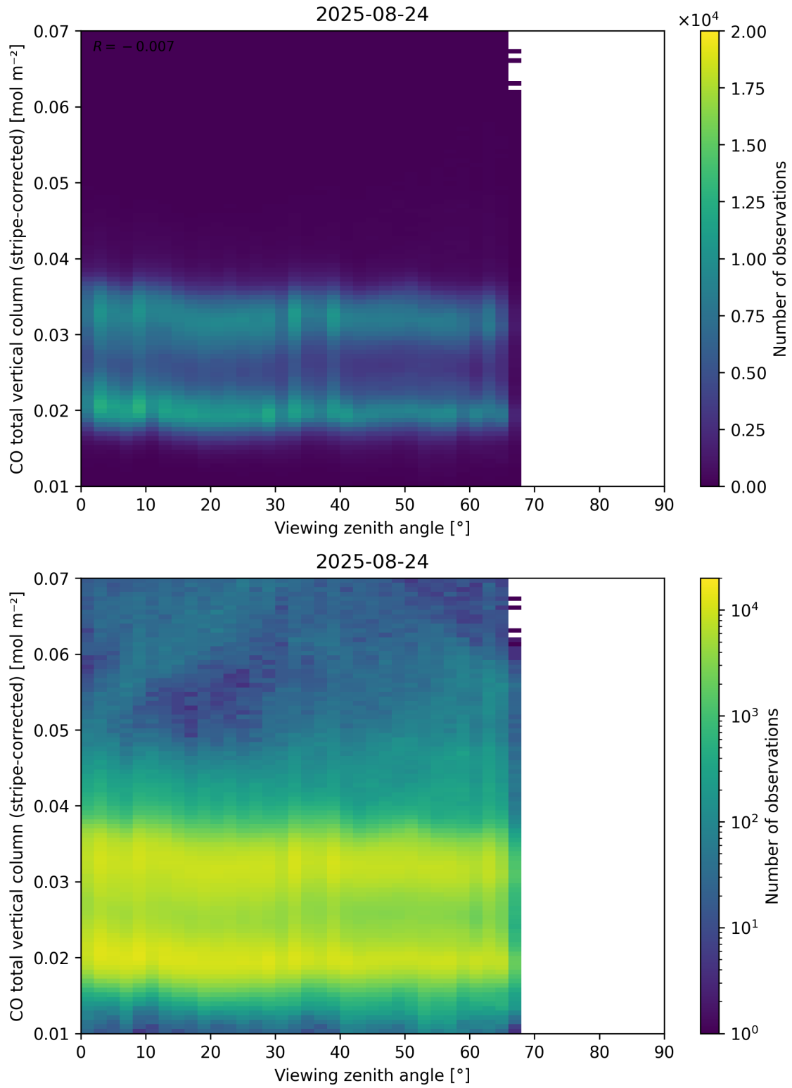
Figure 70: Scatter density plot of “Viewing zenith angle” against “CO total vertical column (stripe-corrected)” for 2025-08-23 to 2025-08-25.
