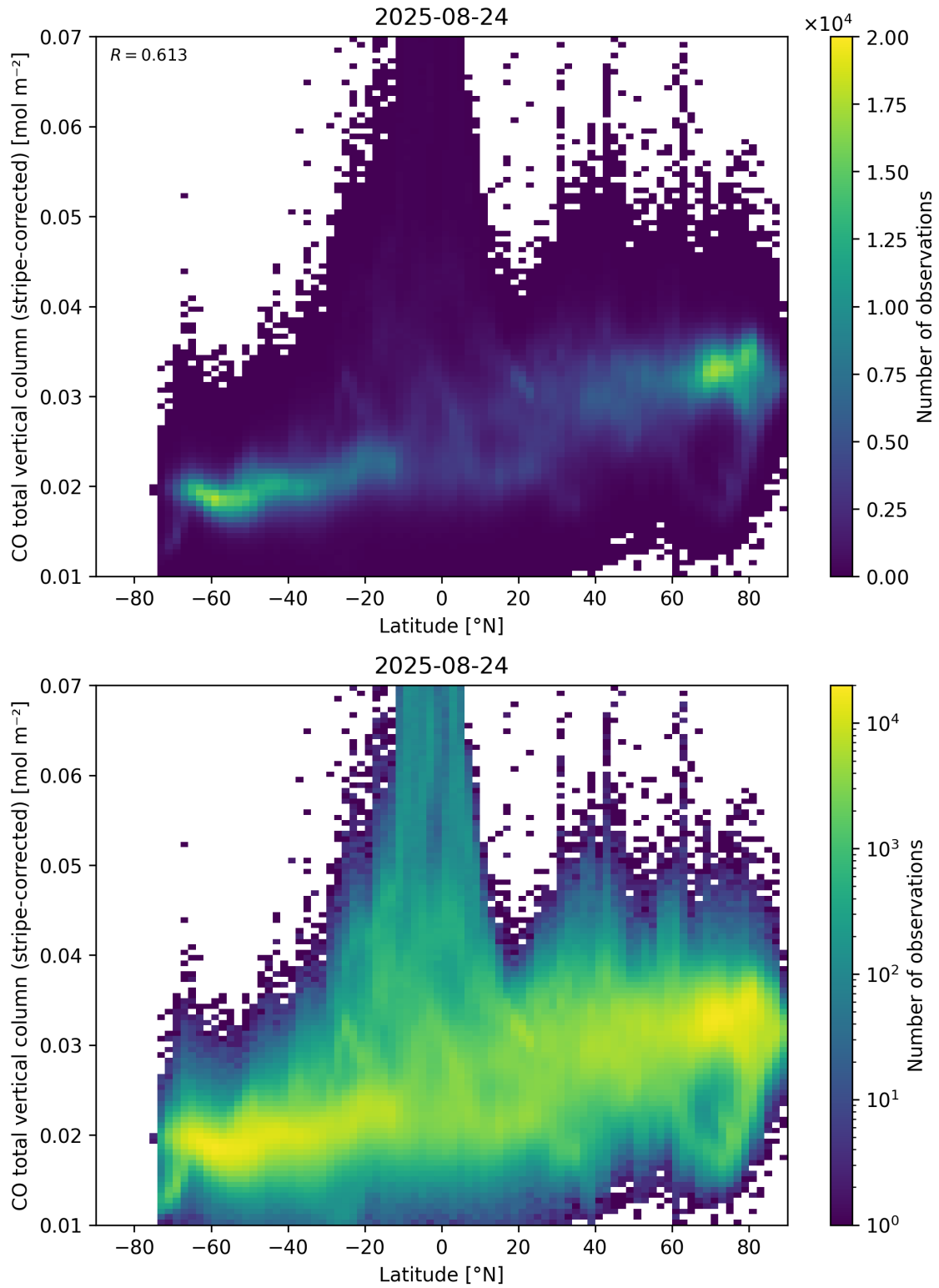
Figure 52: Scatter density plot of “Latitude” against “CO total vertical column (stripe-corrected)” for 2025-08-23 to 2025-08-25.
