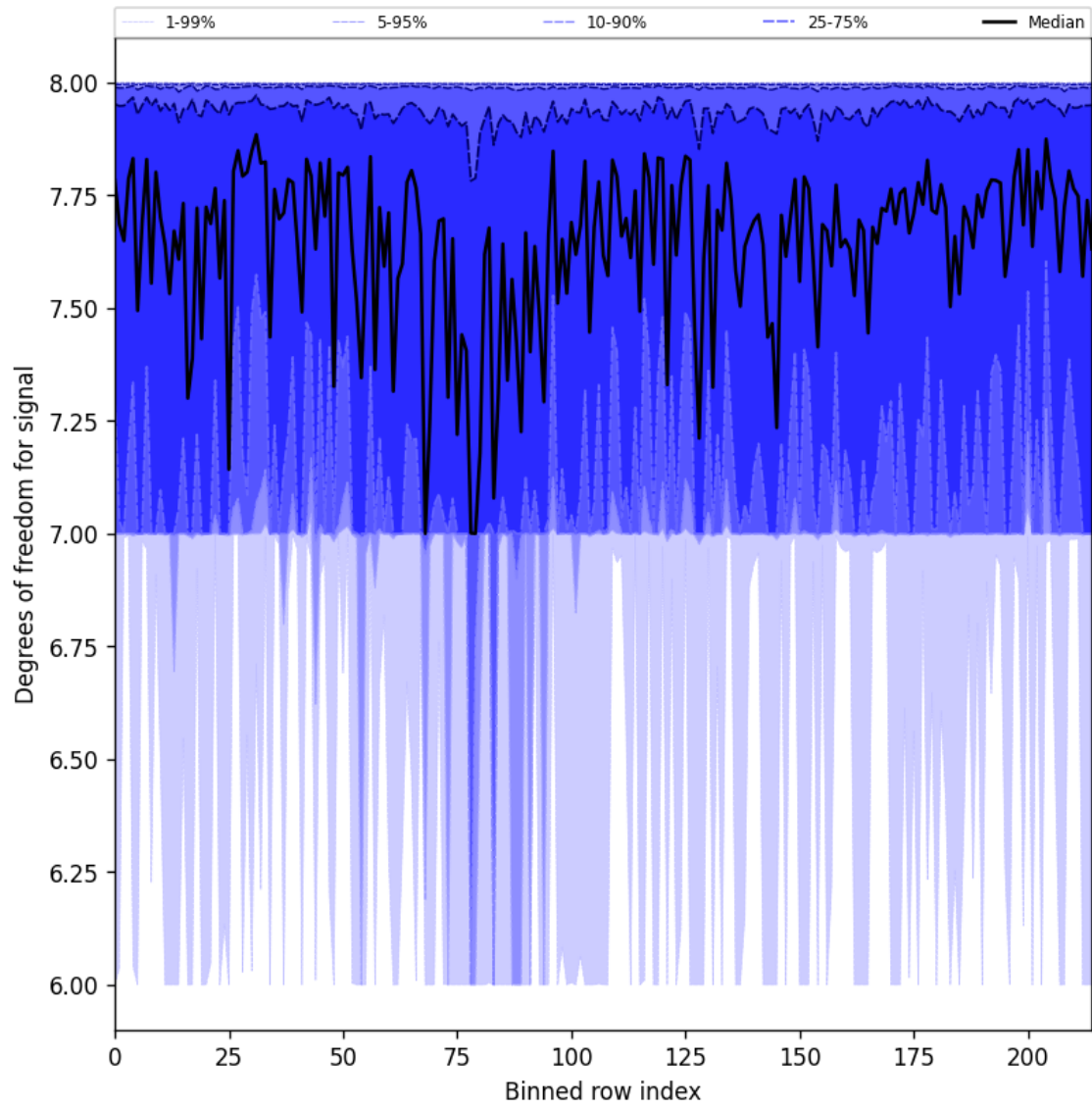
Figure 31: Along track statistics of “Degrees of freedom for signal” for 2025-08-23 to 2025-08-25
