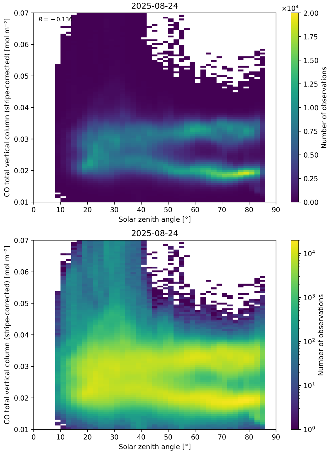
Figure 62: Scatter density plot of “Solar zenith angle” against “CO total vertical column (stripe-corrected)” for 2025-08-23 to 2025-08-25.
