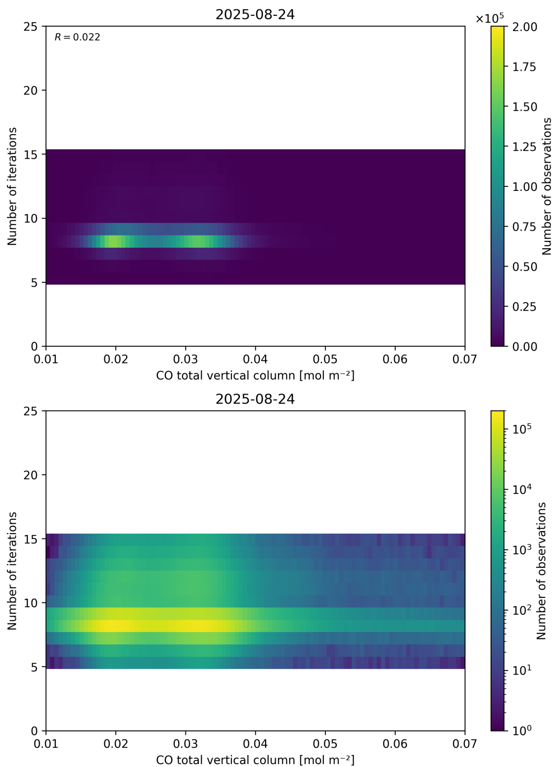
Figure 42: Scatter density plot of “CO total vertical column” against “Number of iterations” for 2025-08-23 to 2025-08-25.
