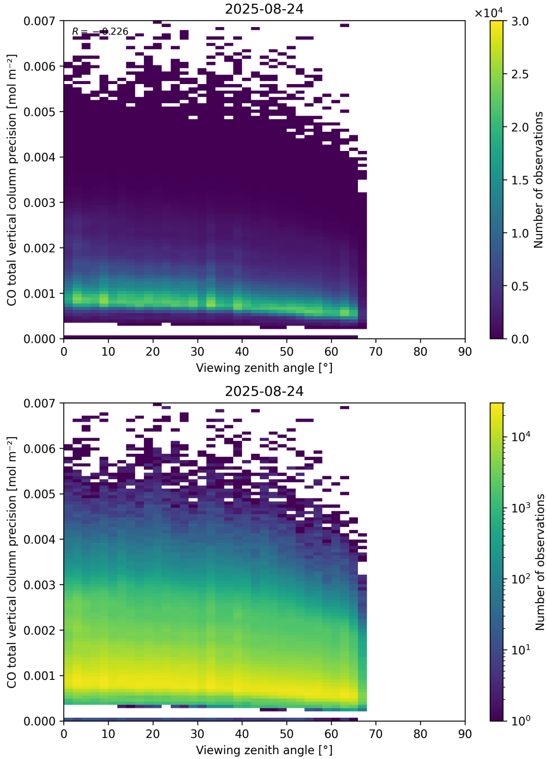
Figure 71: Scatter density plot of “Viewing zenith angle” against “CO total vertical column precision” for 2025-08-23 to 2025-08-25.
