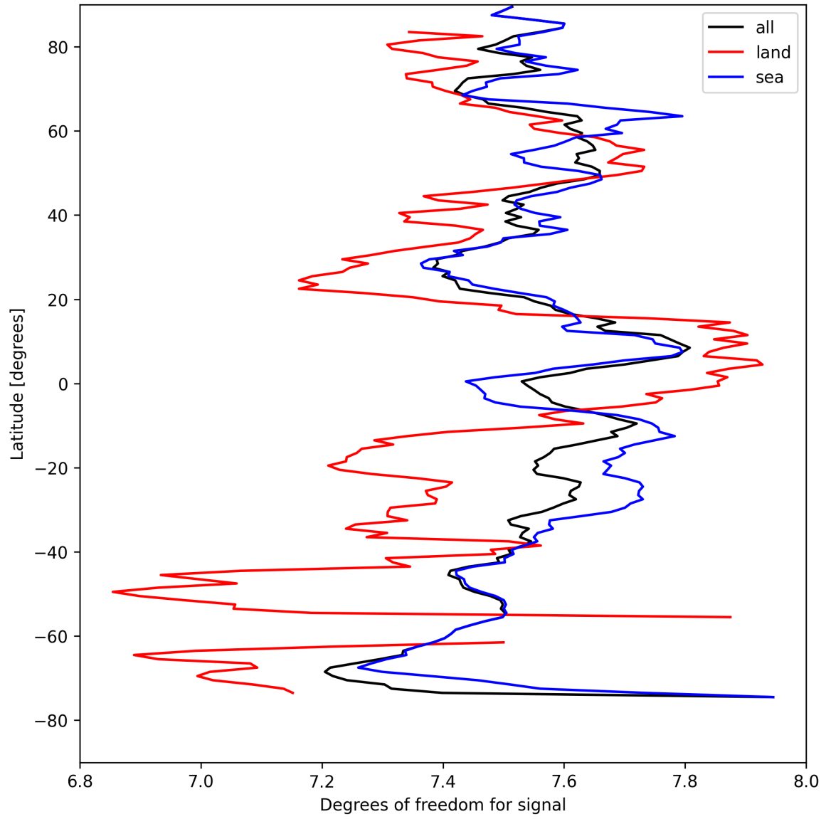
Figure 15: Zonal average of “Degrees of freedom for signal” for 2025-08-23 to 2025-08-25.
