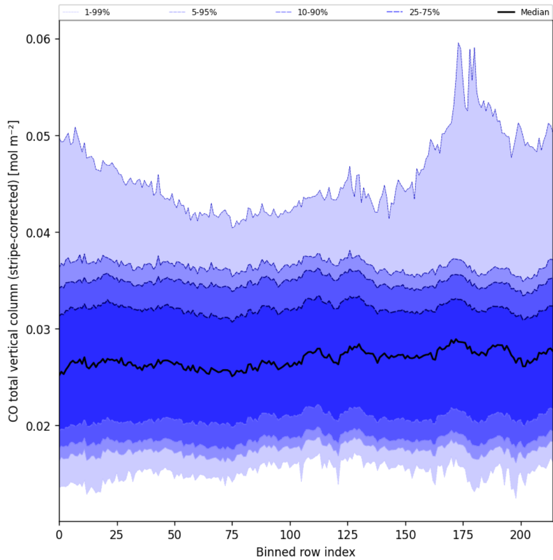
Figure 27: Along track statistics of “CO total vertical column (stripe-corrected)” for 2025-08-23 to 2025-08-25
