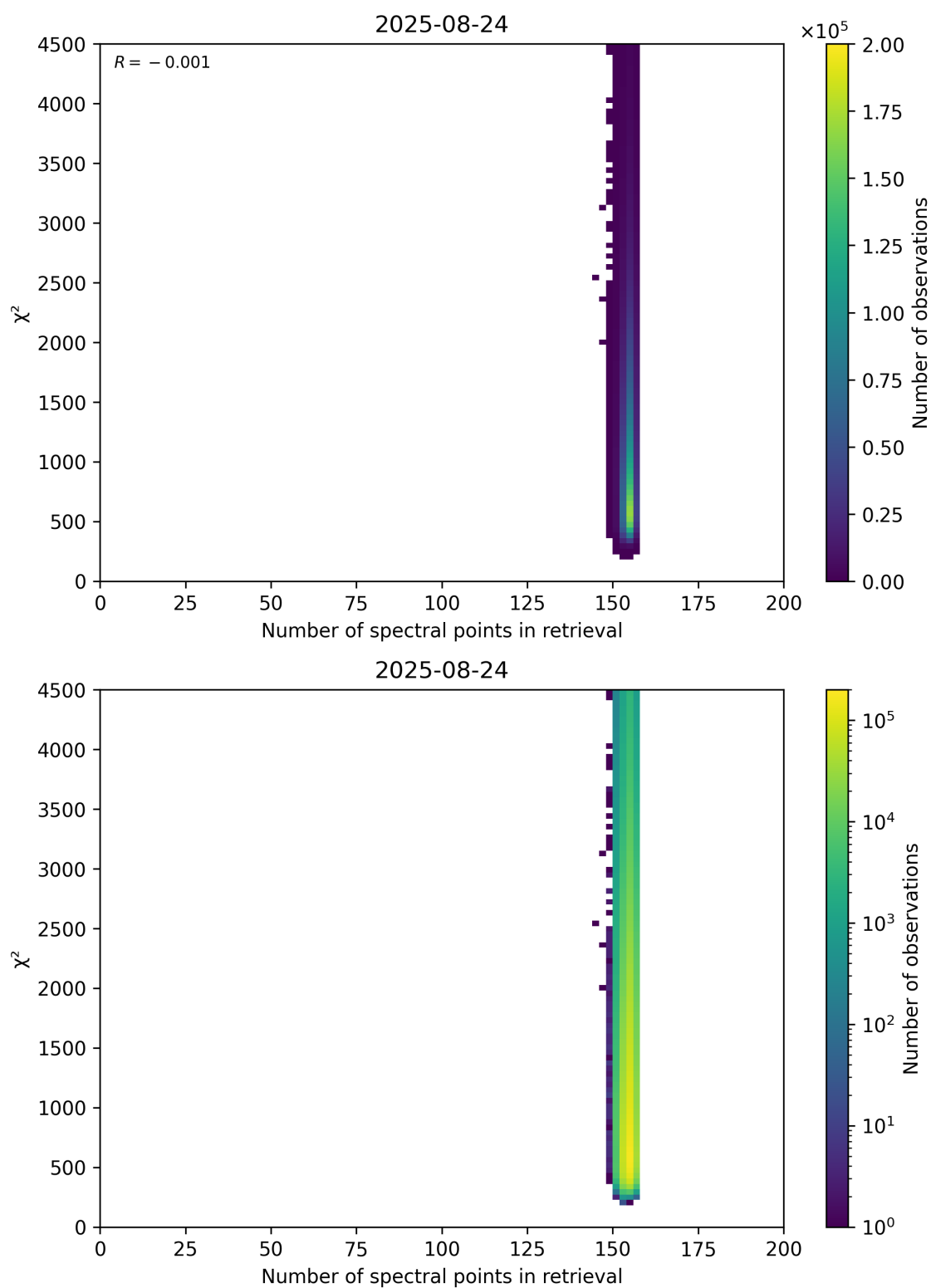
Figure 58: Scatter density plot of “Number of spectral points in retrieval” against “ \chi^2 ” for 2025-08-23 to 2025-08-25.
