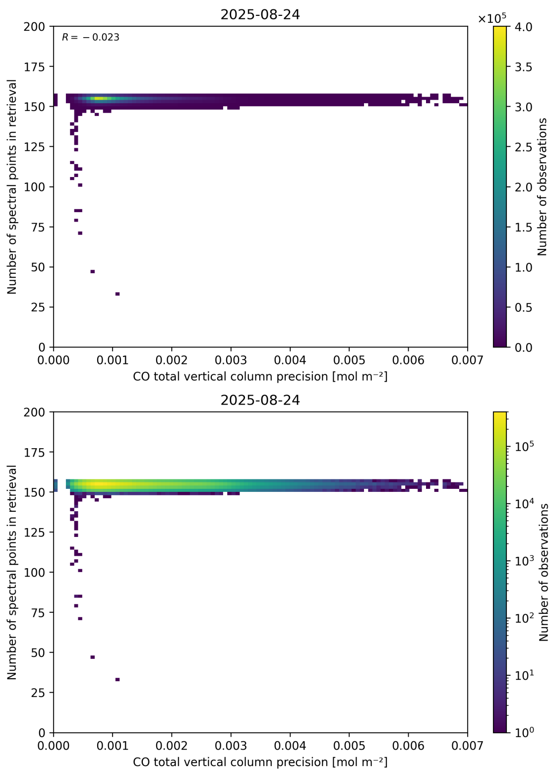
Figure 47: Scatter density plot of “CO total vertical column precision” against “Number of spectral points in retrieval” for 2025-08-23 to 2025-08-25.
