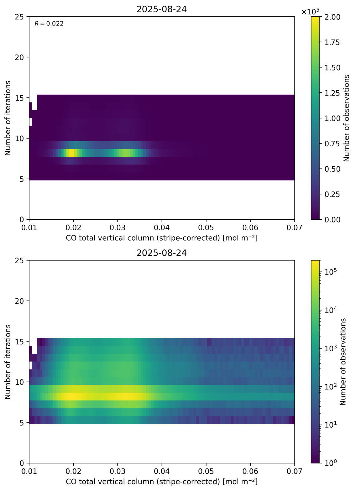
Figure 39: Scatter density plot of “CO total vertical column (stripe-corrected)” against “Number of iterations” for 2025-08-23 to 2025-08-25.
