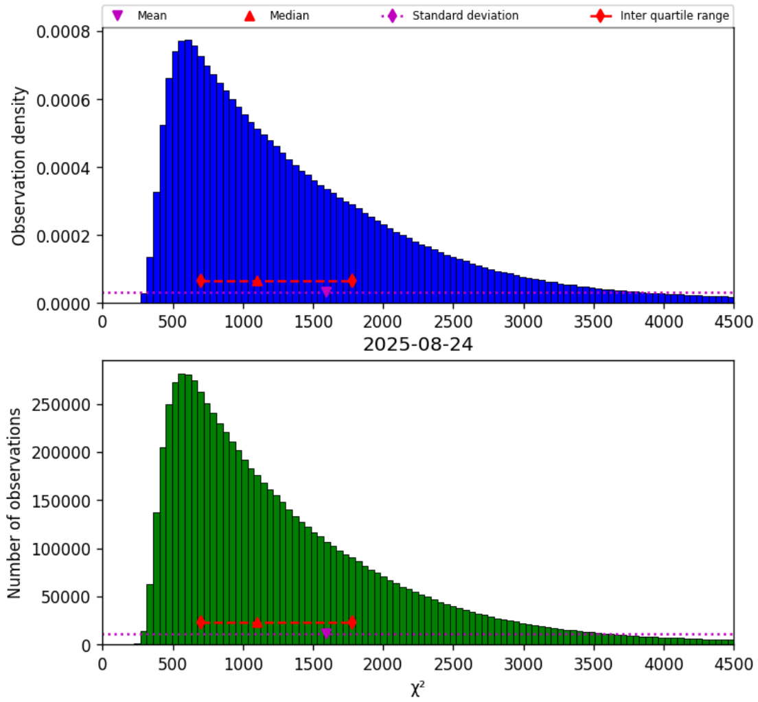
Figure 22: Histogram of " \chi^2 " for 2025-08-23 to 2025-08-25
