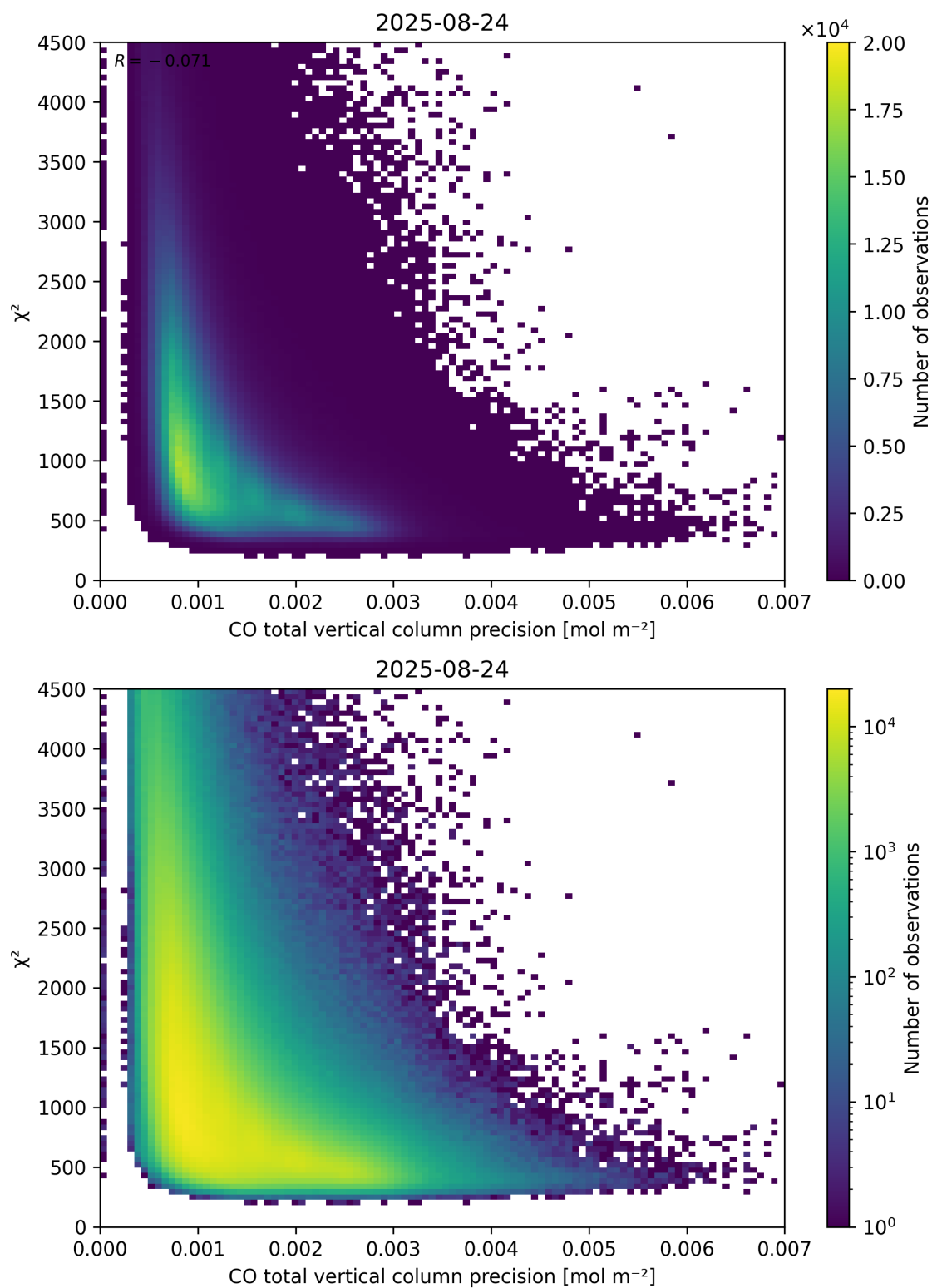
Figure 44: Scatter density plot of “CO total vertical column precision” against “ \chi^2 ” for 2025-08-23 to 2025-08-25.
