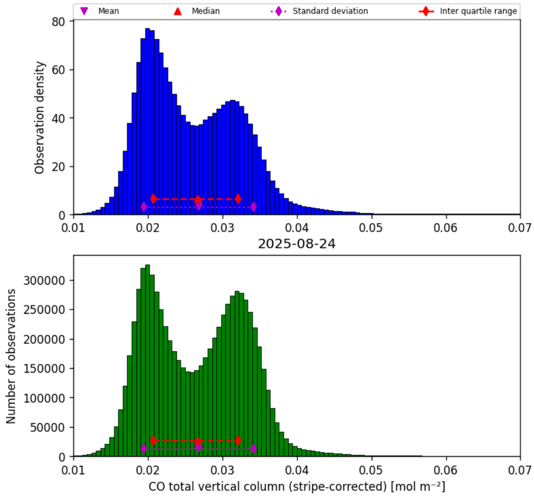
Figure 19: Histogram of “CO total vertical column (stripe-corrected)” for 2025-08-23 to 2025-08-25
