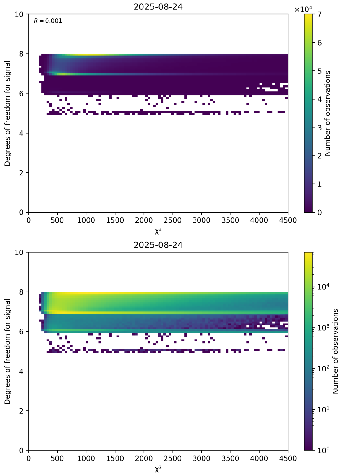
Figure 48: Scatter density plot of “ \chi^2 ” against “Degrees of freedom for signal” for 2025-08-23 to 2025-08-25.
