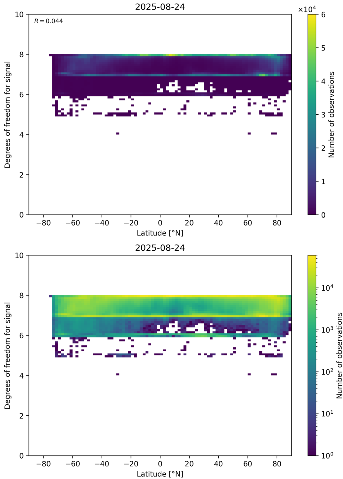
Figure 55: Scatter density plot of “Latitude” against “Degrees of freedom for signal” for 2025-08-23 to 2025-08-25.
