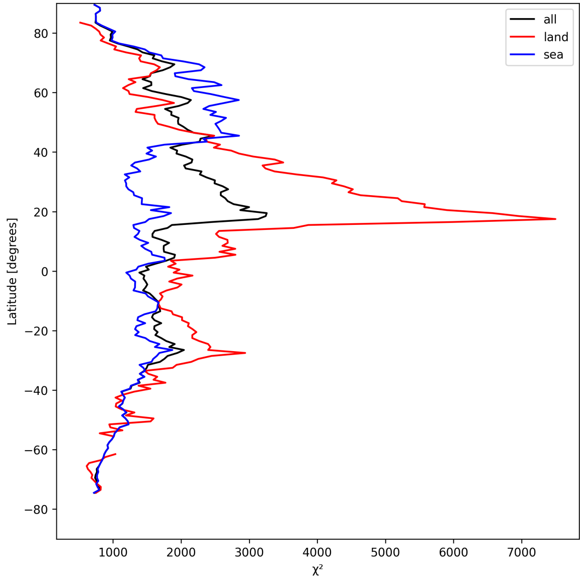
Figure 14: Zonal average of “ \chi^2 ” for 2025-08-25 to 2025-08-27.
