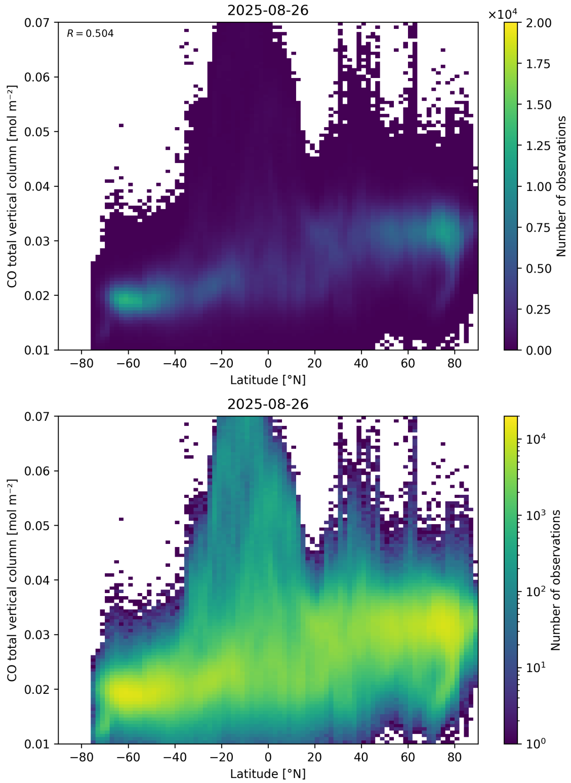
Figure 51: Scatter density plot of “Latitude” against “CO total vertical column” for 2025-08-25 to 2025-08-27.
