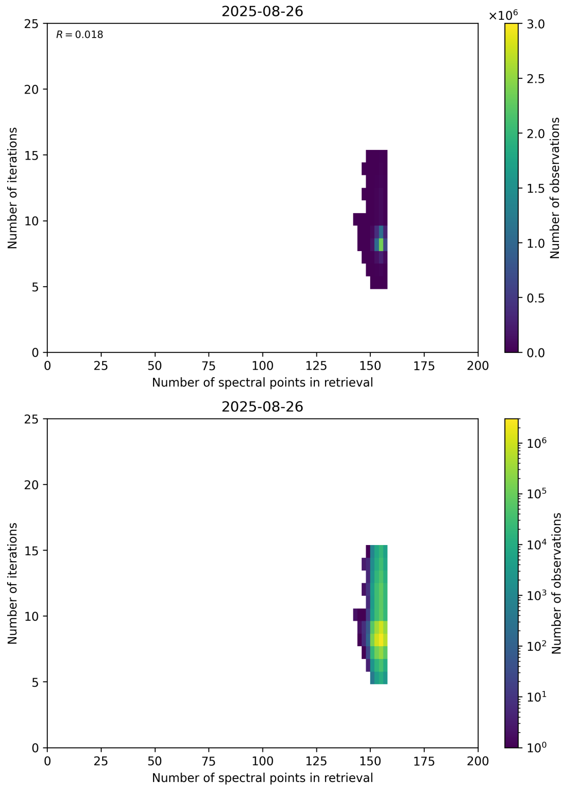
Figure 60: Scatter density plot of “Number of spectral points in retrieval” against “Number of iterations” for 2025-08-25 to 2025-08-27.
