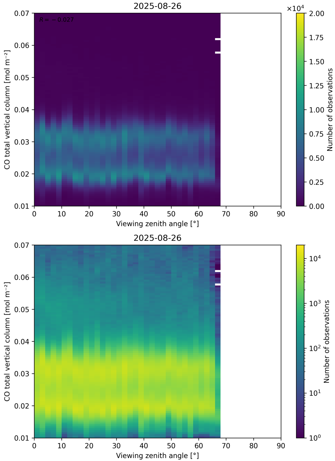
Figure 69: Scatter density plot of “Viewing zenith angle” against “CO total vertical column” for 2025-08-25 to 2025-08-27.
