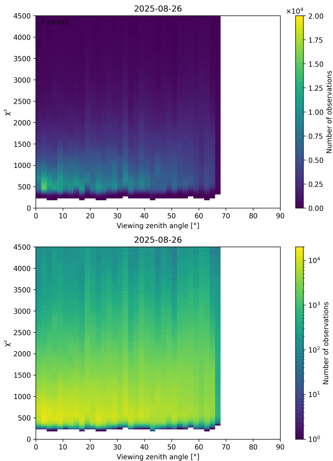
Figure 72: Scatter density plot of “Viewing zenith angle” against “ \chi^2 ” for 2025-08-25 to 2025-08-27.
