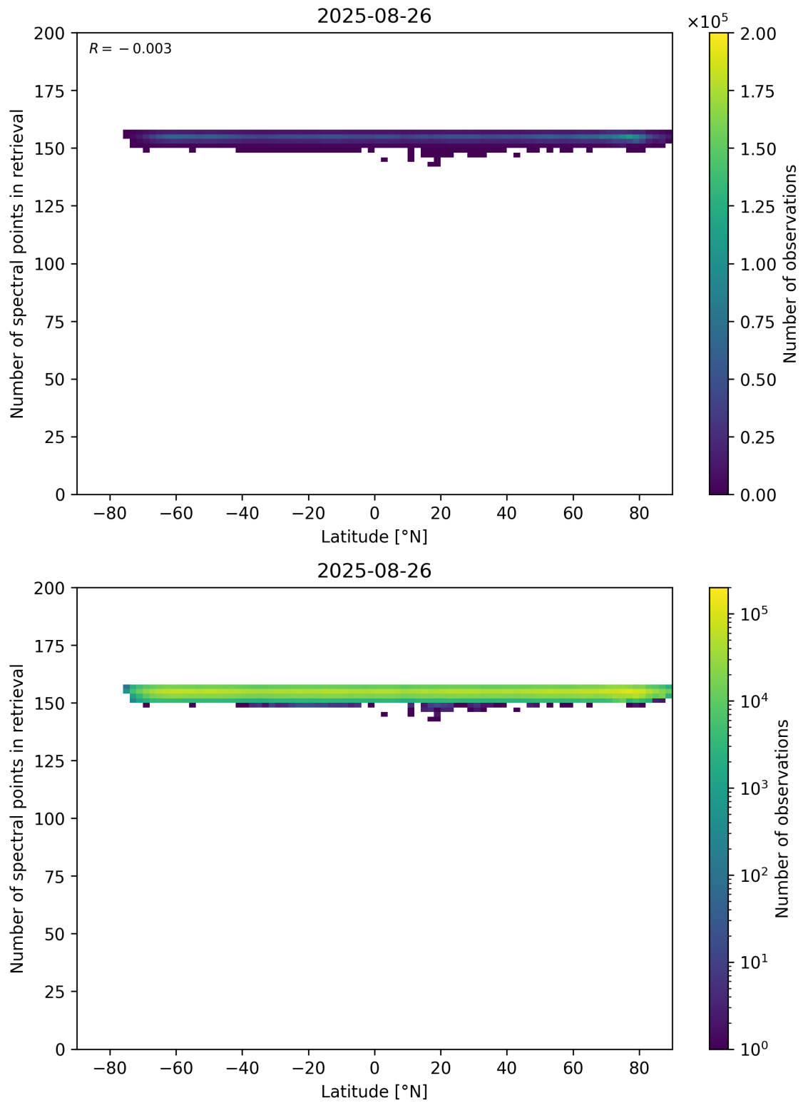
Figure 57: Scatter density plot of “Latitude” against “Number of spectral points in retrieval” for 2025-08-25 to 2025-08-27.
