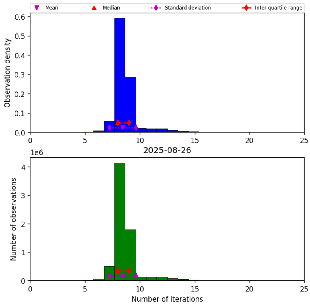
Figure 24: Histogram of “Number of iterations” for 2025-08-25 to 2025-08-27
