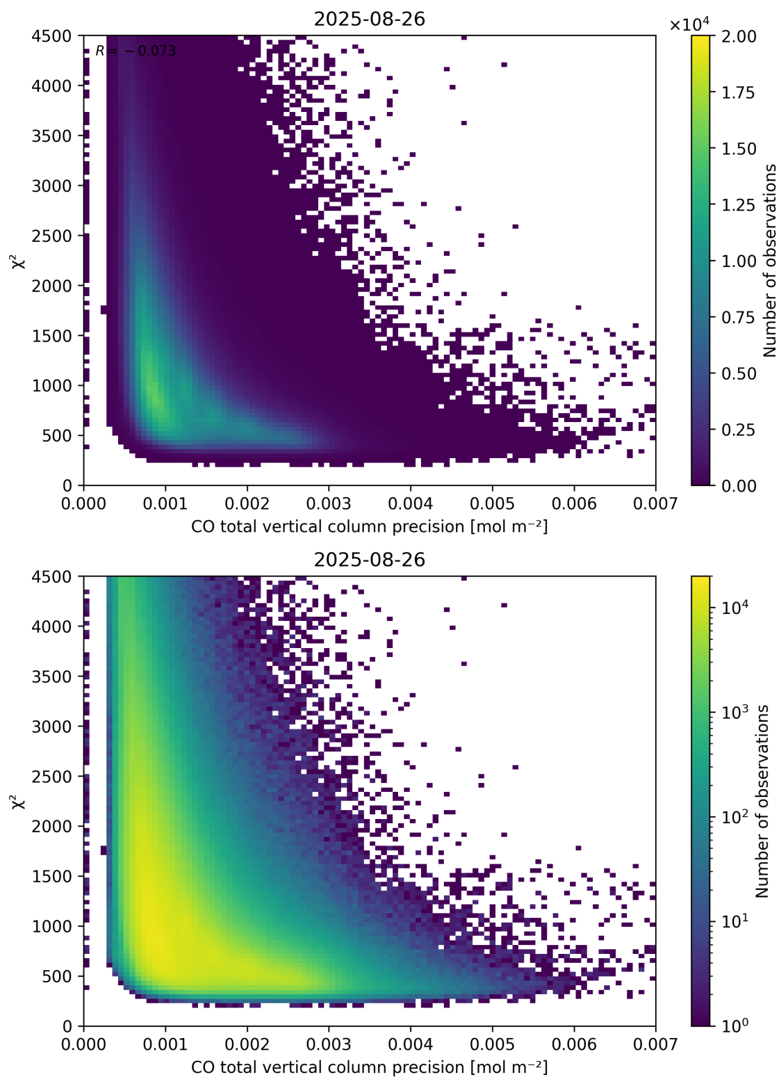
Figure 44: Scatter density plot of “CO total vertical column precision” against “ \chi^2 ” for 2025-08-25 to 2025-08-27.
