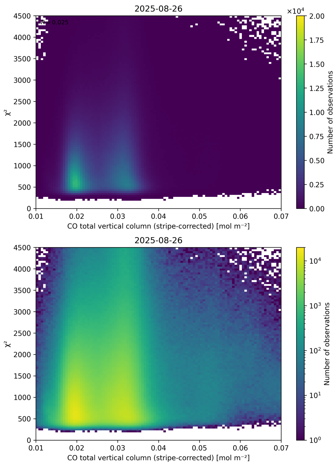
Figure 37: Scatter density plot of “CO total vertical column (stripe-corrected)” against “ \chi^2 ” for 2025-08-25 to 2025-08-27.
