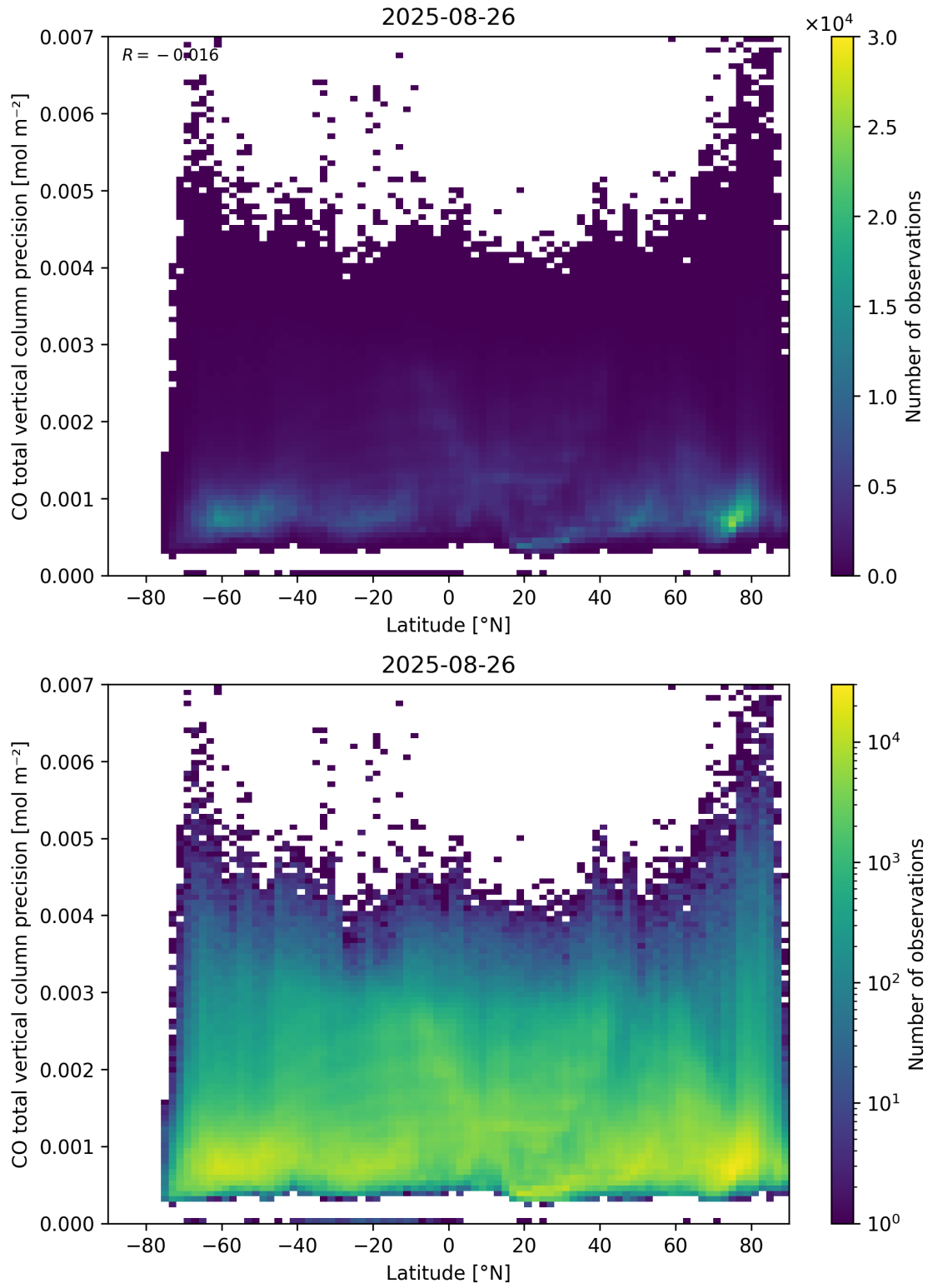
Figure 53: Scatter density plot of “Latitude” against “CO total vertical column precision” for 2025-08-25 to 2025-08-27.
