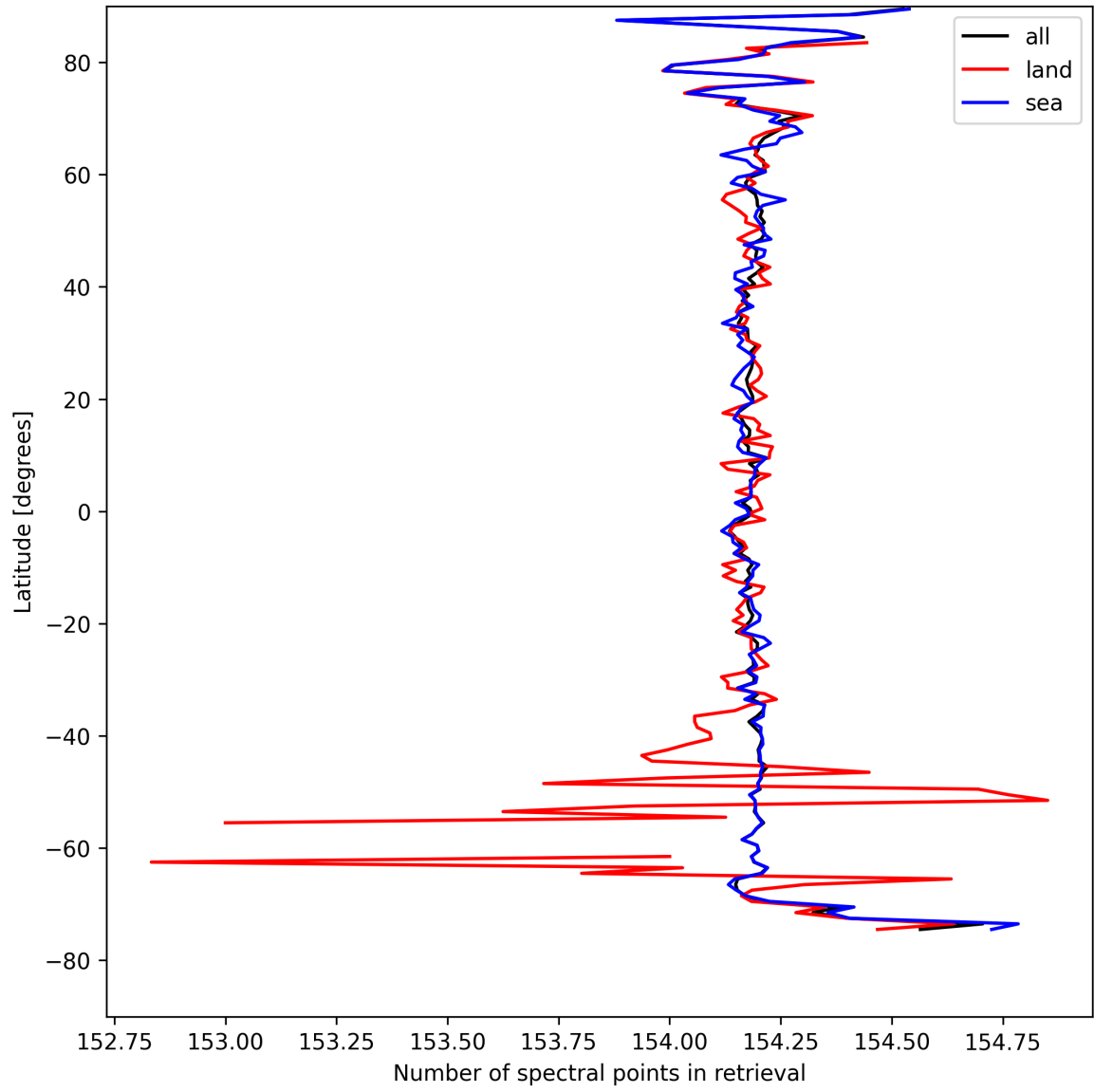
Figure 13: Zonal average of “Number of spectral points in retrieval” for 2025-08-25 to 2025-08-27.
