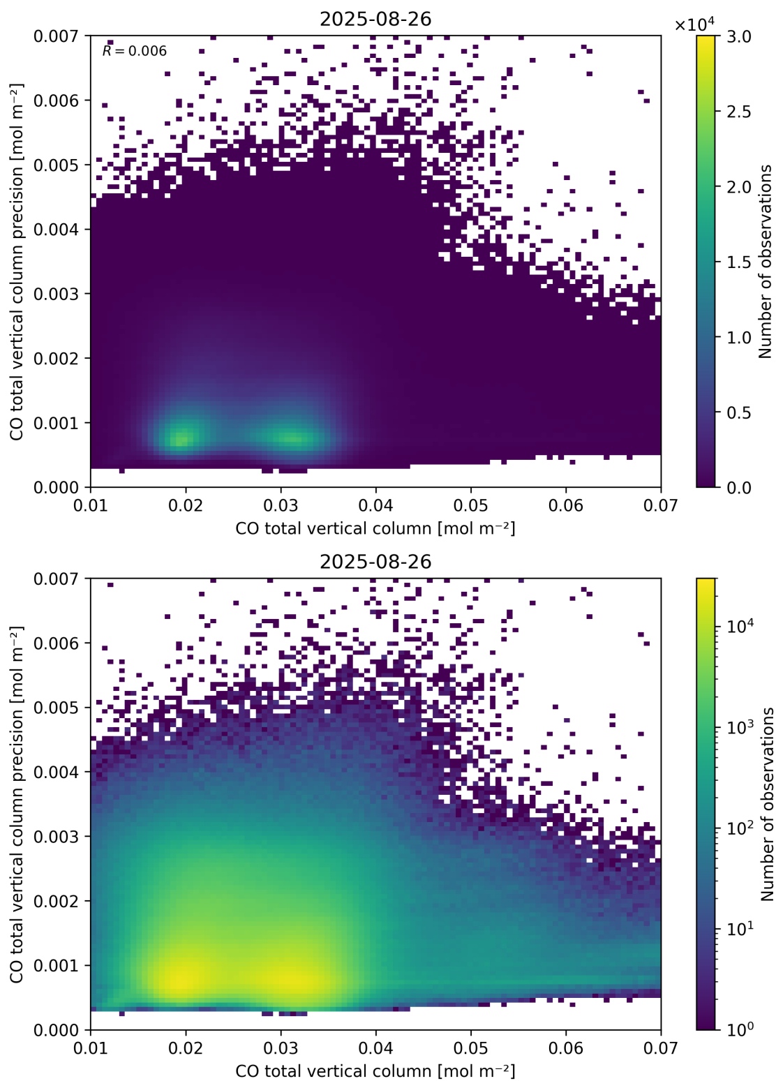
Figure 34: Scatter density plot of “CO total vertical column” against “CO total vertical column precision” for 2025-08-25 to 2025-08-27.
