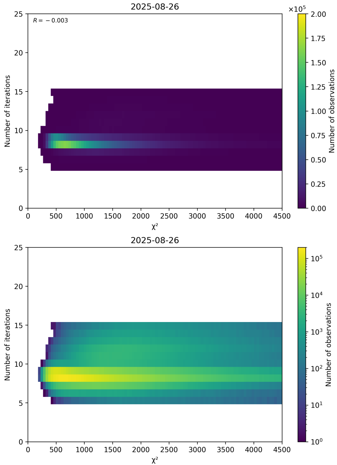
Figure 49: Scatter density plot of “ \chi^2 ” against “Number of iterations” for 2025-08-25 to 2025-08-27.
