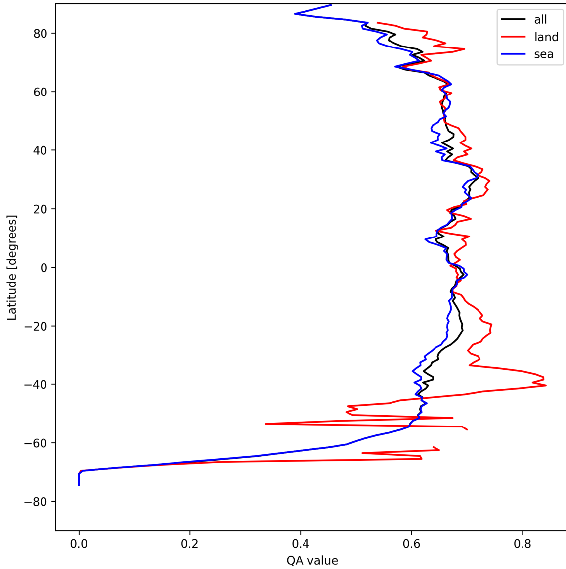
Figure 9: Zonal average of “QA value” for 2025-08-25 to 2025-08-27.
