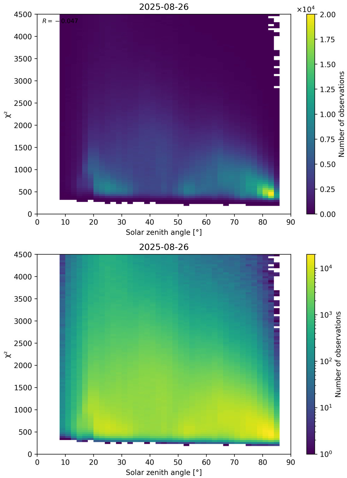
Figure 64: Scatter density plot of “Solar zenith angle” against “ \chi^2 ” for 2025-08-25 to 2025-08-27.
