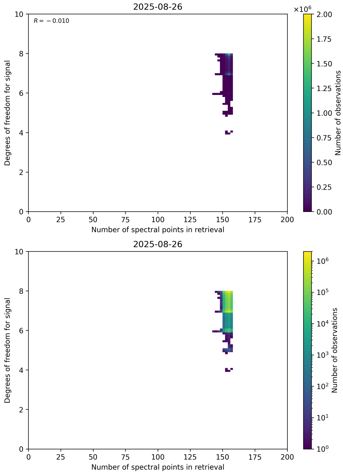
Figure 59: Scatter density plot of “Number of spectral points in retrieval” against “Degrees of freedom for signal” for 2025-08-25 to 2025-08-27.
