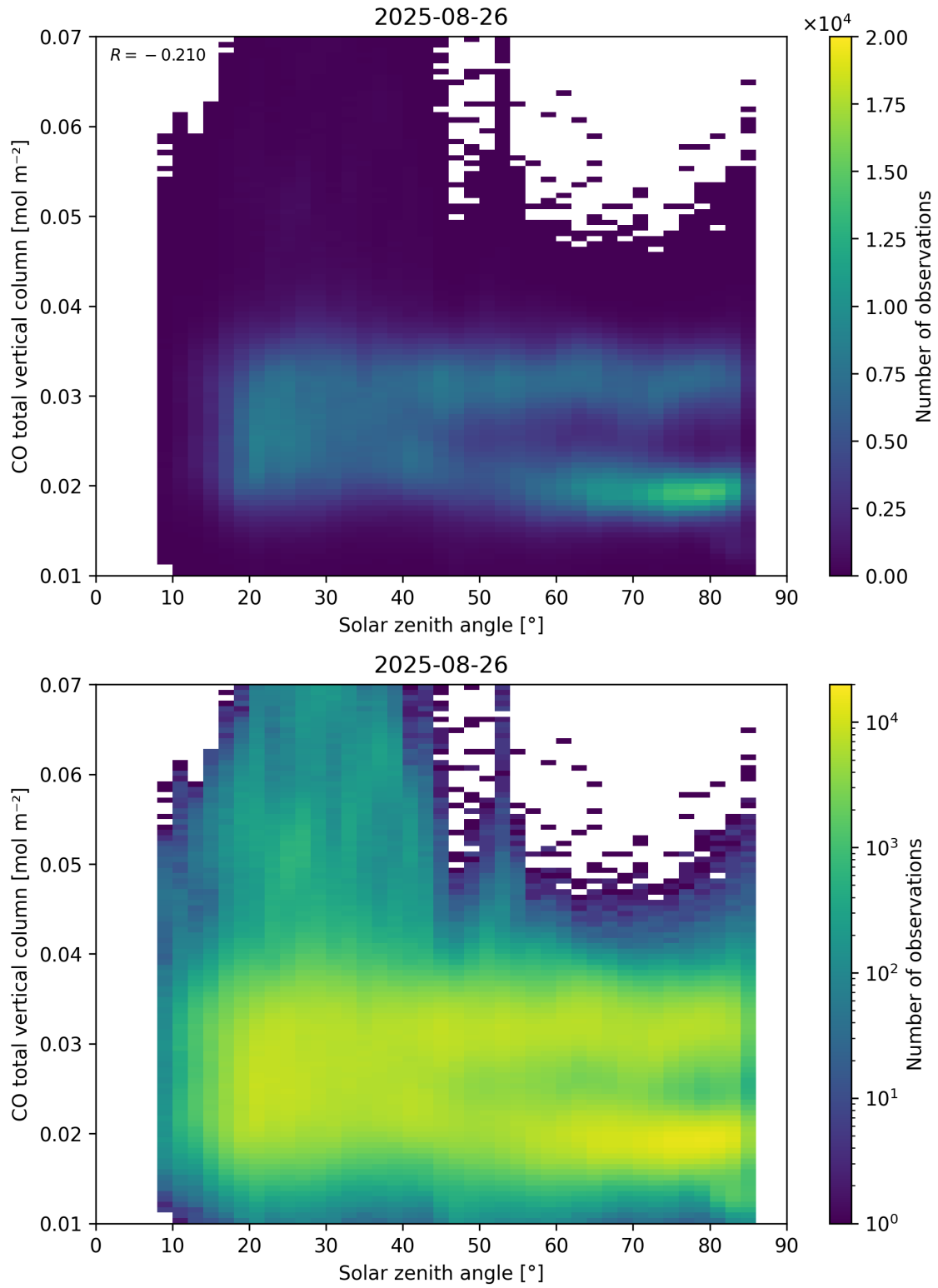
Figure 61: Scatter density plot of “Solar zenith angle” against “CO total vertical column” for 2025-08-25 to 2025-08-27.
