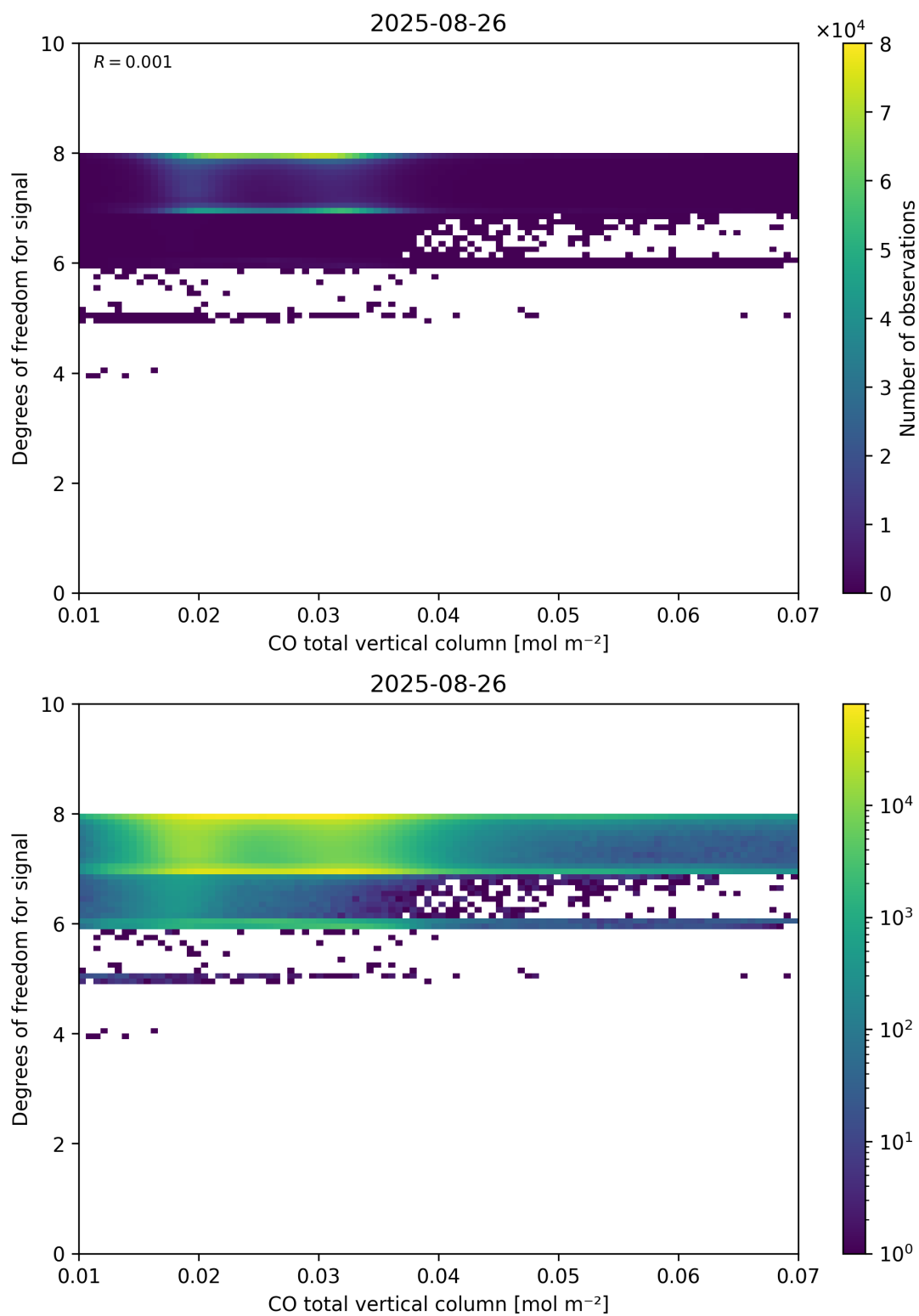
Figure 41: Scatter density plot of “CO total vertical column” against “Degrees of freedom for signal” for 2025-08-25 to 2025-08-27.
