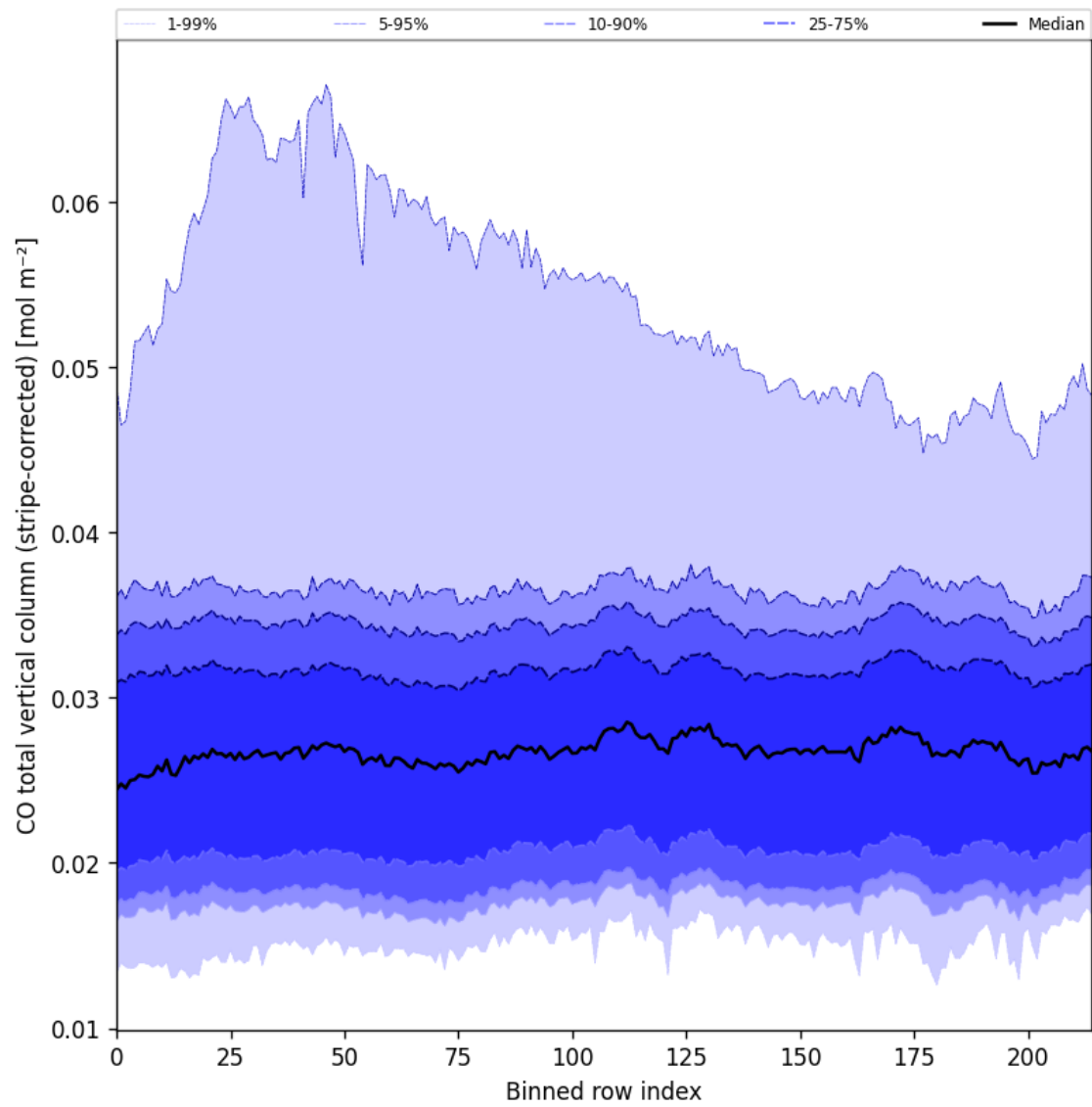
Figure 27: Along track statistics of “CO total vertical column (stripe-corrected)” for 2025-08-25 to 2025-08-27
