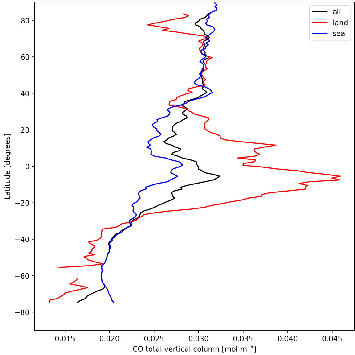
Figure 10: Zonal average of “CO total vertical column” for 2025-08-25 to 2025-08-27.
