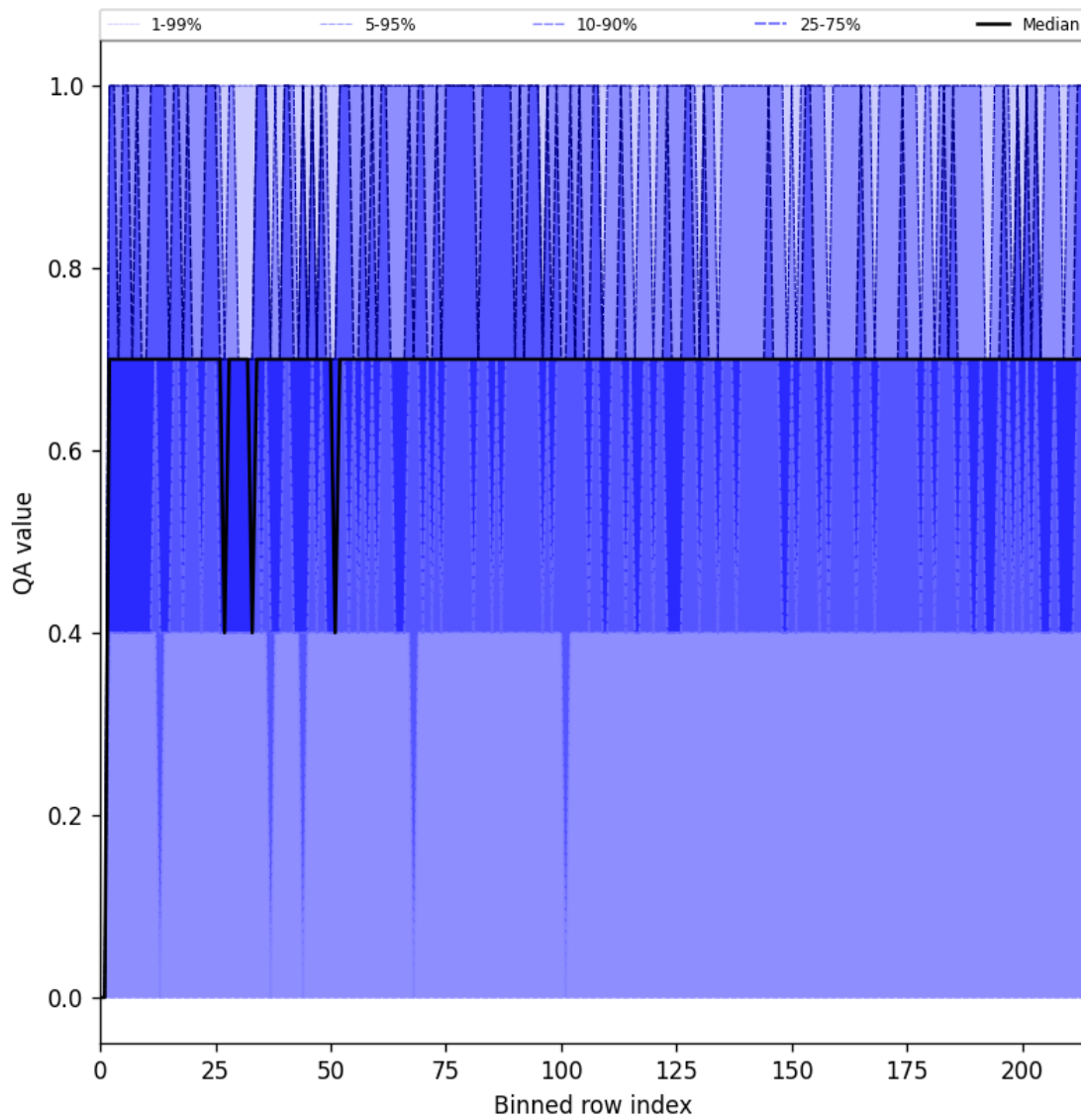
Figure 25: Along track statistics of “QA value” for 2025-08-25 to 2025-08-27
