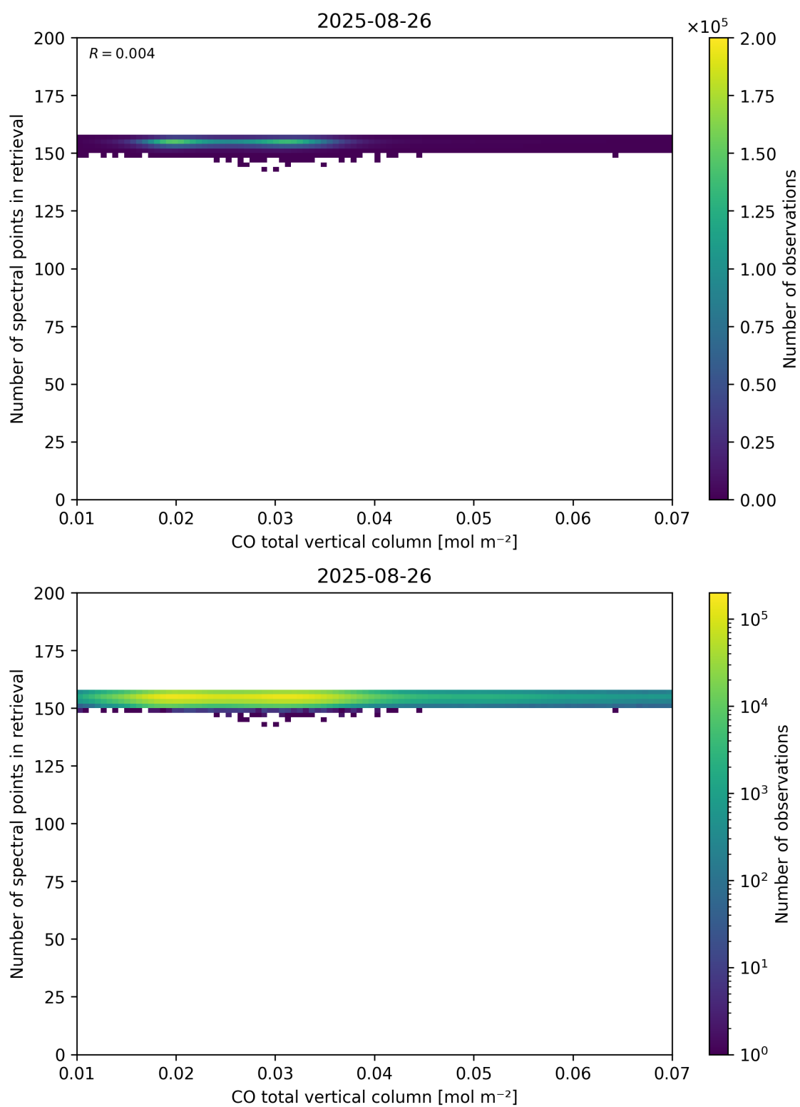
Figure 43: Scatter density plot of “CO total vertical column” against “Number of spectral points in retrieval” for 2025-08-25 to 2025-08-27.
