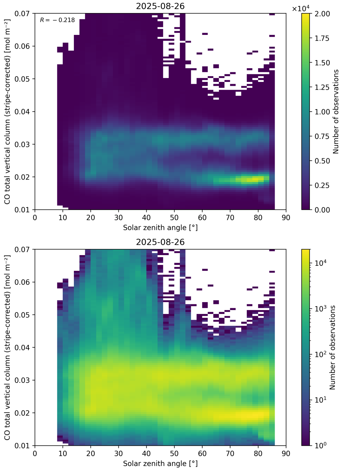
Figure 62: Scatter density plot of “Solar zenith angle” against “CO total vertical column (stripe-corrected)” for 2025-08-25 to 2025-08-27.
