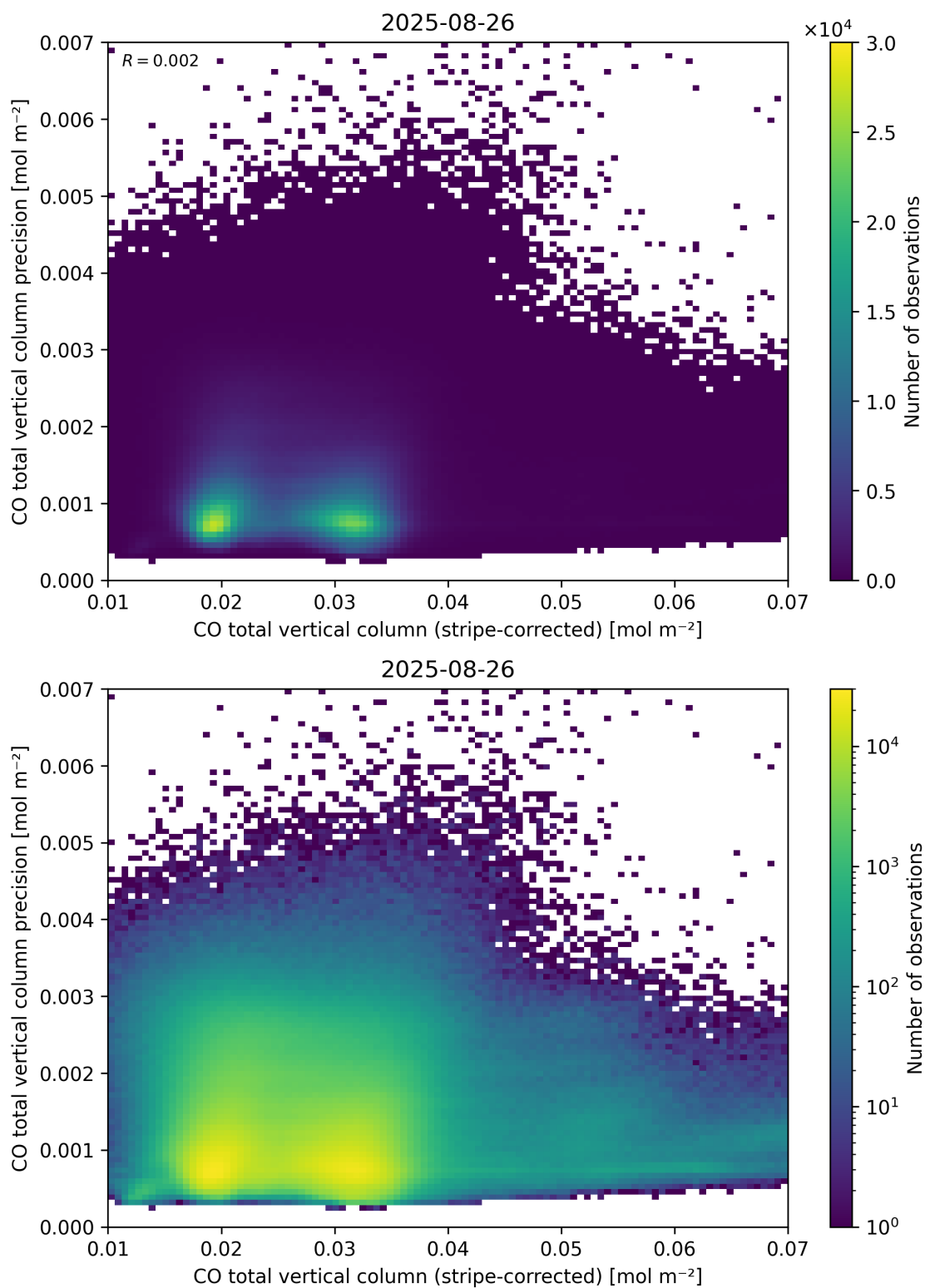
Figure 36: Scatter density plot of “CO total vertical column (stripe-corrected)” against “CO total vertical column precision” for 2025-08-25 to 2025-08-27.
