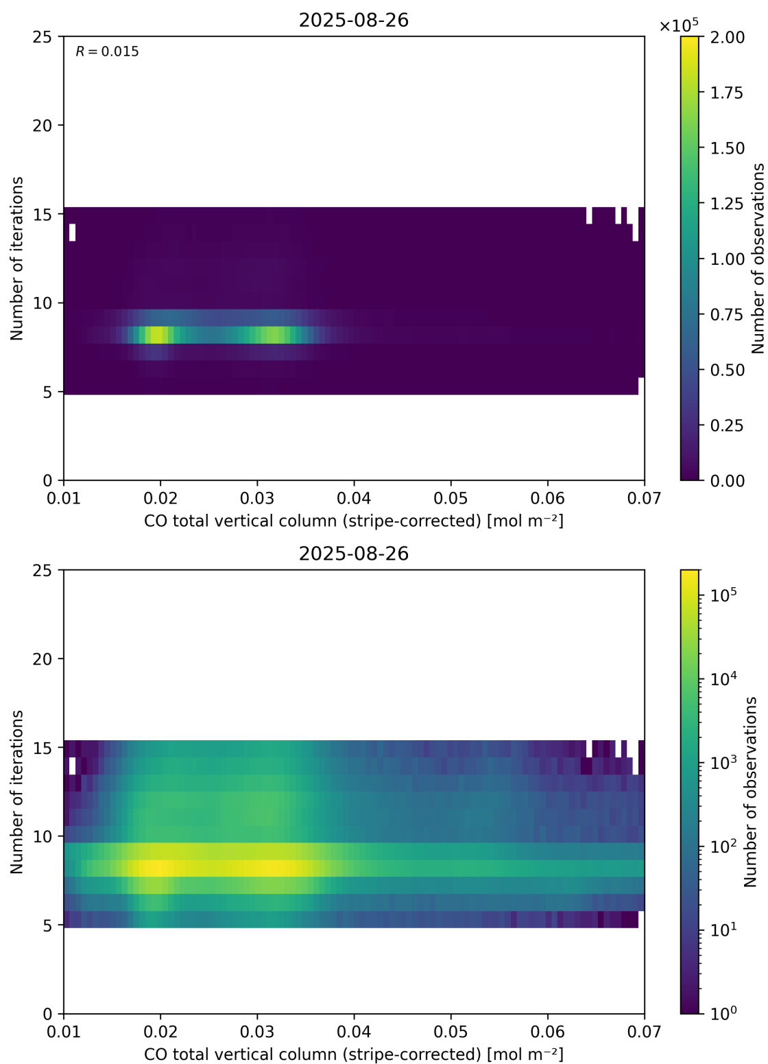
Figure 39: Scatter density plot of “CO total vertical column (stripe-corrected)” against “Number of iterations” for 2025-08-25 to 2025-08-27.
