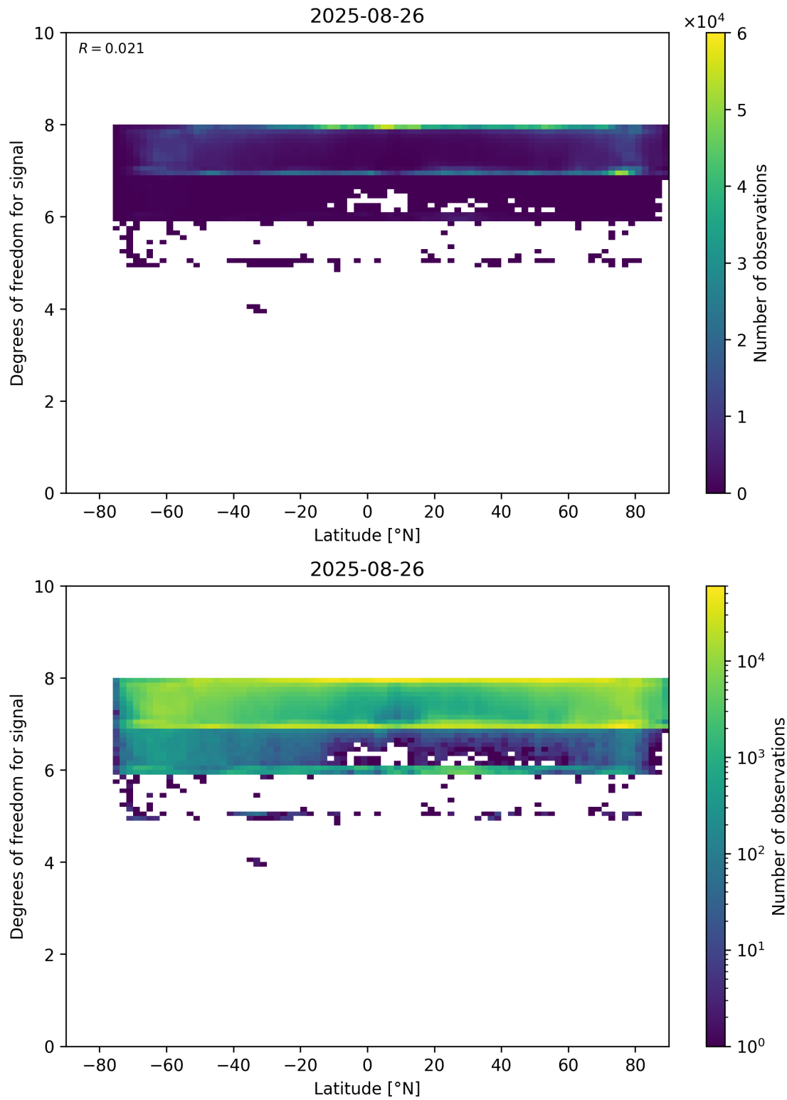
Figure 55: Scatter density plot of “Latitude” against “Degrees of freedom for signal” for 2025-08-25 to 2025-08-27.
