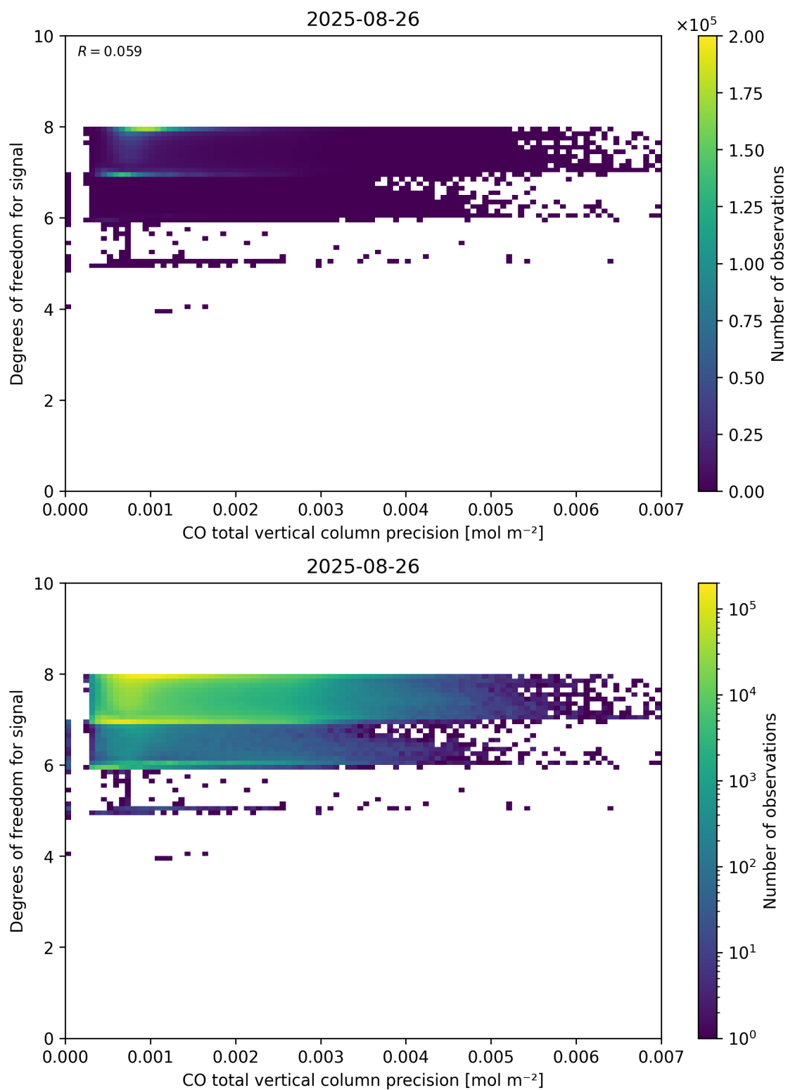
Figure 45: Scatter density plot of “CO total vertical column precision” against “Degrees of freedom for signal” for 2025-08-25 to 2025-08-27.
