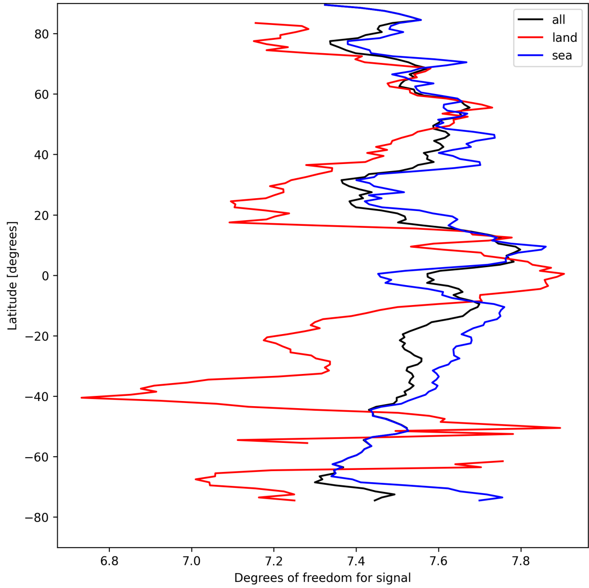
Figure 15: Zonal average of “Degrees of freedom for signal” for 2025-08-25 to 2025-08-27.
