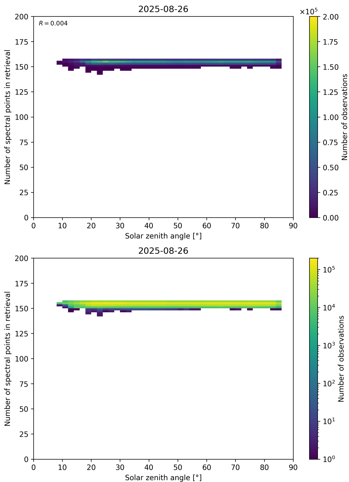
Figure 68: Scatter density plot of “Solar zenith angle” against “Number of spectral points in retrieval” for 2025-08-25 to 2025-08-27.
