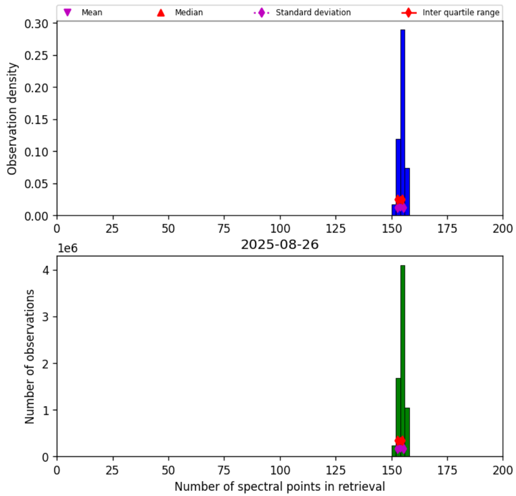
Figure 21: Histogram of “Number of spectral points in retrieval” for 2025-08-25 to 2025-08-27
