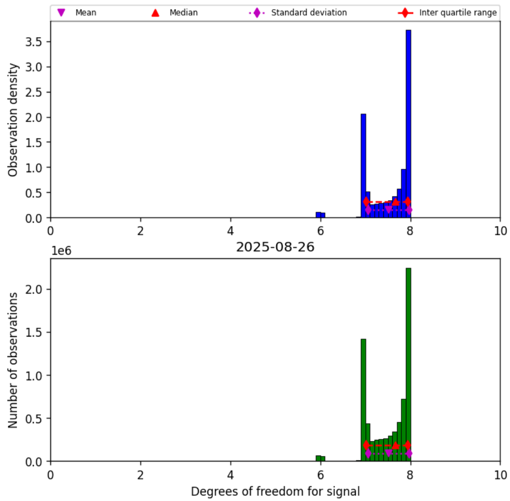
Figure 23: Histogram of “Degrees of freedom for signal” for 2025-08-25 to 2025-08-27
