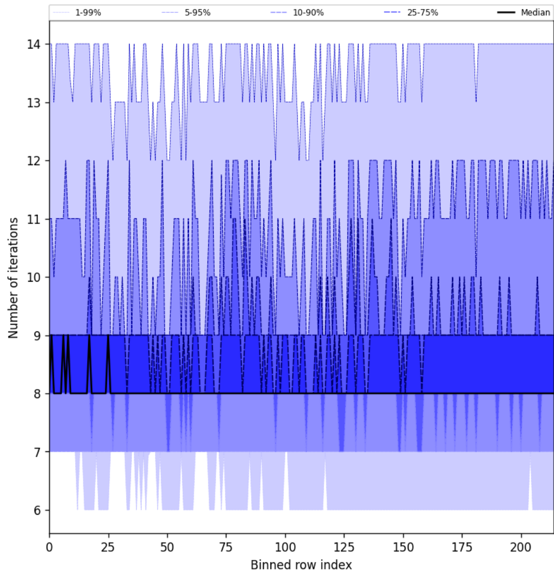
Figure 32: Along track statistics of “Number of iterations” for 2025-08-25 to 2025-08-27
