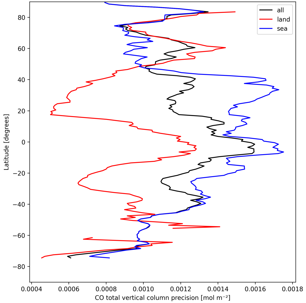
Figure 12: Zonal average of "CO total vertical column precision" for 2025-08-25 to 2025-08-27.
