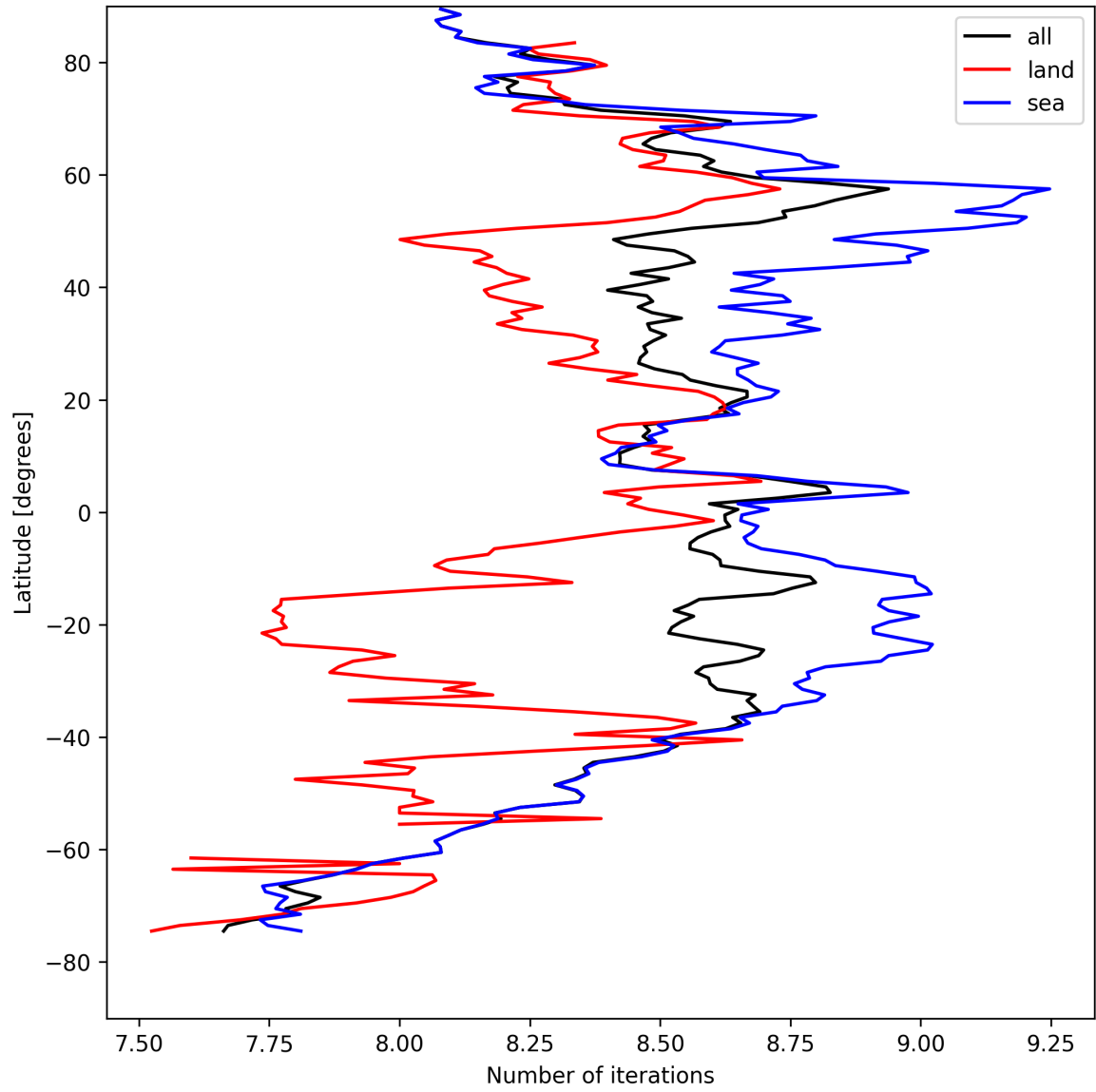
Figure 16: Zonal average of “Number of iterations” for 2025-08-25 to 2025-08-27.
