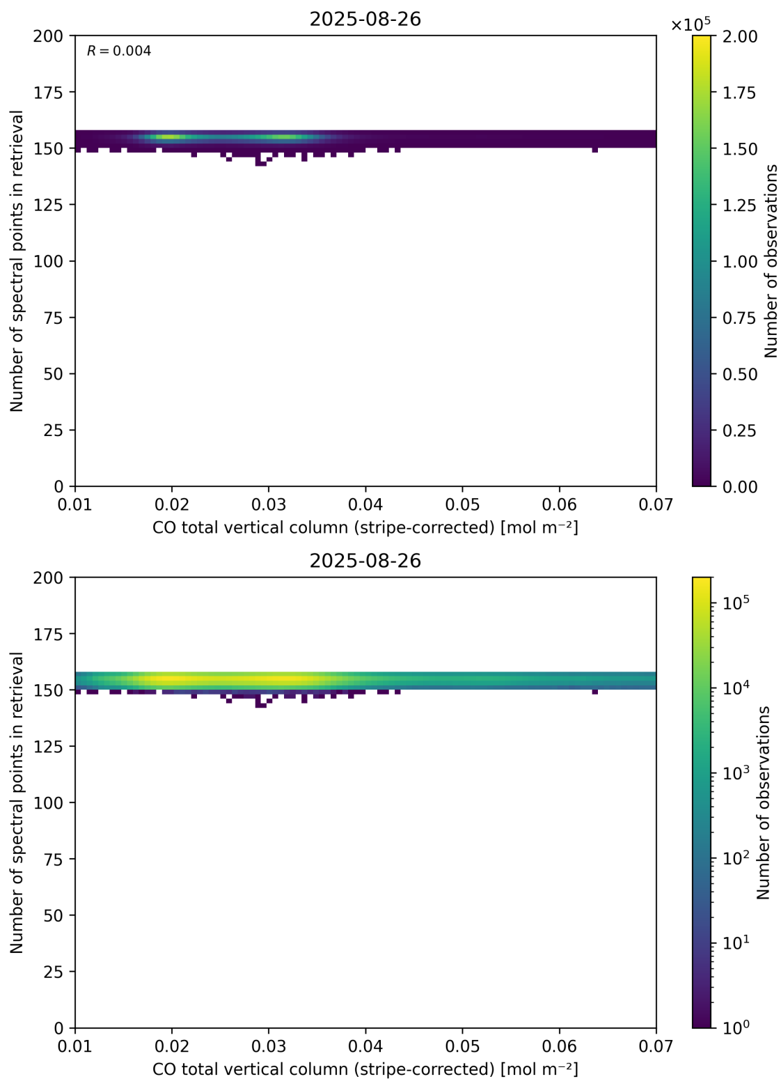
Figure 40: Scatter density plot of “CO total vertical column (stripe-corrected)” against “Number of spectral points in retrieval” for 2025-08-25 to 2025-08-27.
