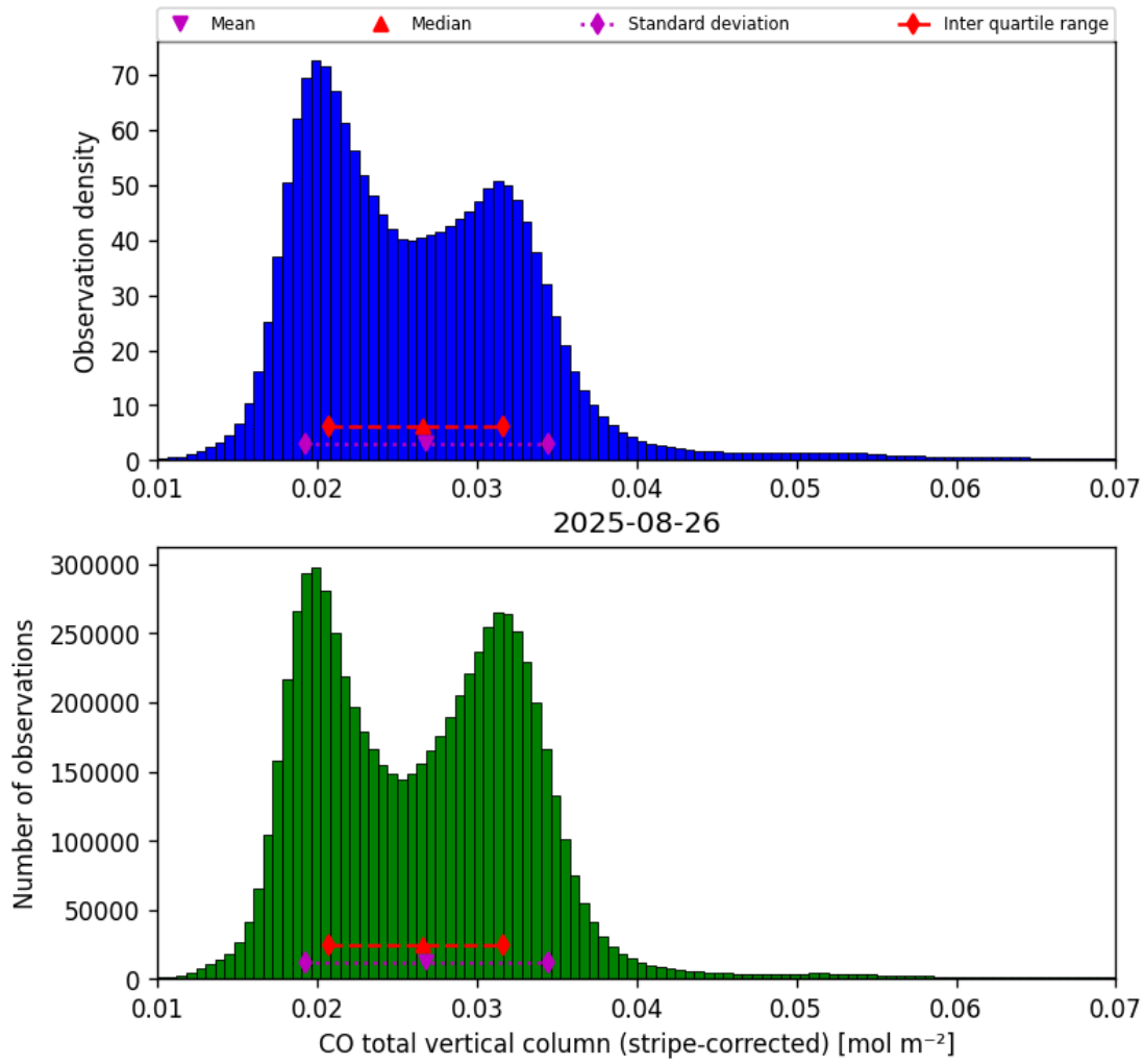
Figure 19: Histogram of “CO total vertical column (stripe-corrected)” for 2025-08-25 to 2025-08-27
