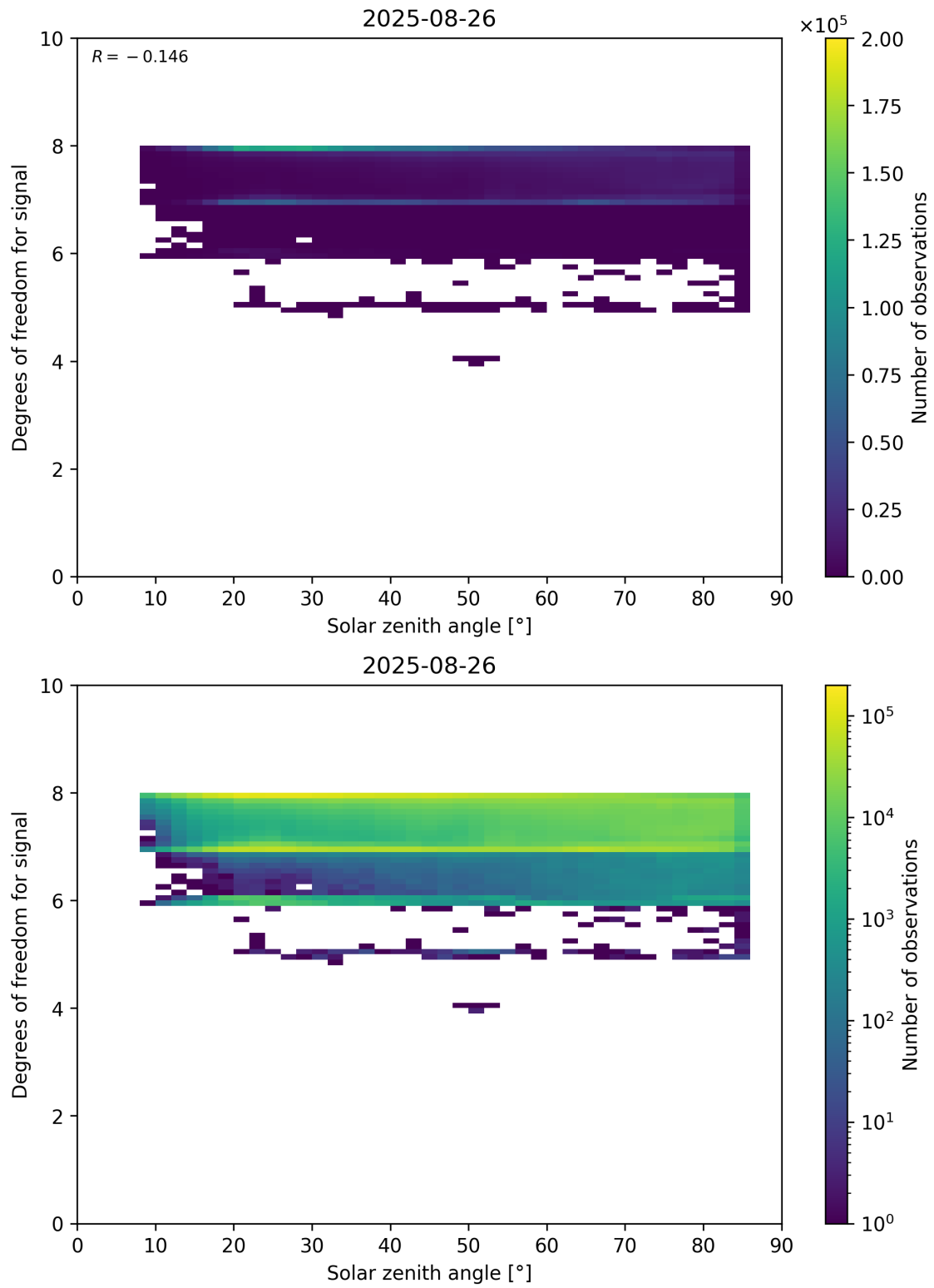
Figure 65: Scatter density plot of “Solar zenith angle” against “Degrees of freedom for signal” for 2025-08-25 to 2025-08-27.
