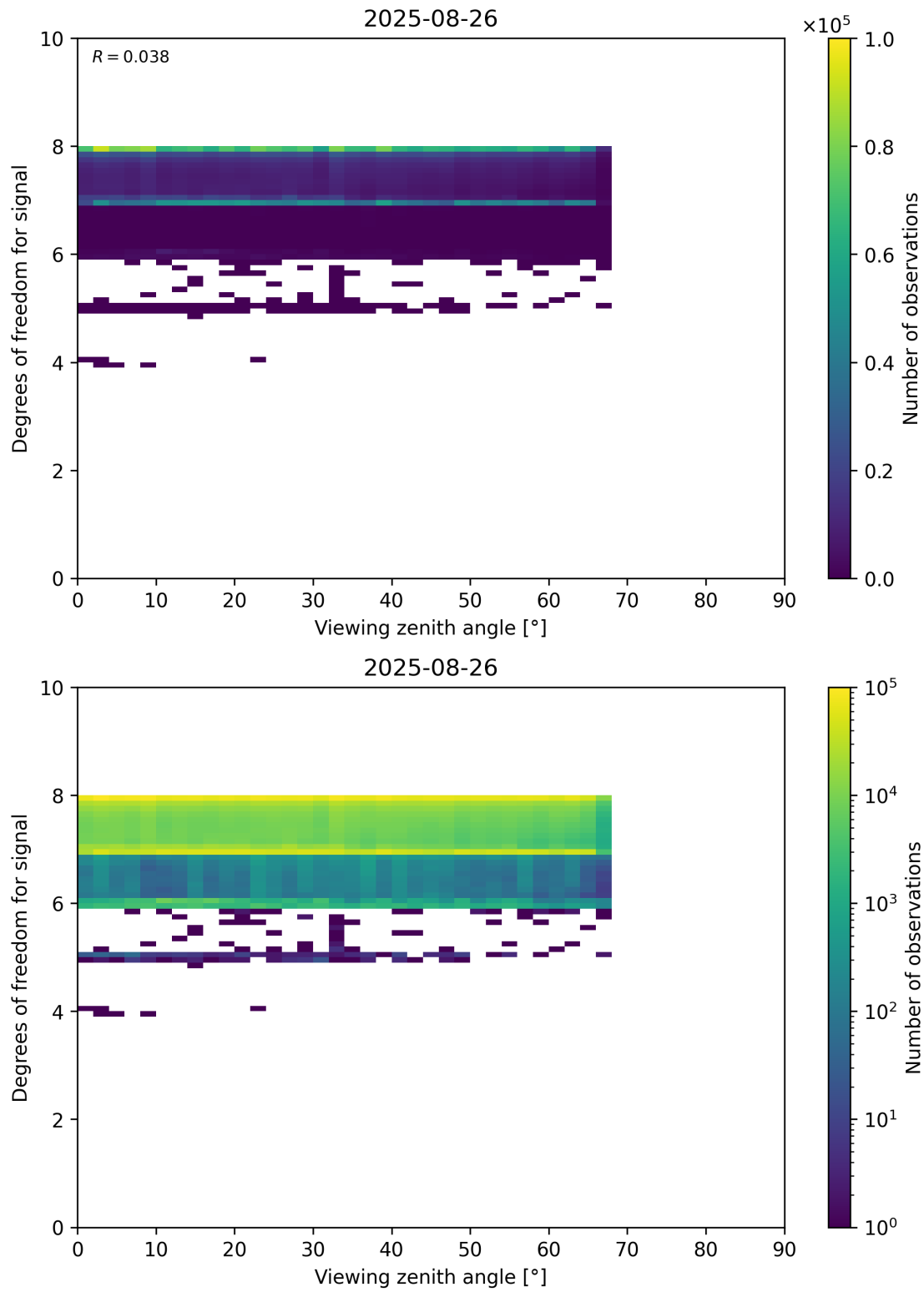
Figure 73: Scatter density plot of “Viewing zenith angle” against “Degrees of freedom for signal” for 2025-08-25 to 2025-08-27.
