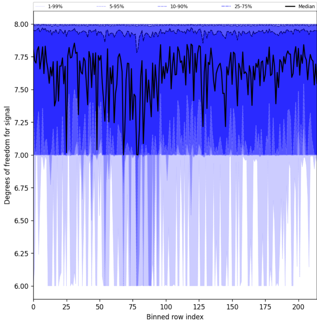
Figure 31: Along track statistics of “Degrees of freedom for signal” for 2025-08-25 to 2025-08-27
