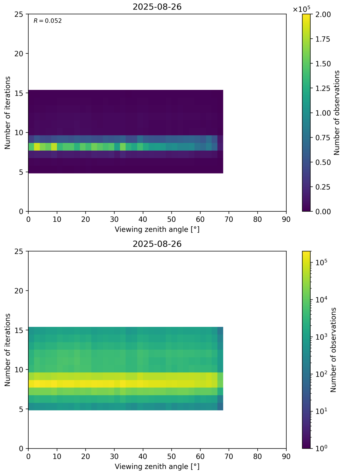
Figure 75: Scatter density plot of “Viewing zenith angle” against “Number of iterations” for 2025-08-25 to 2025-08-27.
