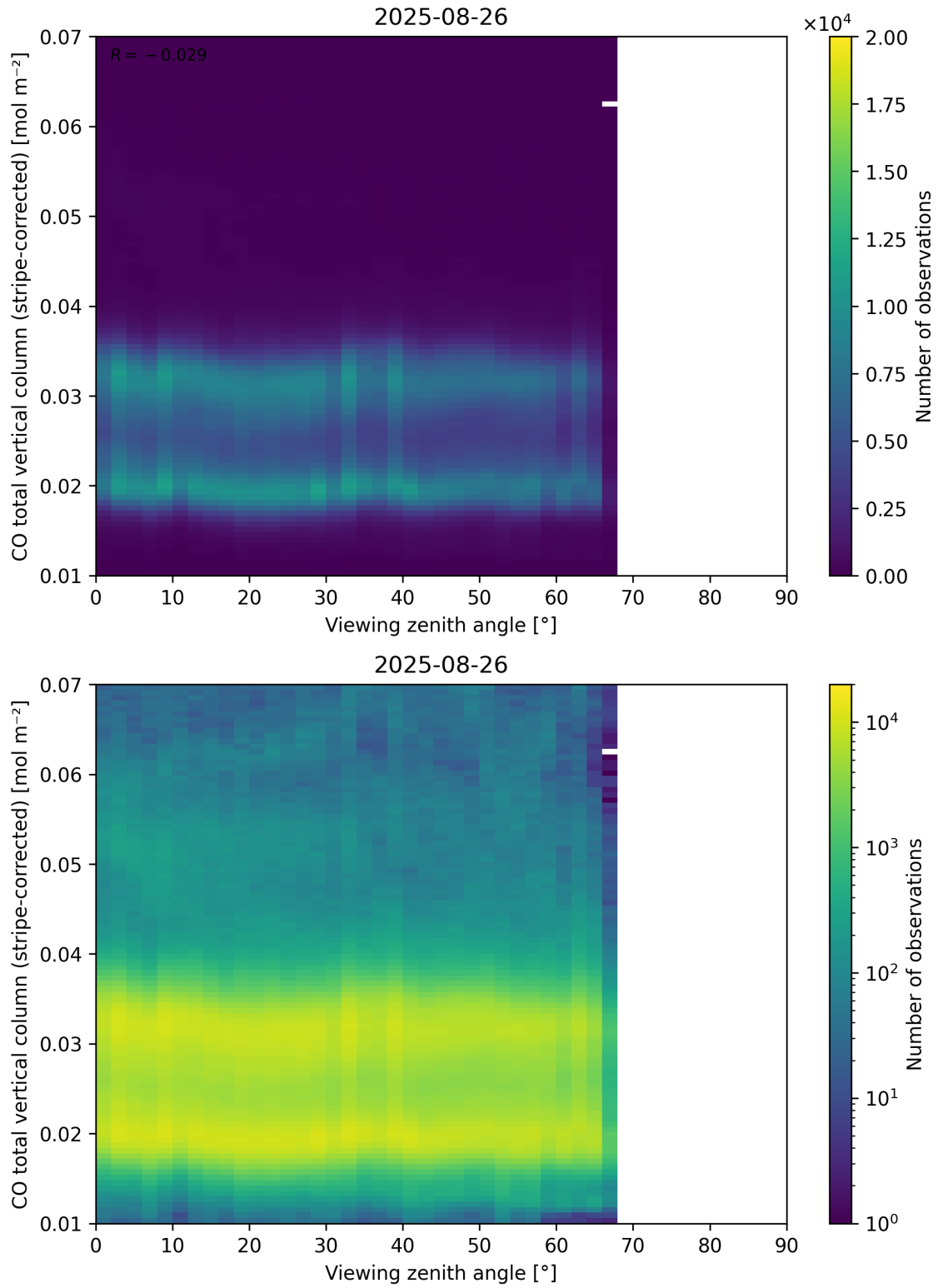
Figure 70: Scatter density plot of “Viewing zenith angle” against “CO total vertical column (stripe-corrected)” for 2025-08-25 to 2025-08-27.
