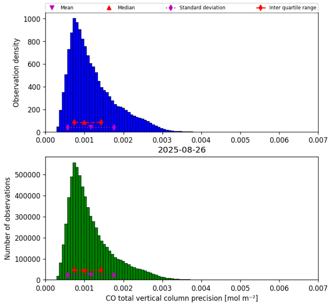
Figure 20: Histogram of “CO total vertical column precision” for 2025-08-25 to 2025-08-27
