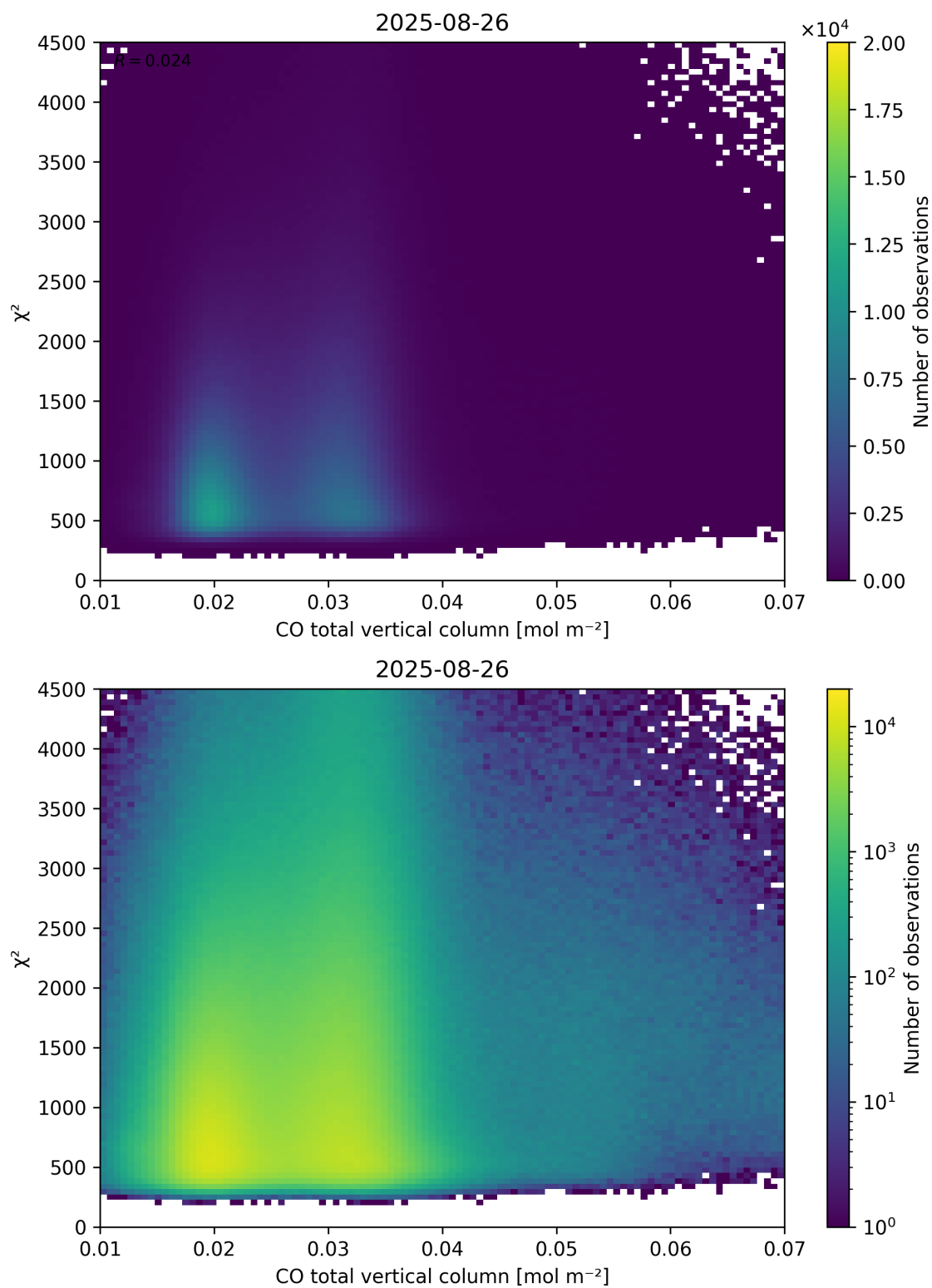
Figure 35: Scatter density plot of “CO total vertical column” against “ \chi^2 ” for 2025-08-25 to 2025-08-27.
