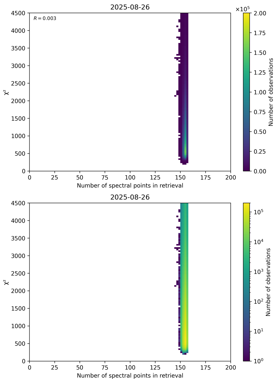
Figure 58: Scatter density plot of “Number of spectral points in retrieval” against “ \chi^2 ” for 2025-08-25 to 2025-08-27.
