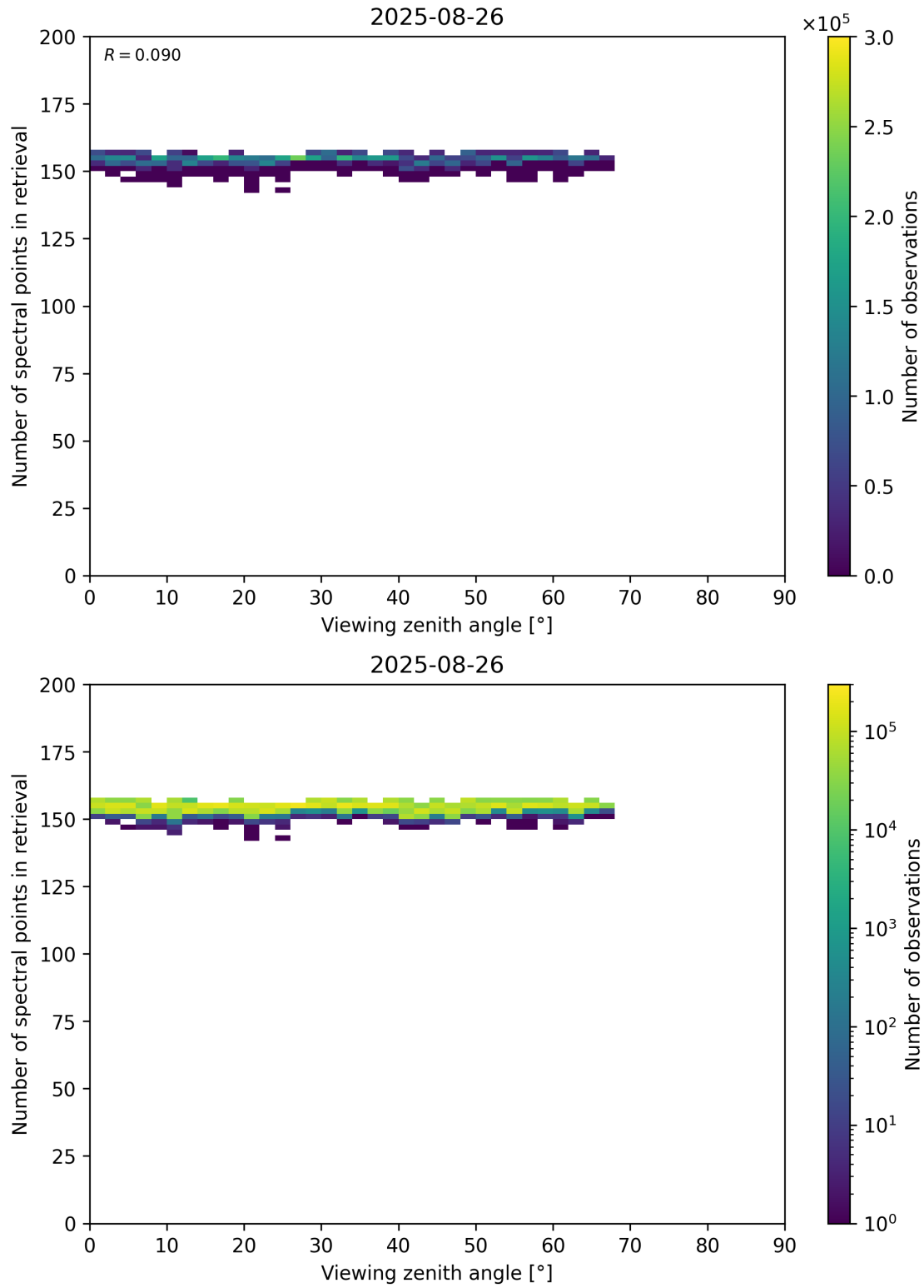
Figure 76: Scatter density plot of “Viewing zenith angle” against “Number of spectral points in retrieval” for 2025-08-25 to 2025-08-27.
