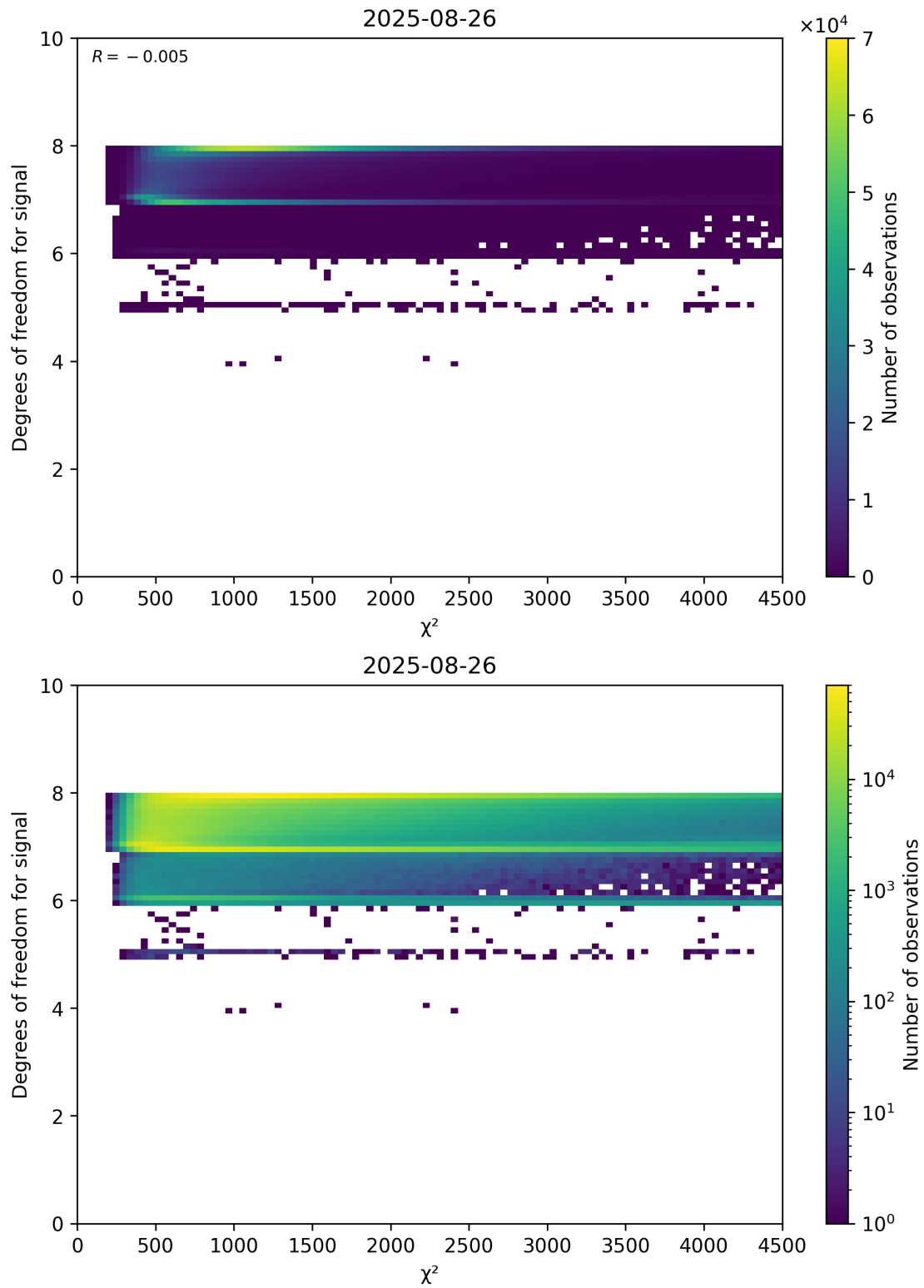
Figure 48: Scatter density plot of “ \chi^2 ” against “Degrees of freedom for signal” for 2025-08-25 to 2025-08-27.
