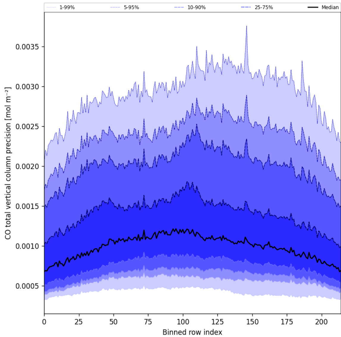
Figure 28: Along track statistics of “CO total vertical column precision” for 2025-08-25 to 2025-08-27
