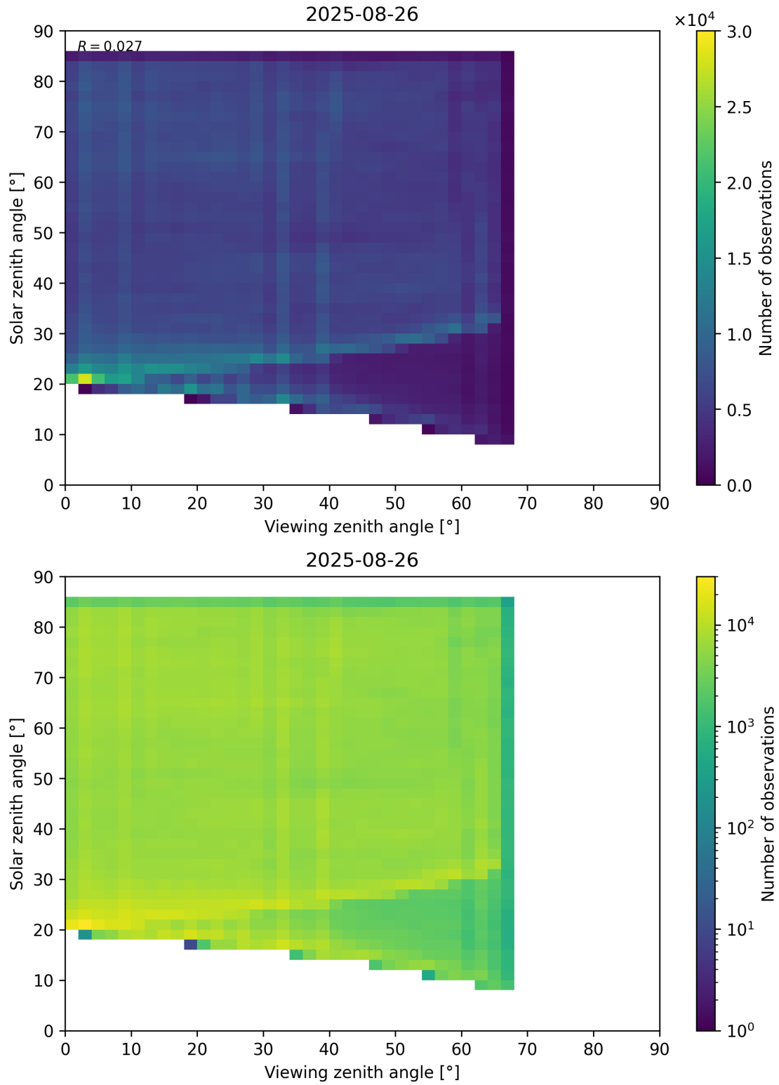
Figure 77: Scatter density plot of “Viewing zenith angle” against “Solar zenith angle” for 2025-08-25 to 2025-08-27.
