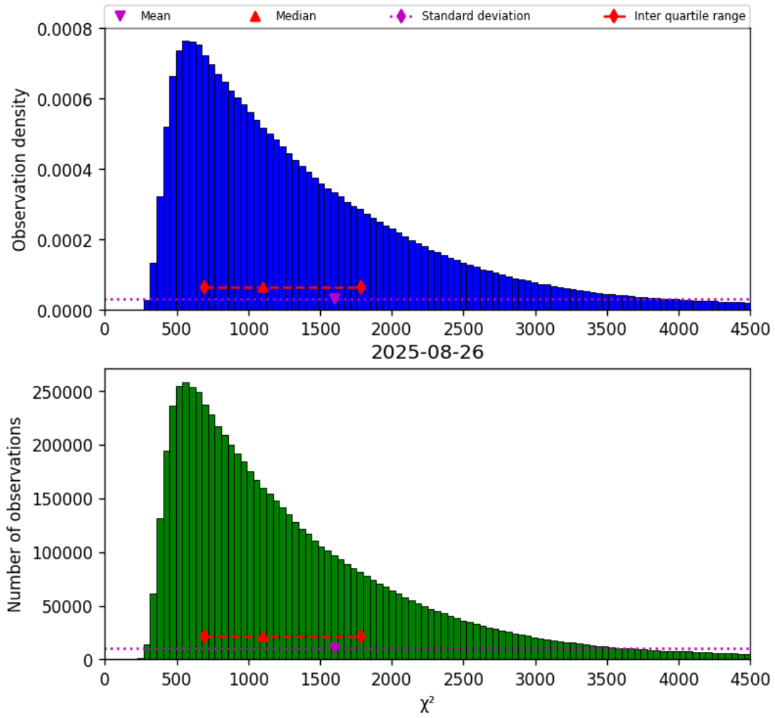
Figure 22: Histogram of “ \chi^2 ” for 2025-08-25 to 2025-08-27
