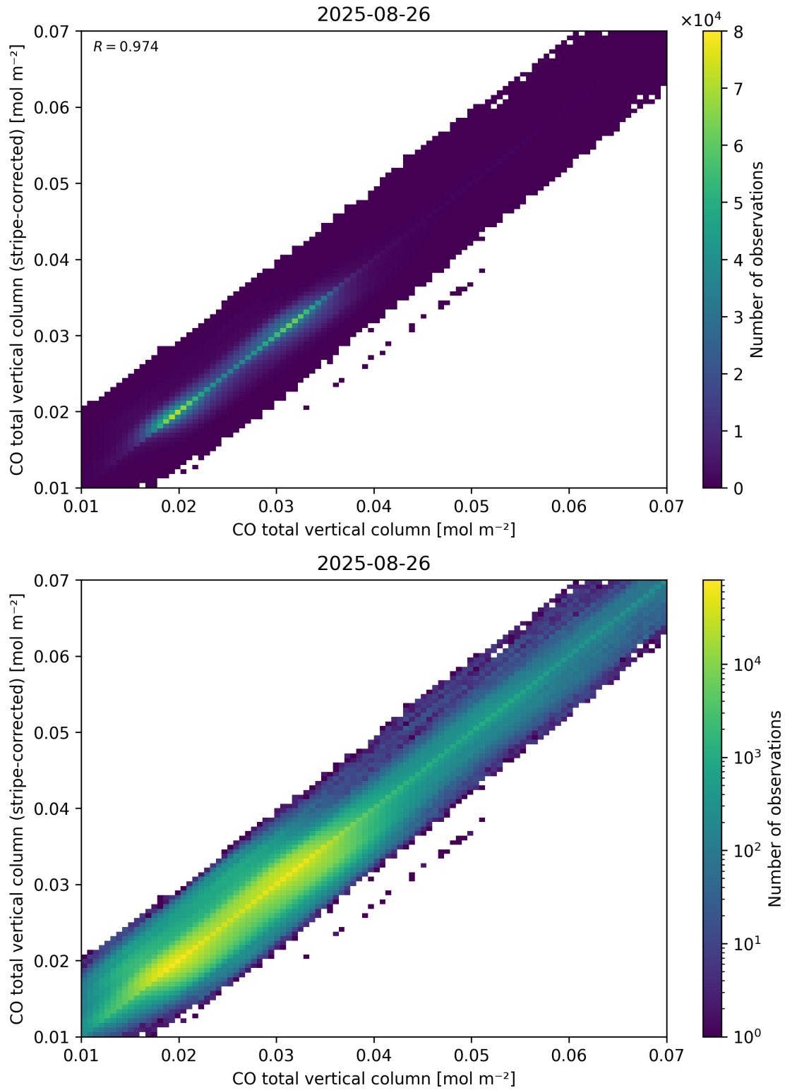
Figure 33: Scatter density plot of “CO total vertical column” against “CO total vertical column (stripe-corrected)” for 2025-08-25 to 2025-08-27.
