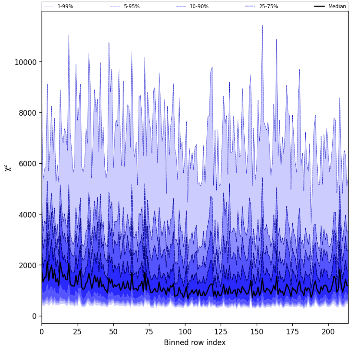
Figure 30: Along track statistics of “ \chi^2 ” for 2025-08-25 to 2025-08-27
