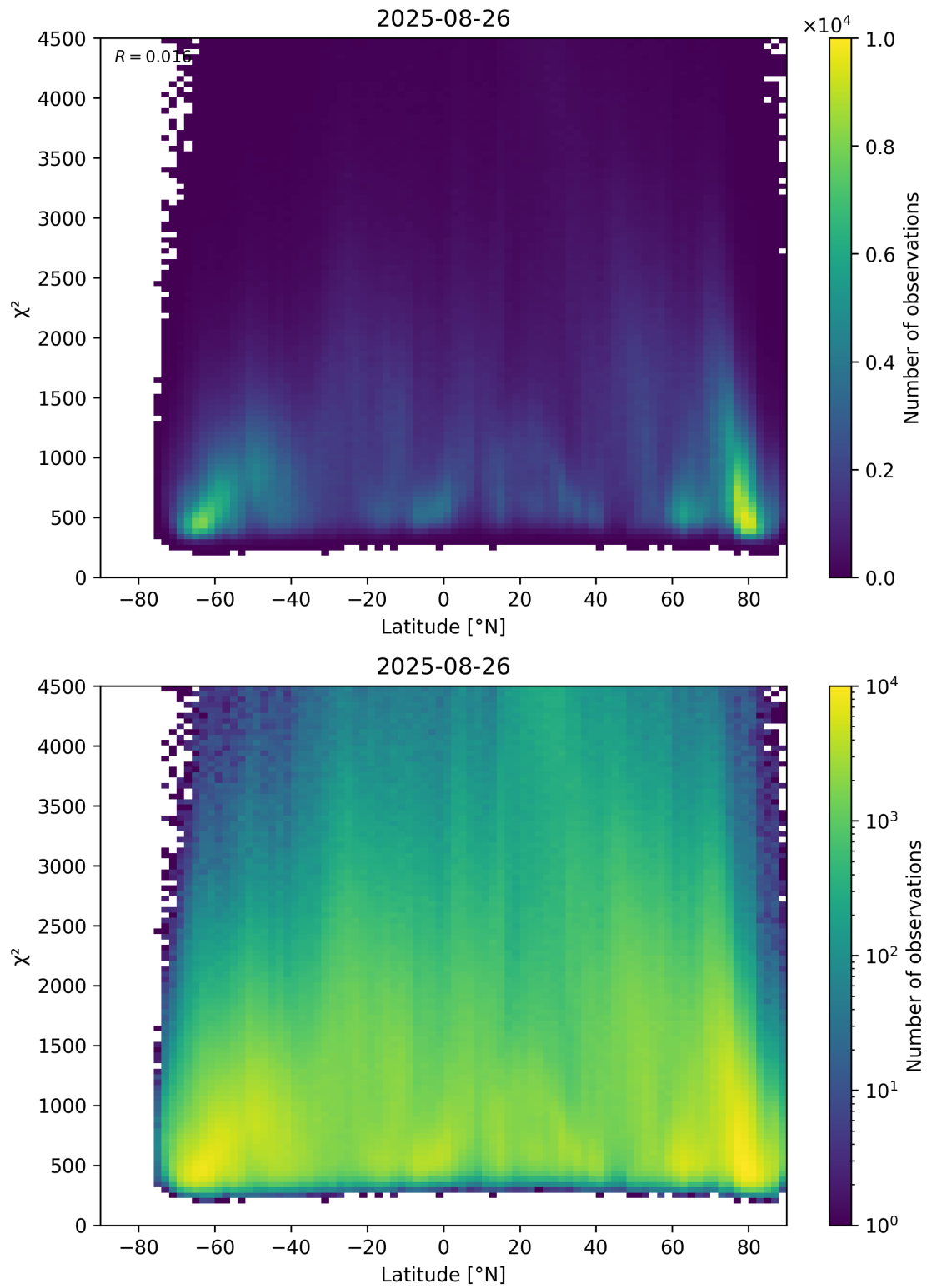
Figure 54: Scatter density plot of “Latitude” against “ \chi^2 ” for 2025-08-25 to 2025-08-27.
