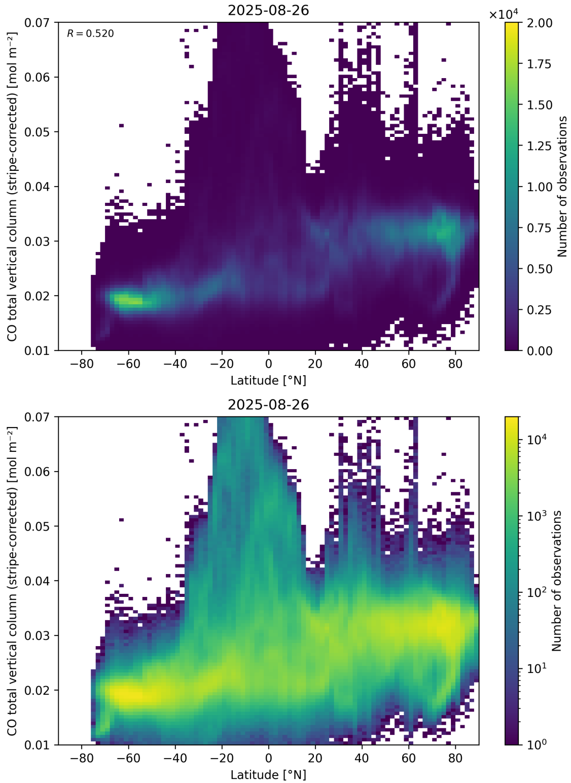
Figure 52: Scatter density plot of “Latitude” against “CO total vertical column (stripe-corrected)” for 2025-08-25 to 2025-08-27.
