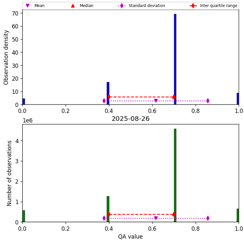
Figure 17: Histogram of “QA value” for 2025-08-25 to 2025-08-27
