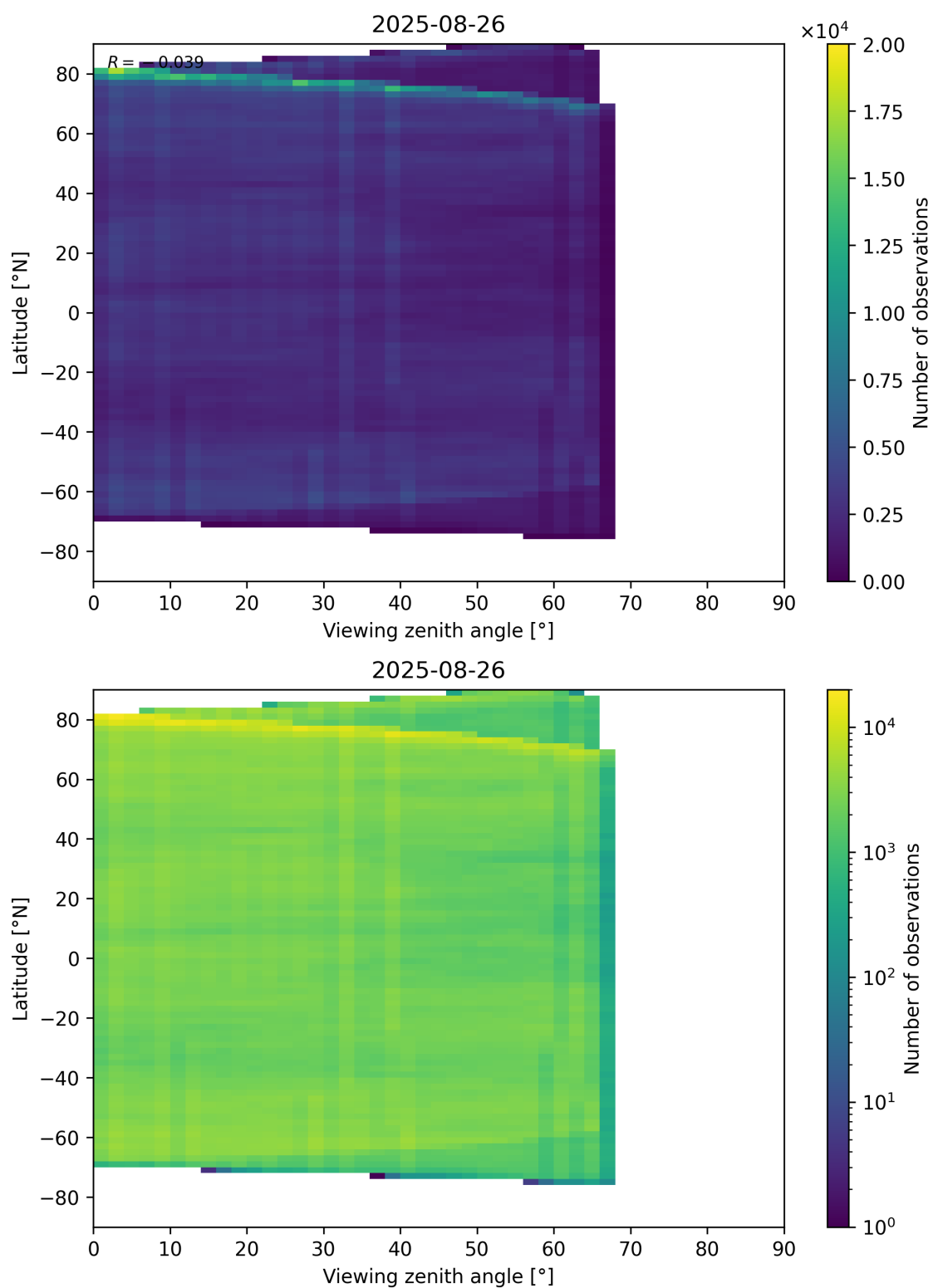
Figure 74: Scatter density plot of “Viewing zenith angle” against “Latitude” for 2025-08-25 to 2025-08-27.
