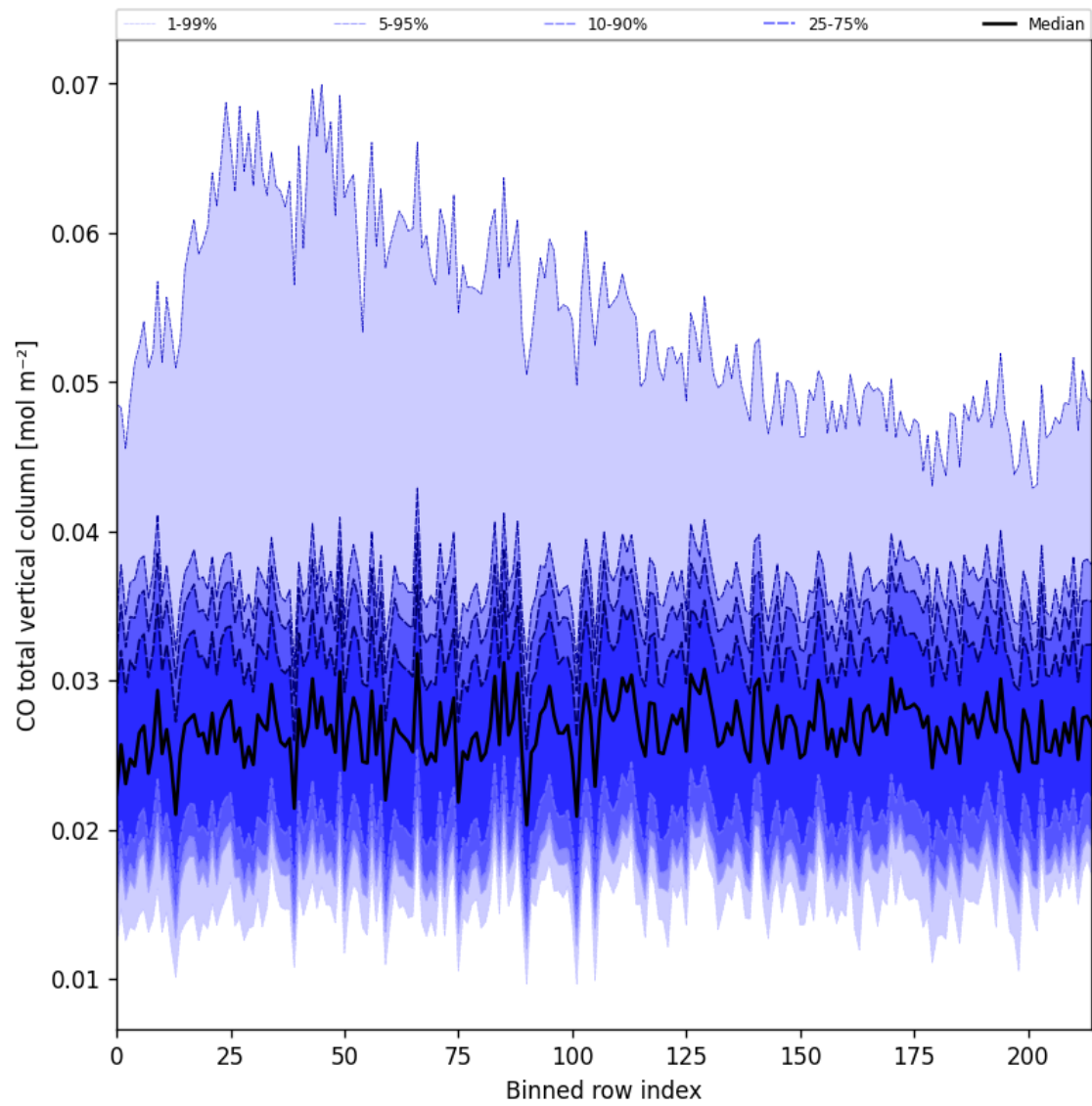
Figure 26: Along track statistics of “CO total vertical column” for 2025-08-25 to 2025-08-27
