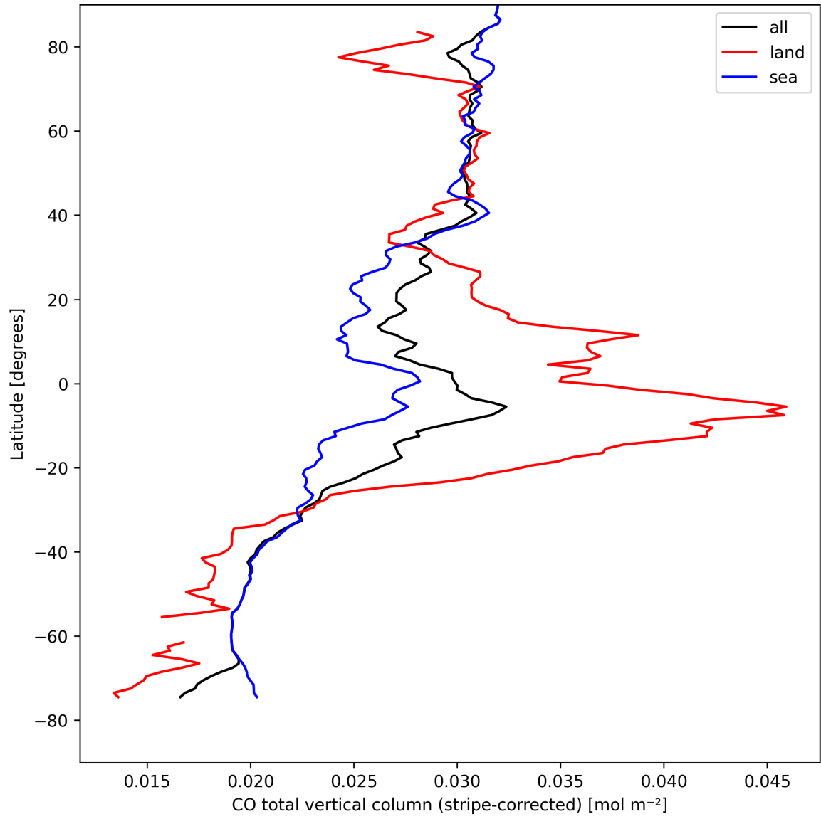
Figure 11: Zonal average of “CO total vertical column (stripe-corrected)” for 2025-08-25 to 2025-08-27.
