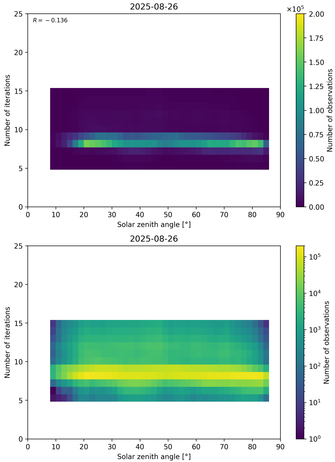
Figure 67: Scatter density plot of “Solar zenith angle” against “Number of iterations” for 2025-08-25 to 2025-08-27.
