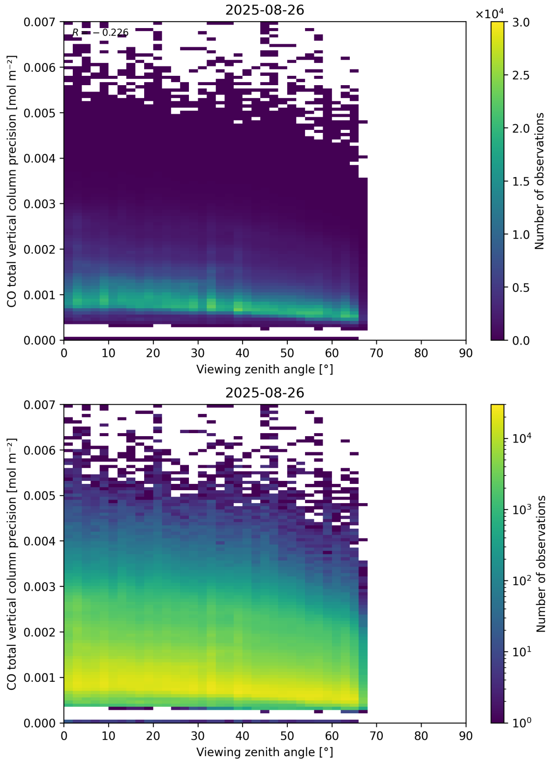
Figure 71: Scatter density plot of “Viewing zenith angle” against “CO total vertical column precision” for 2025-08-25 to 2025-08-27.
