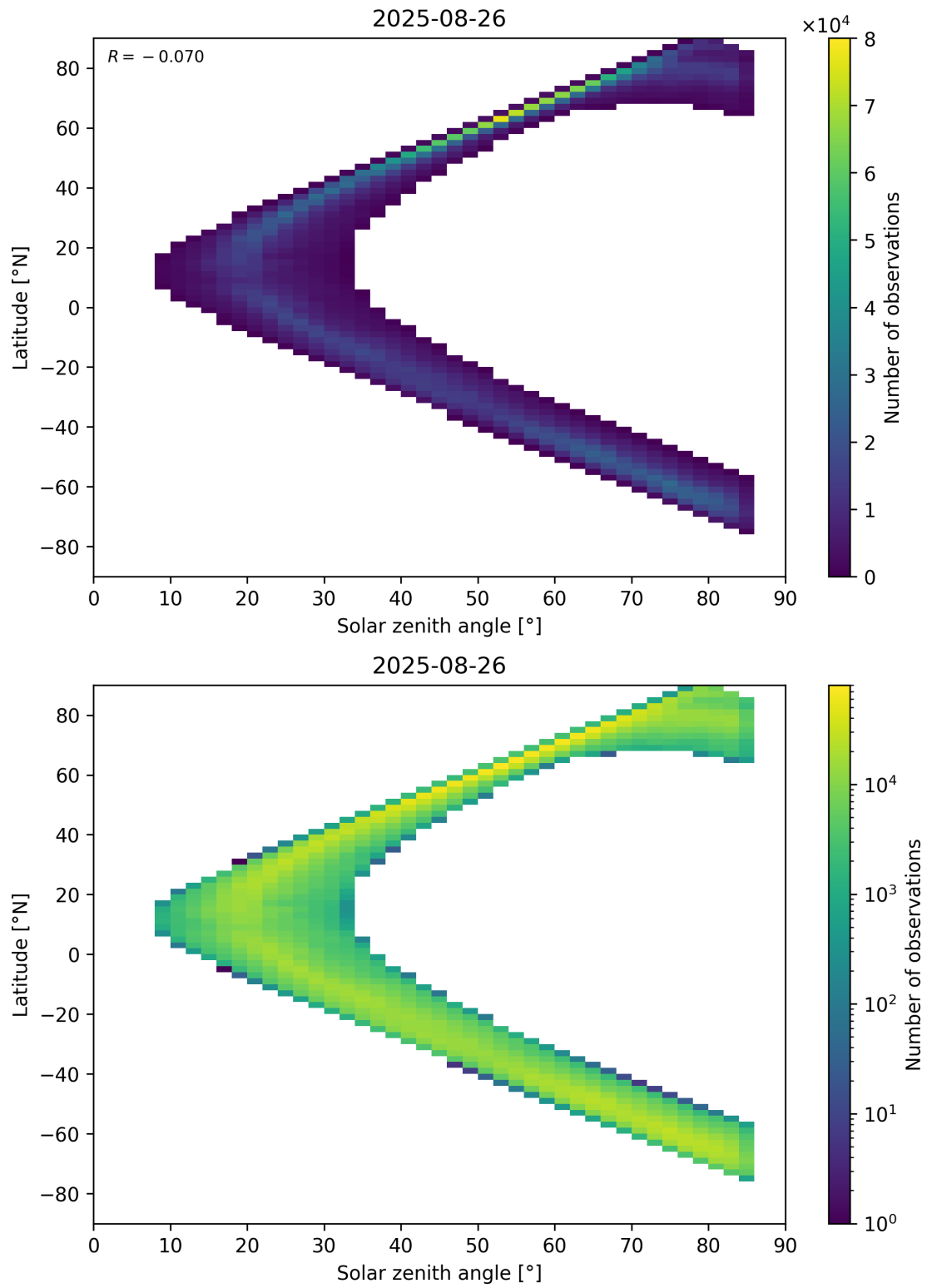
Figure 66: Scatter density plot of “Solar zenith angle” against “Latitude” for 2025-08-25 to 2025-08-27.
