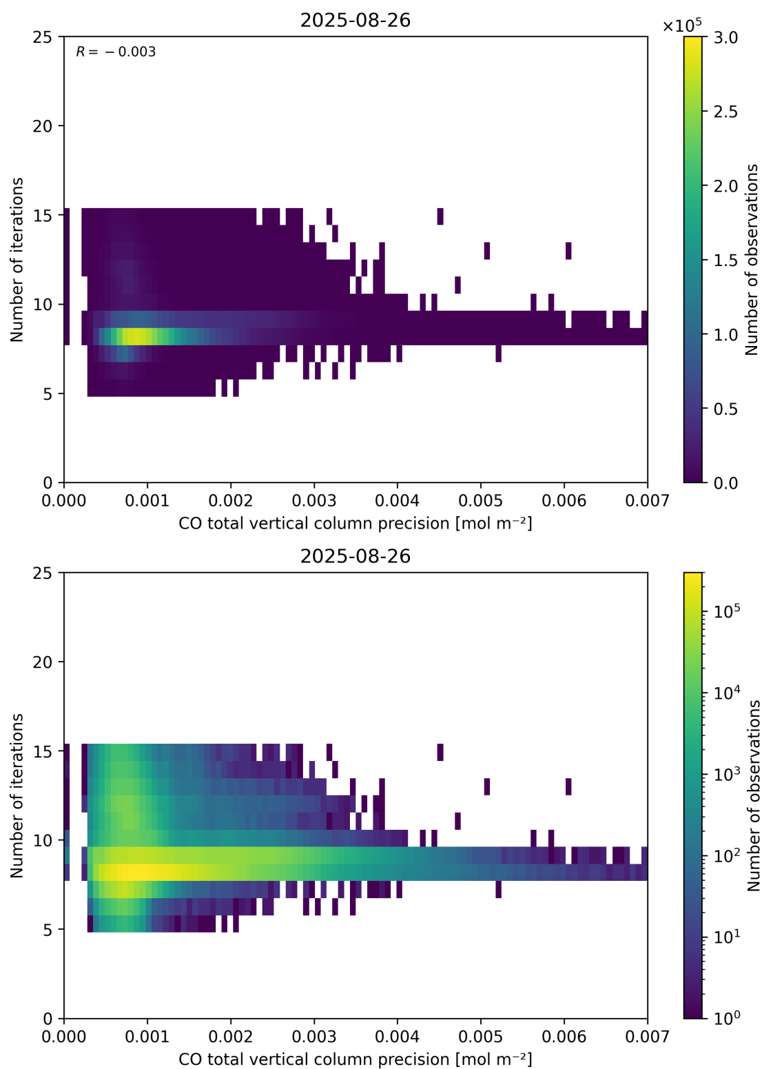
Figure 46: Scatter density plot of “CO total vertical column precision” against “Number of iterations” for 2025-08-25 to 2025-08-27.
