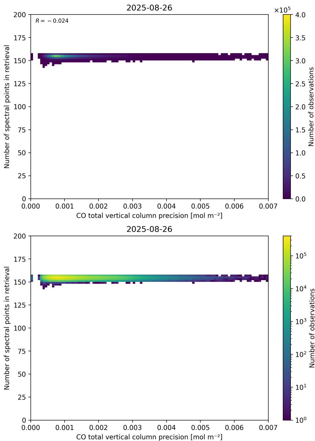
Figure 47: Scatter density plot of “CO total vertical column precision” against “Number of spectral points in retrieval” for 2025-08-25 to 2025-08-27.
