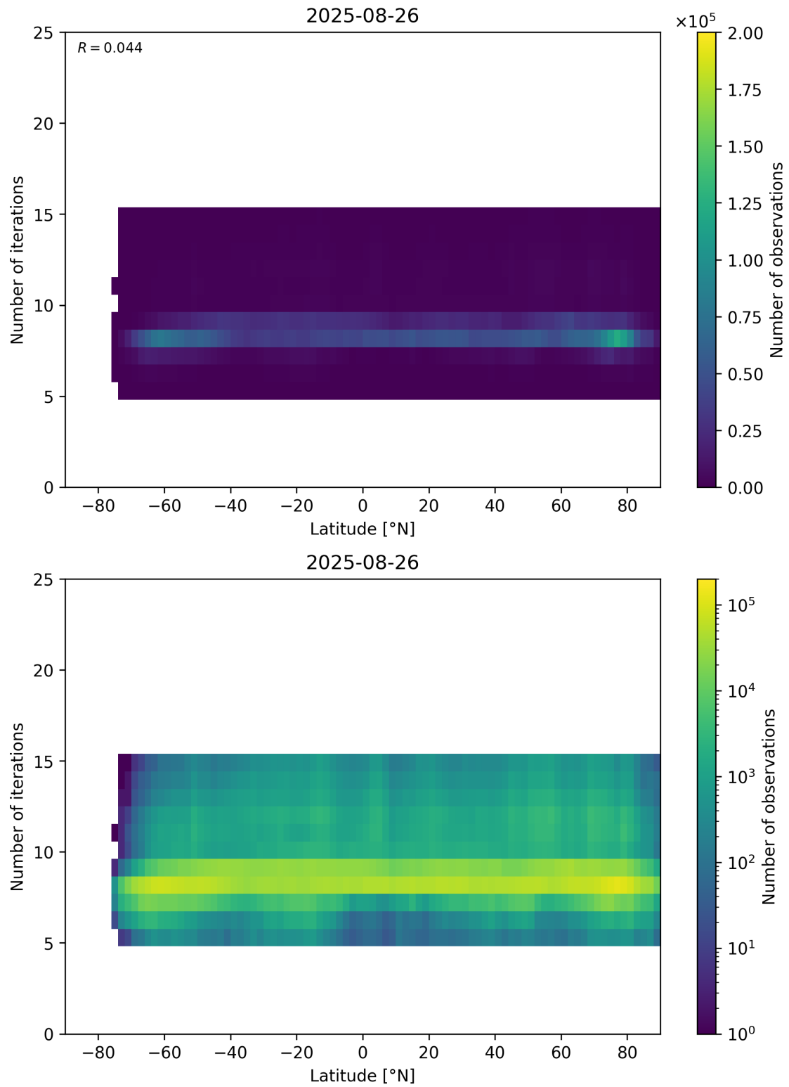
Figure 56: Scatter density plot of “Latitude” against “Number of iterations” for 2025-08-25 to 2025-08-27.
