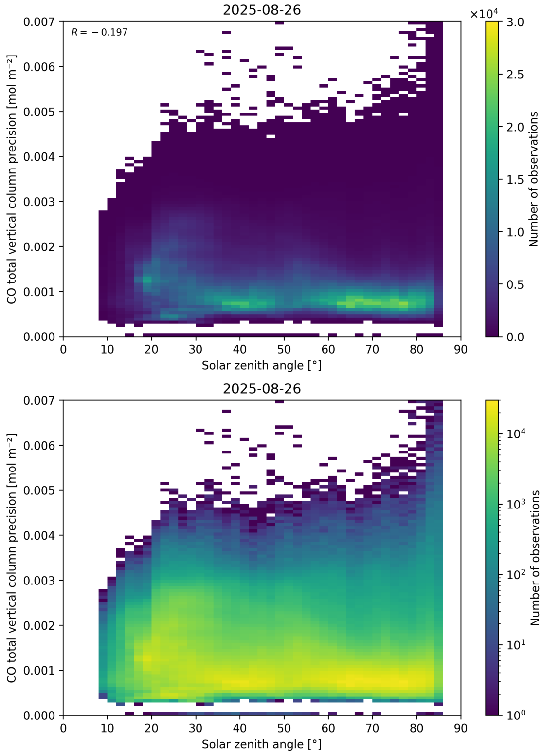
Figure 63: Scatter density plot of “Solar zenith angle” against “CO total vertical column precision” for 2025-08-25 to 2025-08-27.
