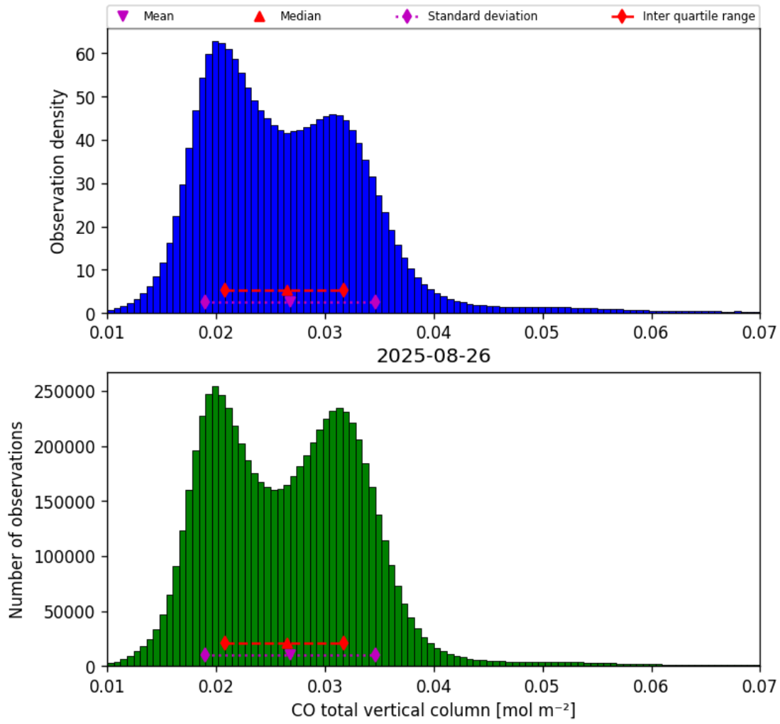
Figure 18: Histogram of “CO total vertical column” for 2025-08-25 to 2025-08-27
