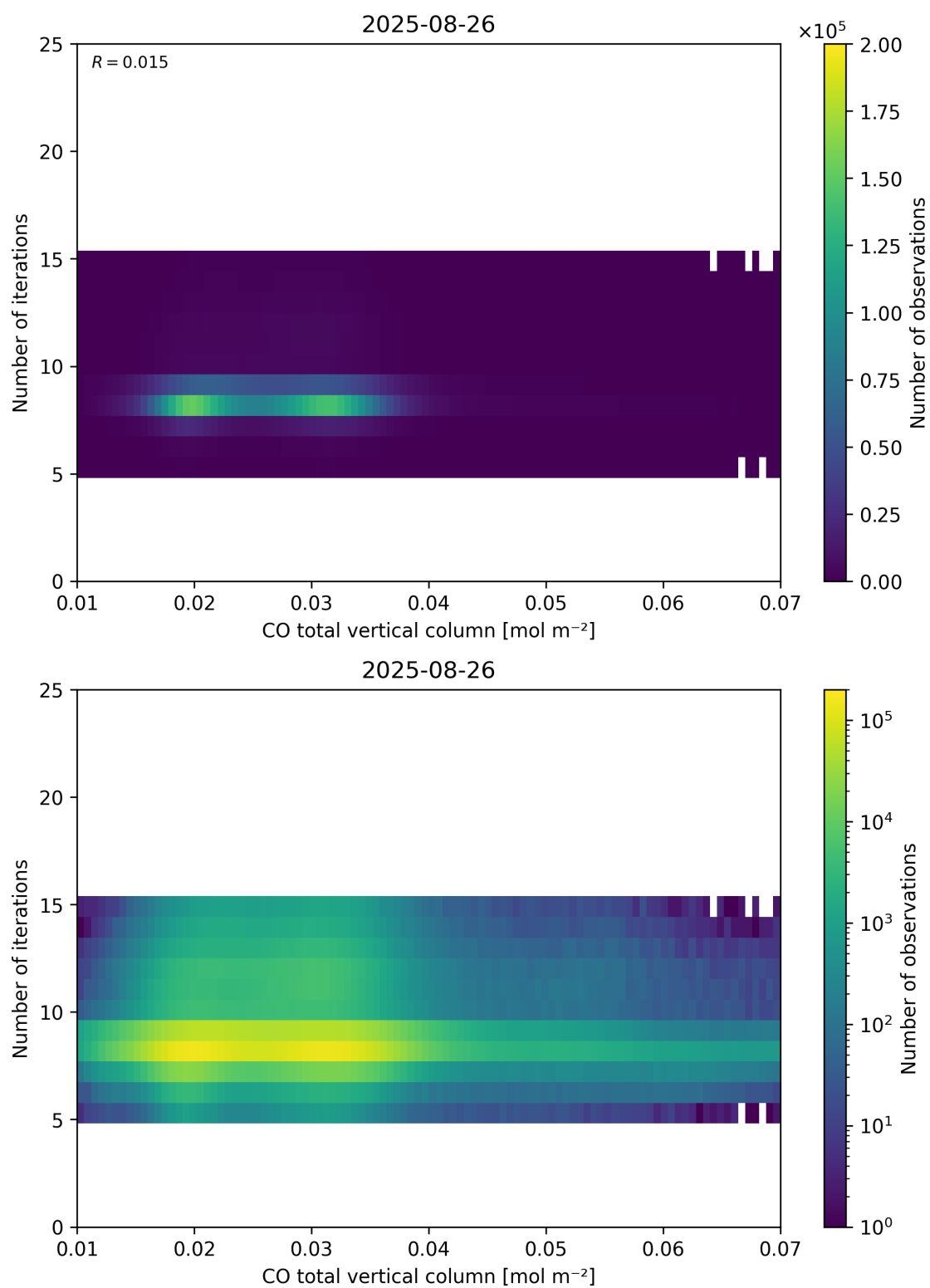
Figure 42: Scatter density plot of “CO total vertical column” against “Number of iterations” for 2025-08-25 to 2025-08-27.
