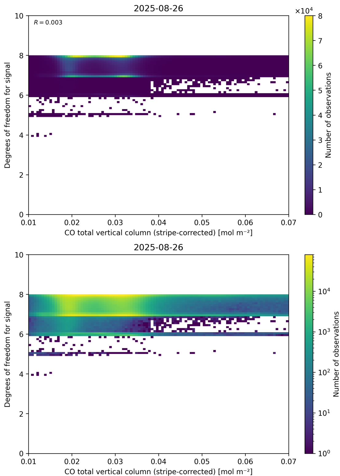
Figure 38: Scatter density plot of “CO total vertical column (stripe-corrected)” against “Degrees of freedom for signal” for 2025-08-25 to 2025-08-27.
