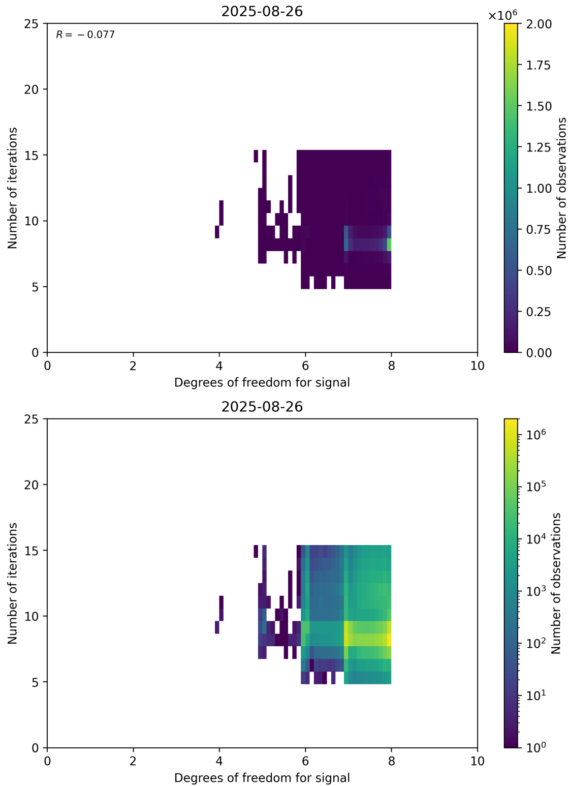
Figure 50: Scatter density plot of “Degrees of freedom for signal” against “Number of iterations” for 2025-08-25 to 2025-08-27.
