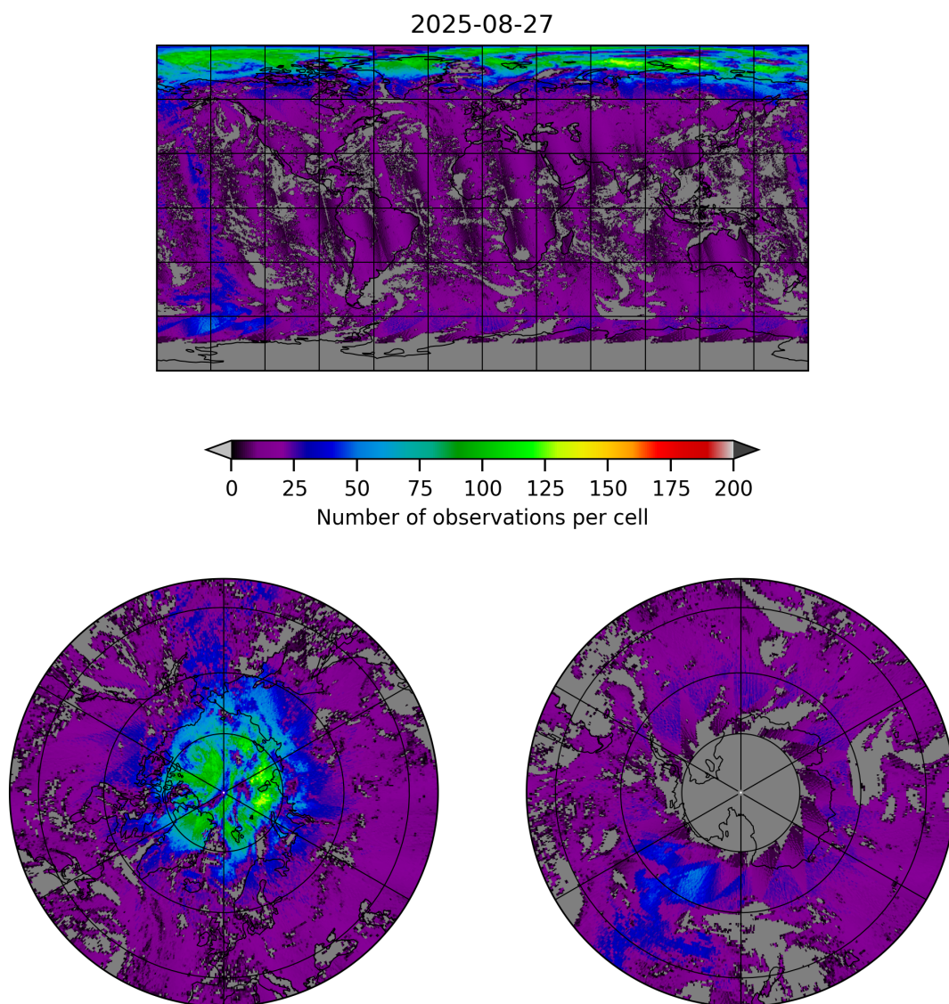
Figure 8: Map of the number of observations for 2025-08-26 to 2025-08-28
