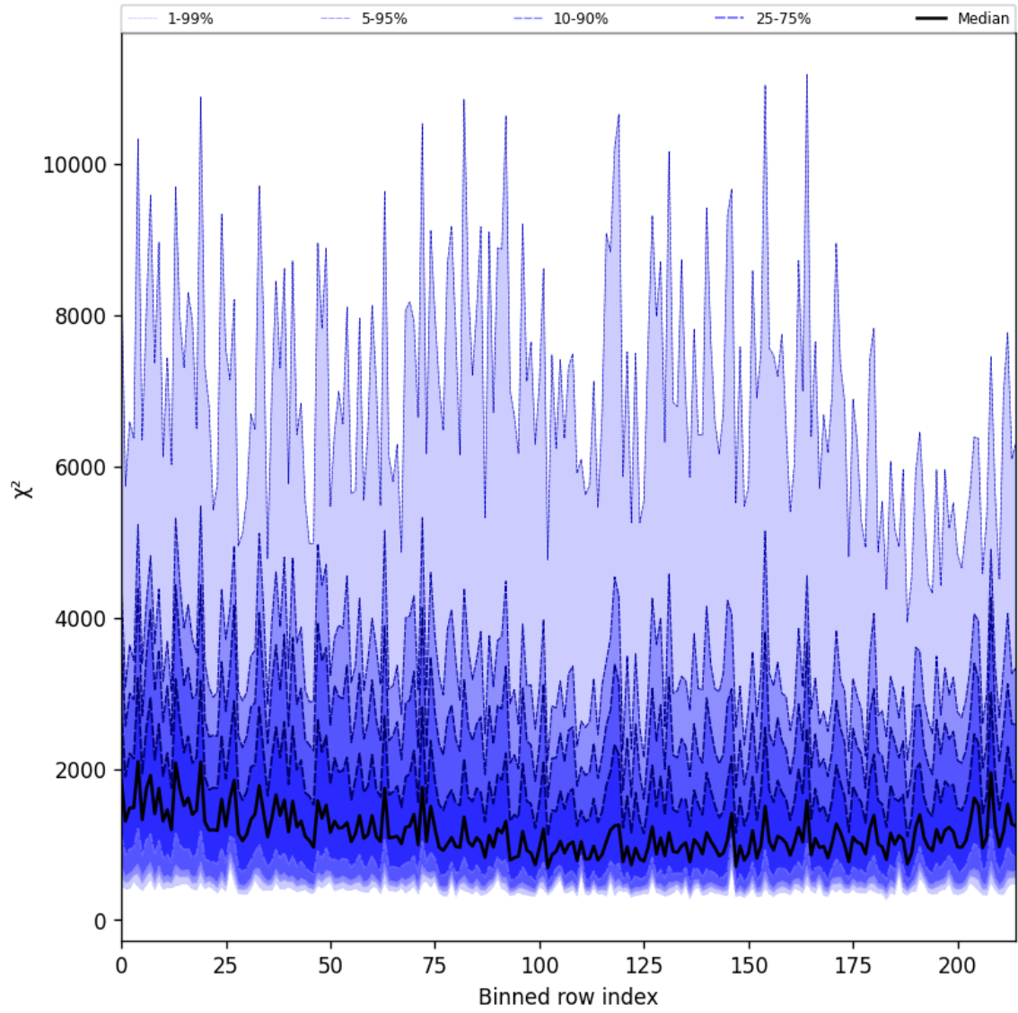
Figure 30: Along track statistics of “ \chi^2 ” for 2025-08-26 to 2025-08-28
