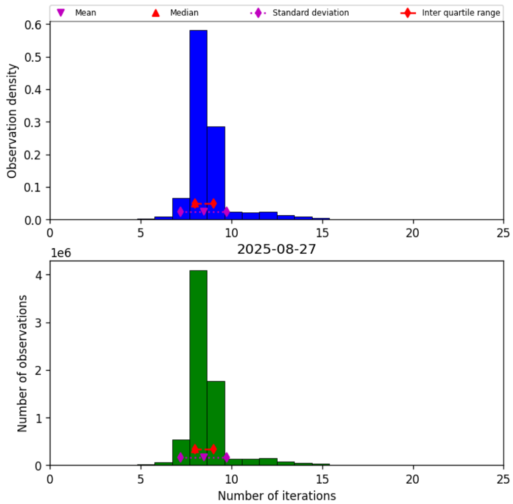
Figure 24: Histogram of “Number of iterations” for 2025-08-26 to 2025-08-28
