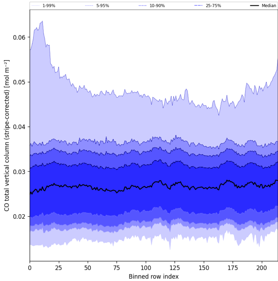
Figure 27: Along track statistics of “CO total vertical column (stripe-corrected)” for 2025-08-26 to 2025-08-28
