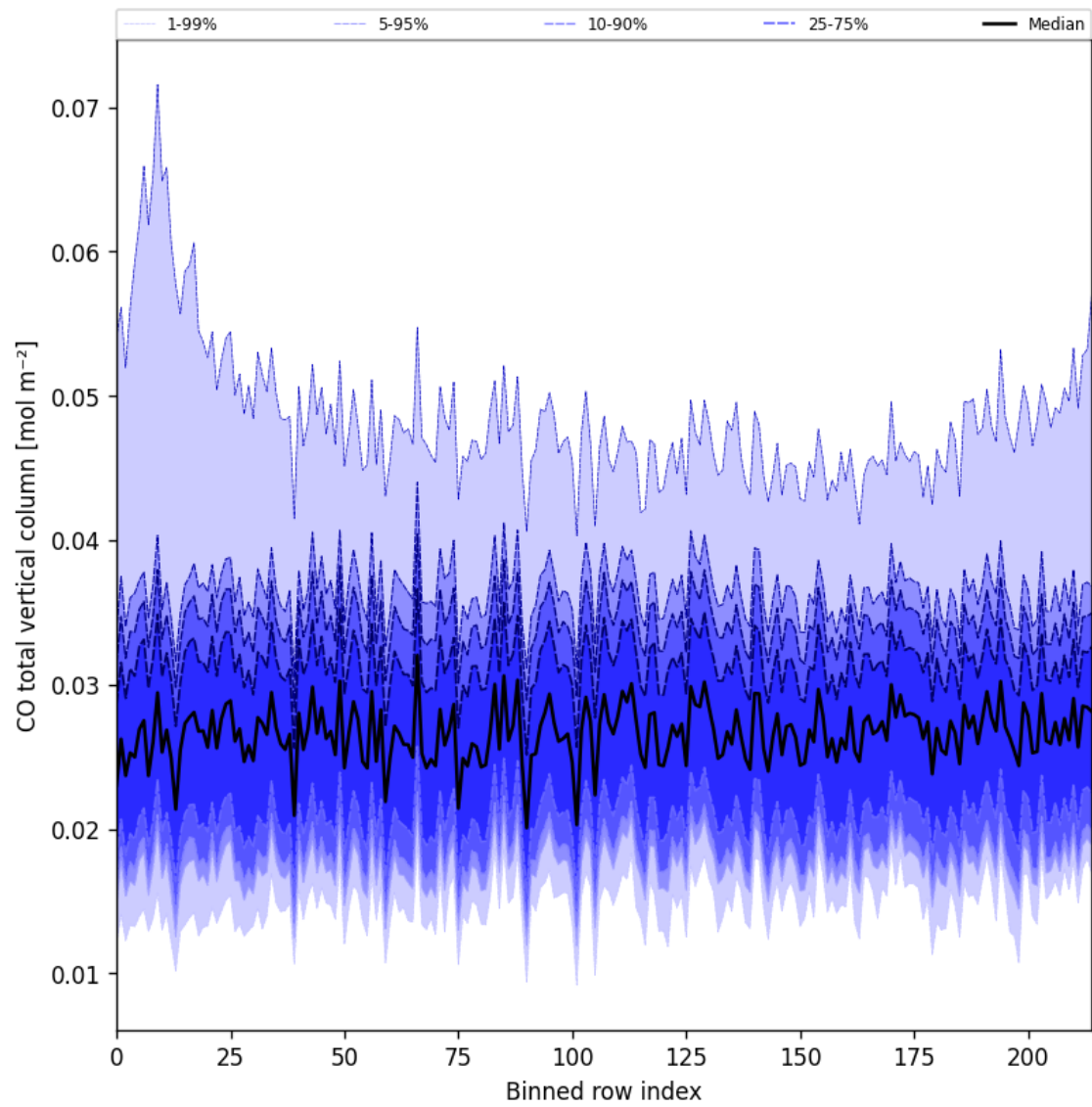
Figure 26: Along track statistics of “CO total vertical column” for 2025-08-26 to 2025-08-28
