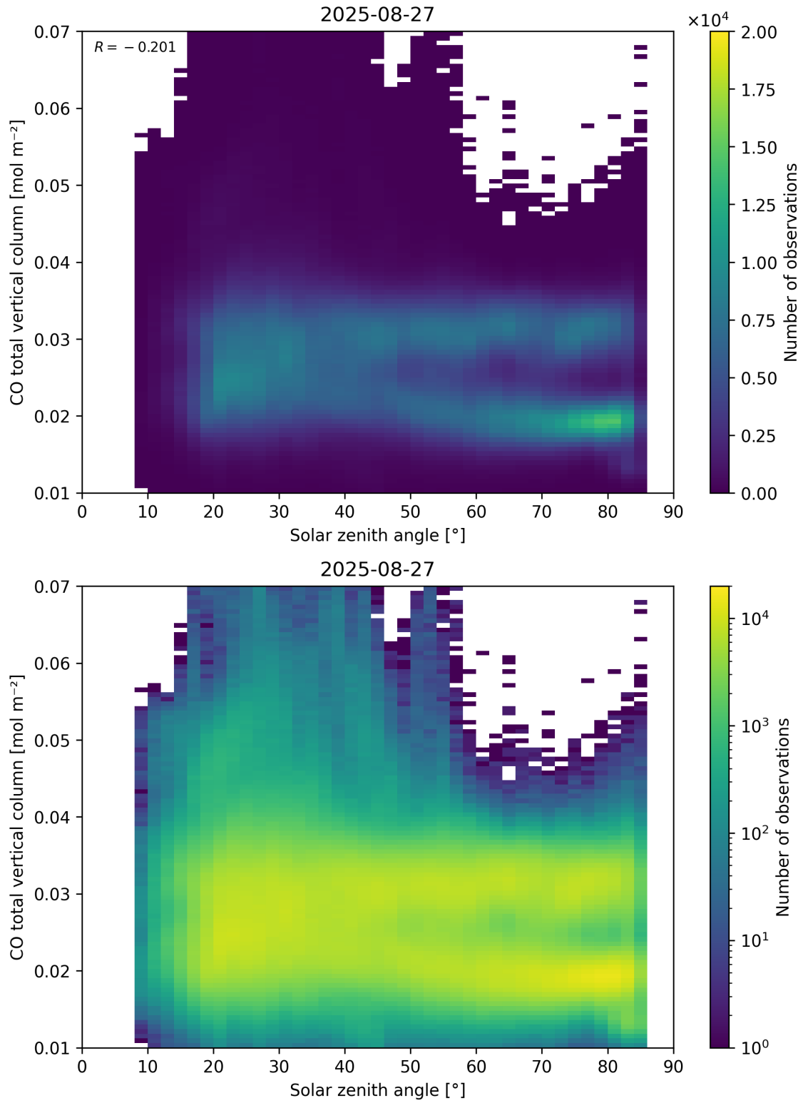
Figure 61: Scatter density plot of “Solar zenith angle” against “CO total vertical column” for 2025-08-26 to 2025-08-28.
