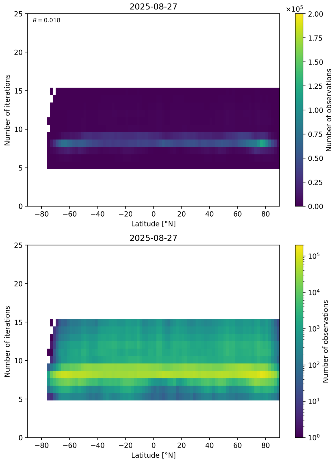
Figure 56: Scatter density plot of “Latitude” against “Number of iterations” for 2025-08-26 to 2025-08-28.
