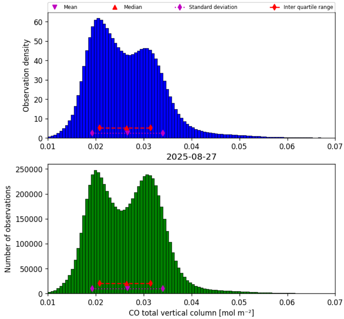
Figure 18: Histogram of “CO total vertical column” for 2025-08-26 to 2025-08-28
