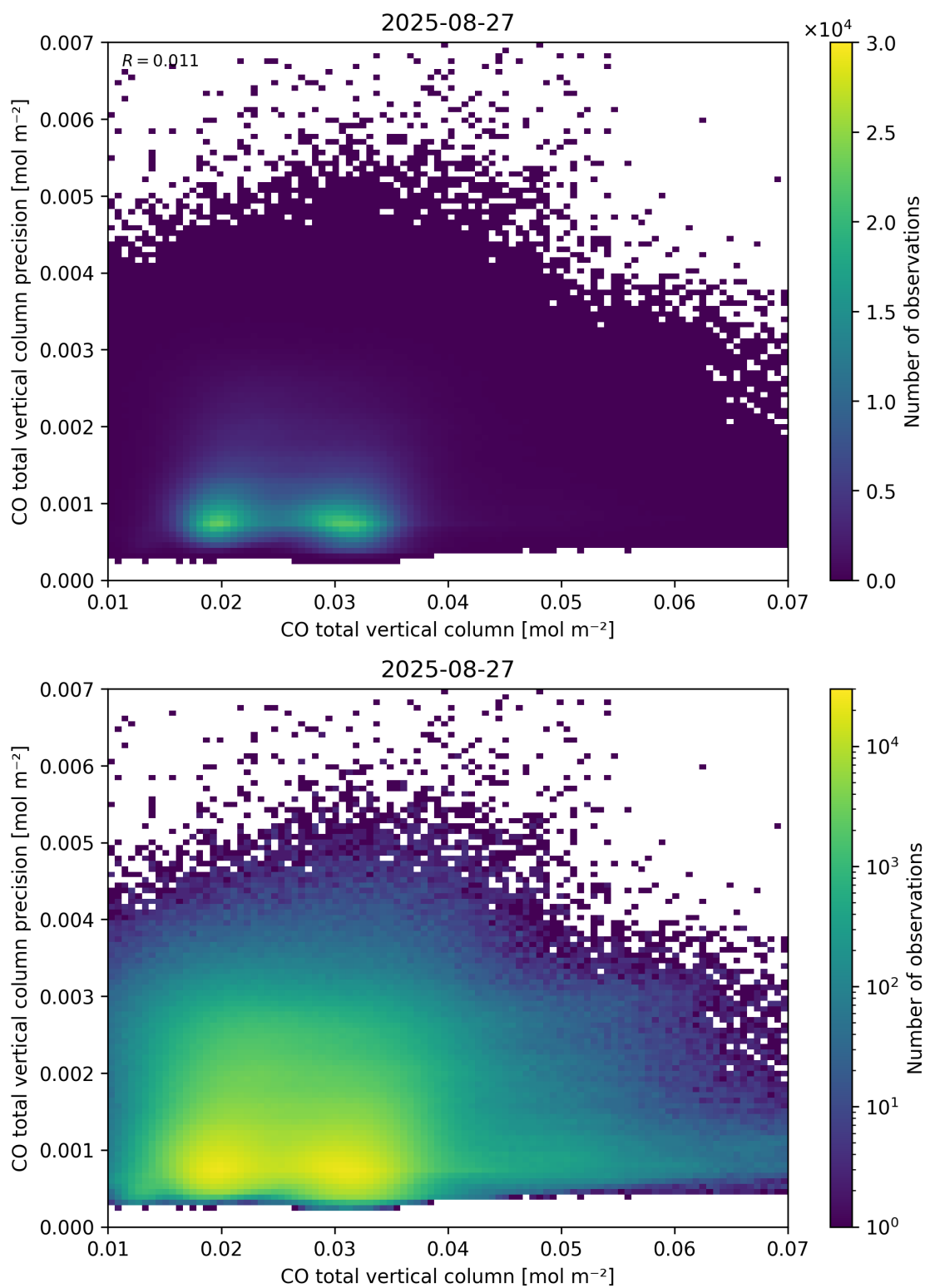
Figure 34: Scatter density plot of “CO total vertical column” against “CO total vertical column precision” for 2025-08-26 to 2025-08-28.
