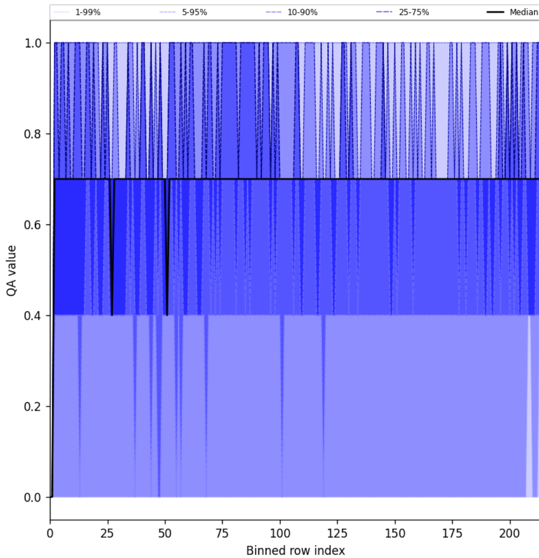
Figure 25: Along track statistics of "QA value" for 2025-08-26 to 2025-08-28
