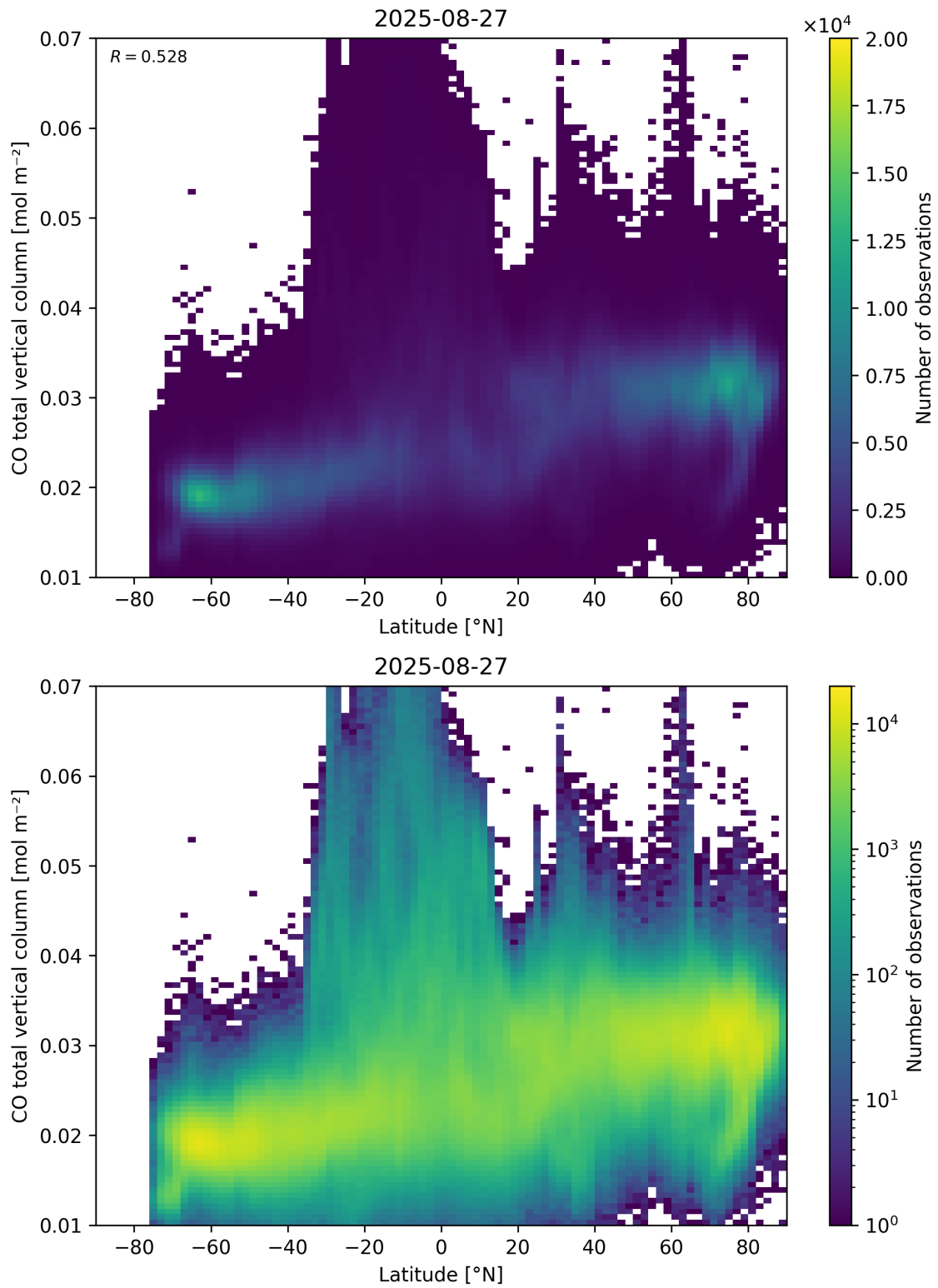
Figure 51: Scatter density plot of “Latitude” against “CO total vertical column” for 2025-08-26 to 2025-08-28.
