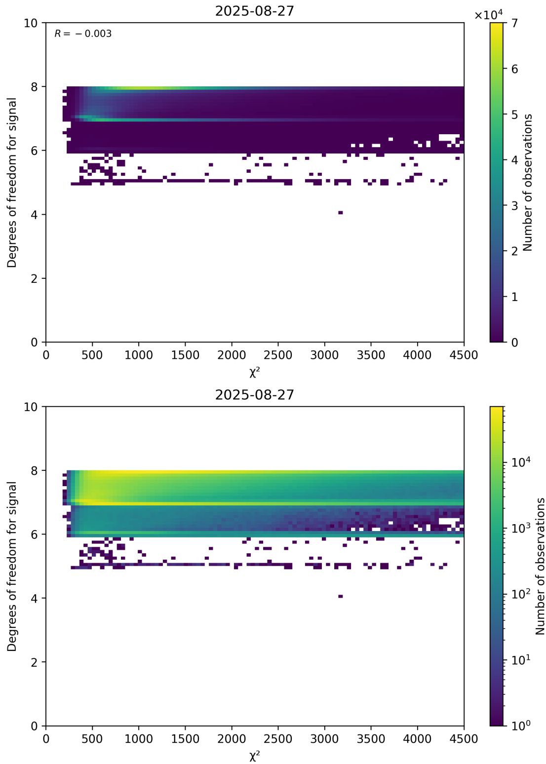
Figure 48: Scatter density plot of “ \chi^2 ” against “Degrees of freedom for signal” for 2025-08-26 to 2025-08-28.
