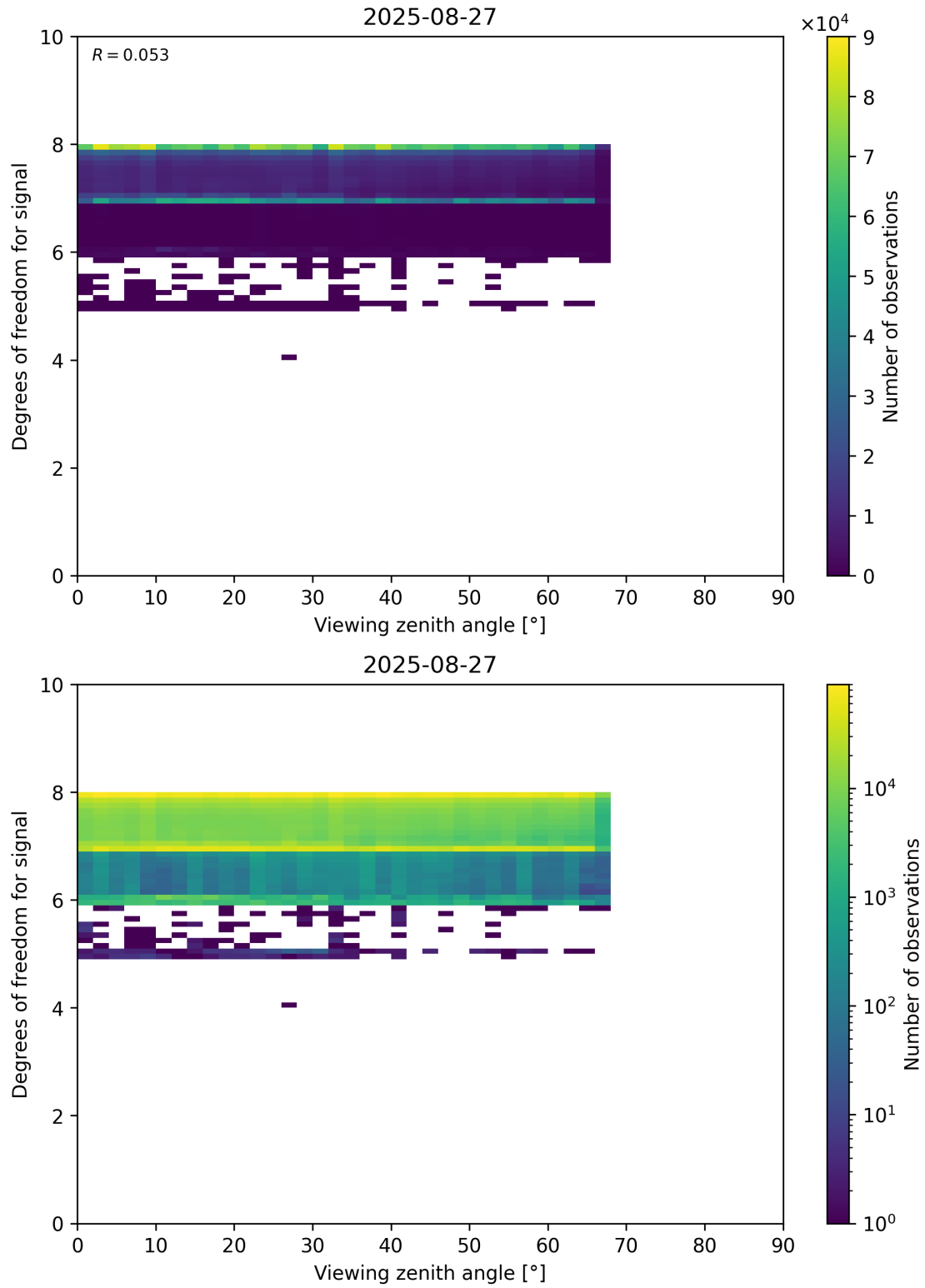
Figure 73: Scatter density plot of “Viewing zenith angle” against “Degrees of freedom for signal” for 2025-08-26 to 2025-08-28.
