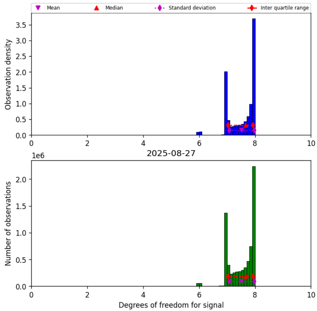
Figure 23: Histogram of “Degrees of freedom for signal” for 2025-08-26 to 2025-08-28
