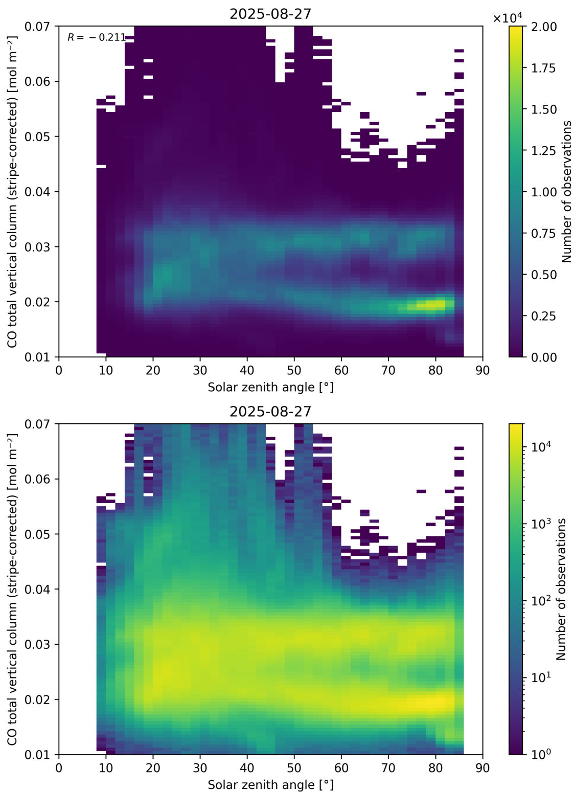
Figure 62: Scatter density plot of “Solar zenith angle” against “CO total vertical column (stripe-corrected)” for 2025-08-26 to 2025-08-28.
