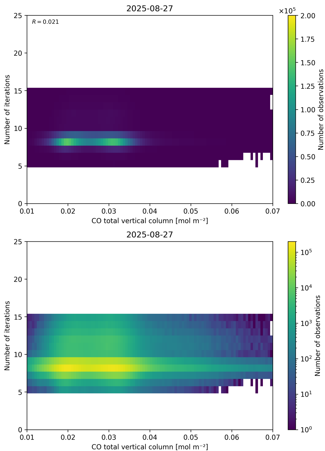
Figure 42: Scatter density plot of “CO total vertical column” against “Number of iterations” for 2025-08-26 to 2025-08-28.
