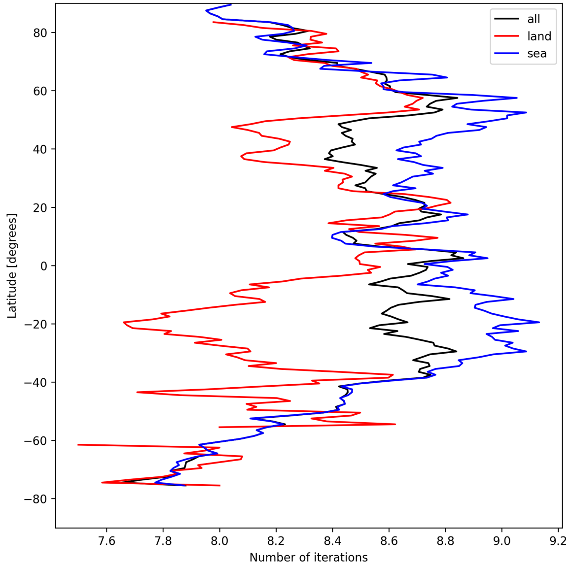
Figure 16: Zonal average of “Number of iterations” for 2025-08-26 to 2025-08-28.
