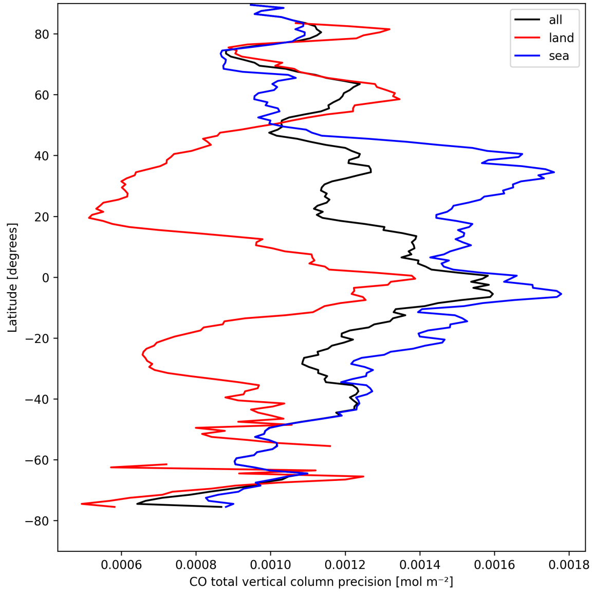
Figure 12: Zonal average of "CO total vertical column precision" for 2025-08-26 to 2025-08-28.
