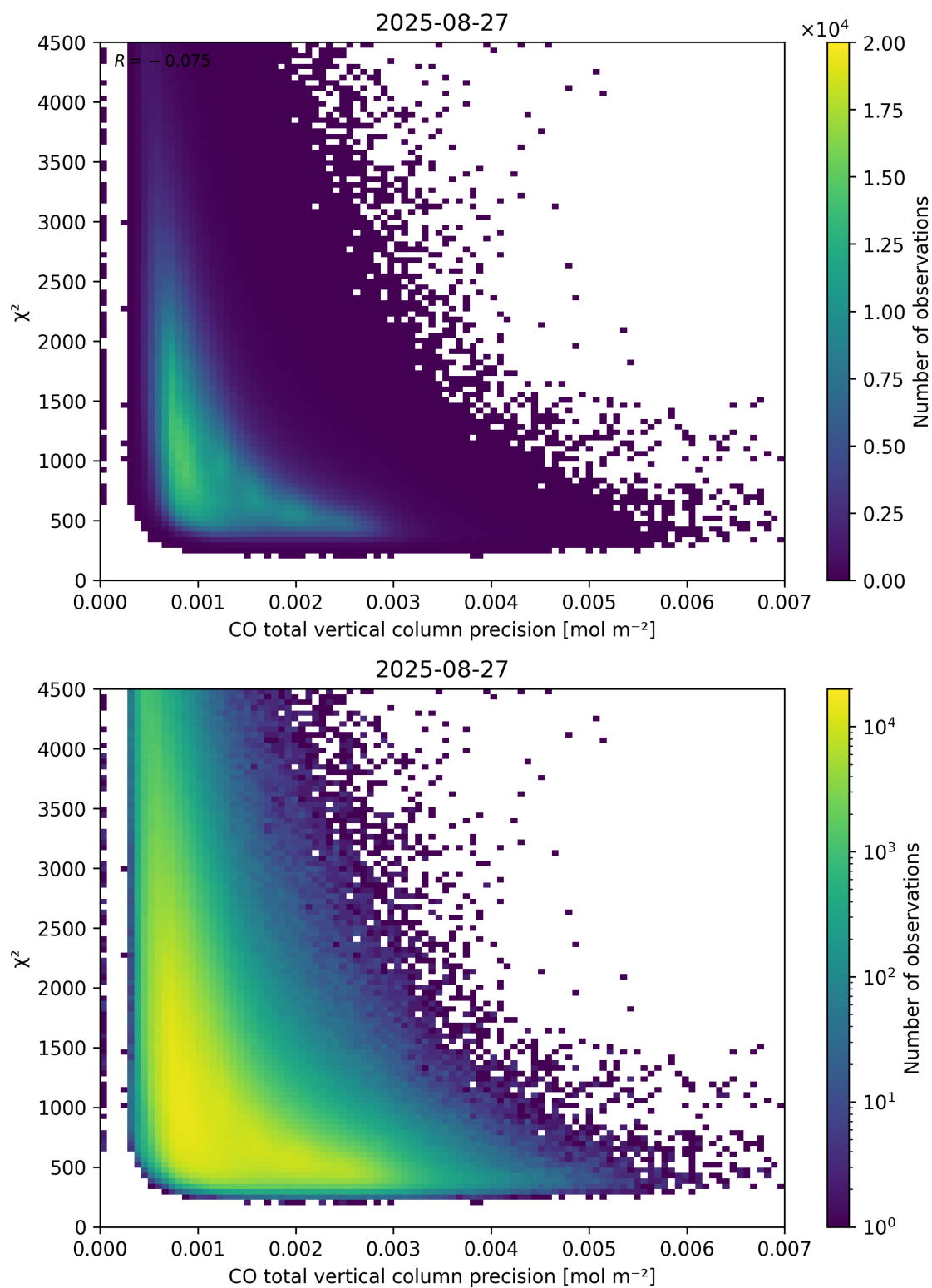
Figure 44: Scatter density plot of “CO total vertical column precision” against “ \chi^2 ” for 2025-08-26 to 2025-08-28.
