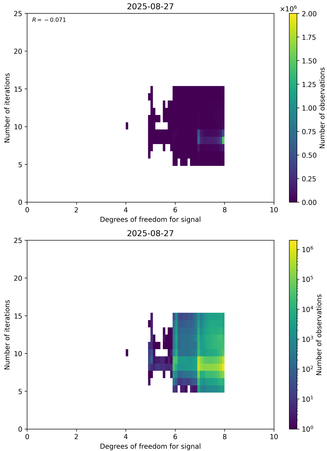
Figure 50: Scatter density plot of “Degrees of freedom for signal” against “Number of iterations” for 2025-08-26 to 2025-08-28.
