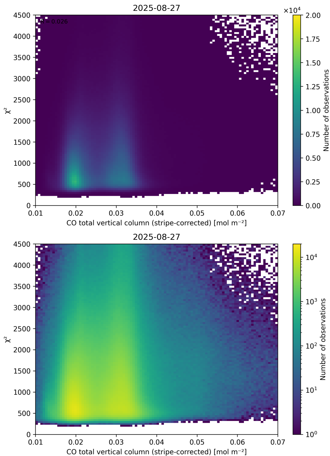
Figure 37: Scatter density plot of “CO total vertical column (stripe-corrected)” against “ \chi^2 ” for 2025-08-26 to 2025-08-28.
