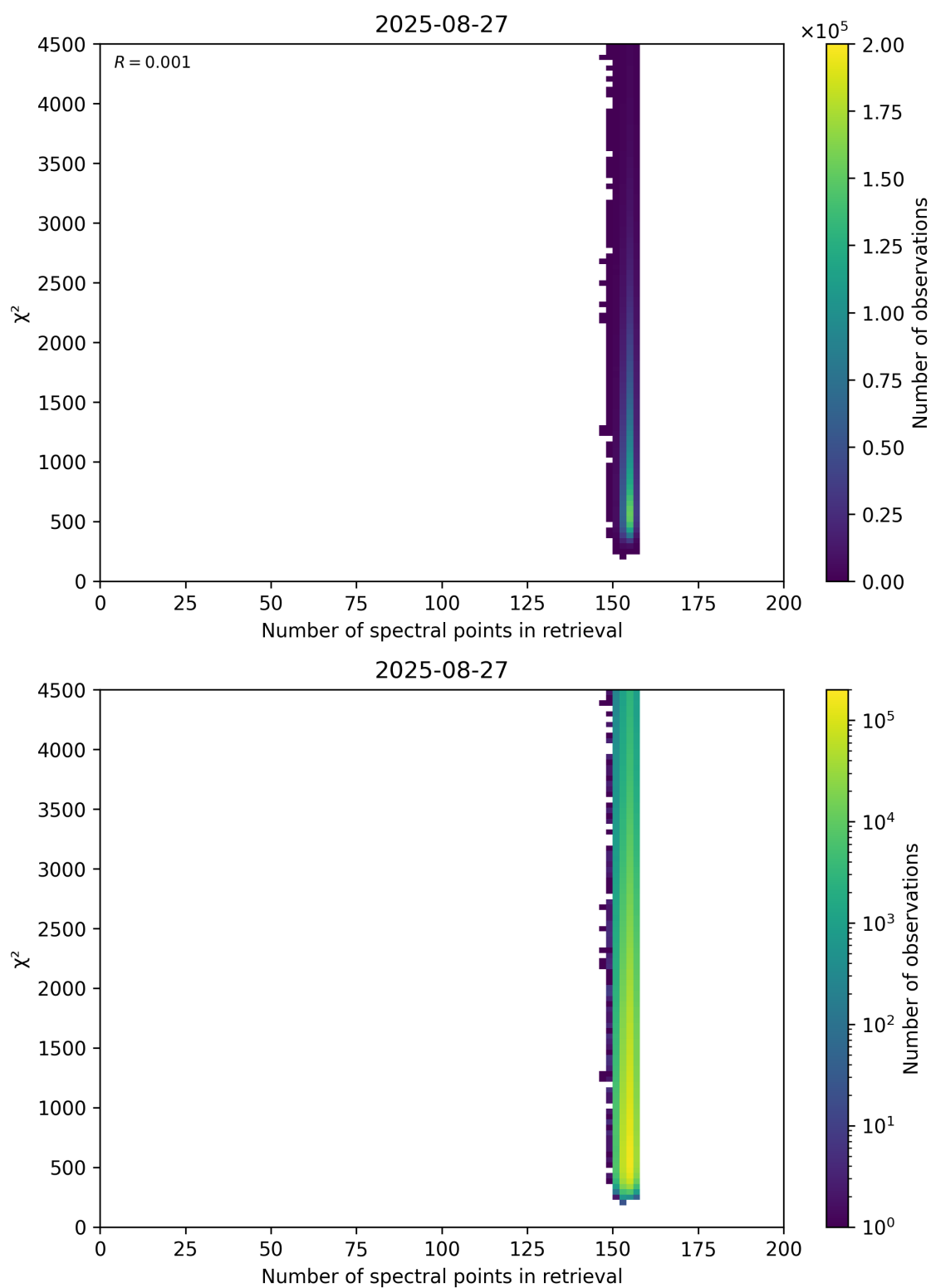
Figure 58: Scatter density plot of “Number of spectral points in retrieval” against “ \chi^2 ” for 2025-08-26 to 2025-08-28.
