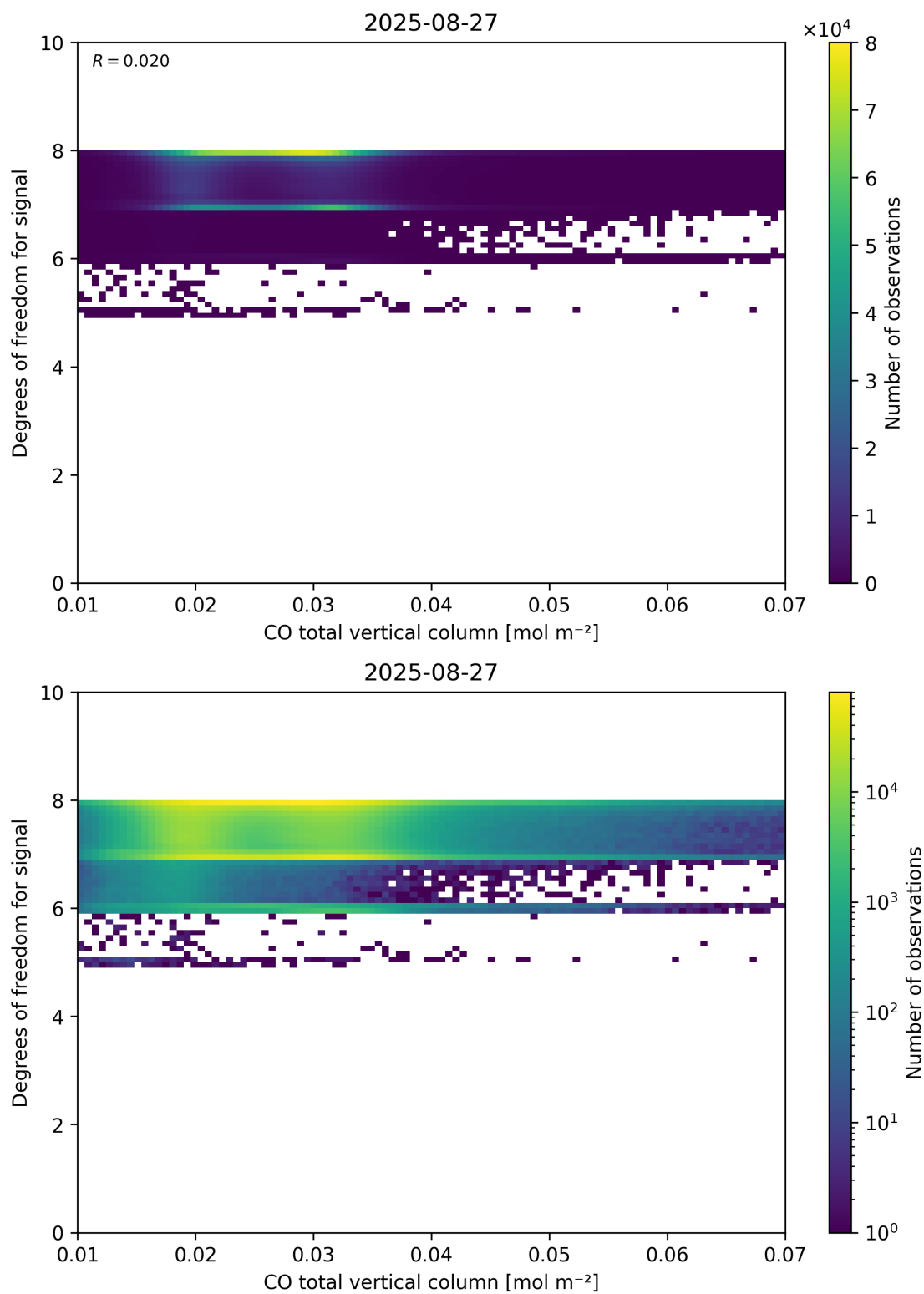
Figure 41: Scatter density plot of “CO total vertical column” against “Degrees of freedom for signal” for 2025-08-26 to 2025-08-28.
