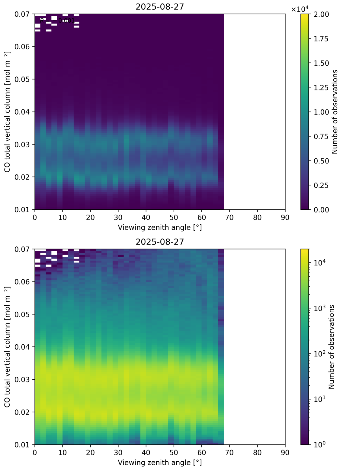
Figure 69: Scatter density plot of “Viewing zenith angle” against “CO total vertical column” for 2025-08-26 to 2025-08-28.
