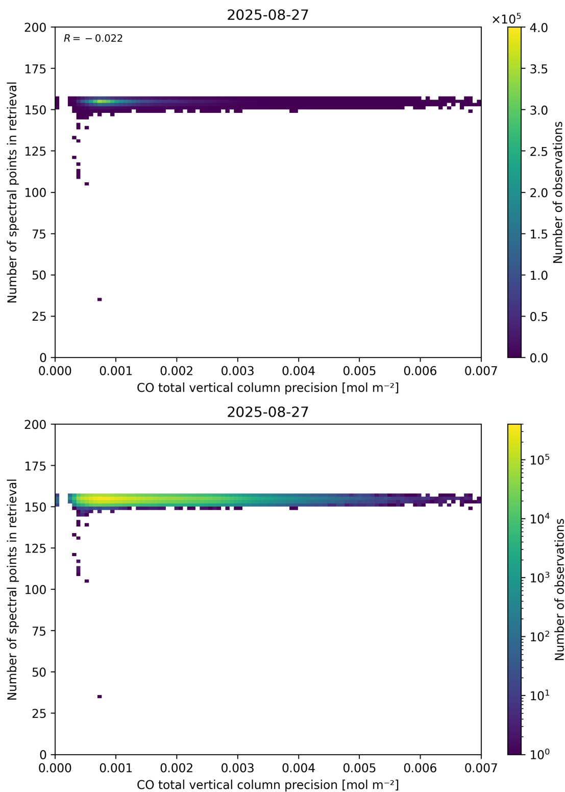
Figure 47: Scatter density plot of “CO total vertical column precision” against “Number of spectral points in retrieval” for 2025-08-26 to 2025-08-28.
