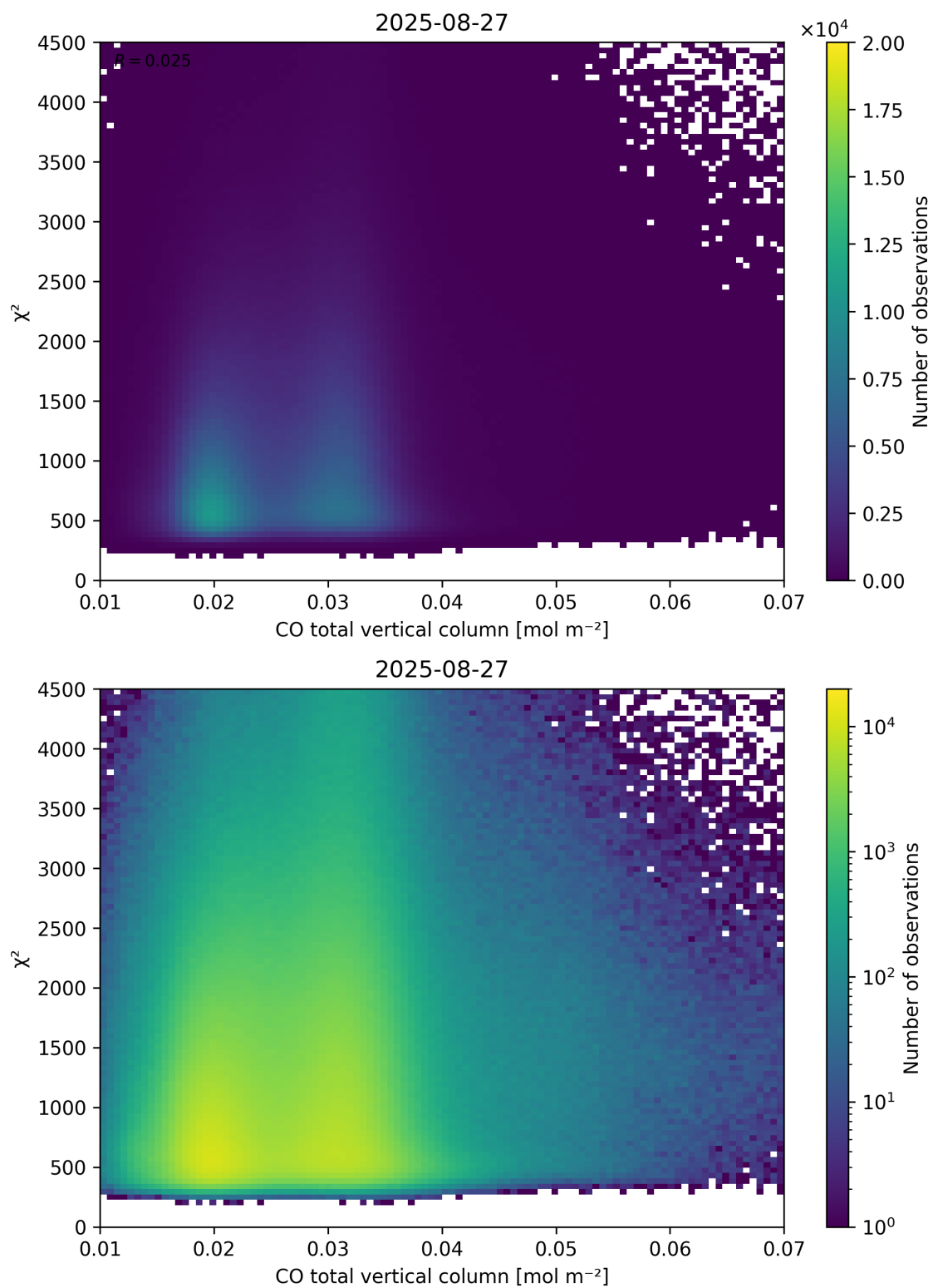
Figure 35: Scatter density plot of “CO total vertical column” against “ \chi^2 ” for 2025-08-26 to 2025-08-28.
