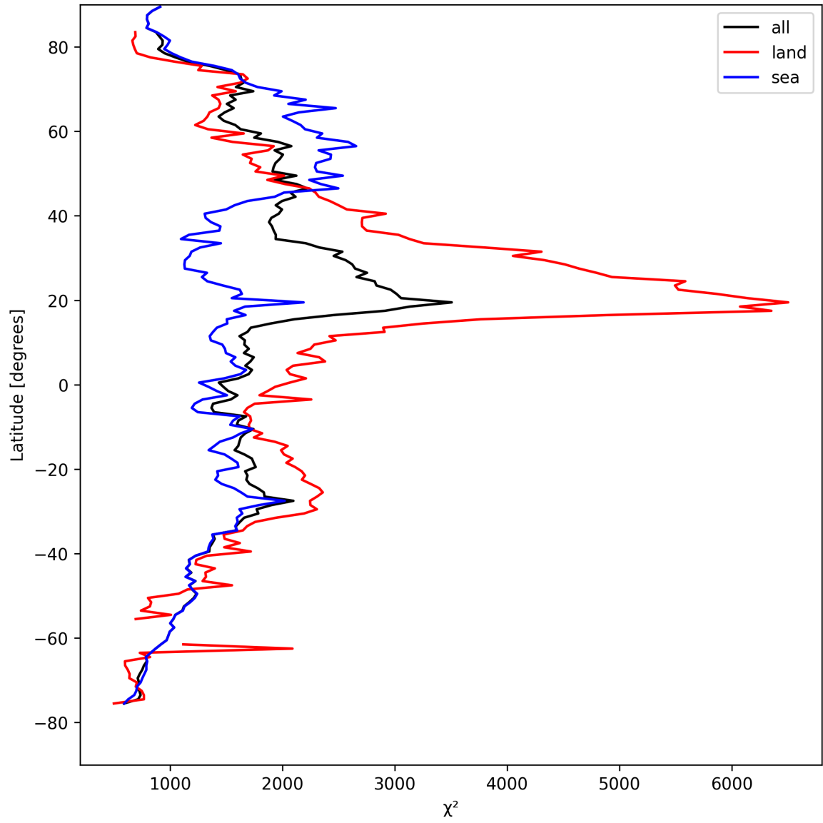
Figure 14: Zonal average of “ \chi^2 ” for 2025-08-26 to 2025-08-28.
