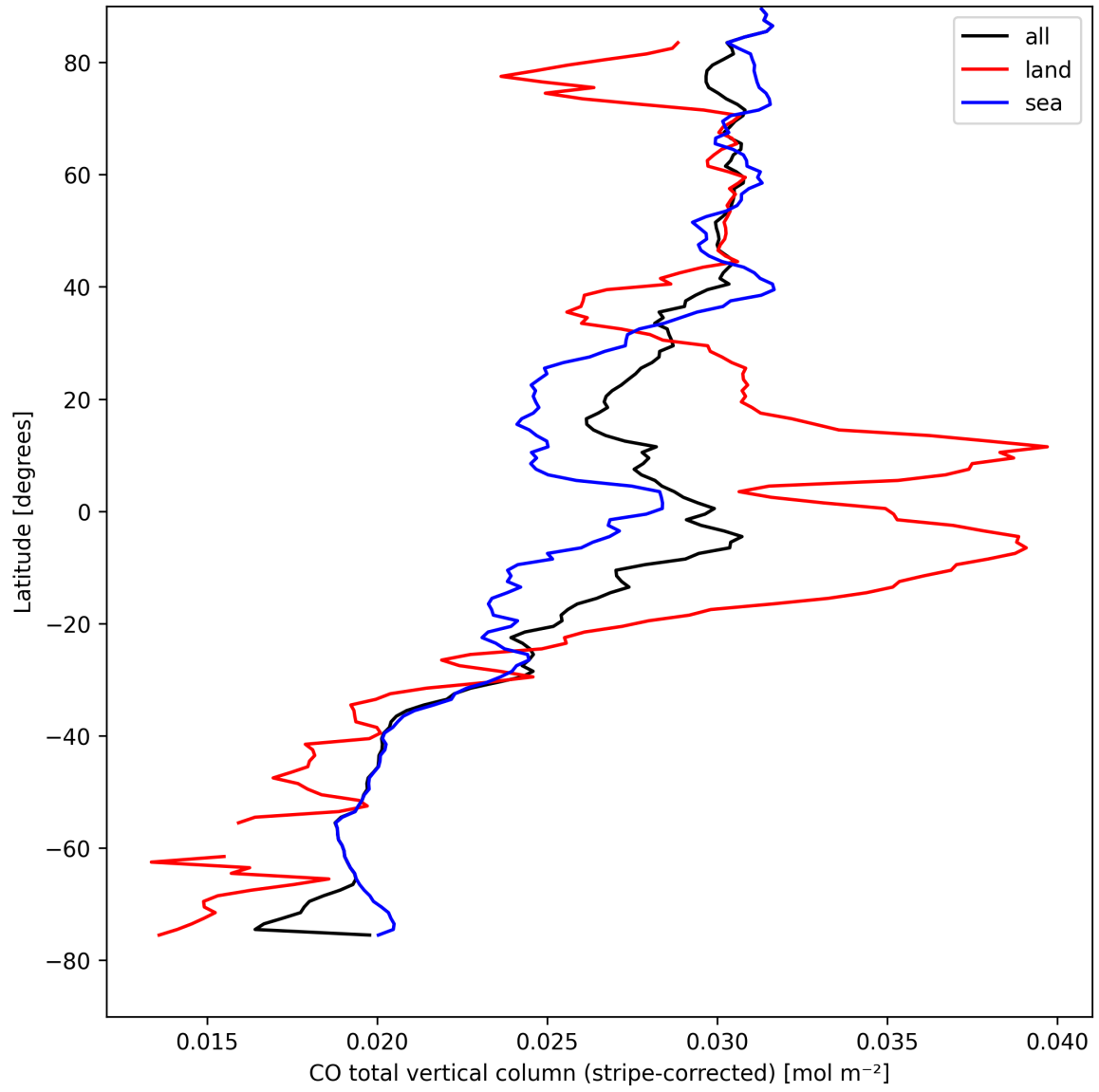
Figure 11: Zonal average of “CO total vertical column (stripe-corrected)” for 2025-08-26 to 2025-08-28.
