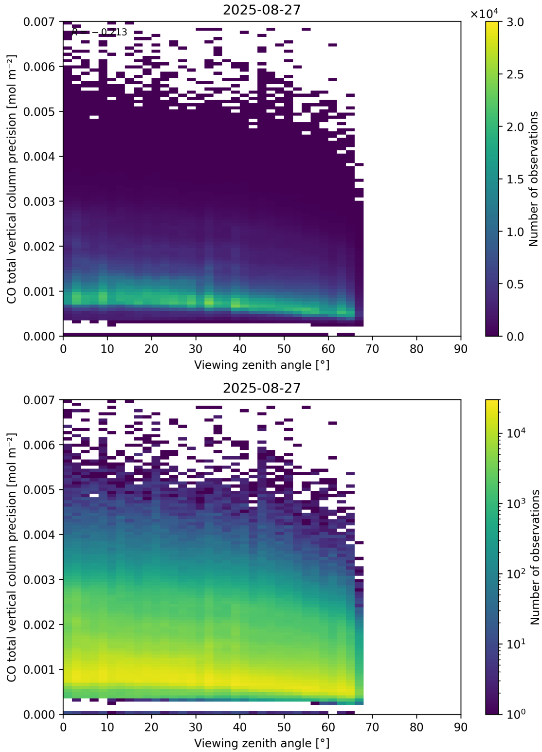
Figure 71: Scatter density plot of “Viewing zenith angle” against “CO total vertical column precision” for 2025-08-26 to 2025-08-28.
