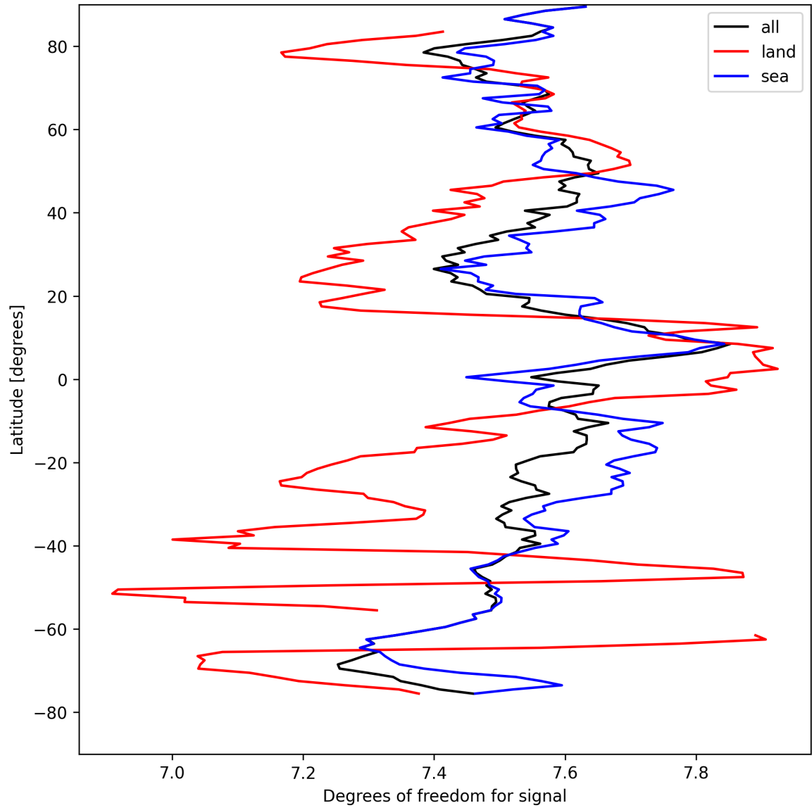
Figure 15: Zonal average of “Degrees of freedom for signal” for 2025-08-26 to 2025-08-28.
