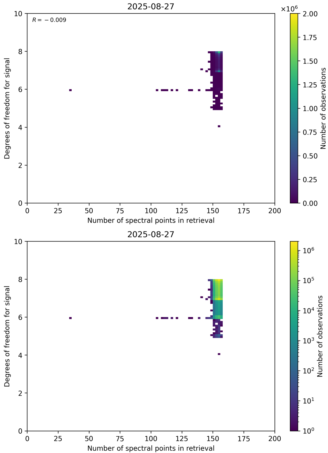
Figure 59: Scatter density plot of “Number of spectral points in retrieval” against “Degrees of freedom for signal” for 2025-08-26 to 2025-08-28.
