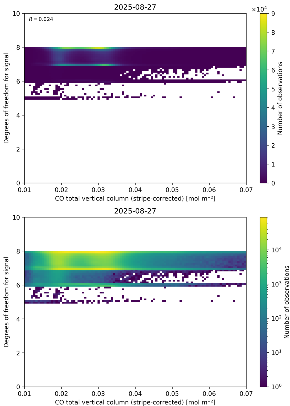
Figure 38: Scatter density plot of “CO total vertical column (stripe-corrected)” against “Degrees of freedom for signal” for 2025-08-26 to 2025-08-28.
