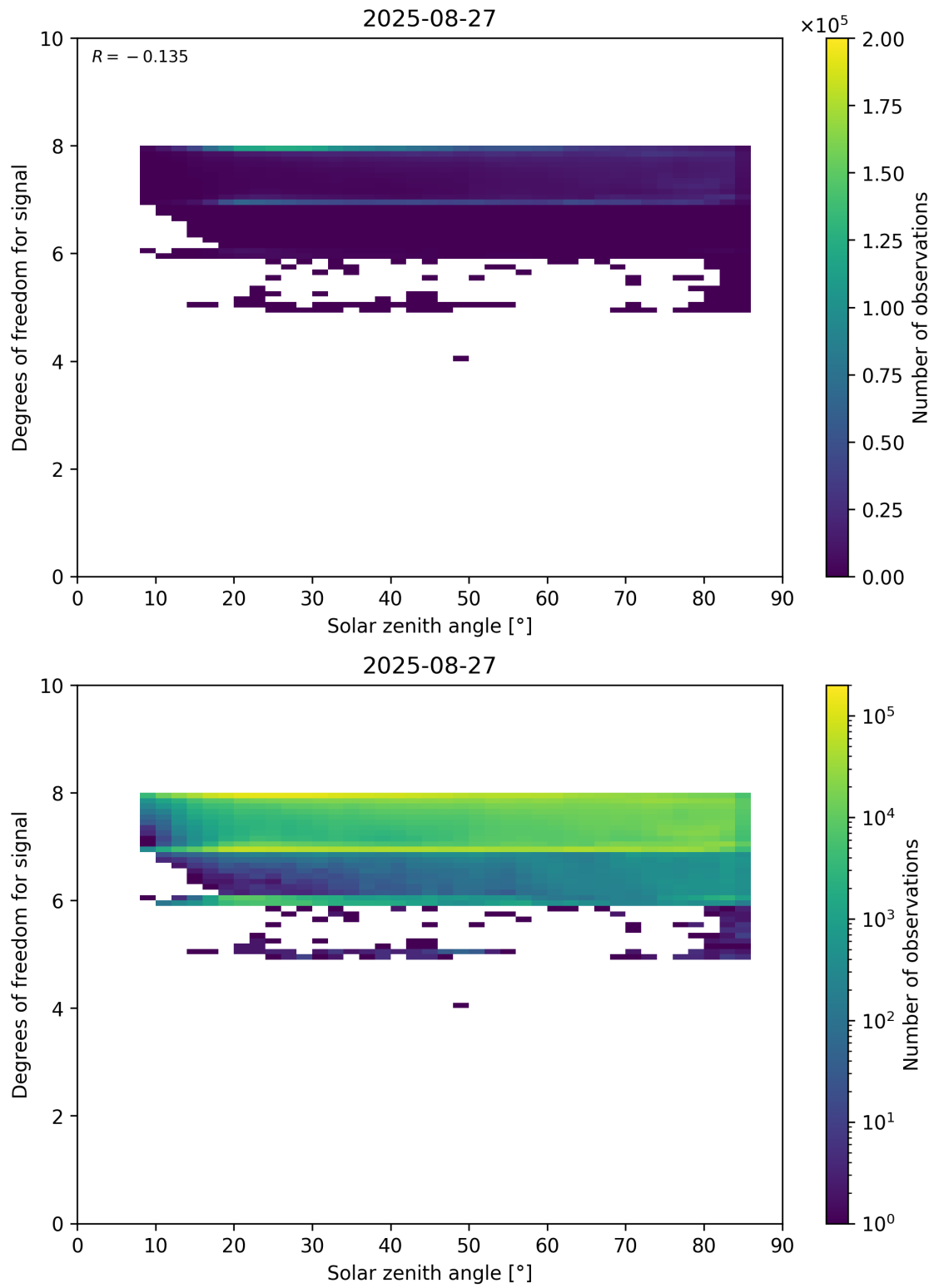
Figure 65: Scatter density plot of “Solar zenith angle” against “Degrees of freedom for signal” for 2025-08-26 to 2025-08-28.
