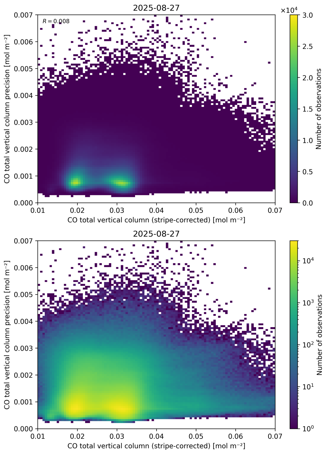
Figure 36: Scatter density plot of “CO total vertical column (stripe-corrected)” against “CO total vertical column precision” for 2025-08-26 to 2025-08-28.
