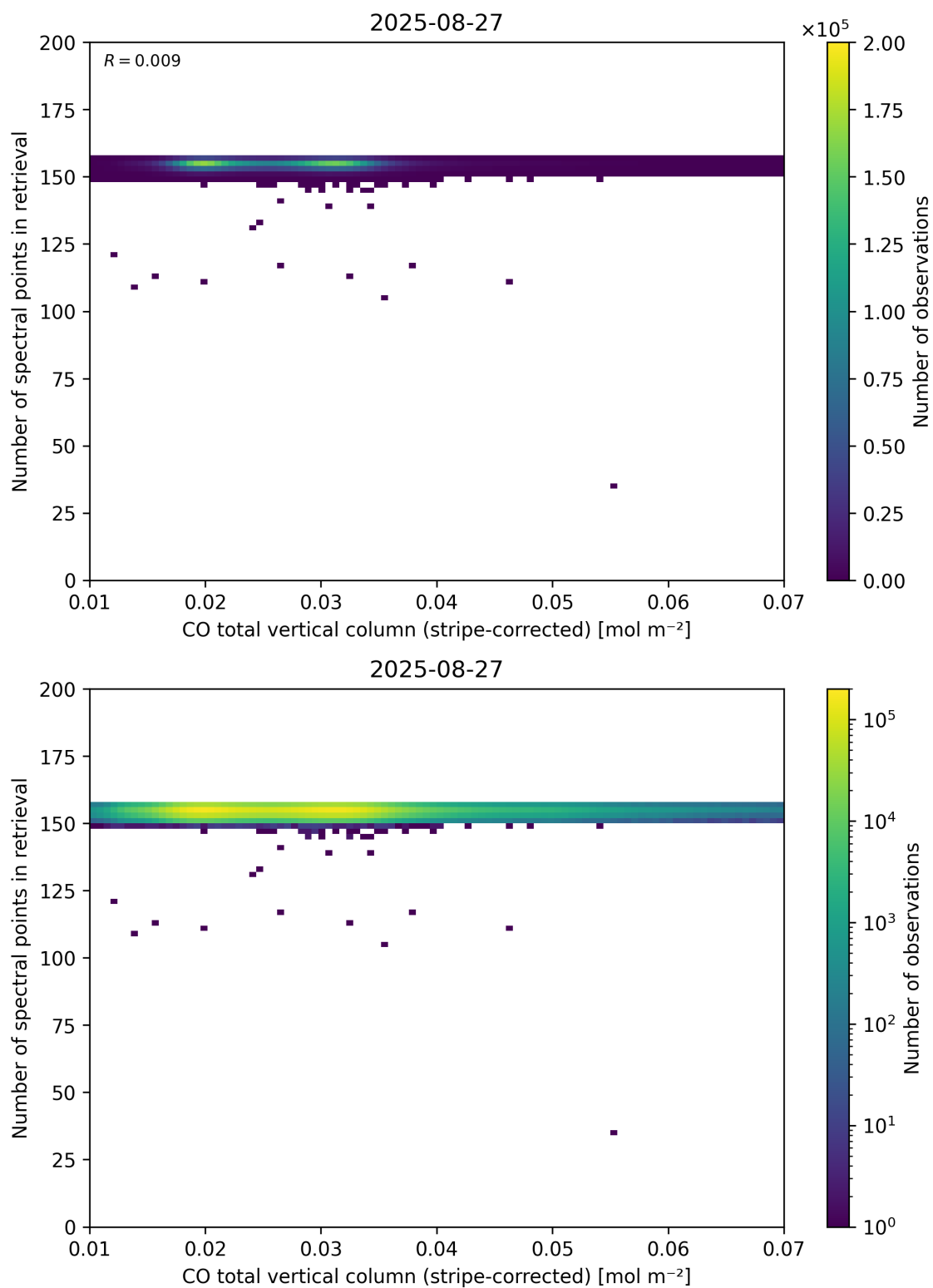
Figure 40: Scatter density plot of “CO total vertical column (stripe-corrected)” against “Number of spectral points in retrieval” for 2025-08-26 to 2025-08-28.
