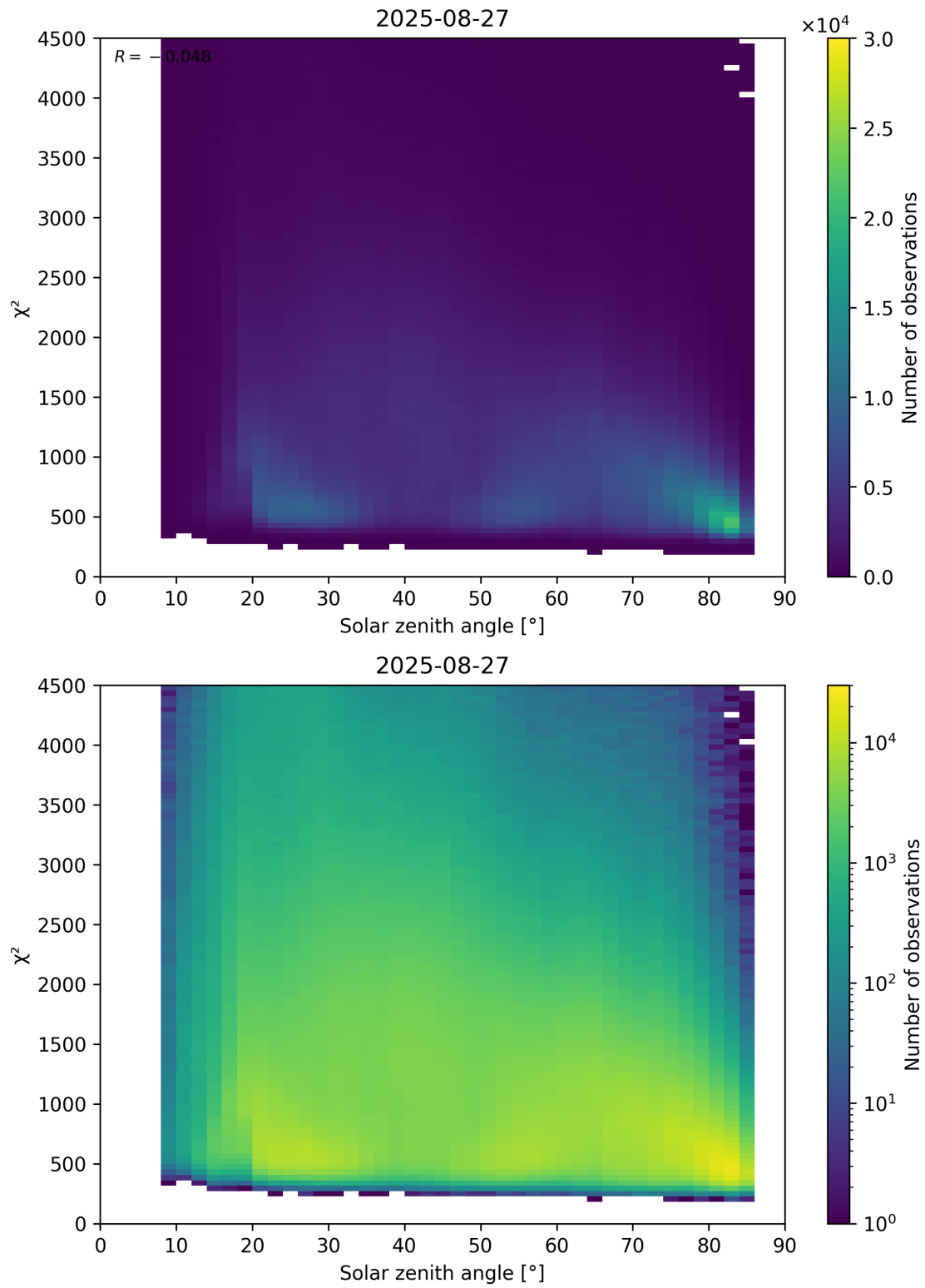
Figure 64: Scatter density plot of “Solar zenith angle” against “ \chi^2 ” for 2025-08-26 to 2025-08-28.
