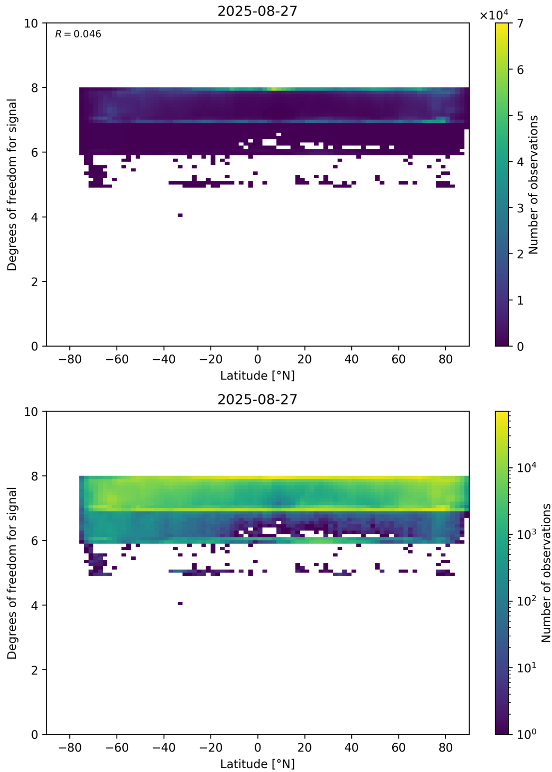
Figure 55: Scatter density plot of “Latitude” against “Degrees of freedom for signal” for 2025-08-26 to 2025-08-28.
