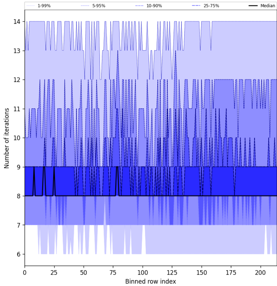
Figure 32: Along track statistics of “Number of iterations” for 2025-08-26 to 2025-08-28
