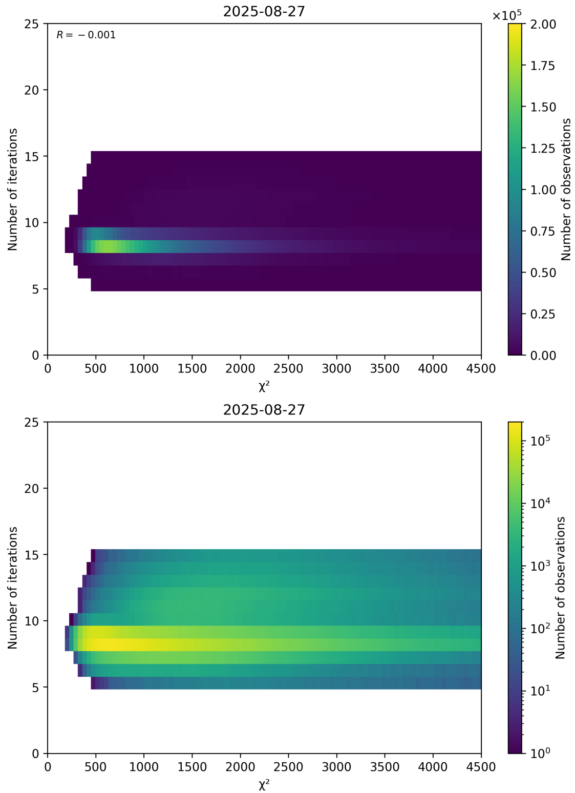
Figure 49: Scatter density plot of “ \chi^2 ” against “Number of iterations” for 2025-08-26 to 2025-08-28.
