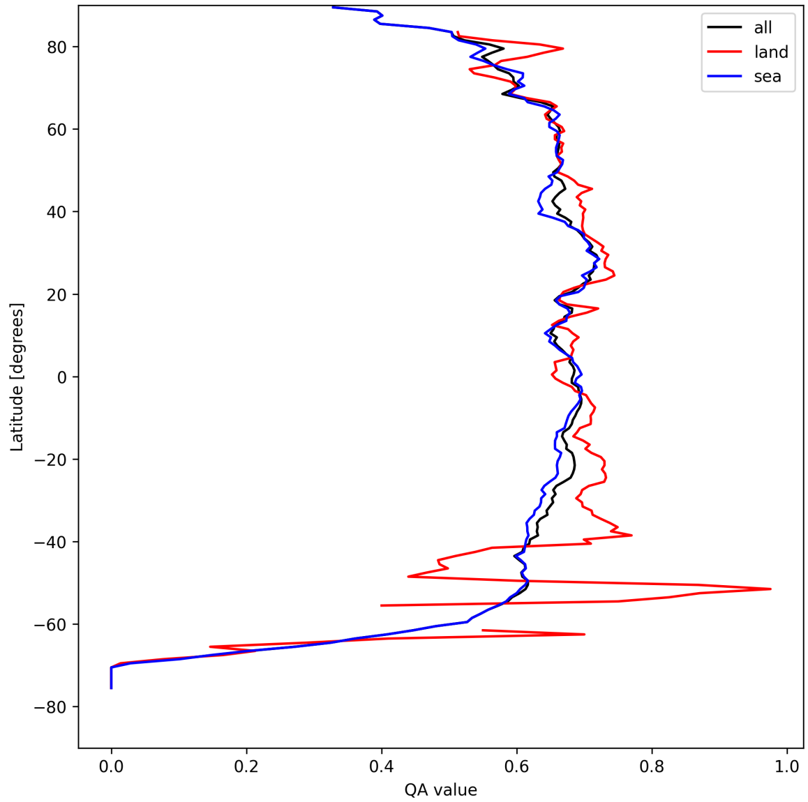
Figure 9: Zonal average of “QA value” for 2025-08-26 to 2025-08-28.
