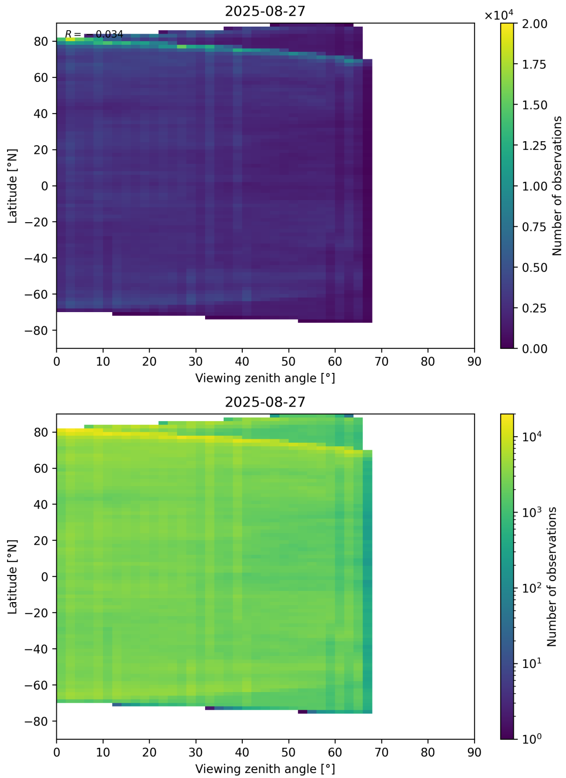
Figure 74: Scatter density plot of “Viewing zenith angle” against “Latitude” for 2025-08-26 to 2025-08-28.
