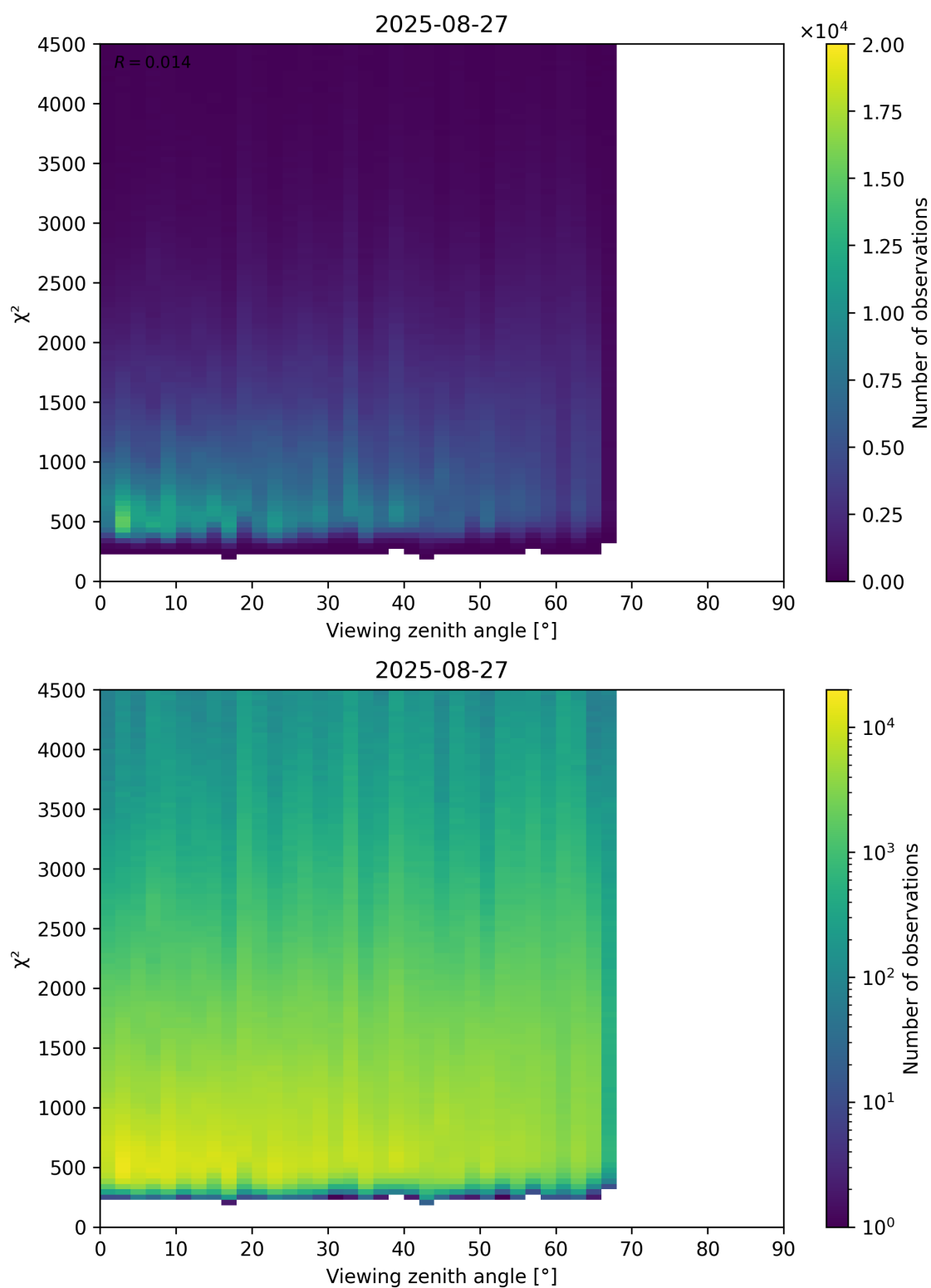
Figure 72: Scatter density plot of “Viewing zenith angle” against “ \chi^2 ” for 2025-08-26 to 2025-08-28.
