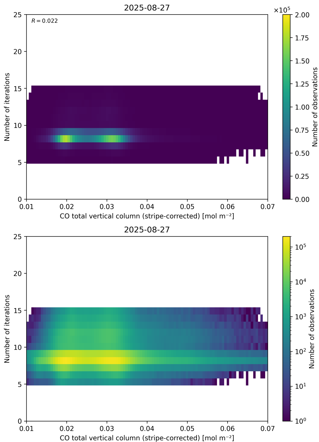
Figure 39: Scatter density plot of “CO total vertical column (stripe-corrected)” against “Number of iterations” for 2025-08-26 to 2025-08-28.
