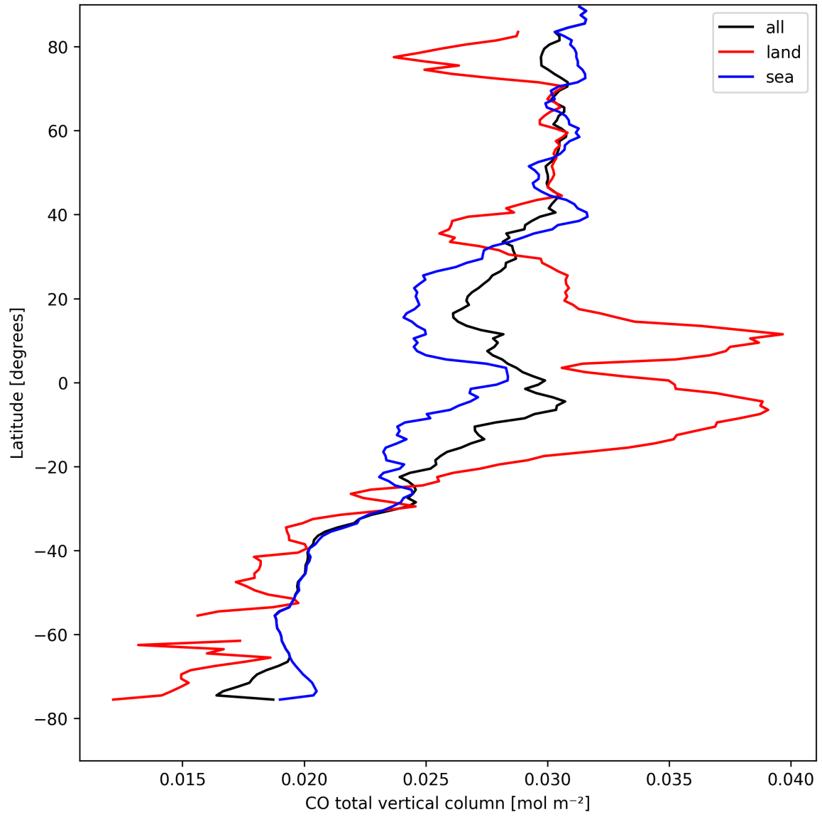
Figure 10: Zonal average of “CO total vertical column” for 2025-08-26 to 2025-08-28.
