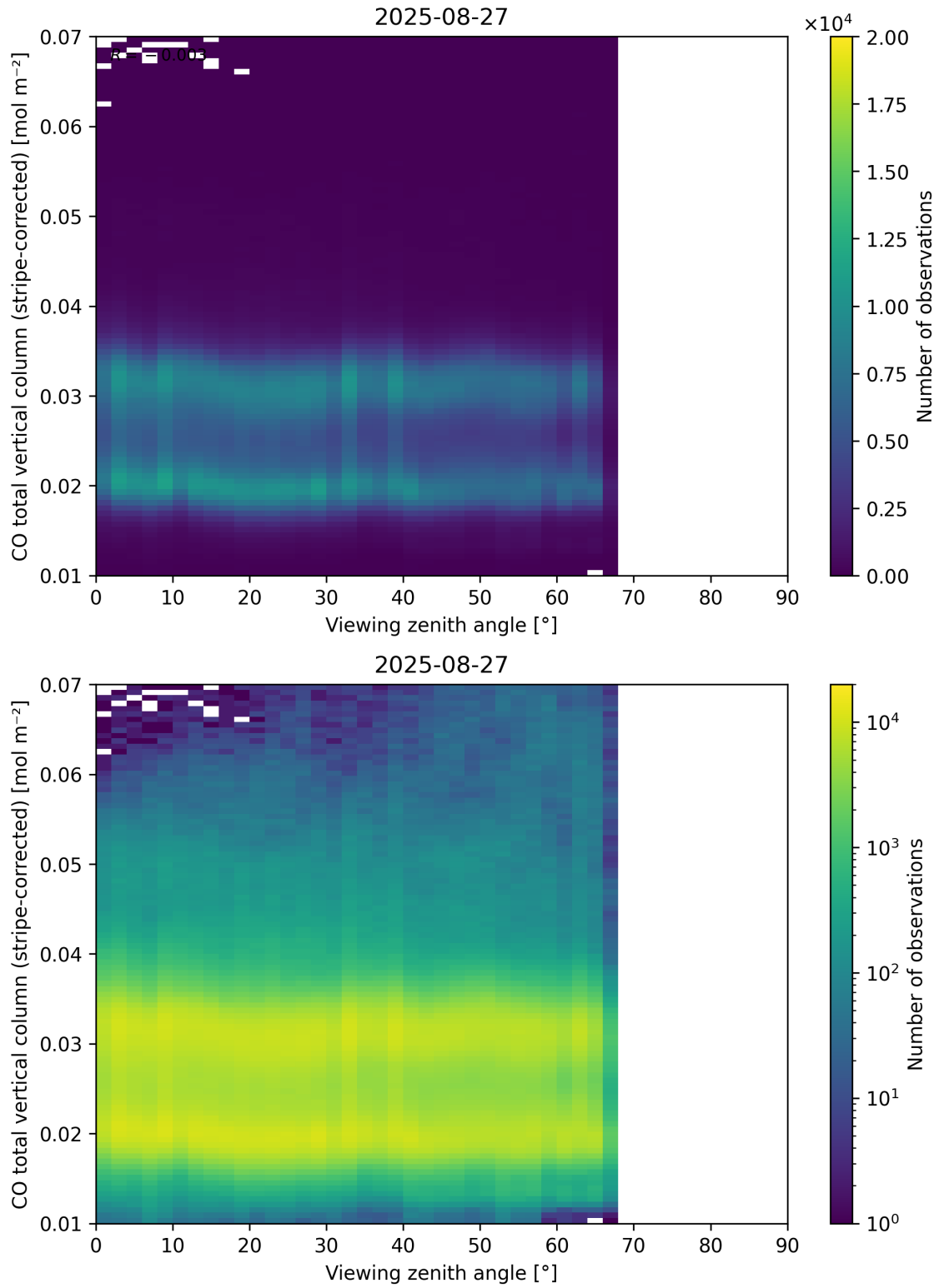
Figure 70: Scatter density plot of “Viewing zenith angle” against “CO total vertical column (stripe-corrected)” for 2025-08-26 to 2025-08-28.
