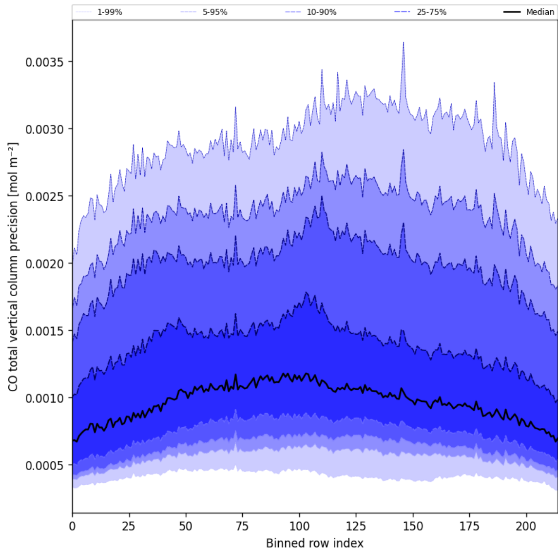
Figure 28: Along track statistics of “CO total vertical column precision” for 2025-08-26 to 2025-08-28
