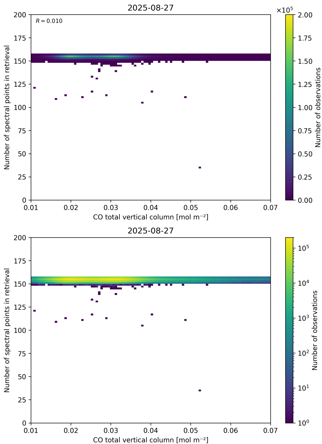
Figure 43: Scatter density plot of “CO total vertical column” against “Number of spectral points in retrieval” for 2025-08-26 to 2025-08-28.
