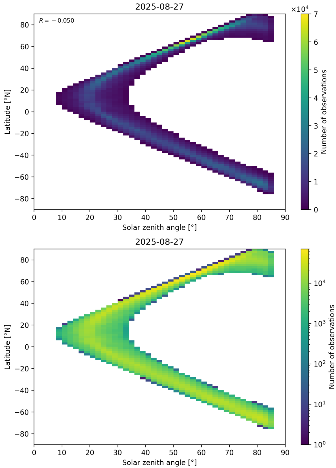
Figure 66: Scatter density plot of “Solar zenith angle” against “Latitude” for 2025-08-26 to 2025-08-28.
