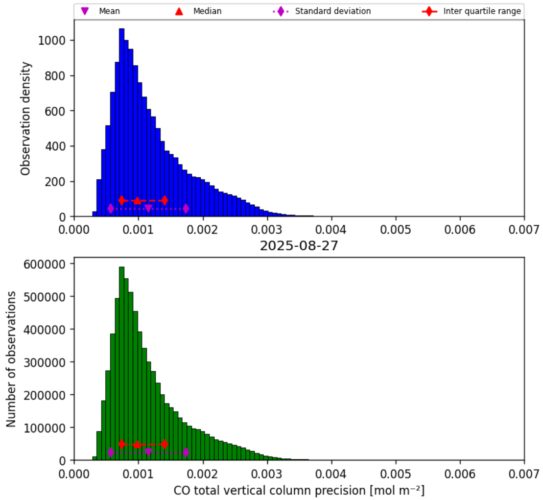
Figure 20: Histogram of “CO total vertical column precision” for 2025-08-26 to 2025-08-28
