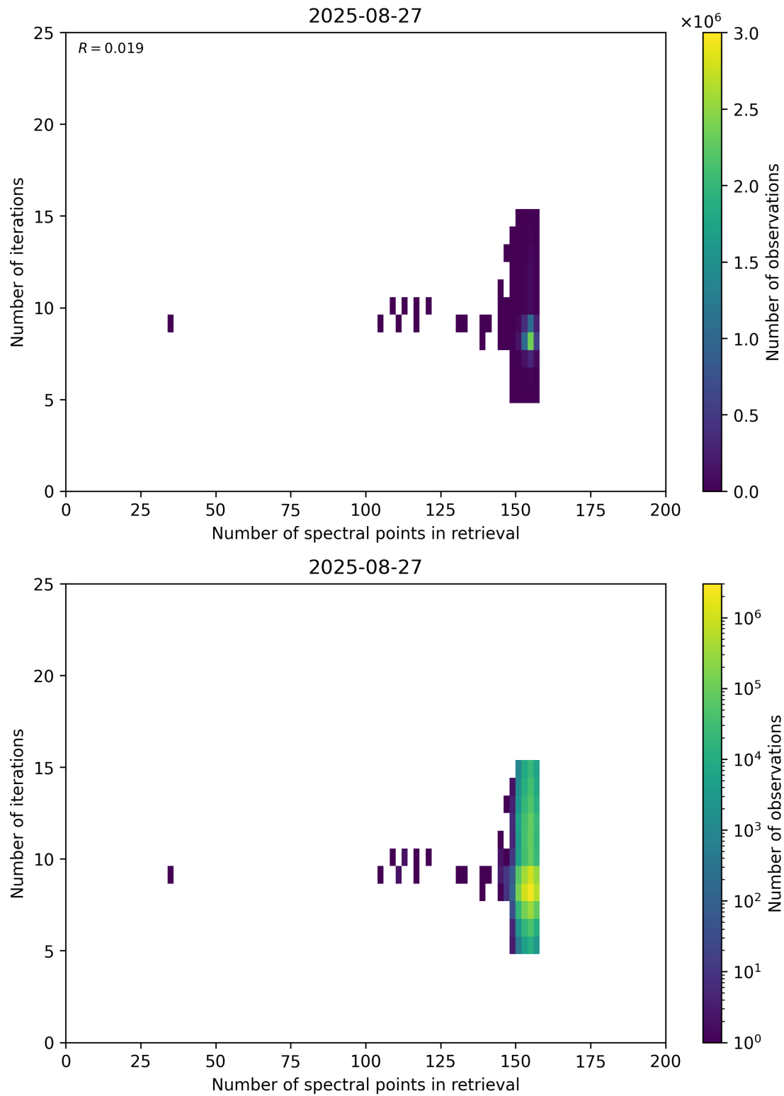
Figure 60: Scatter density plot of “Number of spectral points in retrieval” against “Number of iterations” for 2025-08-26 to 2025-08-28.
