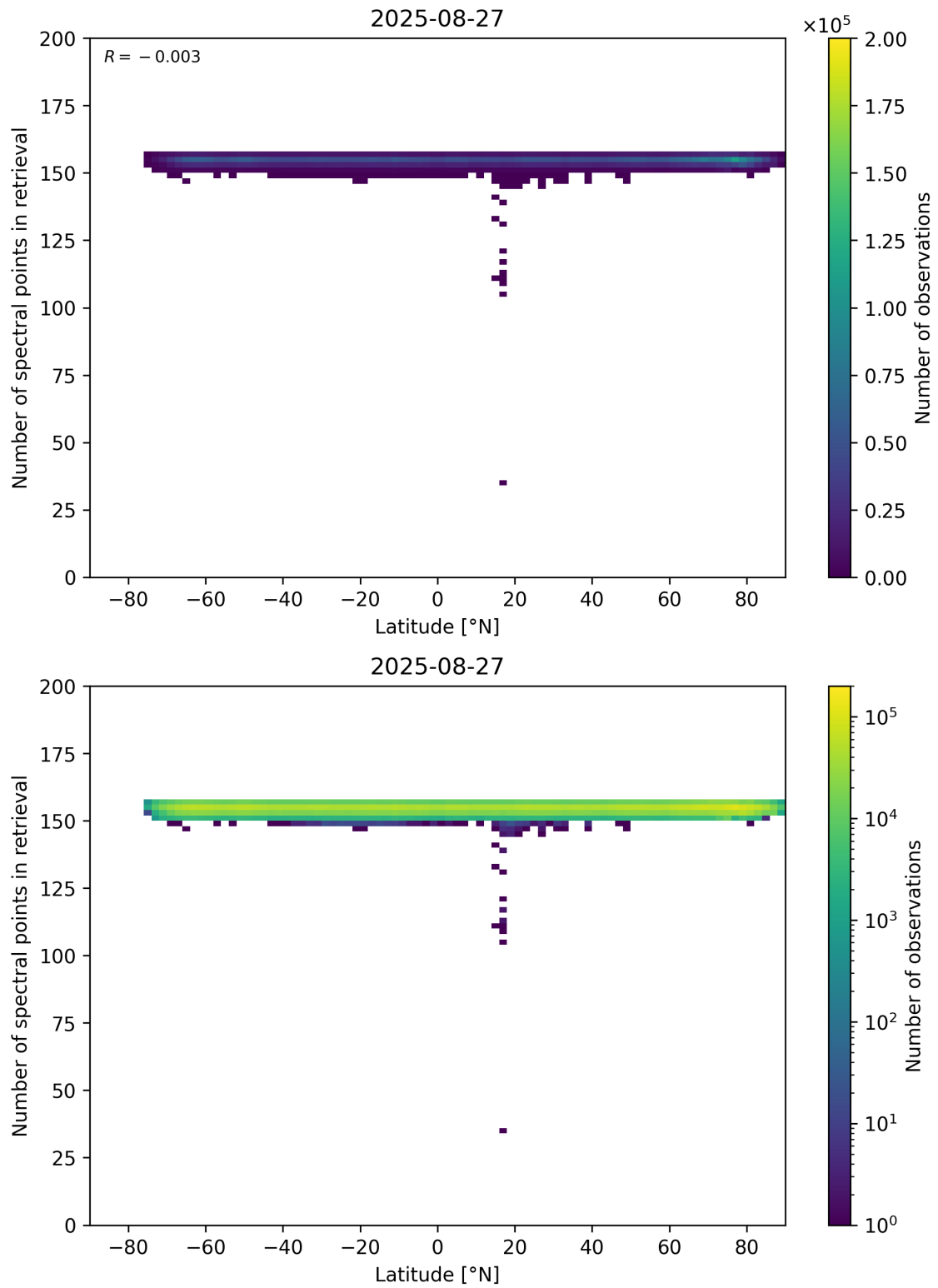
Figure 57: Scatter density plot of “Latitude” against “Number of spectral points in retrieval” for 2025-08-26 to 2025-08-28.
