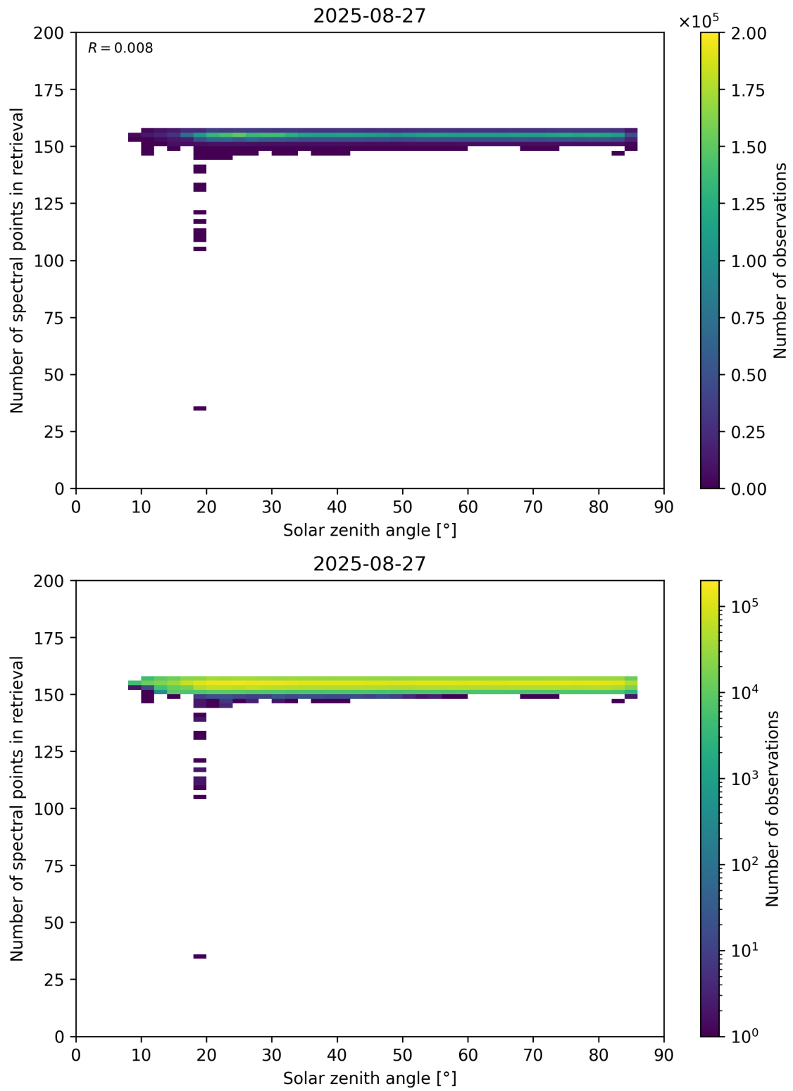
Figure 68: Scatter density plot of “Solar zenith angle” against “Number of spectral points in retrieval” for 2025-08-26 to 2025-08-28.
