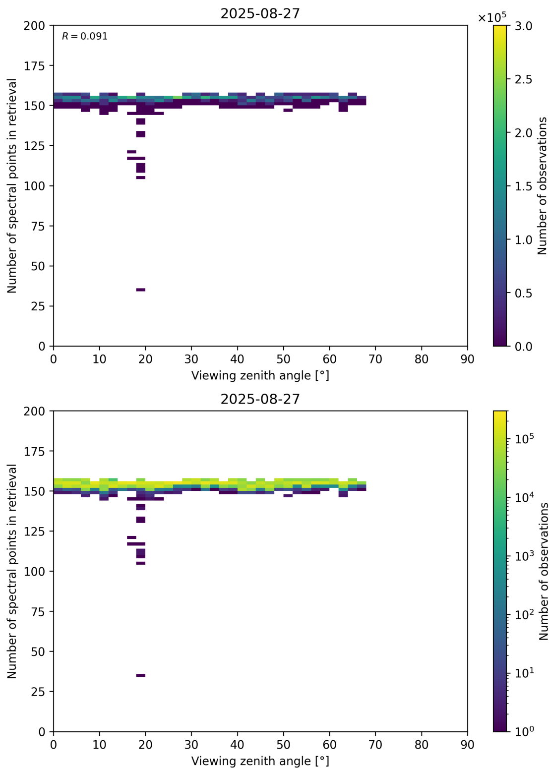
Figure 76: Scatter density plot of “Viewing zenith angle” against “Number of spectral points in retrieval” for 2025-08-26 to 2025-08-28.
