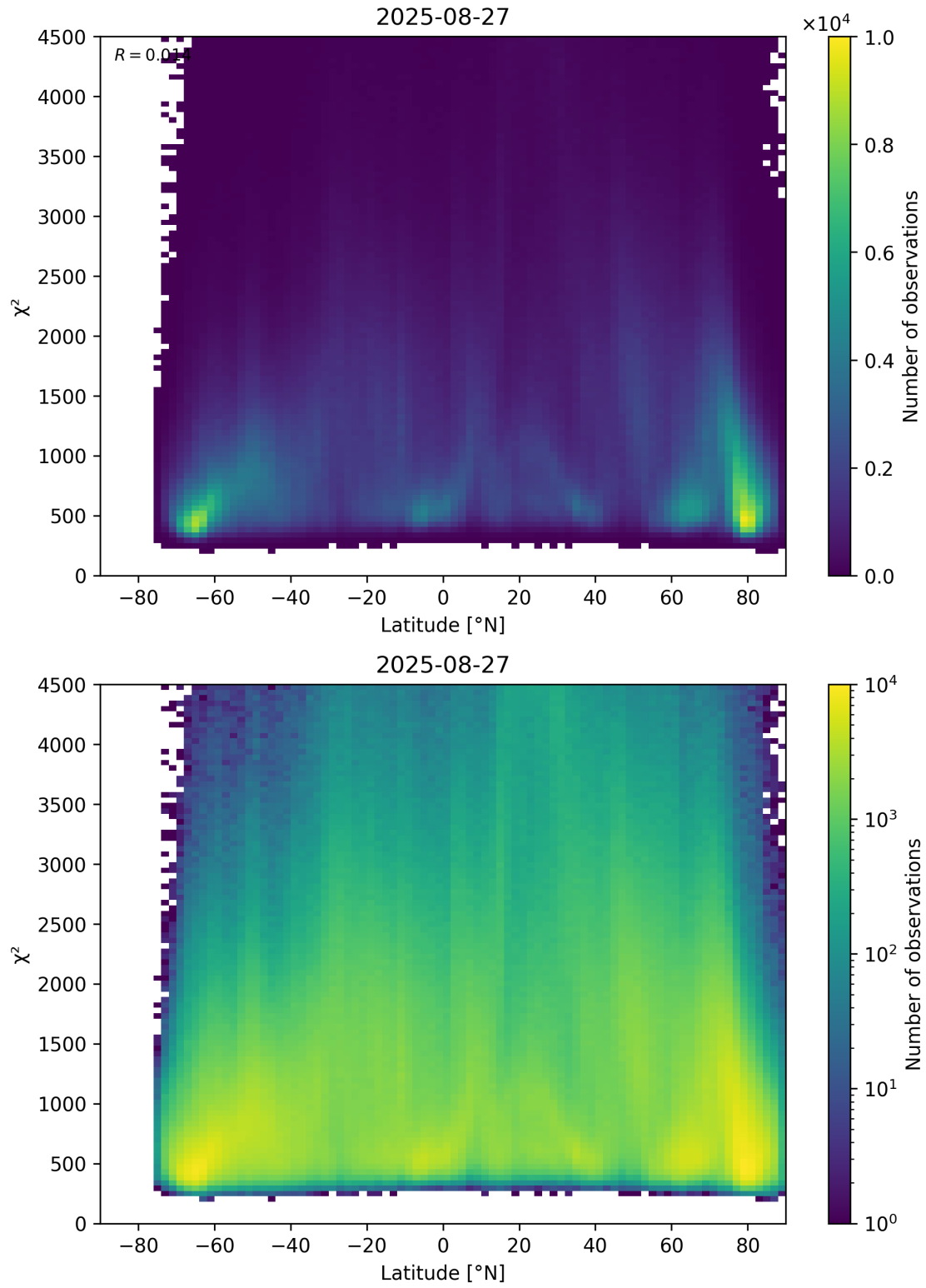
Figure 54: Scatter density plot of “Latitude” against “ \chi^2 ” for 2025-08-26 to 2025-08-28.
