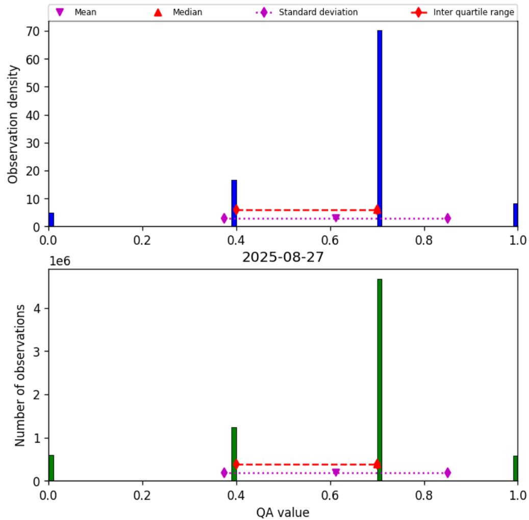
Figure 17: Histogram of “QA value” for 2025-08-26 to 2025-08-28
