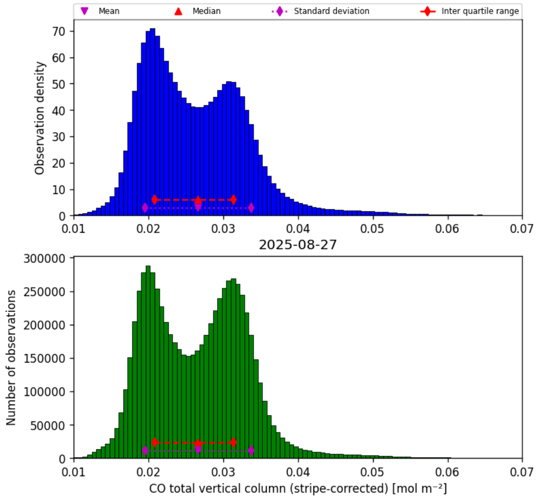
Figure 19: Histogram of “CO total vertical column (stripe-corrected)” for 2025-08-26 to 2025-08-28
