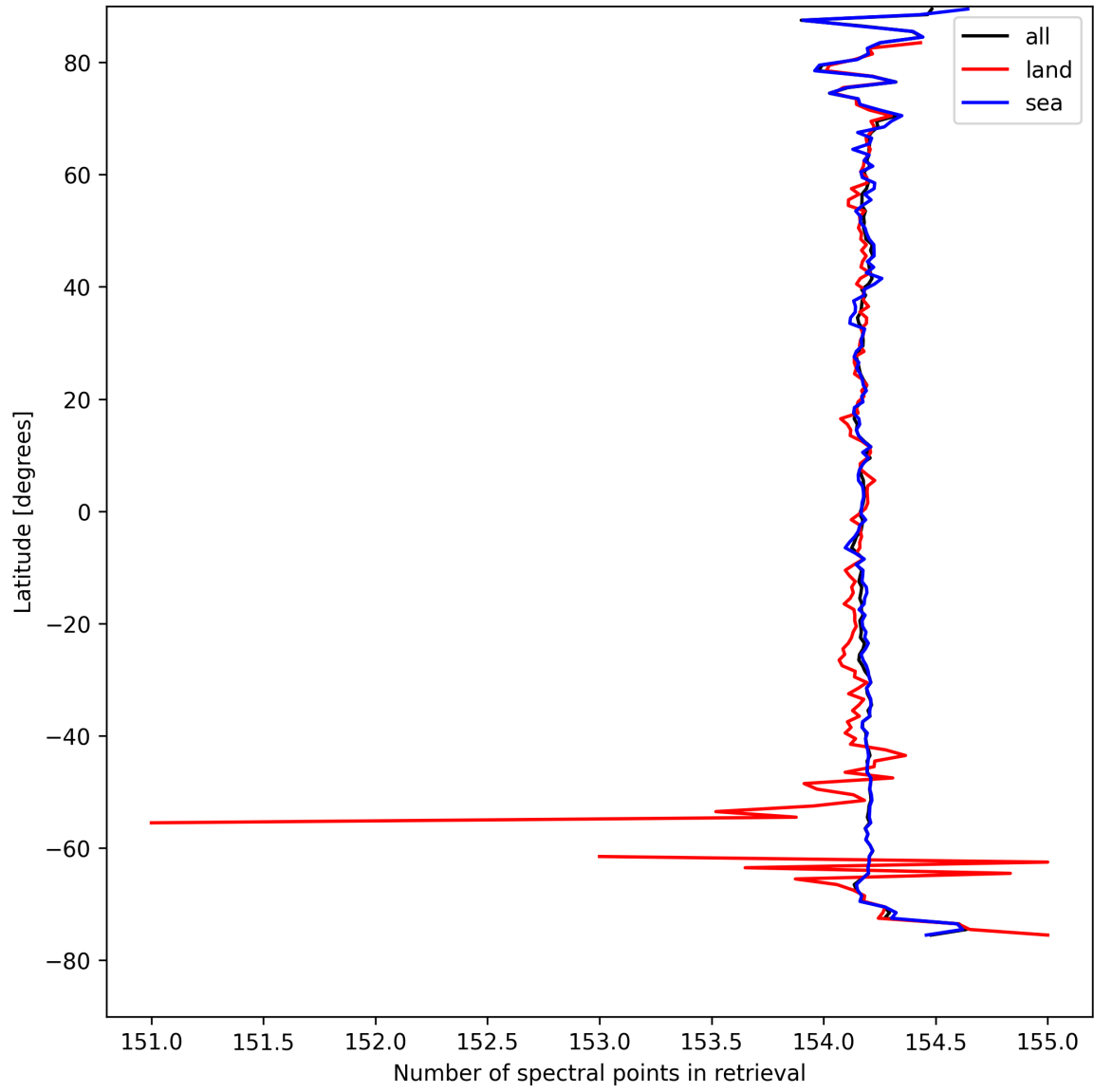
Figure 13: Zonal average of “Number of spectral points in retrieval” for 2025-08-26 to 2025-08-28.
