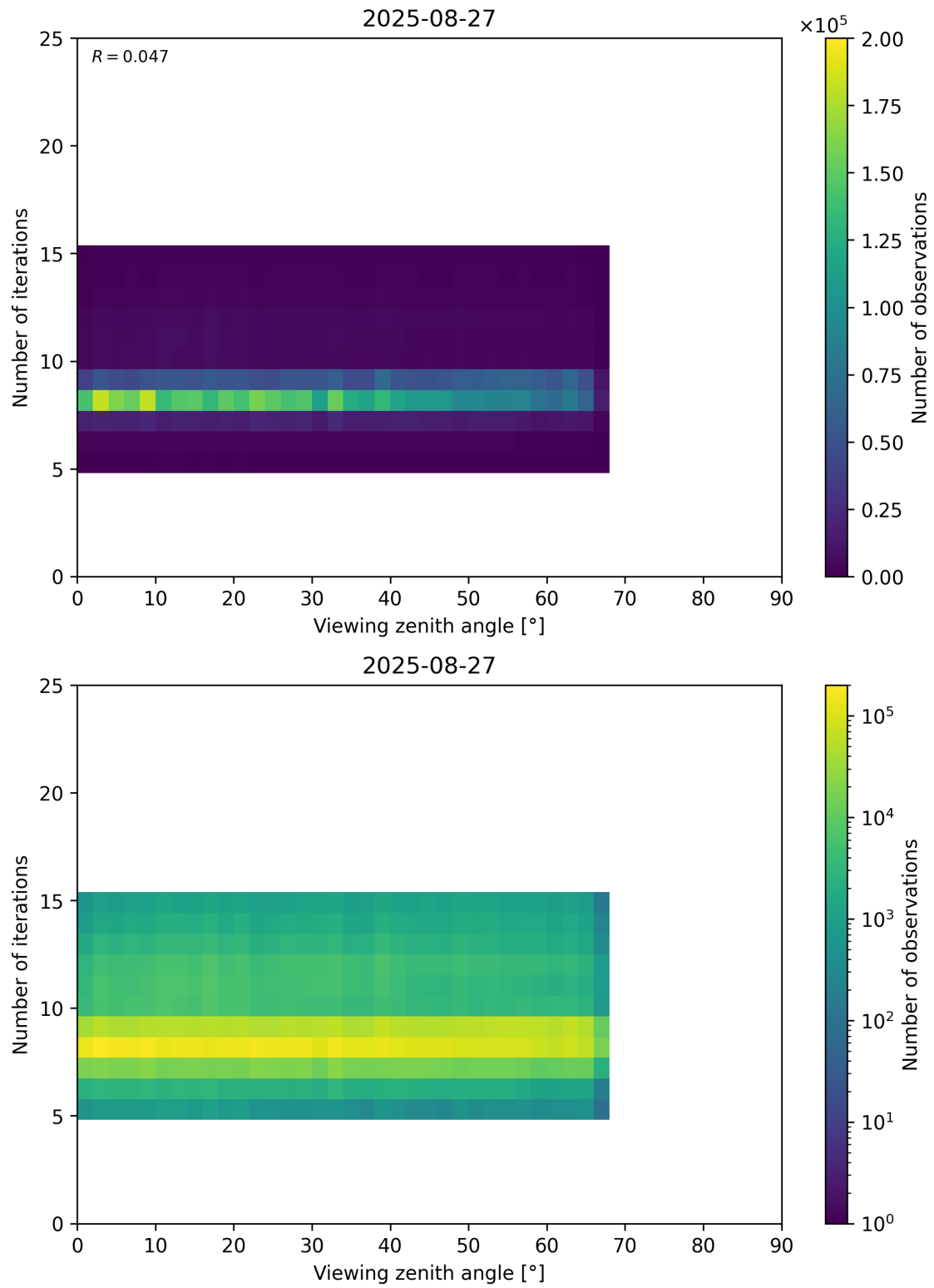
Figure 75: Scatter density plot of “Viewing zenith angle” against “Number of iterations” for 2025-08-26 to 2025-08-28.
