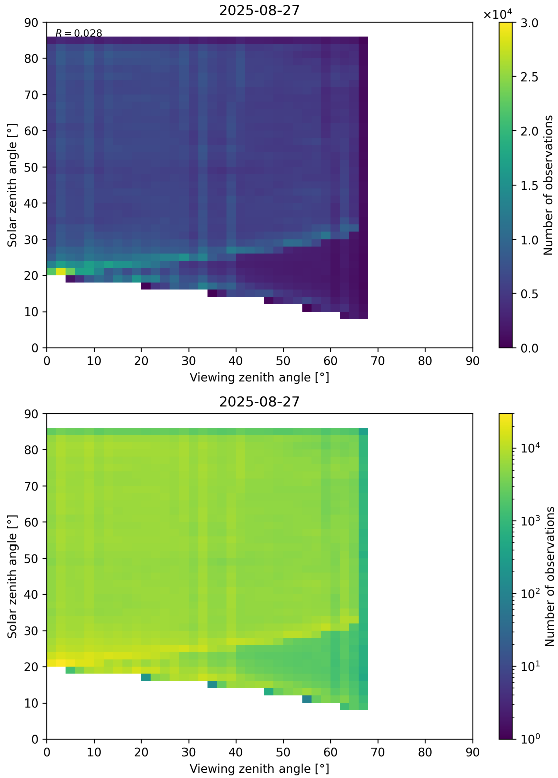
Figure 77: Scatter density plot of “Viewing zenith angle” against “Solar zenith angle” for 2025-08-26 to 2025-08-28.
