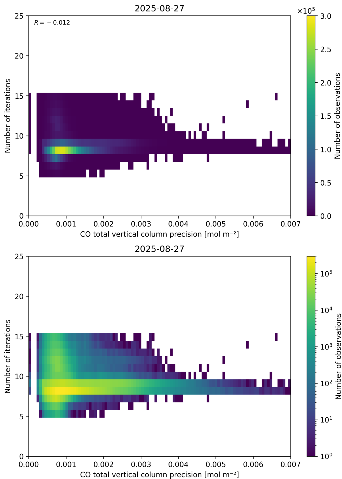
Figure 46: Scatter density plot of “CO total vertical column precision” against “Number of iterations” for 2025-08-26 to 2025-08-28.
