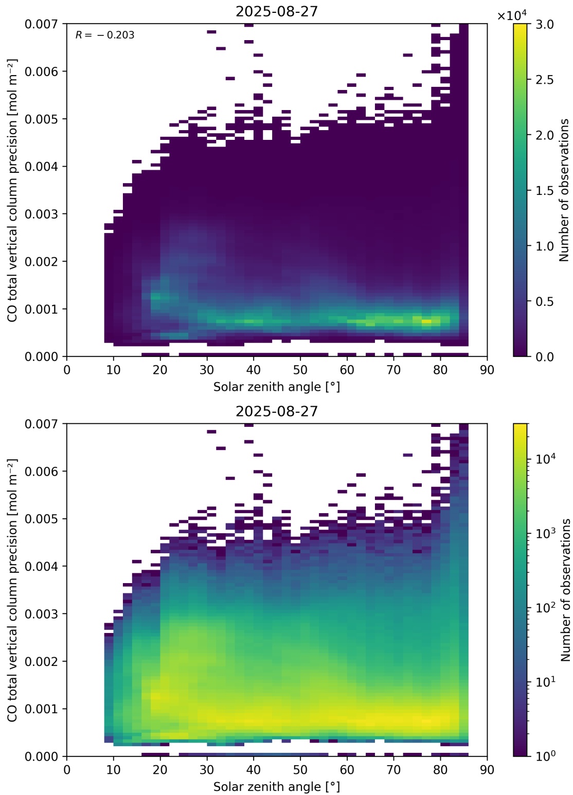
Figure 63: Scatter density plot of “Solar zenith angle” against “CO total vertical column precision” for 2025-08-26 to 2025-08-28.
