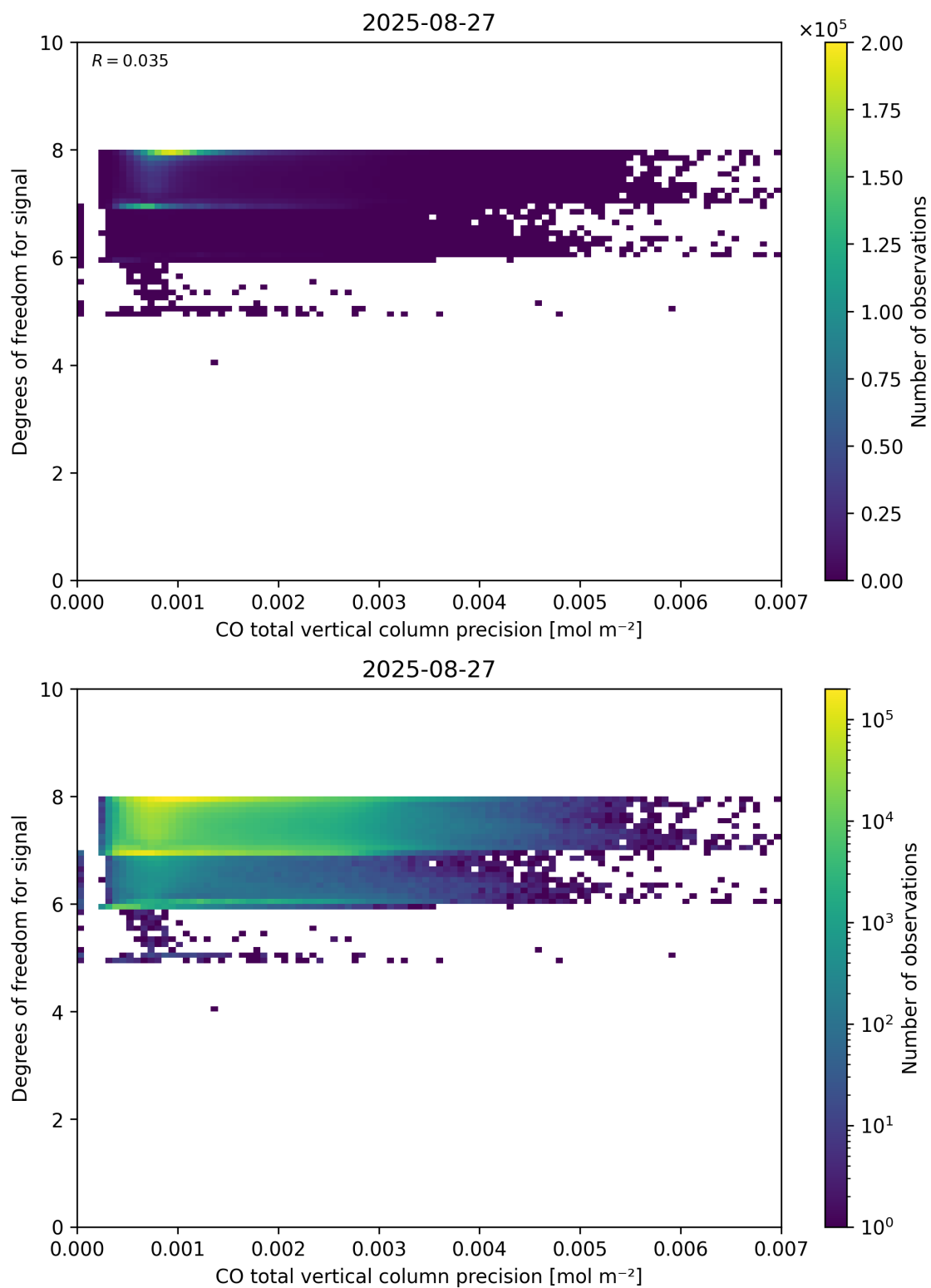
Figure 45: Scatter density plot of “CO total vertical column precision” against “Degrees of freedom for signal” for 2025-08-26 to 2025-08-28.
