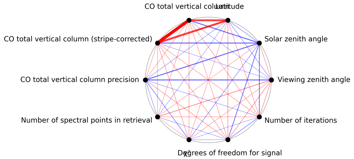
Figure 1: Map of correlation graph for 2025-08-26 to 2025-08-28.
