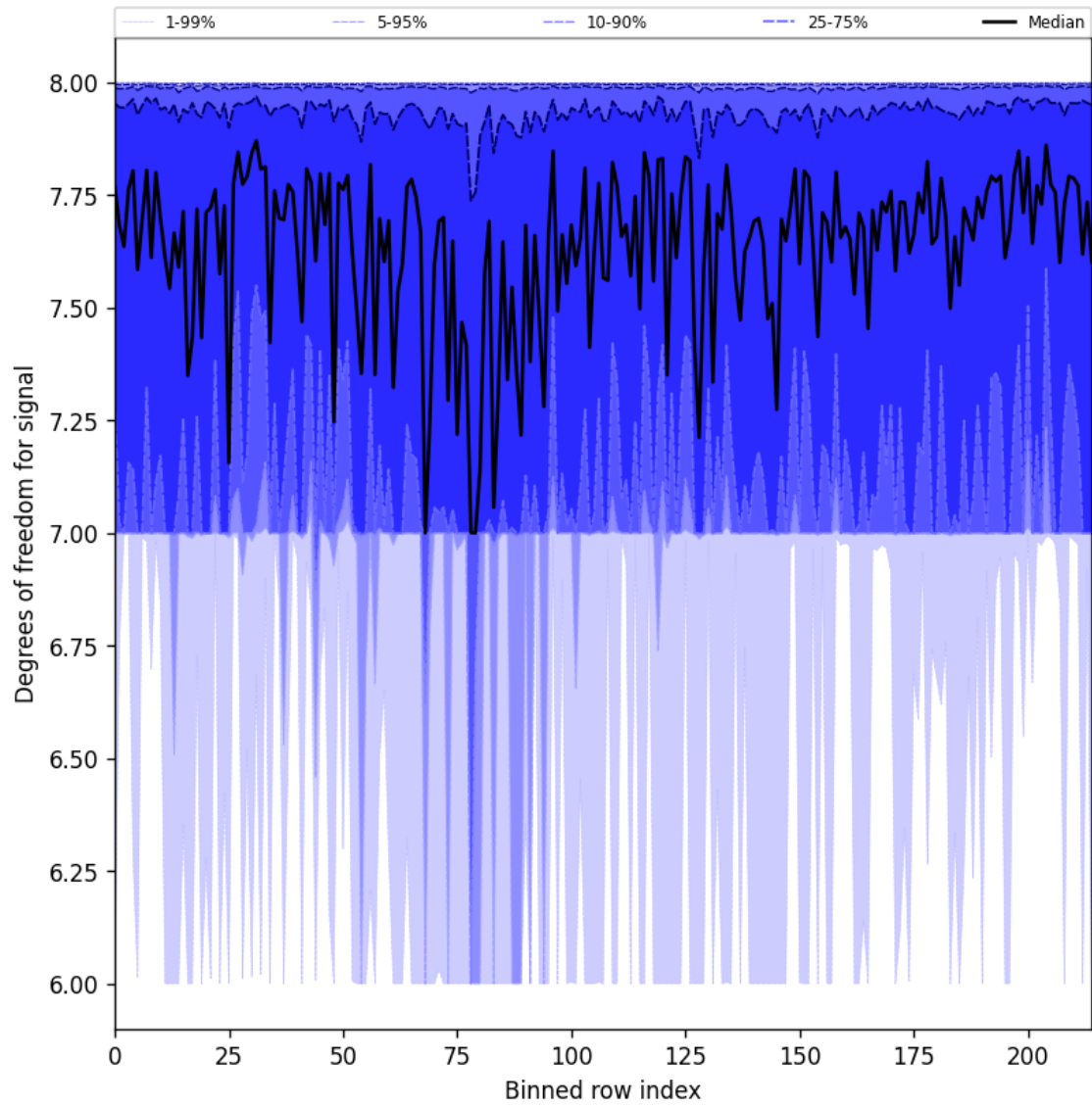
Figure 31: Along track statistics of “Degrees of freedom for signal” for 2025-08-26 to 2025-08-28
