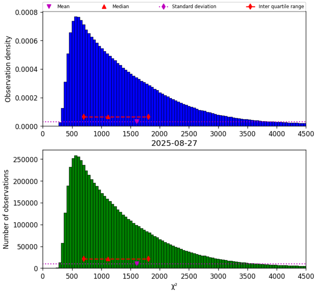
Figure 22: Histogram of “ \chi^2 ” for 2025-08-26 to 2025-08-28
