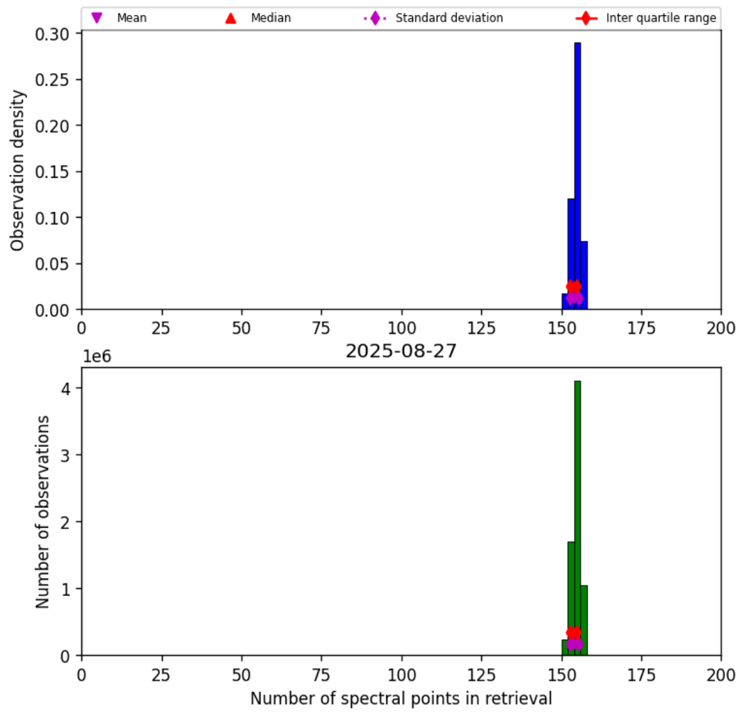
Figure 21: Histogram of “Number of spectral points in retrieval” for 2025-08-26 to 2025-08-28
