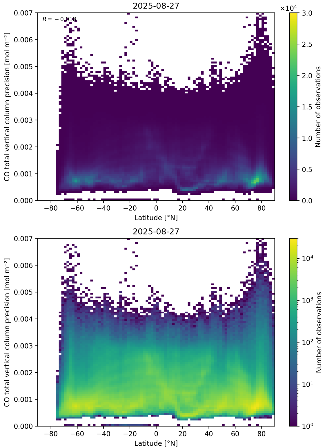
Figure 53: Scatter density plot of “Latitude” against “CO total vertical column precision” for 2025-08-26 to 2025-08-28.
