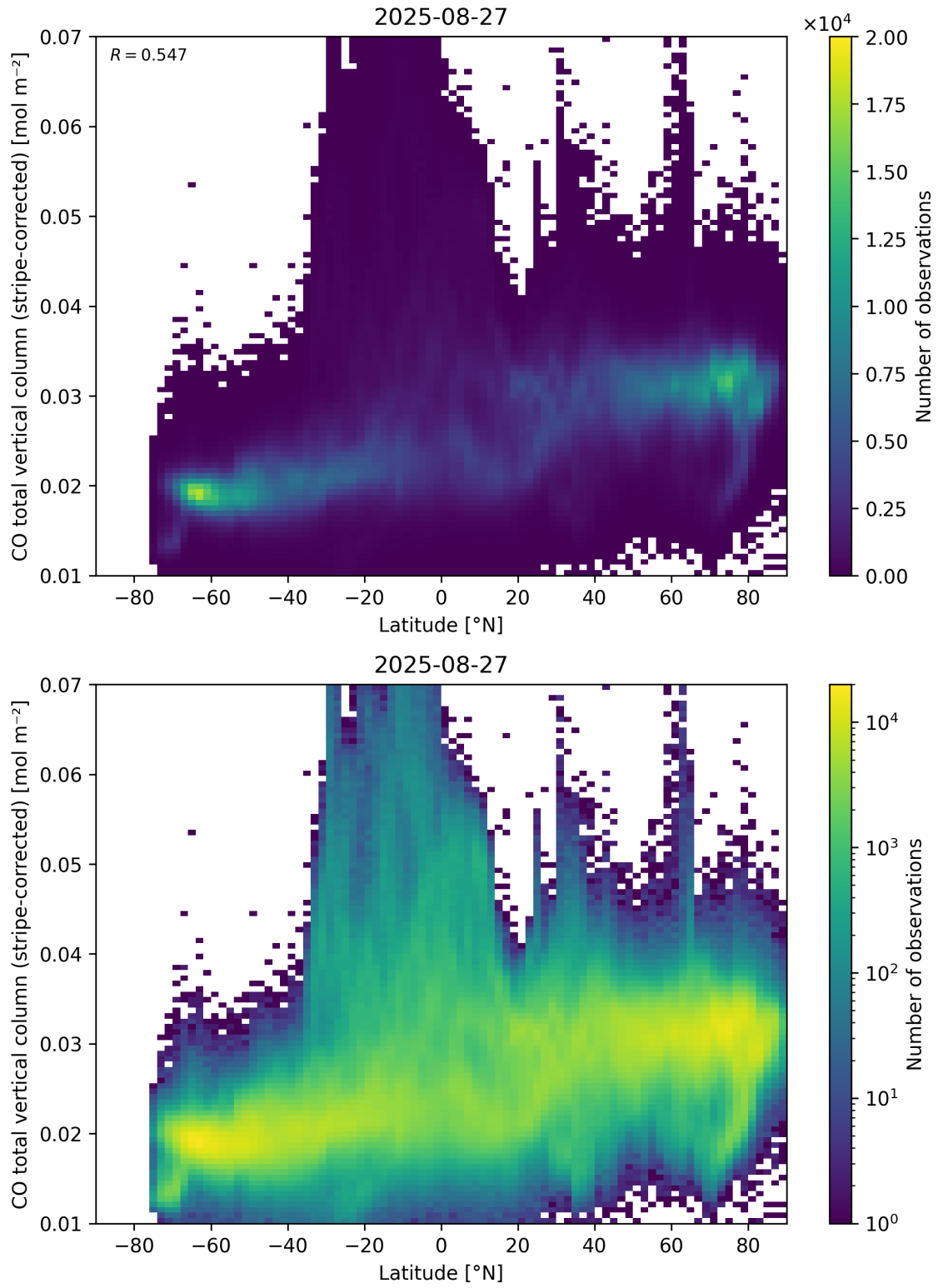
Figure 52: Scatter density plot of “Latitude” against “CO total vertical column (stripe-corrected)” for 2025-08-26 to 2025-08-28.
