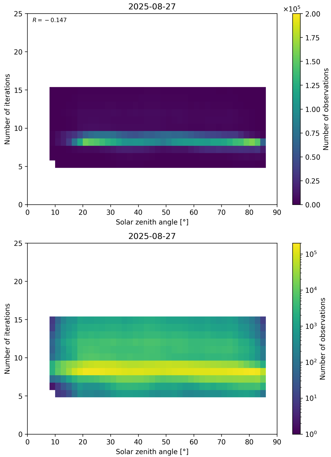
Figure 67: Scatter density plot of “Solar zenith angle” against “Number of iterations” for 2025-08-26 to 2025-08-28.
