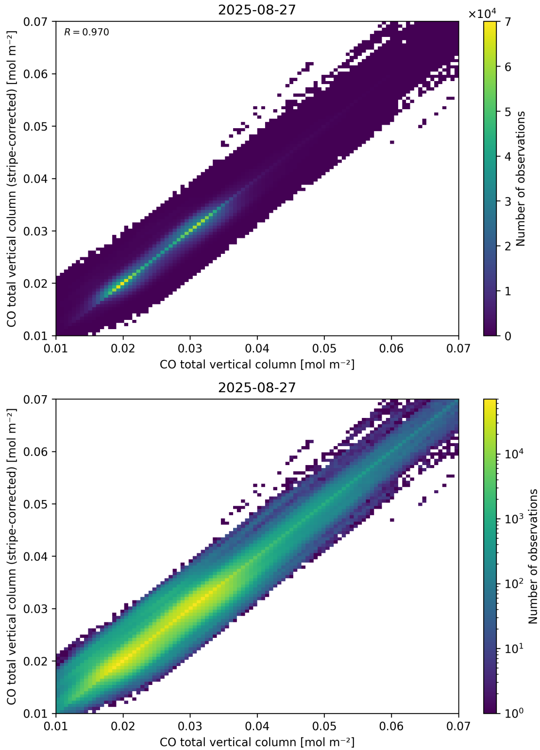
Figure 33: Scatter density plot of “CO total vertical column” against “CO total vertical column (stripe-corrected)” for 2025-08-26 to 2025-08-28.
