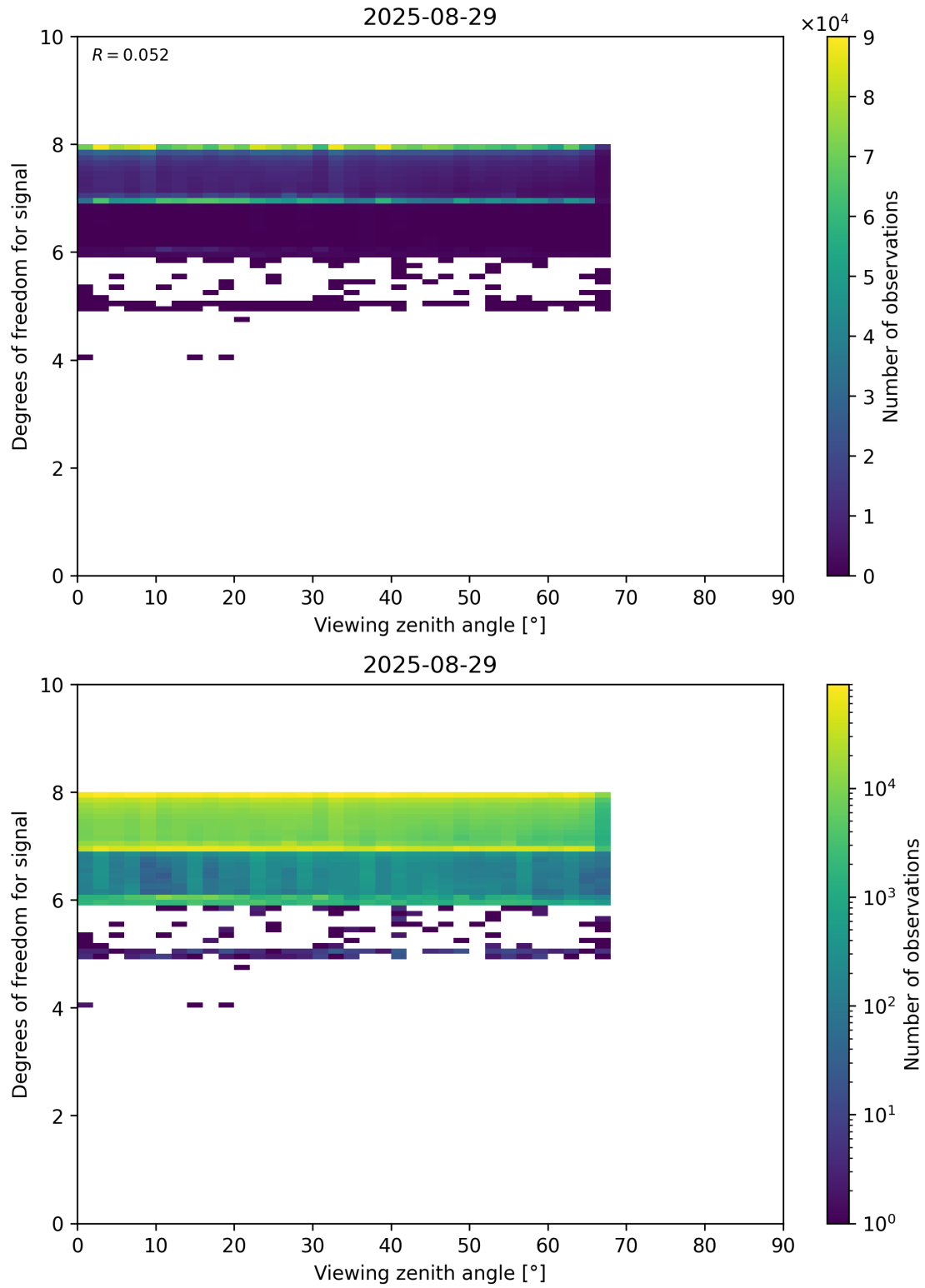
Figure 73: Scatter density plot of “Viewing zenith angle” against “Degrees of freedom for signal” for 2025-08-28 to 2025-08-30.
