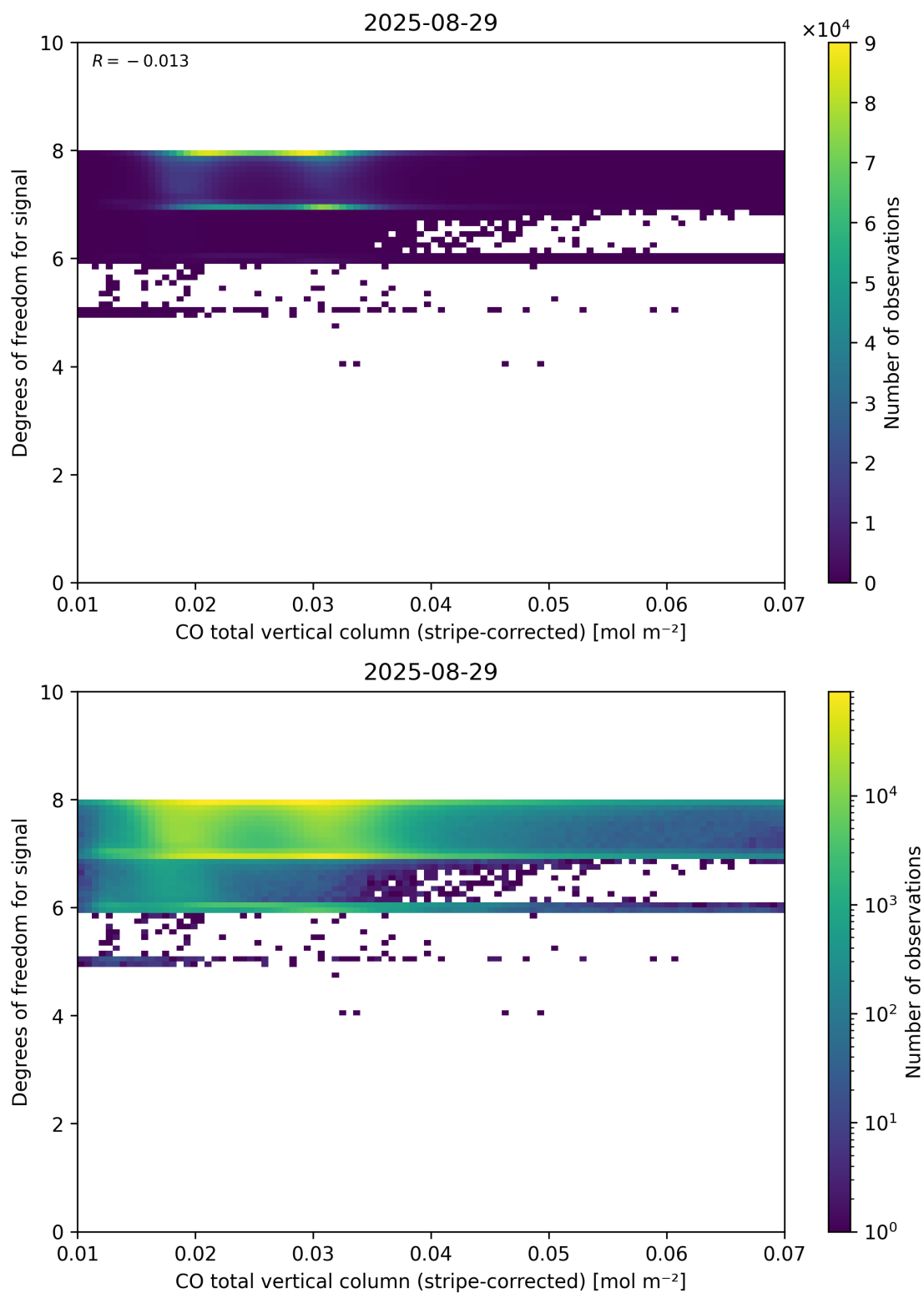
Figure 38: Scatter density plot of “CO total vertical column (stripe-corrected)” against “Degrees of freedom for signal” for 2025-08-28 to 2025-08-30.
