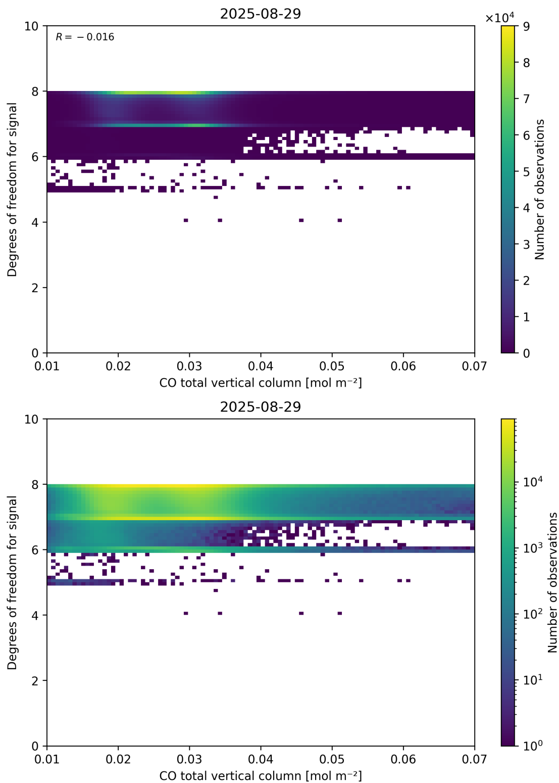
Figure 41: Scatter density plot of “CO total vertical column” against “Degrees of freedom for signal” for 2025-08-28 to 2025-08-30.
