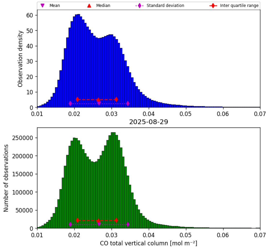
Figure 18: Histogram of “CO total vertical column” for 2025-08-28 to 2025-08-30
