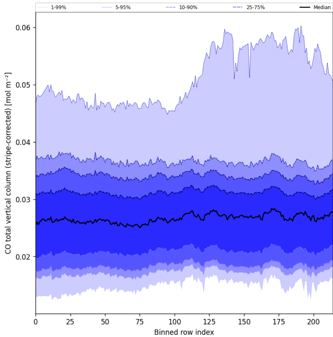
Figure 27: Along track statistics of “CO total vertical column (stripe-corrected)” for 2025-08-28 to 2025-08-30
