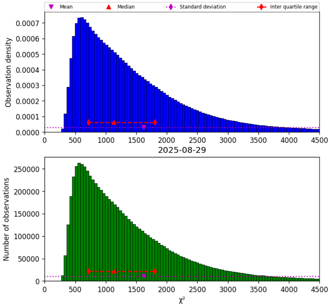
Figure 22: Histogram of “ \chi^2 ” for 2025-08-28 to 2025-08-30
