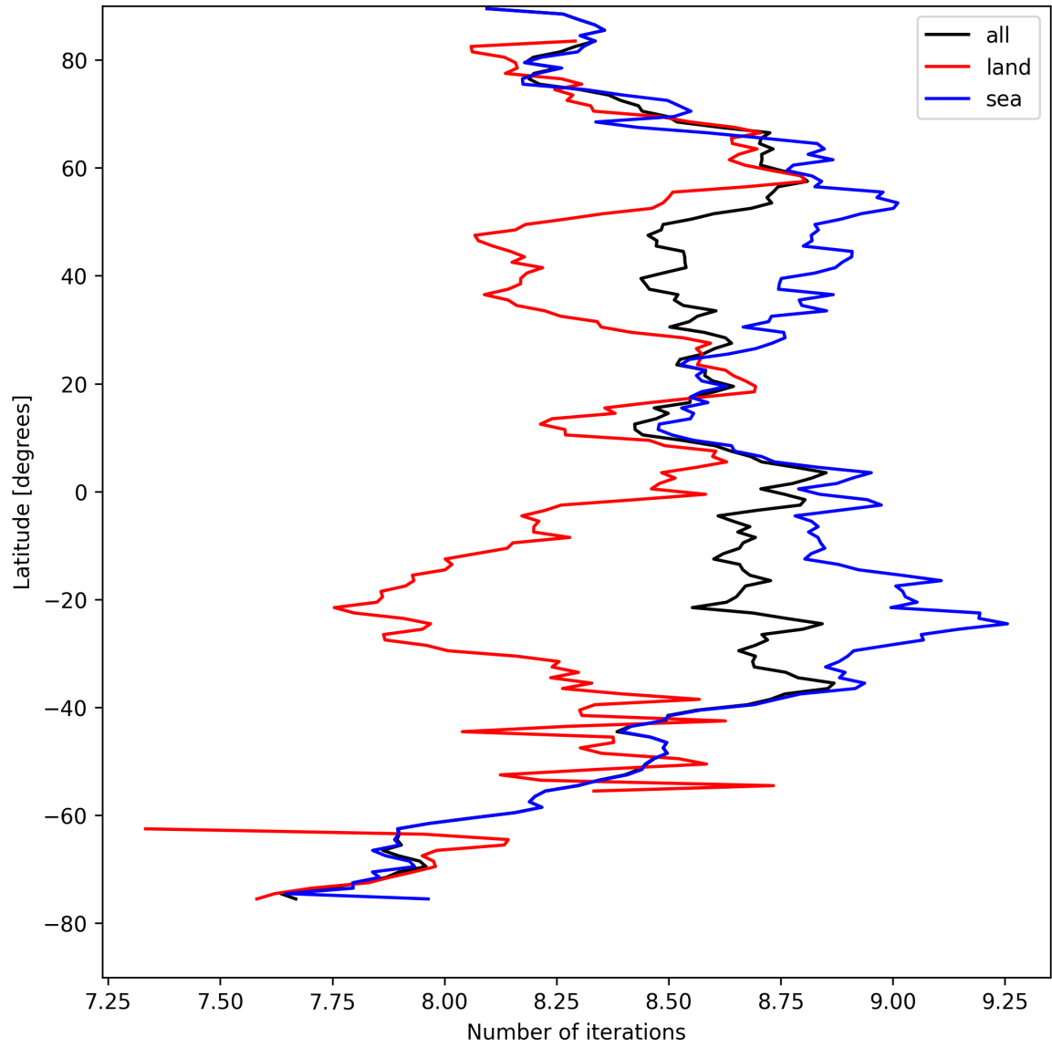
Figure 16: Zonal average of “Number of iterations” for 2025-08-28 to 2025-08-30.
