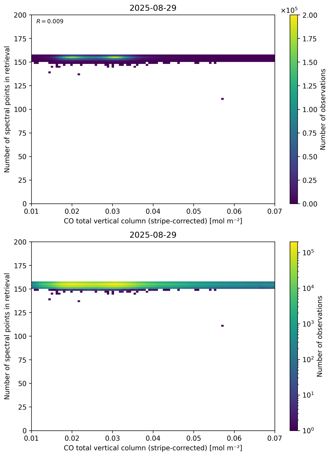
Figure 40: Scatter density plot of “CO total vertical column (stripe-corrected)” against “Number of spectral points in retrieval” for 2025-08-28 to 2025-08-30.
