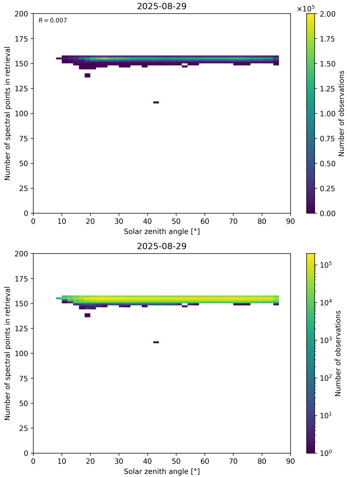
Figure 68: Scatter density plot of “Solar zenith angle” against “Number of spectral points in retrieval” for 2025-08-28 to 2025-08-30.
