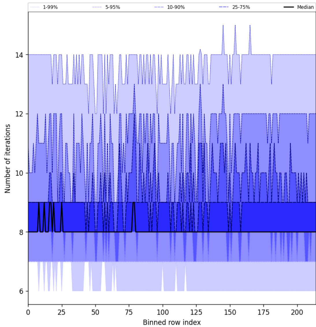
Figure 32: Along track statistics of “Number of iterations” for 2025-08-28 to 2025-08-30
