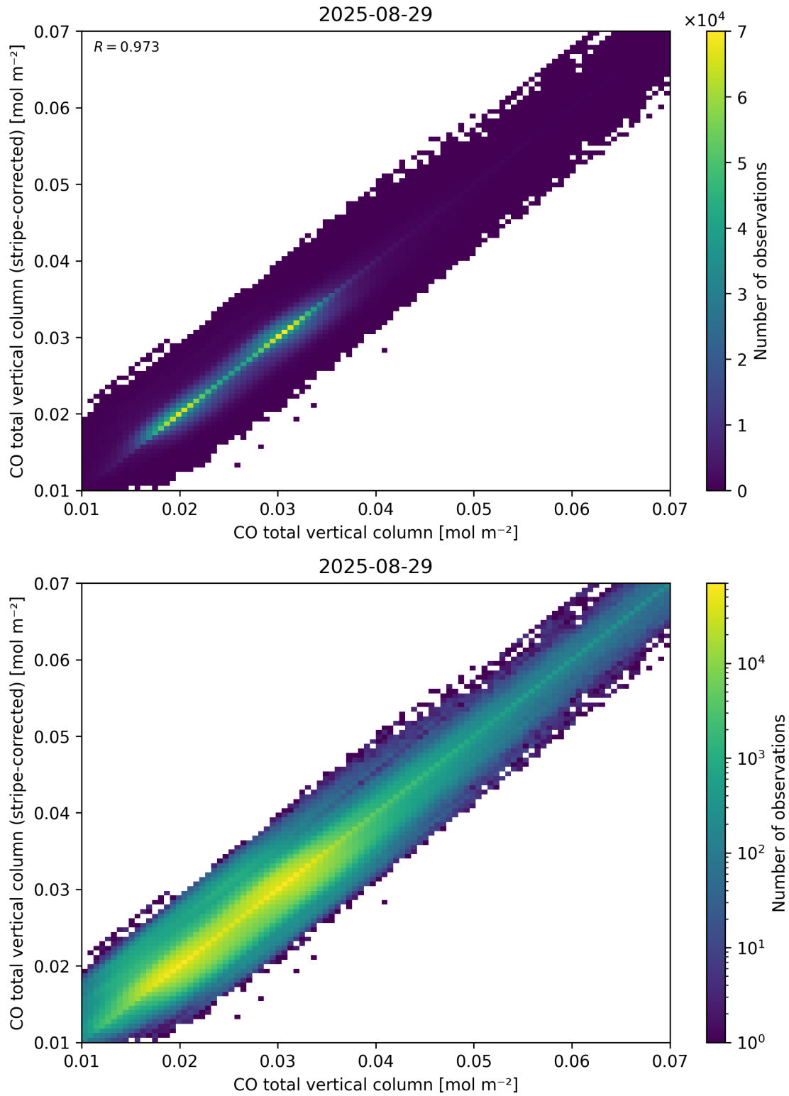
Figure 33: Scatter density plot of “CO total vertical column” against “CO total vertical column (stripe-corrected)” for 2025-08-28 to 2025-08-30.
