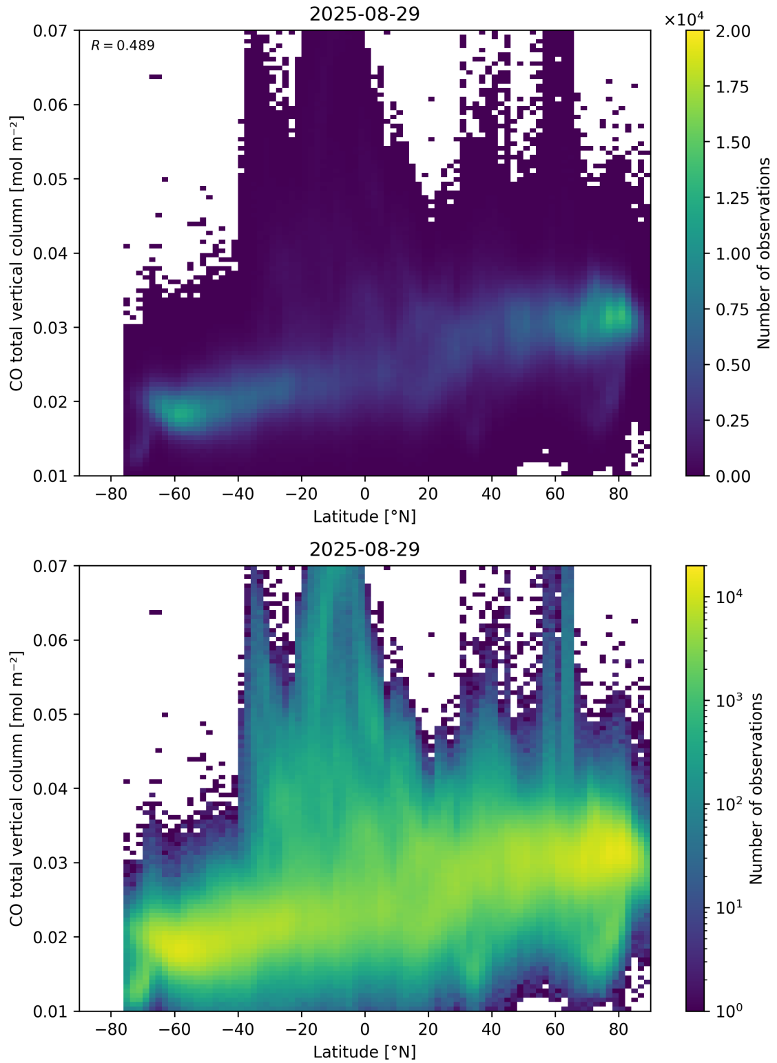
Figure 51: Scatter density plot of “Latitude” against “CO total vertical column” for 2025-08-28 to 2025-08-30.
