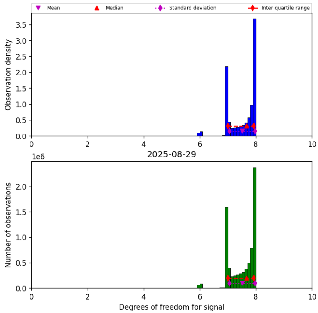
Figure 23: Histogram of “Degrees of freedom for signal” for 2025-08-28 to 2025-08-30
