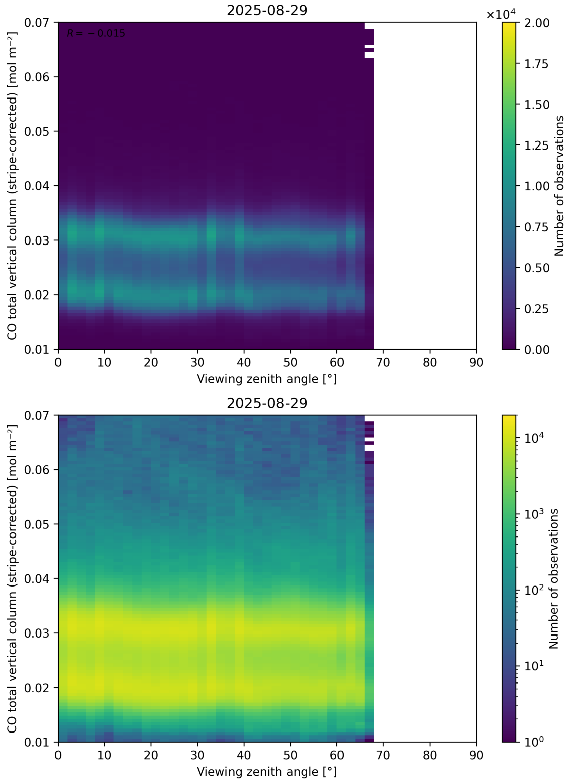
Figure 70: Scatter density plot of “Viewing zenith angle” against “CO total vertical column (stripe-corrected)” for 2025-08-28 to 2025-08-30.
