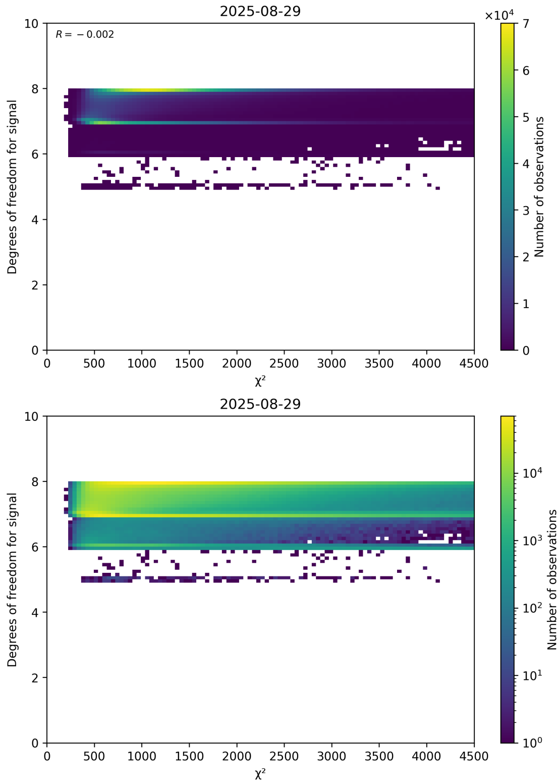
Figure 48: Scatter density plot of “ \chi^2 ” against “Degrees of freedom for signal” for 2025-08-28 to 2025-08-30.
