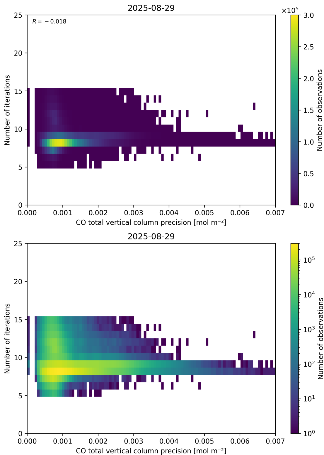
Figure 46: Scatter density plot of “CO total vertical column precision” against “Number of iterations” for 2025-08-28 to 2025-08-30.
