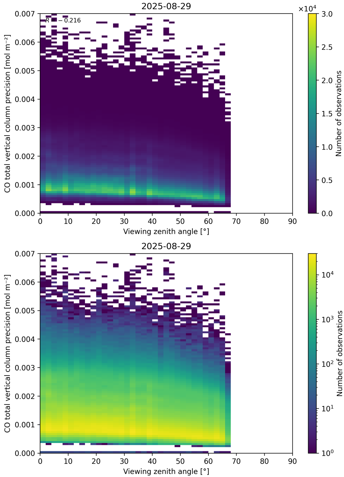
Figure 71: Scatter density plot of “Viewing zenith angle” against “CO total vertical column precision” for 2025-08-28 to 2025-08-30.
