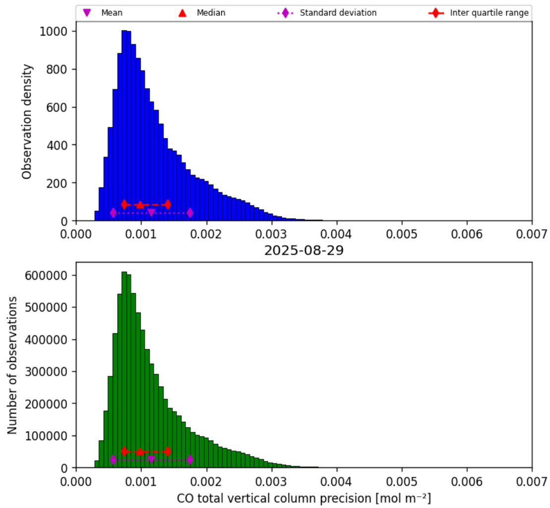
Figure 20: Histogram of “CO total vertical column precision” for 2025-08-28 to 2025-08-30
