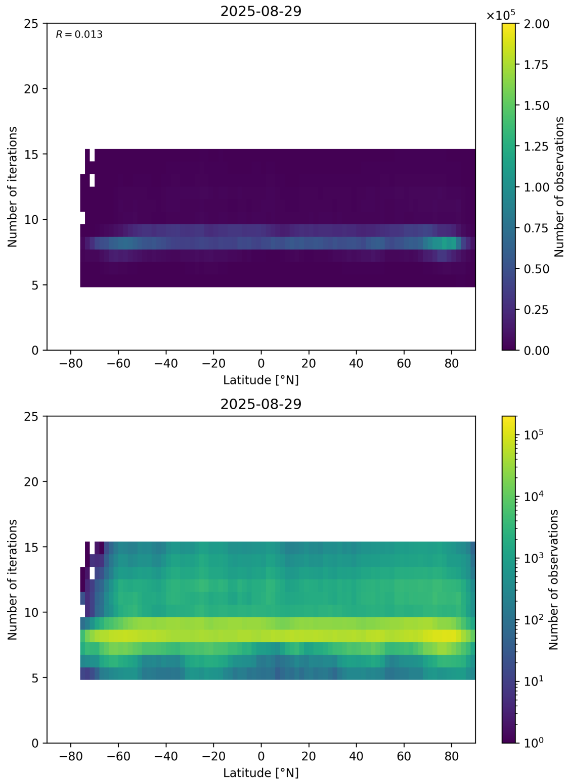
Figure 56: Scatter density plot of “Latitude” against “Number of iterations” for 2025-08-28 to 2025-08-30.
