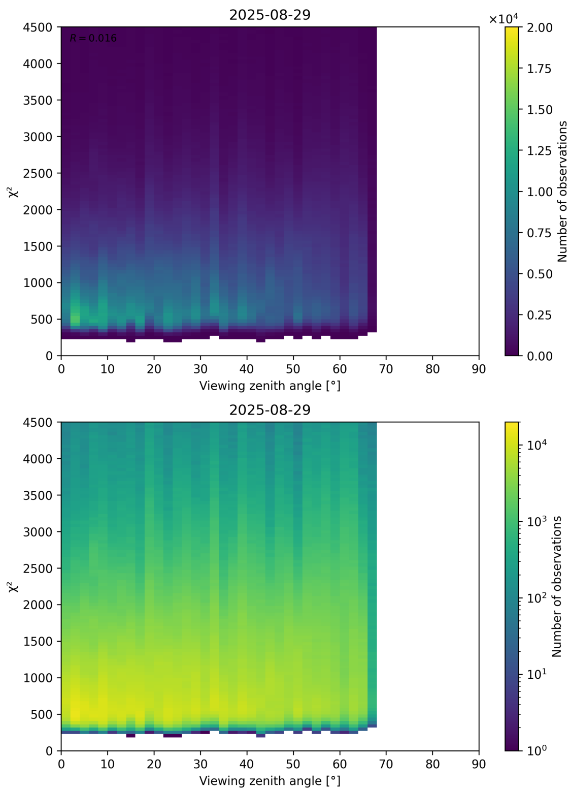
Figure 72: Scatter density plot of “Viewing zenith angle” against “ \chi^2 ” for 2025-08-28 to 2025-08-30.
