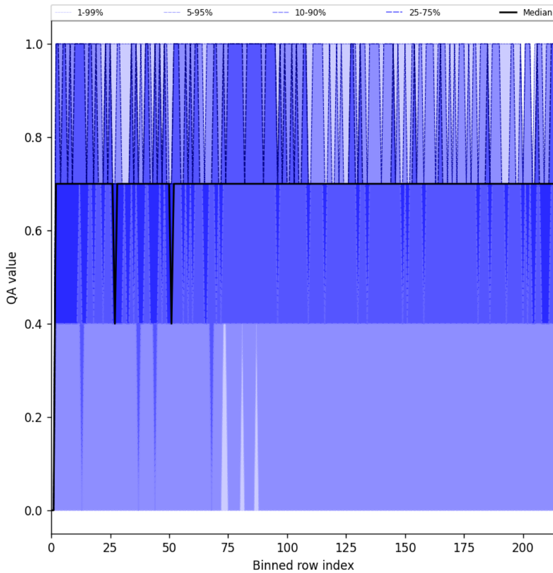
Figure 25: Along track statistics of “QA value” for 2025-08-28 to 2025-08-30
