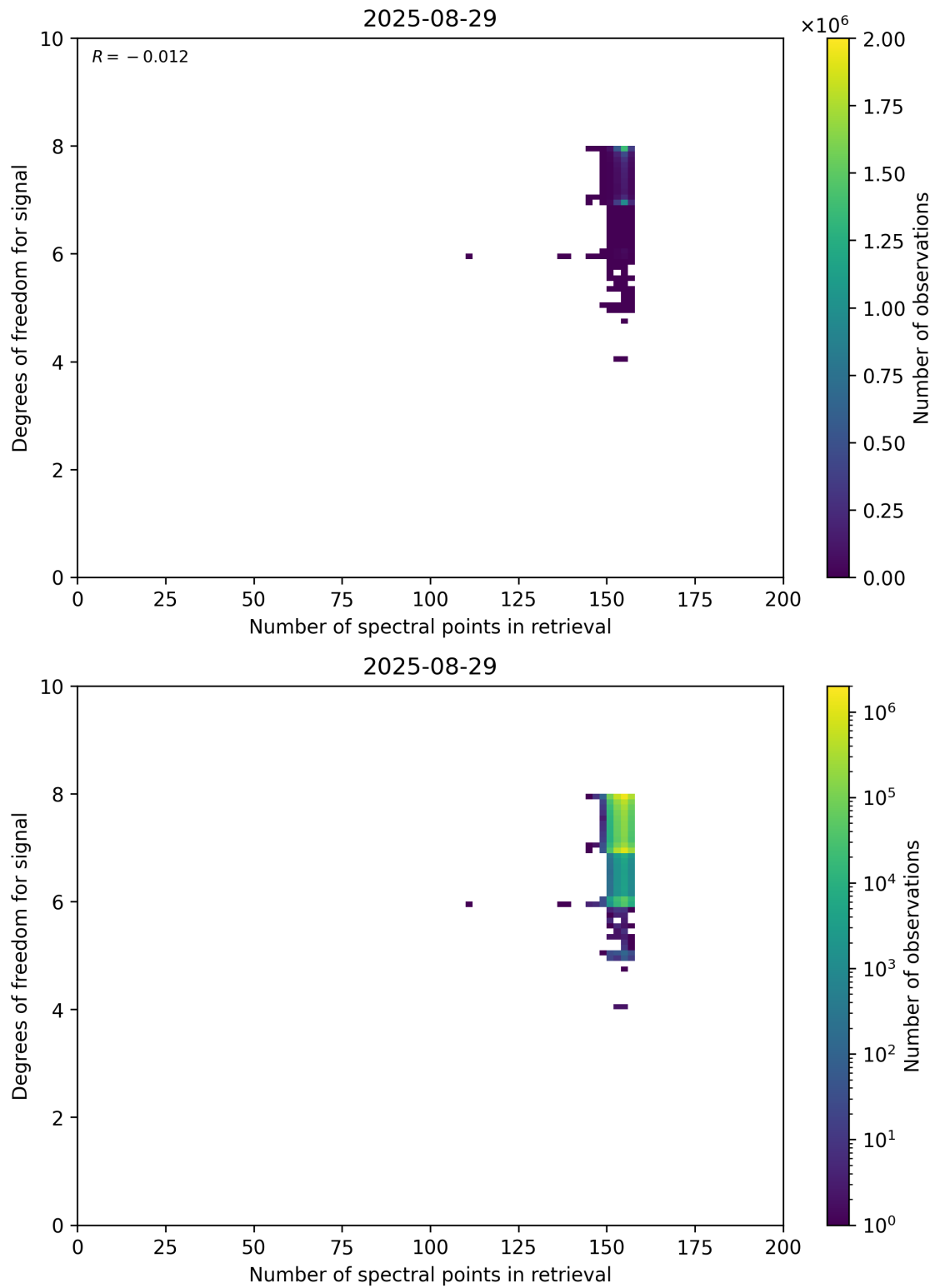
Figure 59: Scatter density plot of “Number of spectral points in retrieval” against “Degrees of freedom for signal” for 2025-08-28 to 2025-08-30.
