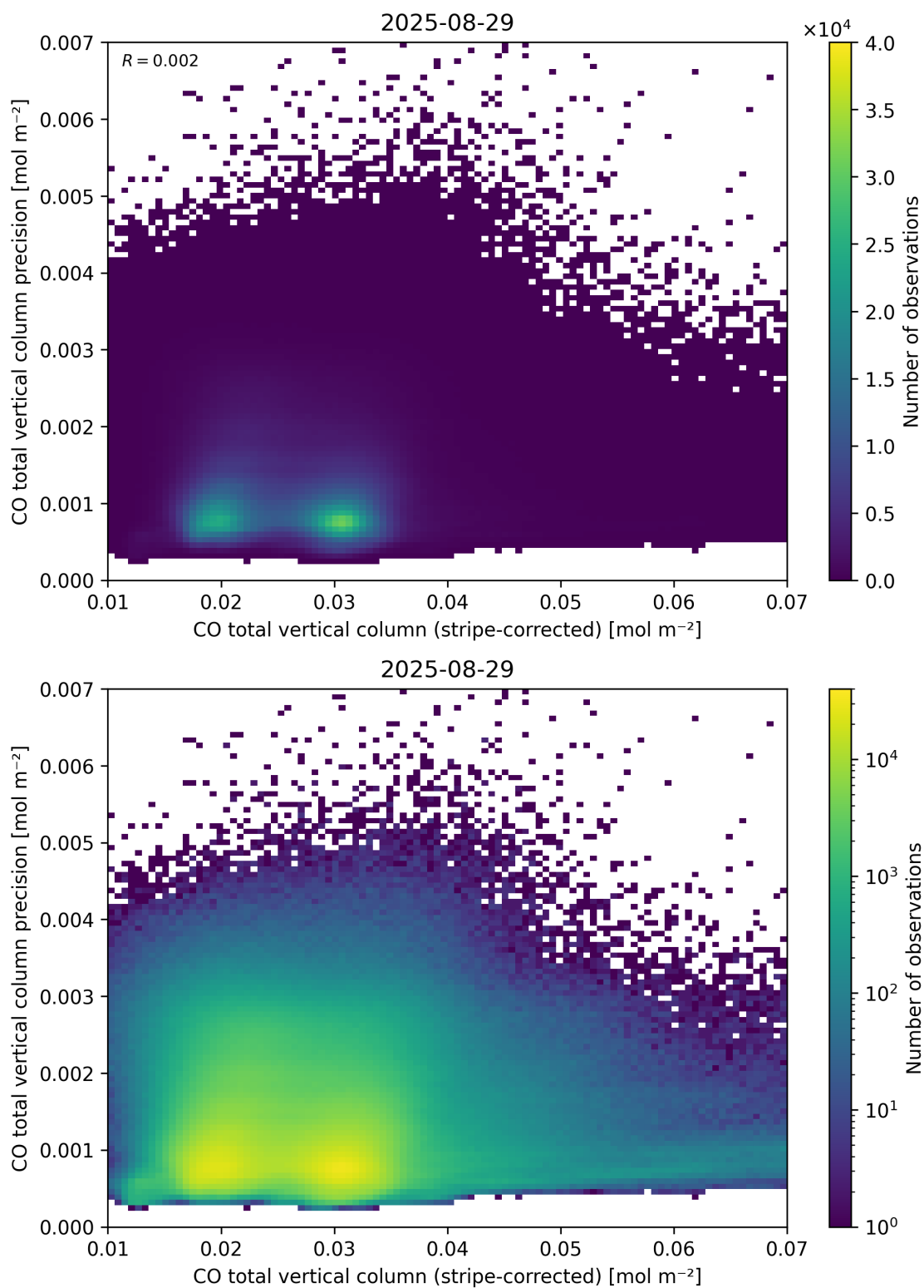
Figure 36: Scatter density plot of “CO total vertical column (stripe-corrected)” against “CO total vertical column precision” for 2025-08-28 to 2025-08-30.
