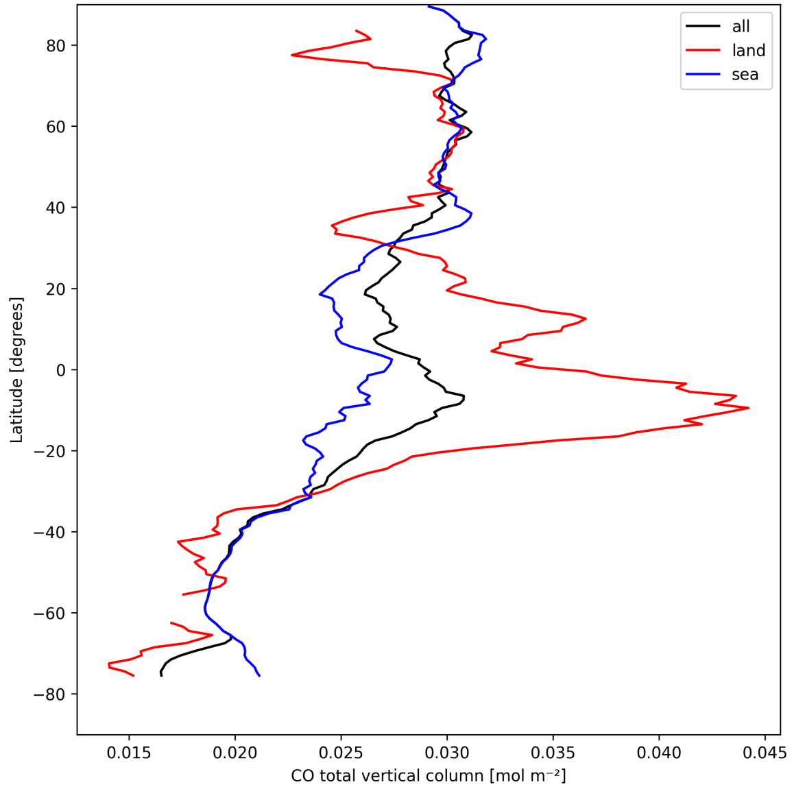
Figure 10: Zonal average of “CO total vertical column” for 2025-08-28 to 2025-08-30.
