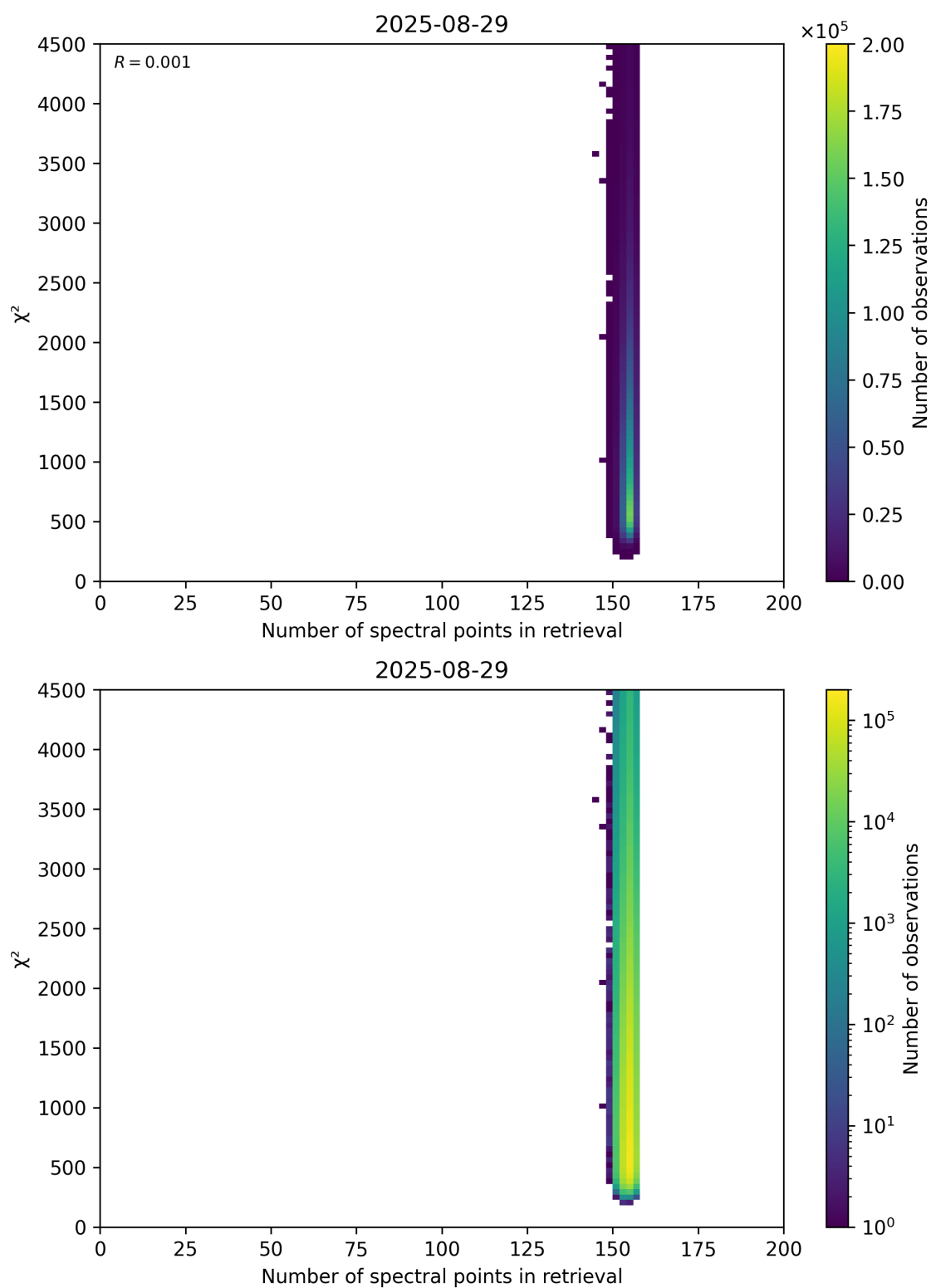
Figure 58: Scatter density plot of “Number of spectral points in retrieval” against “ \chi^2 ” for 2025-08-28 to 2025-08-30.
