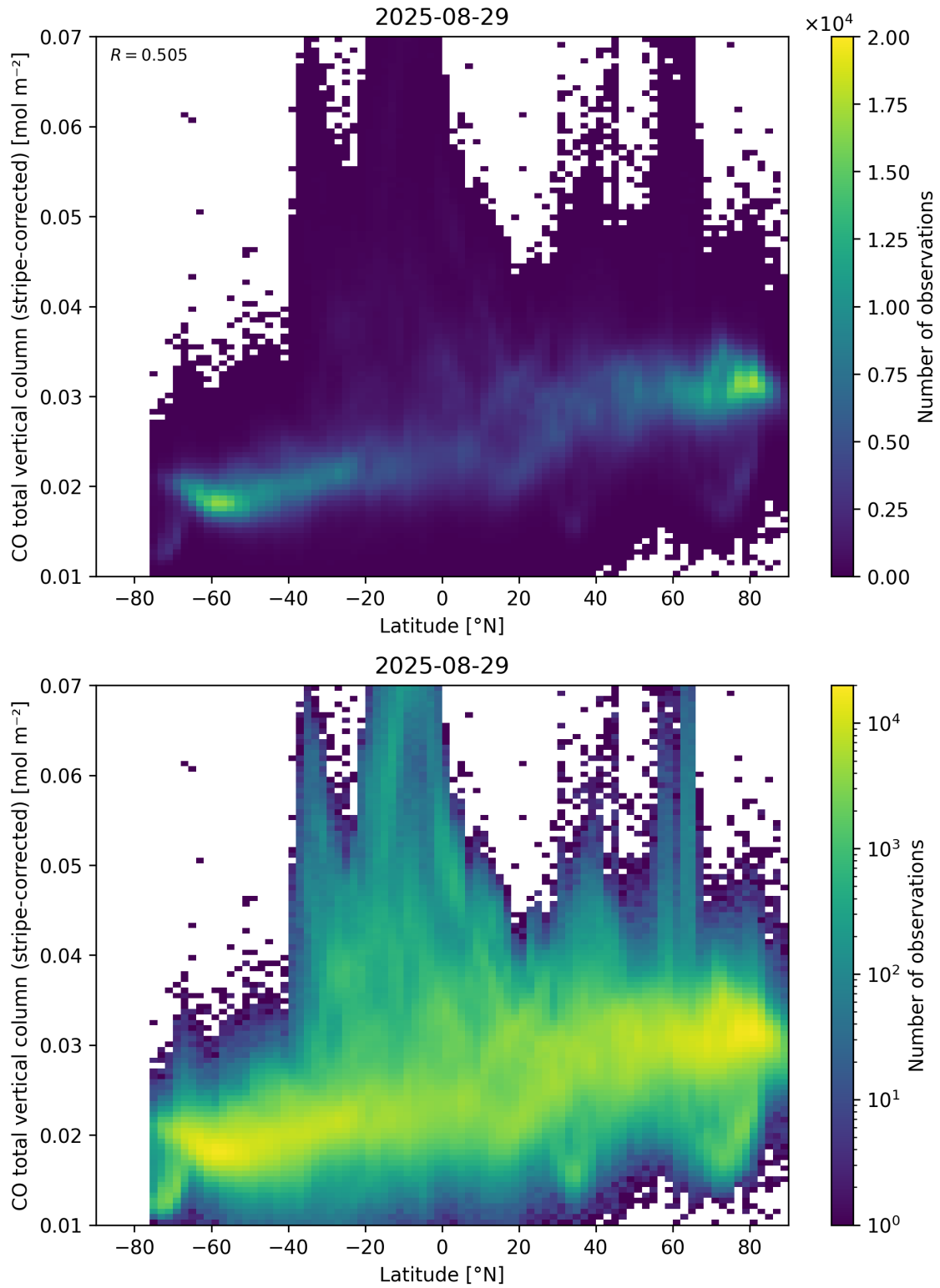
Figure 52: Scatter density plot of “Latitude” against “CO total vertical column (stripe-corrected)” for 2025-08-28 to 2025-08-30.
