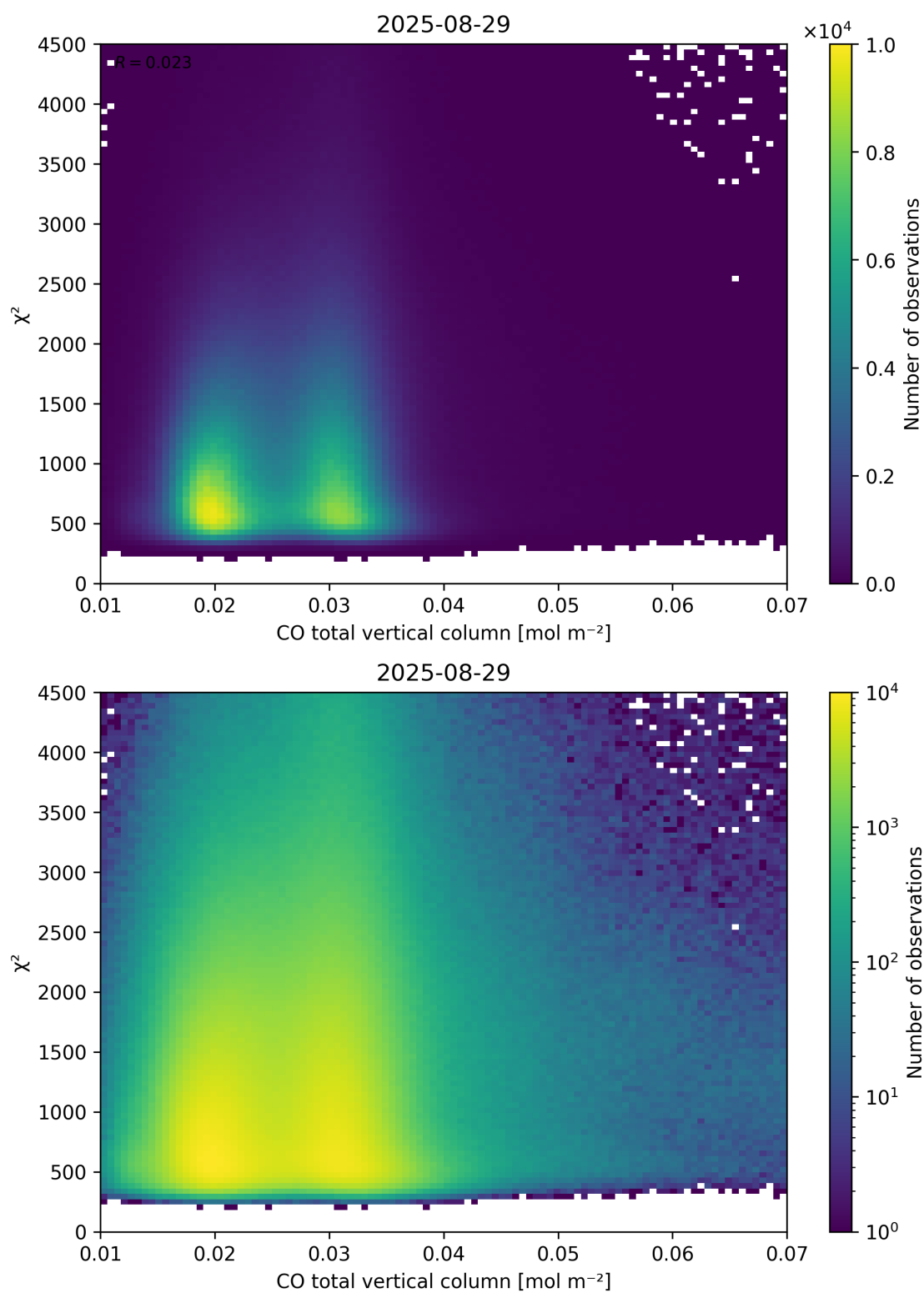
Figure 35: Scatter density plot of “CO total vertical column” against “ \chi^2 ” for 2025-08-28 to 2025-08-30.
