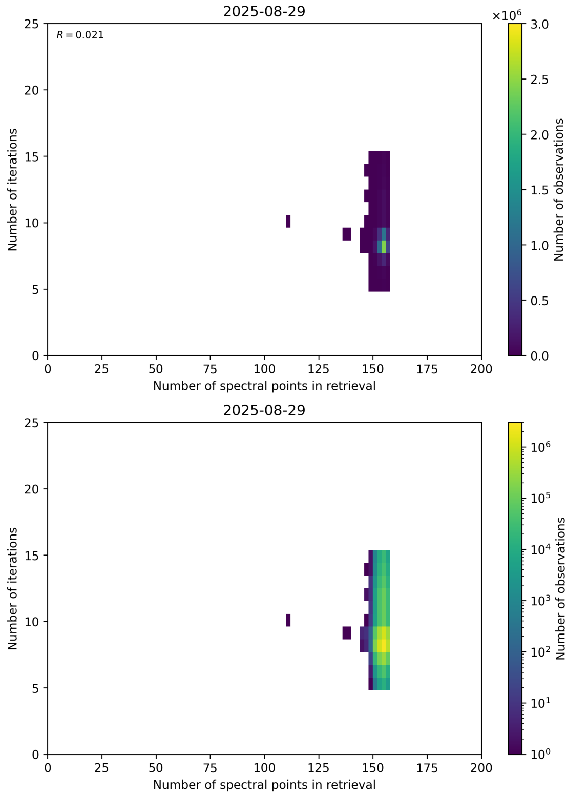
Figure 60: Scatter density plot of “Number of spectral points in retrieval” against “Number of iterations” for 2025-08-28 to 2025-08-30.
