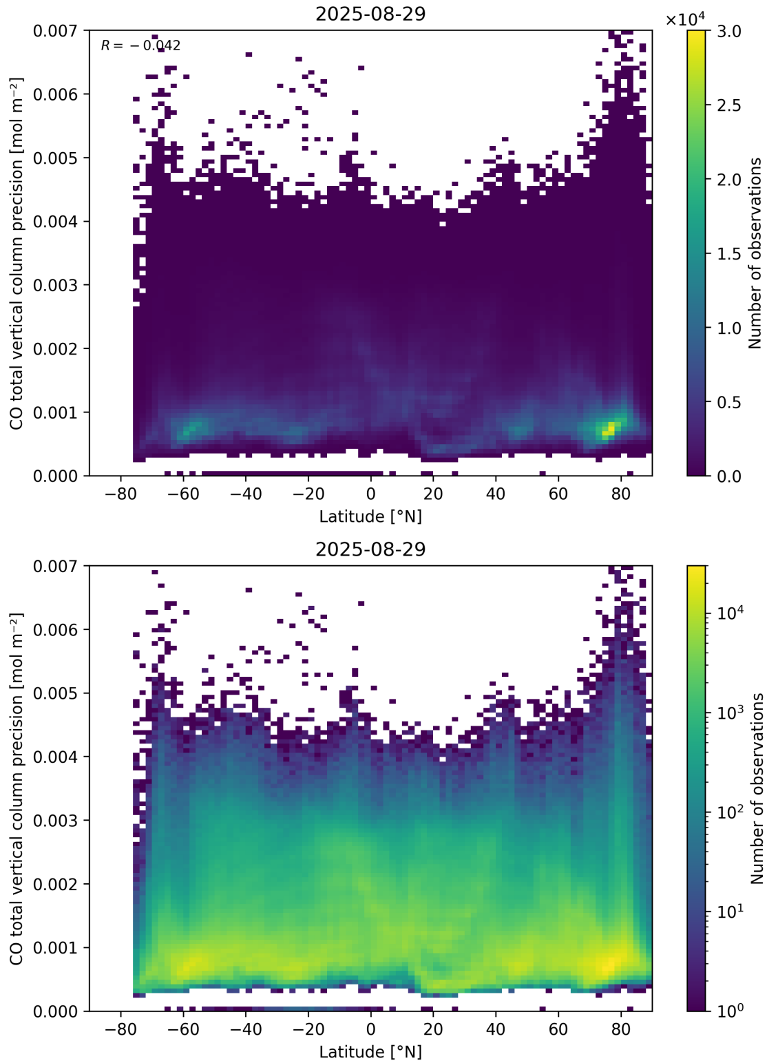
Figure 53: Scatter density plot of “Latitude” against “CO total vertical column precision” for 2025-08-28 to 2025-08-30.
