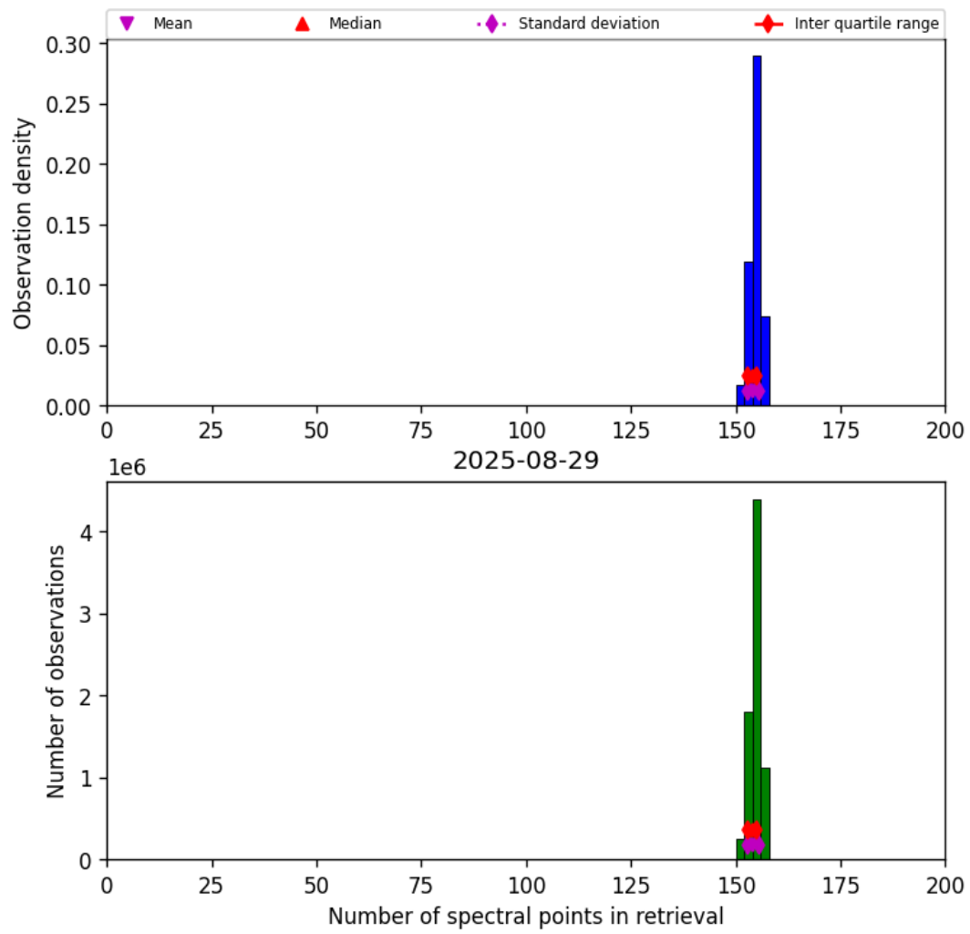
Figure 21: Histogram of “Number of spectral points in retrieval” for 2025-08-28 to 2025-08-30
