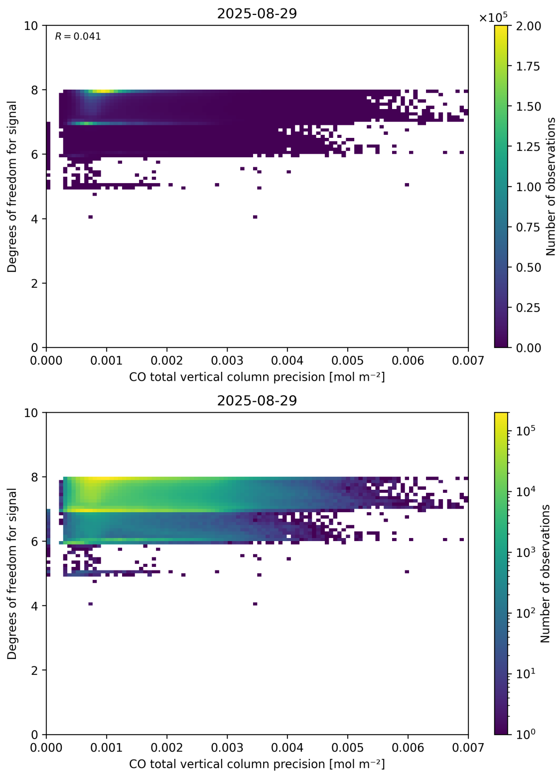
Figure 45: Scatter density plot of “CO total vertical column precision” against “Degrees of freedom for signal” for 2025-08-28 to 2025-08-30.
