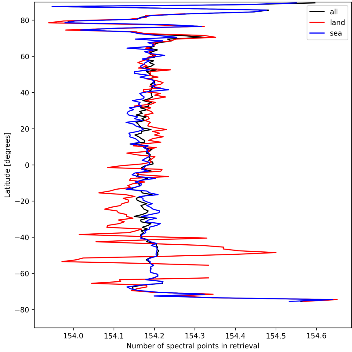
Figure 13: Zonal average of “Number of spectral points in retrieval” for 2025-08-28 to 2025-08-30.
