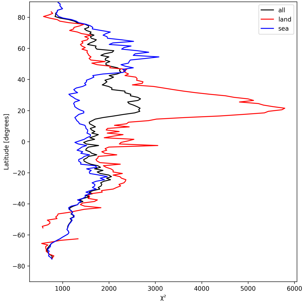
Figure 14: Zonal average of “ \chi^2 ” for 2025-08-28 to 2025-08-30.
