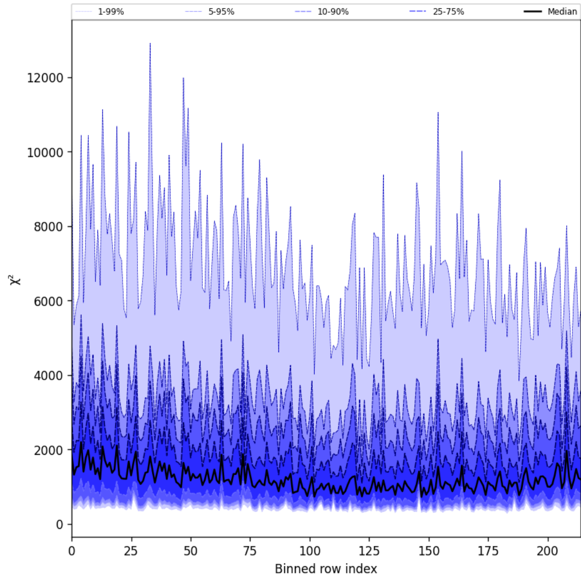
Figure 30: Along track statistics of “ \chi^2 ” for 2025-08-28 to 2025-08-30
