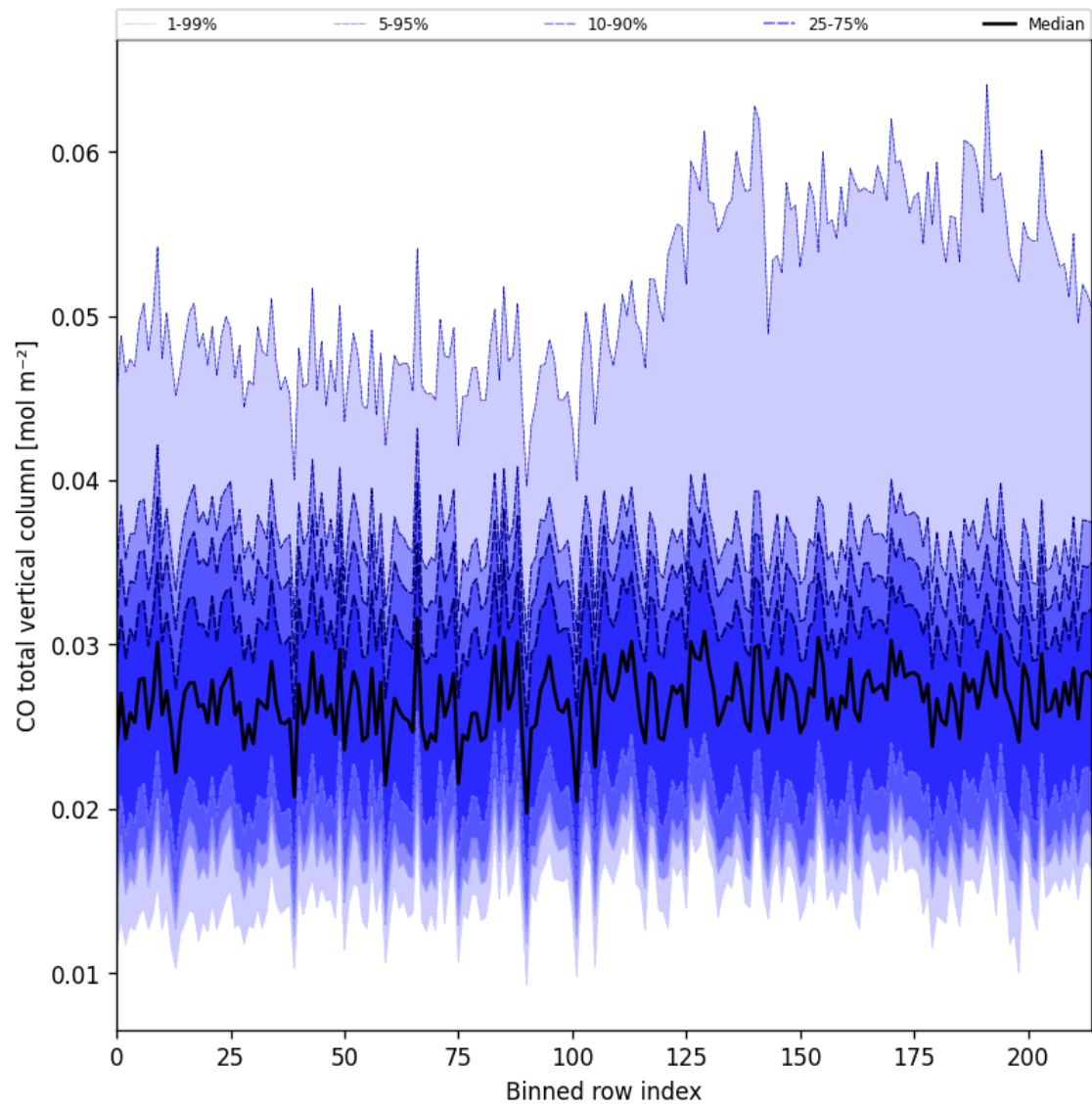
Figure 26: Along track statistics of “CO total vertical column” for 2025-08-28 to 2025-08-30
