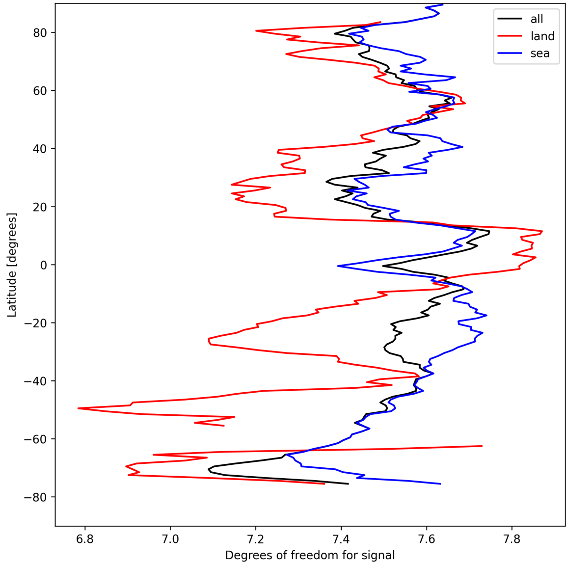
Figure 15: Zonal average of “Degrees of freedom for signal” for 2025-08-28 to 2025-08-30.
