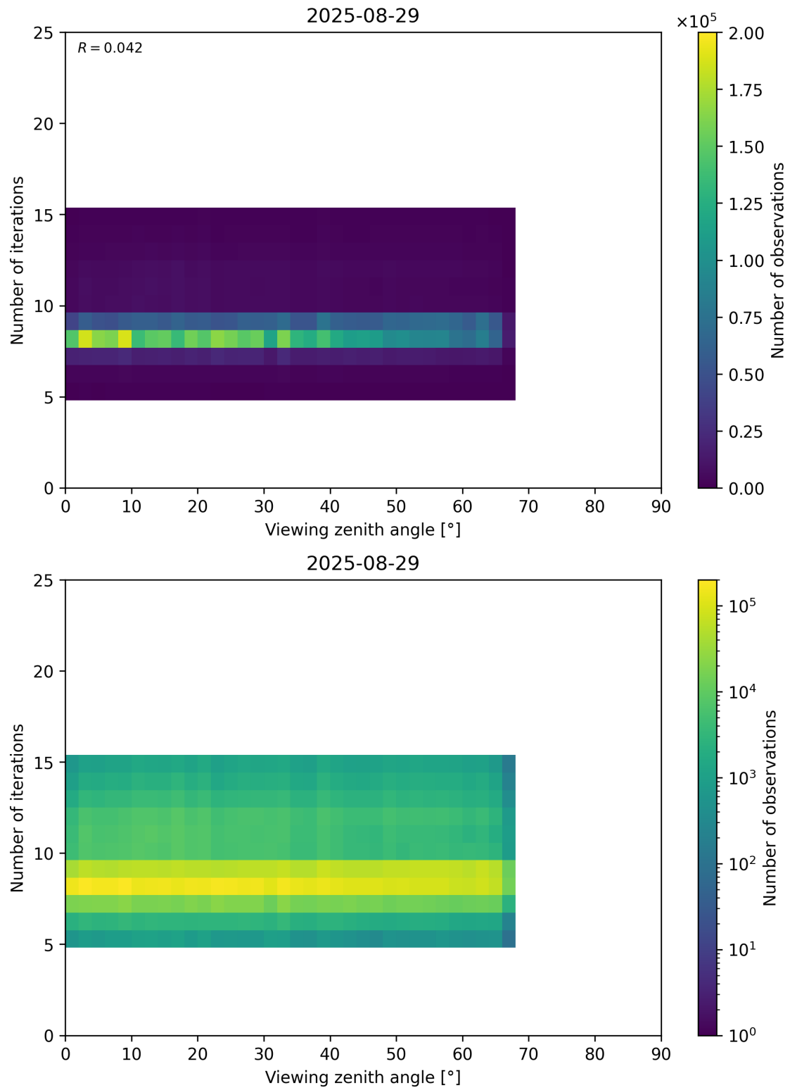
Figure 75: Scatter density plot of “Viewing zenith angle” against “Number of iterations” for 2025-08-28 to 2025-08-30.
