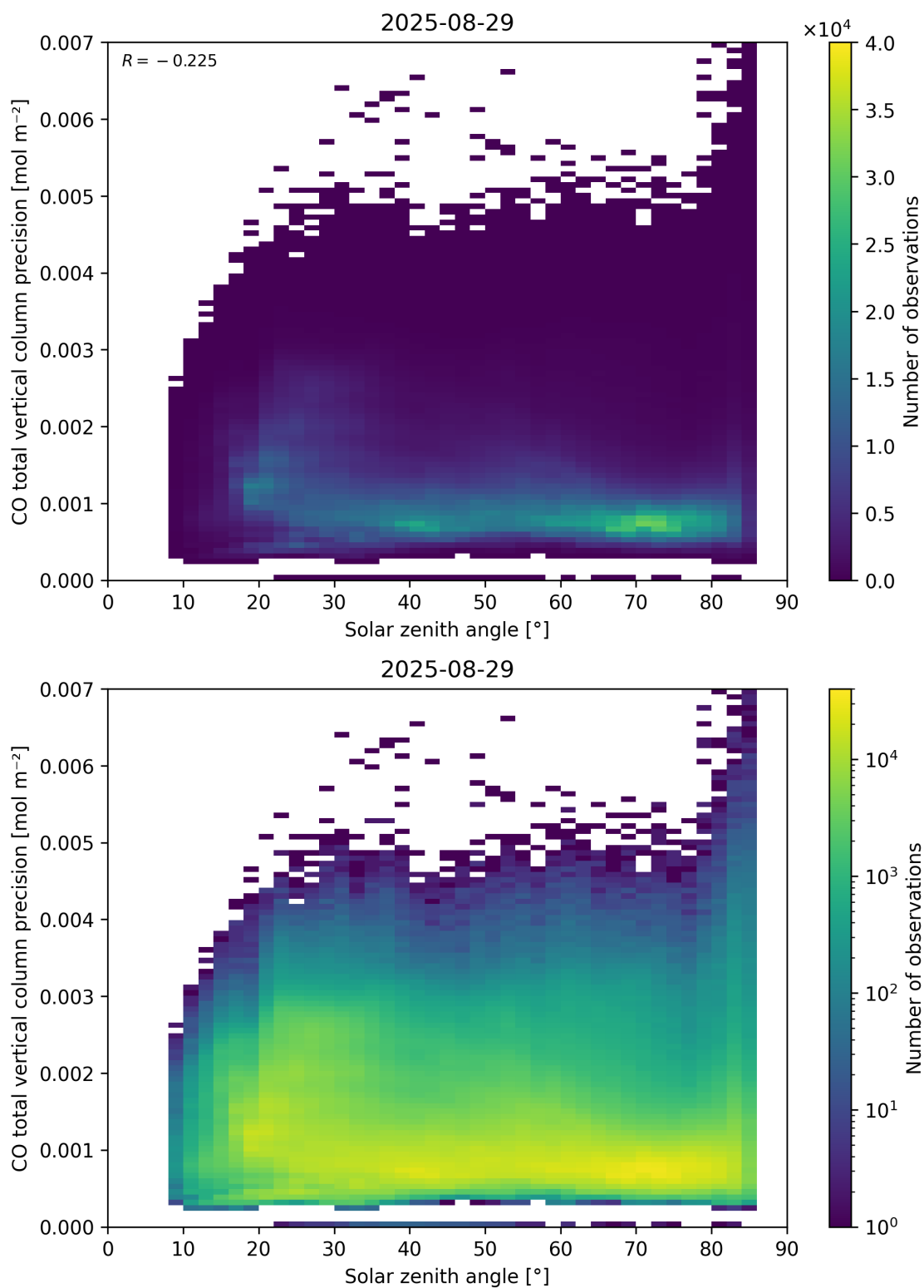
Figure 63: Scatter density plot of “Solar zenith angle” against “CO total vertical column precision” for 2025-08-28 to 2025-08-30.
