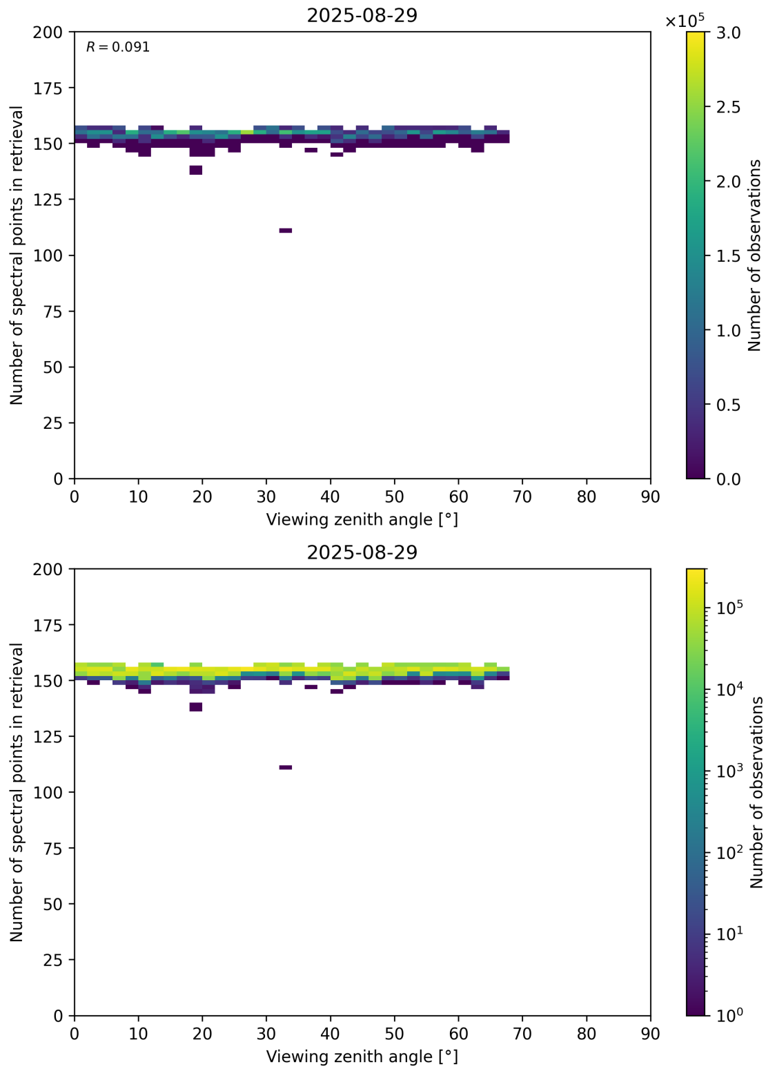
Figure 76: Scatter density plot of “Viewing zenith angle” against “Number of spectral points in retrieval” for 2025-08-28 to 2025-08-30.
