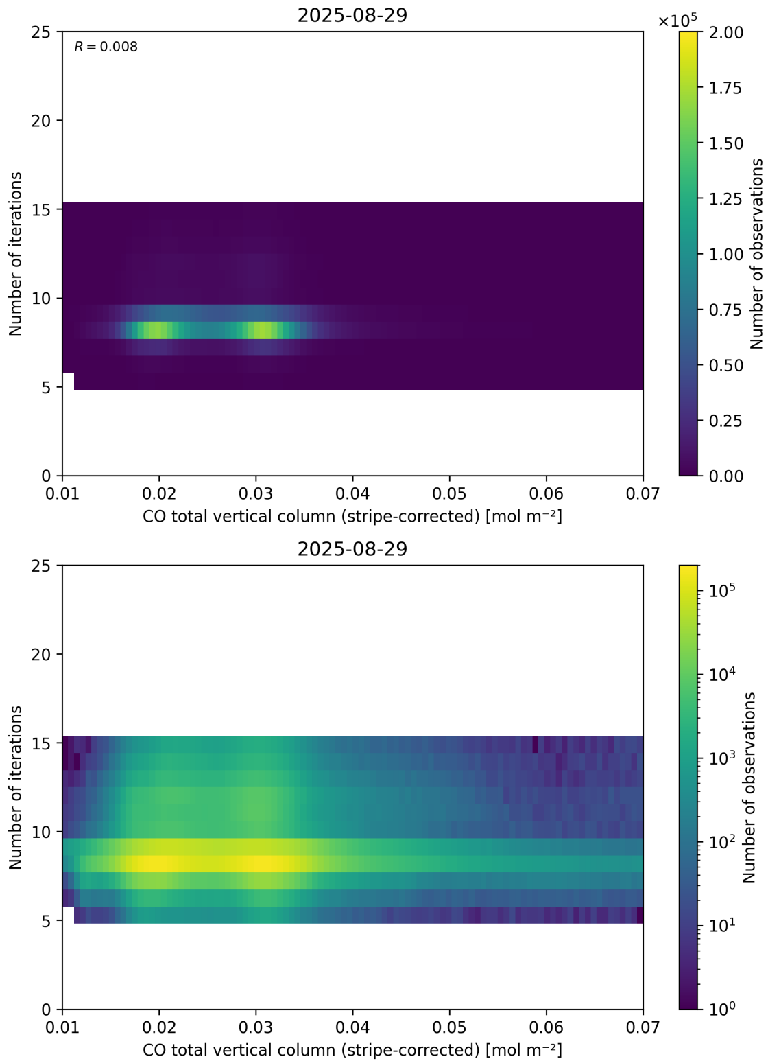
Figure 39: Scatter density plot of “CO total vertical column (stripe-corrected)” against “Number of iterations” for 2025-08-28 to 2025-08-30.
