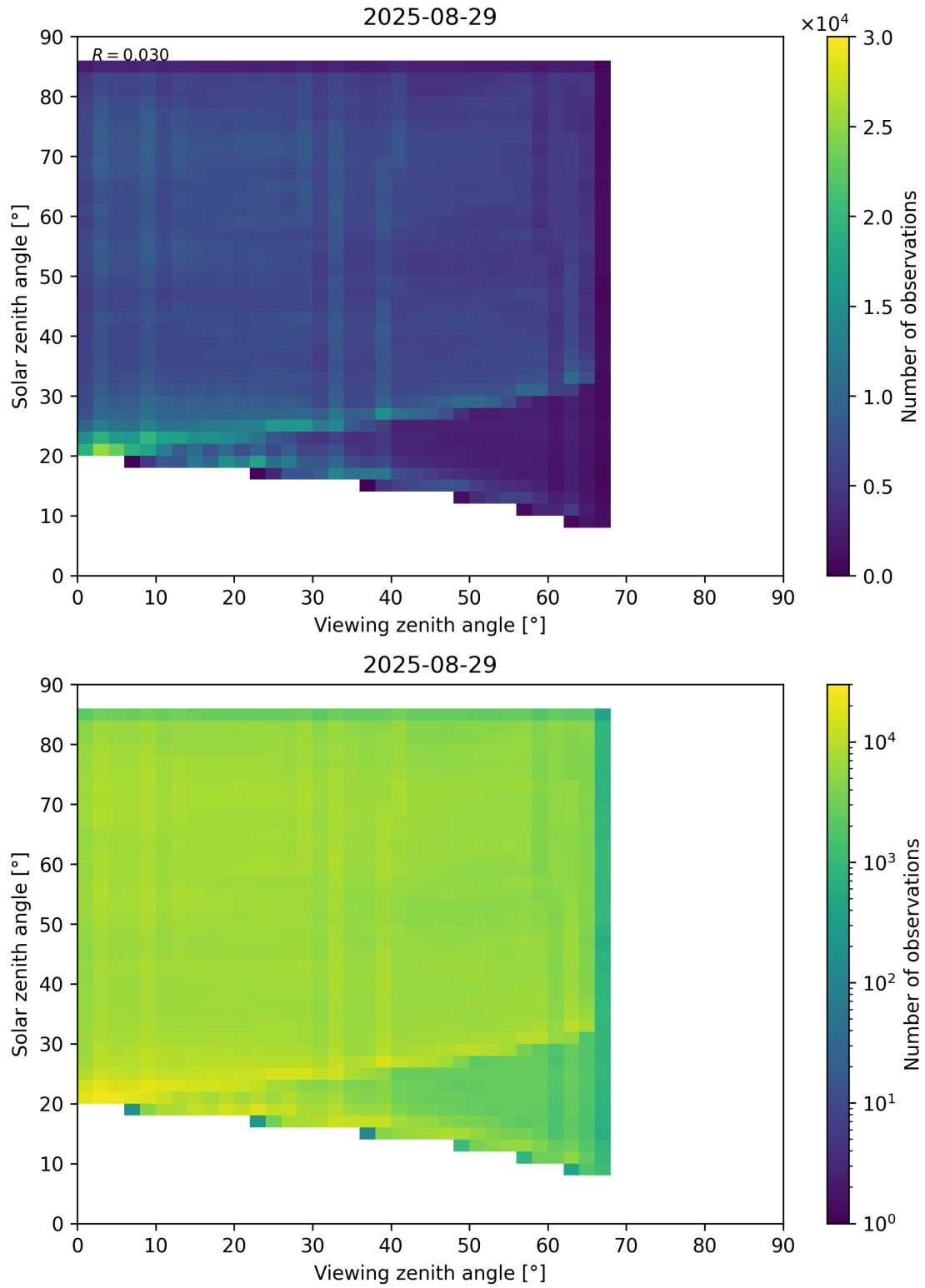
Figure 77: Scatter density plot of “Viewing zenith angle” against “Solar zenith angle” for 2025-08-28 to 2025-08-30.
