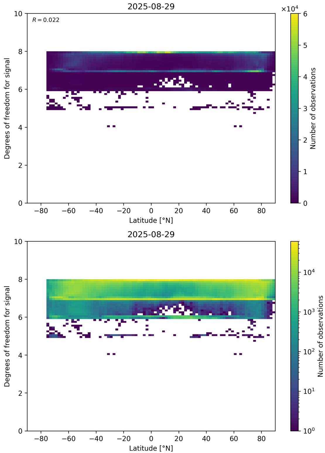
Figure 55: Scatter density plot of “Latitude” against “Degrees of freedom for signal” for 2025-08-28 to 2025-08-30.
