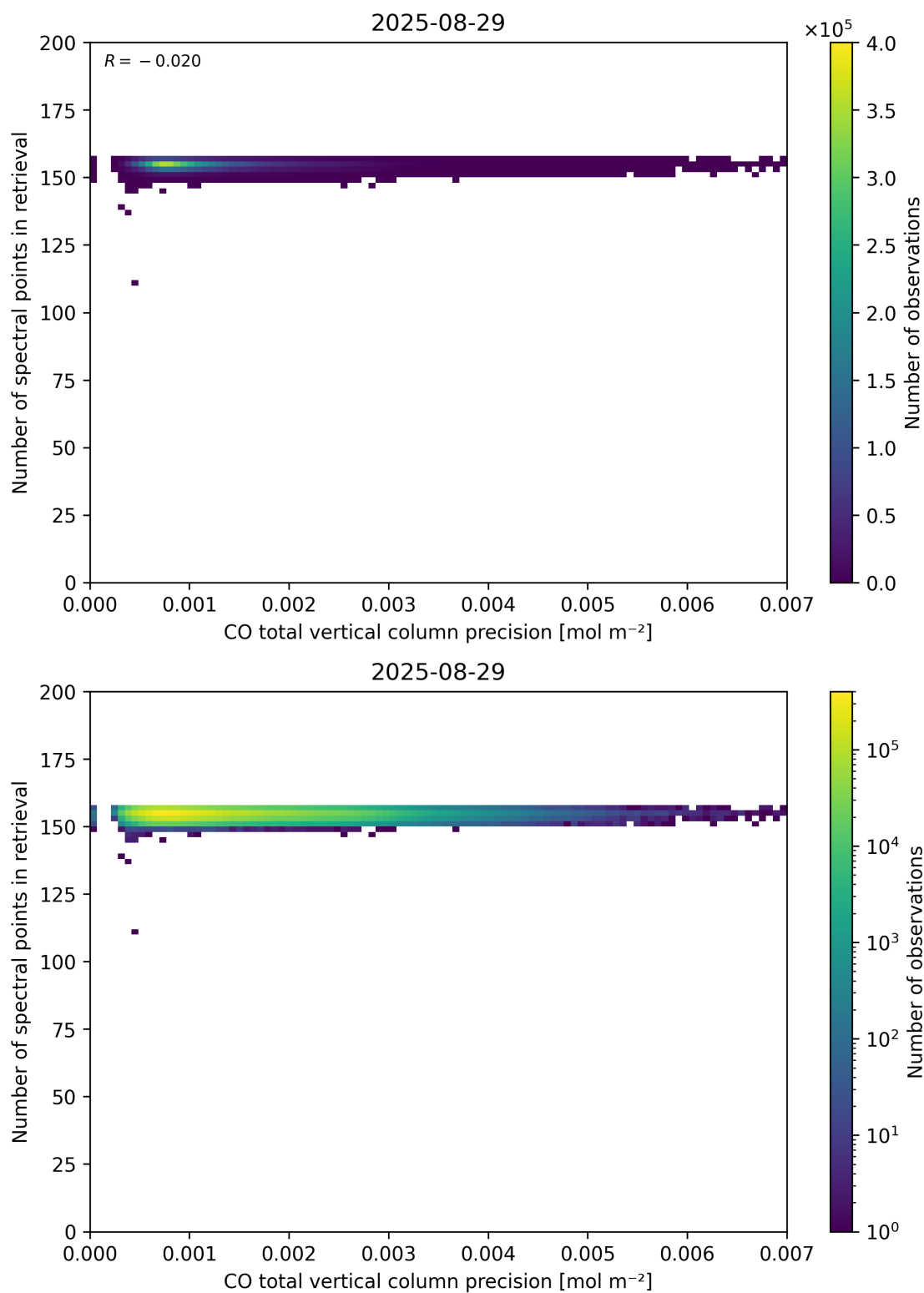
Figure 47: Scatter density plot of “CO total vertical column precision” against “Number of spectral points in retrieval” for 2025-08-28 to 2025-08-30.
