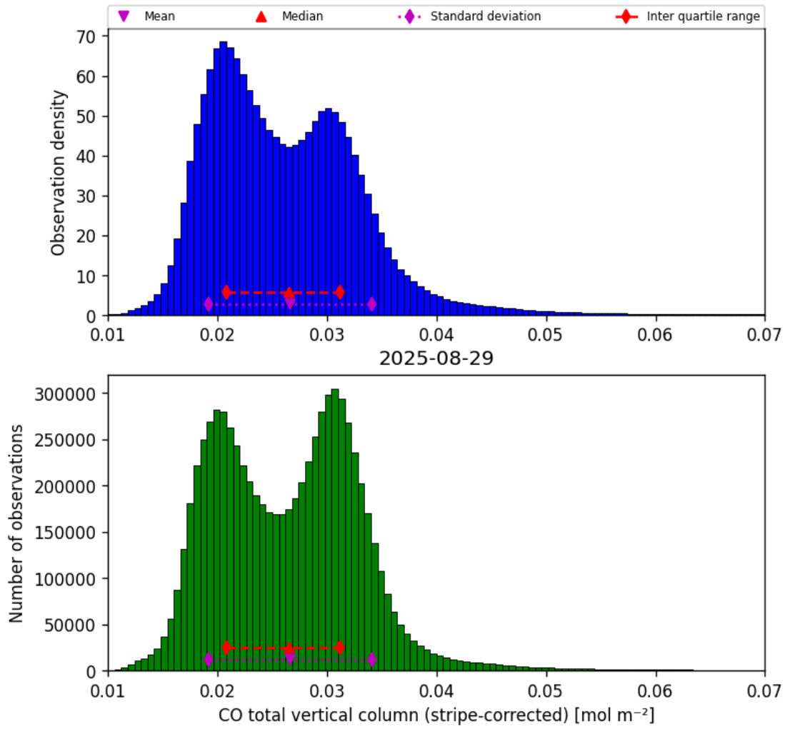
Figure 19: Histogram of “CO total vertical column (stripe-corrected)” for 2025-08-28 to 2025-08-30
