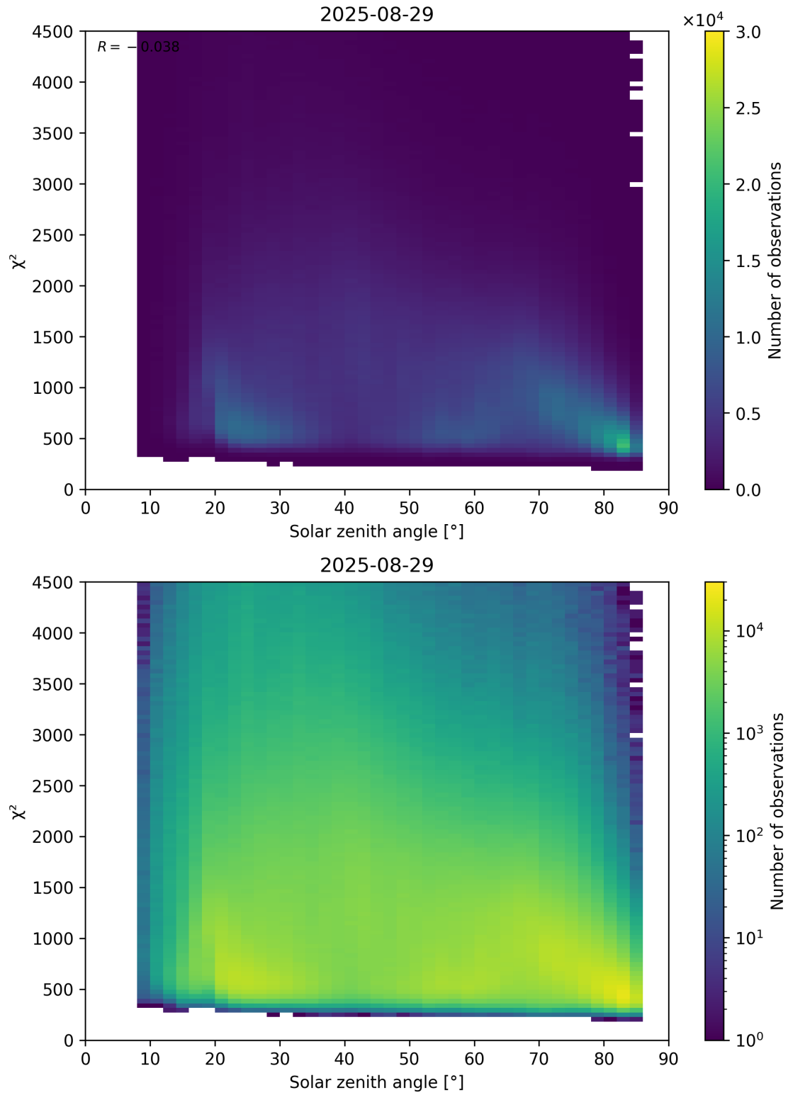
Figure 64: Scatter density plot of “Solar zenith angle” against “ \chi^2 ” for 2025-08-28 to 2025-08-30.
