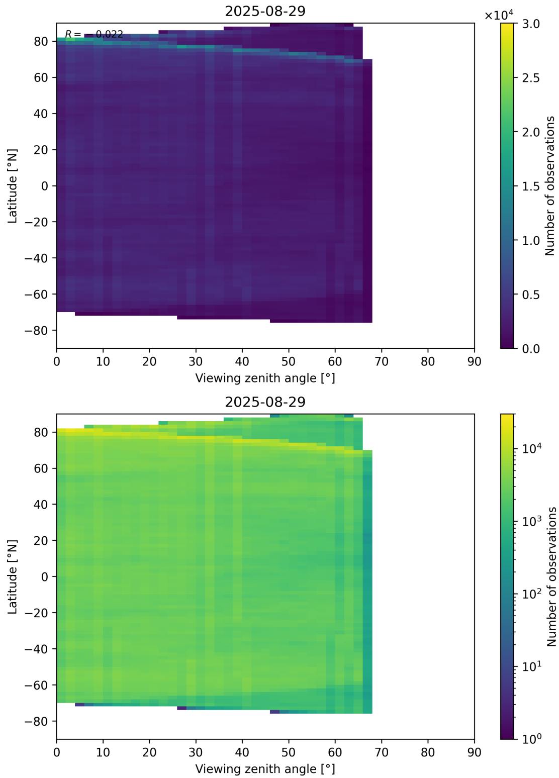
Figure 74: Scatter density plot of “Viewing zenith angle” against “Latitude” for 2025-08-28 to 2025-08-30.
