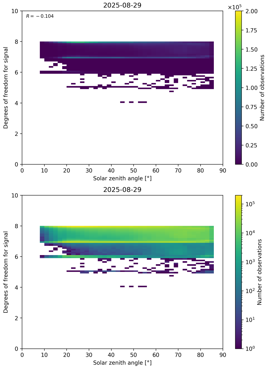
Figure 65: Scatter density plot of “Solar zenith angle” against “Degrees of freedom for signal” for 2025-08-28 to 2025-08-30.
