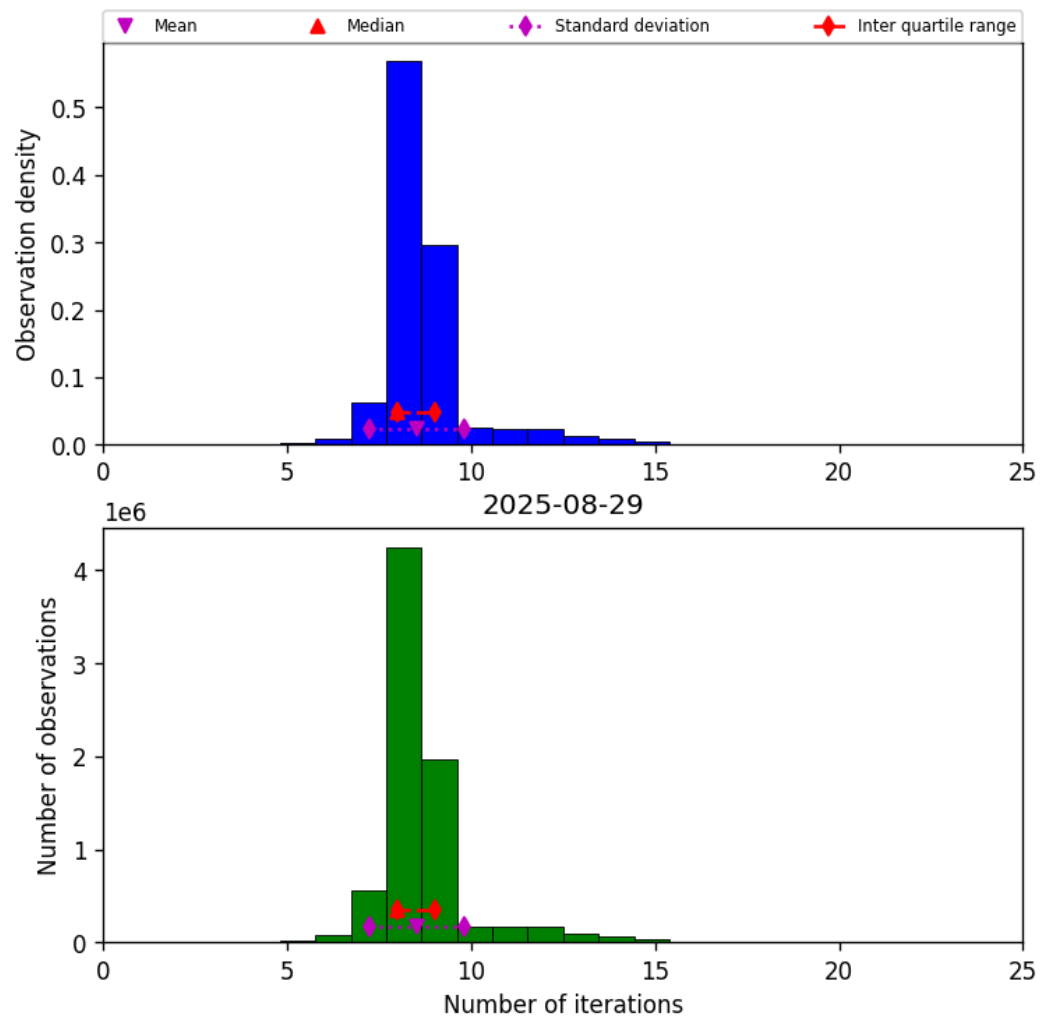
Figure 24: Histogram of “Number of iterations” for 2025-08-28 to 2025-08-30
