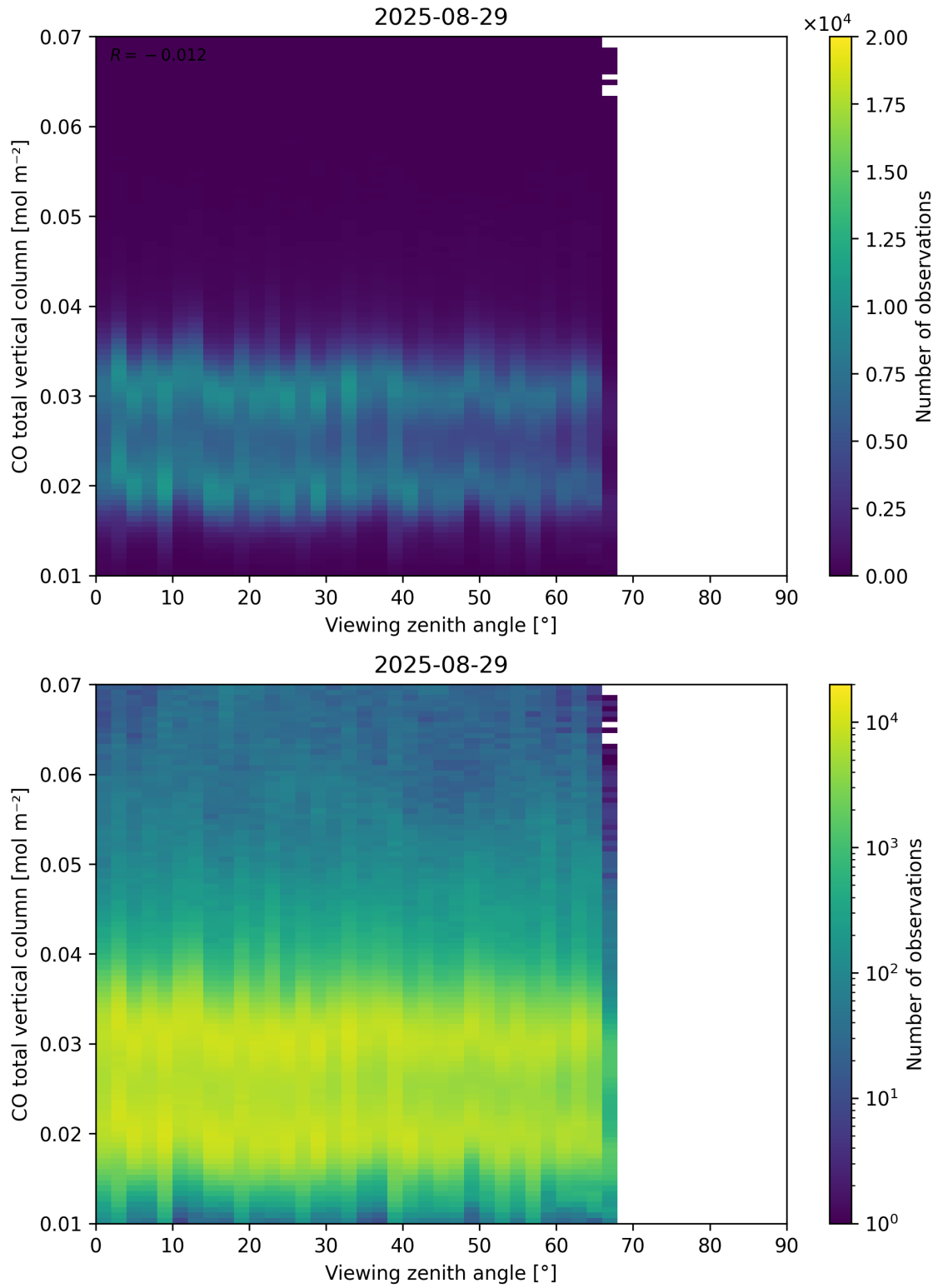
Figure 69: Scatter density plot of “Viewing zenith angle” against “CO total vertical column” for 2025-08-28 to 2025-08-30.
