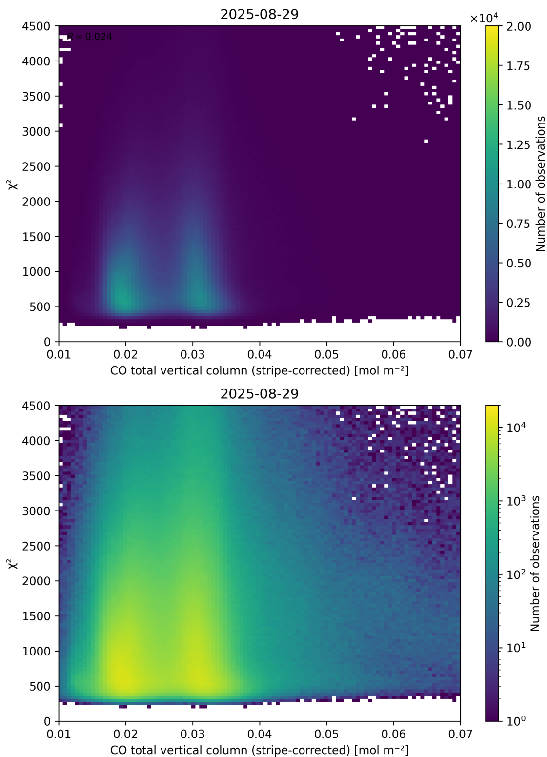
Figure 37: Scatter density plot of “CO total vertical column (stripe-corrected)” against “ \chi^2 ” for 2025-08-28 to 2025-08-30.
