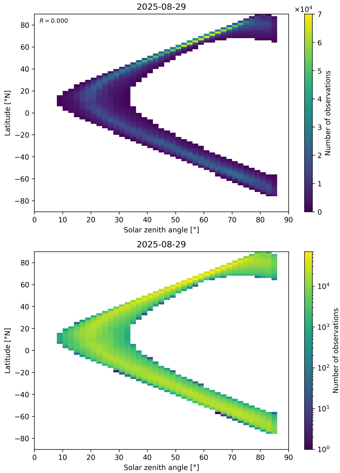
Figure 66: Scatter density plot of “Solar zenith angle” against “Latitude” for 2025-08-28 to 2025-08-30.
