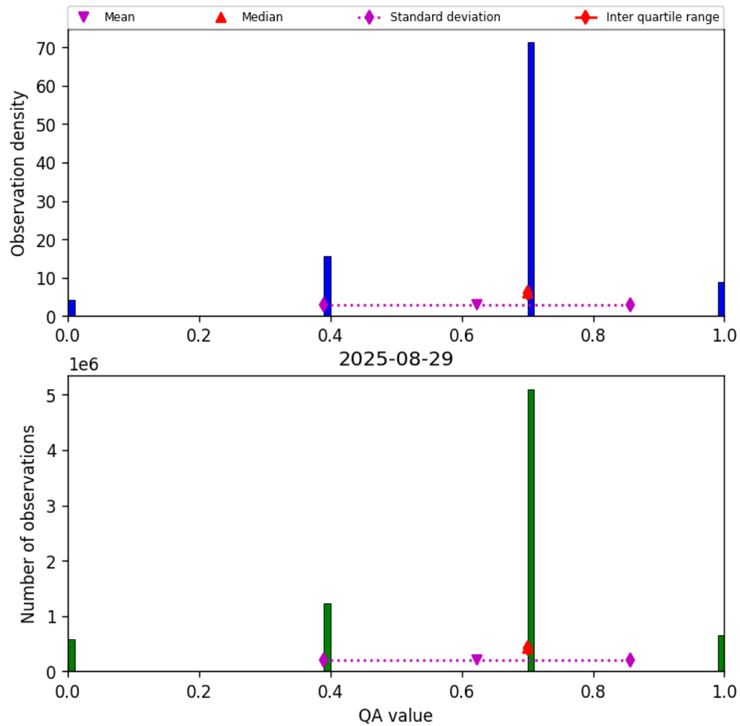
Figure 17: Histogram of “QA value” for 2025-08-28 to 2025-08-30
