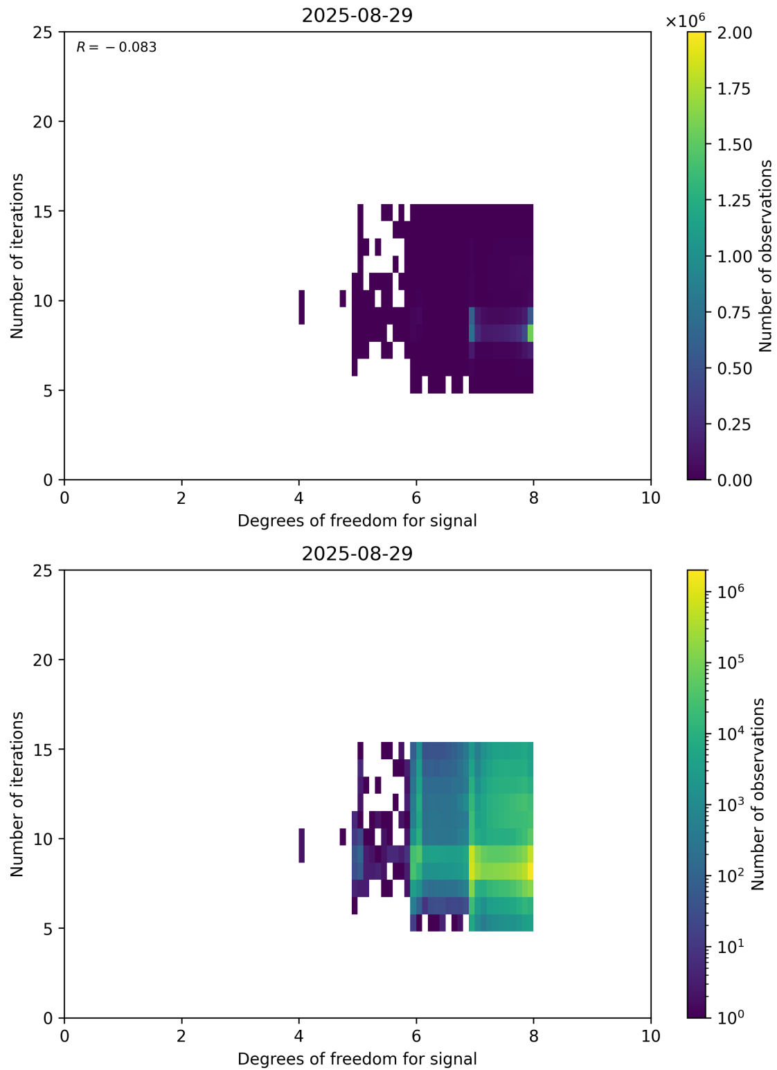
Figure 50: Scatter density plot of “Degrees of freedom for signal” against “Number of iterations” for 2025-08-28 to 2025-08-30.
