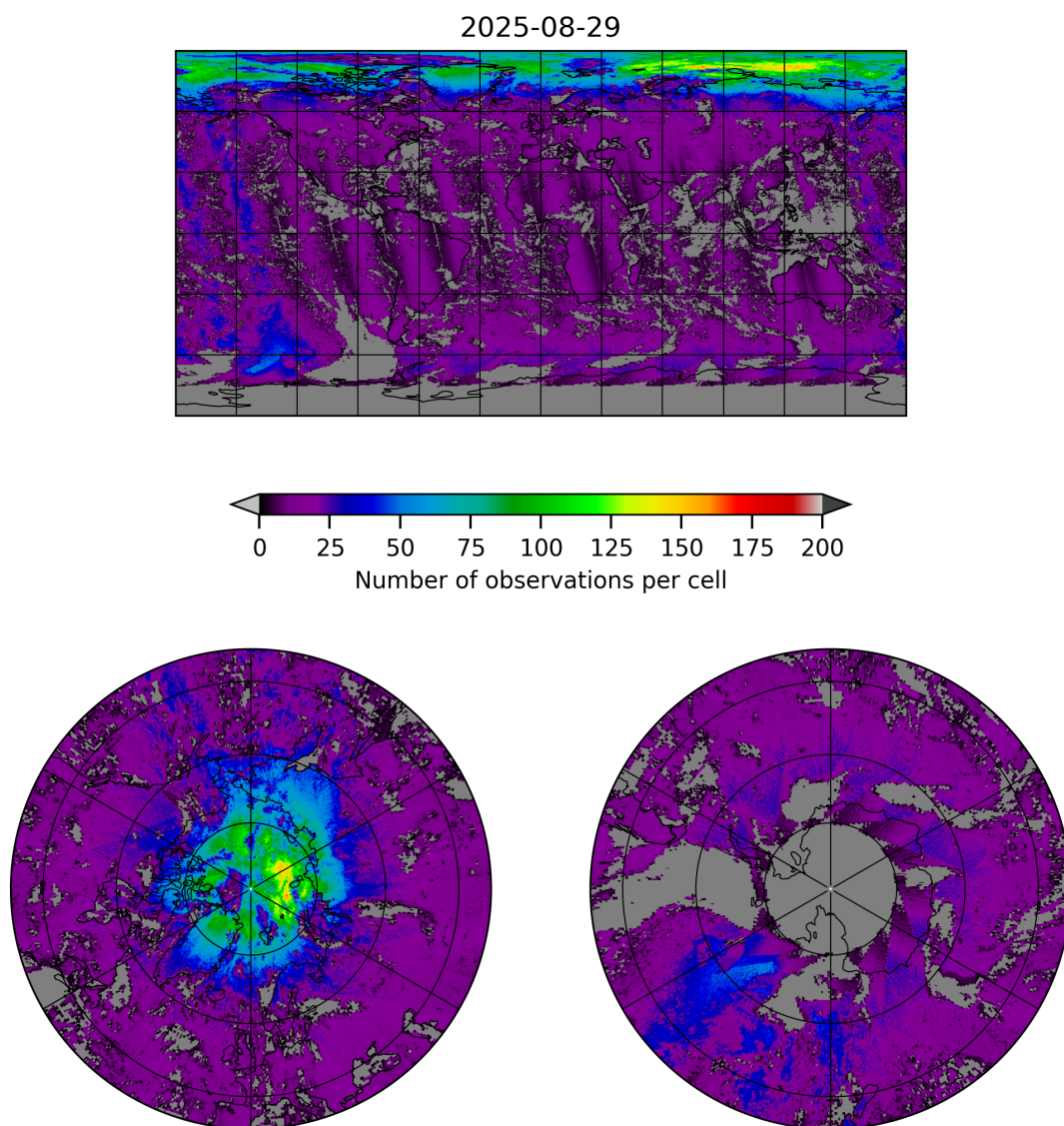
Figure 8: Map of the number of observations for 2025-08-28 to 2025-08-30
