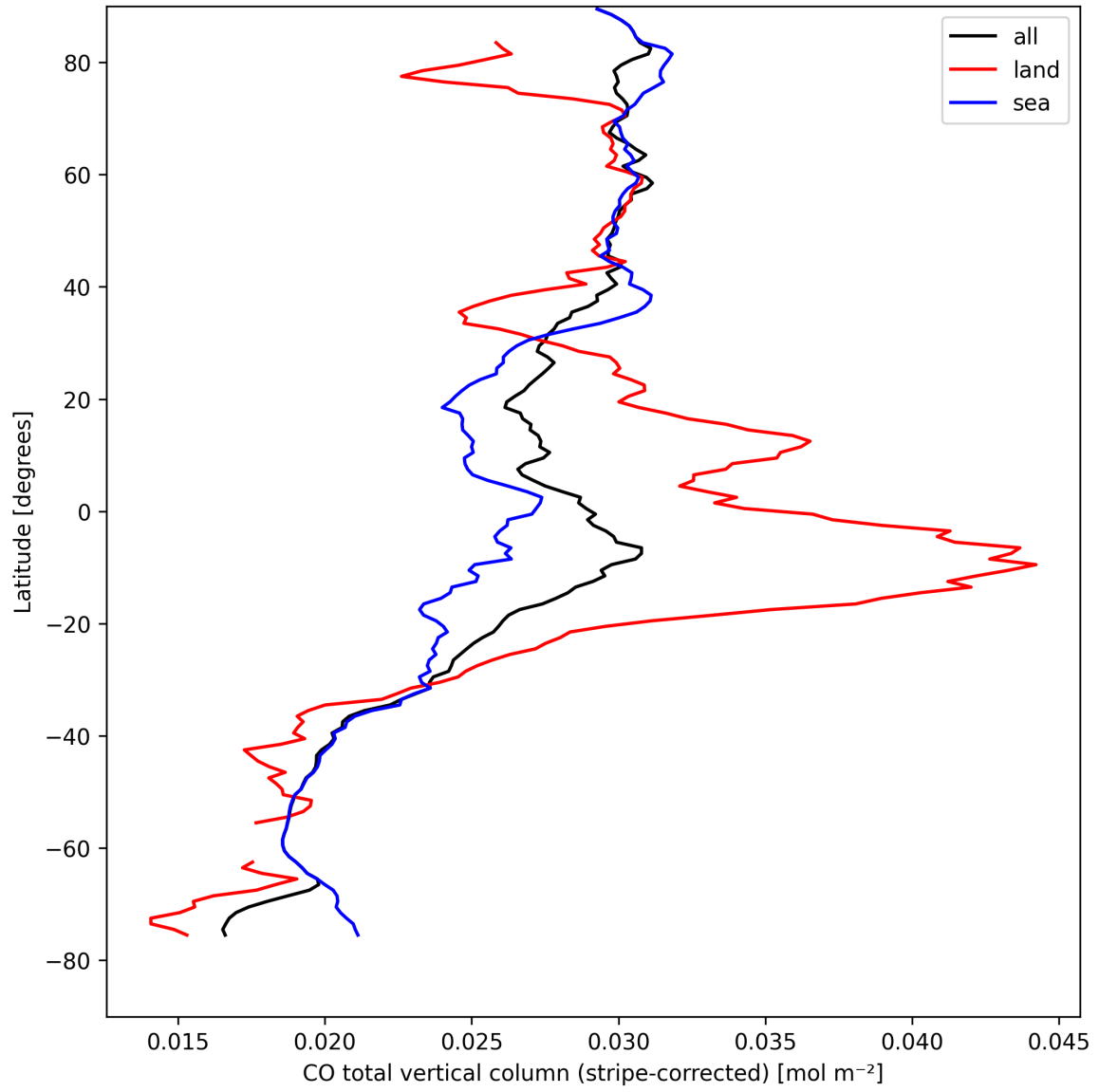
Figure 11: Zonal average of “CO total vertical column (stripe-corrected)” for 2025-08-28 to 2025-08-30.
