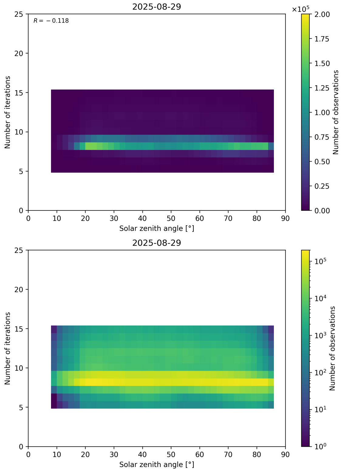
Figure 67: Scatter density plot of “Solar zenith angle” against “Number of iterations” for 2025-08-28 to 2025-08-30.
