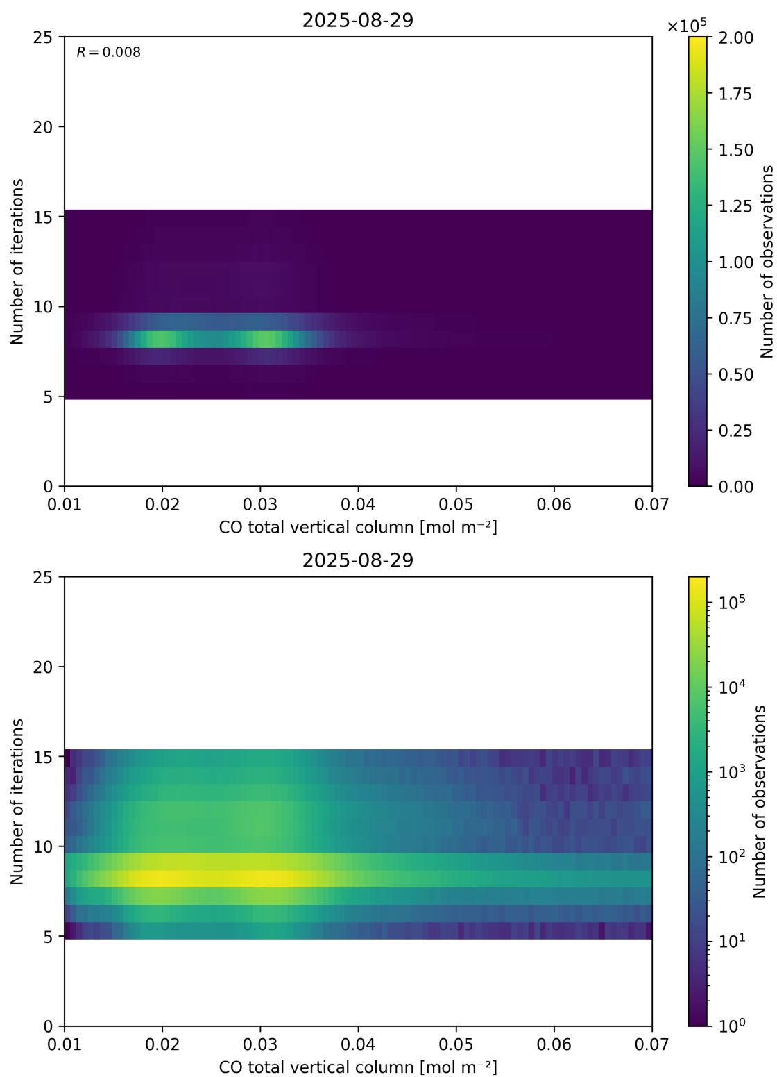
Figure 42: Scatter density plot of “CO total vertical column” against “Number of iterations” for 2025-08-28 to 2025-08-30.
