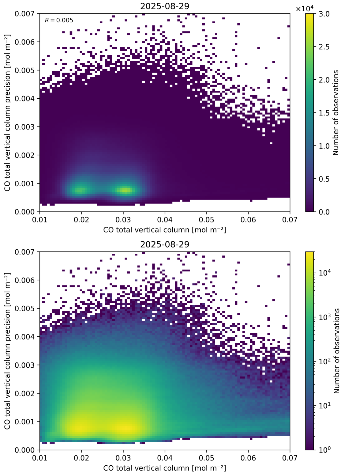
Figure 34: Scatter density plot of “CO total vertical column” against “CO total vertical column precision” for 2025-08-28 to 2025-08-30.
