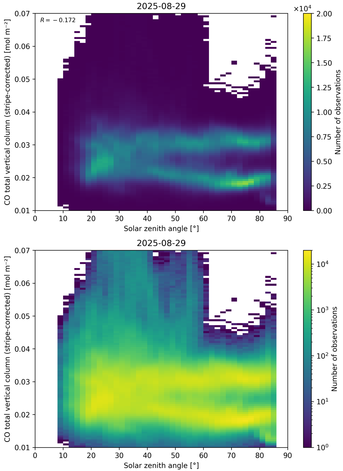
Figure 62: Scatter density plot of “Solar zenith angle” against “CO total vertical column (stripe-corrected)” for 2025-08-28 to 2025-08-30.
