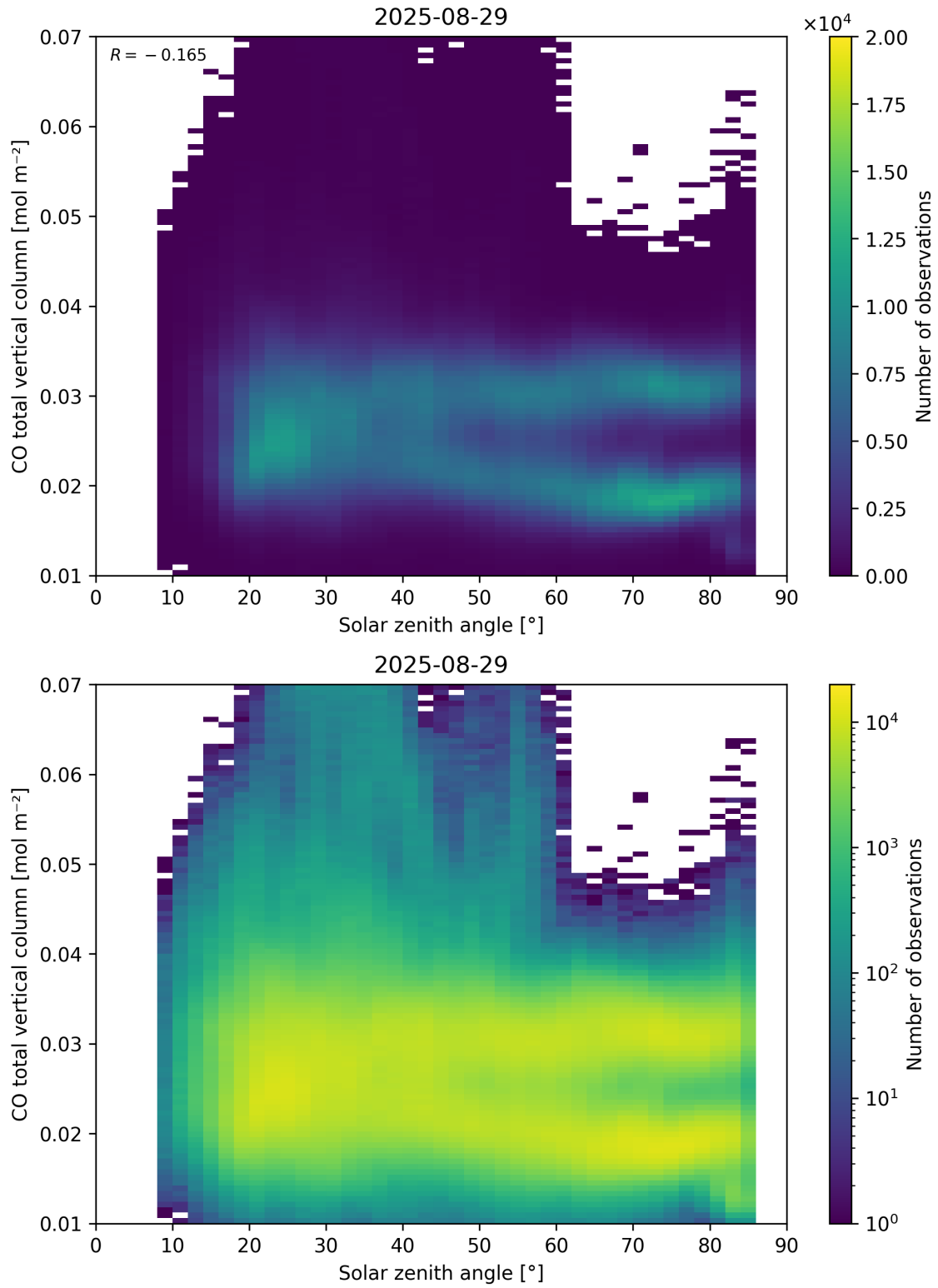
Figure 61: Scatter density plot of “Solar zenith angle” against “CO total vertical column” for 2025-08-28 to 2025-08-30.
