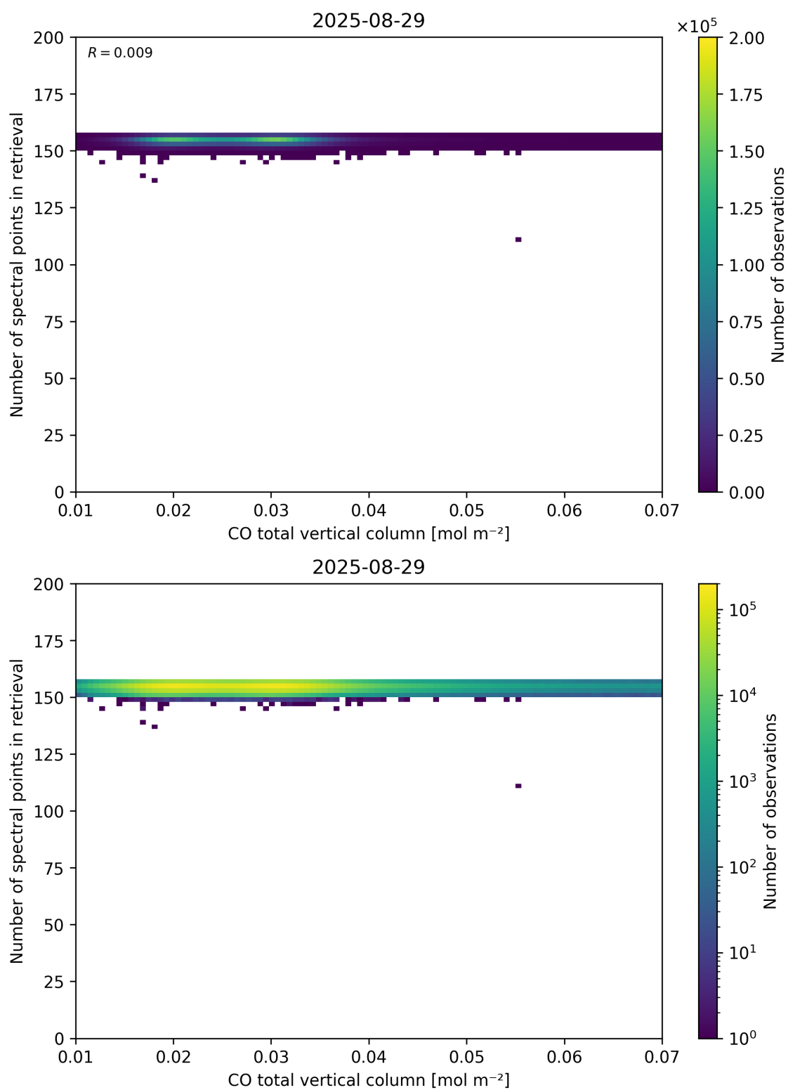
Figure 43: Scatter density plot of “CO total vertical column” against “Number of spectral points in retrieval” for 2025-08-28 to 2025-08-30.
