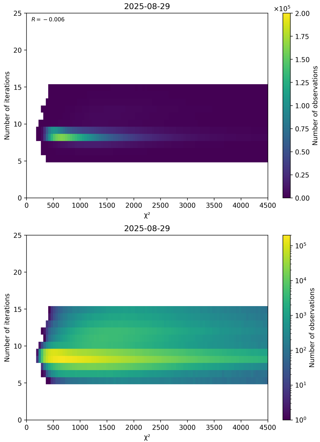
Figure 49: Scatter density plot of “ \chi^2 ” against “Number of iterations” for 2025-08-28 to 2025-08-30.
