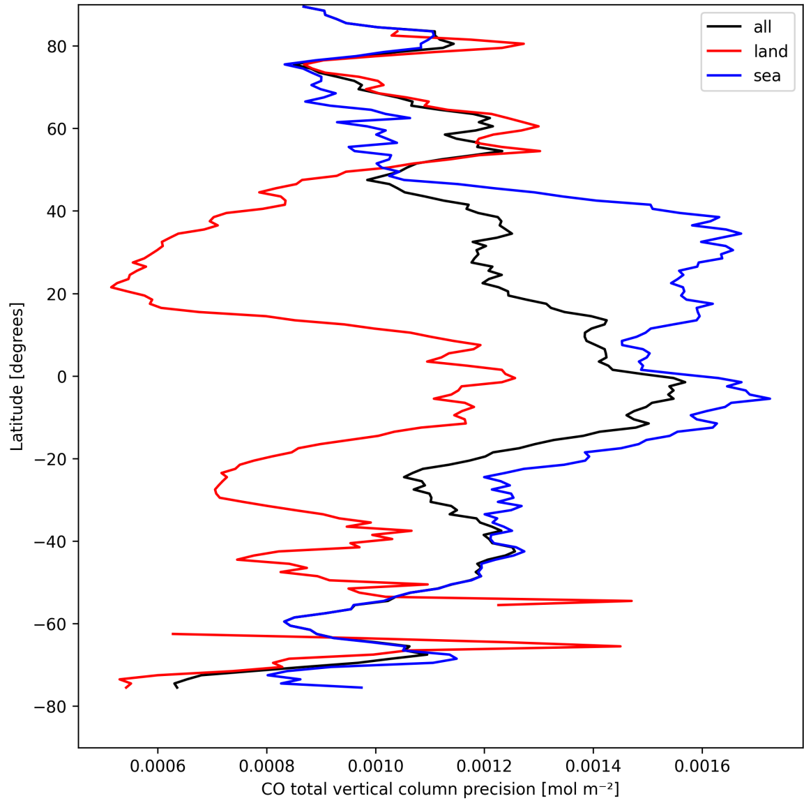
Figure 12: Zonal average of “CO total vertical column precision” for 2025-08-28 to 2025-08-30.
