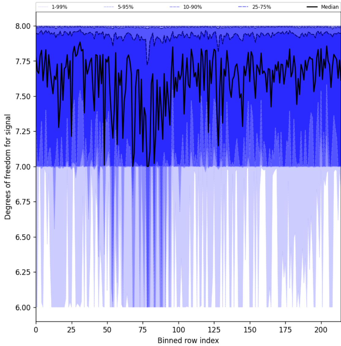
Figure 31: Along track statistics of “Degrees of freedom for signal” for 2025-08-28 to 2025-08-30
