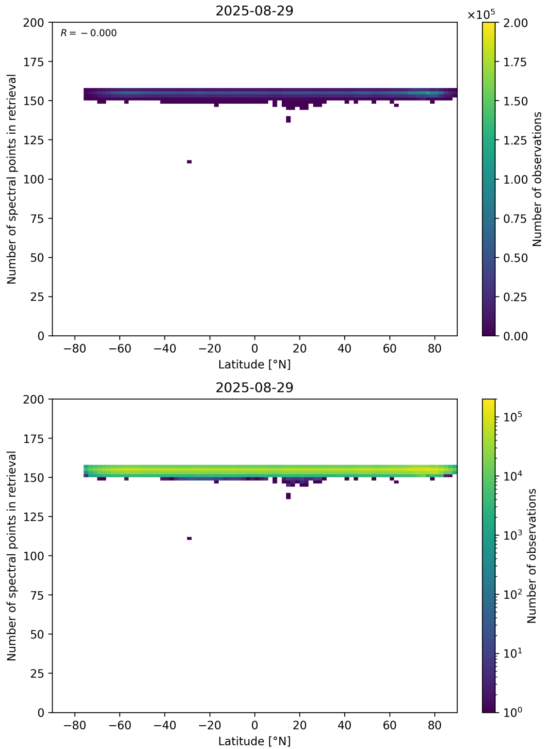
Figure 57: Scatter density plot of “Latitude” against “Number of spectral points in retrieval” for 2025-08-28 to 2025-08-30.
