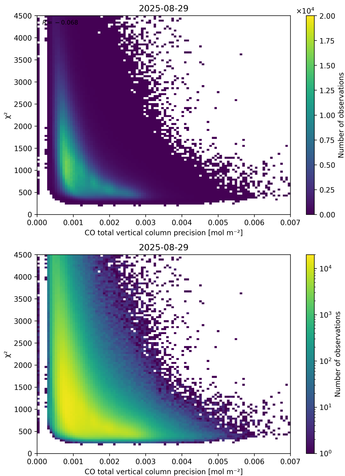
Figure 44: Scatter density plot of “CO total vertical column precision” against “ \chi^2 ” for 2025-08-28 to 2025-08-30.
