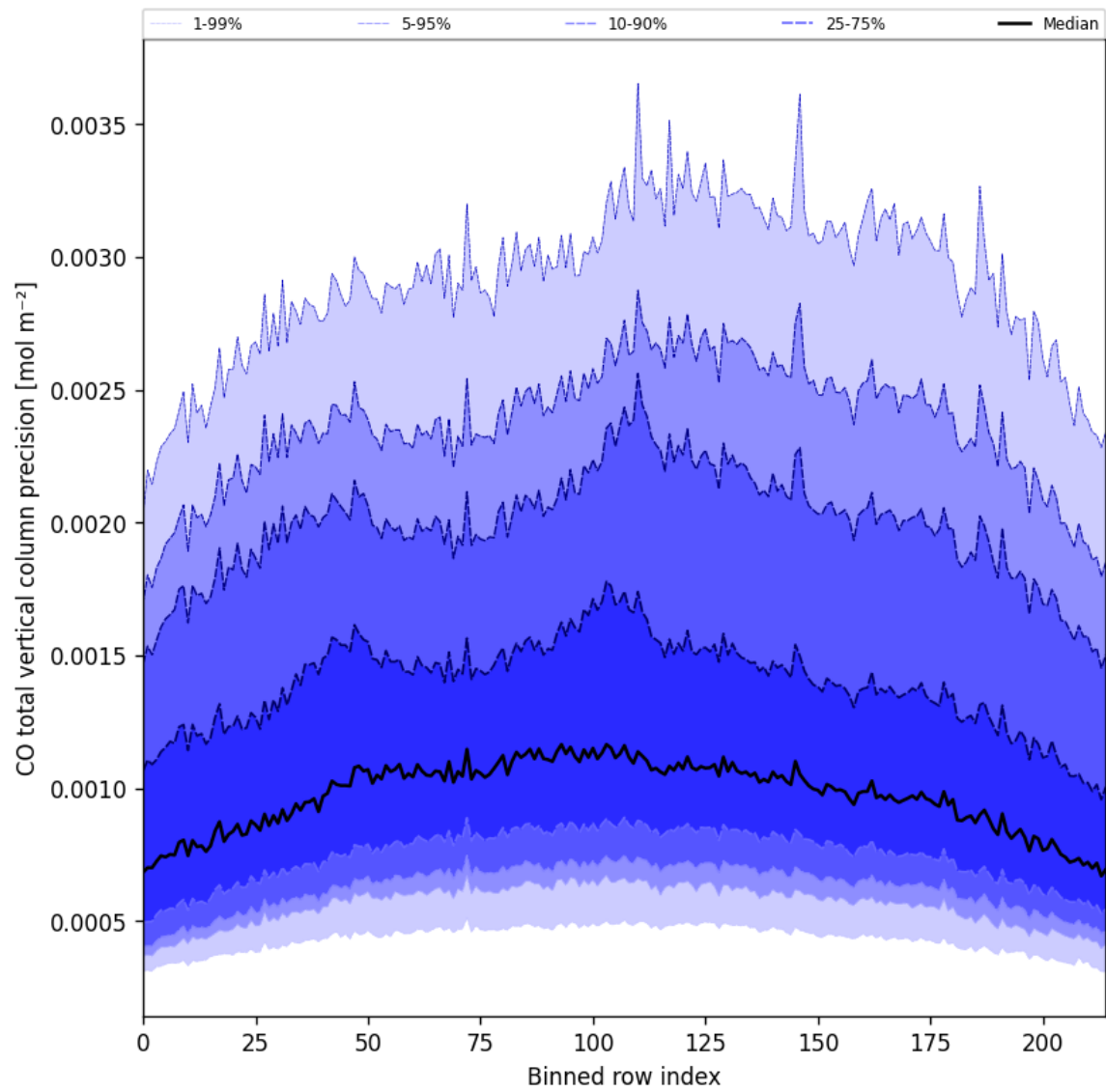
Figure 28: Along track statistics of “CO total vertical column precision” for 2025-08-28 to 2025-08-30
