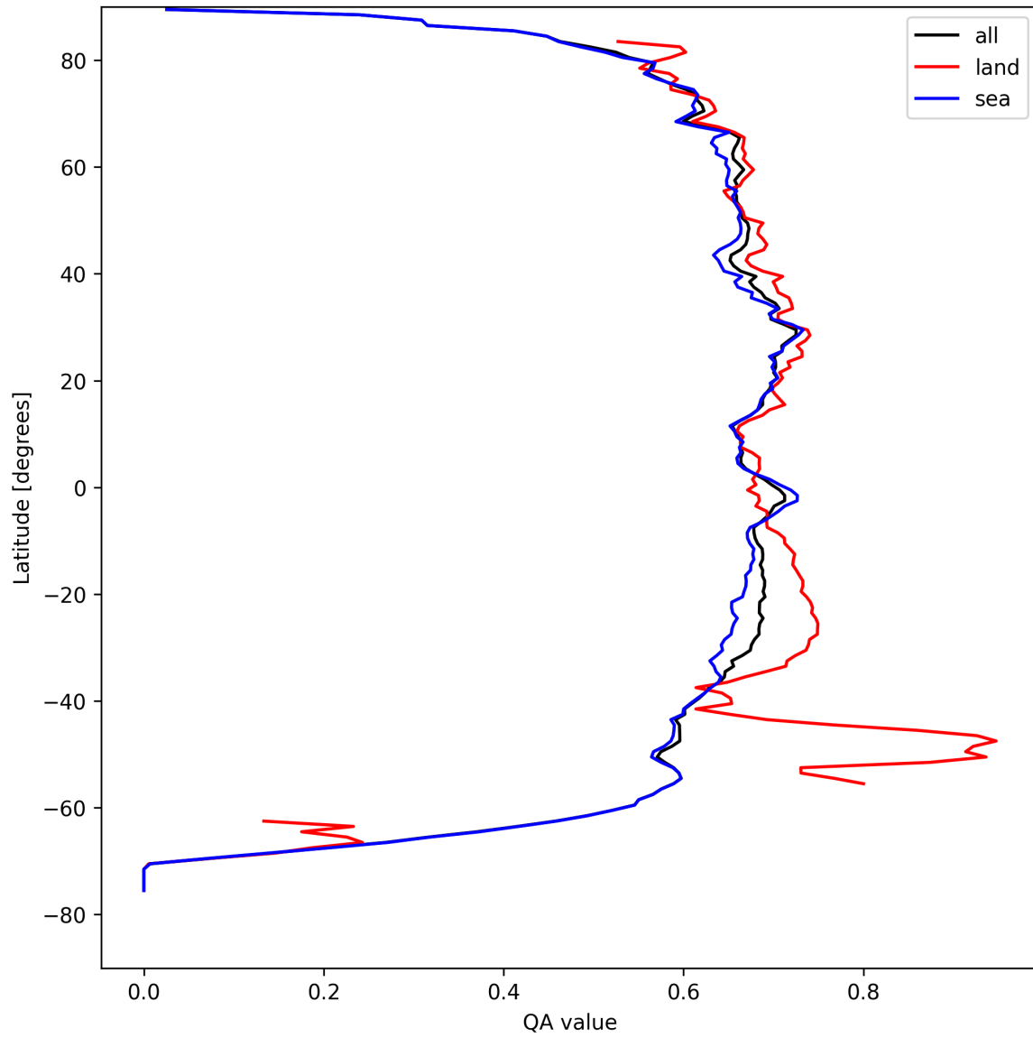
Figure 9: Zonal average of “QA value” for 2025-08-28 to 2025-08-30.
