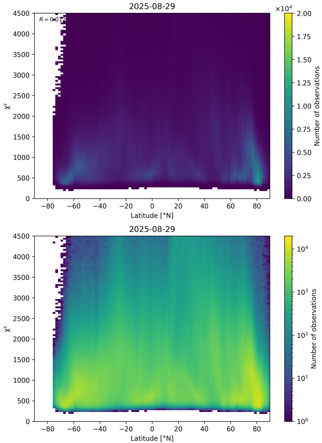
Figure 54: Scatter density plot of “Latitude” against “ \chi^2 ” for 2025-08-28 to 2025-08-30.
