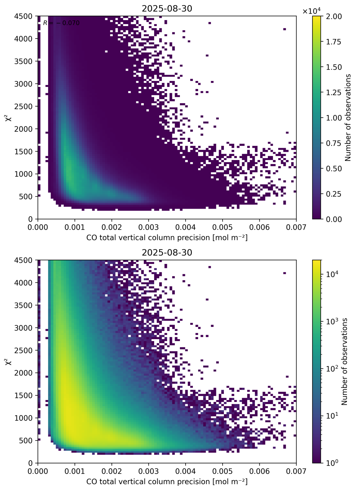
Figure 44: Scatter density plot of “CO total vertical column precision” against “ \chi^2 ” for 2025-08-30 to 2025-08-31.
