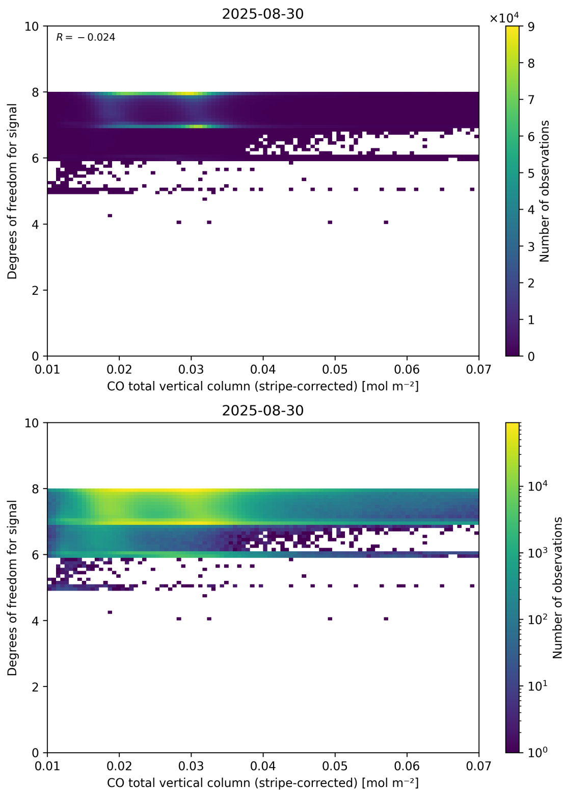
Figure 38: Scatter density plot of “CO total vertical column (stripe-corrected)” against “Degrees of freedom for signal” for 2025-08-30 to 2025-08-31.
