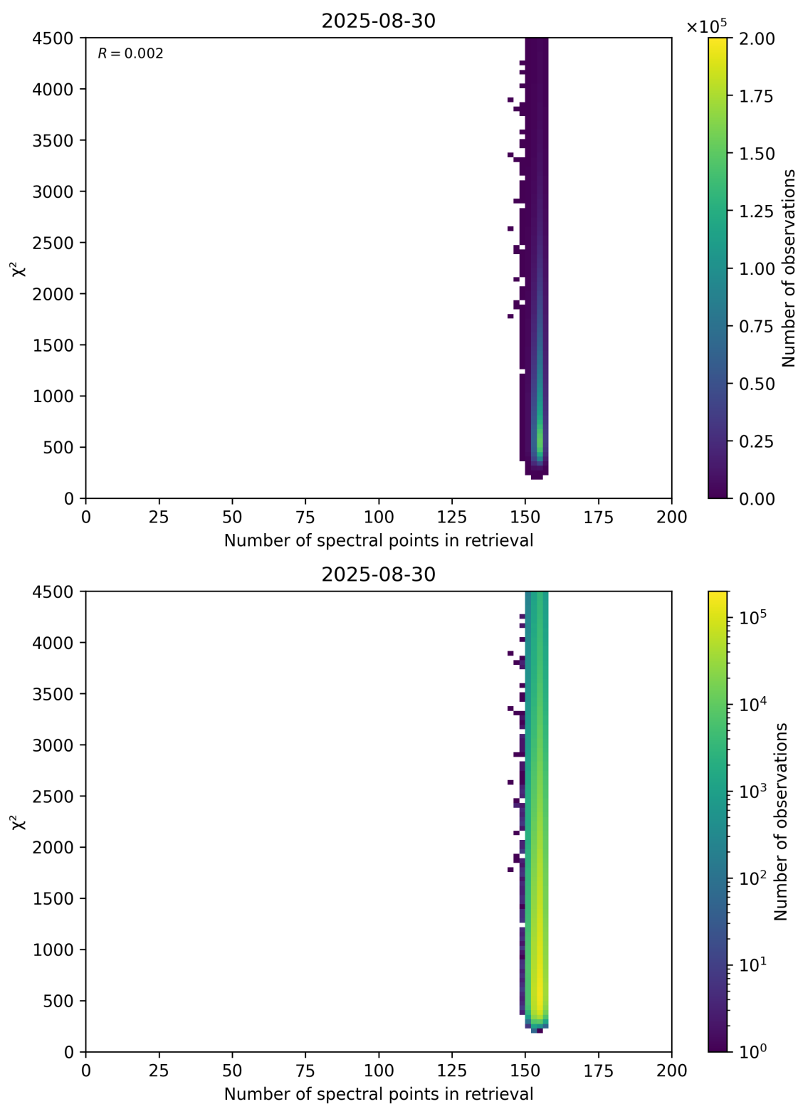
Figure 58: Scatter density plot of “Number of spectral points in retrieval” against “ \chi^2 ” for 2025-08-30 to 2025-08-31.
