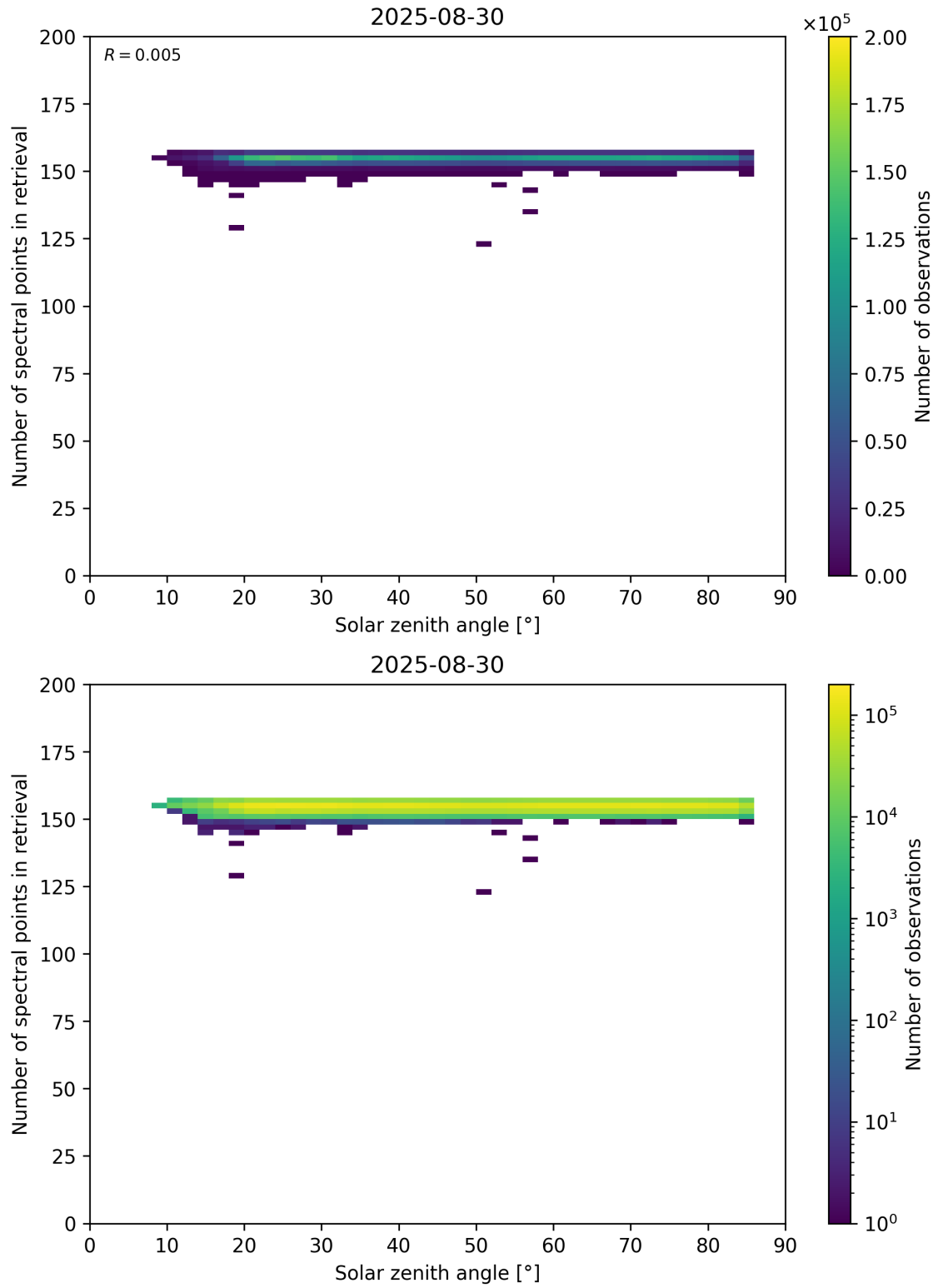
Figure 68: Scatter density plot of “Solar zenith angle” against “Number of spectral points in retrieval” for 2025-08-30 to 2025-08-31.
