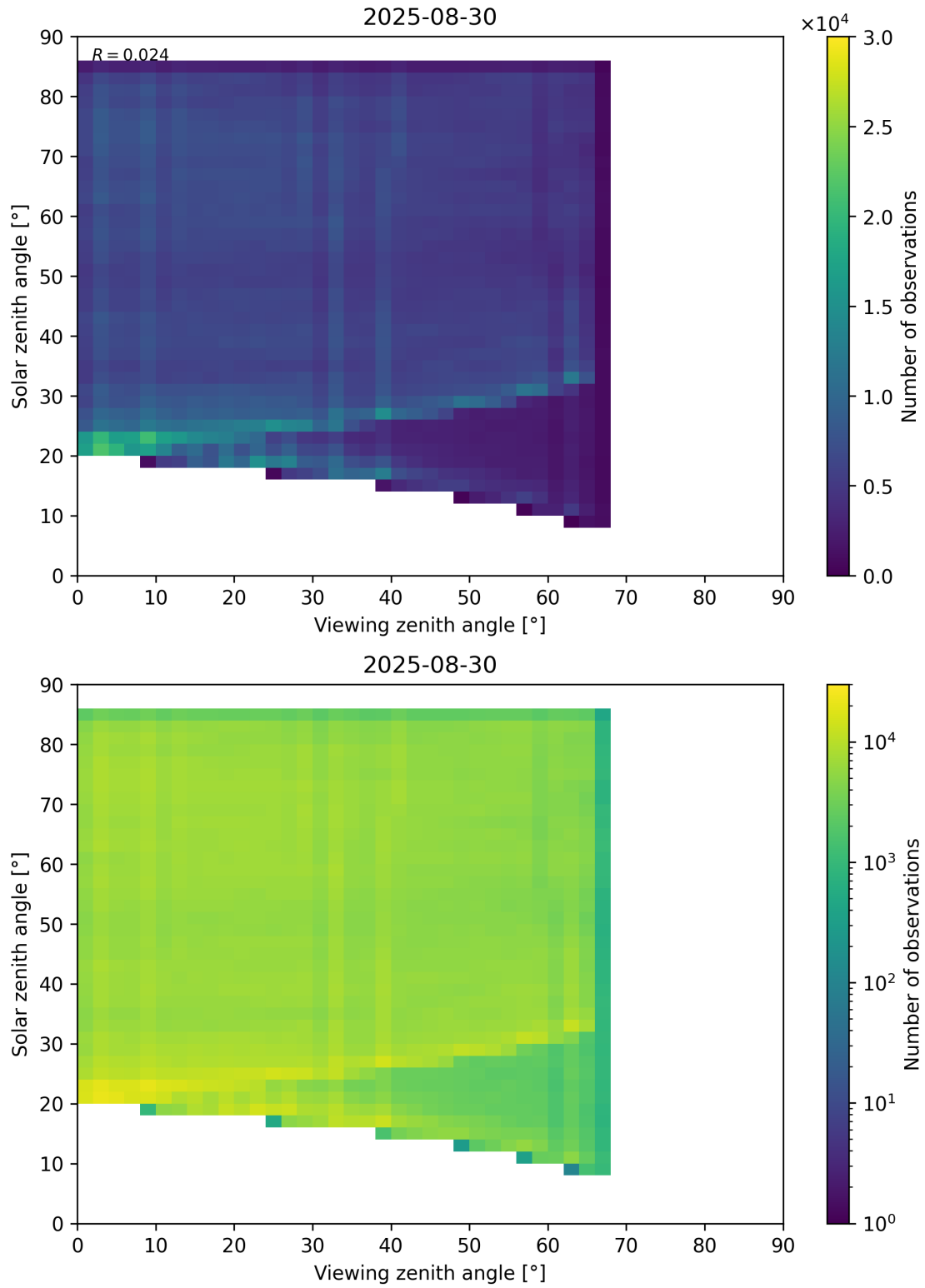
Figure 77: Scatter density plot of “Viewing zenith angle” against “Solar zenith angle” for 2025-08-30 to 2025-08-31.
