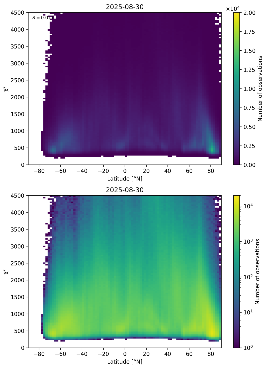
Figure 54: Scatter density plot of “Latitude” against “ \chi^2 ” for 2025-08-30 to 2025-08-31.
