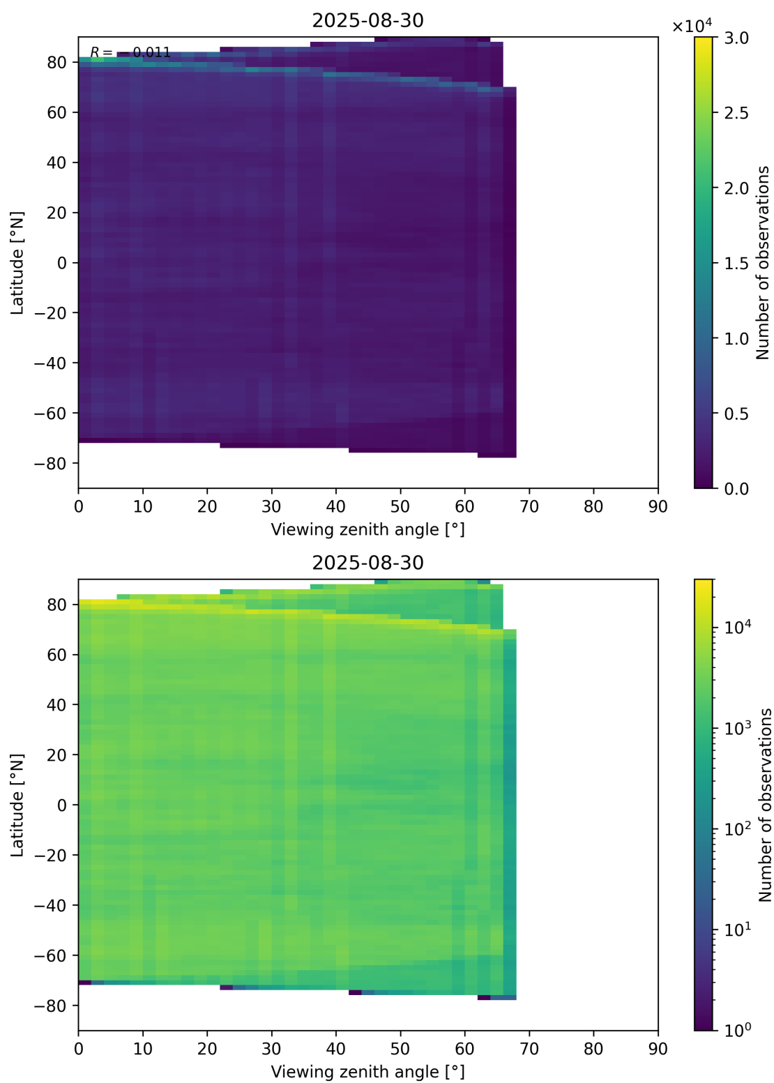
Figure 74: Scatter density plot of “Viewing zenith angle” against “Latitude” for 2025-08-30 to 2025-08-31.
