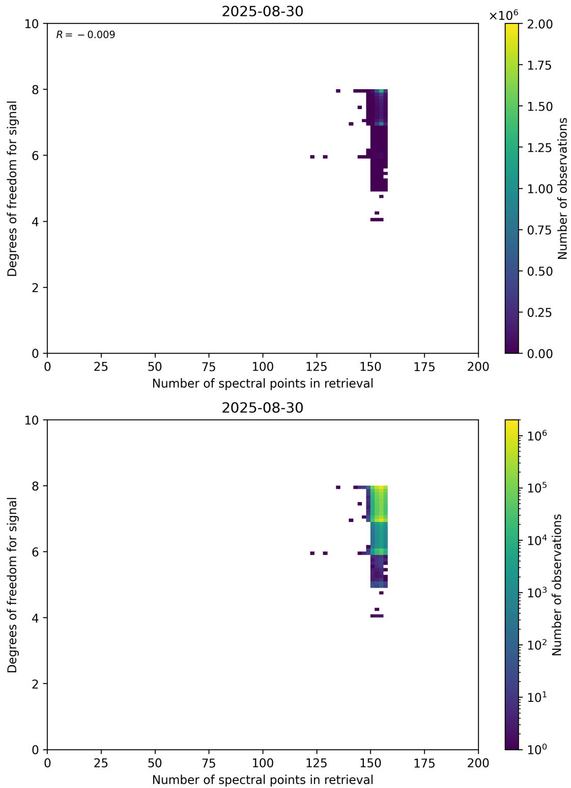
Figure 59: Scatter density plot of “Number of spectral points in retrieval” against “Degrees of freedom for signal” for 2025-08-30 to 2025-08-31.
