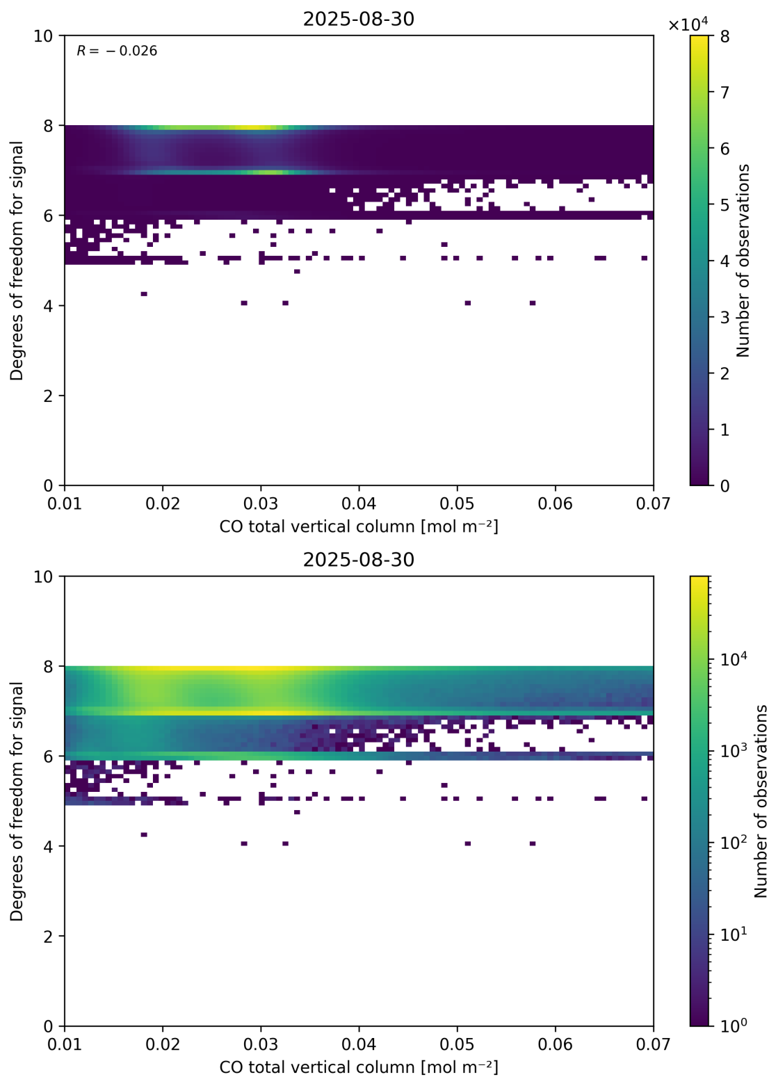
Figure 41: Scatter density plot of “CO total vertical column” against “Degrees of freedom for signal” for 2025-08-30 to 2025-08-31.
