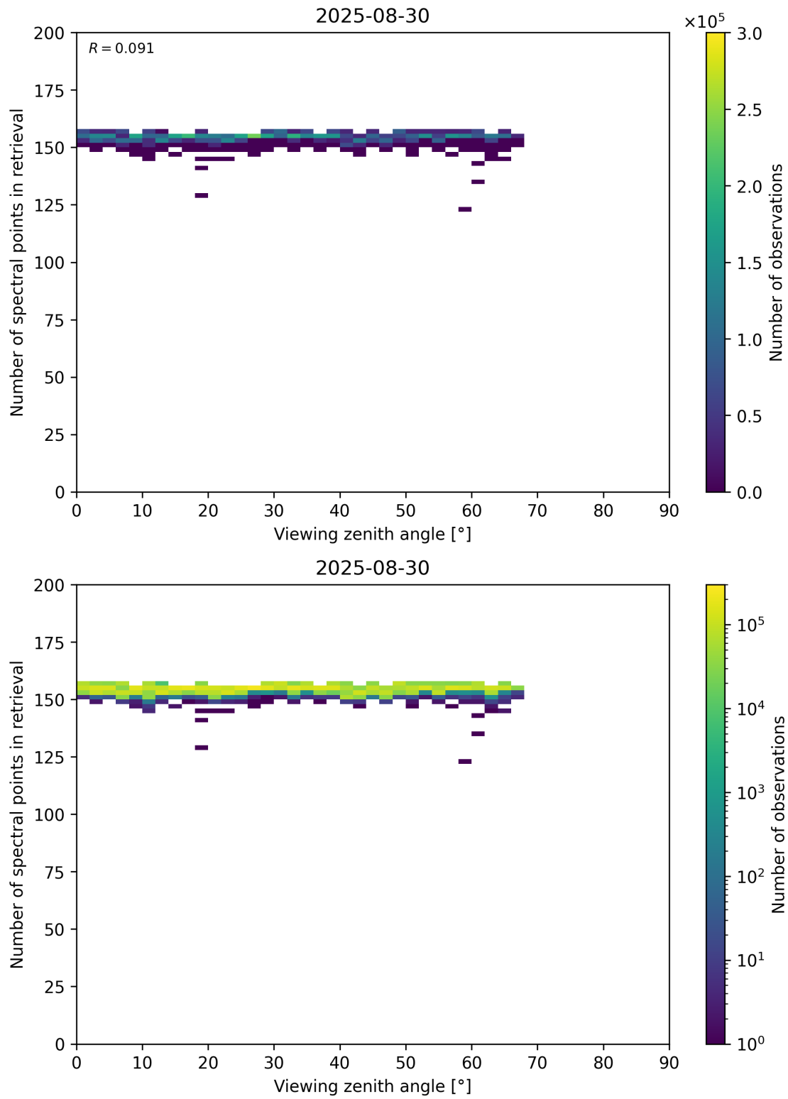
Figure 76: Scatter density plot of “Viewing zenith angle” against “Number of spectral points in retrieval” for 2025-08-30 to 2025-08-31.
