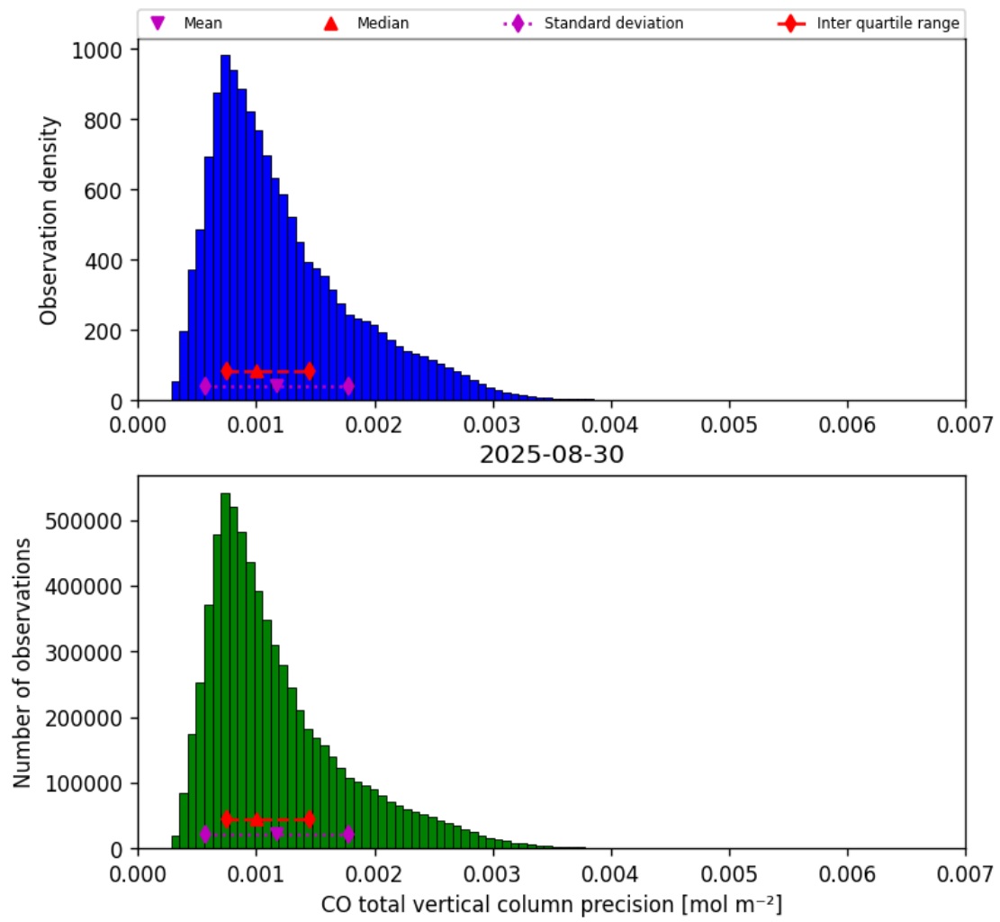
Figure 20: Histogram of “CO total vertical column precision” for 2025-08-30 to 2025-08-31
