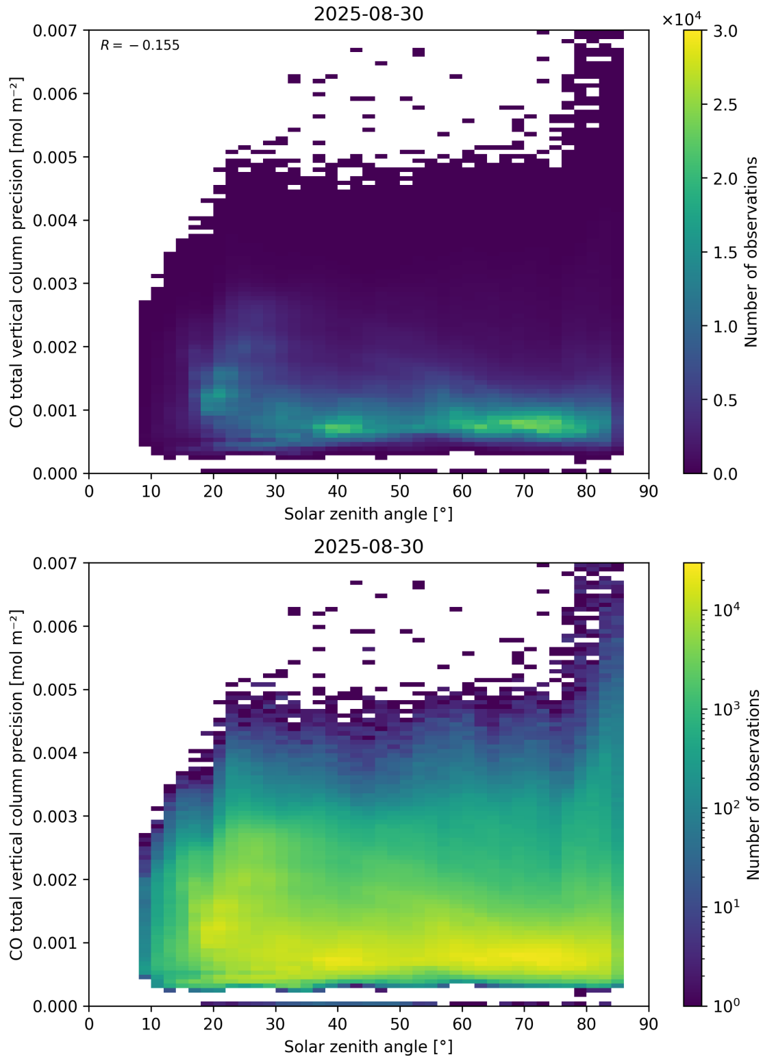
Figure 63: Scatter density plot of “Solar zenith angle” against “CO total vertical column precision” for 2025-08-30 to 2025-08-31.
