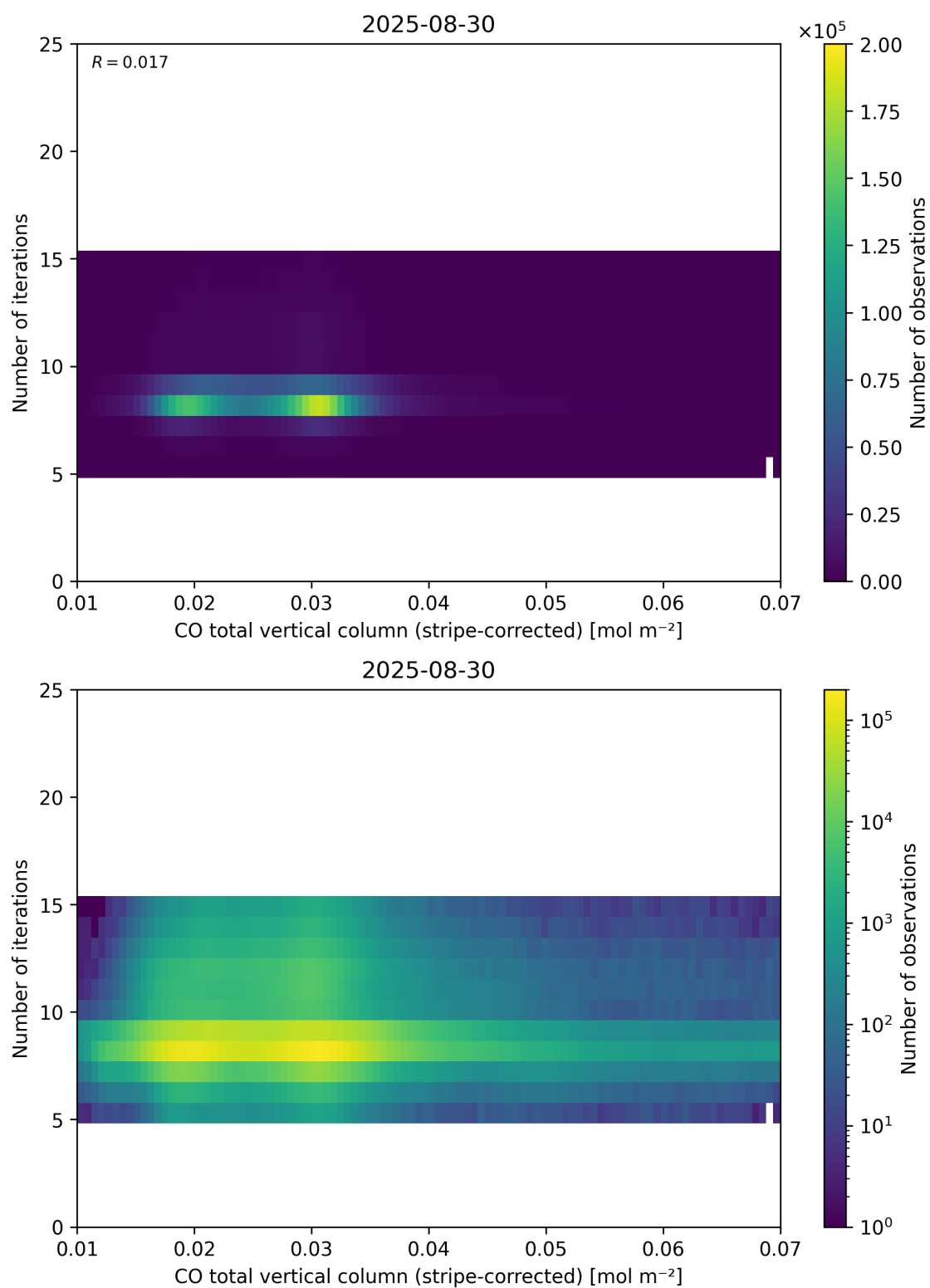
Figure 39: Scatter density plot of “CO total vertical column (stripe-corrected)” against “Number of iterations” for 2025-08-30 to 2025-08-31.
