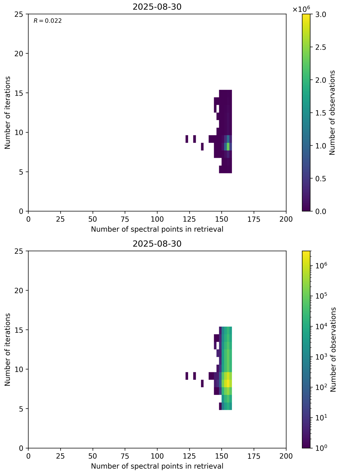
Figure 60: Scatter density plot of “Number of spectral points in retrieval” against “Number of iterations” for 2025-08-30 to 2025-08-31.
