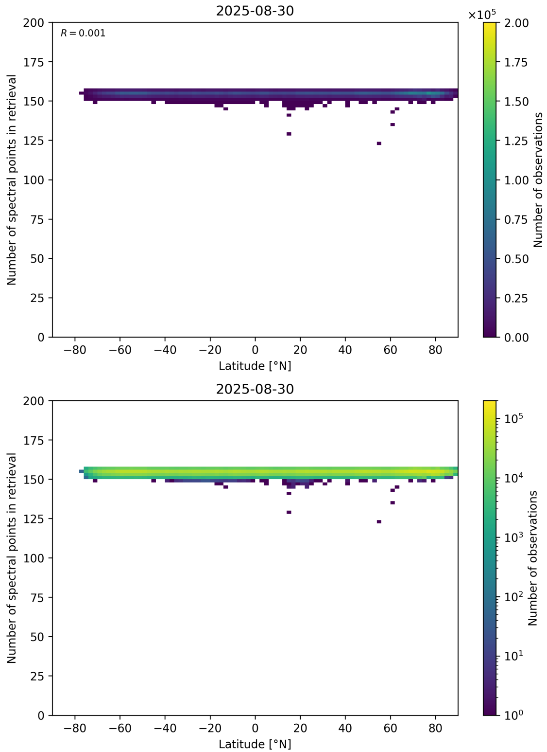
Figure 57: Scatter density plot of “Latitude” against “Number of spectral points in retrieval” for 2025-08-30 to 2025-08-31.
