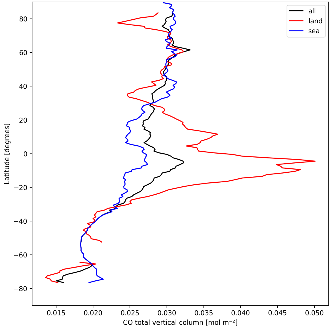
Figure 10: Zonal average of “CO total vertical column” for 2025-08-30 to 2025-08-31.
