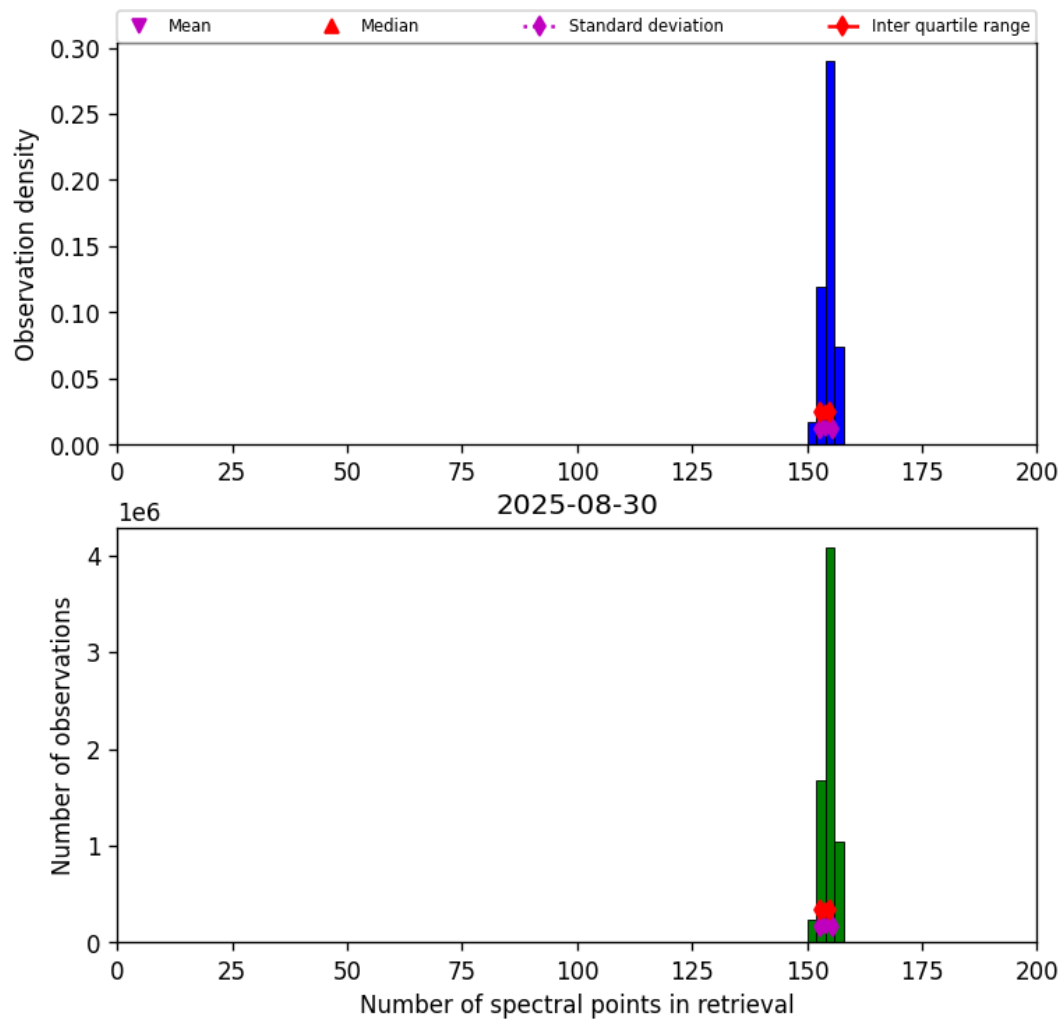
Figure 21: Histogram of “Number of spectral points in retrieval” for 2025-08-30 to 2025-08-31
