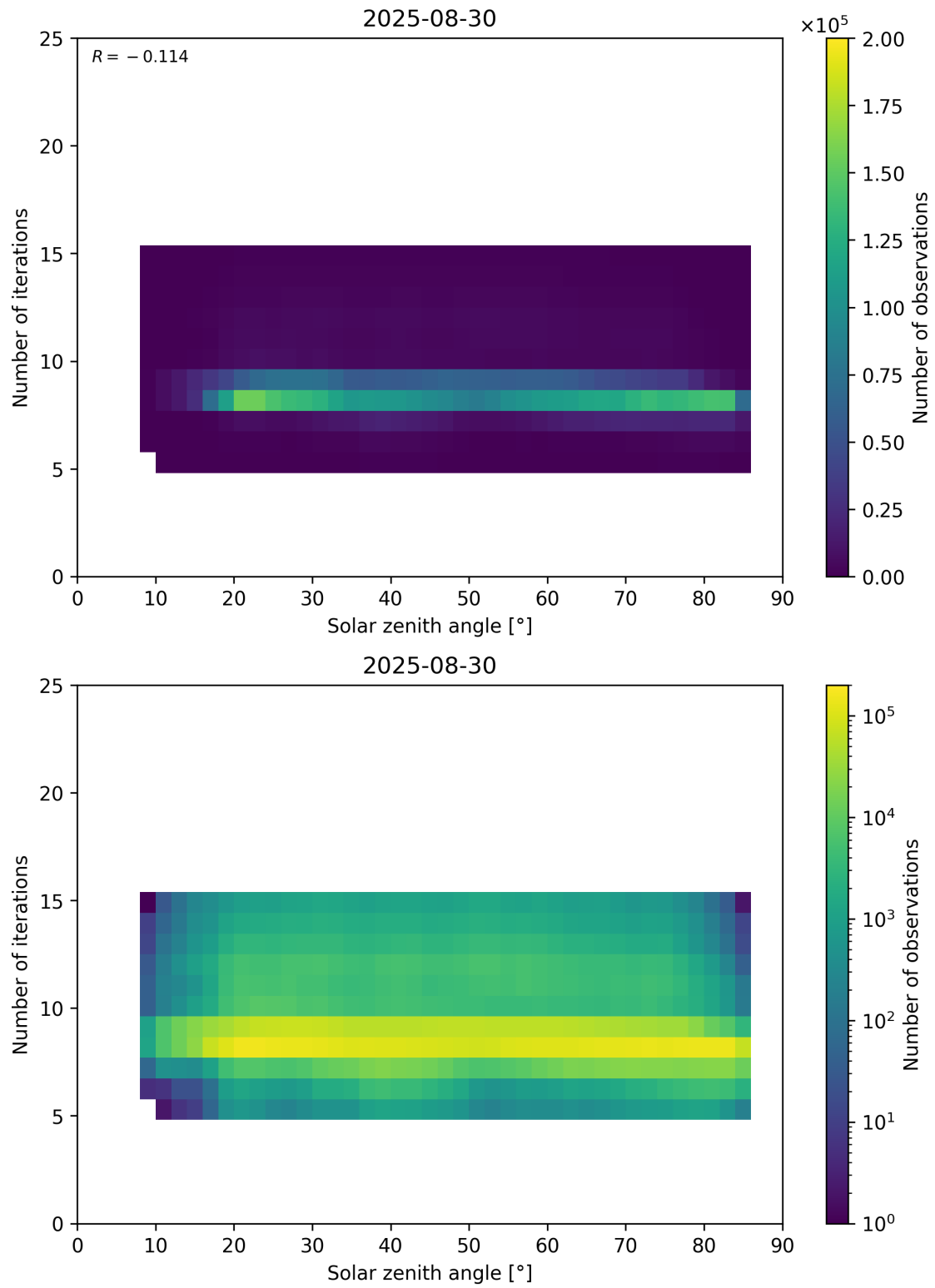
Figure 67: Scatter density plot of “Solar zenith angle” against “Number of iterations” for 2025-08-30 to 2025-08-31.
