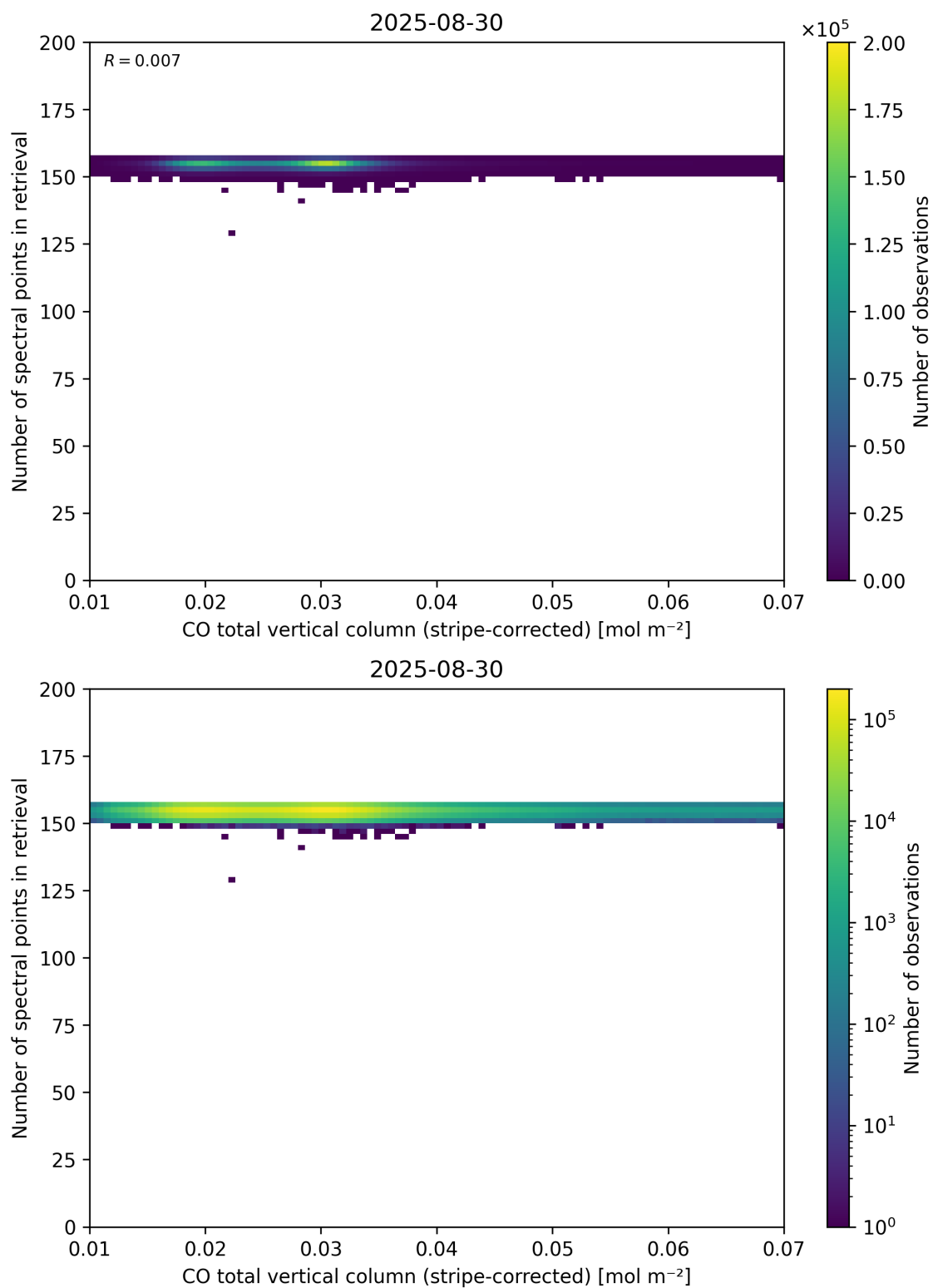
Figure 40: Scatter density plot of “CO total vertical column (stripe-corrected)” against “Number of spectral points in retrieval” for 2025-08-30 to 2025-08-31.
