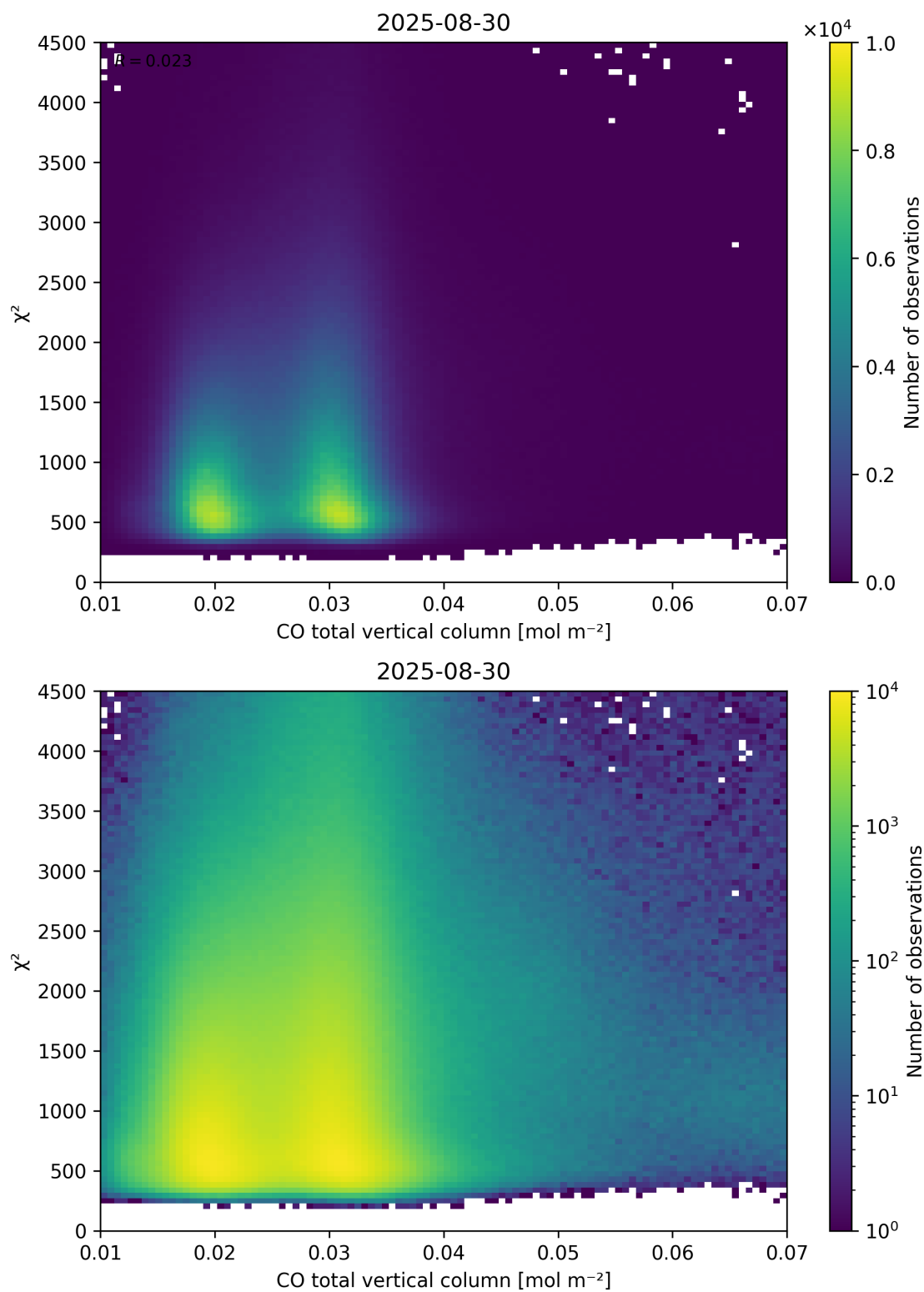
Figure 35: Scatter density plot of “CO total vertical column” against “ \chi^2 ” for 2025-08-30 to 2025-08-31.
