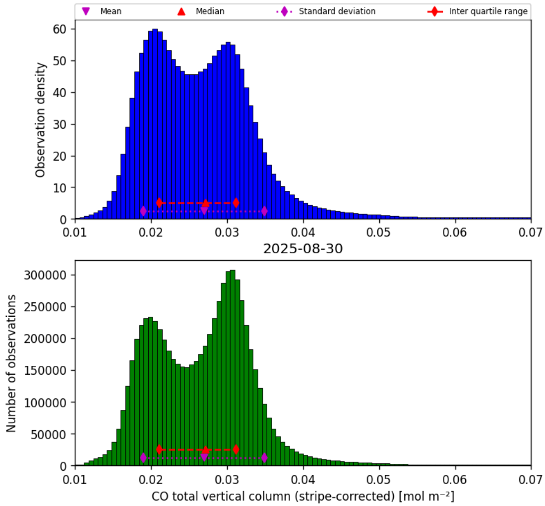
Figure 19: Histogram of “CO total vertical column (stripe-corrected)” for 2025-08-30 to 2025-08-31
