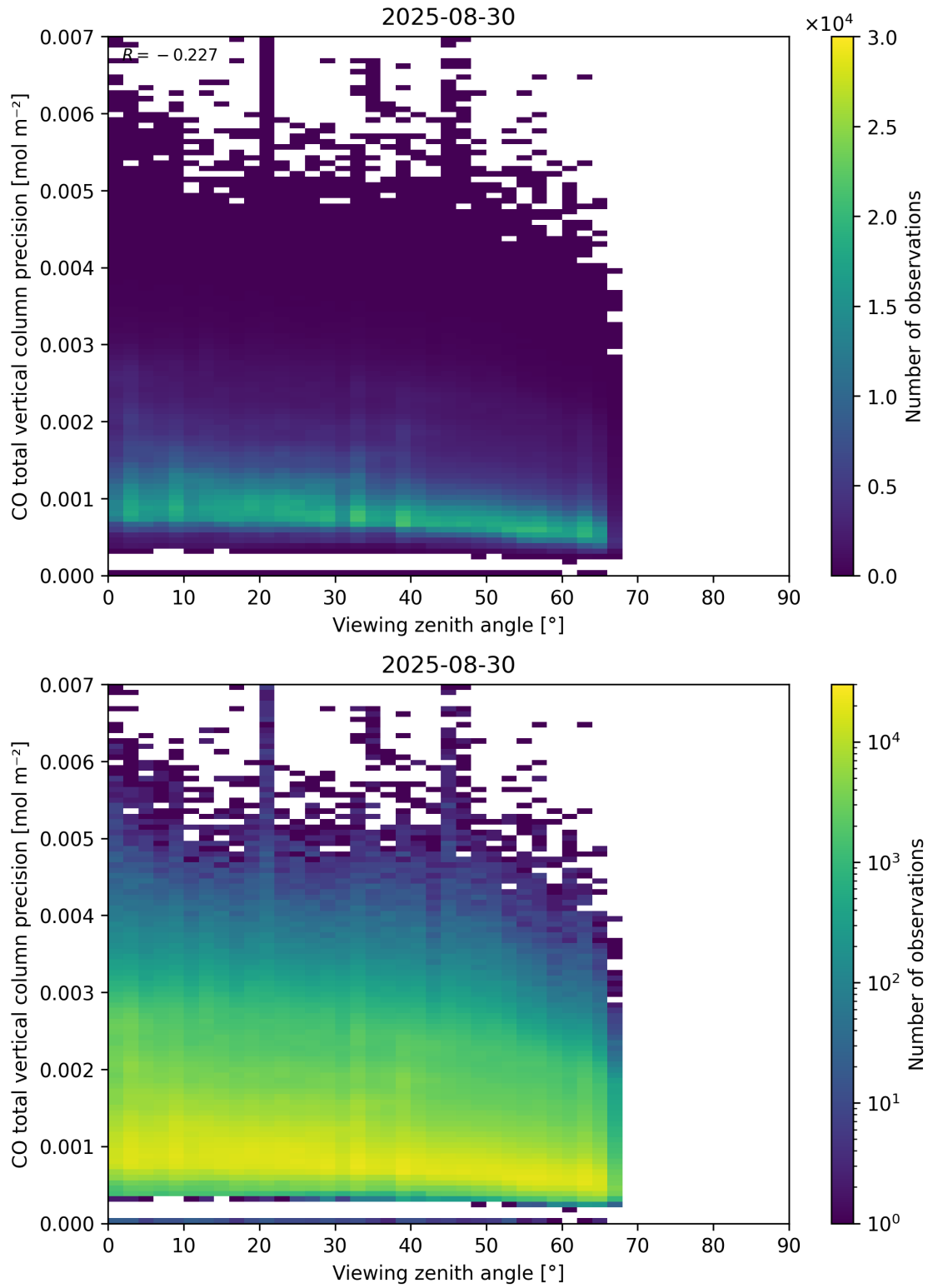
Figure 71: Scatter density plot of “Viewing zenith angle” against “CO total vertical column precision” for 2025-08-30 to 2025-08-31.
