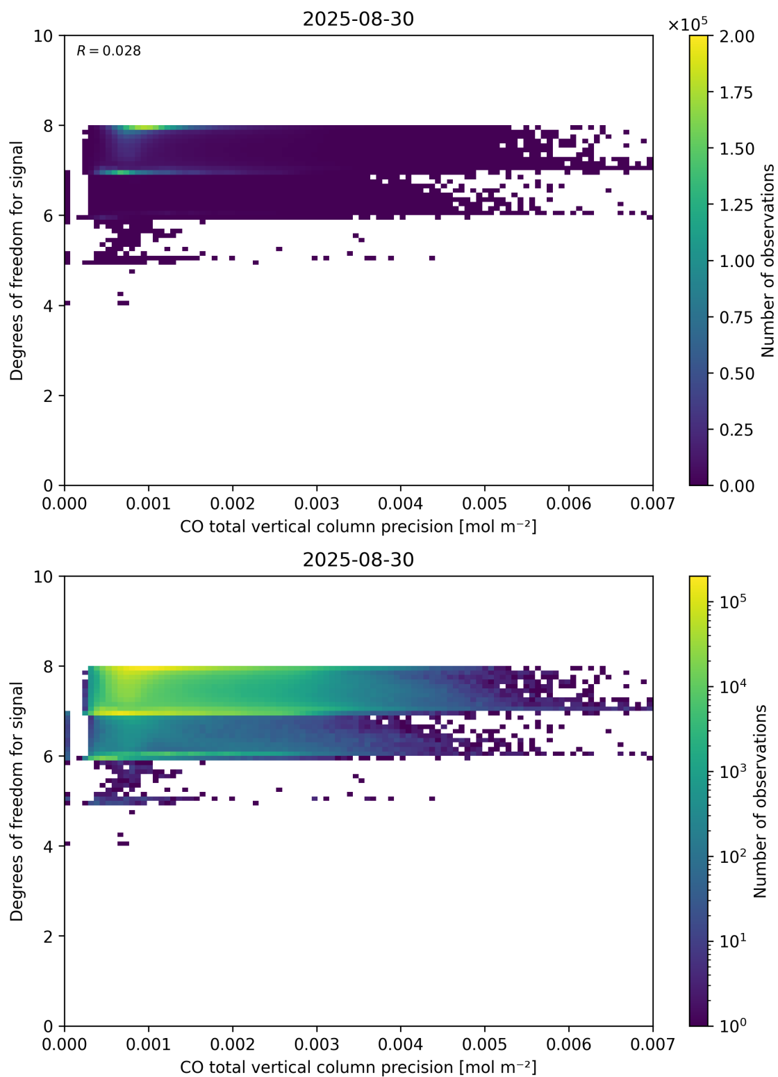
Figure 45: Scatter density plot of “CO total vertical column precision” against “Degrees of freedom for signal” for 2025-08-30 to 2025-08-31.
