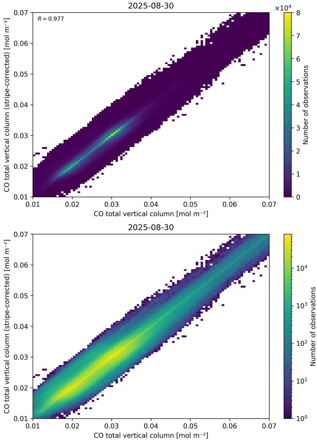
Figure 33: Scatter density plot of “CO total vertical column” against “CO total vertical column (stripe-corrected)” for 2025-08-30 to 2025-08-31.
