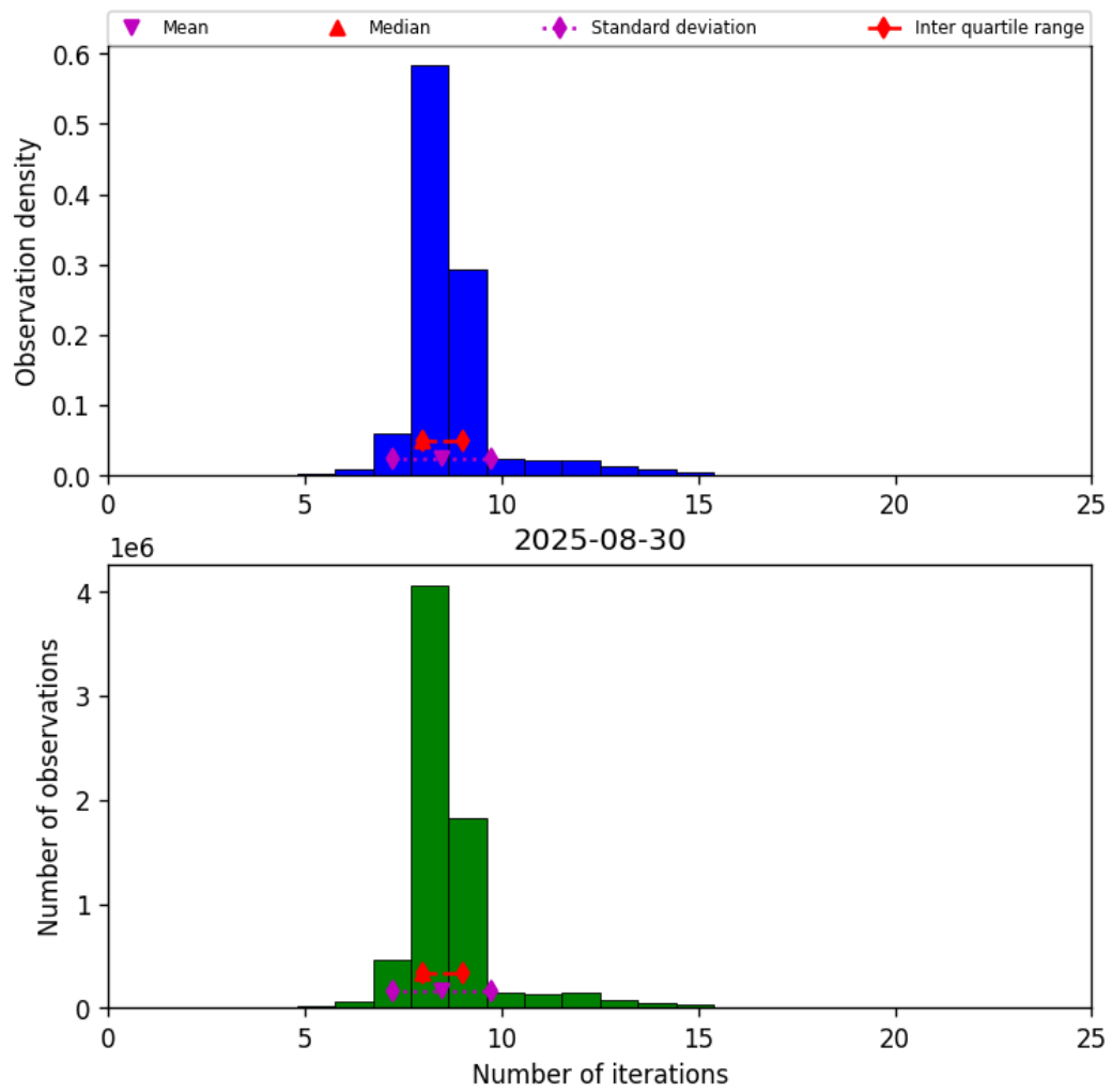
Figure 24: Histogram of “Number of iterations” for 2025-08-30 to 2025-08-31
