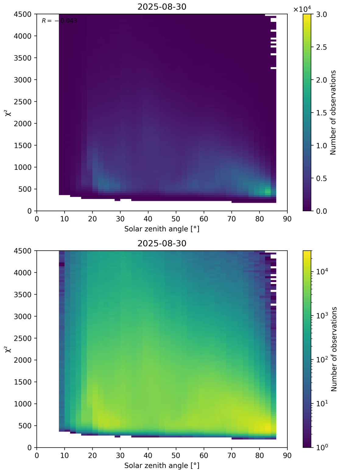
Figure 64: Scatter density plot of “Solar zenith angle” against “ \chi^2 ” for 2025-08-30 to 2025-08-31.
