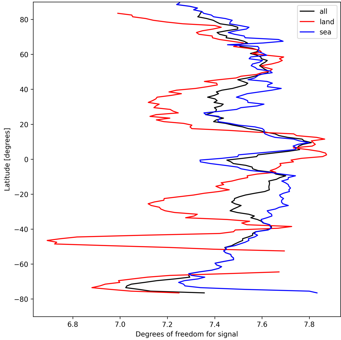
Figure 15: Zonal average of “Degrees of freedom for signal” for 2025-08-30 to 2025-08-31.
