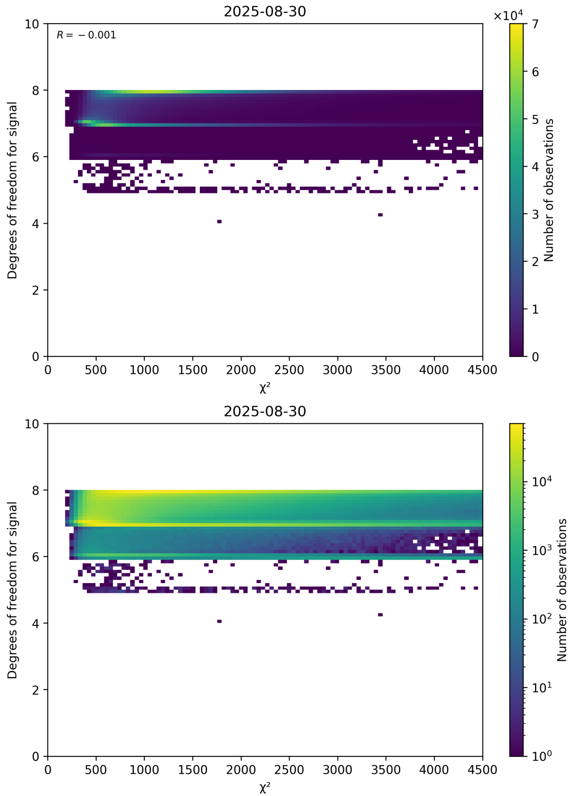
Figure 48: Scatter density plot of “ \chi^2 ” against “Degrees of freedom for signal” for 2025-08-30 to 2025-08-31.
