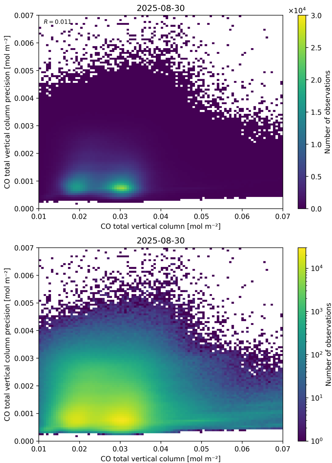
Figure 34: Scatter density plot of “CO total vertical column” against “CO total vertical column precision” for 2025-08-30 to 2025-08-31.
