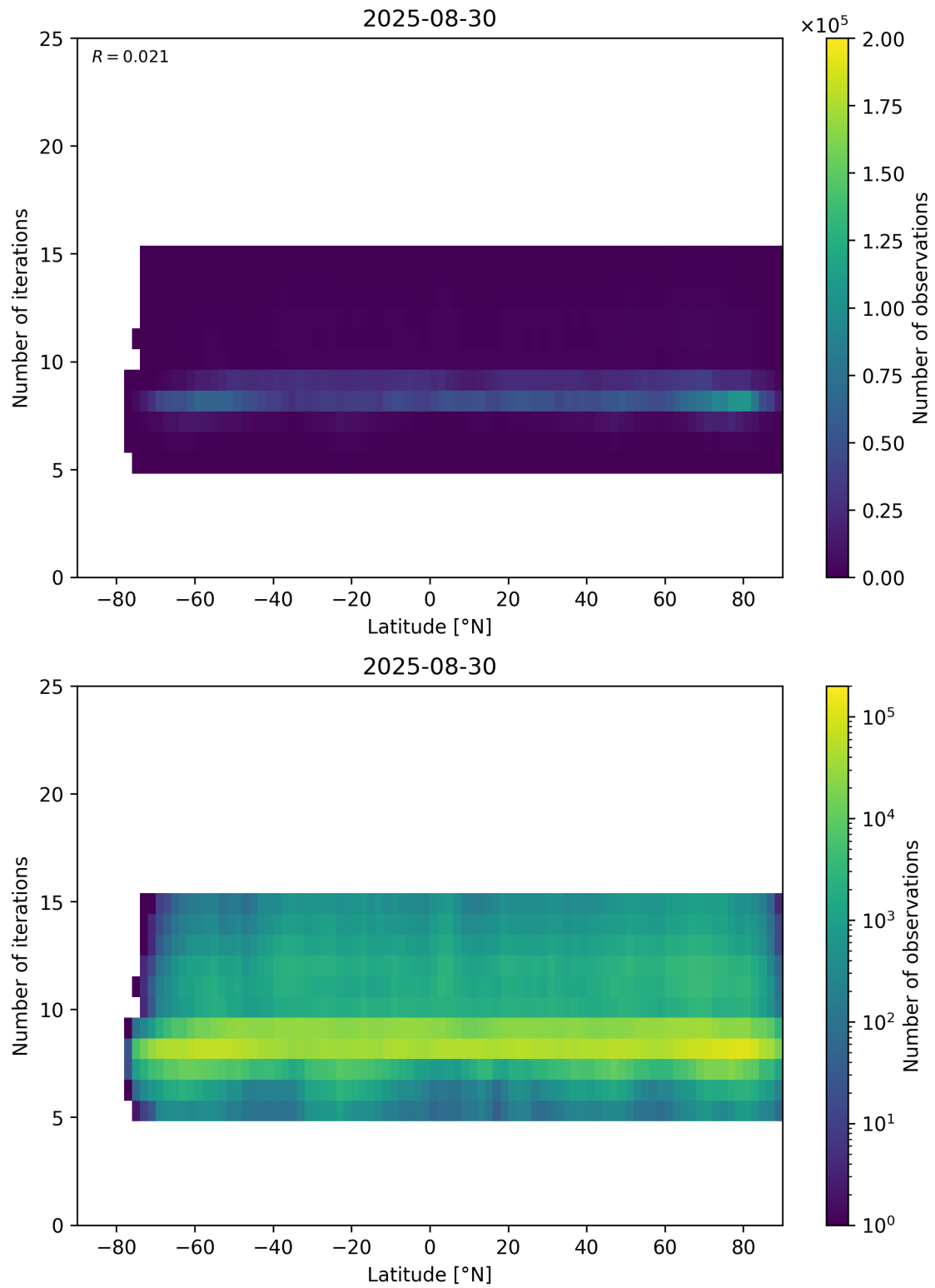
Figure 56: Scatter density plot of “Latitude” against “Number of iterations” for 2025-08-30 to 2025-08-31.
