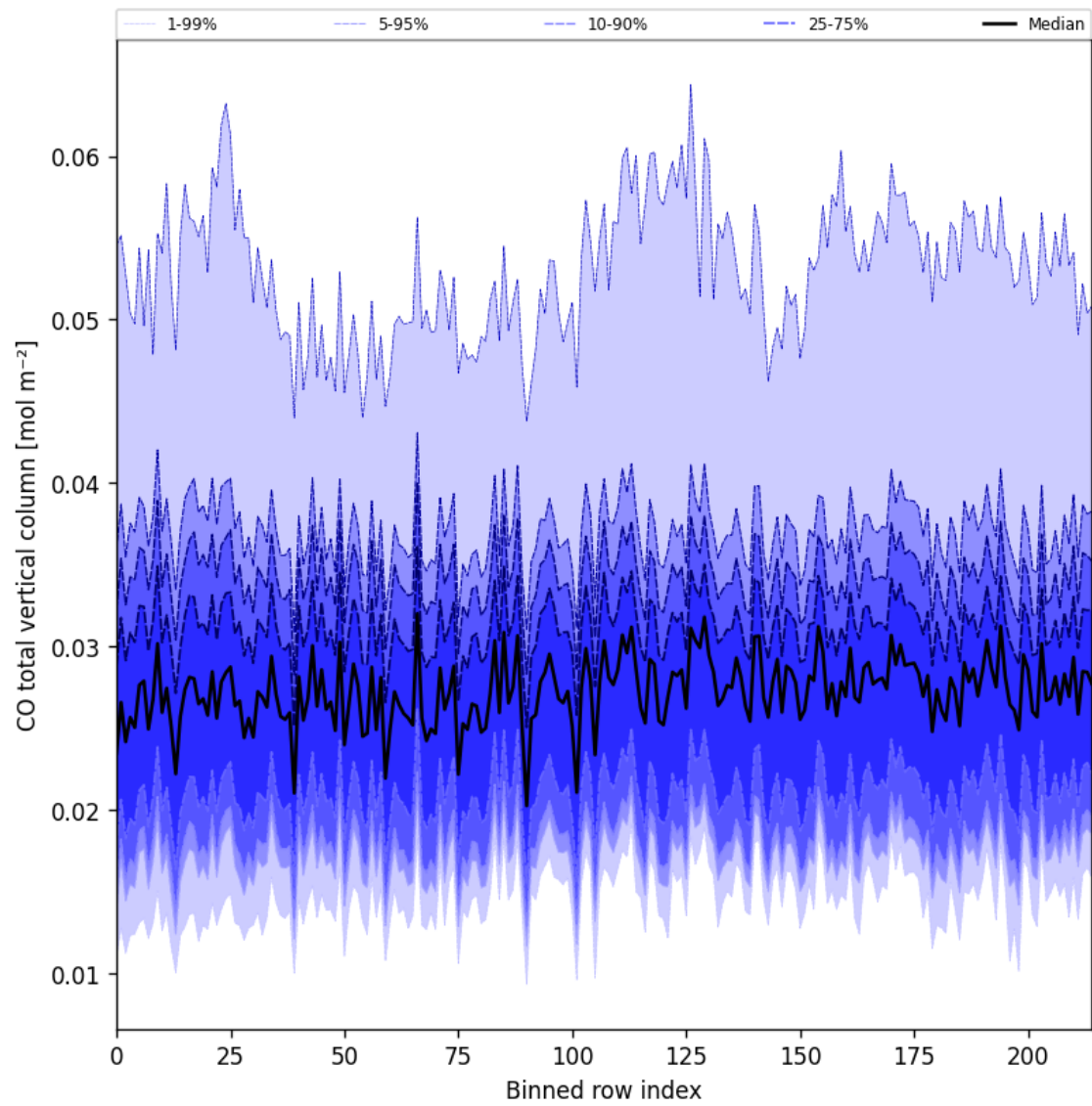
Figure 26: Along track statistics of “CO total vertical column” for 2025-08-30 to 2025-08-31
