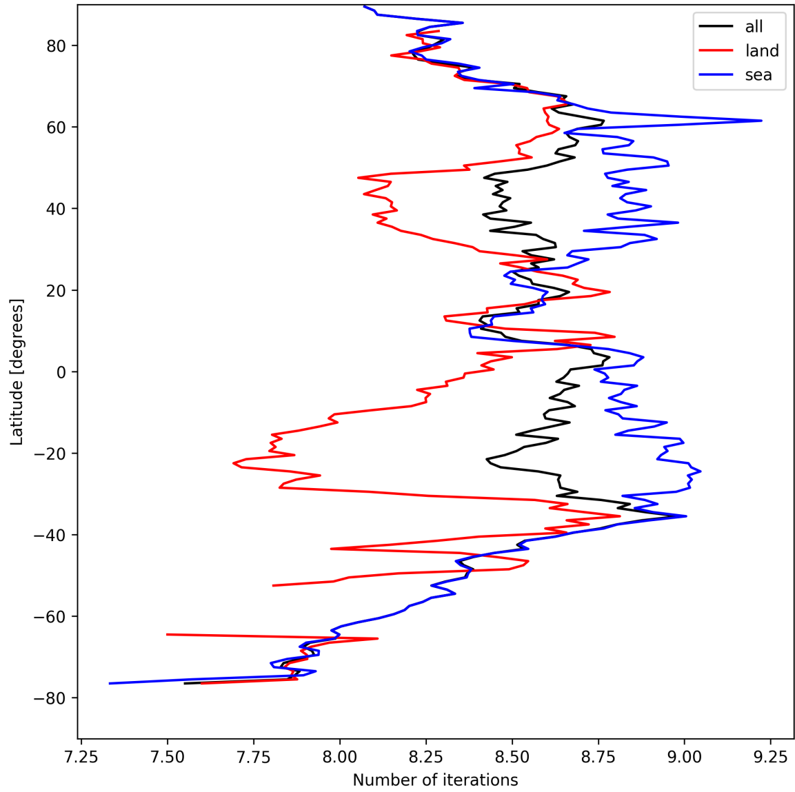
Figure 16: Zonal average of “Number of iterations” for 2025-08-30 to 2025-08-31.
