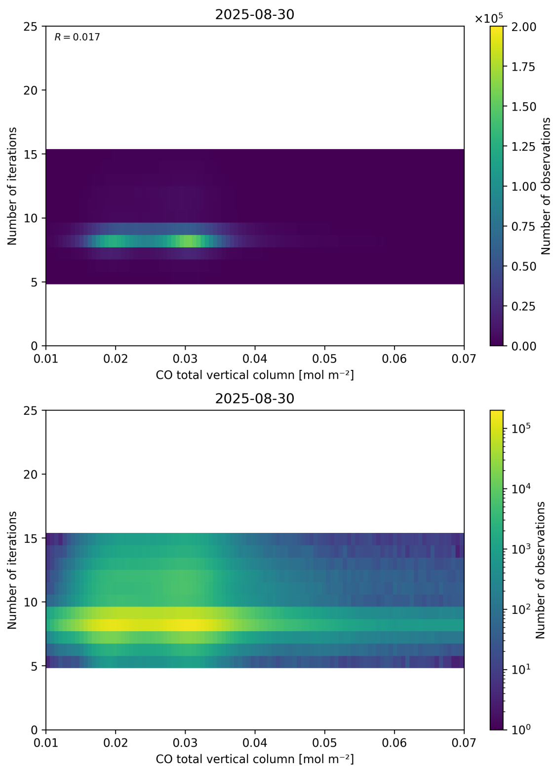
Figure 42: Scatter density plot of “CO total vertical column” against “Number of iterations” for 2025-08-30 to 2025-08-31.
