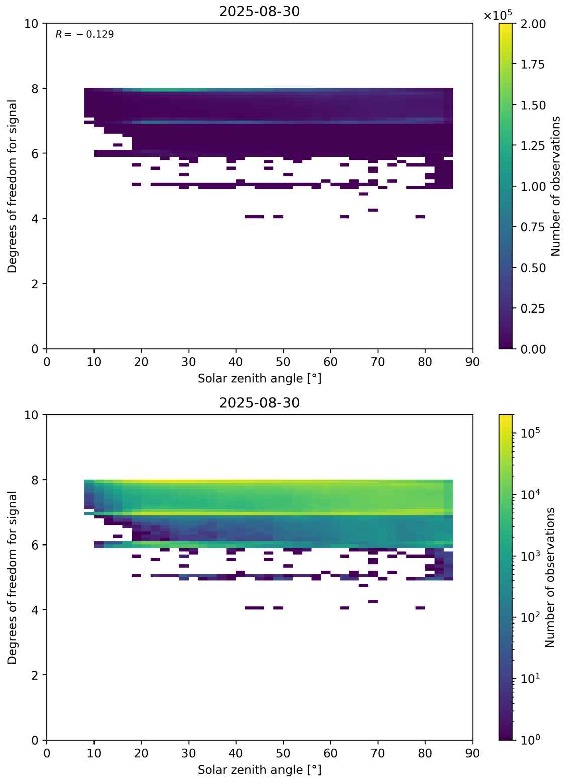
Figure 65: Scatter density plot of “Solar zenith angle” against “Degrees of freedom for signal” for 2025-08-30 to 2025-08-31.
