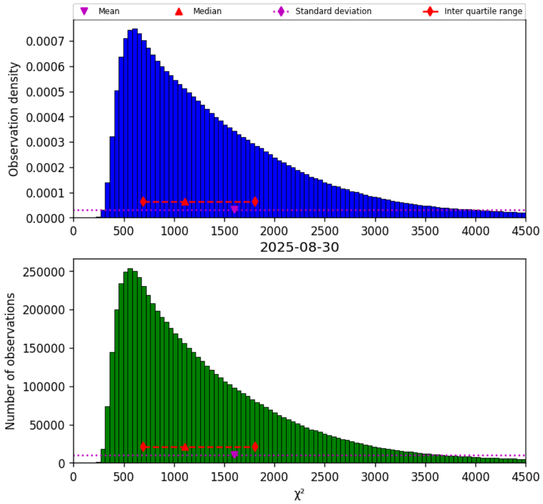
Figure 22: Histogram of " \chi^2 " for 2025-08-30 to 2025-08-31
