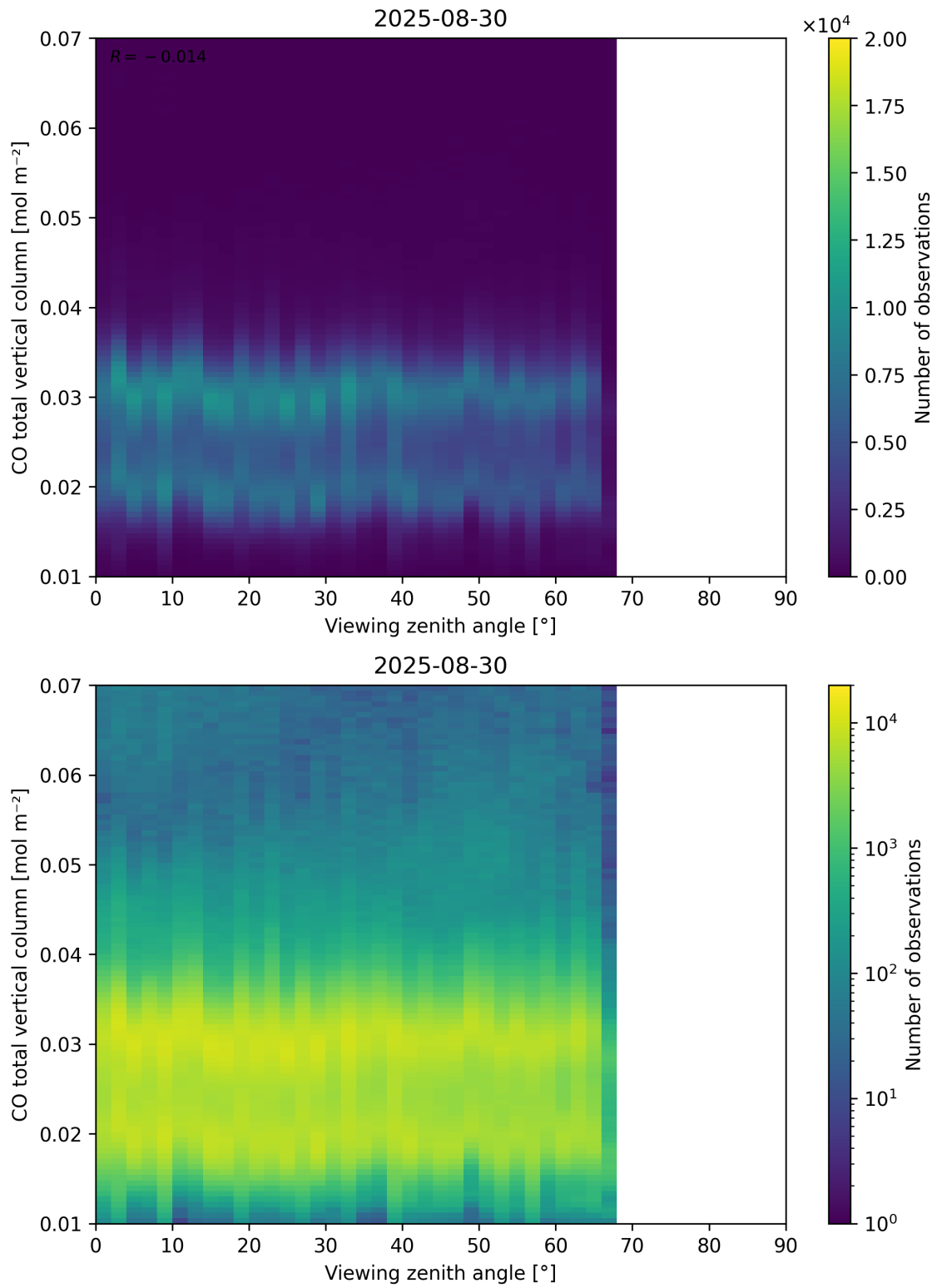
Figure 69: Scatter density plot of “Viewing zenith angle” against “CO total vertical column” for 2025-08-30 to 2025-08-31.
