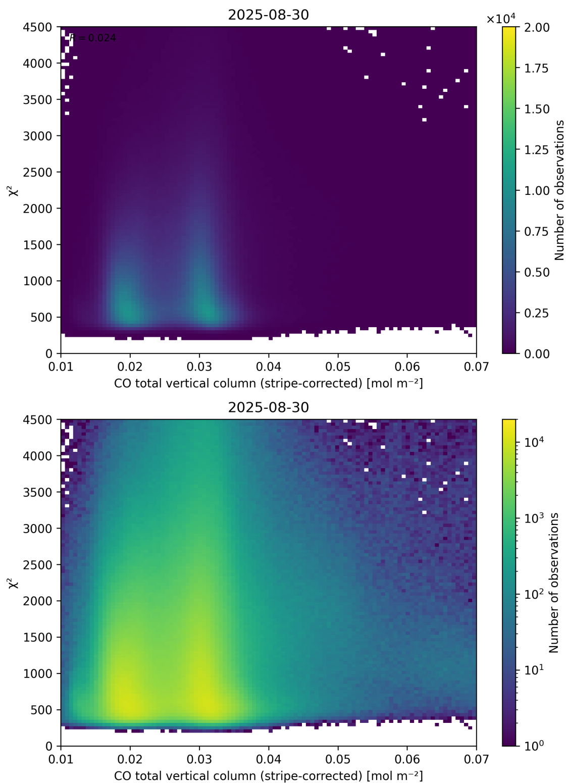
Figure 37: Scatter density plot of “CO total vertical column (stripe-corrected)” against “ \chi^2 ” for 2025-08-30 to 2025-08-31.
