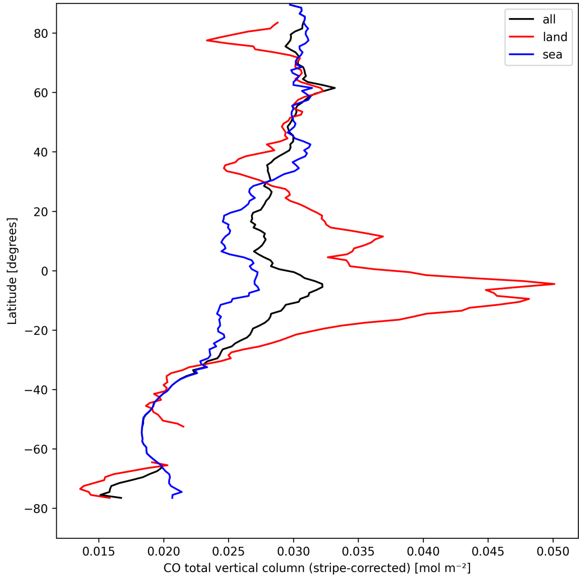
Figure 11: Zonal average of “CO total vertical column (stripe-corrected)” for 2025-08-30 to 2025-08-31.
