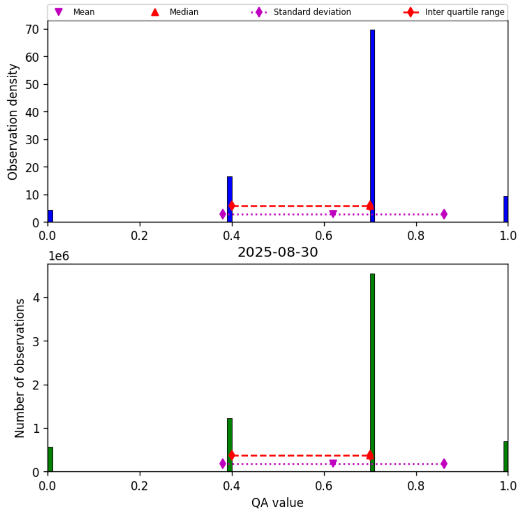
Figure 17: Histogram of “QA value” for 2025-08-30 to 2025-08-31
