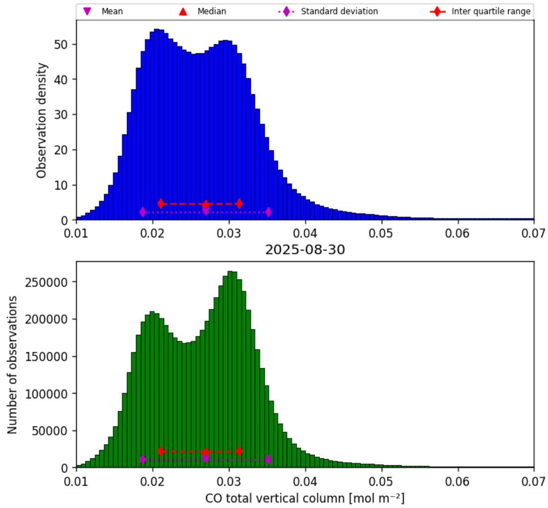
Figure 18: Histogram of “CO total vertical column” for 2025-08-30 to 2025-08-31
