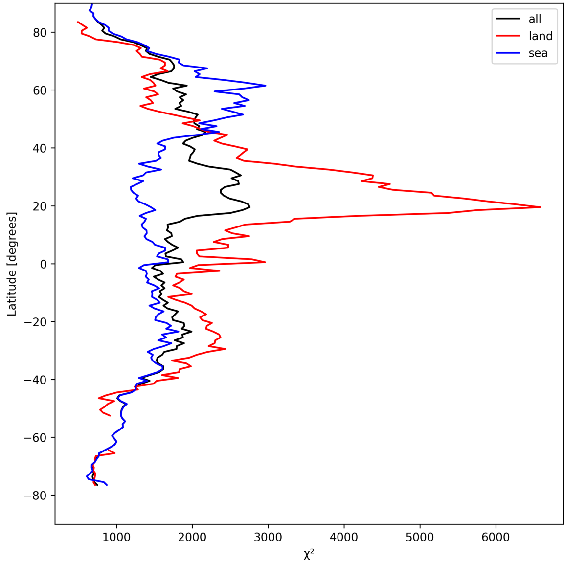
Figure 14: Zonal average of “ \chi^2 ” for 2025-08-30 to 2025-08-31.
