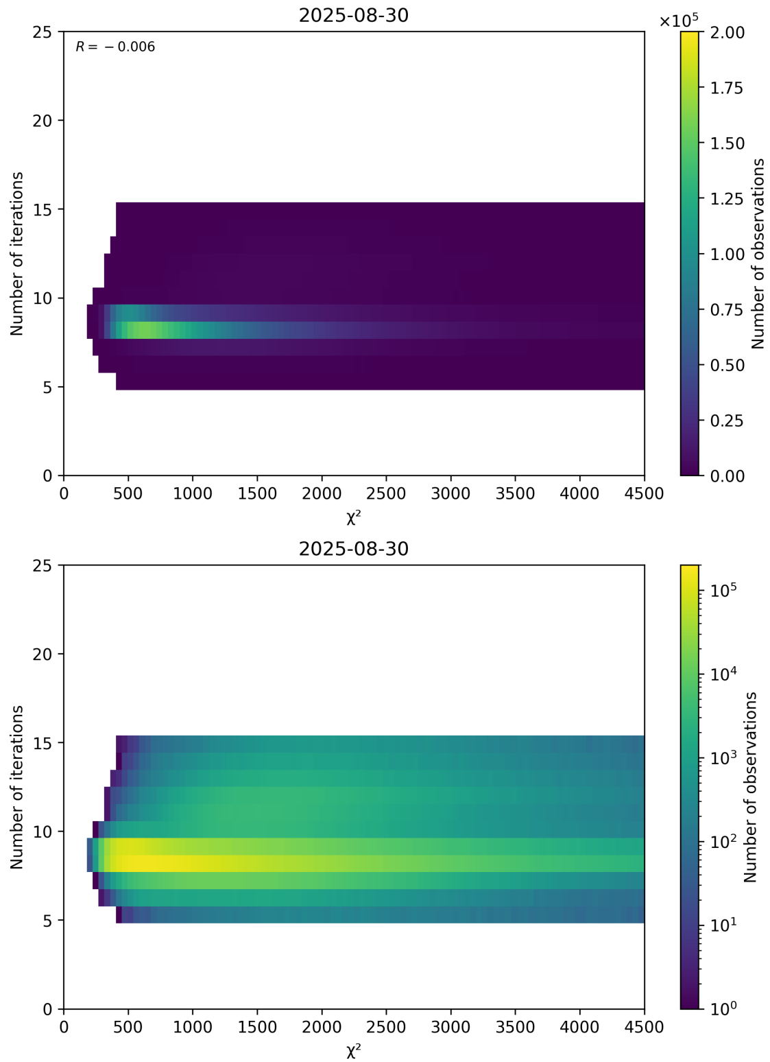
Figure 49: Scatter density plot of “ \chi^2 ” against “Number of iterations” for 2025-08-30 to 2025-08-31.
