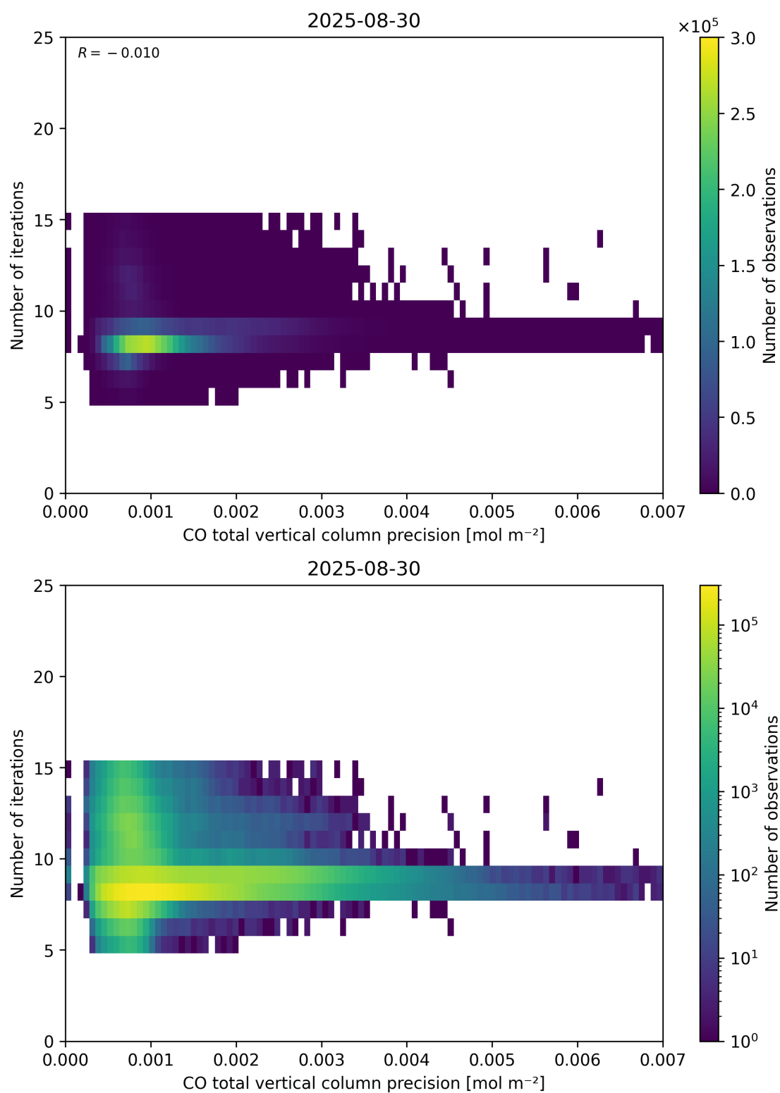
Figure 46: Scatter density plot of “CO total vertical column precision” against “Number of iterations” for 2025-08-30 to 2025-08-31.
