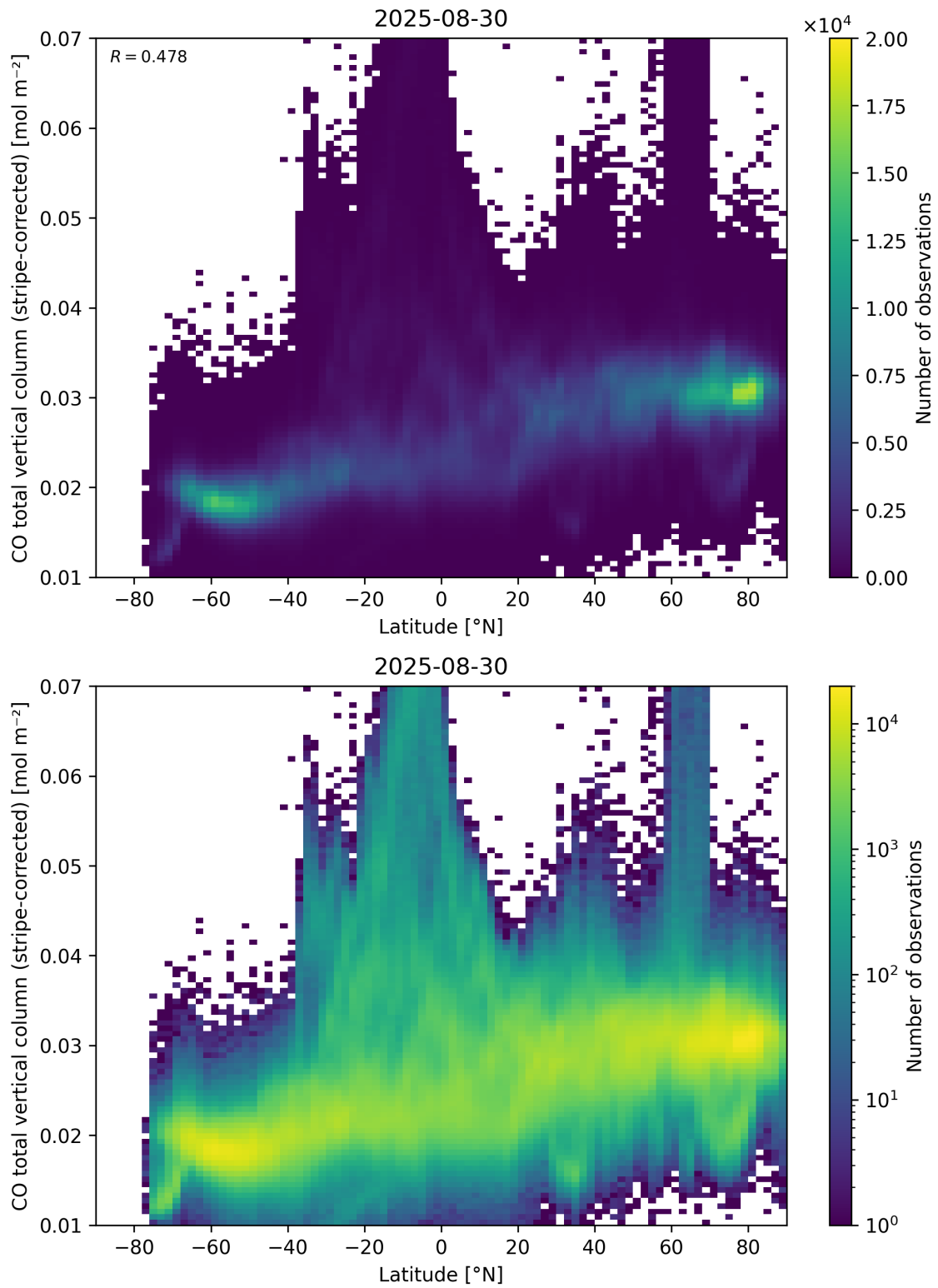
Figure 52: Scatter density plot of “Latitude” against “CO total vertical column (stripe-corrected)” for 2025-08-30 to 2025-08-31.
