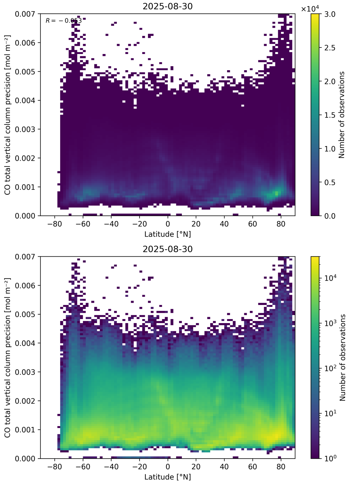
Figure 53: Scatter density plot of “Latitude” against “CO total vertical column precision” for 2025-08-30 to 2025-08-31.
