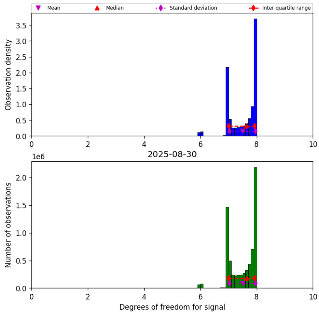
Figure 23: Histogram of “Degrees of freedom for signal” for 2025-08-30 to 2025-08-31
