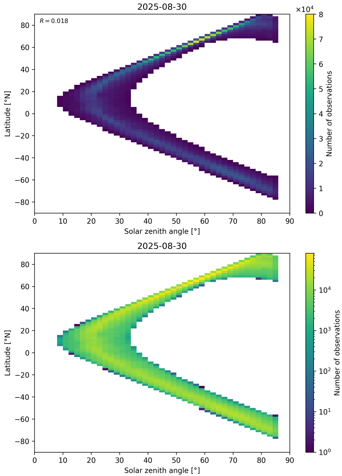
Figure 66: Scatter density plot of “Solar zenith angle” against “Latitude” for 2025-08-30 to 2025-08-31.
