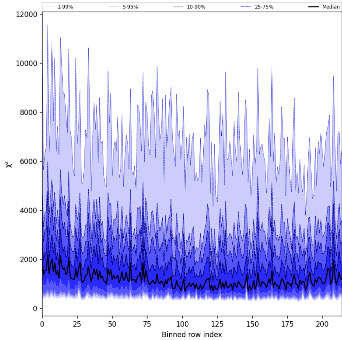
Figure 30: Along track statistics of “ \chi^2 ” for 2025-08-30 to 2025-08-31
