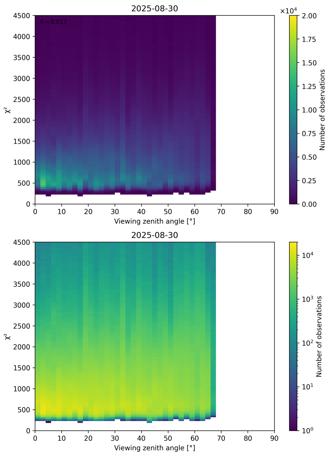
Figure 72: Scatter density plot of “Viewing zenith angle” against “ \chi^2 ” for 2025-08-30 to 2025-08-31.
