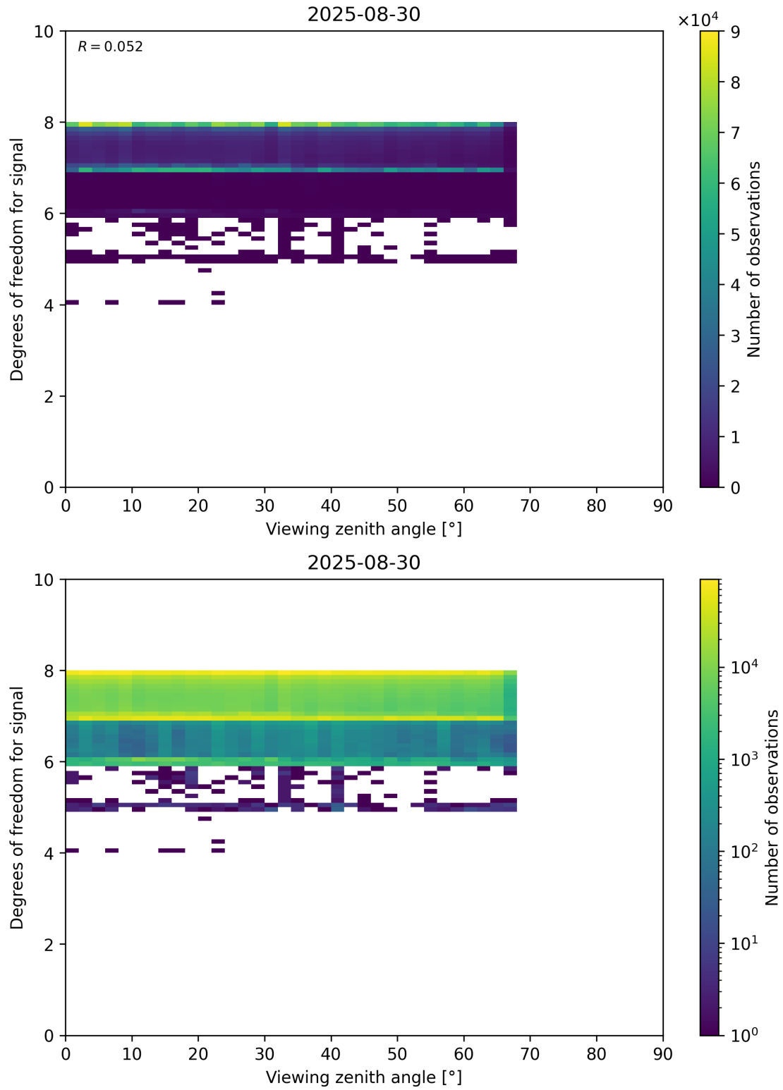
Figure 73: Scatter density plot of “Viewing zenith angle” against “Degrees of freedom for signal” for 2025-08-30 to 2025-08-31.
