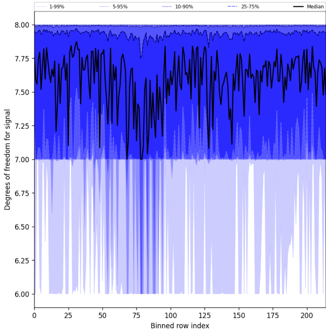
Figure 31: Along track statistics of “Degrees of freedom for signal” for 2025-08-30 to 2025-08-31
