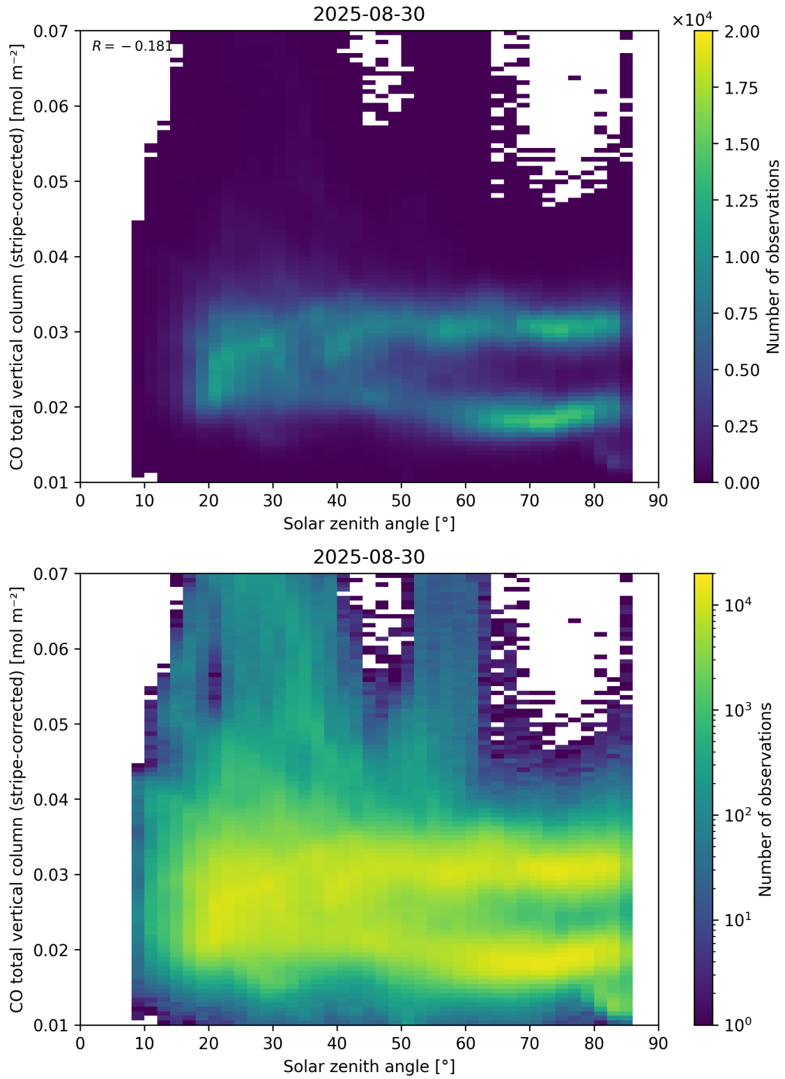
Figure 62: Scatter density plot of “Solar zenith angle” against “CO total vertical column (stripe-corrected)” for 2025-08-30 to 2025-08-31.
