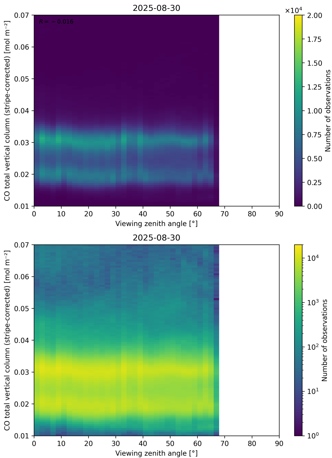
Figure 70: Scatter density plot of “Viewing zenith angle” against “CO total vertical column (stripe-corrected)” for 2025-08-30 to 2025-08-31.
