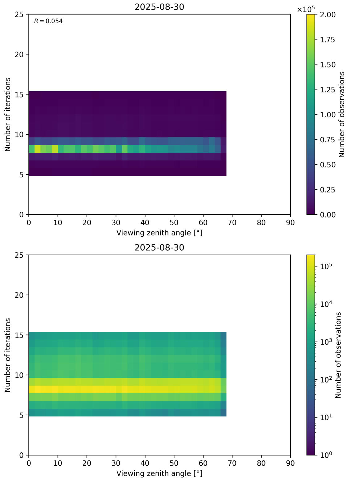
Figure 75: Scatter density plot of “Viewing zenith angle” against “Number of iterations” for 2025-08-30 to 2025-08-31.
