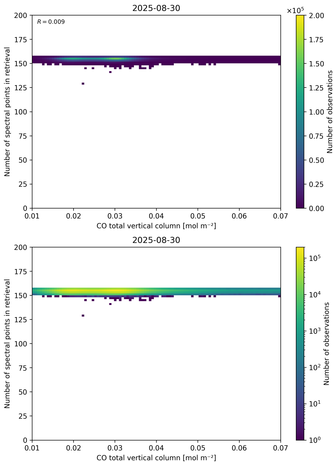
Figure 43: Scatter density plot of “CO total vertical column” against “Number of spectral points in retrieval” for 2025-08-30 to 2025-08-31.
