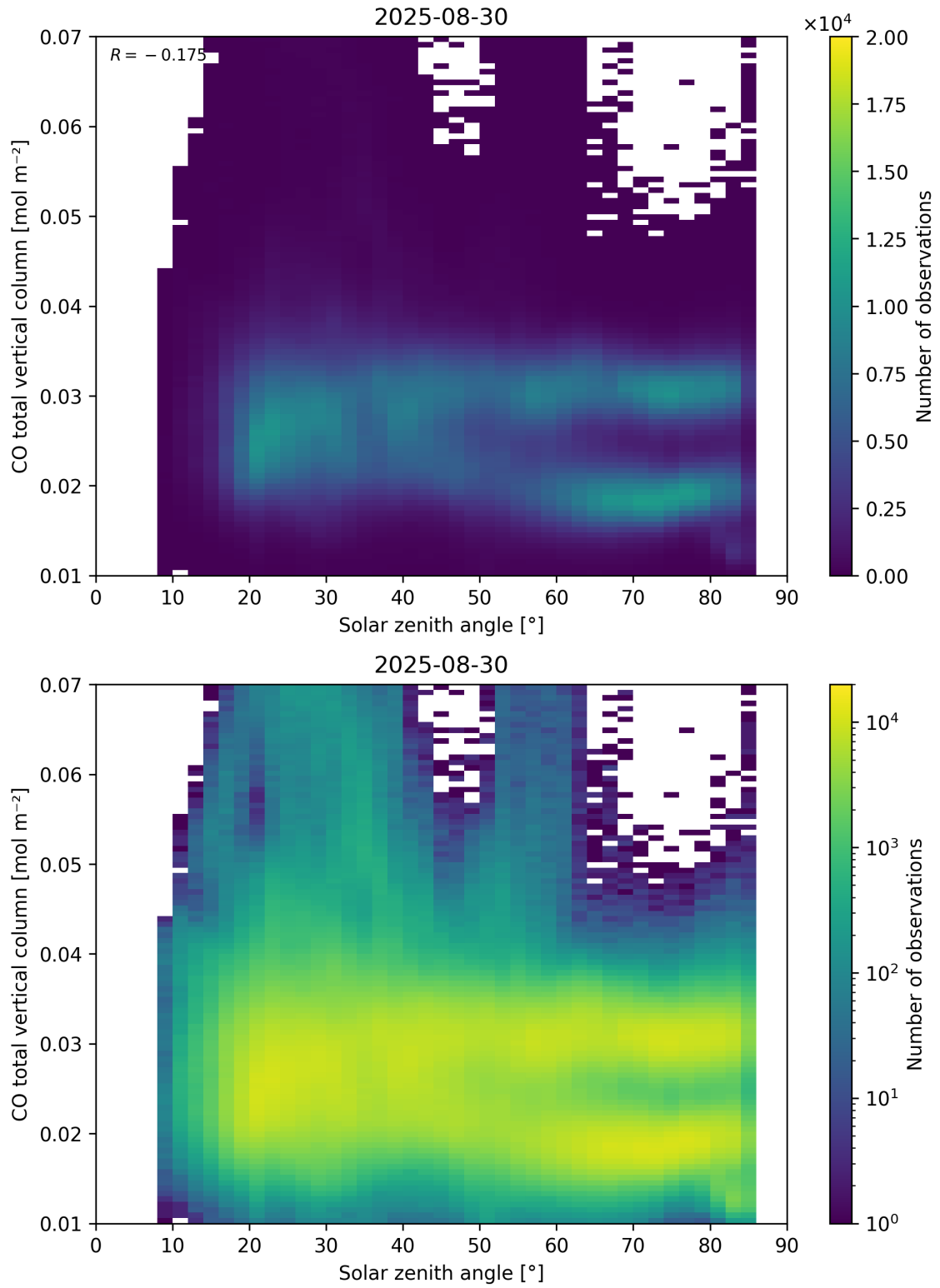
Figure 61: Scatter density plot of “Solar zenith angle” against “CO total vertical column” for 2025-08-30 to 2025-08-31.
