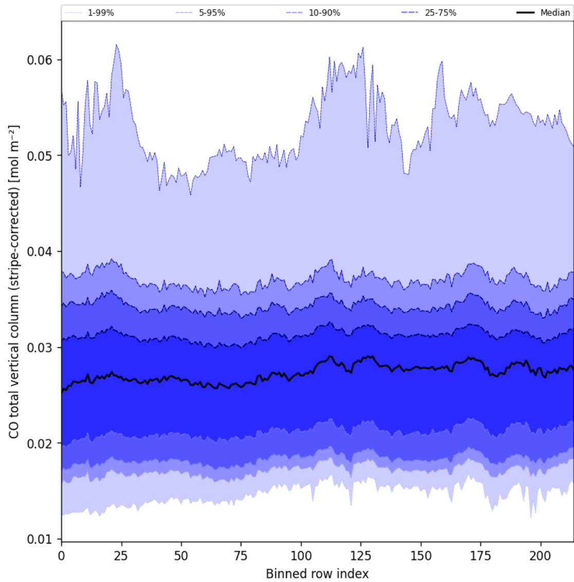
Figure 27: Along track statistics of “CO total vertical column (stripe-corrected)” for 2025-08-30 to 2025-08-31
