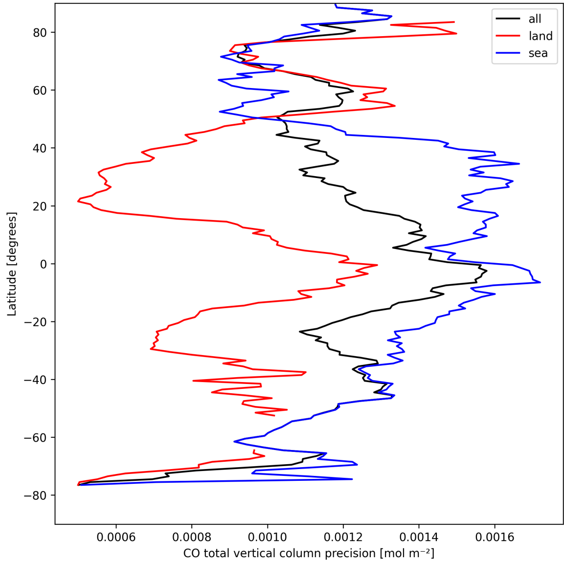
Figure 12: Zonal average of “CO total vertical column precision” for 2025-08-30 to 2025-08-31.
