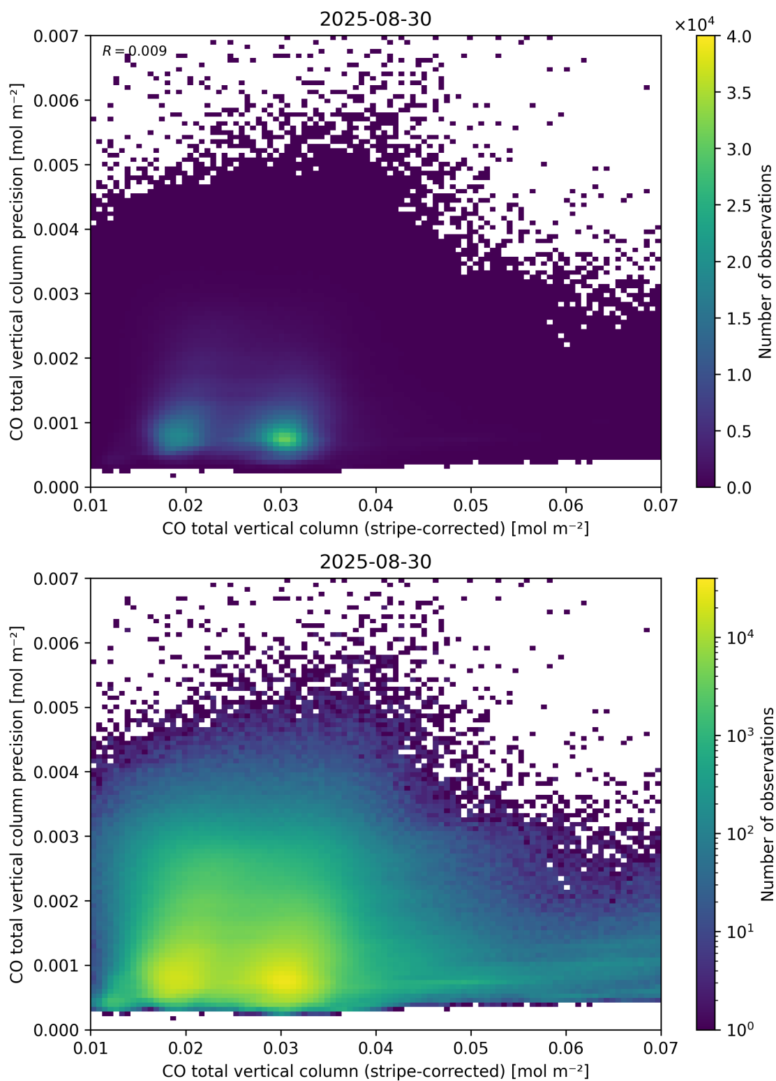
Figure 36: Scatter density plot of “CO total vertical column (stripe-corrected)” against “CO total vertical column precision” for 2025-08-30 to 2025-08-31.
