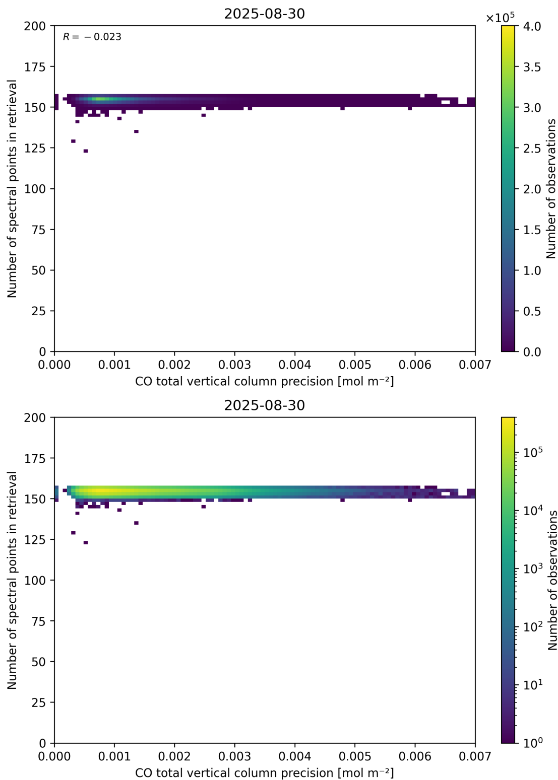
Figure 47: Scatter density plot of “CO total vertical column precision” against “Number of spectral points in retrieval” for 2025-08-30 to 2025-08-31.
