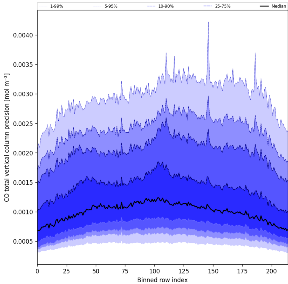
Figure 28: Along track statistics of “CO total vertical column precision” for 2025-08-30 to 2025-08-31
