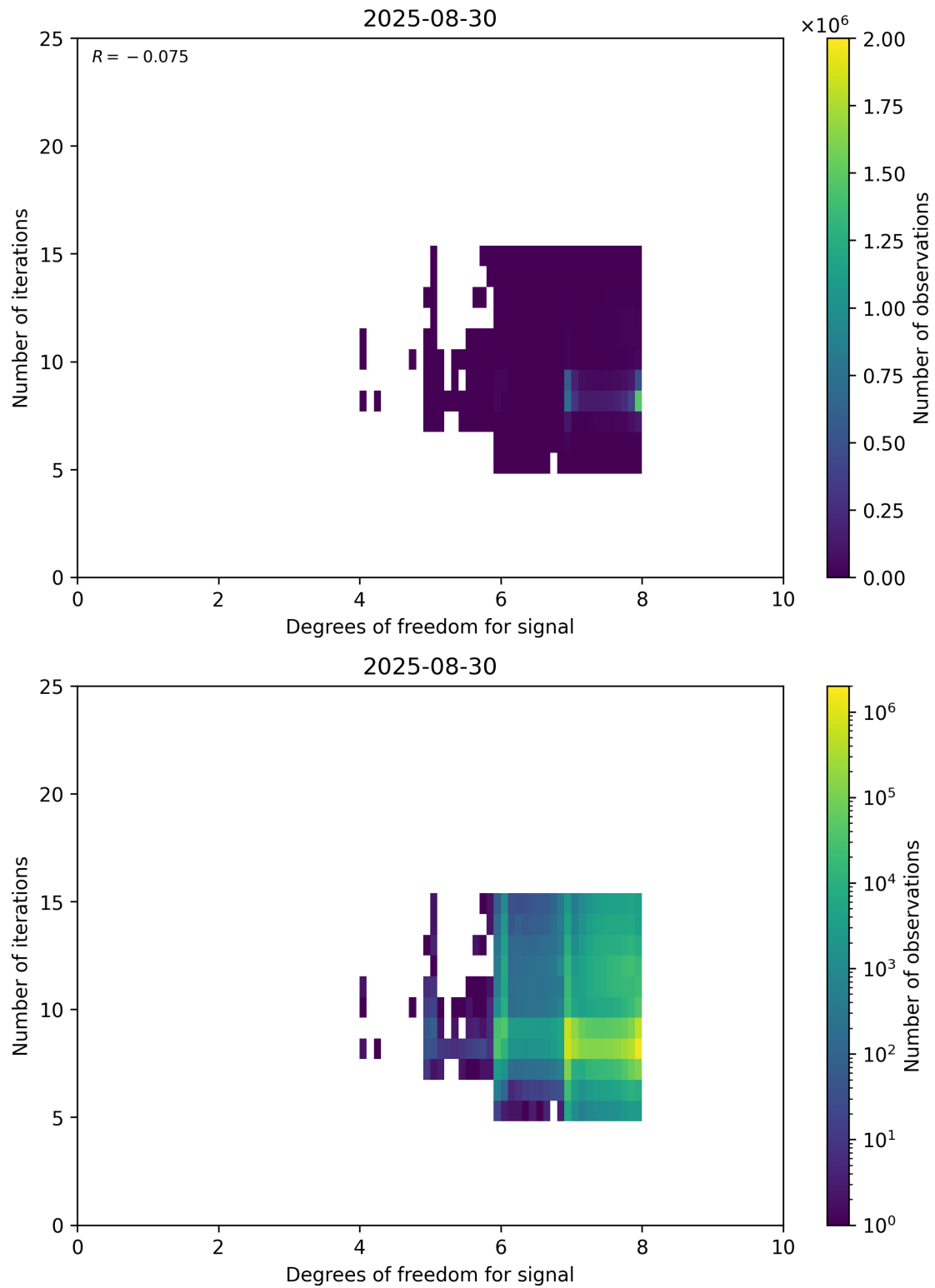
Figure 50: Scatter density plot of “Degrees of freedom for signal” against “Number of iterations” for 2025-08-30 to 2025-08-31.
