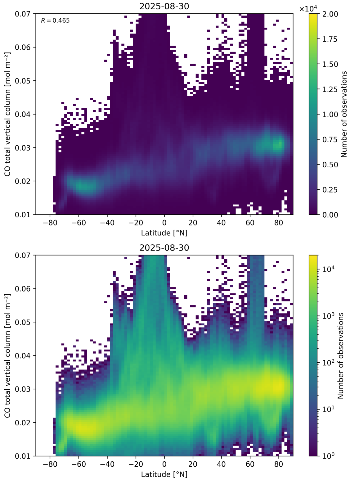
Figure 51: Scatter density plot of “Latitude” against “CO total vertical column” for 2025-08-30 to 2025-08-31.
