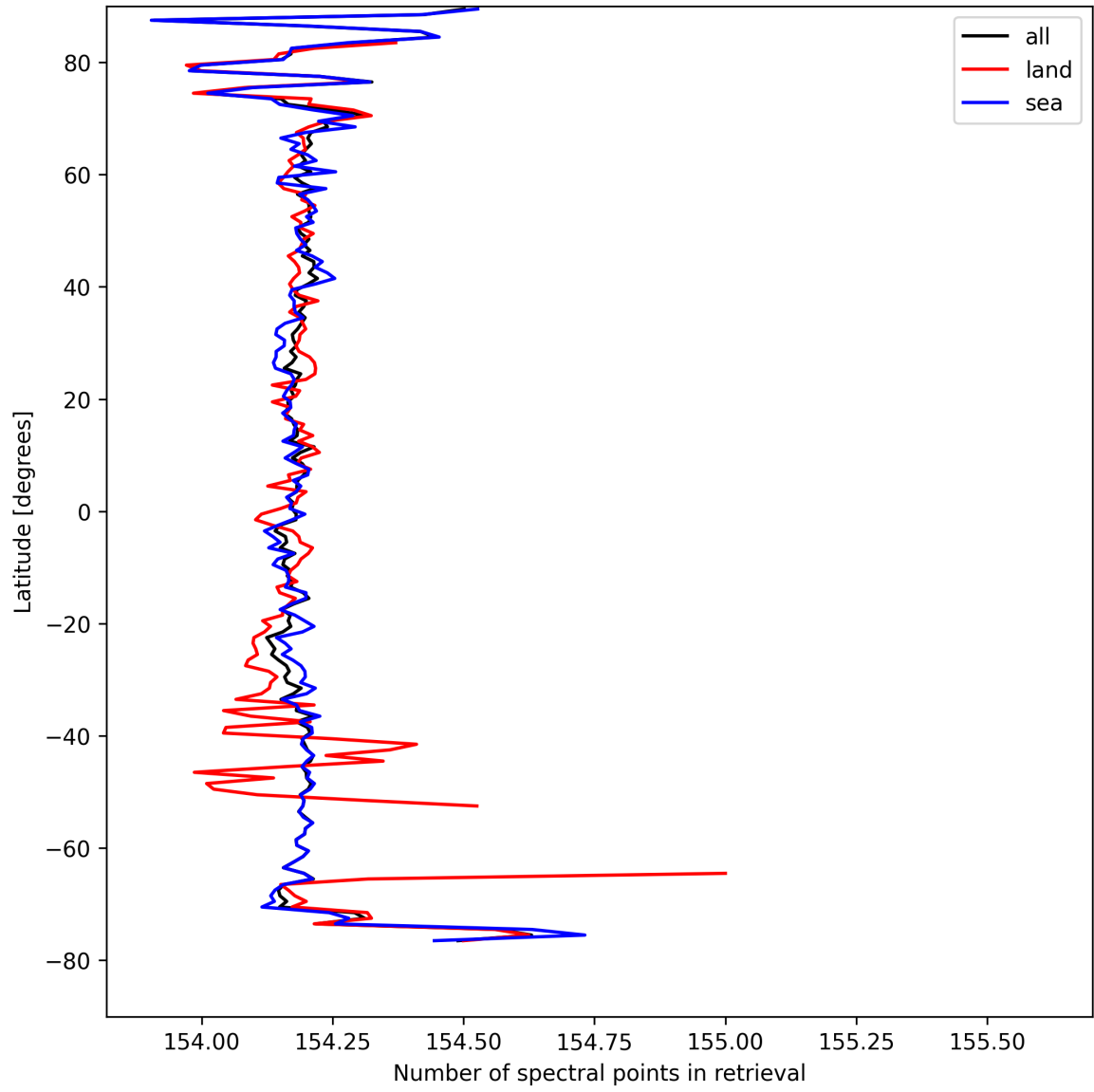
Figure 13: Zonal average of “Number of spectral points in retrieval” for 2025-08-30 to 2025-08-31.
