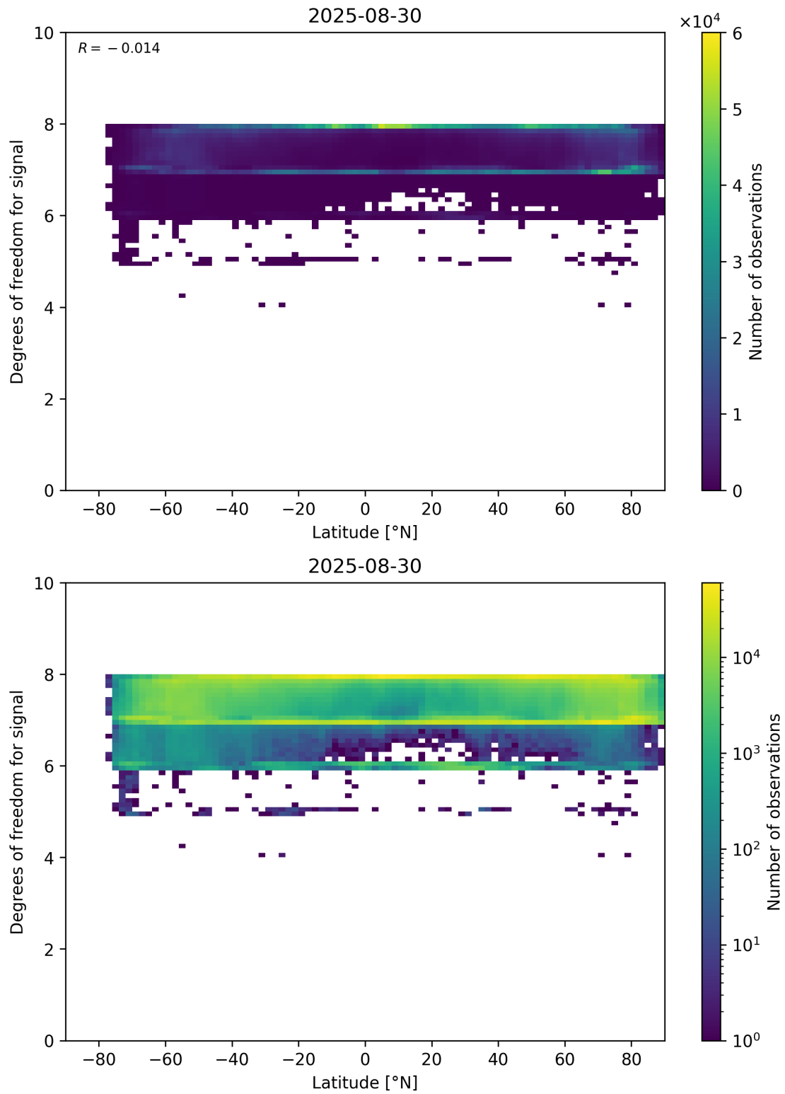
Figure 55: Scatter density plot of “Latitude” against “Degrees of freedom for signal” for 2025-08-30 to 2025-08-31.
