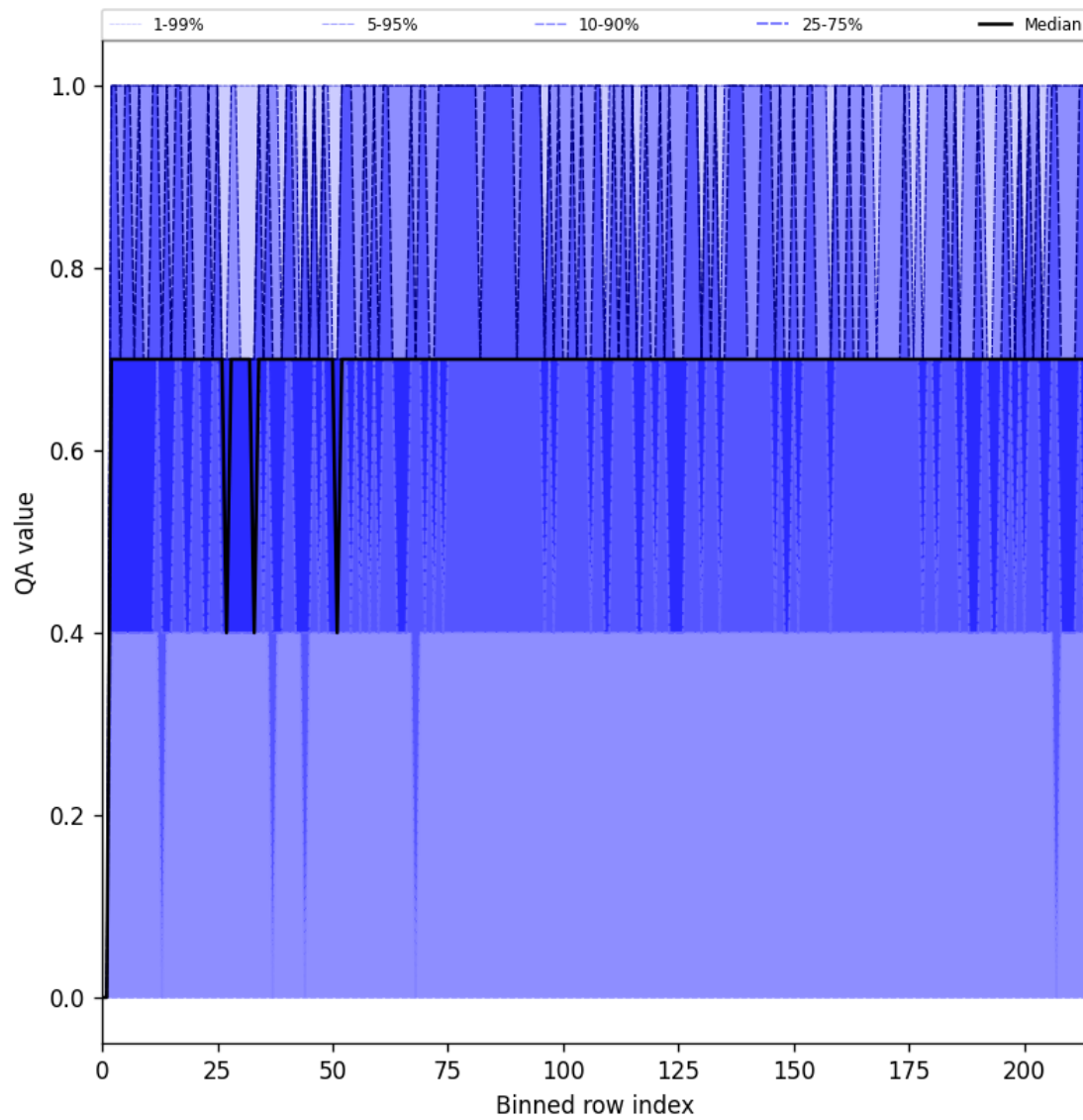
Figure 25: Along track statistics of “QA value” for 2025-08-30 to 2025-08-31
