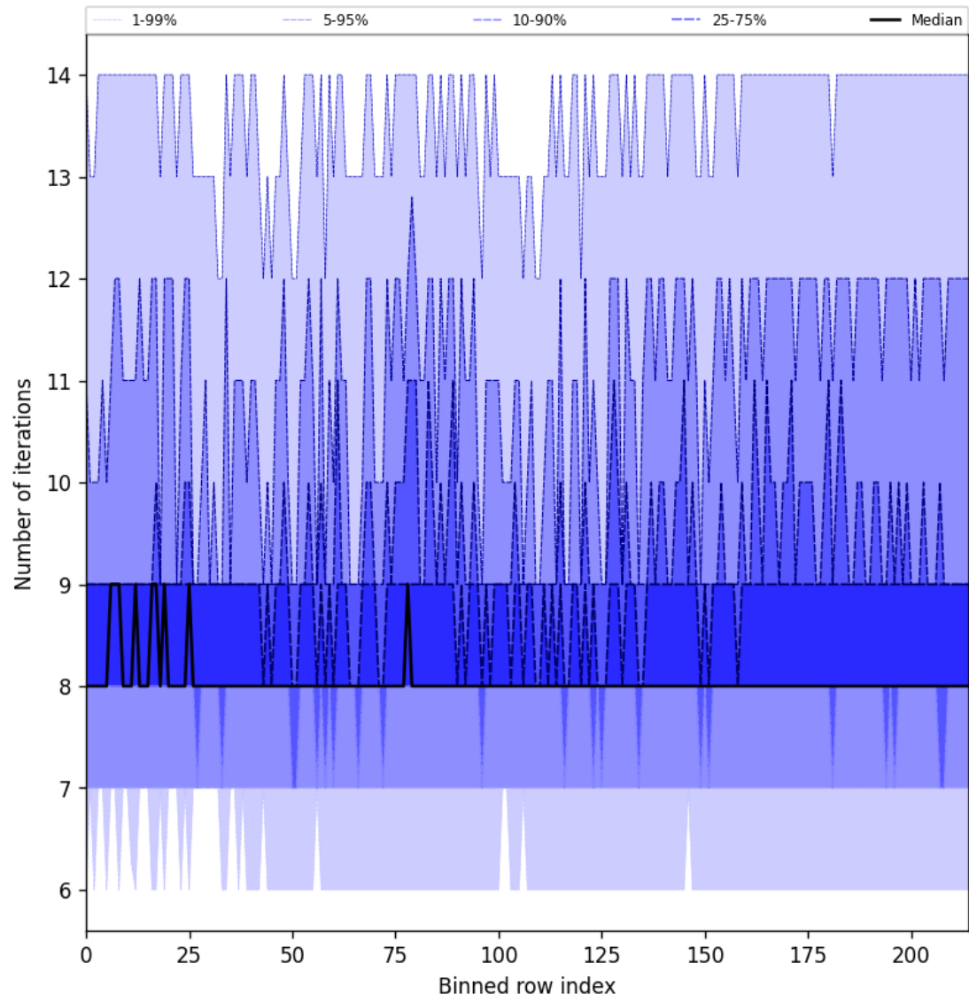
Figure 32: Along track statistics of “Number of iterations” for 2025-08-30 to 2025-08-31
