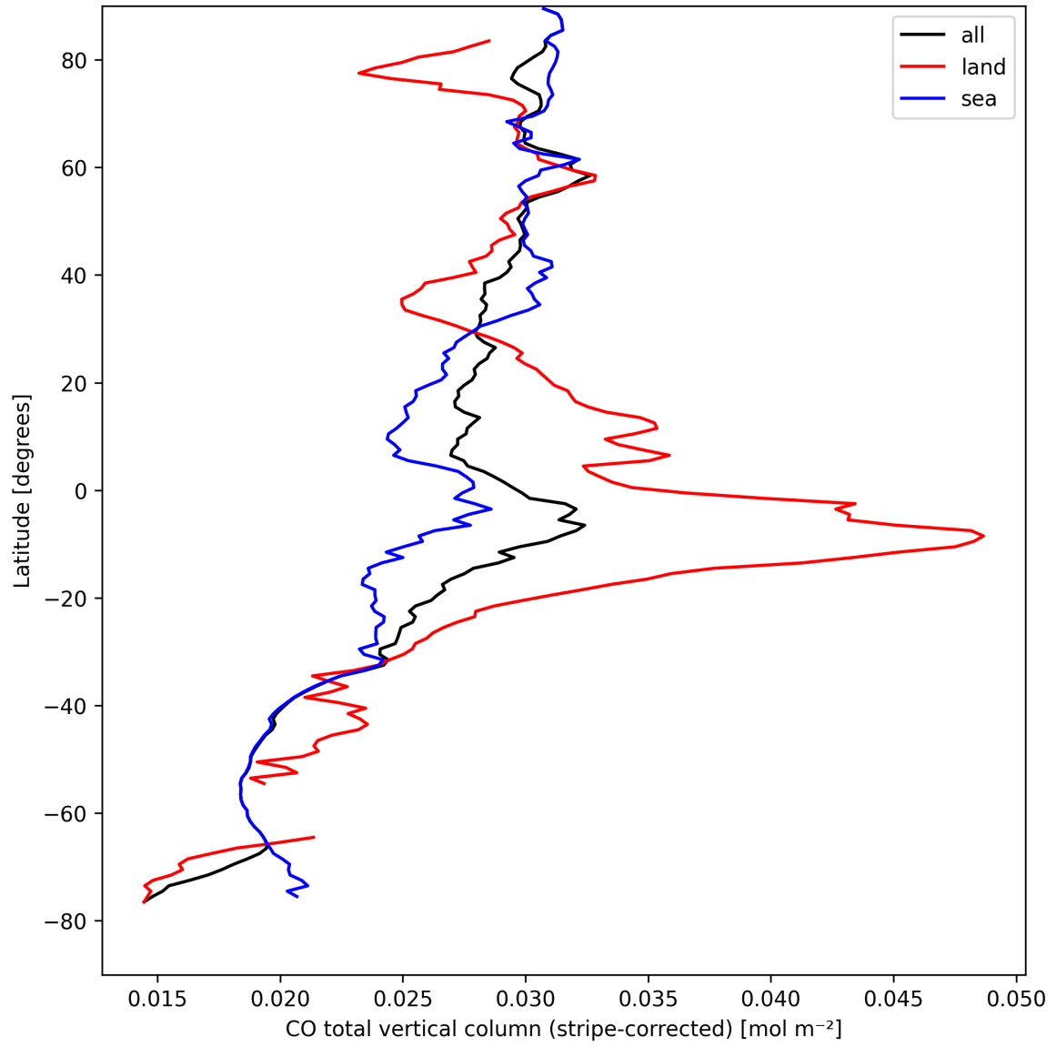
Figure 11: Zonal average of “CO total vertical column (stripe-corrected)” for 2025-08-30 to 2025-09-01.
