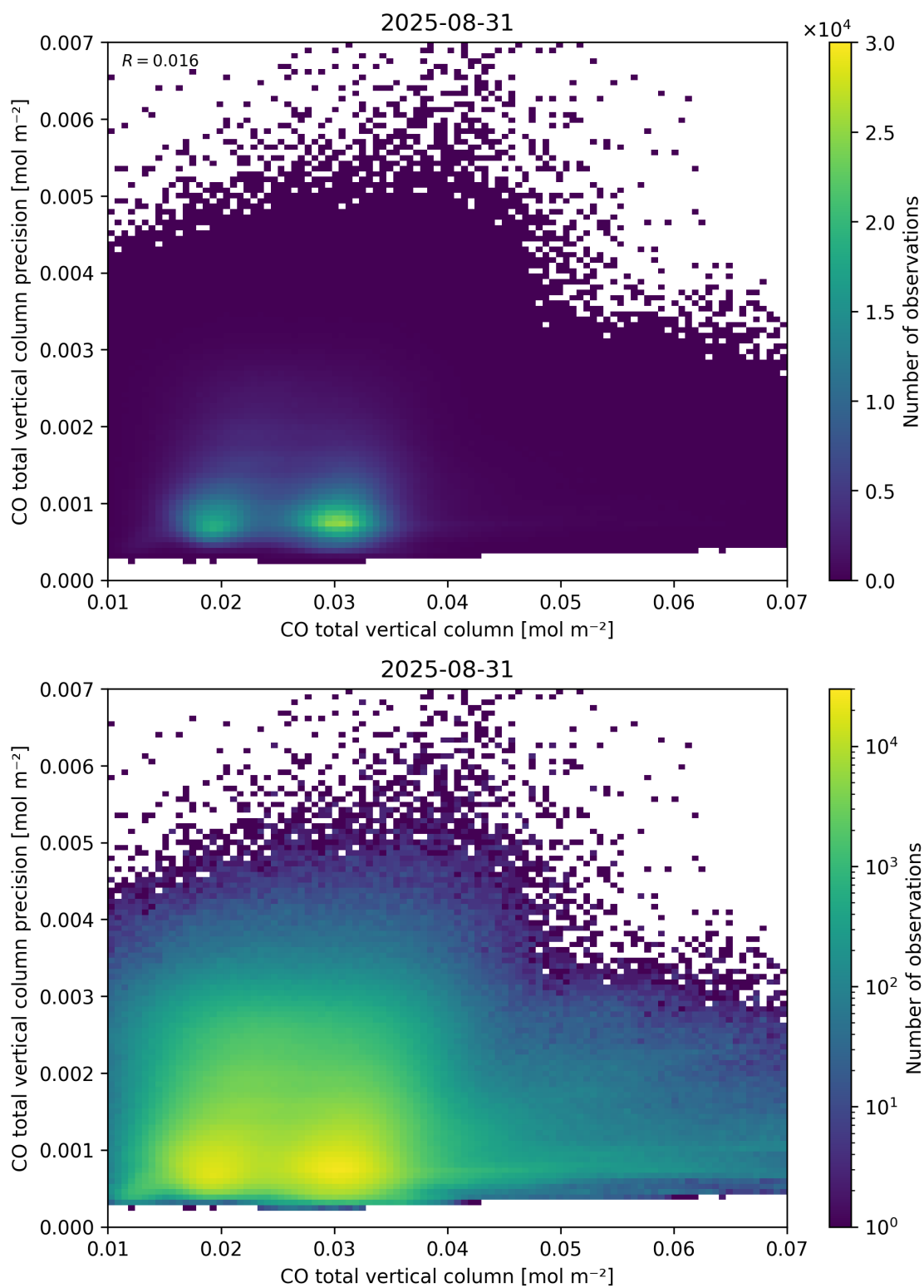
Figure 34: Scatter density plot of “CO total vertical column” against “CO total vertical column precision” for 2025-08-30 to 2025-09-01.
