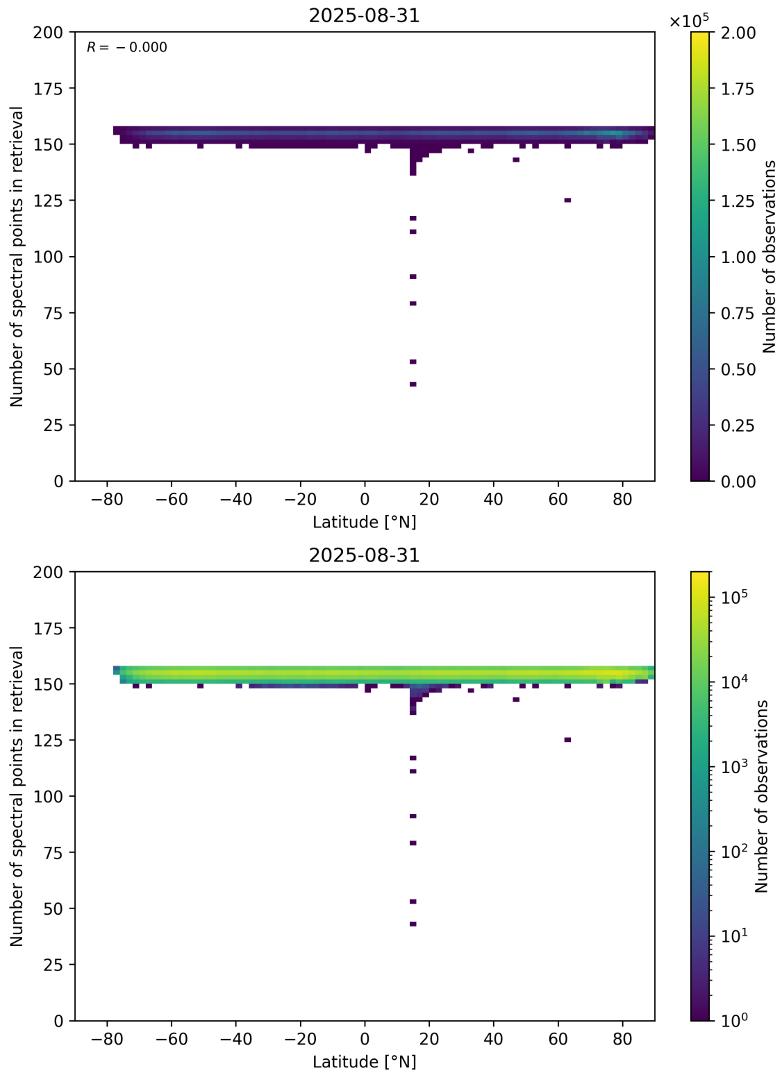
Figure 57: Scatter density plot of “Latitude” against “Number of spectral points in retrieval” for 2025-08-30 to 2025-09-01.
