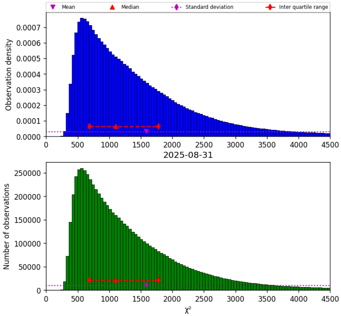
Figure 22: Histogram of " \chi^2 " for 2025-08-30 to 2025-09-01
