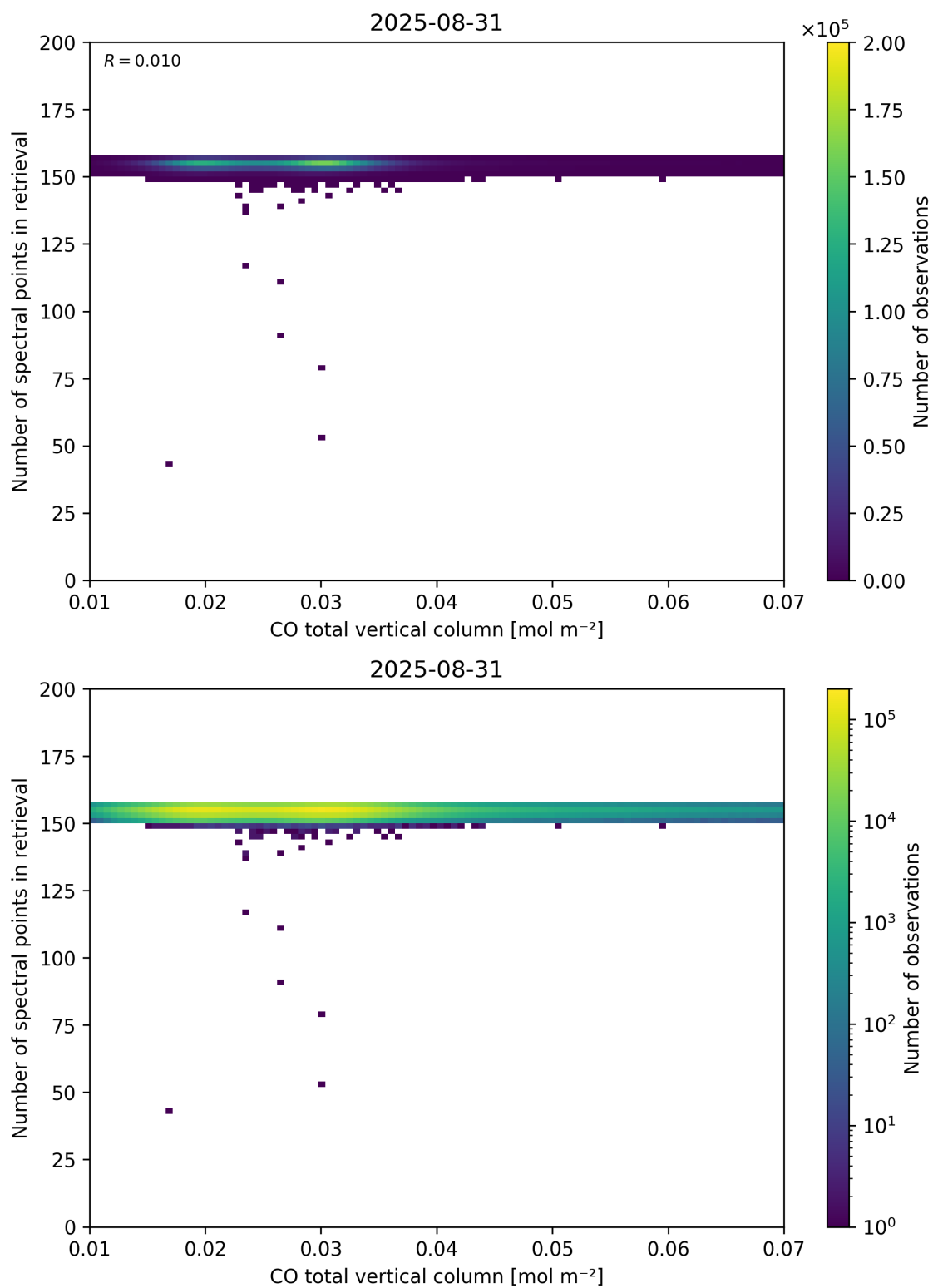
Figure 43: Scatter density plot of “CO total vertical column” against “Number of spectral points in retrieval” for 2025-08-30 to 2025-09-01.
