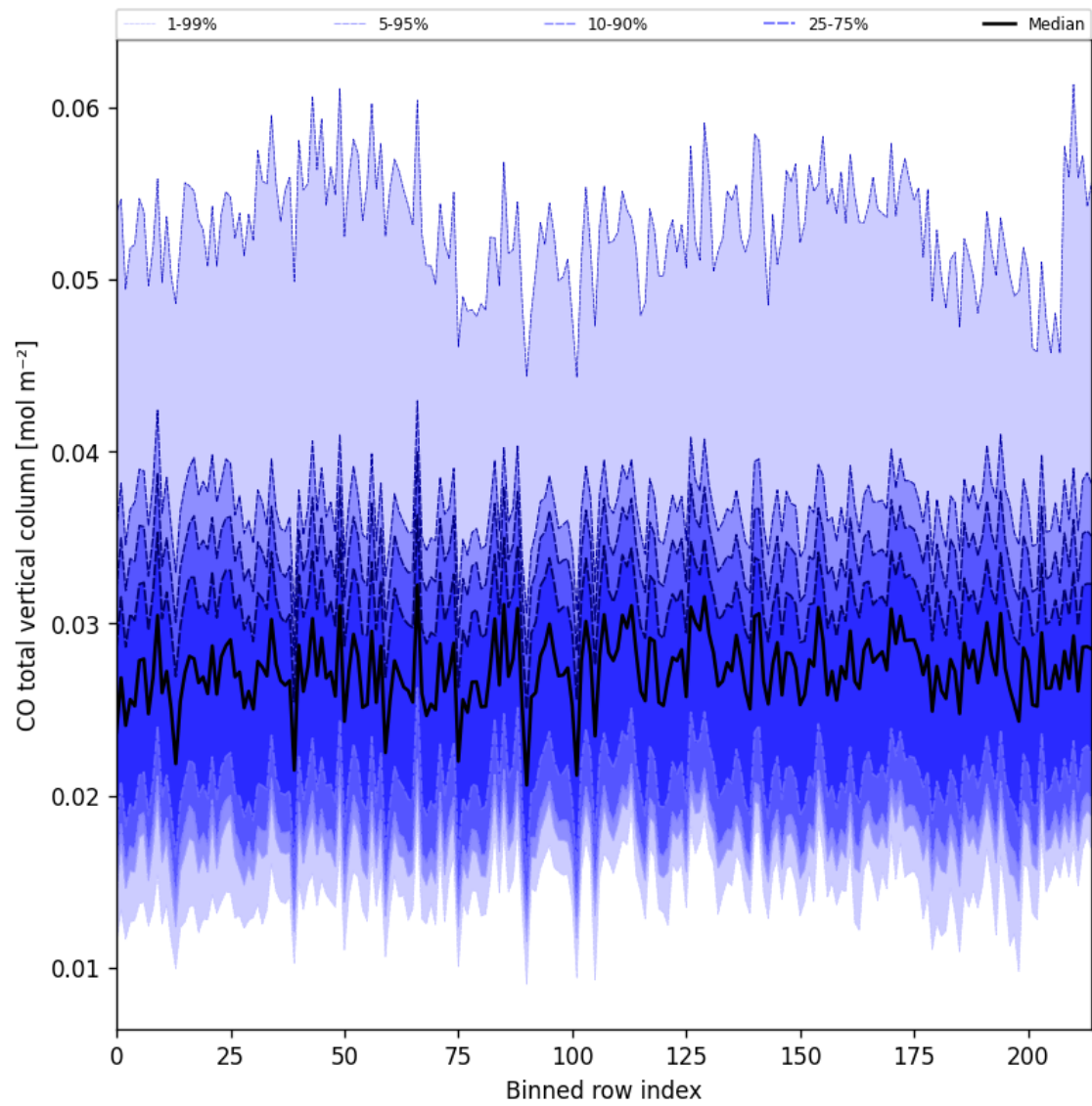
Figure 26: Along track statistics of “CO total vertical column” for 2025-08-30 to 2025-09-01
