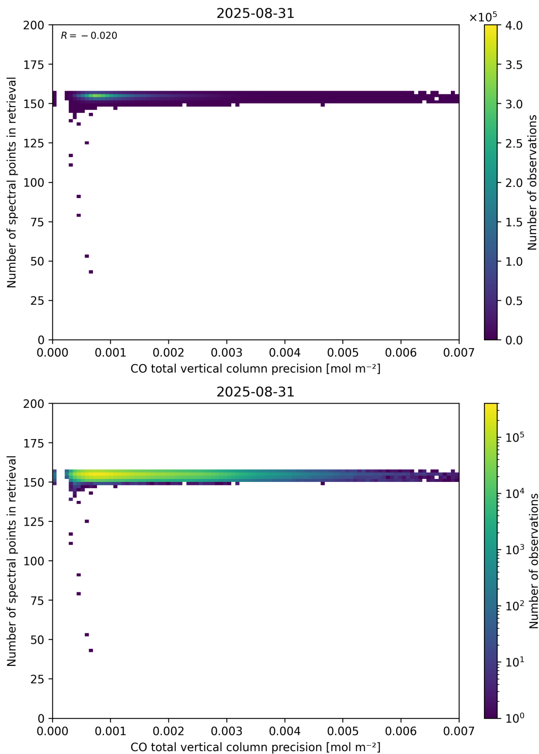
Figure 47: Scatter density plot of “CO total vertical column precision” against “Number of spectral points in retrieval” for 2025-08-30 to 2025-09-01.
