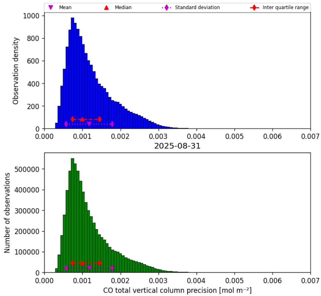
Figure 20: Histogram of “CO total vertical column precision” for 2025-08-30 to 2025-09-01
