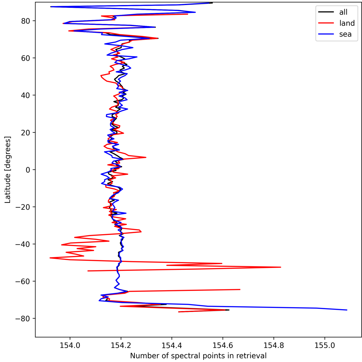
Figure 13: Zonal average of “Number of spectral points in retrieval” for 2025-08-30 to 2025-09-01.
