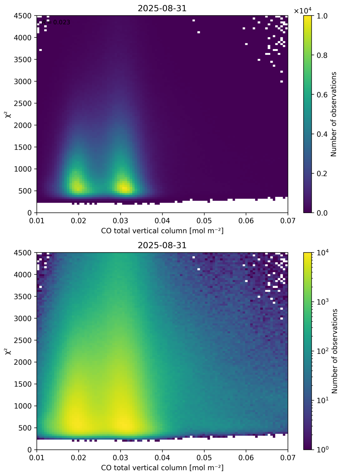
Figure 35: Scatter density plot of “CO total vertical column” against “ \chi^2 ” for 2025-08-30 to 2025-09-01.
