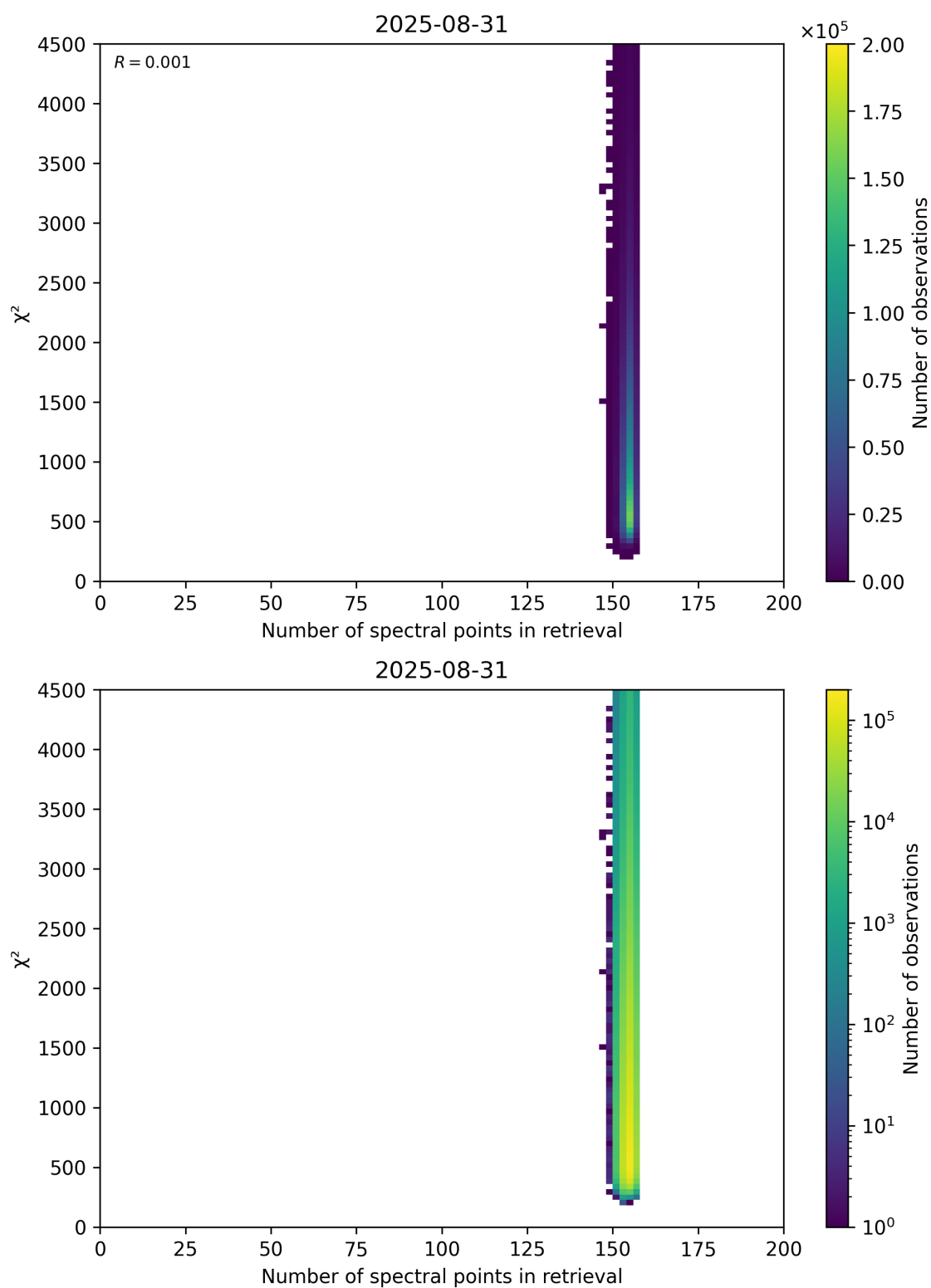
Figure 58: Scatter density plot of “Number of spectral points in retrieval” against “ \chi^2 ” for 2025-08-30 to 2025-09-01.
