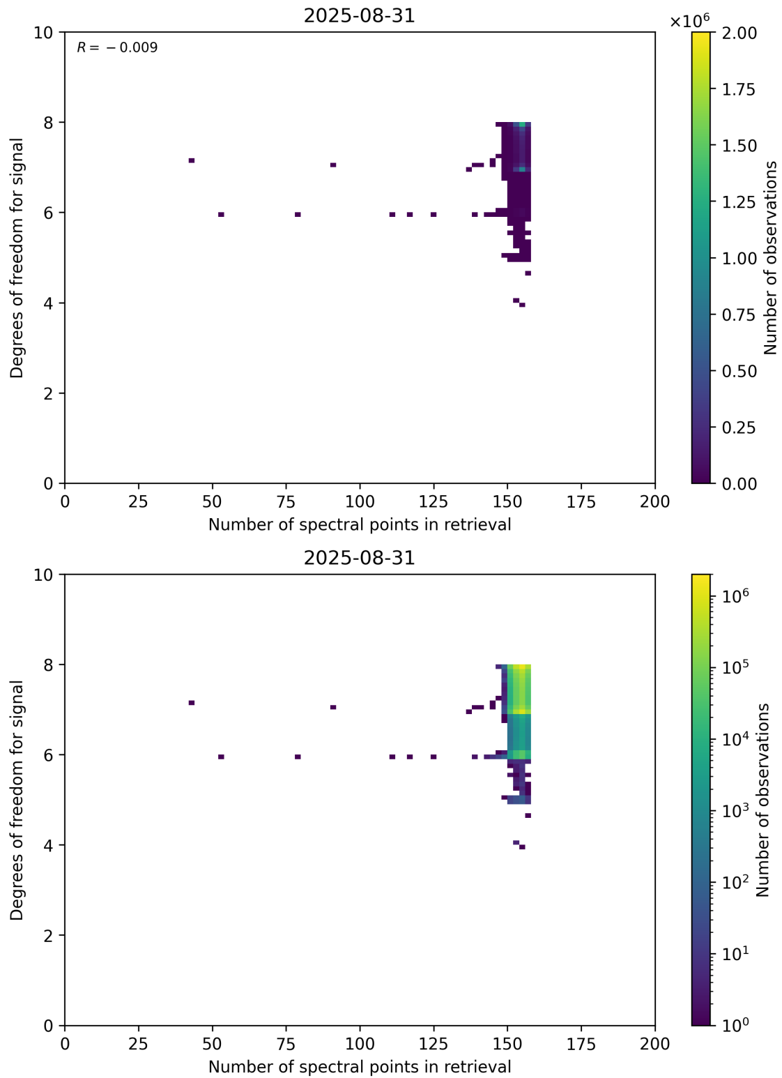
Figure 59: Scatter density plot of “Number of spectral points in retrieval” against “Degrees of freedom for signal” for 2025-08-30 to 2025-09-01.
