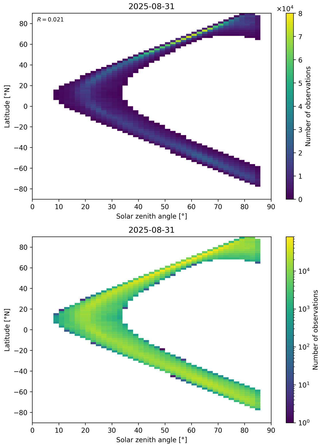
Figure 66: Scatter density plot of “Solar zenith angle” against “Latitude” for 2025-08-30 to 2025-09-01.
