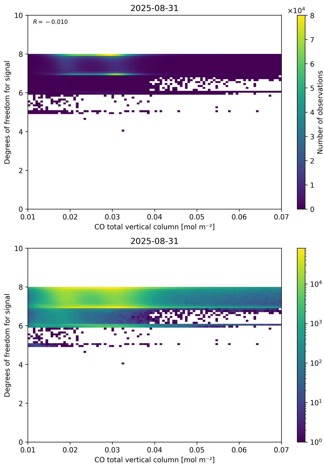
Figure 41: Scatter density plot of “CO total vertical column” against “Degrees of freedom for signal” for 2025-08-30 to 2025-09-01.
