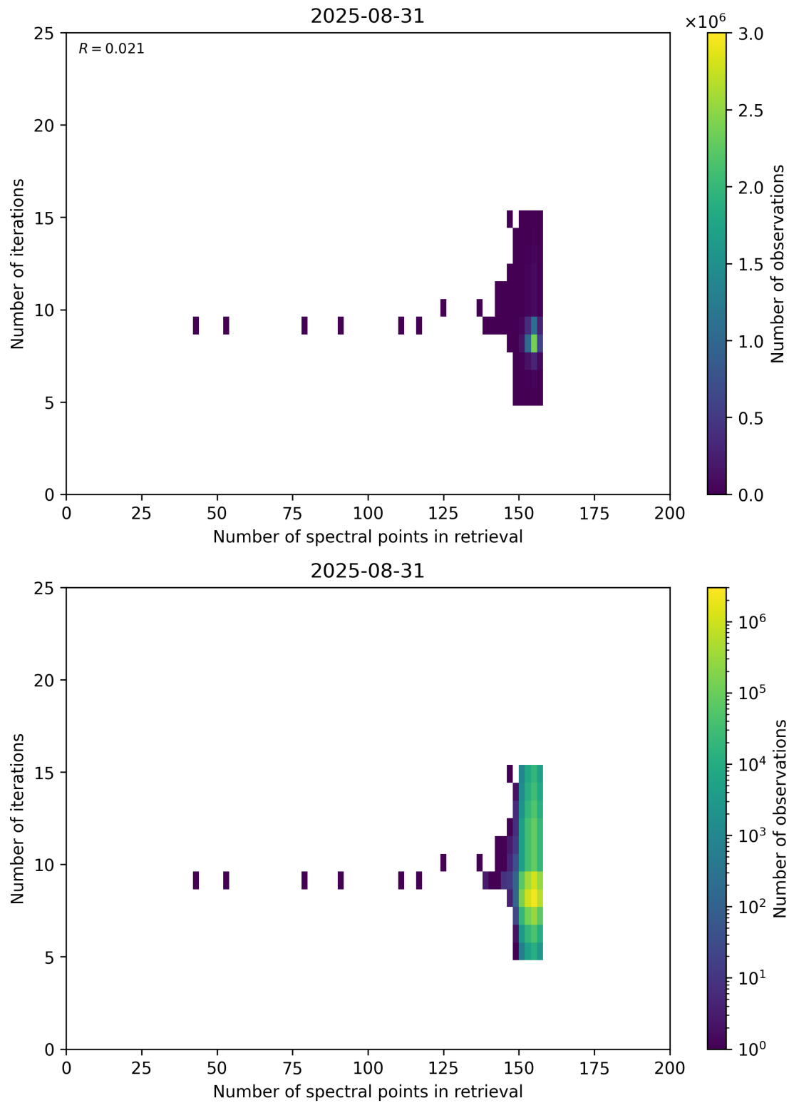
Figure 60: Scatter density plot of “Number of spectral points in retrieval” against “Number of iterations” for 2025-08-30 to 2025-09-01.
