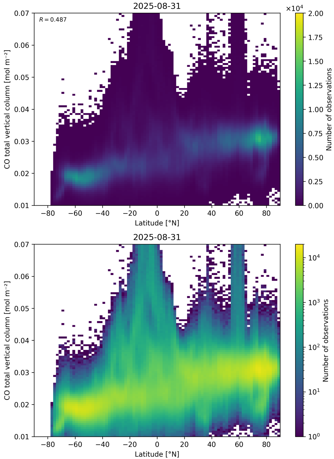
Figure 51: Scatter density plot of “Latitude” against “CO total vertical column” for 2025-08-30 to 2025-09-01.
