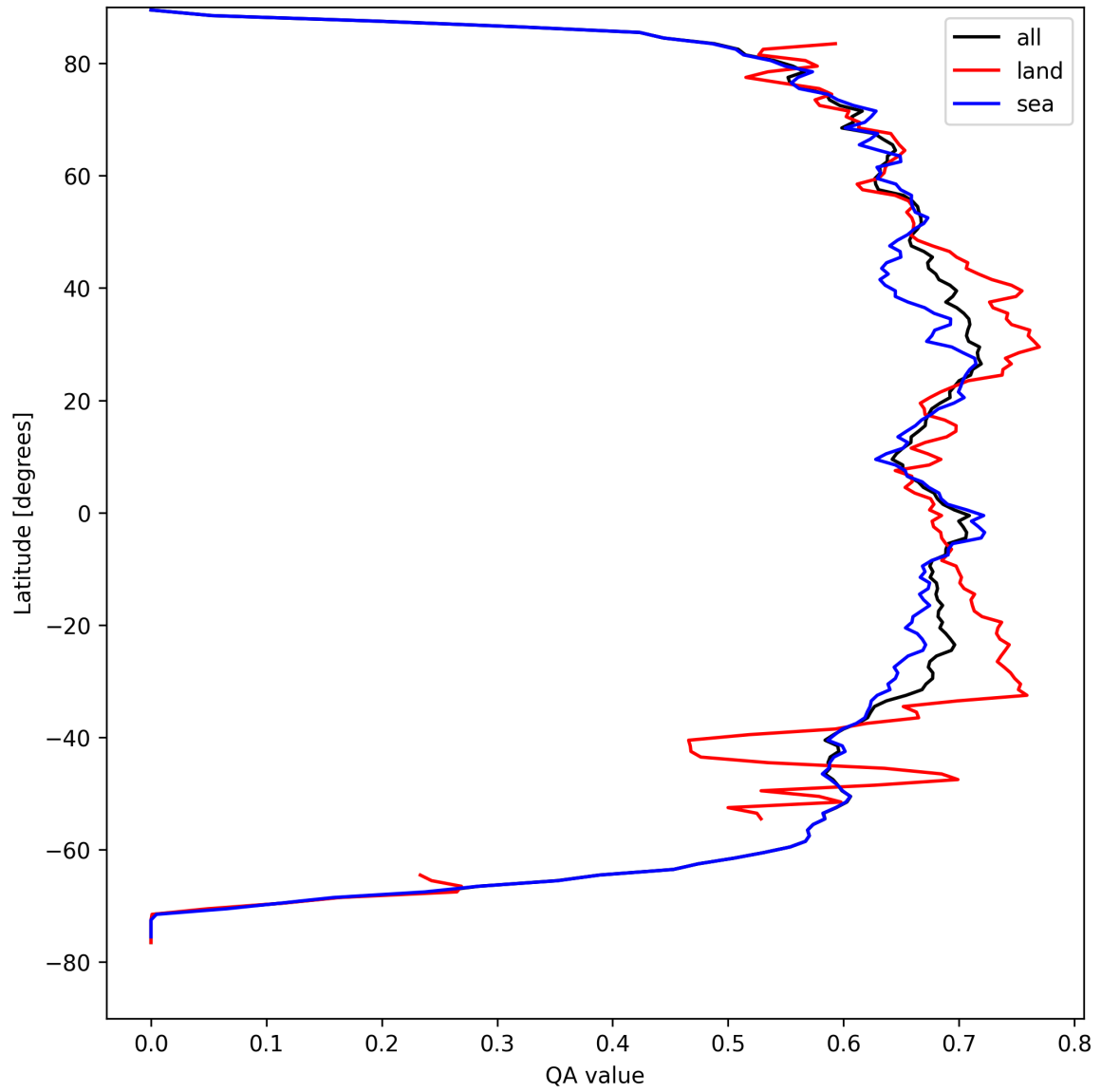
Figure 9: Zonal average of “QA value” for 2025-08-30 to 2025-09-01.
