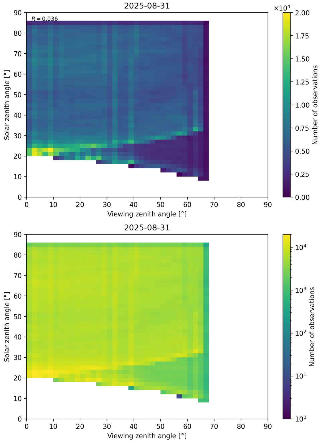
Figure 77: Scatter density plot of “Viewing zenith angle” against “Solar zenith angle” for 2025-08-30 to 2025-09-01.
