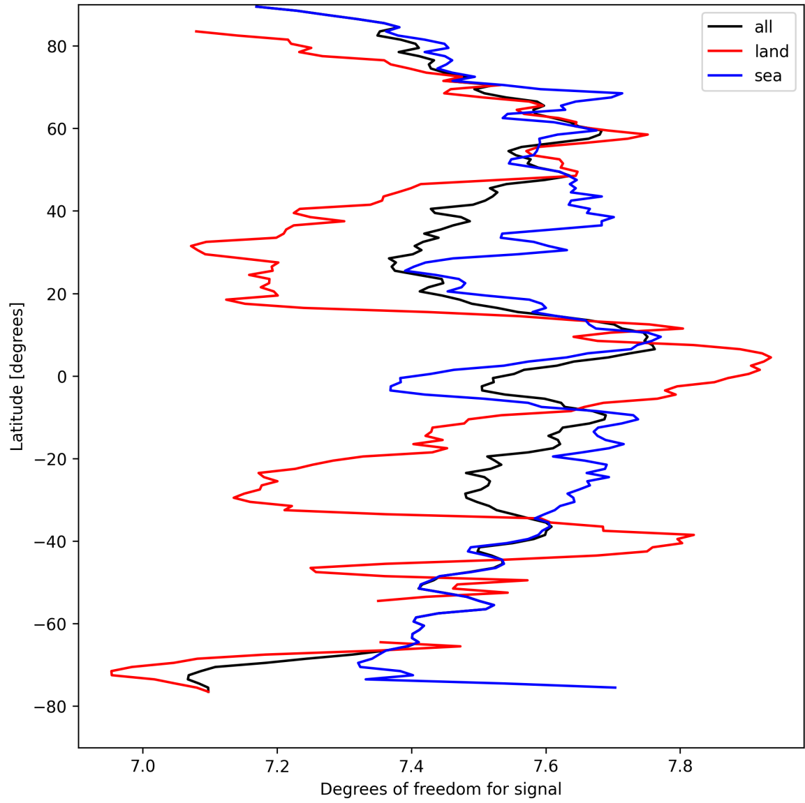
Figure 15: Zonal average of “Degrees of freedom for signal” for 2025-08-30 to 2025-09-01.
