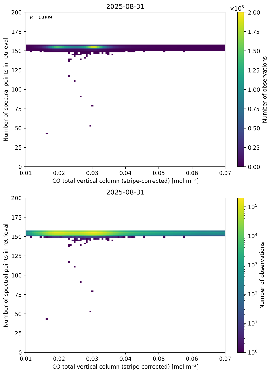
Figure 40: Scatter density plot of “CO total vertical column (stripe-corrected)” against “Number of spectral points in retrieval” for 2025-08-30 to 2025-09-01.
