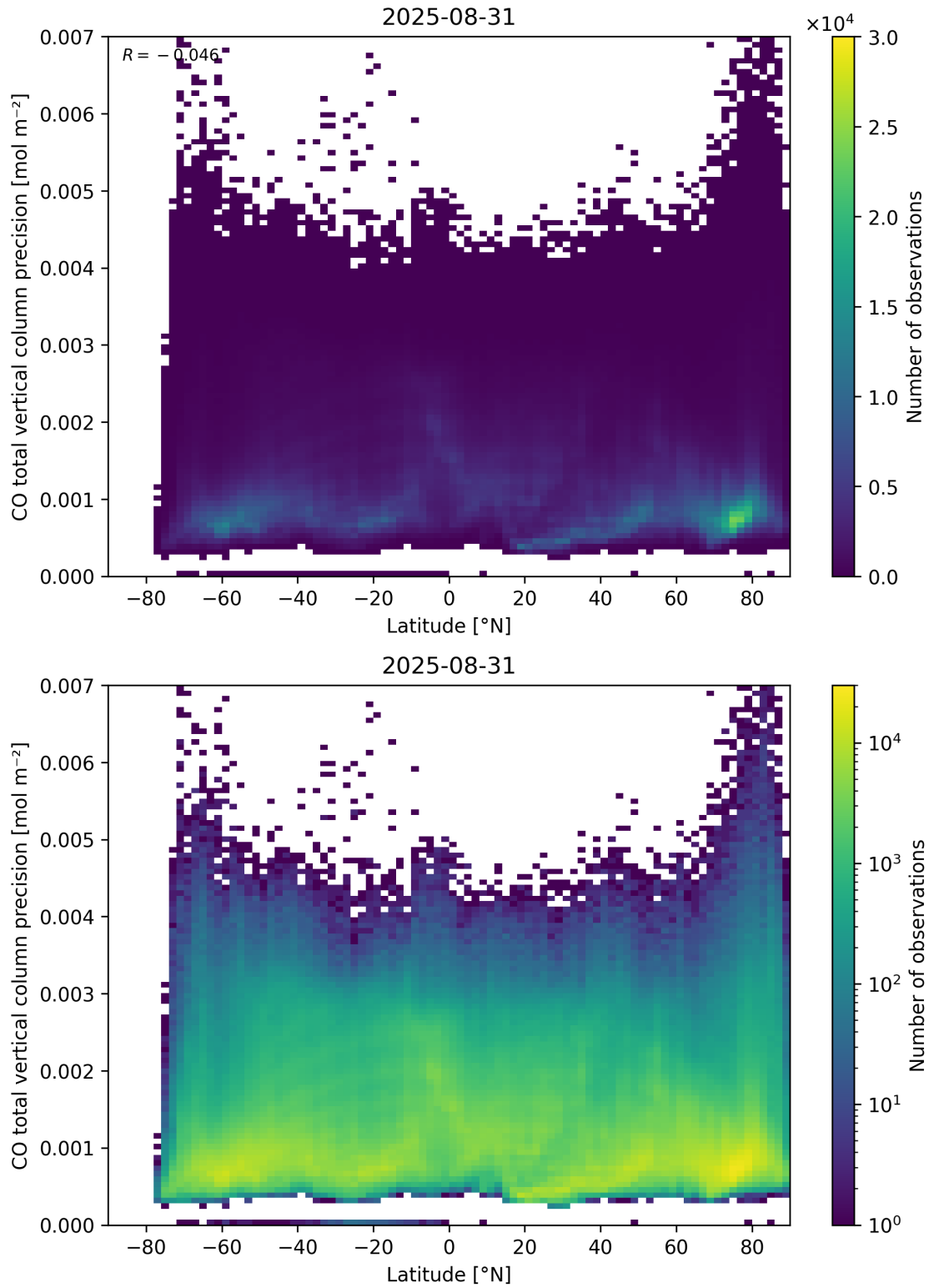
Figure 53: Scatter density plot of “Latitude” against “CO total vertical column precision” for 2025-08-30 to 2025-09-01.
