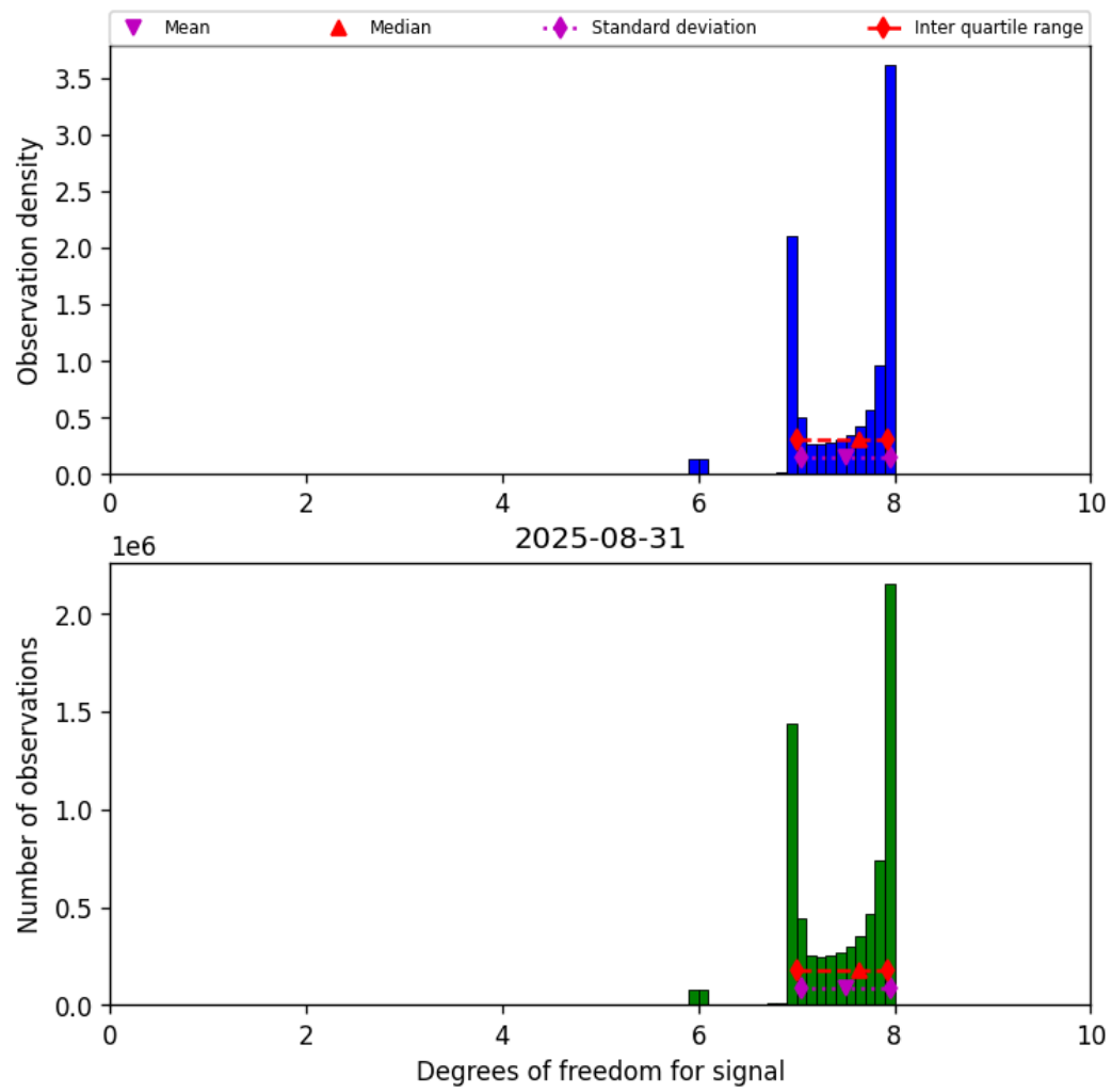
Figure 23: Histogram of “Degrees of freedom for signal” for 2025-08-30 to 2025-09-01
