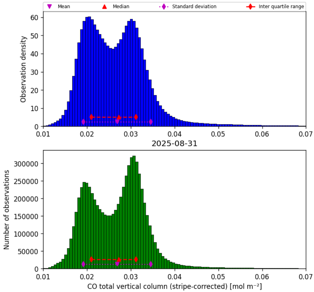
Figure 19: Histogram of “CO total vertical column (stripe-corrected)” for 2025-08-30 to 2025-09-01
