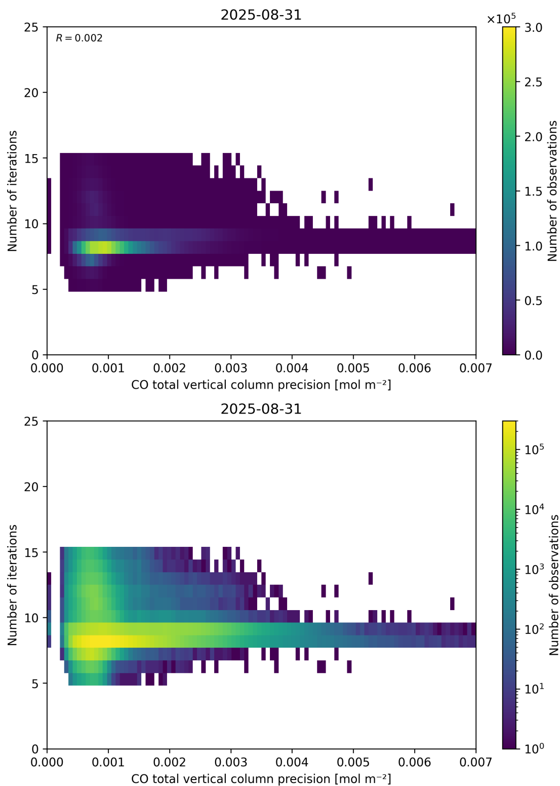
Figure 46: Scatter density plot of “CO total vertical column precision” against “Number of iterations” for 2025-08-30 to 2025-09-01.
