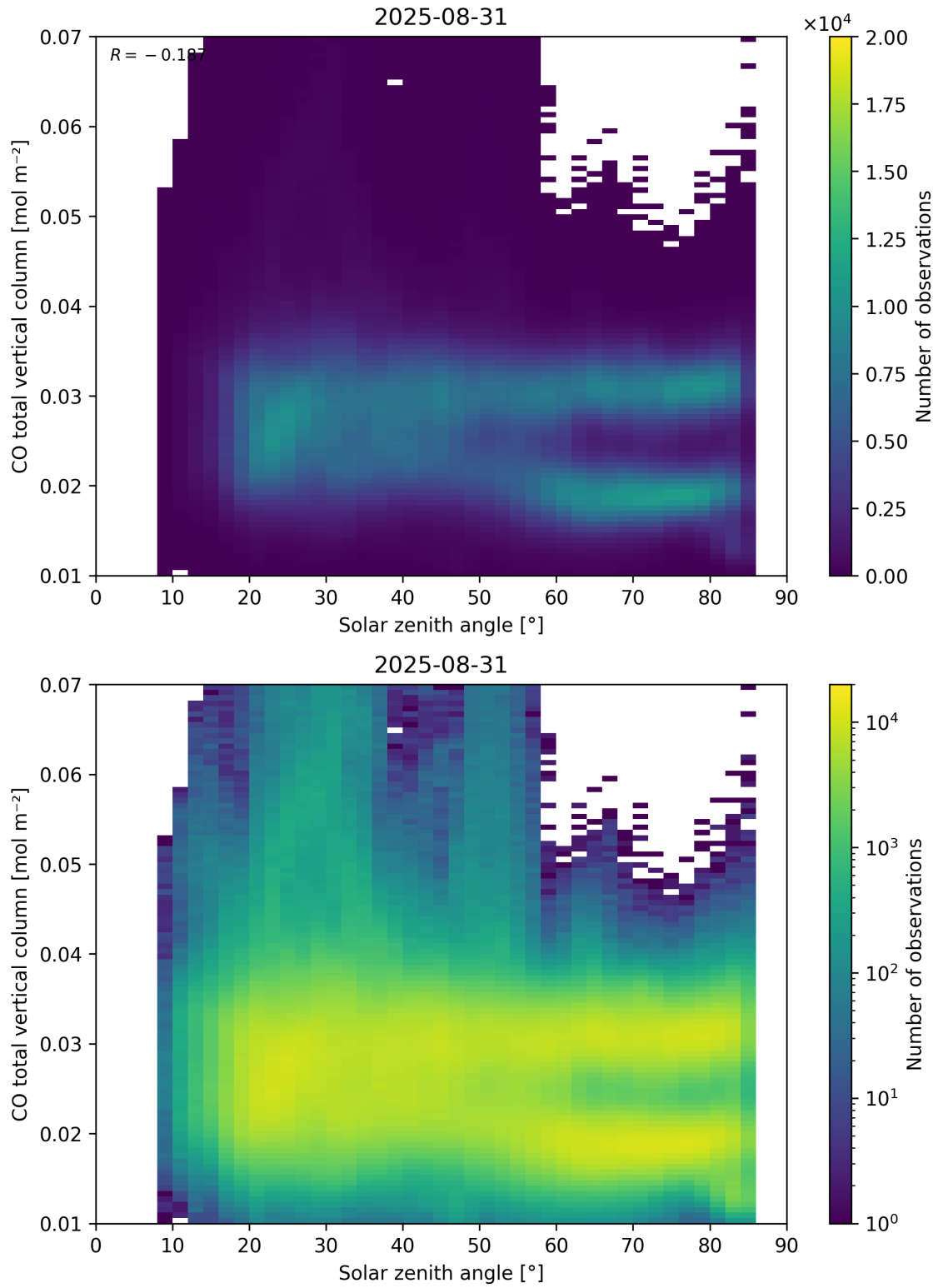
Figure 61: Scatter density plot of “Solar zenith angle” against “CO total vertical column” for 2025-08-30 to 2025-09-01.
