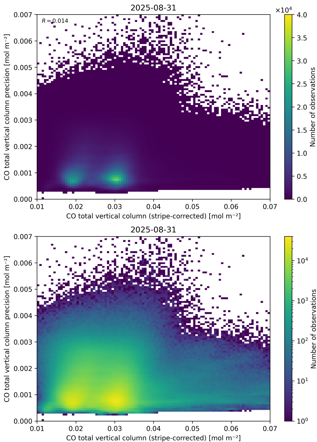
Figure 36: Scatter density plot of “CO total vertical column (stripe-corrected)” against “CO total vertical column precision” for 2025-08-30 to 2025-09-01.
