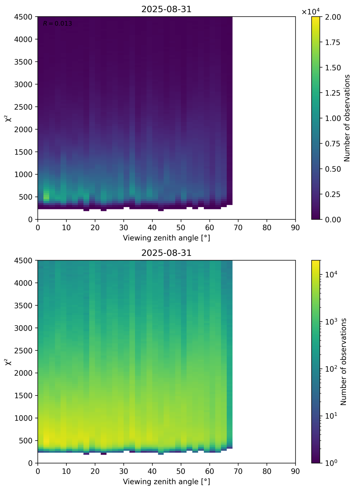
Figure 72: Scatter density plot of “Viewing zenith angle” against “ \chi^2 ” for 2025-08-30 to 2025-09-01.
