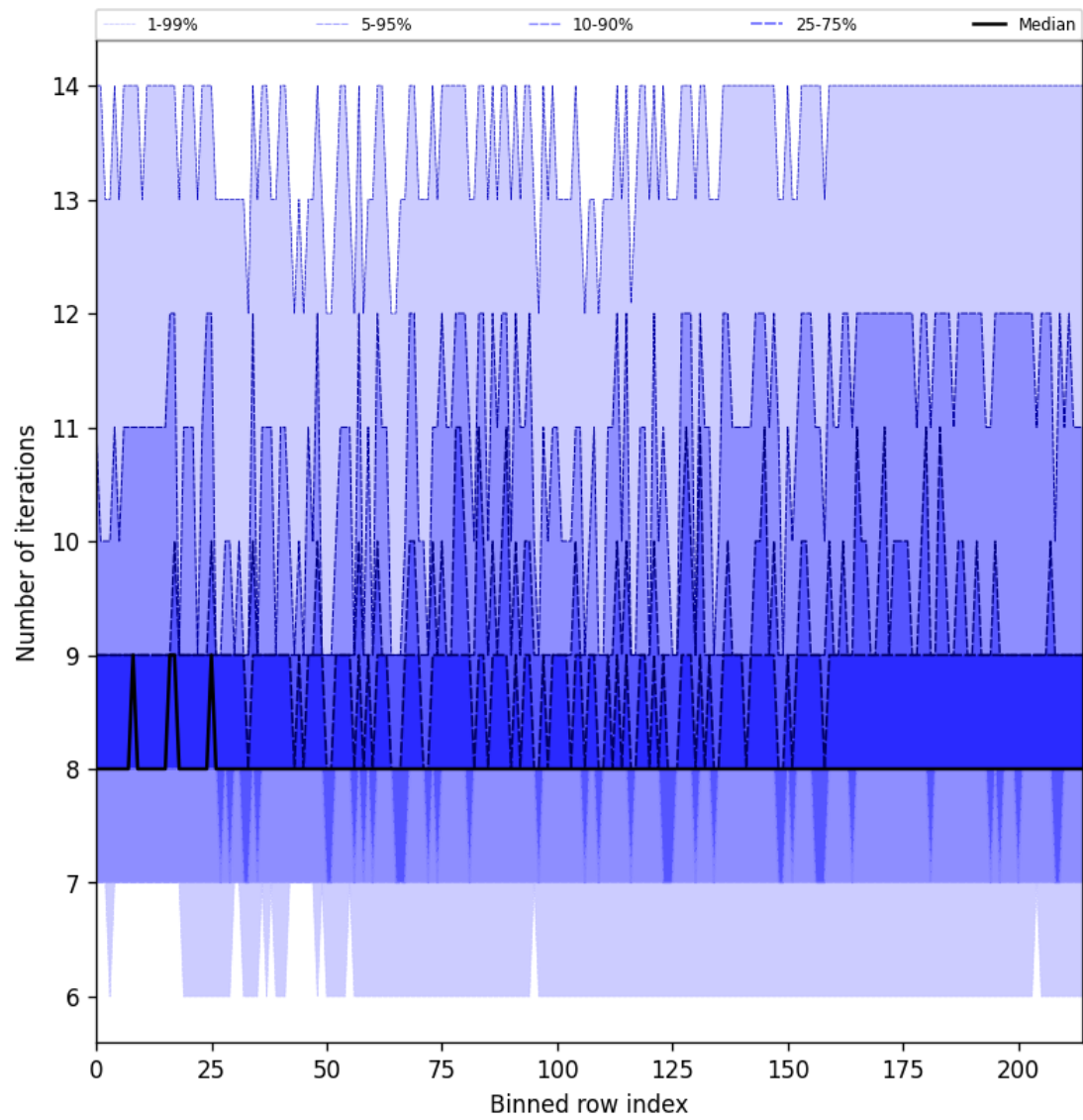
Figure 32: Along track statistics of “Number of iterations” for 2025-08-30 to 2025-09-01
