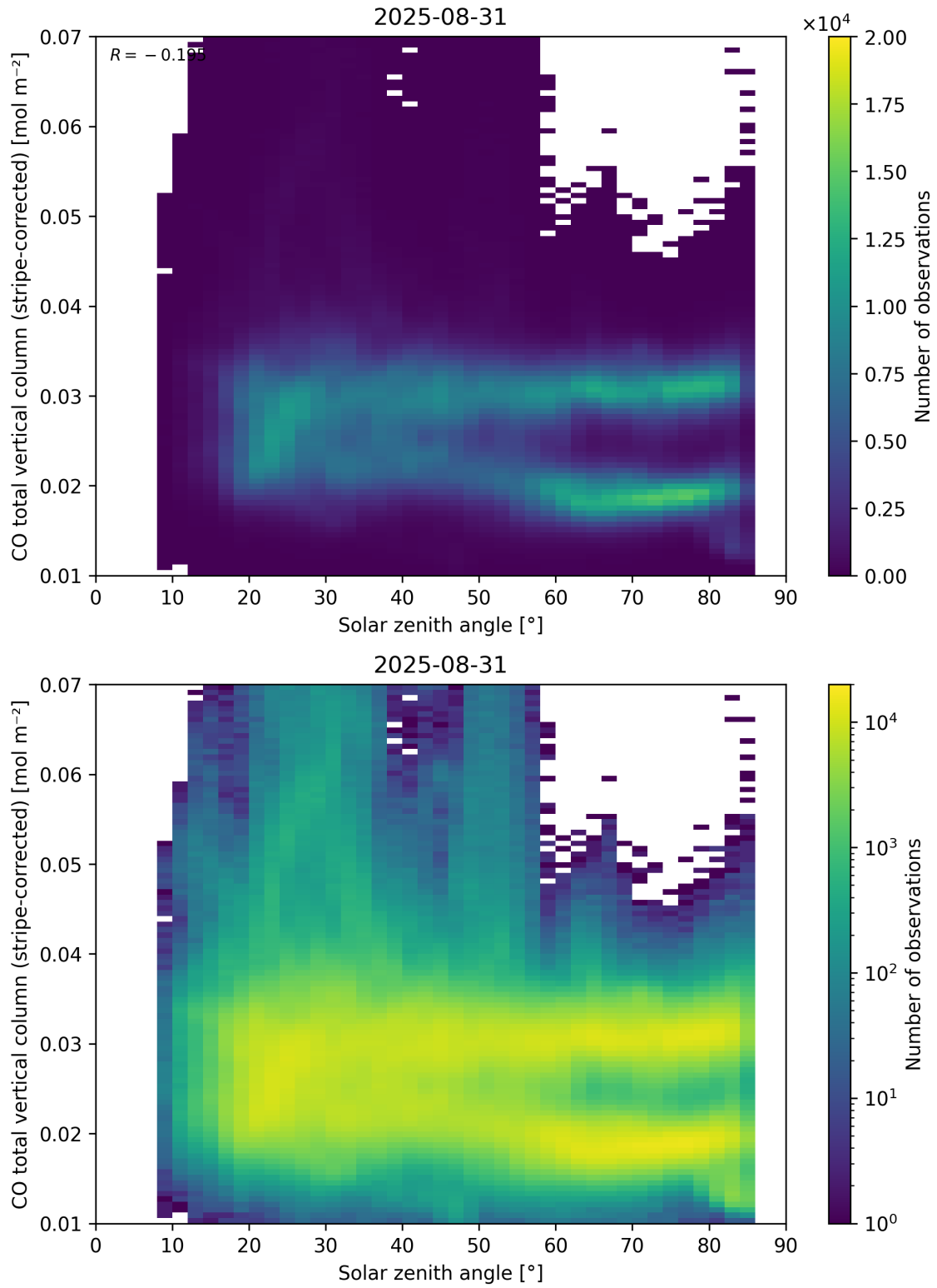
Figure 62: Scatter density plot of “Solar zenith angle” against “CO total vertical column (stripe-corrected)” for 2025-08-30 to 2025-09-01.
