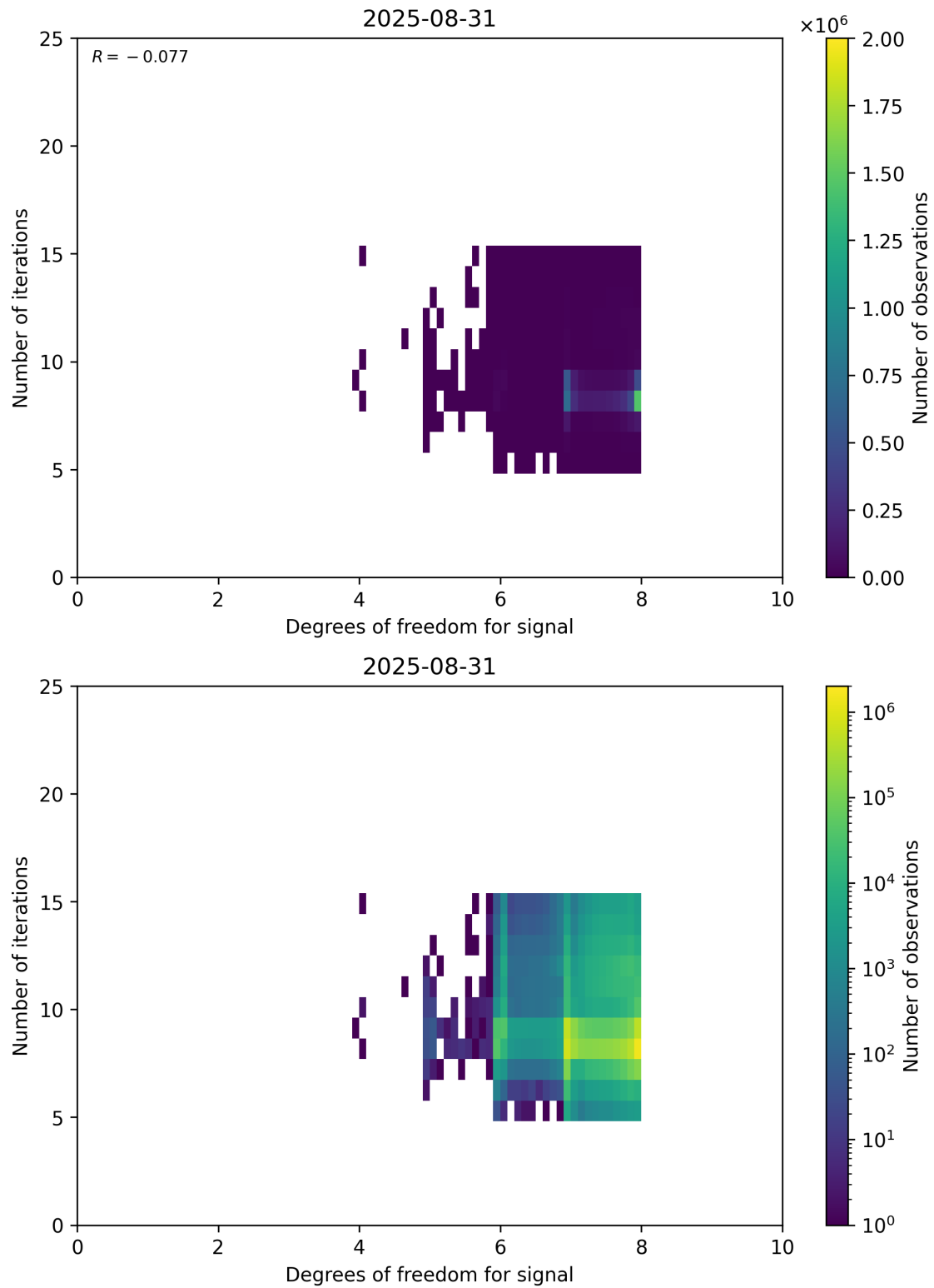
Figure 50: Scatter density plot of “Degrees of freedom for signal” against “Number of iterations” for 2025-08-30 to 2025-09-01.
