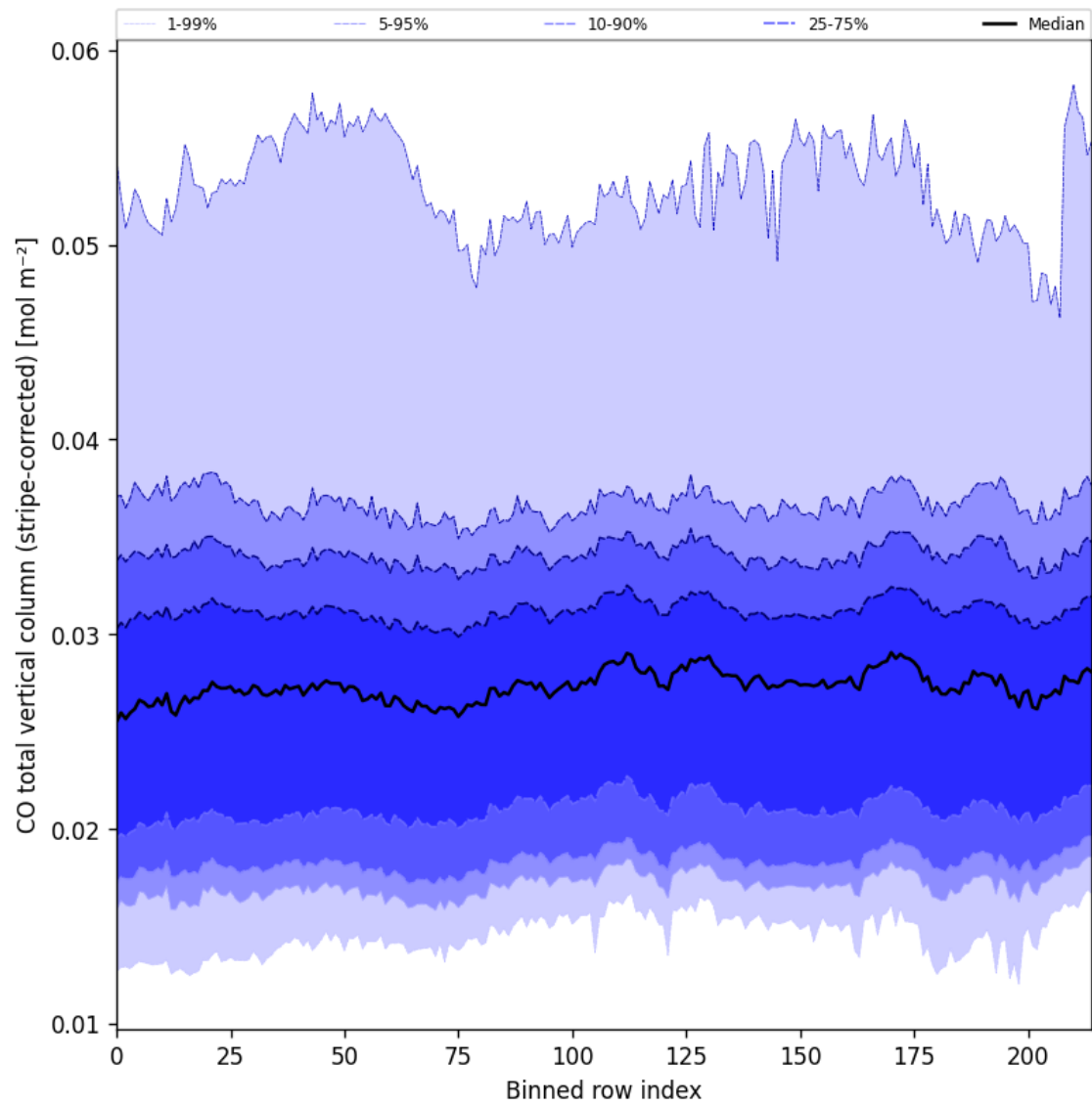
Figure 27: Along track statistics of “CO total vertical column (stripe-corrected)” for 2025-08-30 to 2025-09-01
