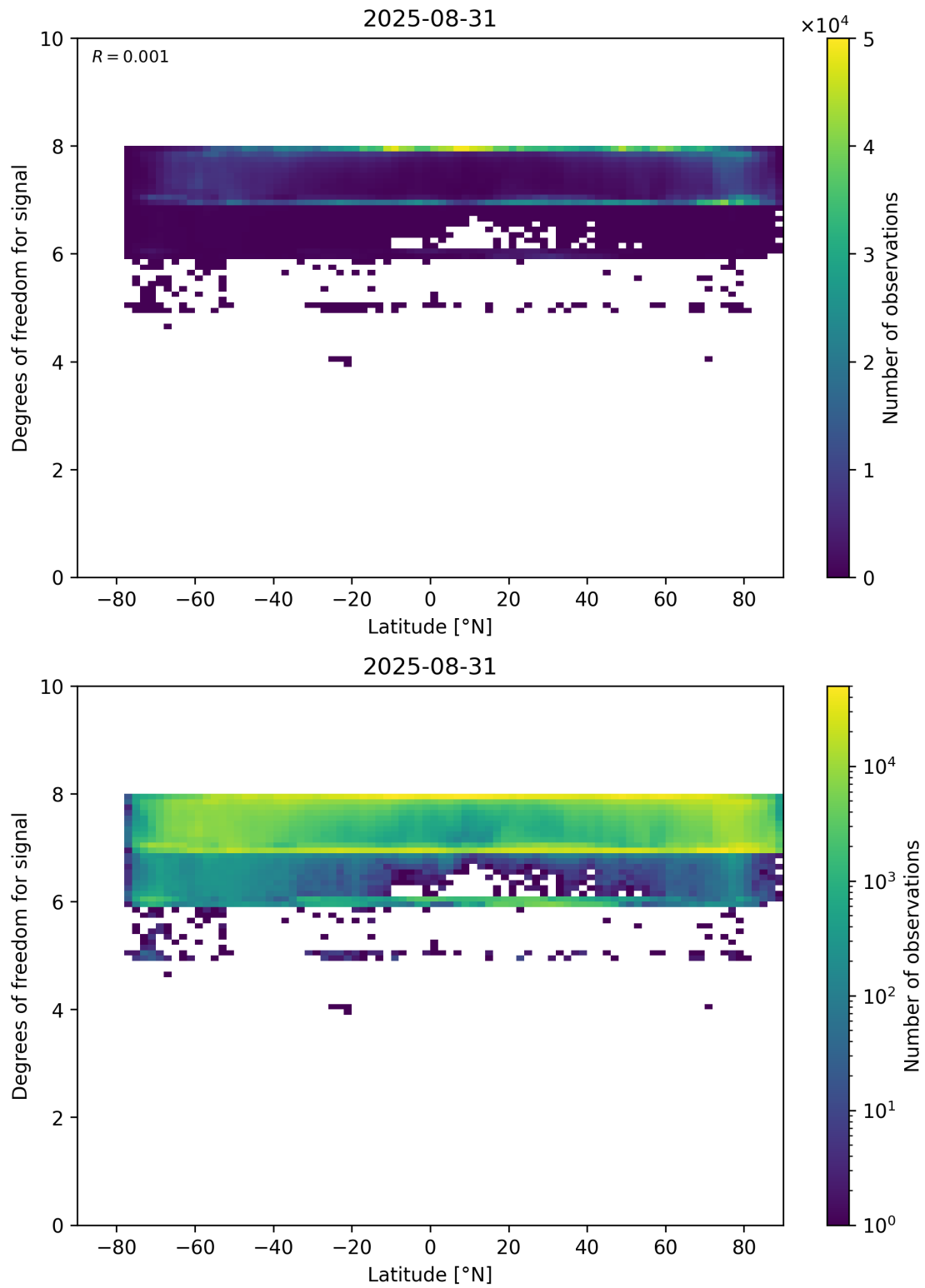
Figure 55: Scatter density plot of “Latitude” against “Degrees of freedom for signal” for 2025-08-30 to 2025-09-01.
