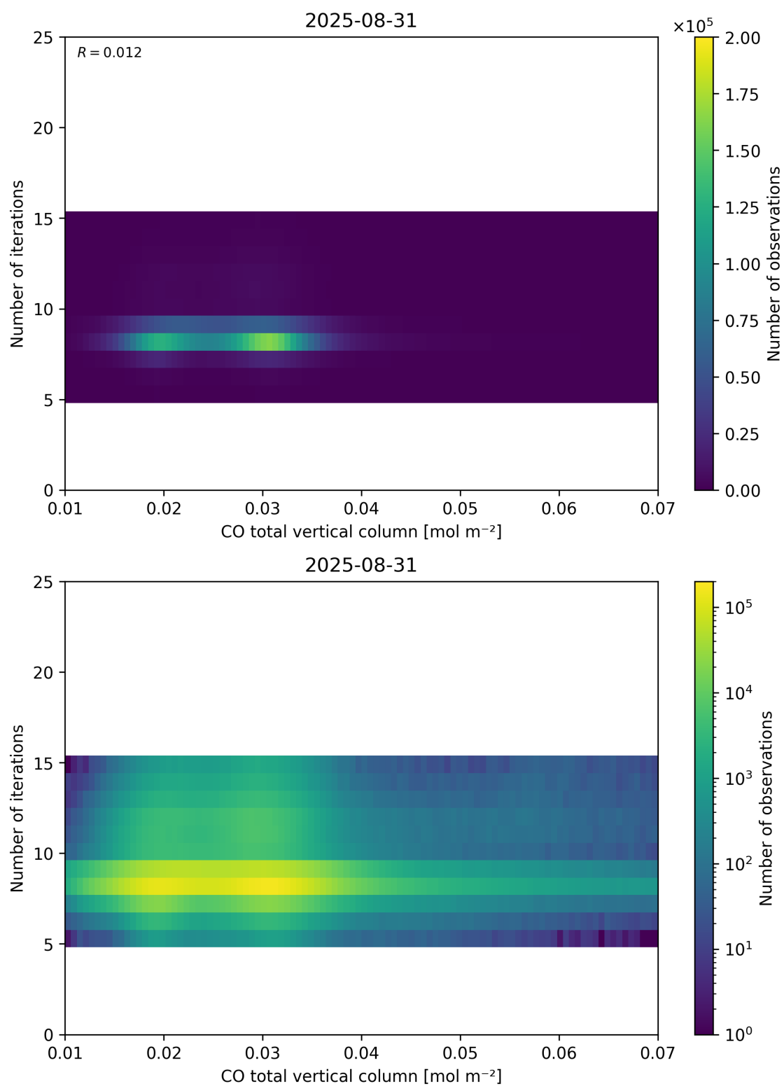
Figure 42: Scatter density plot of “CO total vertical column” against “Number of iterations” for 2025-08-30 to 2025-09-01.
