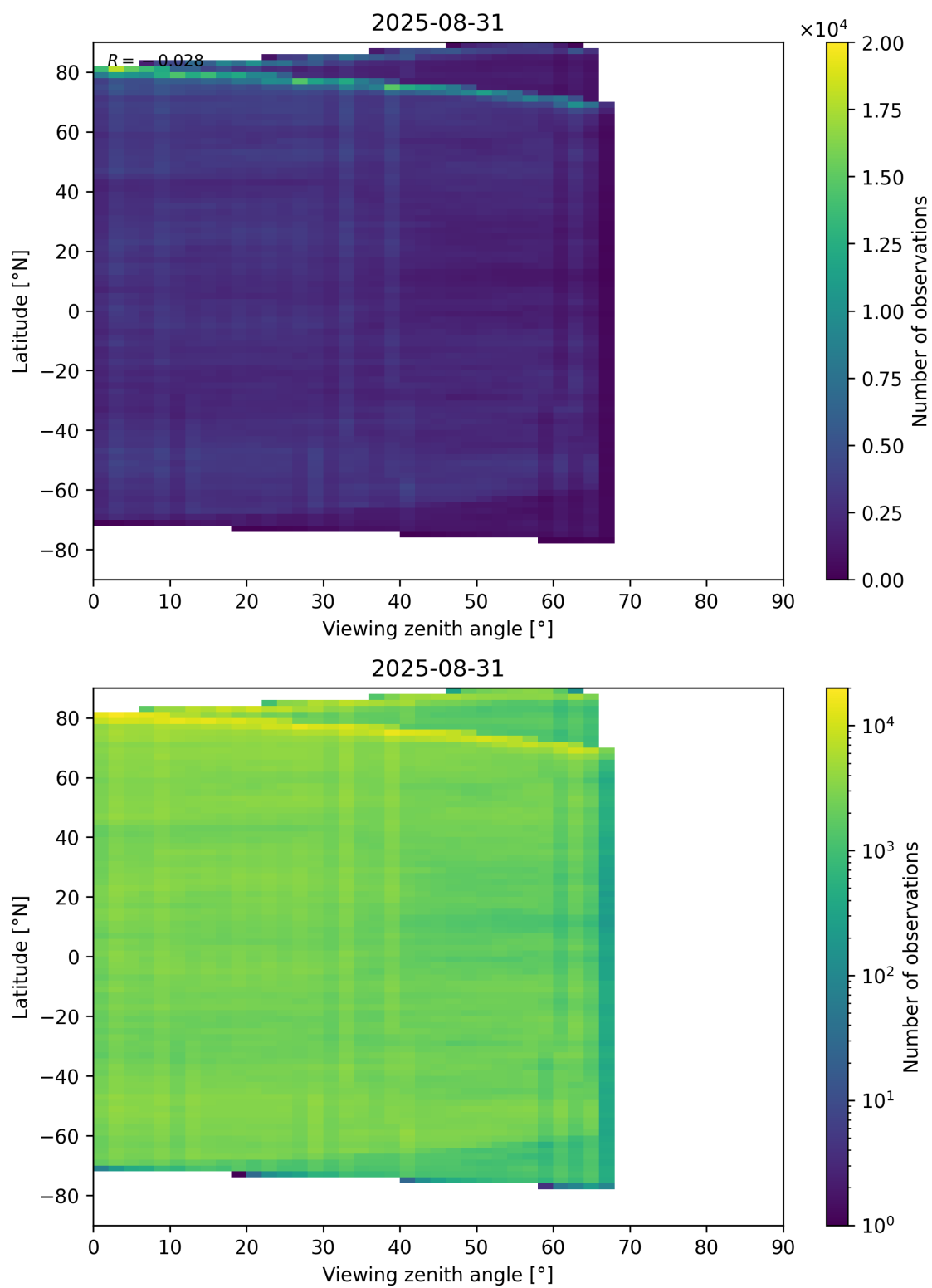
Figure 74: Scatter density plot of “Viewing zenith angle” against “Latitude” for 2025-08-30 to 2025-09-01.
