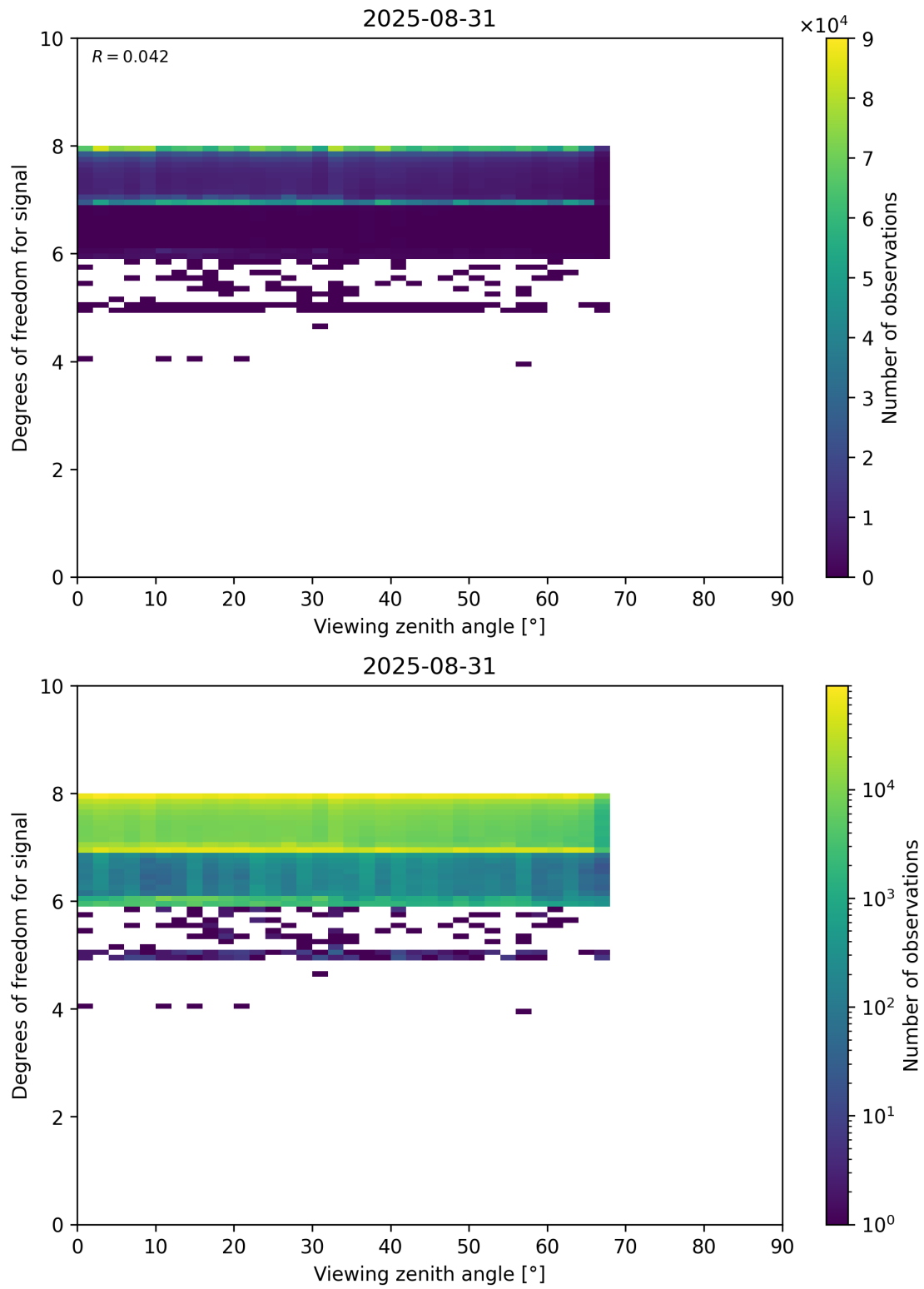
Figure 73: Scatter density plot of “Viewing zenith angle” against “Degrees of freedom for signal” for 2025-08-30 to 2025-09-01.
