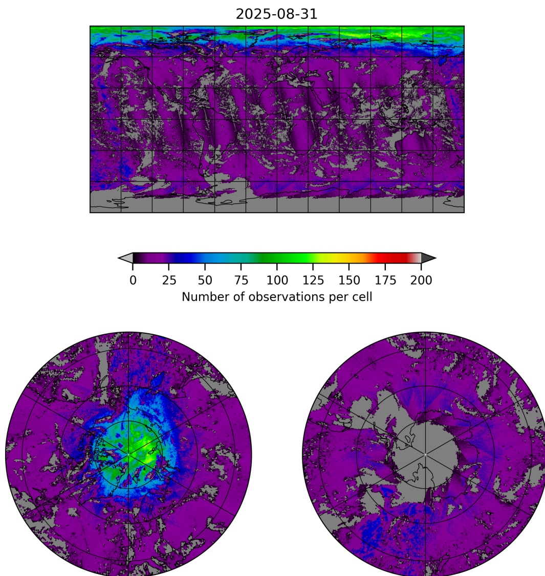
Figure 8: Map of the number of observations for 2025-08-30 to 2025-09-01
