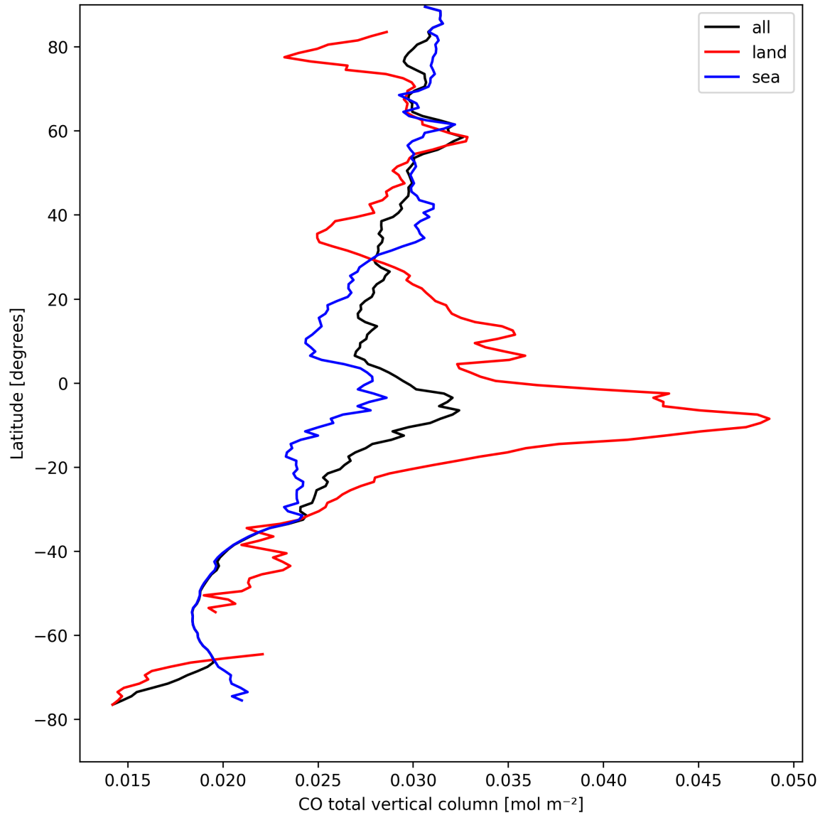
Figure 10: Zonal average of “CO total vertical column” for 2025-08-30 to 2025-09-01.
