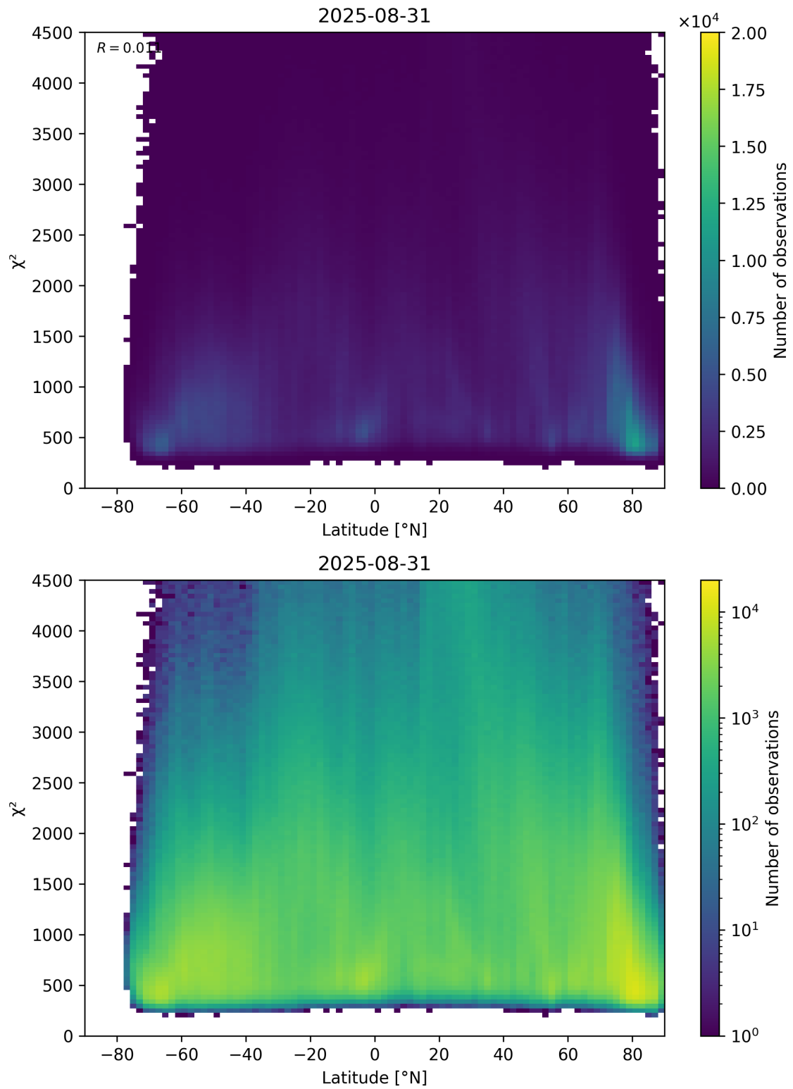
Figure 54: Scatter density plot of “Latitude” against “ \chi^2 ” for 2025-08-30 to 2025-09-01.
