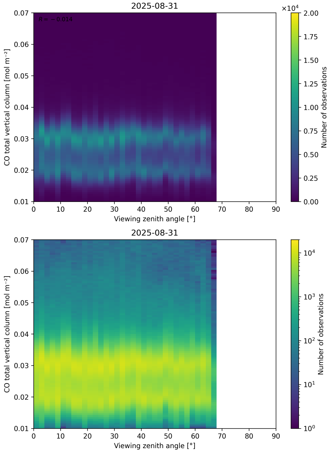
Figure 69: Scatter density plot of “Viewing zenith angle” against “CO total vertical column” for 2025-08-30 to 2025-09-01.
