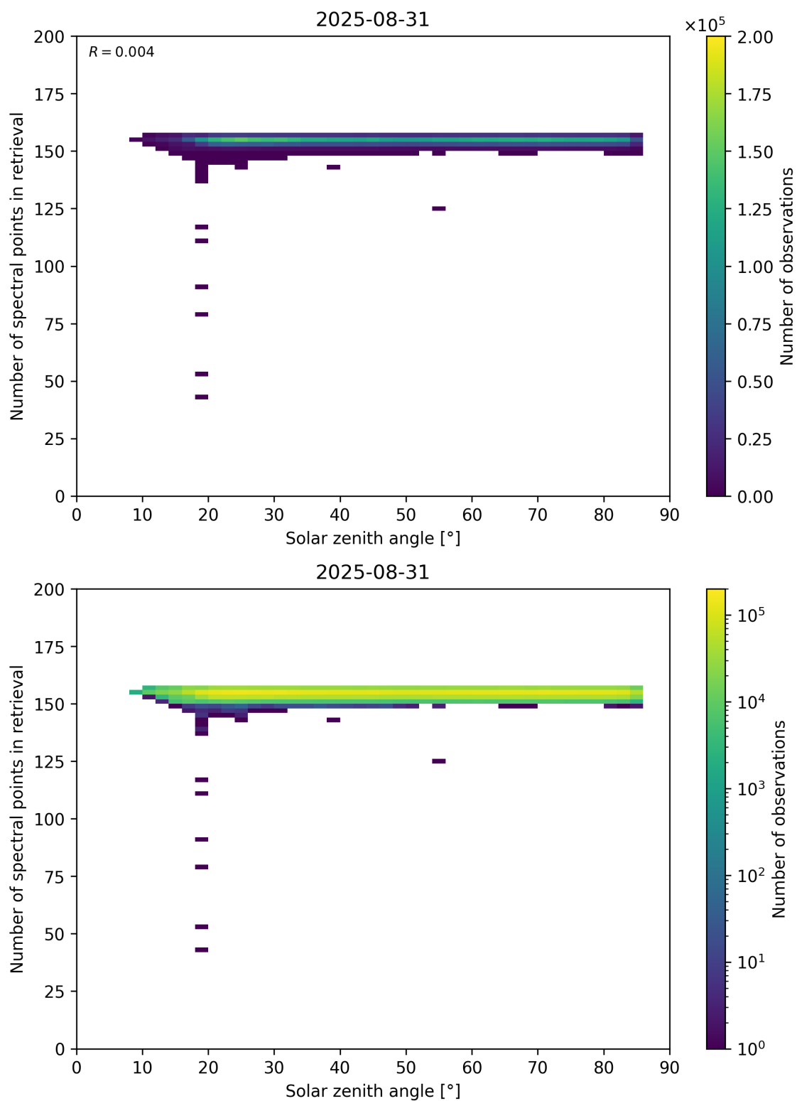
Figure 68: Scatter density plot of “Solar zenith angle” against “Number of spectral points in retrieval” for 2025-08-30 to 2025-09-01.
