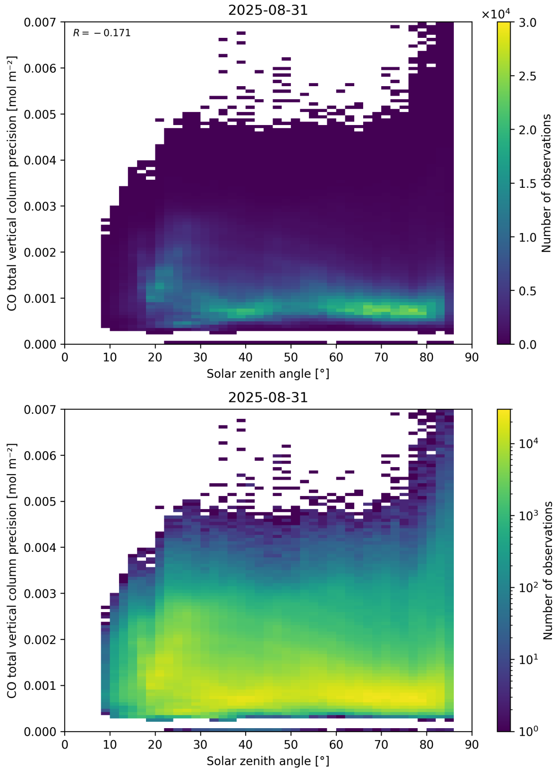
Figure 63: Scatter density plot of “Solar zenith angle” against “CO total vertical column precision” for 2025-08-30 to 2025-09-01.
