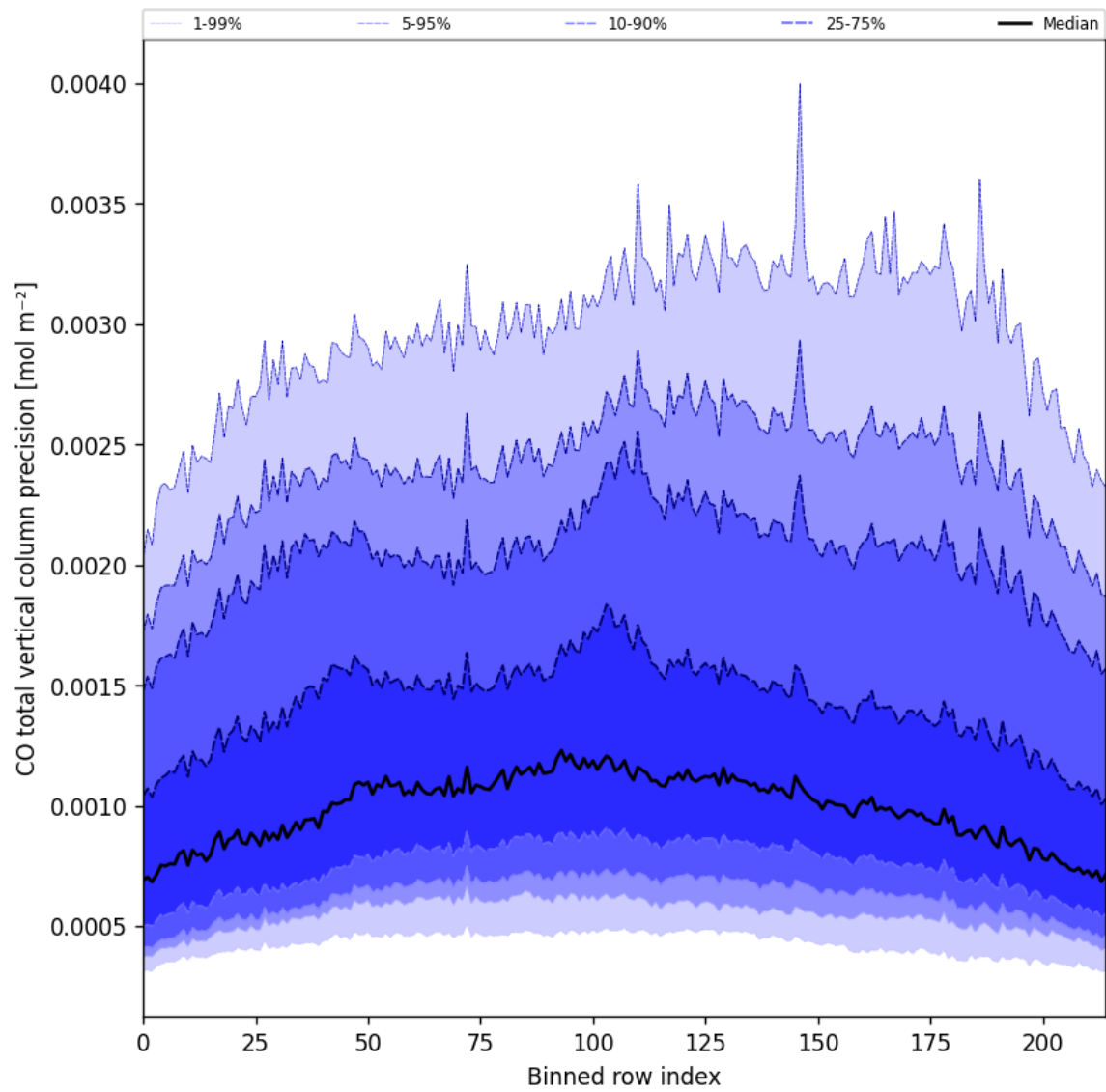
Figure 28: Along track statistics of “CO total vertical column precision” for 2025-08-30 to 2025-09-01
