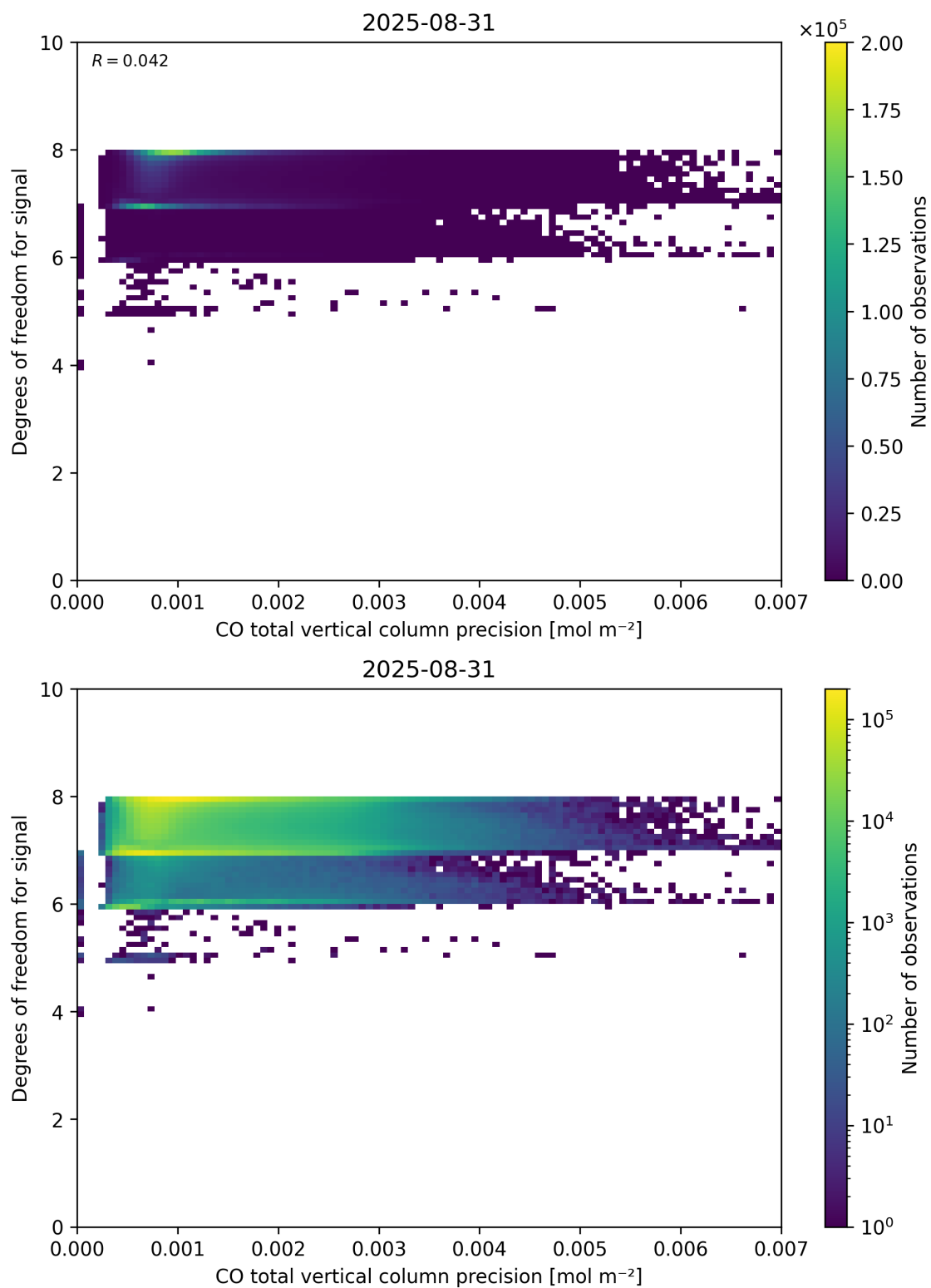
Figure 45: Scatter density plot of “CO total vertical column precision” against “Degrees of freedom for signal” for 2025-08-30 to 2025-09-01.
