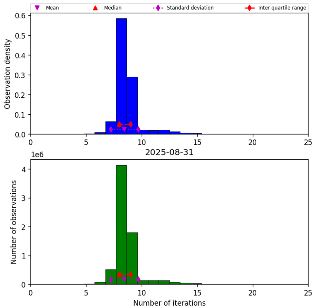
Figure 24: Histogram of “Number of iterations” for 2025-08-30 to 2025-09-01
