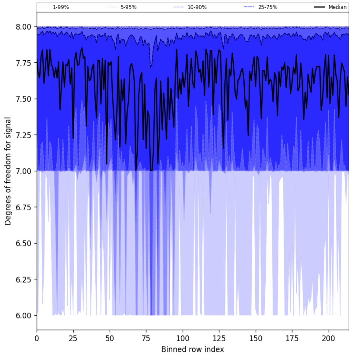
Figure 31: Along track statistics of “Degrees of freedom for signal” for 2025-08-30 to 2025-09-01
