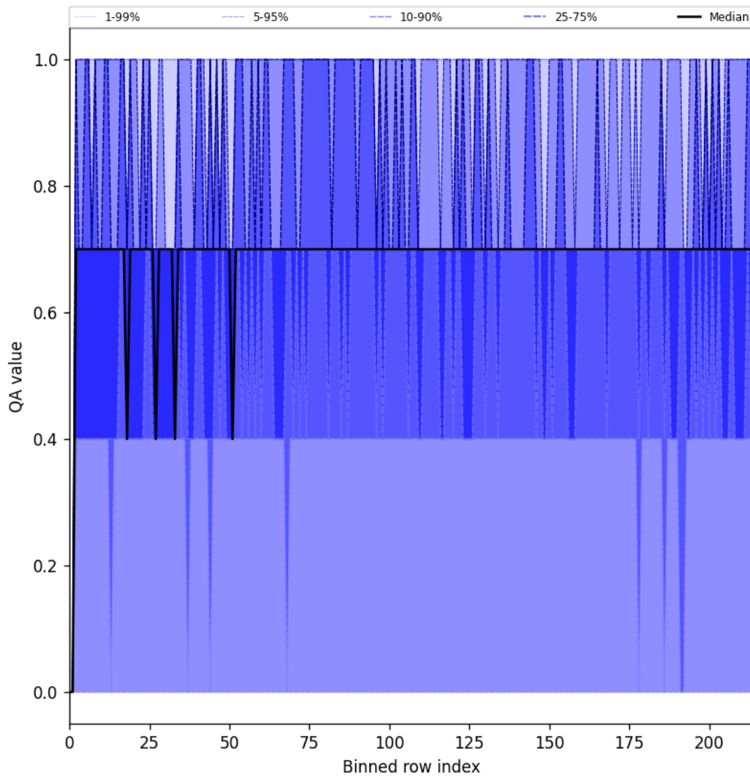
Figure 25: Along track statistics of “QA value” for 2025-08-30 to 2025-09-01
