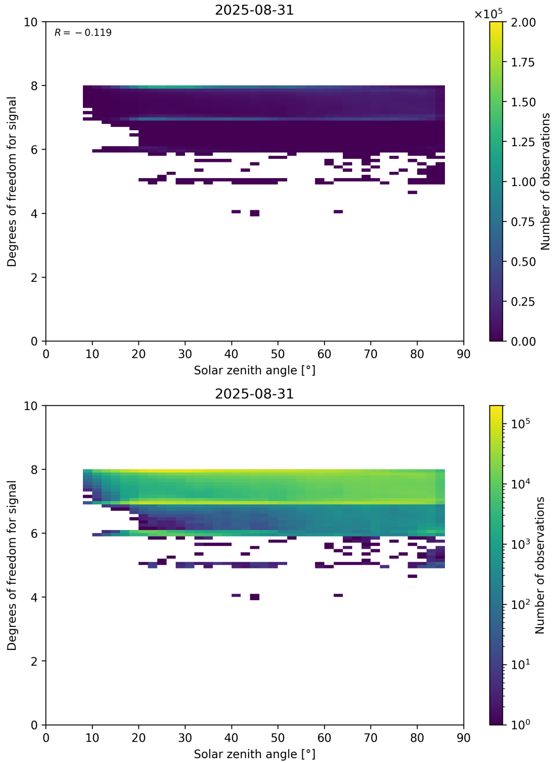
Figure 65: Scatter density plot of “Solar zenith angle” against “Degrees of freedom for signal” for 2025-08-30 to 2025-09-01.
