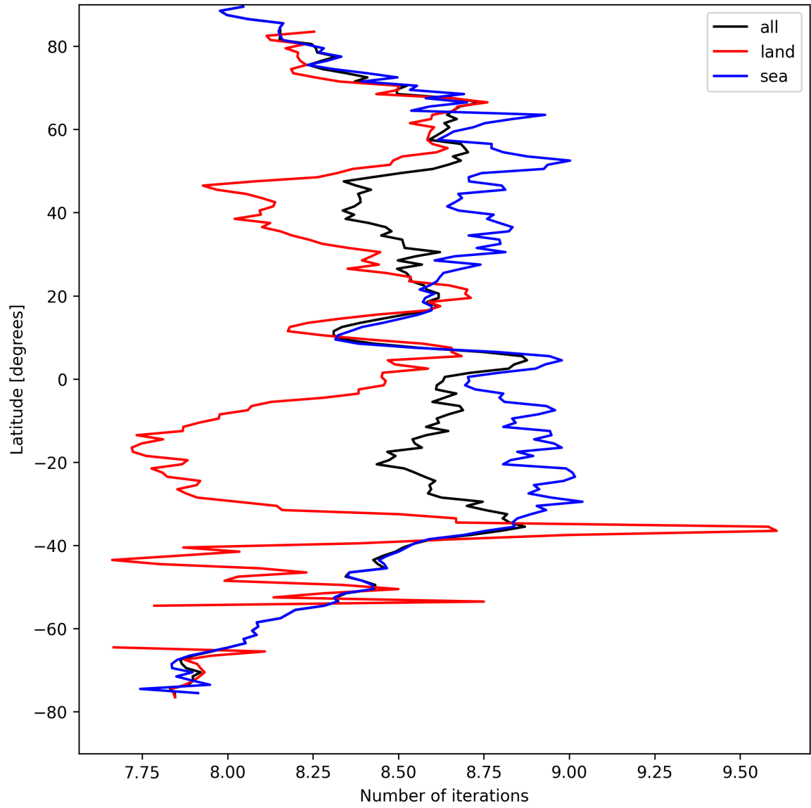
Figure 16: Zonal average of “Number of iterations” for 2025-08-30 to 2025-09-01.
