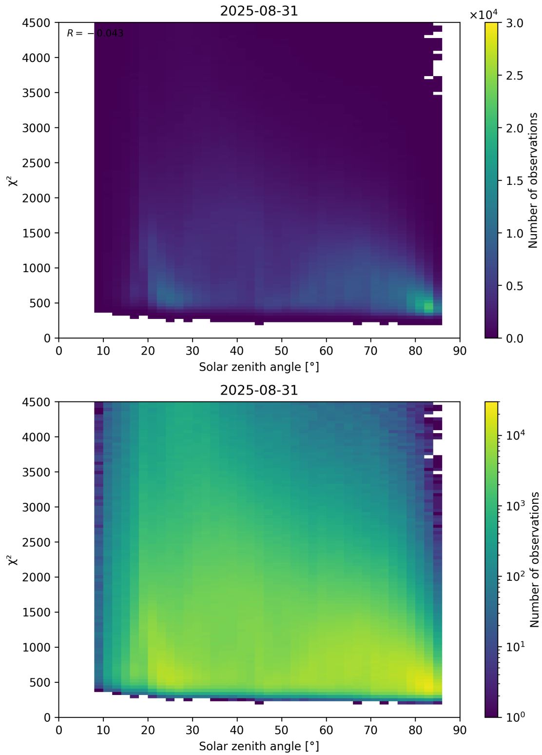
Figure 64: Scatter density plot of “Solar zenith angle” against “ \chi^2 ” for 2025-08-30 to 2025-09-01.
