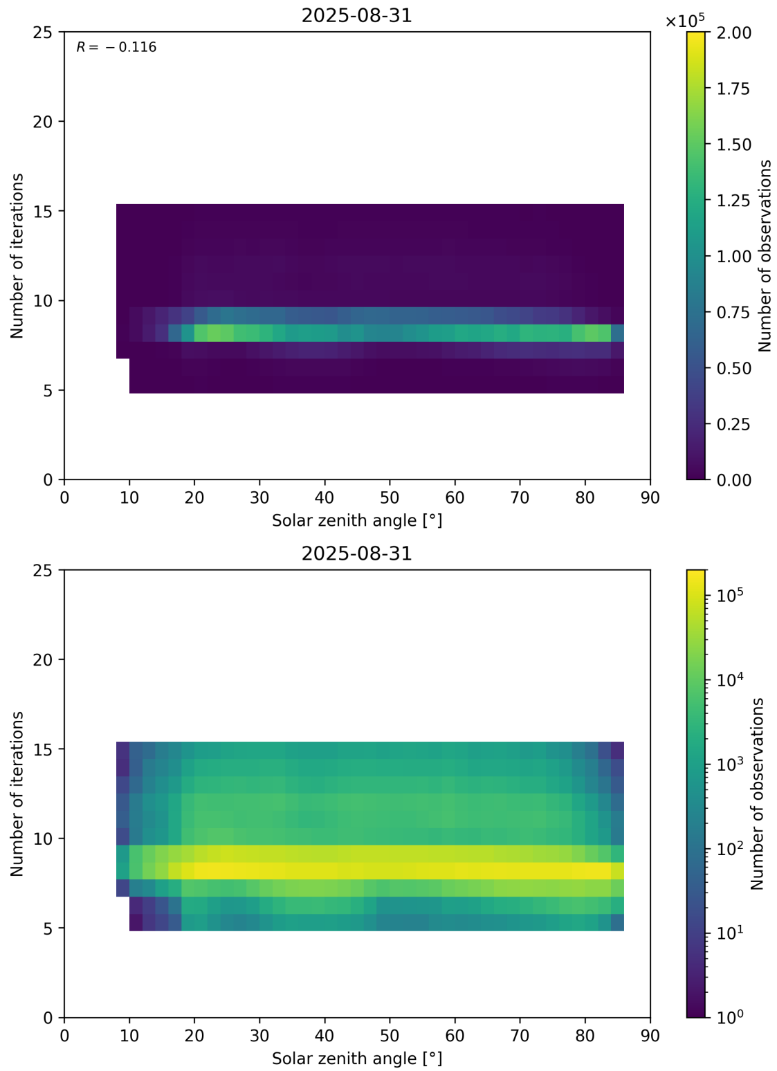
Figure 67: Scatter density plot of “Solar zenith angle” against “Number of iterations” for 2025-08-30 to 2025-09-01.
