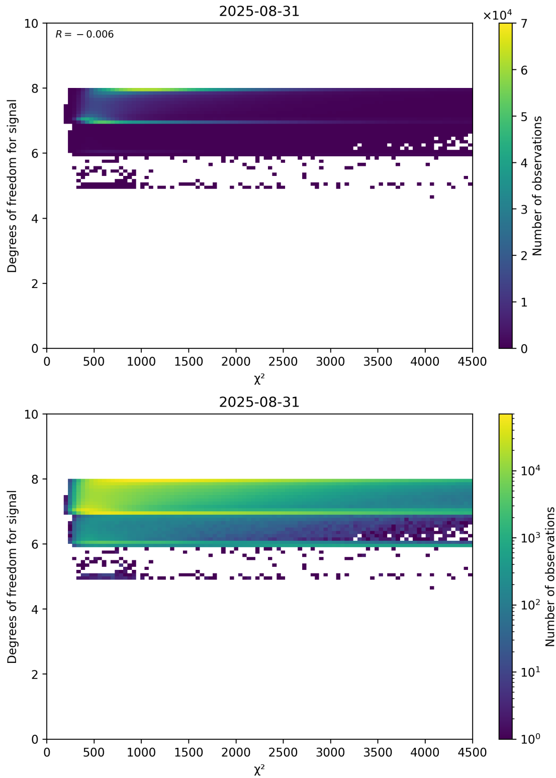
Figure 48: Scatter density plot of “ \chi^2 ” against “Degrees of freedom for signal” for 2025-08-30 to 2025-09-01.
