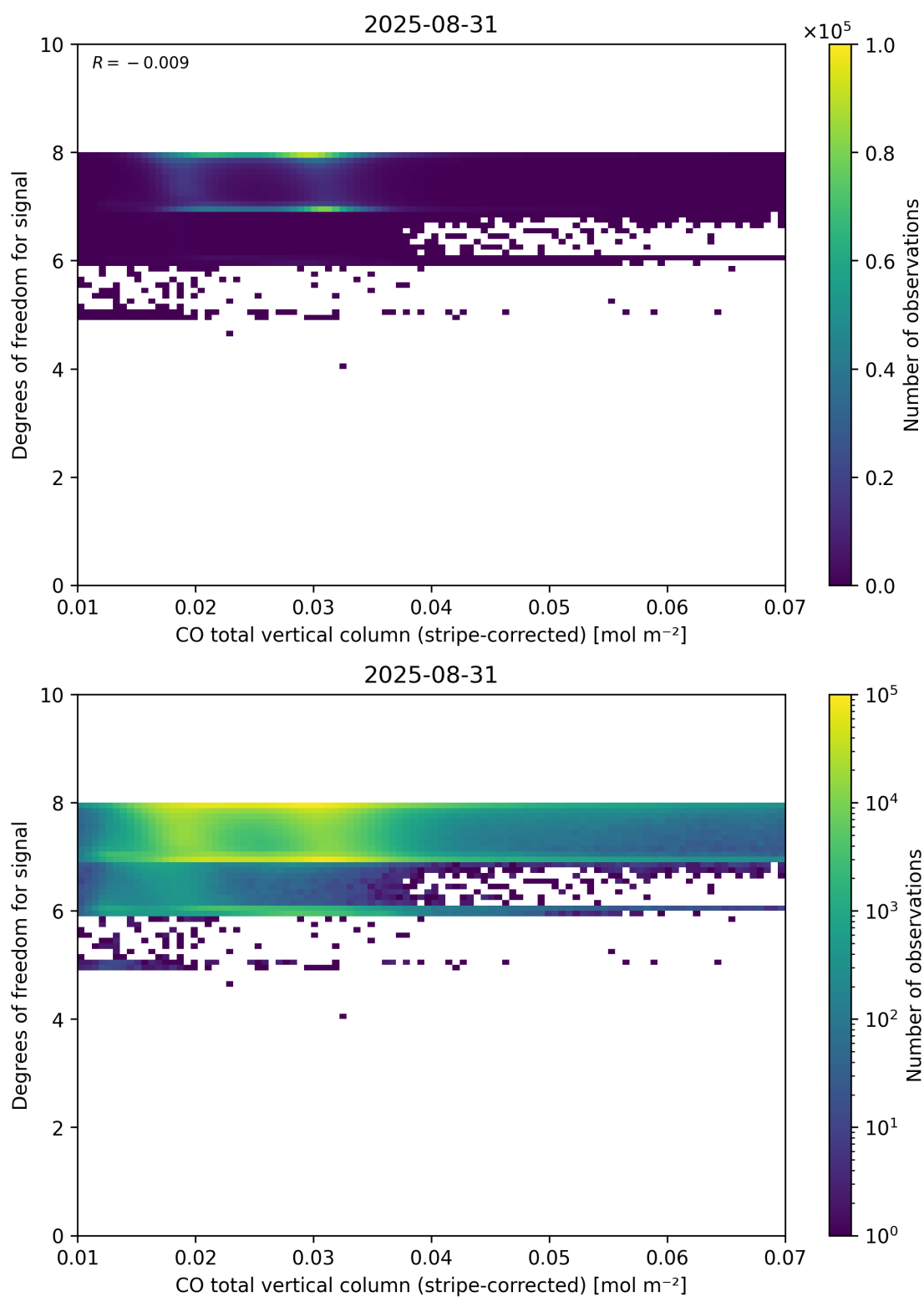
Figure 38: Scatter density plot of “CO total vertical column (stripe-corrected)” against “Degrees of freedom for signal” for 2025-08-30 to 2025-09-01.
