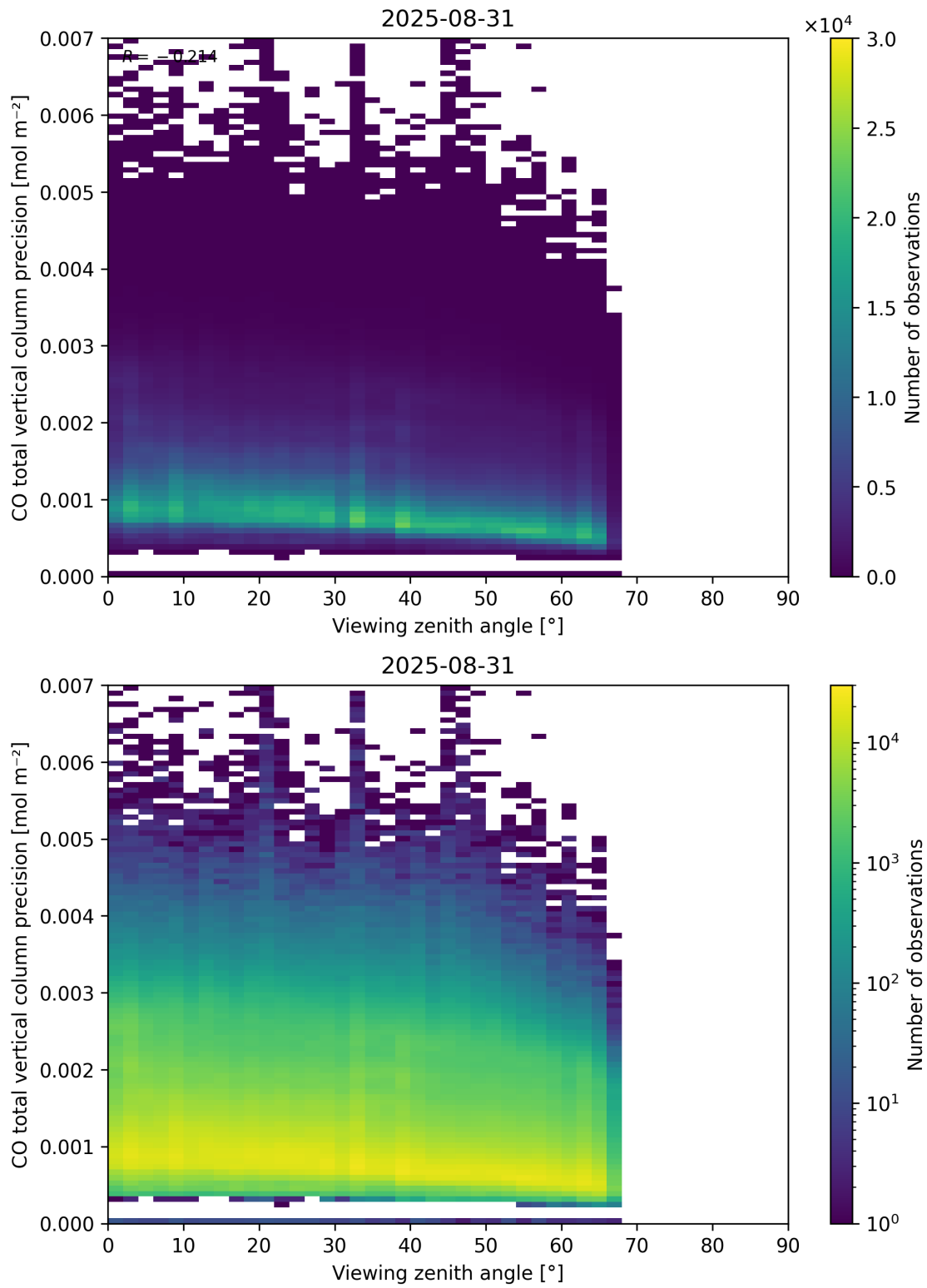
Figure 71: Scatter density plot of “Viewing zenith angle” against “CO total vertical column precision” for 2025-08-30 to 2025-09-01.
