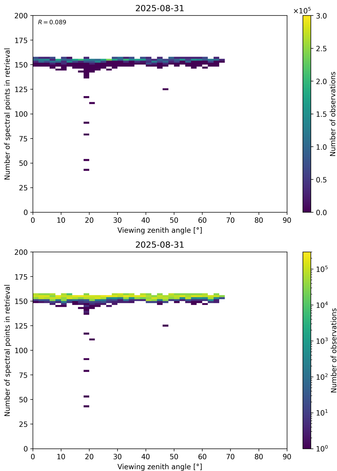
Figure 76: Scatter density plot of “Viewing zenith angle” against “Number of spectral points in retrieval” for 2025-08-30 to 2025-09-01.
