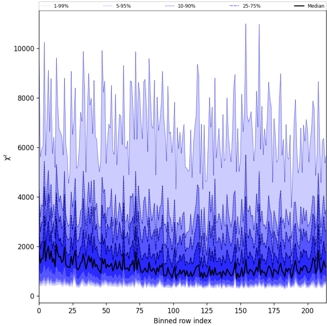
Figure 30: Along track statistics of “ \chi^2 ” for 2025-08-30 to 2025-09-01
