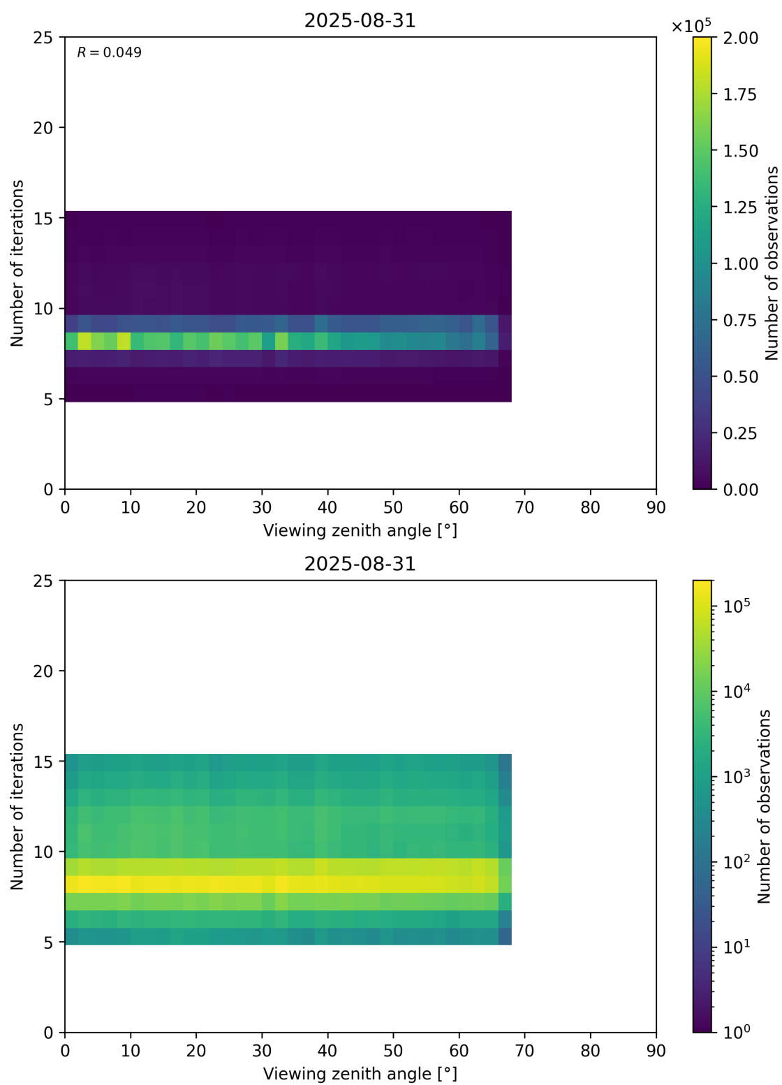
Figure 75: Scatter density plot of “Viewing zenith angle” against “Number of iterations” for 2025-08-30 to 2025-09-01.
