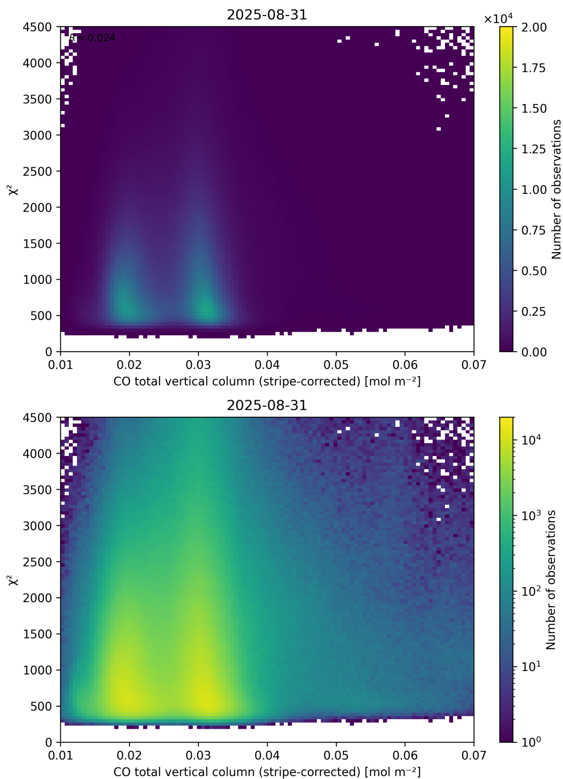
Figure 37: Scatter density plot of “CO total vertical column (stripe-corrected)” against “ \chi^2 ” for 2025-08-30 to 2025-09-01.
