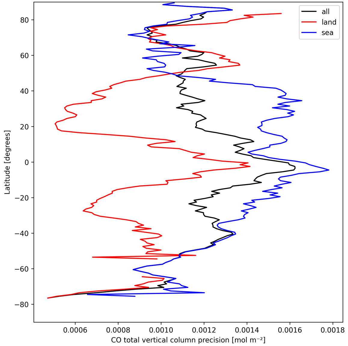
Figure 12: Zonal average of “CO total vertical column precision” for 2025-08-30 to 2025-09-01.
