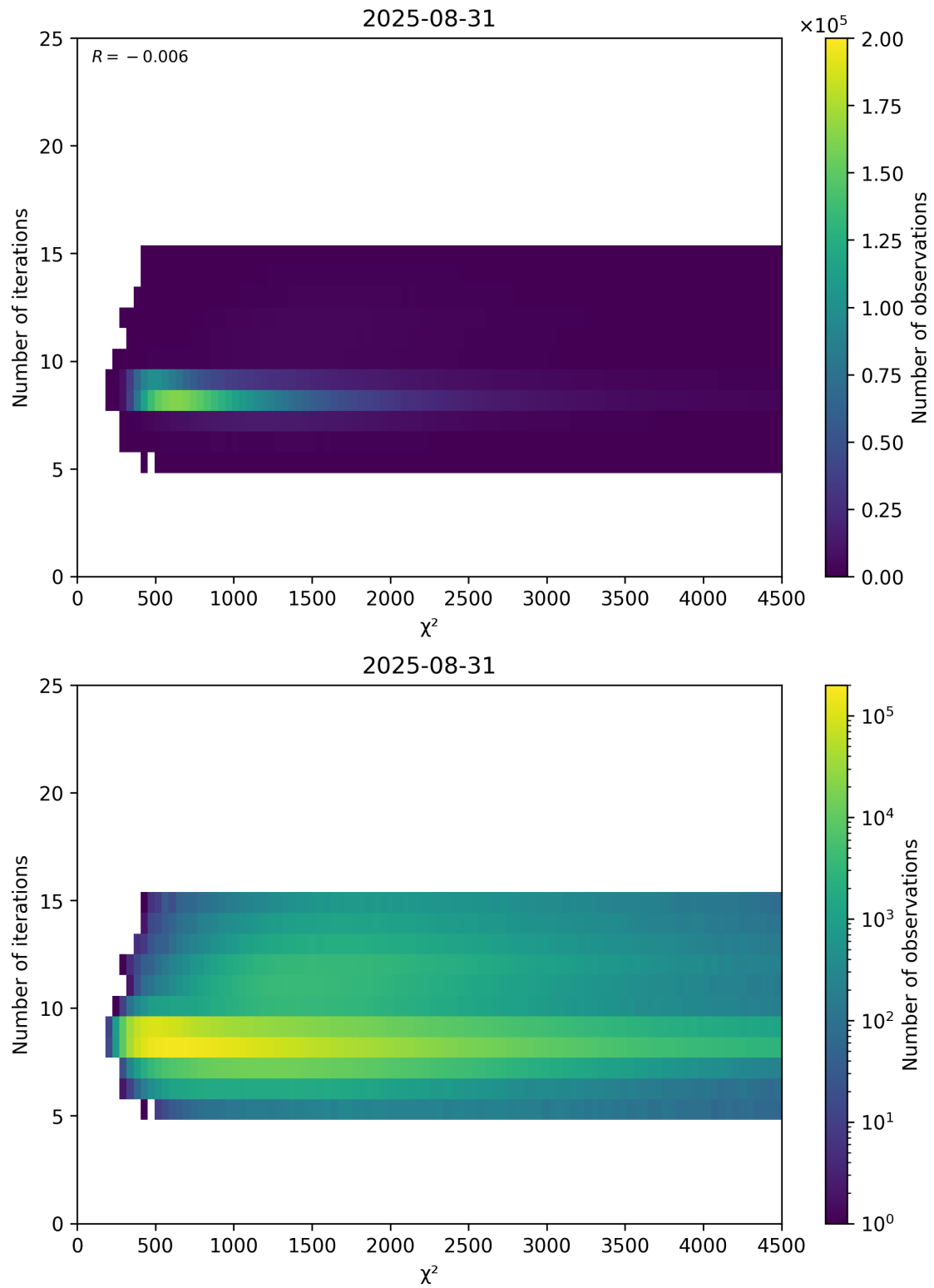
Figure 49: Scatter density plot of “ \chi^2 ” against “Number of iterations” for 2025-08-30 to 2025-09-01.
