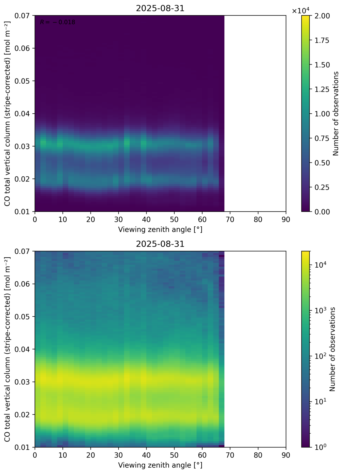
Figure 70: Scatter density plot of “Viewing zenith angle” against “CO total vertical column (stripe-corrected)” for 2025-08-30 to 2025-09-01.
