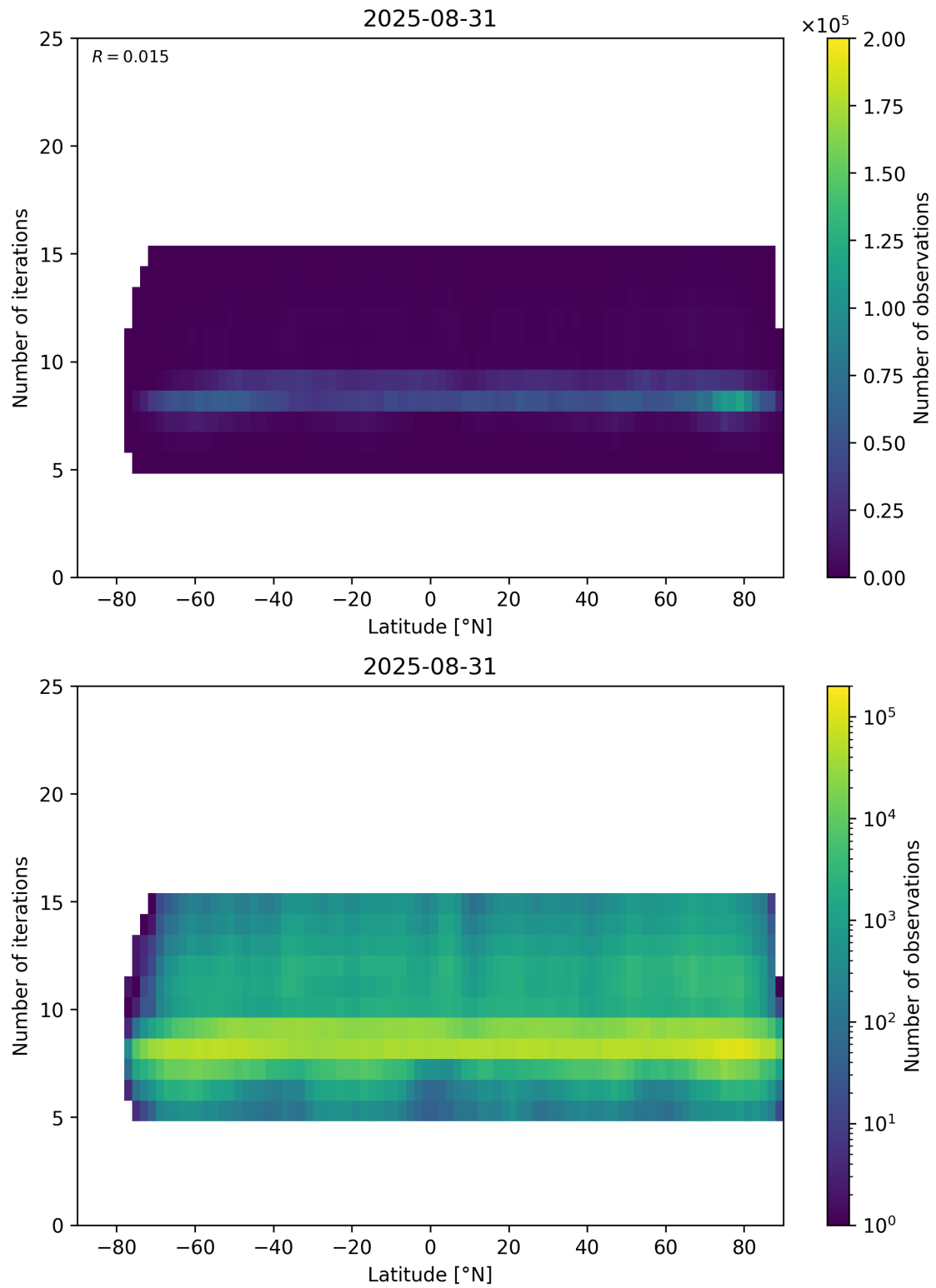
Figure 56: Scatter density plot of “Latitude” against “Number of iterations” for 2025-08-30 to 2025-09-01.
