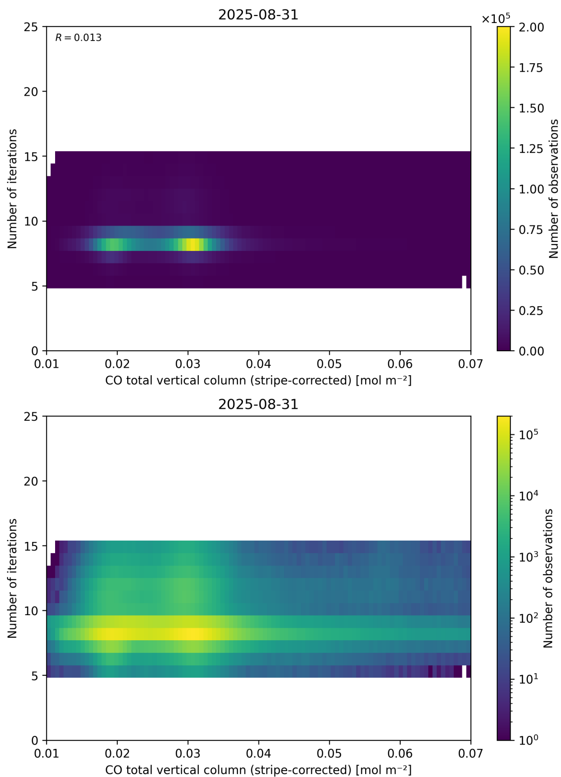
Figure 39: Scatter density plot of “CO total vertical column (stripe-corrected)” against “Number of iterations” for 2025-08-30 to 2025-09-01.
