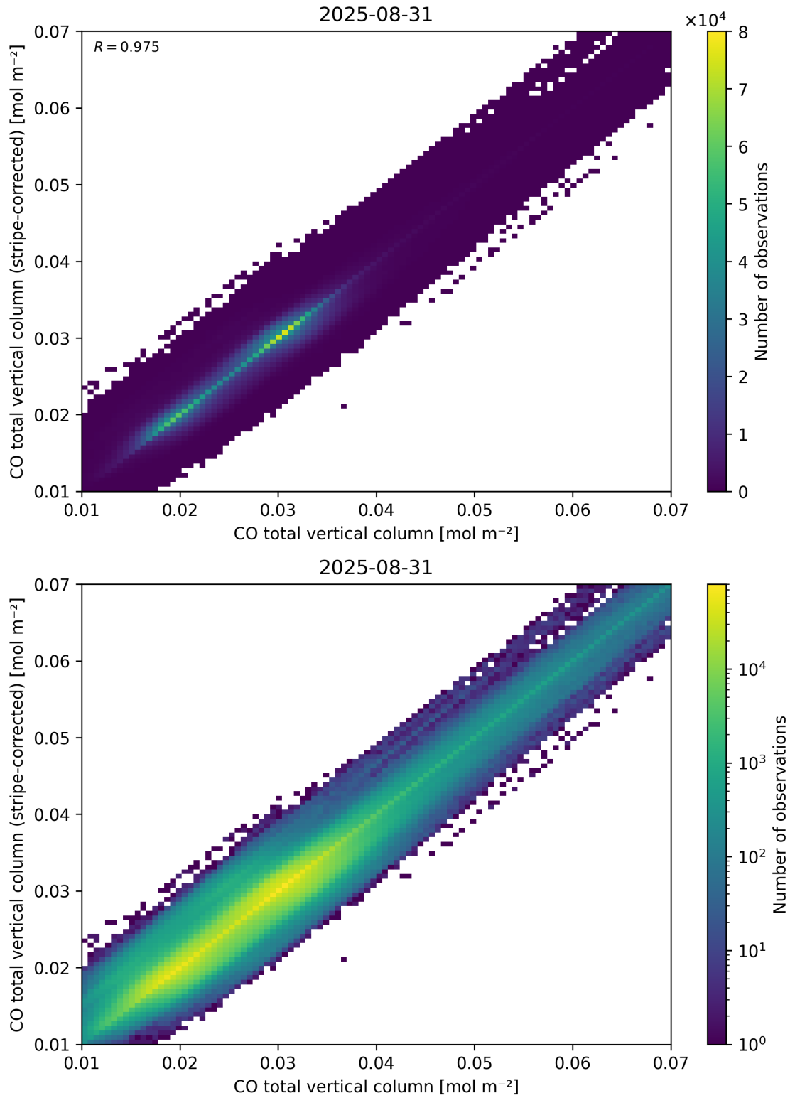
Figure 33: Scatter density plot of “CO total vertical column” against “CO total vertical column (stripe-corrected)” for 2025-08-30 to 2025-09-01.
