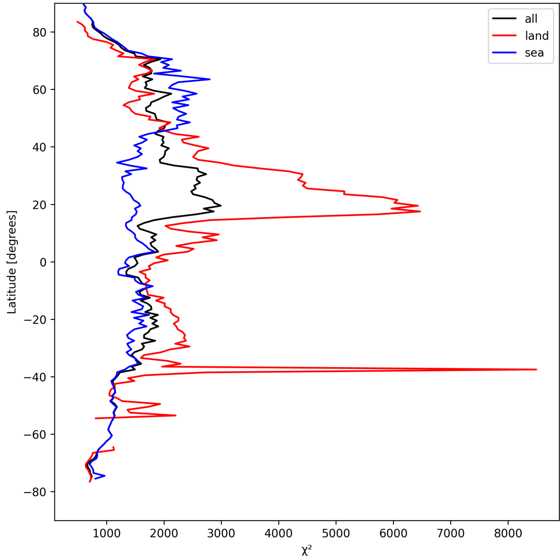
Figure 14: Zonal average of “ \chi^2 ” for 2025-08-30 to 2025-09-01.
