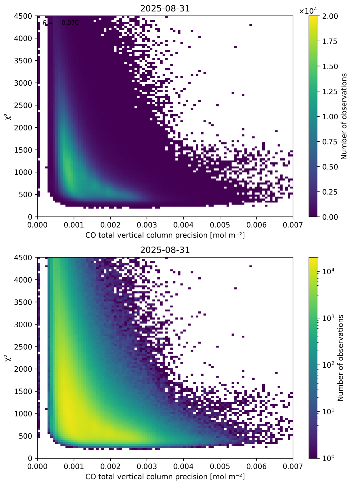
Figure 44: Scatter density plot of “CO total vertical column precision” against “ \chi^2 ” for 2025-08-30 to 2025-09-01.
