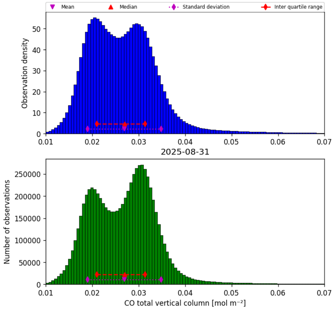
Figure 18: Histogram of “CO total vertical column” for 2025-08-30 to 2025-09-01
