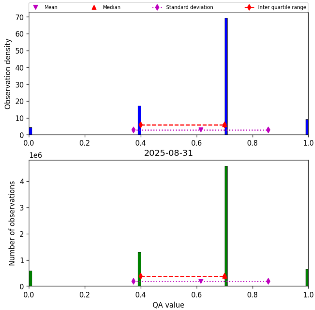
Figure 17: Histogram of “QA value” for 2025-08-30 to 2025-09-01
