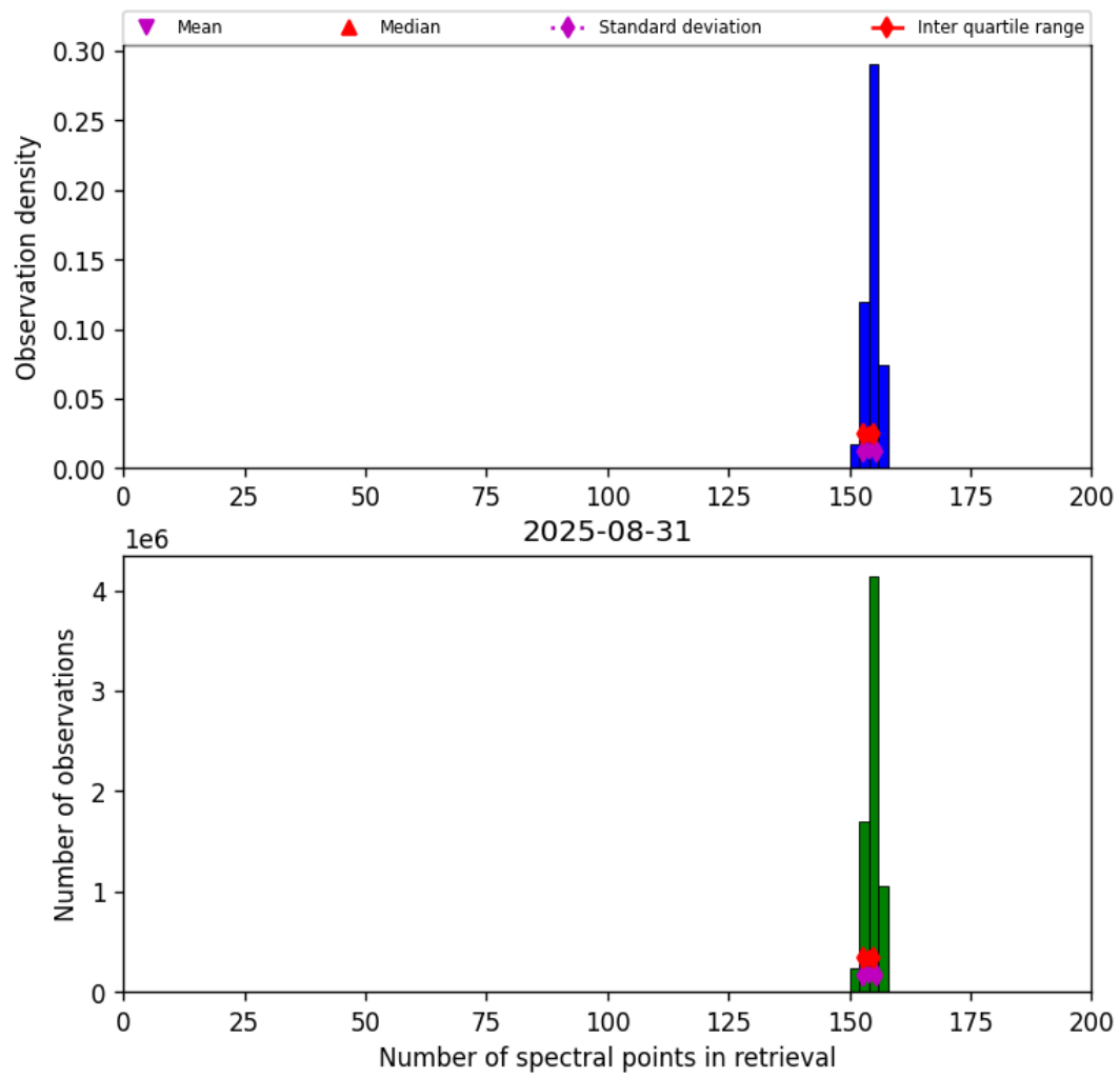
Figure 21: Histogram of “Number of spectral points in retrieval” for 2025-08-30 to 2025-09-01
