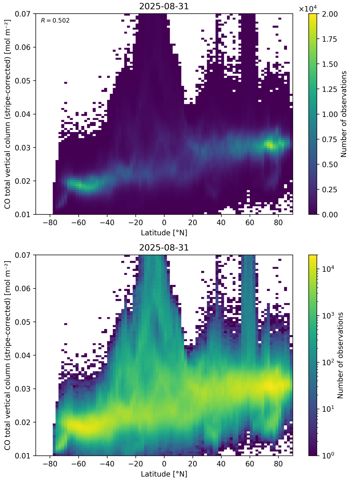
Figure 52: Scatter density plot of “Latitude” against “CO total vertical column (stripe-corrected)” for 2025-08-30 to 2025-09-01.
