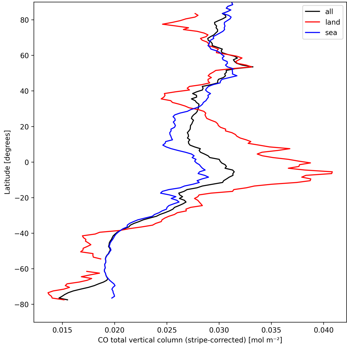
Figure 11: Zonal average of “CO total vertical column (stripe-corrected)” for 2025-09-01 to 2025-09-03.
