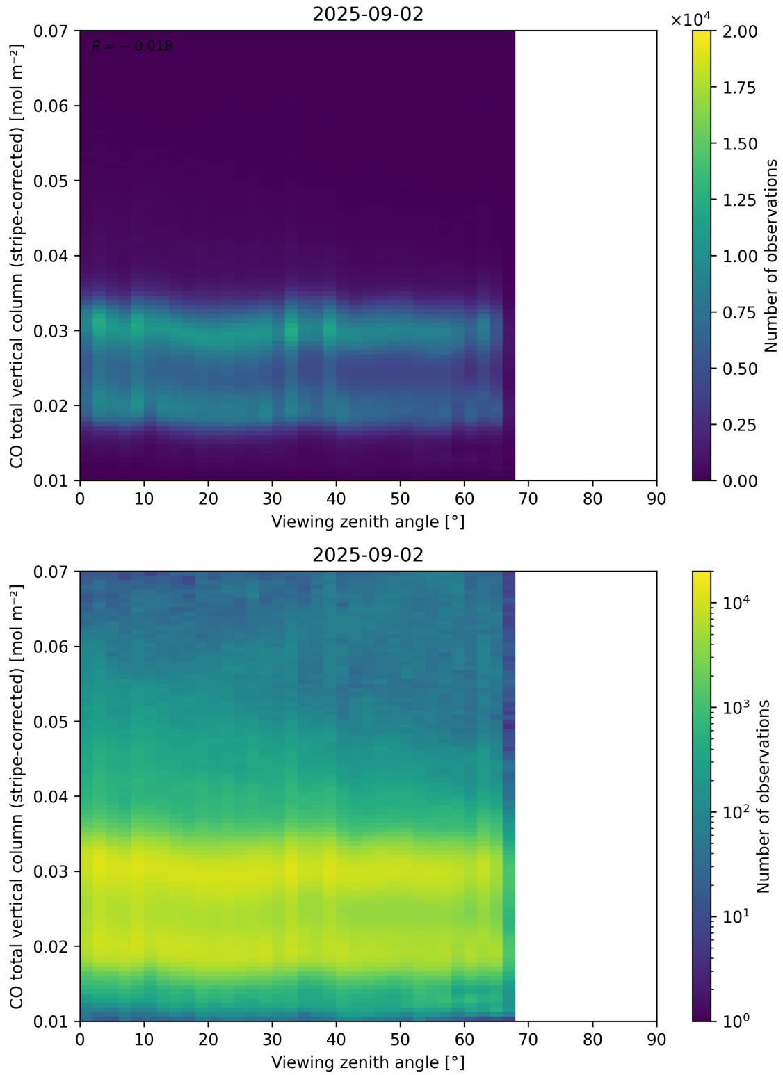
Figure 70: Scatter density plot of “Viewing zenith angle” against “CO total vertical column (stripe-corrected)” for 2025-09-01 to 2025-09-03.
