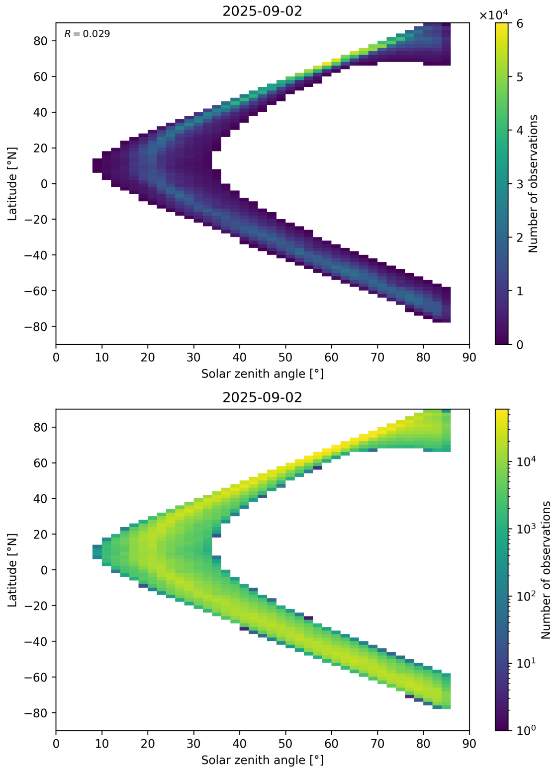
Figure 66: Scatter density plot of “Solar zenith angle” against “Latitude” for 2025-09-01 to 2025-09-03.
