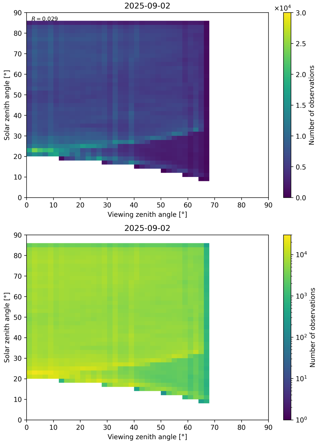
Figure 77: Scatter density plot of “Viewing zenith angle” against “Solar zenith angle” for 2025-09-01 to 2025-09-03.
