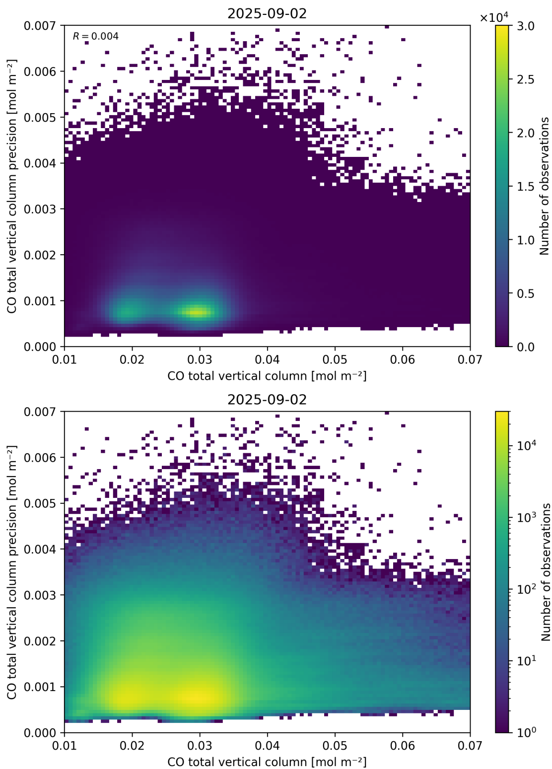
Figure 34: Scatter density plot of “CO total vertical column” against “CO total vertical column precision” for 2025-09-01 to 2025-09-03.
