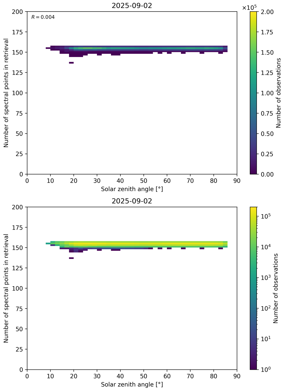
Figure 68: Scatter density plot of “Solar zenith angle” against “Number of spectral points in retrieval” for 2025-09-01 to 2025-09-03.
