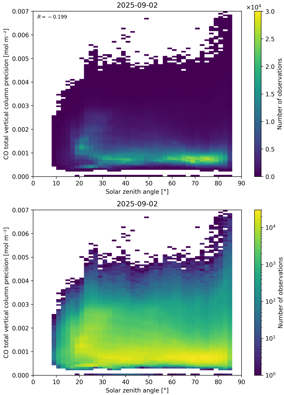
Figure 63: Scatter density plot of “Solar zenith angle” against “CO total vertical column precision” for 2025-09-01 to 2025-09-03.
