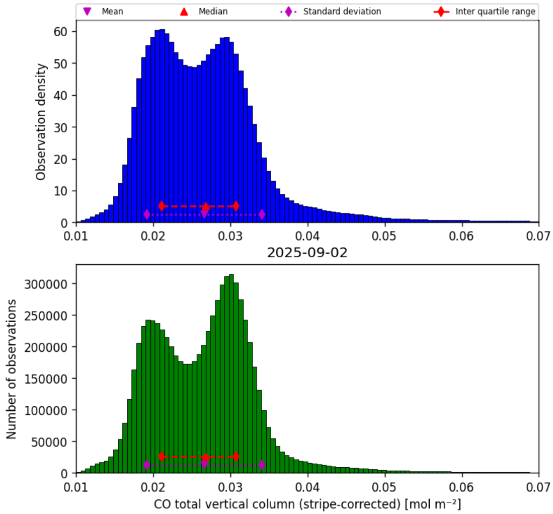
Figure 19: Histogram of “CO total vertical column (stripe-corrected)” for 2025-09-01 to 2025-09-03
