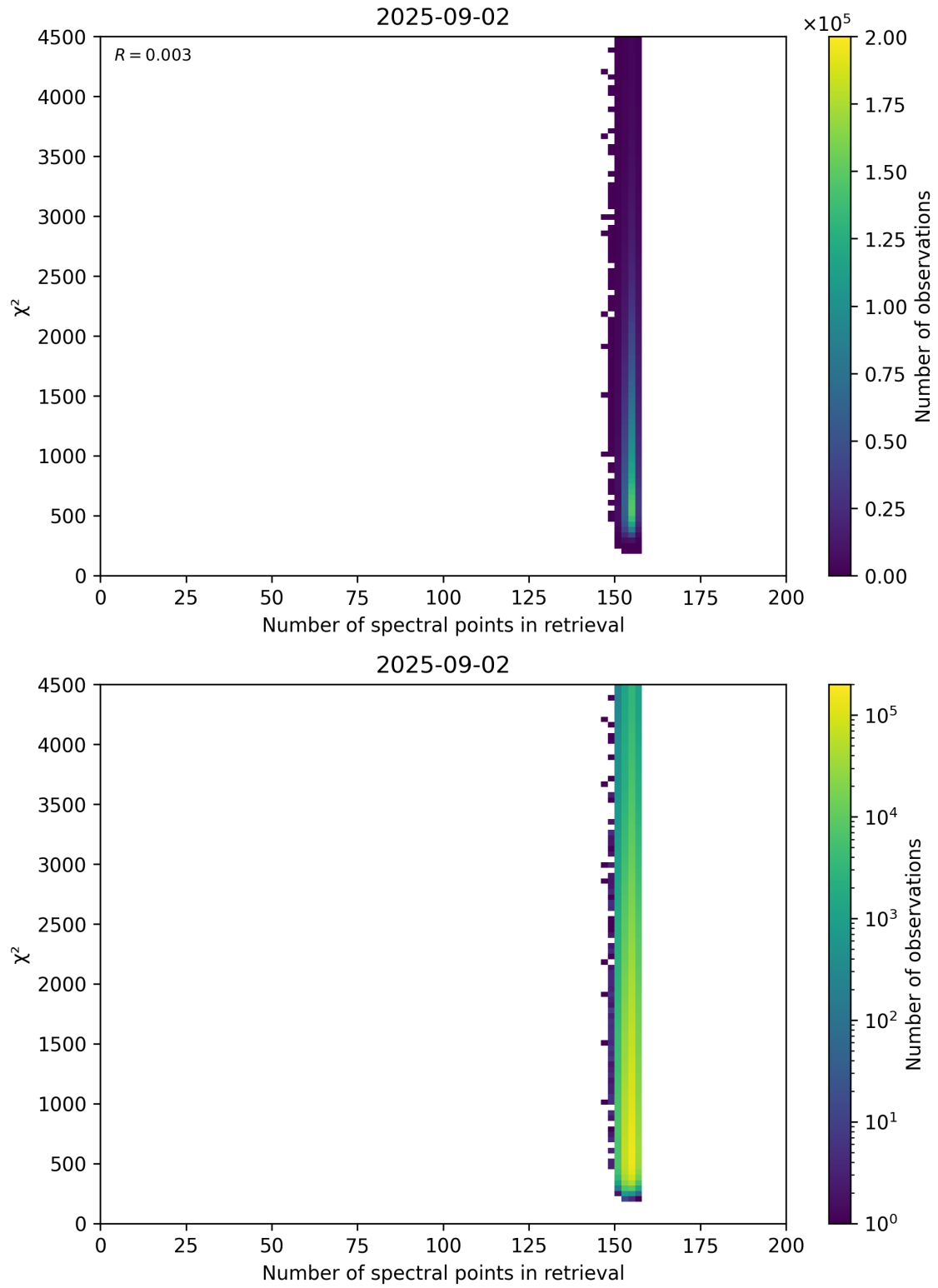
Figure 58: Scatter density plot of “Number of spectral points in retrieval” against “ \chi^2 ” for 2025-09-01 to 2025-09-03.
