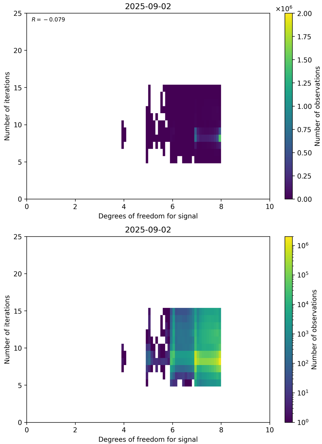
Figure 50: Scatter density plot of “Degrees of freedom for signal” against “Number of iterations” for 2025-09-01 to 2025-09-03.
