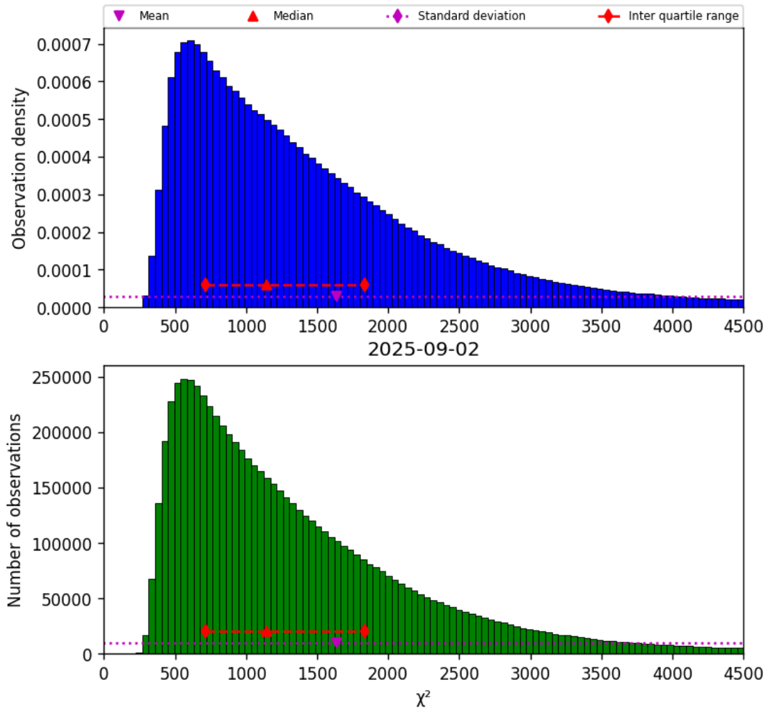
Figure 22: Histogram of " \chi^2 " for 2025-09-01 to 2025-09-03
