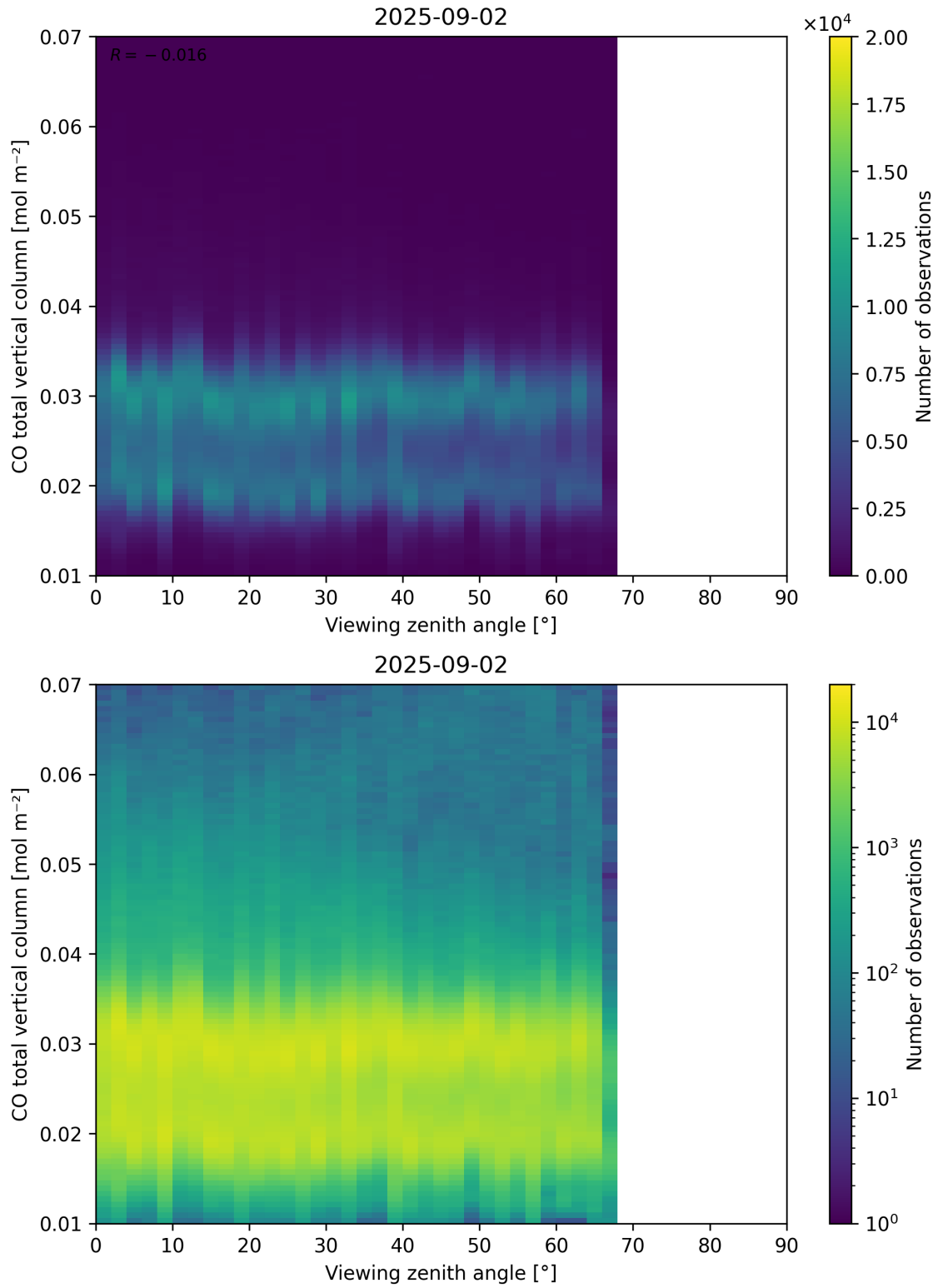
Figure 69: Scatter density plot of “Viewing zenith angle” against “CO total vertical column” for 2025-09-01 to 2025-09-03.
