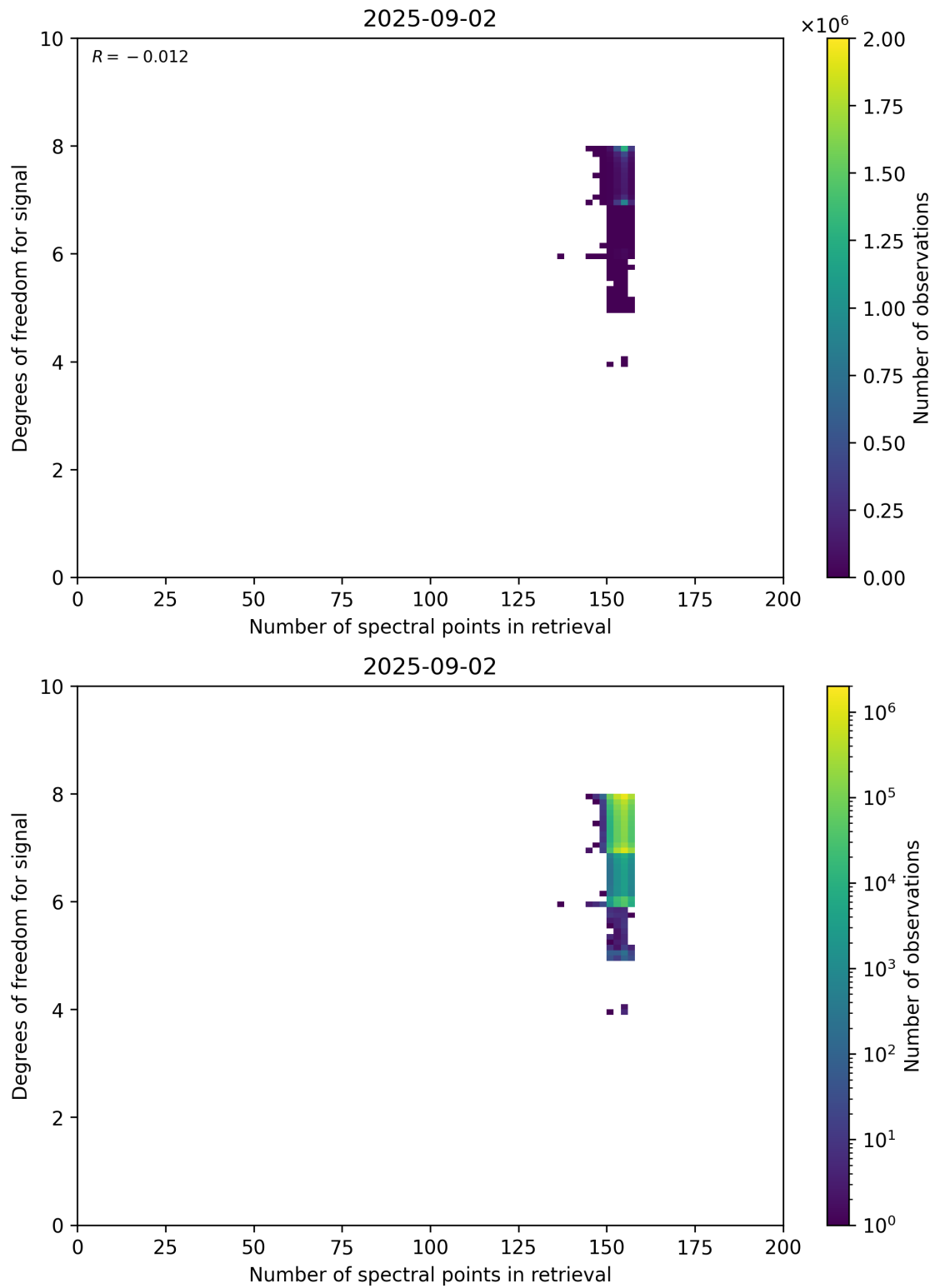
Figure 59: Scatter density plot of “Number of spectral points in retrieval” against “Degrees of freedom for signal” for 2025-09-01 to 2025-09-03.
