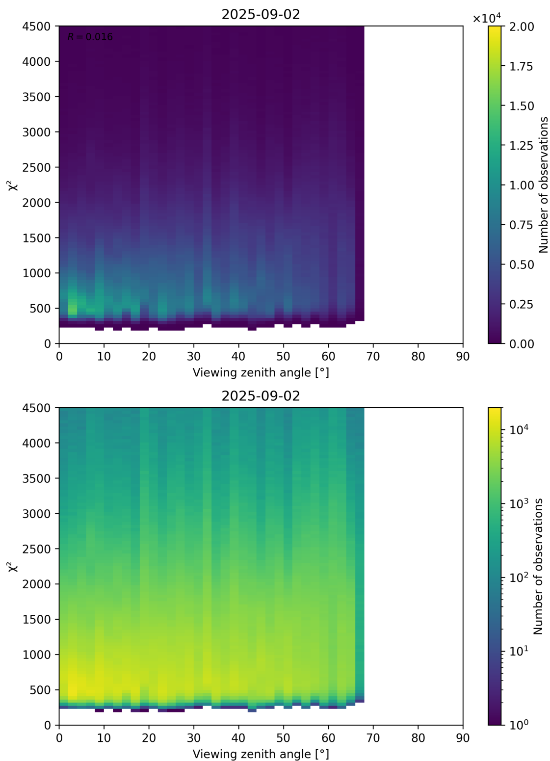
Figure 72: Scatter density plot of “Viewing zenith angle” against “ \chi^2 ” for 2025-09-01 to 2025-09-03.
