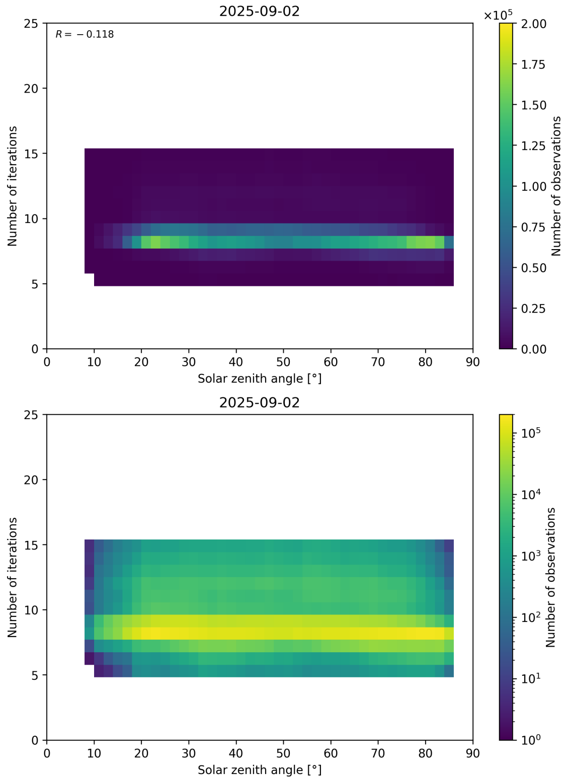
Figure 67: Scatter density plot of “Solar zenith angle” against “Number of iterations” for 2025-09-01 to 2025-09-03.
