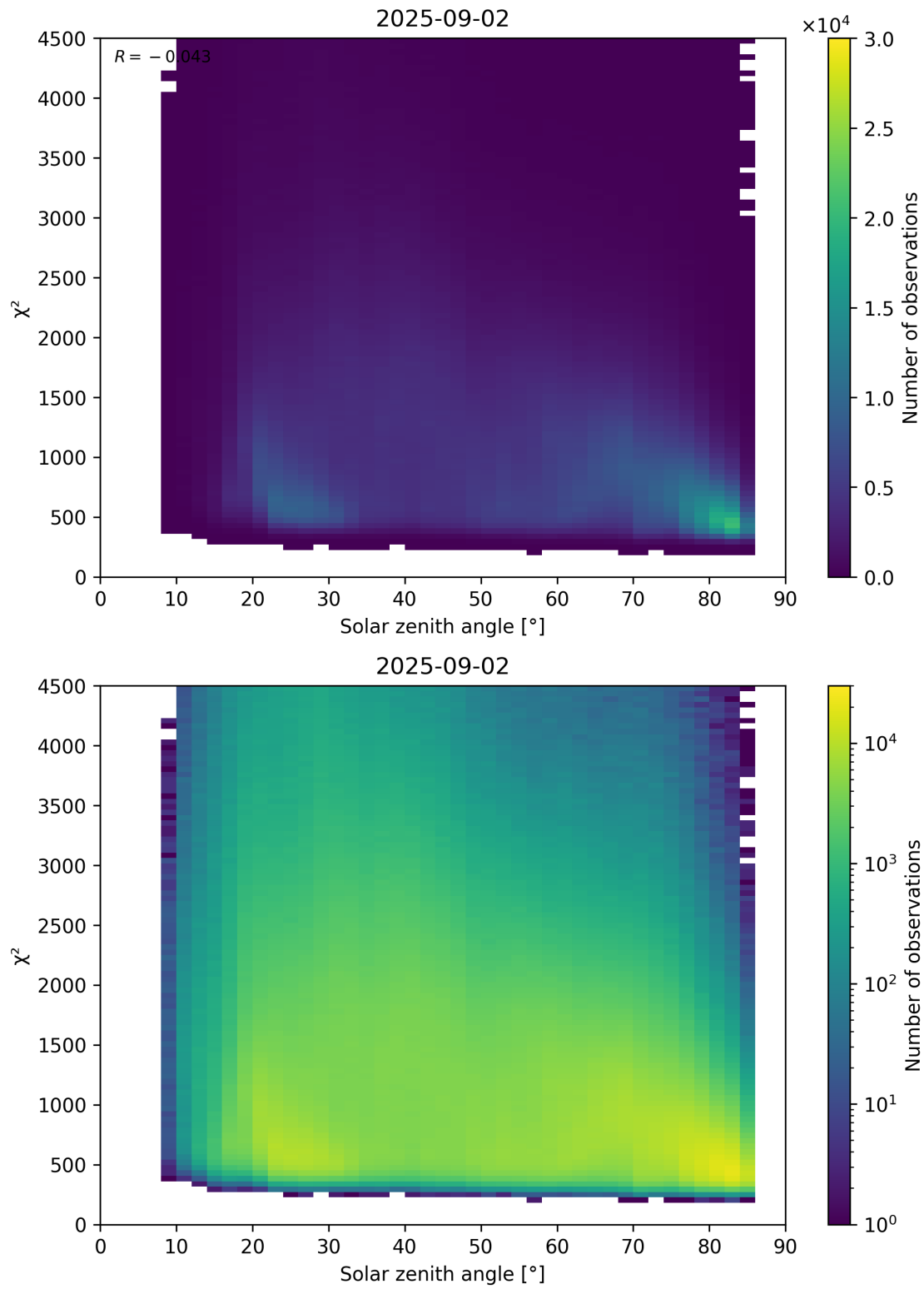
Figure 64: Scatter density plot of “Solar zenith angle” against “ \chi^2 ” for 2025-09-01 to 2025-09-03.
