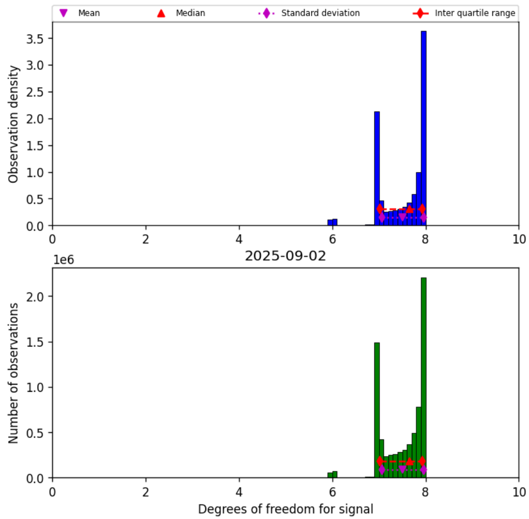
Figure 23: Histogram of “Degrees of freedom for signal” for 2025-09-01 to 2025-09-03
