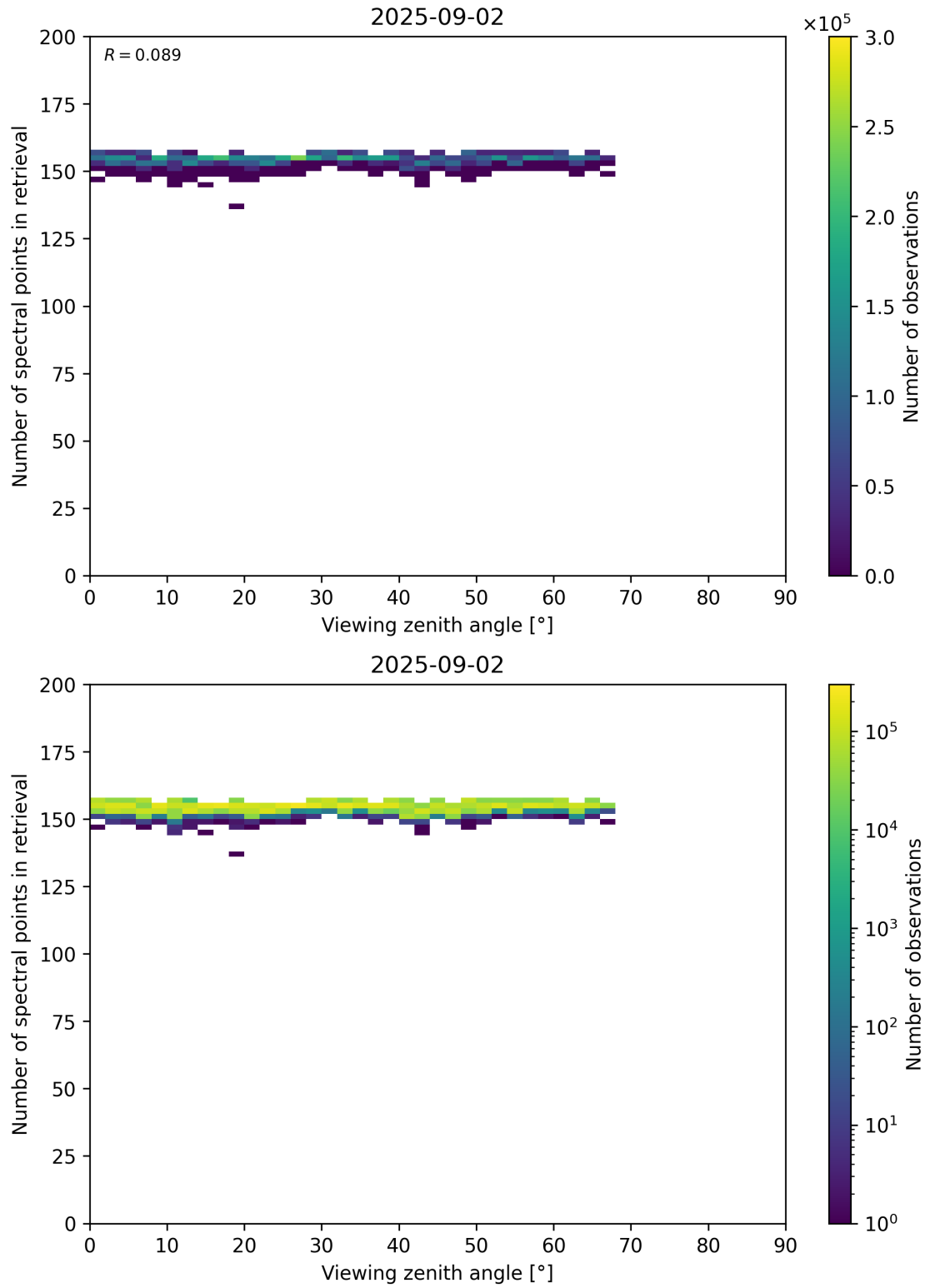
Figure 76: Scatter density plot of “Viewing zenith angle” against “Number of spectral points in retrieval” for 2025-09-01 to 2025-09-03.
