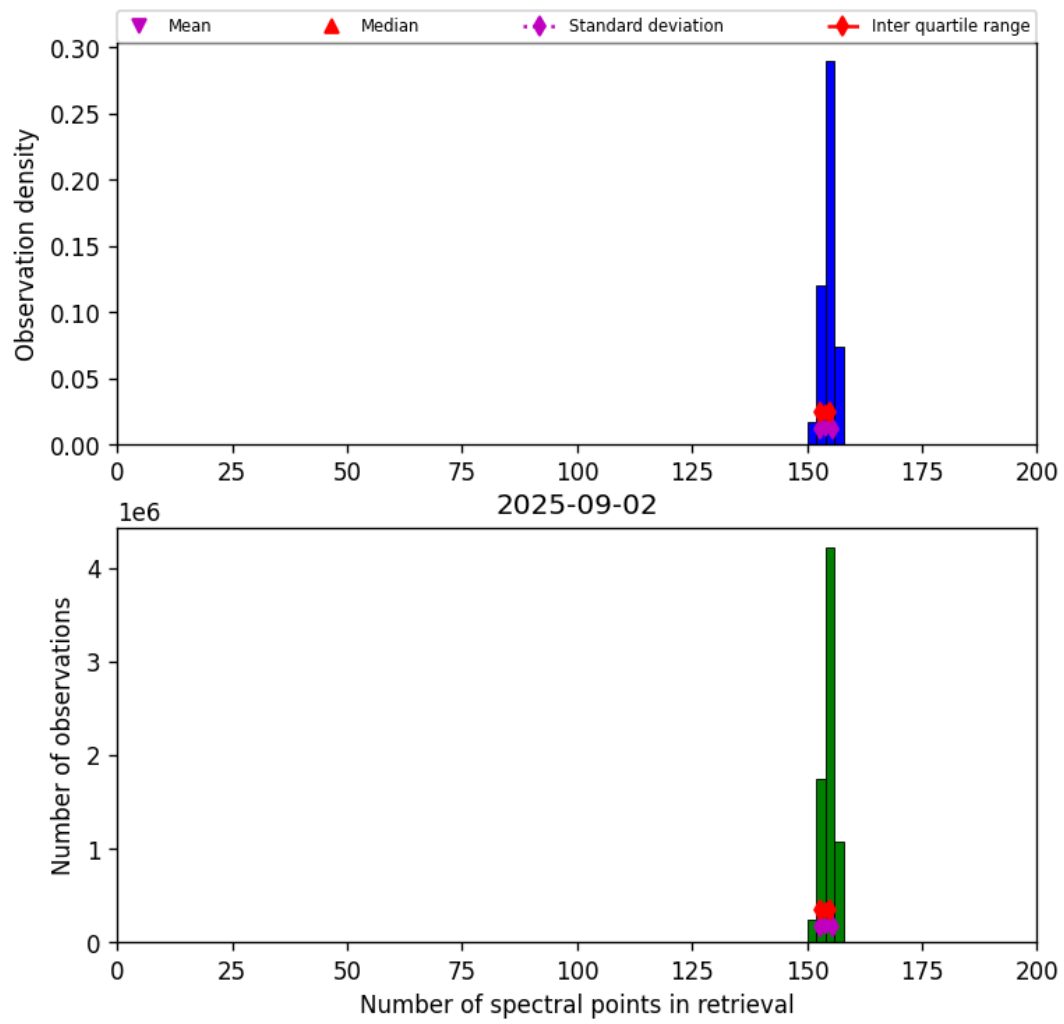
Figure 21: Histogram of “Number of spectral points in retrieval” for 2025-09-01 to 2025-09-03
