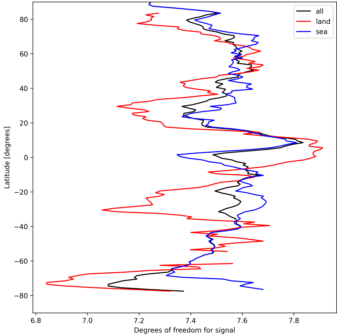
Figure 15: Zonal average of “Degrees of freedom for signal” for 2025-09-01 to 2025-09-03.
