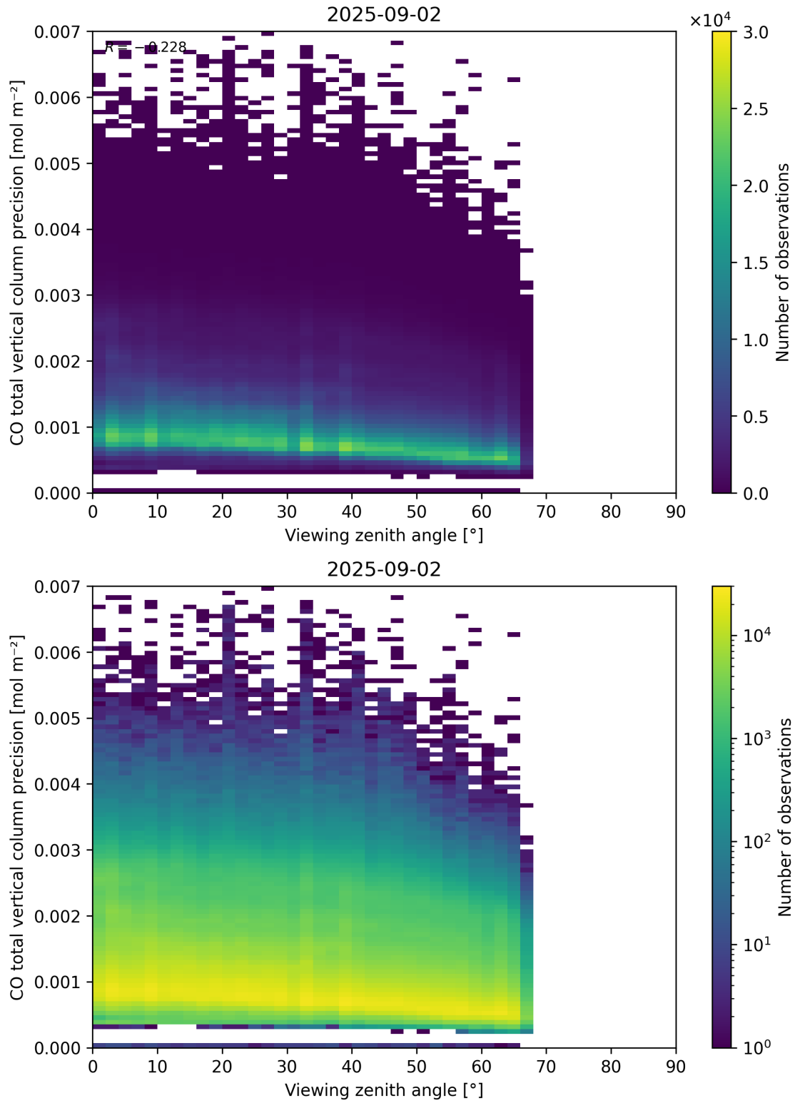
Figure 71: Scatter density plot of “Viewing zenith angle” against “CO total vertical column precision” for 2025-09-01 to 2025-09-03.
