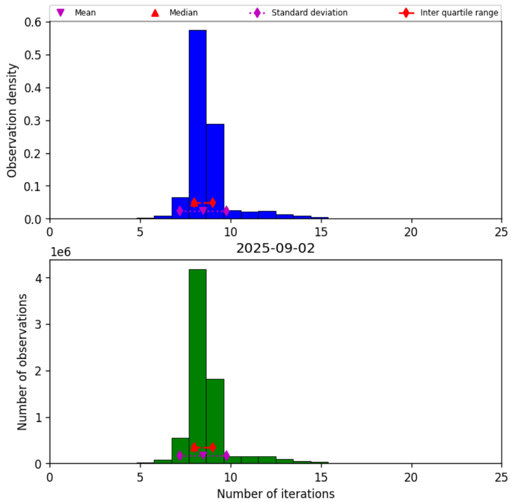
Figure 24: Histogram of “Number of iterations” for 2025-09-01 to 2025-09-03
