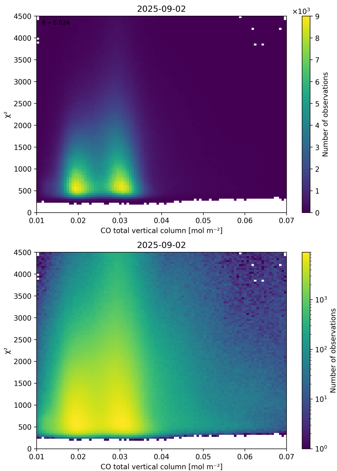
Figure 35: Scatter density plot of “CO total vertical column” against “ \chi^2 ” for 2025-09-01 to 2025-09-03.
