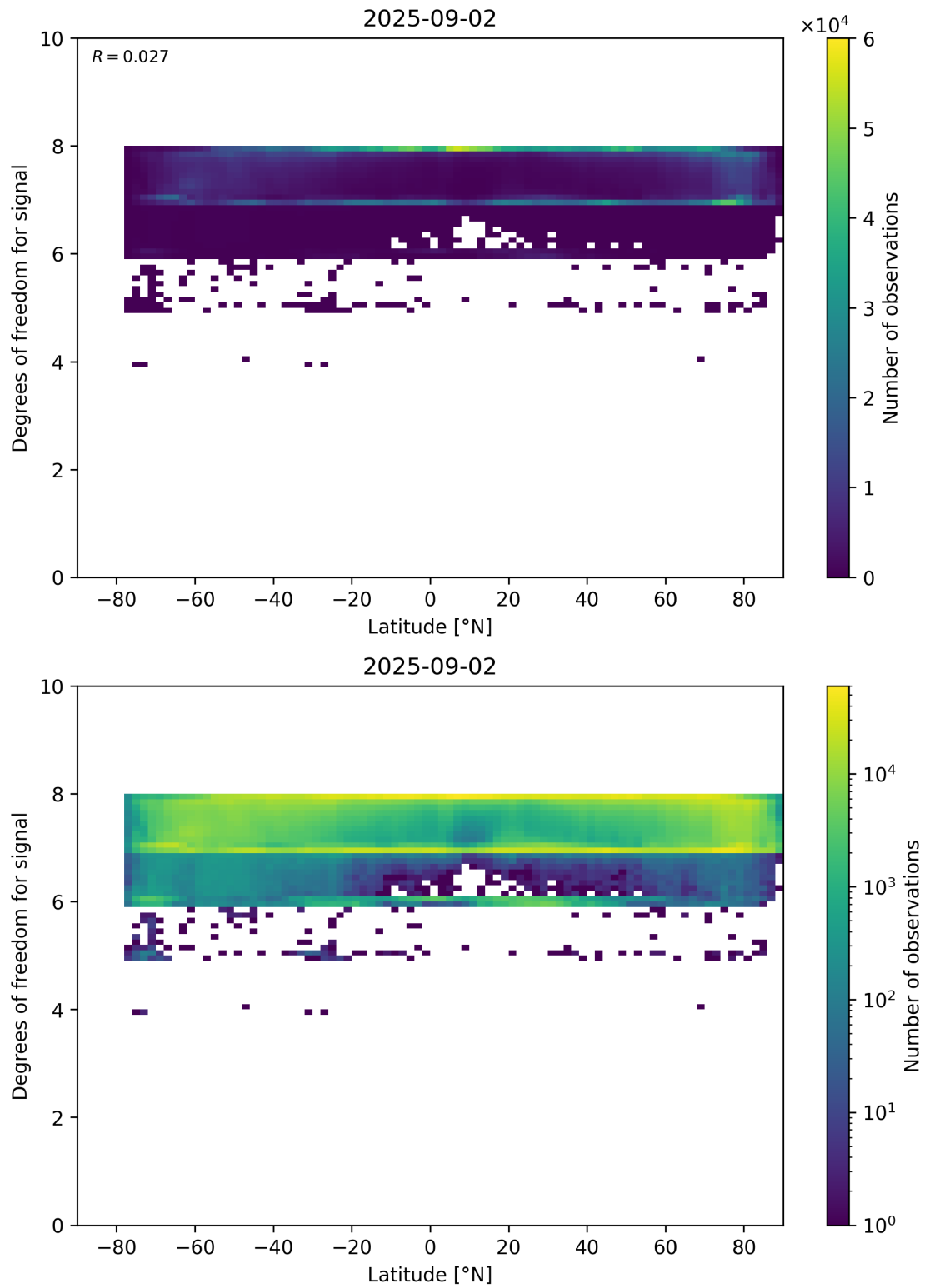
Figure 55: Scatter density plot of “Latitude” against “Degrees of freedom for signal” for 2025-09-01 to 2025-09-03.
