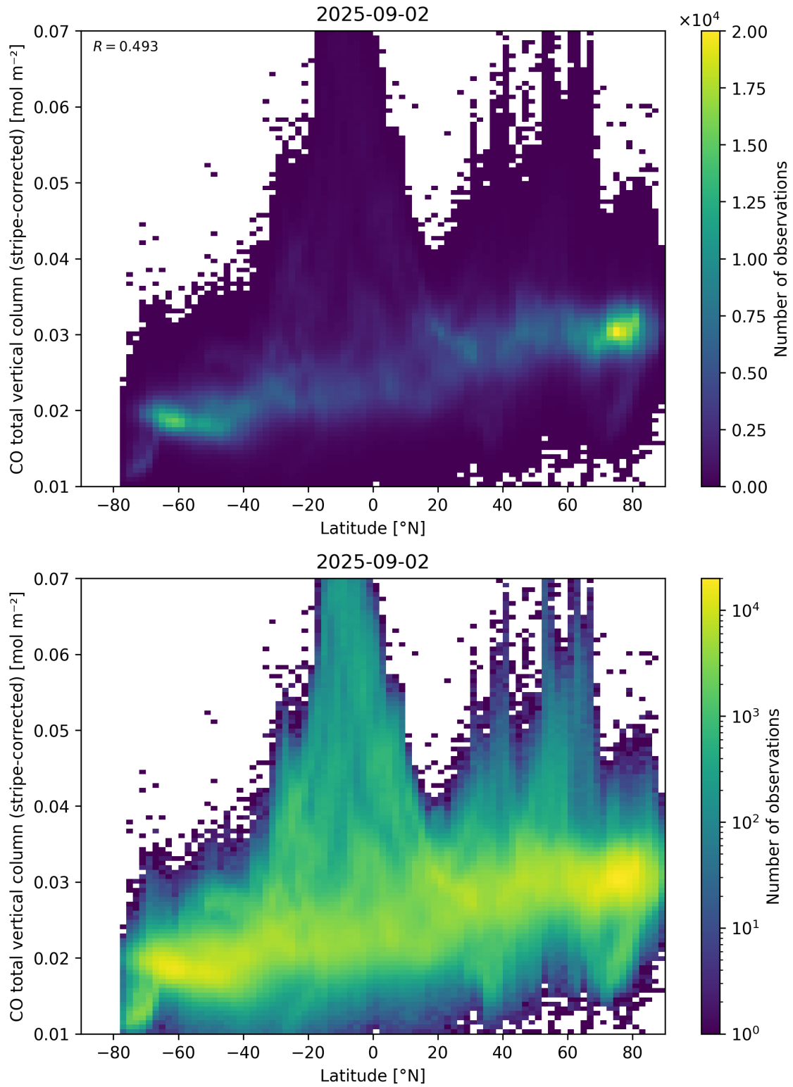
Figure 52: Scatter density plot of “Latitude” against “CO total vertical column (stripe-corrected)” for 2025-09-01 to 2025-09-03.
