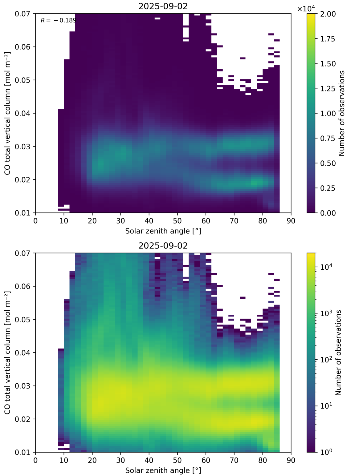
Figure 61: Scatter density plot of “Solar zenith angle” against “CO total vertical column” for 2025-09-01 to 2025-09-03.
