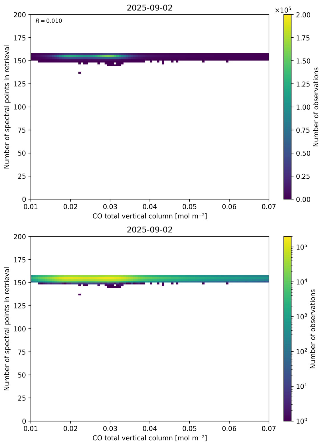
Figure 43: Scatter density plot of “CO total vertical column” against “Number of spectral points in retrieval” for 2025-09-01 to 2025-09-03.
