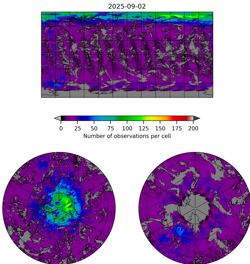
Figure 8: Map of the number of observations for 2025-09-01 to 2025-09-03
