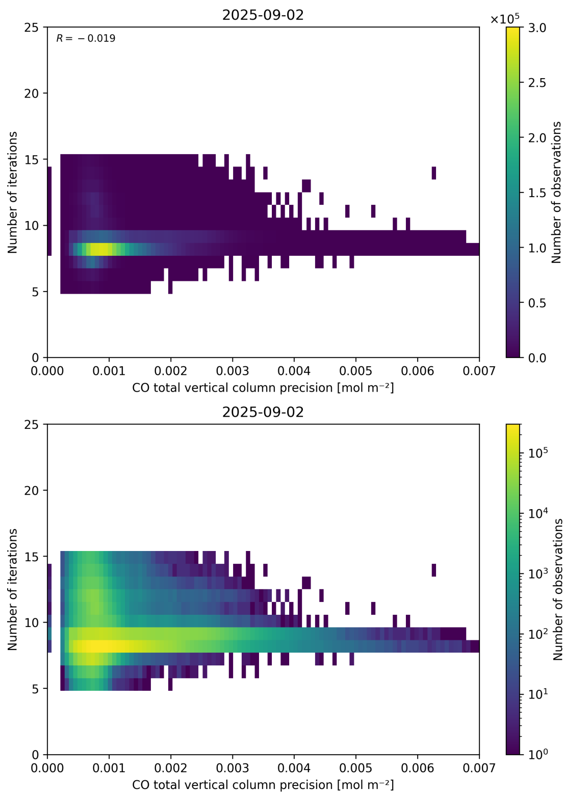
Figure 46: Scatter density plot of “CO total vertical column precision” against “Number of iterations” for 2025-09-01 to 2025-09-03.
