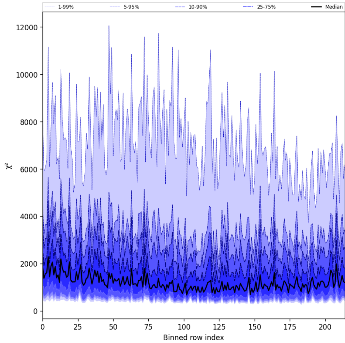
Figure 30: Along track statistics of “ \chi^2 ” for 2025-09-01 to 2025-09-03
