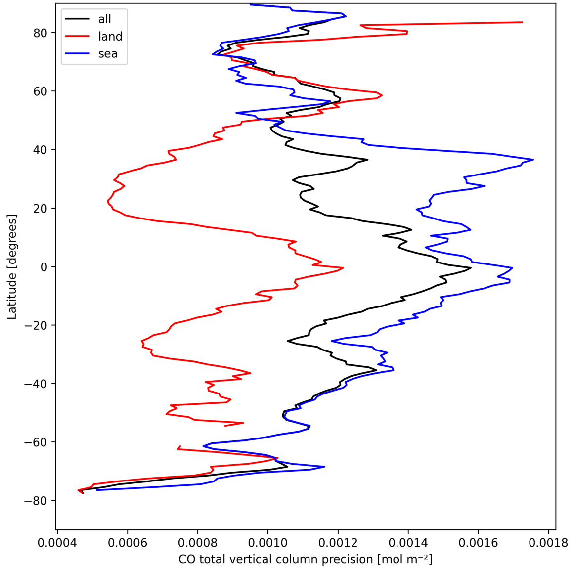
Figure 12: Zonal average of “CO total vertical column precision” for 2025-09-01 to 2025-09-03.
