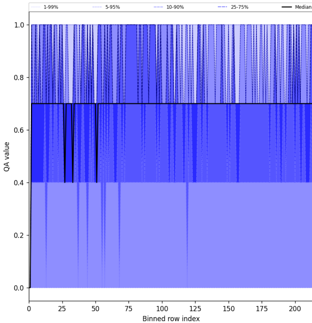
Figure 25: Along track statistics of “QA value” for 2025-09-01 to 2025-09-03
