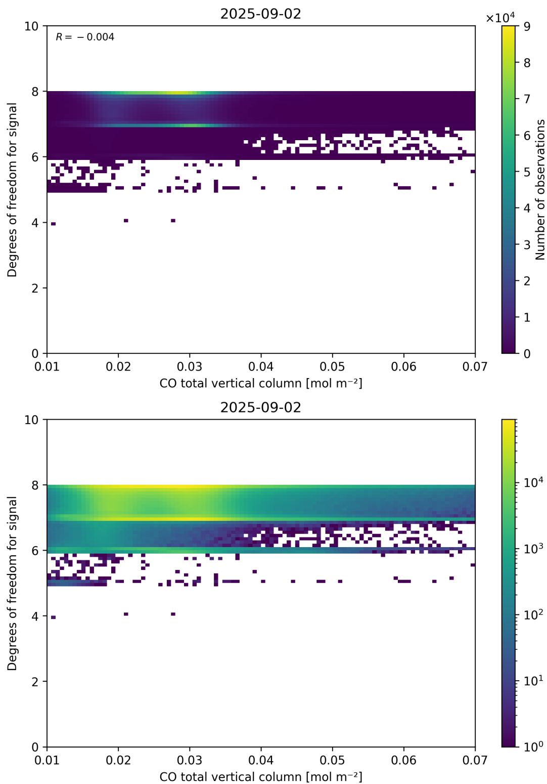
Figure 41: Scatter density plot of “CO total vertical column” against “Degrees of freedom for signal” for 2025-09-01 to 2025-09-03.
