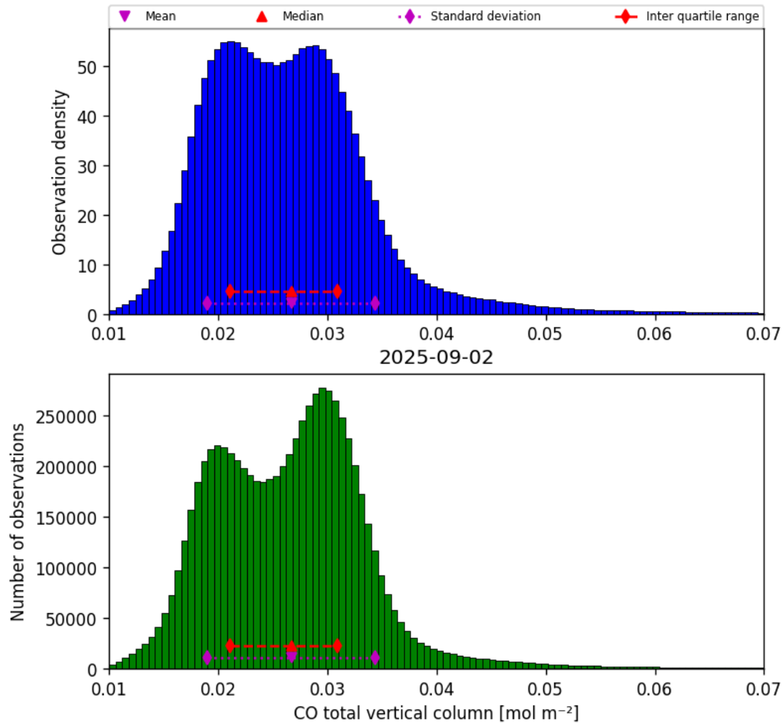
Figure 18: Histogram of “CO total vertical column” for 2025-09-01 to 2025-09-03
