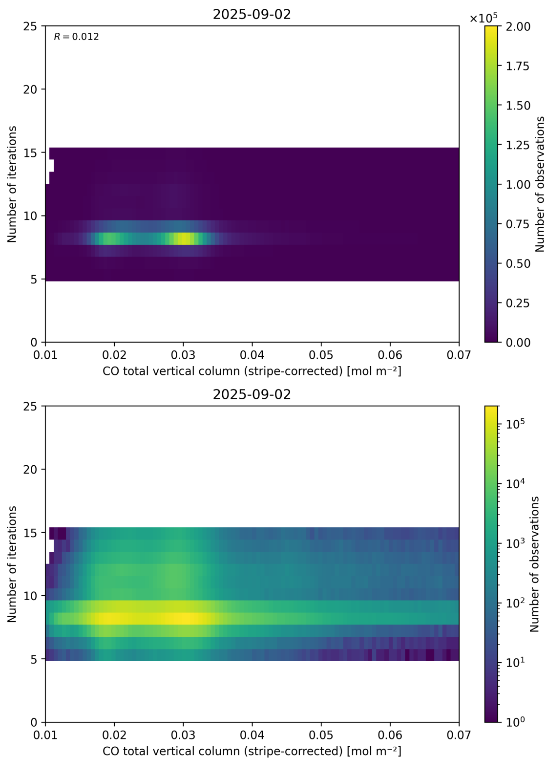
Figure 39: Scatter density plot of “CO total vertical column (stripe-corrected)” against “Number of iterations” for 2025-09-01 to 2025-09-03.
