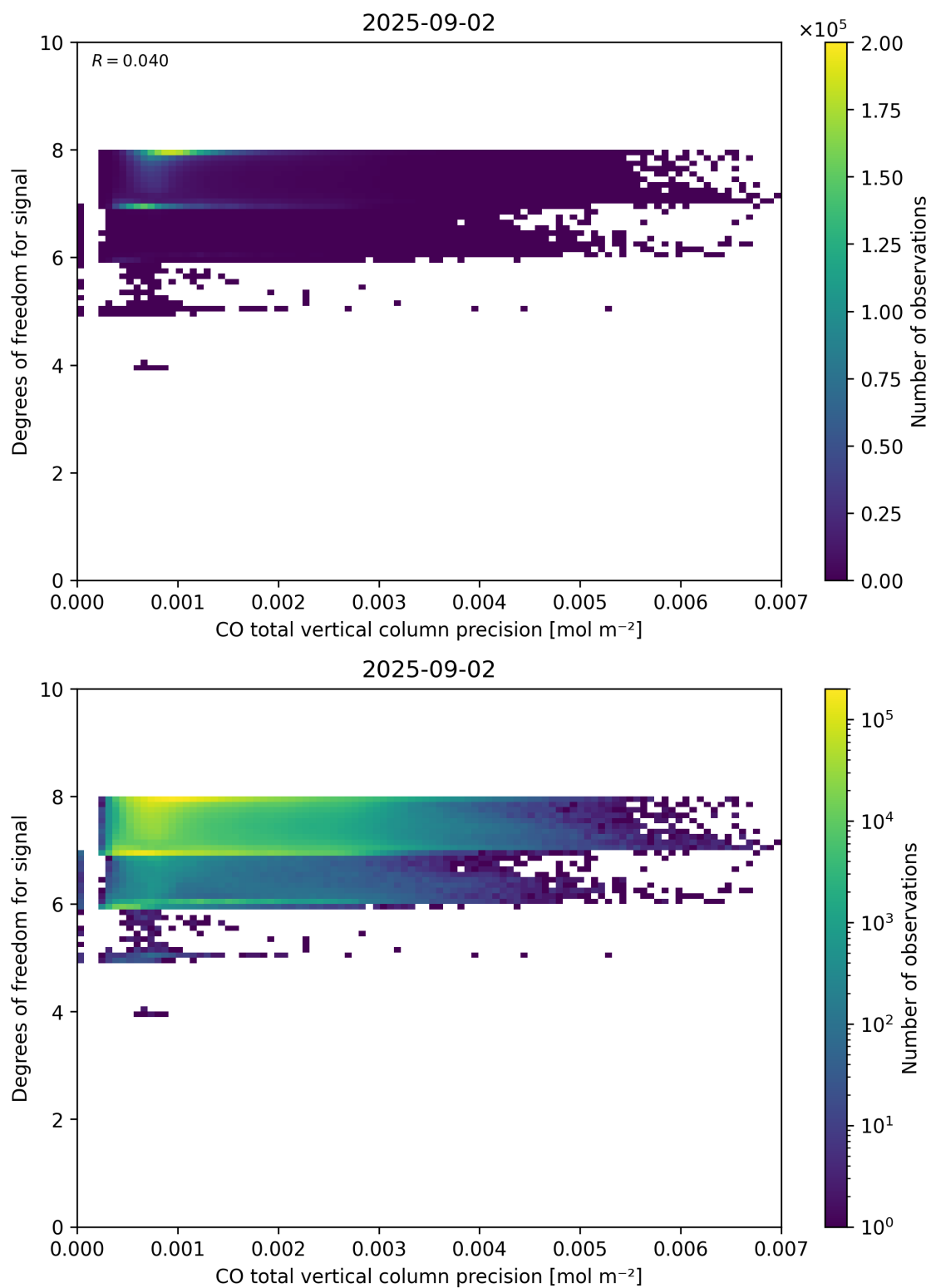
Figure 45: Scatter density plot of “CO total vertical column precision” against “Degrees of freedom for signal” for 2025-09-01 to 2025-09-03.
