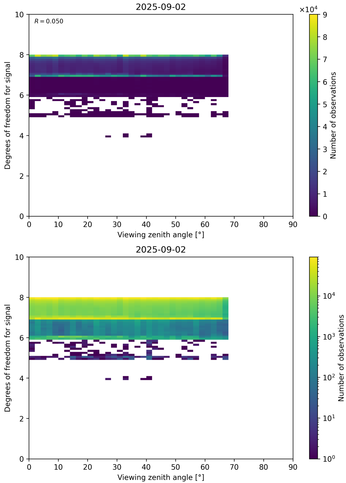
Figure 73: Scatter density plot of “Viewing zenith angle” against “Degrees of freedom for signal” for 2025-09-01 to 2025-09-03.
