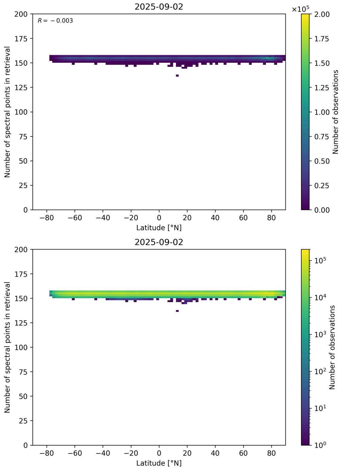
Figure 57: Scatter density plot of “Latitude” against “Number of spectral points in retrieval” for 2025-09-01 to 2025-09-03.
