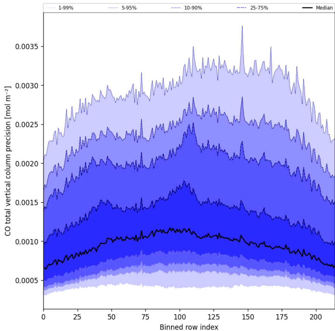
Figure 28: Along track statistics of “CO total vertical column precision” for 2025-09-01 to 2025-09-03
