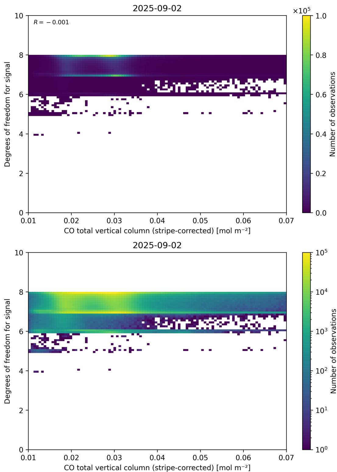
Figure 38: Scatter density plot of “CO total vertical column (stripe-corrected)” against “Degrees of freedom for signal” for 2025-09-01 to 2025-09-03.
