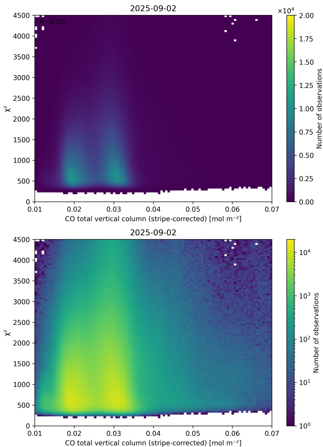
Figure 37: Scatter density plot of “CO total vertical column (stripe-corrected)” against “ \chi^2 ” for 2025-09-01 to 2025-09-03.
