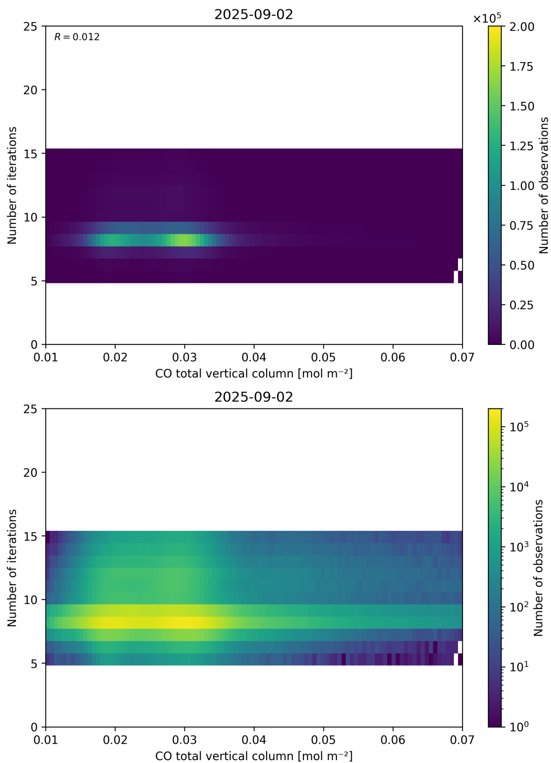
Figure 42: Scatter density plot of “CO total vertical column” against “Number of iterations” for 2025-09-01 to 2025-09-03.
