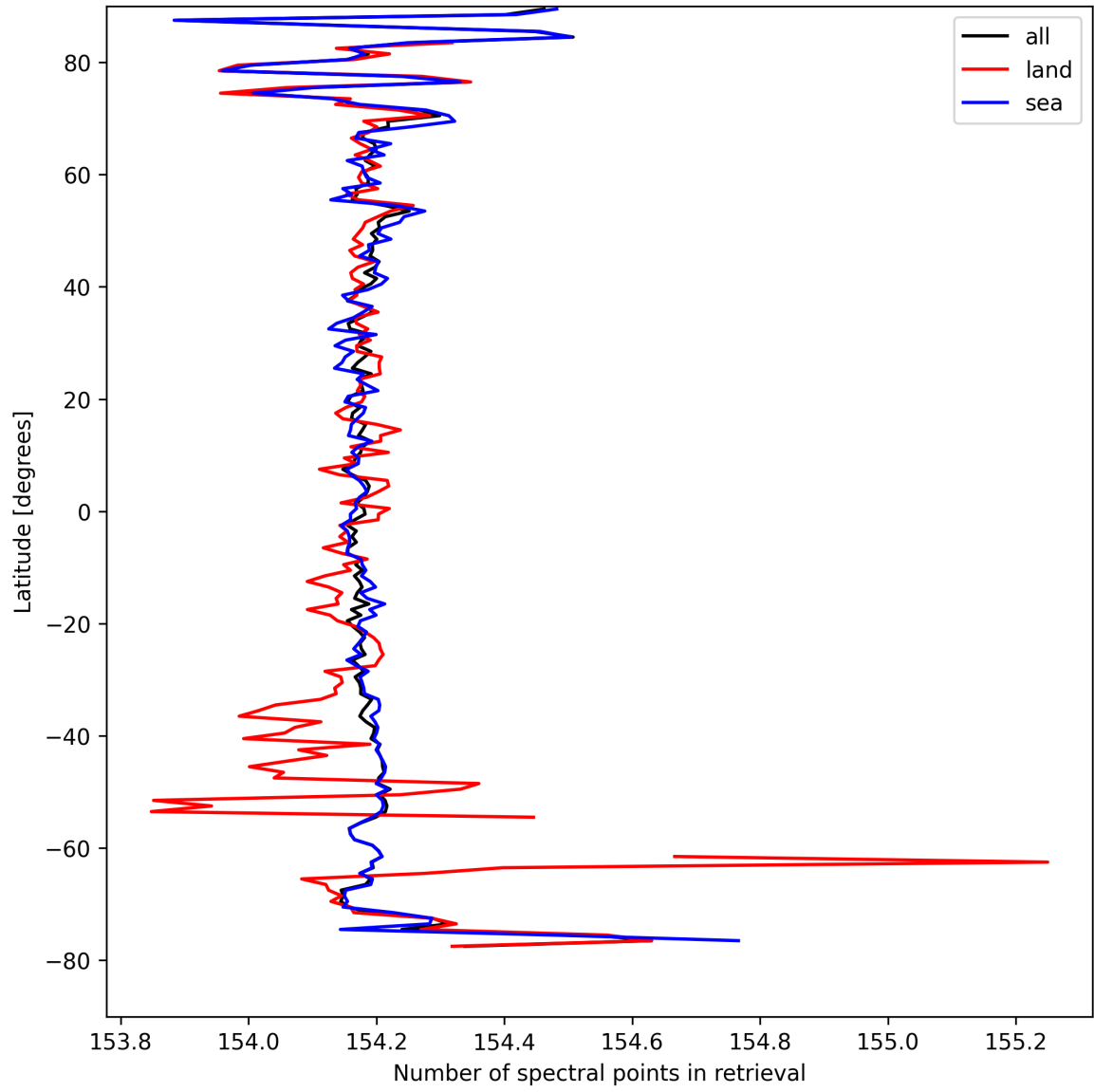
Figure 13: Zonal average of “Number of spectral points in retrieval” for 2025-09-01 to 2025-09-03.
