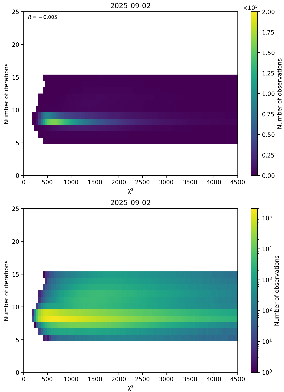
Figure 49: Scatter density plot of “ \chi^2 ” against “Number of iterations” for 2025-09-01 to 2025-09-03.
