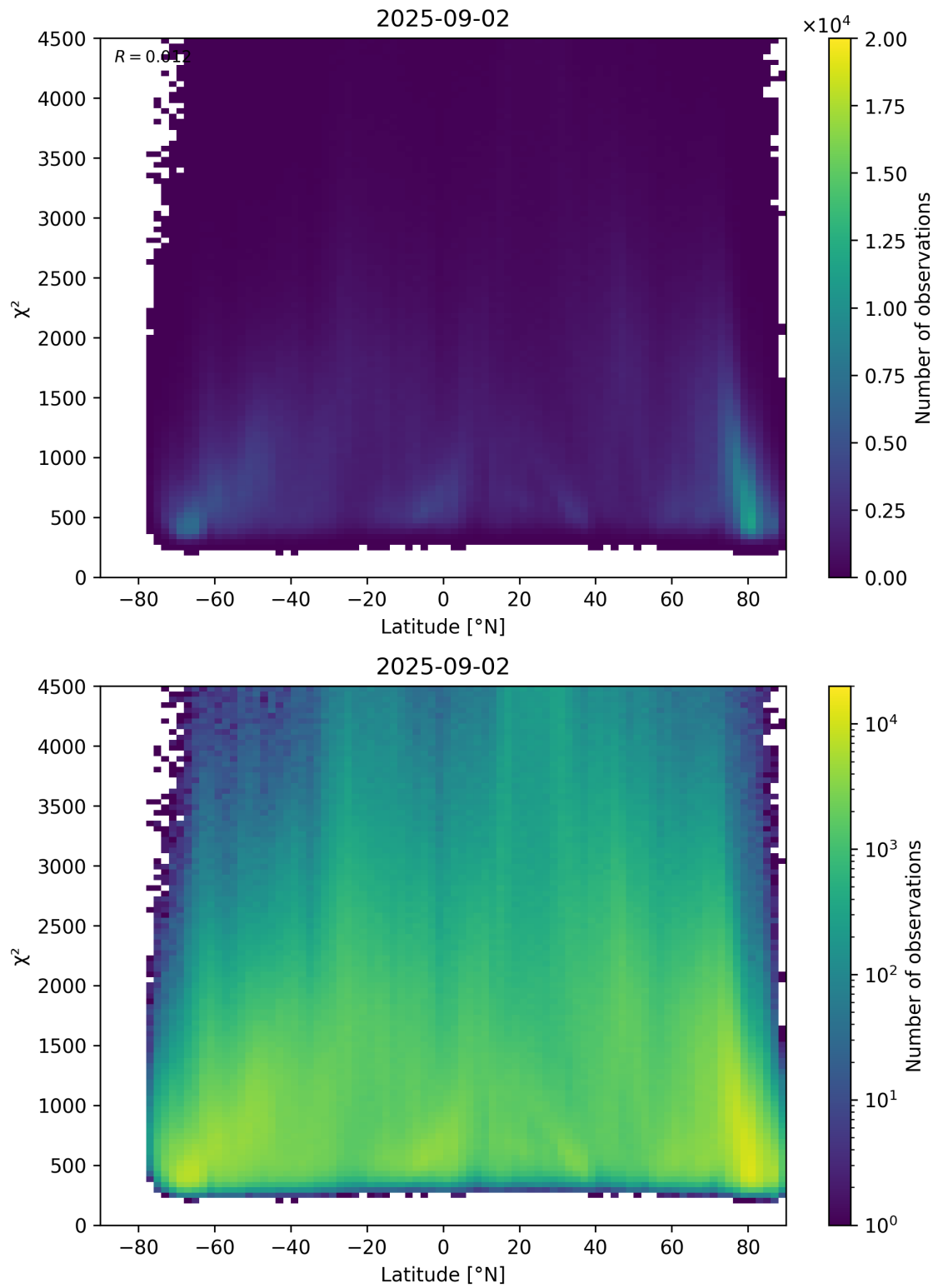
Figure 54: Scatter density plot of “Latitude” against “ \chi^2 ” for 2025-09-01 to 2025-09-03.
