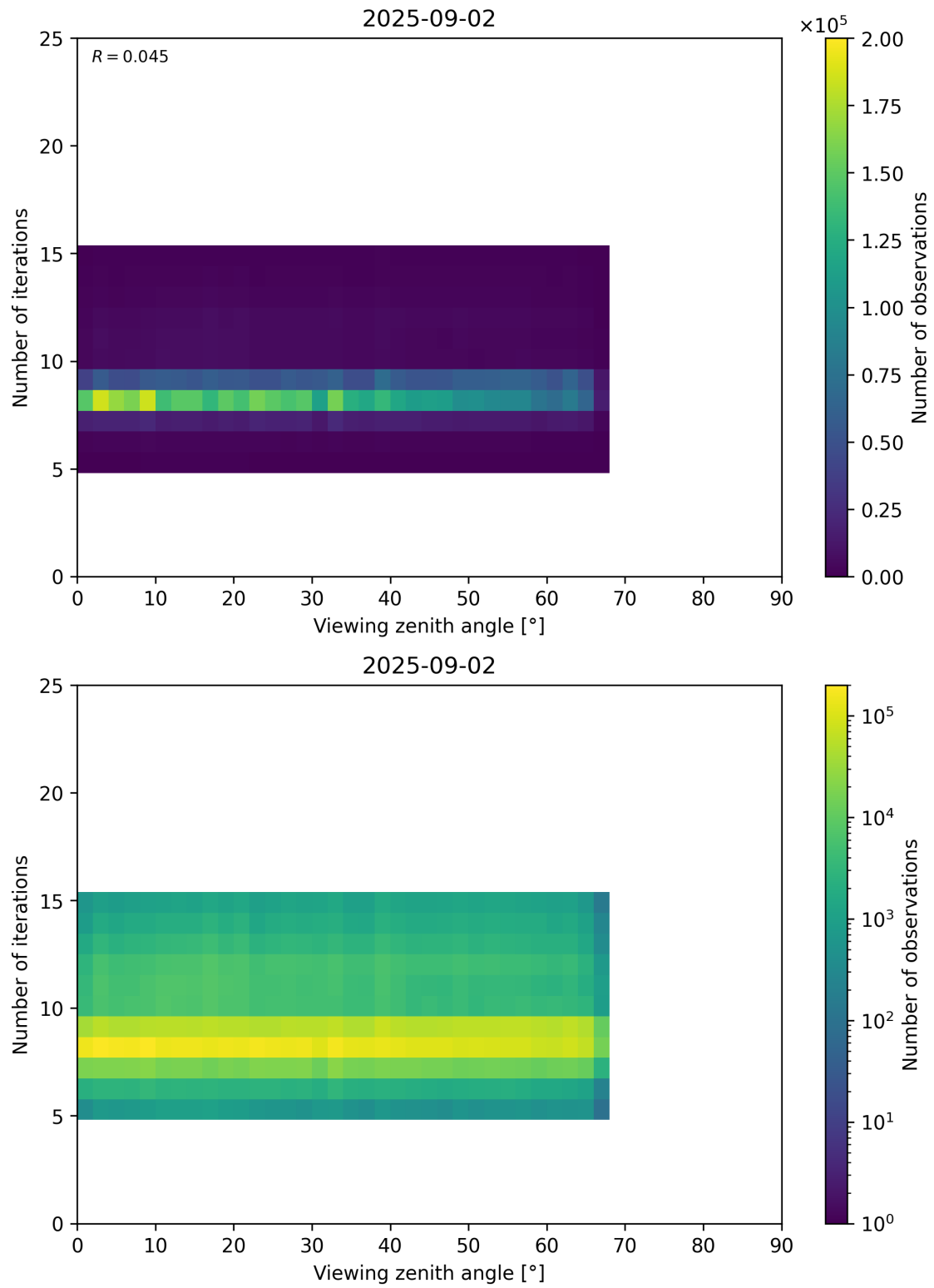
Figure 75: Scatter density plot of “Viewing zenith angle” against “Number of iterations” for 2025-09-01 to 2025-09-03.
