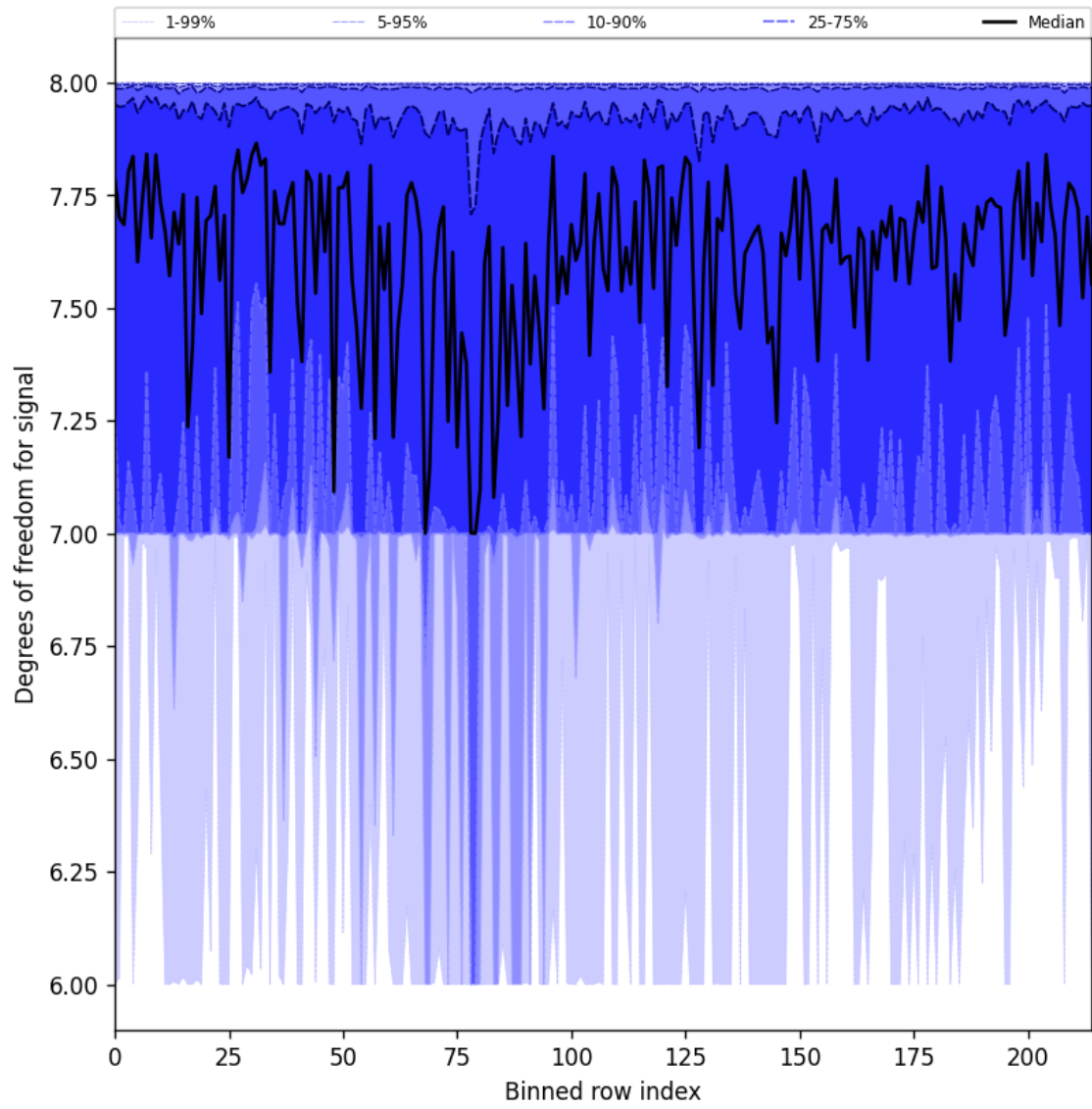
Figure 31: Along track statistics of “Degrees of freedom for signal” for 2025-09-01 to 2025-09-03
