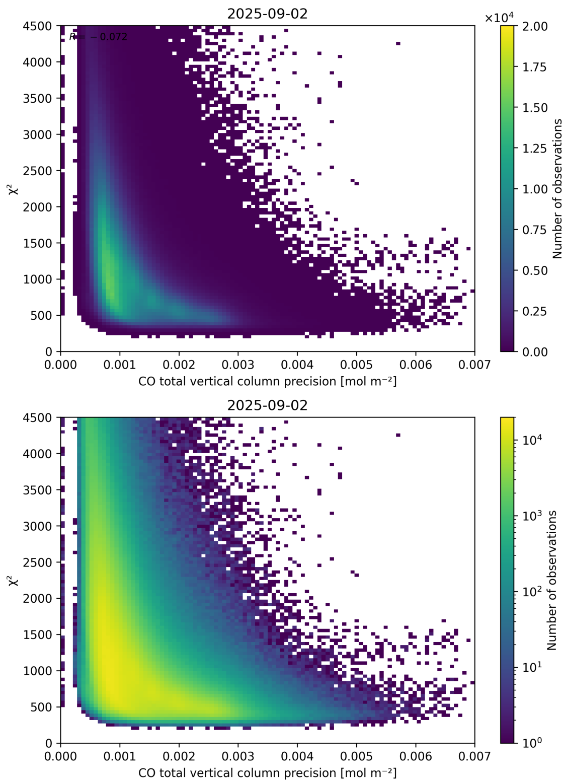
Figure 44: Scatter density plot of “CO total vertical column precision” against “ \chi^2 ” for 2025-09-01 to 2025-09-03.
