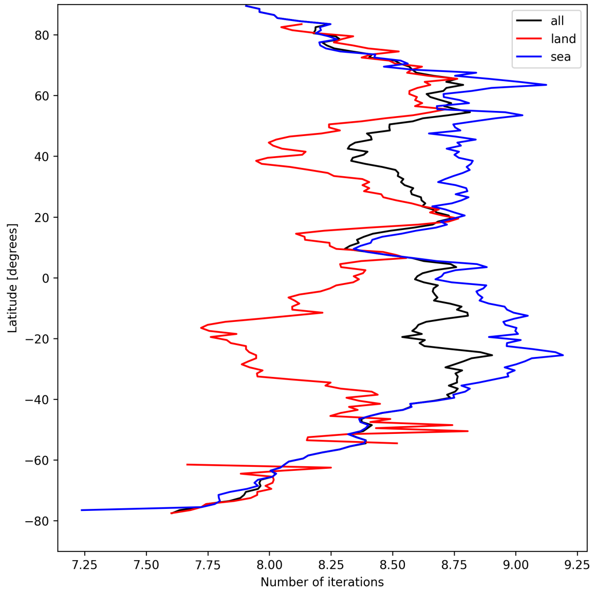
Figure 16: Zonal average of “Number of iterations” for 2025-09-01 to 2025-09-03.
