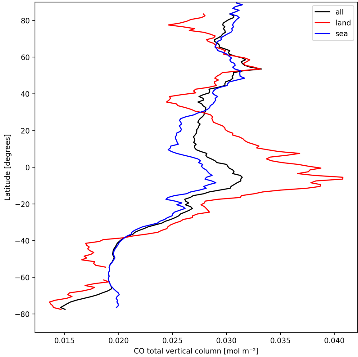
Figure 10: Zonal average of “CO total vertical column” for 2025-09-01 to 2025-09-03.
