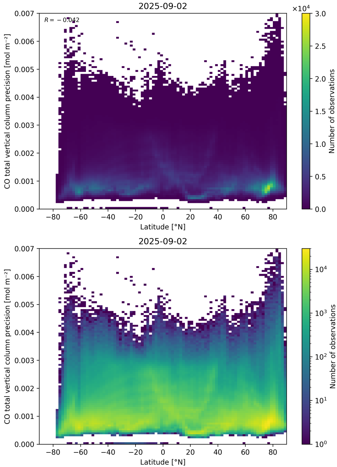
Figure 53: Scatter density plot of “Latitude” against “CO total vertical column precision” for 2025-09-01 to 2025-09-03.
