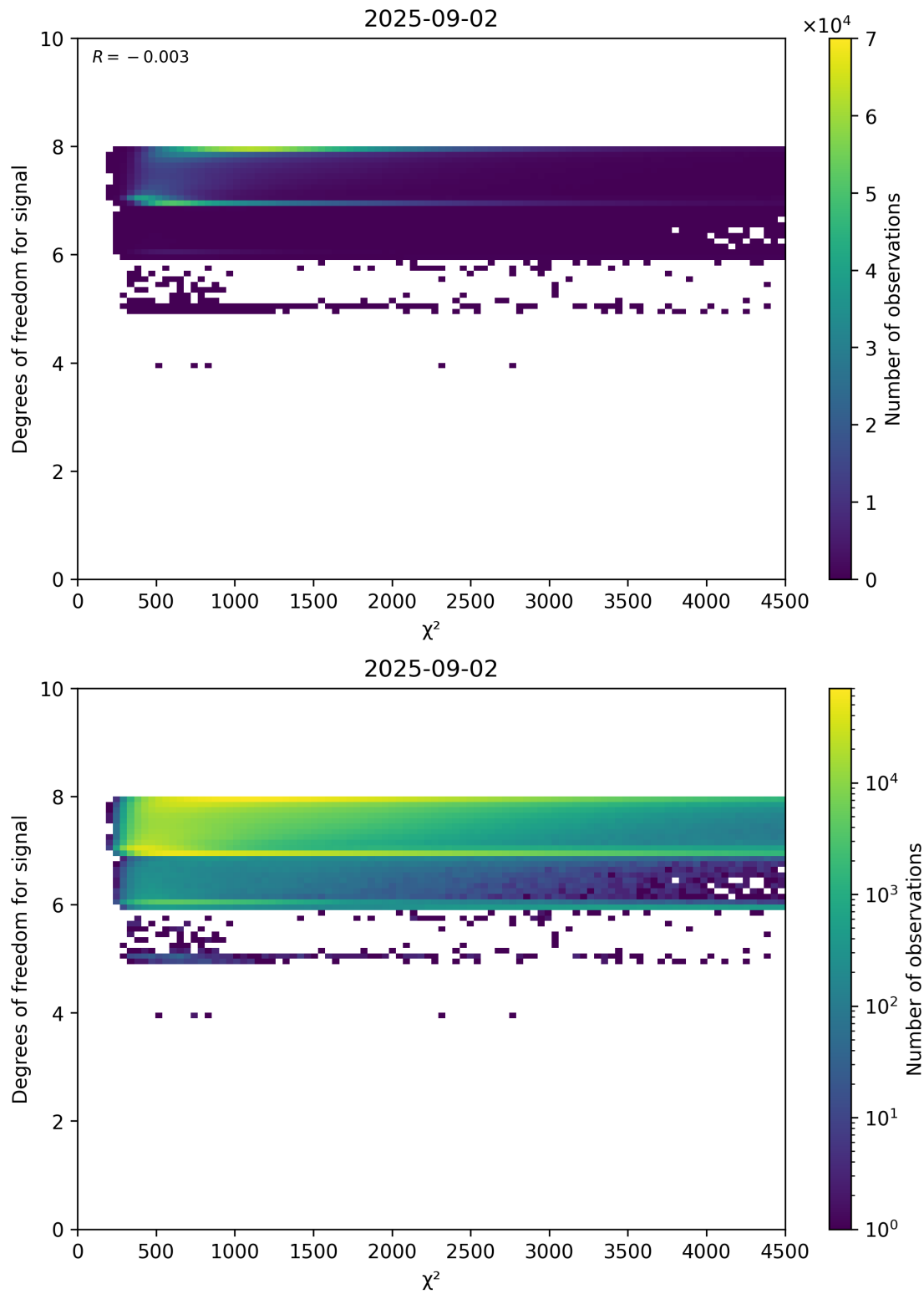
Figure 48: Scatter density plot of “ \chi^2 ” against “Degrees of freedom for signal” for 2025-09-01 to 2025-09-03.
