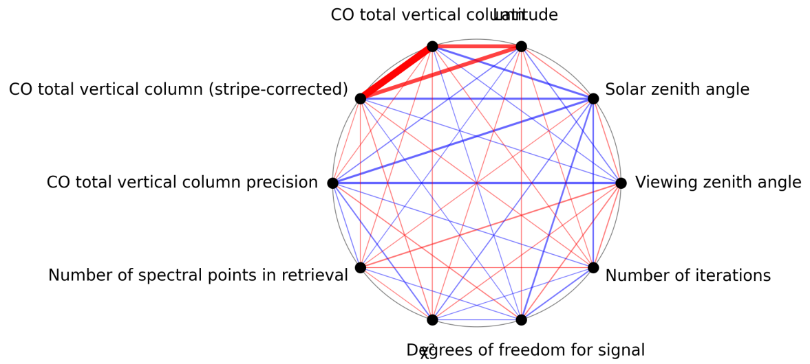
Figure 1: Map of correlation graph for 2025-09-01 to 2025-09-03.
