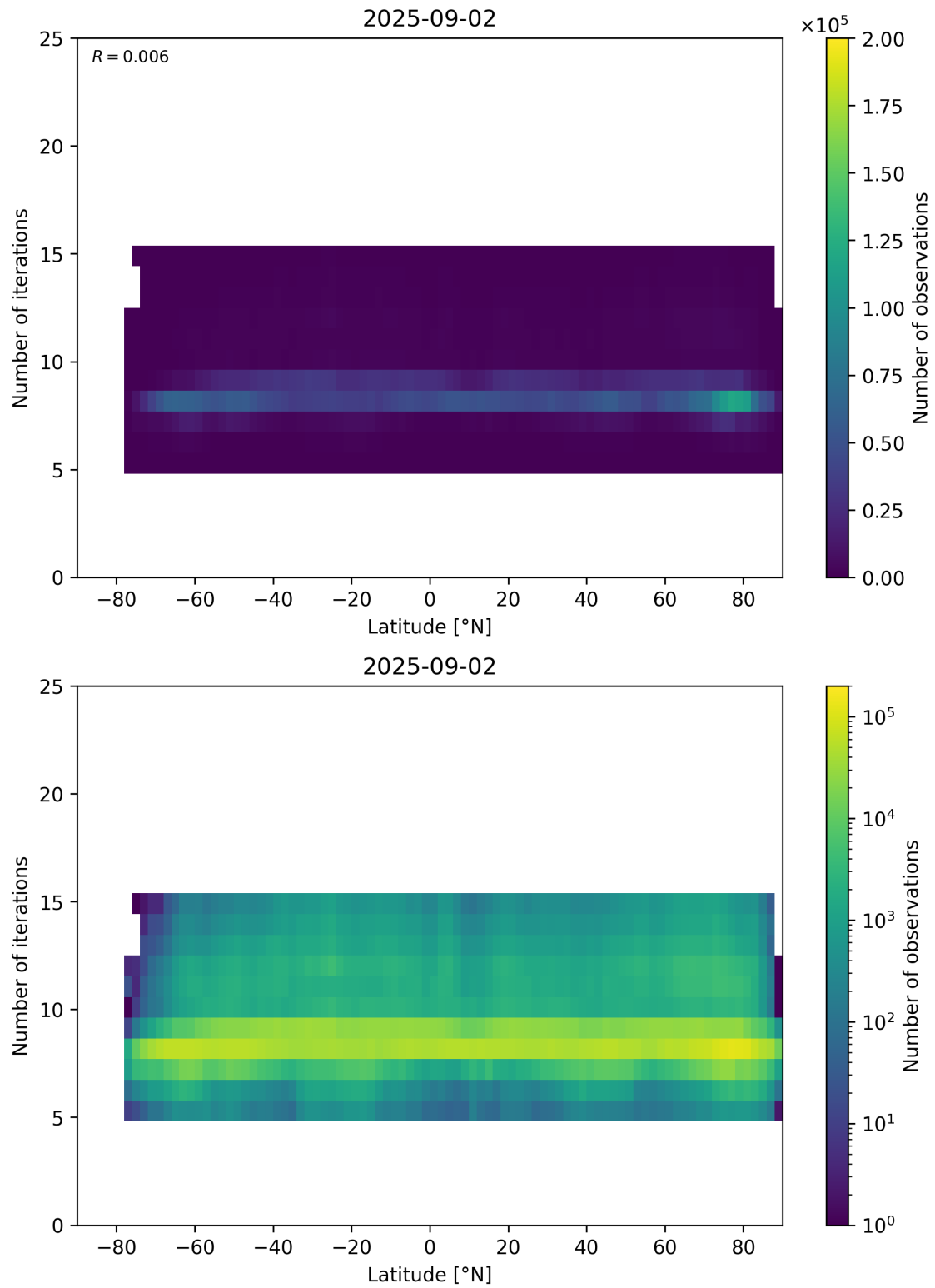
Figure 56: Scatter density plot of “Latitude” against “Number of iterations” for 2025-09-01 to 2025-09-03.
