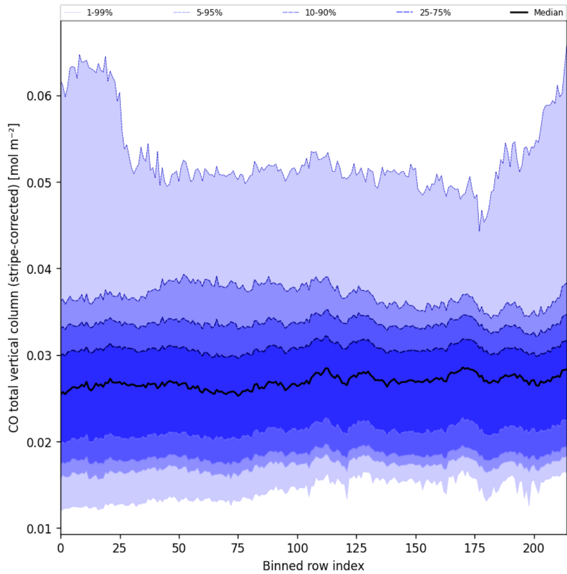
Figure 27: Along track statistics of “CO total vertical column (stripe-corrected)” for 2025-09-01 to 2025-09-03
