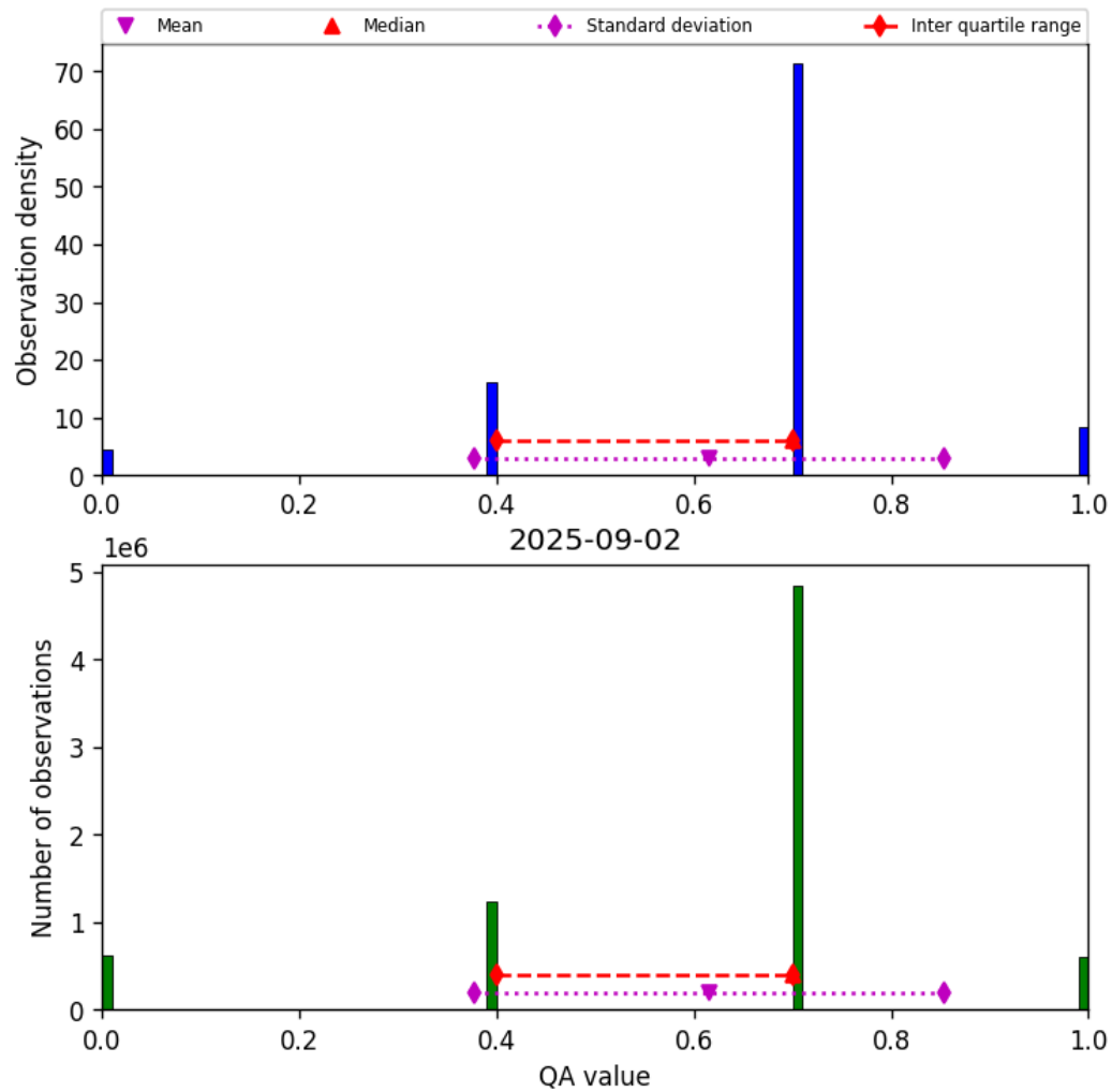
Figure 17: Histogram of “QA value” for 2025-09-01 to 2025-09-03
