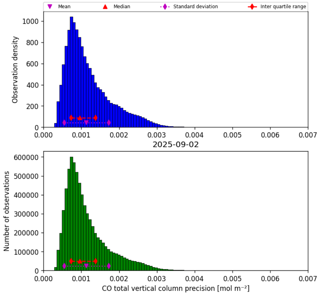
Figure 20: Histogram of “CO total vertical column precision” for 2025-09-01 to 2025-09-03
