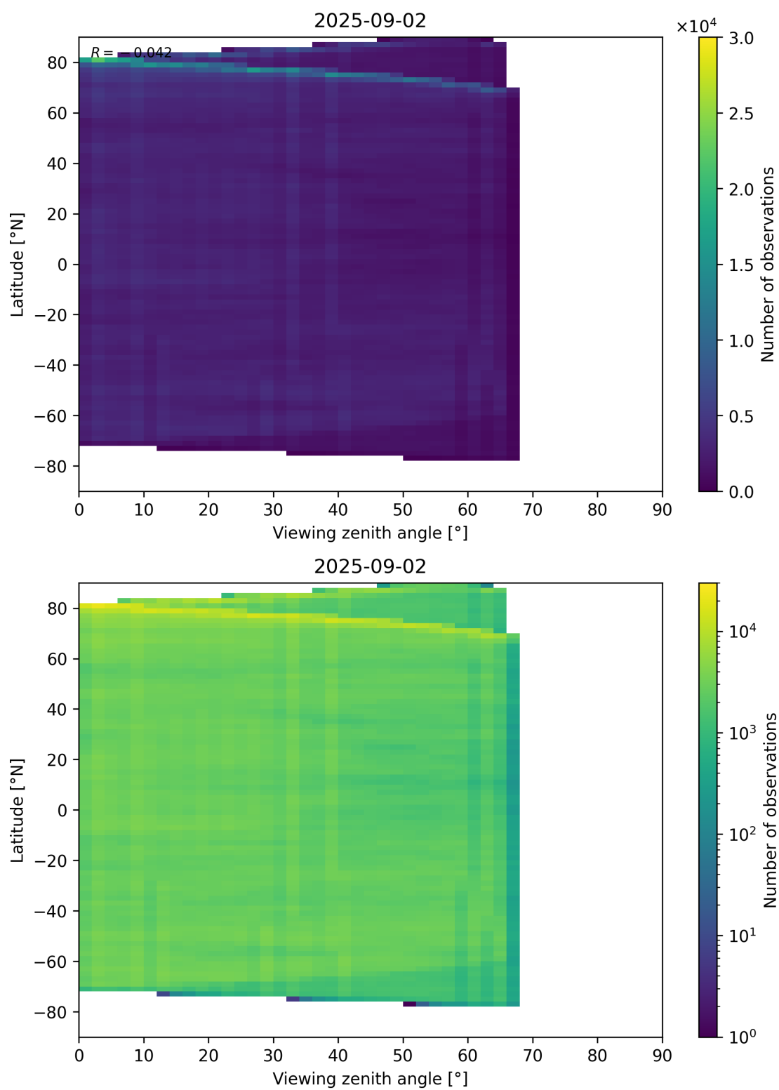
Figure 74: Scatter density plot of “Viewing zenith angle” against “Latitude” for 2025-09-01 to 2025-09-03.
