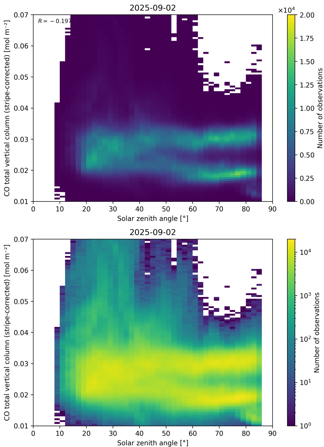
Figure 62: Scatter density plot of “Solar zenith angle” against “CO total vertical column (stripe-corrected)” for 2025-09-01 to 2025-09-03.
