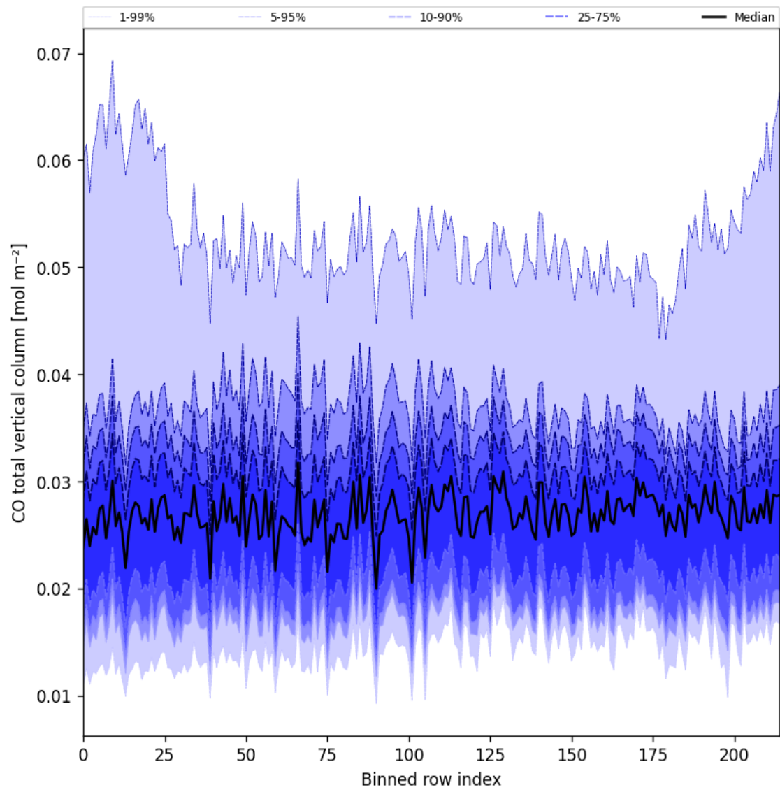
Figure 26: Along track statistics of “CO total vertical column” for 2025-09-01 to 2025-09-03
