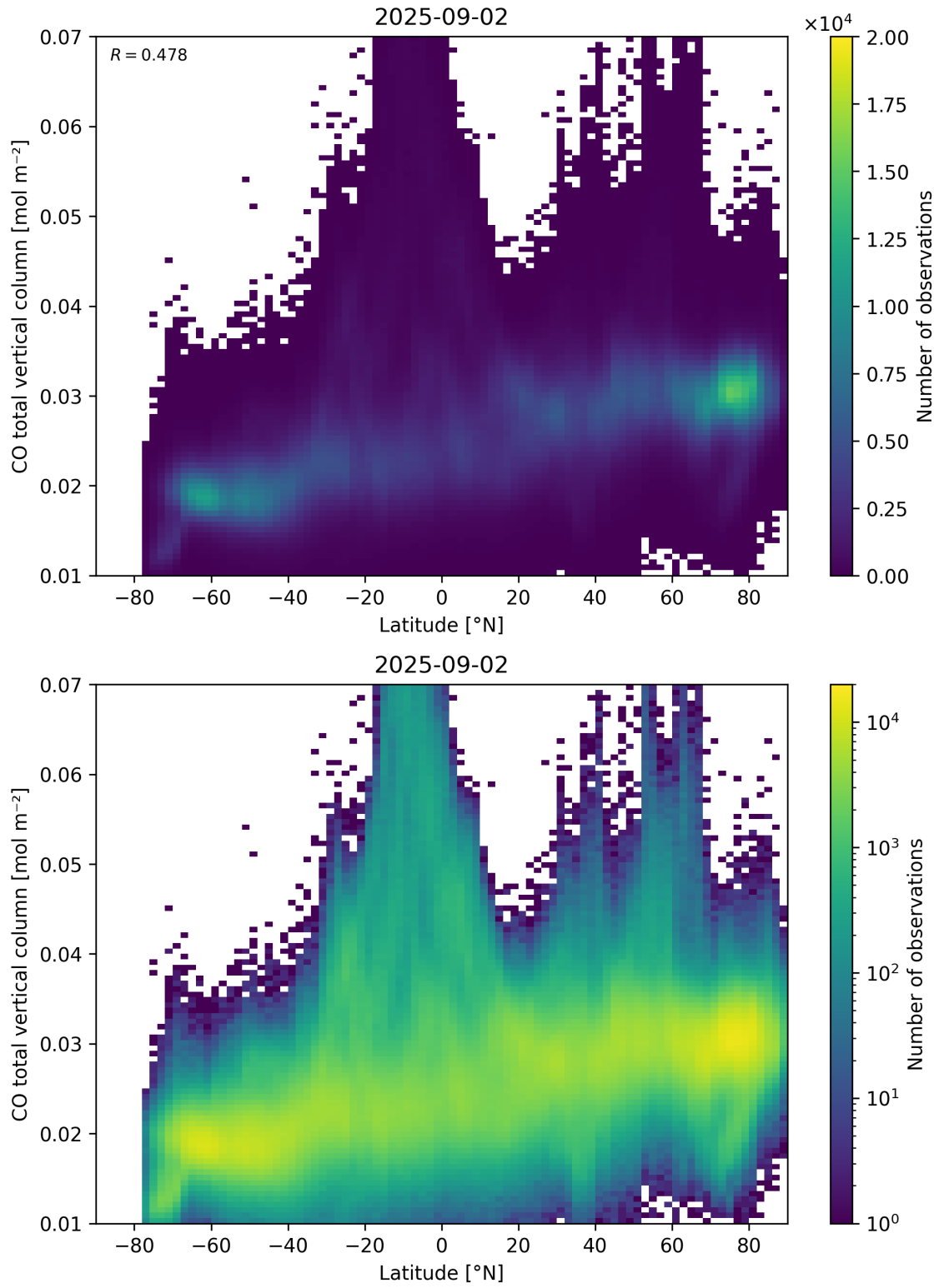
Figure 51: Scatter density plot of “Latitude” against “CO total vertical column” for 2025-09-01 to 2025-09-03.
