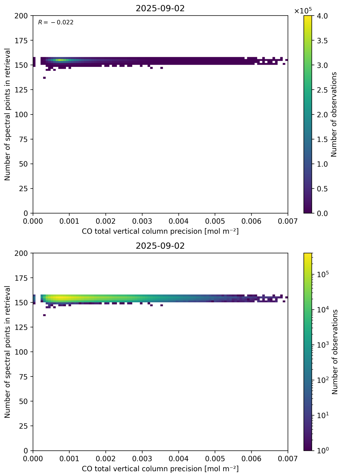
Figure 47: Scatter density plot of “CO total vertical column precision” against “Number of spectral points in retrieval” for 2025-09-01 to 2025-09-03.
