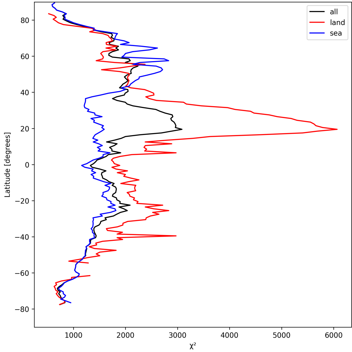
Figure 14: Zonal average of “ \chi^2 ” for 2025-09-01 to 2025-09-03.
