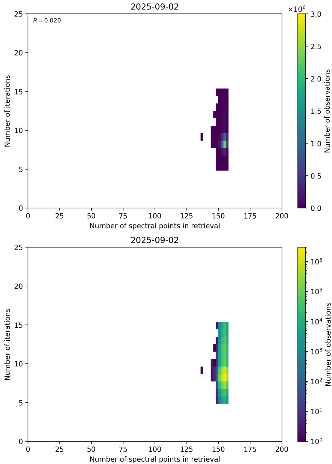
Figure 60: Scatter density plot of “Number of spectral points in retrieval” against “Number of iterations” for 2025-09-01 to 2025-09-03.
