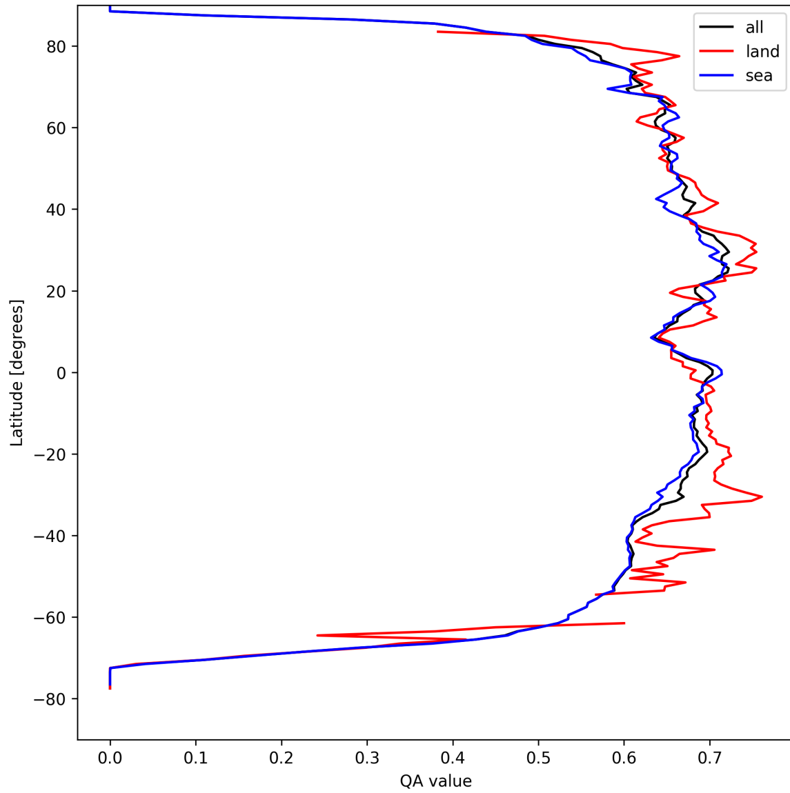
Figure 9: Zonal average of “QA value” for 2025-09-01 to 2025-09-03.
