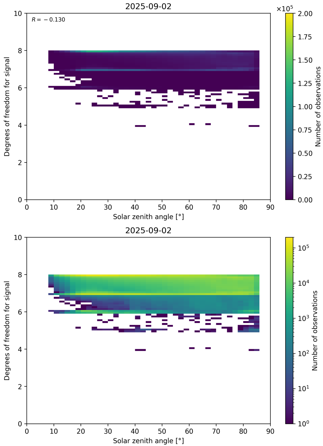
Figure 65: Scatter density plot of “Solar zenith angle” against “Degrees of freedom for signal” for 2025-09-01 to 2025-09-03.
