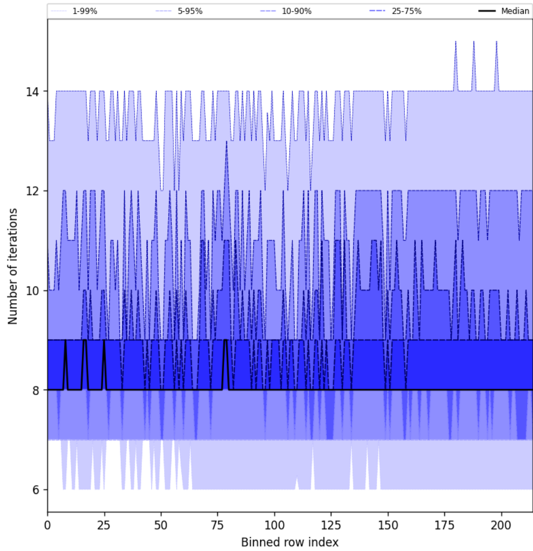
Figure 32: Along track statistics of “Number of iterations” for 2025-09-01 to 2025-09-03
