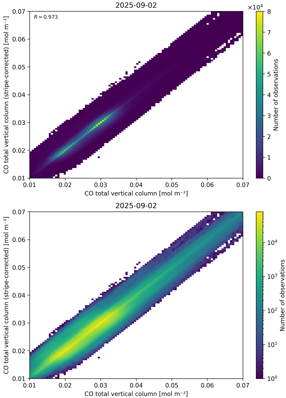
Figure 33: Scatter density plot of “CO total vertical column” against “CO total vertical column (stripe-corrected)” for 2025-09-01 to 2025-09-03.
