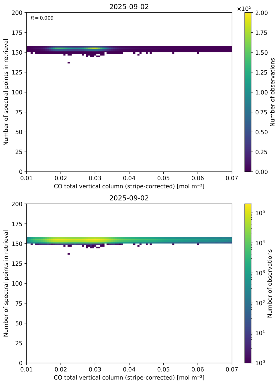
Figure 40: Scatter density plot of “CO total vertical column (stripe-corrected)” against “Number of spectral points in retrieval” for 2025-09-01 to 2025-09-03.
