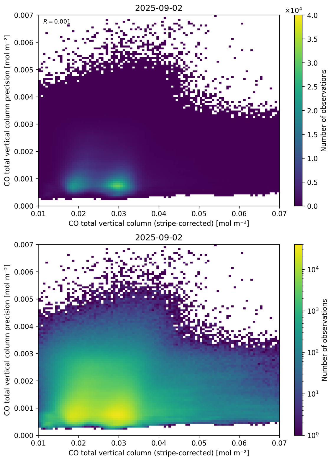
Figure 36: Scatter density plot of “CO total vertical column (stripe-corrected)” against “CO total vertical column precision” for 2025-09-01 to 2025-09-03.
