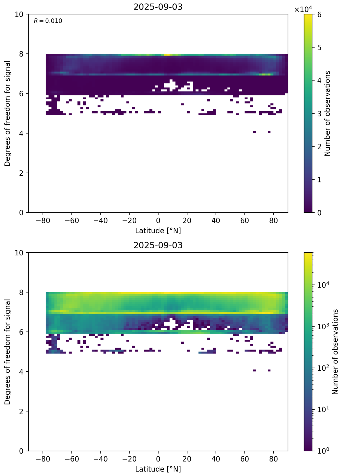
Figure 55: Scatter density plot of “Latitude” against “Degrees of freedom for signal” for 2025-09-02 to 2025-09-04.
