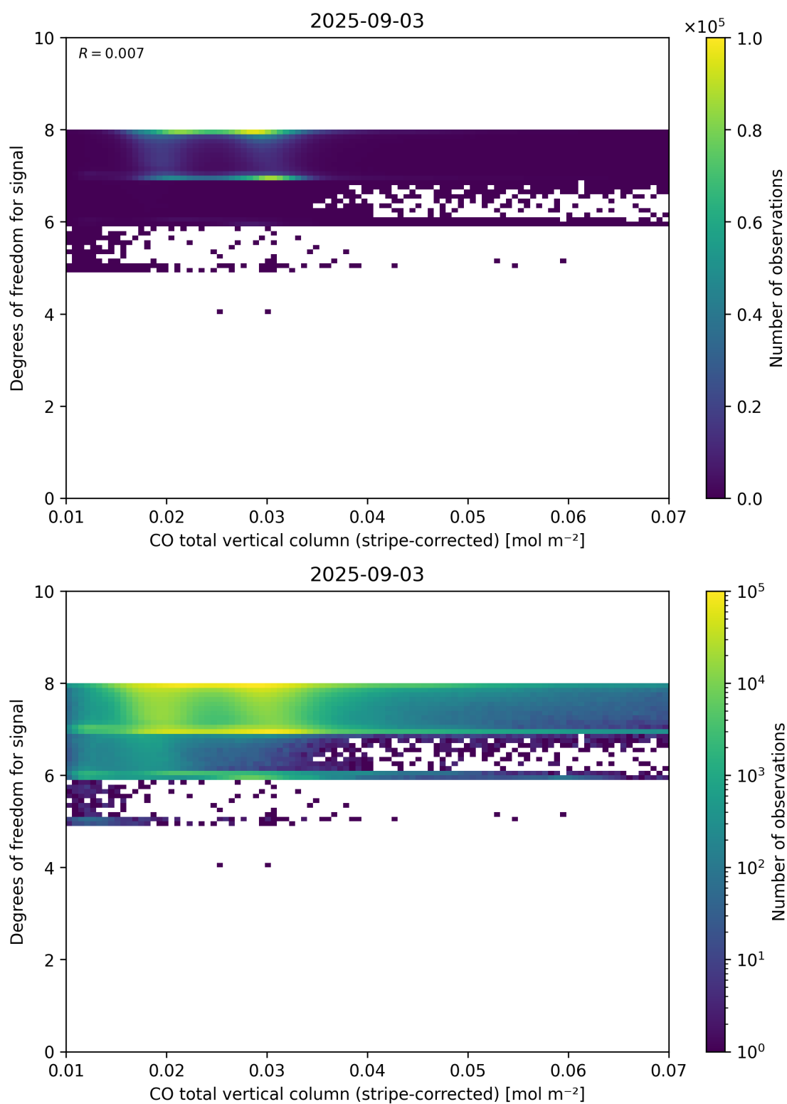
Figure 38: Scatter density plot of “CO total vertical column (stripe-corrected)” against “Degrees of freedom for signal” for 2025-09-02 to 2025-09-04.
