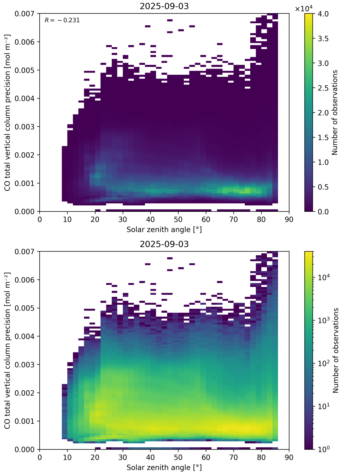
Figure 63: Scatter density plot of “Solar zenith angle” against “CO total vertical column precision” for 2025-09-02 to 2025-09-04.
