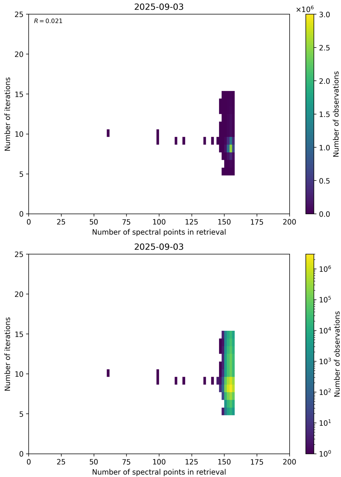
Figure 60: Scatter density plot of “Number of spectral points in retrieval” against “Number of iterations” for 2025-09-02 to 2025-09-04.
