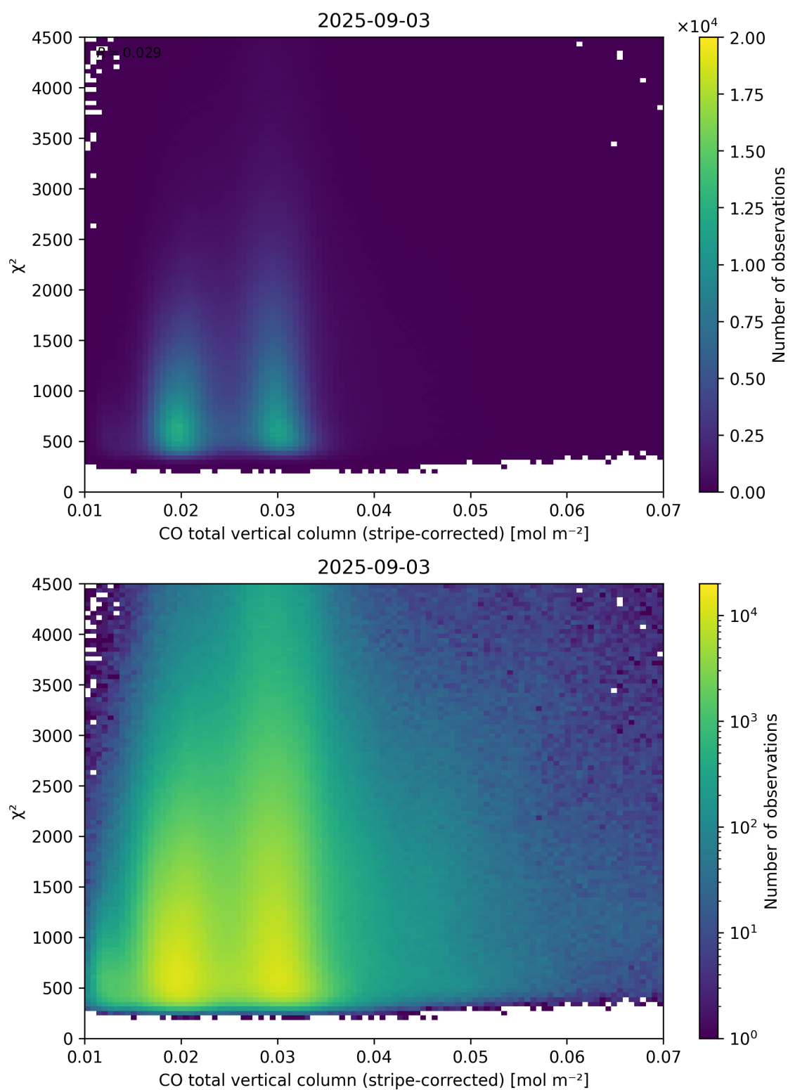
Figure 37: Scatter density plot of “CO total vertical column (stripe-corrected)” against “ \chi^2 ” for 2025-09-02 to 2025-09-04.
