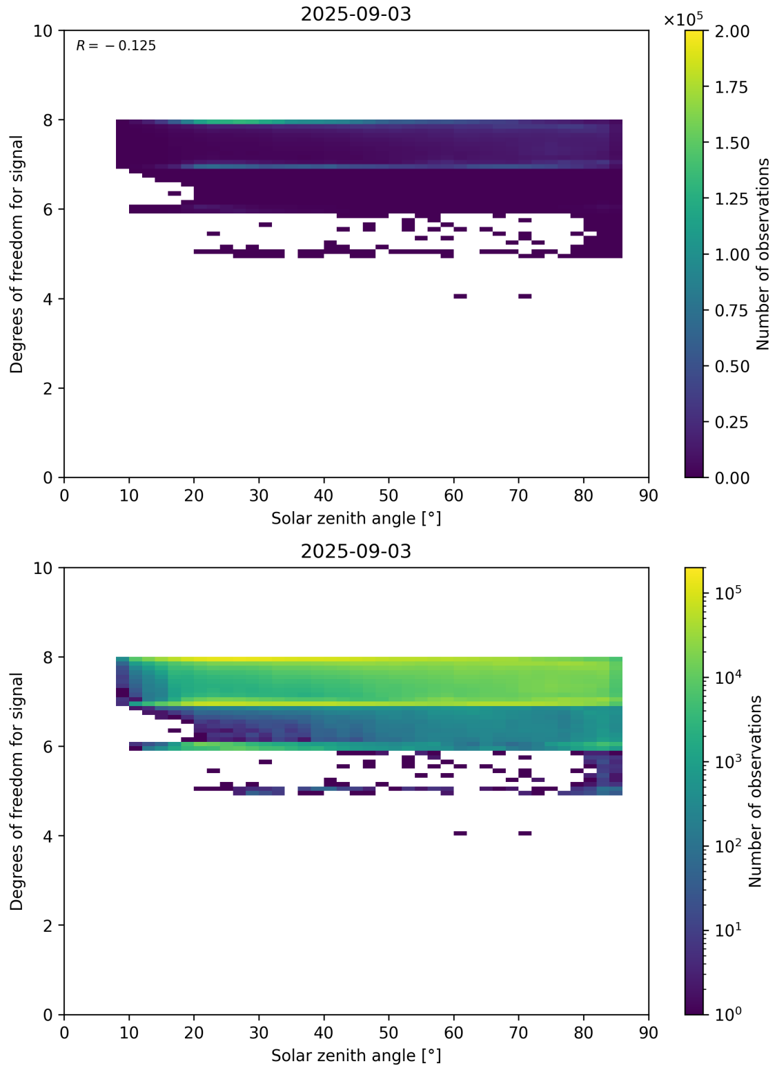
Figure 65: Scatter density plot of “Solar zenith angle” against “Degrees of freedom for signal” for 2025-09-02 to 2025-09-04.
