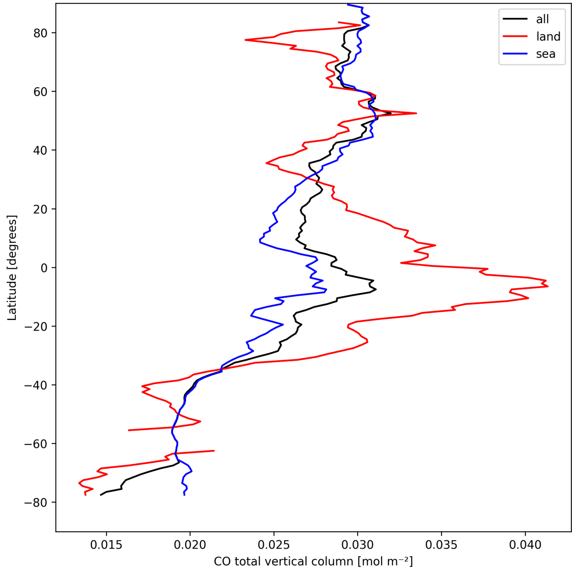
Figure 10: Zonal average of “CO total vertical column” for 2025-09-02 to 2025-09-04.
