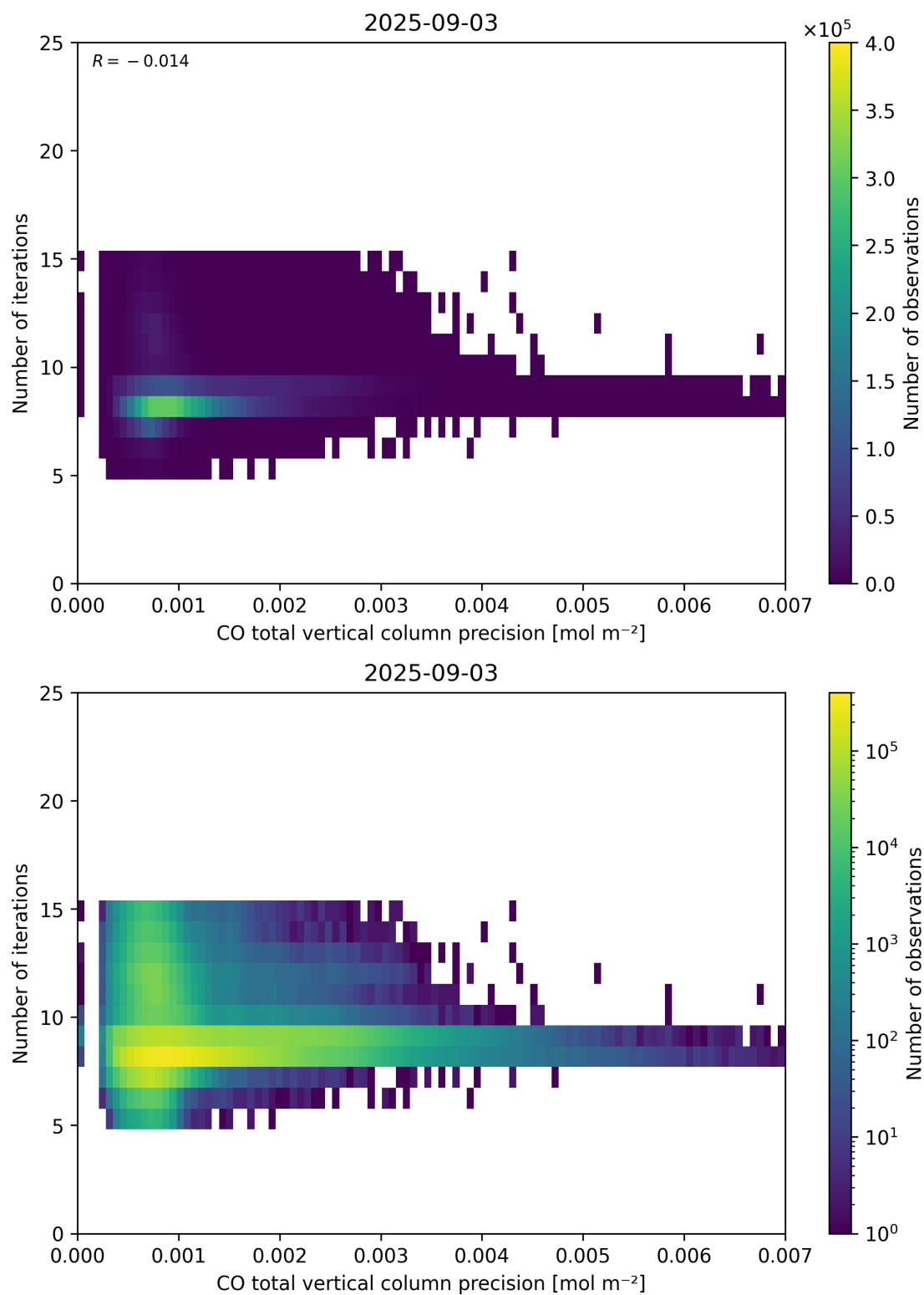
Figure 46: Scatter density plot of “CO total vertical column precision” against “Number of iterations” for 2025-09-02 to 2025-09-04.
