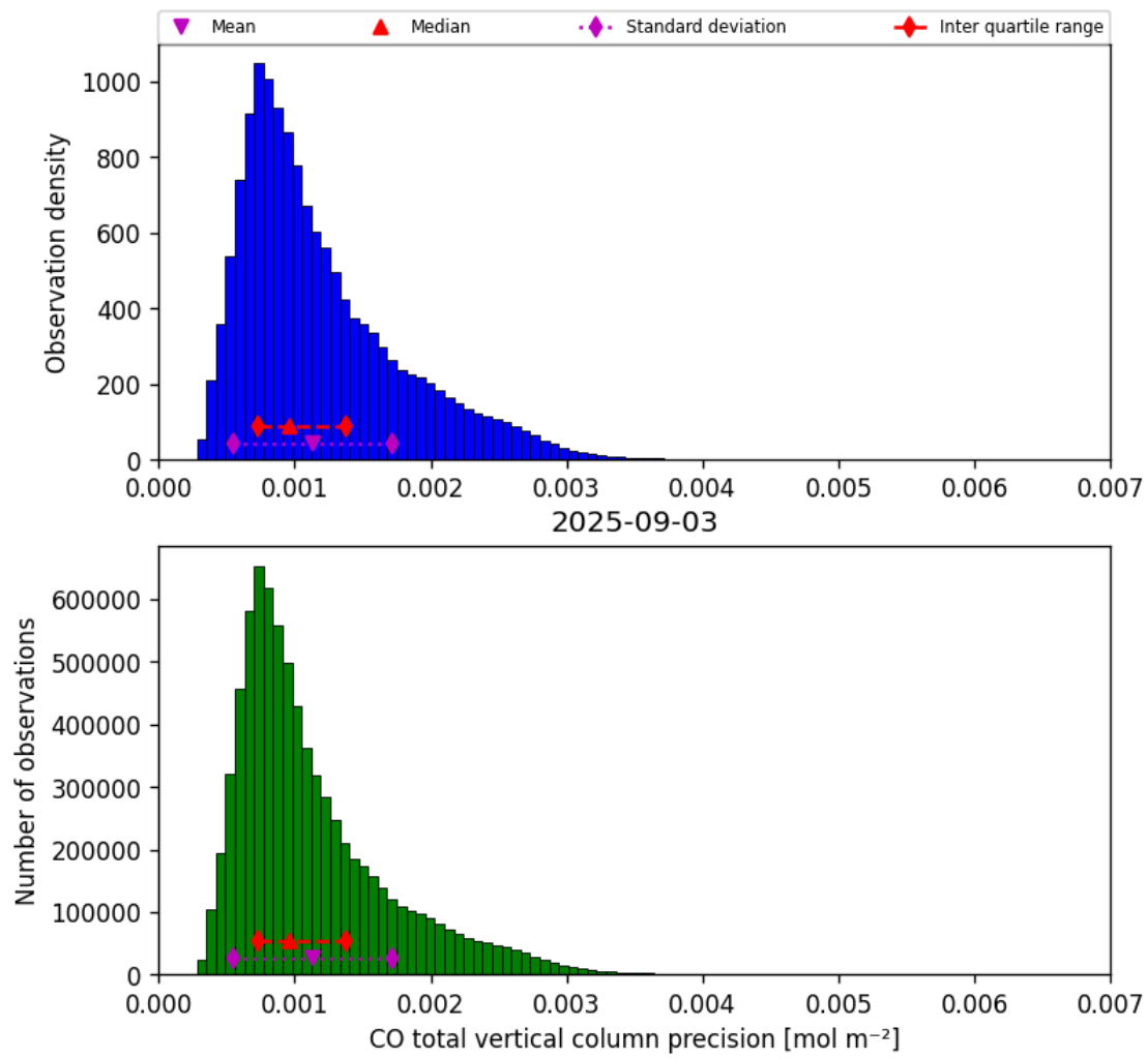
Figure 20: Histogram of “CO total vertical column precision” for 2025-09-02 to 2025-09-04
