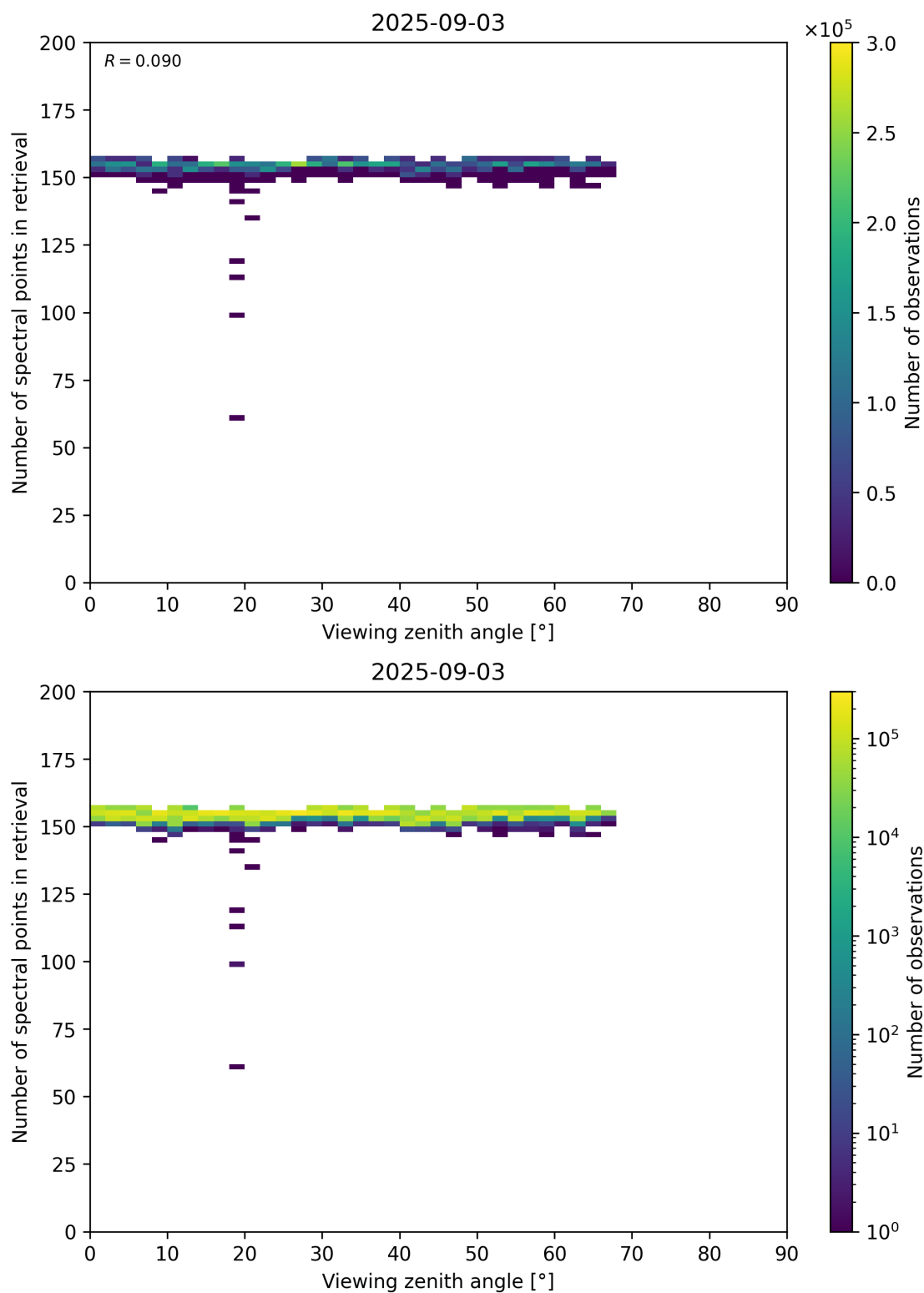
Figure 76: Scatter density plot of “Viewing zenith angle” against “Number of spectral points in retrieval” for 2025-09-02 to 2025-09-04.
