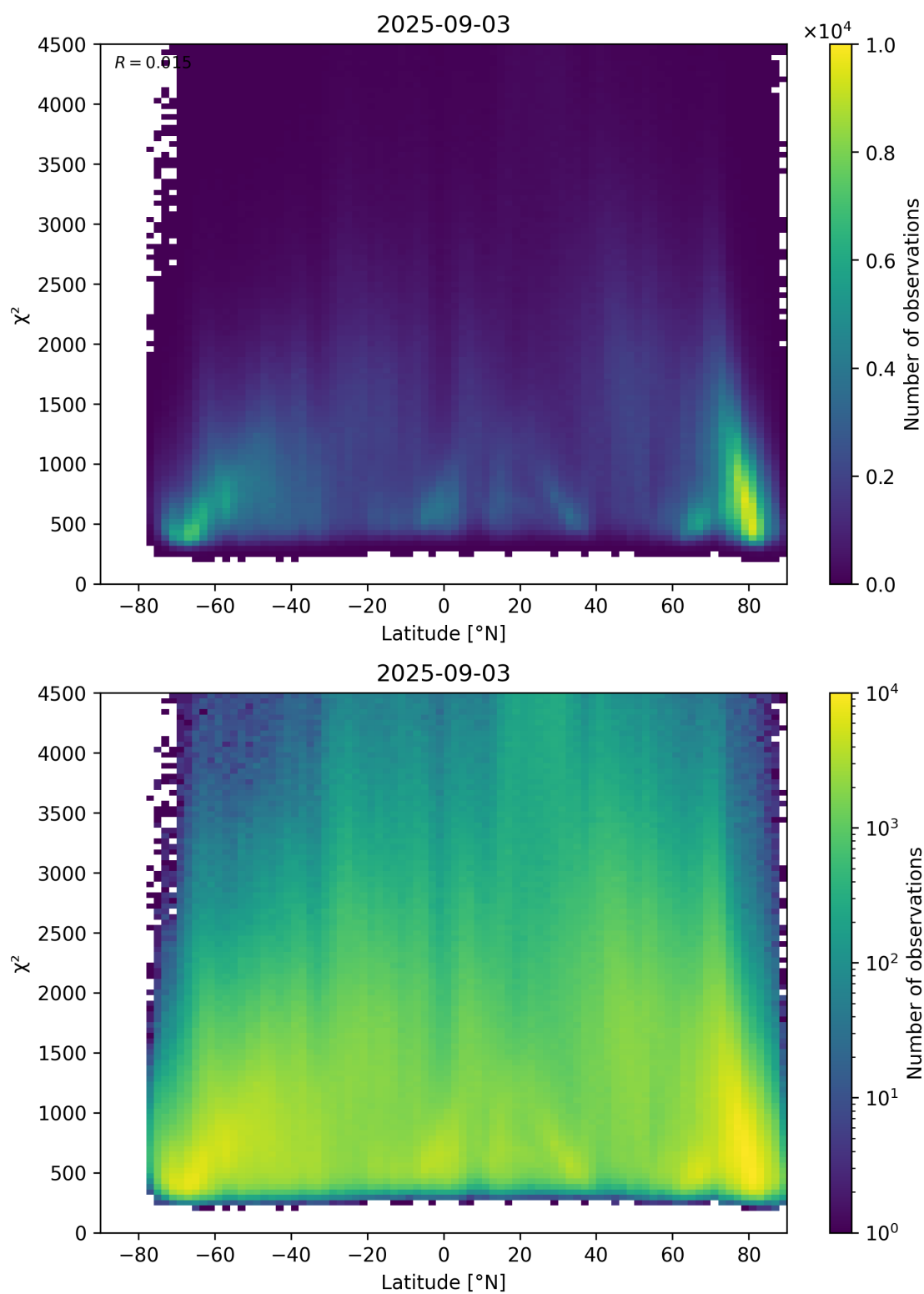
Figure 54: Scatter density plot of “Latitude” against “ \chi^2 ” for 2025-09-02 to 2025-09-04.
