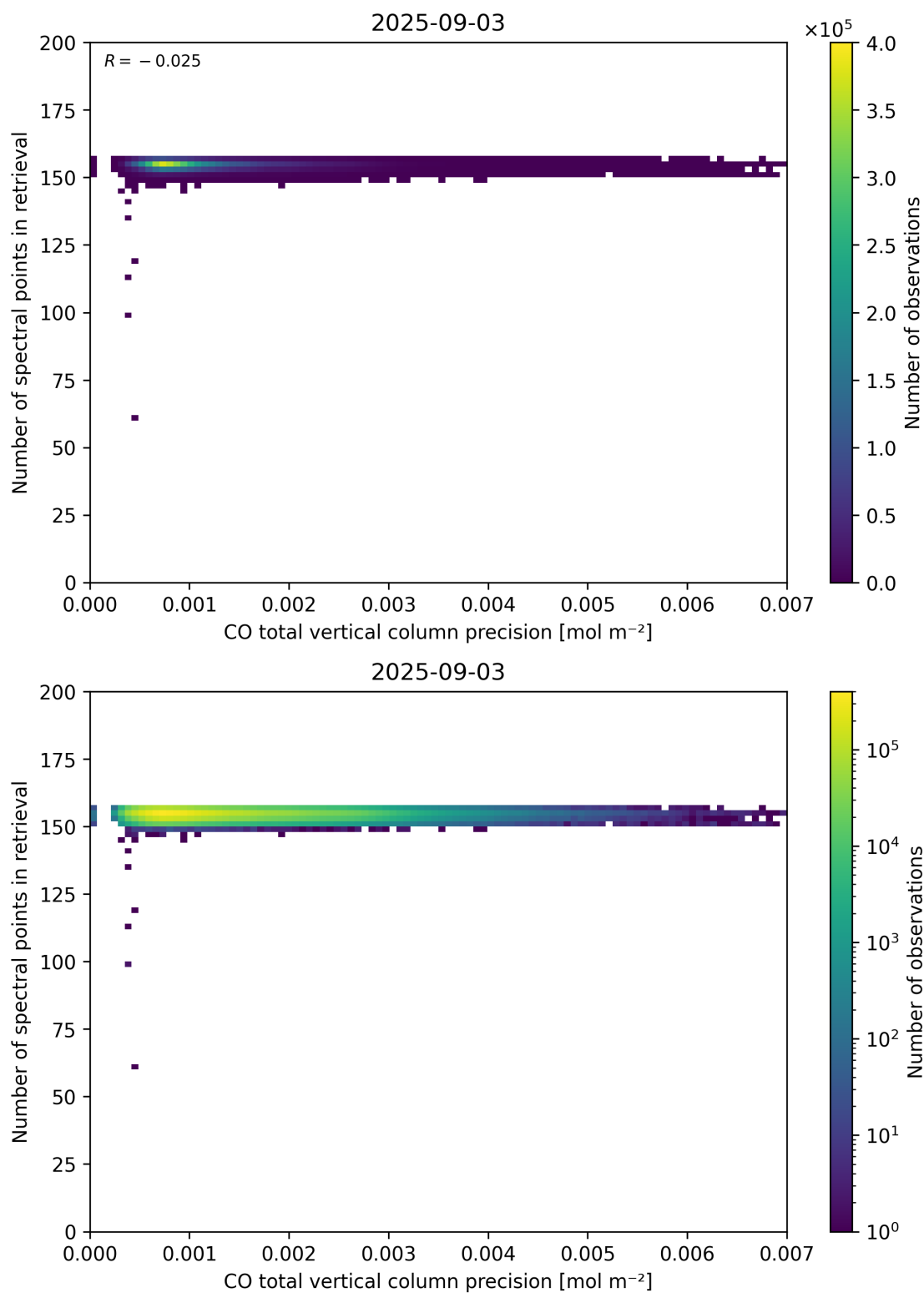
Figure 47: Scatter density plot of “CO total vertical column precision” against “Number of spectral points in retrieval” for 2025-09-02 to 2025-09-04.
