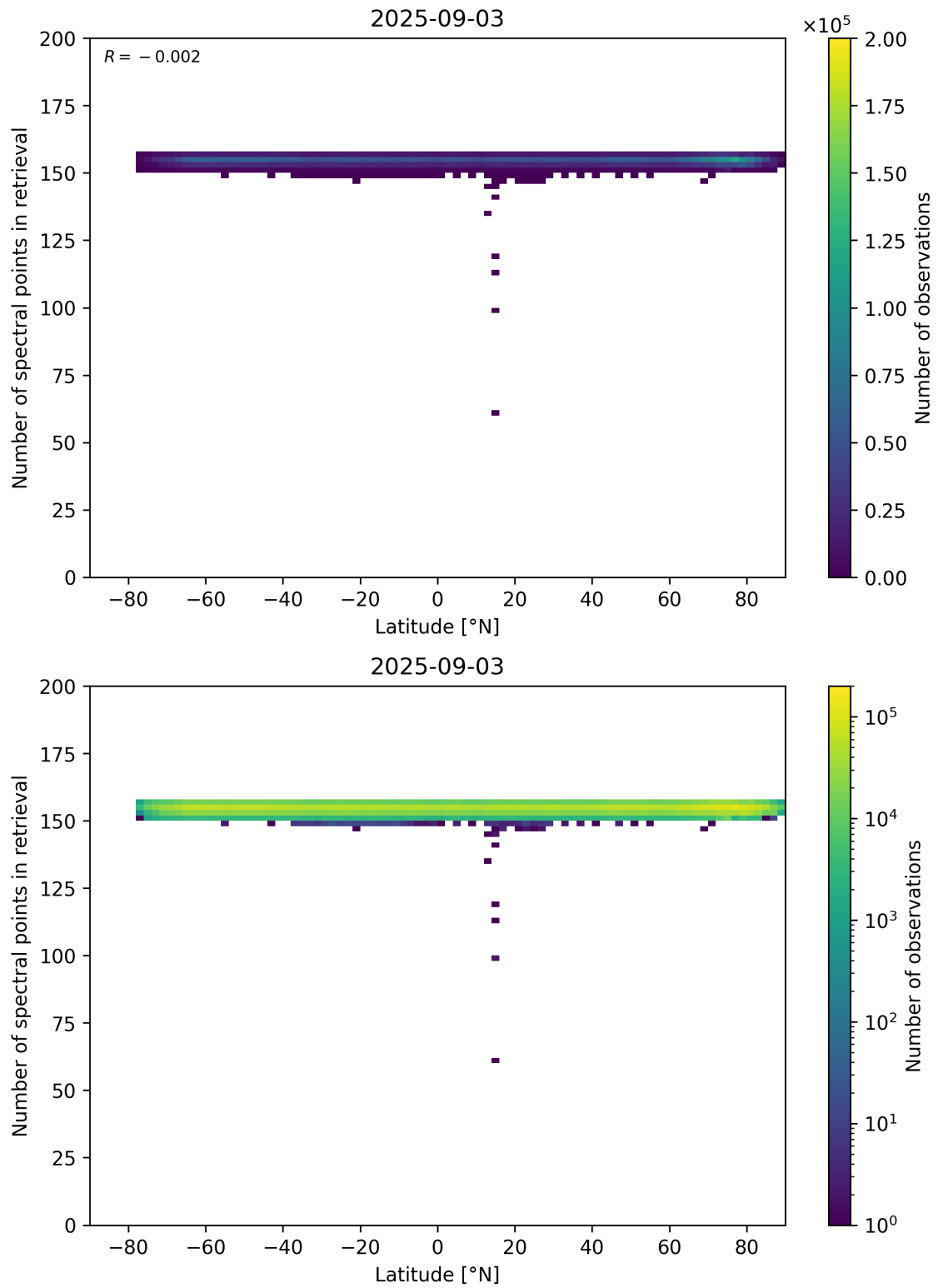
Figure 57: Scatter density plot of “Latitude” against “Number of spectral points in retrieval” for 2025-09-02 to 2025-09-04.
