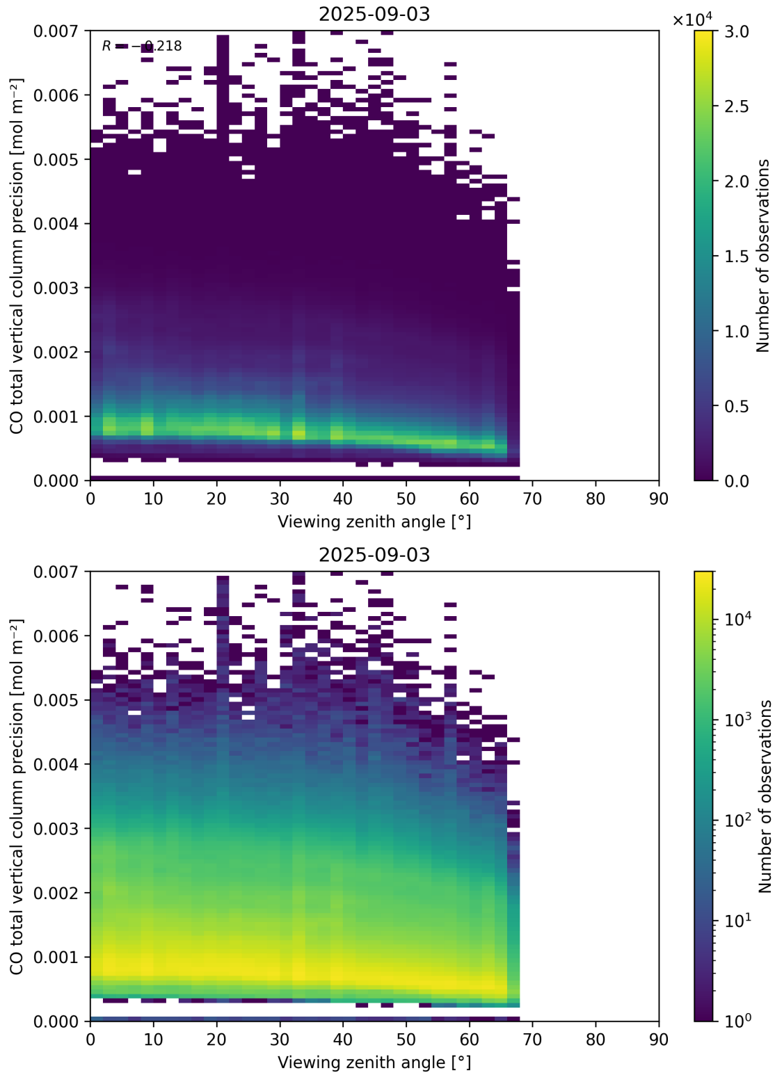
Figure 71: Scatter density plot of “Viewing zenith angle” against “CO total vertical column precision” for 2025-09-02 to 2025-09-04.
