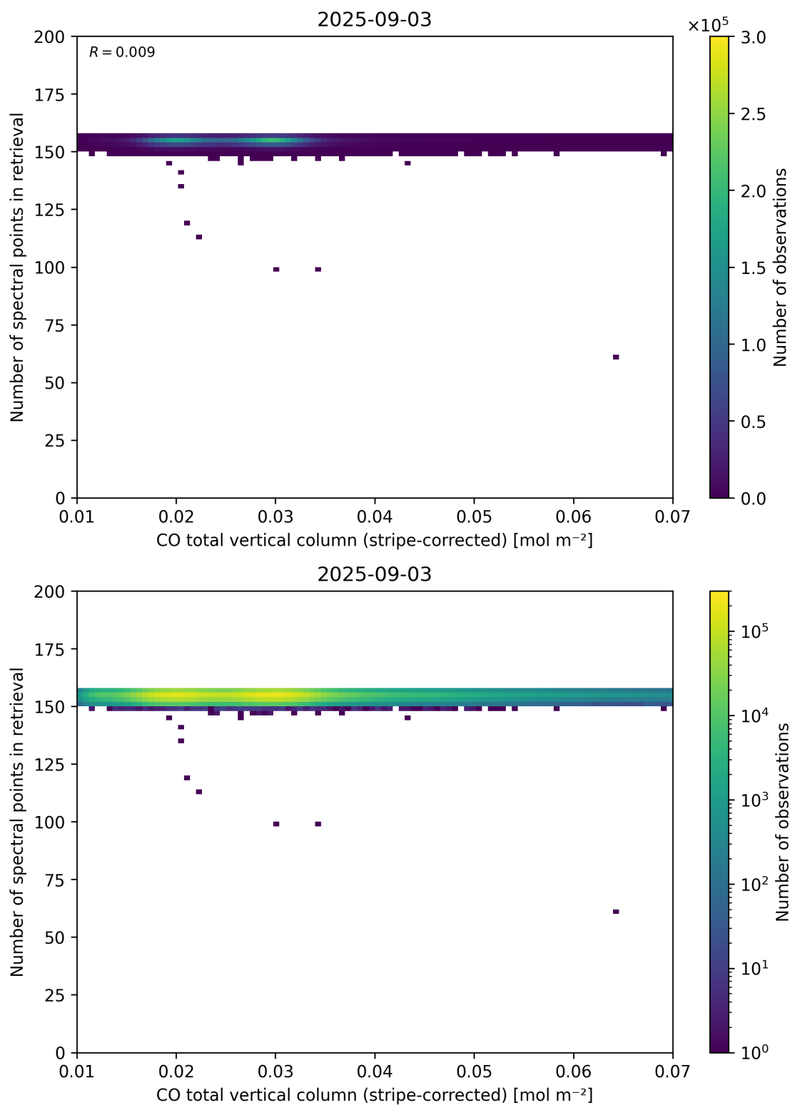
Figure 40: Scatter density plot of “CO total vertical column (stripe-corrected)” against “Number of spectral points in retrieval” for 2025-09-02 to 2025-09-04.
