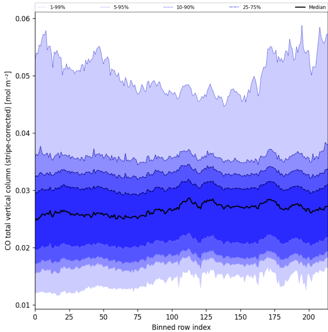
Figure 27: Along track statistics of “CO total vertical column (stripe-corrected)” for 2025-09-02 to 2025-09-04
