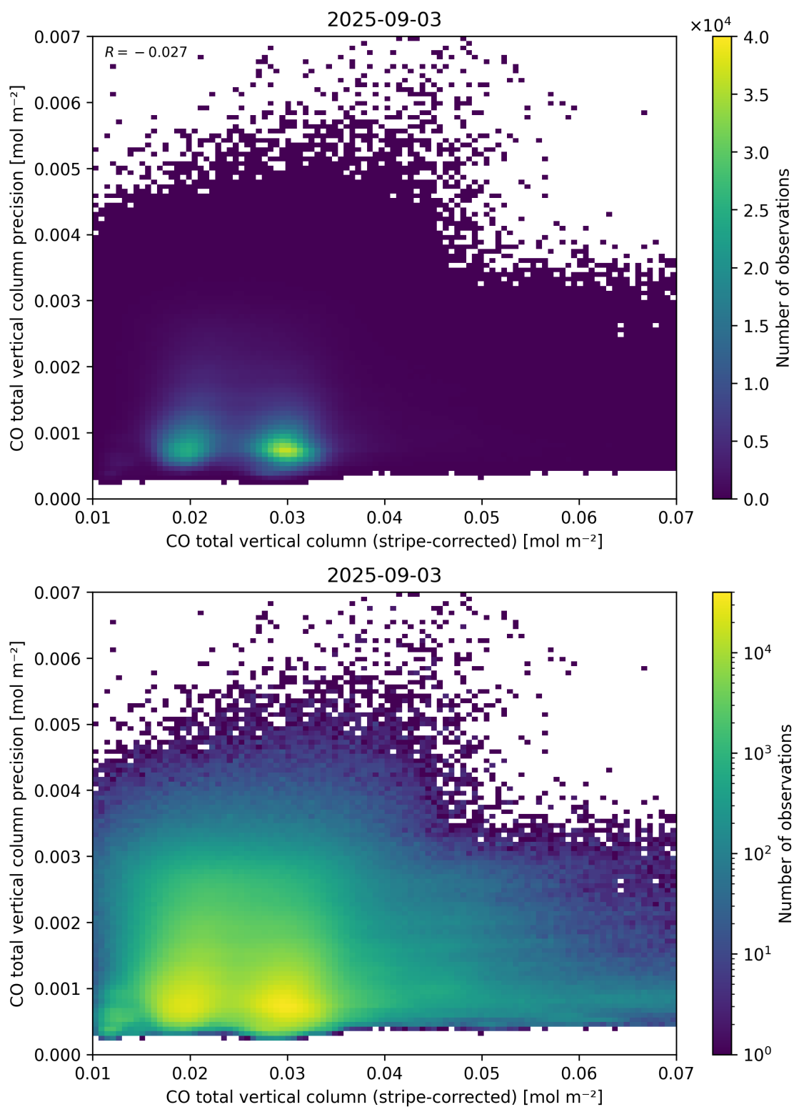
Figure 36: Scatter density plot of “CO total vertical column (stripe-corrected)” against “CO total vertical column precision” for 2025-09-02 to 2025-09-04.
