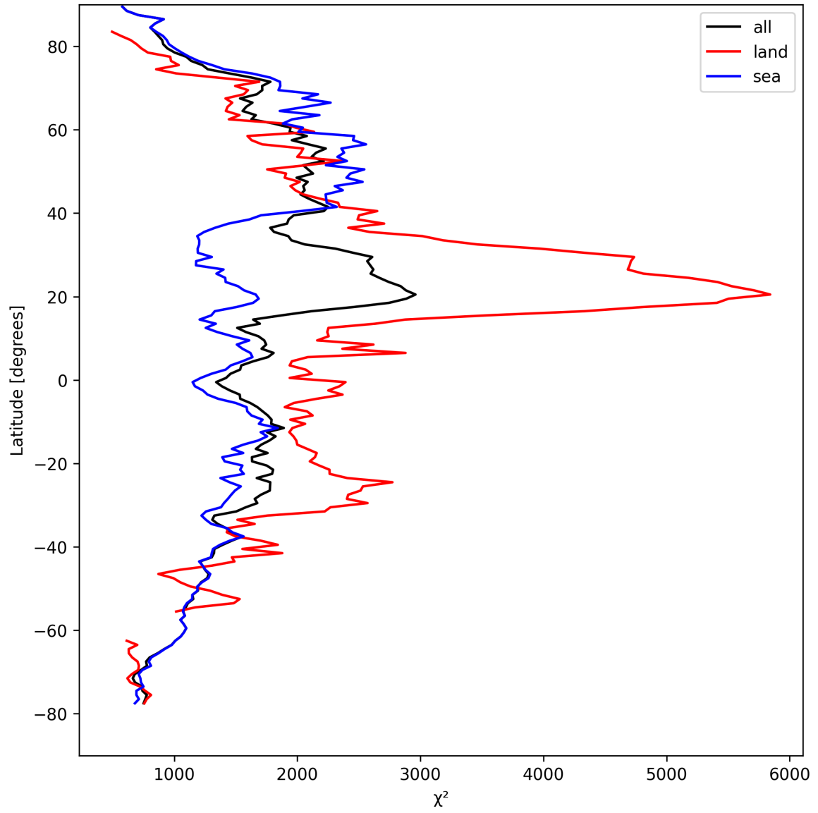
Figure 14: Zonal average of “ \chi^2 ” for 2025-09-02 to 2025-09-04.
