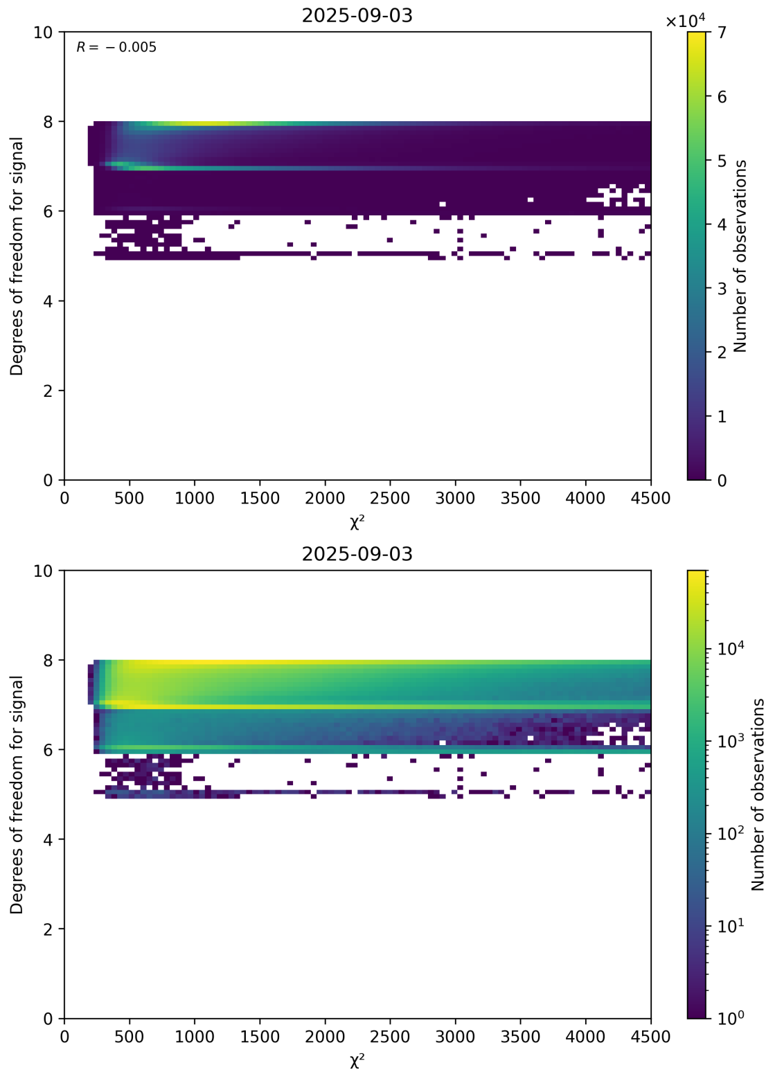
Figure 48: Scatter density plot of " \chi^2 " against "Degrees of freedom for signal" for 2025-09-02 to 2025-09-04.
