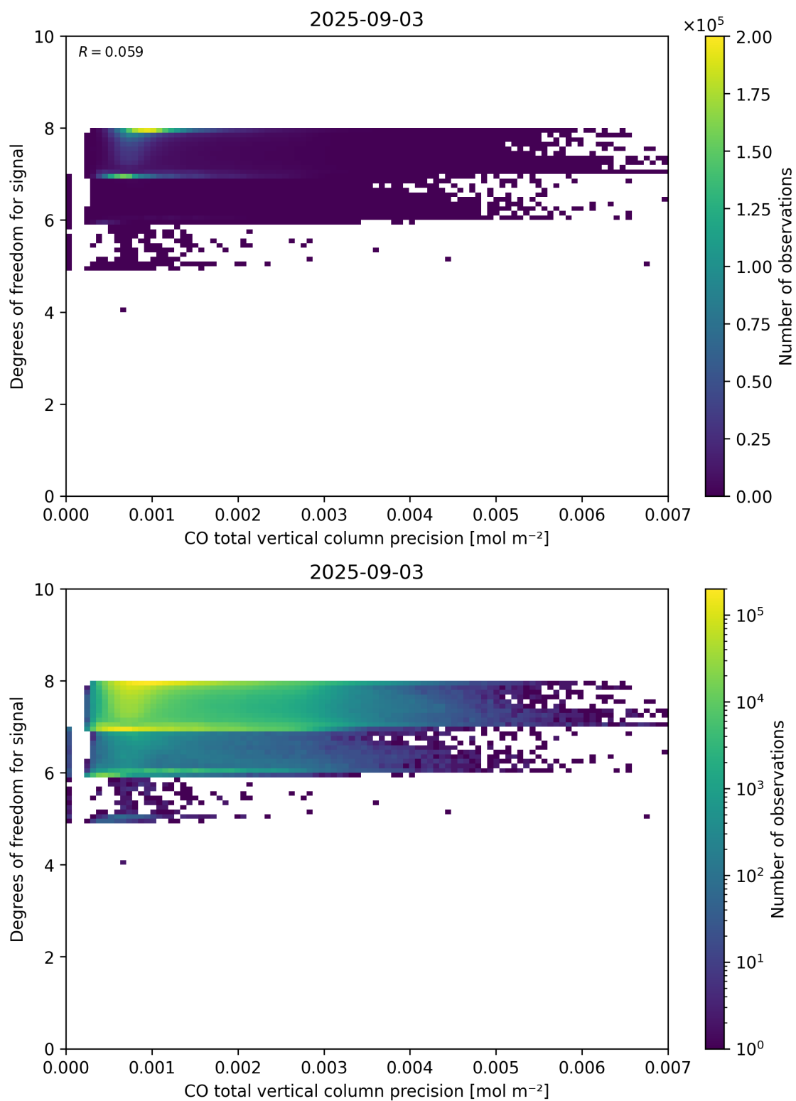
Figure 45: Scatter density plot of “CO total vertical column precision” against “Degrees of freedom for signal” for 2025-09-02 to 2025-09-04.
