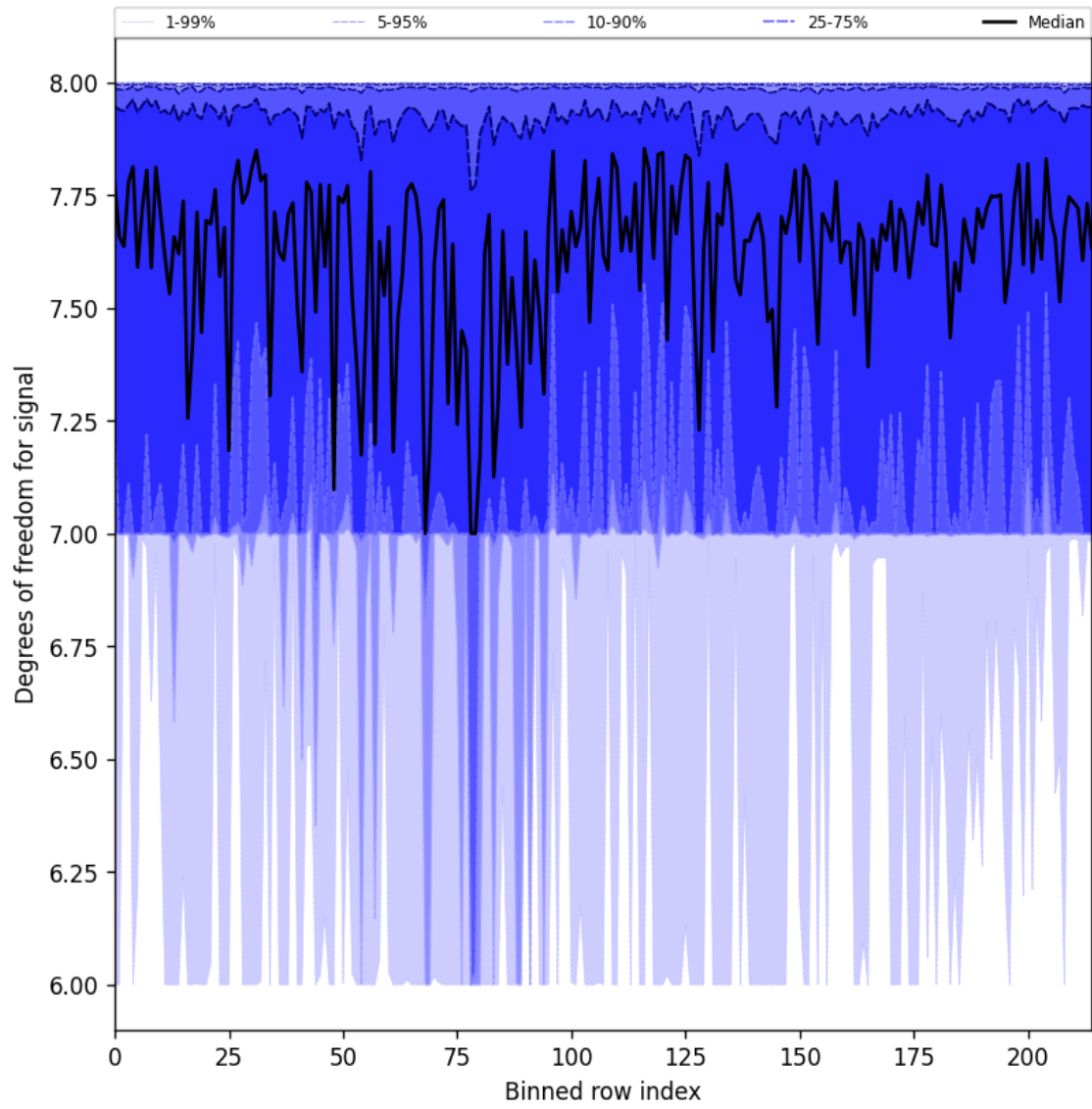
Figure 31: Along track statistics of “Degrees of freedom for signal” for 2025-09-02 to 2025-09-04
