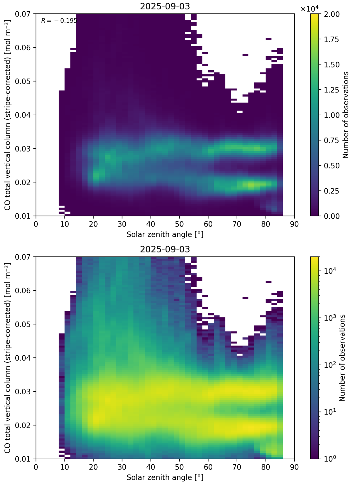
Figure 62: Scatter density plot of “Solar zenith angle” against “CO total vertical column (stripe-corrected)” for 2025-09-02 to 2025-09-04.
