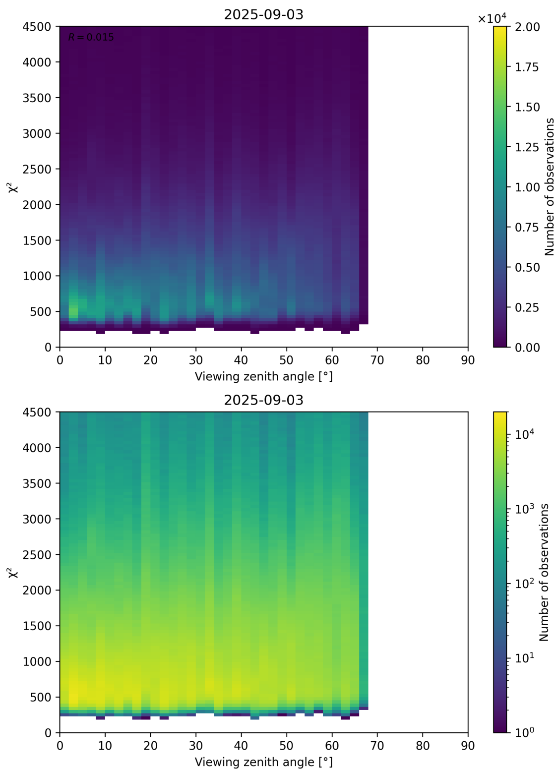
Figure 72: Scatter density plot of “Viewing zenith angle” against “ \chi^2 ” for 2025-09-02 to 2025-09-04.
