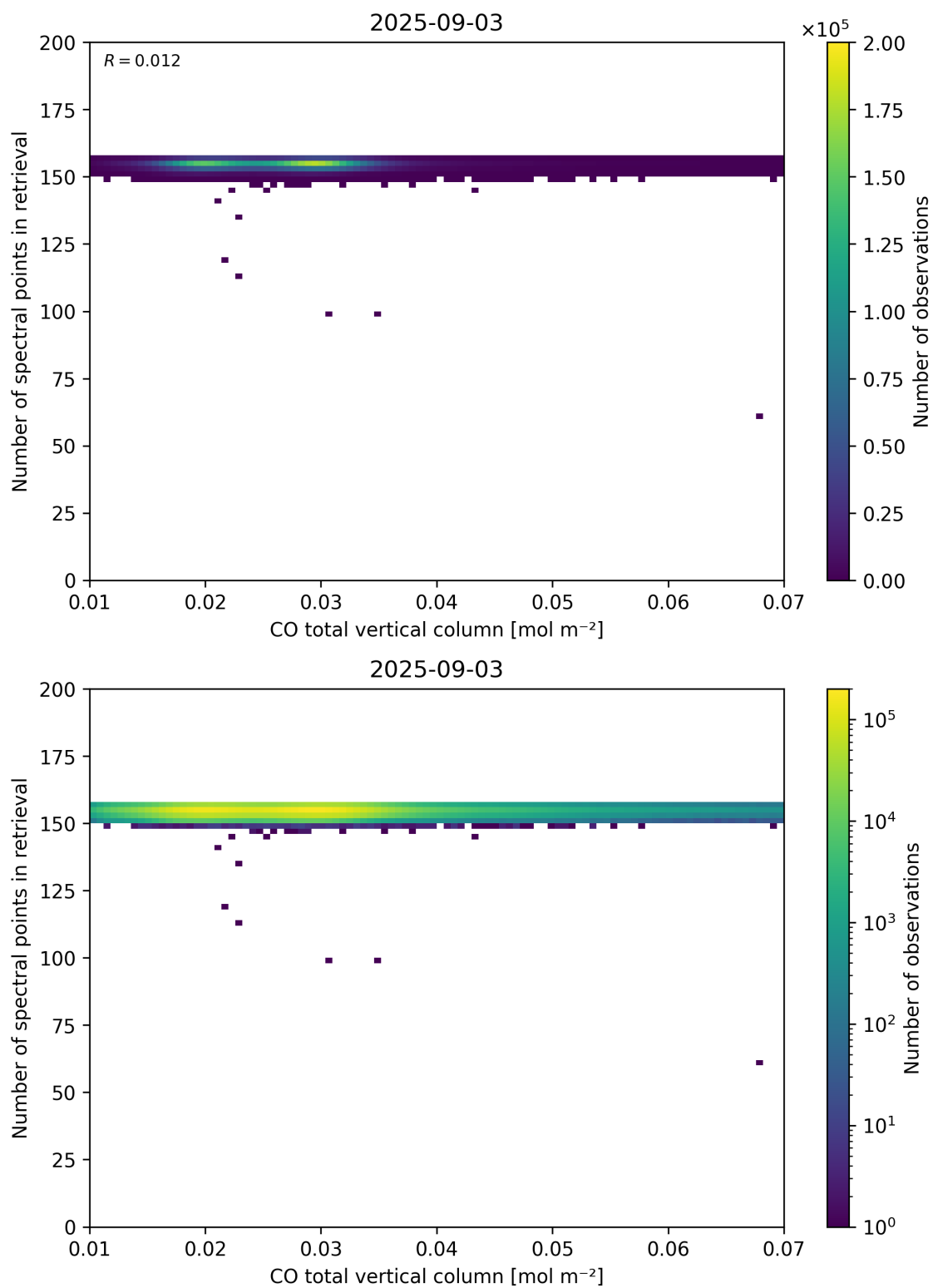
Figure 43: Scatter density plot of “CO total vertical column” against “Number of spectral points in retrieval” for 2025-09-02 to 2025-09-04.
