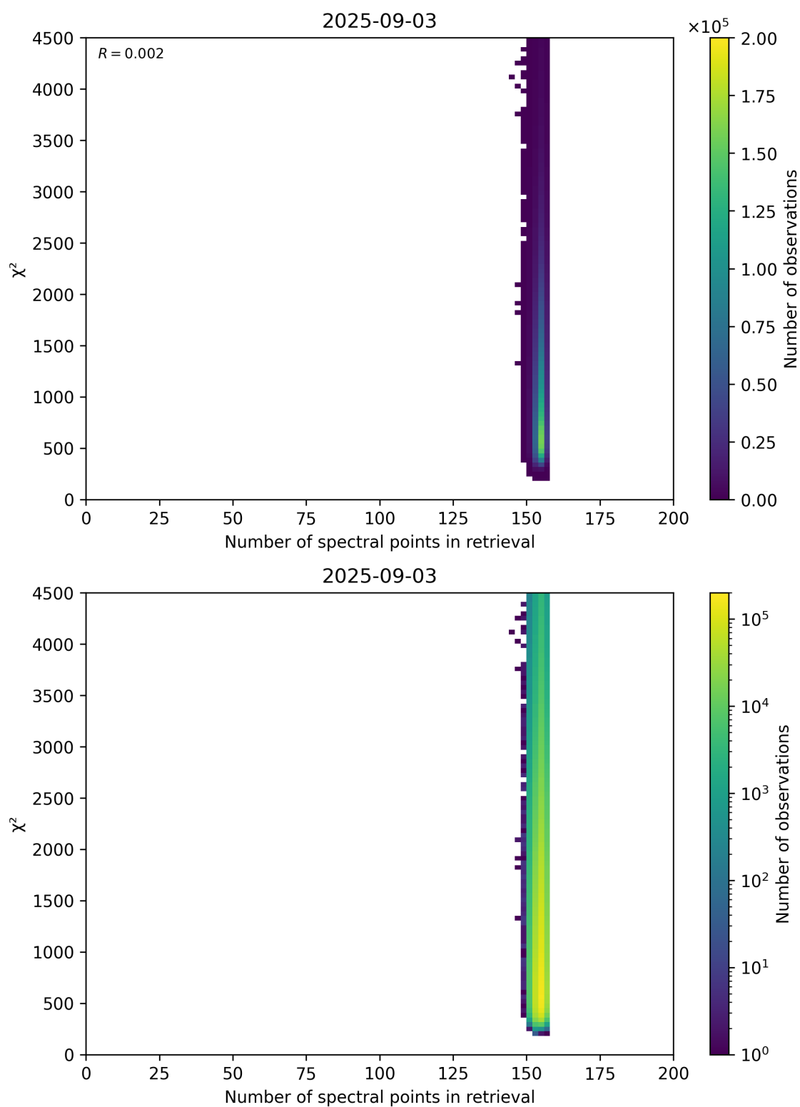
Figure 58: Scatter density plot of “Number of spectral points in retrieval” against “ \chi^2 ” for 2025-09-02 to 2025-09-04.
