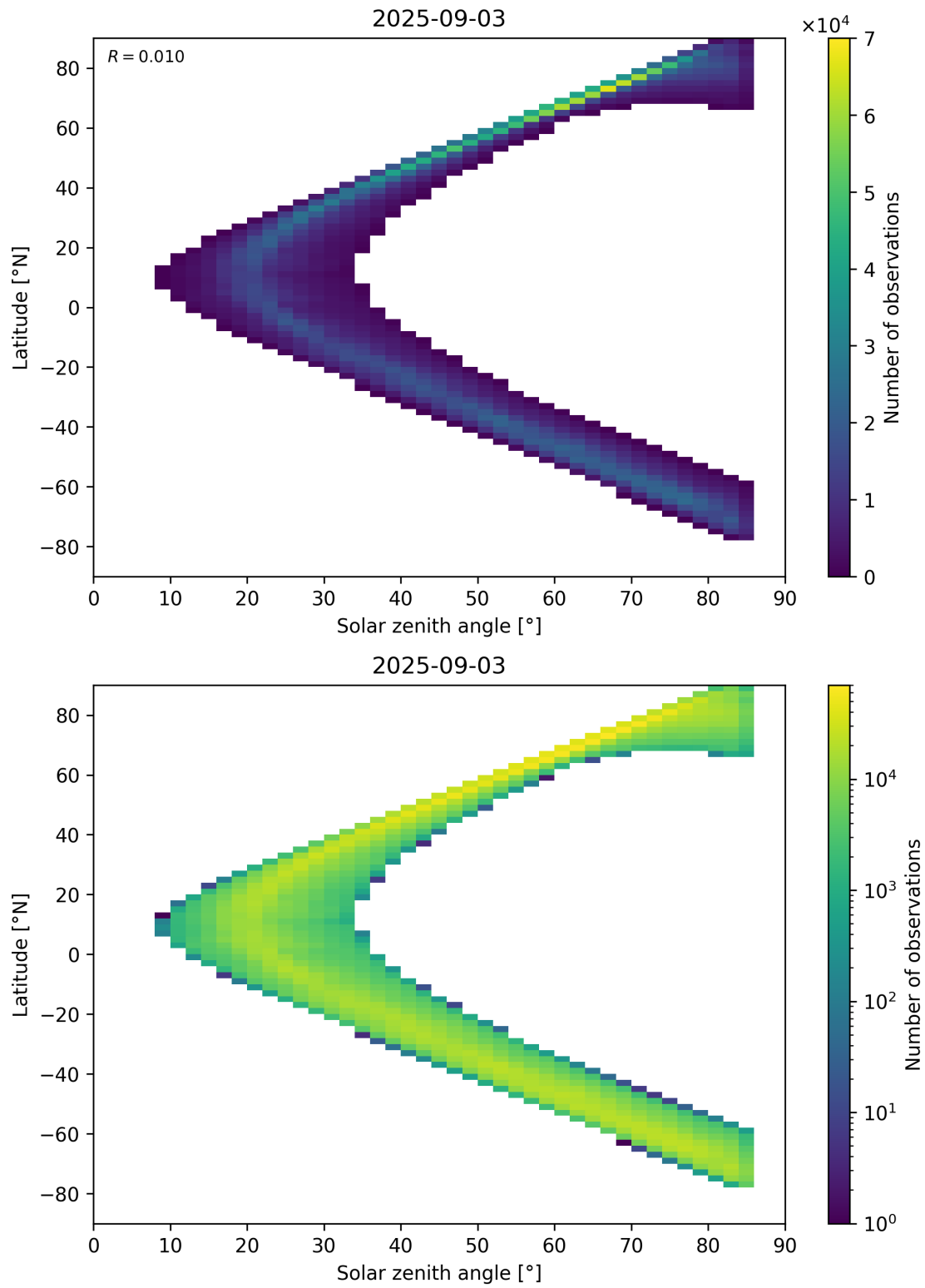
Figure 66: Scatter density plot of “Solar zenith angle” against “Latitude” for 2025-09-02 to 2025-09-04.
