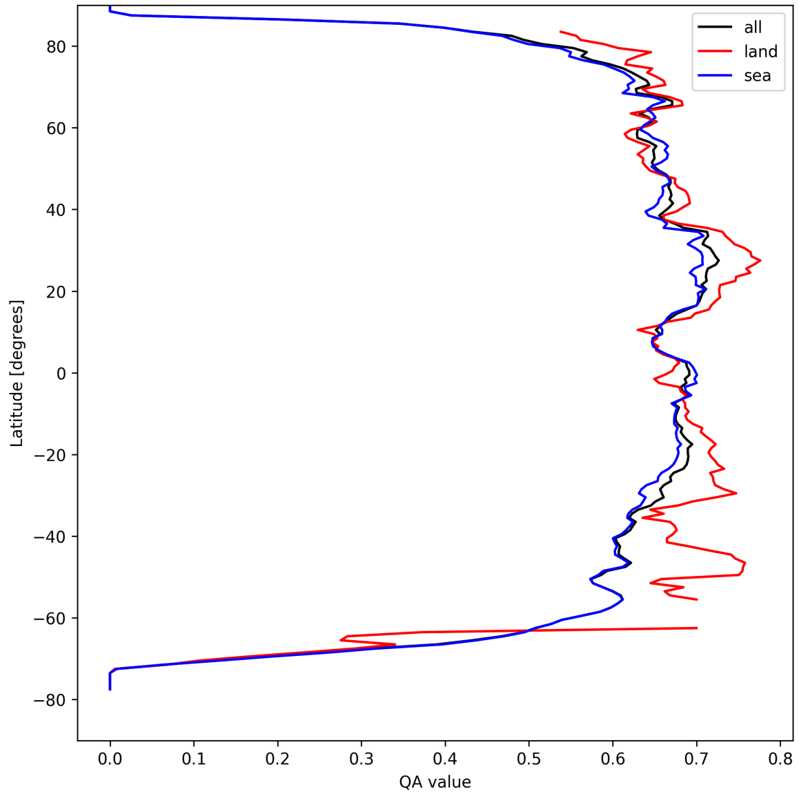
Figure 9: Zonal average of “QA value” for 2025-09-02 to 2025-09-04.
