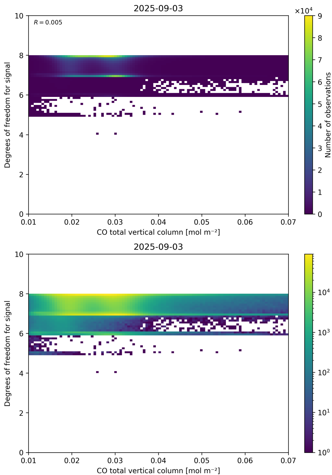
Figure 41: Scatter density plot of “CO total vertical column” against “Degrees of freedom for signal” for 2025-09-02 to 2025-09-04.
