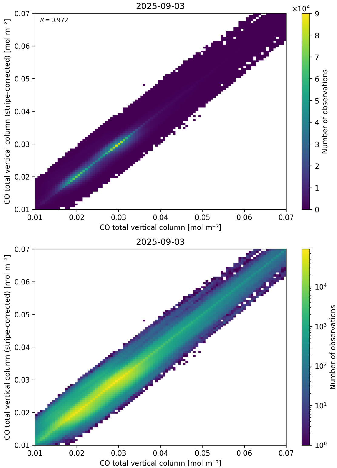
Figure 33: Scatter density plot of “CO total vertical column” against “CO total vertical column (stripe-corrected)” for 2025-09-02 to 2025-09-04.
