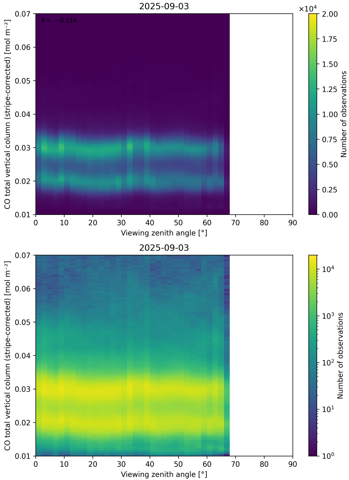
Figure 70: Scatter density plot of “Viewing zenith angle” against “CO total vertical column (stripe-corrected)” for 2025-09-02 to 2025-09-04.
