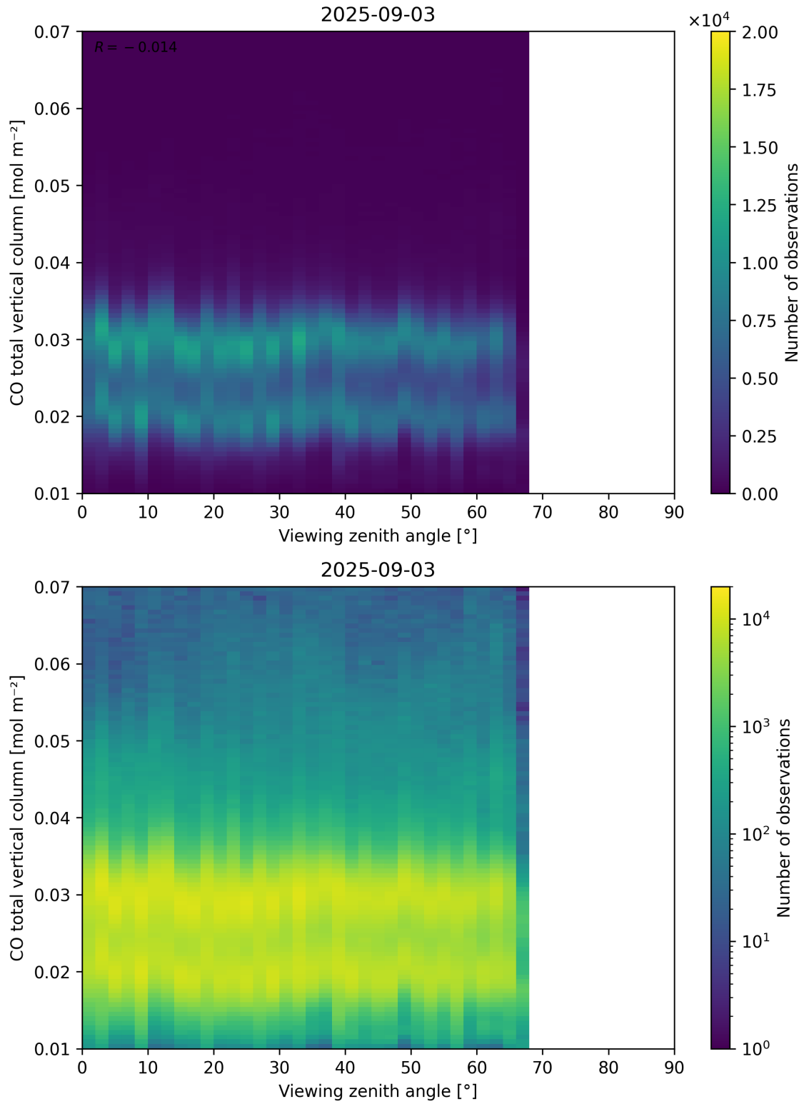
Figure 69: Scatter density plot of “Viewing zenith angle” against “CO total vertical column” for 2025-09-02 to 2025-09-04.
