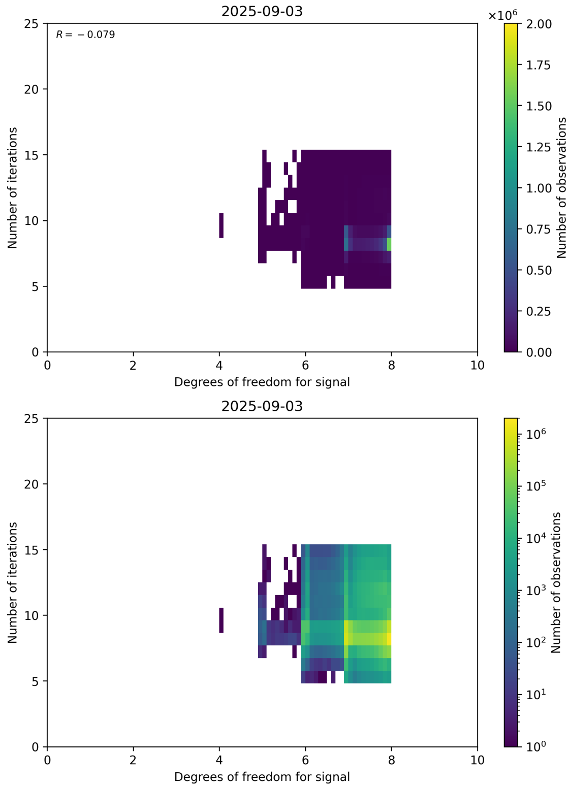
Figure 50: Scatter density plot of “Degrees of freedom for signal” against “Number of iterations” for 2025-09-02 to 2025-09-04.
