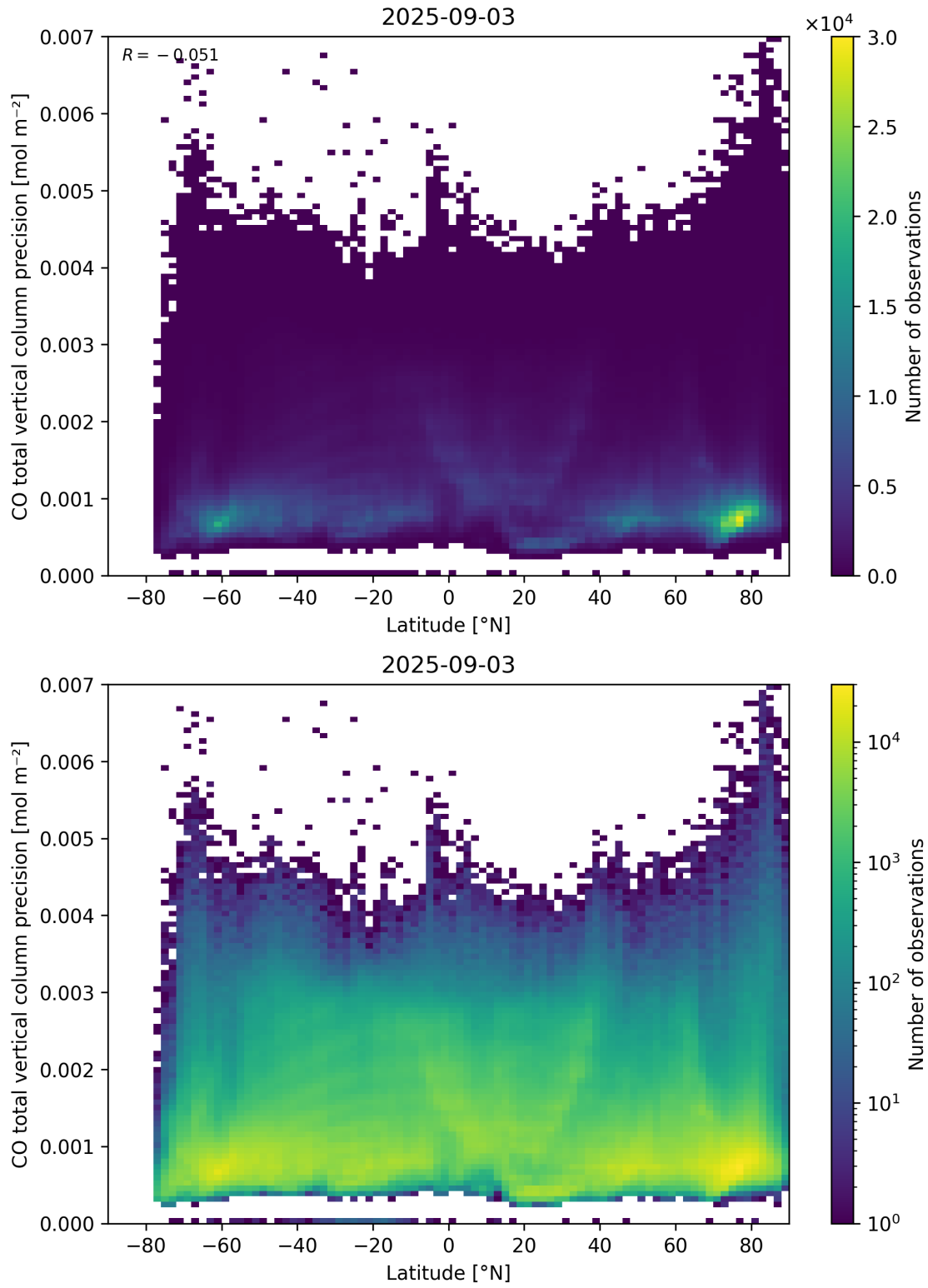
Figure 53: Scatter density plot of “Latitude” against “CO total vertical column precision” for 2025-09-02 to 2025-09-04.
