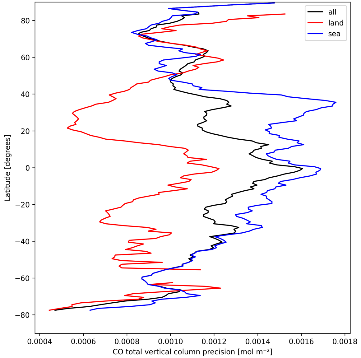
Figure 12: Zonal average of “CO total vertical column precision” for 2025-09-02 to 2025-09-04.
