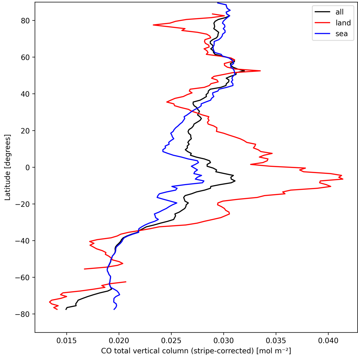
Figure 11: Zonal average of “CO total vertical column (stripe-corrected)” for 2025-09-02 to 2025-09-04.
