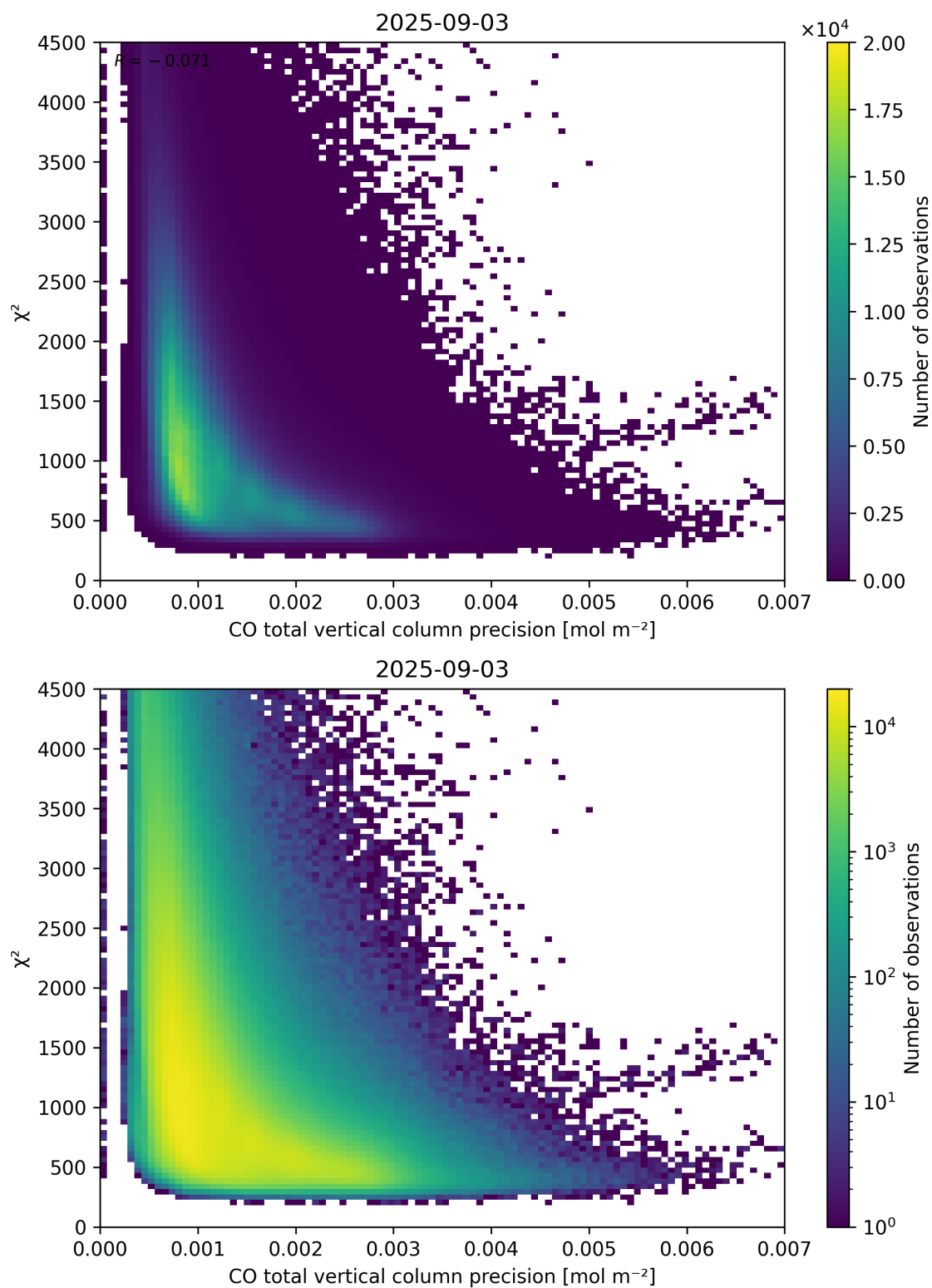
Figure 44: Scatter density plot of “CO total vertical column precision” against “ \chi^2 ” for 2025-09-02 to 2025-09-04.
