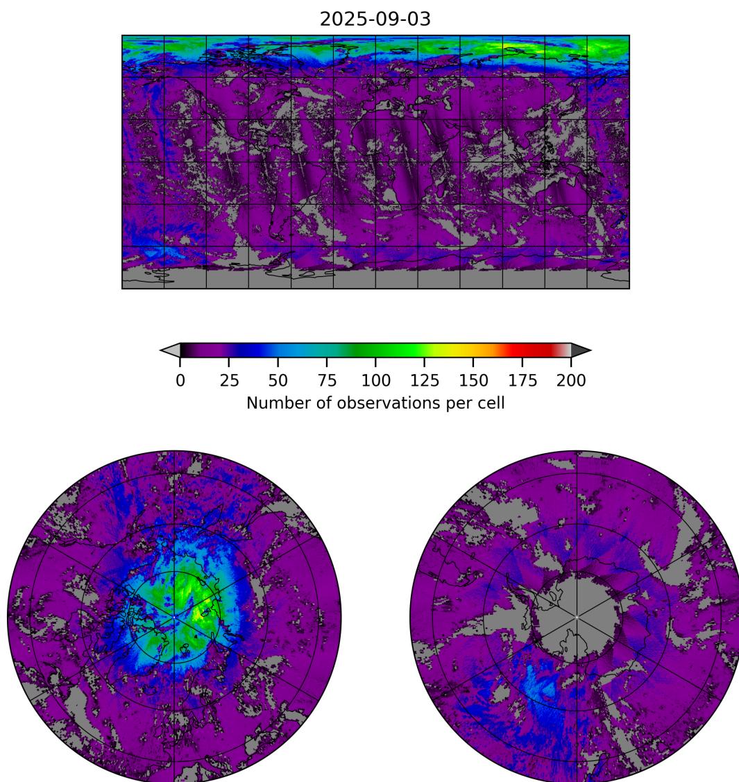
Figure 8: Map of the number of observations for 2025-09-02 to 2025-09-04
