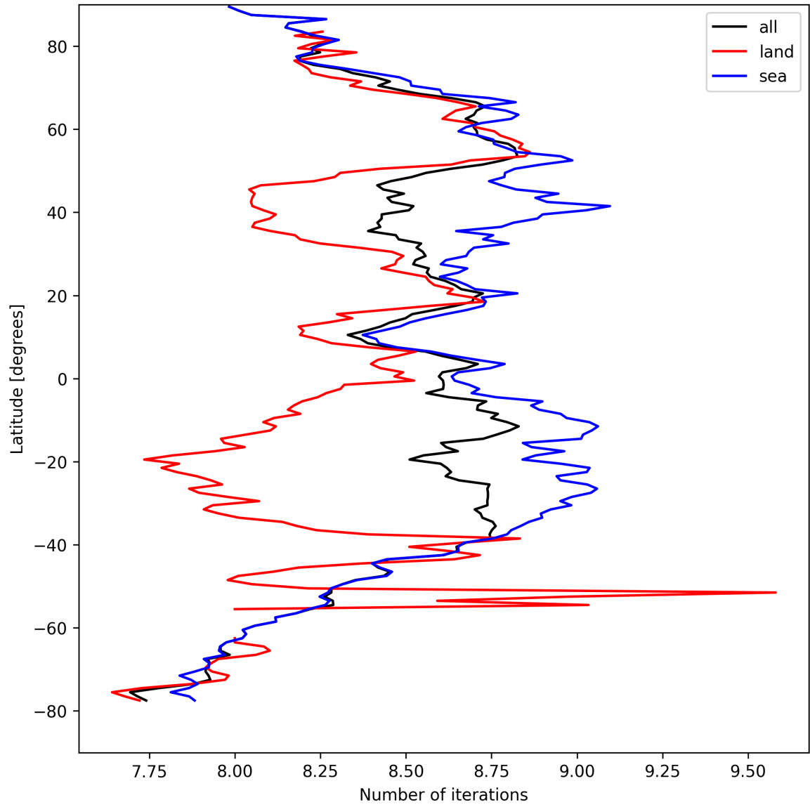
Figure 16: Zonal average of “Number of iterations” for 2025-09-02 to 2025-09-04.
