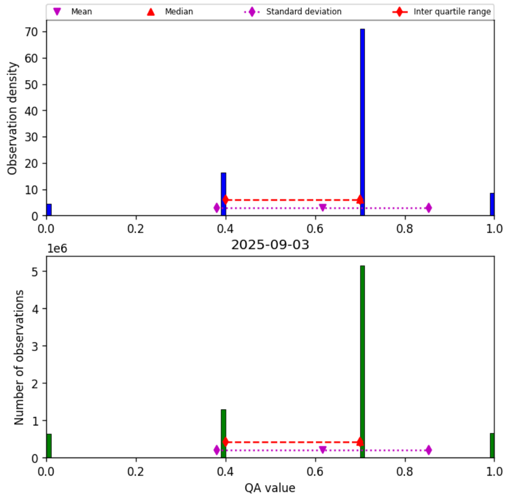
Figure 17: Histogram of “QA value” for 2025-09-02 to 2025-09-04
