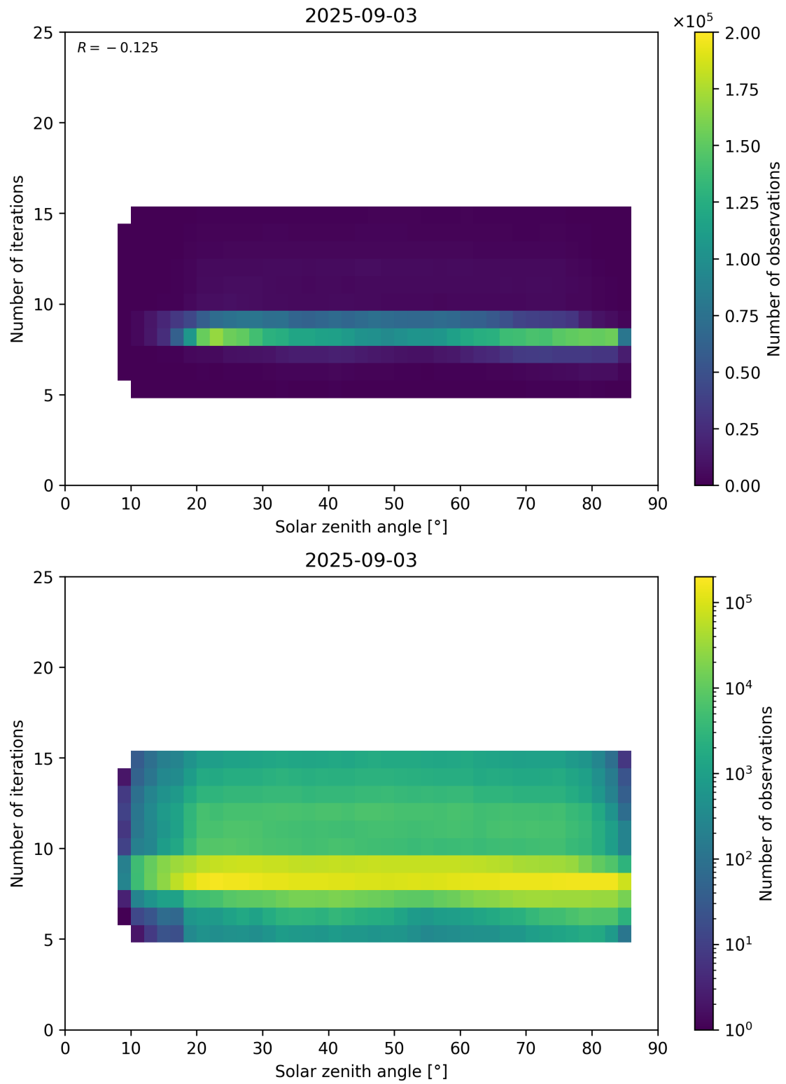
Figure 67: Scatter density plot of “Solar zenith angle” against “Number of iterations” for 2025-09-02 to 2025-09-04.
