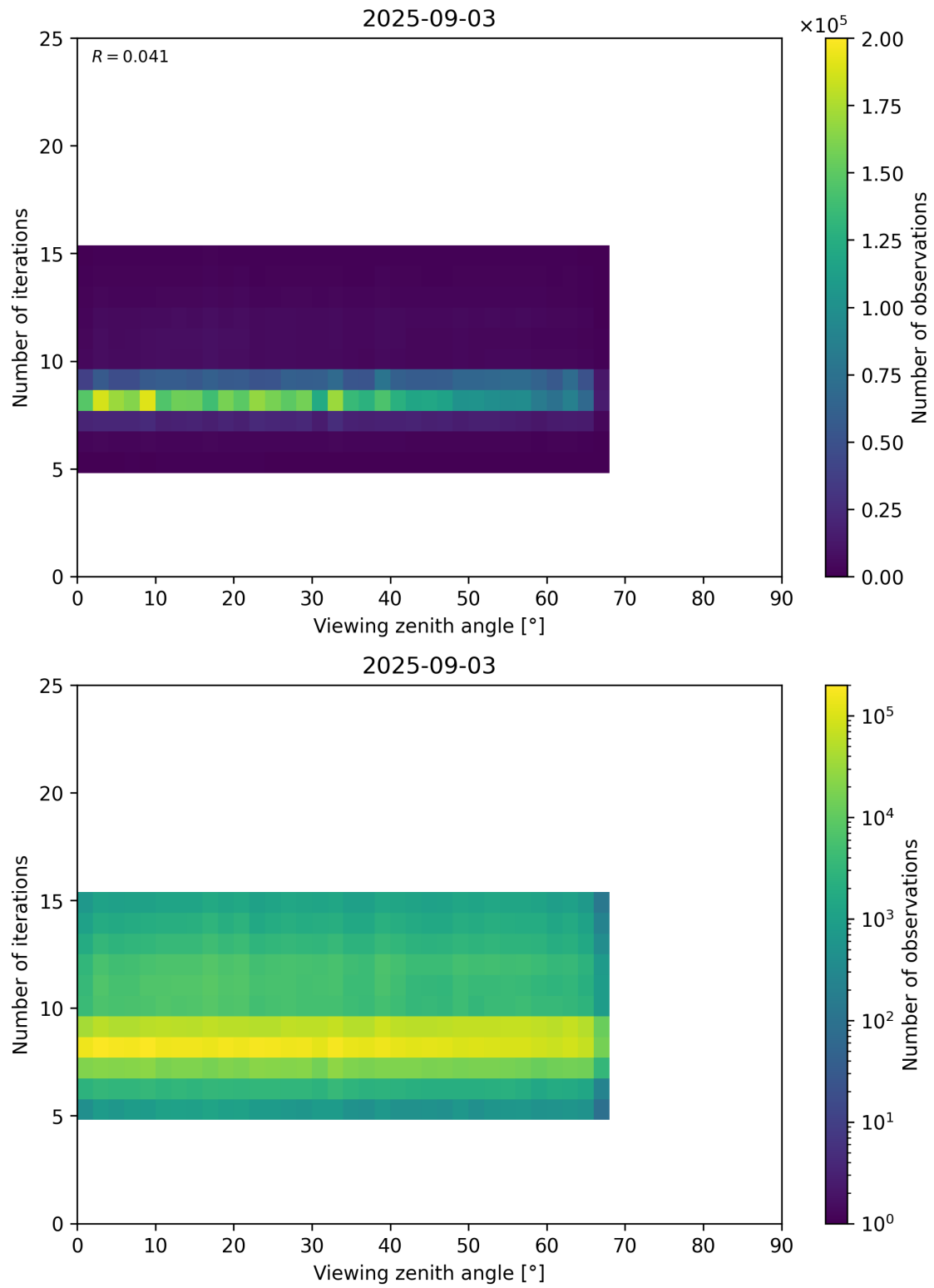
Figure 75: Scatter density plot of “Viewing zenith angle” against “Number of iterations” for 2025-09-02 to 2025-09-04.
