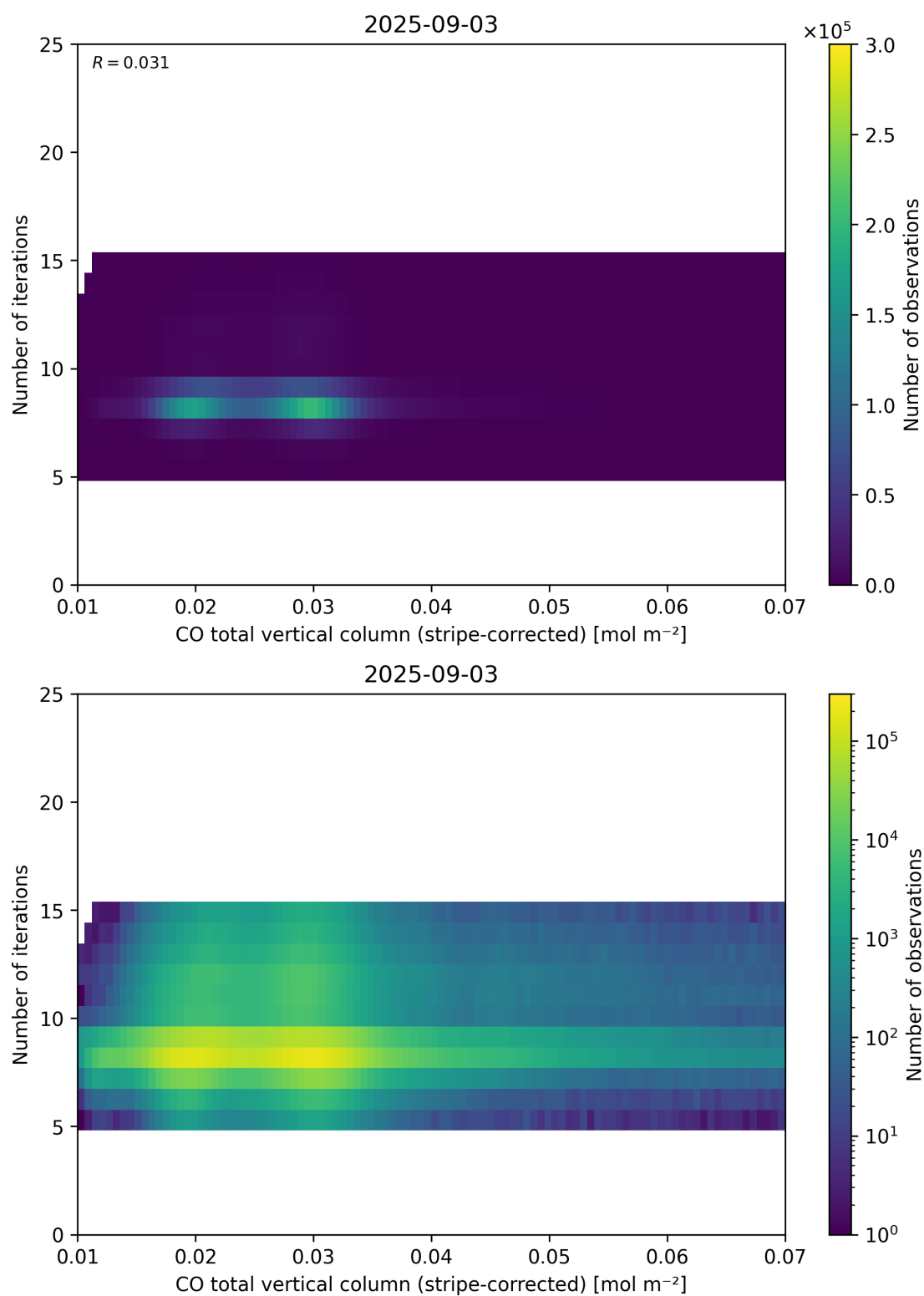
Figure 39: Scatter density plot of “CO total vertical column (stripe-corrected)” against “Number of iterations” for 2025-09-02 to 2025-09-04.
