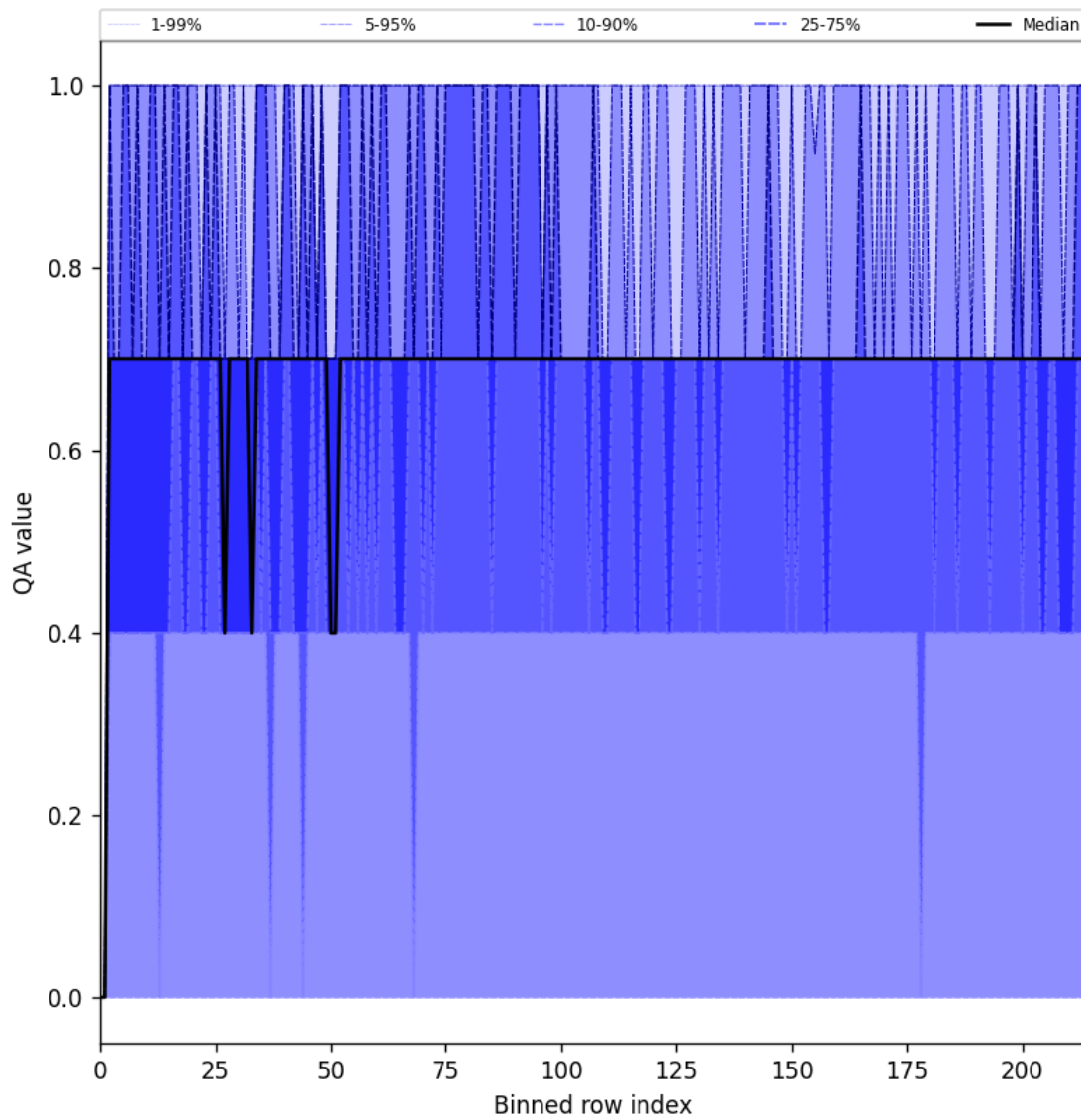
Figure 25: Along track statistics of "QA value" for 2025-09-02 to 2025-09-04
