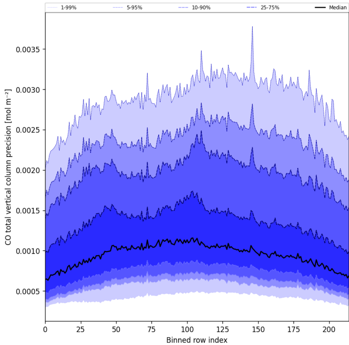
Figure 28: Along track statistics of “CO total vertical column precision” for 2025-09-02 to 2025-09-04
