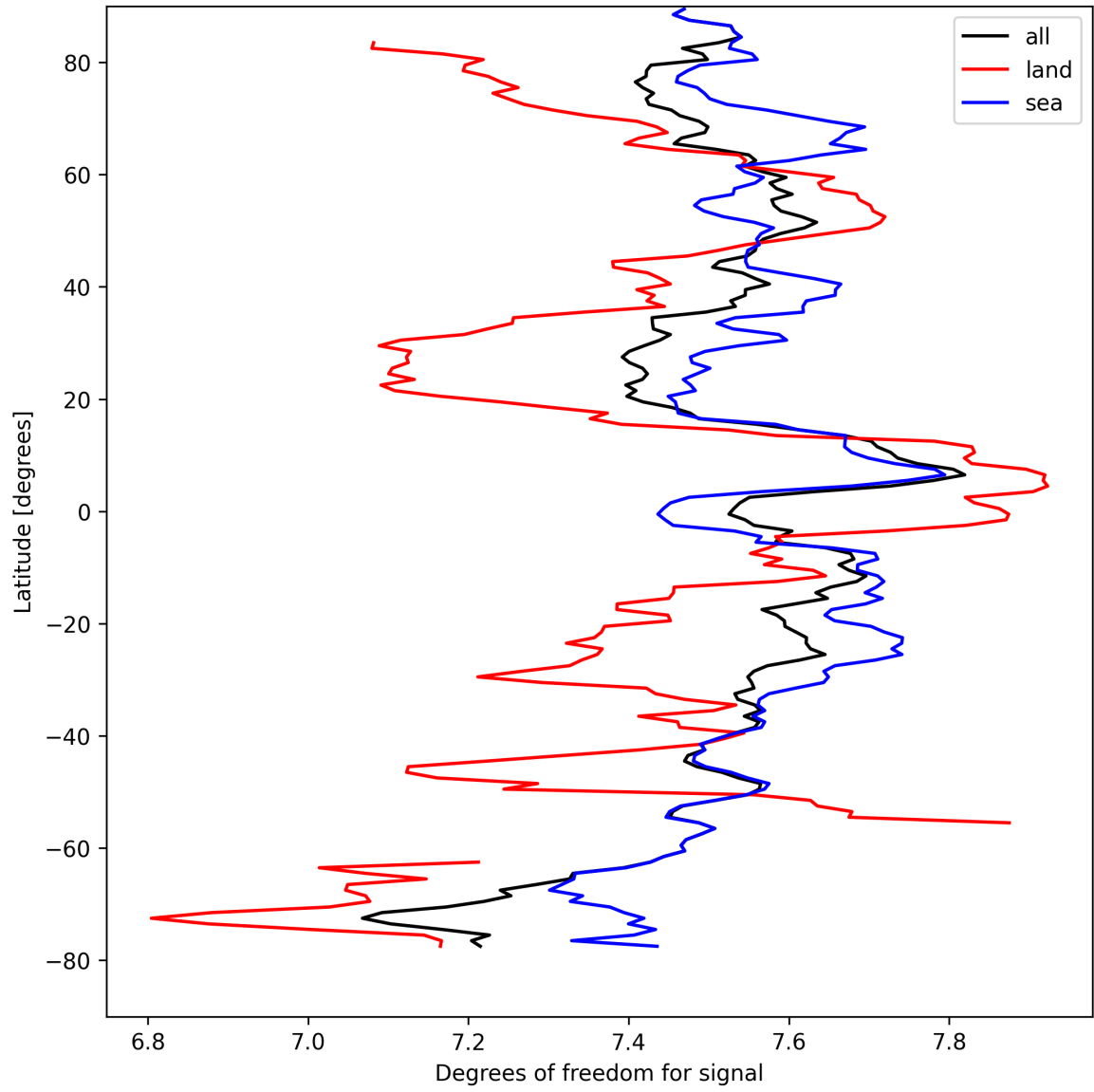
Figure 15: Zonal average of “Degrees of freedom for signal” for 2025-09-02 to 2025-09-04.
