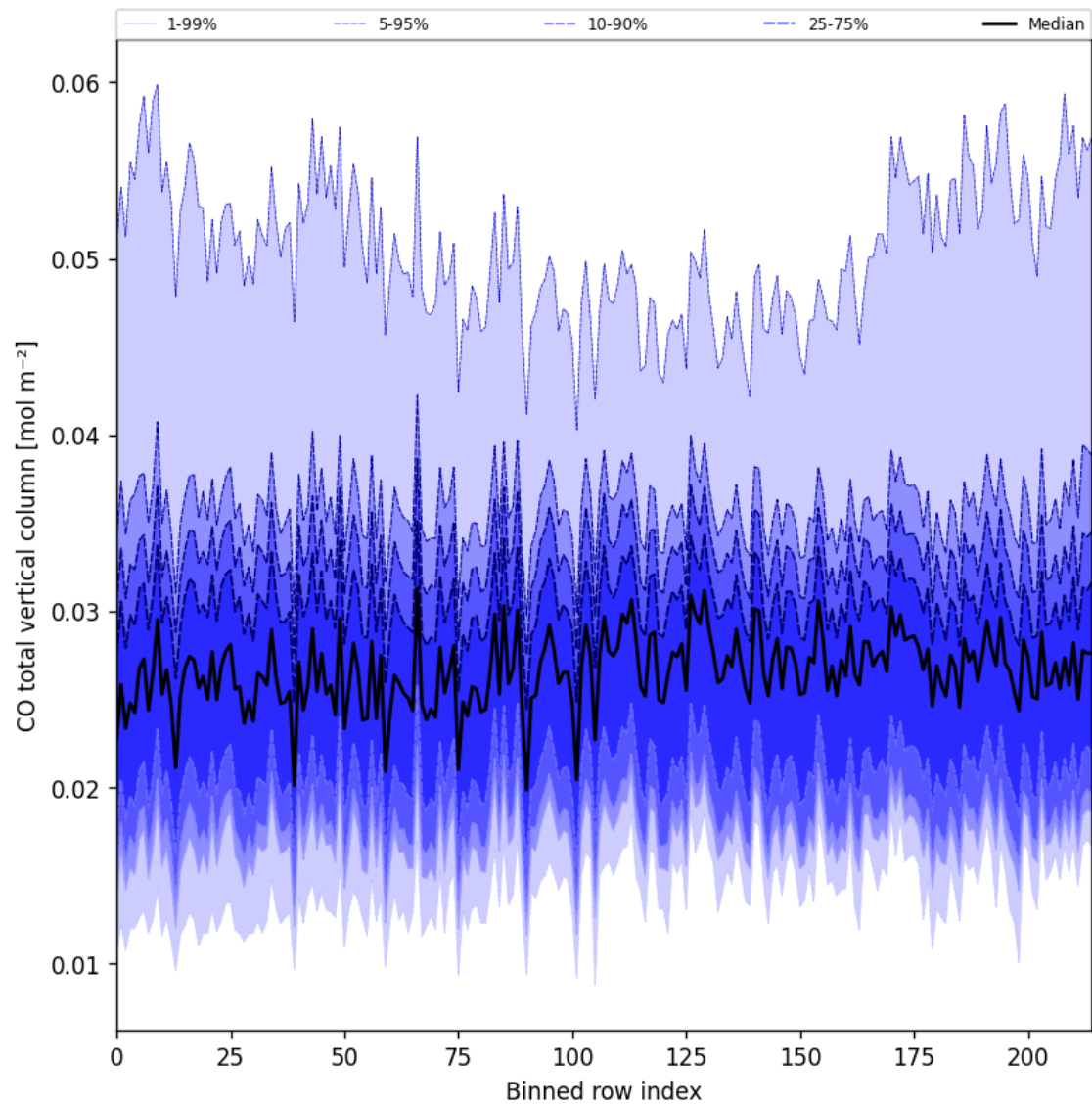
Figure 26: Along track statistics of “CO total vertical column” for 2025-09-02 to 2025-09-04
