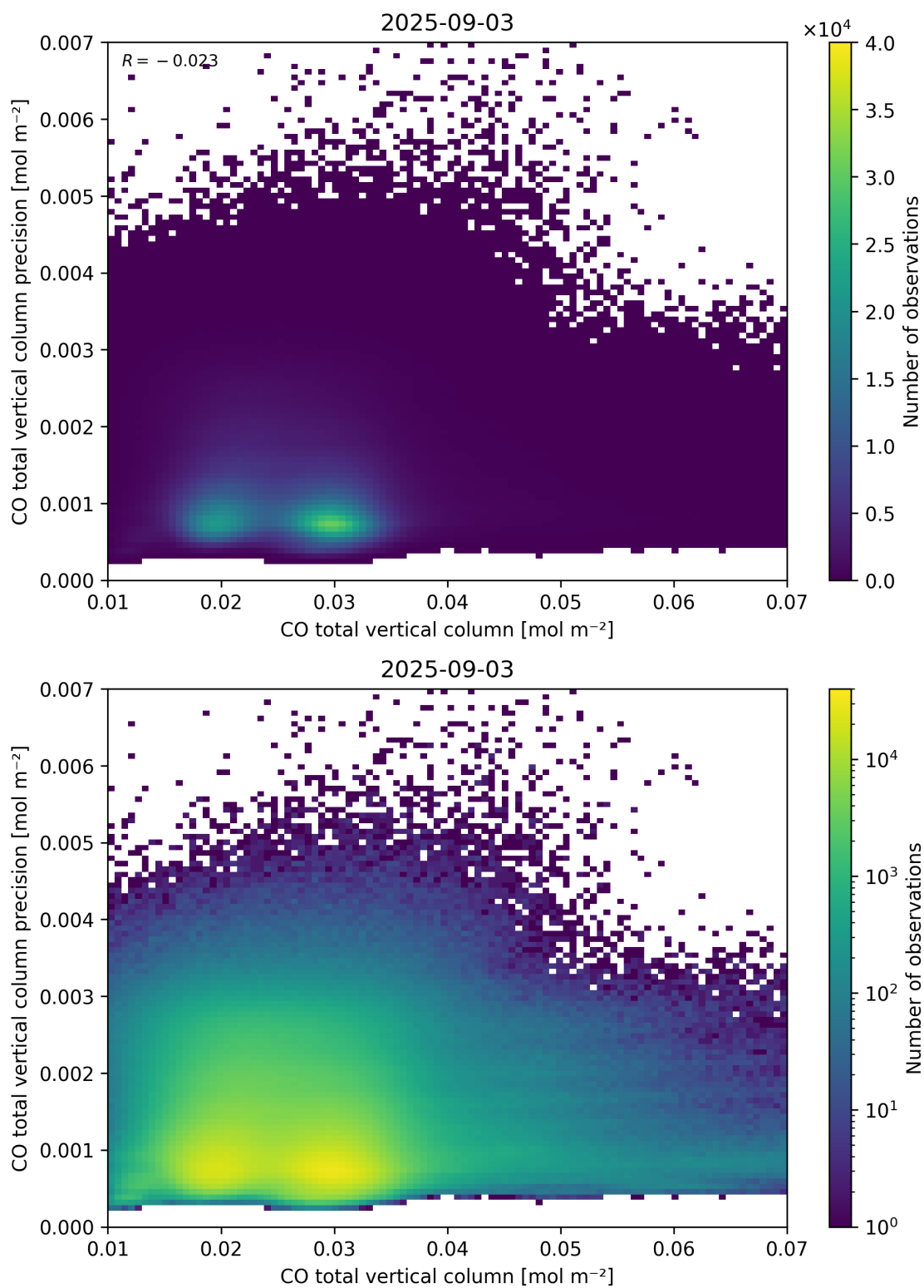
Figure 34: Scatter density plot of “CO total vertical column” against “CO total vertical column precision” for 2025-09-02 to 2025-09-04.
