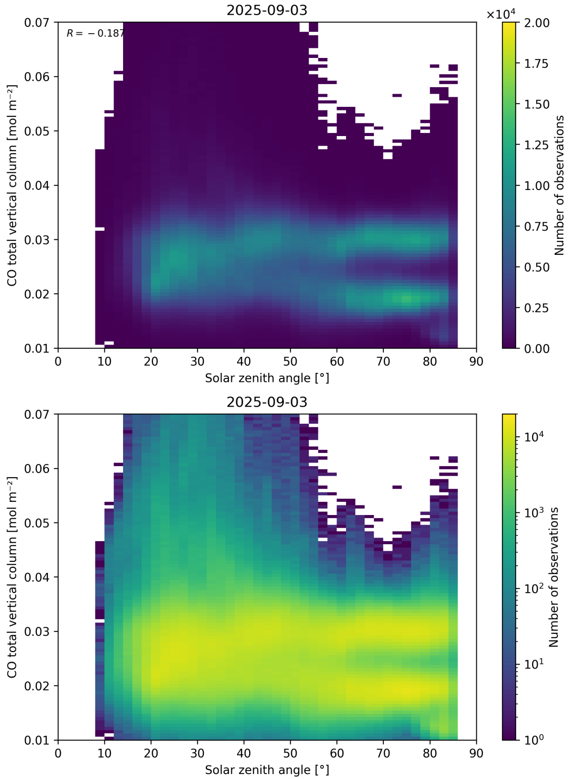
Figure 61: Scatter density plot of “Solar zenith angle” against “CO total vertical column” for 2025-09-02 to 2025-09-04.
