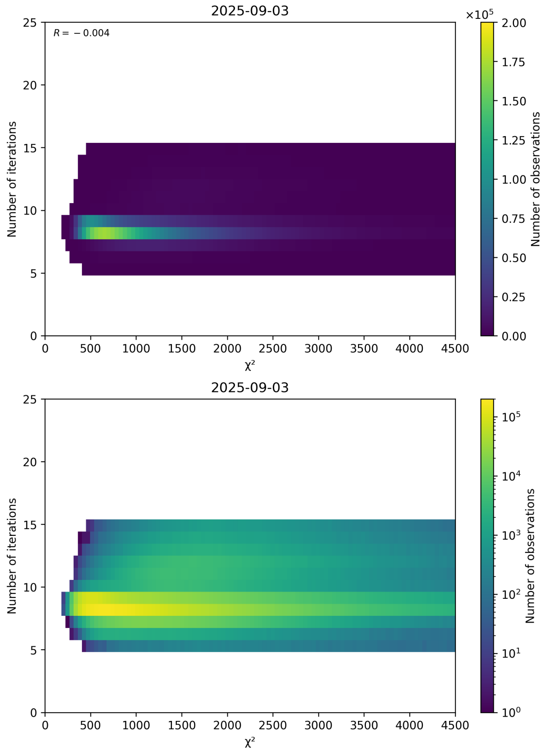
Figure 49: Scatter density plot of “ \chi^2 ” against “Number of iterations” for 2025-09-02 to 2025-09-04.
