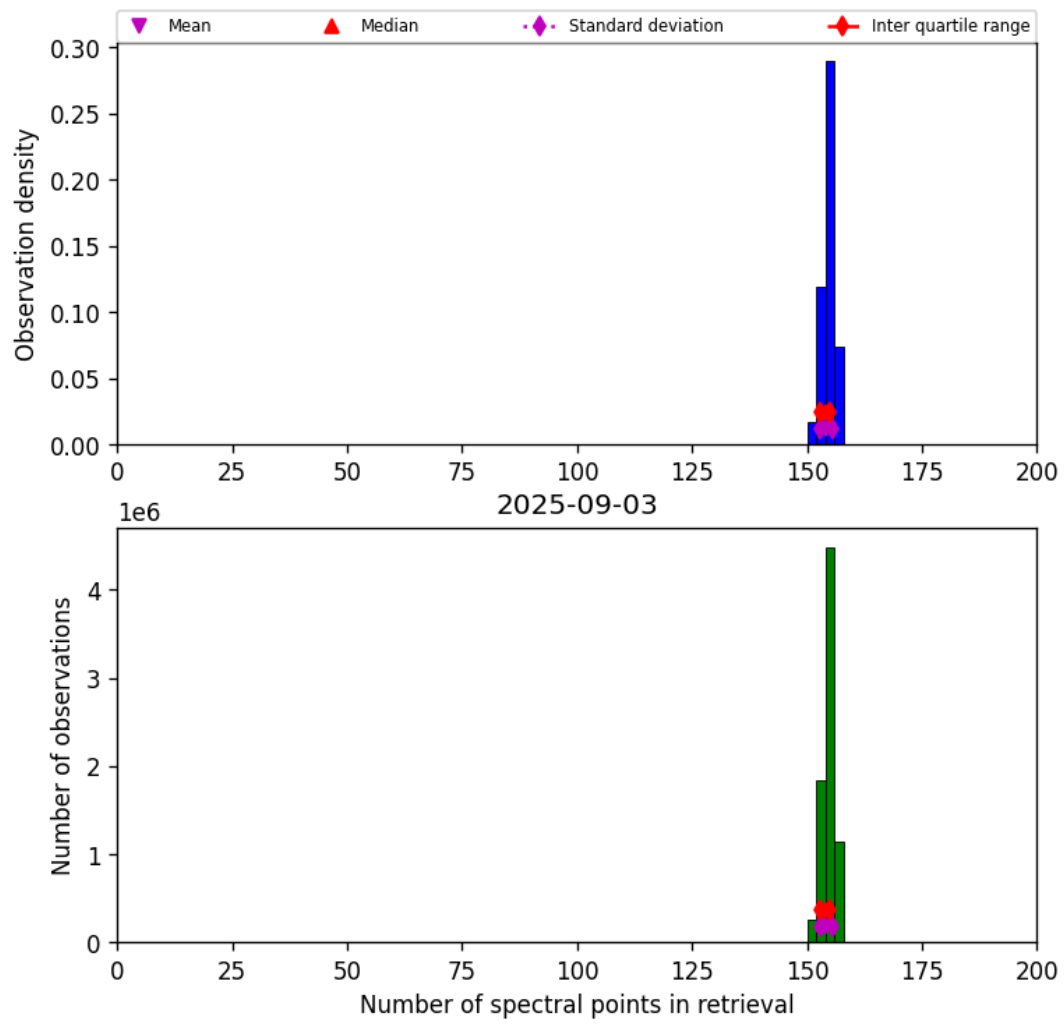
Figure 21: Histogram of “Number of spectral points in retrieval” for 2025-09-02 to 2025-09-04
