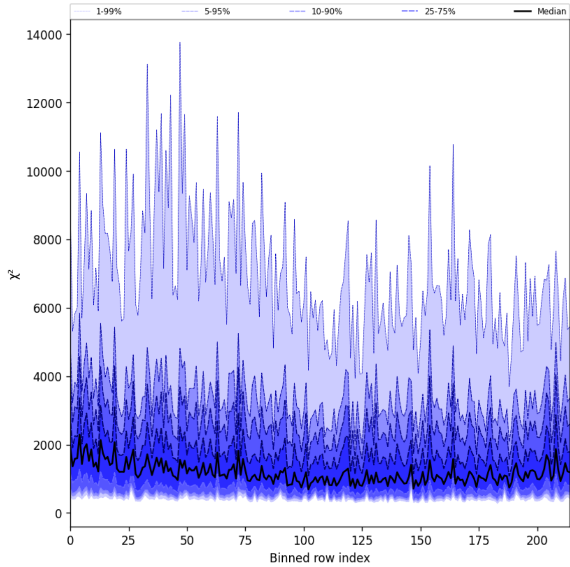
Figure 30: Along track statistics of “ \chi^2 ” for 2025-09-02 to 2025-09-04
