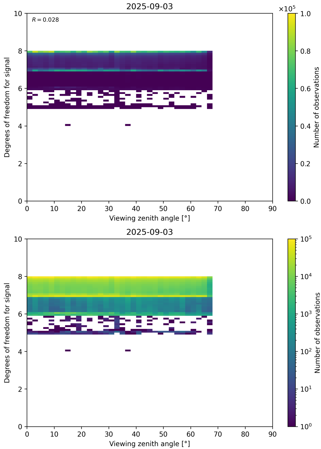
Figure 73: Scatter density plot of “Viewing zenith angle” against “Degrees of freedom for signal” for 2025-09-02 to 2025-09-04.
