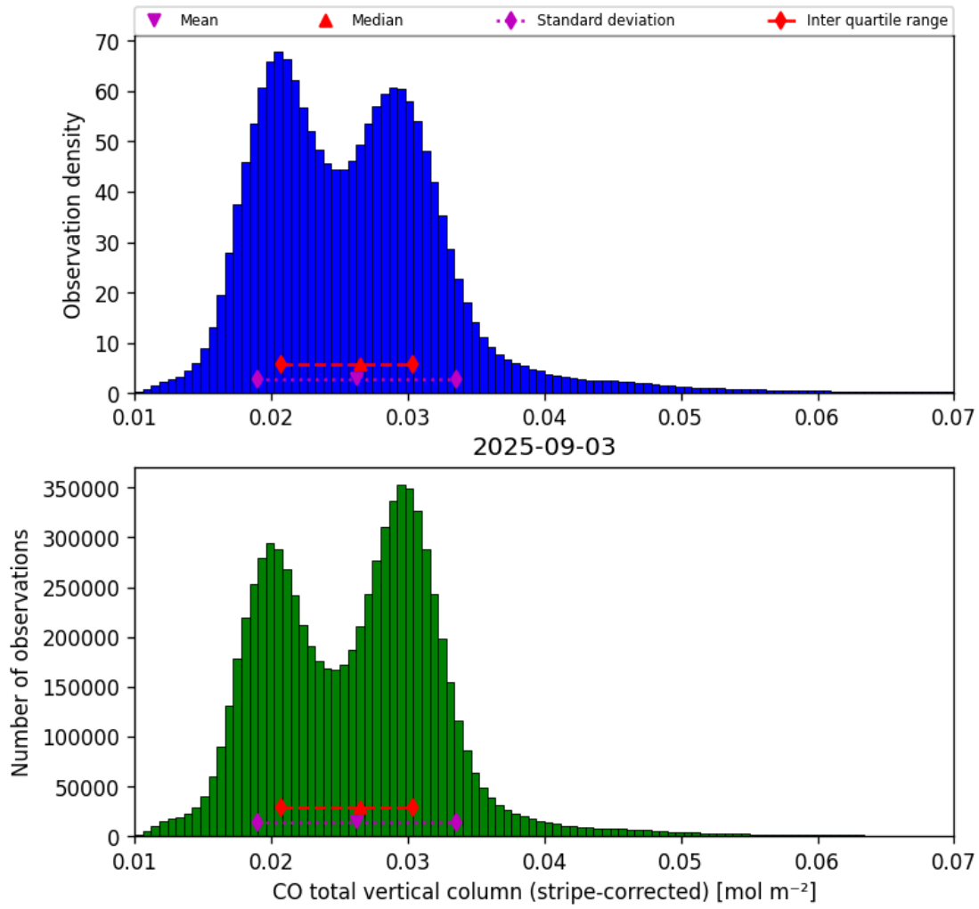
Figure 19: Histogram of “CO total vertical column (stripe-corrected)” for 2025-09-02 to 2025-09-04
