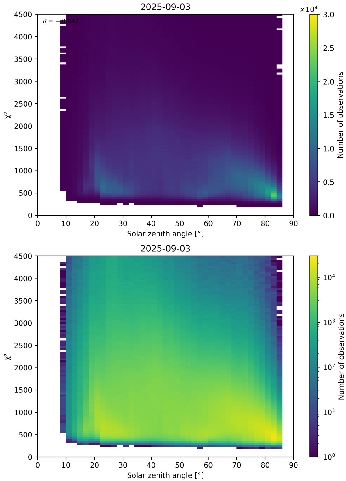
Figure 64: Scatter density plot of “Solar zenith angle” against “ \chi^2 ” for 2025-09-02 to 2025-09-04.
