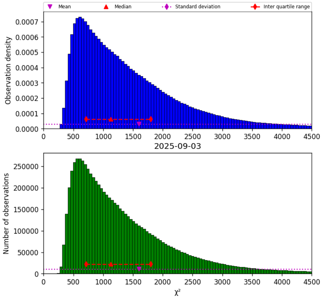
Figure 22: Histogram of “ \chi^2 ” for 2025-09-02 to 2025-09-04
