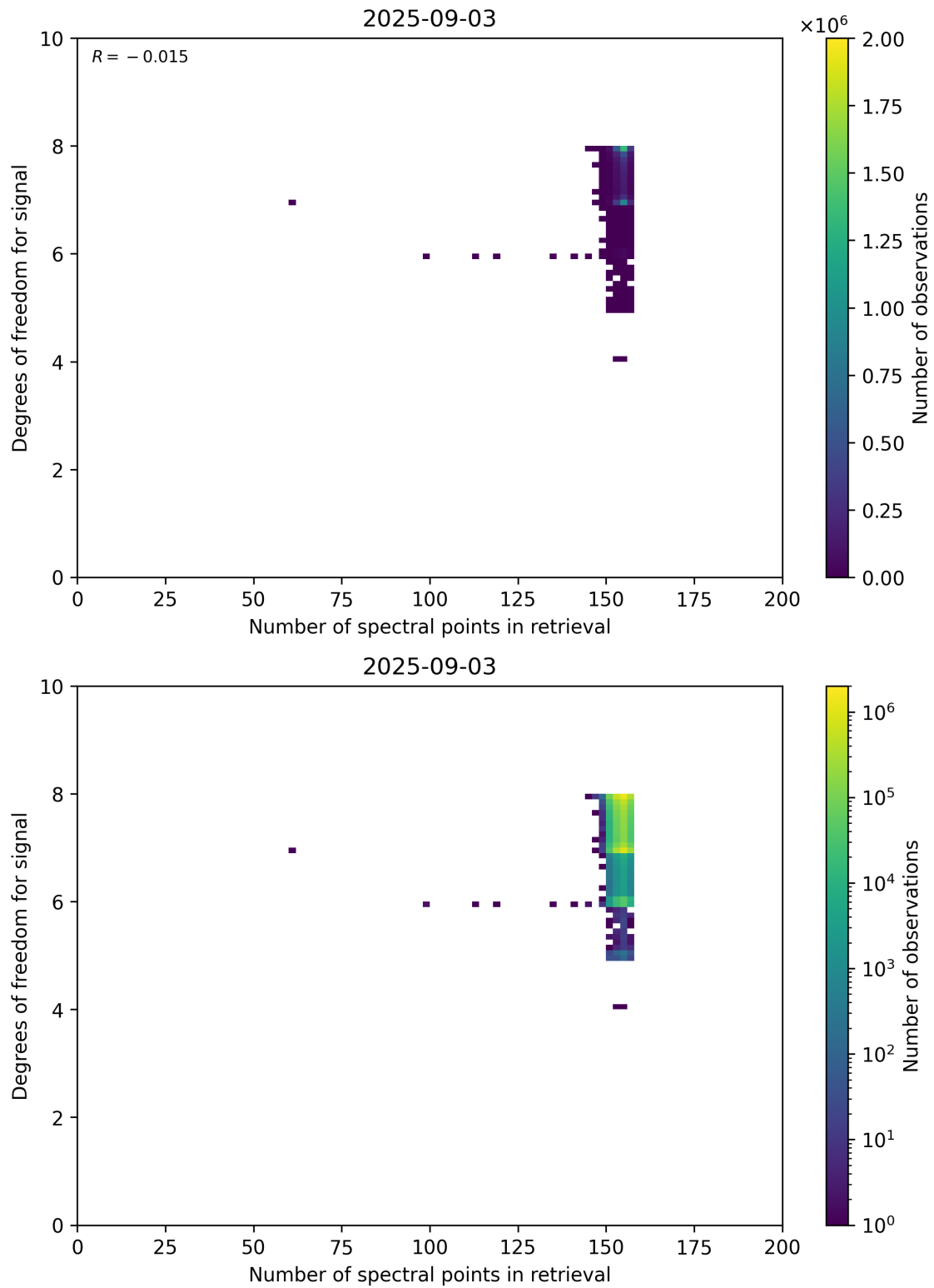
Figure 59: Scatter density plot of “Number of spectral points in retrieval” against “Degrees of freedom for signal” for 2025-09-02 to 2025-09-04.
