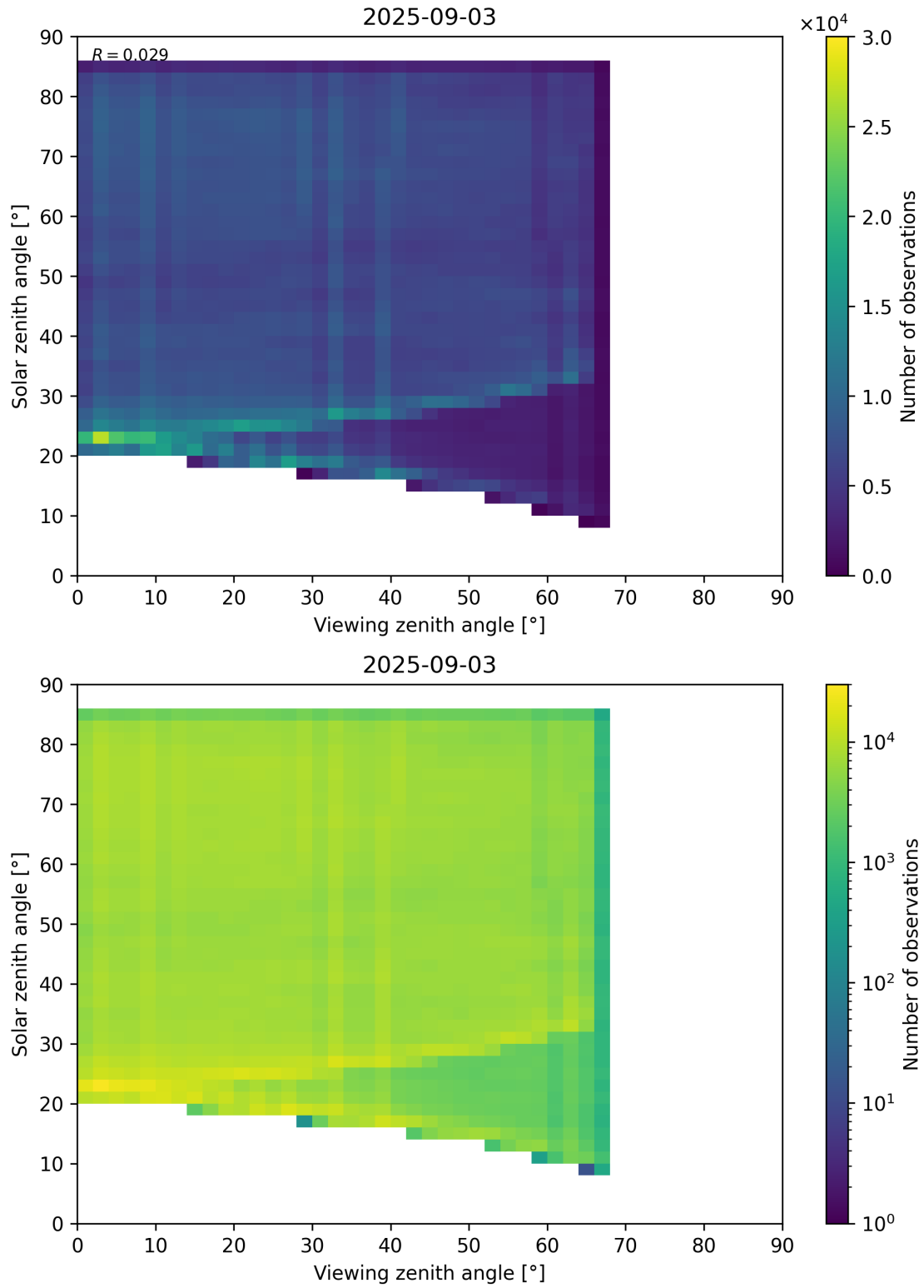
Figure 77: Scatter density plot of “Viewing zenith angle” against “Solar zenith angle” for 2025-09-02 to 2025-09-04.
