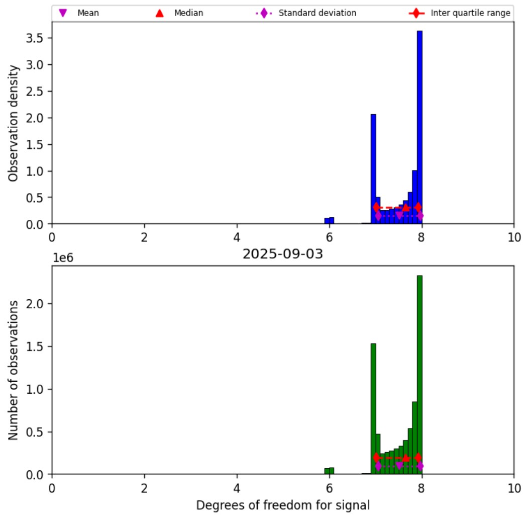
Figure 23: Histogram of “Degrees of freedom for signal” for 2025-09-02 to 2025-09-04
