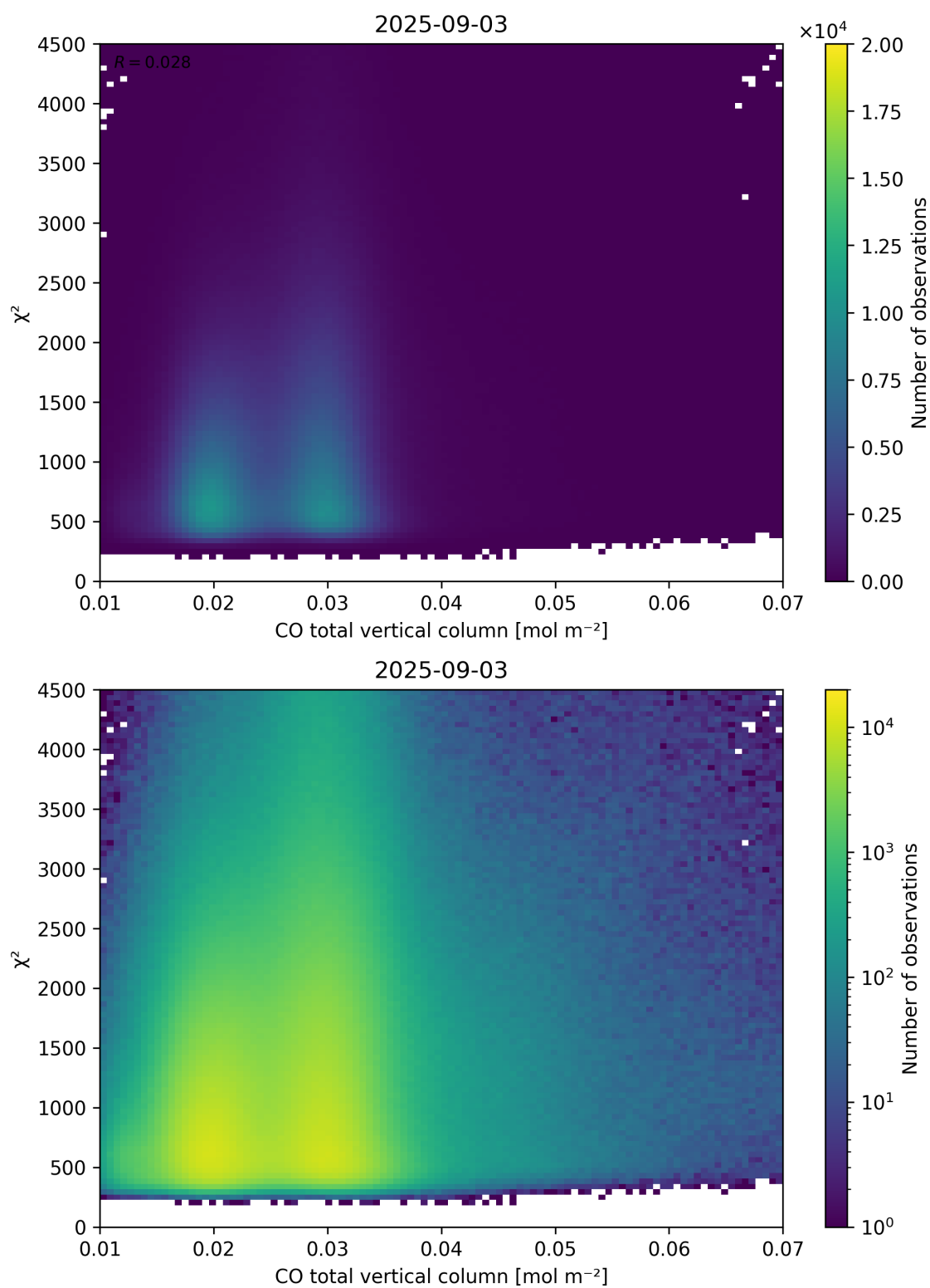
Figure 35: Scatter density plot of “CO total vertical column” against “ \chi^2 ” for 2025-09-02 to 2025-09-04.
