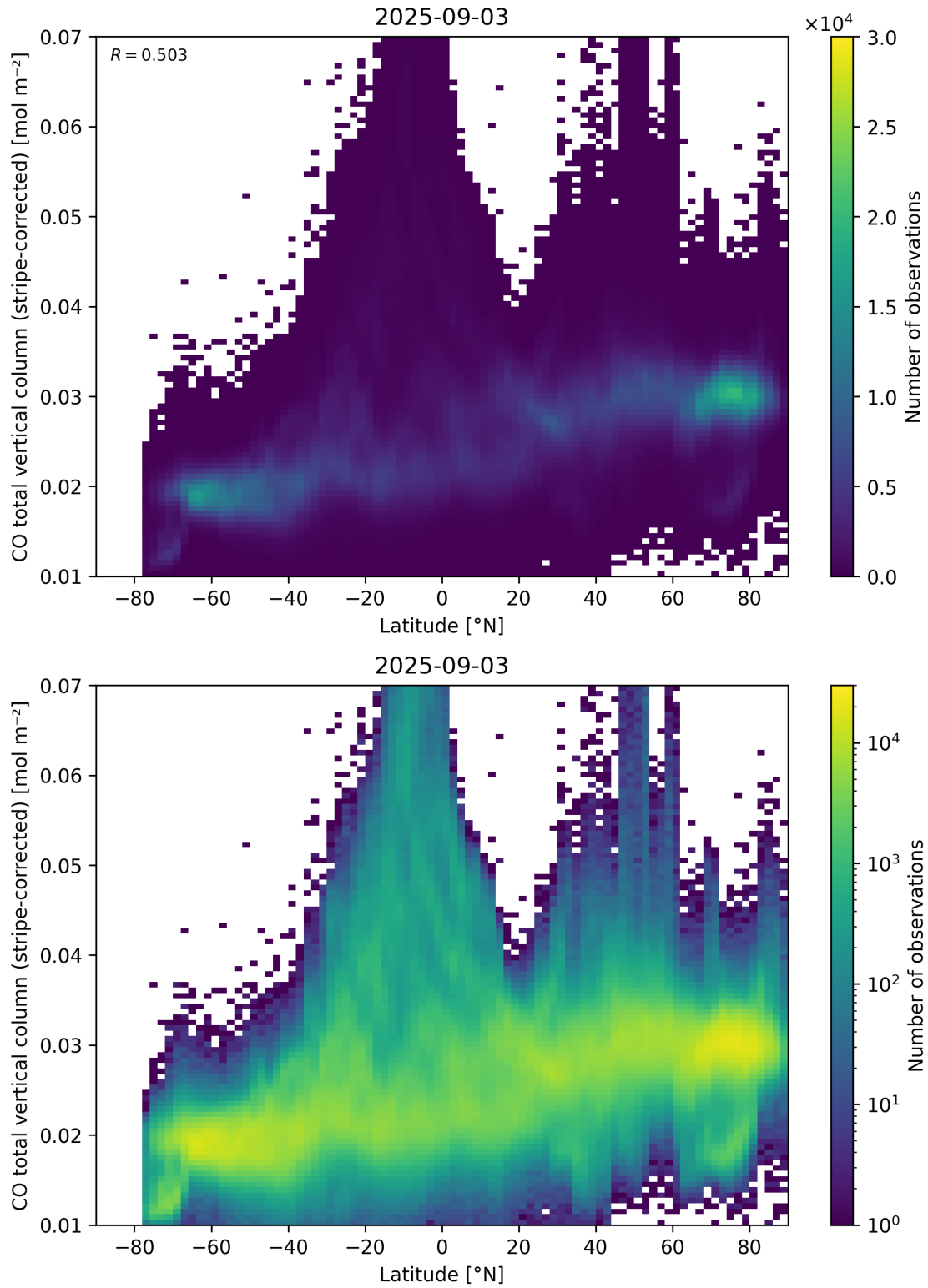
Figure 52: Scatter density plot of “Latitude” against “CO total vertical column (stripe-corrected)” for 2025-09-02 to 2025-09-04.
