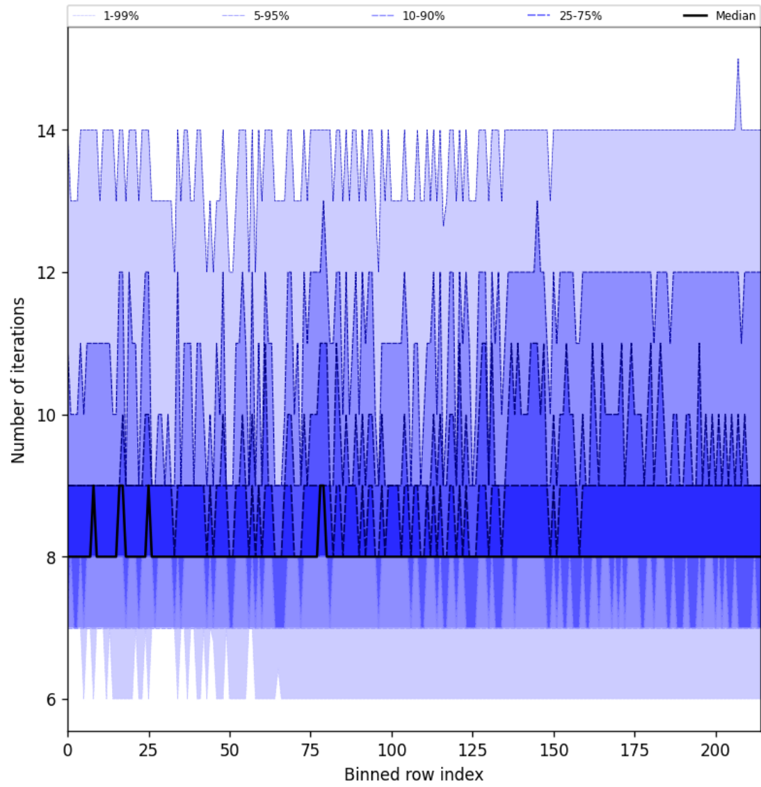
Figure 32: Along track statistics of “Number of iterations” for 2025-09-02 to 2025-09-04
