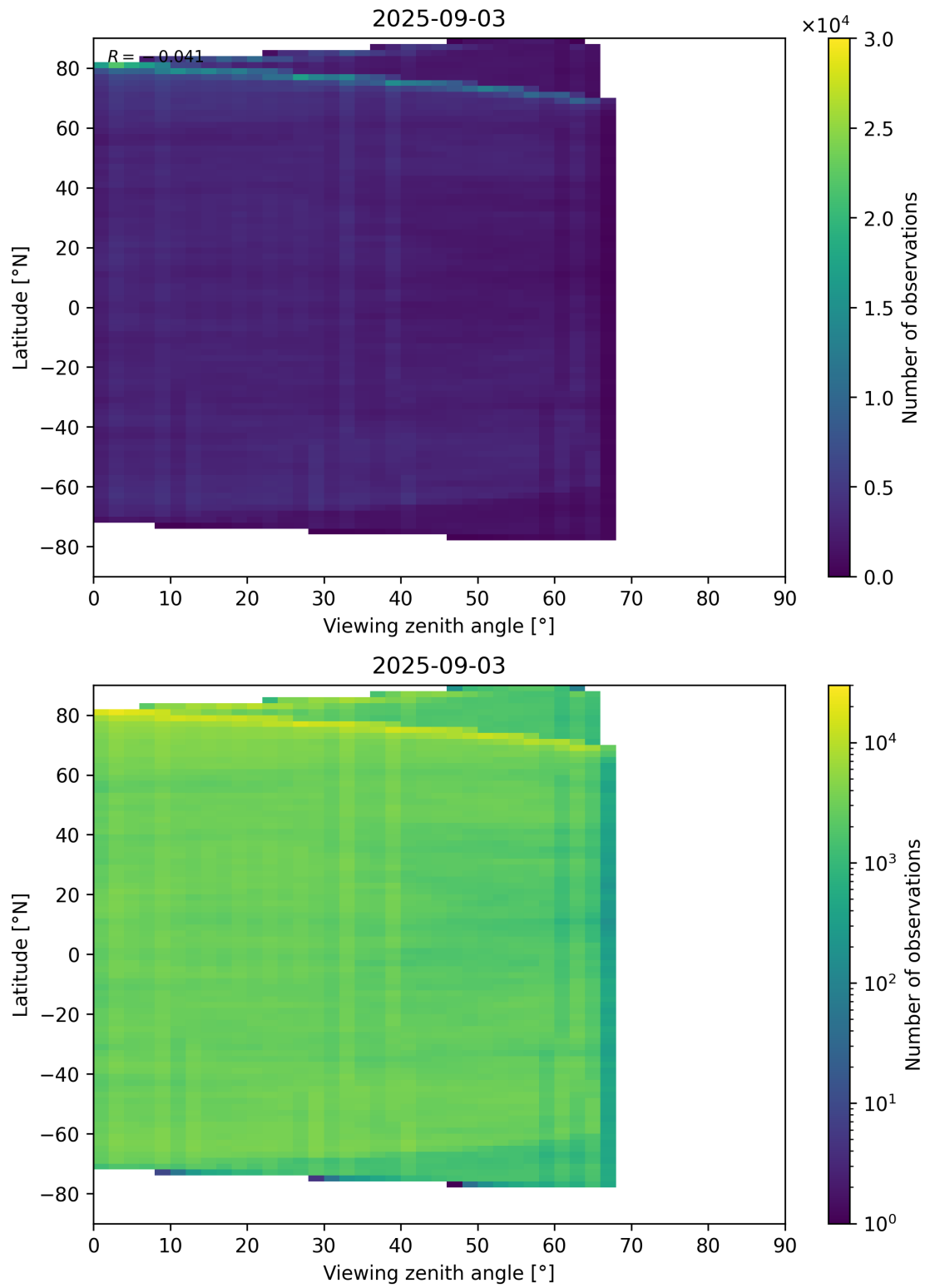
Figure 74: Scatter density plot of “Viewing zenith angle” against “Latitude” for 2025-09-02 to 2025-09-04.
