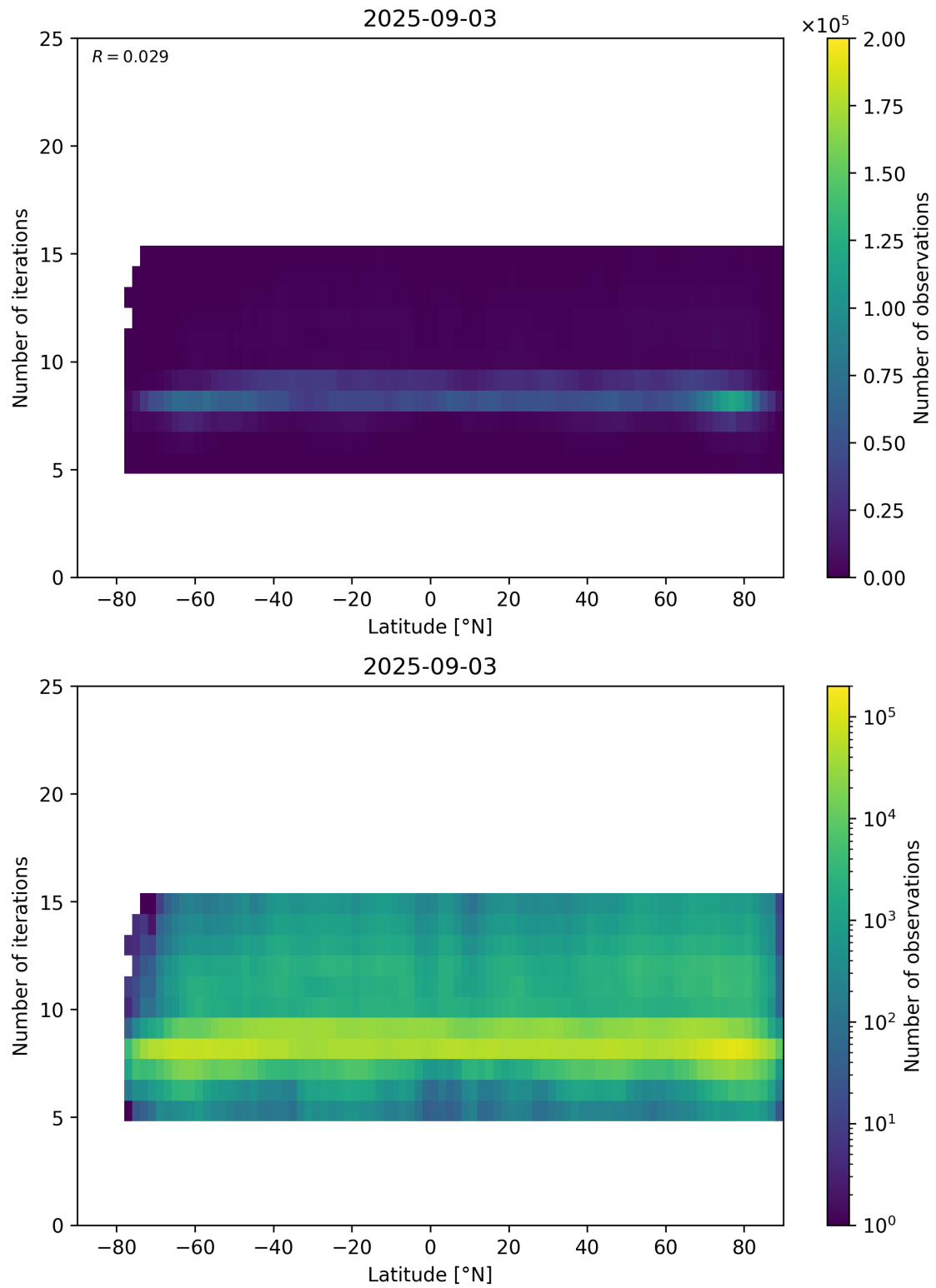
Figure 56: Scatter density plot of “Latitude” against “Number of iterations” for 2025-09-02 to 2025-09-04.
