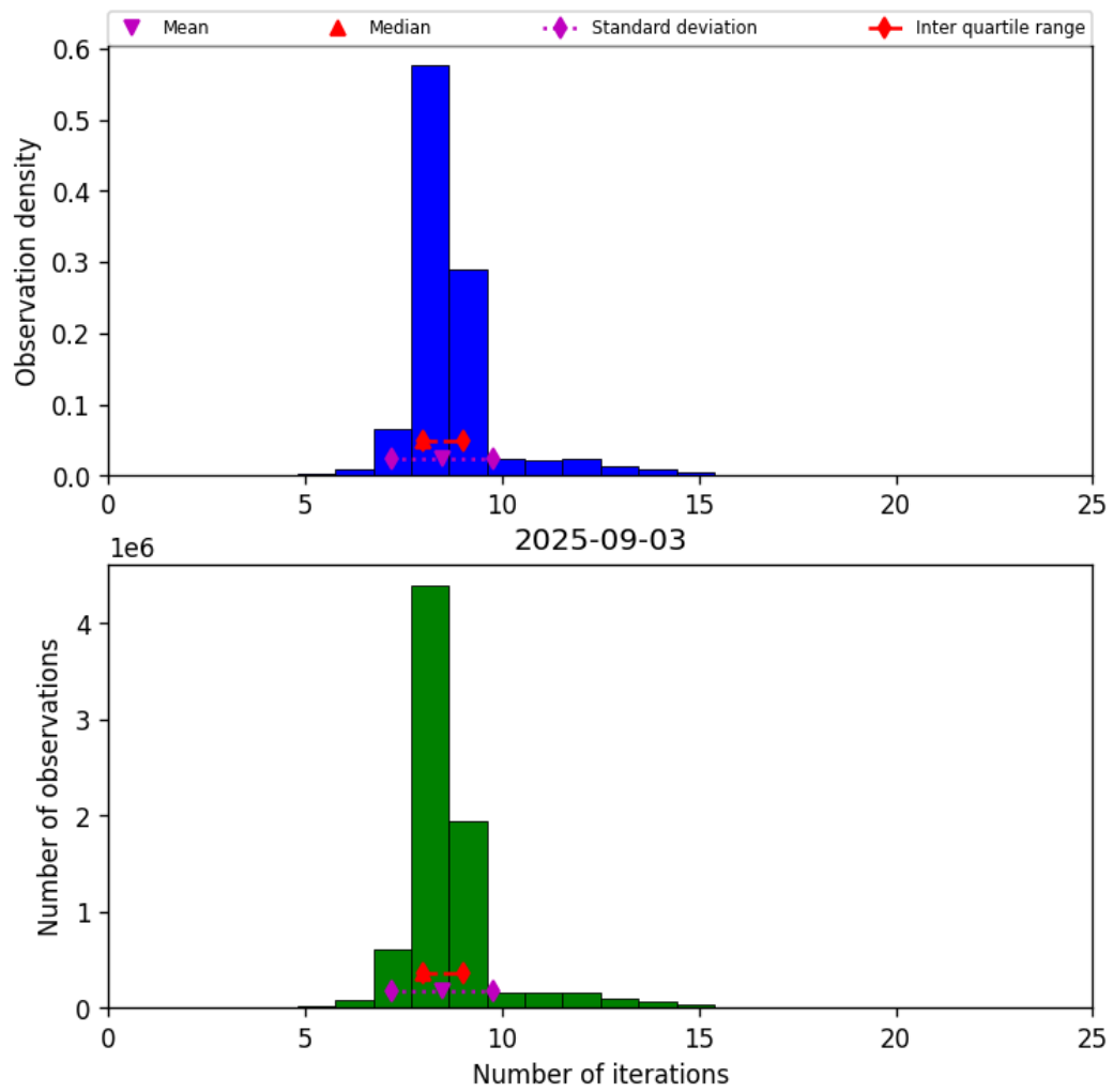
Figure 24: Histogram of “Number of iterations” for 2025-09-02 to 2025-09-04
