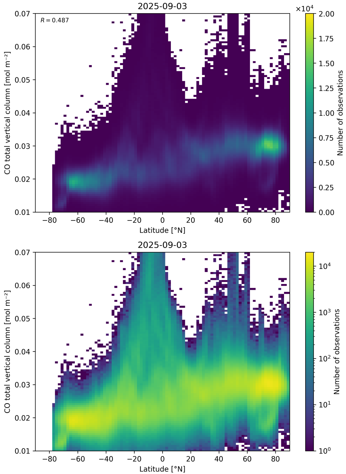
Figure 51: Scatter density plot of “Latitude” against “CO total vertical column” for 2025-09-02 to 2025-09-04.
