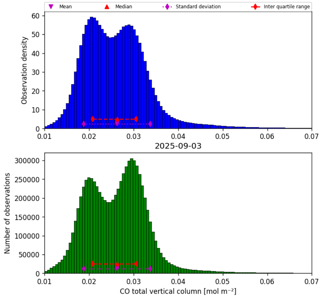
Figure 18: Histogram of “CO total vertical column” for 2025-09-02 to 2025-09-04
