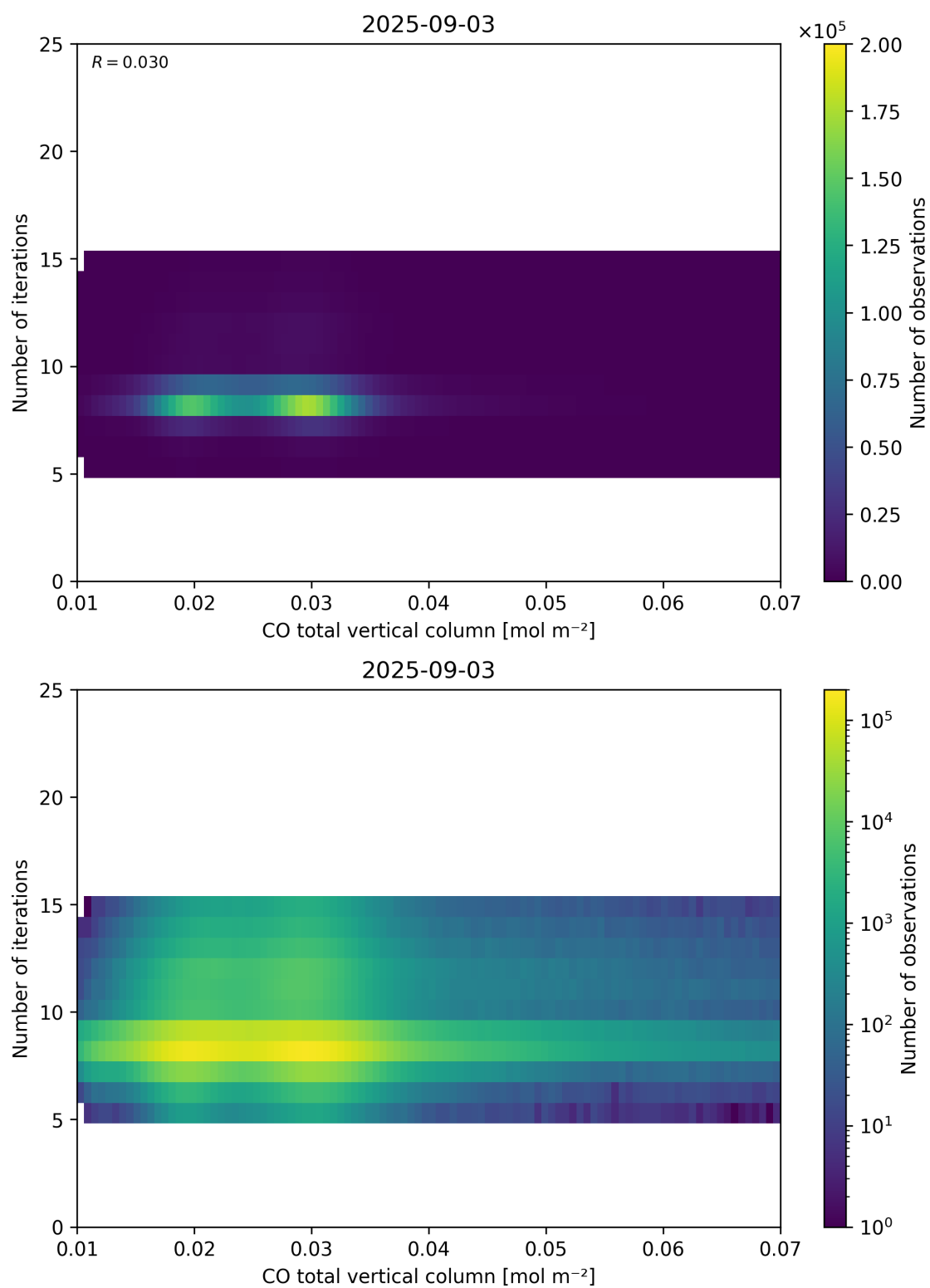
Figure 42: Scatter density plot of “CO total vertical column” against “Number of iterations” for 2025-09-02 to 2025-09-04.
