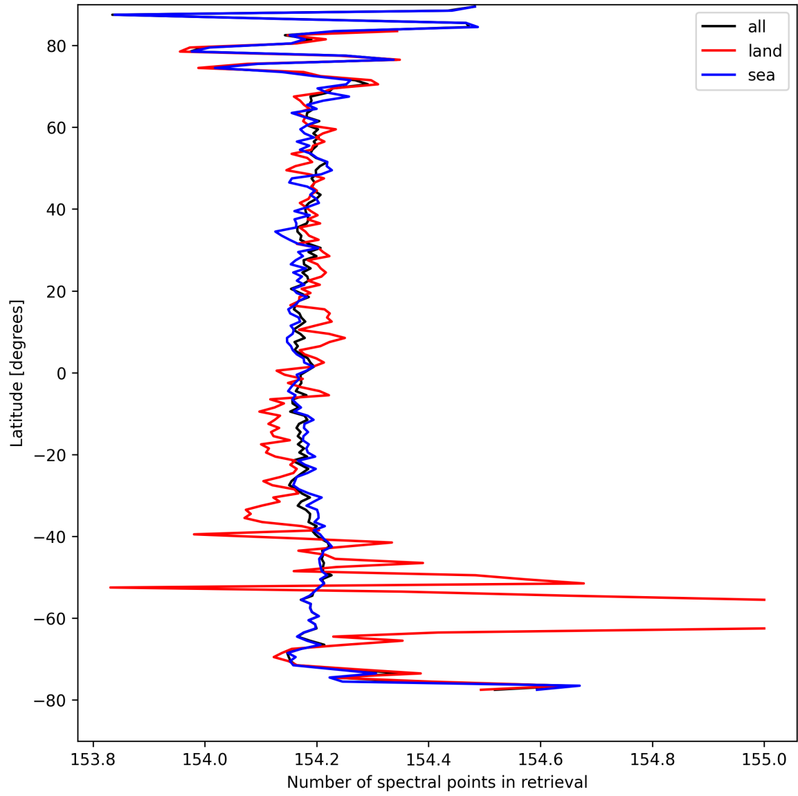
Figure 13: Zonal average of “Number of spectral points in retrieval” for 2025-09-02 to 2025-09-04.
