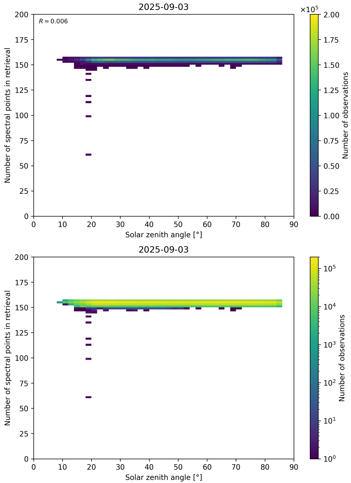
Figure 68: Scatter density plot of “Solar zenith angle” against “Number of spectral points in retrieval” for 2025-09-02 to 2025-09-04.
