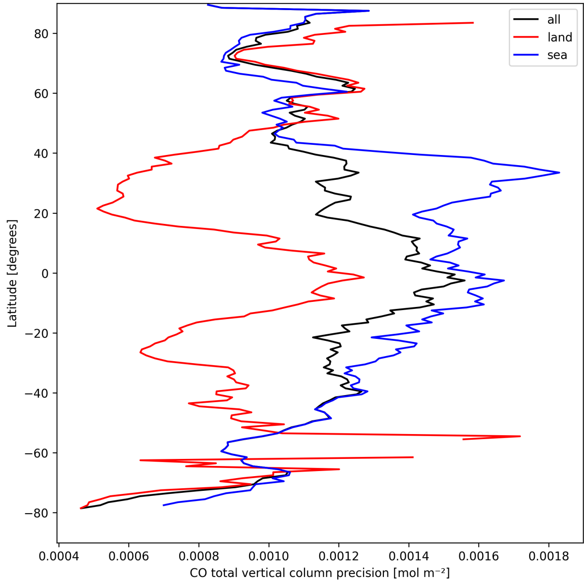
Figure 12: Zonal average of "CO total vertical column precision" for 2025-09-04 to 2025-09-05.
