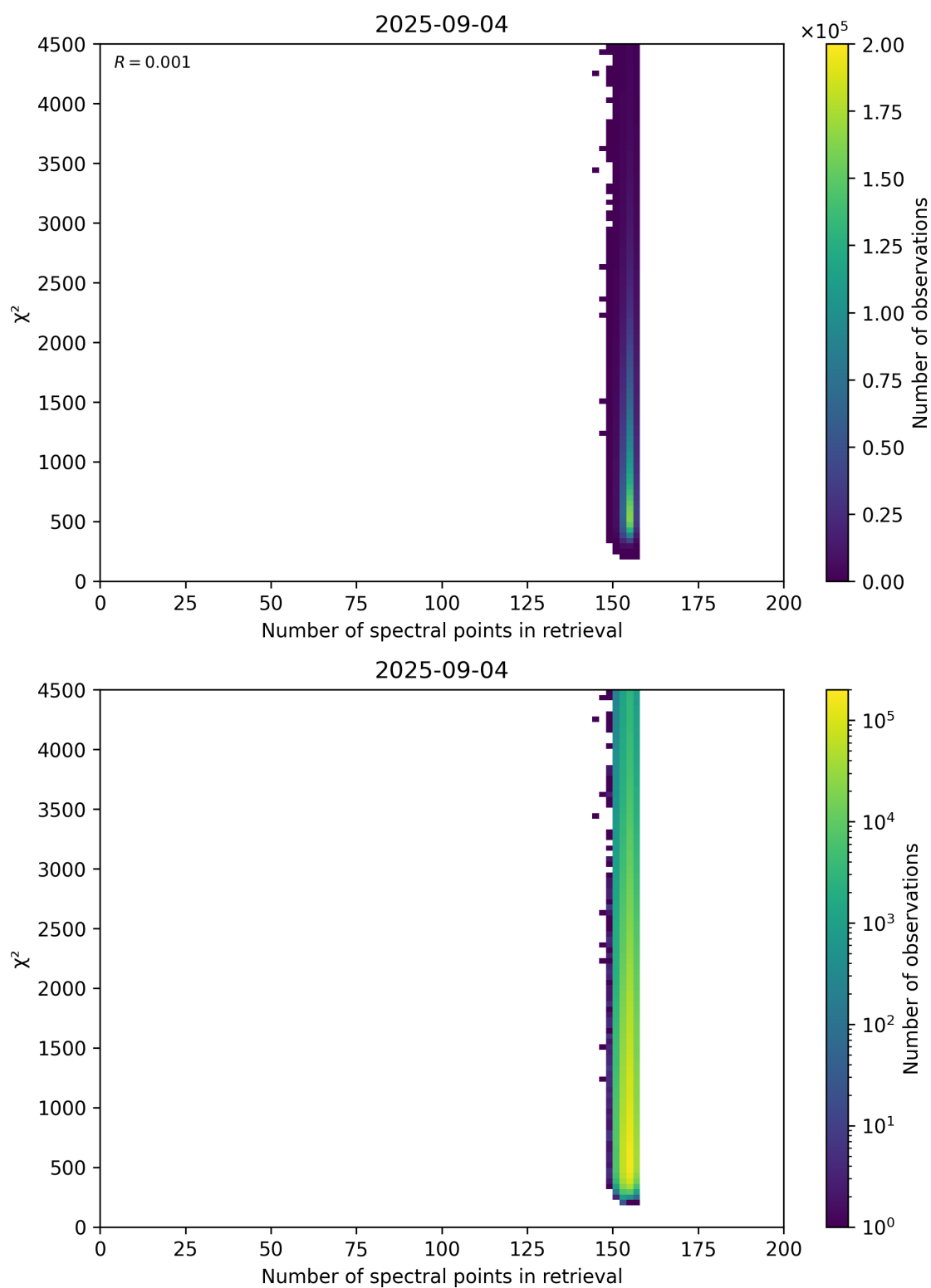
Figure 58: Scatter density plot of “Number of spectral points in retrieval” against “ \chi^2 ” for 2025-09-04 to 2025-09-05.
