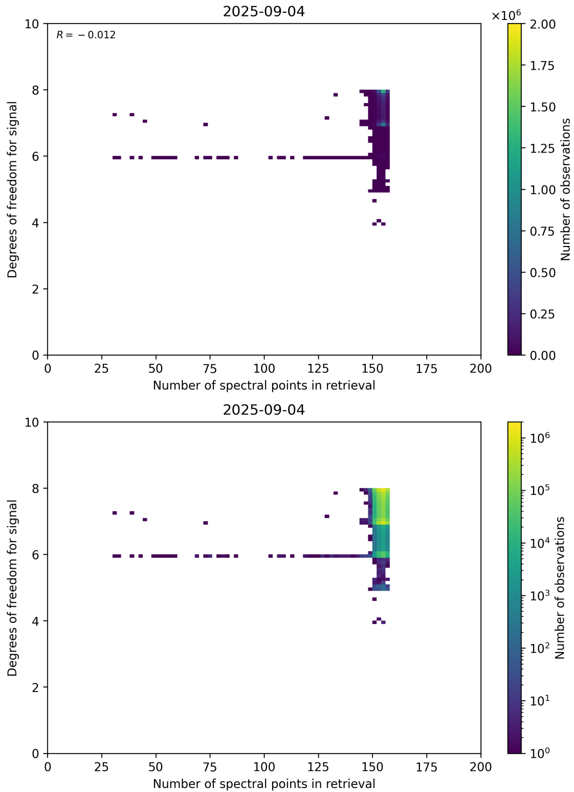
Figure 59: Scatter density plot of “Number of spectral points in retrieval” against “Degrees of freedom for signal” for 2025-09-04 to 2025-09-05.
