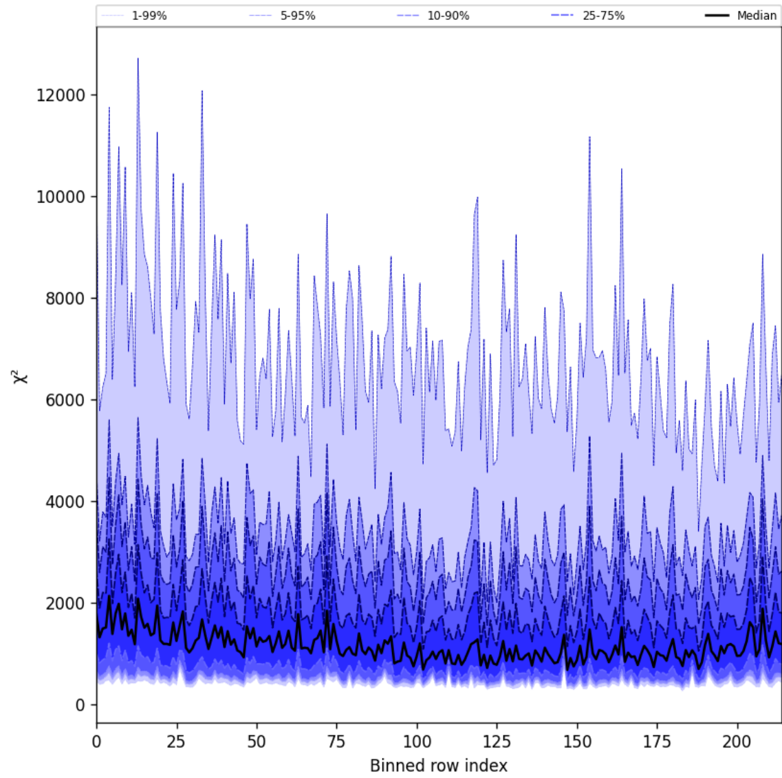
Figure 30: Along track statistics of “ \chi^2 ” for 2025-09-04 to 2025-09-05
