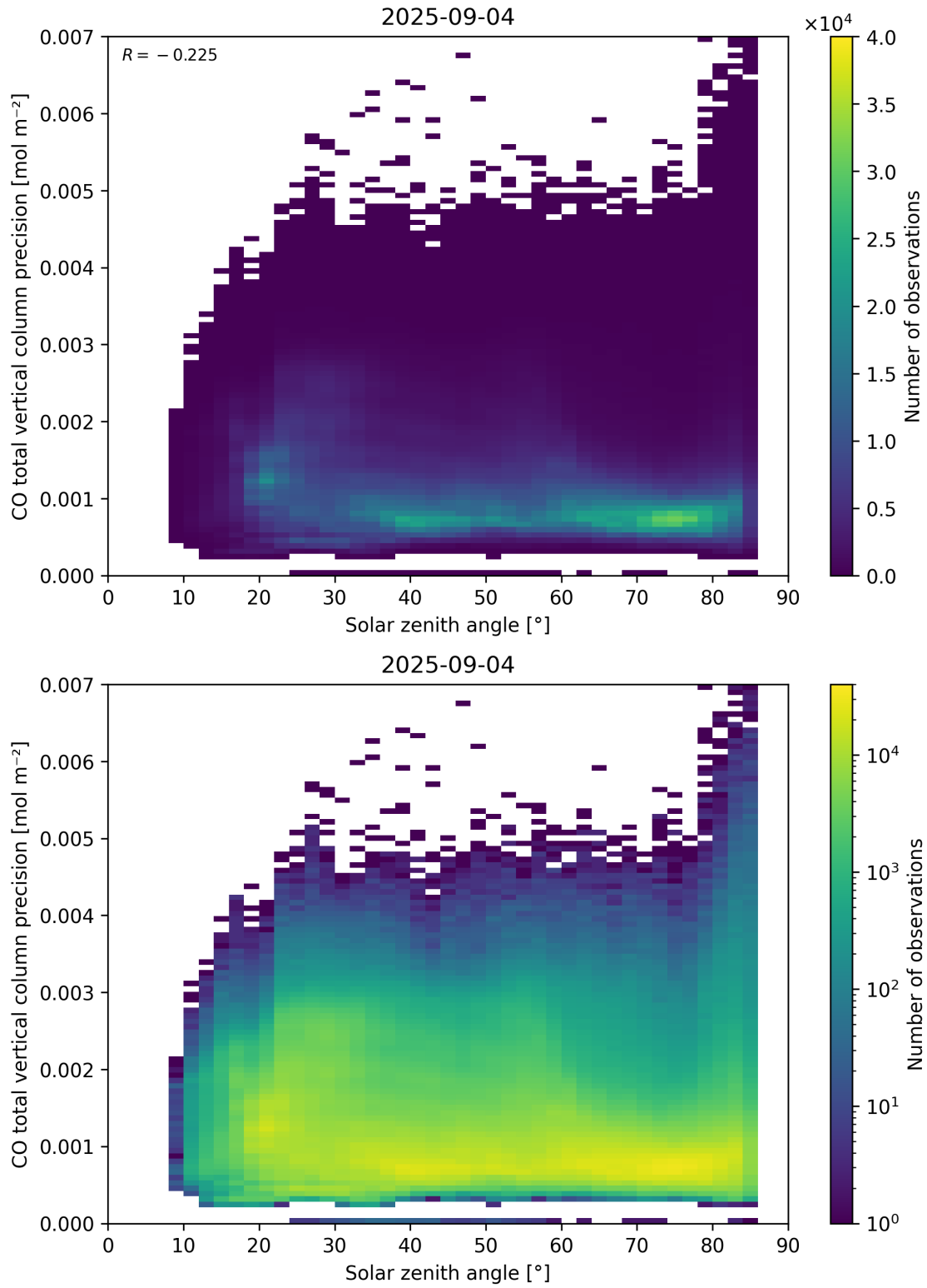
Figure 63: Scatter density plot of “Solar zenith angle” against “CO total vertical column precision” for 2025-09-04 to 2025-09-05.
