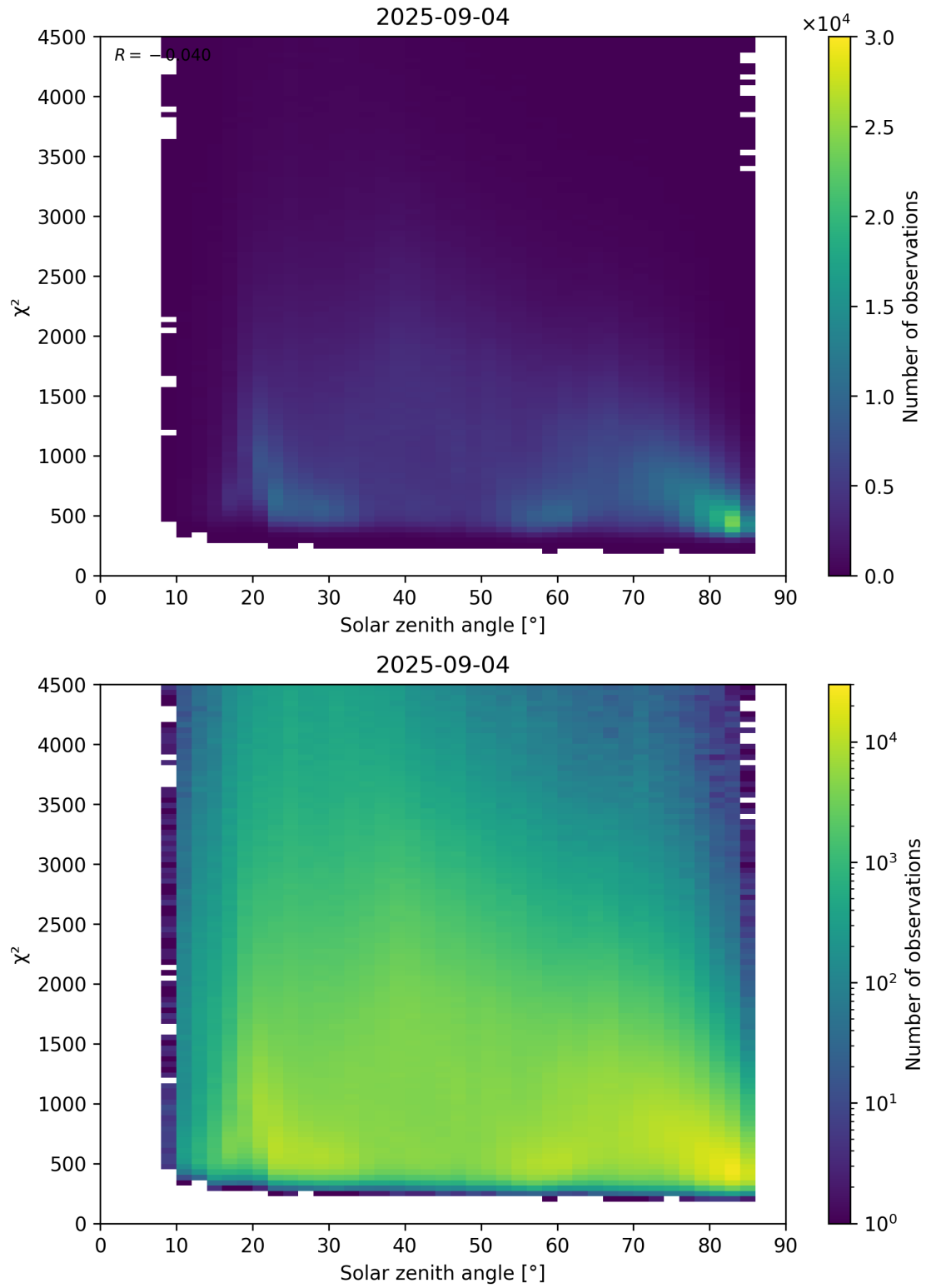
Figure 64: Scatter density plot of “Solar zenith angle” against “ \chi^2 ” for 2025-09-04 to 2025-09-05.
