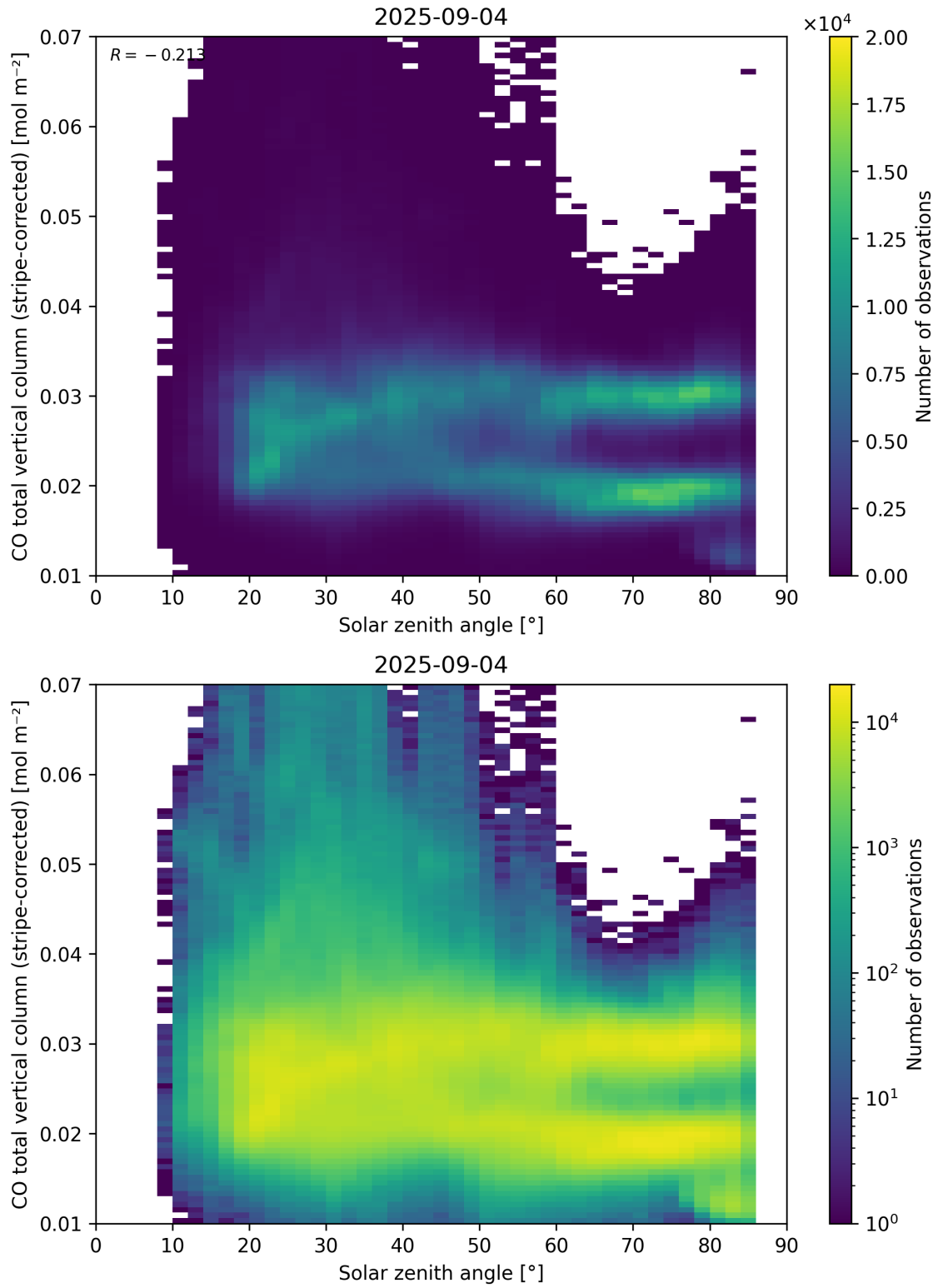
Figure 62: Scatter density plot of “Solar zenith angle” against “CO total vertical column (stripe-corrected)” for 2025-09-04 to 2025-09-05.
