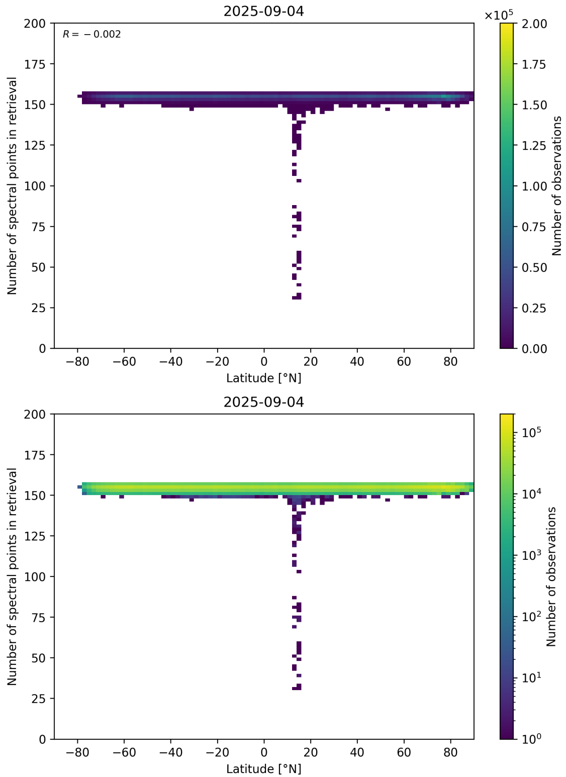
Figure 57: Scatter density plot of “Latitude” against “Number of spectral points in retrieval” for 2025-09-04 to 2025-09-05.
