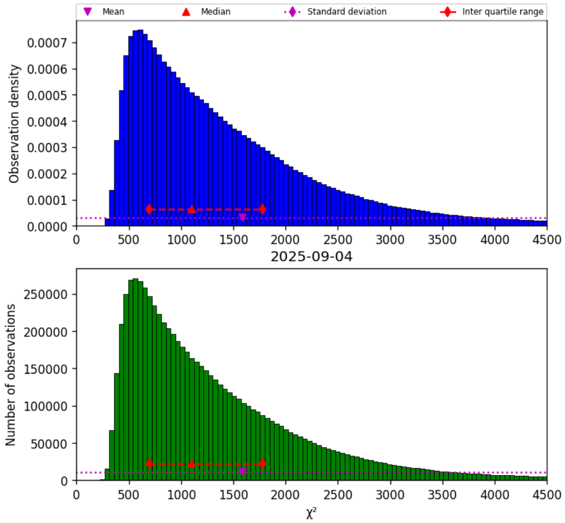
Figure 22: Histogram of " \chi^2 " for 2025-09-04 to 2025-09-05
