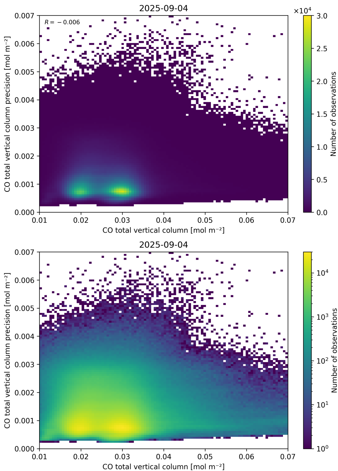
Figure 34: Scatter density plot of “CO total vertical column” against “CO total vertical column precision” for 2025-09-04 to 2025-09-05.
