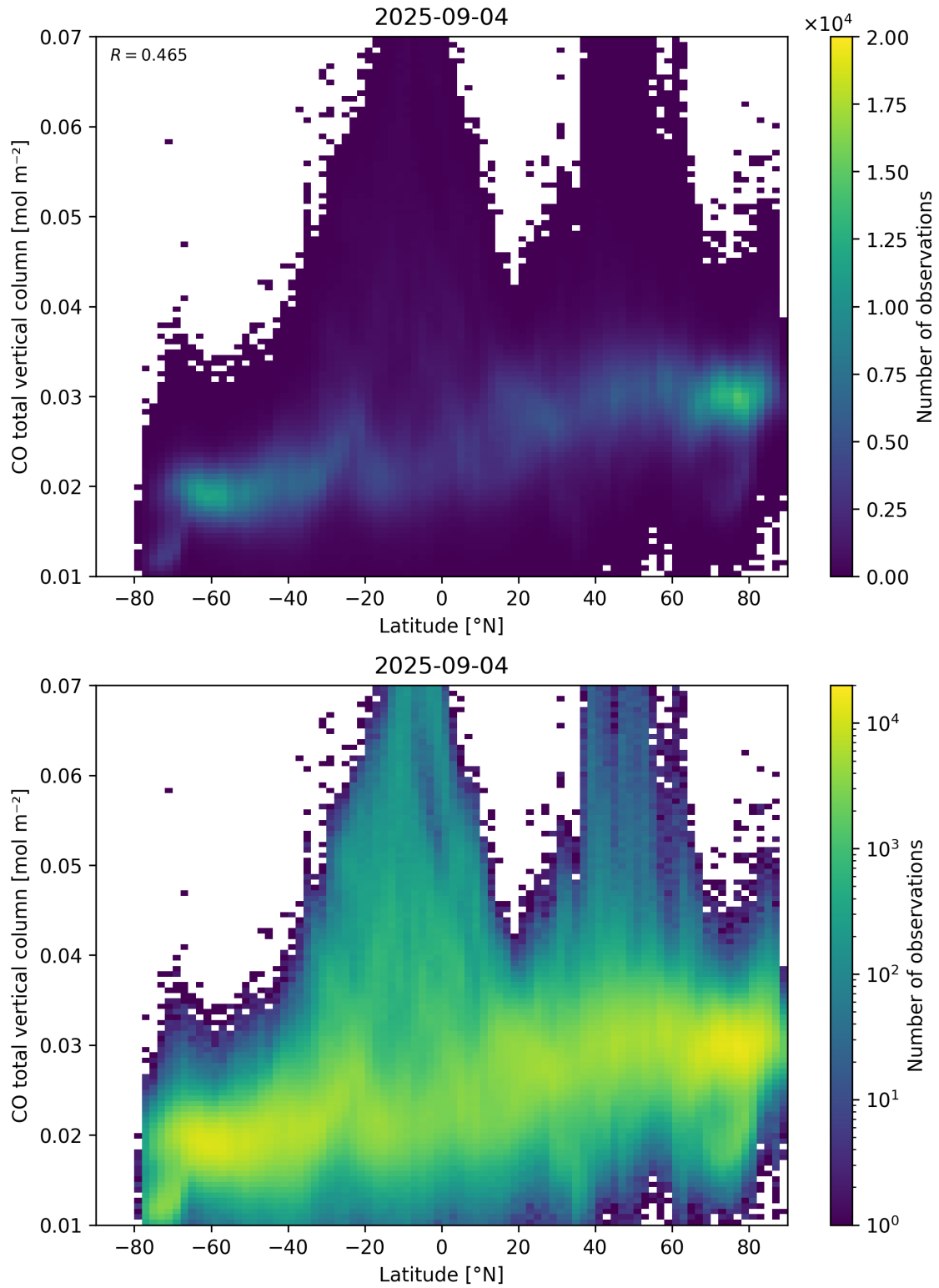
Figure 51: Scatter density plot of “Latitude” against “CO total vertical column” for 2025-09-04 to 2025-09-05.
