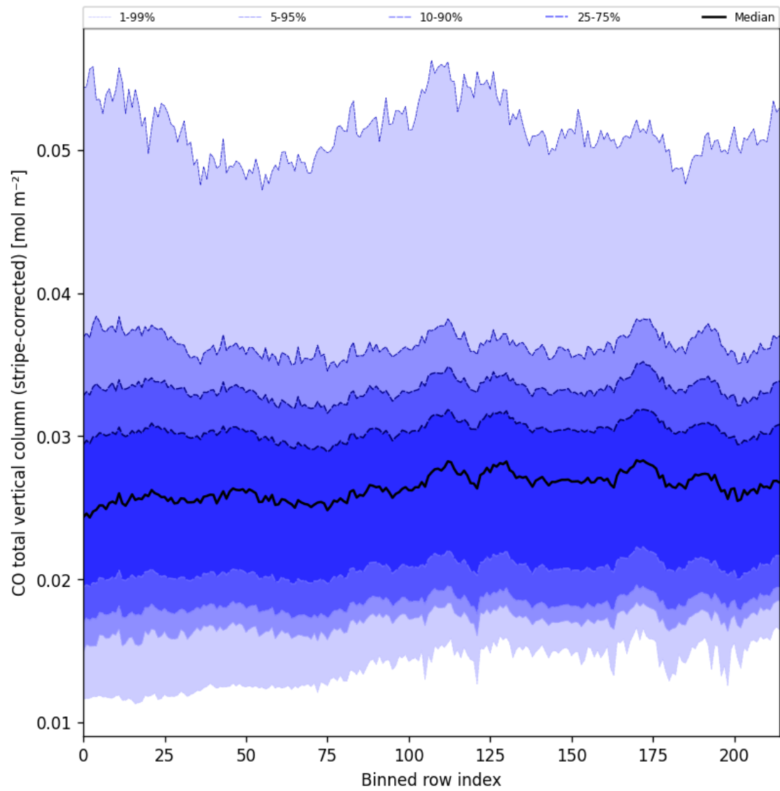
Figure 27: Along track statistics of “CO total vertical column (stripe-corrected)” for 2025-09-04 to 2025-09-05
