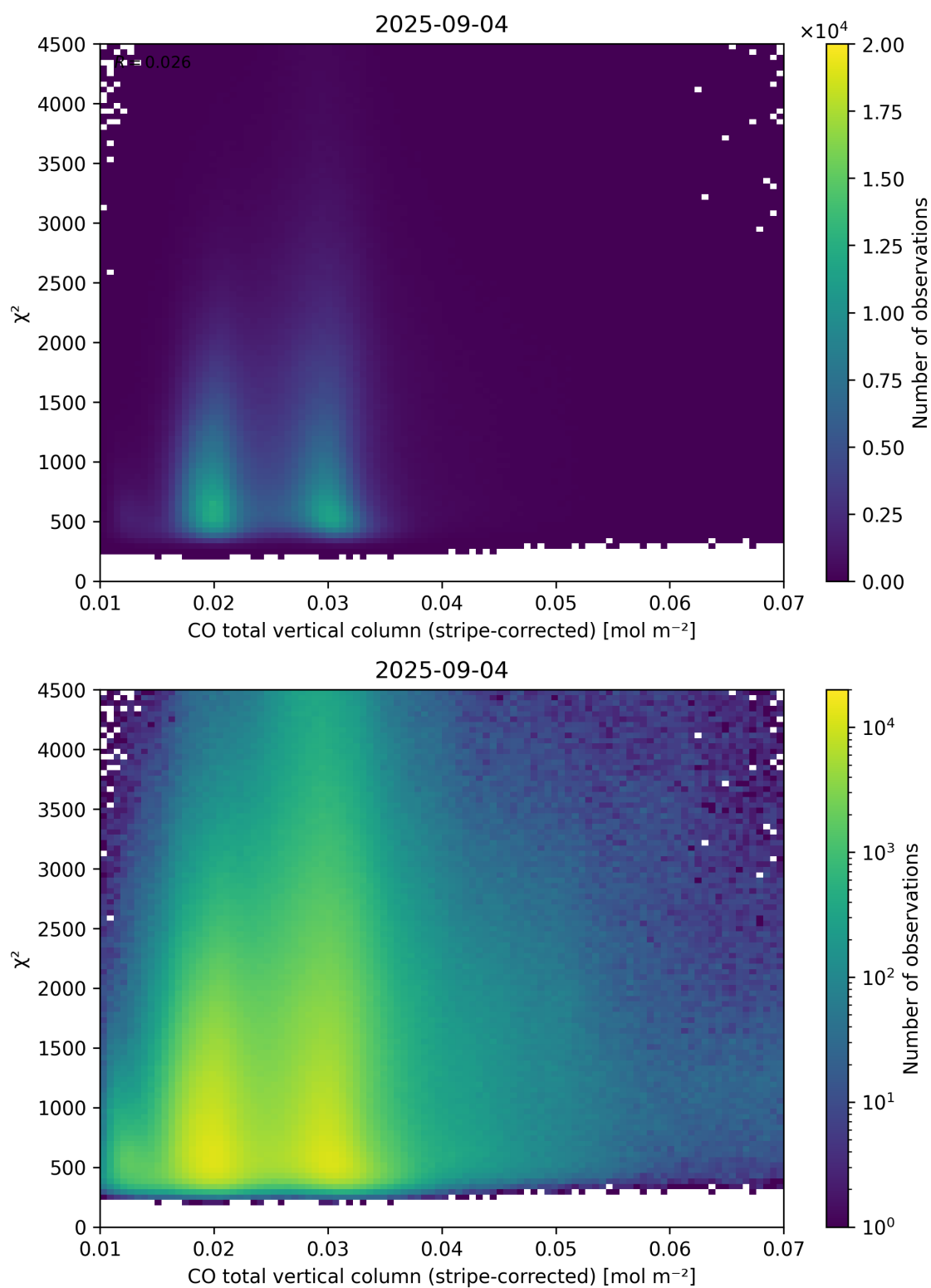
Figure 37: Scatter density plot of “CO total vertical column (stripe-corrected)” against “ \chi^2 ” for 2025-09-04 to 2025-09-05.
