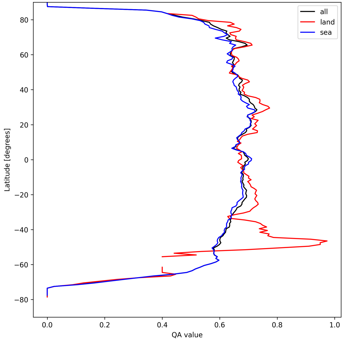
Figure 9: Zonal average of “QA value” for 2025-09-04 to 2025-09-05.
