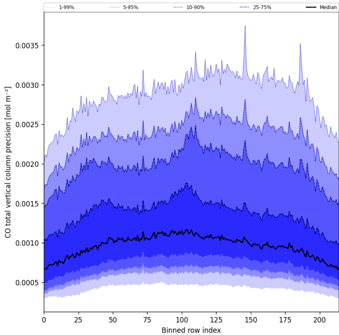
Figure 28: Along track statistics of “CO total vertical column precision” for 2025-09-04 to 2025-09-05
