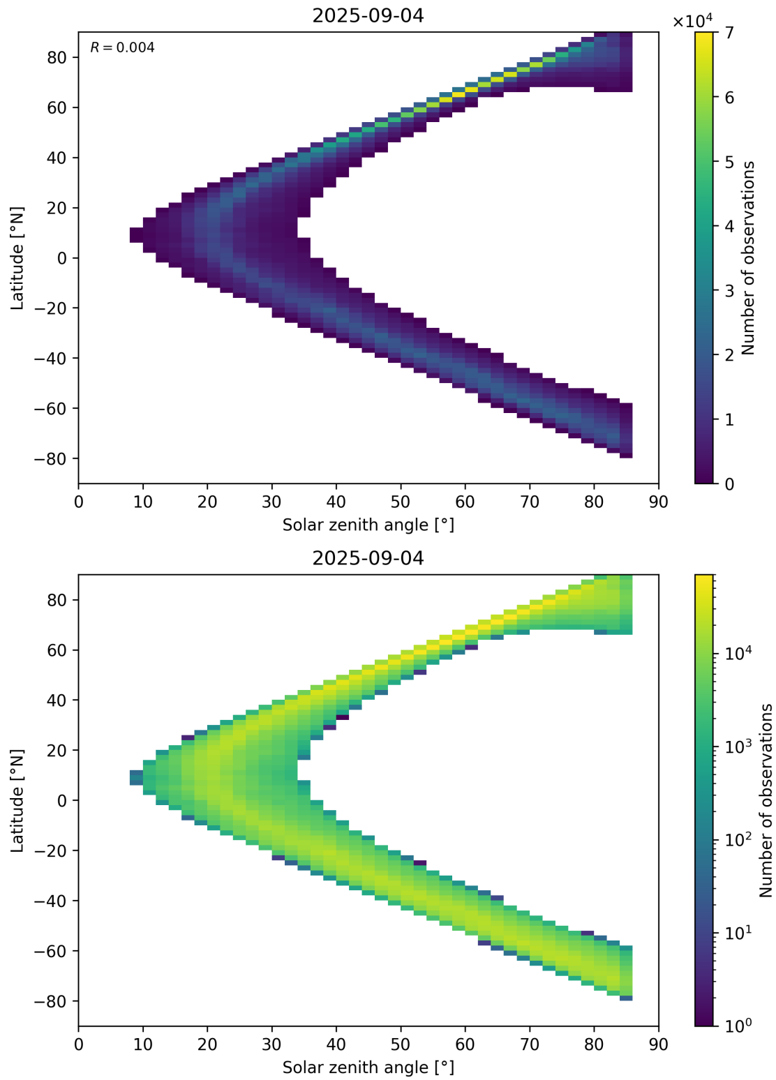
Figure 66: Scatter density plot of “Solar zenith angle” against “Latitude” for 2025-09-04 to 2025-09-05.
