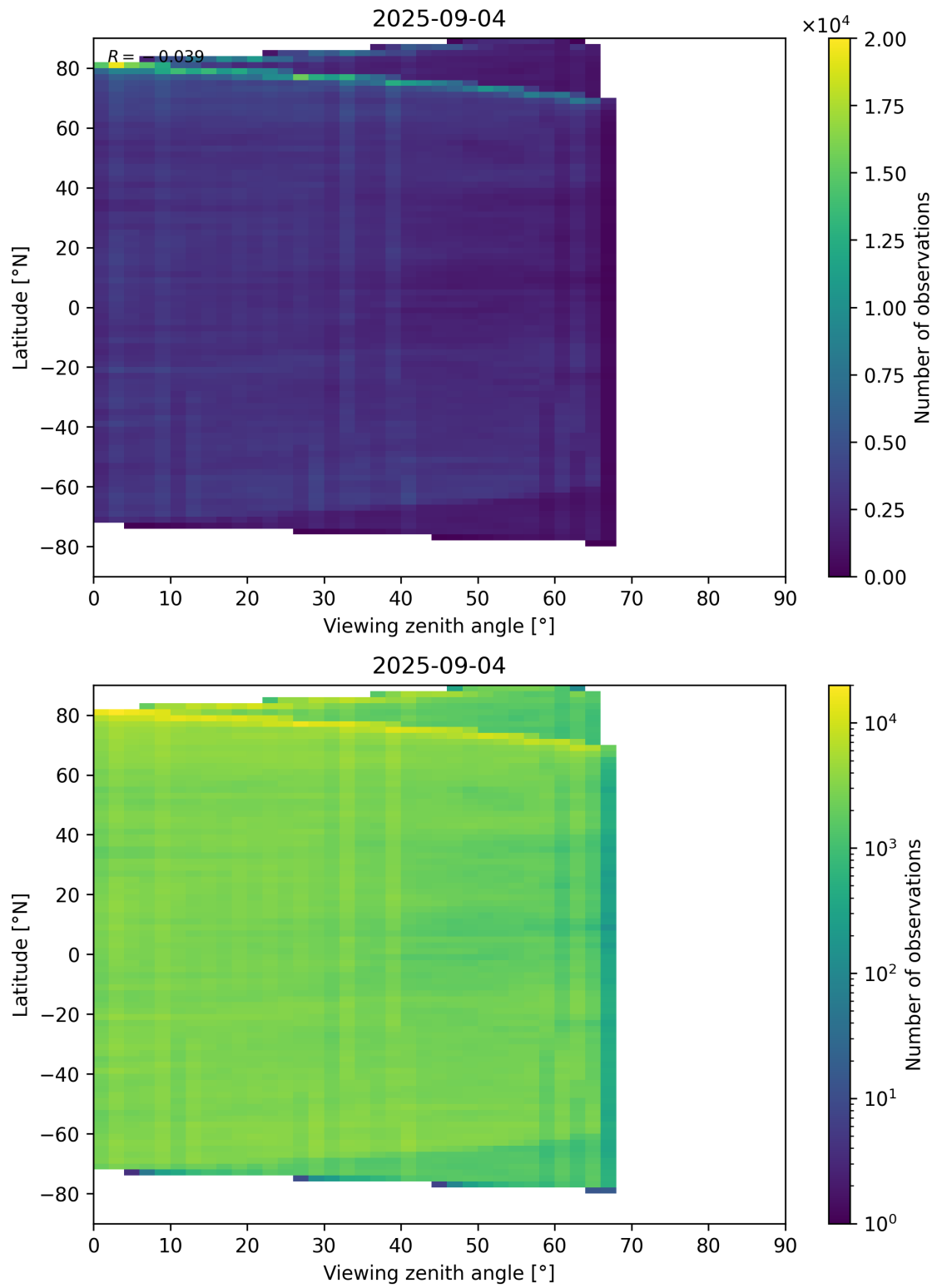
Figure 74: Scatter density plot of “Viewing zenith angle” against “Latitude” for 2025-09-04 to 2025-09-05.
