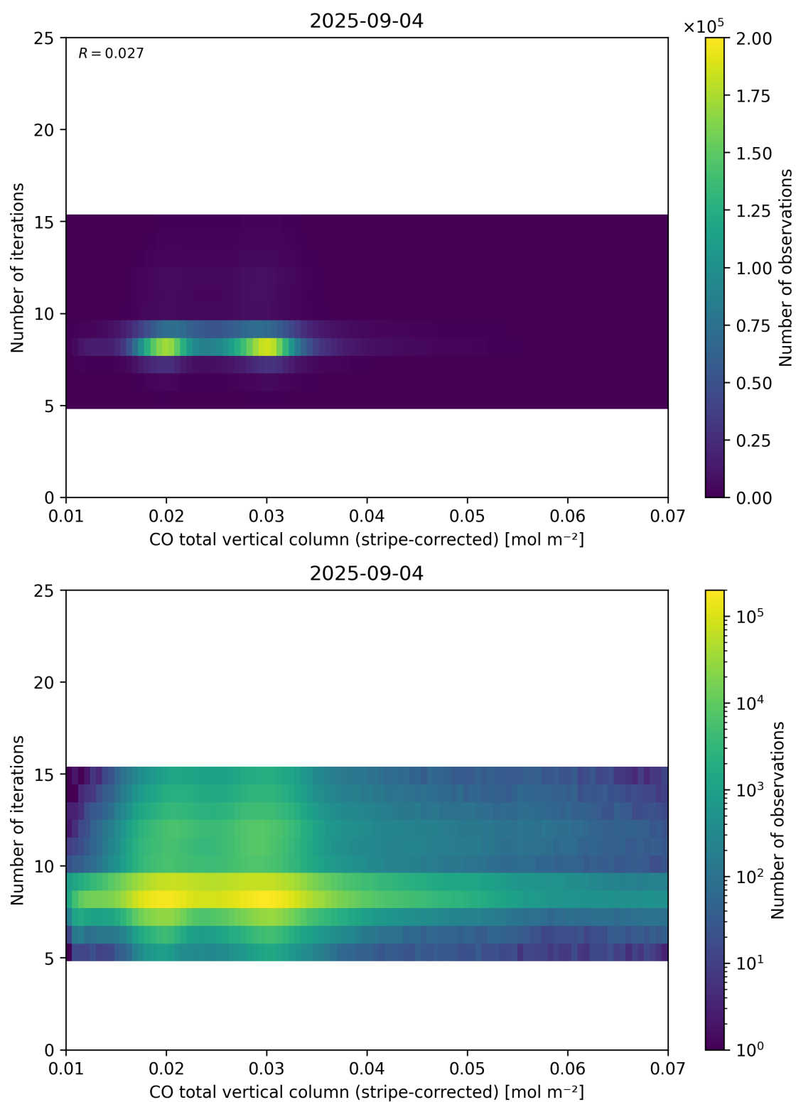
Figure 39: Scatter density plot of “CO total vertical column (stripe-corrected)” against “Number of iterations” for 2025-09-04 to 2025-09-05.
