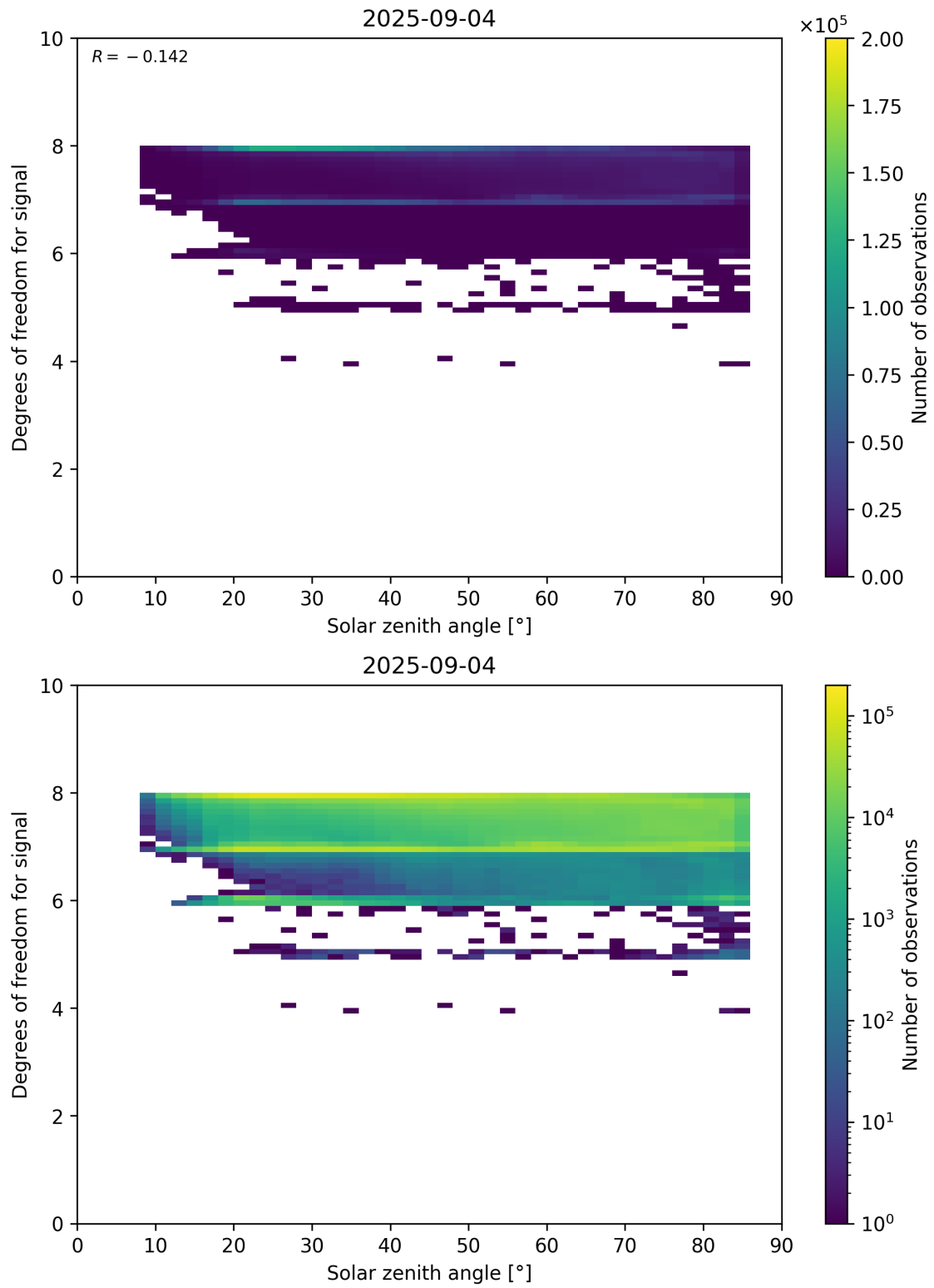
Figure 65: Scatter density plot of “Solar zenith angle” against “Degrees of freedom for signal” for 2025-09-04 to 2025-09-05.
