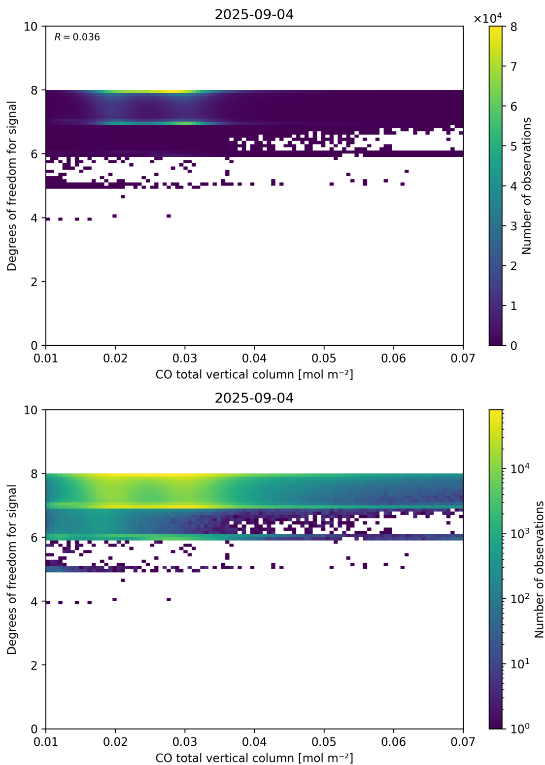
Figure 41: Scatter density plot of “CO total vertical column” against “Degrees of freedom for signal” for 2025-09-04 to 2025-09-05.
