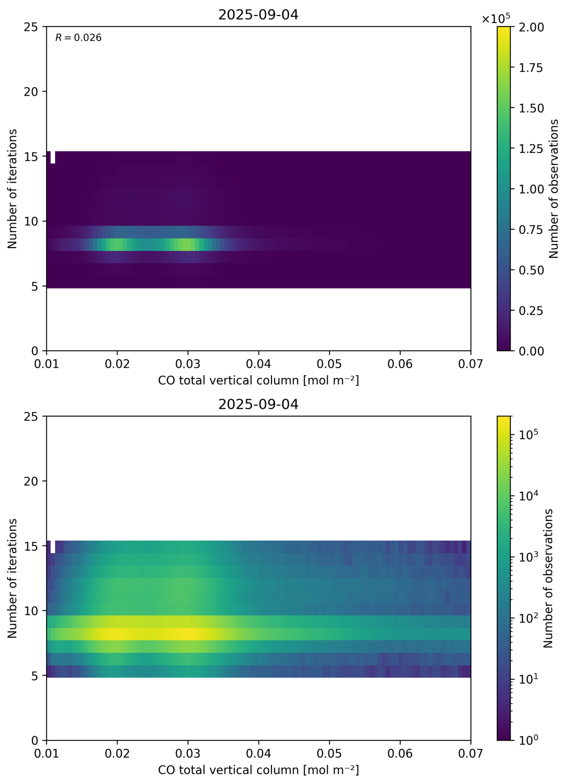
Figure 42: Scatter density plot of “CO total vertical column” against “Number of iterations” for 2025-09-04 to 2025-09-05.
