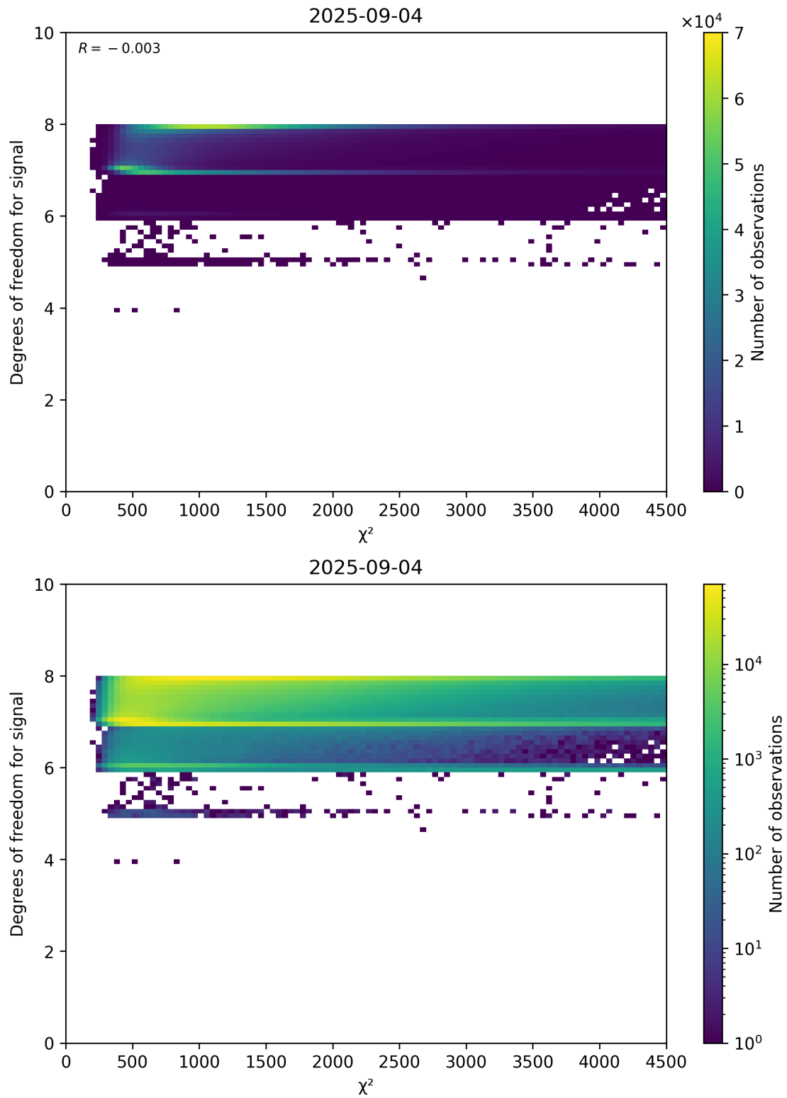
Figure 48: Scatter density plot of “ \chi^2 ” against “Degrees of freedom for signal” for 2025-09-04 to 2025-09-05.
