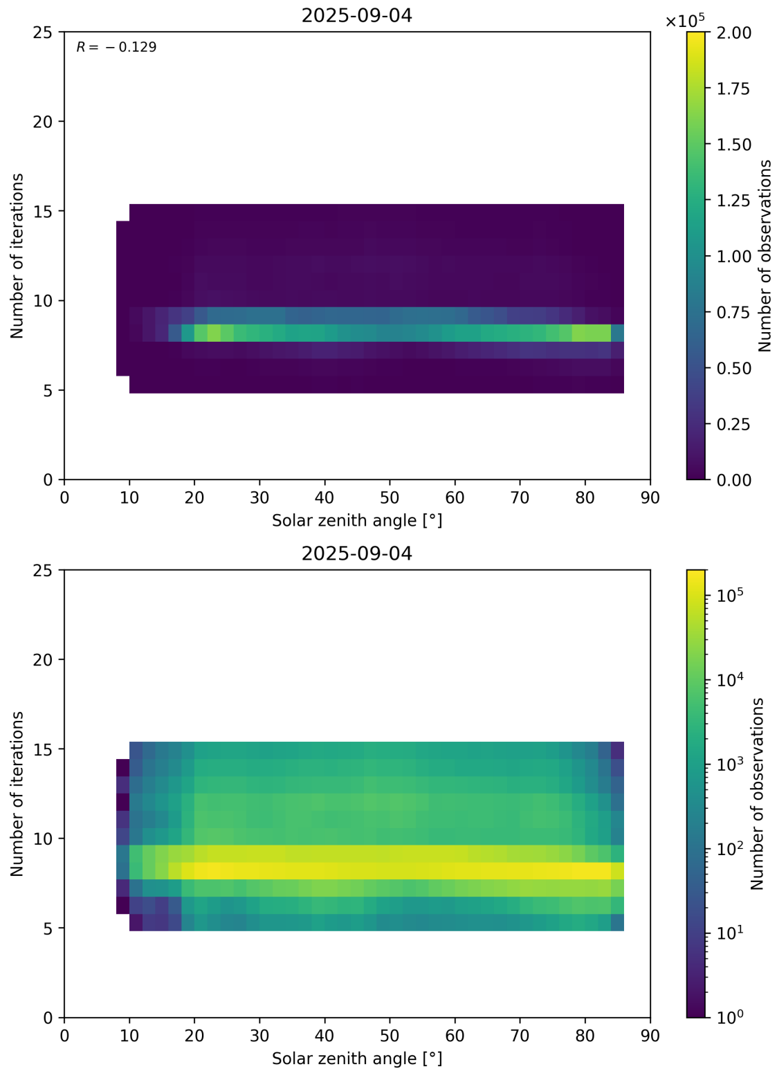
Figure 67: Scatter density plot of “Solar zenith angle” against “Number of iterations” for 2025-09-04 to 2025-09-05.
