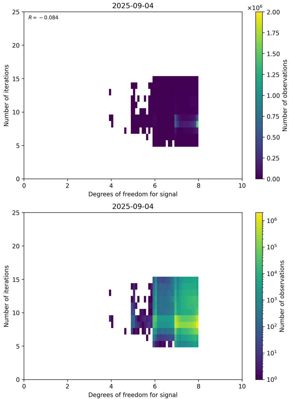
Figure 50: Scatter density plot of “Degrees of freedom for signal” against “Number of iterations” for 2025-09-04 to 2025-09-05.
