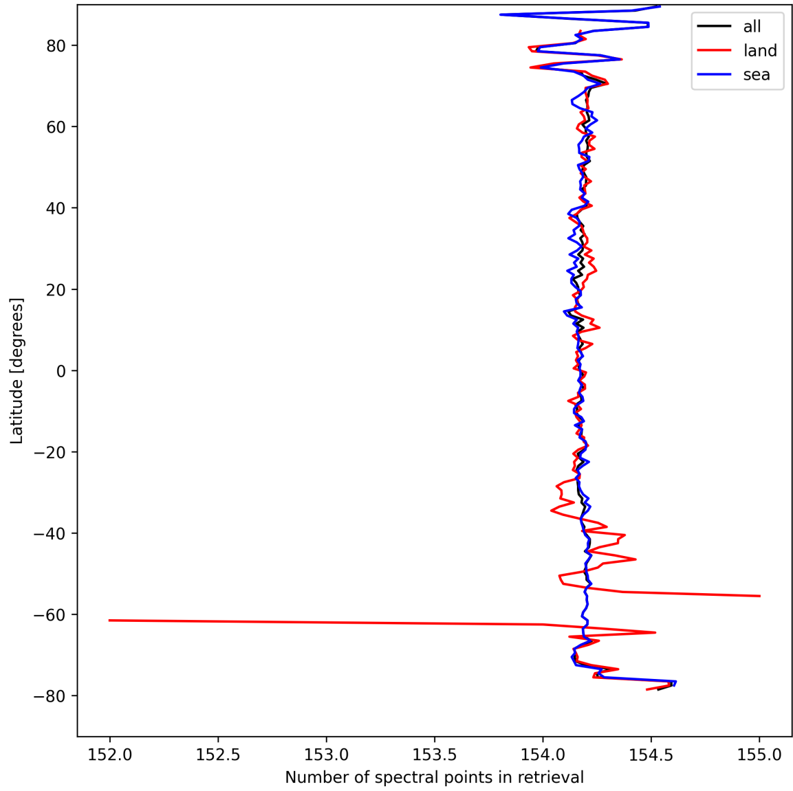
Figure 13: Zonal average of “Number of spectral points in retrieval” for 2025-09-04 to 2025-09-05.
