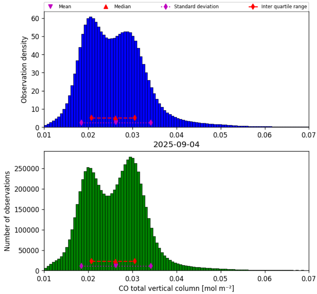
Figure 18: Histogram of “CO total vertical column” for 2025-09-04 to 2025-09-05
