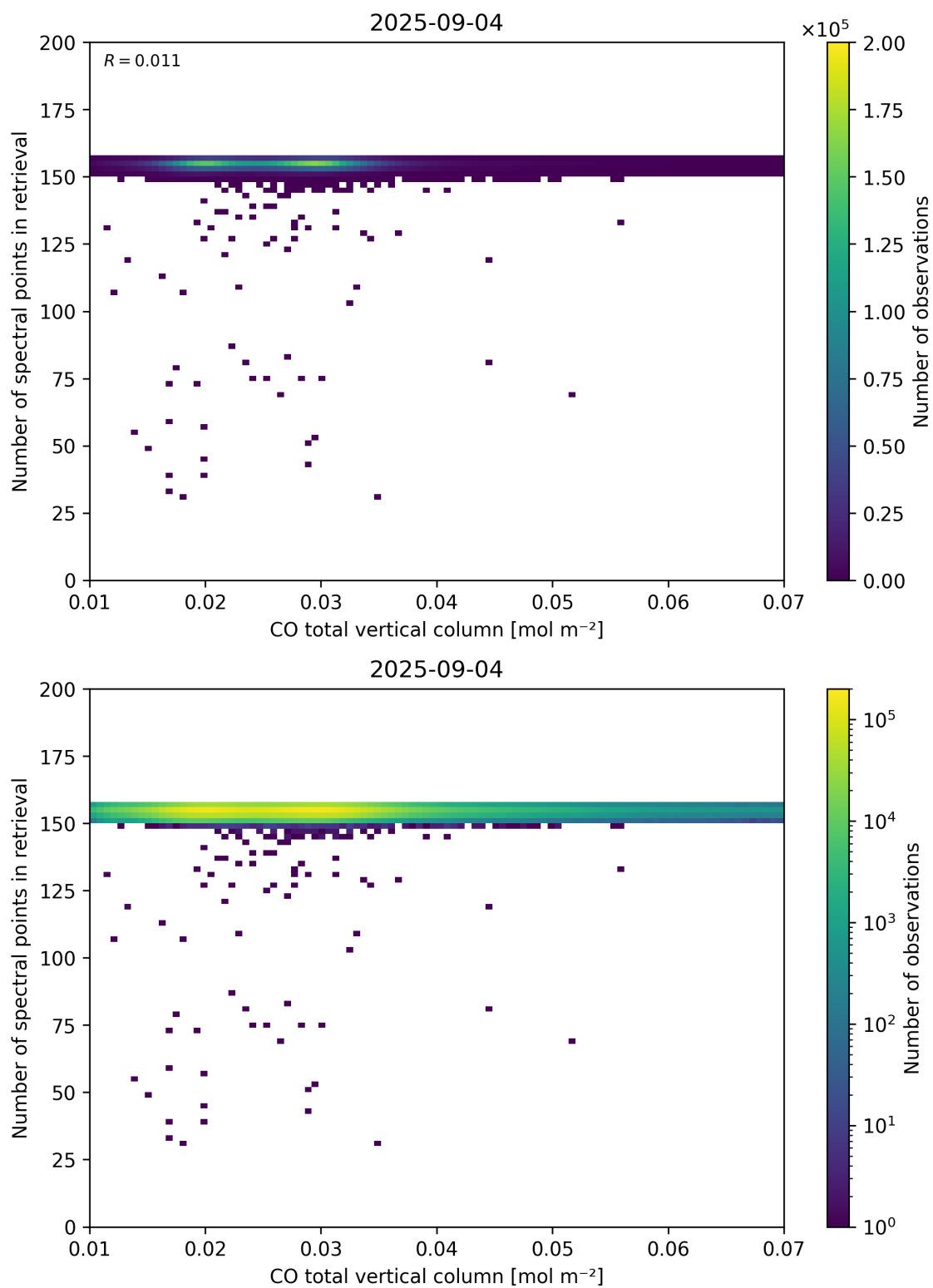
Figure 43: Scatter density plot of “CO total vertical column” against “Number of spectral points in retrieval” for 2025-09-04 to 2025-09-05.
