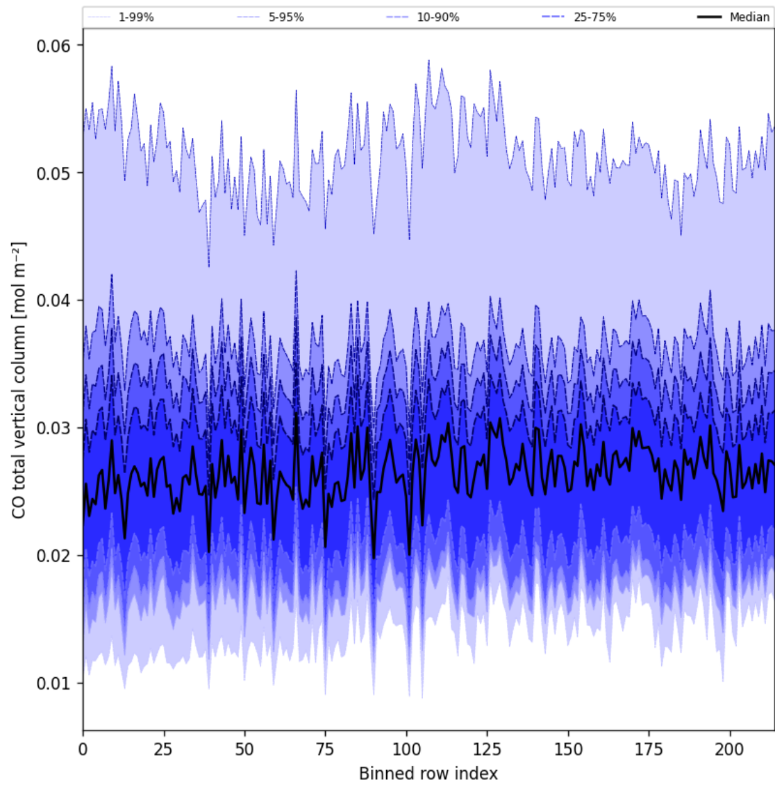
Figure 26: Along track statistics of “CO total vertical column” for 2025-09-04 to 2025-09-05
