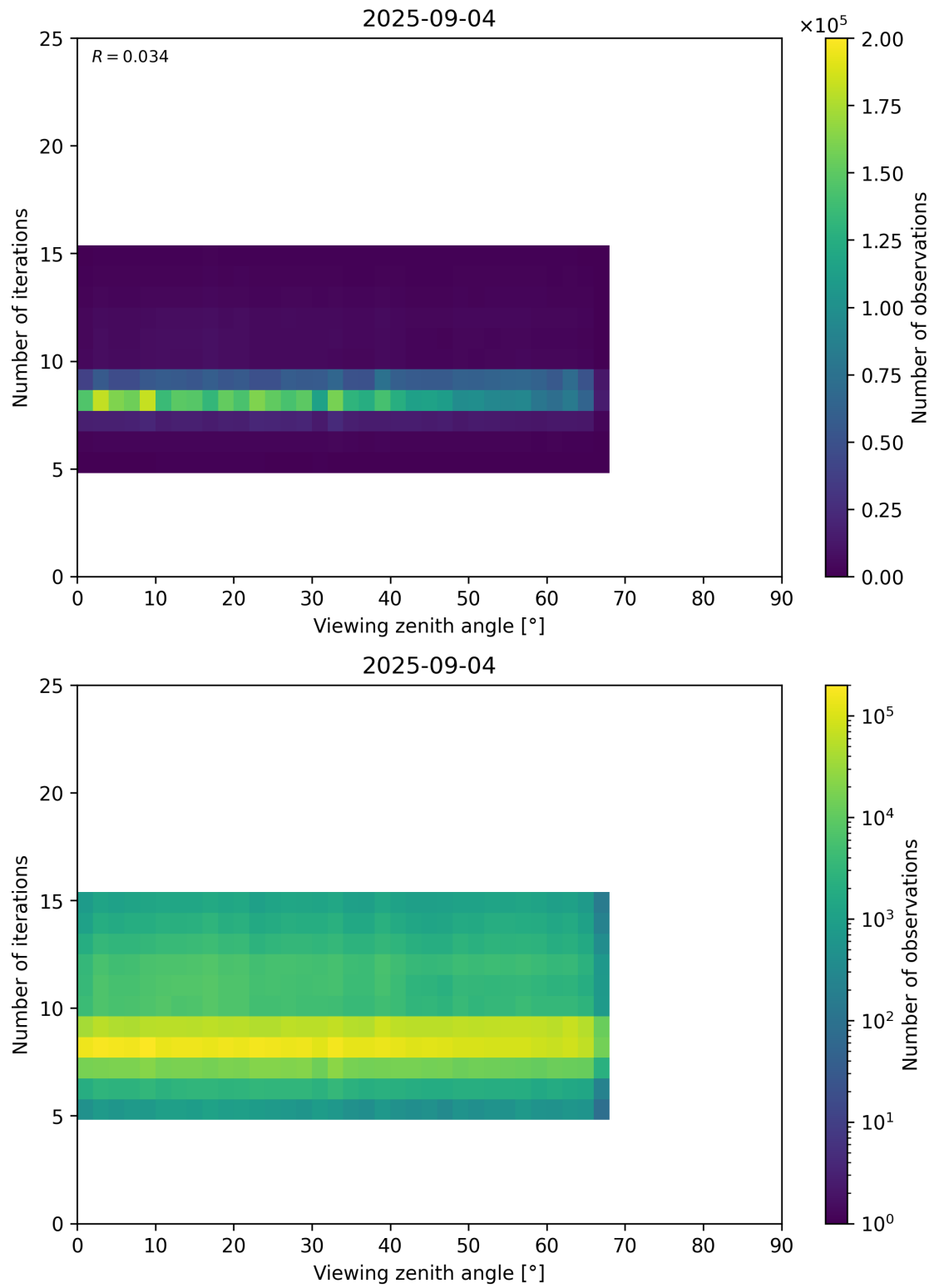
Figure 75: Scatter density plot of “Viewing zenith angle” against “Number of iterations” for 2025-09-04 to 2025-09-05.
