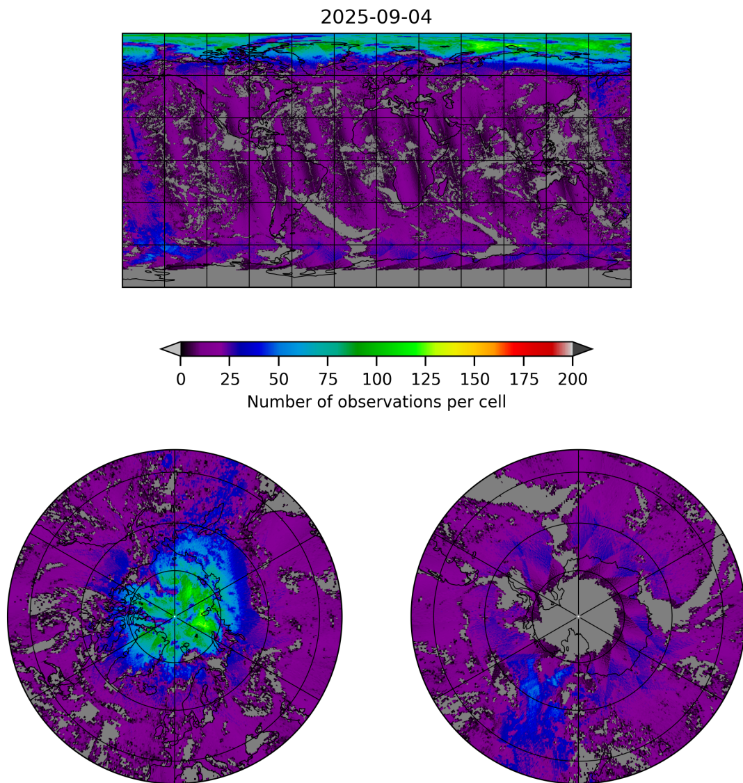
Figure 8: Map of the number of observations for 2025-09-04 to 2025-09-05
