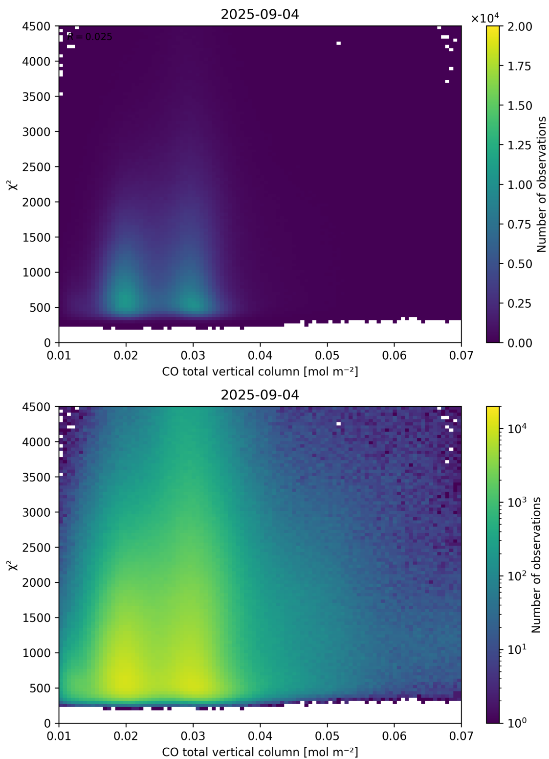
Figure 35: Scatter density plot of “CO total vertical column” against “ \chi^2 ” for 2025-09-04 to 2025-09-05.
