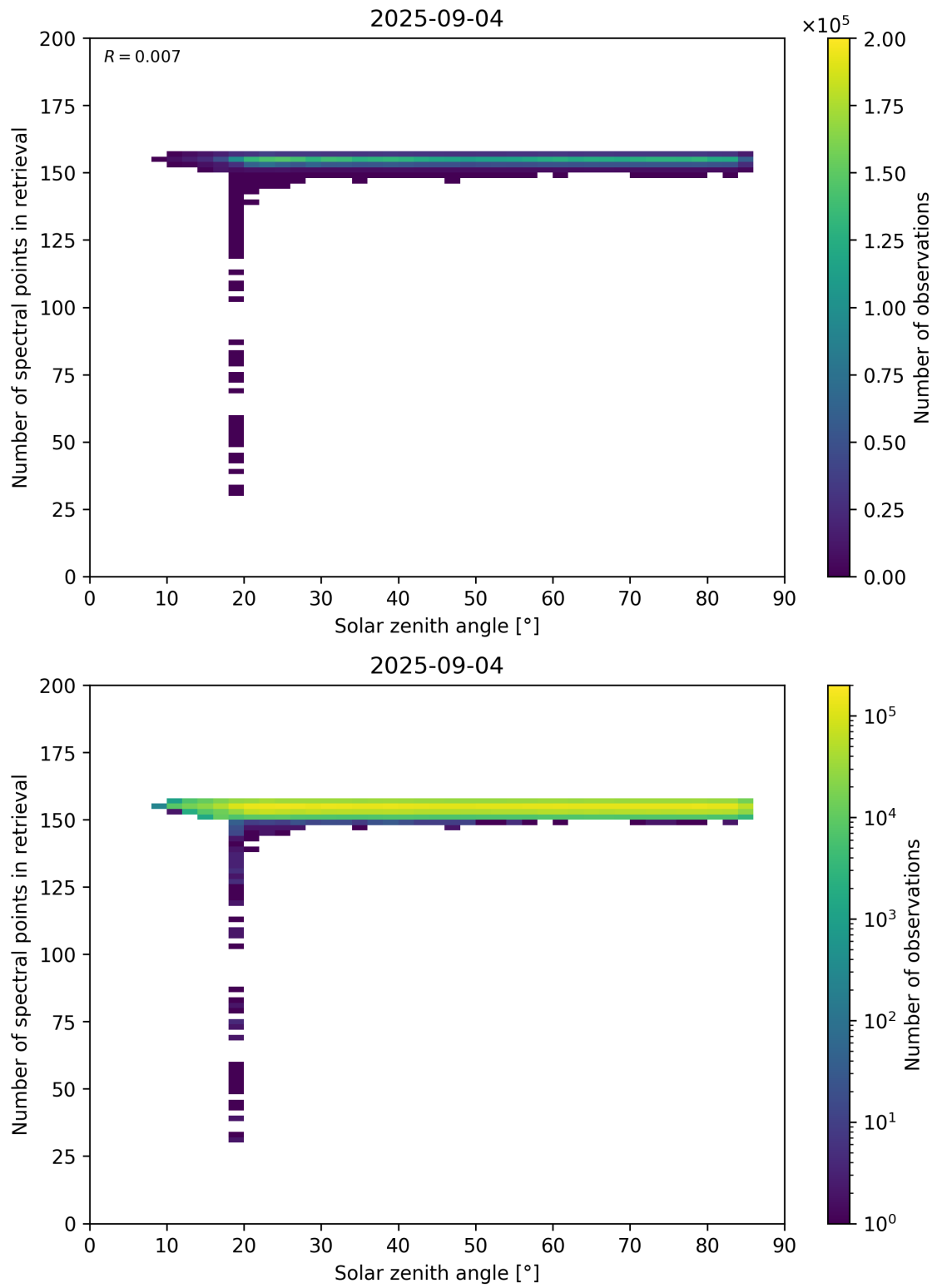
Figure 68: Scatter density plot of “Solar zenith angle” against “Number of spectral points in retrieval” for 2025-09-04 to 2025-09-05.
