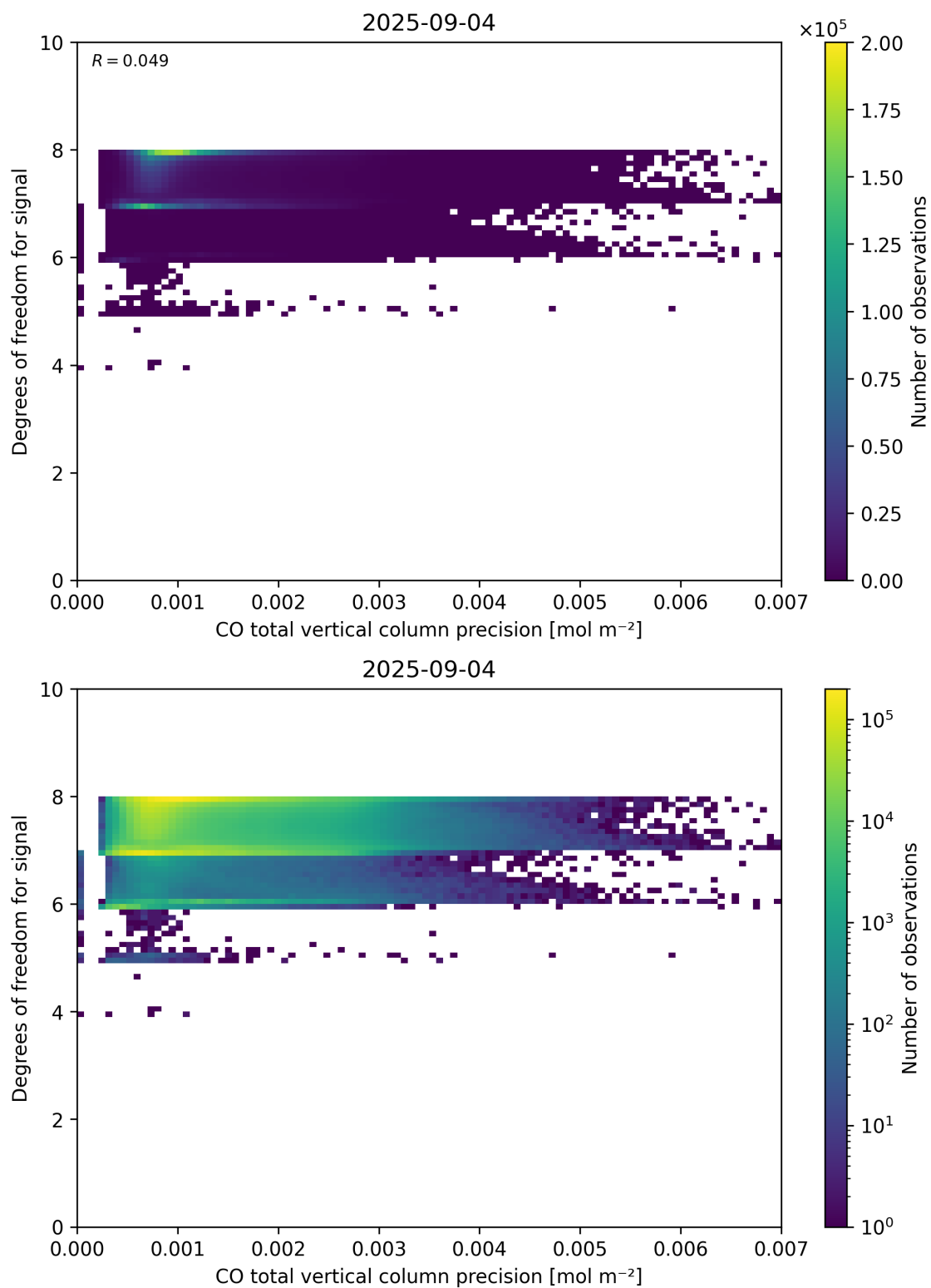
Figure 45: Scatter density plot of “CO total vertical column precision” against “Degrees of freedom for signal” for 2025-09-04 to 2025-09-05.
