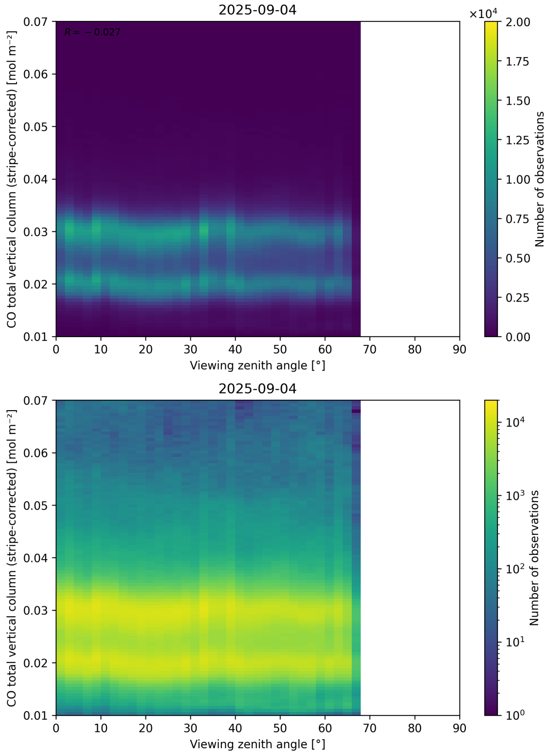
Figure 70: Scatter density plot of “Viewing zenith angle” against “CO total vertical column (stripe-corrected)” for 2025-09-04 to 2025-09-05.
