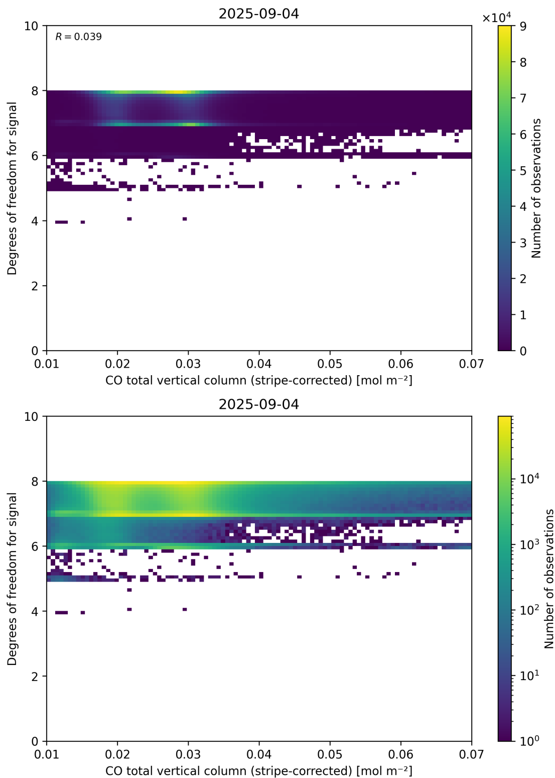
Figure 38: Scatter density plot of “CO total vertical column (stripe-corrected)” against “Degrees of freedom for signal” for 2025-09-04 to 2025-09-05.
