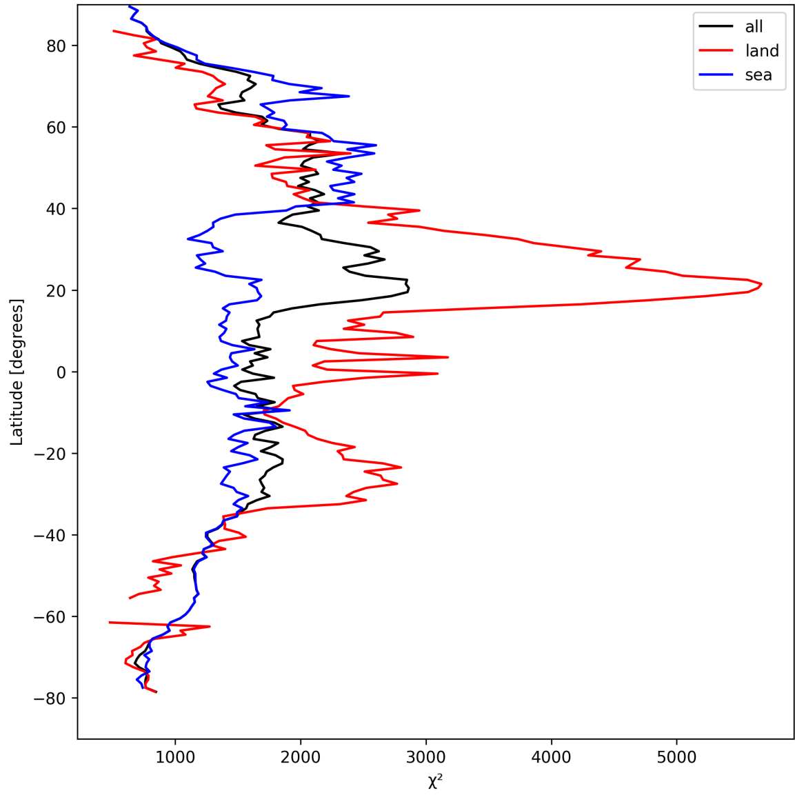
Figure 14: Zonal average of “ \chi^2 ” for 2025-09-04 to 2025-09-05.
