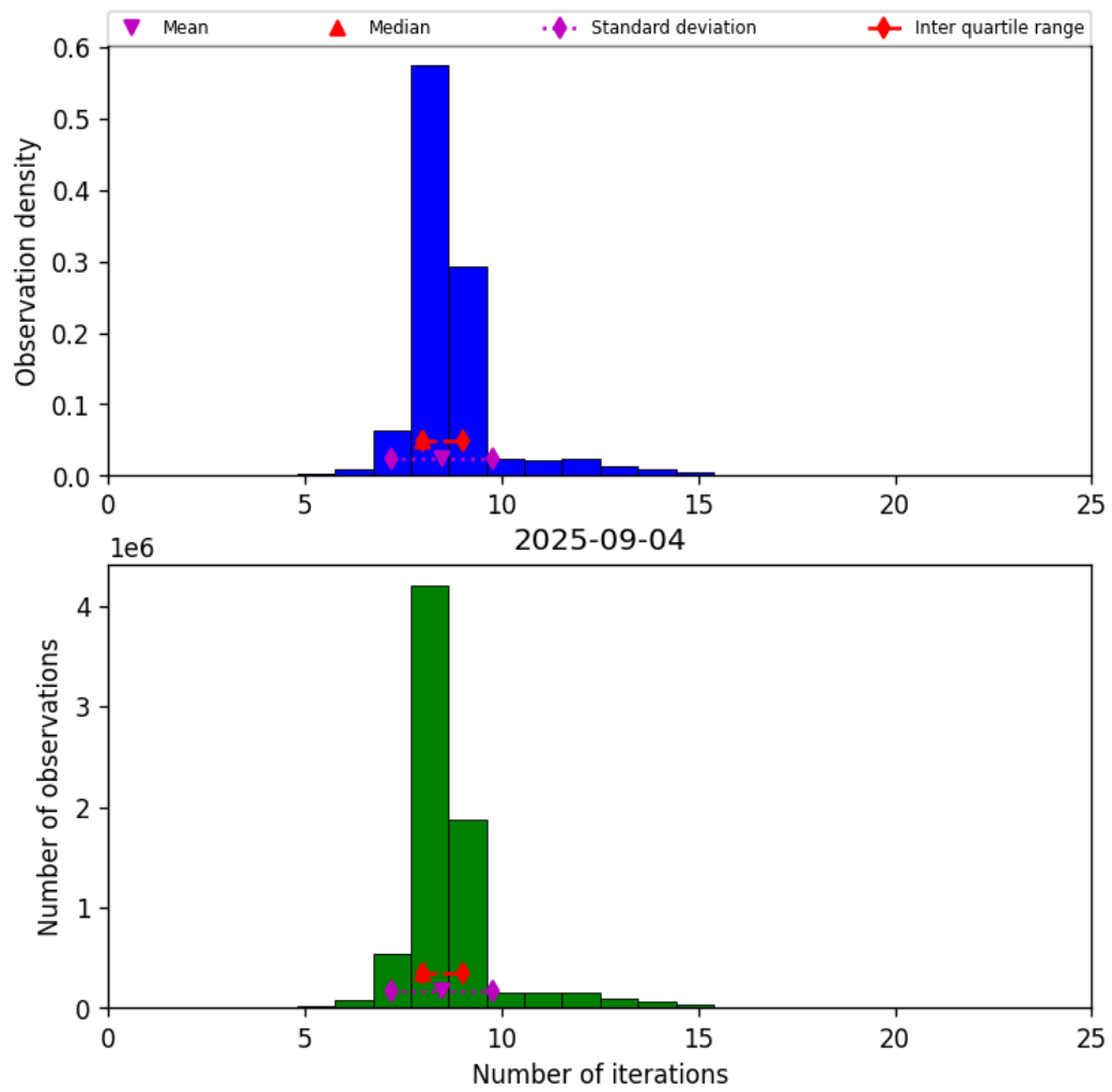
Figure 24: Histogram of “Number of iterations” for 2025-09-04 to 2025-09-05
