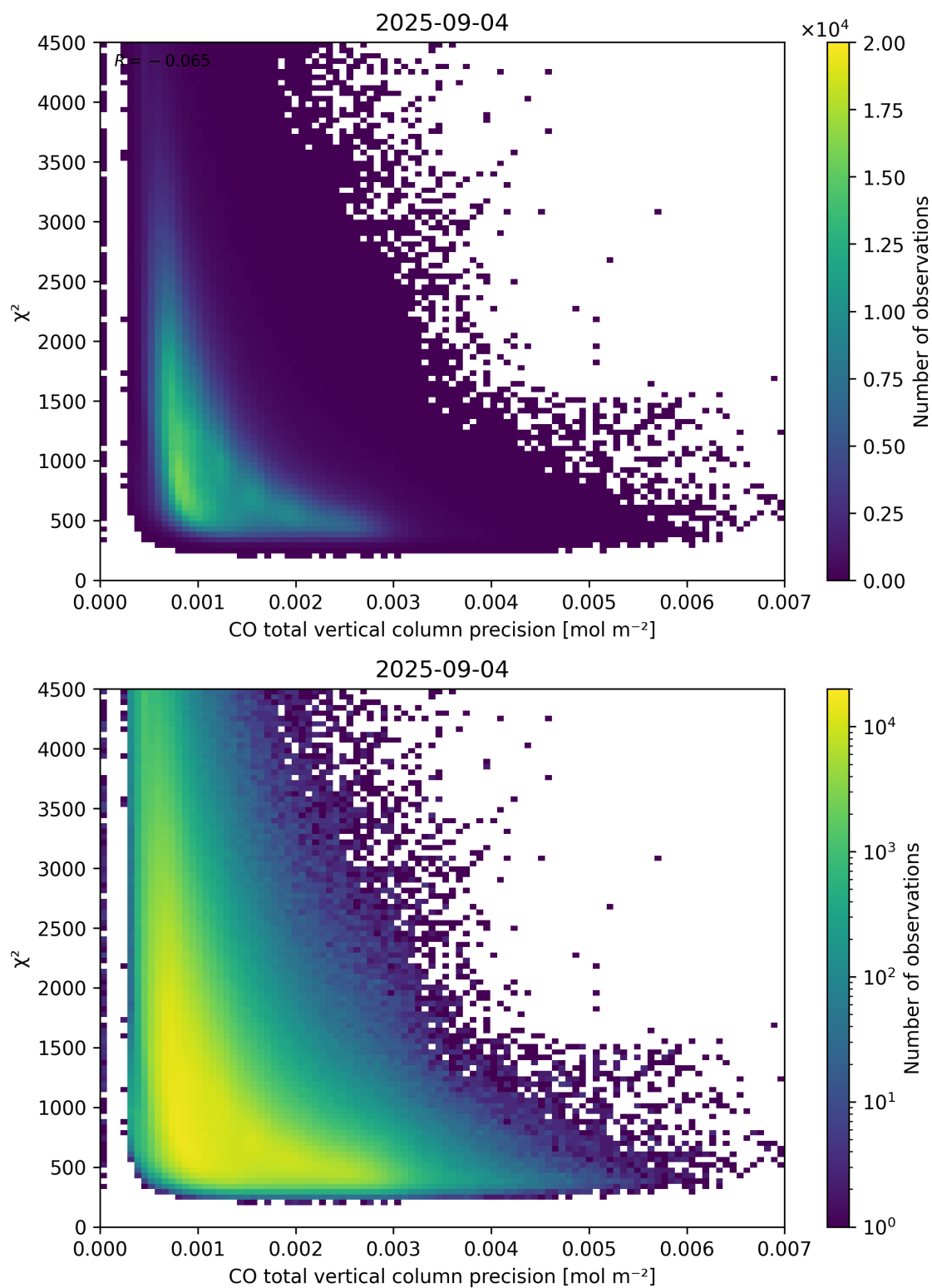
Figure 44: Scatter density plot of “CO total vertical column precision” against “ \chi^2 ” for 2025-09-04 to 2025-09-05.
