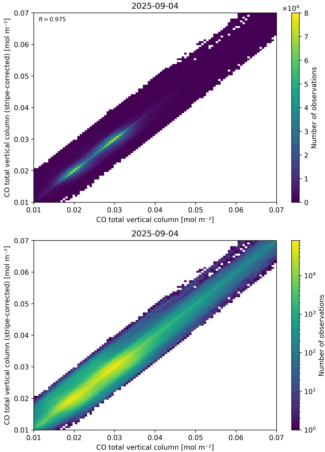
Figure 33: Scatter density plot of “CO total vertical column” against “CO total vertical column (stripe-corrected)” for 2025-09-04 to 2025-09-05.
