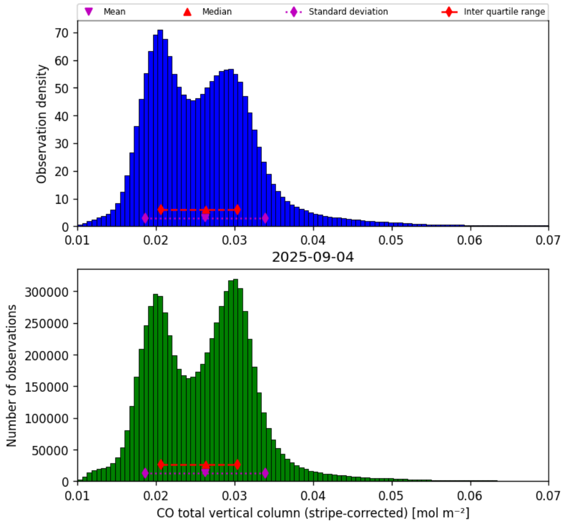
Figure 19: Histogram of “CO total vertical column (stripe-corrected)” for 2025-09-04 to 2025-09-05
