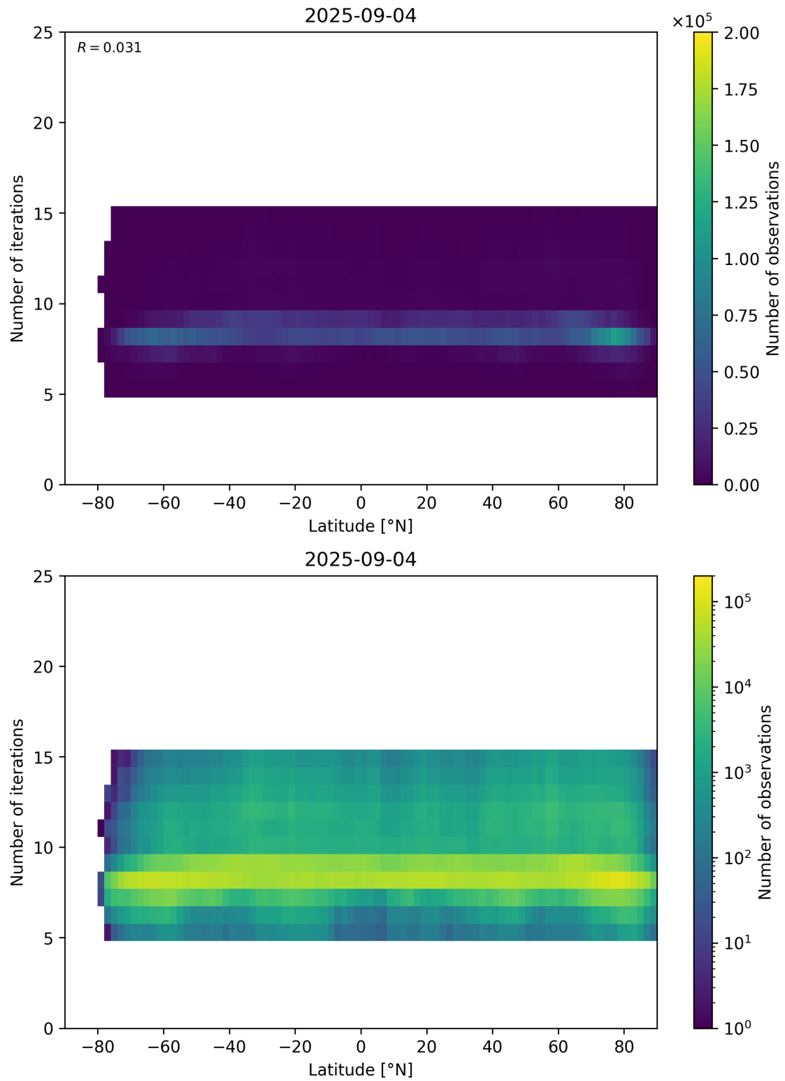
Figure 56: Scatter density plot of “Latitude” against “Number of iterations” for 2025-09-04 to 2025-09-05.
