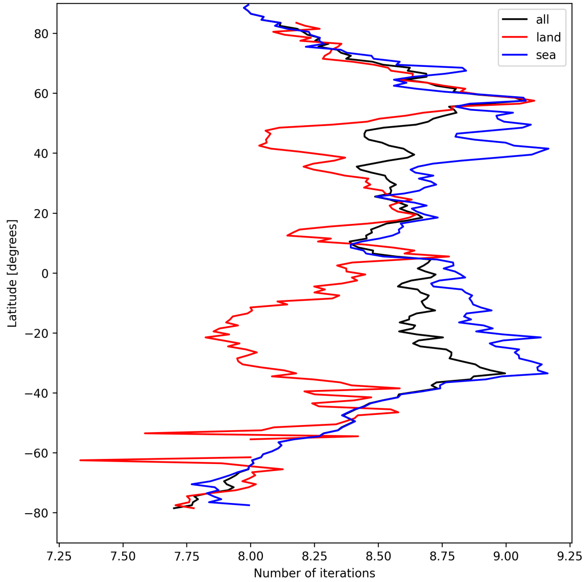
Figure 16: Zonal average of “Number of iterations” for 2025-09-04 to 2025-09-05.
