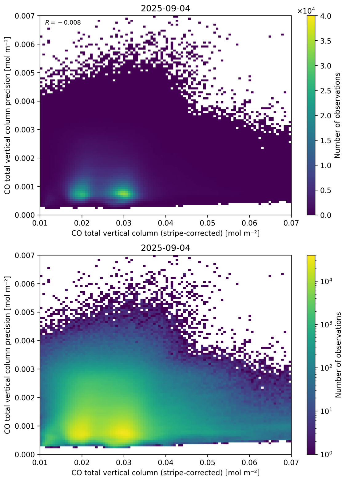
Figure 36: Scatter density plot of “CO total vertical column (stripe-corrected)” against “CO total vertical column precision” for 2025-09-04 to 2025-09-05.
