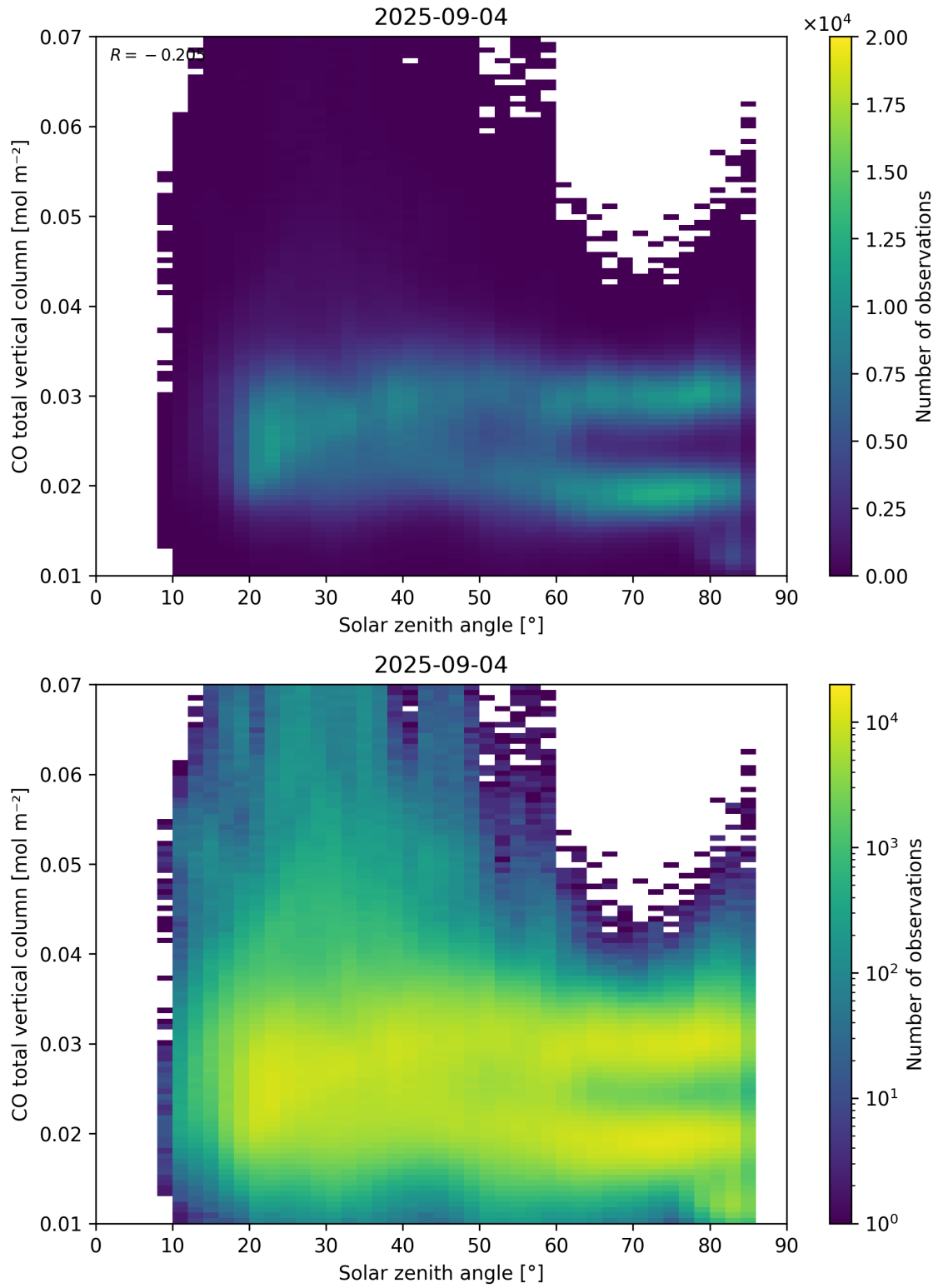
Figure 61: Scatter density plot of “Solar zenith angle” against “CO total vertical column” for 2025-09-04 to 2025-09-05.
