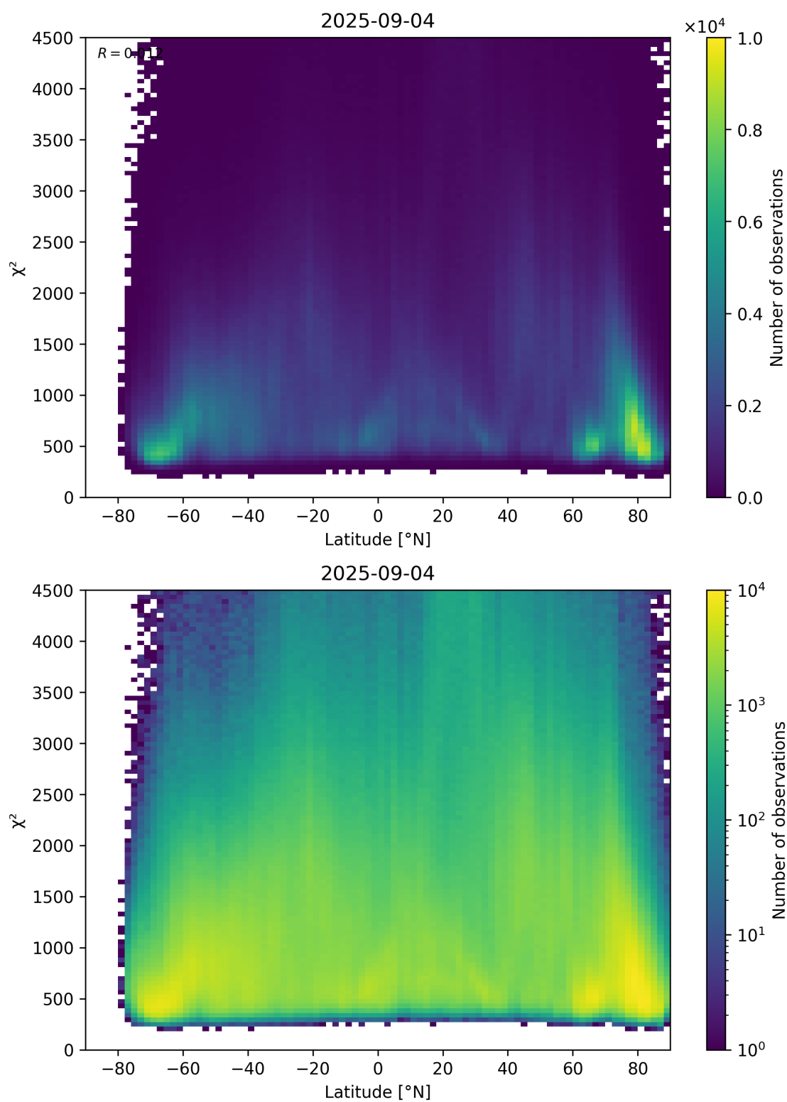
Figure 54: Scatter density plot of “Latitude” against “ \chi^2 ” for 2025-09-04 to 2025-09-05.
