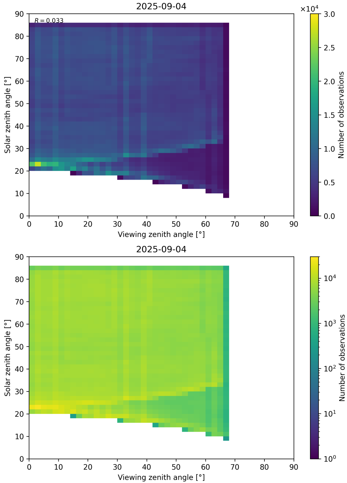
Figure 77: Scatter density plot of “Viewing zenith angle” against “Solar zenith angle” for 2025-09-04 to 2025-09-05.
