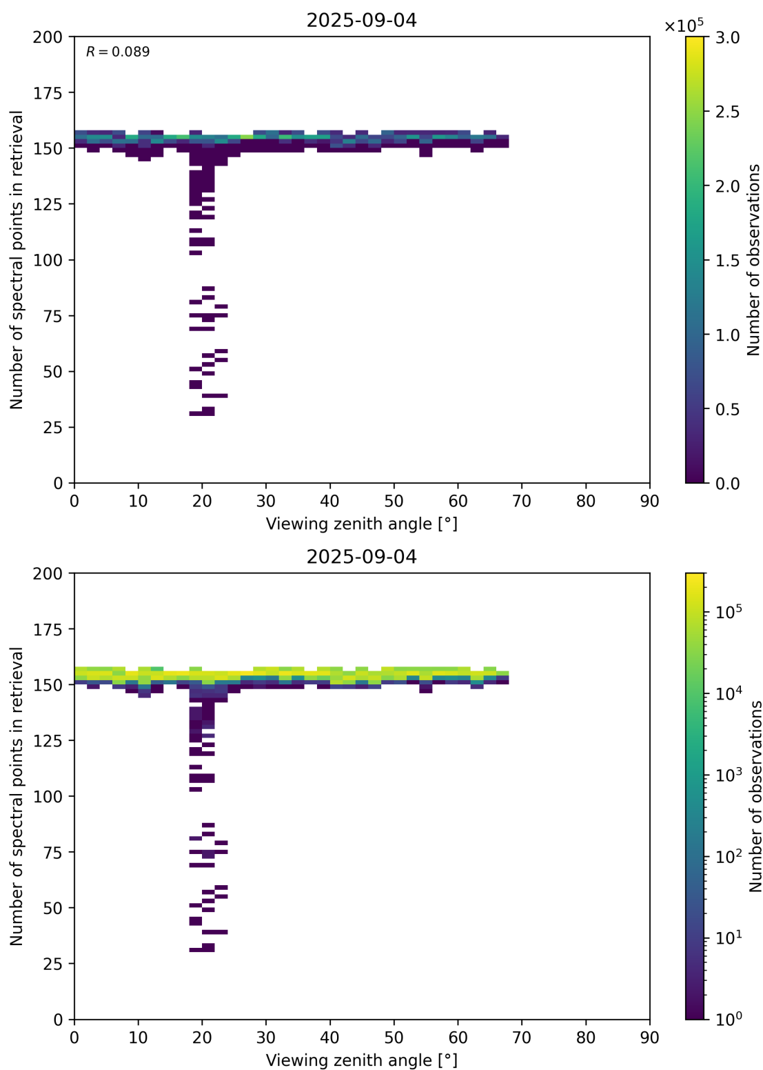
Figure 76: Scatter density plot of “Viewing zenith angle” against “Number of spectral points in retrieval” for 2025-09-04 to 2025-09-05.
