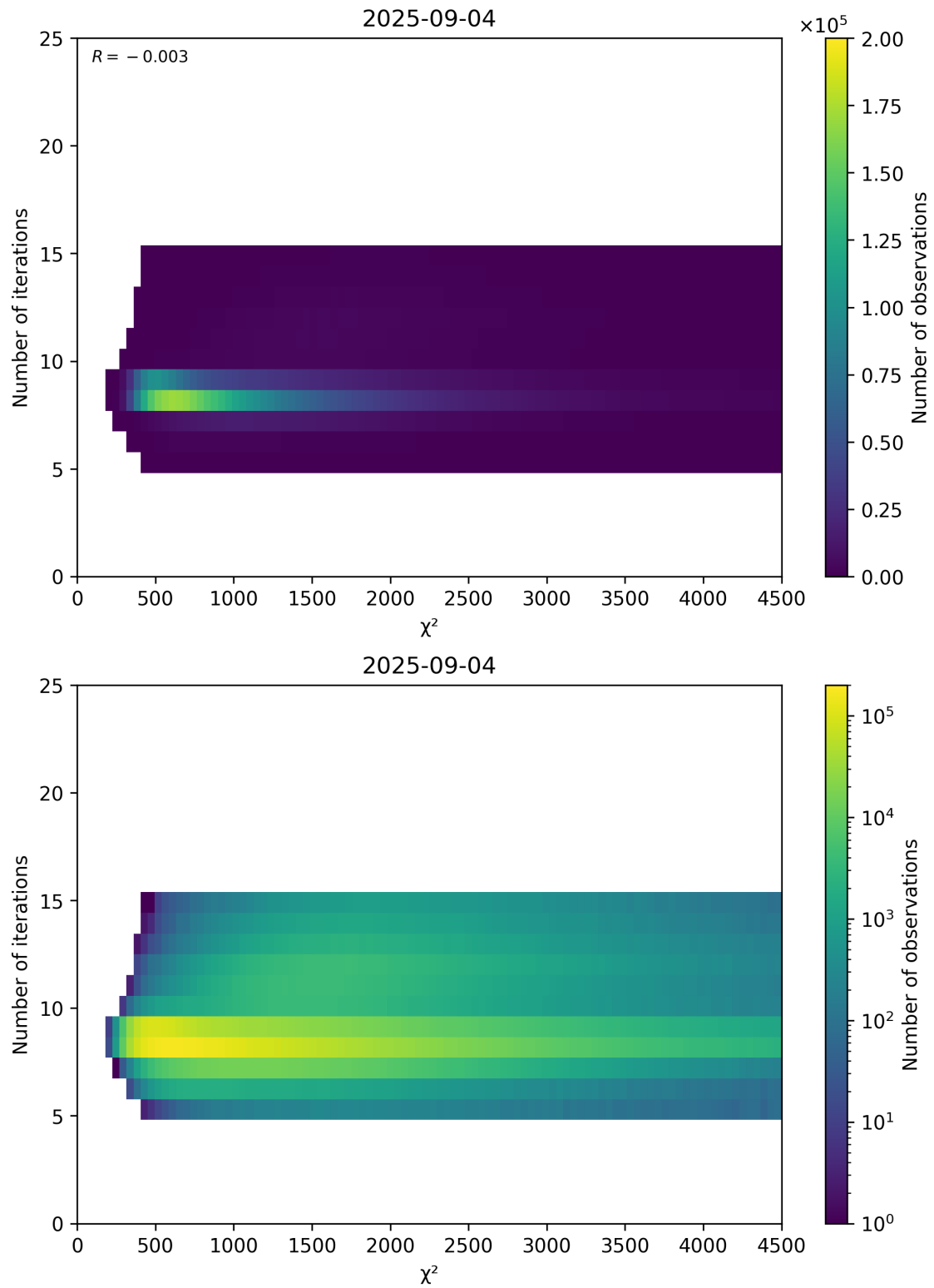
Figure 49: Scatter density plot of “ \chi^2 ” against “Number of iterations” for 2025-09-04 to 2025-09-05.
