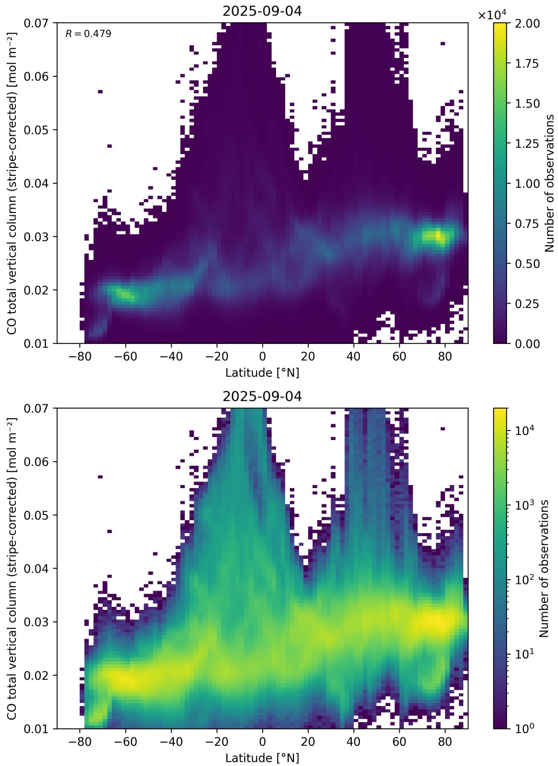
Figure 52: Scatter density plot of “Latitude” against “CO total vertical column (stripe-corrected)” for 2025-09-04 to 2025-09-05.
