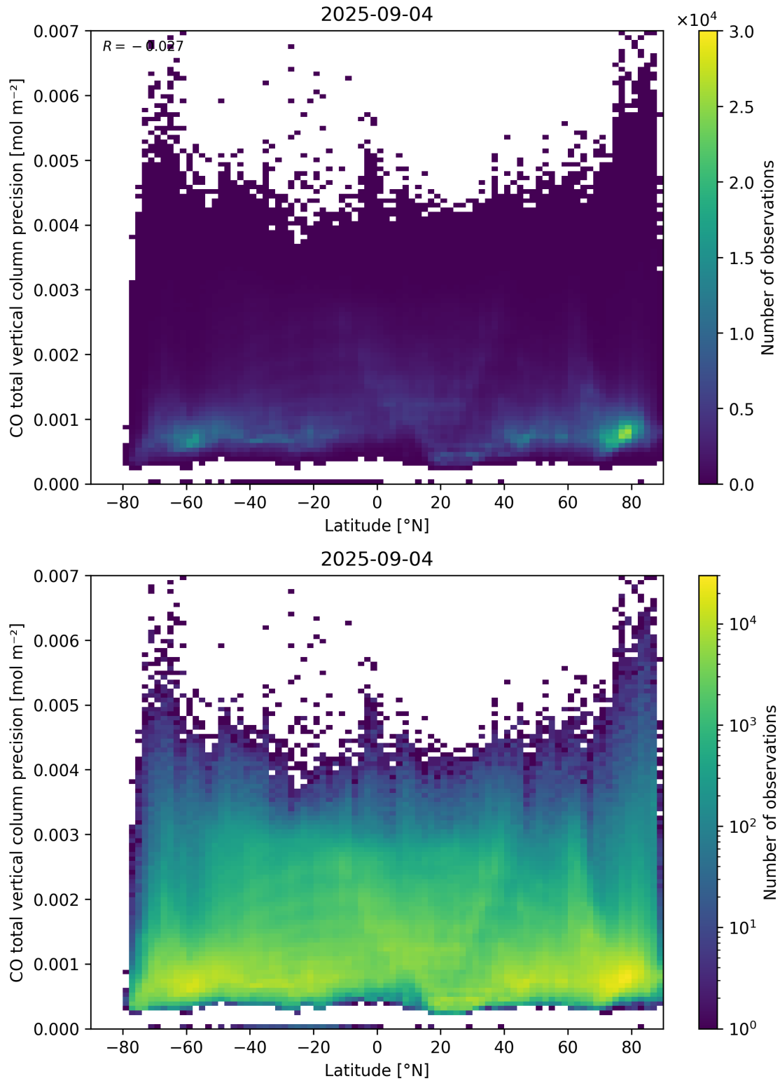
Figure 53: Scatter density plot of “Latitude” against “CO total vertical column precision” for 2025-09-04 to 2025-09-05.
