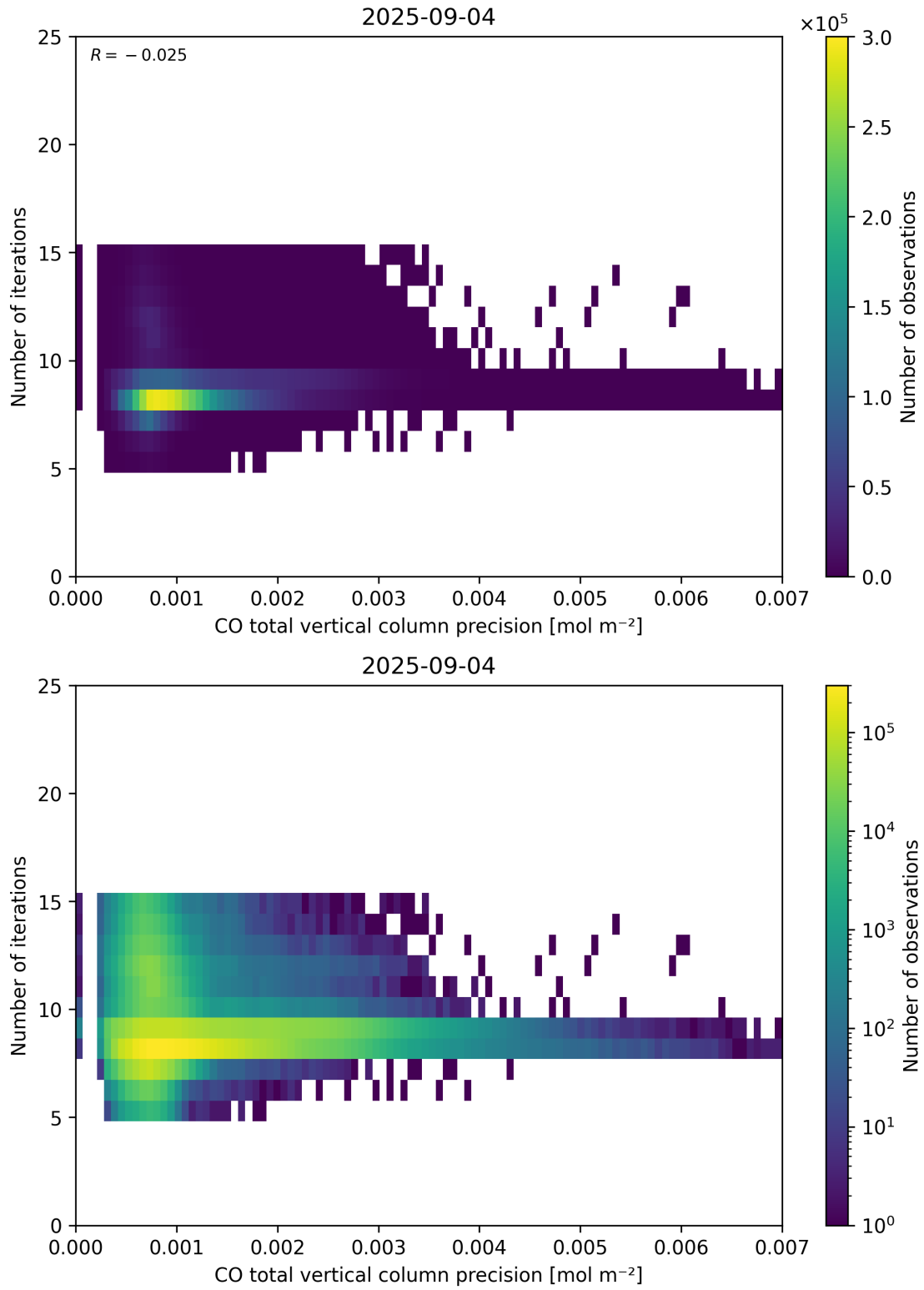
Figure 46: Scatter density plot of “CO total vertical column precision” against “Number of iterations” for 2025-09-04 to 2025-09-05.
