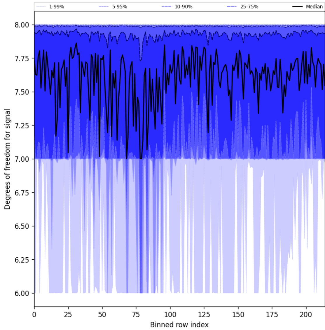
Figure 31: Along track statistics of “Degrees of freedom for signal” for 2025-09-04 to 2025-09-05
