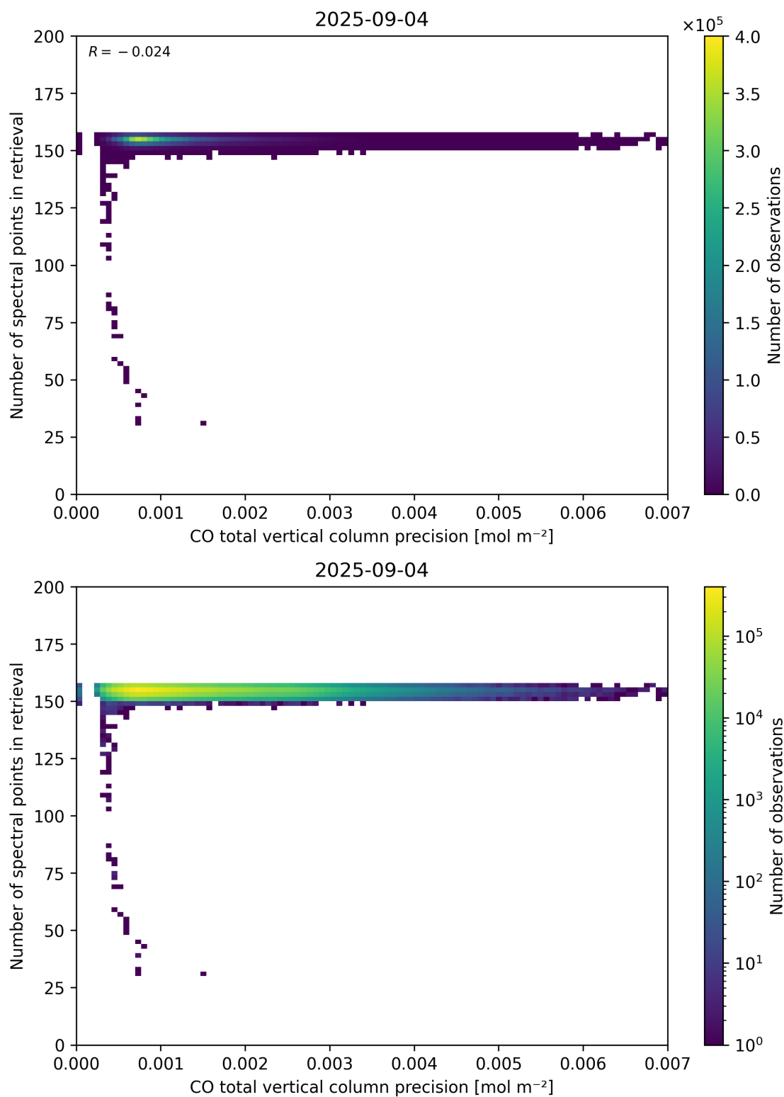
Figure 47: Scatter density plot of “CO total vertical column precision” against “Number of spectral points in retrieval” for 2025-09-04 to 2025-09-05.
