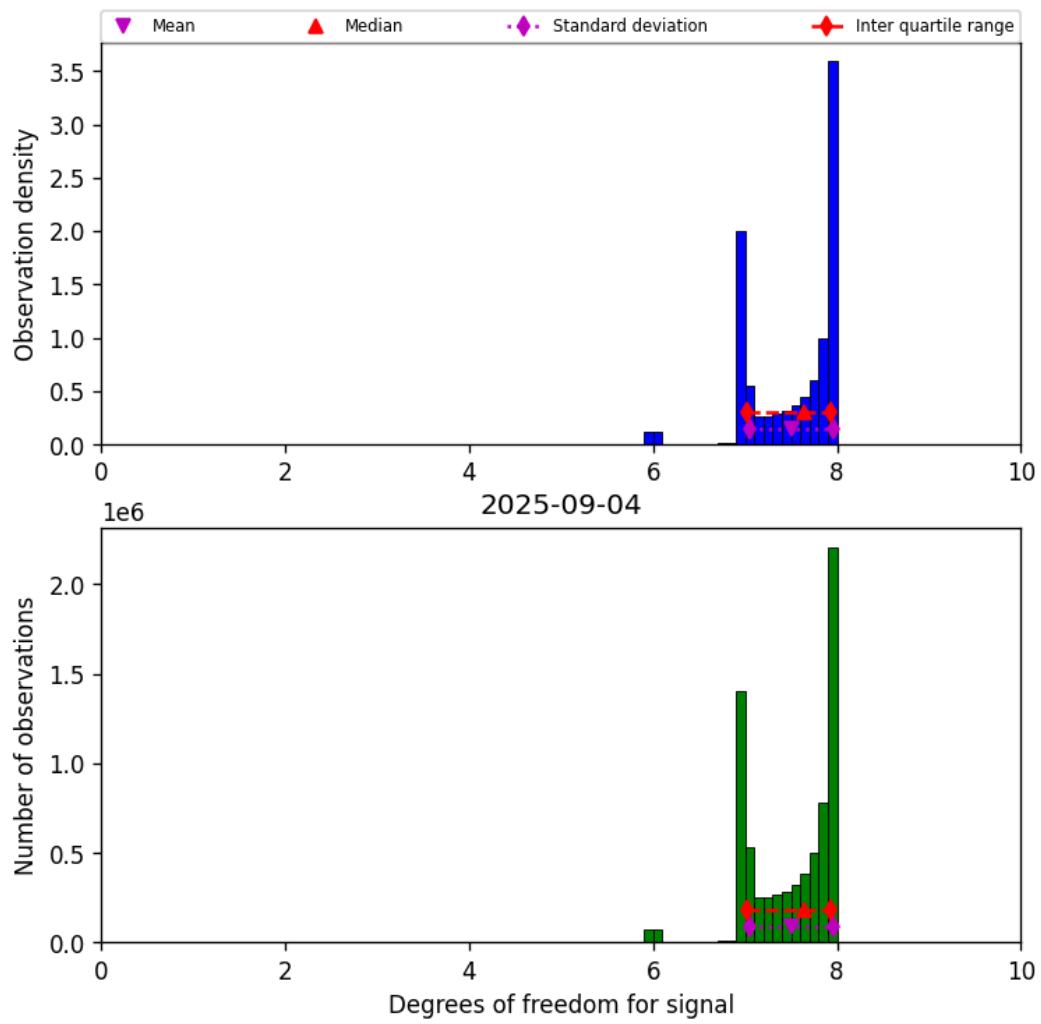
Figure 23: Histogram of “Degrees of freedom for signal” for 2025-09-04 to 2025-09-05
