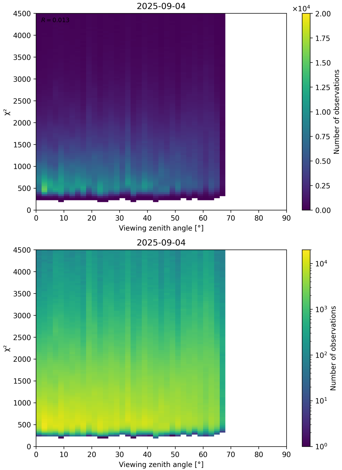
Figure 72: Scatter density plot of “Viewing zenith angle” against “ \chi^2 ” for 2025-09-04 to 2025-09-05.
