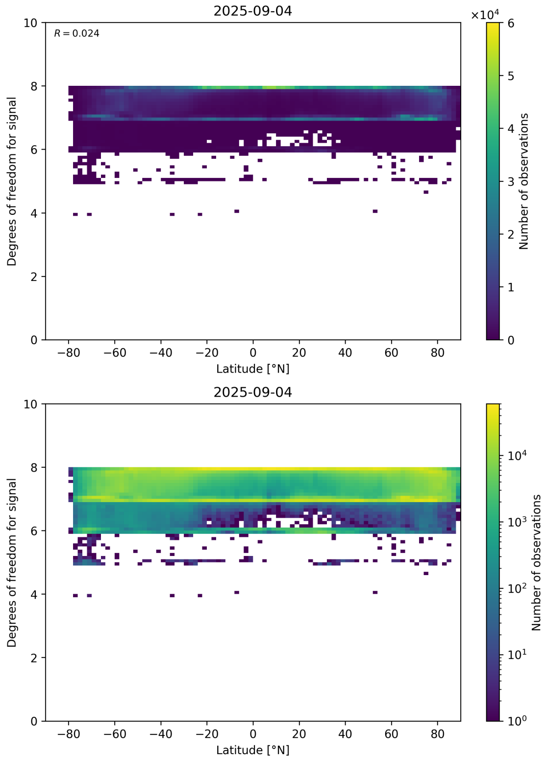
Figure 55: Scatter density plot of “Latitude” against “Degrees of freedom for signal” for 2025-09-04 to 2025-09-05.
