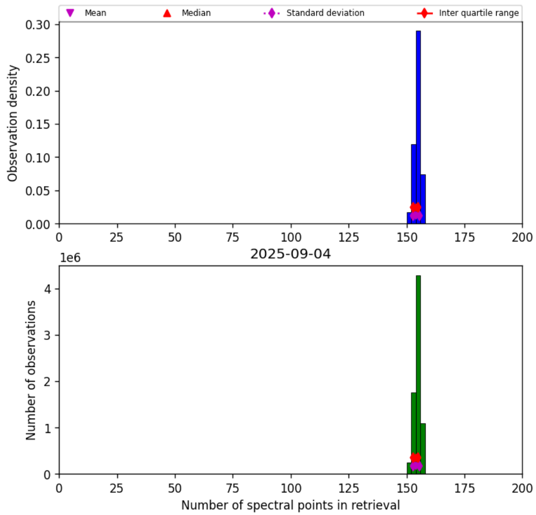
Figure 21: Histogram of “Number of spectral points in retrieval” for 2025-09-04 to 2025-09-05
