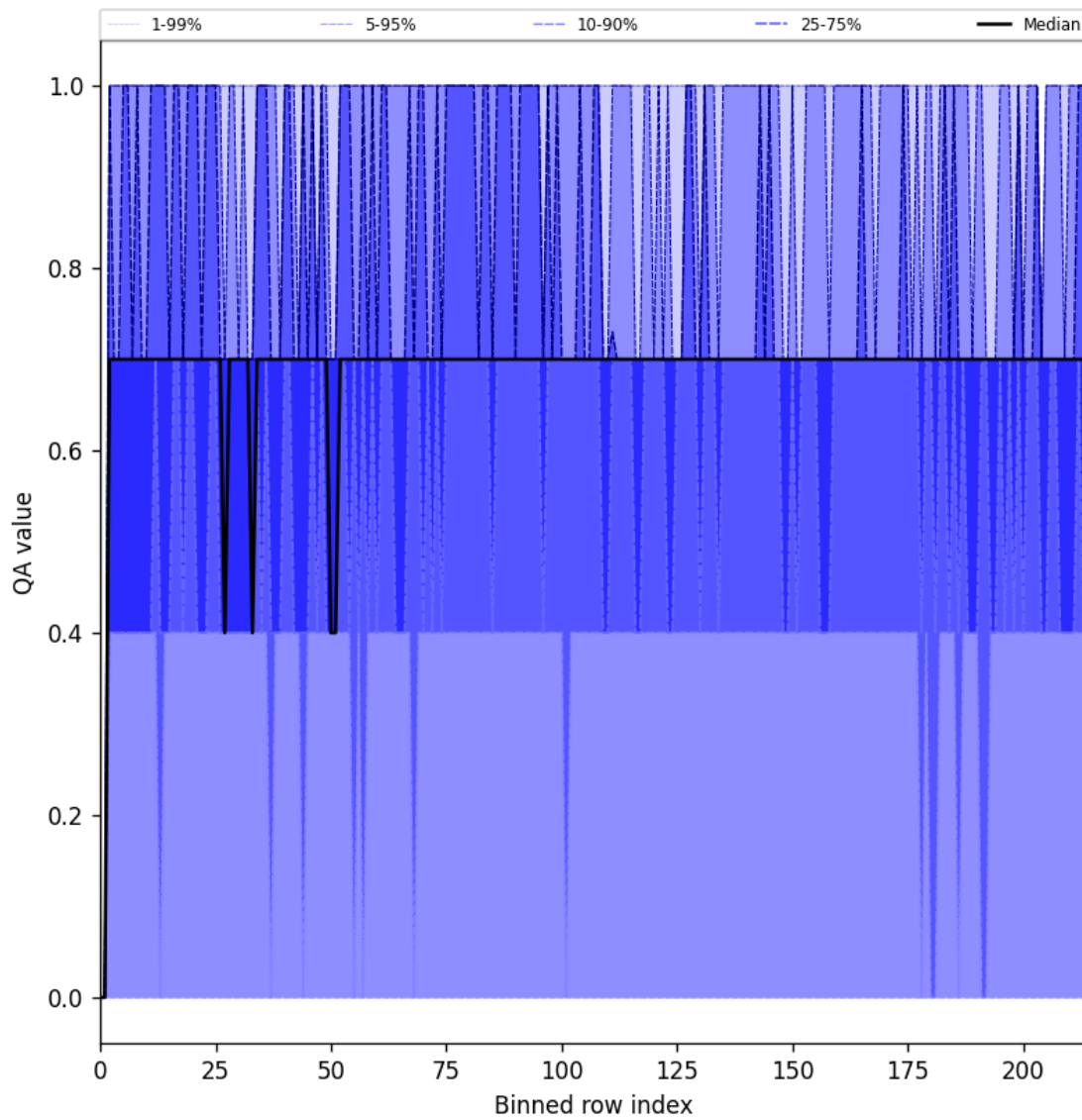
Figure 25: Along track statistics of “QA value” for 2025-09-04 to 2025-09-05
