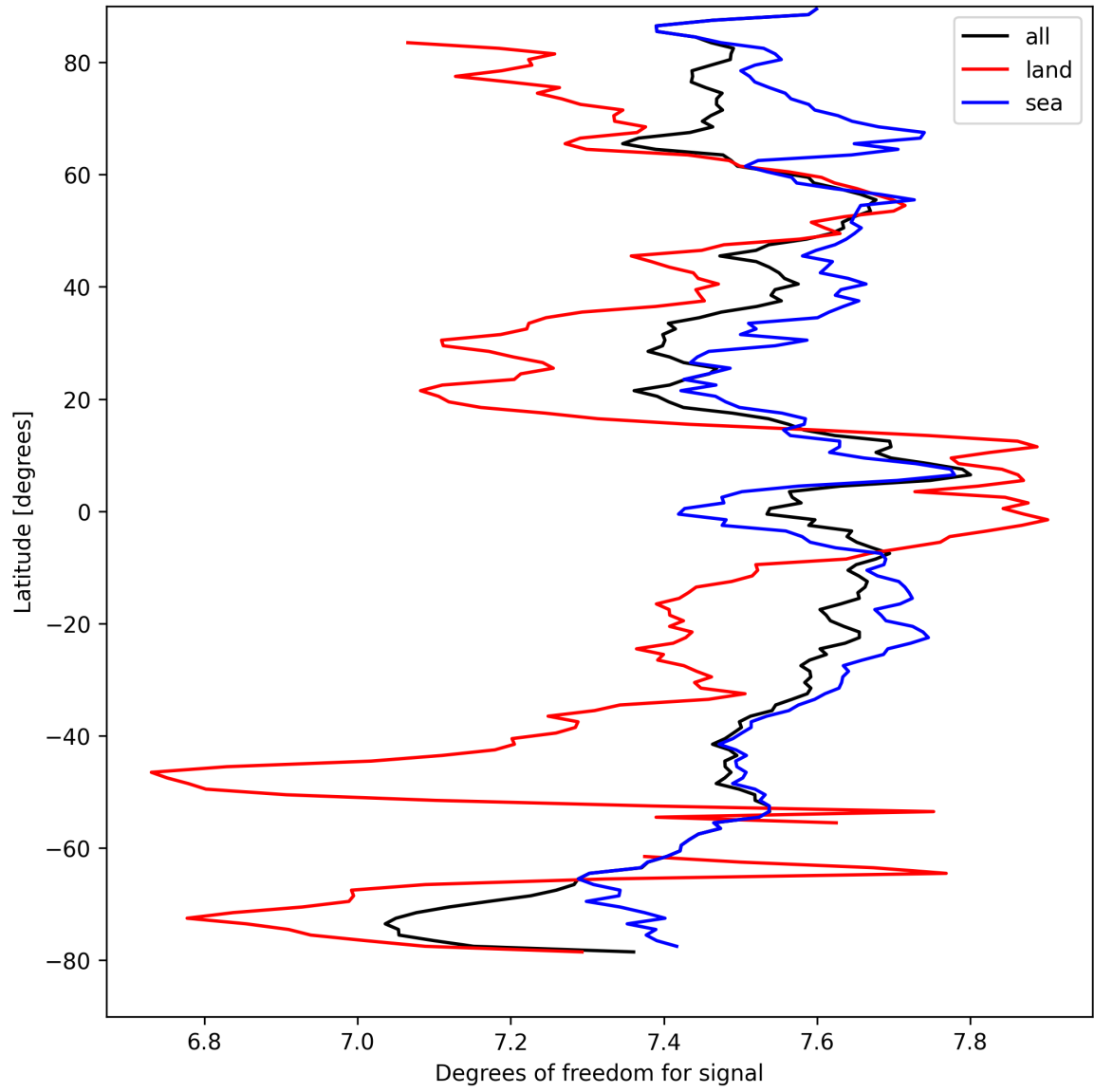
Figure 15: Zonal average of “Degrees of freedom for signal” for 2025-09-04 to 2025-09-05.
