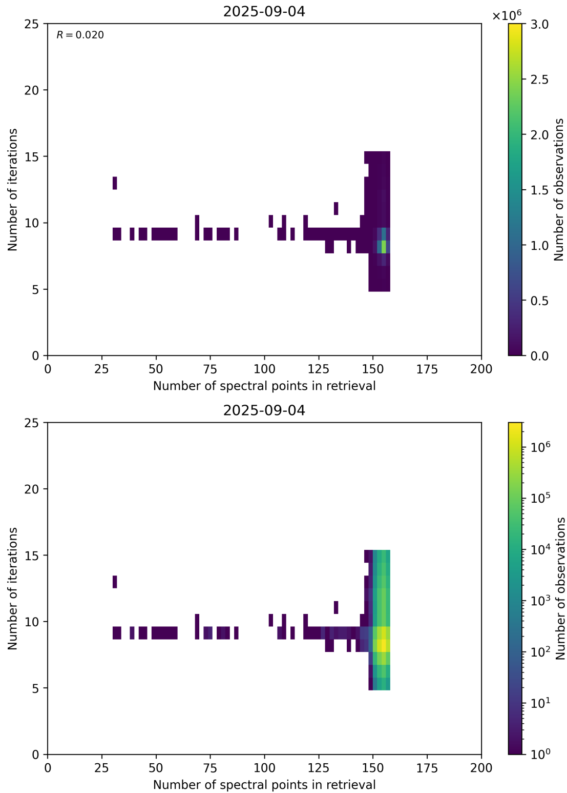
Figure 60: Scatter density plot of “Number of spectral points in retrieval” against “Number of iterations” for 2025-09-04 to 2025-09-05.
