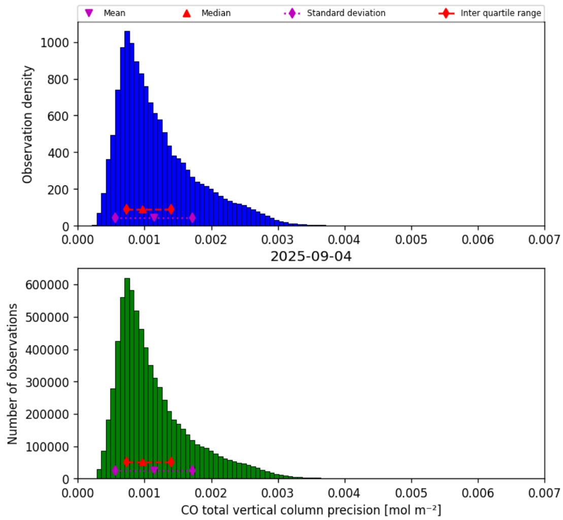
Figure 20: Histogram of “CO total vertical column precision” for 2025-09-04 to 2025-09-05
