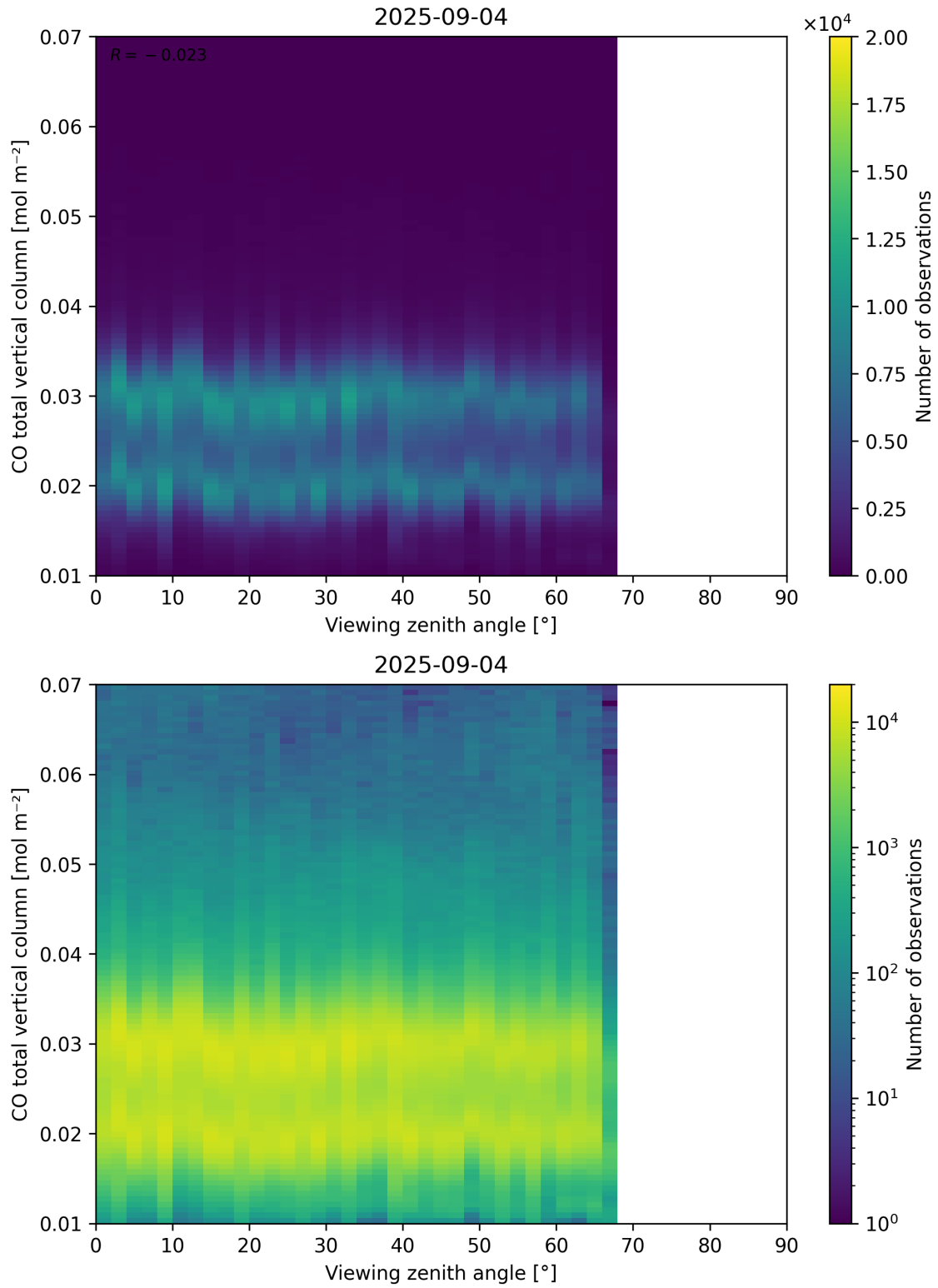
Figure 69: Scatter density plot of “Viewing zenith angle” against “CO total vertical column” for 2025-09-04 to 2025-09-05.
