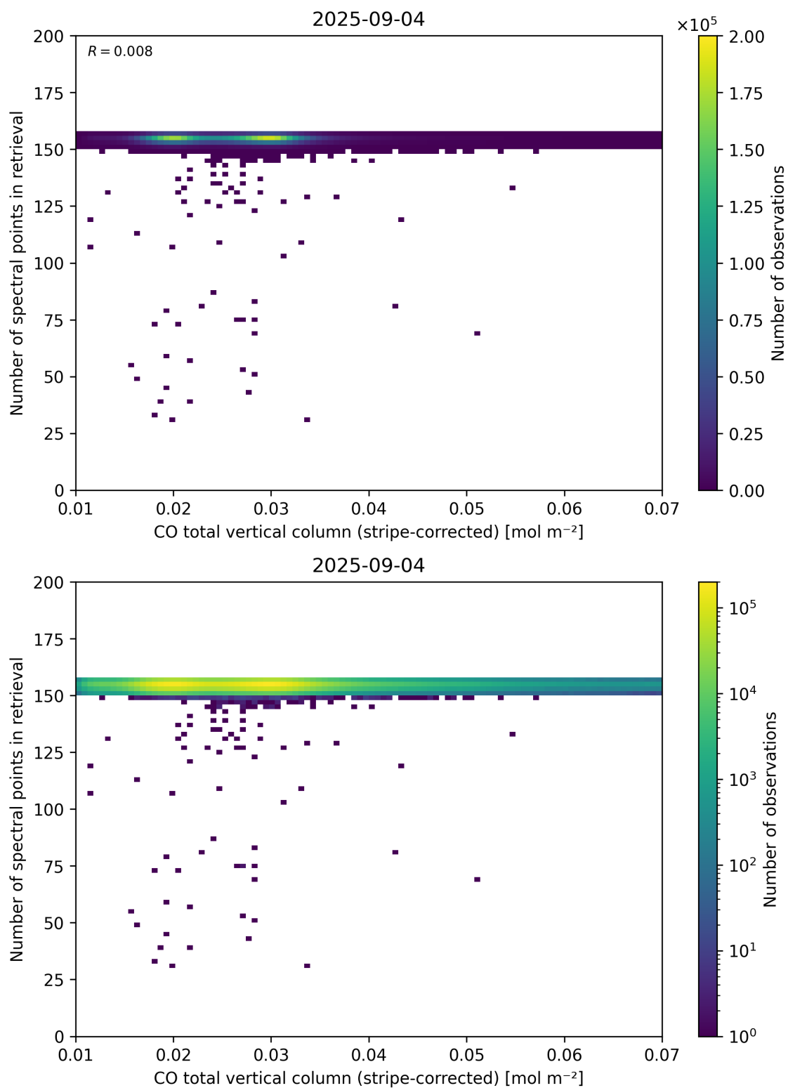
Figure 40: Scatter density plot of “CO total vertical column (stripe-corrected)” against “Number of spectral points in retrieval” for 2025-09-04 to 2025-09-05.
