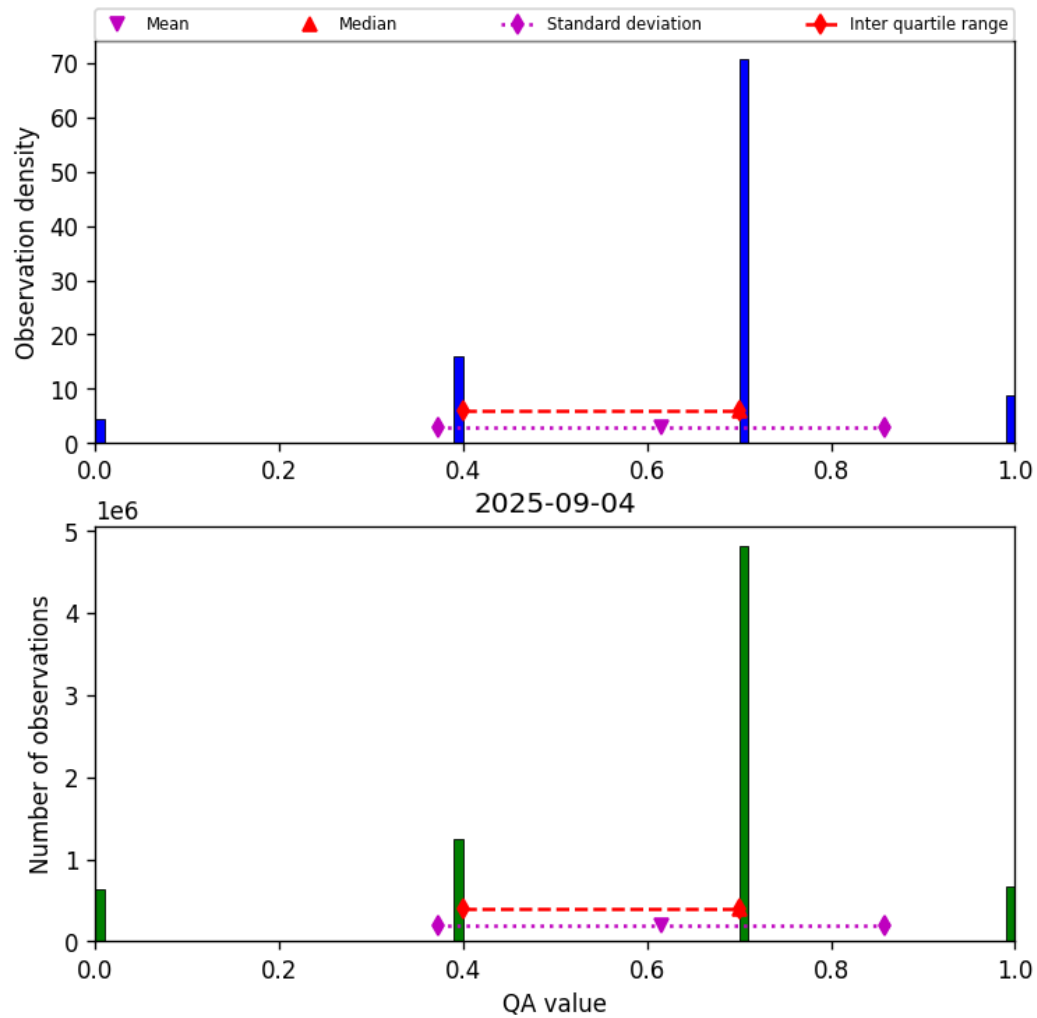
Figure 17: Histogram of “QA value” for 2025-09-04 to 2025-09-05
