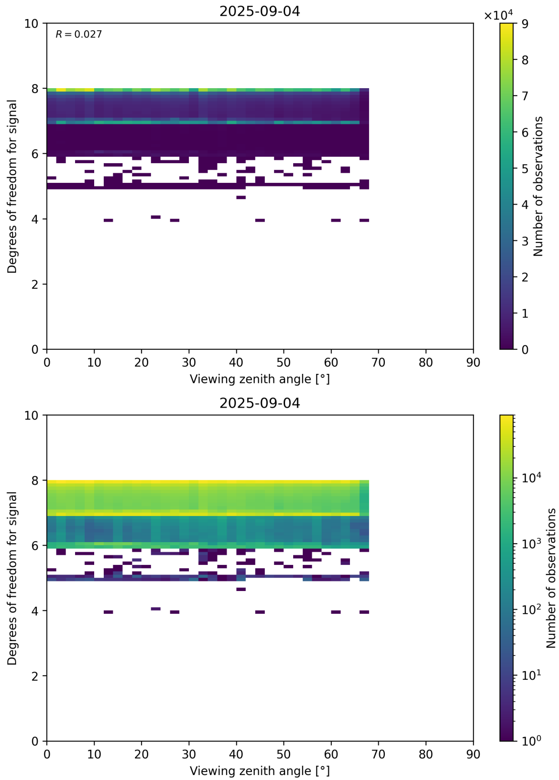
Figure 73: Scatter density plot of “Viewing zenith angle” against “Degrees of freedom for signal” for 2025-09-04 to 2025-09-05.
