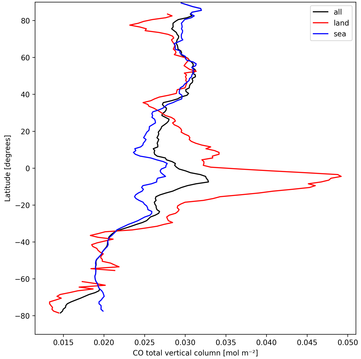
Figure 10: Zonal average of “CO total vertical column” for 2025-09-04 to 2025-09-05.
