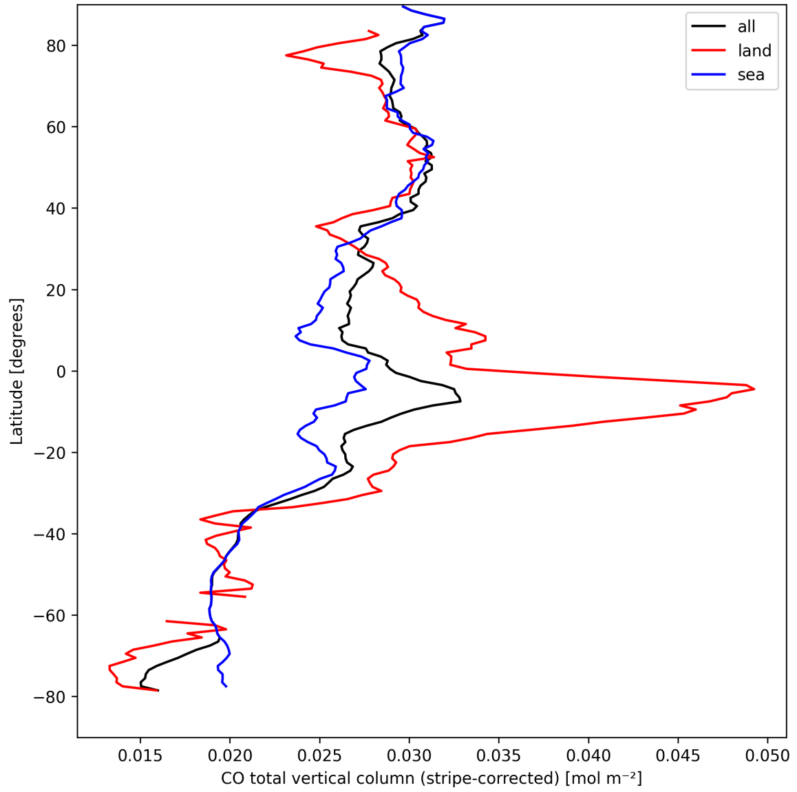
Figure 11: Zonal average of “CO total vertical column (stripe-corrected)” for 2025-09-04 to 2025-09-05.
