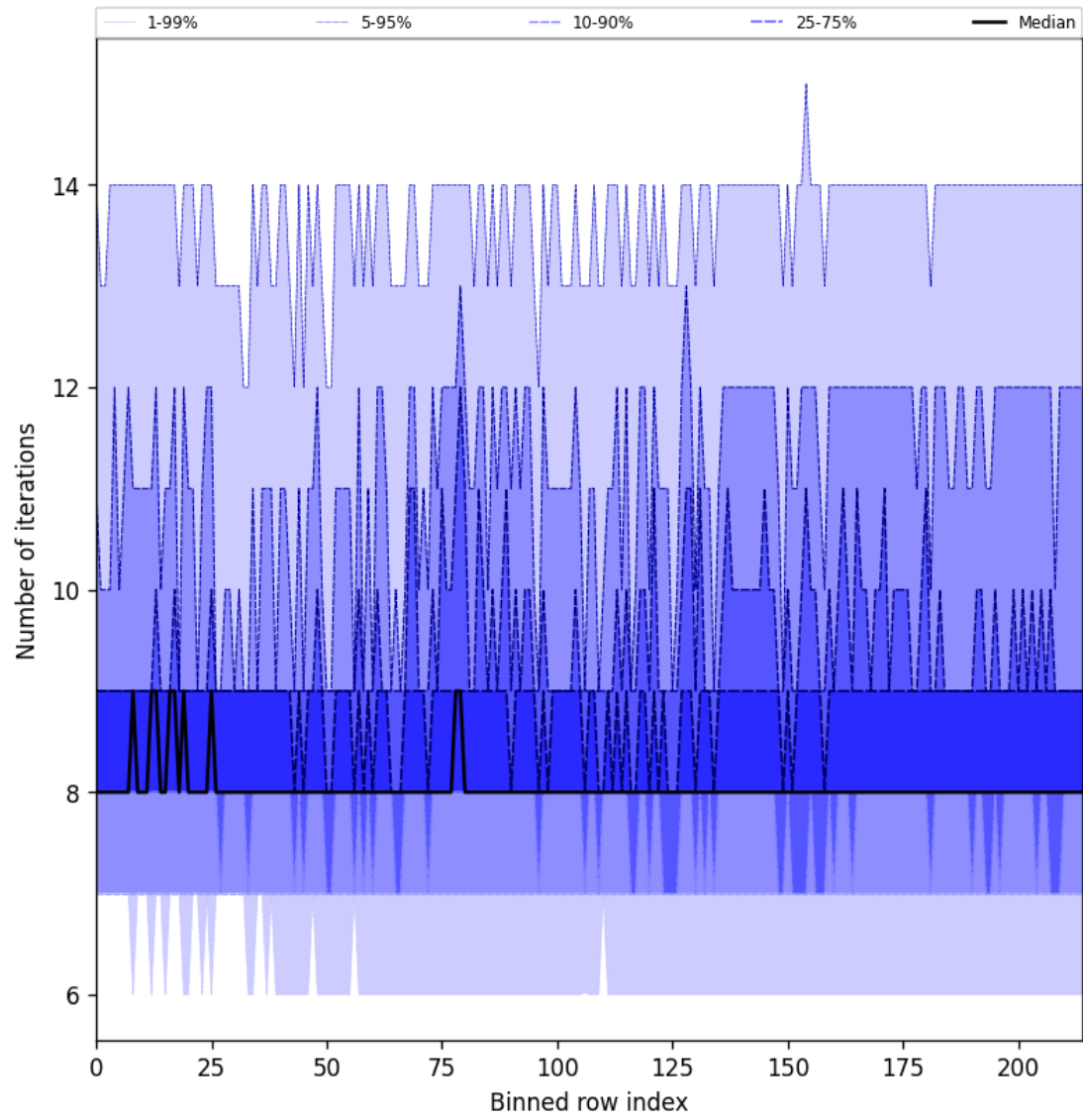
Figure 32: Along track statistics of “Number of iterations” for 2025-09-04 to 2025-09-05
