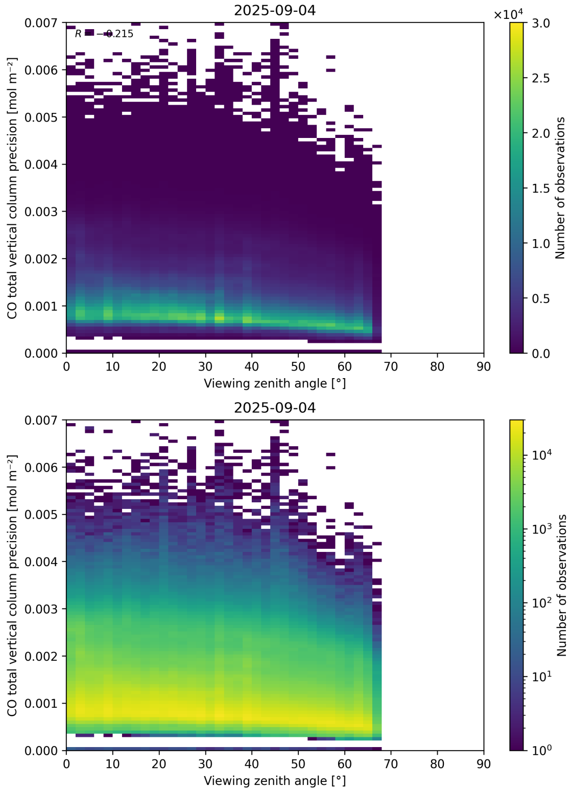
Figure 71: Scatter density plot of “Viewing zenith angle” against “CO total vertical column precision” for 2025-09-04 to 2025-09-05.
