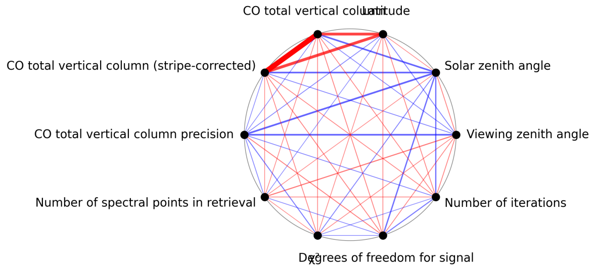
Figure 1: Map of correlation graph for 2025-09-04 to 2025-09-05.
