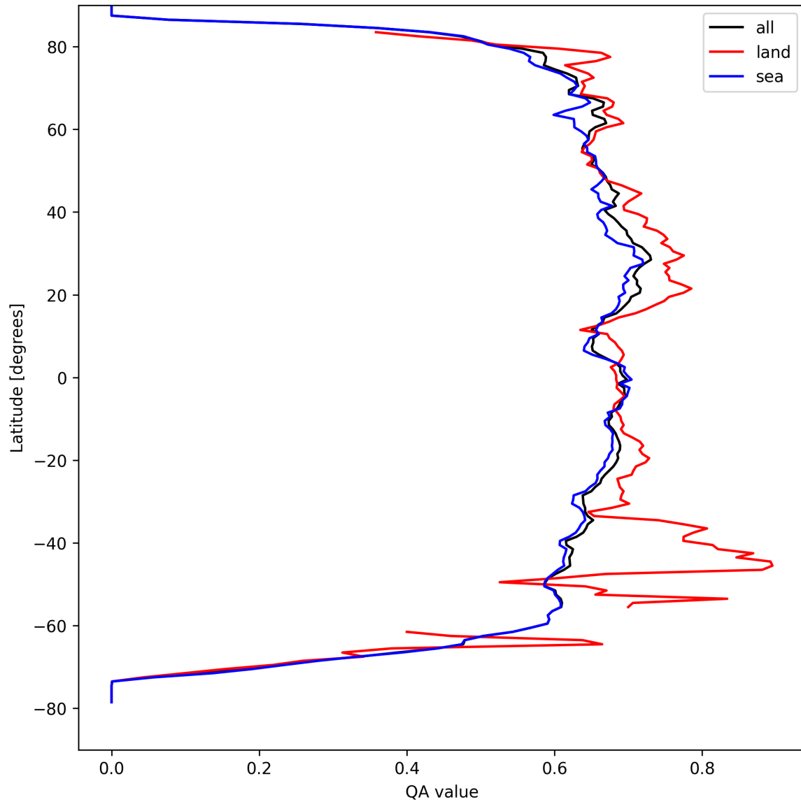
Figure 9: Zonal average of “QA value” for 2025-09-04 to 2025-09-06.
