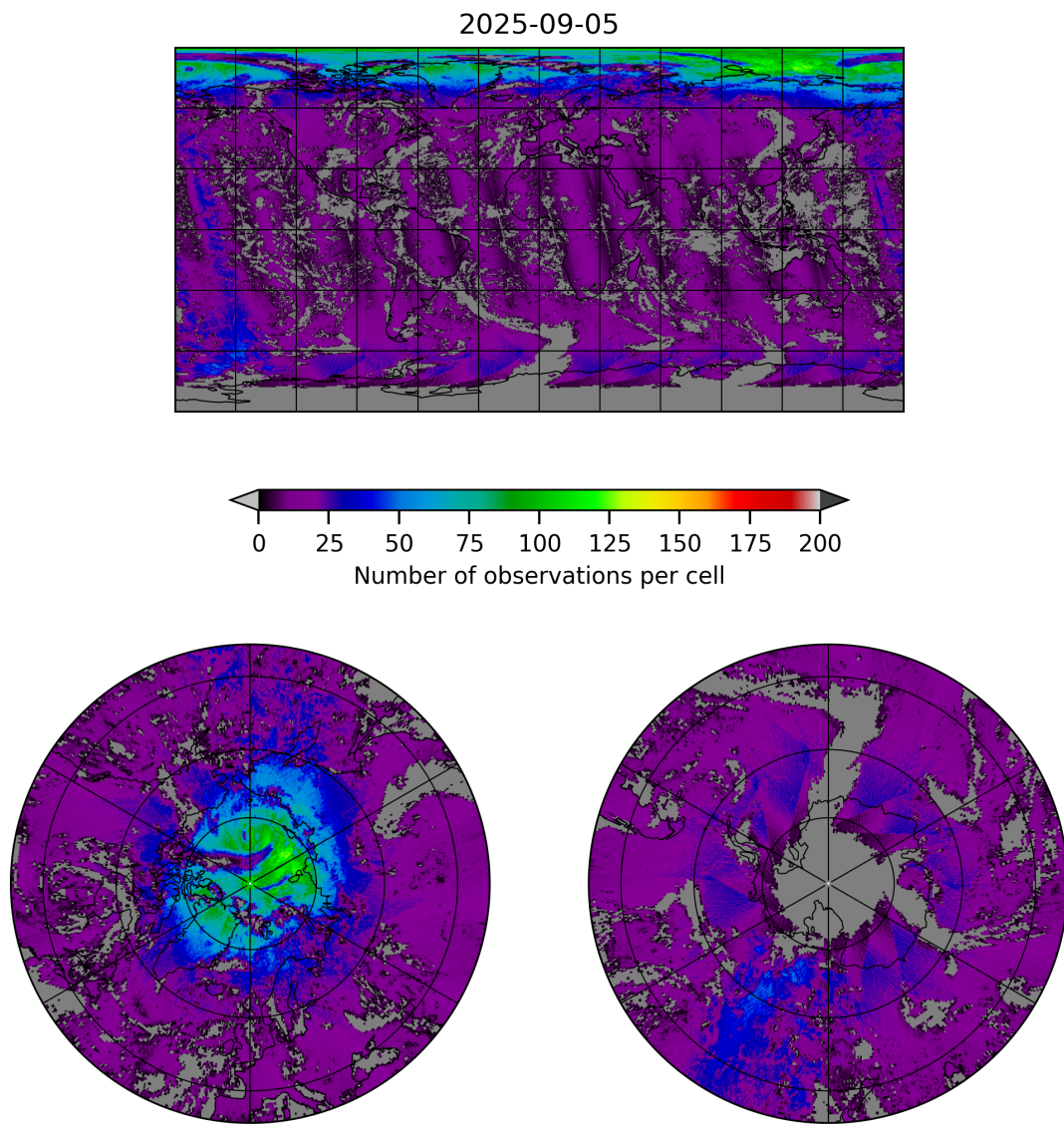
Figure 8: Map of the number of observations for 2025-09-04 to 2025-09-06
