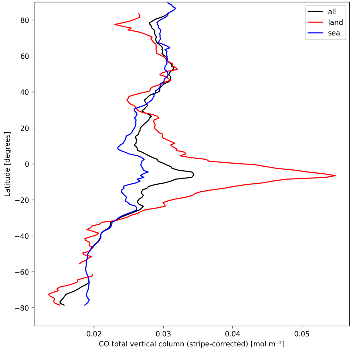
Figure 11: Zonal average of “CO total vertical column (stripe-corrected)” for 2025-09-04 to 2025-09-06.
