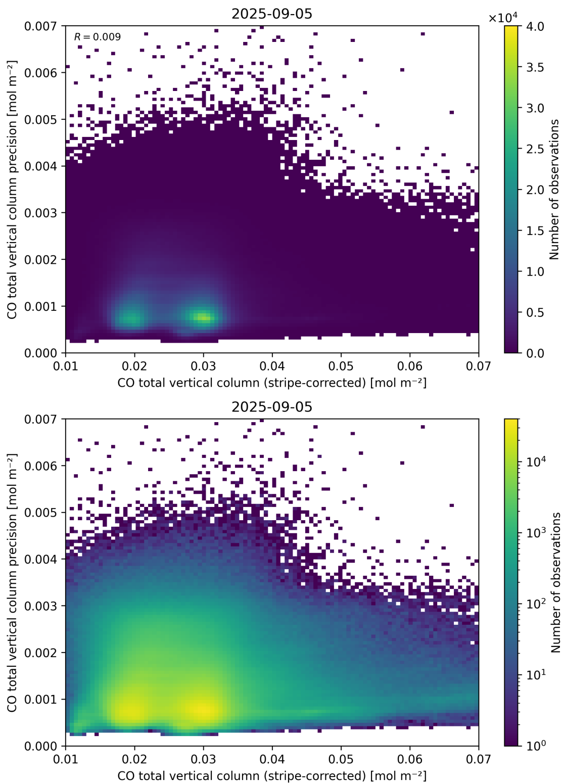
Figure 36: Scatter density plot of “CO total vertical column (stripe-corrected)” against “CO total vertical column precision” for 2025-09-04 to 2025-09-06.
