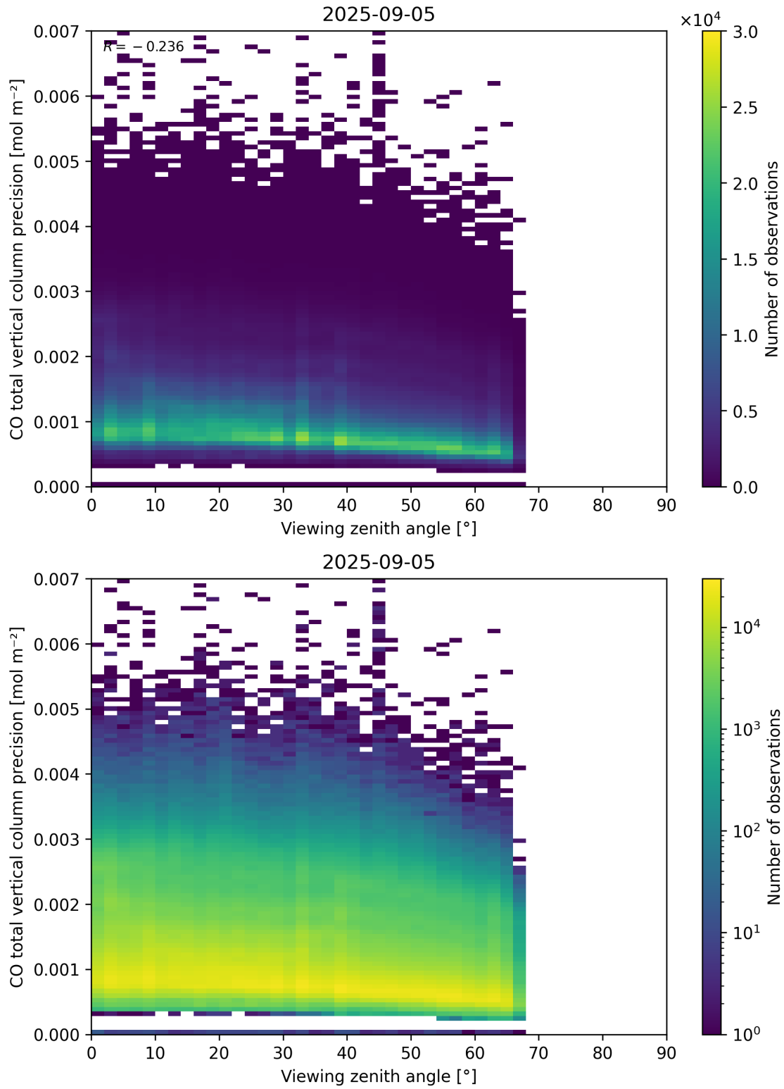
Figure 71: Scatter density plot of “Viewing zenith angle” against “CO total vertical column precision” for 2025-09-04 to 2025-09-06.
