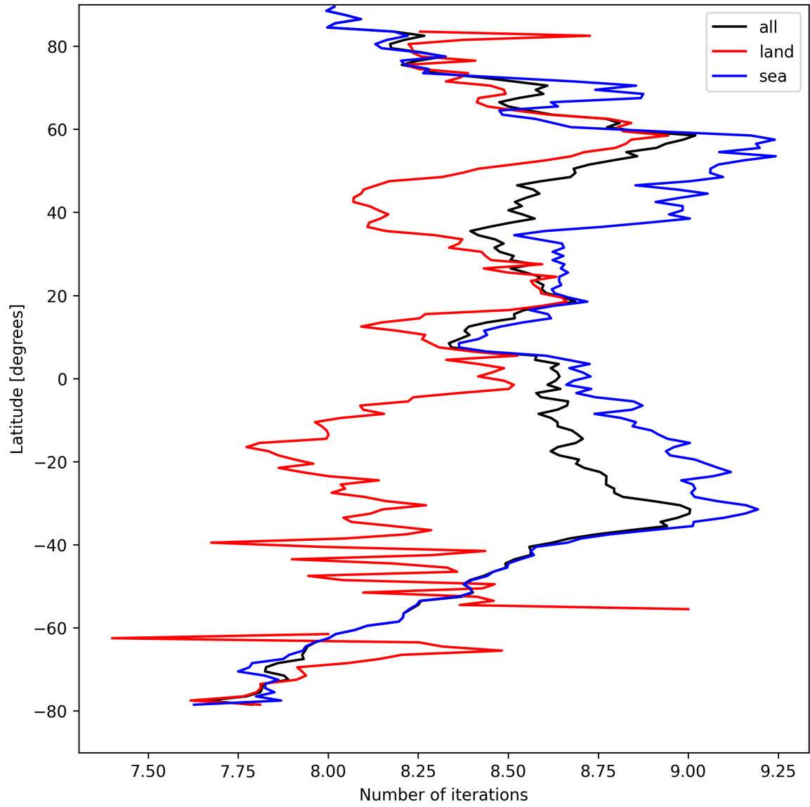
Figure 16: Zonal average of “Number of iterations” for 2025-09-04 to 2025-09-06.
