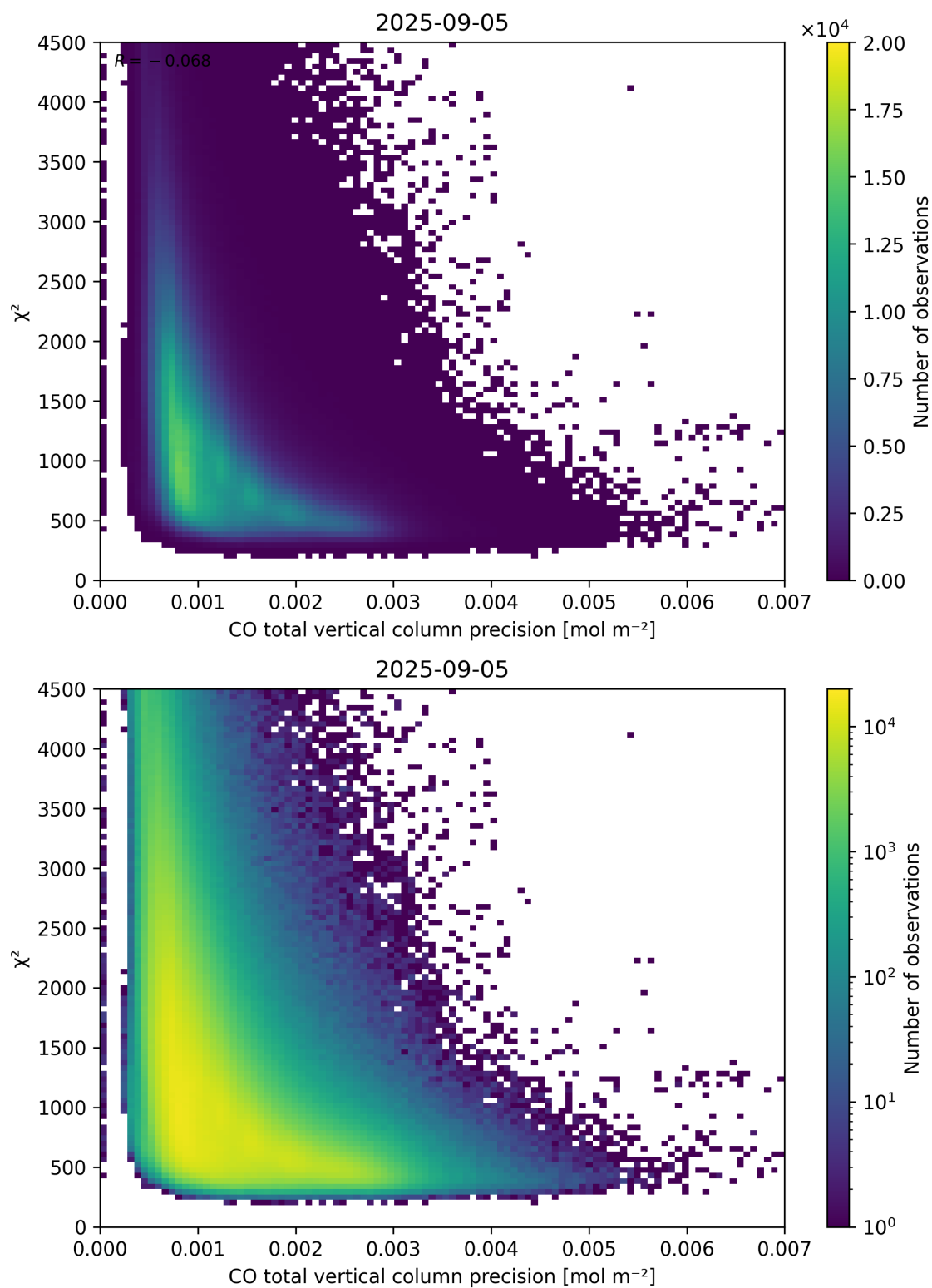
Figure 44: Scatter density plot of “CO total vertical column precision” against “ \chi^2 ” for 2025-09-04 to 2025-09-06.
