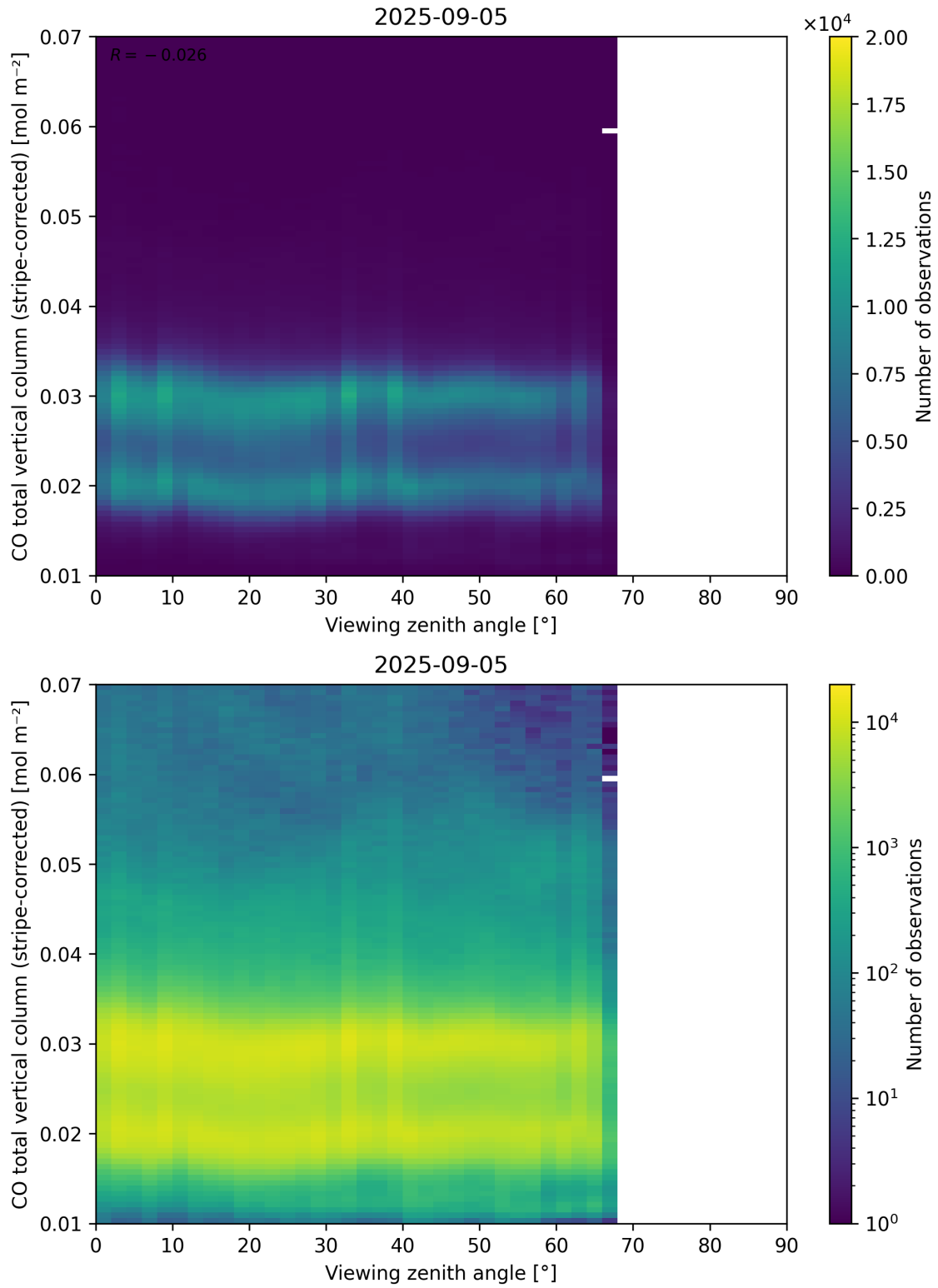
Figure 70: Scatter density plot of “Viewing zenith angle” against “CO total vertical column (stripe-corrected)” for 2025-09-04 to 2025-09-06.
