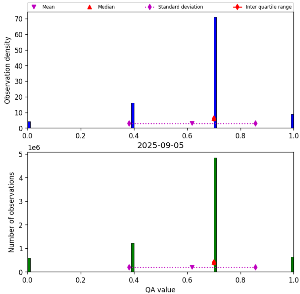
Figure 17: Histogram of “QA value” for 2025-09-04 to 2025-09-06
