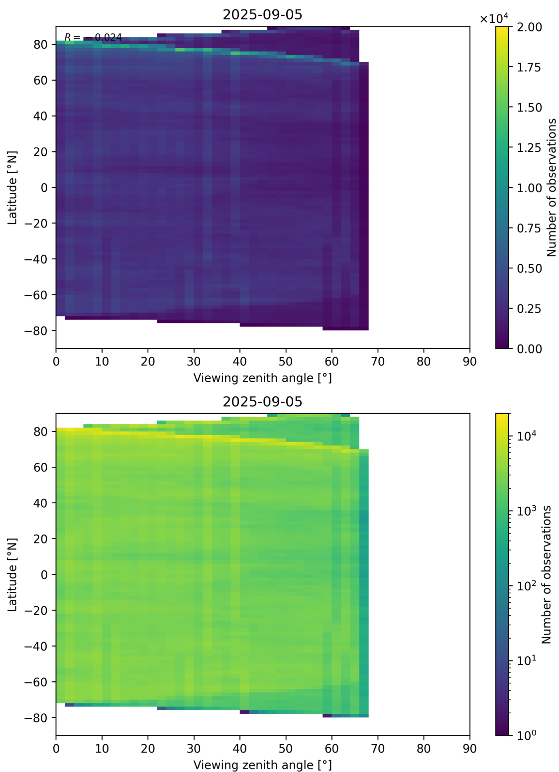
Figure 74: Scatter density plot of “Viewing zenith angle” against “Latitude” for 2025-09-04 to 2025-09-06.
