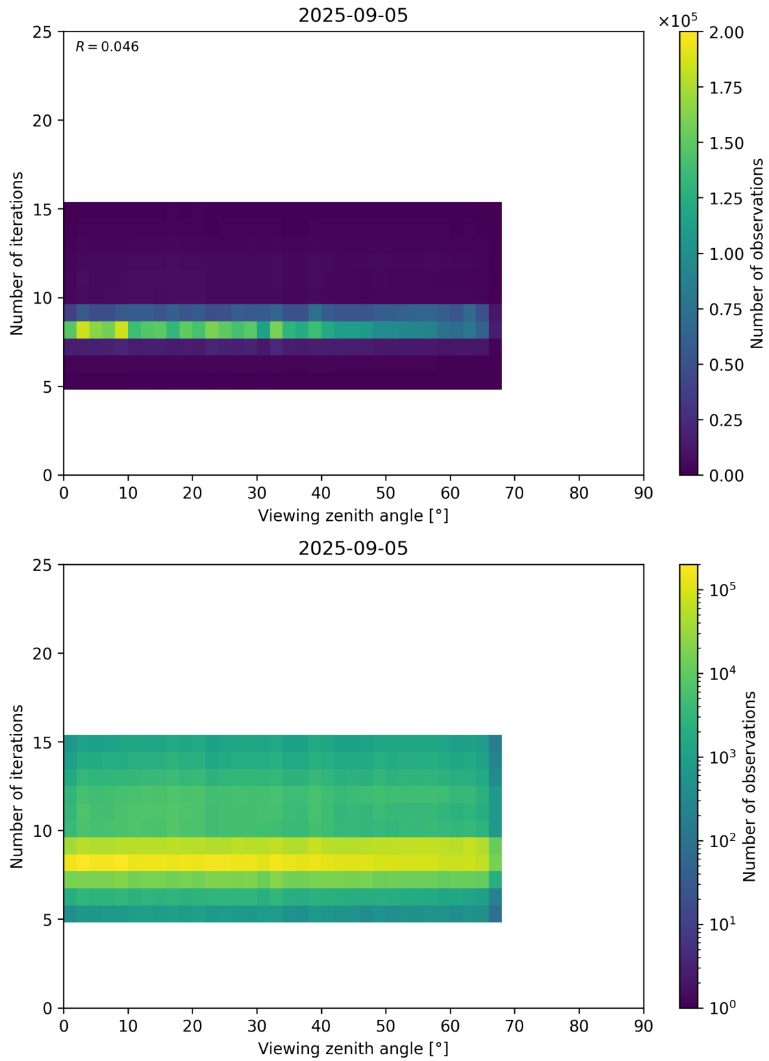
Figure 75: Scatter density plot of “Viewing zenith angle” against “Number of iterations” for 2025-09-04 to 2025-09-06.
