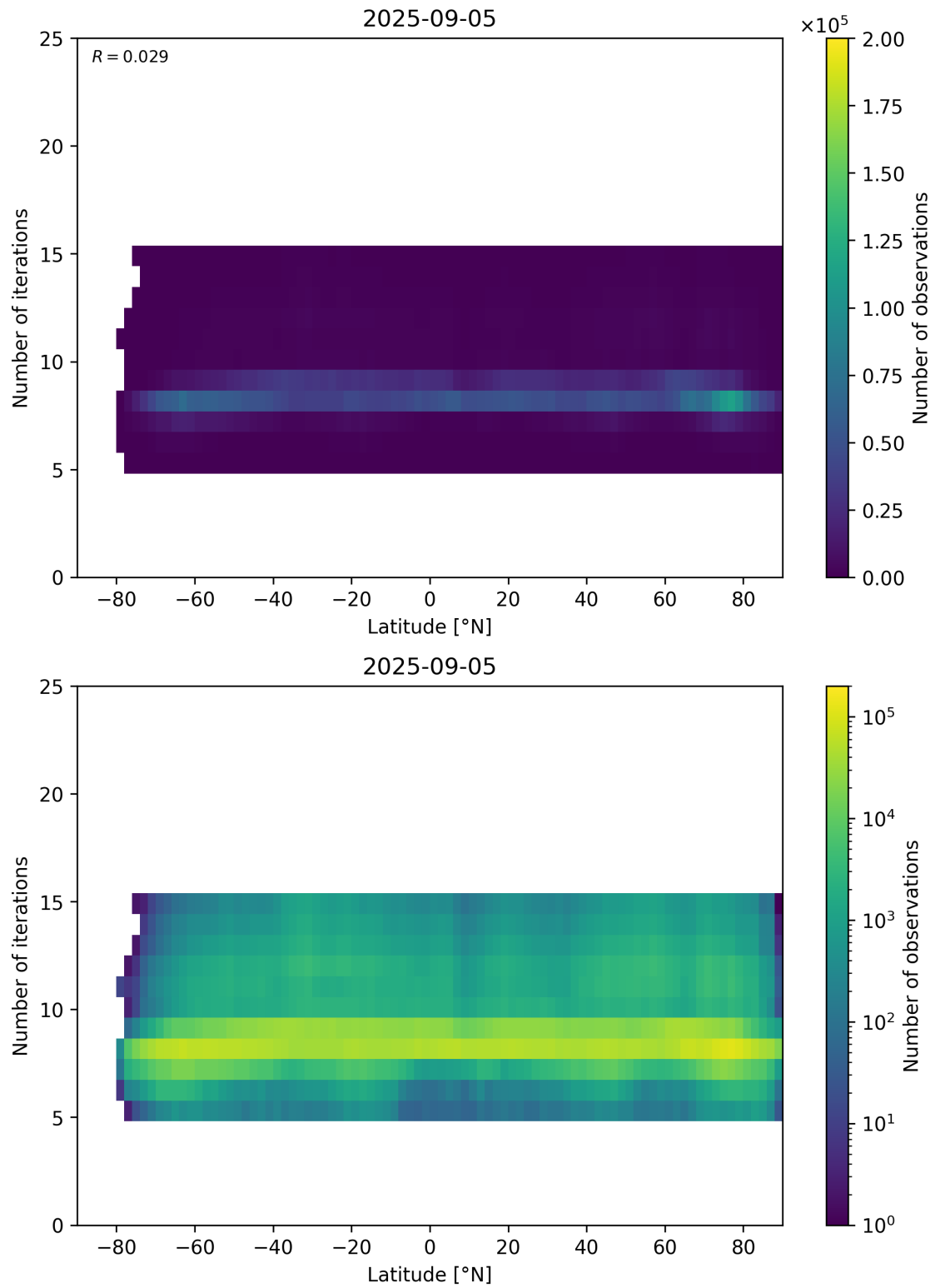
Figure 56: Scatter density plot of “Latitude” against “Number of iterations” for 2025-09-04 to 2025-09-06.
