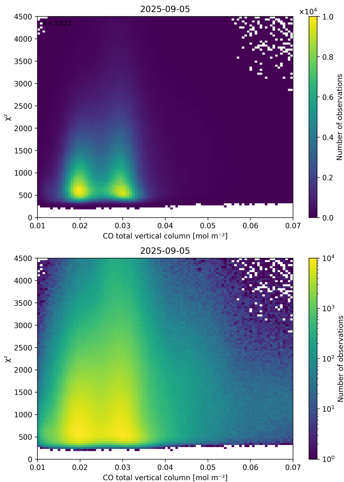
Figure 35: Scatter density plot of “CO total vertical column” against “ \chi^2 ” for 2025-09-04 to 2025-09-06.
