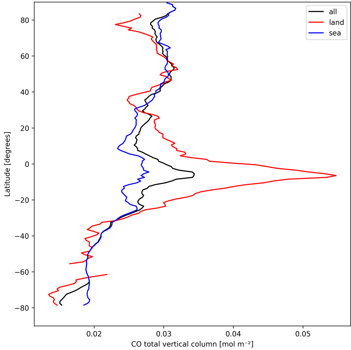
Figure 10: Zonal average of “CO total vertical column” for 2025-09-04 to 2025-09-06.
