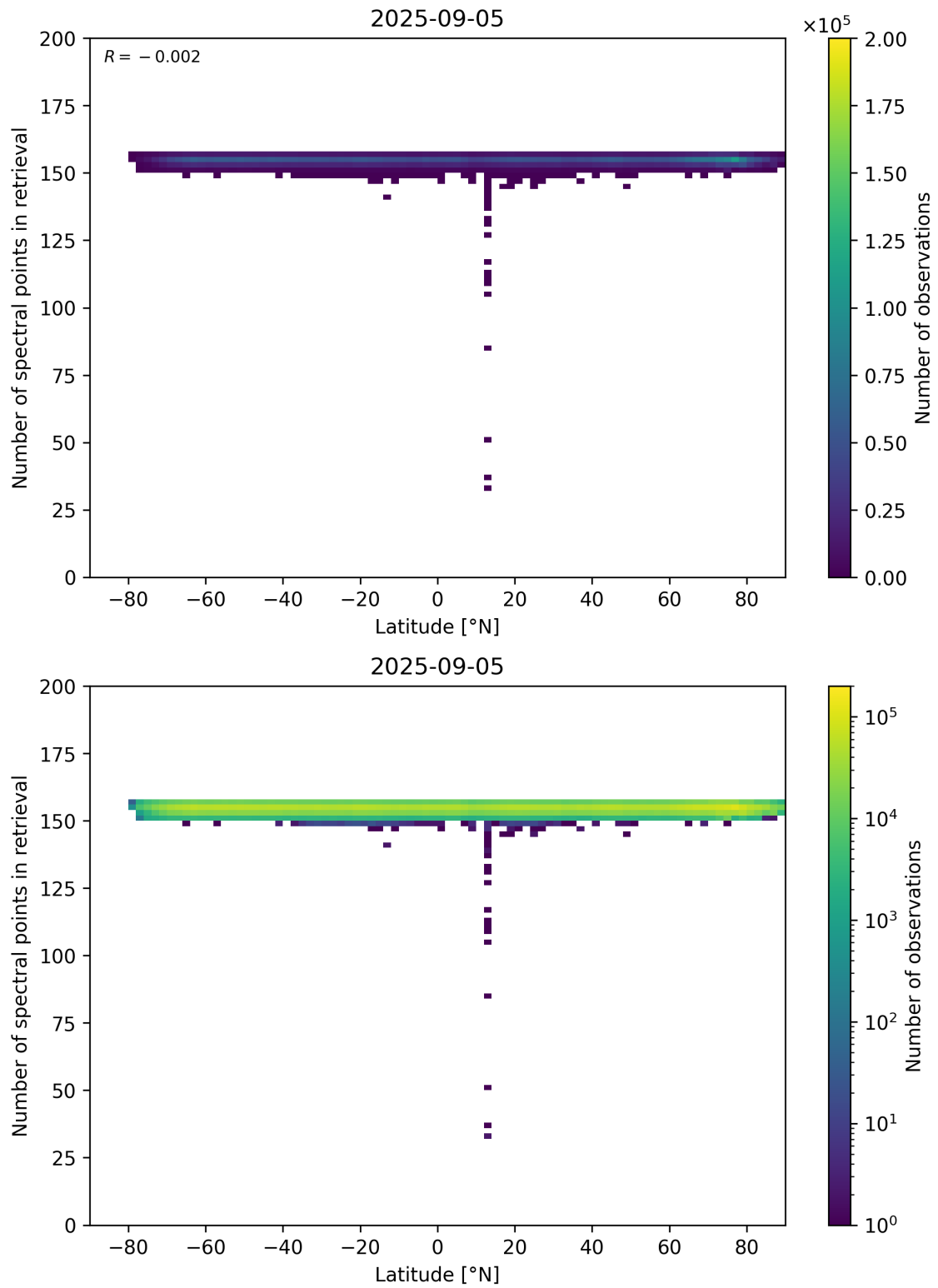
Figure 57: Scatter density plot of “Latitude” against “Number of spectral points in retrieval” for 2025-09-04 to 2025-09-06.
