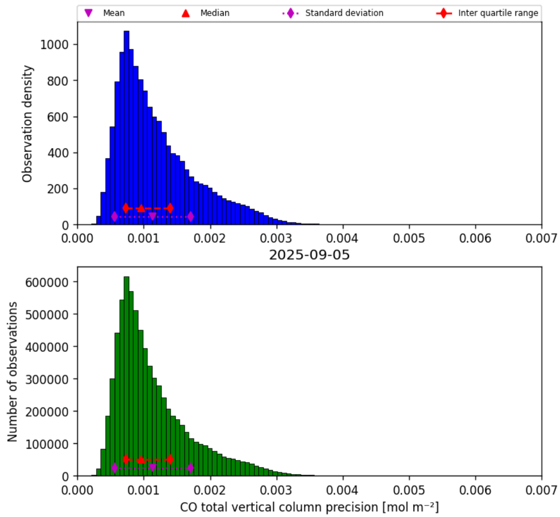
Figure 20: Histogram of “CO total vertical column precision” for 2025-09-04 to 2025-09-06
