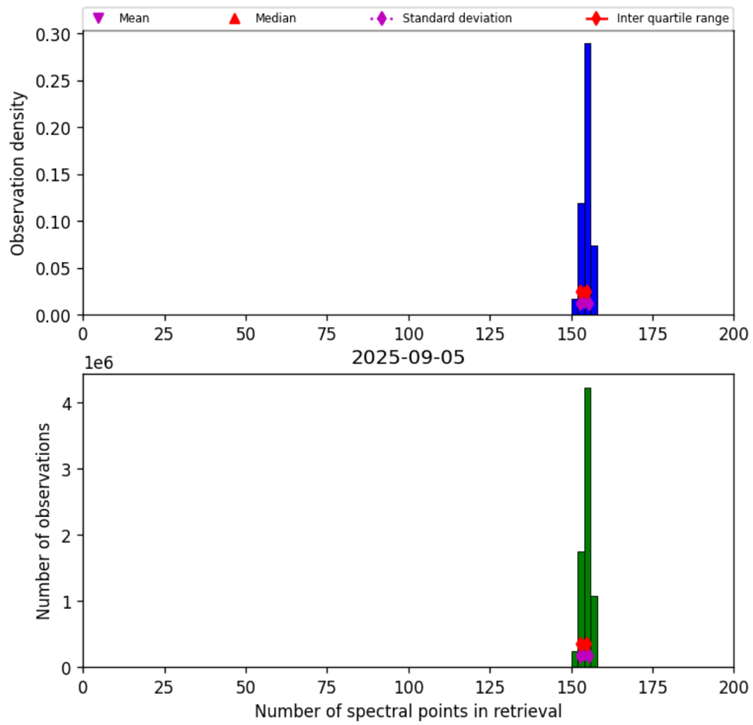
Figure 21: Histogram of “Number of spectral points in retrieval” for 2025-09-04 to 2025-09-06
