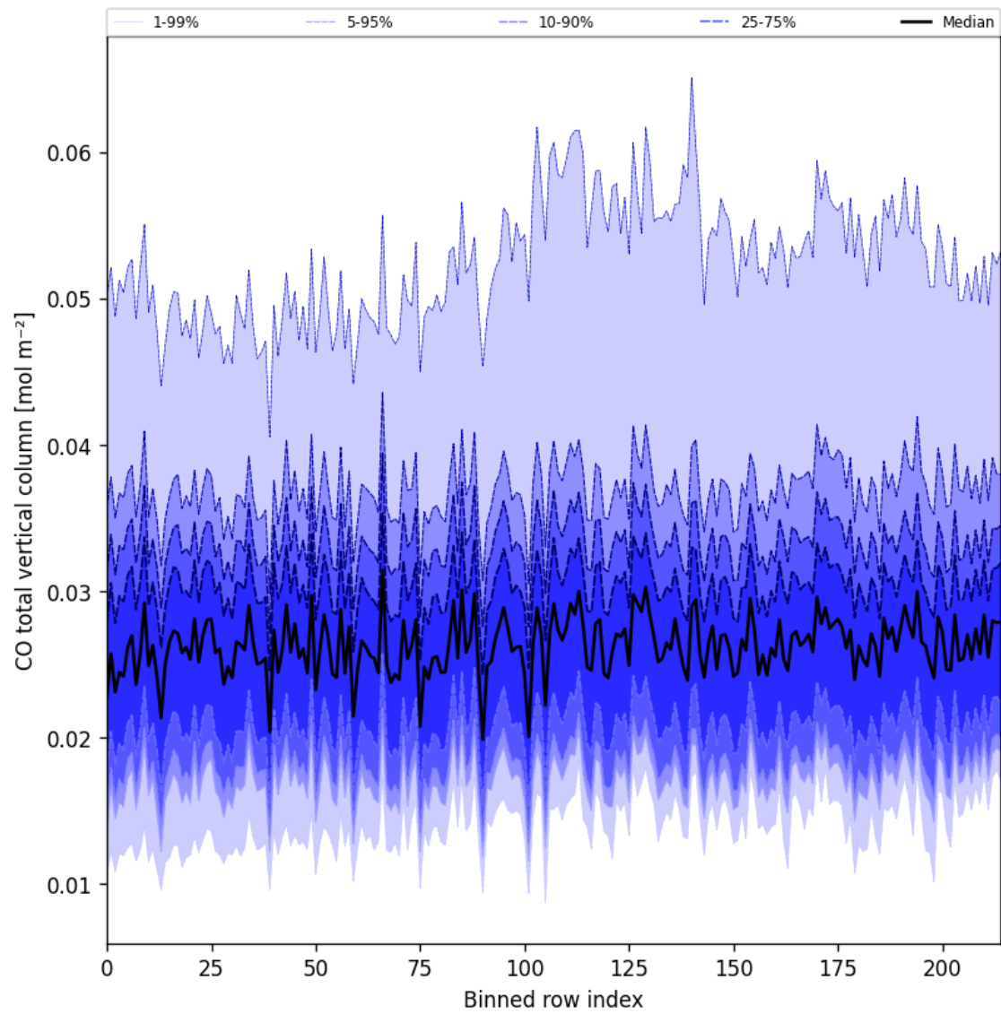
Figure 26: Along track statistics of “CO total vertical column” for 2025-09-04 to 2025-09-06
