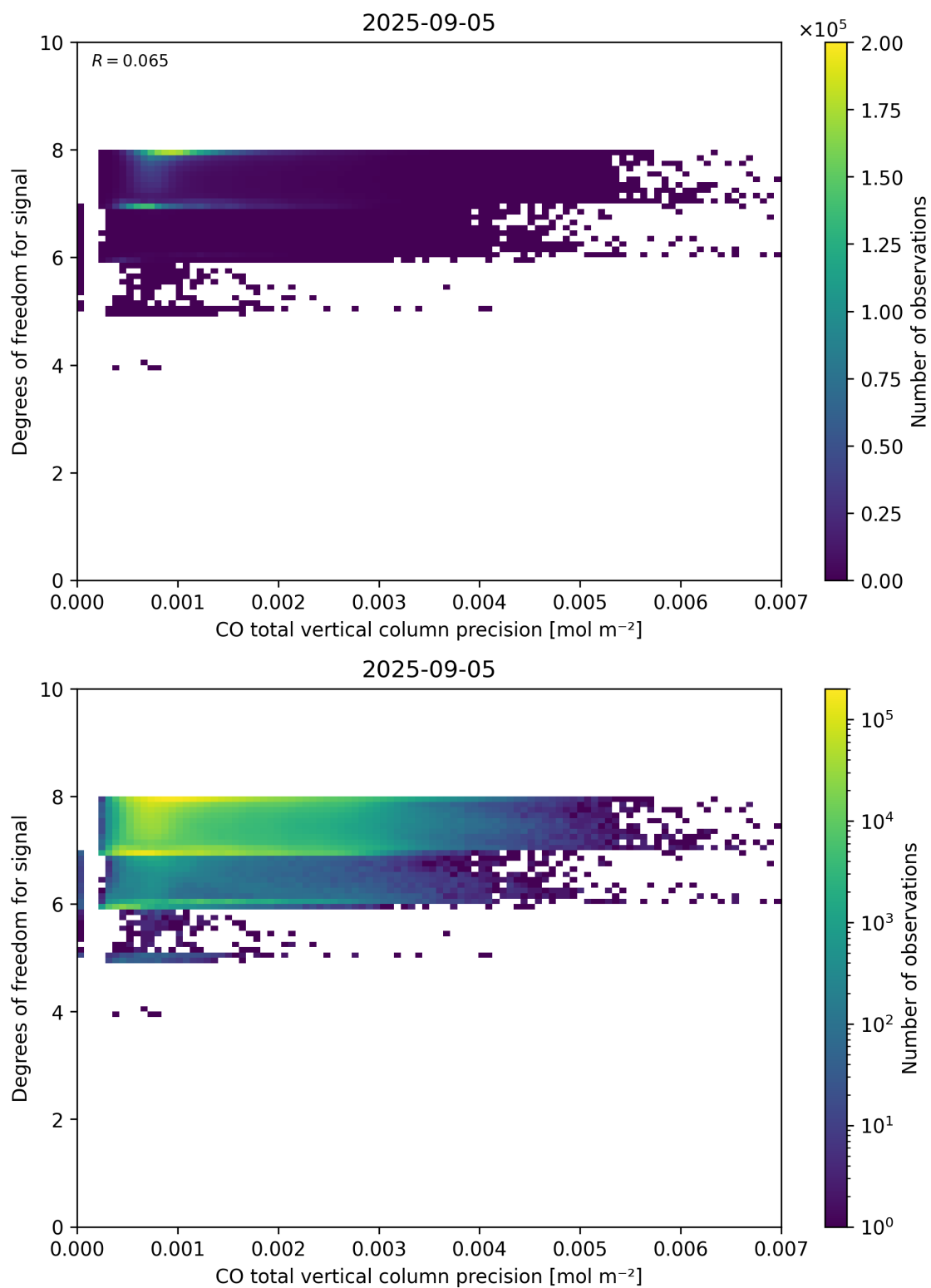
Figure 45: Scatter density plot of “CO total vertical column precision” against “Degrees of freedom for signal” for 2025-09-04 to 2025-09-06.
