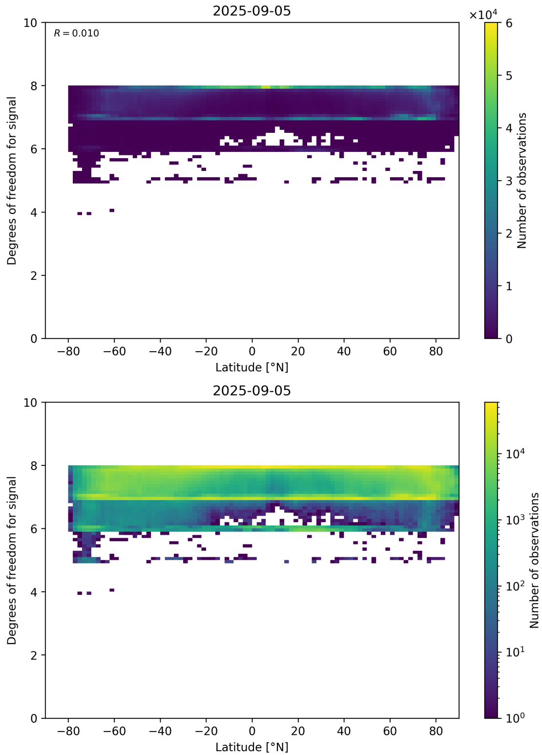
Figure 55: Scatter density plot of “Latitude” against “Degrees of freedom for signal” for 2025-09-04 to 2025-09-06.
