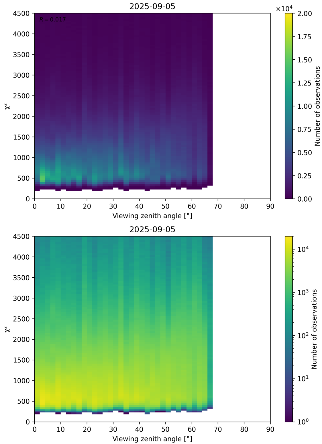
Figure 72: Scatter density plot of “Viewing zenith angle” against “ \chi^2 ” for 2025-09-04 to 2025-09-06.
