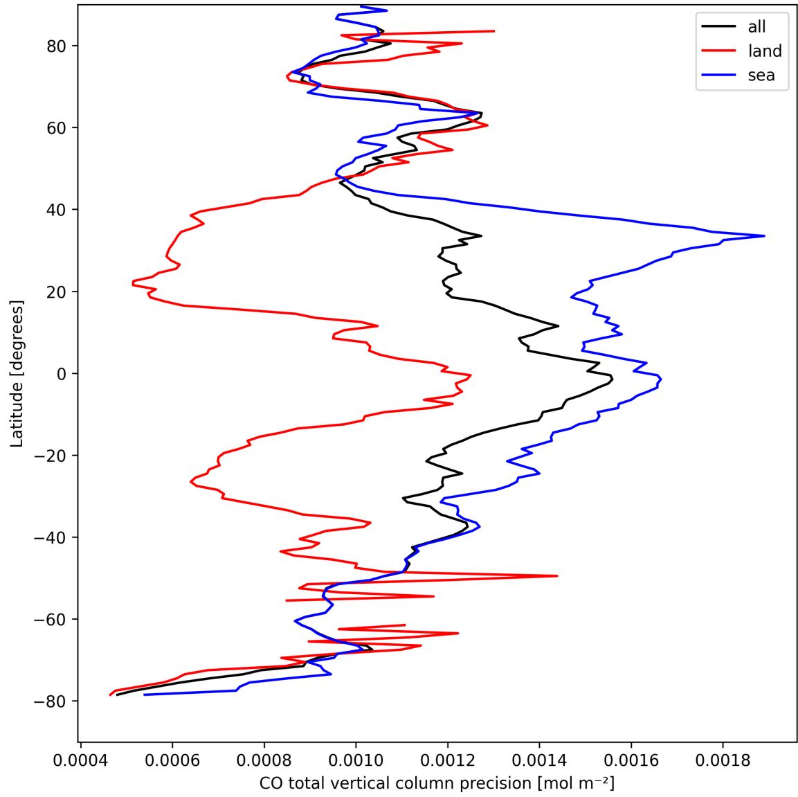
Figure 12: Zonal average of “CO total vertical column precision” for 2025-09-04 to 2025-09-06.
