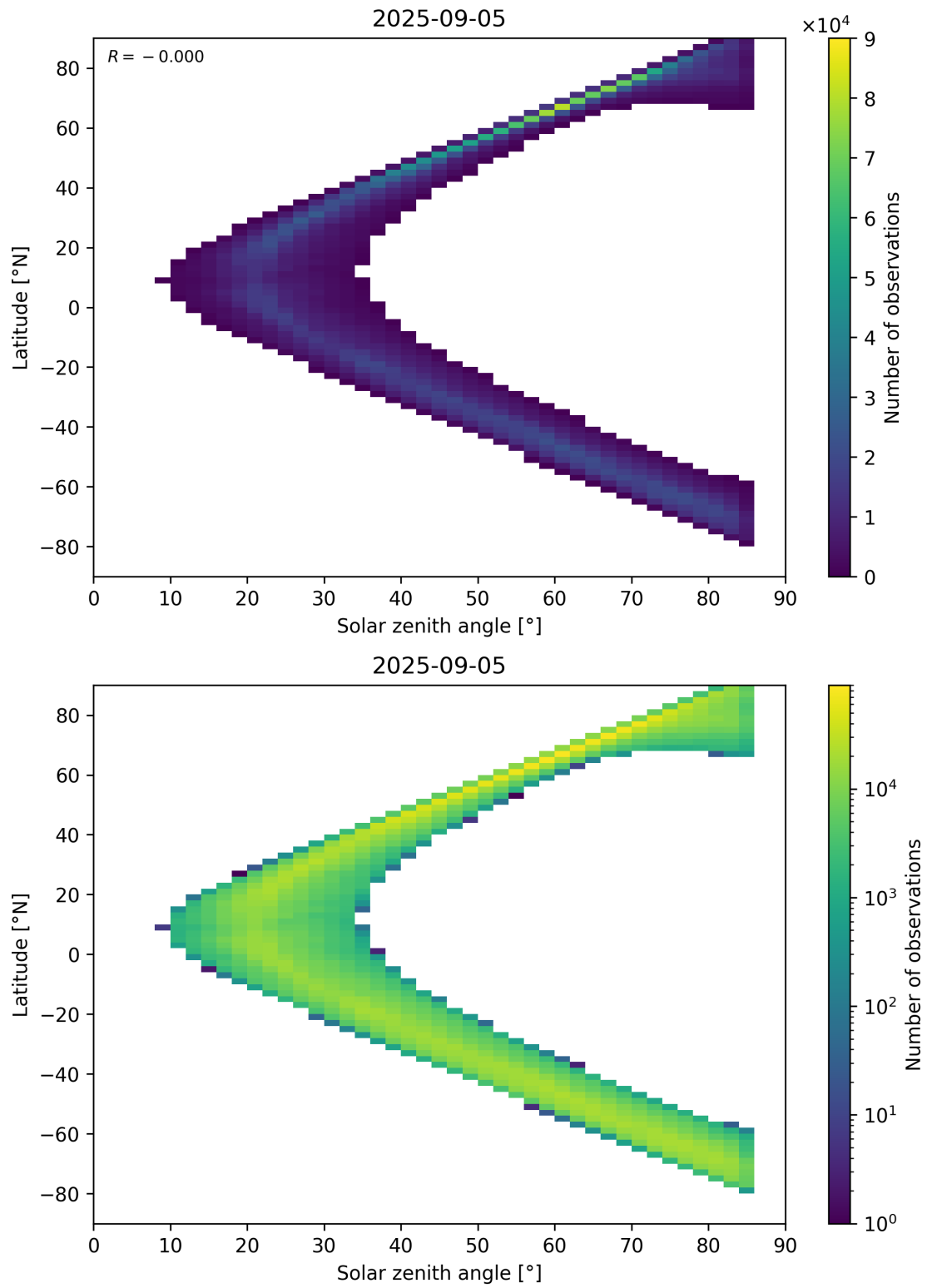
Figure 66: Scatter density plot of “Solar zenith angle” against “Latitude” for 2025-09-04 to 2025-09-06.
