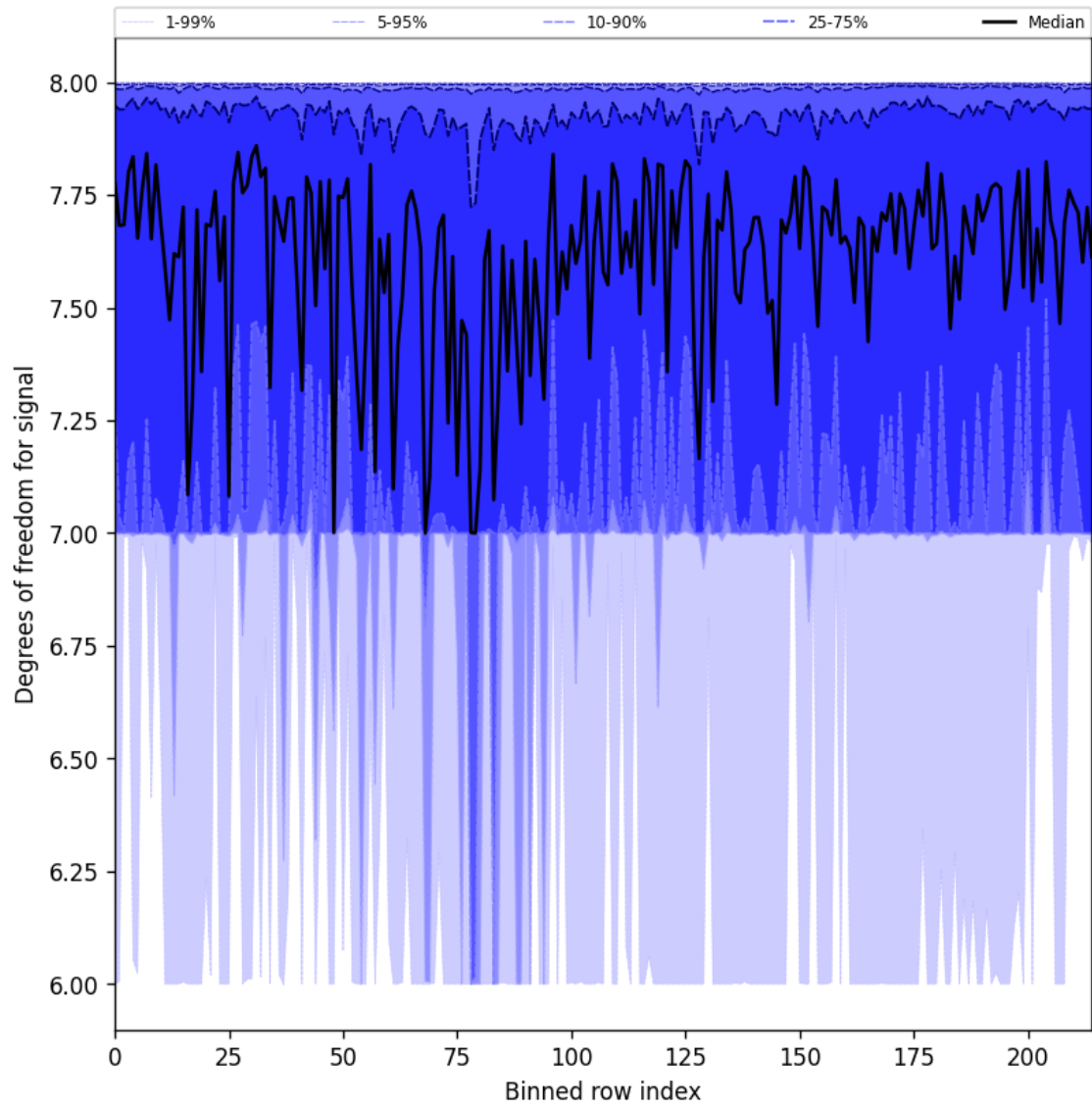
Figure 31: Along track statistics of “Degrees of freedom for signal” for 2025-09-04 to 2025-09-06
