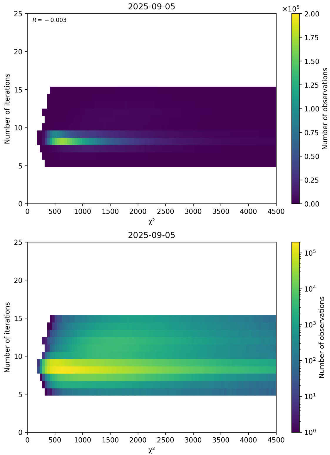
Figure 49: Scatter density plot of “ \chi^2 ” against “Number of iterations” for 2025-09-04 to 2025-09-06.
