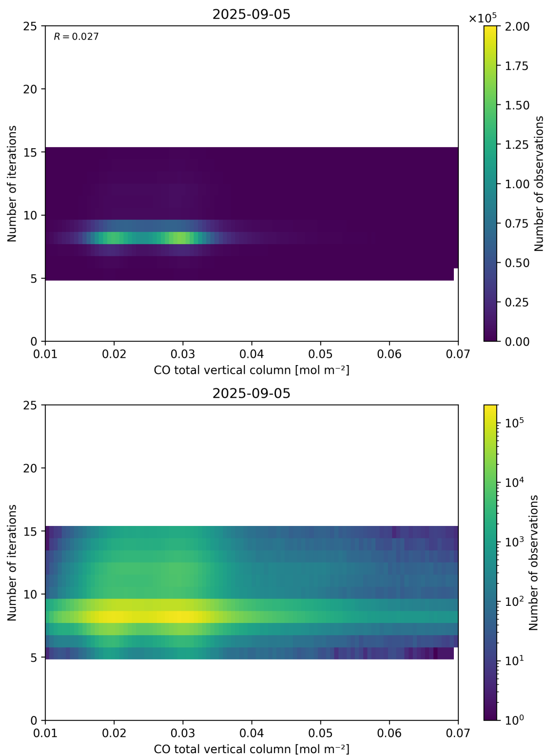
Figure 42: Scatter density plot of “CO total vertical column” against “Number of iterations” for 2025-09-04 to 2025-09-06.
