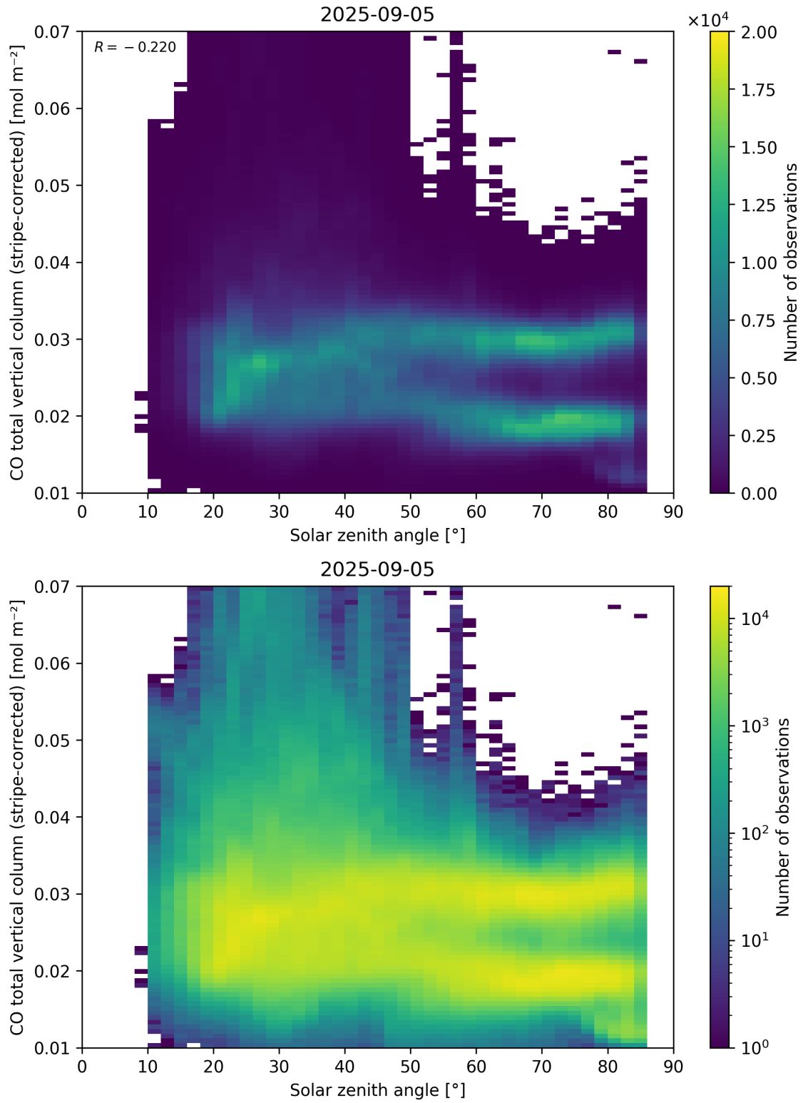
Figure 62: Scatter density plot of “Solar zenith angle” against “CO total vertical column (stripe-corrected)” for 2025-09-04 to 2025-09-06.
