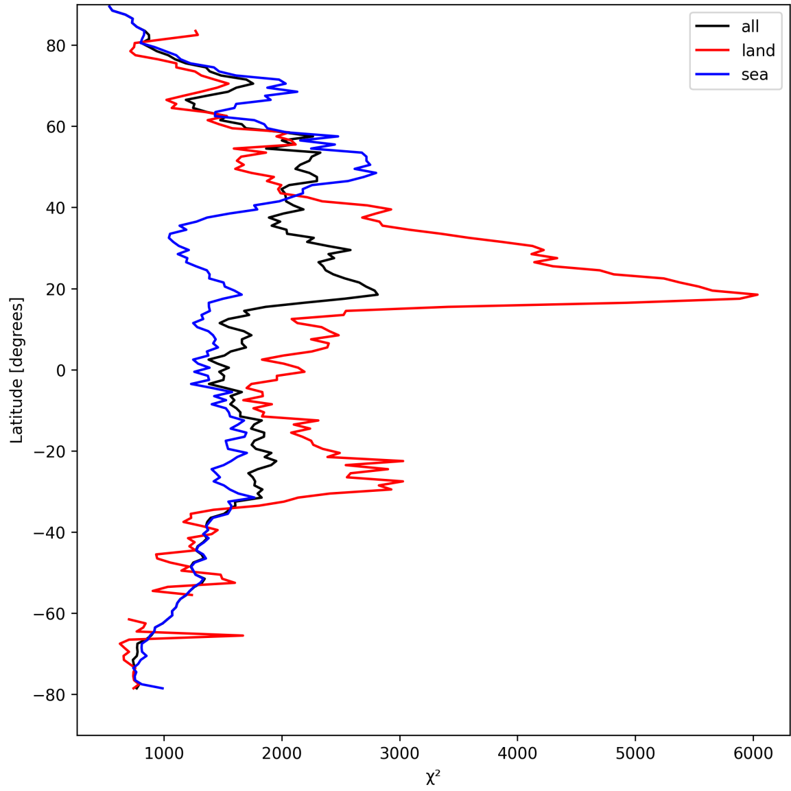
Figure 14: Zonal average of “ \chi^2 ” for 2025-09-04 to 2025-09-06.
