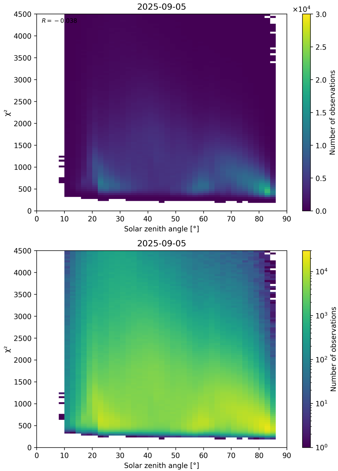
Figure 64: Scatter density plot of “Solar zenith angle” against “ \chi^2 ” for 2025-09-04 to 2025-09-06.
