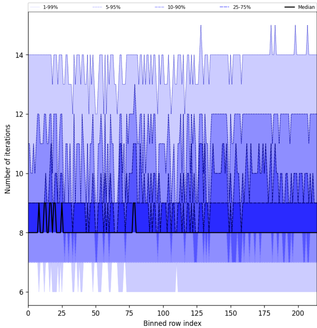
Figure 32: Along track statistics of “Number of iterations” for 2025-09-04 to 2025-09-06
