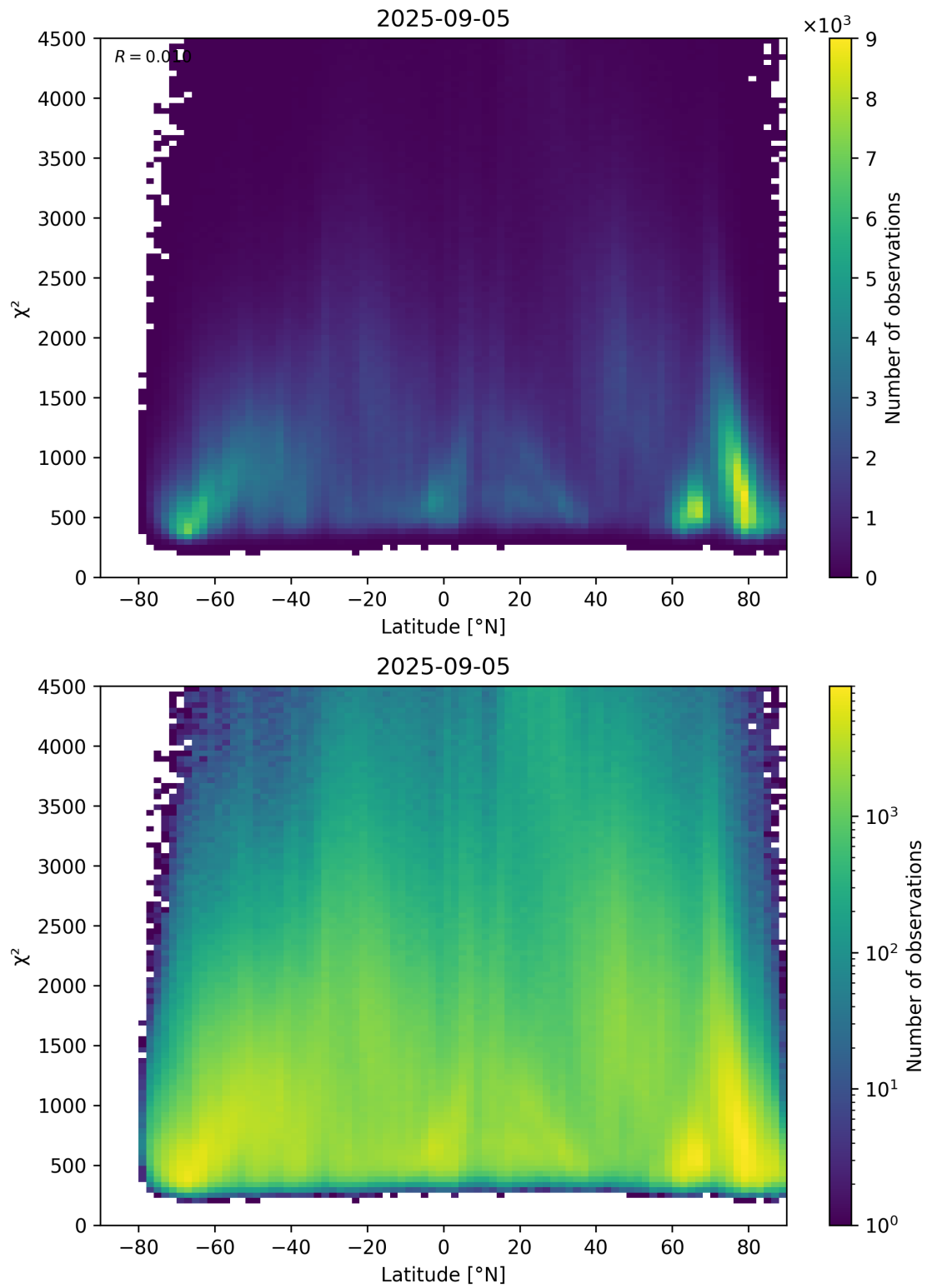
Figure 54: Scatter density plot of “Latitude” against “ \chi^2 ” for 2025-09-04 to 2025-09-06.
