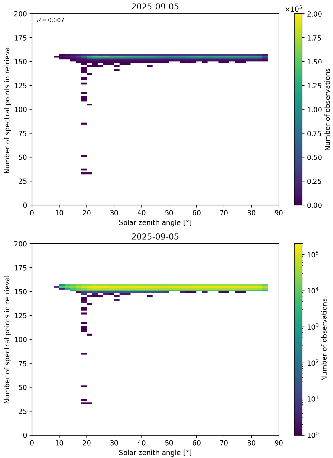
Figure 68: Scatter density plot of “Solar zenith angle” against “Number of spectral points in retrieval” for 2025-09-04 to 2025-09-06.
