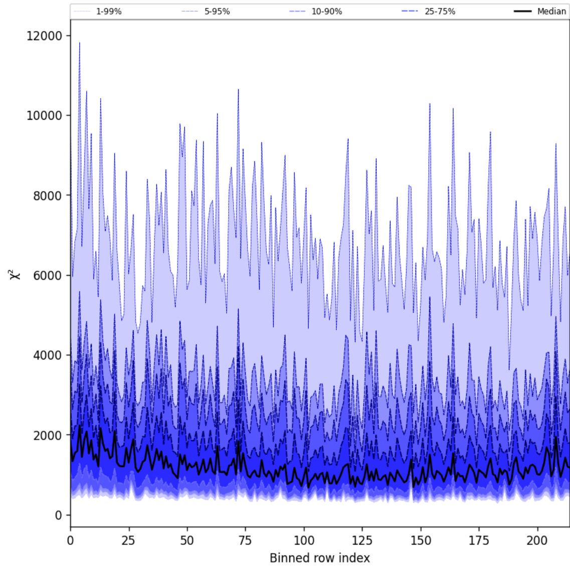
Figure 30: Along track statistics of “ \chi^2 ” for 2025-09-04 to 2025-09-06
