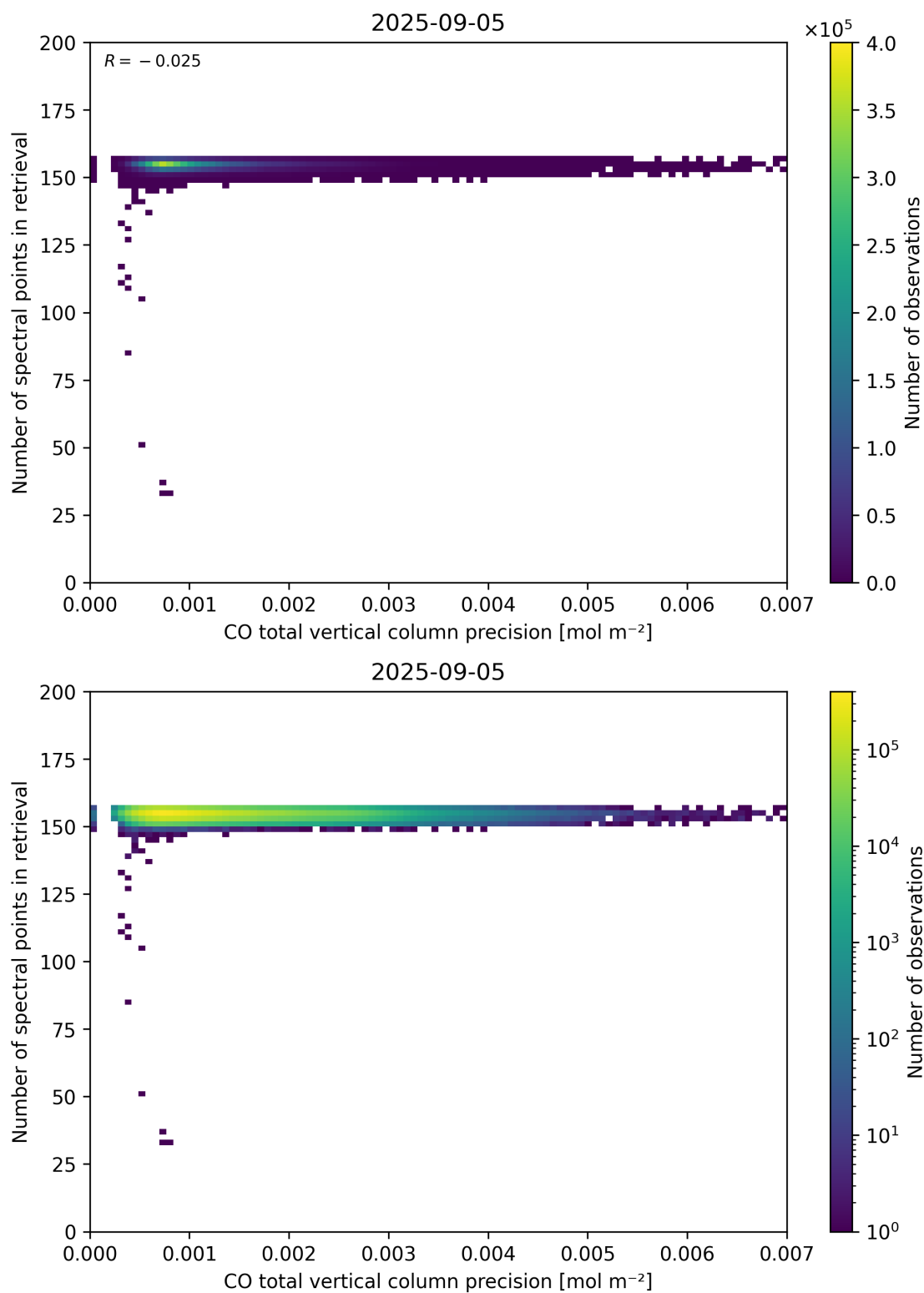
Figure 47: Scatter density plot of “CO total vertical column precision” against “Number of spectral points in retrieval” for 2025-09-04 to 2025-09-06.
