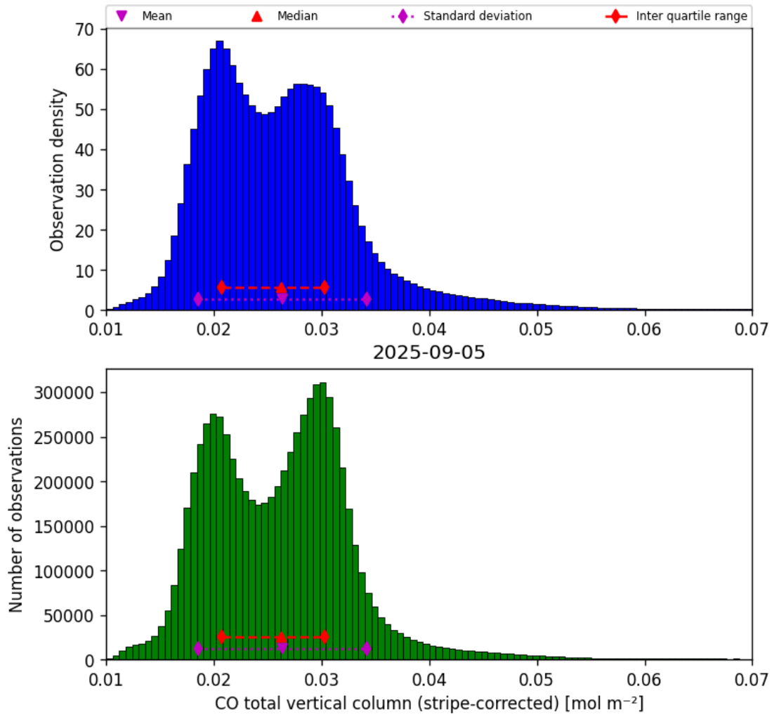
Figure 19: Histogram of “CO total vertical column (stripe-corrected)” for 2025-09-04 to 2025-09-06
