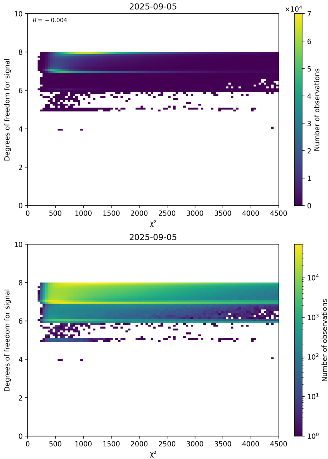
Figure 48: Scatter density plot of “ \chi^2 ” against “Degrees of freedom for signal” for 2025-09-04 to 2025-09-06.
