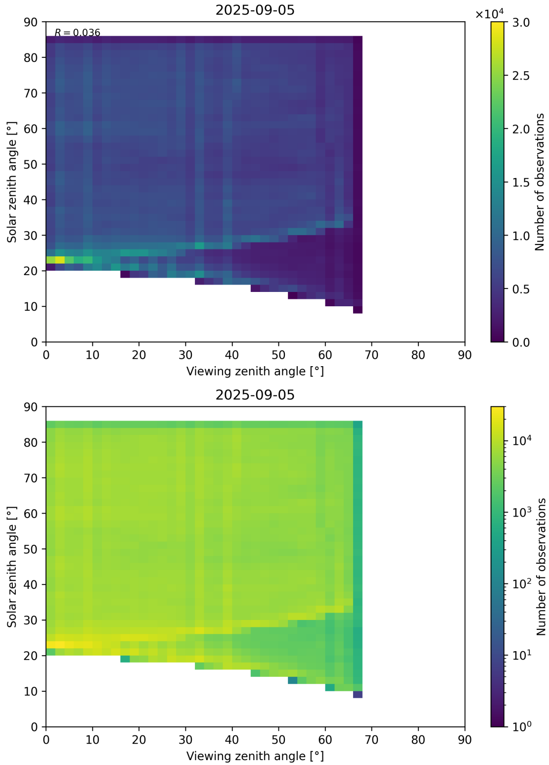
Figure 77: Scatter density plot of “Viewing zenith angle” against “Solar zenith angle” for 2025-09-04 to 2025-09-06.
