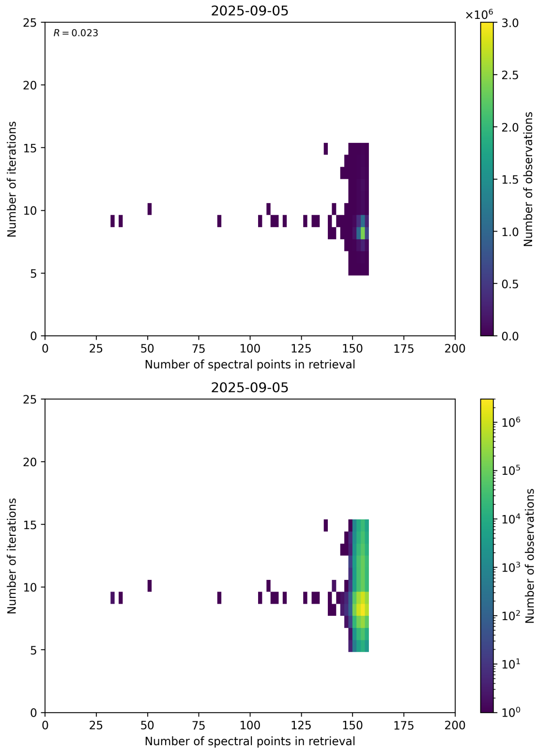
Figure 60: Scatter density plot of “Number of spectral points in retrieval” against “Number of iterations” for 2025-09-04 to 2025-09-06.
