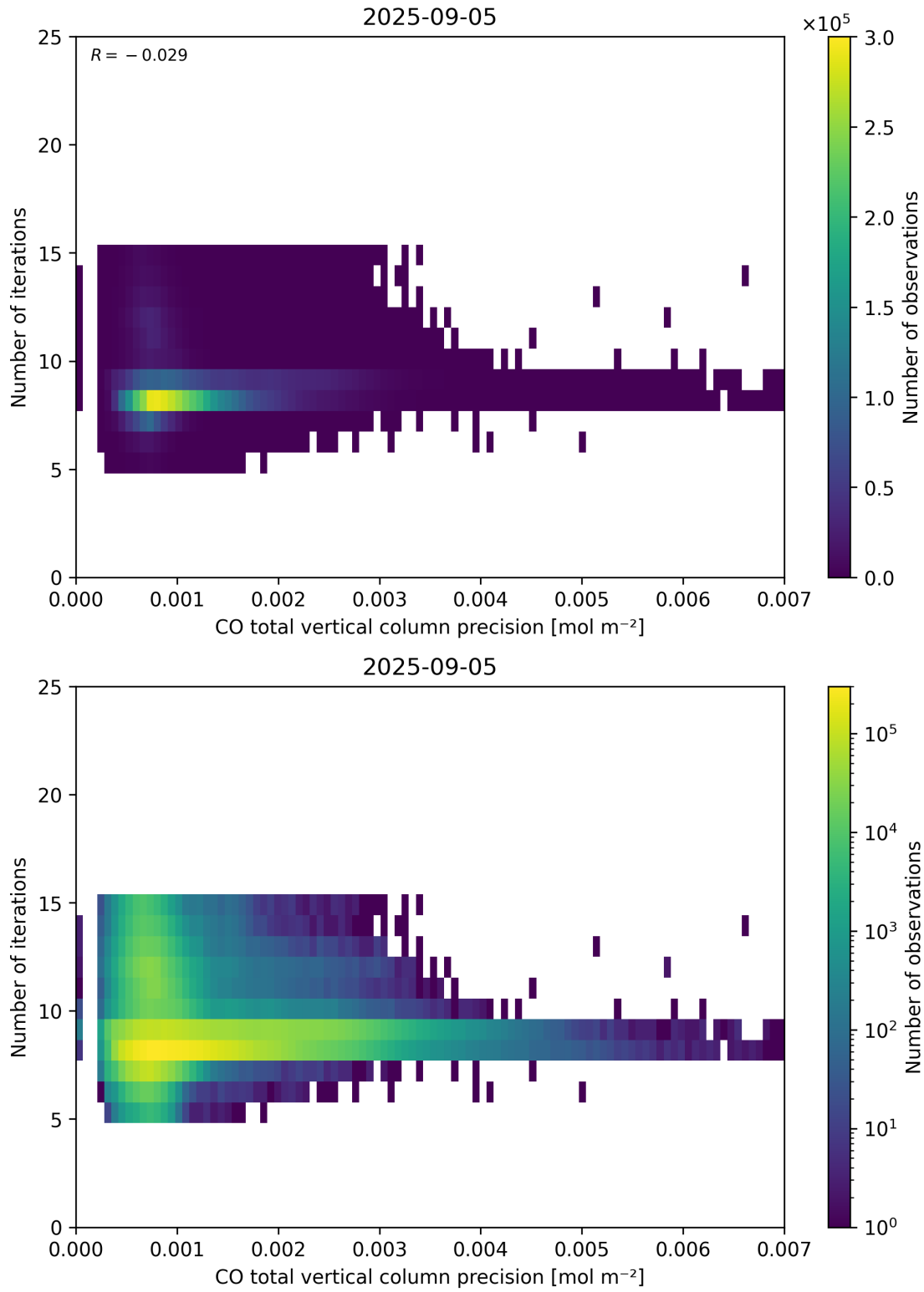
Figure 46: Scatter density plot of “CO total vertical column precision” against “Number of iterations” for 2025-09-04 to 2025-09-06.
