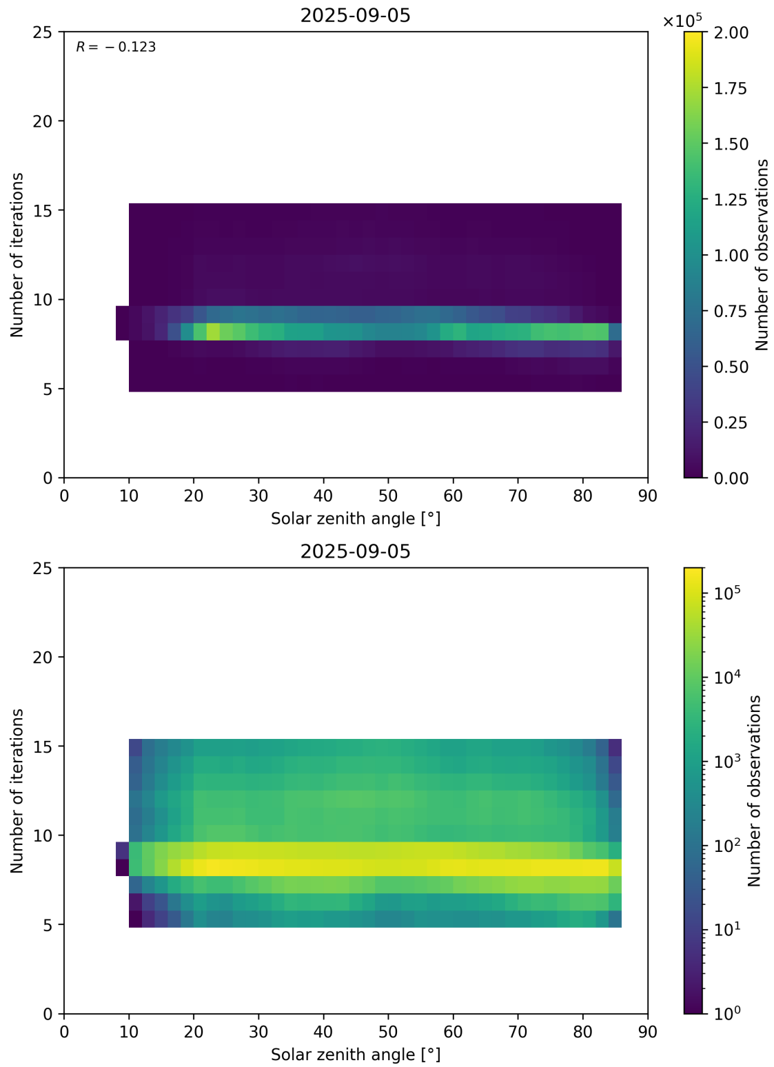
Figure 67: Scatter density plot of “Solar zenith angle” against “Number of iterations” for 2025-09-04 to 2025-09-06.
