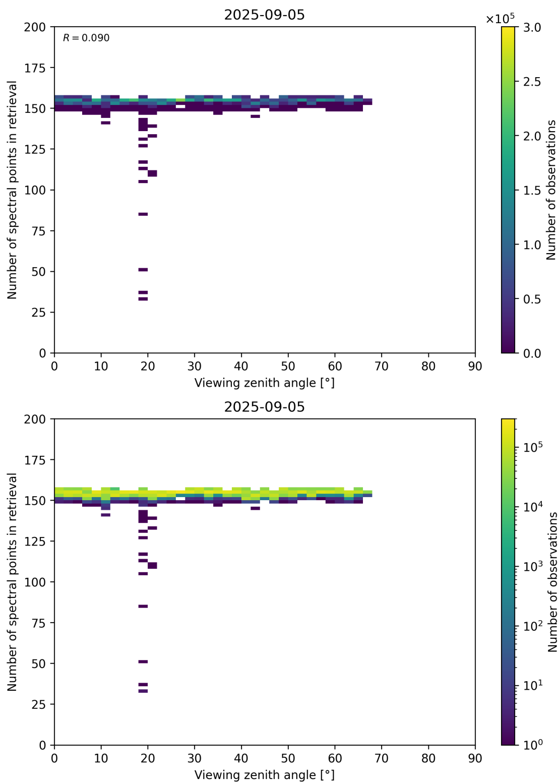
Figure 76: Scatter density plot of “Viewing zenith angle” against “Number of spectral points in retrieval” for 2025-09-04 to 2025-09-06.
