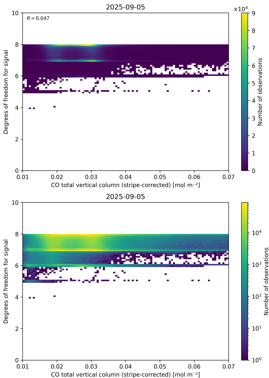
Figure 38: Scatter density plot of “CO total vertical column (stripe-corrected)” against “Degrees of freedom for signal” for 2025-09-04 to 2025-09-06.
