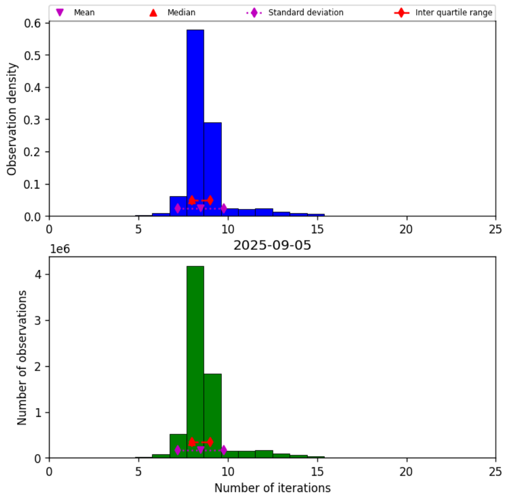
Figure 24: Histogram of “Number of iterations” for 2025-09-04 to 2025-09-06
