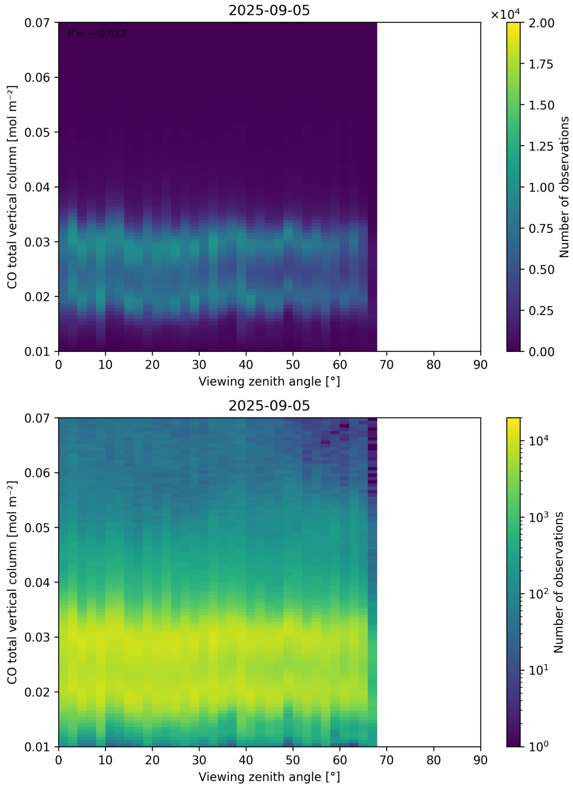
Figure 69: Scatter density plot of “Viewing zenith angle” against “CO total vertical column” for 2025-09-04 to 2025-09-06.
