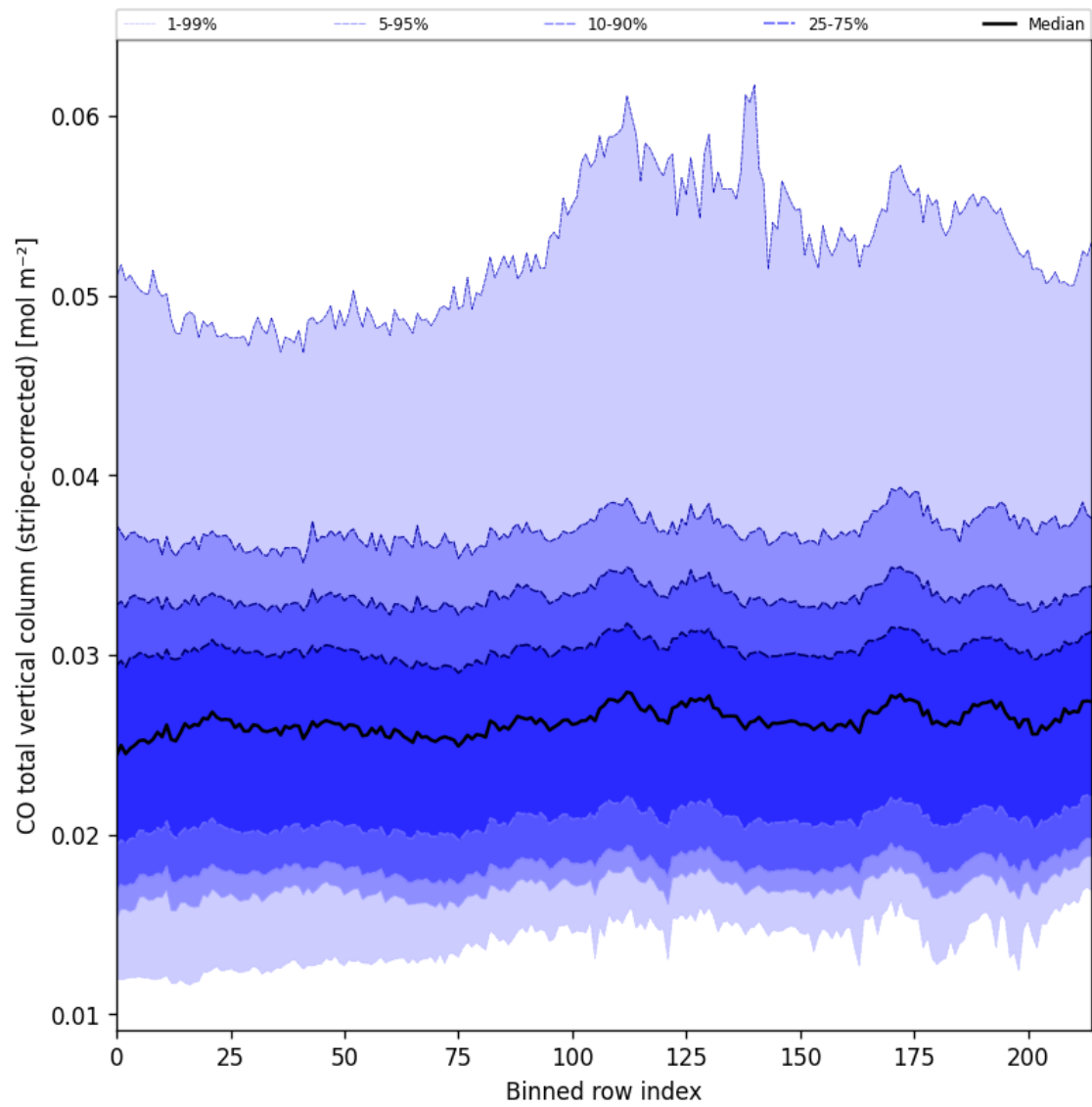
Figure 27: Along track statistics of “CO total vertical column (stripe-corrected)” for 2025-09-04 to 2025-09-06
