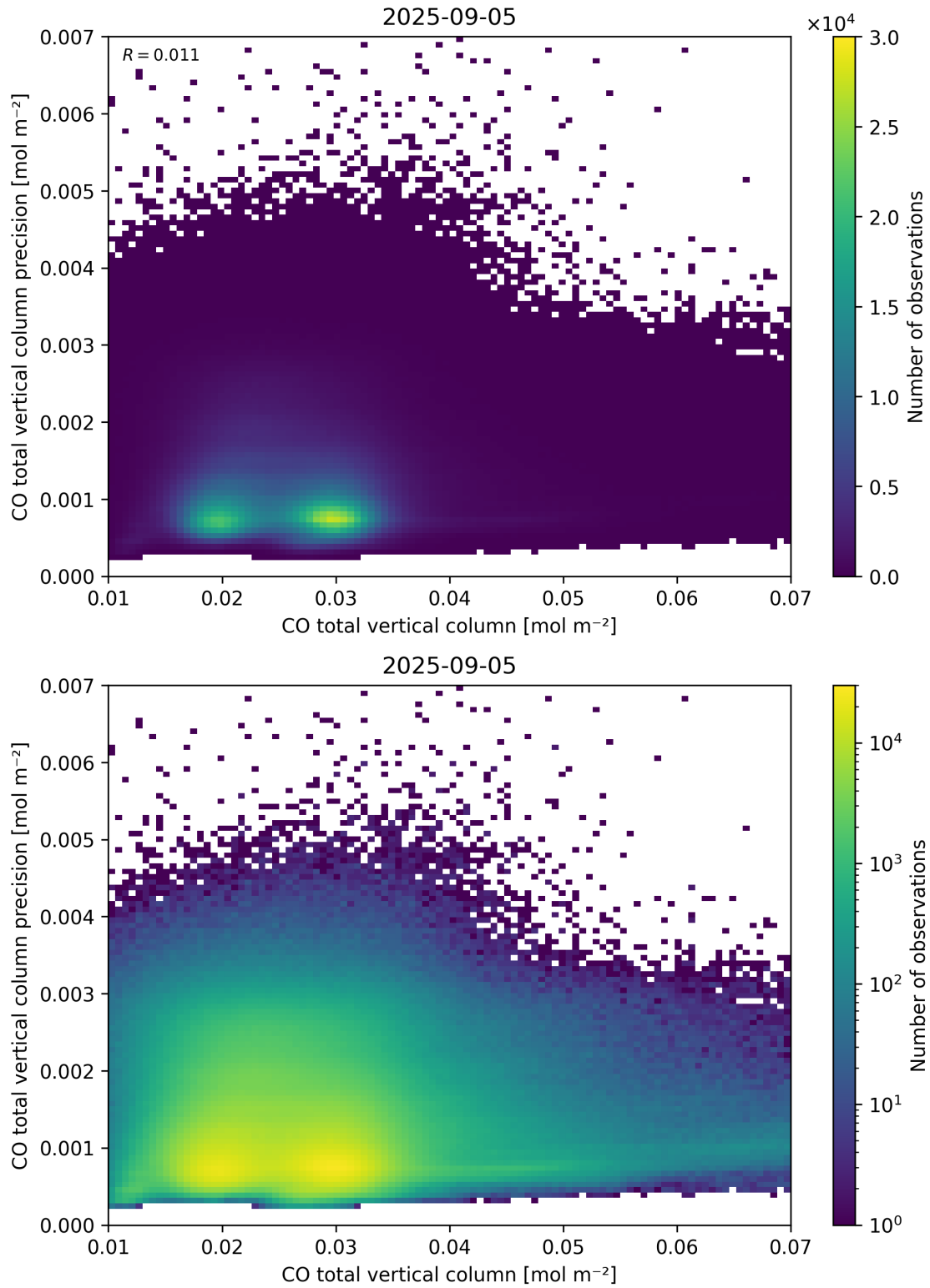
Figure 34: Scatter density plot of “CO total vertical column” against “CO total vertical column precision” for 2025-09-04 to 2025-09-06.
