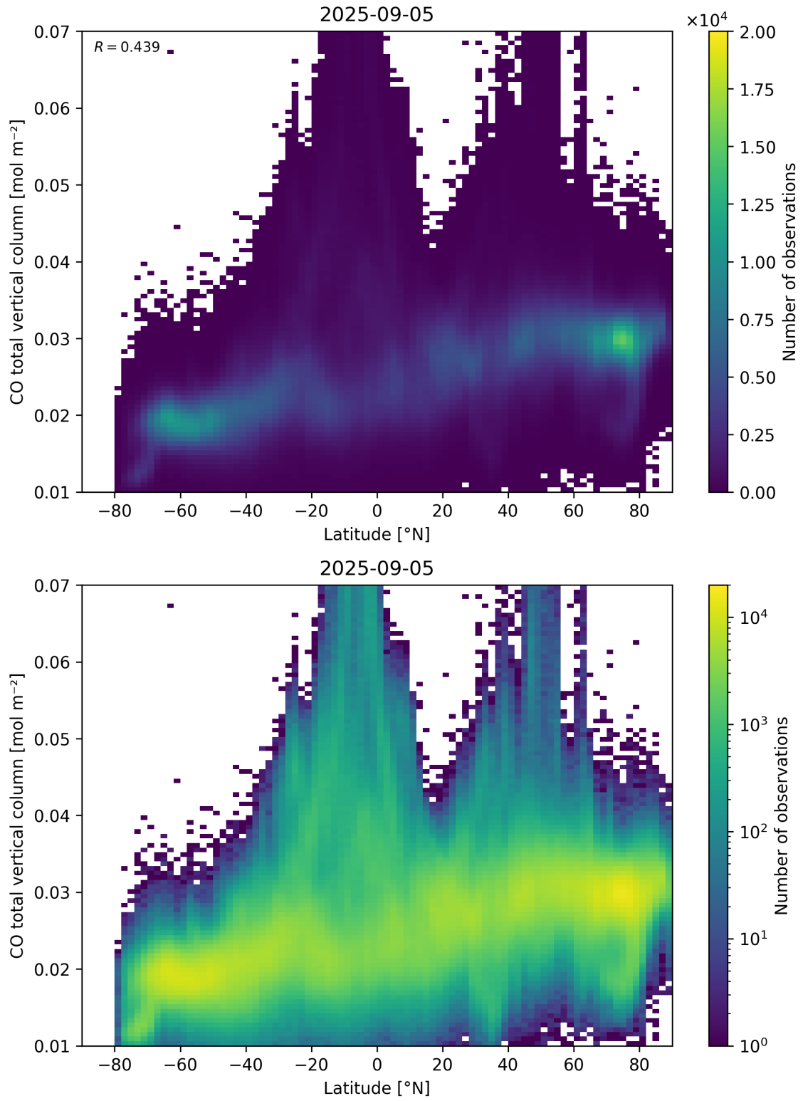
Figure 51: Scatter density plot of “Latitude” against “CO total vertical column” for 2025-09-04 to 2025-09-06.
