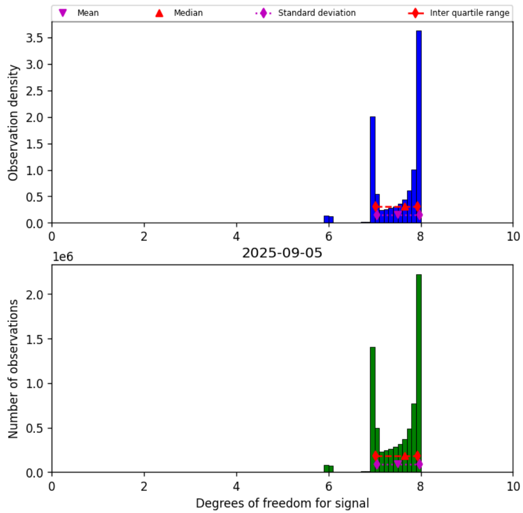
Figure 23: Histogram of “Degrees of freedom for signal” for 2025-09-04 to 2025-09-06
