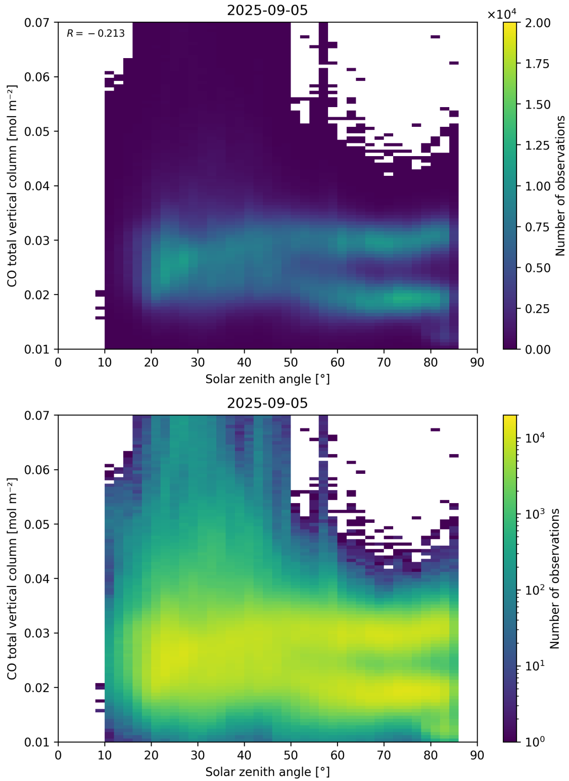
Figure 61: Scatter density plot of “Solar zenith angle” against “CO total vertical column” for 2025-09-04 to 2025-09-06.
