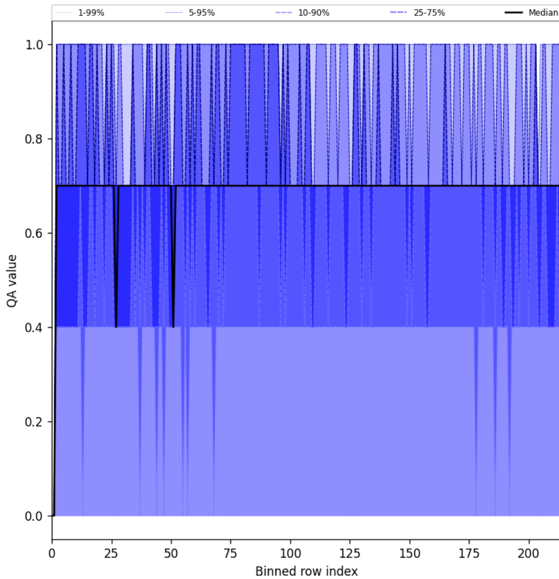
Figure 25: Along track statistics of “QA value” for 2025-09-04 to 2025-09-06
