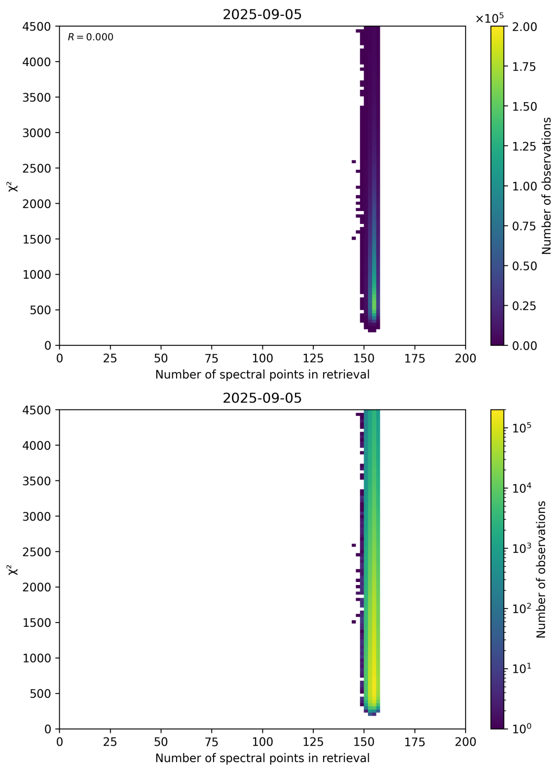
Figure 58: Scatter density plot of “Number of spectral points in retrieval” against “ \chi^2 ” for 2025-09-04 to 2025-09-06.
