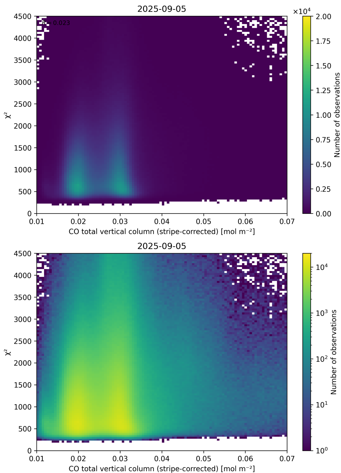
Figure 37: Scatter density plot of “CO total vertical column (stripe-corrected)” against “ \chi^2 ” for 2025-09-04 to 2025-09-06.
