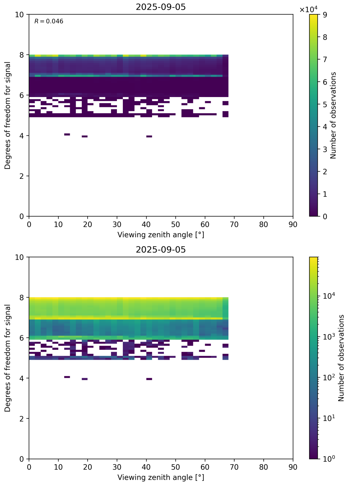
Figure 73: Scatter density plot of “Viewing zenith angle” against “Degrees of freedom for signal” for 2025-09-04 to 2025-09-06.
