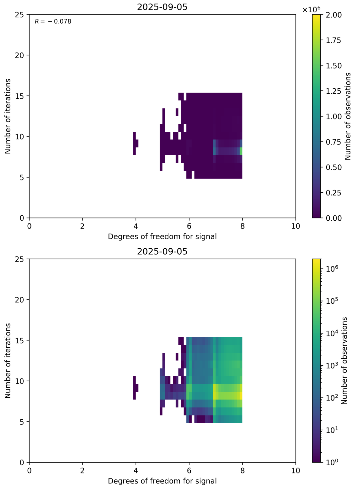
Figure 50: Scatter density plot of “Degrees of freedom for signal” against “Number of iterations” for 2025-09-04 to 2025-09-06.
