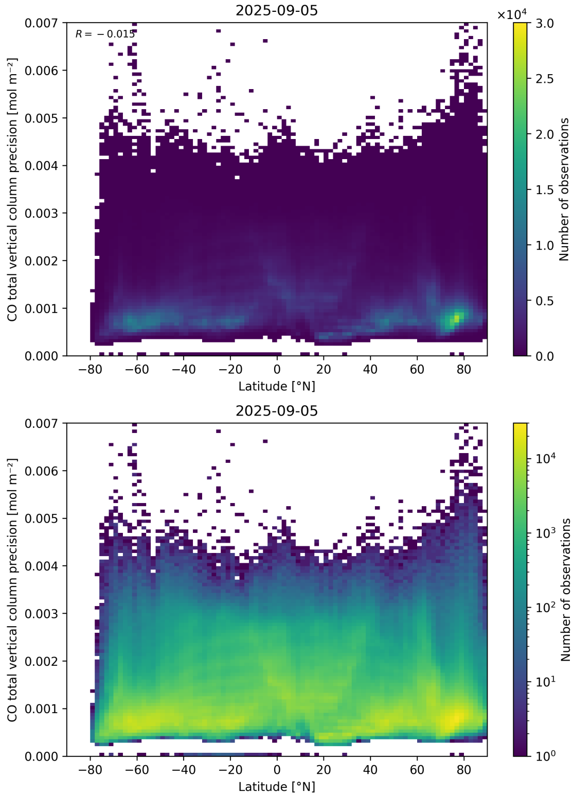
Figure 53: Scatter density plot of “Latitude” against “CO total vertical column precision” for 2025-09-04 to 2025-09-06.
