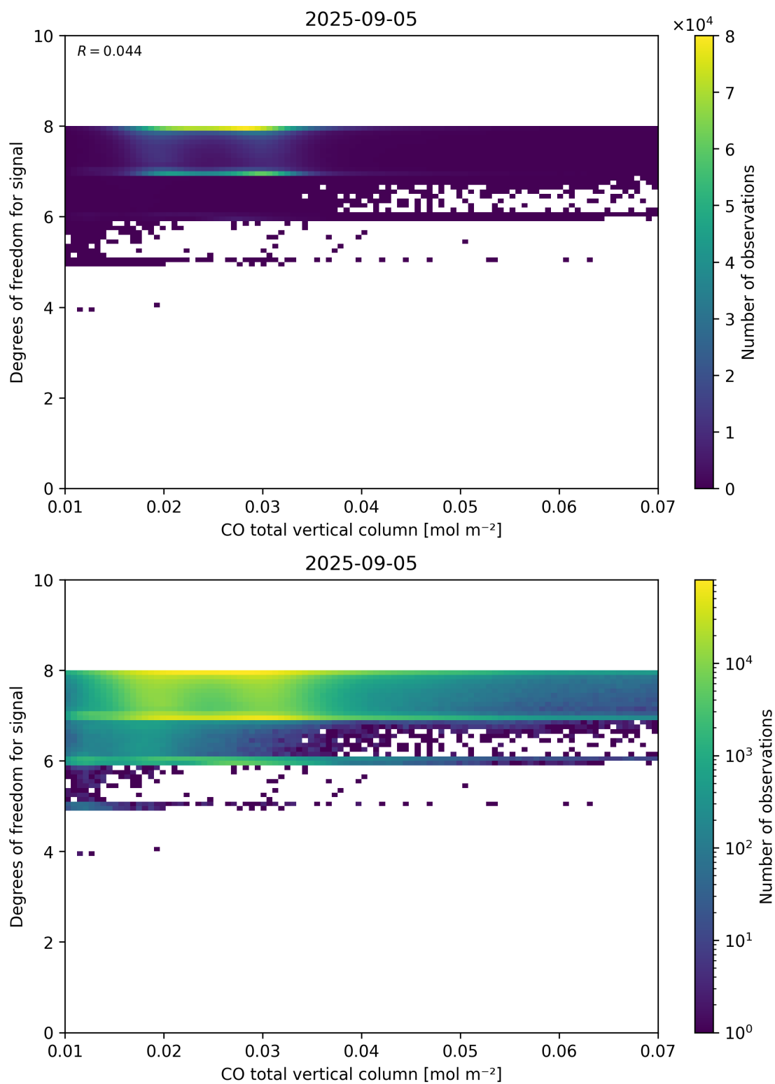
Figure 41: Scatter density plot of “CO total vertical column” against “Degrees of freedom for signal” for 2025-09-04 to 2025-09-06.
