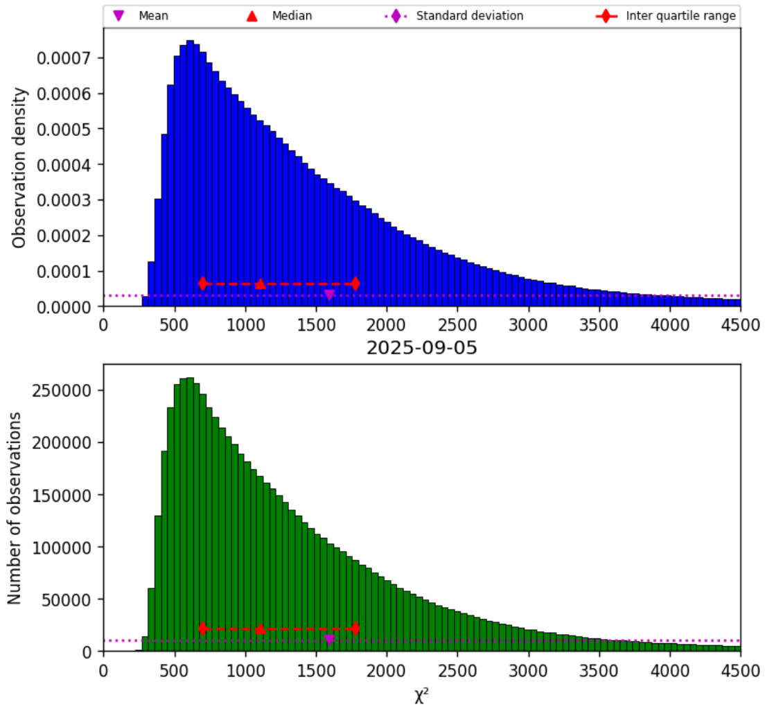
Figure 22: Histogram of “ \chi^2 ” for 2025-09-04 to 2025-09-06
