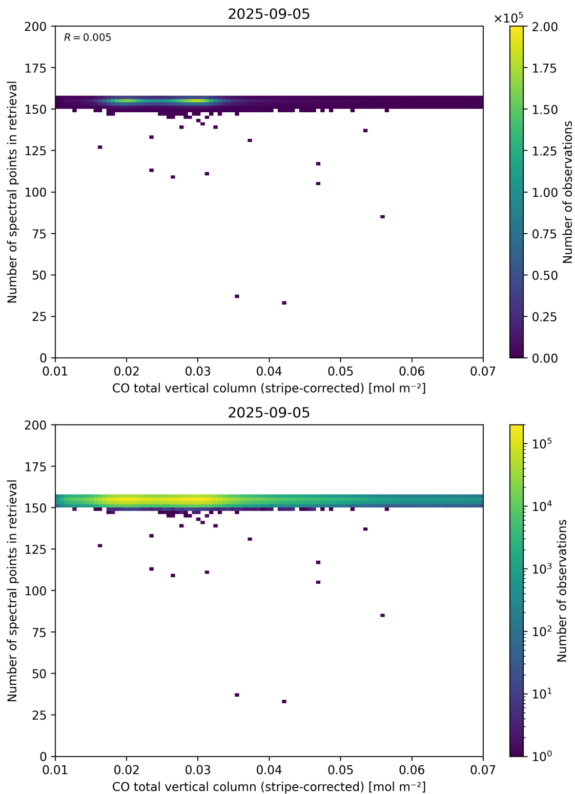
Figure 40: Scatter density plot of “CO total vertical column (stripe-corrected)” against “Number of spectral points in retrieval” for 2025-09-04 to 2025-09-06.
