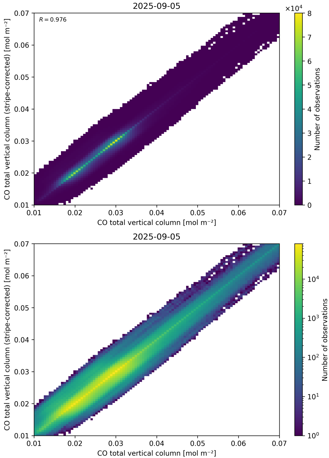
Figure 33: Scatter density plot of “CO total vertical column” against “CO total vertical column (stripe-corrected)” for 2025-09-04 to 2025-09-06.
