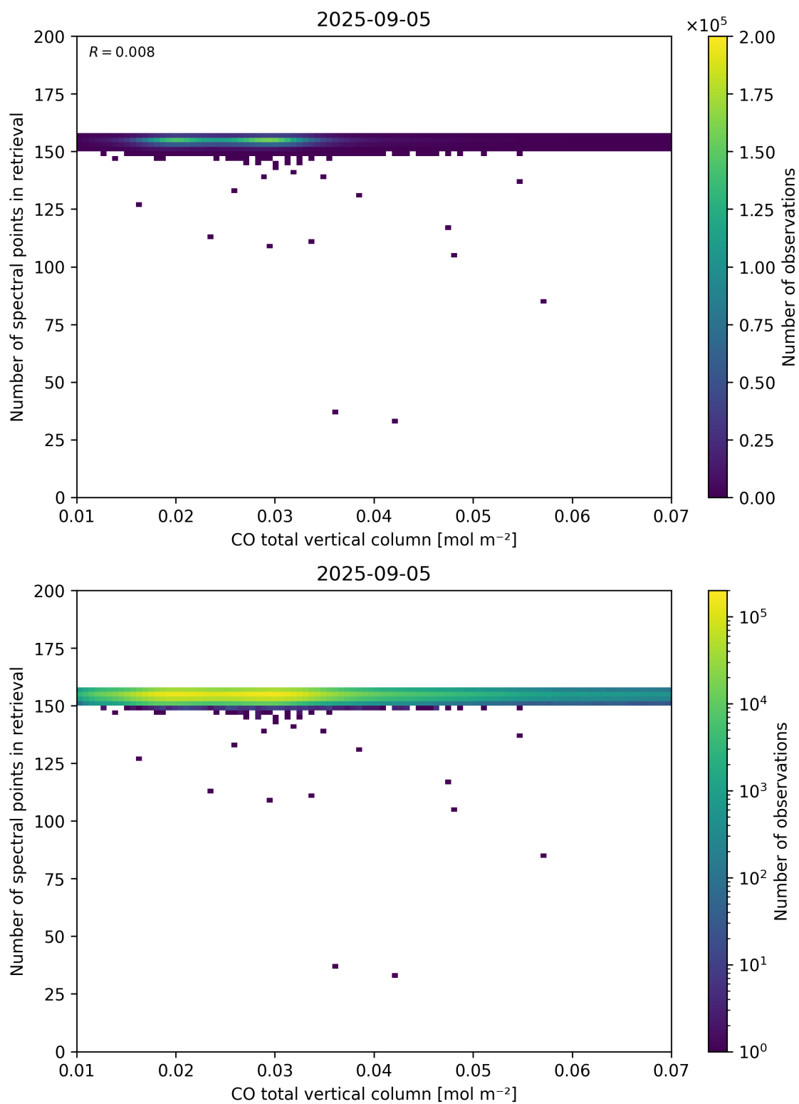
Figure 43: Scatter density plot of “CO total vertical column” against “Number of spectral points in retrieval” for 2025-09-04 to 2025-09-06.
