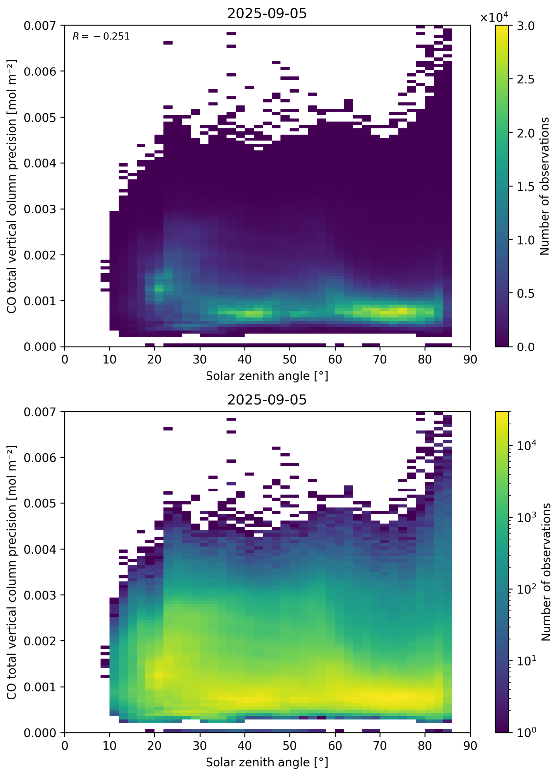
Figure 63: Scatter density plot of “Solar zenith angle” against “CO total vertical column precision” for 2025-09-04 to 2025-09-06.
