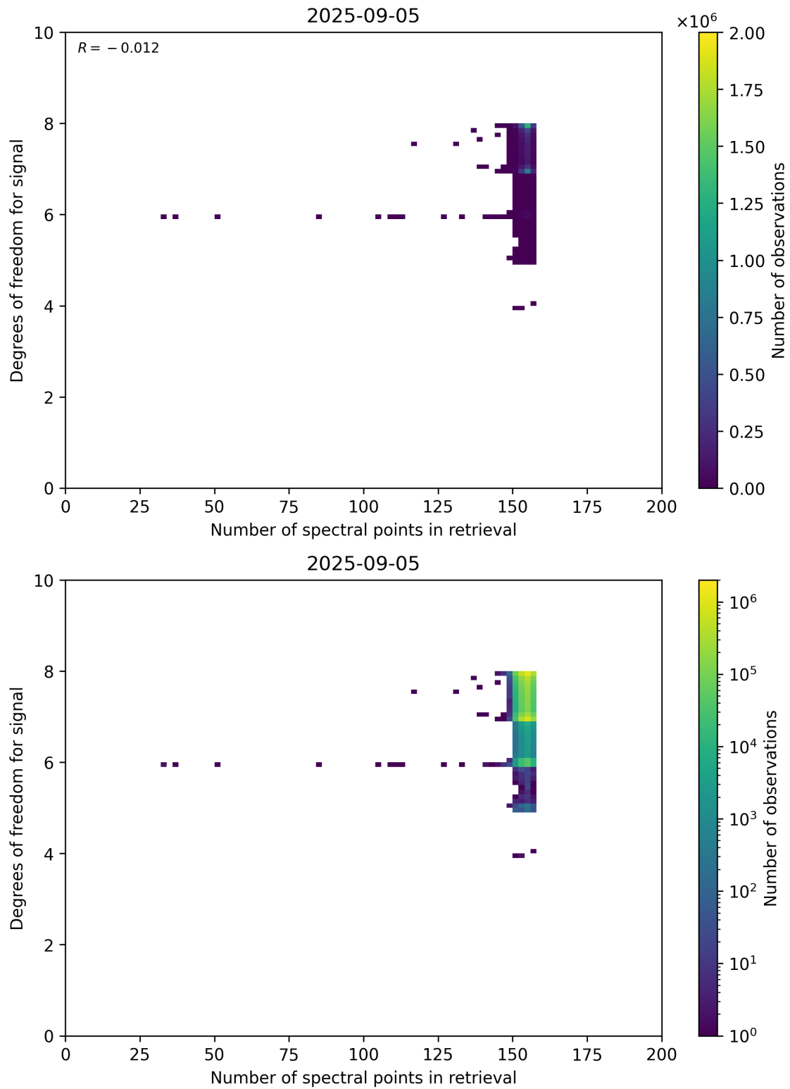
Figure 59: Scatter density plot of “Number of spectral points in retrieval” against “Degrees of freedom for signal” for 2025-09-04 to 2025-09-06.
