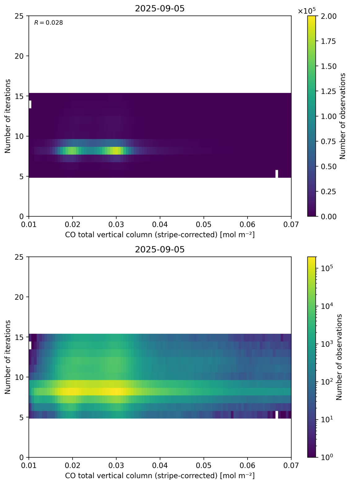
Figure 39: Scatter density plot of “CO total vertical column (stripe-corrected)” against “Number of iterations” for 2025-09-04 to 2025-09-06.
