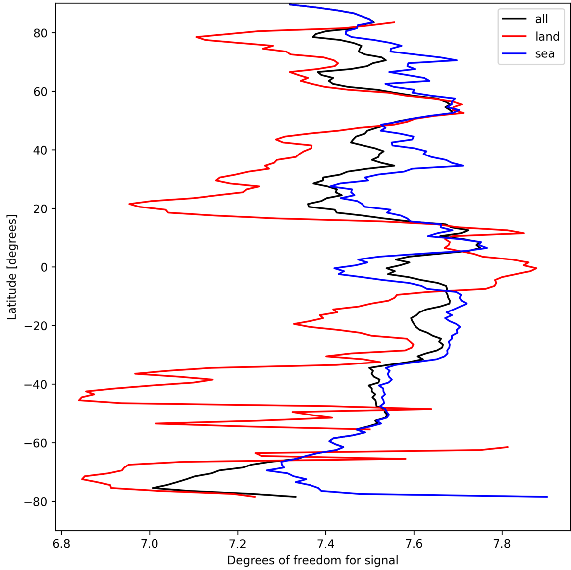
Figure 15: Zonal average of “Degrees of freedom for signal” for 2025-09-04 to 2025-09-06.
