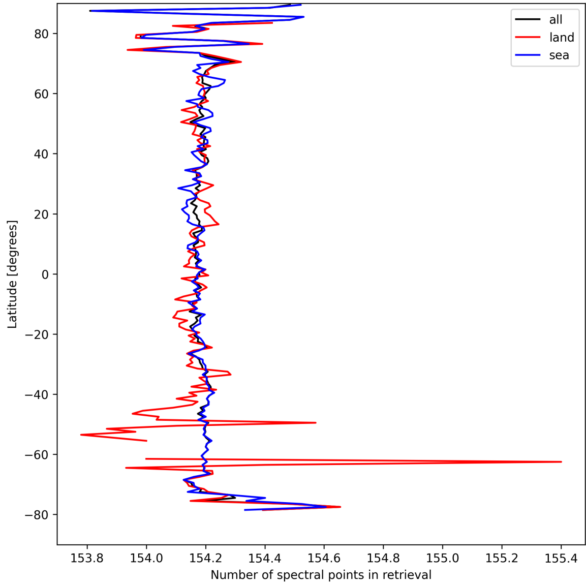
Figure 13: Zonal average of “Number of spectral points in retrieval” for 2025-09-04 to 2025-09-06.
