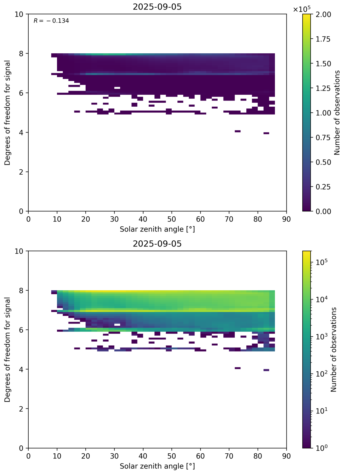
Figure 65: Scatter density plot of “Solar zenith angle” against “Degrees of freedom for signal” for 2025-09-04 to 2025-09-06.
