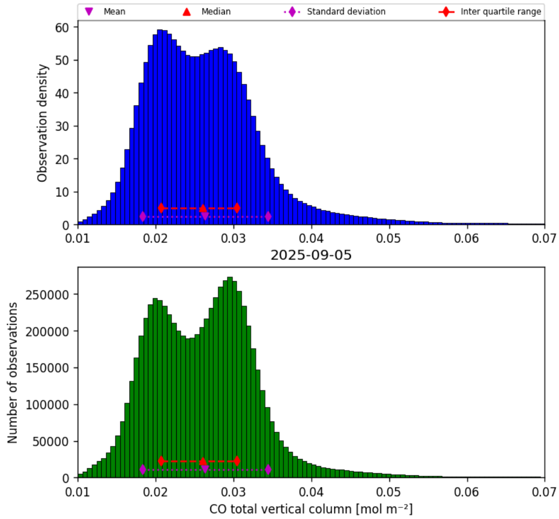
Figure 18: Histogram of “CO total vertical column” for 2025-09-04 to 2025-09-06
