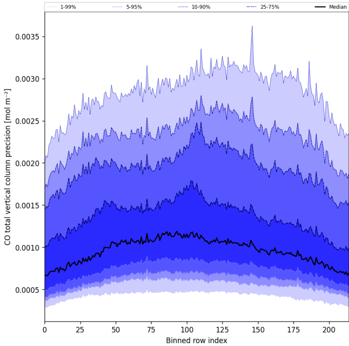
Figure 28: Along track statistics of “CO total vertical column precision” for 2025-09-04 to 2025-09-06
