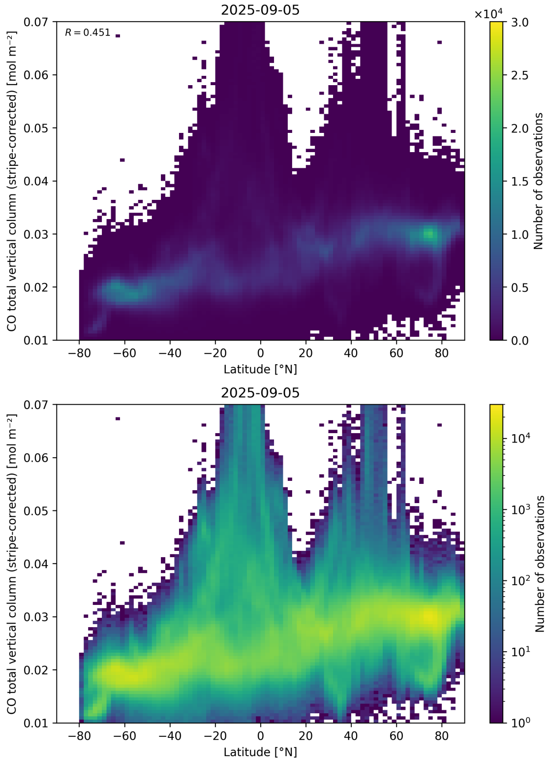
Figure 52: Scatter density plot of “Latitude” against “CO total vertical column (stripe-corrected)” for 2025-09-04 to 2025-09-06.
