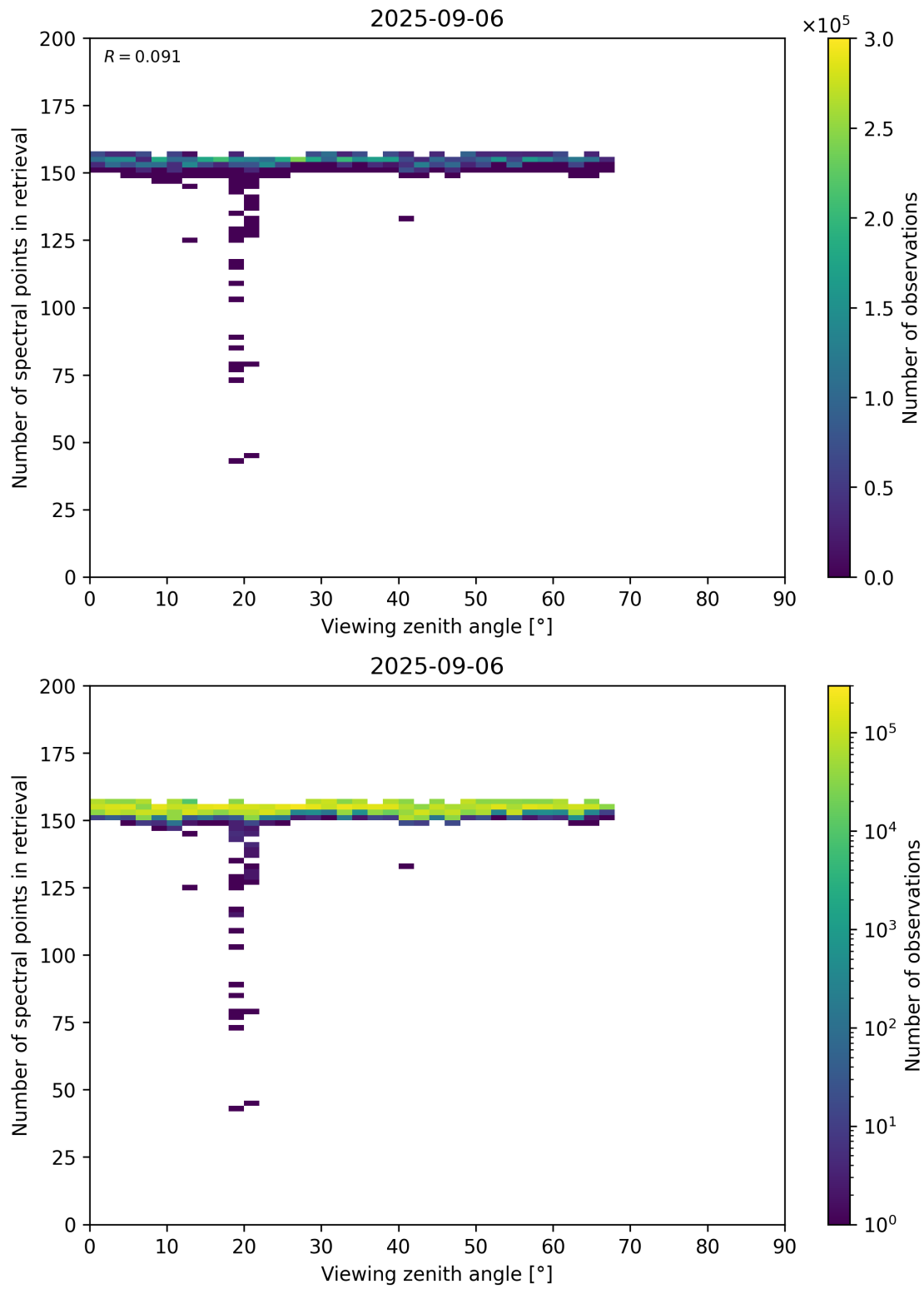
Figure 76: Scatter density plot of “Viewing zenith angle” against “Number of spectral points in retrieval” for 2025-09-05 to 2025-09-07.
