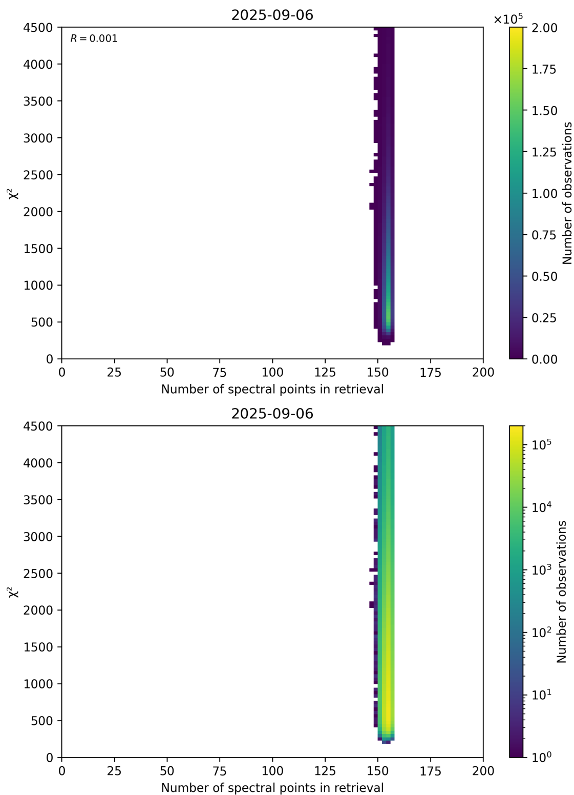
Figure 58: Scatter density plot of “Number of spectral points in retrieval” against “ \chi^2 ” for 2025-09-05 to 2025-09-07.
