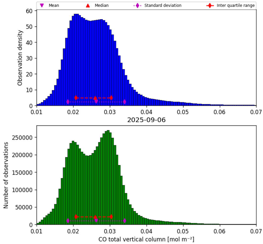
Figure 18: Histogram of “CO total vertical column” for 2025-09-05 to 2025-09-07
