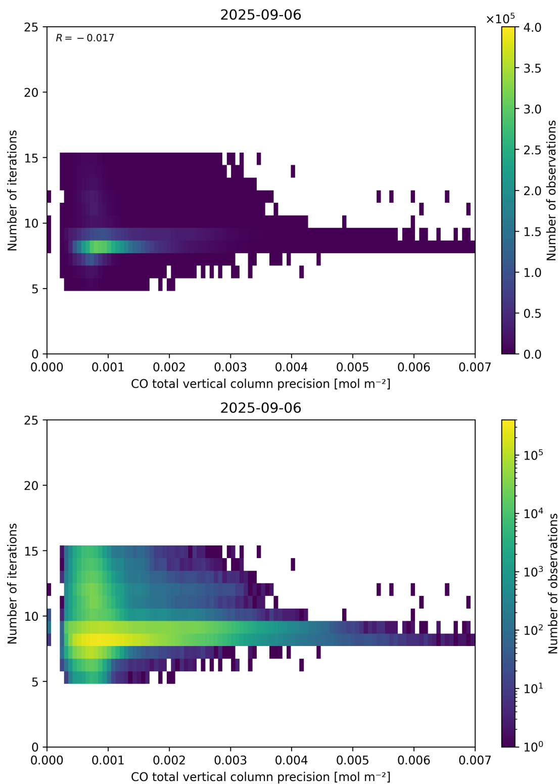
Figure 46: Scatter density plot of “CO total vertical column precision” against “Number of iterations” for 2025-09-05 to 2025-09-07.
