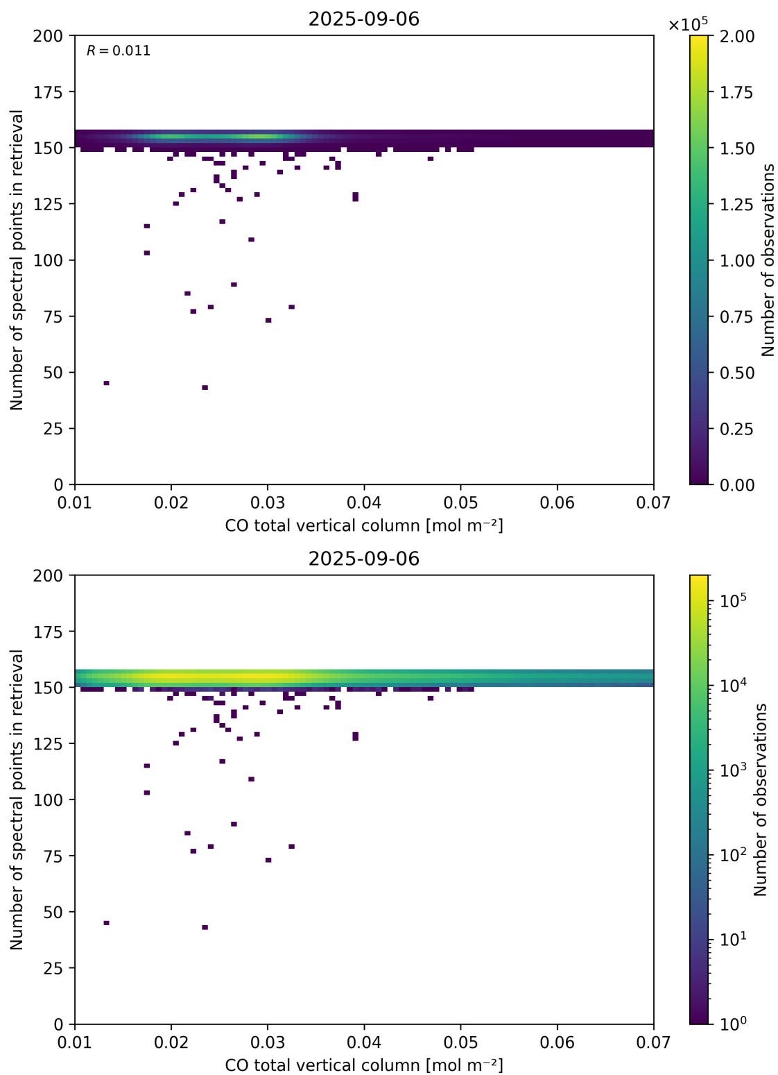
Figure 43: Scatter density plot of “CO total vertical column” against “Number of spectral points in retrieval” for 2025-09-05 to 2025-09-07.
