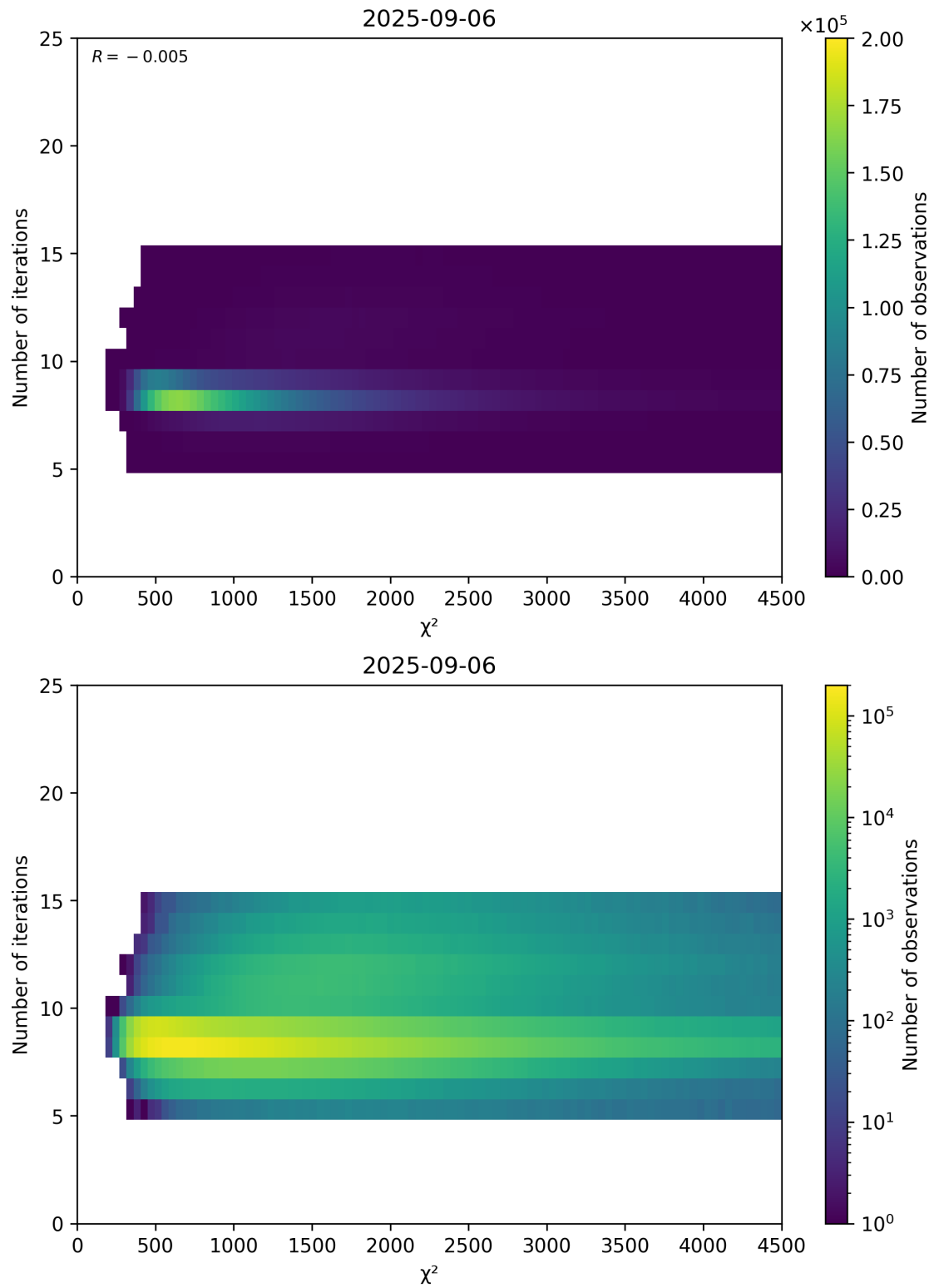
Figure 49: Scatter density plot of “ \chi^2 ” against “Number of iterations” for 2025-09-05 to 2025-09-07.
