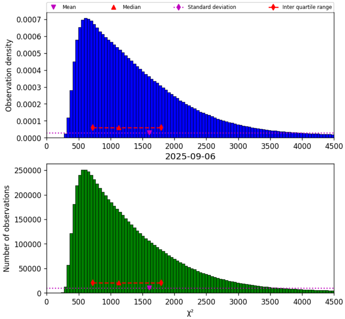
Figure 22: Histogram of " \chi^2 " for 2025-09-05 to 2025-09-07
