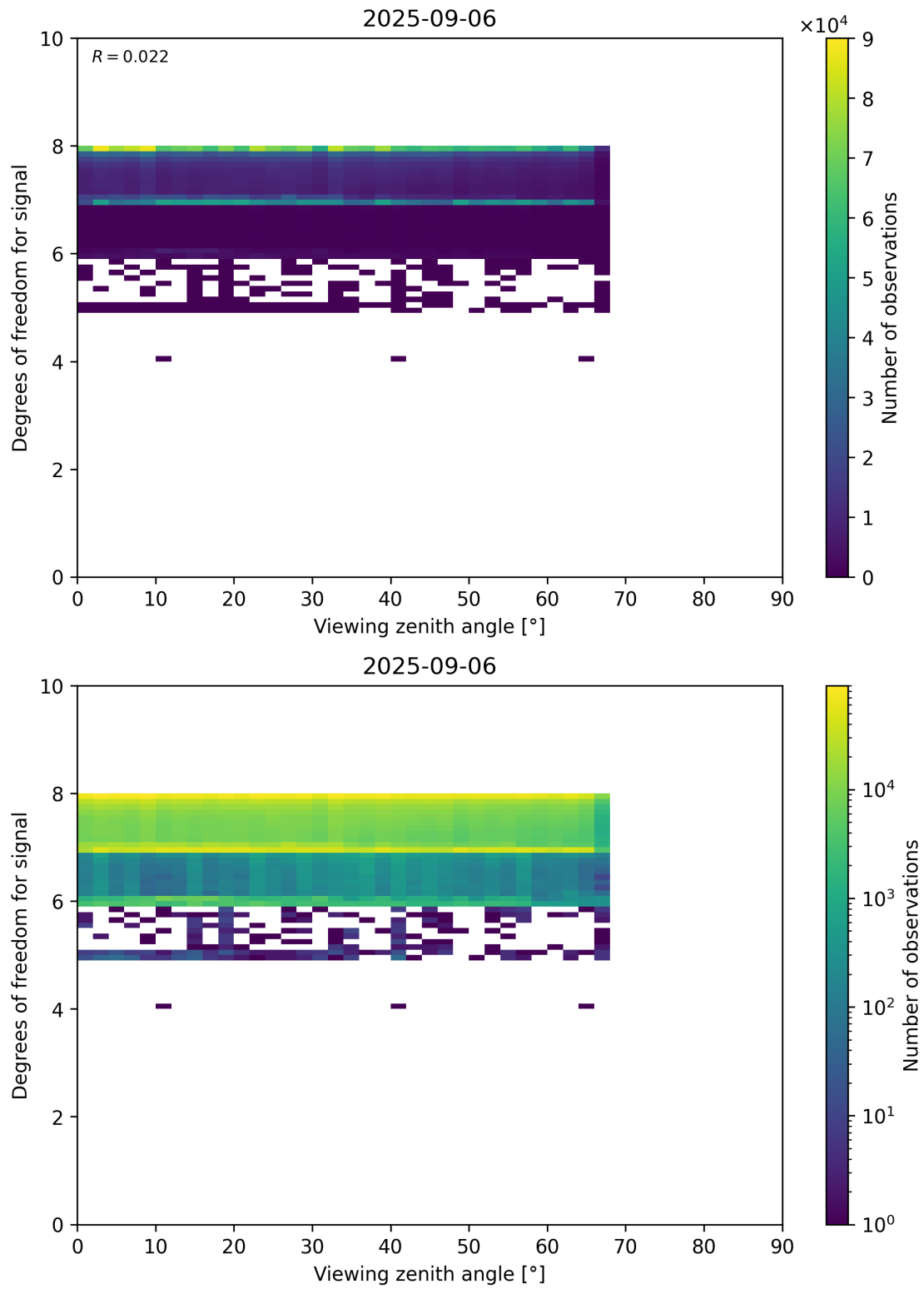
Figure 73: Scatter density plot of “Viewing zenith angle” against “Degrees of freedom for signal” for 2025-09-05 to 2025-09-07.
