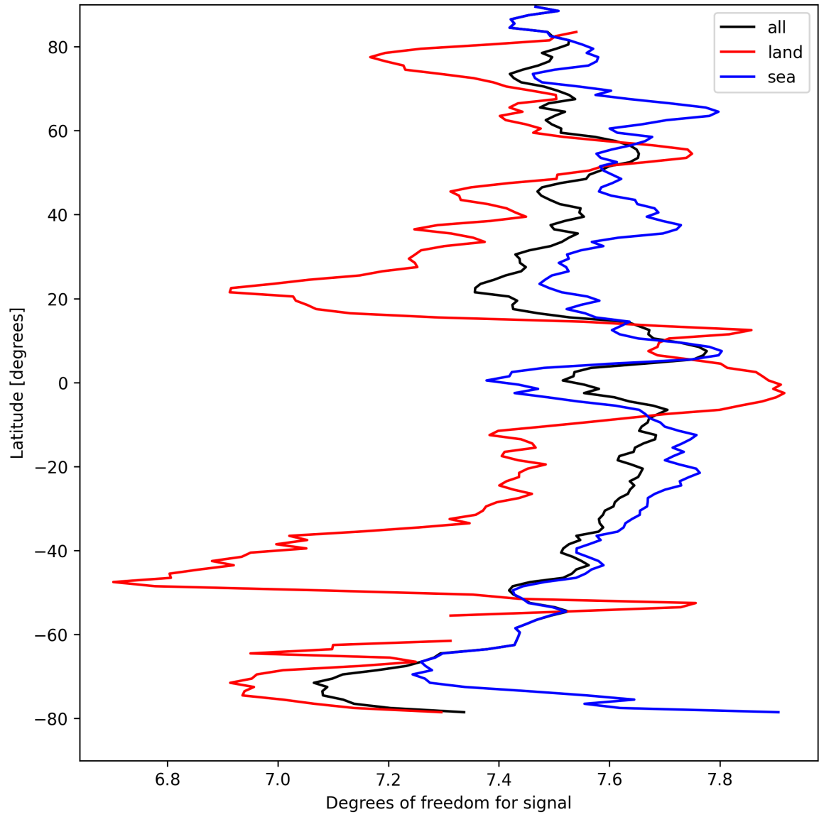
Figure 15: Zonal average of “Degrees of freedom for signal” for 2025-09-05 to 2025-09-07.
