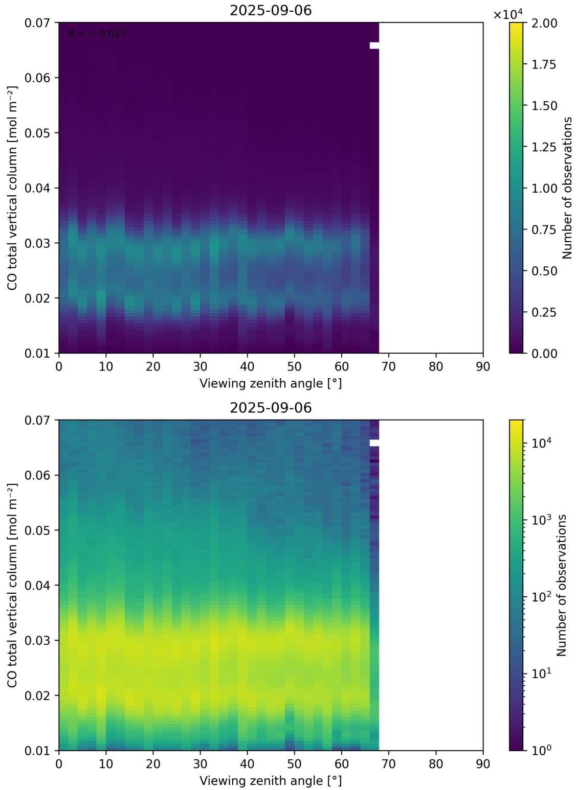
Figure 69: Scatter density plot of “Viewing zenith angle” against “CO total vertical column” for 2025-09-05 to 2025-09-07.
