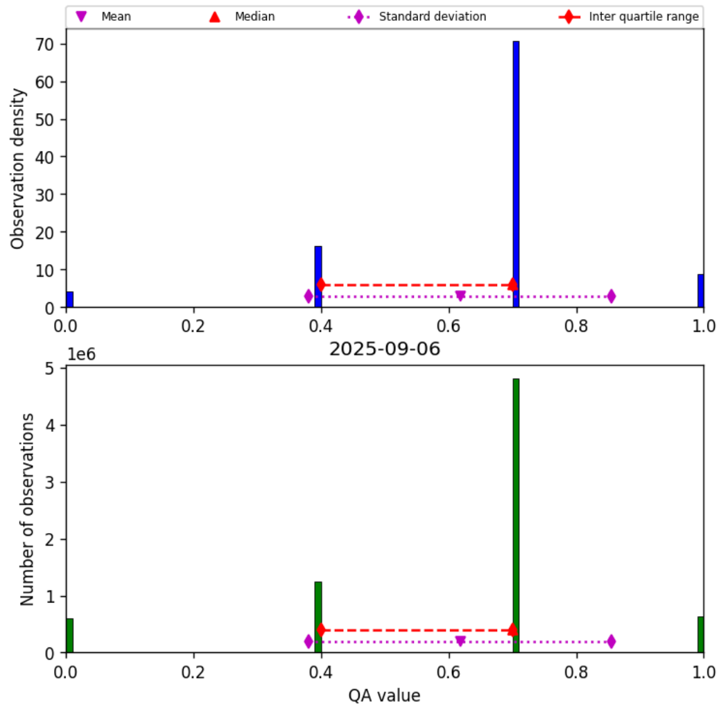
Figure 17: Histogram of “QA value” for 2025-09-05 to 2025-09-07
