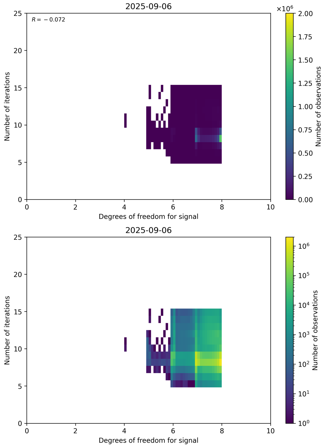
Figure 50: Scatter density plot of “Degrees of freedom for signal” against “Number of iterations” for 2025-09-05 to 2025-09-07.
