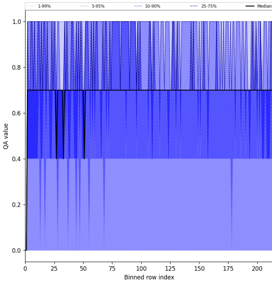
Figure 25: Along track statistics of “QA value” for 2025-09-05 to 2025-09-07
