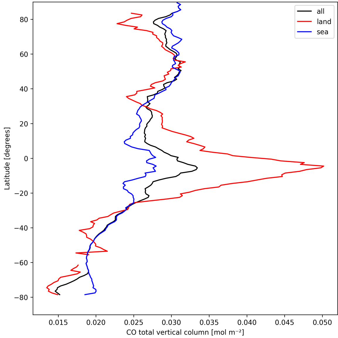
Figure 10: Zonal average of “CO total vertical column” for 2025-09-05 to 2025-09-07.
