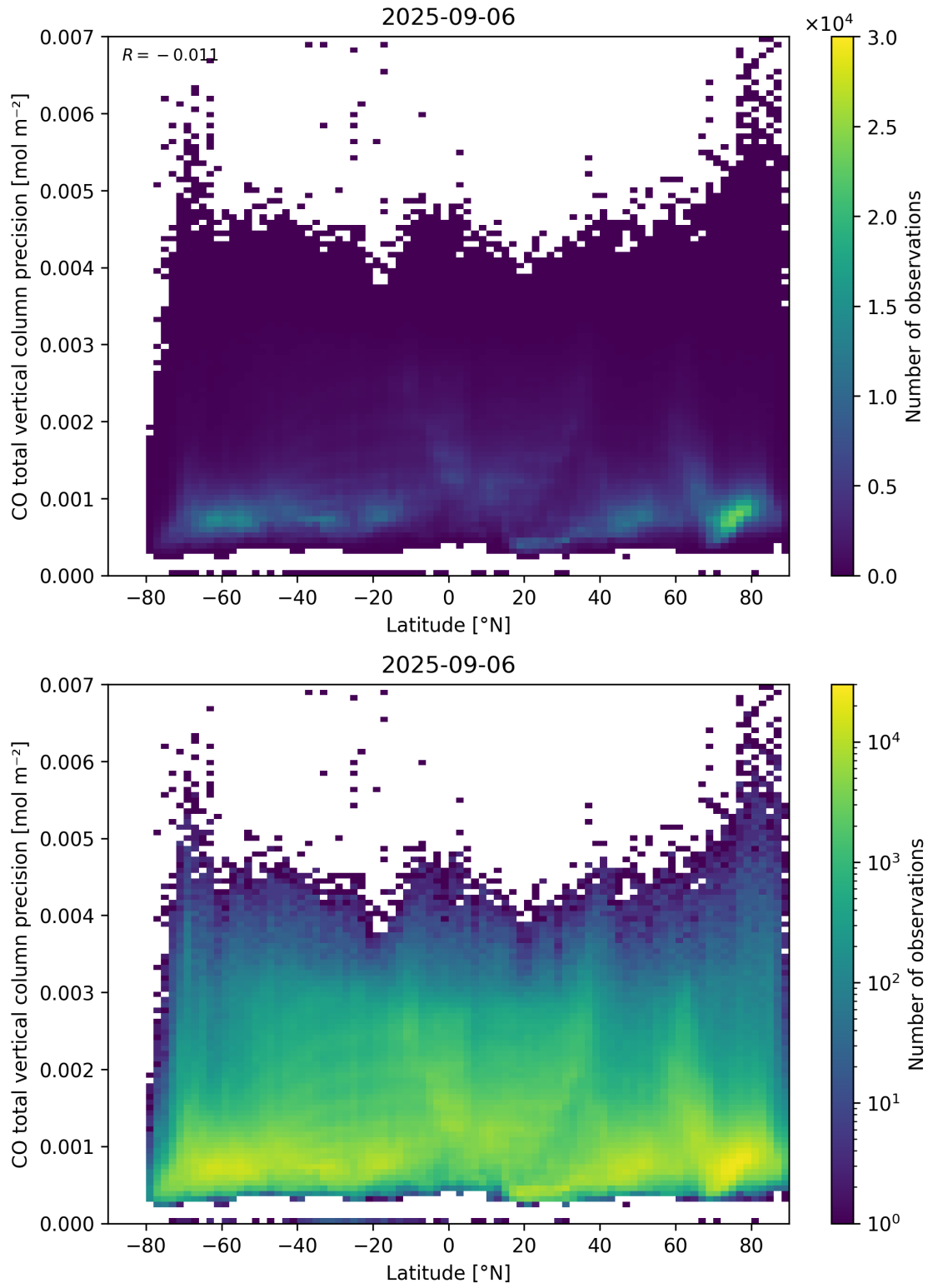
Figure 53: Scatter density plot of “Latitude” against “CO total vertical column precision” for 2025-09-05 to 2025-09-07.
