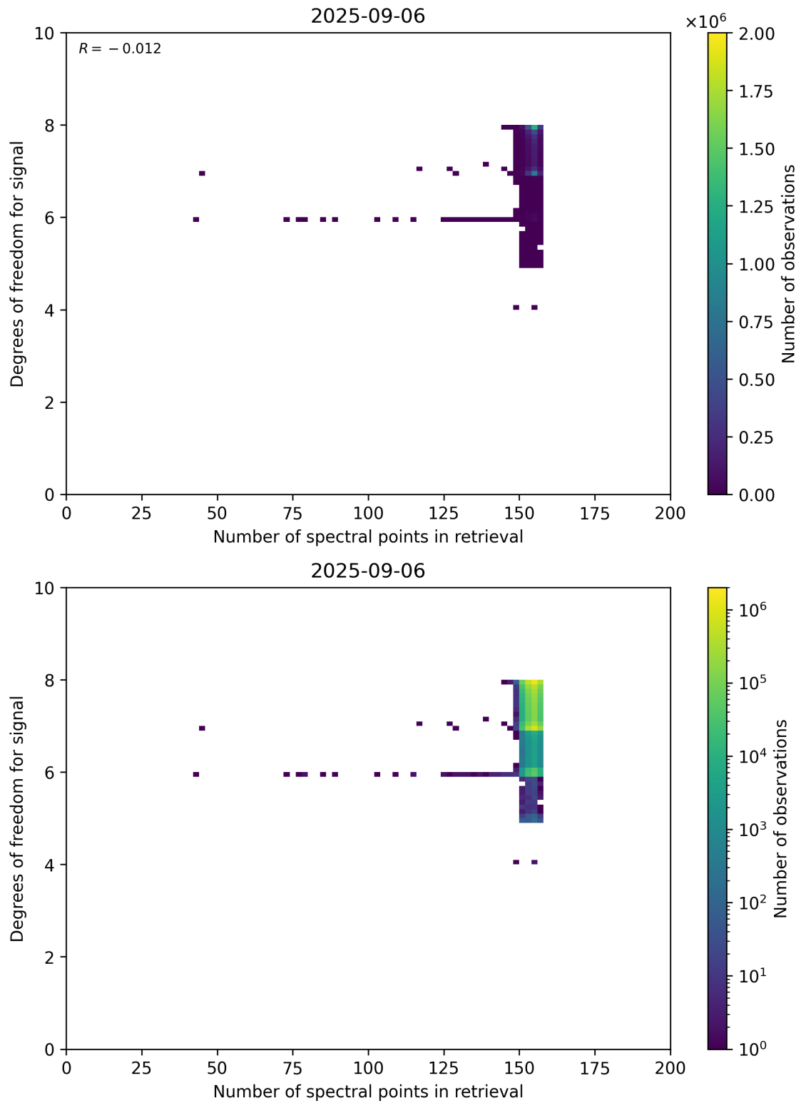
Figure 59: Scatter density plot of “Number of spectral points in retrieval” against “Degrees of freedom for signal” for 2025-09-05 to 2025-09-07.
