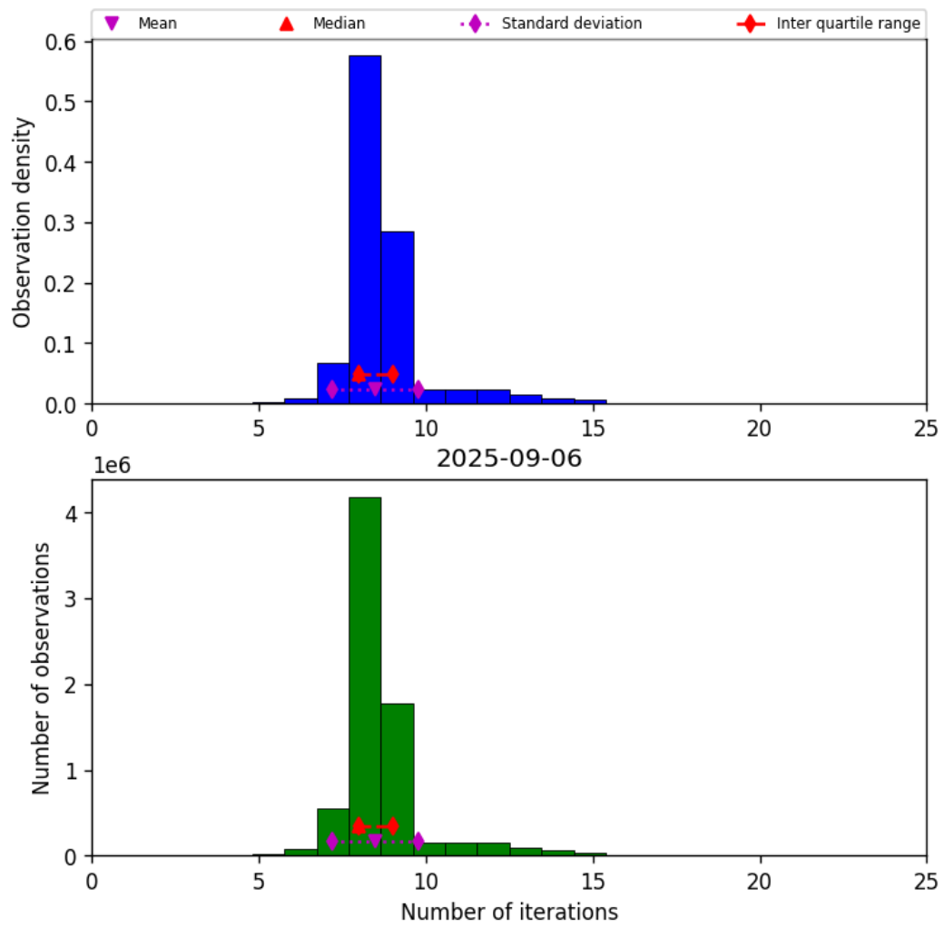
Figure 24: Histogram of “Number of iterations” for 2025-09-05 to 2025-09-07
