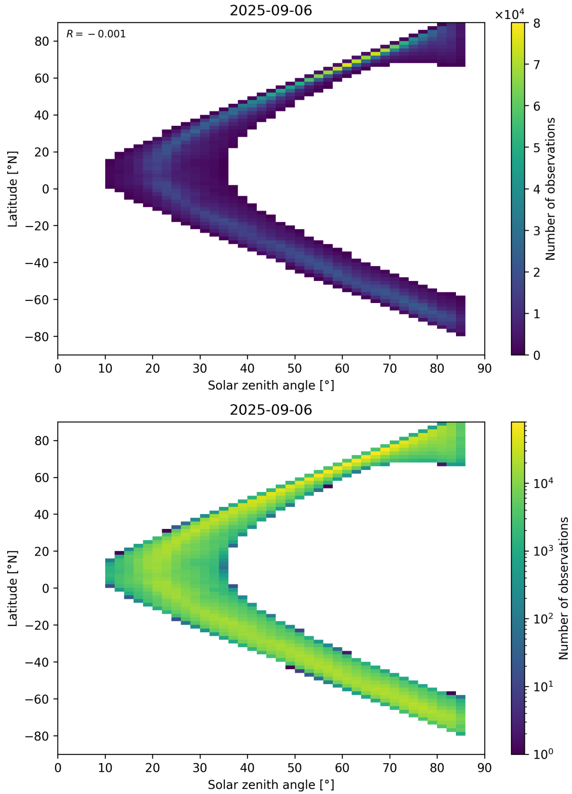
Figure 66: Scatter density plot of “Solar zenith angle” against “Latitude” for 2025-09-05 to 2025-09-07.
