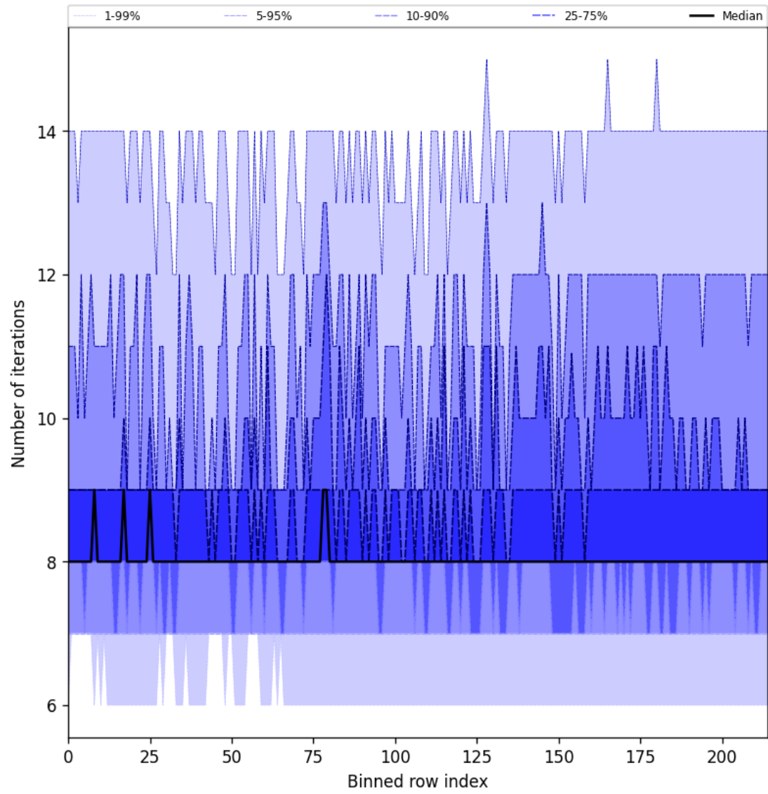
Figure 32: Along track statistics of “Number of iterations” for 2025-09-05 to 2025-09-07
