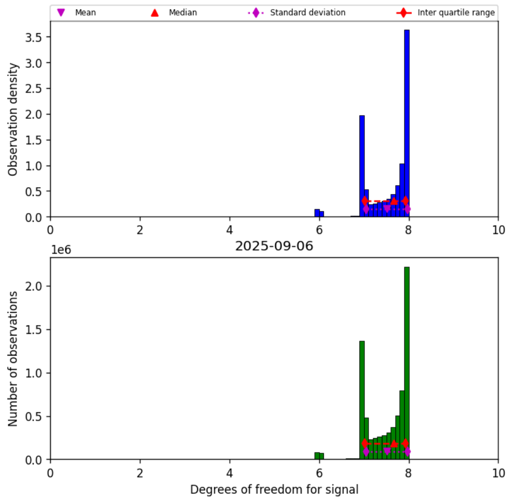
Figure 23: Histogram of “Degrees of freedom for signal” for 2025-09-05 to 2025-09-07
