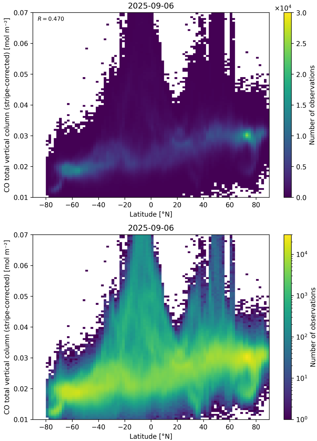
Figure 52: Scatter density plot of “Latitude” against “CO total vertical column (stripe-corrected)” for 2025-09-05 to 2025-09-07.
