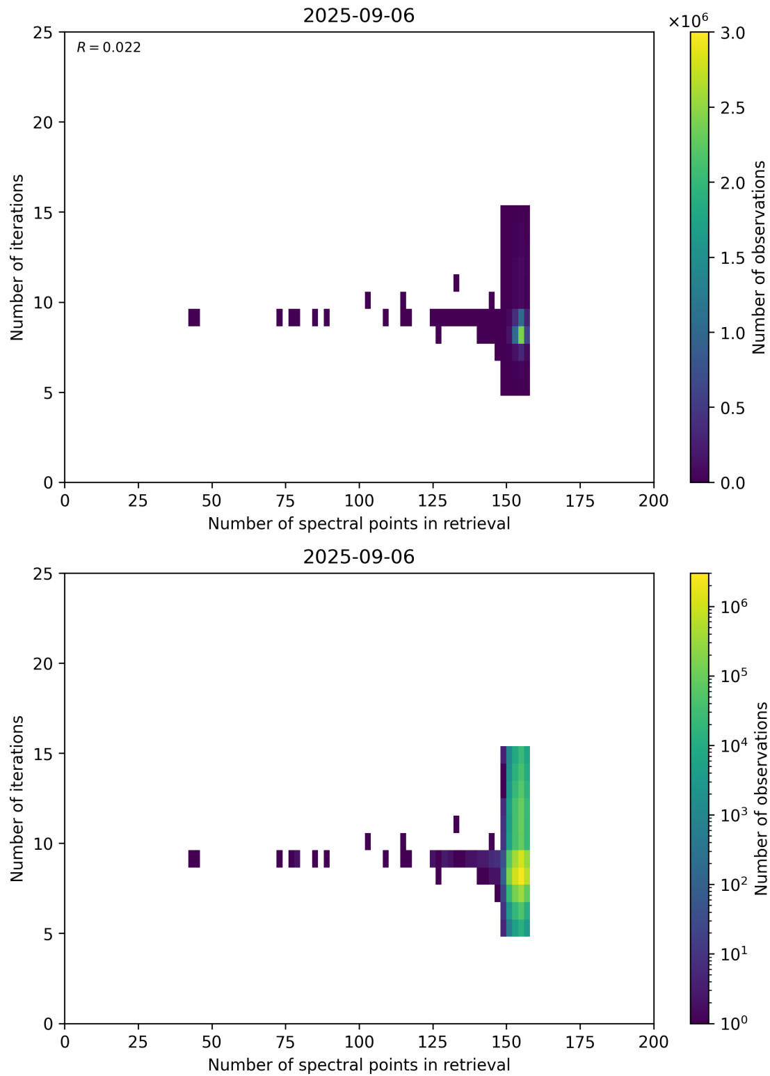
Figure 60: Scatter density plot of “Number of spectral points in retrieval” against “Number of iterations” for 2025-09-05 to 2025-09-07.
