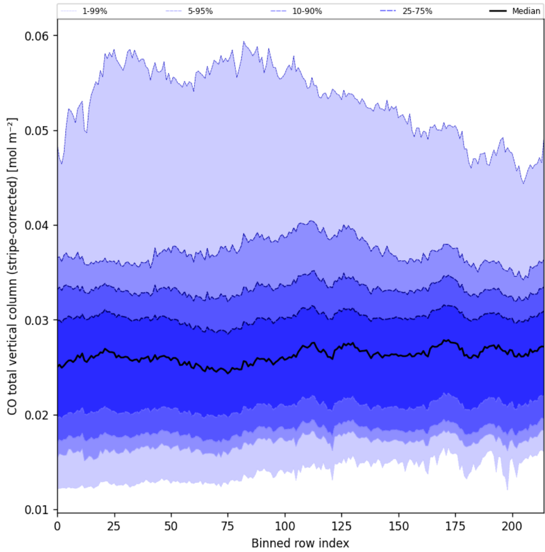
Figure 27: Along track statistics of “CO total vertical column (stripe-corrected)” for 2025-09-05 to 2025-09-07
