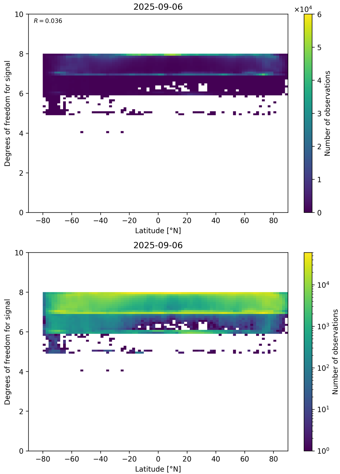
Figure 55: Scatter density plot of “Latitude” against “Degrees of freedom for signal” for 2025-09-05 to 2025-09-07.
