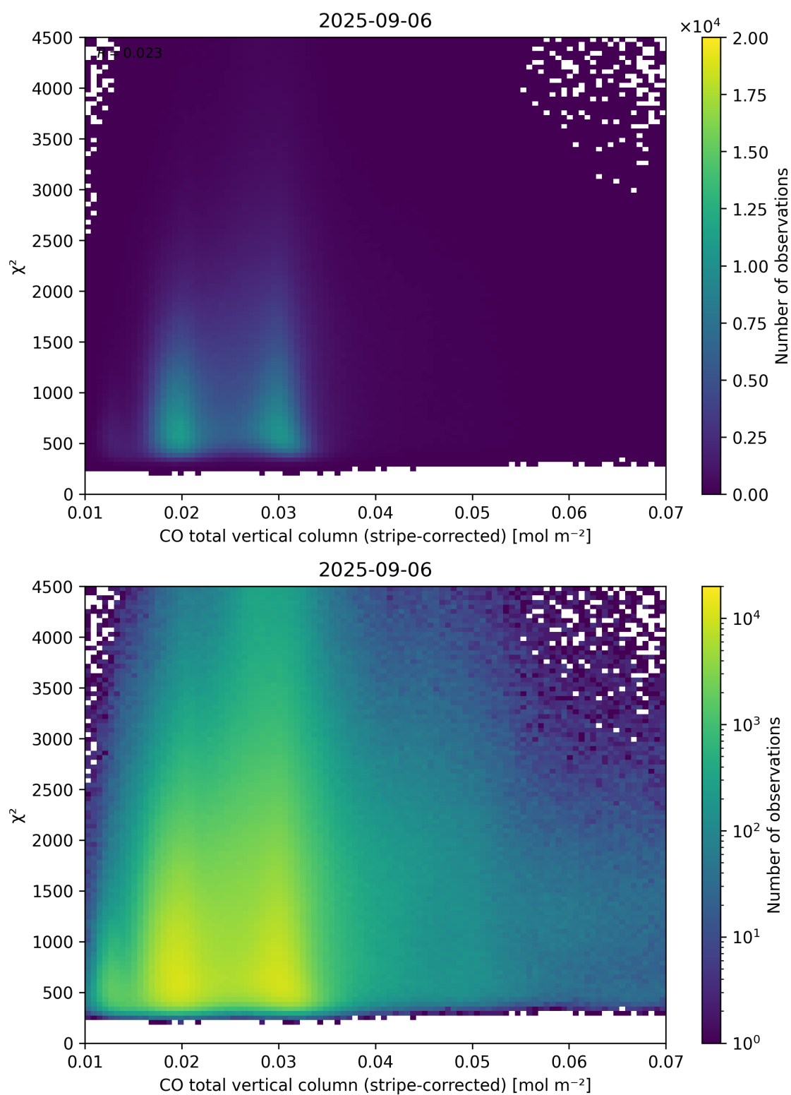
Figure 37: Scatter density plot of “CO total vertical column (stripe-corrected)” against “ \chi^2 ” for 2025-09-05 to 2025-09-07.
