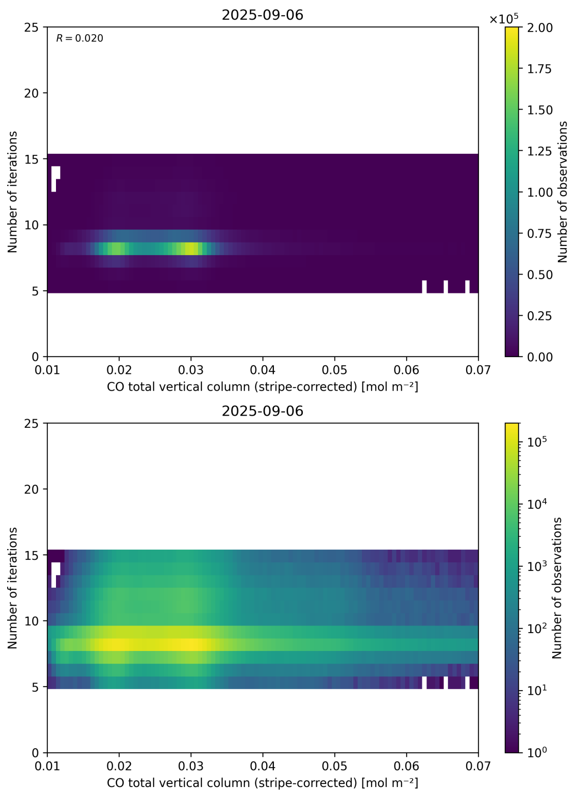
Figure 39: Scatter density plot of “CO total vertical column (stripe-corrected)” against “Number of iterations” for 2025-09-05 to 2025-09-07.
