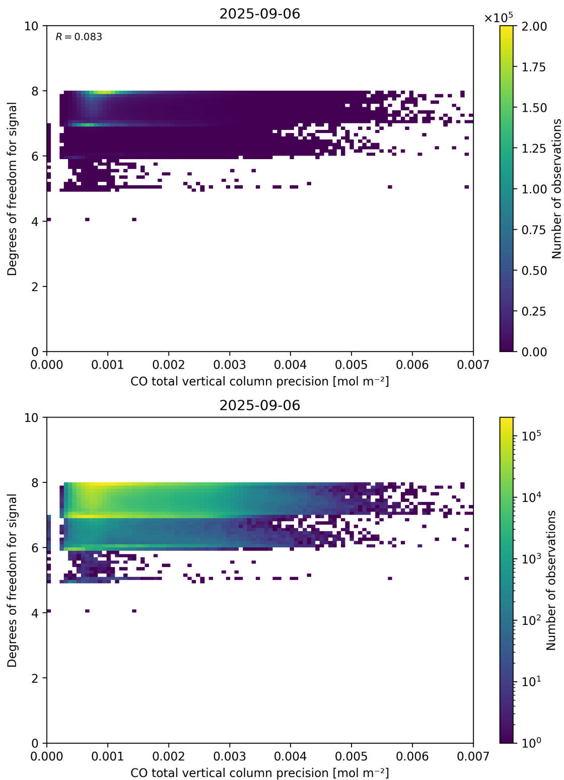
Figure 45: Scatter density plot of “CO total vertical column precision” against “Degrees of freedom for signal” for 2025-09-05 to 2025-09-07.
