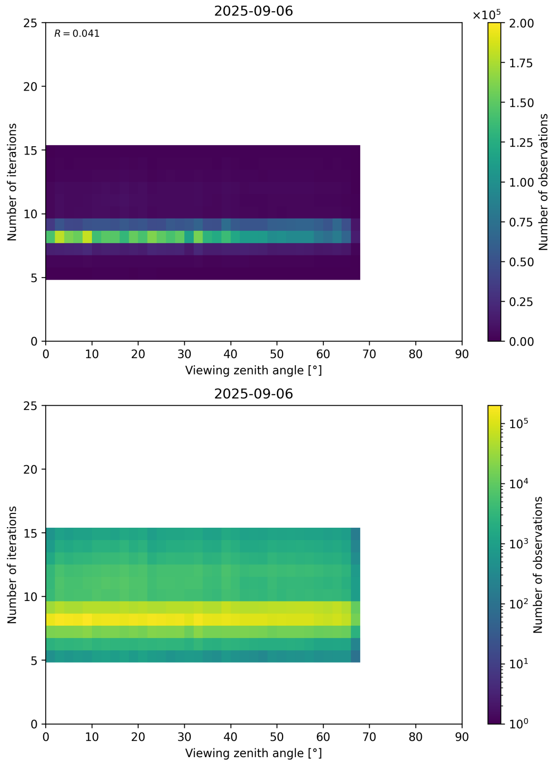
Figure 75: Scatter density plot of “Viewing zenith angle” against “Number of iterations” for 2025-09-05 to 2025-09-07.
