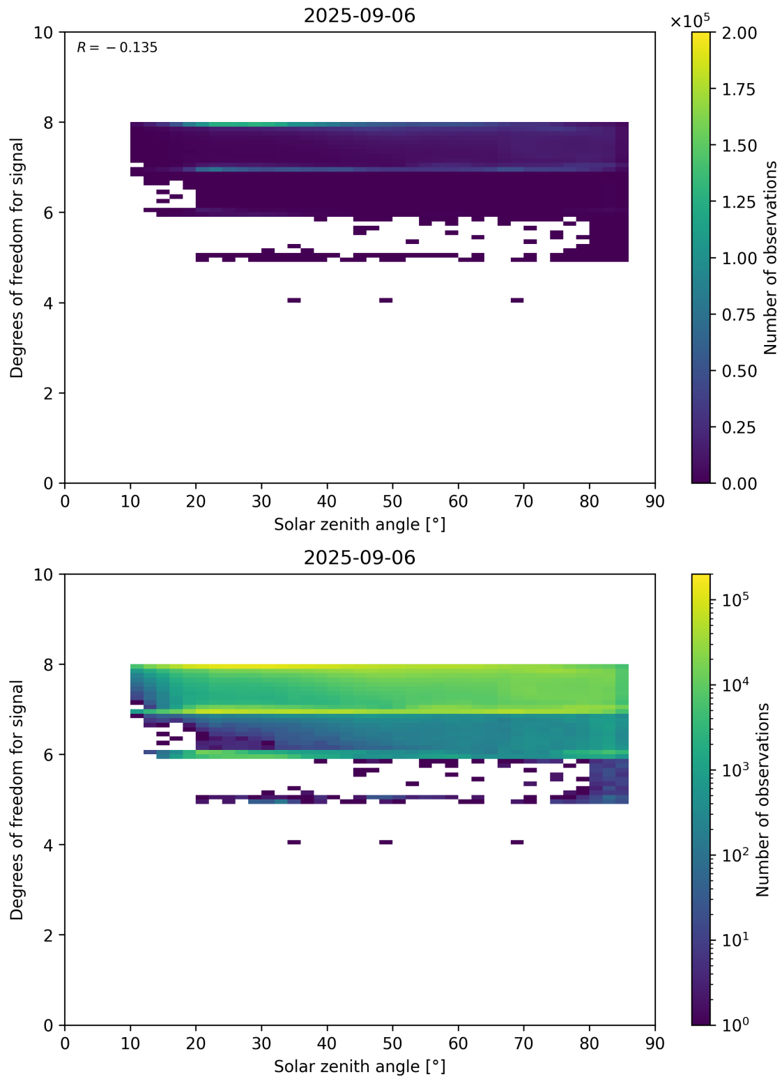
Figure 65: Scatter density plot of “Solar zenith angle” against “Degrees of freedom for signal” for 2025-09-05 to 2025-09-07.
