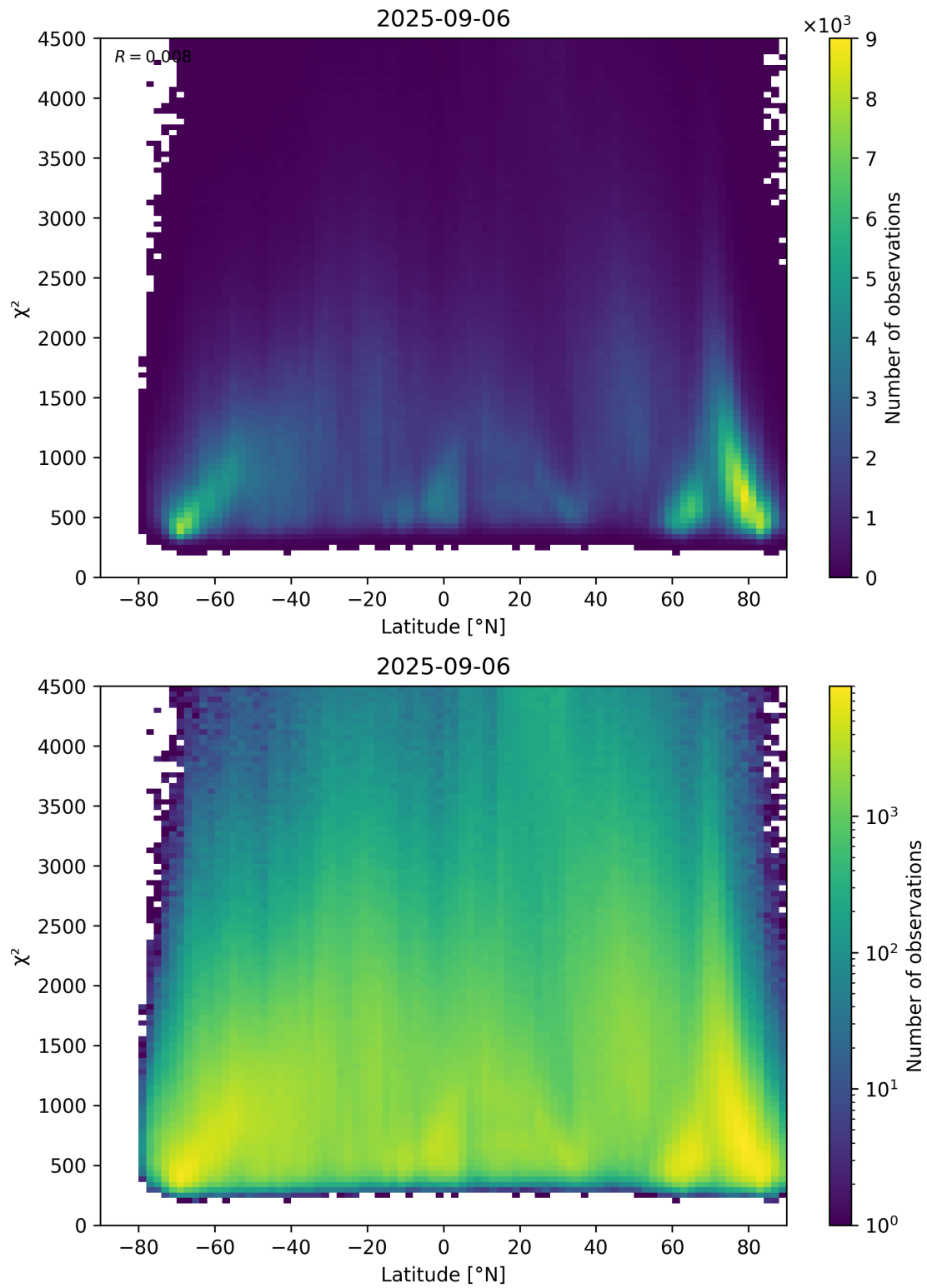
Figure 54: Scatter density plot of “Latitude” against “ \chi^2 ” for 2025-09-05 to 2025-09-07.
