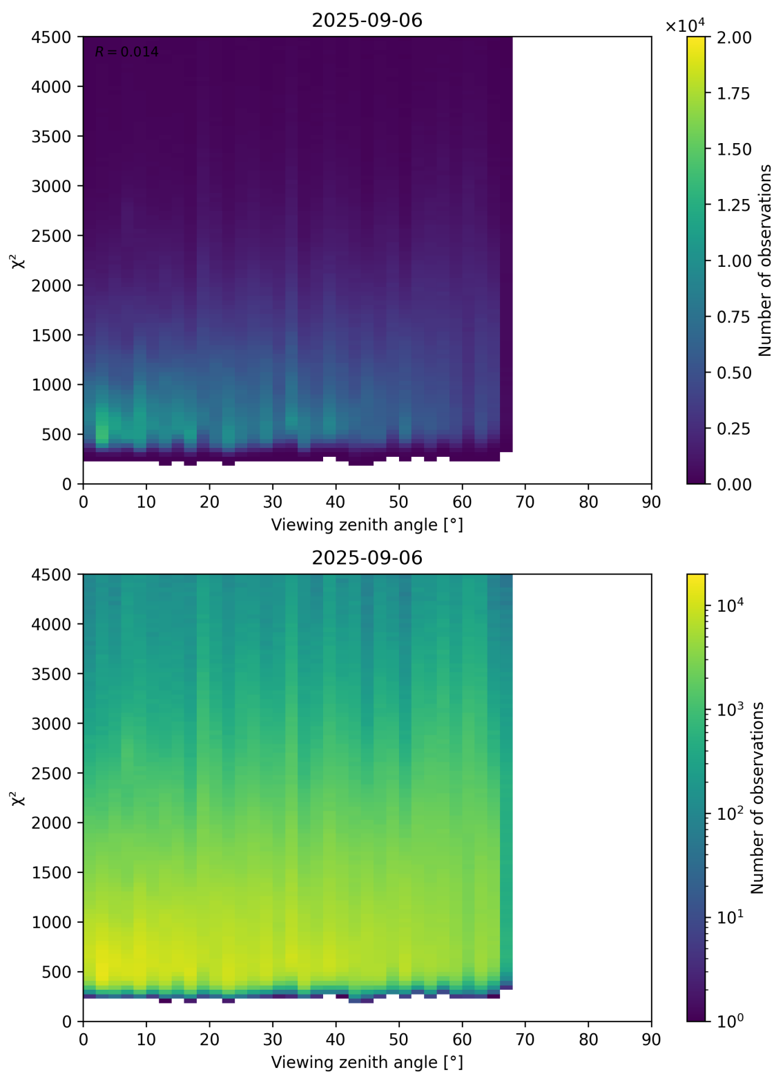
Figure 72: Scatter density plot of “Viewing zenith angle” against “ \chi^2 ” for 2025-09-05 to 2025-09-07.
