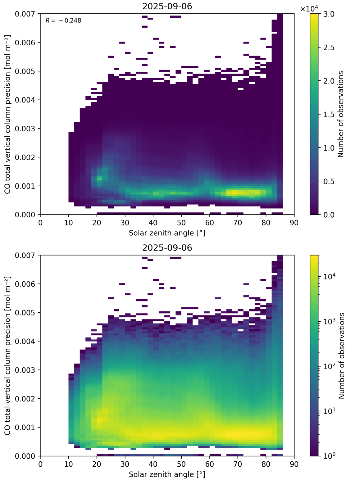
Figure 63: Scatter density plot of “Solar zenith angle” against “CO total vertical column precision” for 2025-09-05 to 2025-09-07.
