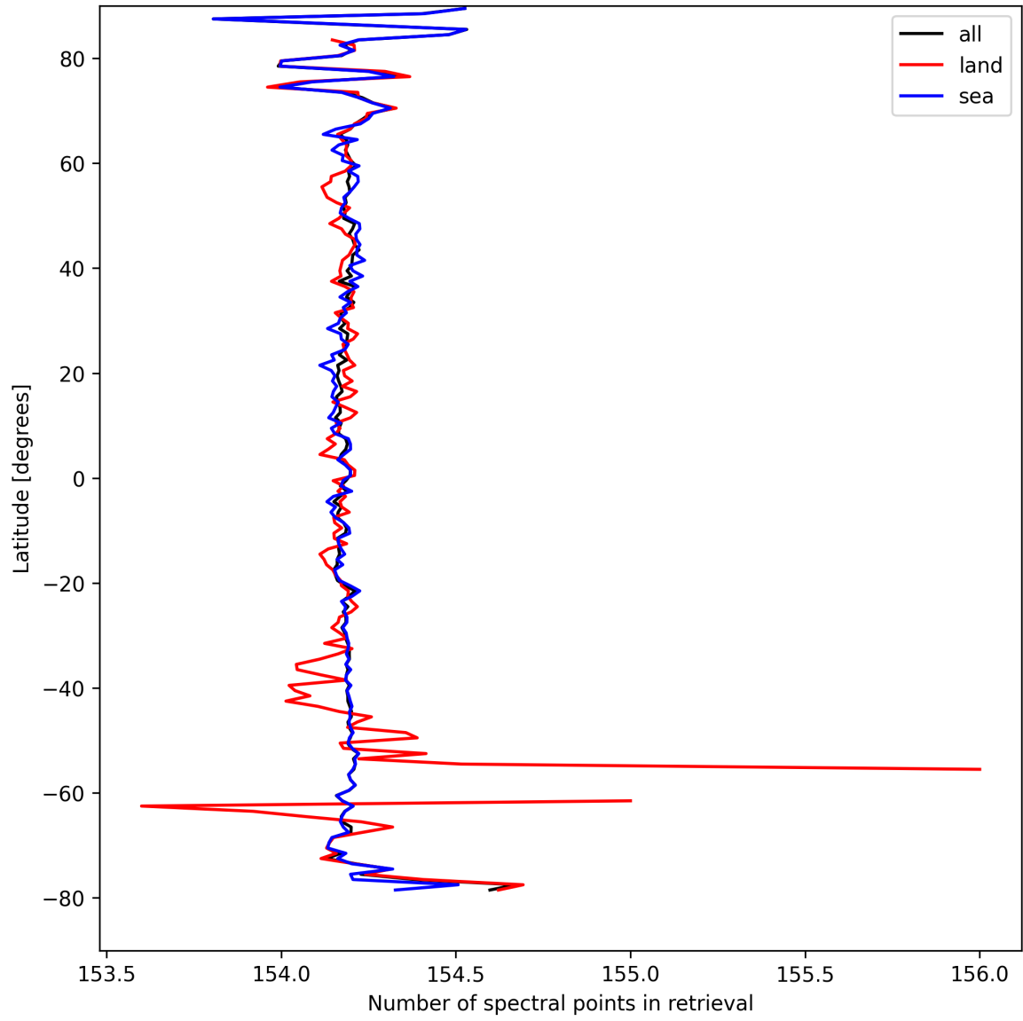
Figure 13: Zonal average of “Number of spectral points in retrieval” for 2025-09-05 to 2025-09-07.
