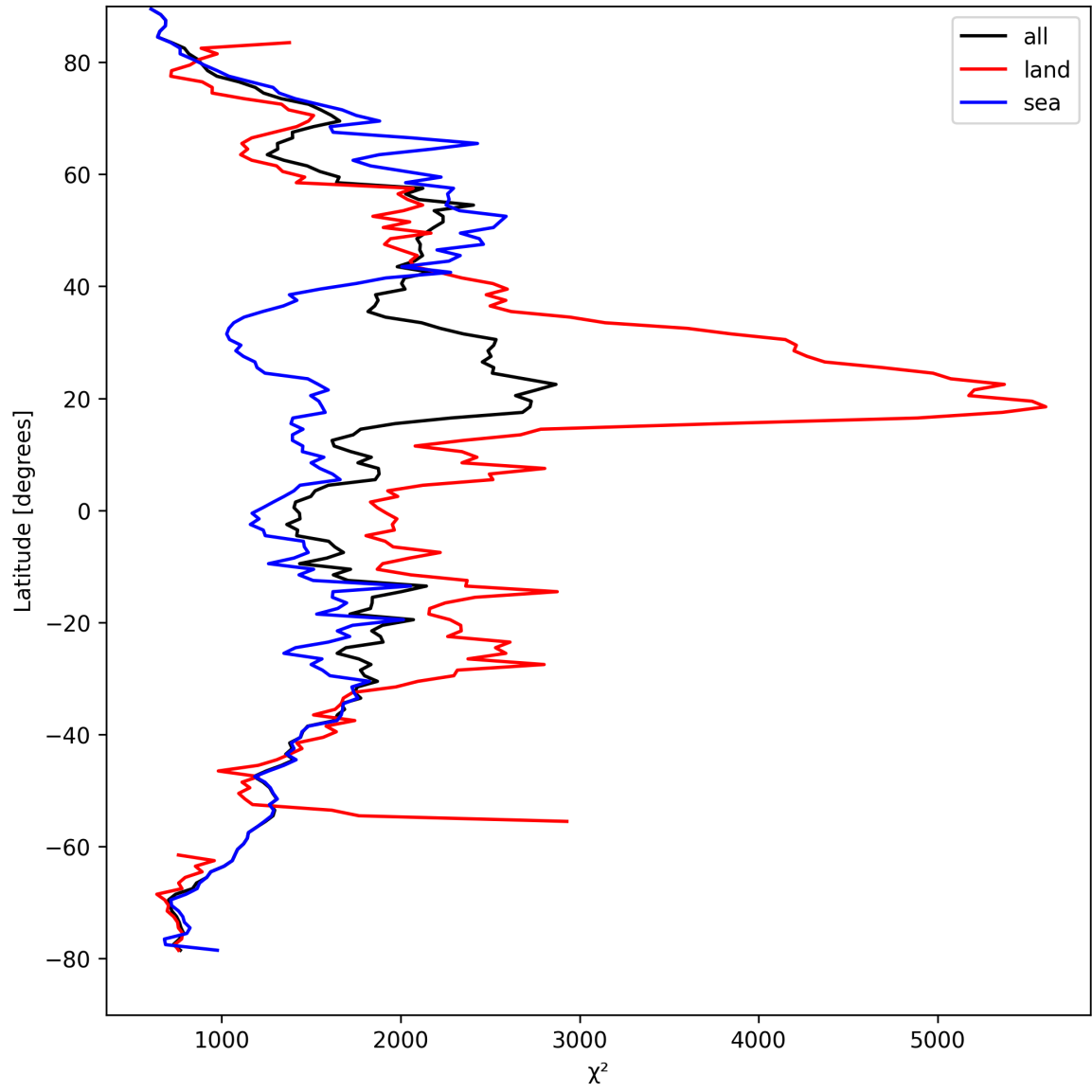
Figure 14: Zonal average of “ \chi^2 ” for 2025-09-05 to 2025-09-07.
