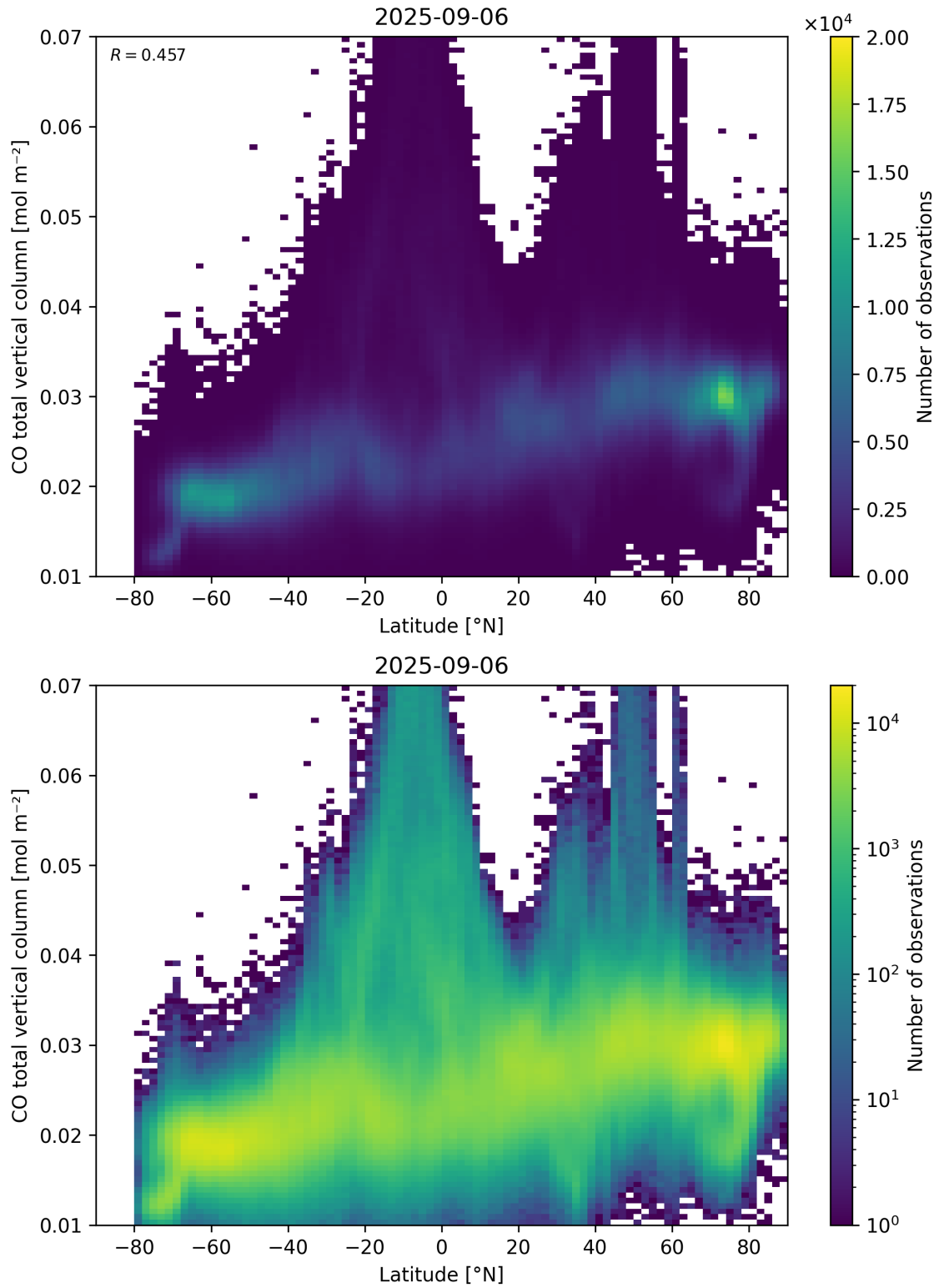
Figure 51: Scatter density plot of “Latitude” against “CO total vertical column” for 2025-09-05 to 2025-09-07.
