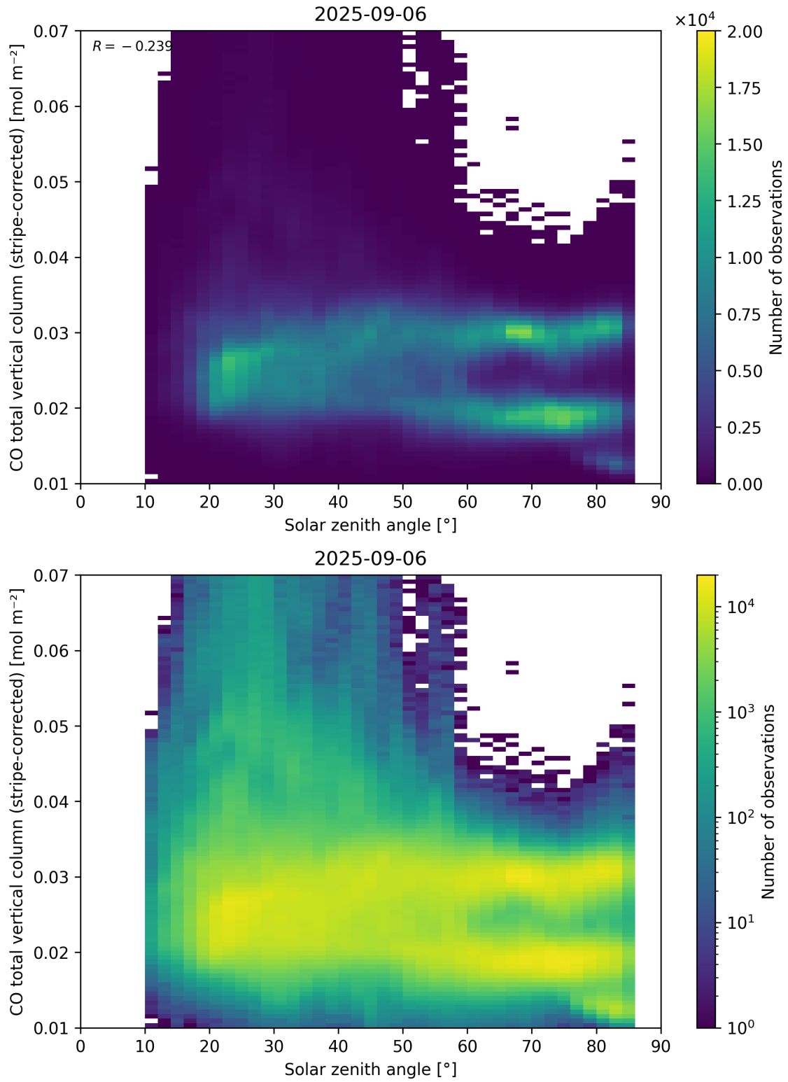
Figure 62: Scatter density plot of “Solar zenith angle” against “CO total vertical column (stripe-corrected)” for 2025-09-05 to 2025-09-07.
