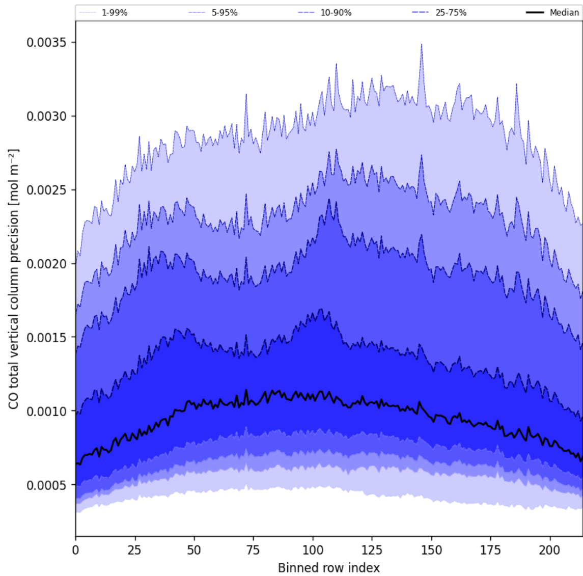
Figure 28: Along track statistics of “CO total vertical column precision” for 2025-09-05 to 2025-09-07
