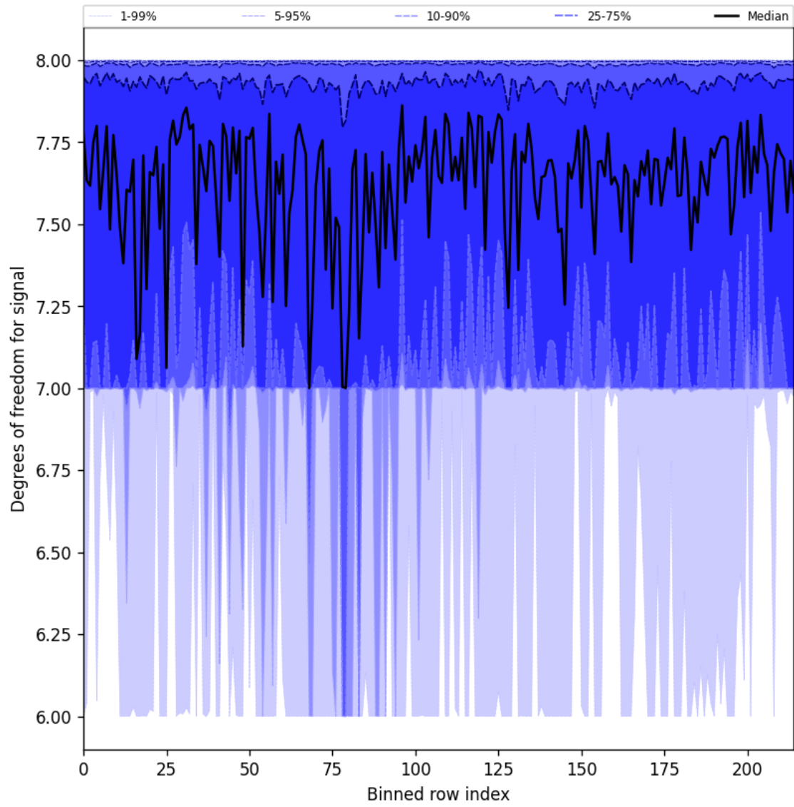
Figure 31: Along track statistics of “Degrees of freedom for signal” for 2025-09-05 to 2025-09-07
