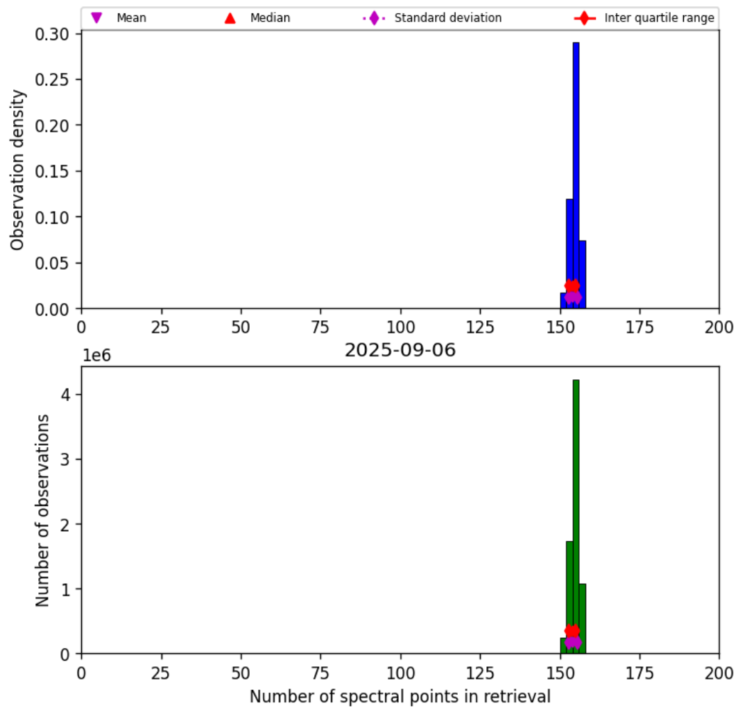
Figure 21: Histogram of “Number of spectral points in retrieval” for 2025-09-05 to 2025-09-07
