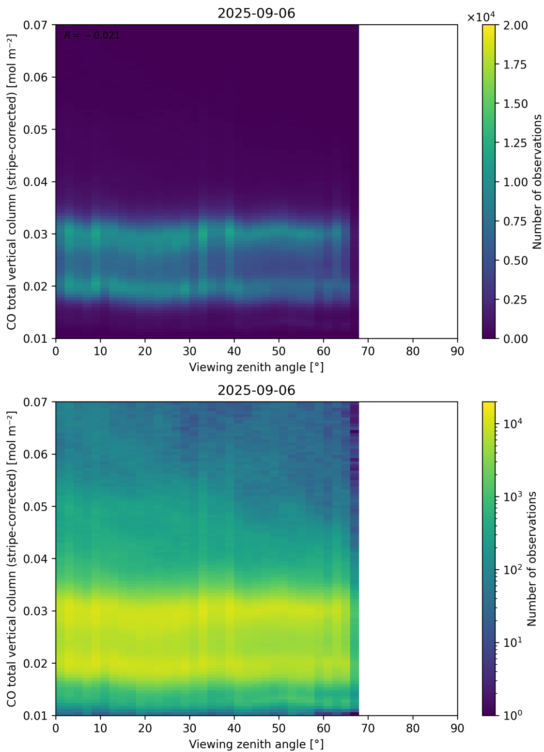
Figure 70: Scatter density plot of “Viewing zenith angle” against “CO total vertical column (stripe-corrected)” for 2025-09-05 to 2025-09-07.
