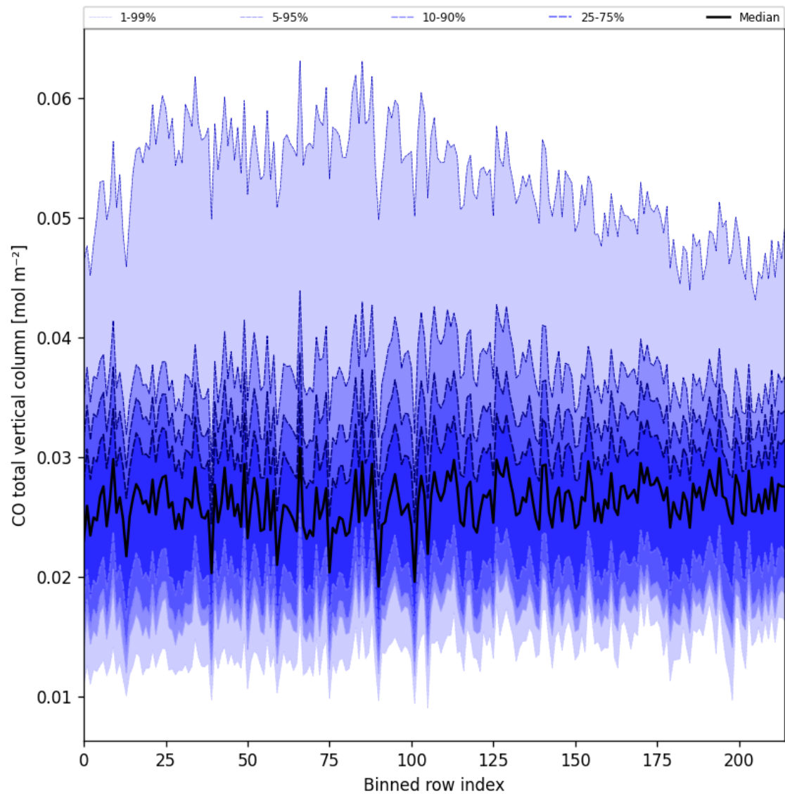
Figure 26: Along track statistics of “CO total vertical column” for 2025-09-05 to 2025-09-07
