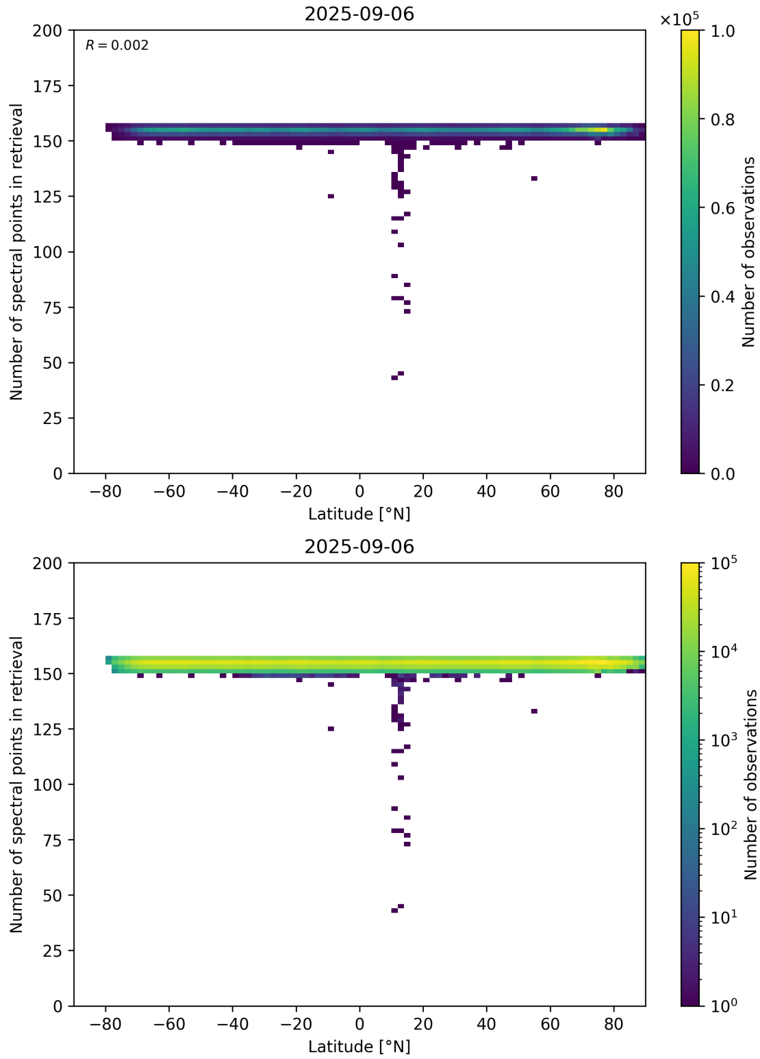
Figure 57: Scatter density plot of “Latitude” against “Number of spectral points in retrieval” for 2025-09-05 to 2025-09-07.
