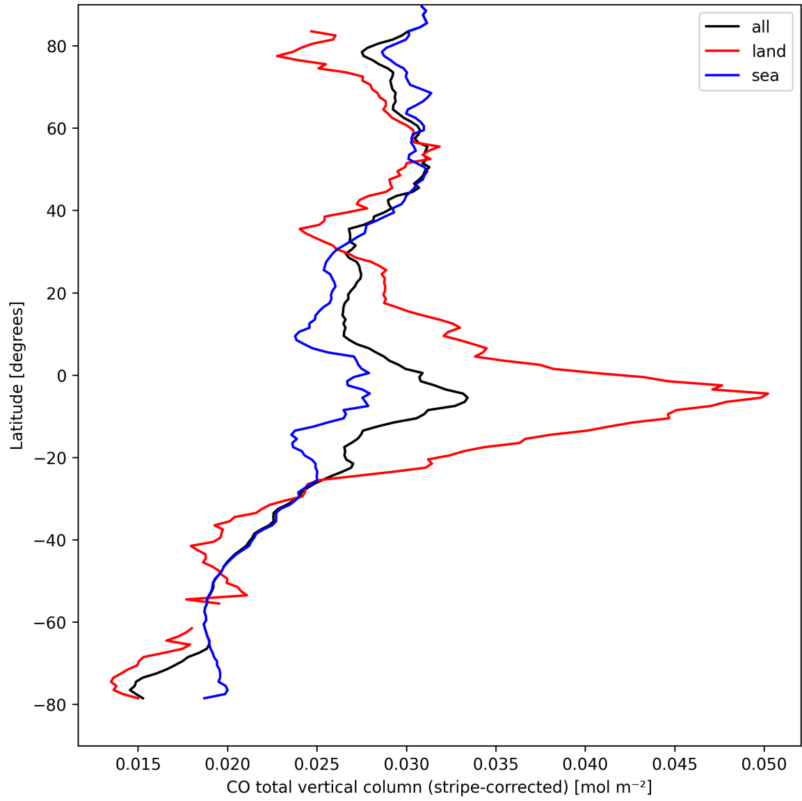
Figure 11: Zonal average of “CO total vertical column (stripe-corrected)” for 2025-09-05 to 2025-09-07.
