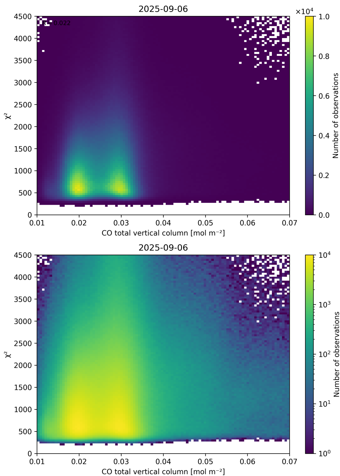
Figure 35: Scatter density plot of “CO total vertical column” against “ \chi^2 ” for 2025-09-05 to 2025-09-07.
