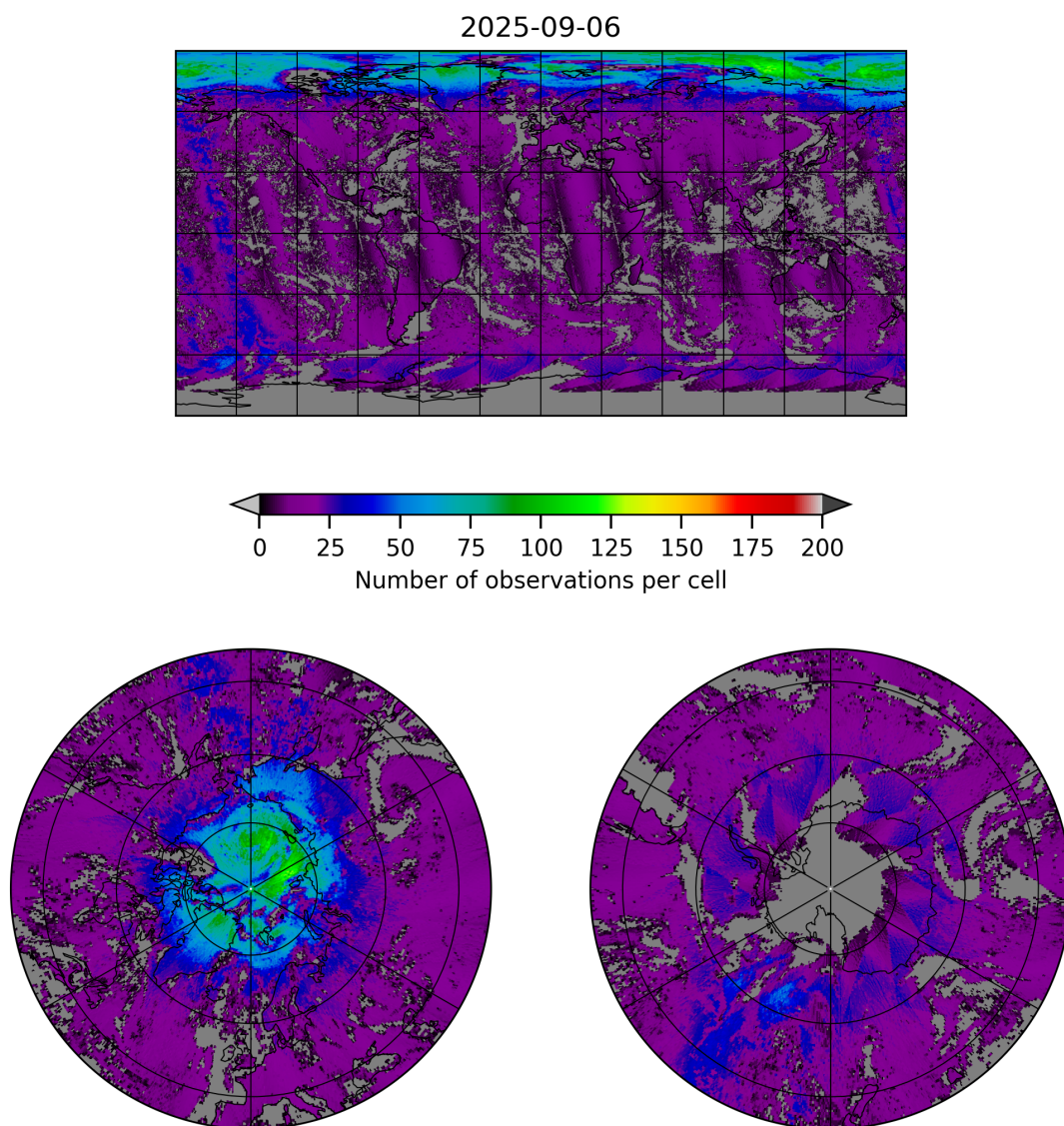
Figure 8: Map of the number of observations for 2025-09-05 to 2025-09-07
