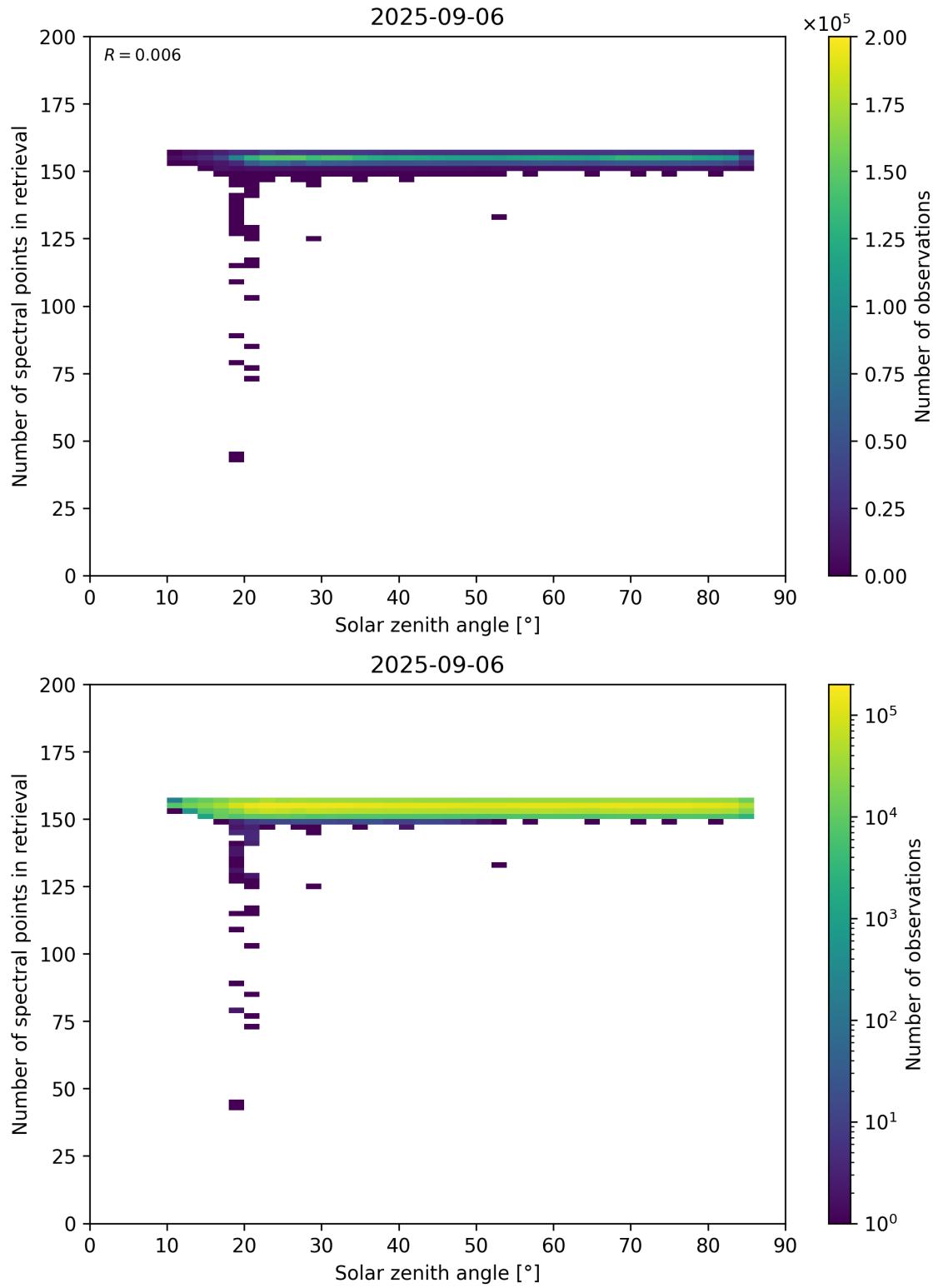
Figure 68: Scatter density plot of “Solar zenith angle” against “Number of spectral points in retrieval” for 2025-09-05 to 2025-09-07.
