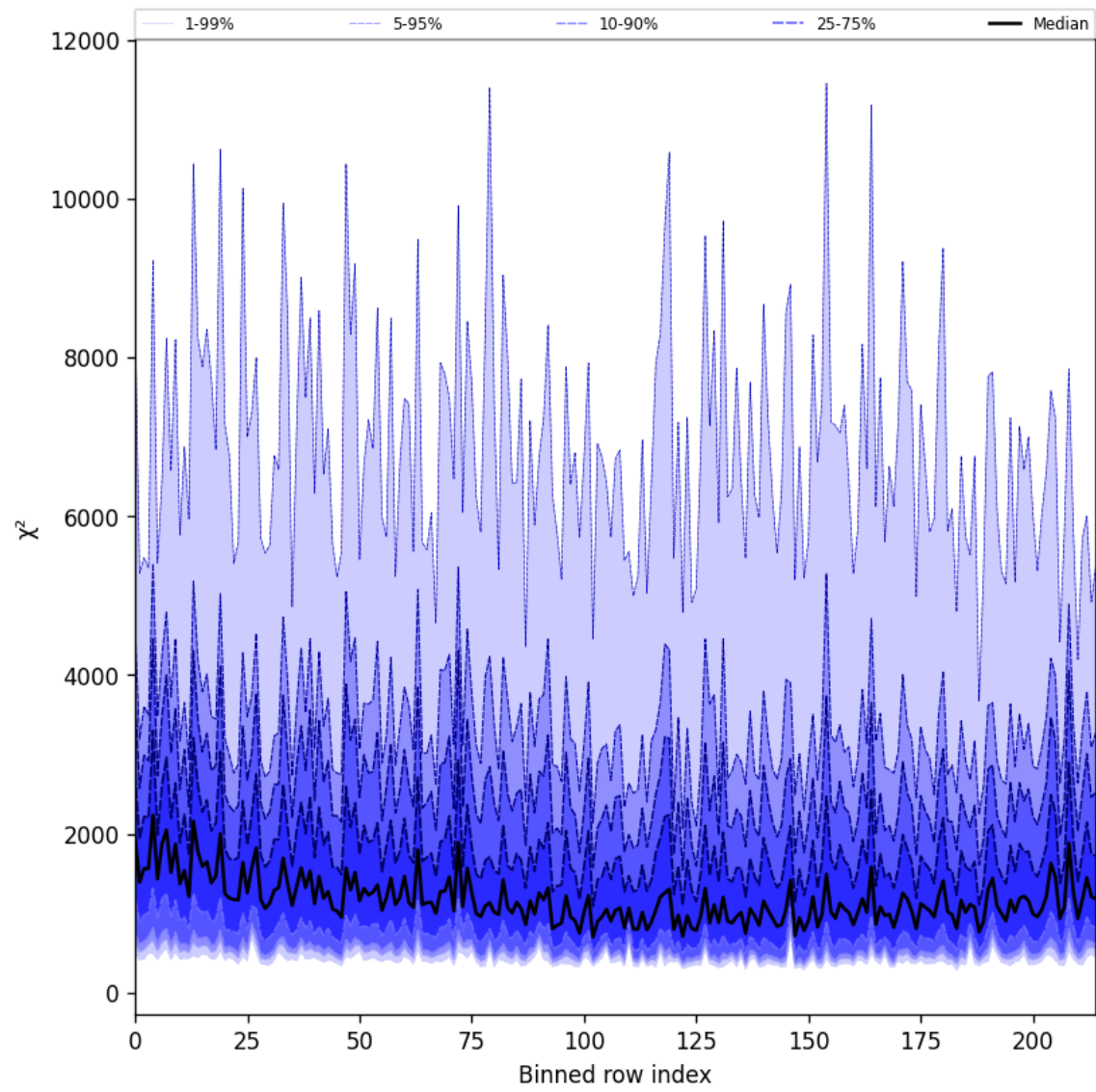
Figure 30: Along track statistics of “ \chi^2 ” for 2025-09-05 to 2025-09-07
