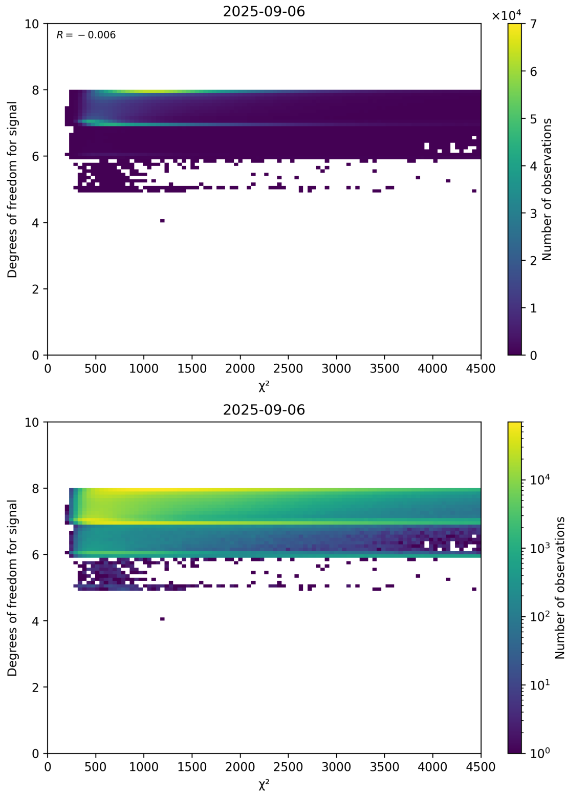
Figure 48: Scatter density plot of “ \chi^2 ” against “Degrees of freedom for signal” for 2025-09-05 to 2025-09-07.
