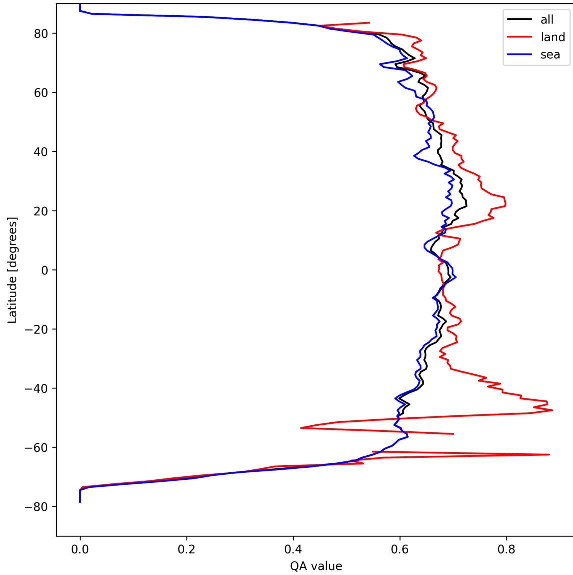
Figure 9: Zonal average of “QA value” for 2025-09-05 to 2025-09-07.
