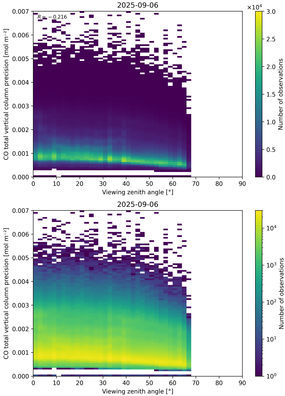
Figure 71: Scatter density plot of “Viewing zenith angle” against “CO total vertical column precision” for 2025-09-05 to 2025-09-07.
