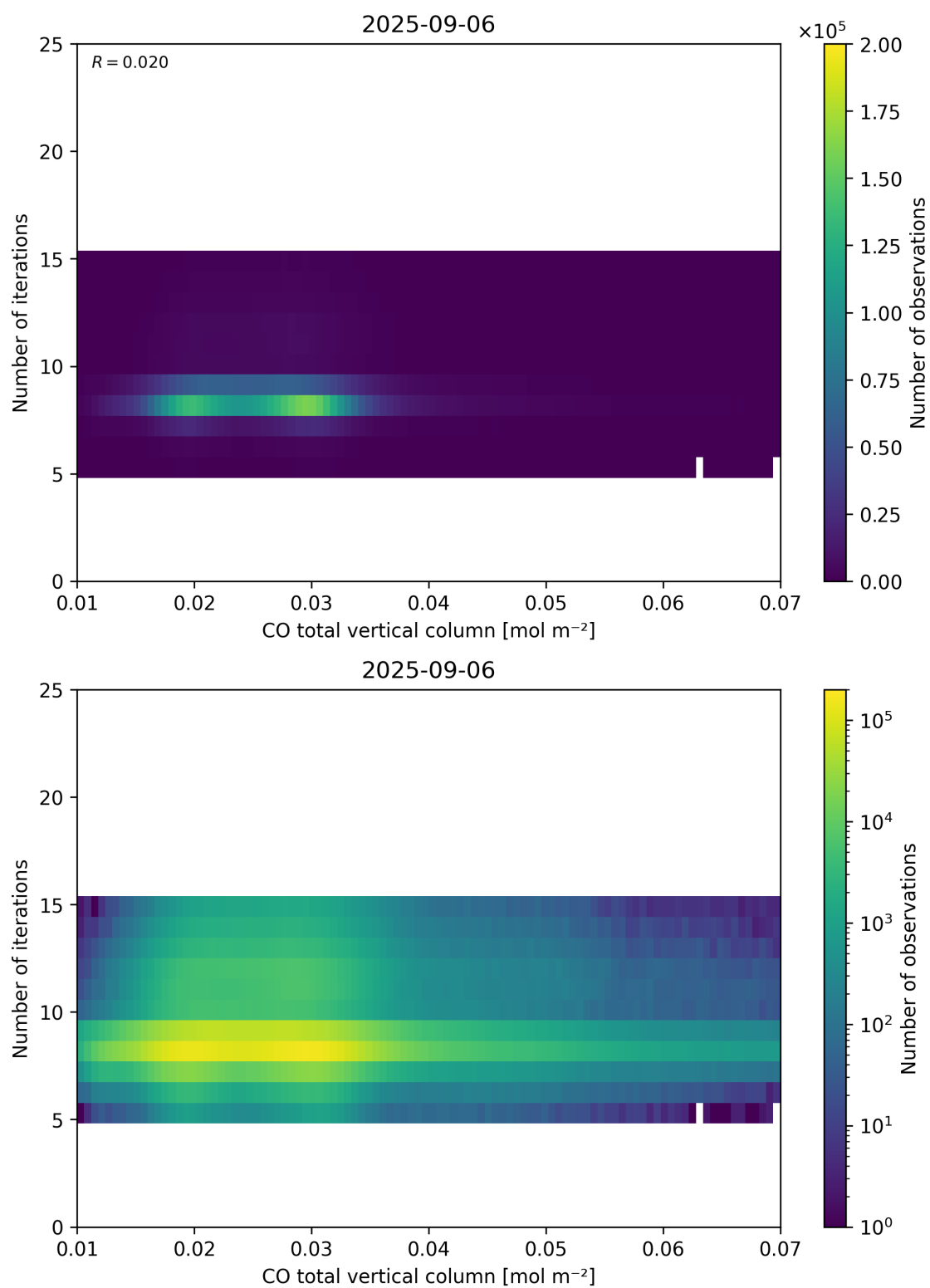
Figure 42: Scatter density plot of “CO total vertical column” against “Number of iterations” for 2025-09-05 to 2025-09-07.
