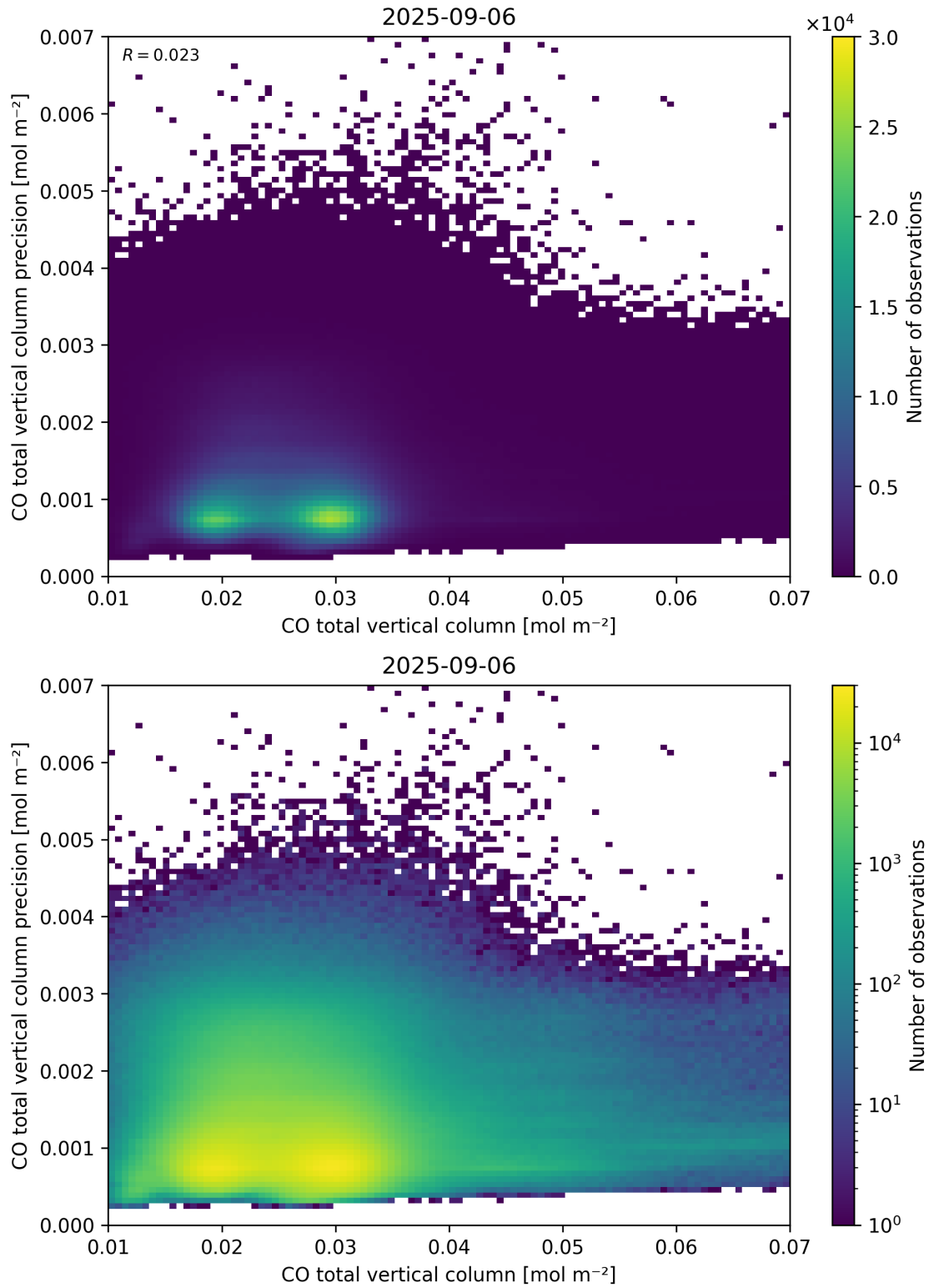
Figure 34: Scatter density plot of “CO total vertical column” against “CO total vertical column precision” for 2025-09-05 to 2025-09-07.
