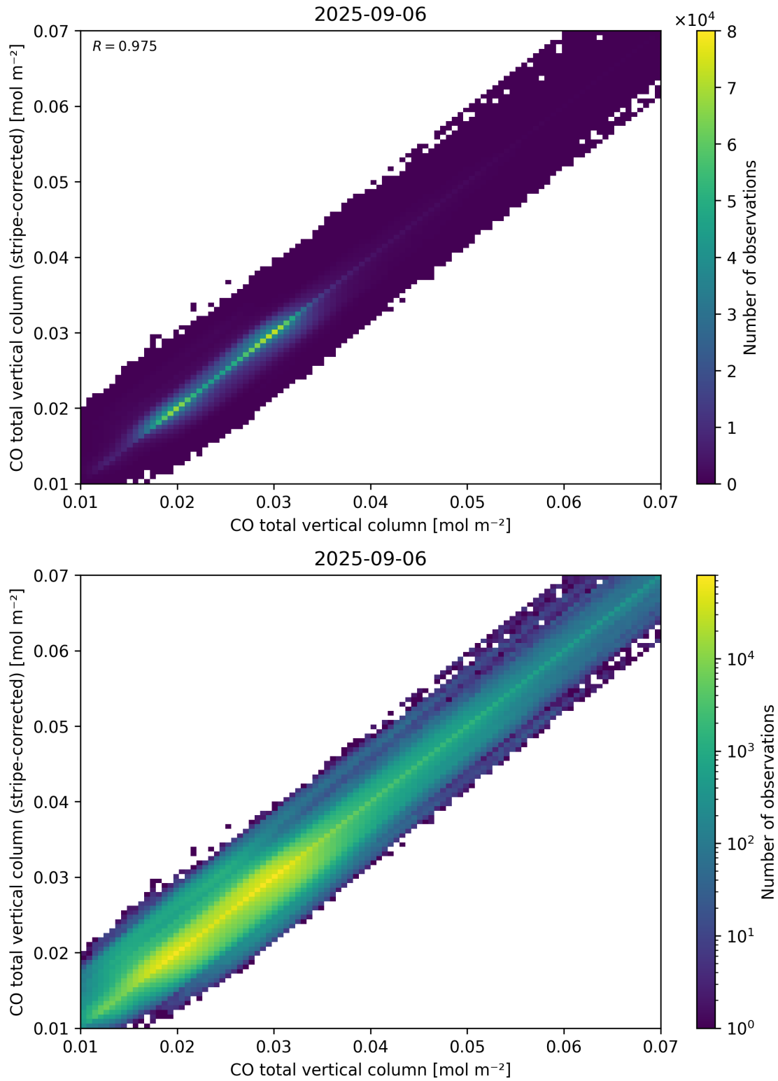
Figure 33: Scatter density plot of “CO total vertical column” against “CO total vertical column (stripe-corrected)” for 2025-09-05 to 2025-09-07.
