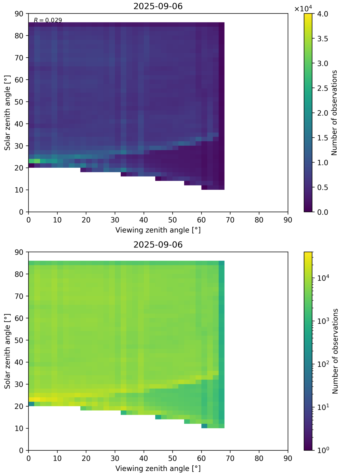
Figure 77: Scatter density plot of “Viewing zenith angle” against “Solar zenith angle” for 2025-09-05 to 2025-09-07.
