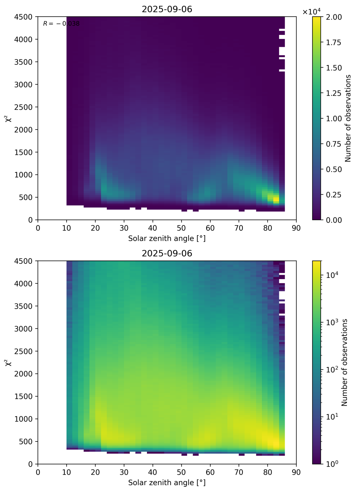
Figure 64: Scatter density plot of “Solar zenith angle” against “ \chi^2 ” for 2025-09-05 to 2025-09-07.
