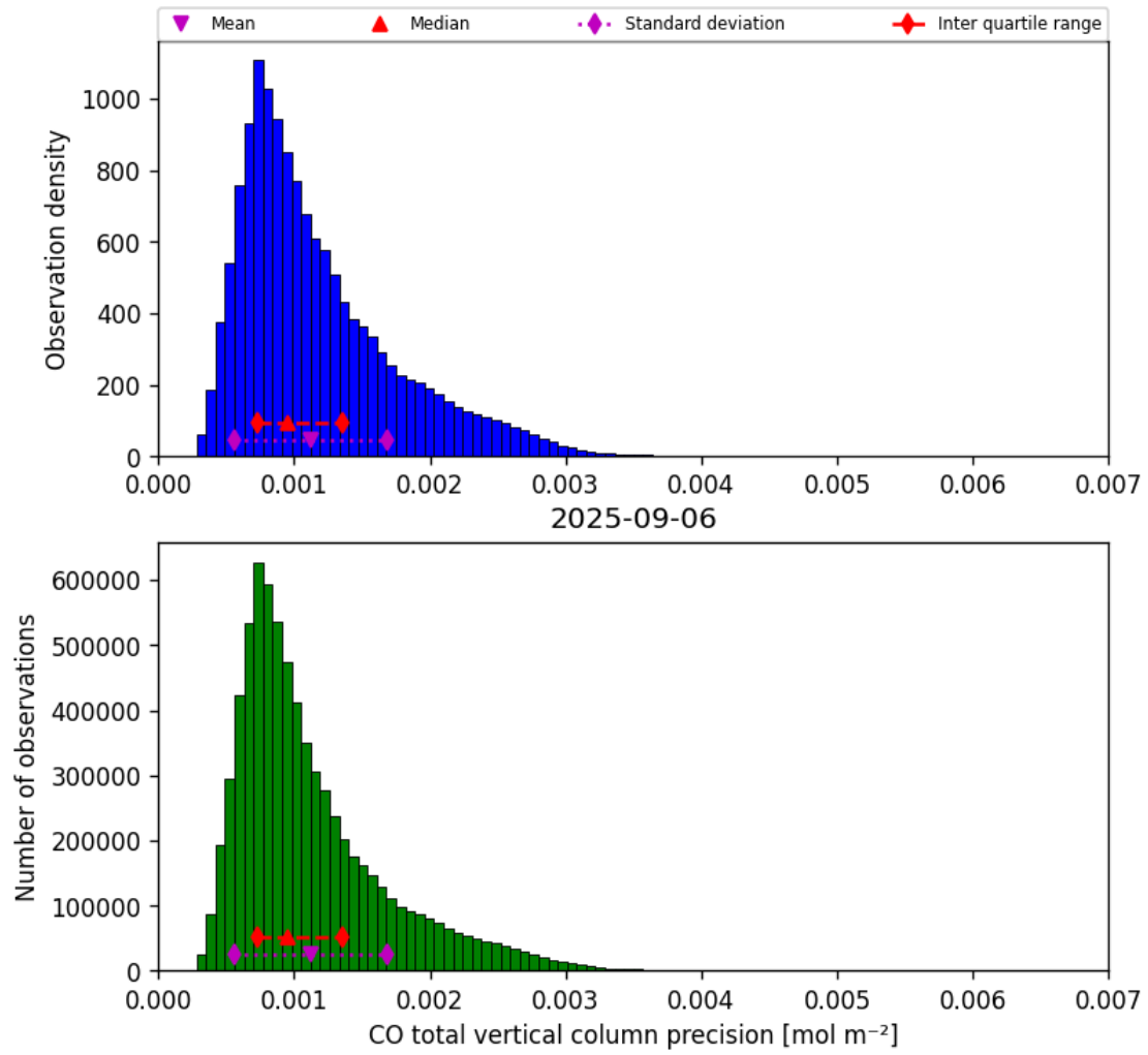
Figure 20: Histogram of “CO total vertical column precision” for 2025-09-05 to 2025-09-07
