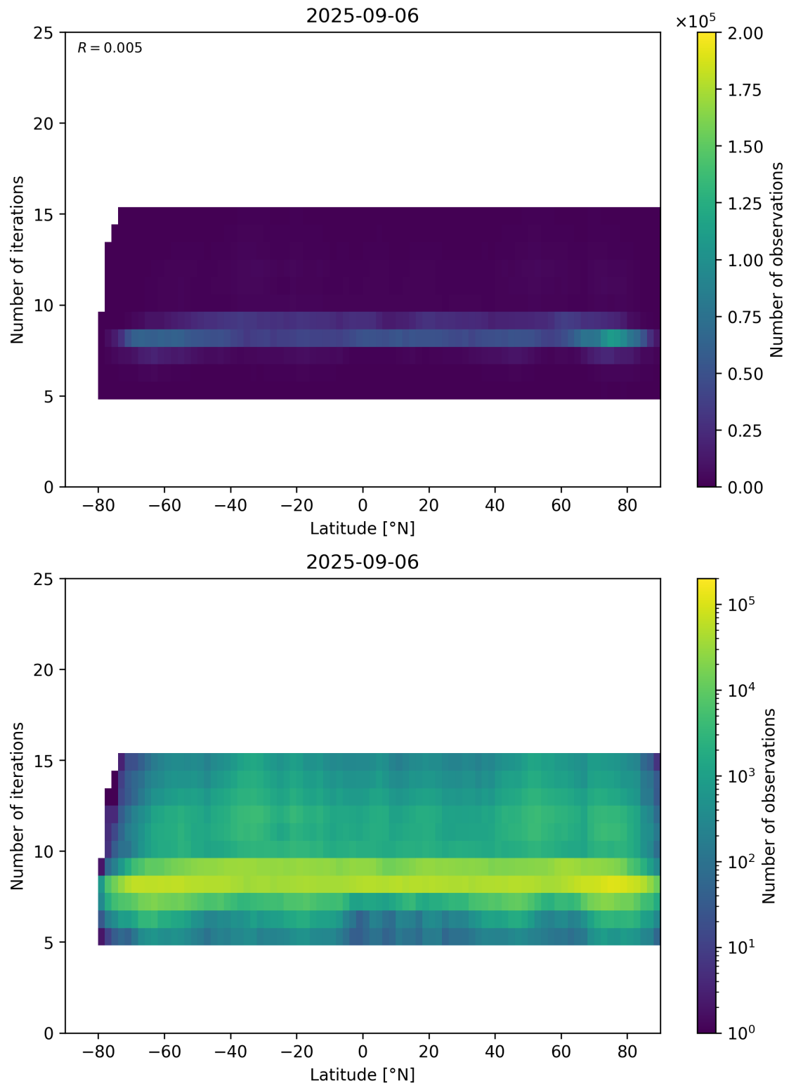
Figure 56: Scatter density plot of “Latitude” against “Number of iterations” for 2025-09-05 to 2025-09-07.
