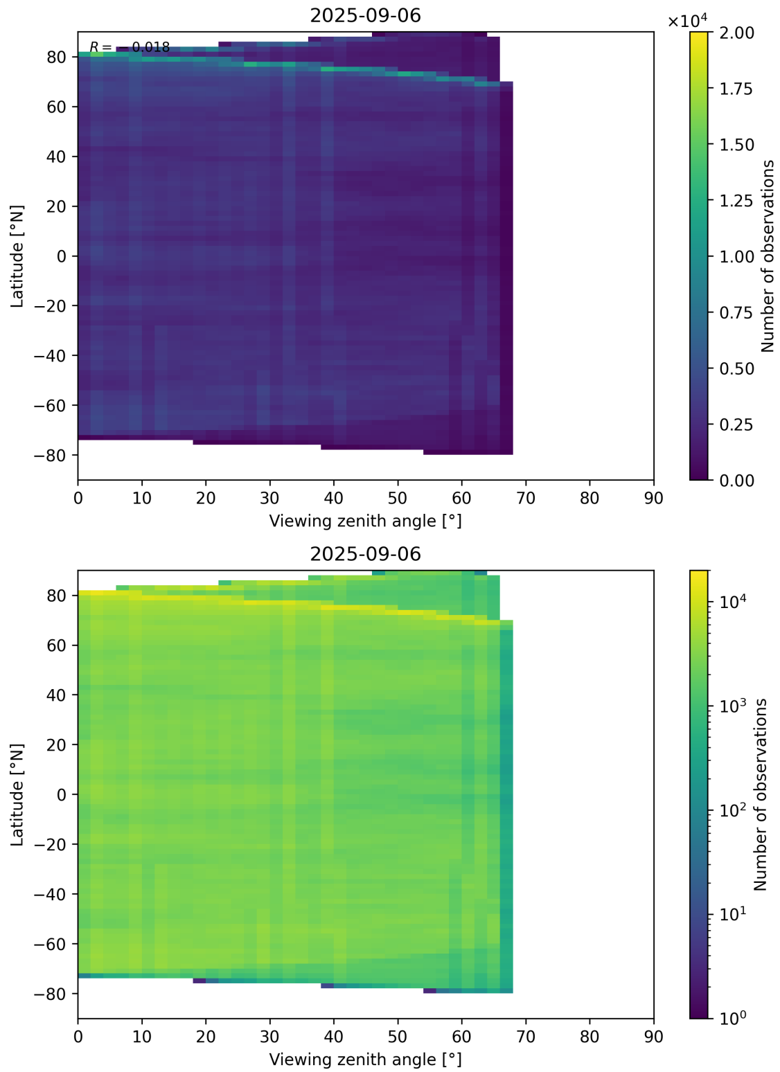
Figure 74: Scatter density plot of “Viewing zenith angle” against “Latitude” for 2025-09-05 to 2025-09-07.
