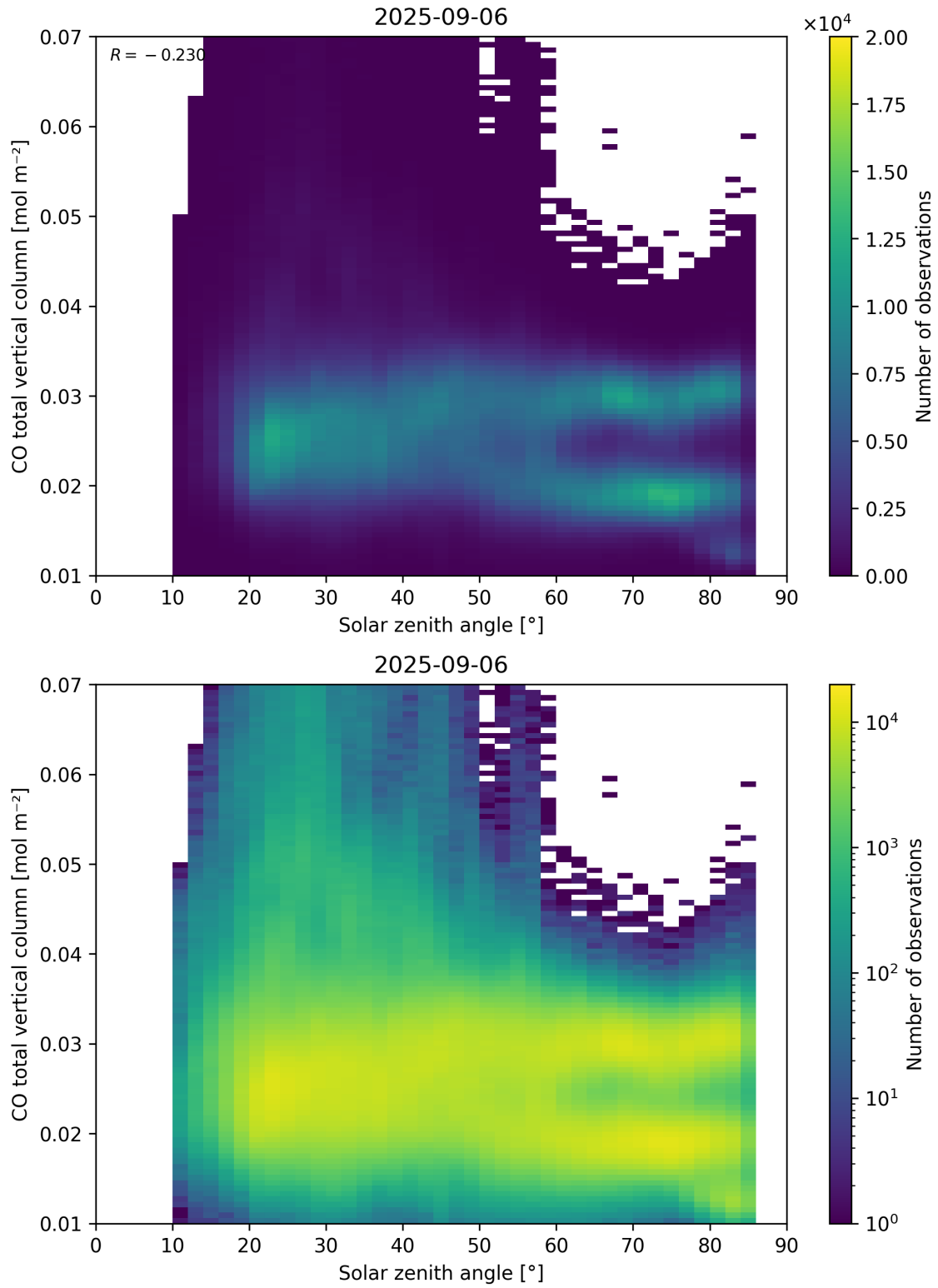
Figure 61: Scatter density plot of “Solar zenith angle” against “CO total vertical column” for 2025-09-05 to 2025-09-07.
