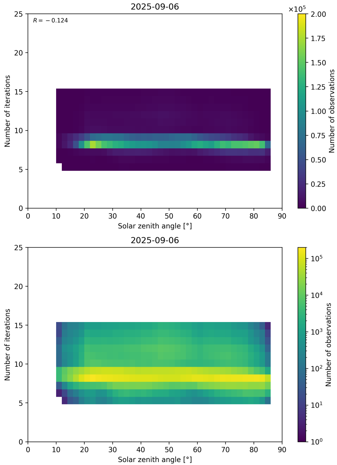
Figure 67: Scatter density plot of “Solar zenith angle” against “Number of iterations” for 2025-09-05 to 2025-09-07.
