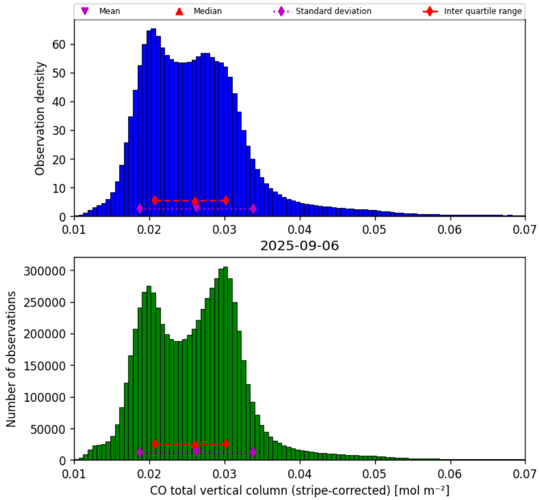
Figure 19: Histogram of “CO total vertical column (stripe-corrected)” for 2025-09-05 to 2025-09-07
