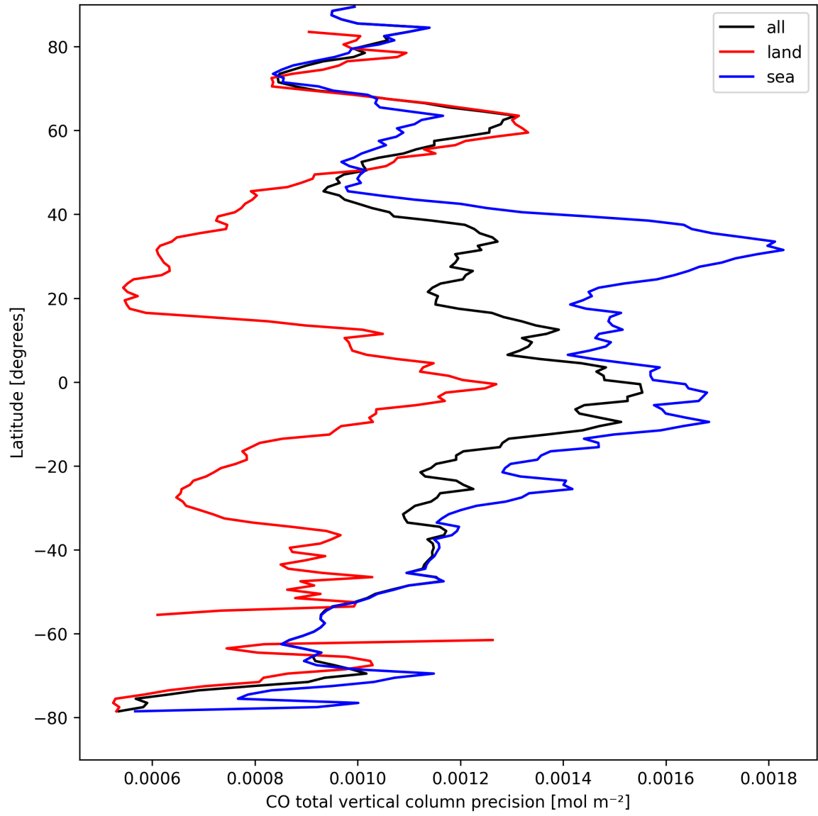
Figure 12: Zonal average of “CO total vertical column precision” for 2025-09-05 to 2025-09-07.
