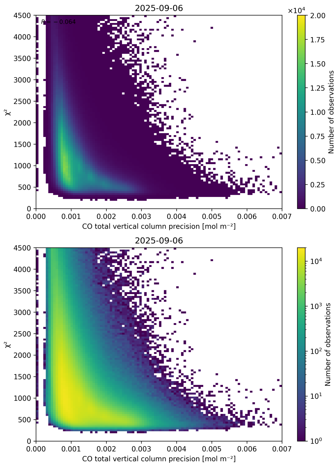
Figure 44: Scatter density plot of “CO total vertical column precision” against “ \chi^2 ” for 2025-09-05 to 2025-09-07.
