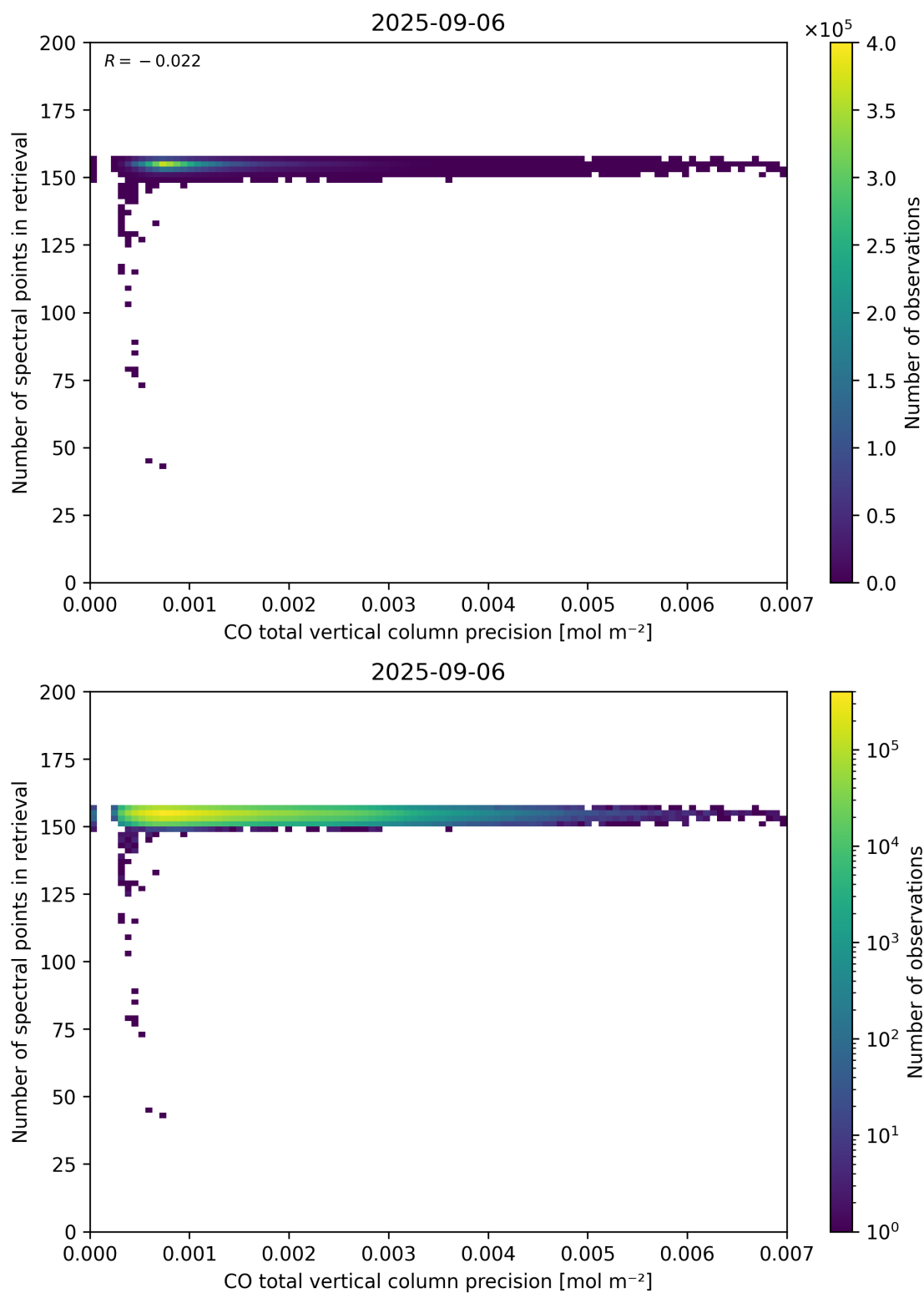
Figure 47: Scatter density plot of “CO total vertical column precision” against “Number of spectral points in retrieval” for 2025-09-05 to 2025-09-07.
