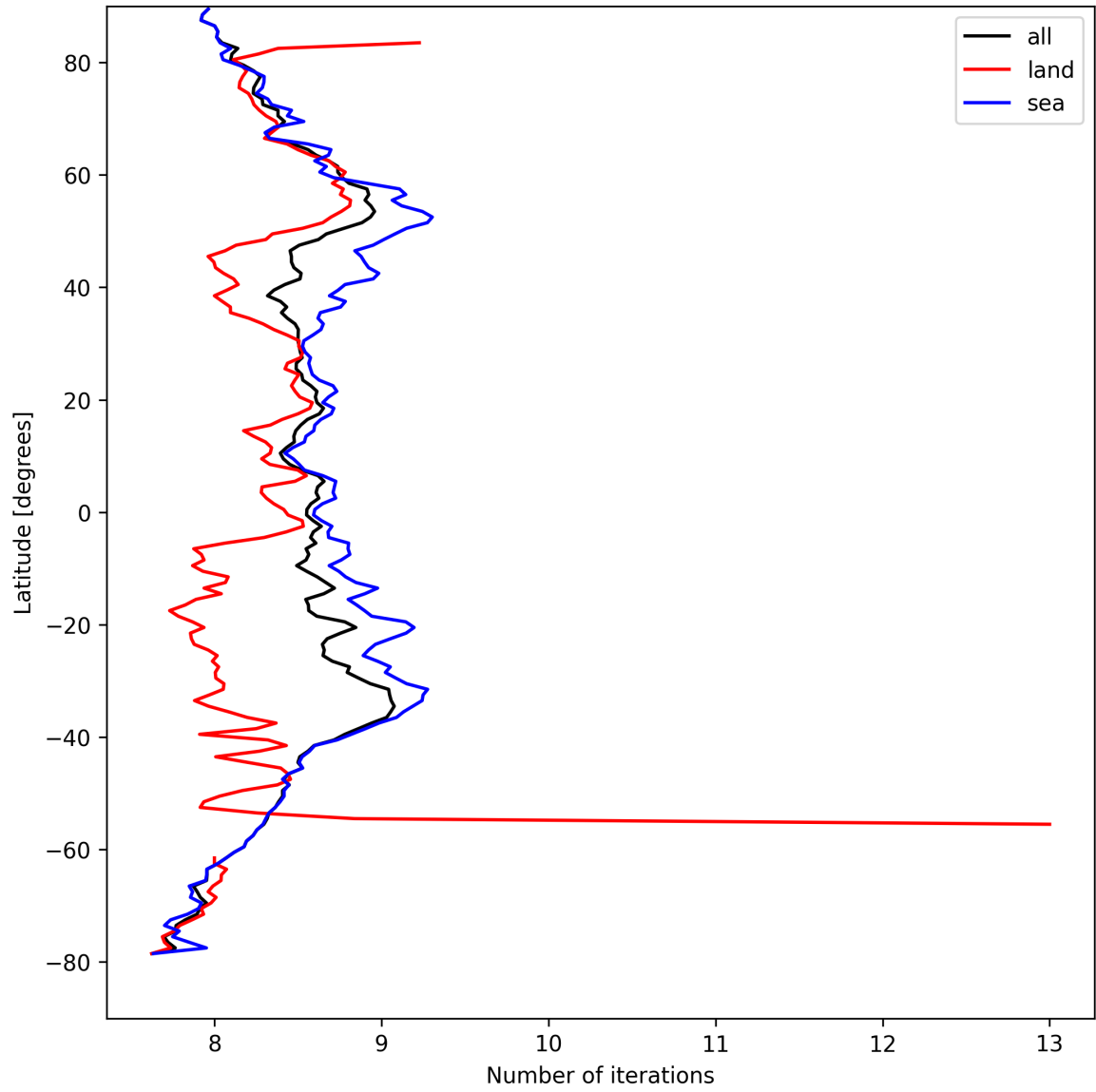
Figure 16: Zonal average of “Number of iterations” for 2025-09-05 to 2025-09-07.
