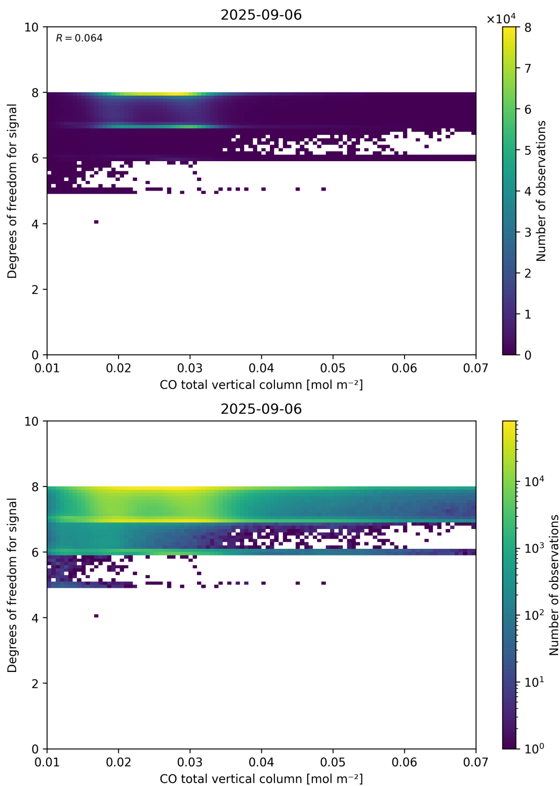
Figure 41: Scatter density plot of “CO total vertical column” against “Degrees of freedom for signal” for 2025-09-05 to 2025-09-07.
