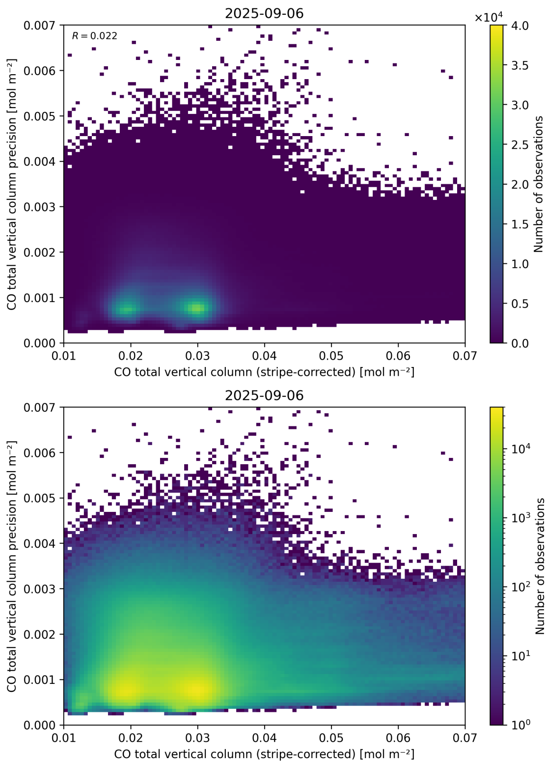
Figure 36: Scatter density plot of “CO total vertical column (stripe-corrected)” against “CO total vertical column precision” for 2025-09-05 to 2025-09-07.
