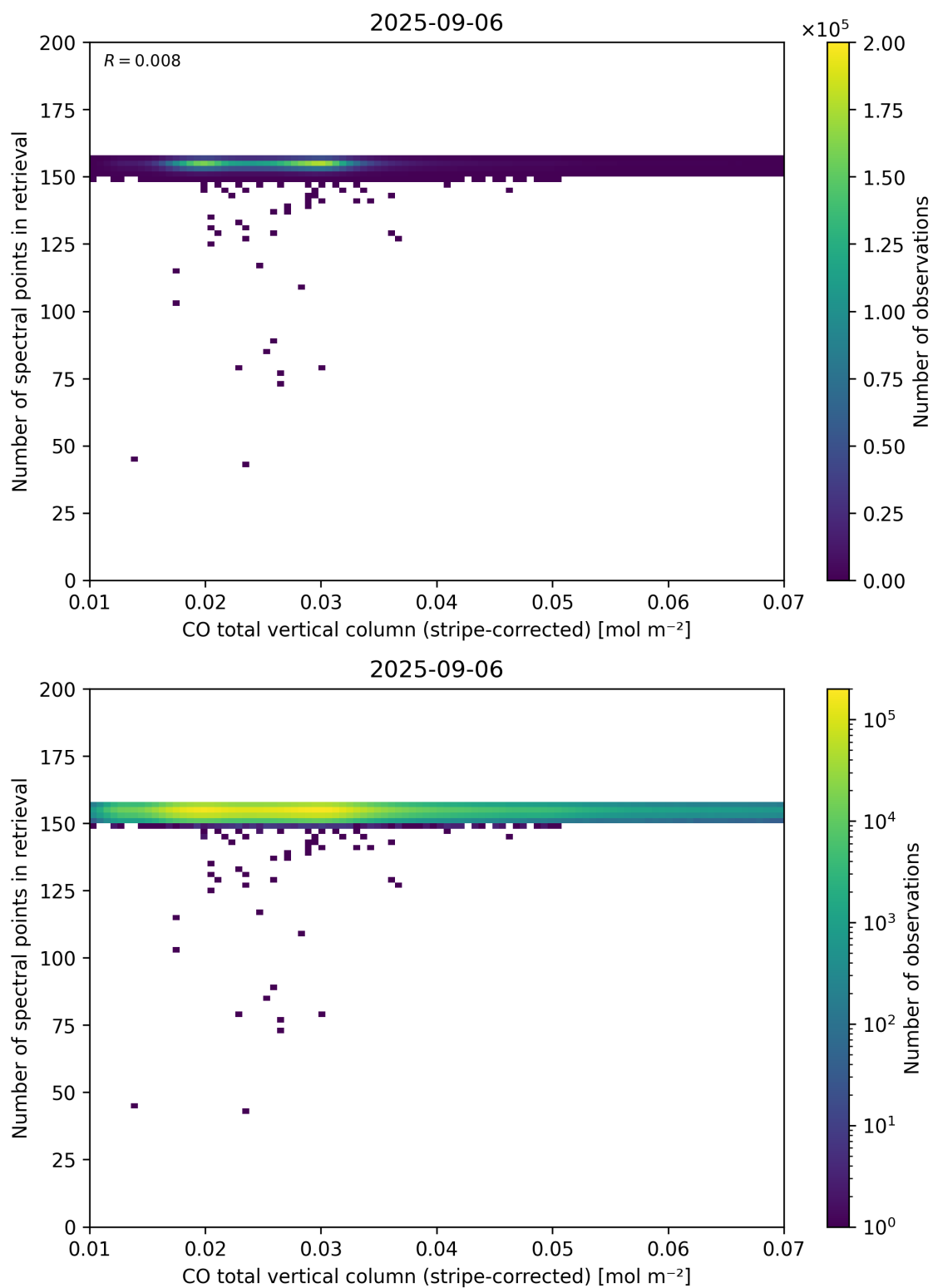
Figure 40: Scatter density plot of “CO total vertical column (stripe-corrected)” against “Number of spectral points in retrieval” for 2025-09-05 to 2025-09-07.
