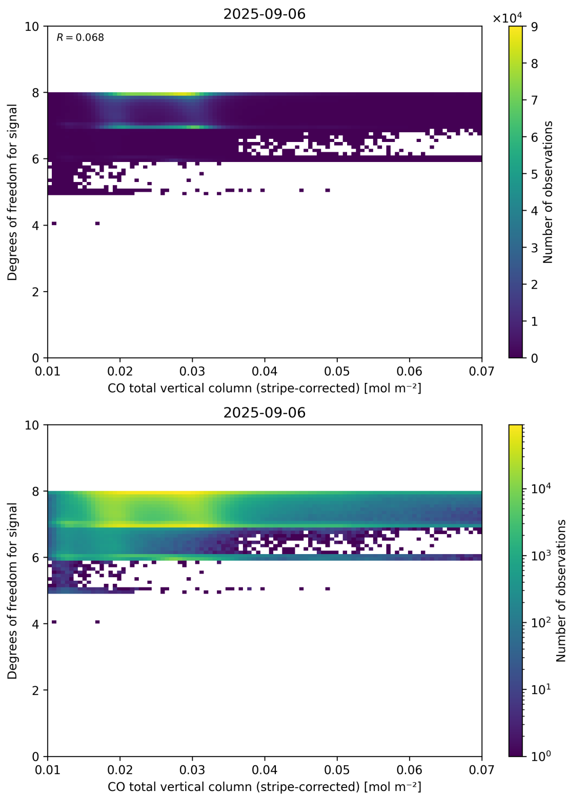
Figure 38: Scatter density plot of “CO total vertical column (stripe-corrected)” against “Degrees of freedom for signal” for 2025-09-05 to 2025-09-07.
