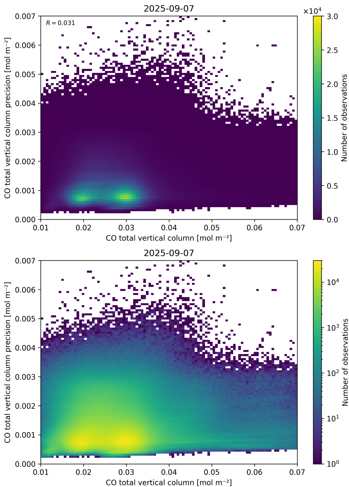
Figure 34: Scatter density plot of “CO total vertical column” against “CO total vertical column precision” for 2025-09-06 to 2025-09-08.
