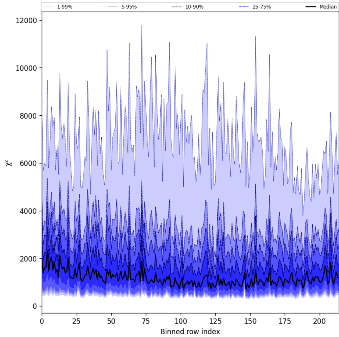
Figure 30: Along track statistics of “ \chi^2 ” for 2025-09-06 to 2025-09-08
