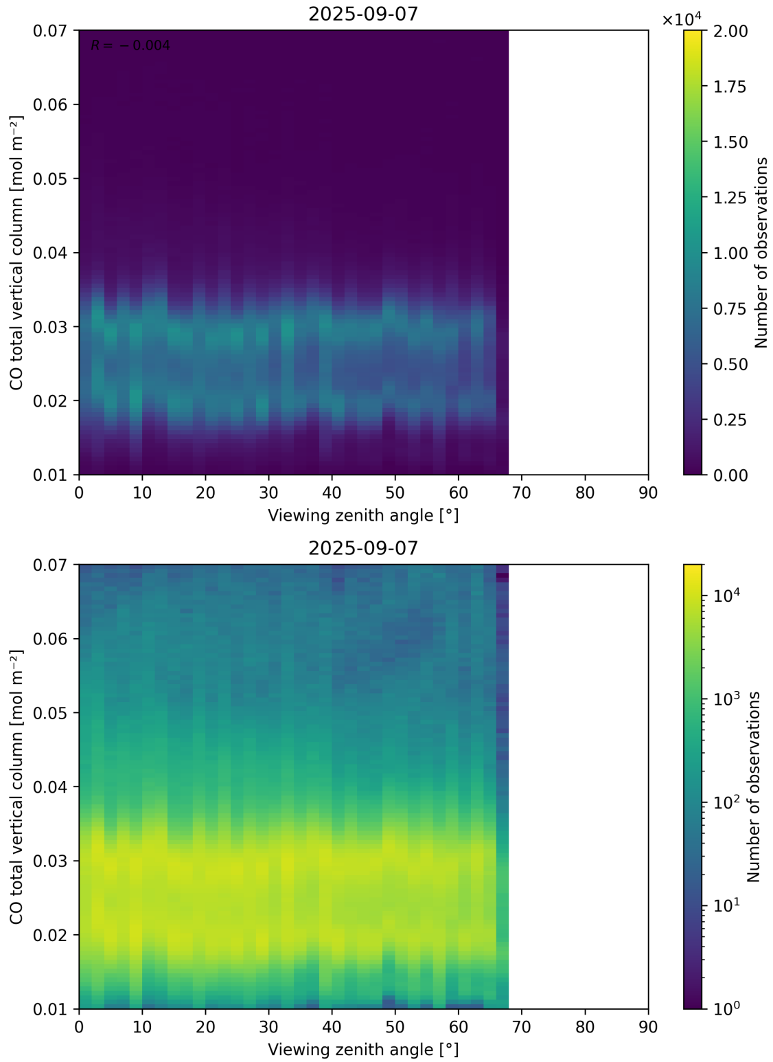
Figure 69: Scatter density plot of “Viewing zenith angle” against “CO total vertical column” for 2025-09-06 to 2025-09-08.
