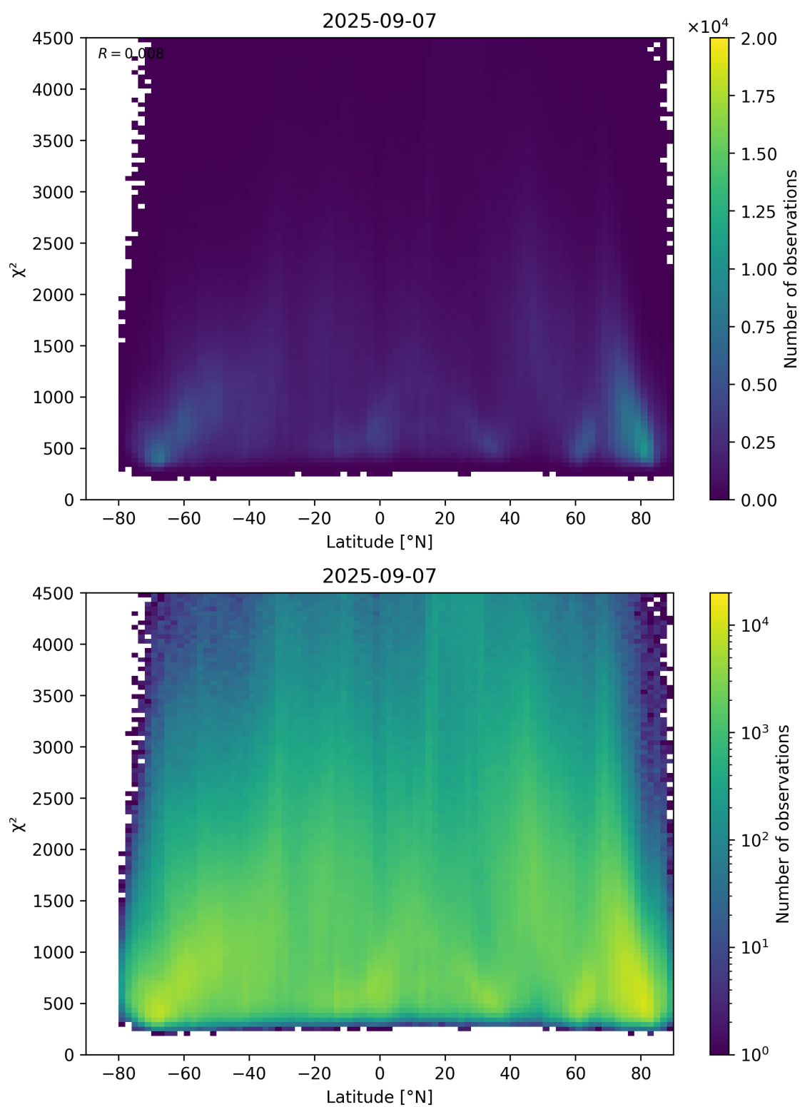
Figure 54: Scatter density plot of “Latitude” against “ \chi^2 ” for 2025-09-06 to 2025-09-08.
