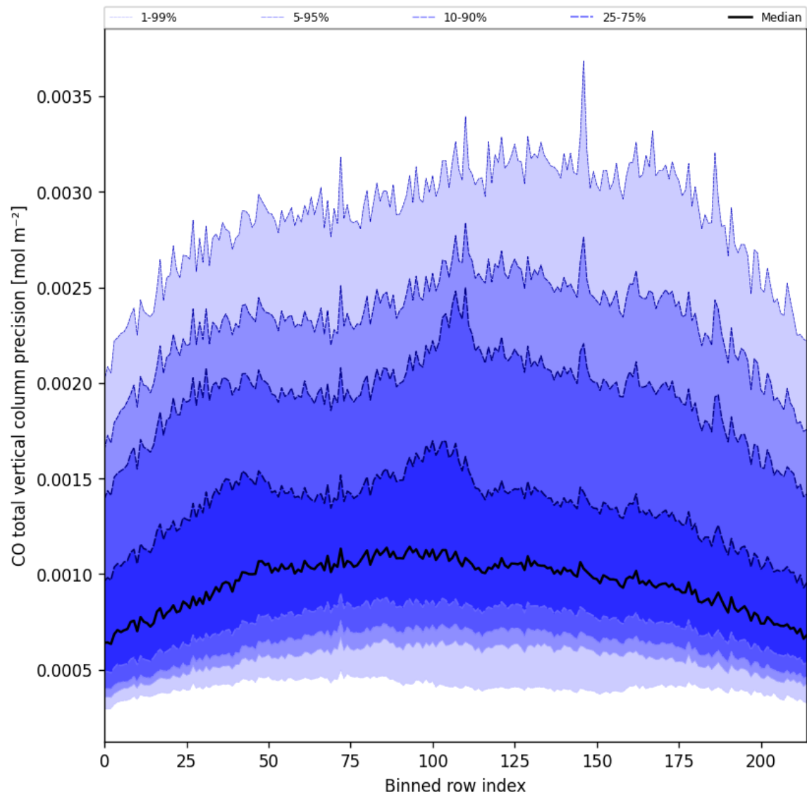
Figure 28: Along track statistics of “CO total vertical column precision” for 2025-09-06 to 2025-09-08
