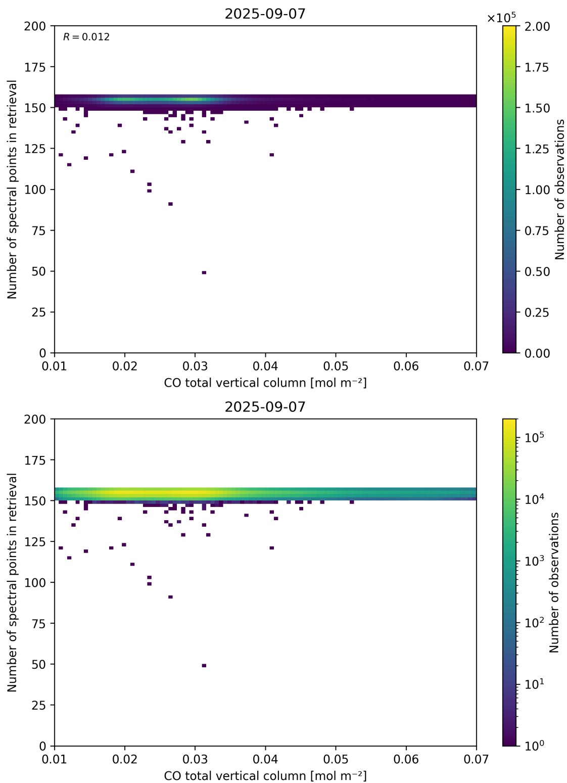
Figure 43: Scatter density plot of “CO total vertical column” against “Number of spectral points in retrieval” for 2025-09-06 to 2025-09-08.
