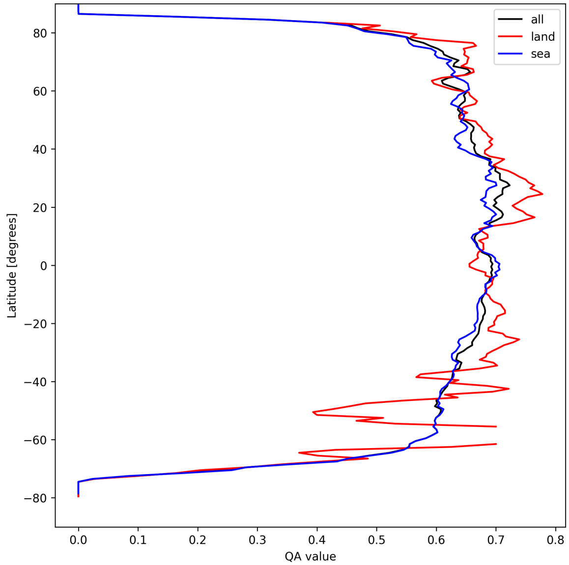
Figure 9: Zonal average of “QA value” for 2025-09-06 to 2025-09-08.
