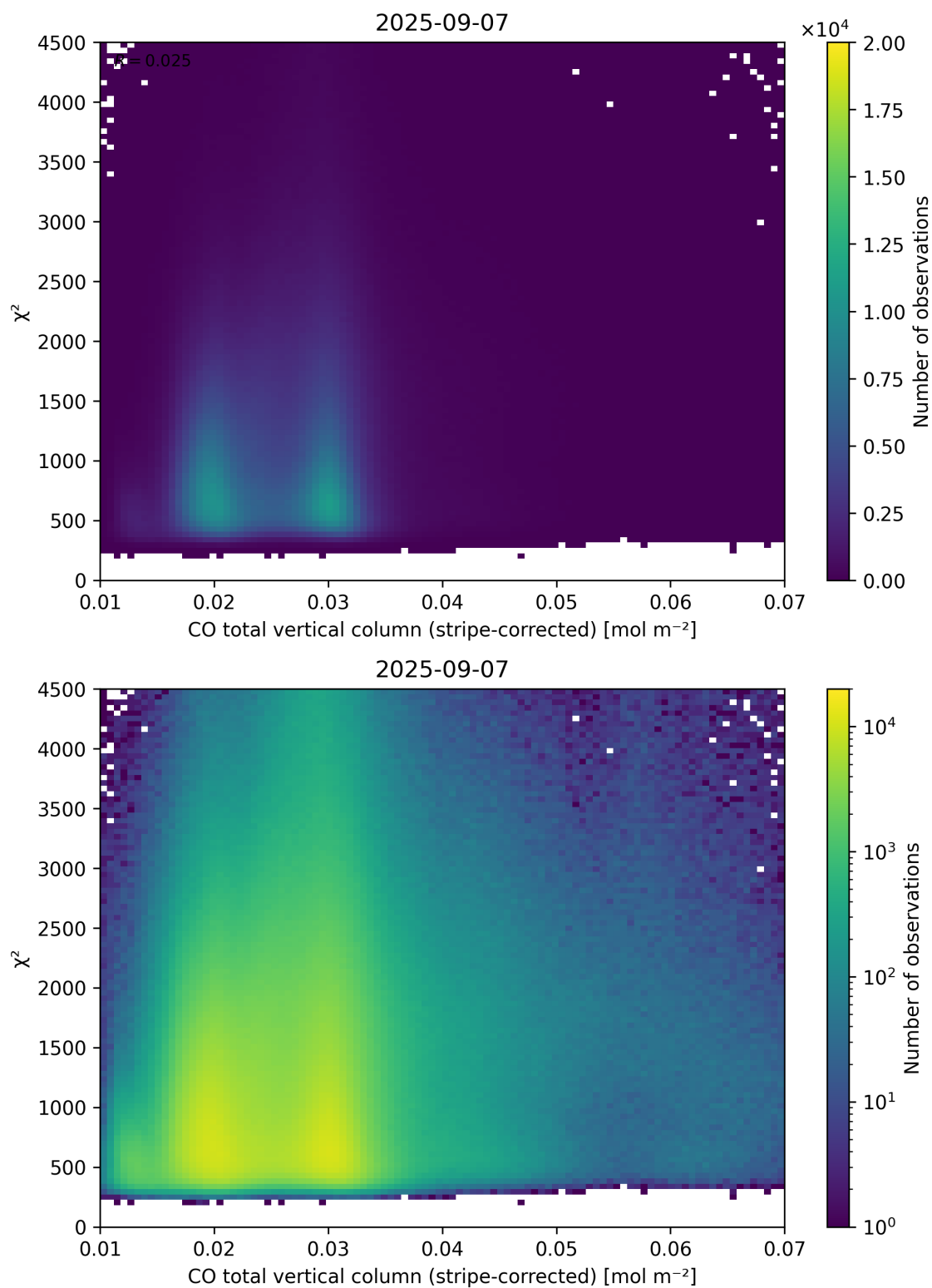
Figure 37: Scatter density plot of “CO total vertical column (stripe-corrected)” against “ \chi^2 ” for 2025-09-06 to 2025-09-08.
