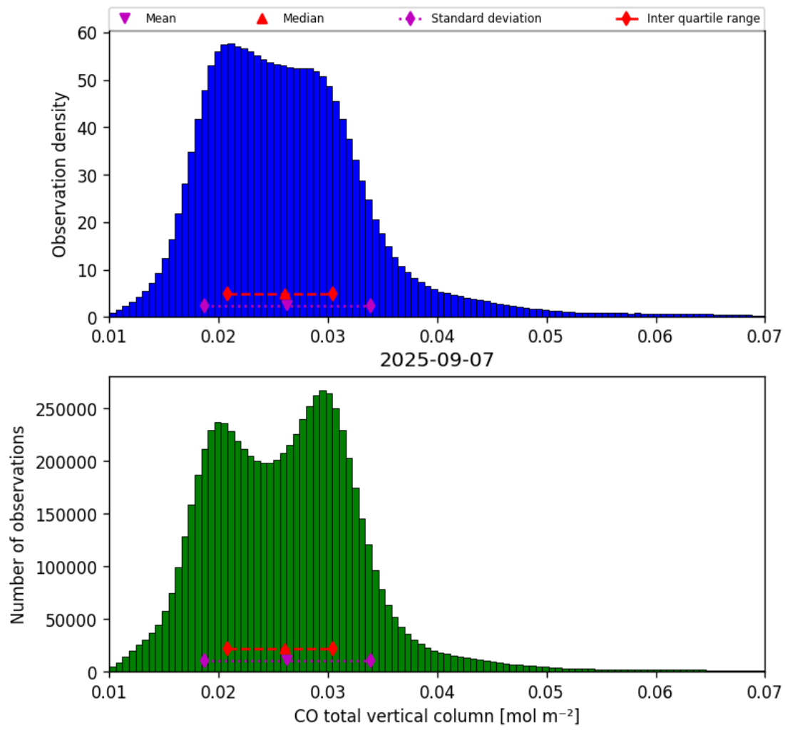
Figure 18: Histogram of “CO total vertical column” for 2025-09-06 to 2025-09-08
