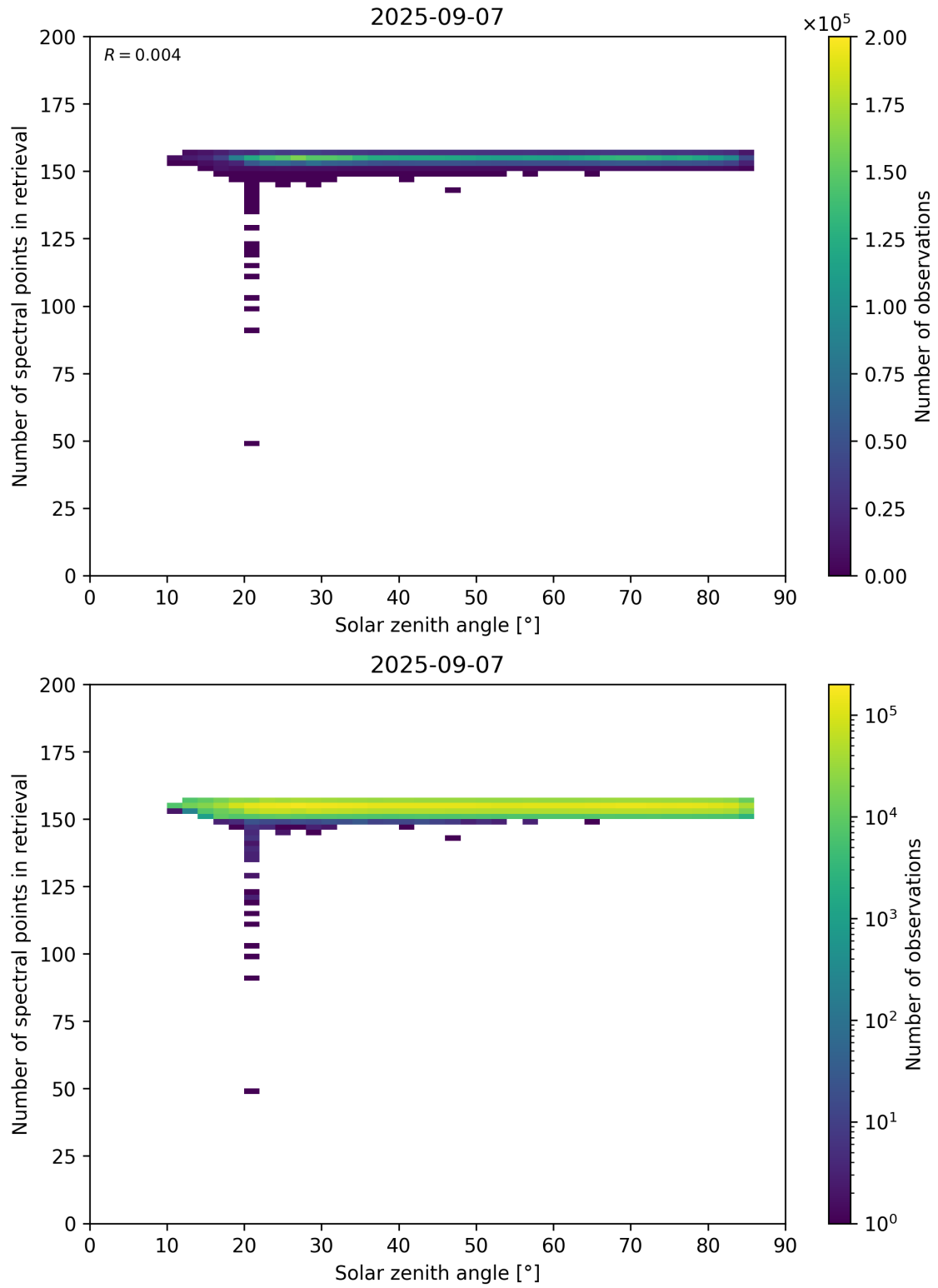
Figure 68: Scatter density plot of “Solar zenith angle” against “Number of spectral points in retrieval” for 2025-09-06 to 2025-09-08.
