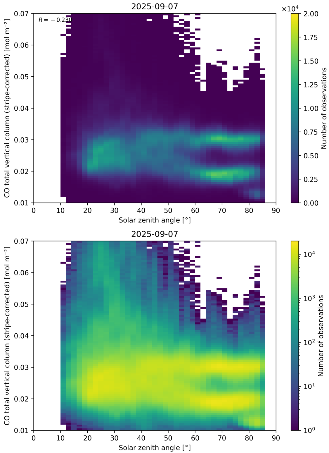
Figure 62: Scatter density plot of “Solar zenith angle” against “CO total vertical column (stripe-corrected)” for 2025-09-06 to 2025-09-08.
