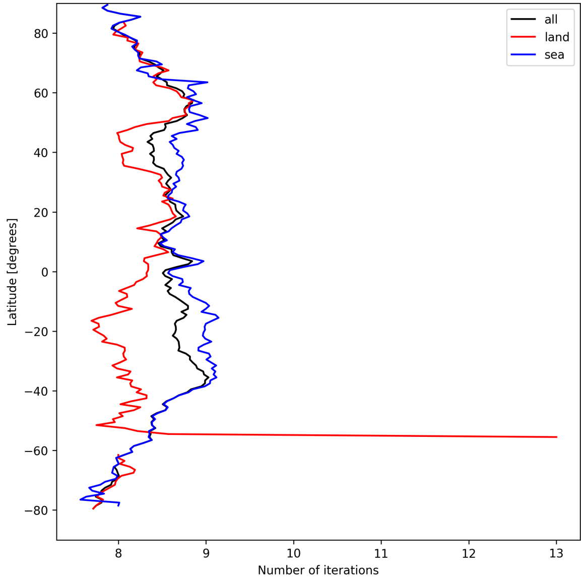
Figure 16: Zonal average of “Number of iterations” for 2025-09-06 to 2025-09-08.
