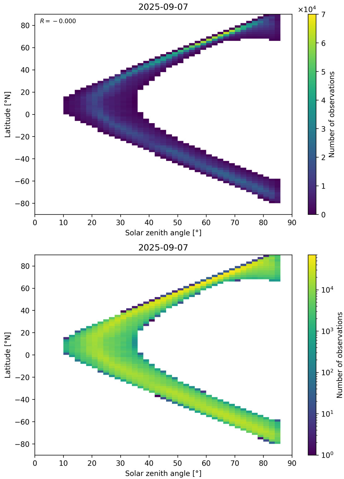
Figure 66: Scatter density plot of “Solar zenith angle” against “Latitude” for 2025-09-06 to 2025-09-08.
