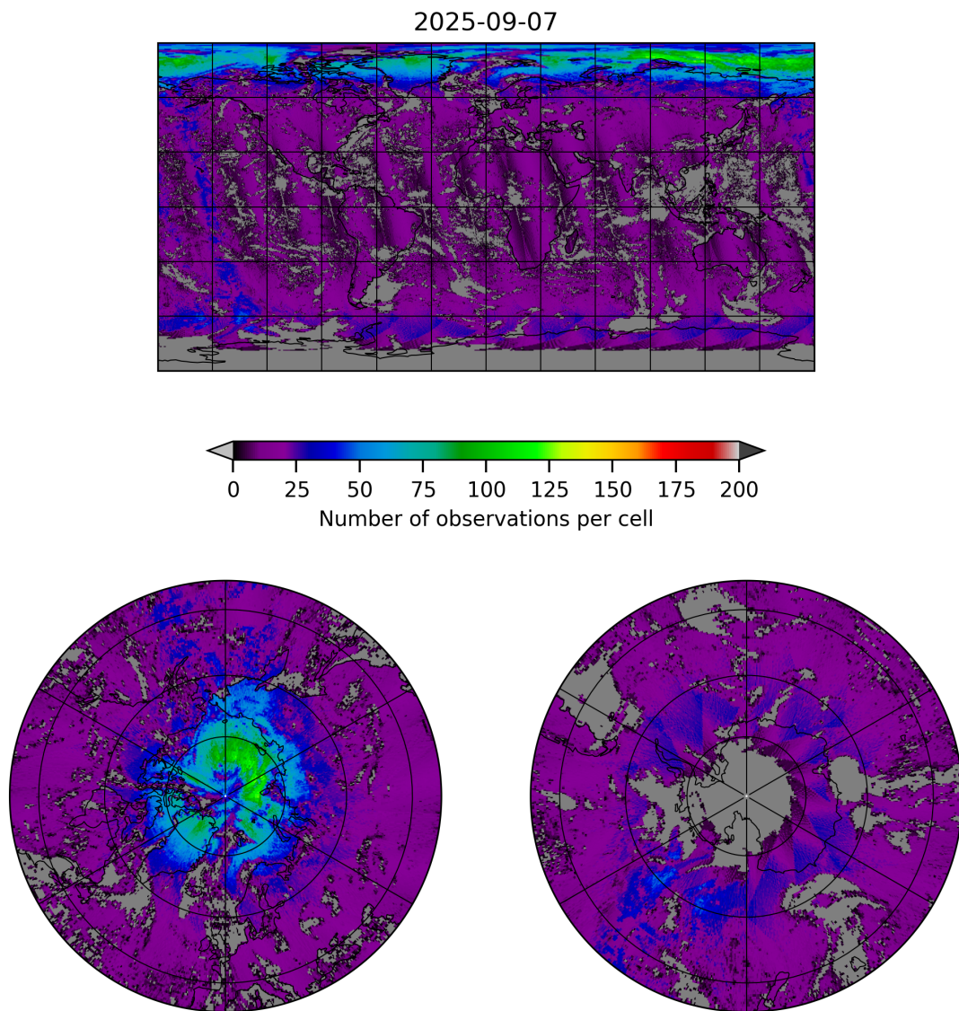
Figure 8: Map of the number of observations for 2025-09-06 to 2025-09-08
