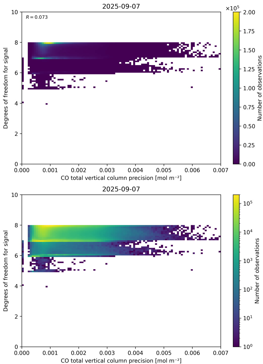
Figure 45: Scatter density plot of “CO total vertical column precision” against “Degrees of freedom for signal” for 2025-09-06 to 2025-09-08.
