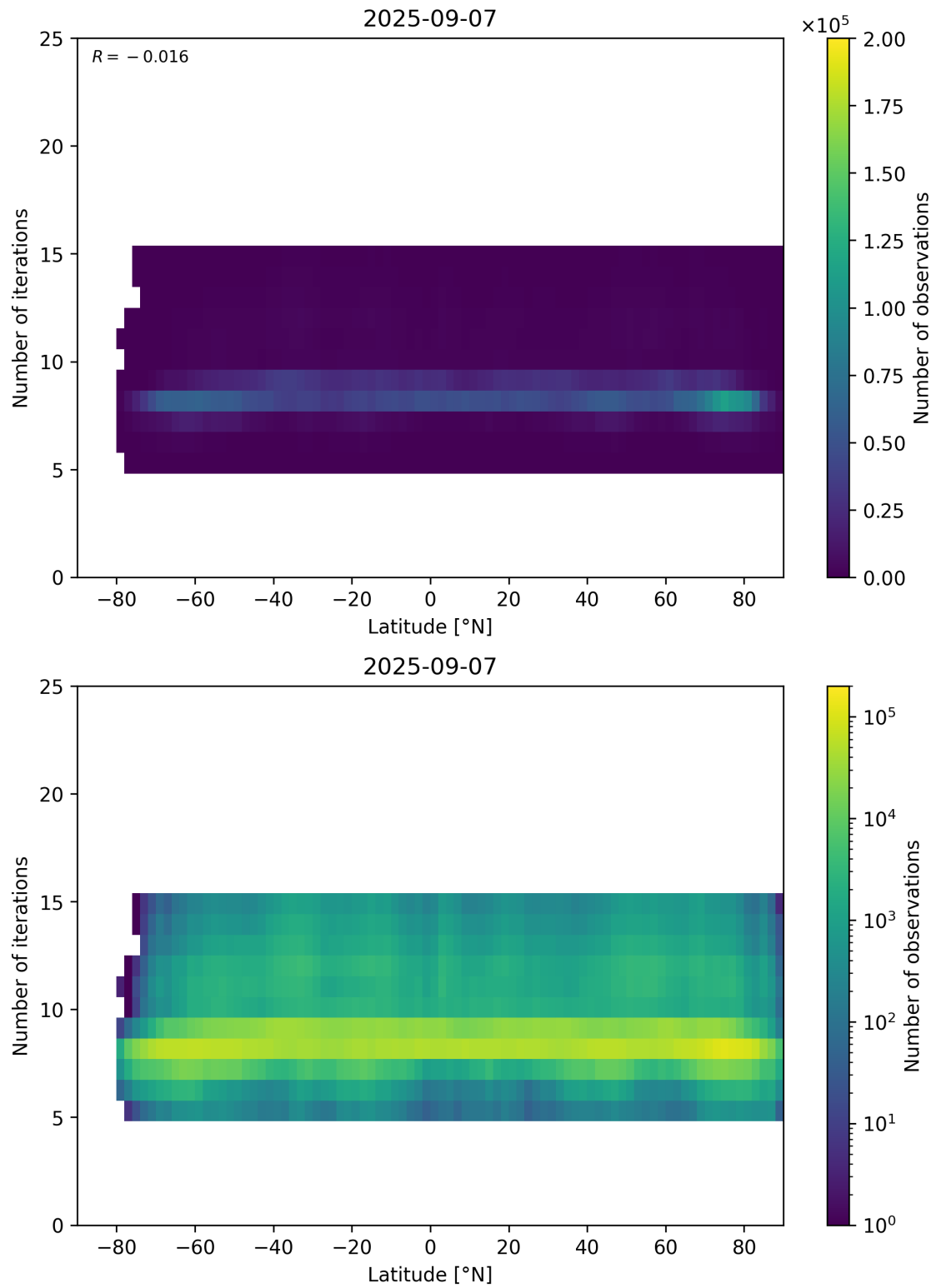
Figure 56: Scatter density plot of “Latitude” against “Number of iterations” for 2025-09-06 to 2025-09-08.
