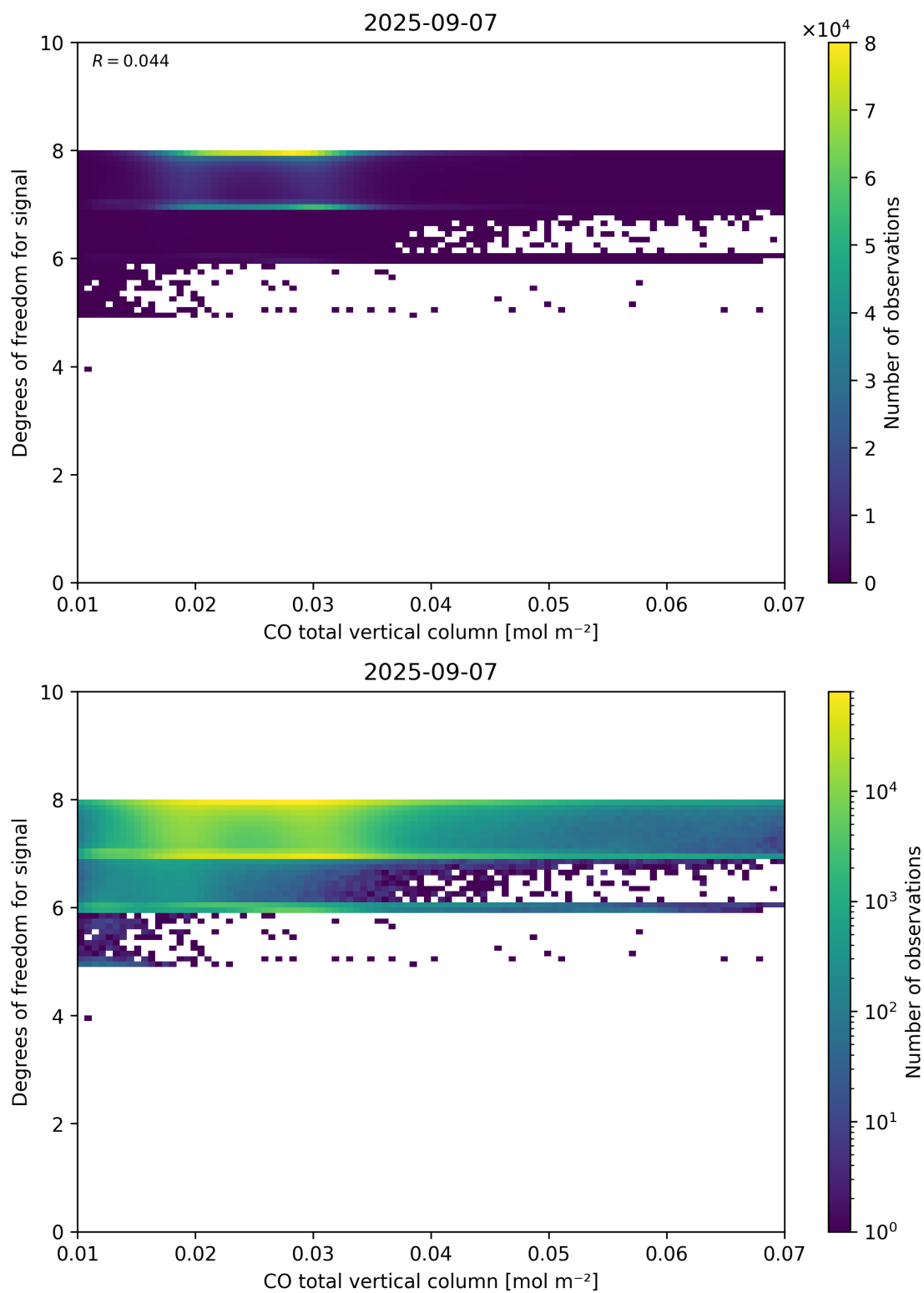
Figure 41: Scatter density plot of “CO total vertical column” against “Degrees of freedom for signal” for 2025-09-06 to 2025-09-08.
