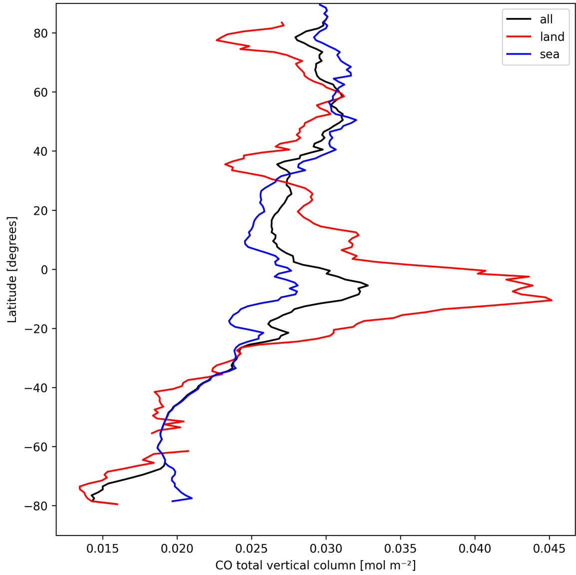
Figure 10: Zonal average of “CO total vertical column” for 2025-09-06 to 2025-09-08.
