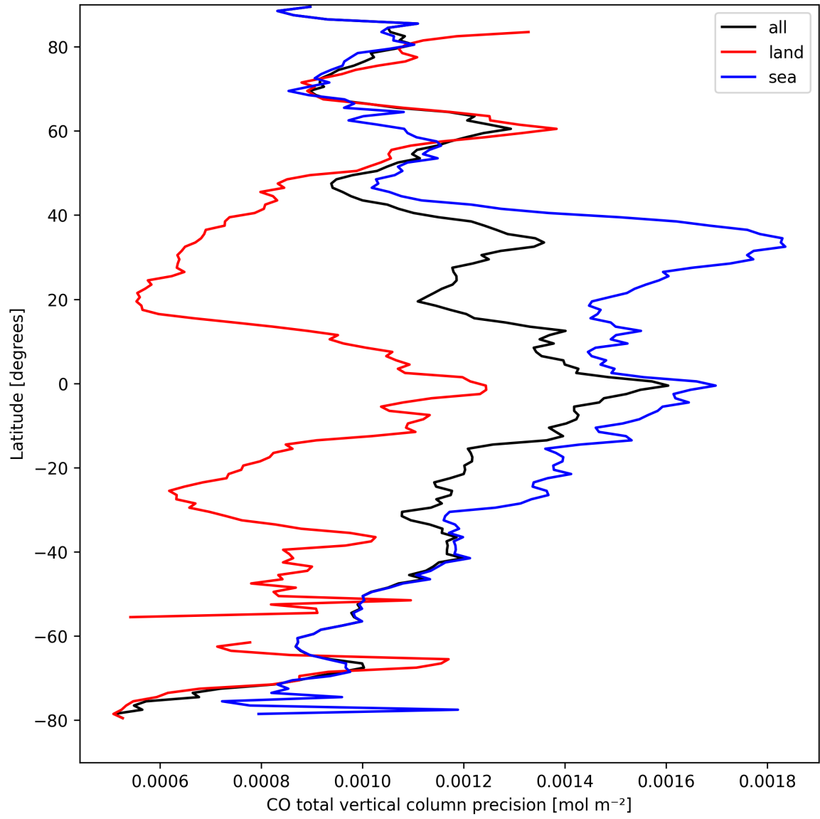
Figure 12: Zonal average of “CO total vertical column precision” for 2025-09-06 to 2025-09-08.
