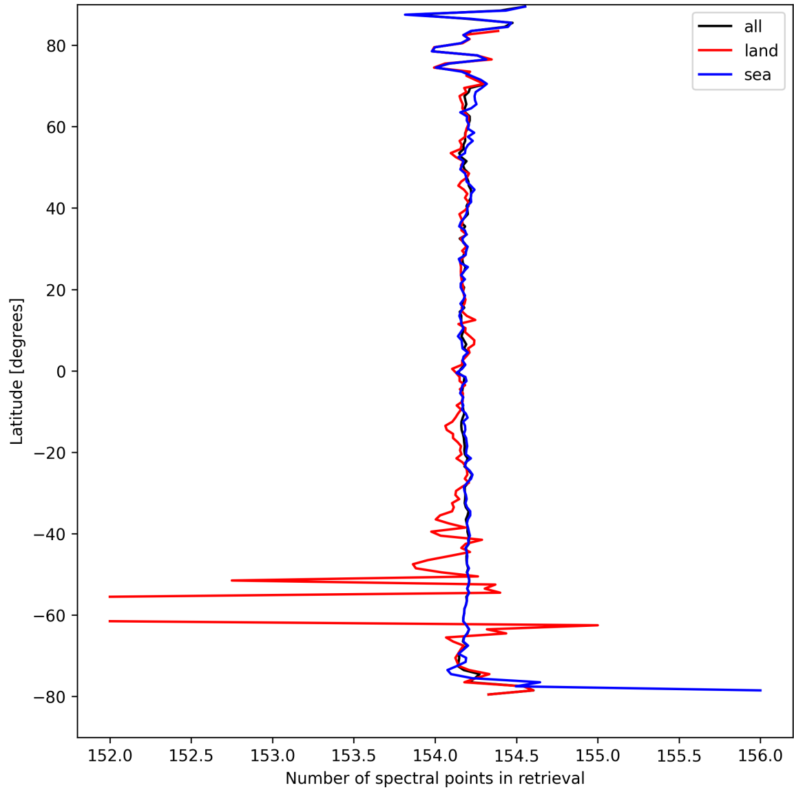
Figure 13: Zonal average of “Number of spectral points in retrieval” for 2025-09-06 to 2025-09-08.
