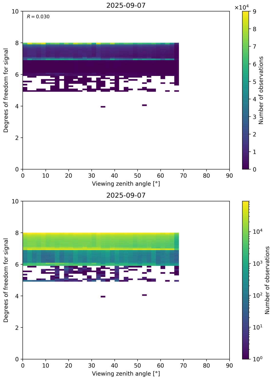
Figure 73: Scatter density plot of “Viewing zenith angle” against “Degrees of freedom for signal” for 2025-09-06 to 2025-09-08.
