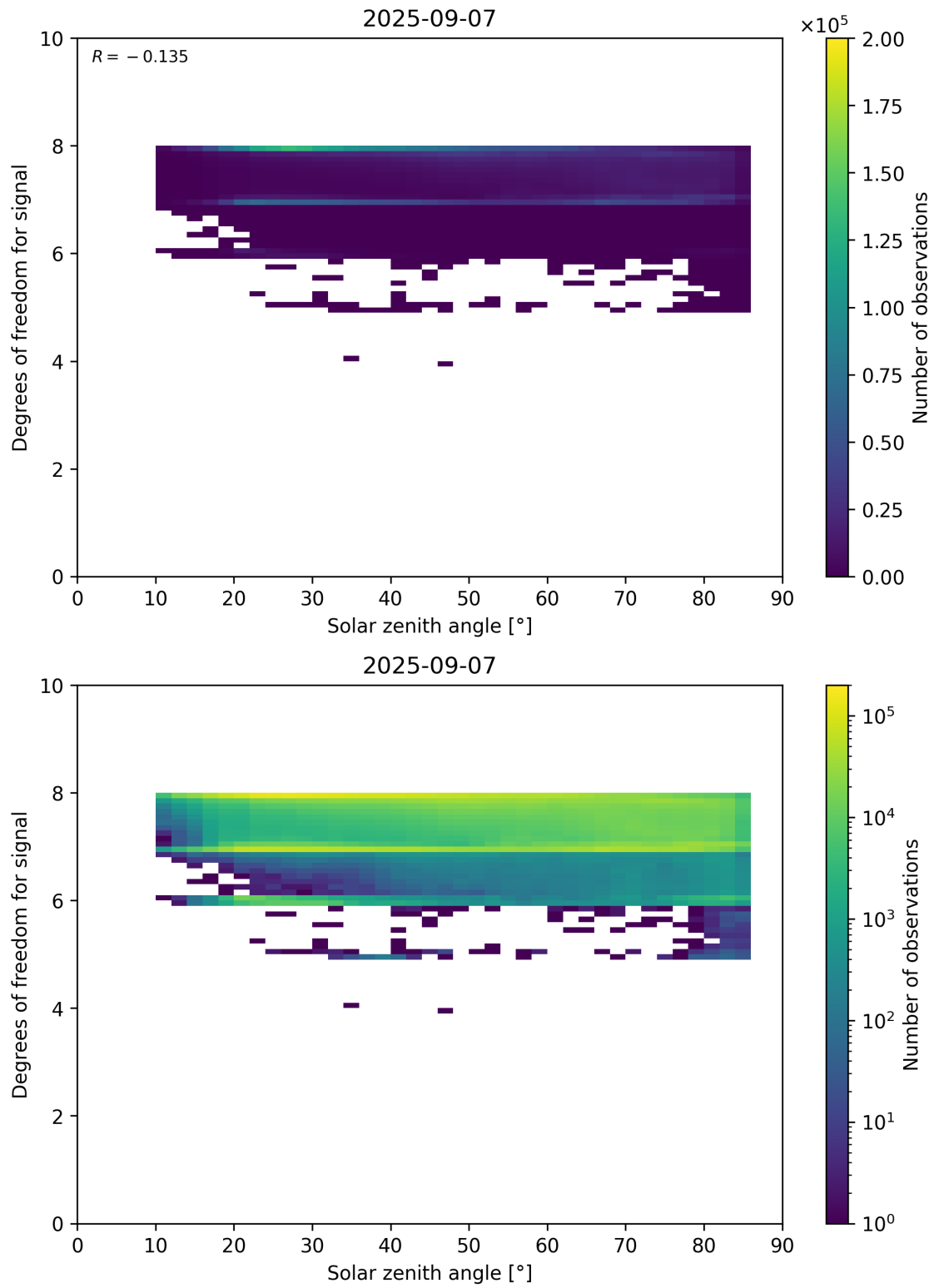
Figure 65: Scatter density plot of “Solar zenith angle” against “Degrees of freedom for signal” for 2025-09-06 to 2025-09-08.
