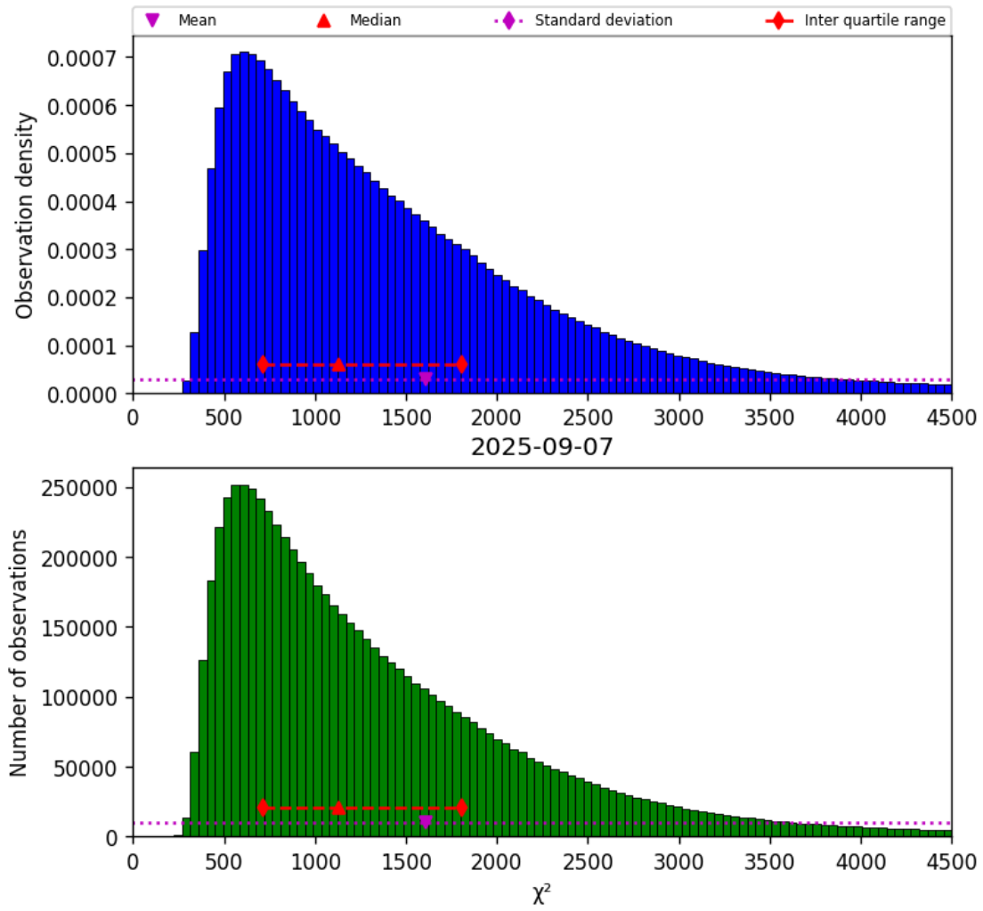
Figure 22: Histogram of " \chi^2 " for 2025-09-06 to 2025-09-08
