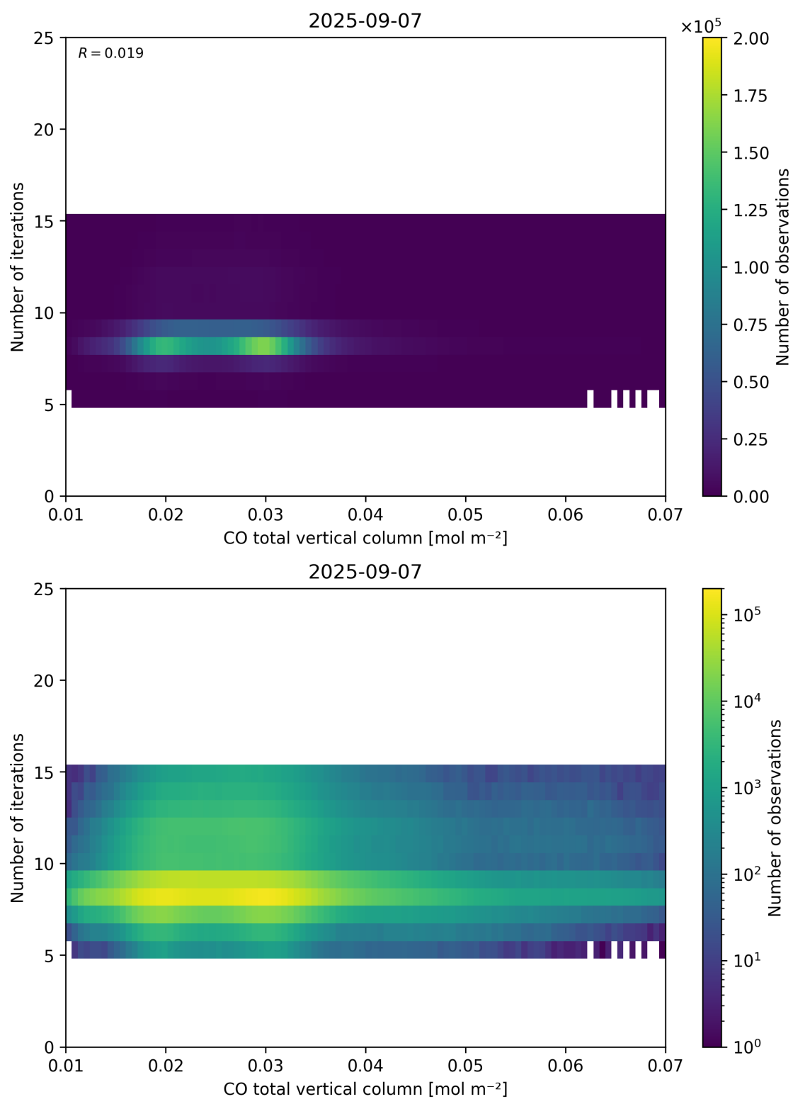
Figure 42: Scatter density plot of “CO total vertical column” against “Number of iterations” for 2025-09-06 to 2025-09-08.
