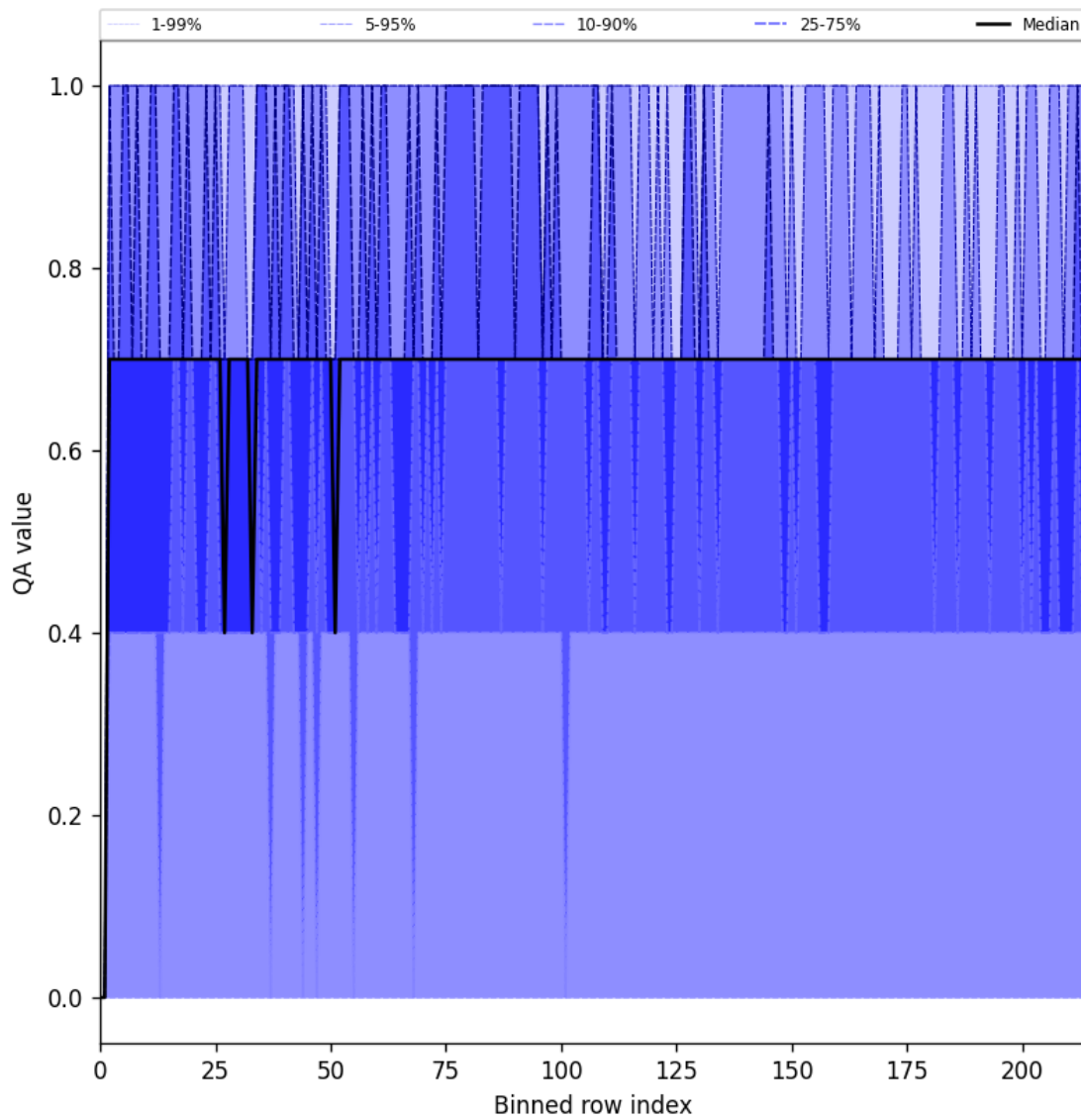
Figure 25: Along track statistics of “QA value” for 2025-09-06 to 2025-09-08
