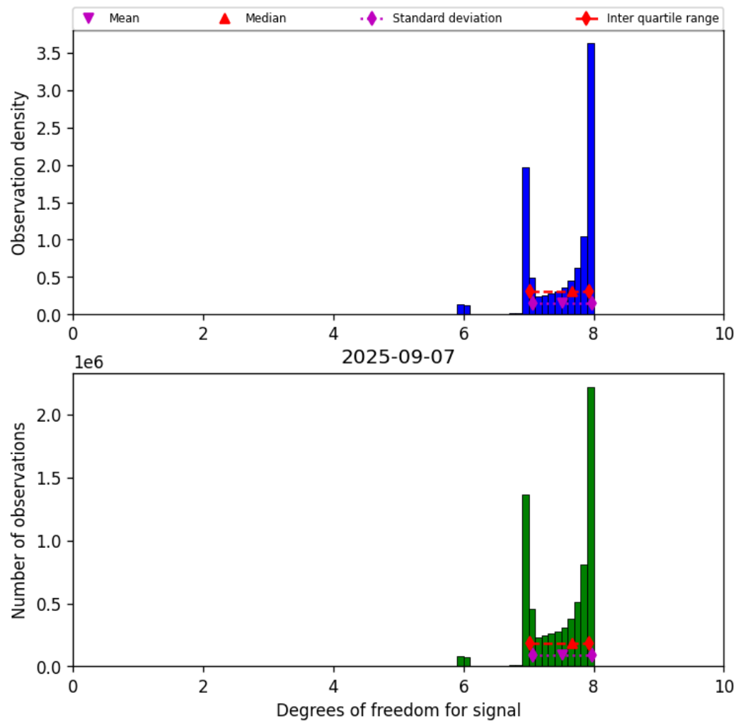
Figure 23: Histogram of “Degrees of freedom for signal” for 2025-09-06 to 2025-09-08
