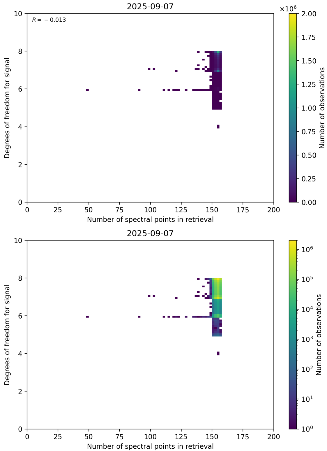
Figure 59: Scatter density plot of “Number of spectral points in retrieval” against “Degrees of freedom for signal” for 2025-09-06 to 2025-09-08.
