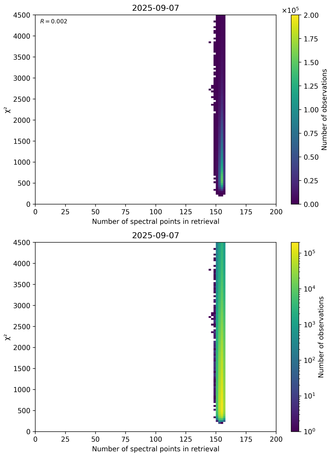
Figure 58: Scatter density plot of “Number of spectral points in retrieval” against “ \chi^2 ” for 2025-09-06 to 2025-09-08.
