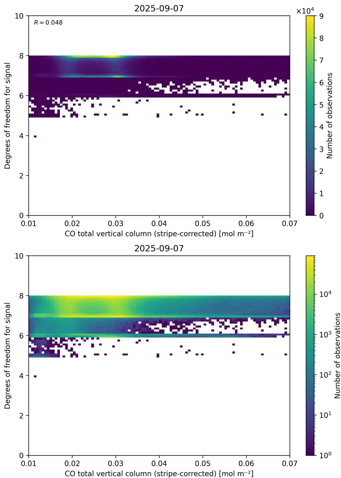
Figure 38: Scatter density plot of “CO total vertical column (stripe-corrected)” against “Degrees of freedom for signal” for 2025-09-06 to 2025-09-08.
