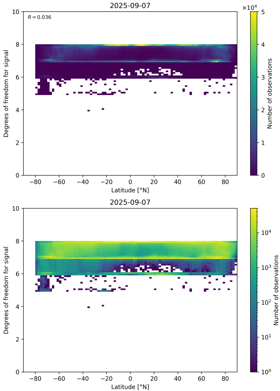
Figure 55: Scatter density plot of “Latitude” against “Degrees of freedom for signal” for 2025-09-06 to 2025-09-08.
