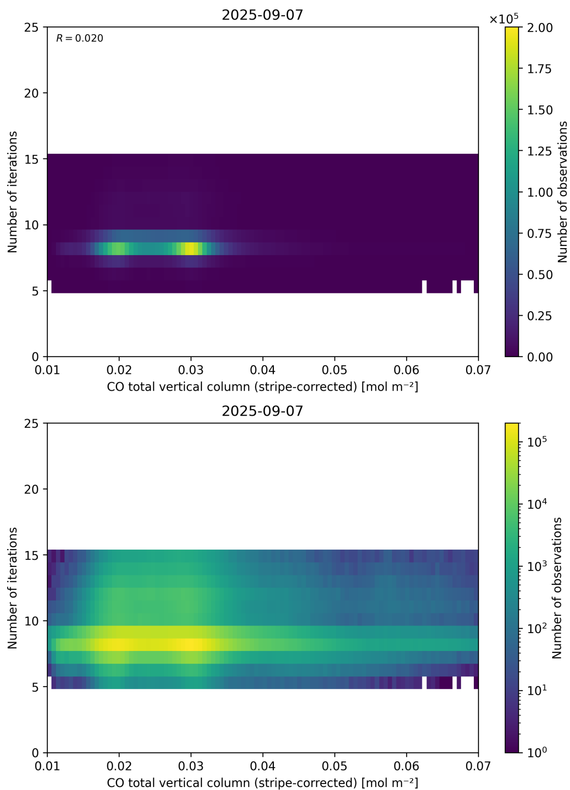
Figure 39: Scatter density plot of “CO total vertical column (stripe-corrected)” against “Number of iterations” for 2025-09-06 to 2025-09-08.
