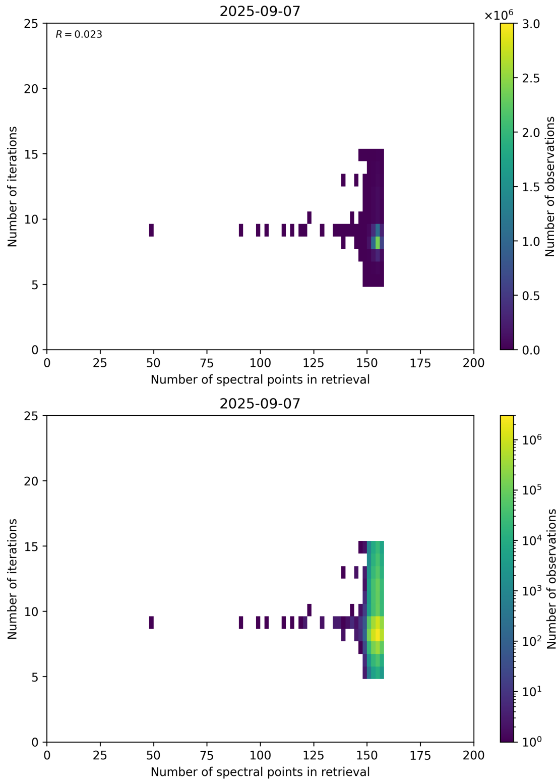
Figure 60: Scatter density plot of “Number of spectral points in retrieval” against “Number of iterations” for 2025-09-06 to 2025-09-08.
