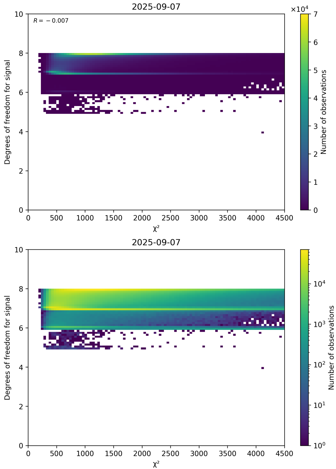
Figure 48: Scatter density plot of “ \chi^2 ” against “Degrees of freedom for signal” for 2025-09-06 to 2025-09-08.
