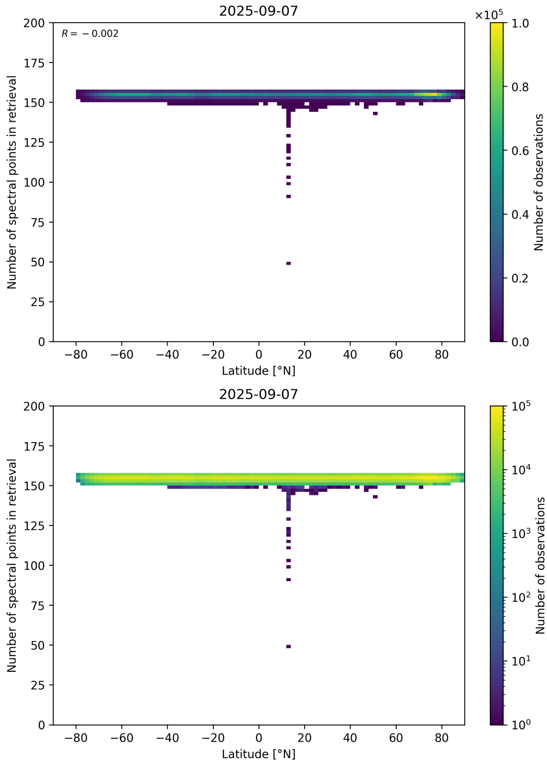
Figure 57: Scatter density plot of “Latitude” against “Number of spectral points in retrieval” for 2025-09-06 to 2025-09-08.
