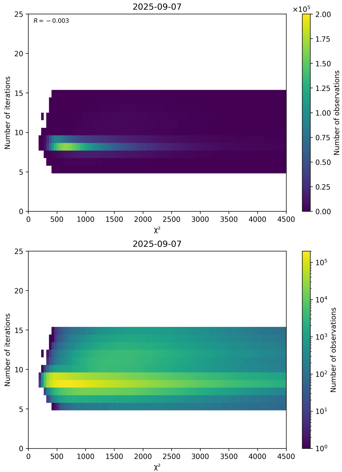
Figure 49: Scatter density plot of “ \chi^2 ” against “Number of iterations” for 2025-09-06 to 2025-09-08.
