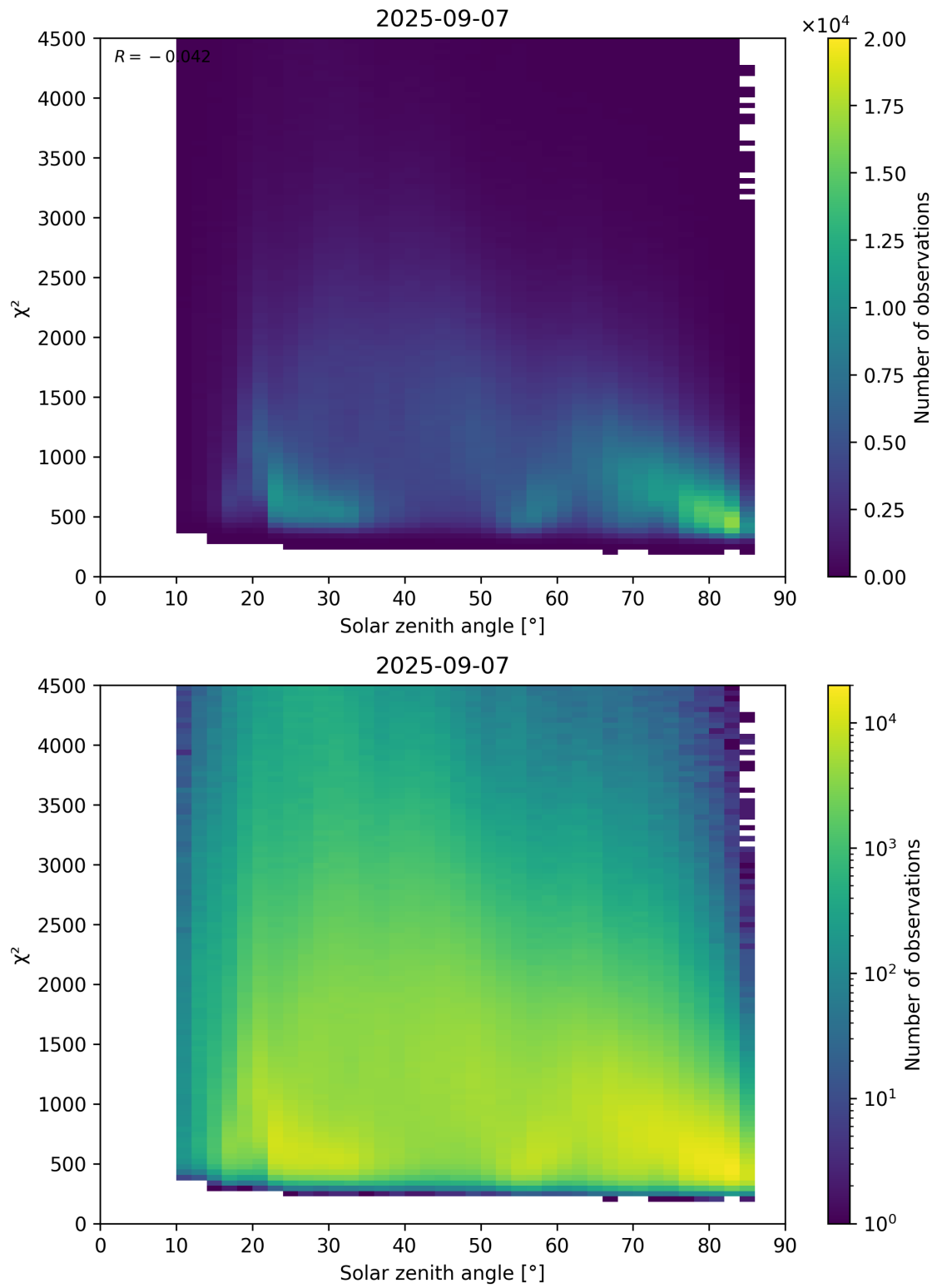
Figure 64: Scatter density plot of “Solar zenith angle” against “ \chi^2 ” for 2025-09-06 to 2025-09-08.
