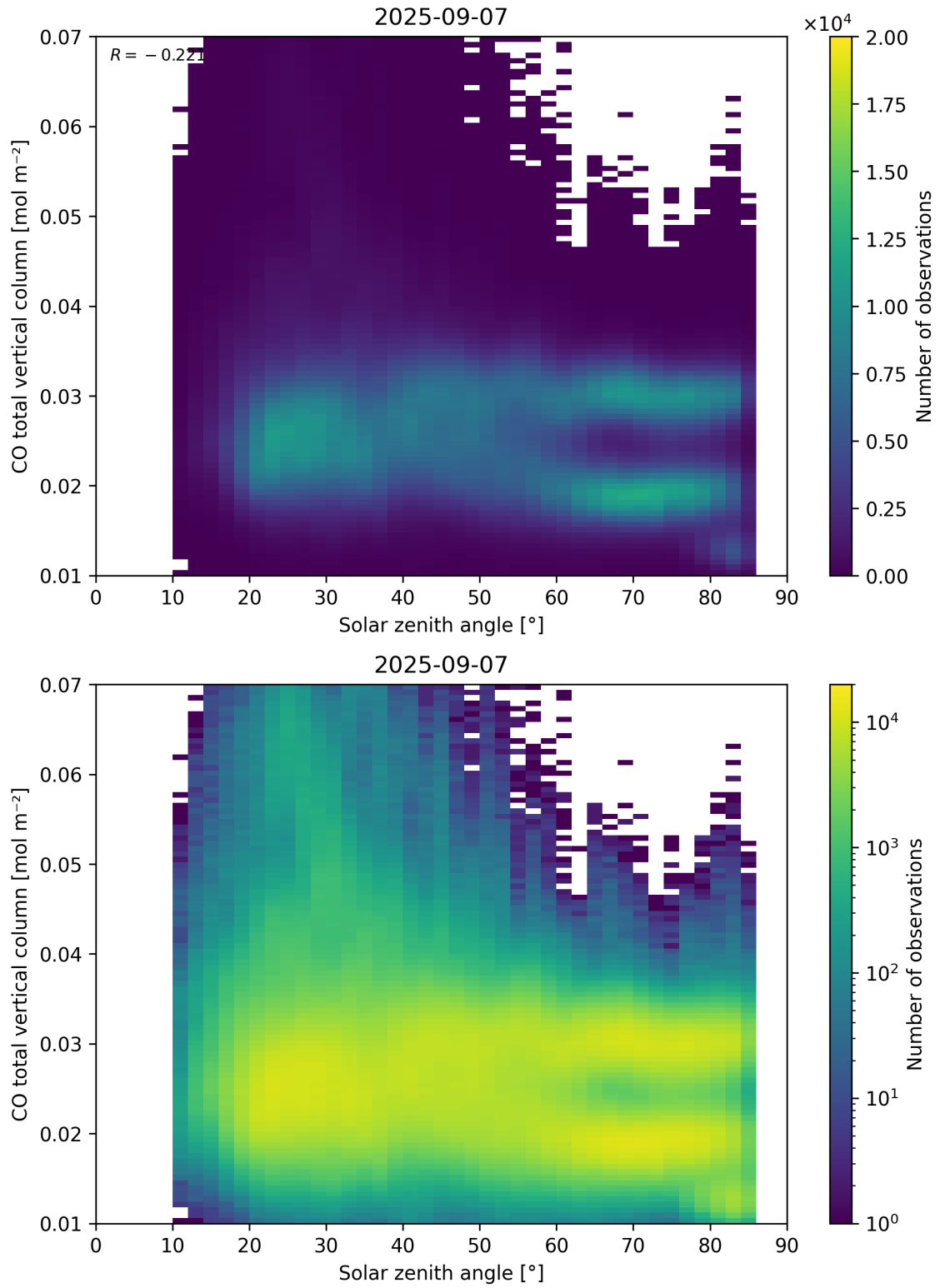
Figure 61: Scatter density plot of “Solar zenith angle” against “CO total vertical column” for 2025-09-06 to 2025-09-08.
