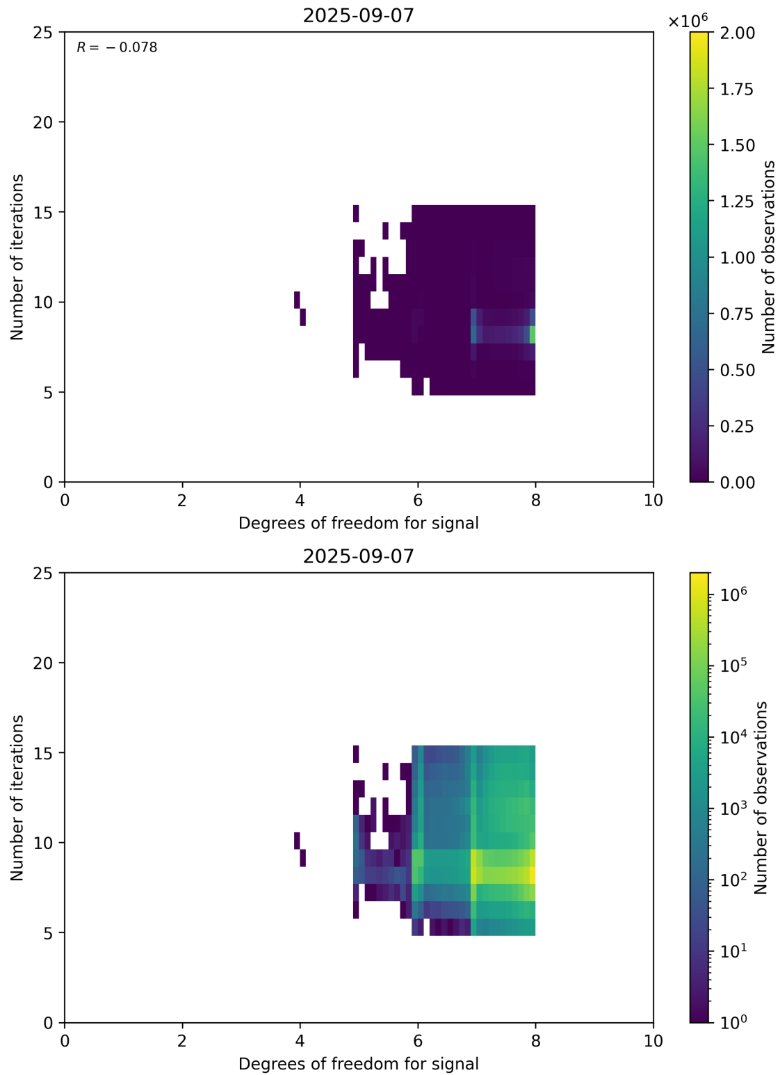
Figure 50: Scatter density plot of “Degrees of freedom for signal” against “Number of iterations” for 2025-09-06 to 2025-09-08.
