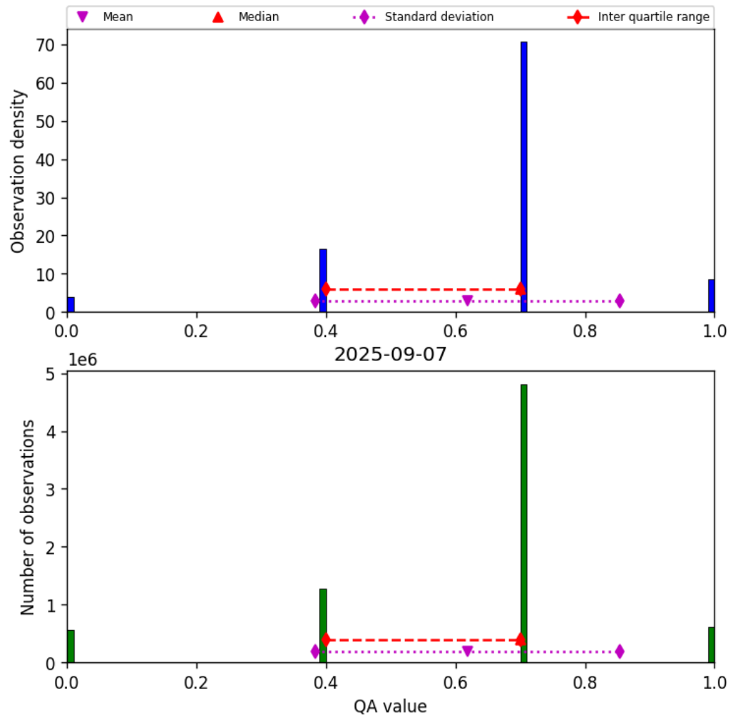
Figure 17: Histogram of “QA value” for 2025-09-06 to 2025-09-08
