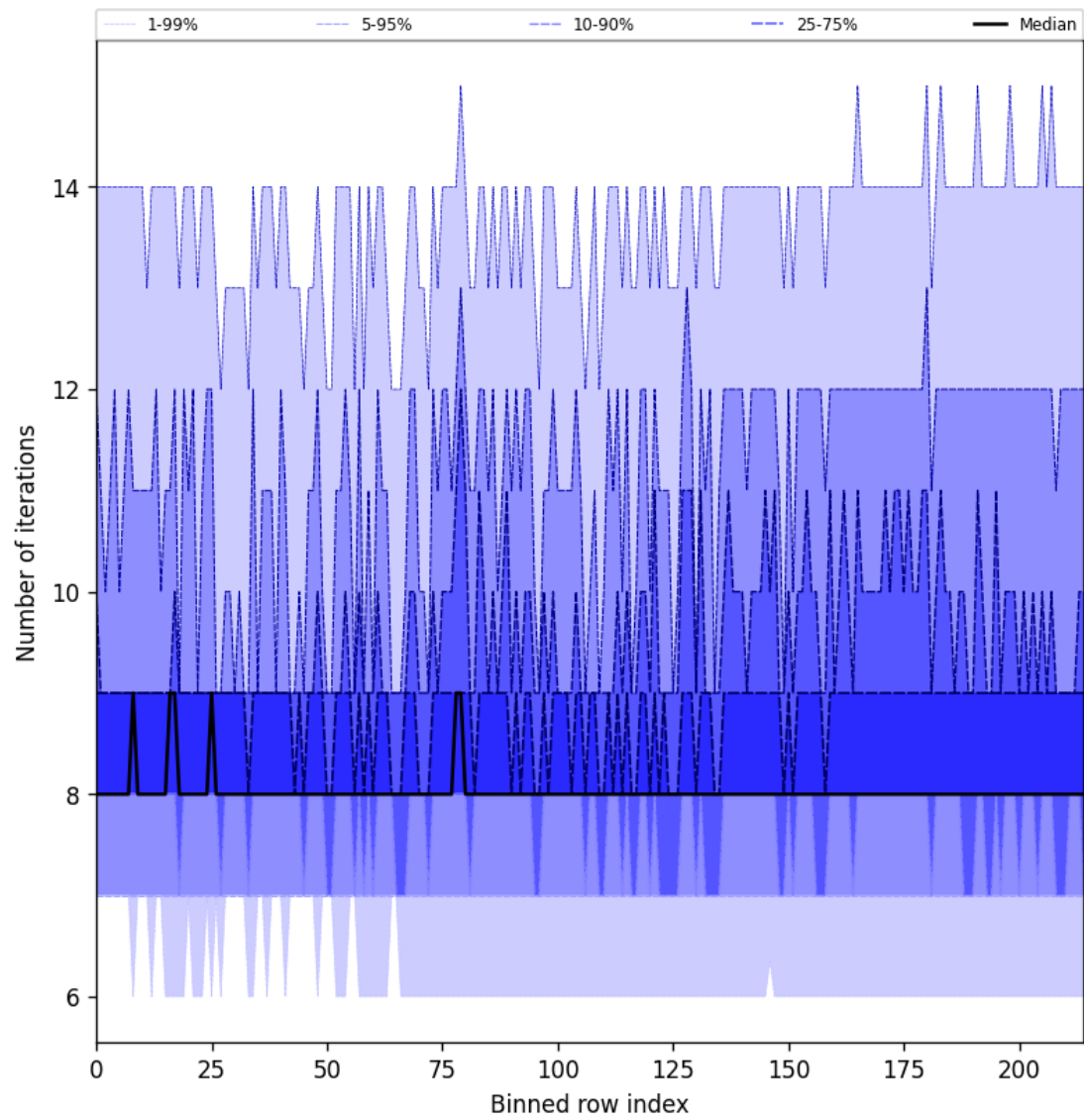
Figure 32: Along track statistics of “Number of iterations” for 2025-09-06 to 2025-09-08
