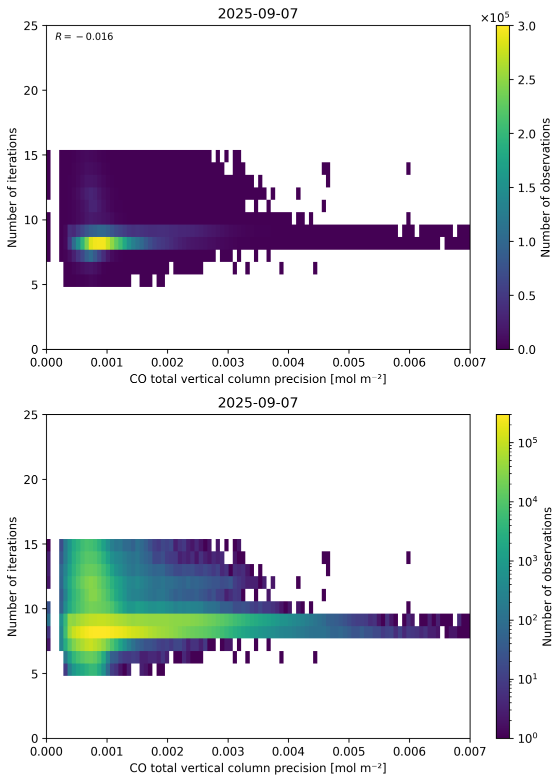
Figure 46: Scatter density plot of “CO total vertical column precision” against “Number of iterations” for 2025-09-06 to 2025-09-08.
