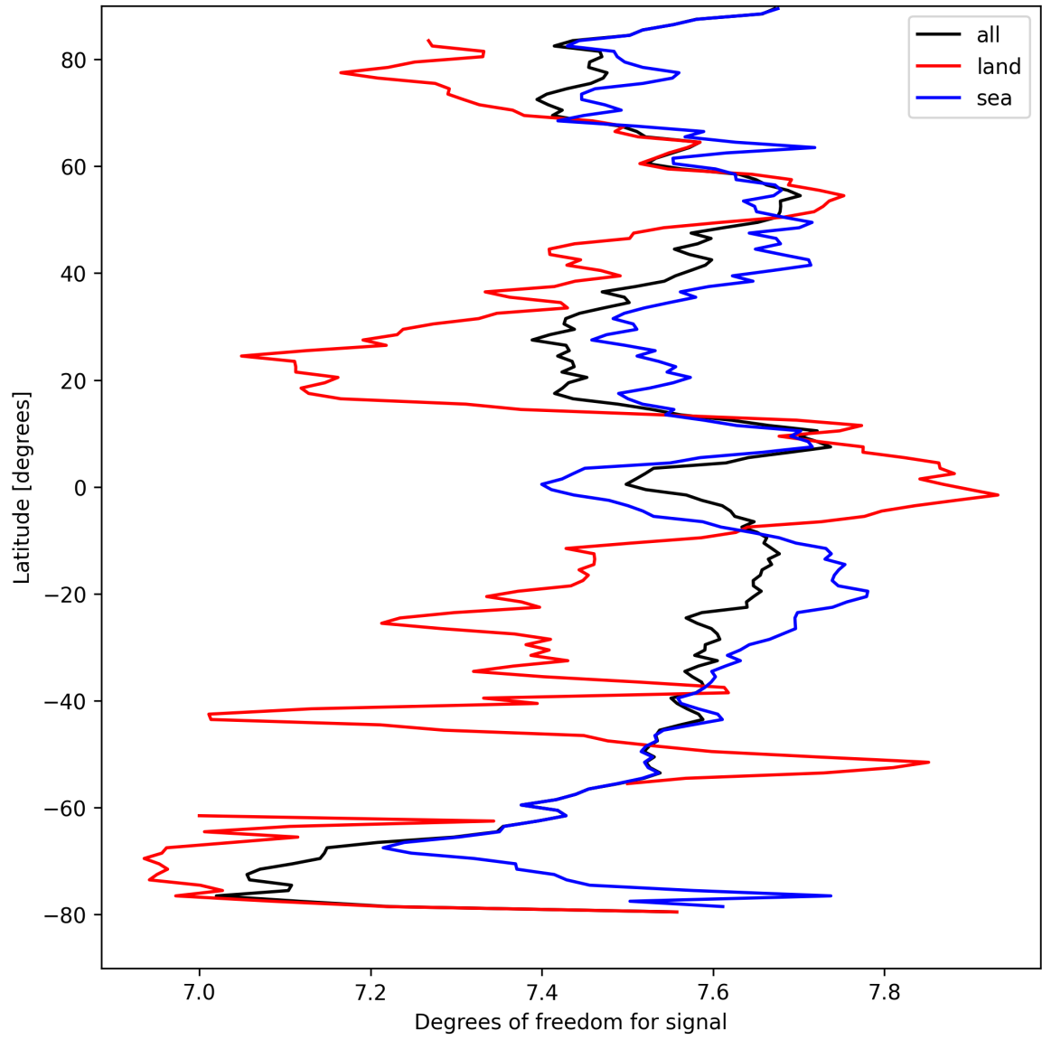
Figure 15: Zonal average of “Degrees of freedom for signal” for 2025-09-06 to 2025-09-08.
