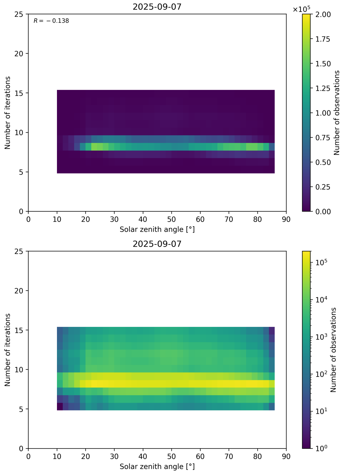
Figure 67: Scatter density plot of “Solar zenith angle” against “Number of iterations” for 2025-09-06 to 2025-09-08.
