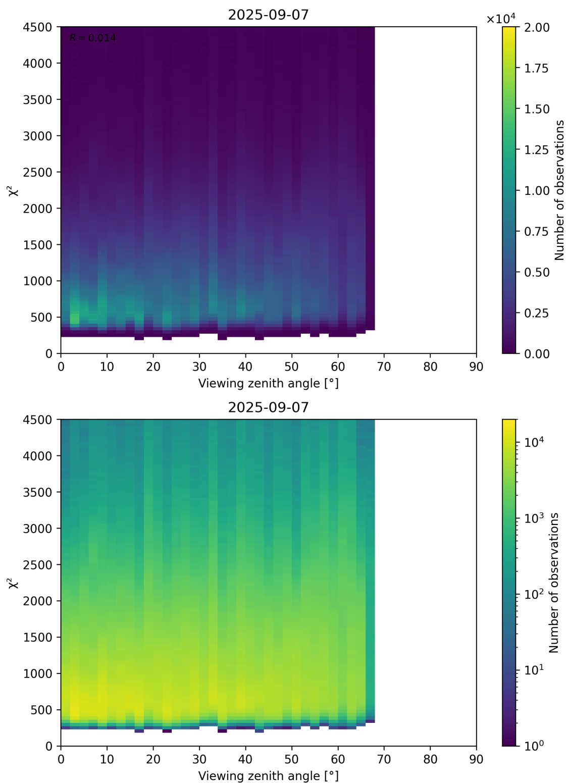
Figure 72: Scatter density plot of “Viewing zenith angle” against “ \chi^2 ” for 2025-09-06 to 2025-09-08.
