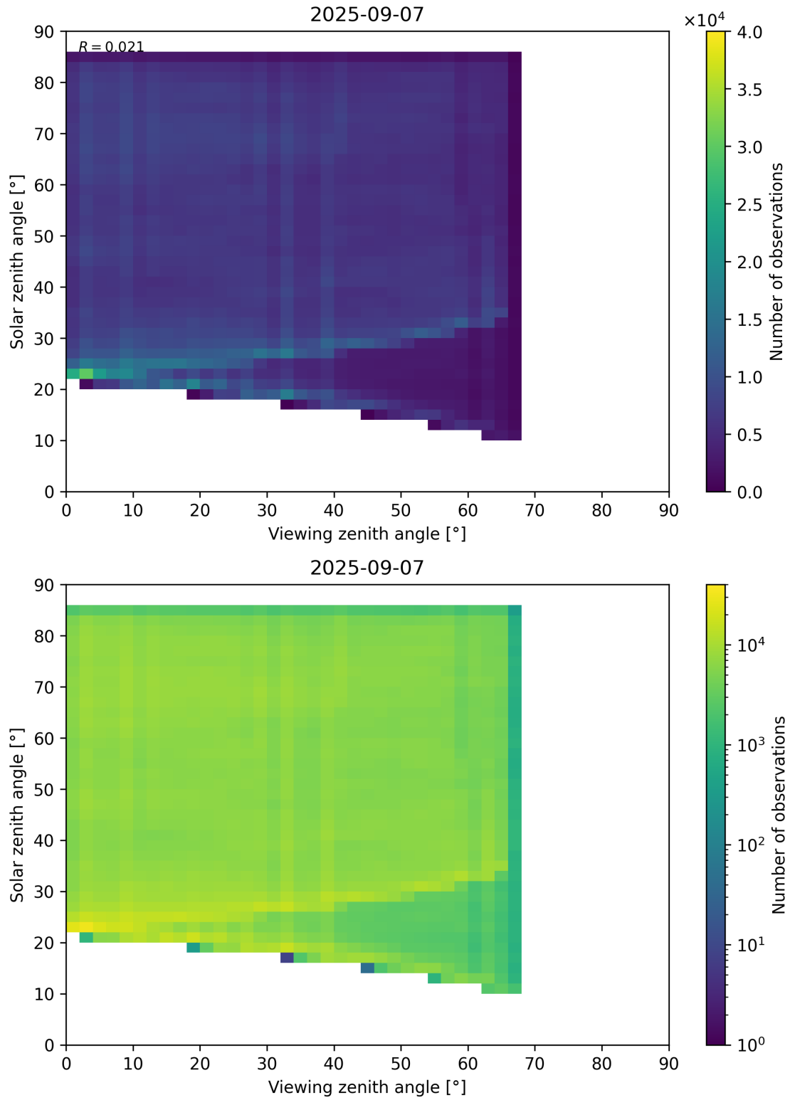
Figure 77: Scatter density plot of “Viewing zenith angle” against “Solar zenith angle” for 2025-09-06 to 2025-09-08.
