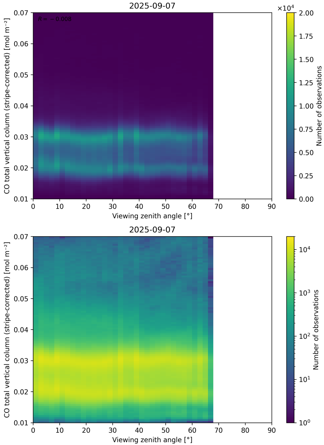
Figure 70: Scatter density plot of “Viewing zenith angle” against “CO total vertical column (stripe-corrected)” for 2025-09-06 to 2025-09-08.
