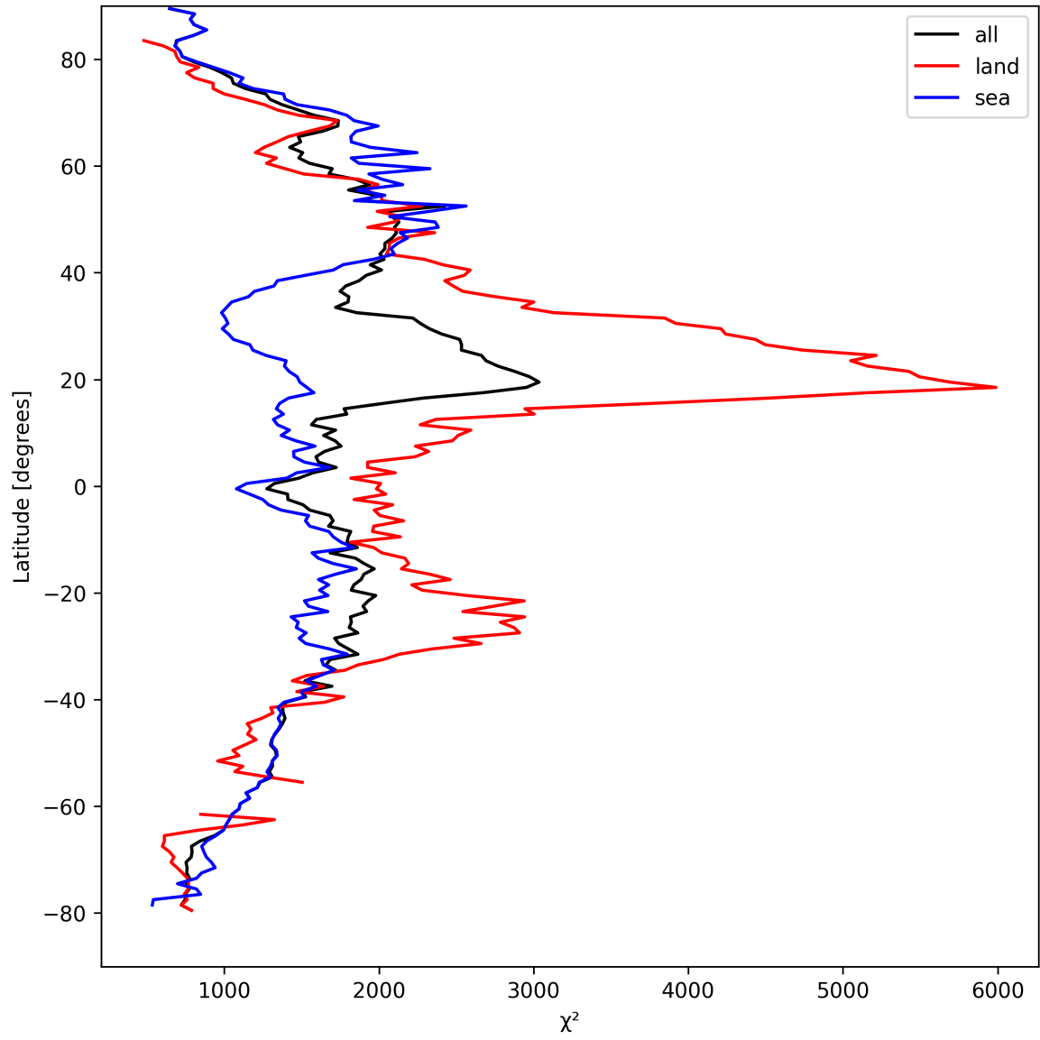
Figure 14: Zonal average of “ \chi^2 ” for 2025-09-06 to 2025-09-08.
