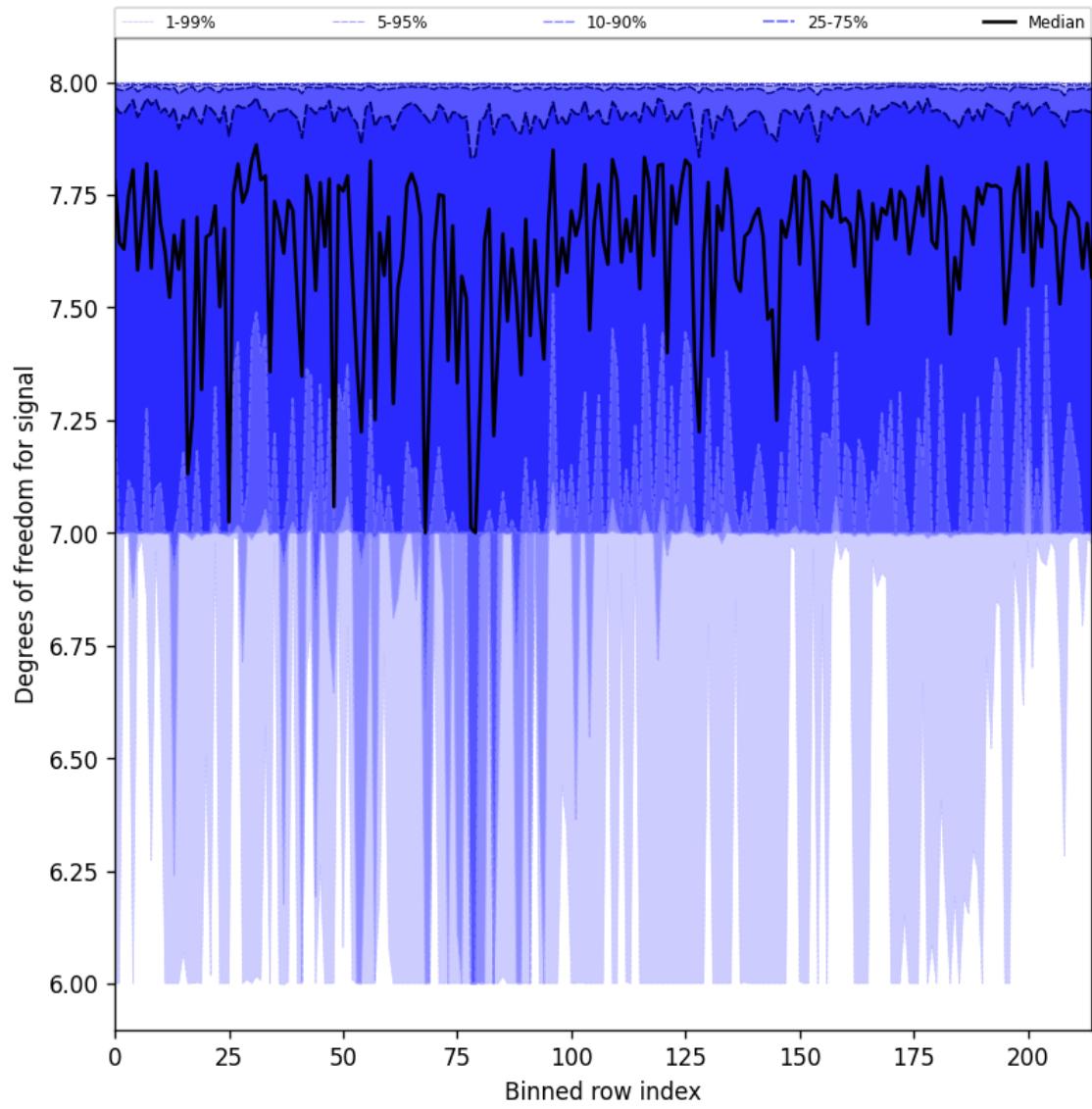
Figure 31: Along track statistics of “Degrees of freedom for signal” for 2025-09-06 to 2025-09-08
