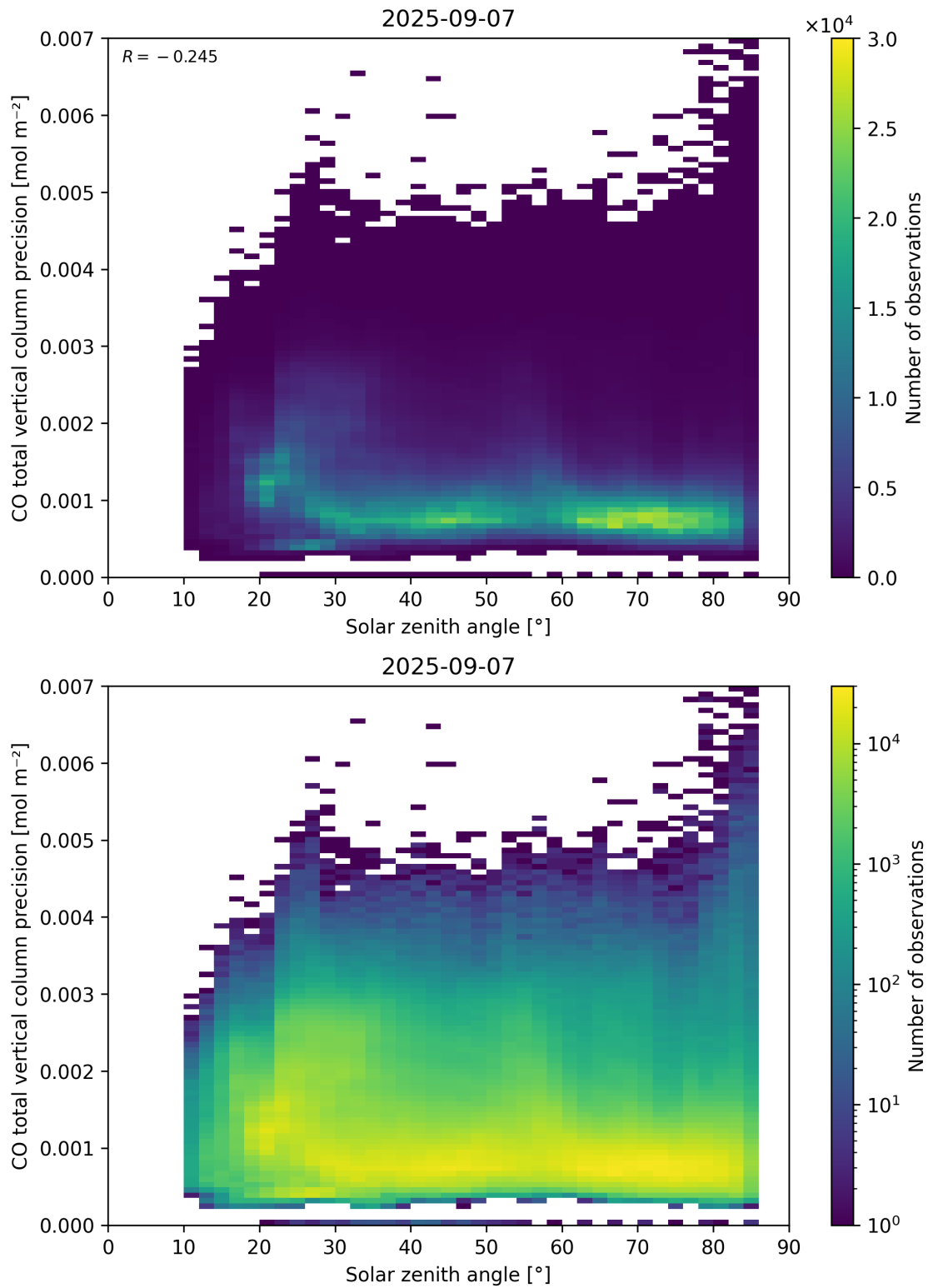
Figure 63: Scatter density plot of “Solar zenith angle” against “CO total vertical column precision” for 2025-09-06 to 2025-09-08.
