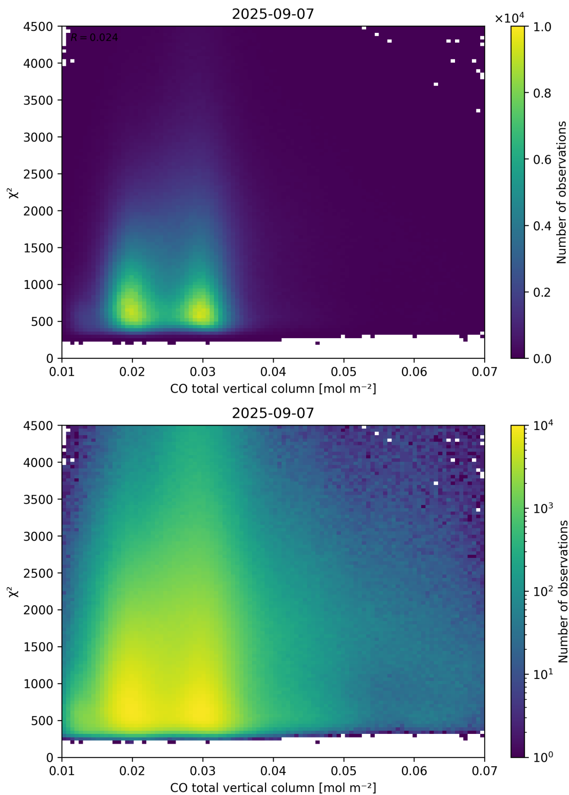
Figure 35: Scatter density plot of “CO total vertical column” against “ \chi^2 ” for 2025-09-06 to 2025-09-08.
