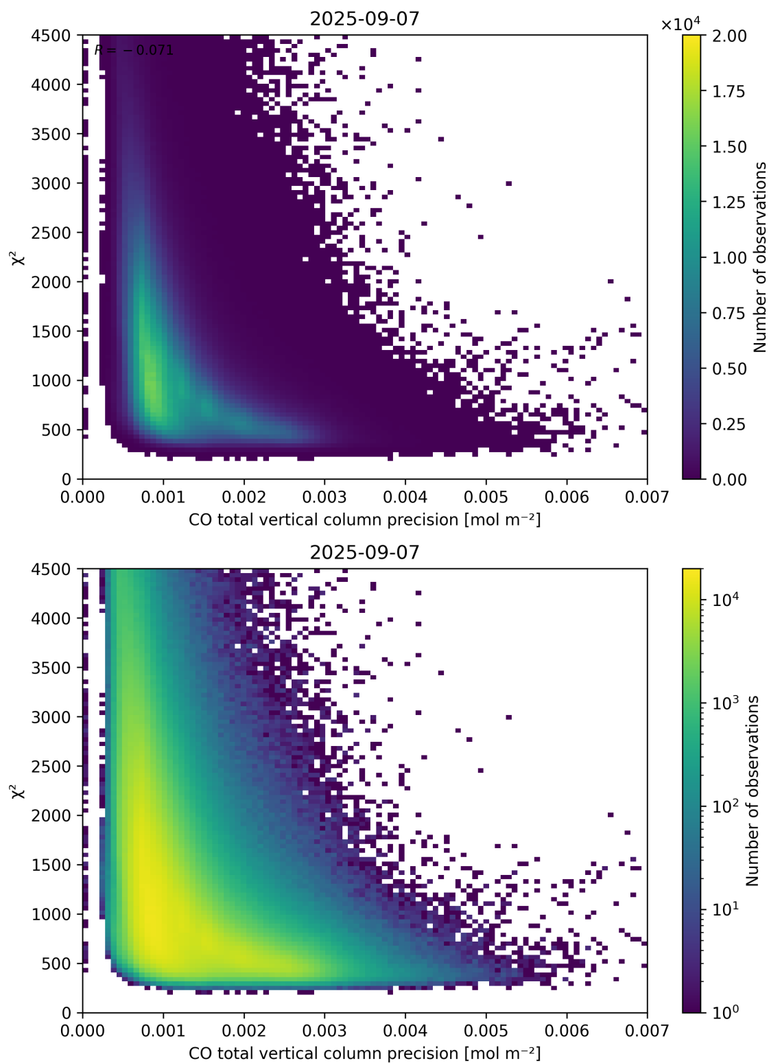
Figure 44: Scatter density plot of “CO total vertical column precision” against “ \chi^2 ” for 2025-09-06 to 2025-09-08.
