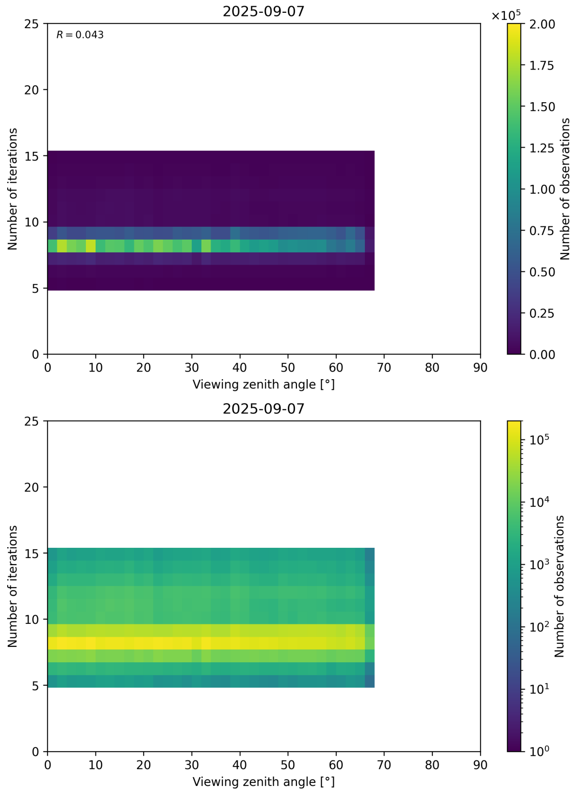
Figure 75: Scatter density plot of “Viewing zenith angle” against “Number of iterations” for 2025-09-06 to 2025-09-08.
