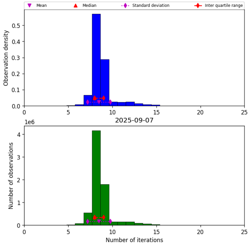
Figure 24: Histogram of “Number of iterations” for 2025-09-06 to 2025-09-08
