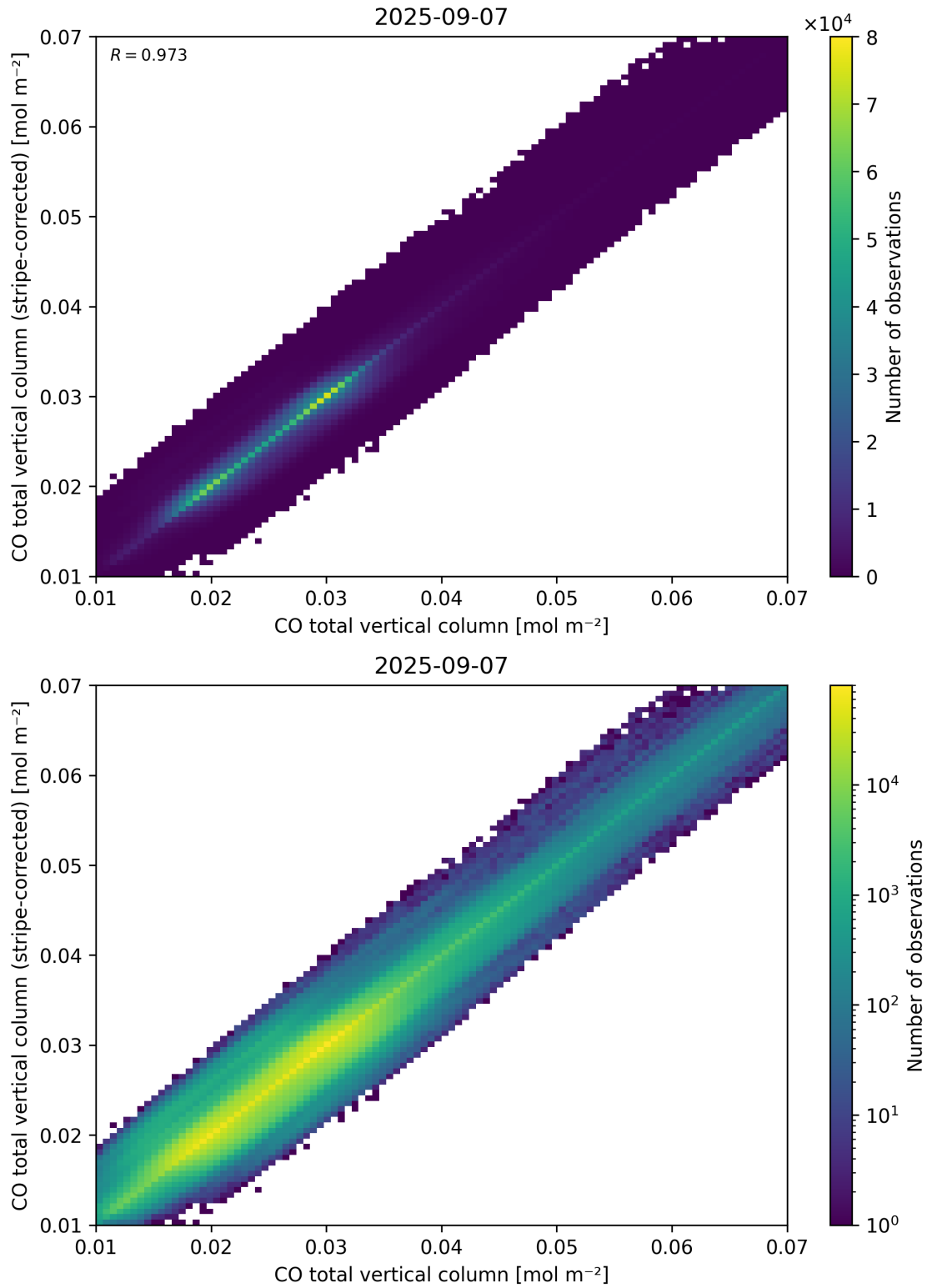
Figure 33: Scatter density plot of “CO total vertical column” against “CO total vertical column (stripe-corrected)” for 2025-09-06 to 2025-09-08.
