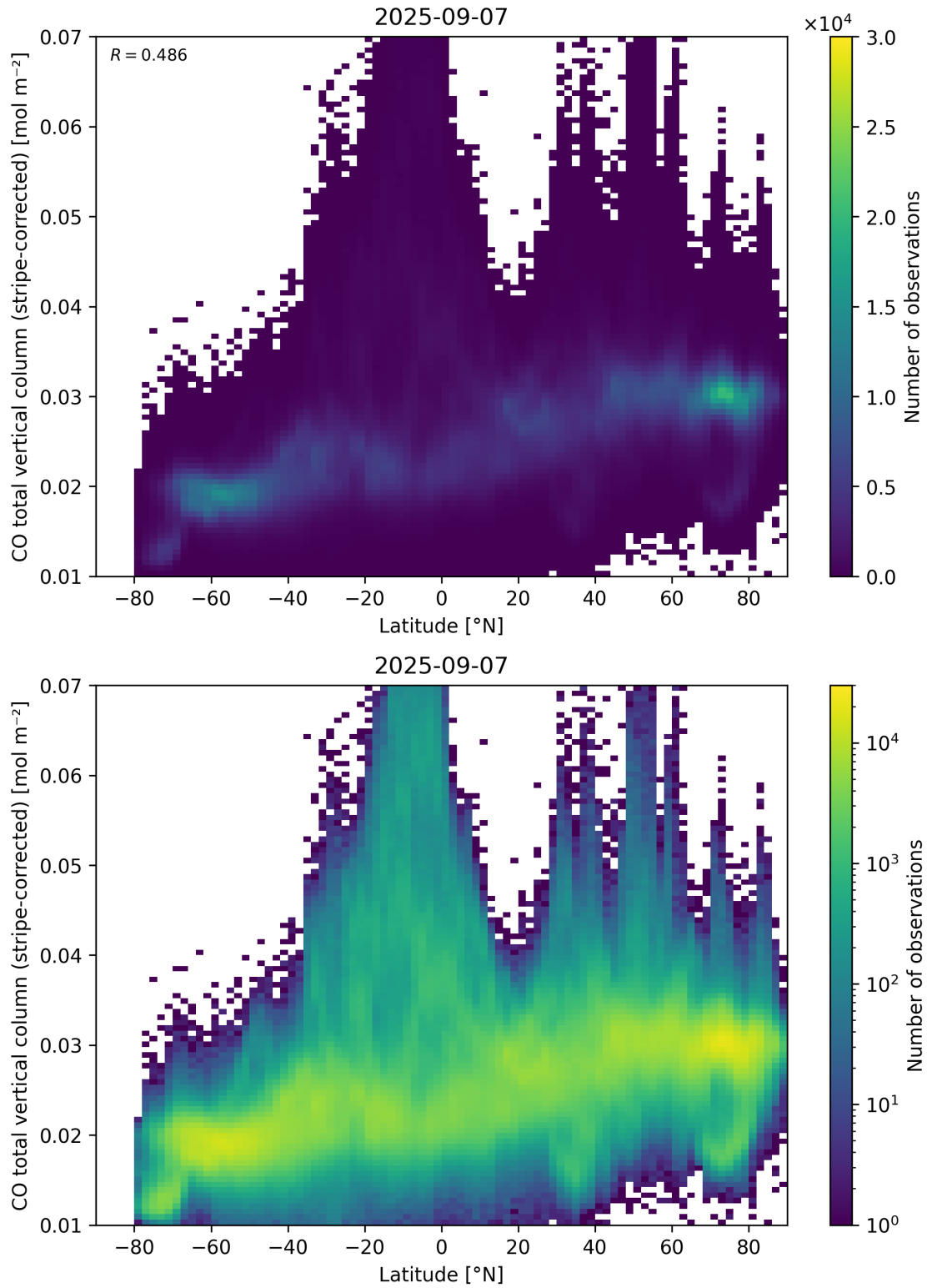
Figure 52: Scatter density plot of “Latitude” against “CO total vertical column (stripe-corrected)” for 2025-09-06 to 2025-09-08.
