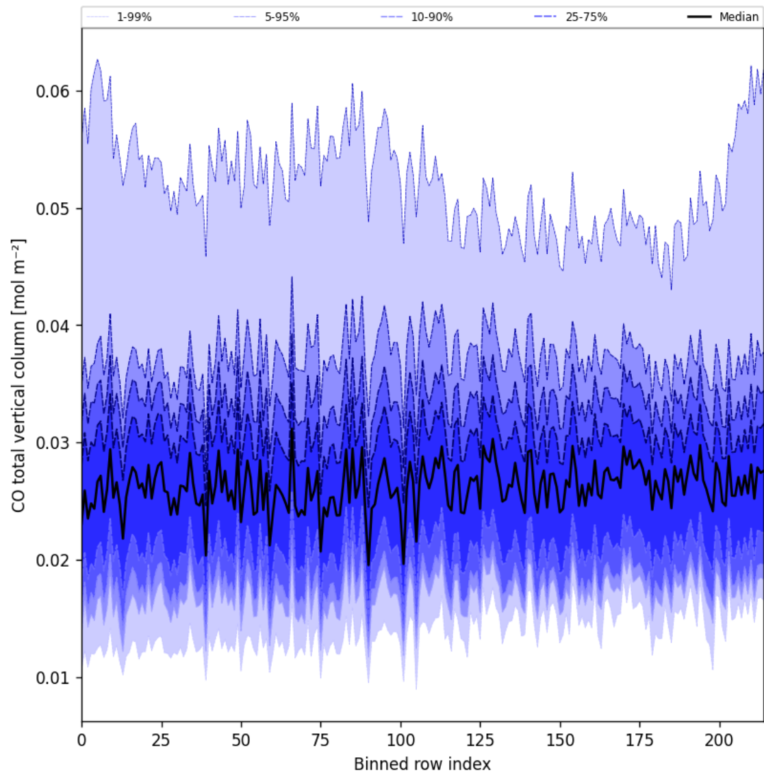
Figure 26: Along track statistics of “CO total vertical column” for 2025-09-06 to 2025-09-08
