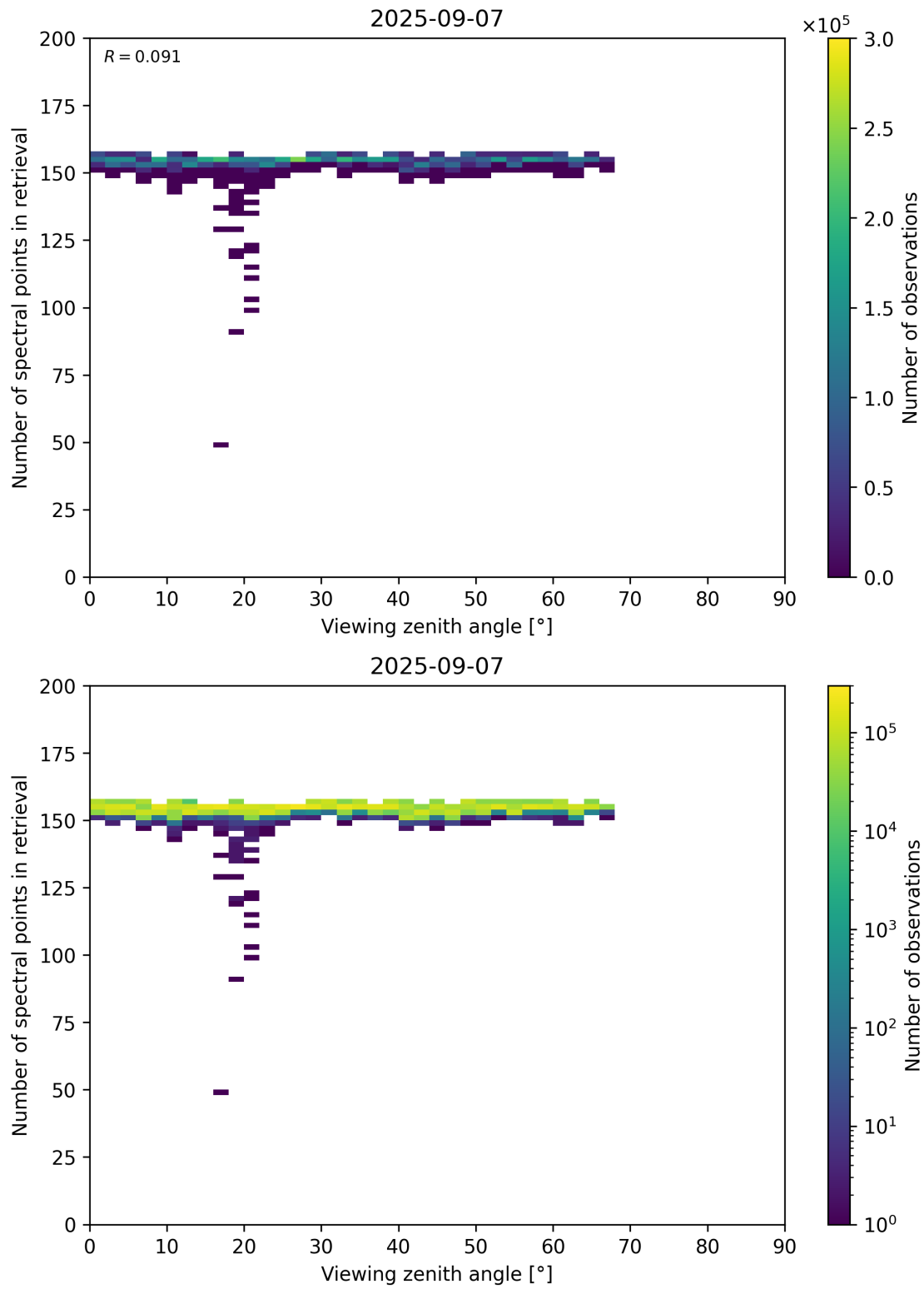
Figure 76: Scatter density plot of “Viewing zenith angle” against “Number of spectral points in retrieval” for 2025-09-06 to 2025-09-08.
