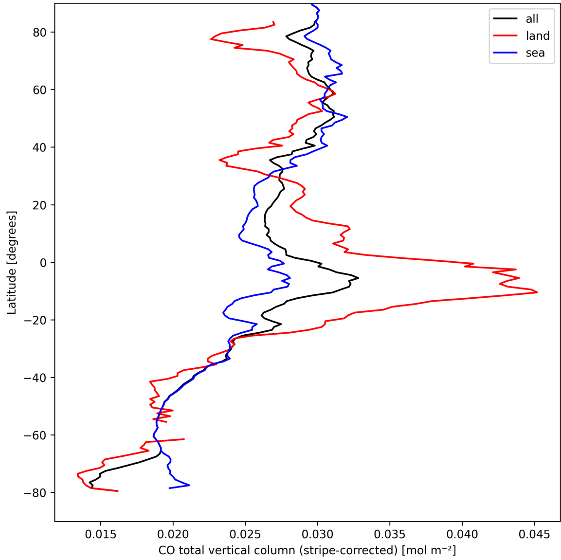
Figure 11: Zonal average of “CO total vertical column (stripe-corrected)” for 2025-09-06 to 2025-09-08.
