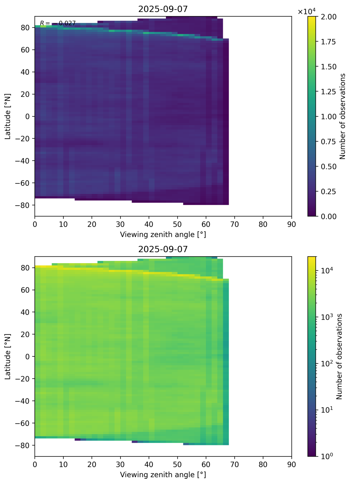
Figure 74: Scatter density plot of “Viewing zenith angle” against “Latitude” for 2025-09-06 to 2025-09-08.
