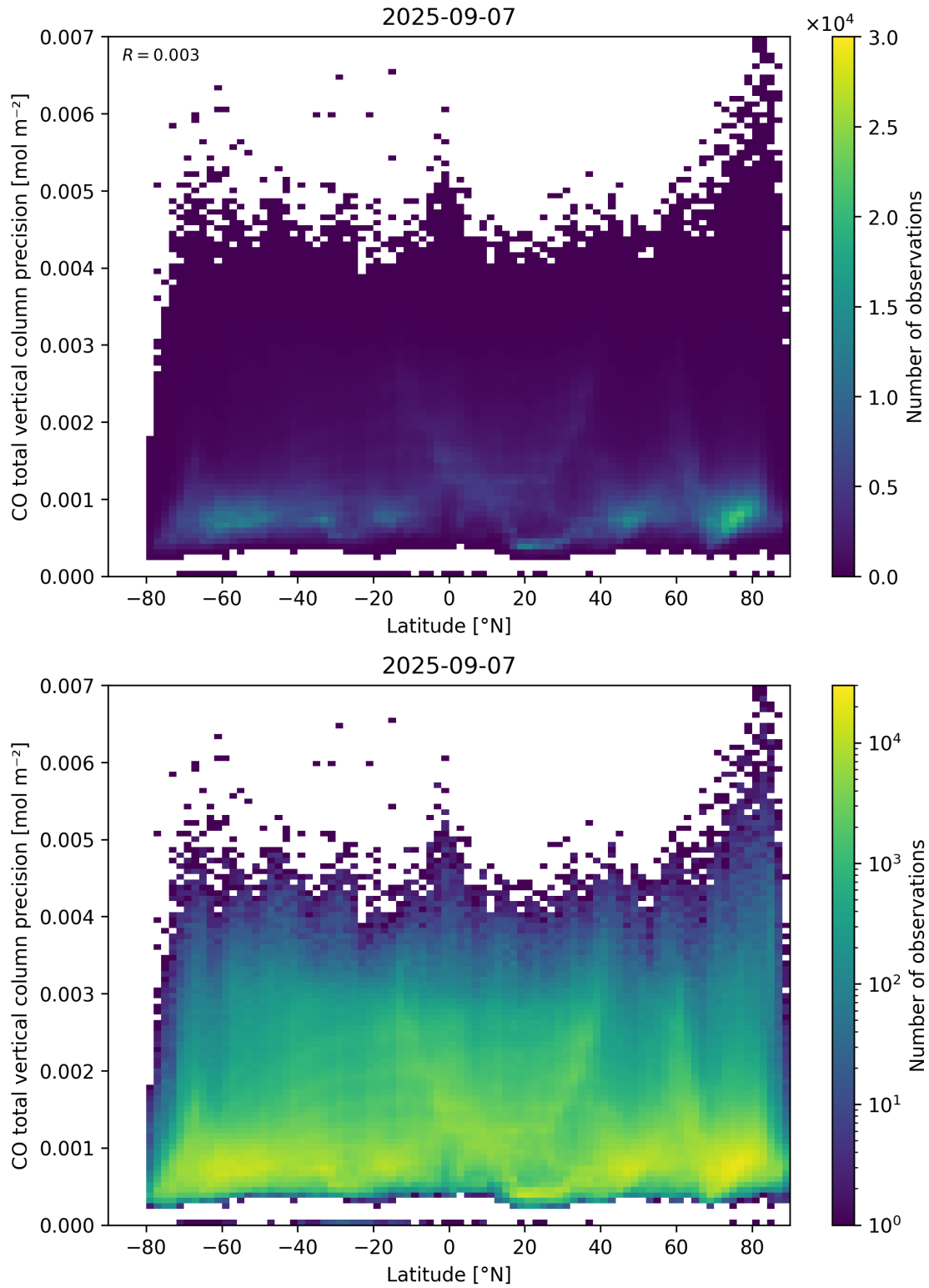
Figure 53: Scatter density plot of “Latitude” against “CO total vertical column precision” for 2025-09-06 to 2025-09-08.
