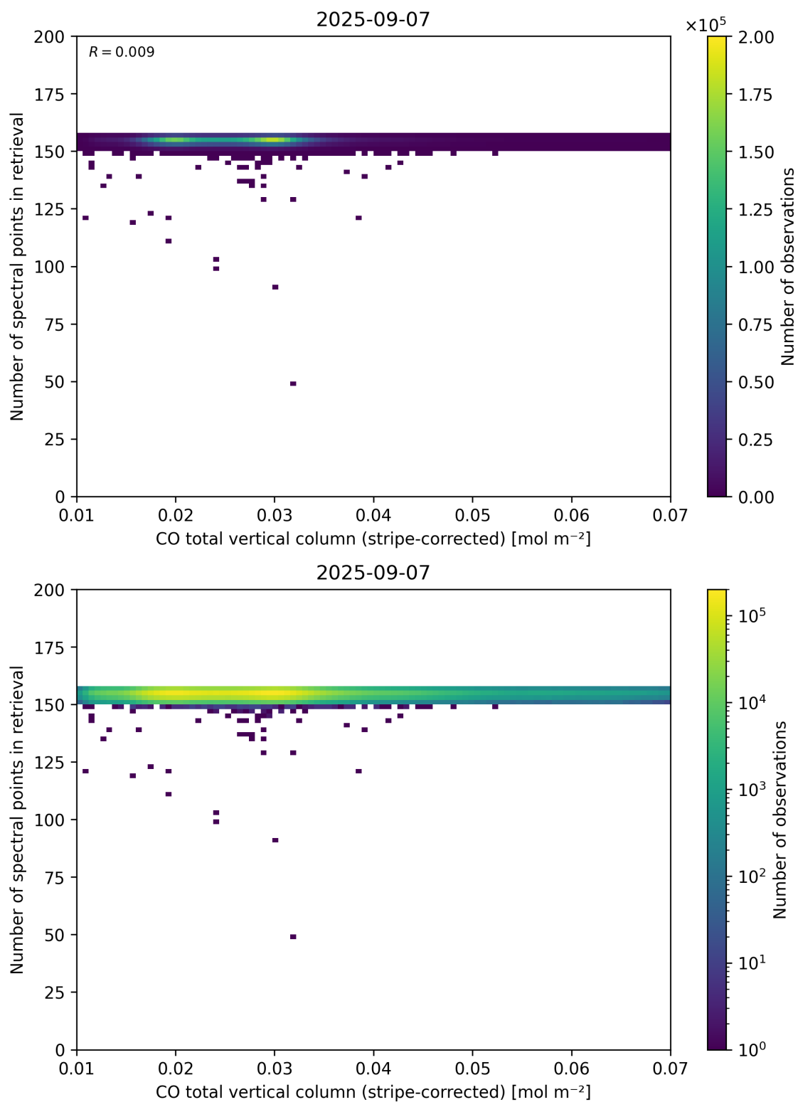
Figure 40: Scatter density plot of “CO total vertical column (stripe-corrected)” against “Number of spectral points in retrieval” for 2025-09-06 to 2025-09-08.
