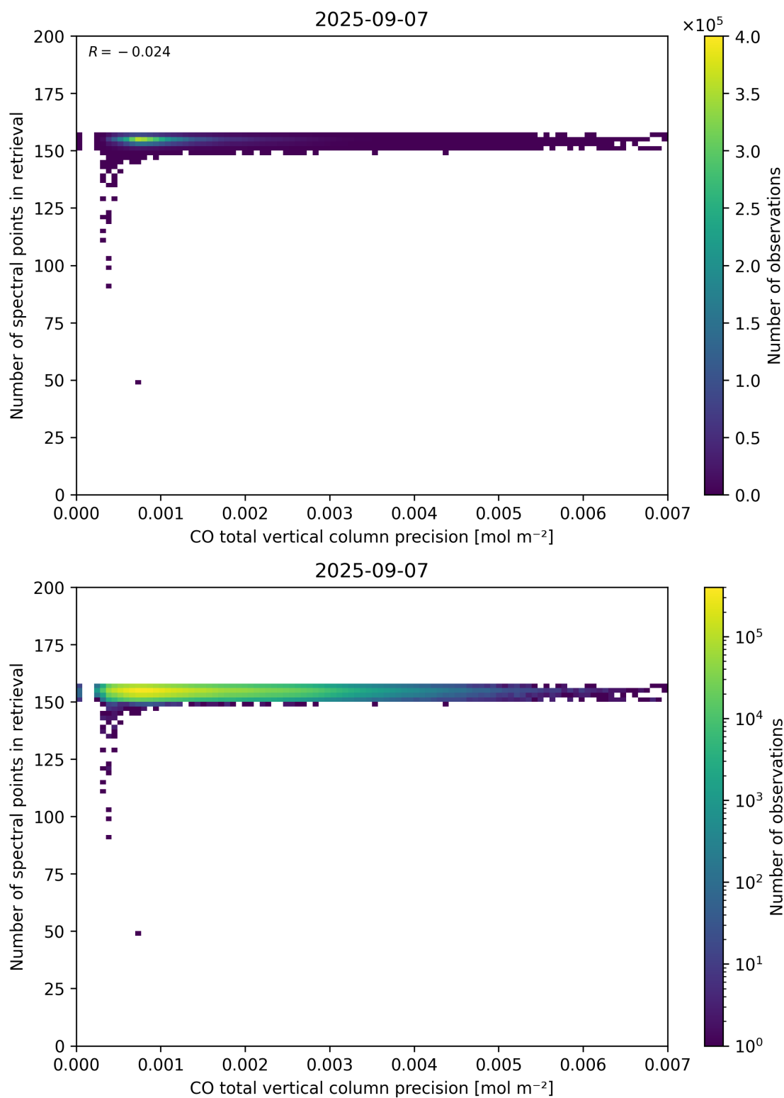
Figure 47: Scatter density plot of “CO total vertical column precision” against “Number of spectral points in retrieval” for 2025-09-06 to 2025-09-08.
