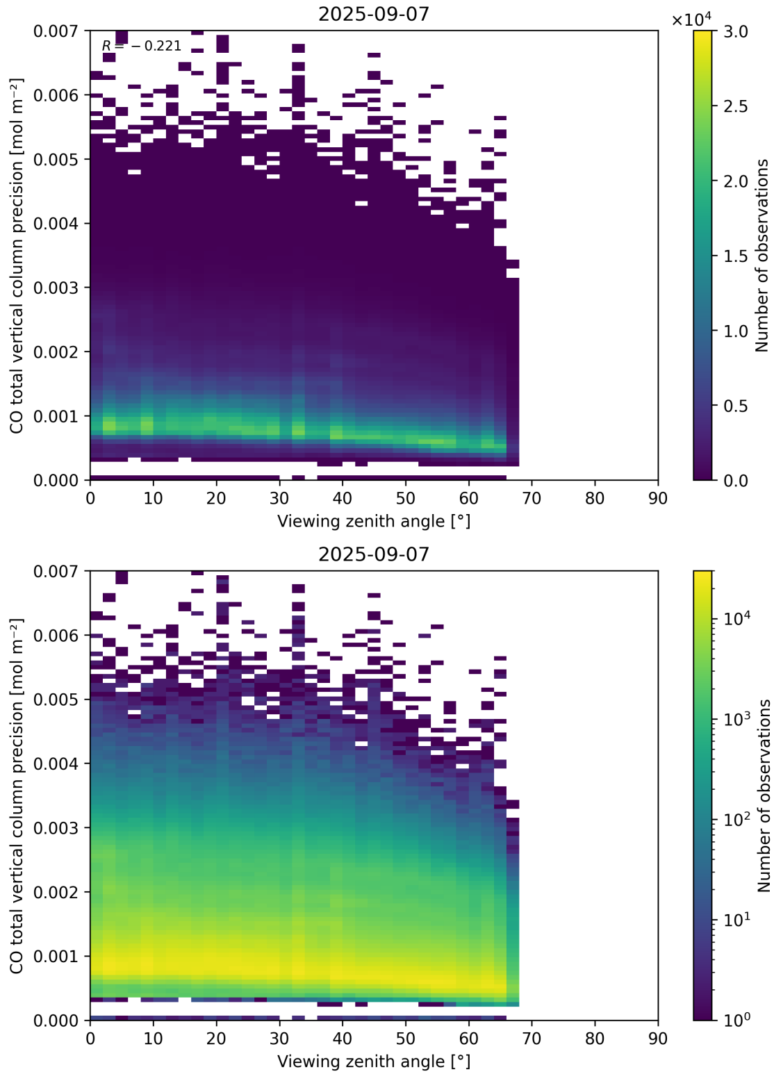
Figure 71: Scatter density plot of “Viewing zenith angle” against “CO total vertical column precision” for 2025-09-06 to 2025-09-08.
