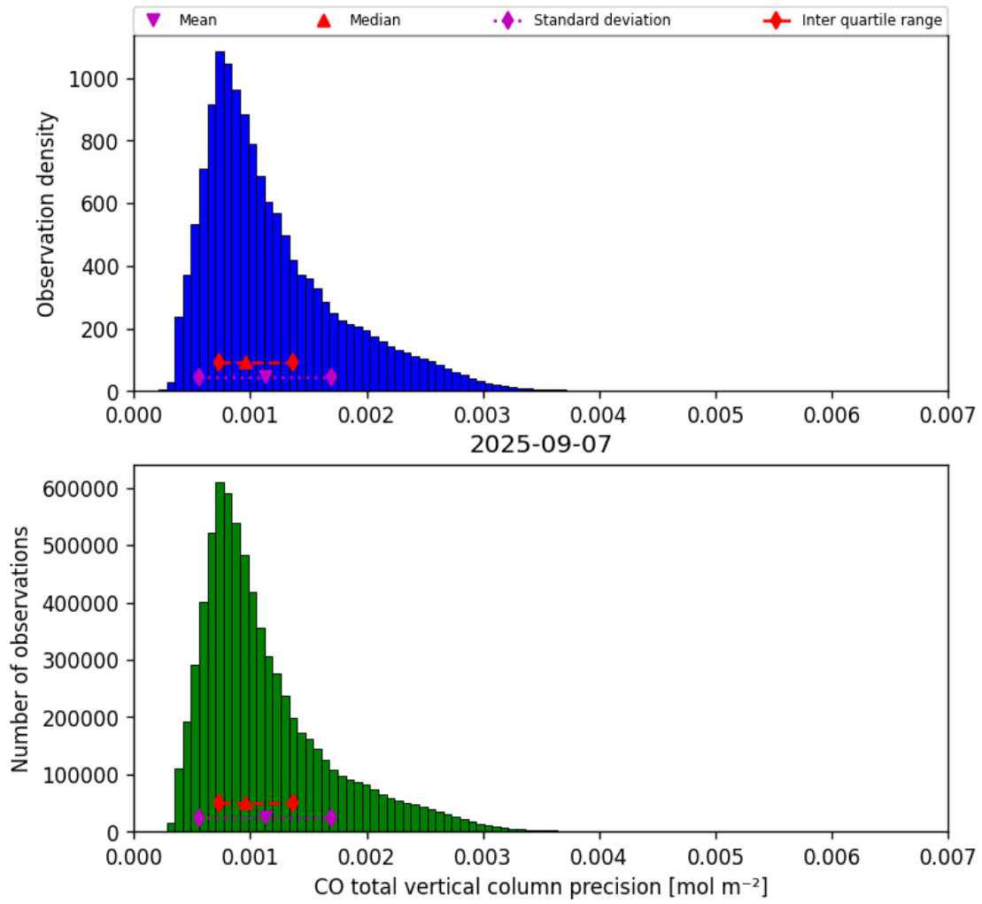
Figure 20: Histogram of “CO total vertical column precision” for 2025-09-06 to 2025-09-08
