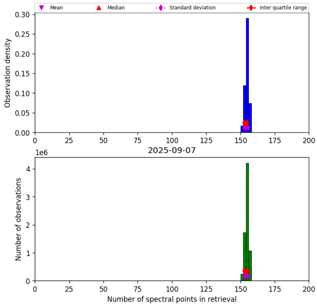
Figure 21: Histogram of “Number of spectral points in retrieval” for 2025-09-06 to 2025-09-08
