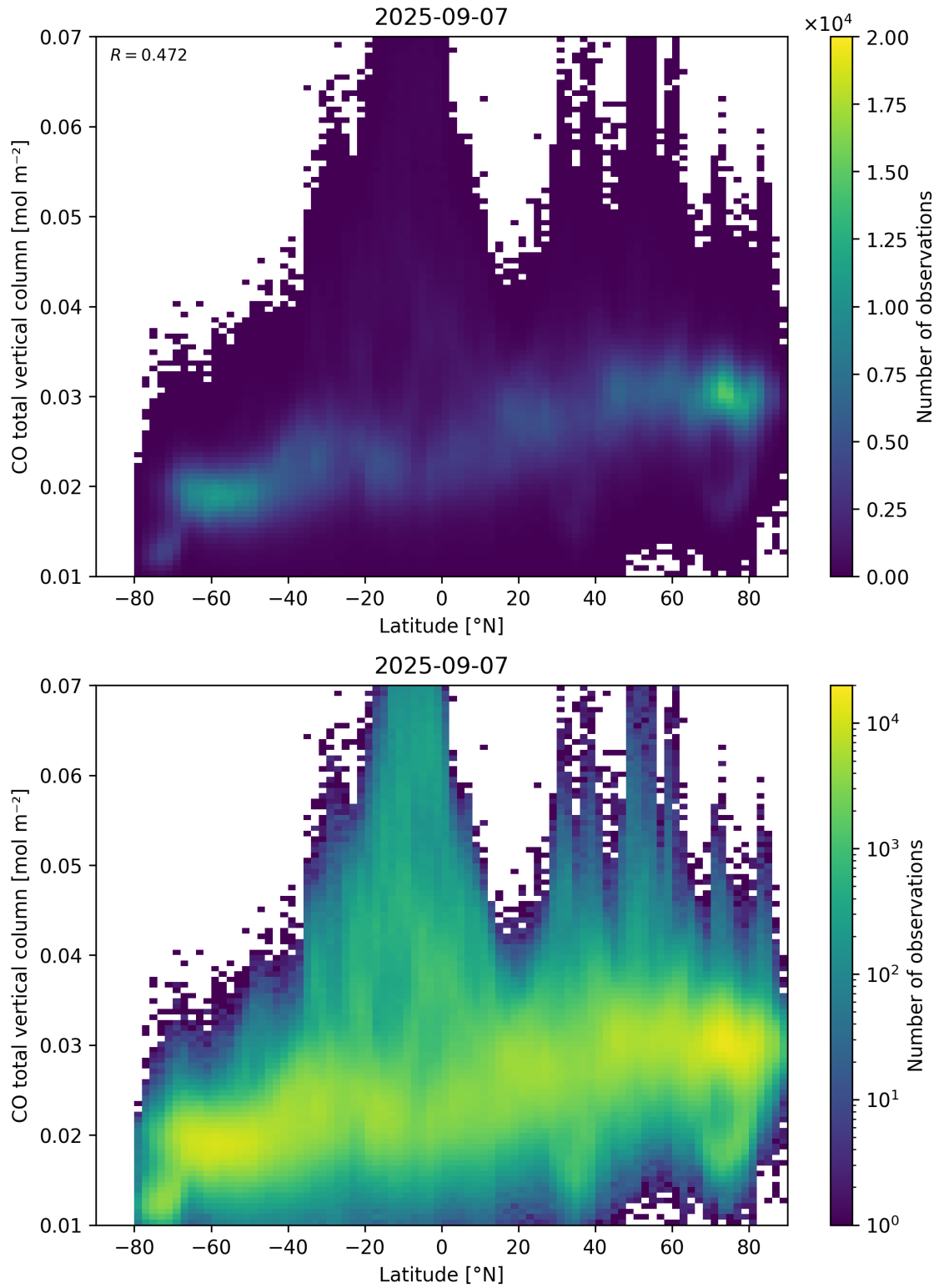
Figure 51: Scatter density plot of “Latitude” against “CO total vertical column” for 2025-09-06 to 2025-09-08.
