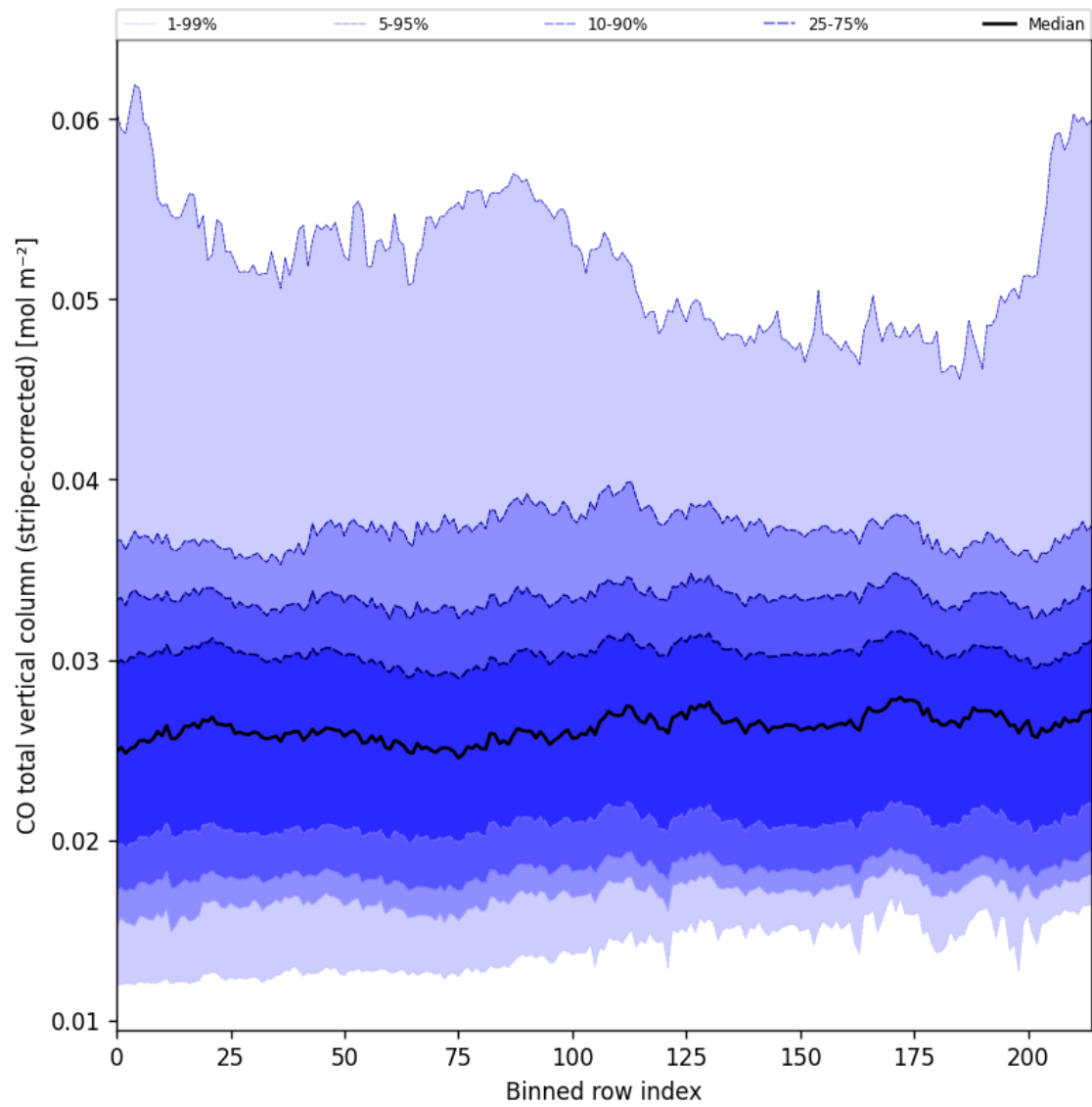
Figure 27: Along track statistics of “CO total vertical column (stripe-corrected)” for 2025-09-06 to 2025-09-08
