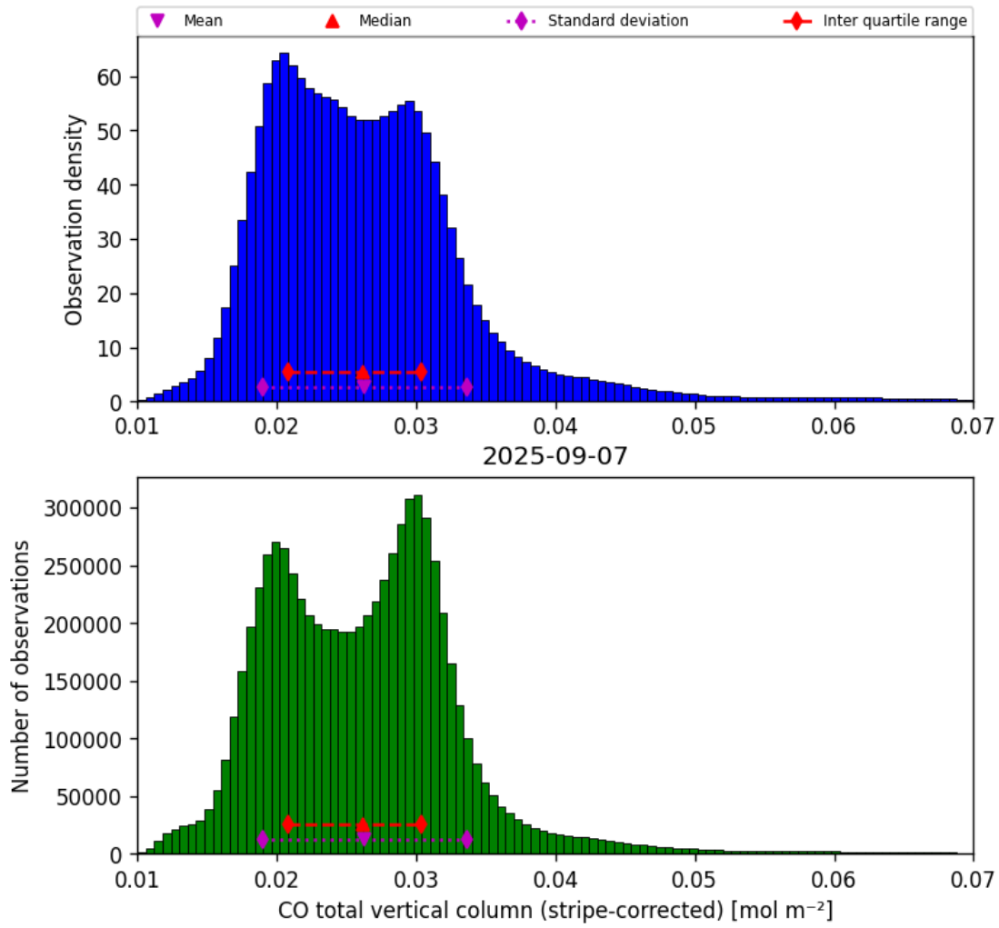
Figure 19: Histogram of “CO total vertical column (stripe-corrected)” for 2025-09-06 to 2025-09-08
