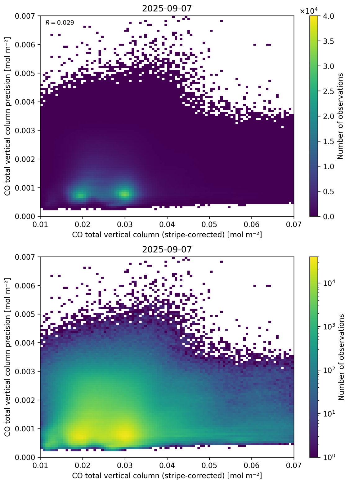
Figure 36: Scatter density plot of “CO total vertical column (stripe-corrected)” against “CO total vertical column precision” for 2025-09-06 to 2025-09-08.
