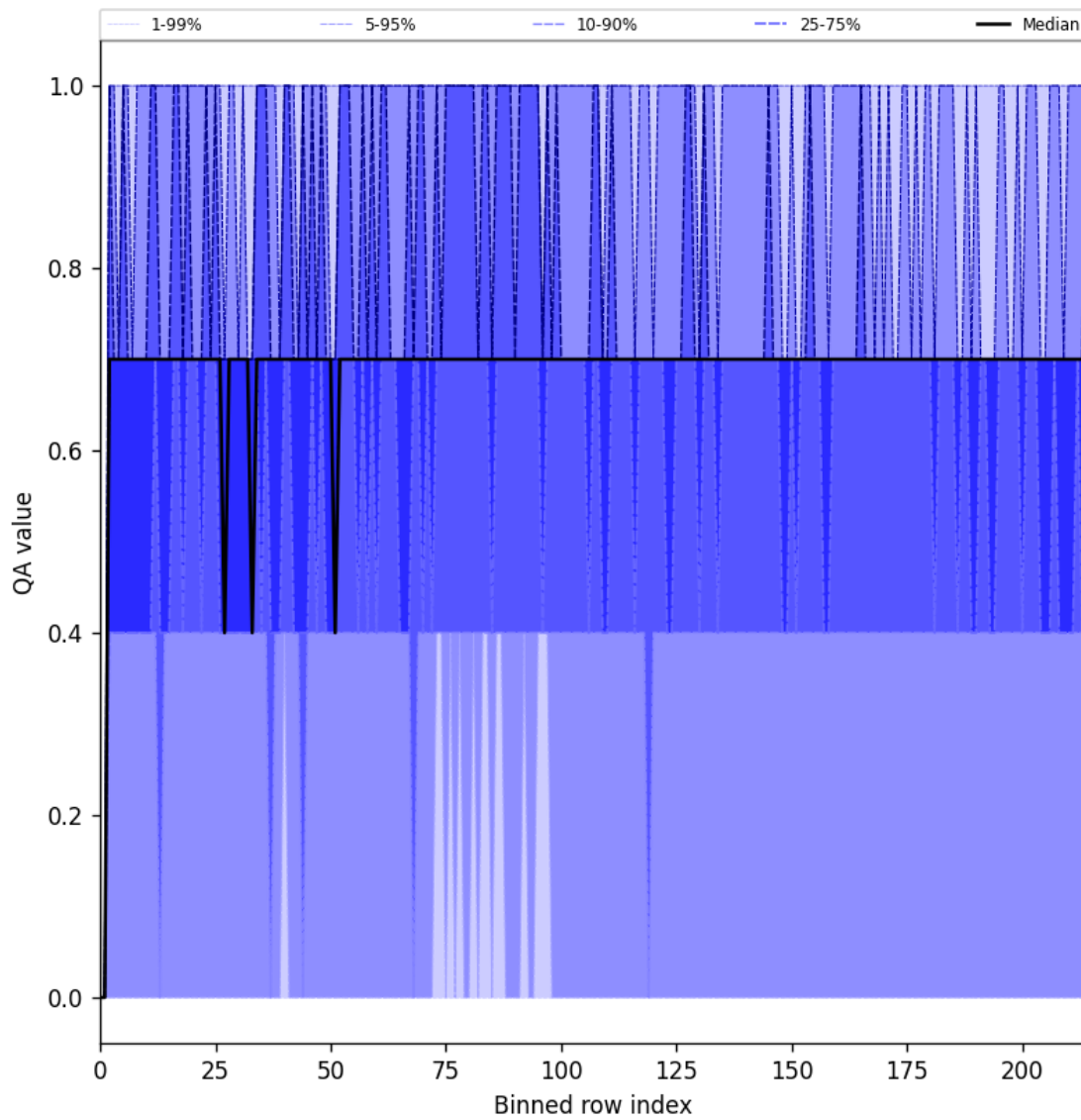
Figure 25: Along track statistics of “QA value” for 2025-09-07 to 2025-09-09
