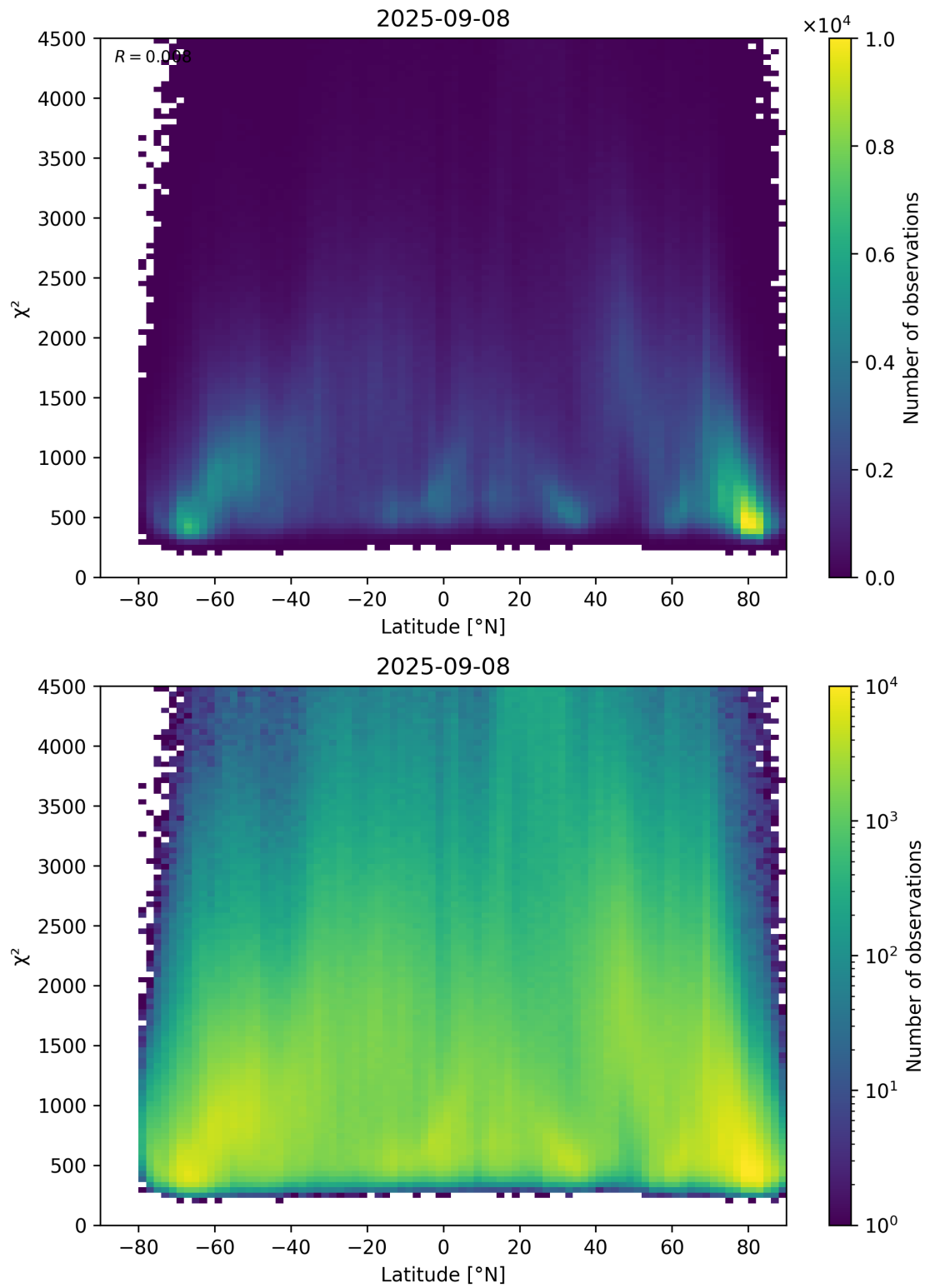
Figure 54: Scatter density plot of “Latitude” against “ \chi^2 ” for 2025-09-07 to 2025-09-09.
