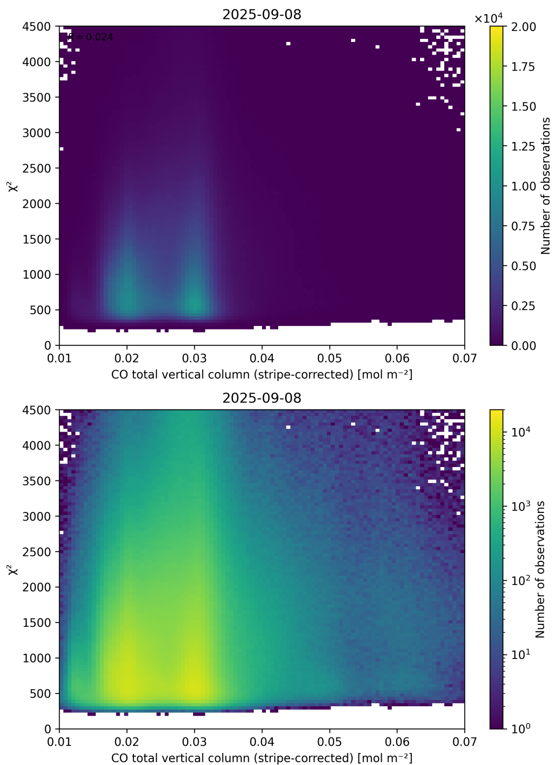
Figure 37: Scatter density plot of “CO total vertical column (stripe-corrected)” against “ \chi^2 ” for 2025-09-07 to 2025-09-09.
