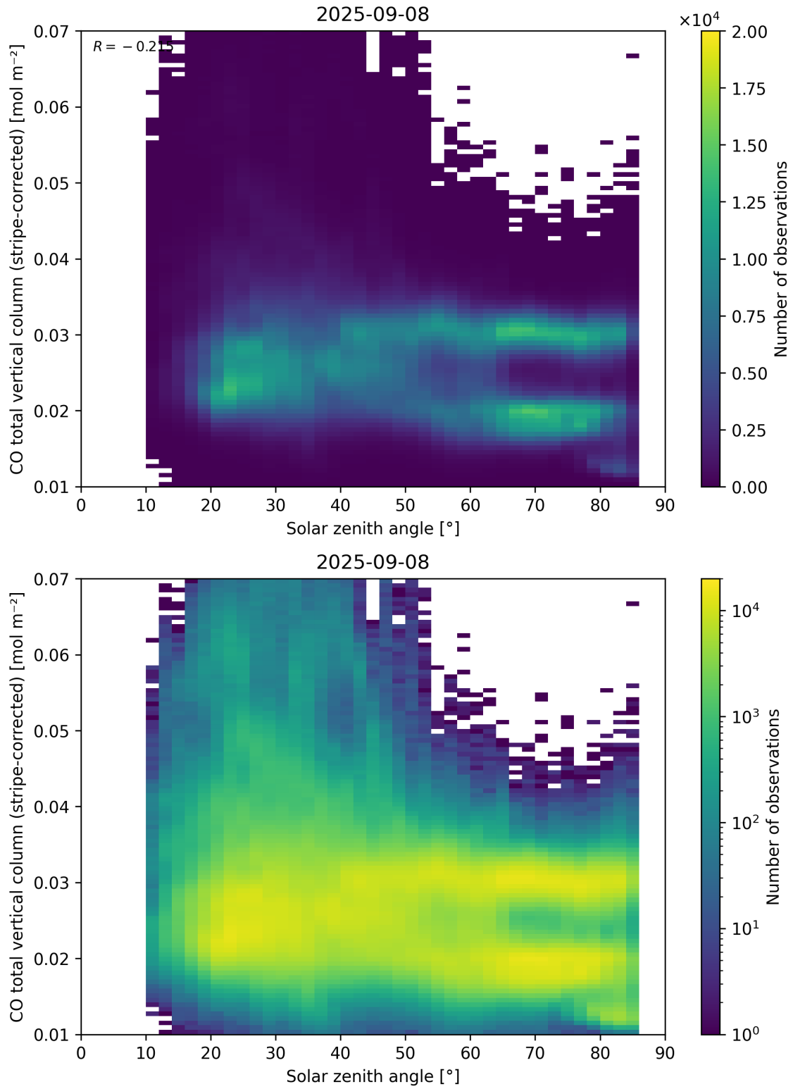
Figure 62: Scatter density plot of “Solar zenith angle” against “CO total vertical column (stripe-corrected)” for 2025-09-07 to 2025-09-09.
