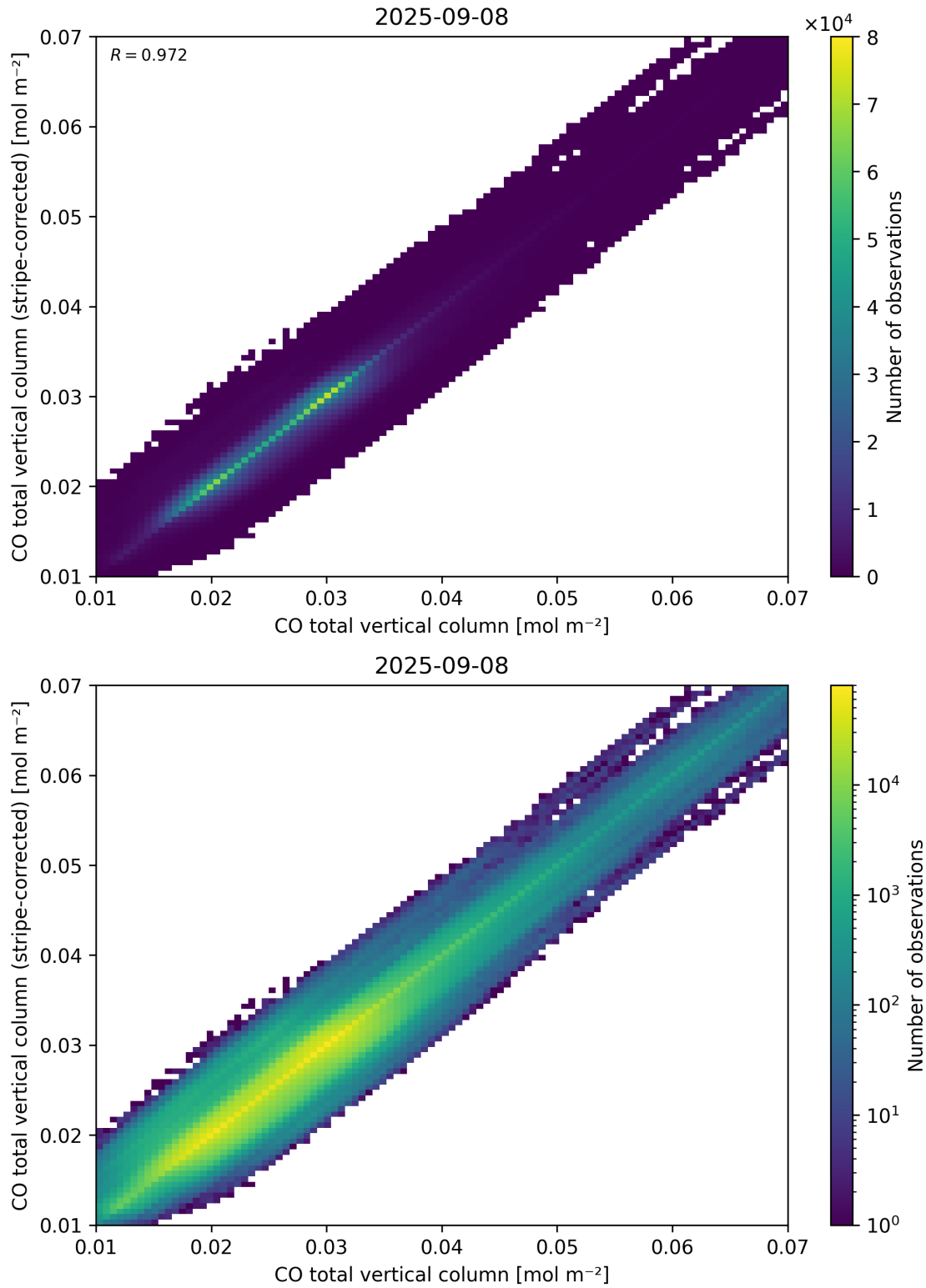
Figure 33: Scatter density plot of “CO total vertical column” against “CO total vertical column (stripe-corrected)” for 2025-09-07 to 2025-09-09.
