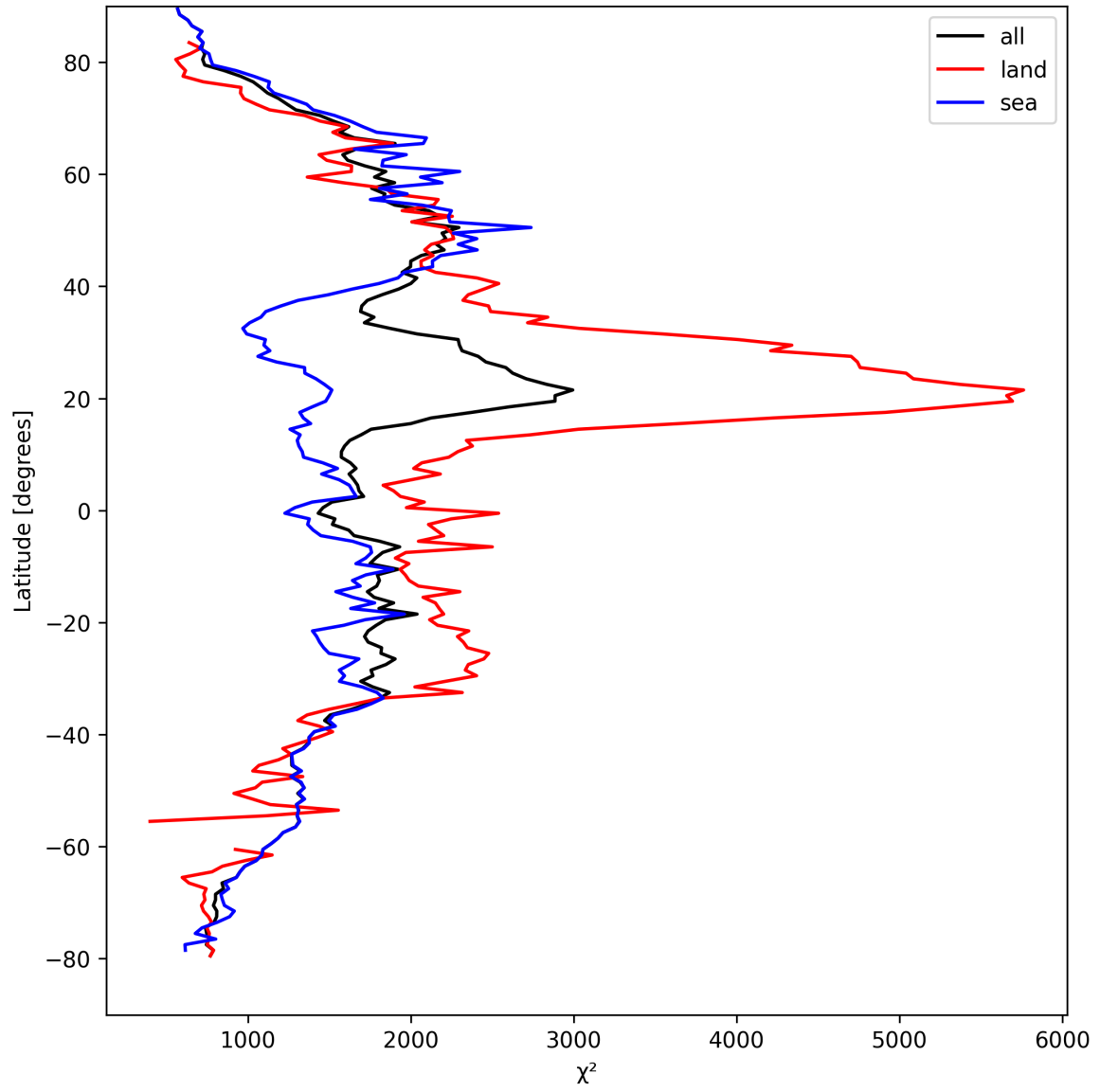
Figure 14: Zonal average of “ \chi^2 ” for 2025-09-07 to 2025-09-09.
