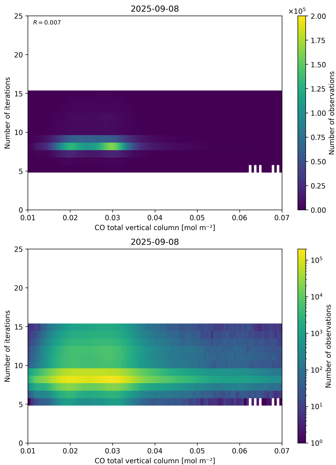
Figure 42: Scatter density plot of “CO total vertical column” against “Number of iterations” for 2025-09-07 to 2025-09-09.
