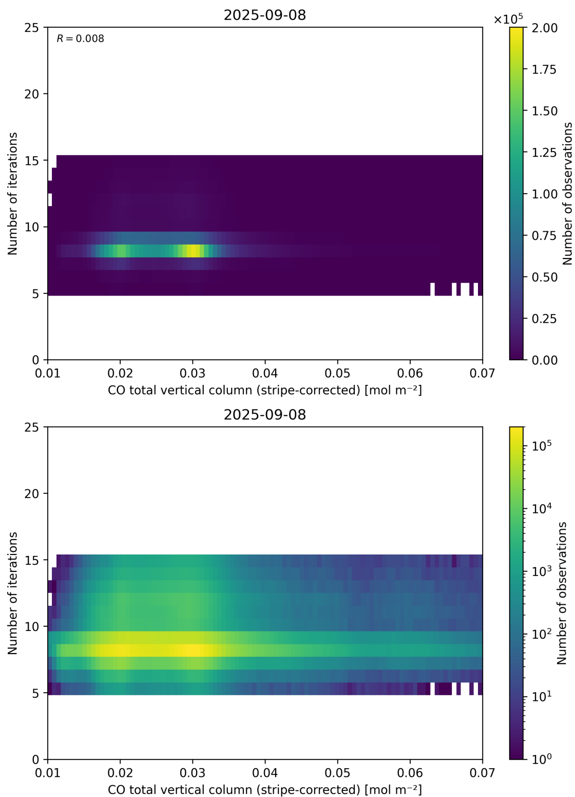
Figure 39: Scatter density plot of “CO total vertical column (stripe-corrected)” against “Number of iterations” for 2025-09-07 to 2025-09-09.
