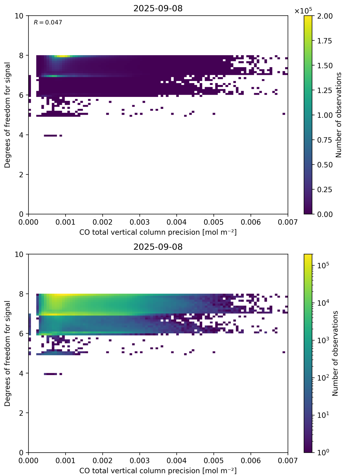
Figure 45: Scatter density plot of “CO total vertical column precision” against “Degrees of freedom for signal” for 2025-09-07 to 2025-09-09.
