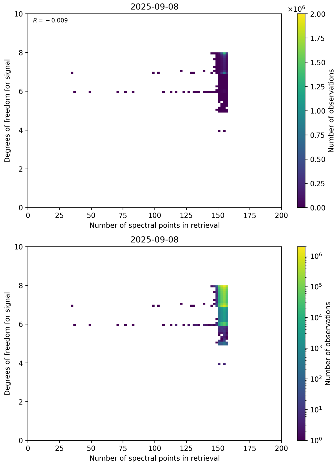
Figure 59: Scatter density plot of “Number of spectral points in retrieval” against “Degrees of freedom for signal” for 2025-09-07 to 2025-09-09.
