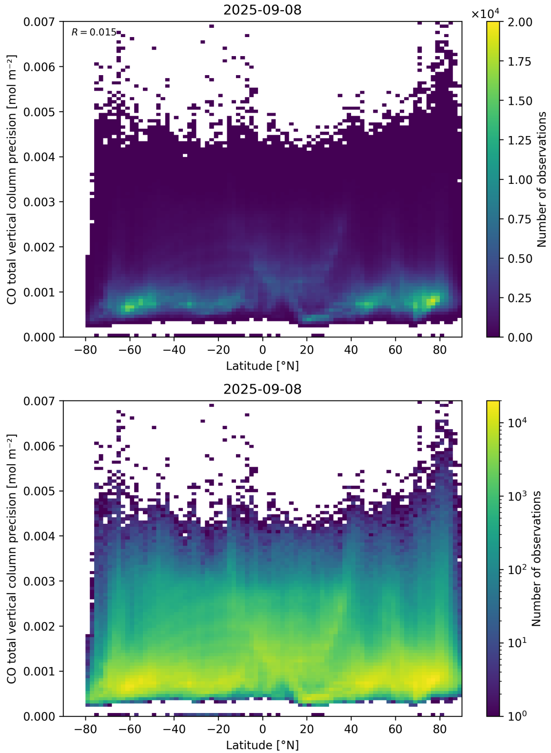
Figure 53: Scatter density plot of “Latitude” against “CO total vertical column precision” for 2025-09-07 to 2025-09-09.
