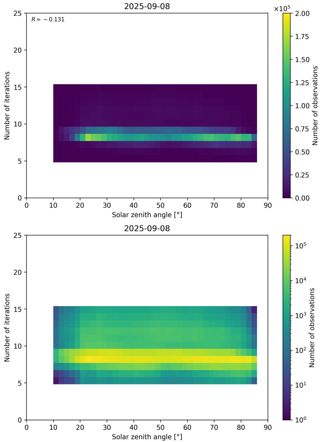
Figure 67: Scatter density plot of “Solar zenith angle” against “Number of iterations” for 2025-09-07 to 2025-09-09.
