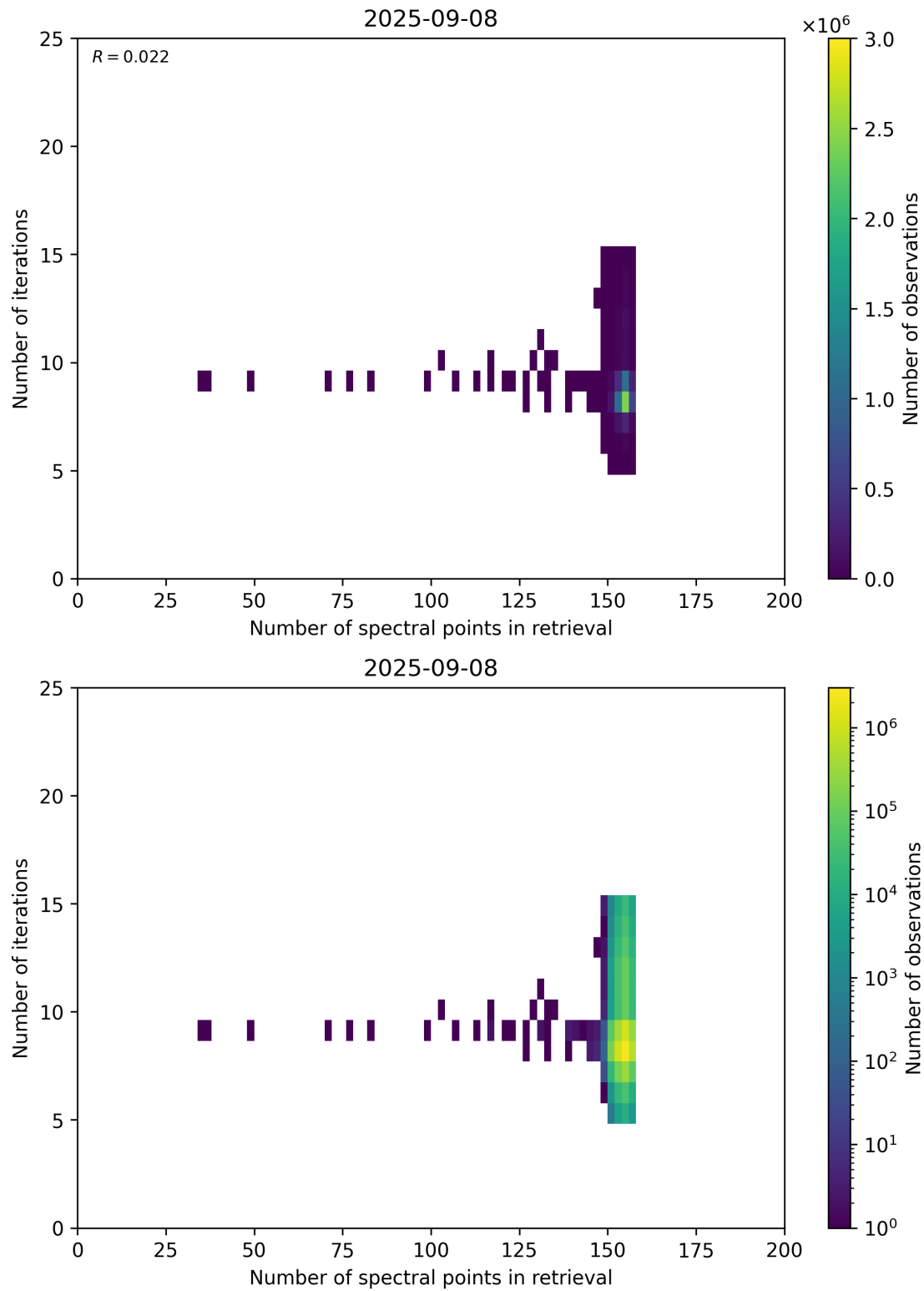
Figure 60: Scatter density plot of “Number of spectral points in retrieval” against “Number of iterations” for 2025-09-07 to 2025-09-09.
