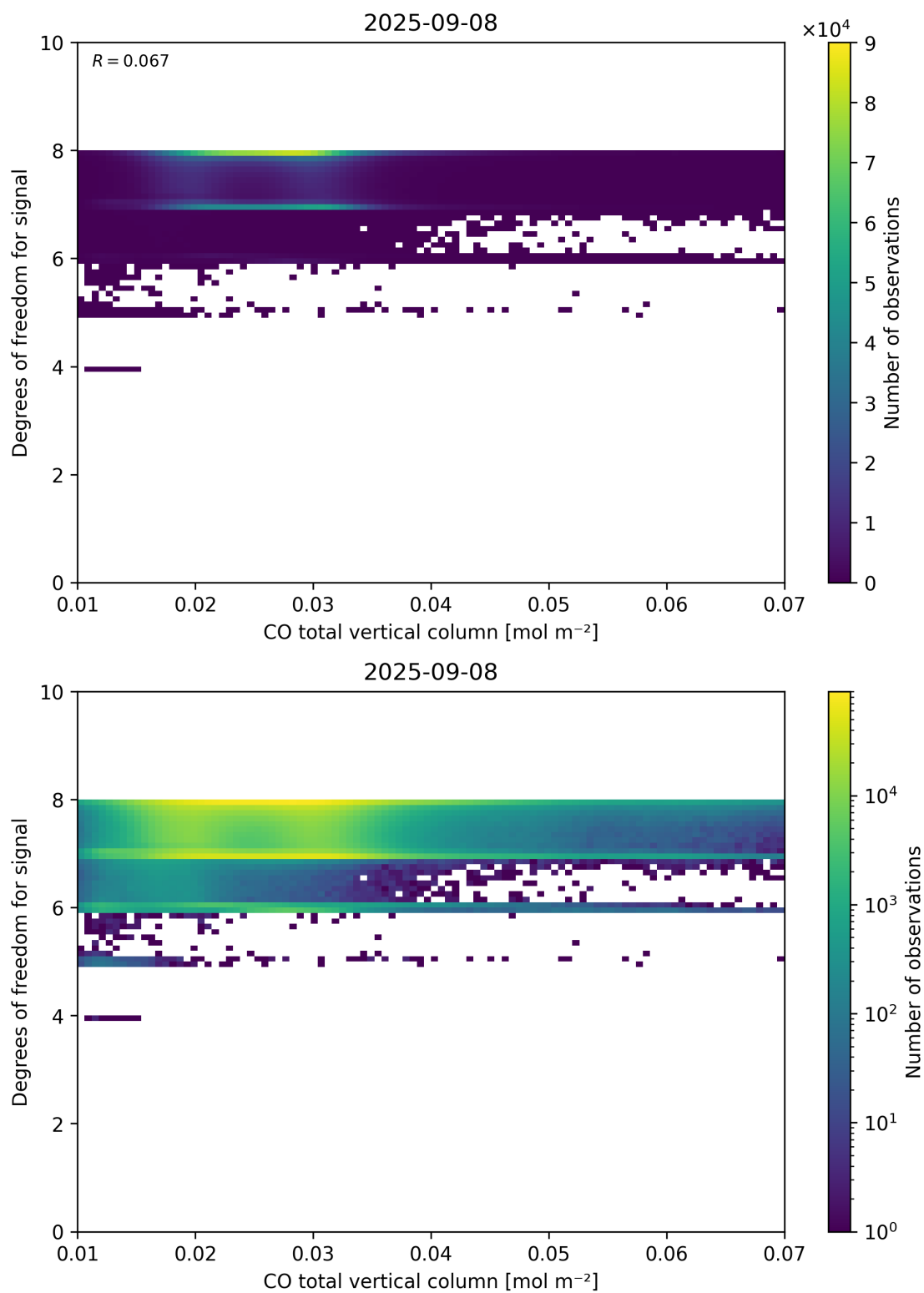
Figure 41: Scatter density plot of “CO total vertical column” against “Degrees of freedom for signal” for 2025-09-07 to 2025-09-09.
