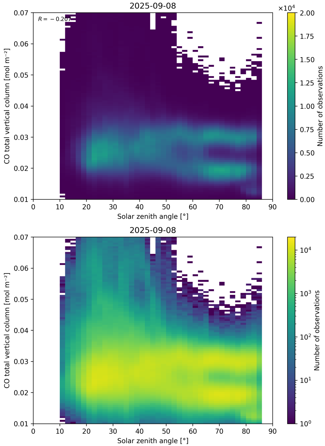
Figure 61: Scatter density plot of “Solar zenith angle” against “CO total vertical column” for 2025-09-07 to 2025-09-09.
