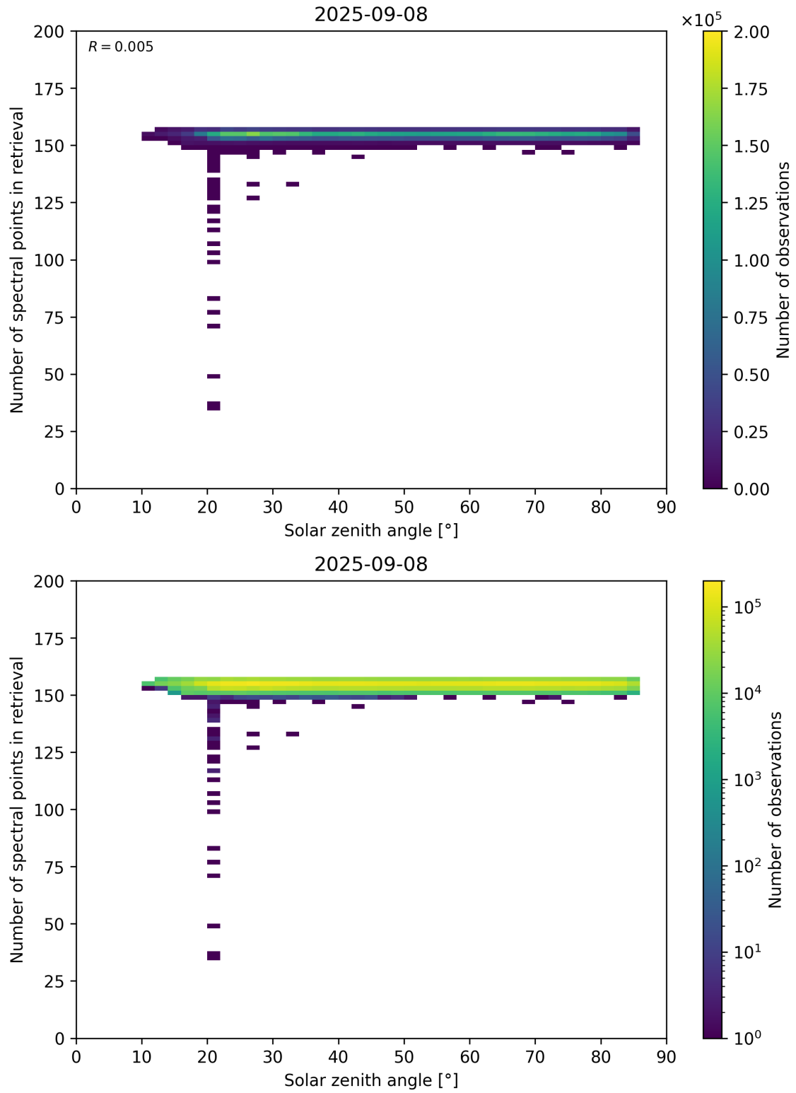
Figure 68: Scatter density plot of “Solar zenith angle” against “Number of spectral points in retrieval” for 2025-09-07 to 2025-09-09.
