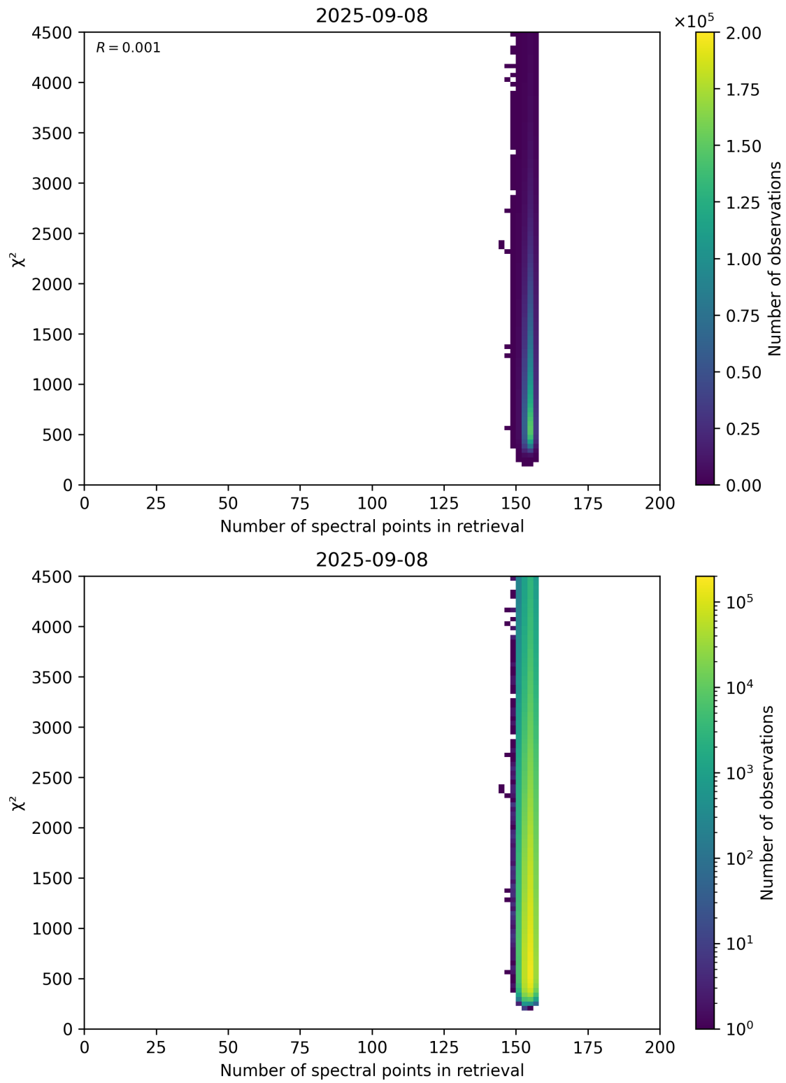
Figure 58: Scatter density plot of “Number of spectral points in retrieval” against “ \chi^2 ” for 2025-09-07 to 2025-09-09.
