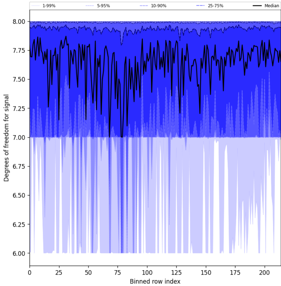
Figure 31: Along track statistics of “Degrees of freedom for signal” for 2025-09-07 to 2025-09-09
