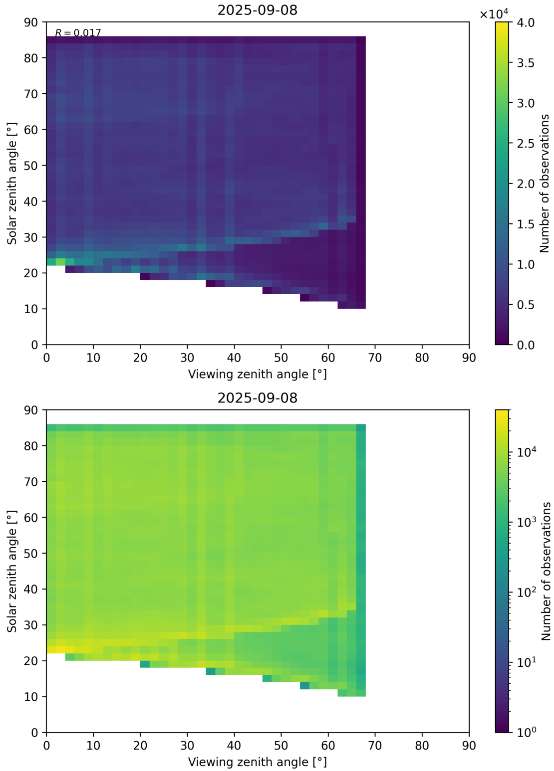
Figure 77: Scatter density plot of “Viewing zenith angle” against “Solar zenith angle” for 2025-09-07 to 2025-09-09.
