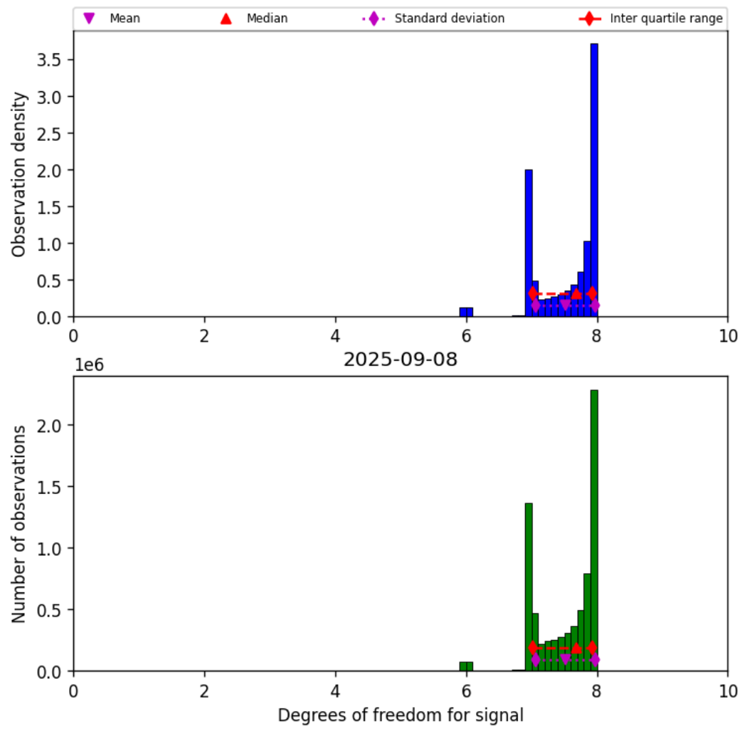
Figure 23: Histogram of “Degrees of freedom for signal” for 2025-09-07 to 2025-09-09
