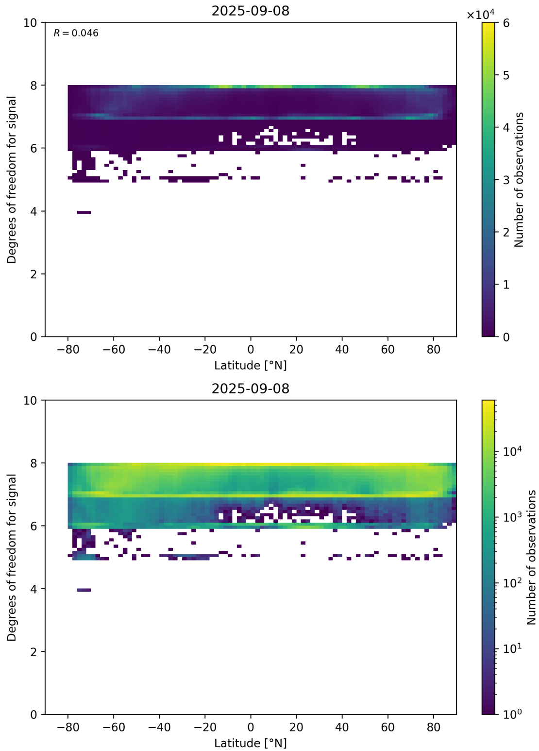
Figure 55: Scatter density plot of “Latitude” against “Degrees of freedom for signal” for 2025-09-07 to 2025-09-09.
