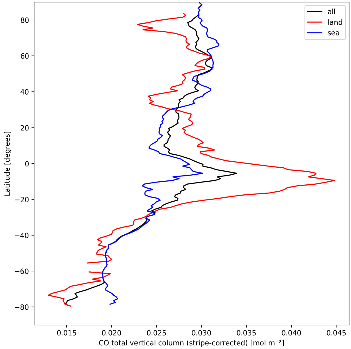
Figure 11: Zonal average of “CO total vertical column (stripe-corrected)” for 2025-09-07 to 2025-09-09.
