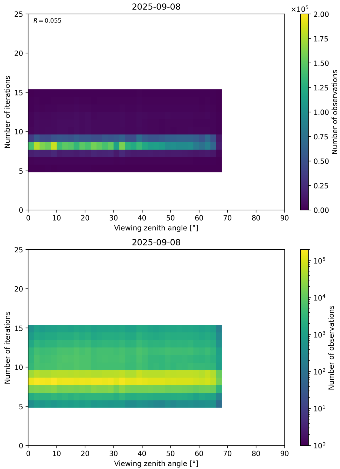
Figure 75: Scatter density plot of “Viewing zenith angle” against “Number of iterations” for 2025-09-07 to 2025-09-09.
