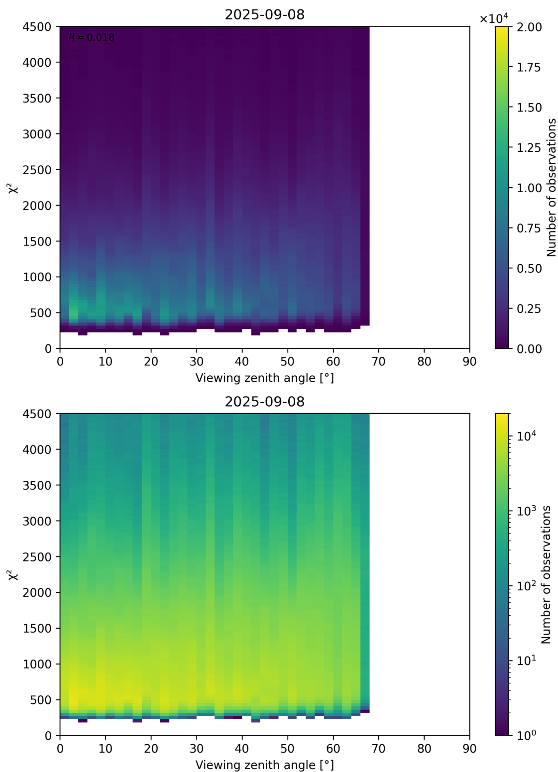
Figure 72: Scatter density plot of “Viewing zenith angle” against “ \chi^2 ” for 2025-09-07 to 2025-09-09.
