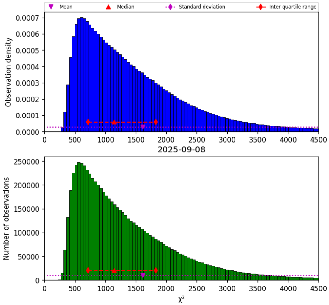
Figure 22: Histogram of " \chi^2 " for 2025-09-07 to 2025-09-09
