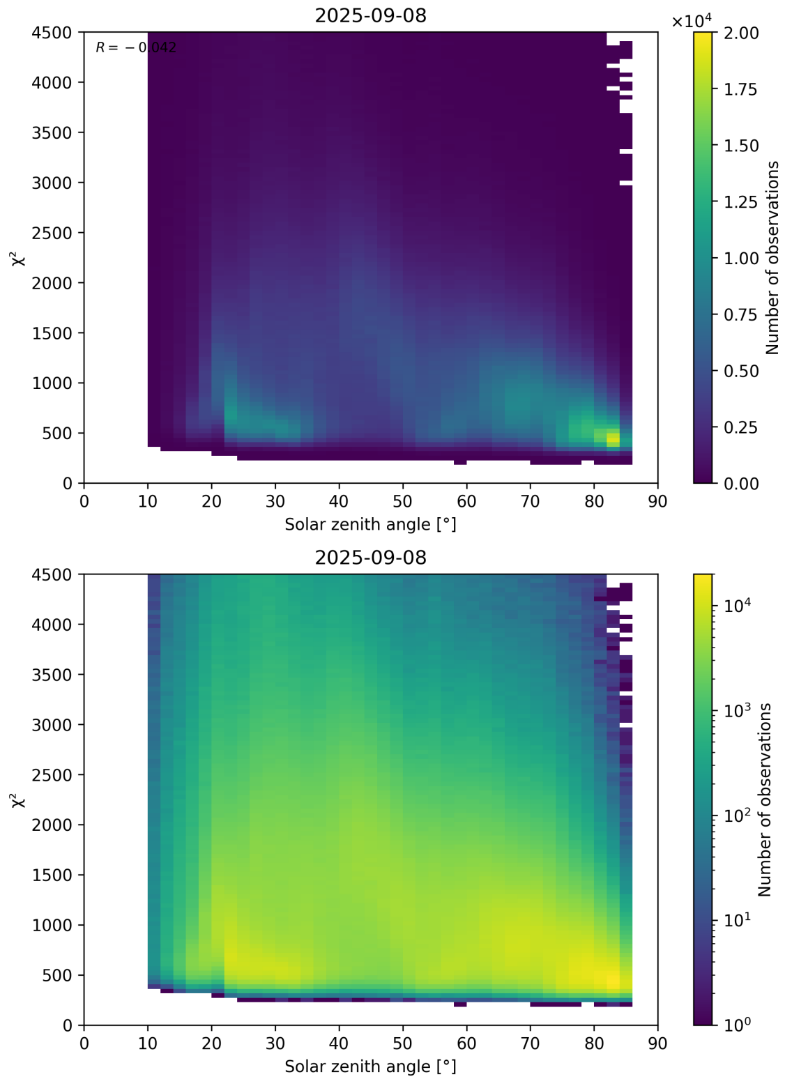
Figure 64: Scatter density plot of “Solar zenith angle” against “ \chi^2 ” for 2025-09-07 to 2025-09-09.
