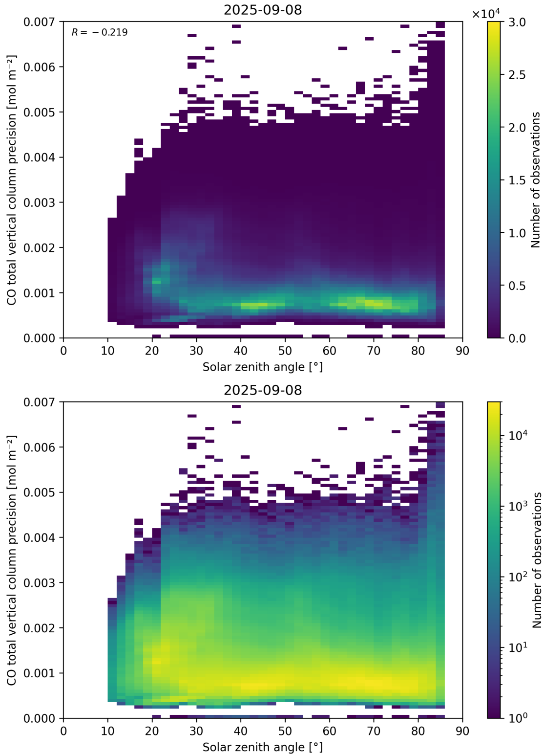
Figure 63: Scatter density plot of “Solar zenith angle” against “CO total vertical column precision” for 2025-09-07 to 2025-09-09.
