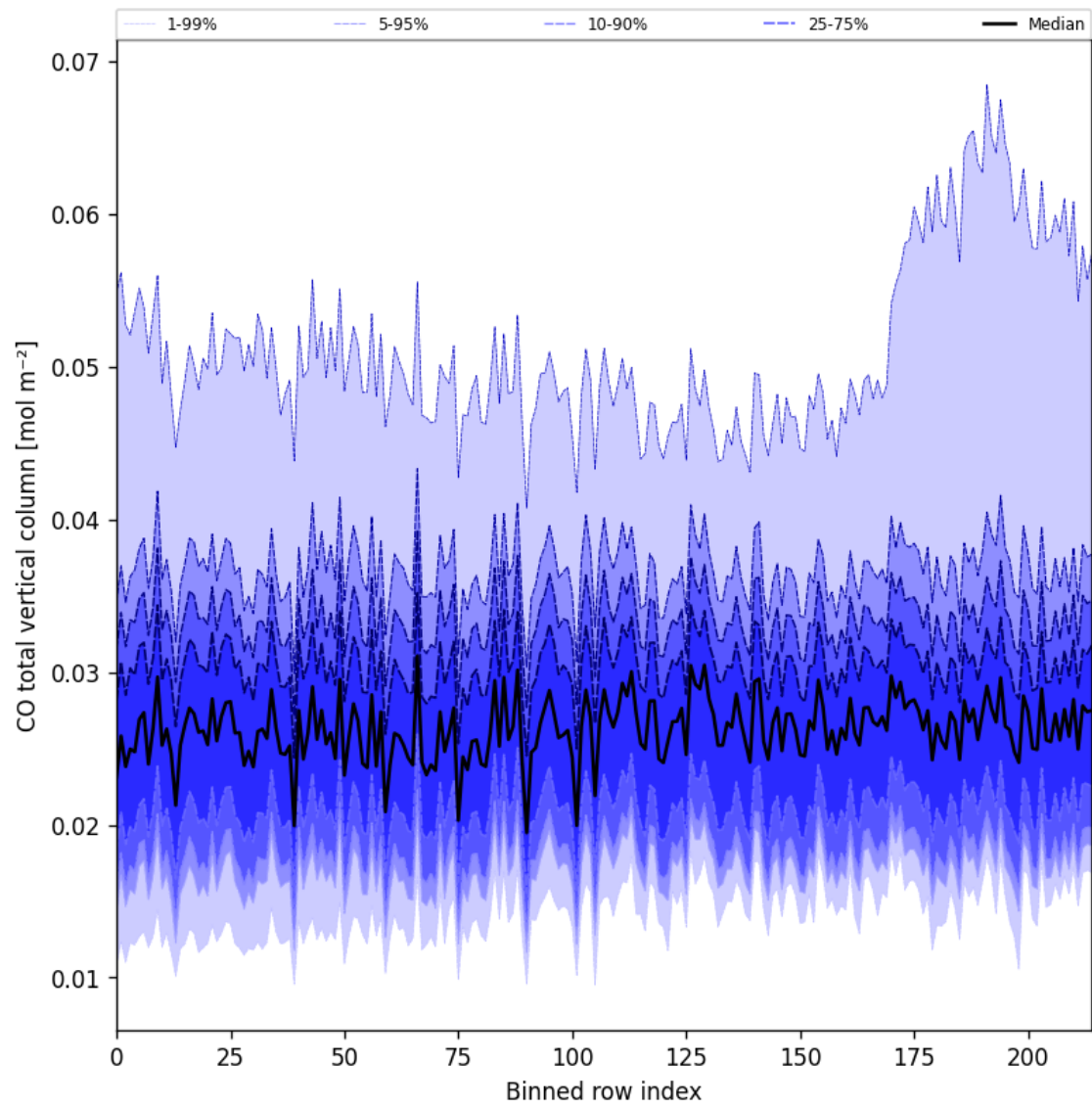
Figure 26: Along track statistics of “CO total vertical column” for 2025-09-07 to 2025-09-09
