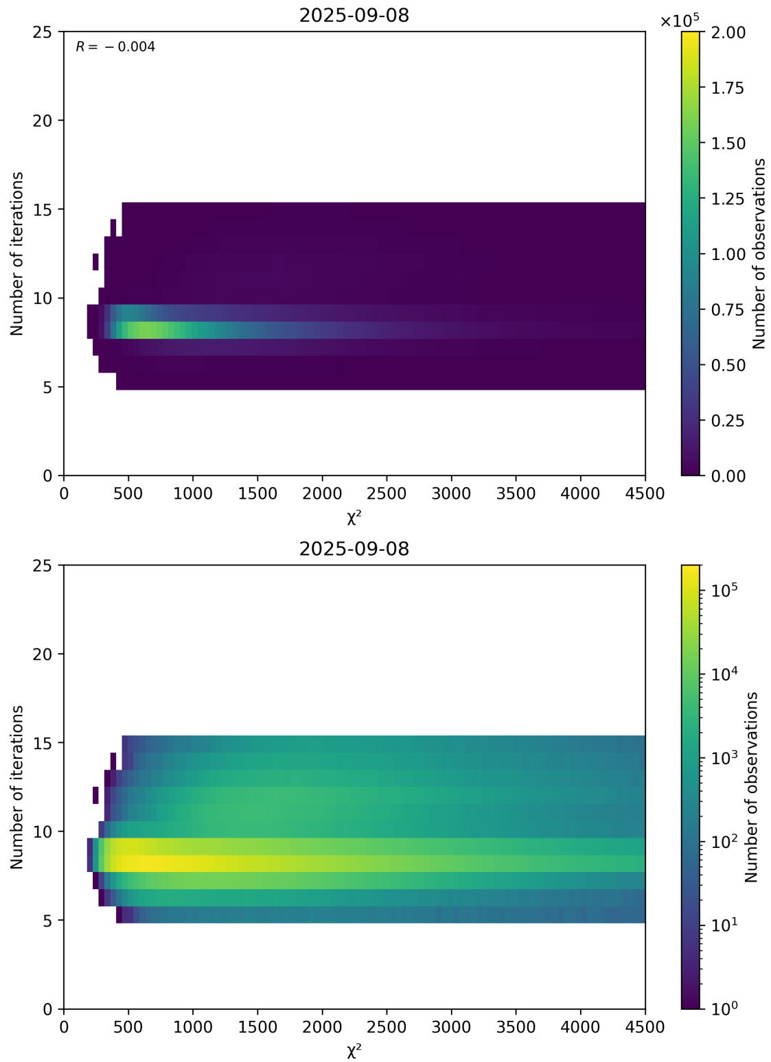
Figure 49: Scatter density plot of “ \chi^2 ” against “Number of iterations” for 2025-09-07 to 2025-09-09.
