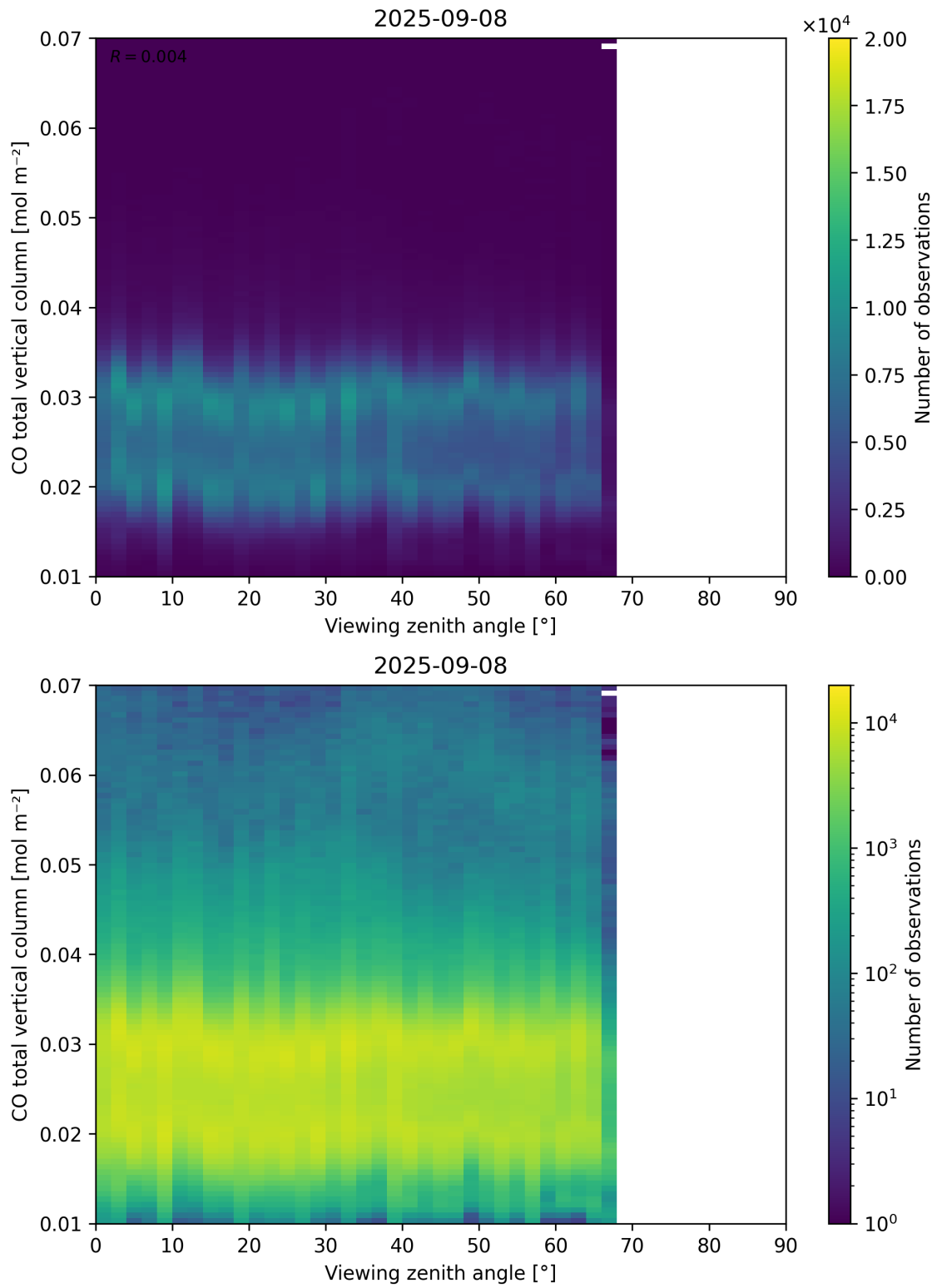
Figure 69: Scatter density plot of “Viewing zenith angle” against “CO total vertical column” for 2025-09-07 to 2025-09-09.
