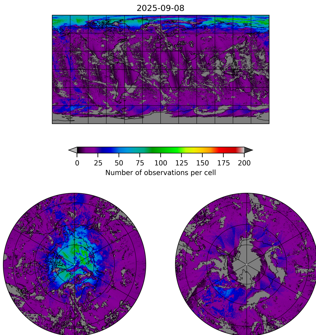
Figure 8: Map of the number of observations for 2025-09-07 to 2025-09-09
