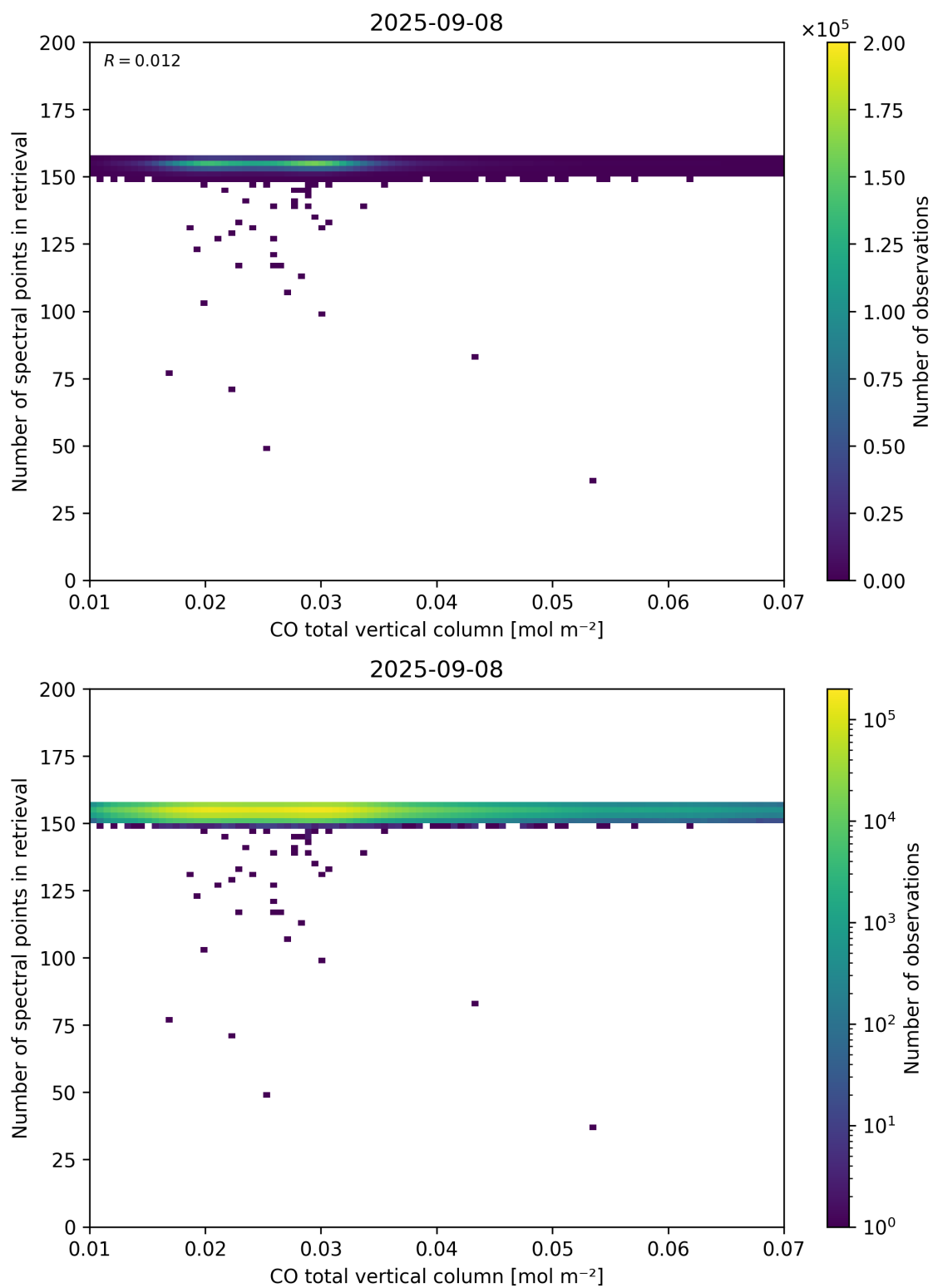
Figure 43: Scatter density plot of “CO total vertical column” against “Number of spectral points in retrieval” for 2025-09-07 to 2025-09-09.
