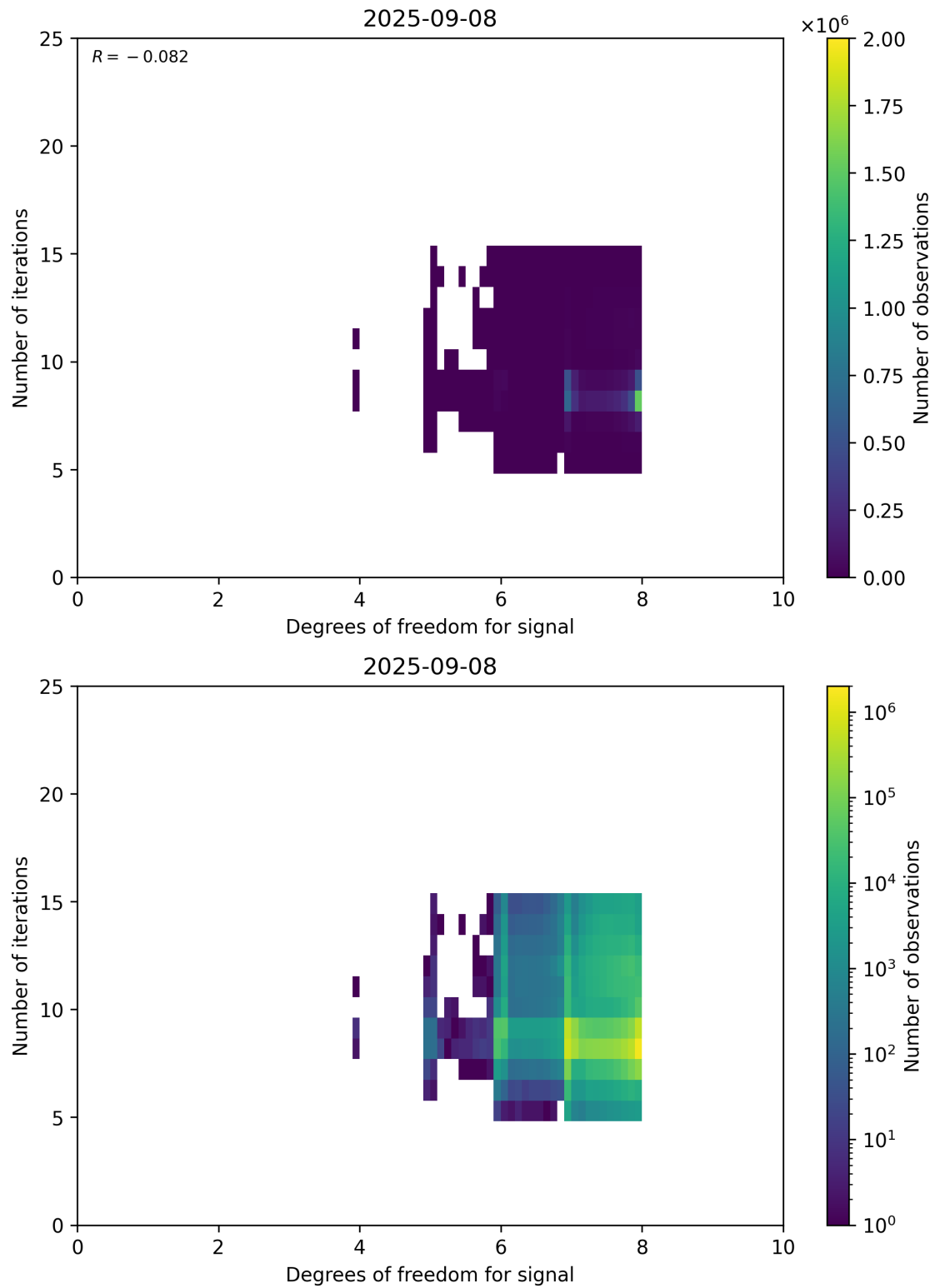
Figure 50: Scatter density plot of “Degrees of freedom for signal” against “Number of iterations” for 2025-09-07 to 2025-09-09.
