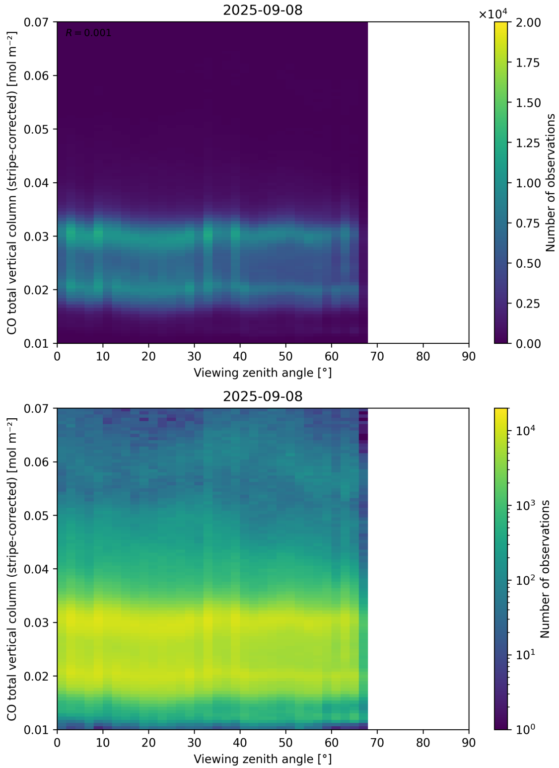
Figure 70: Scatter density plot of “Viewing zenith angle” against “CO total vertical column (stripe-corrected)” for 2025-09-07 to 2025-09-09.
