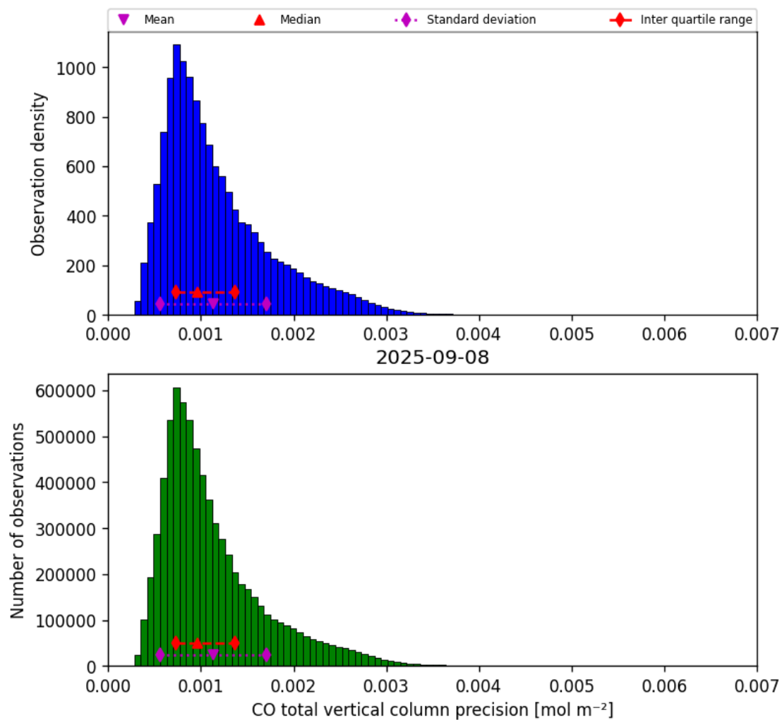
Figure 20: Histogram of “CO total vertical column precision” for 2025-09-07 to 2025-09-09
