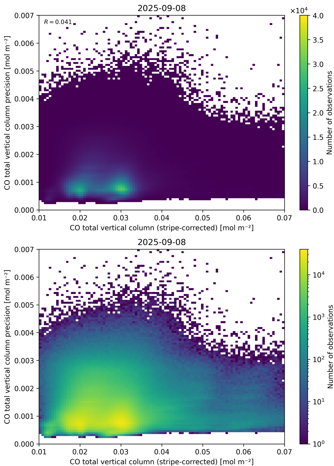
Figure 36: Scatter density plot of “CO total vertical column (stripe-corrected)” against “CO total vertical column precision” for 2025-09-07 to 2025-09-09.
