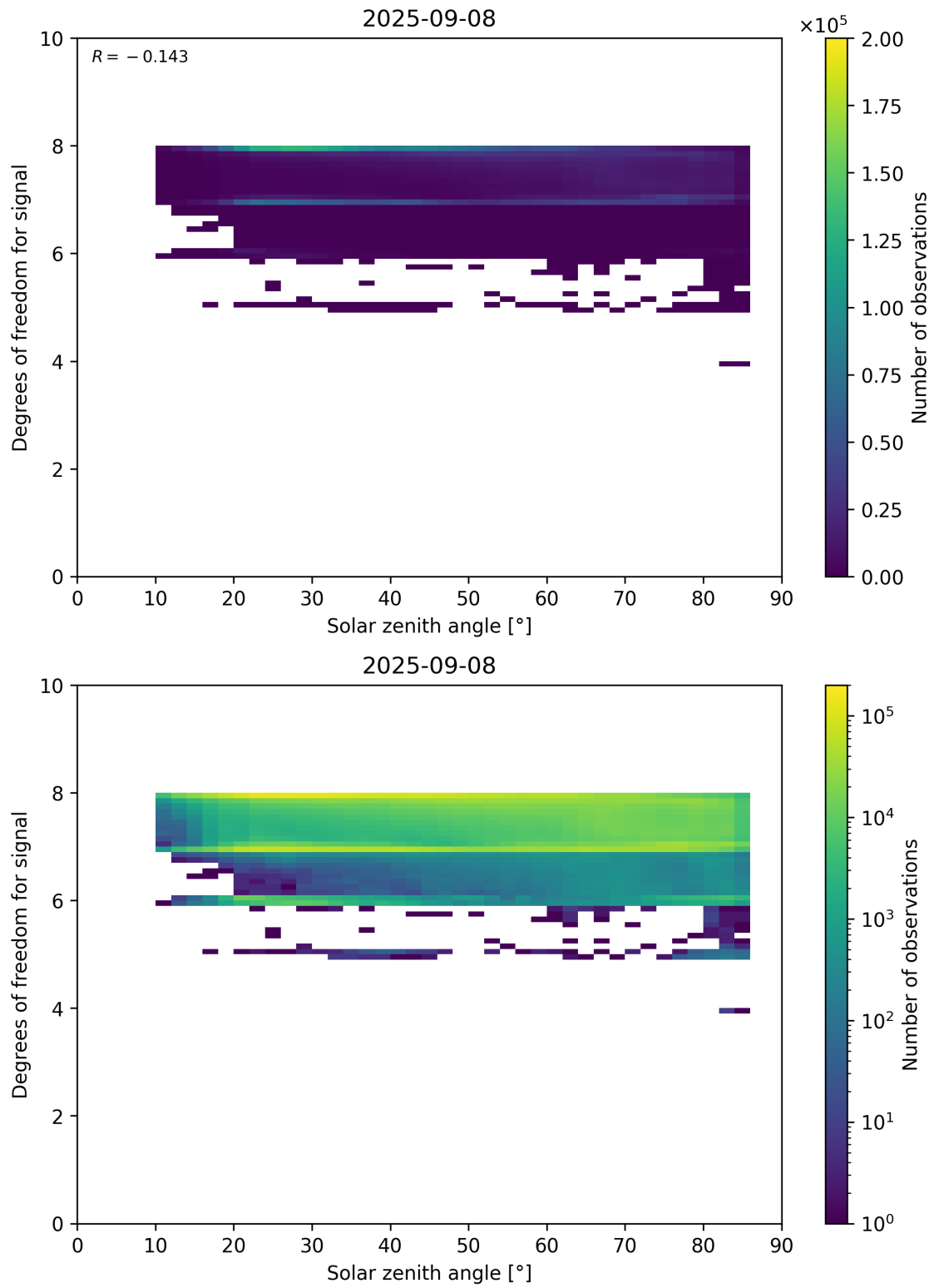
Figure 65: Scatter density plot of “Solar zenith angle” against “Degrees of freedom for signal” for 2025-09-07 to 2025-09-09.
