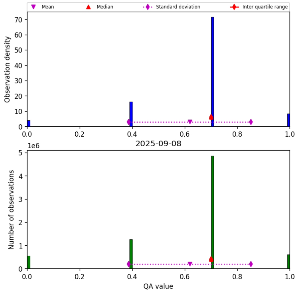
Figure 17: Histogram of “QA value” for 2025-09-07 to 2025-09-09
