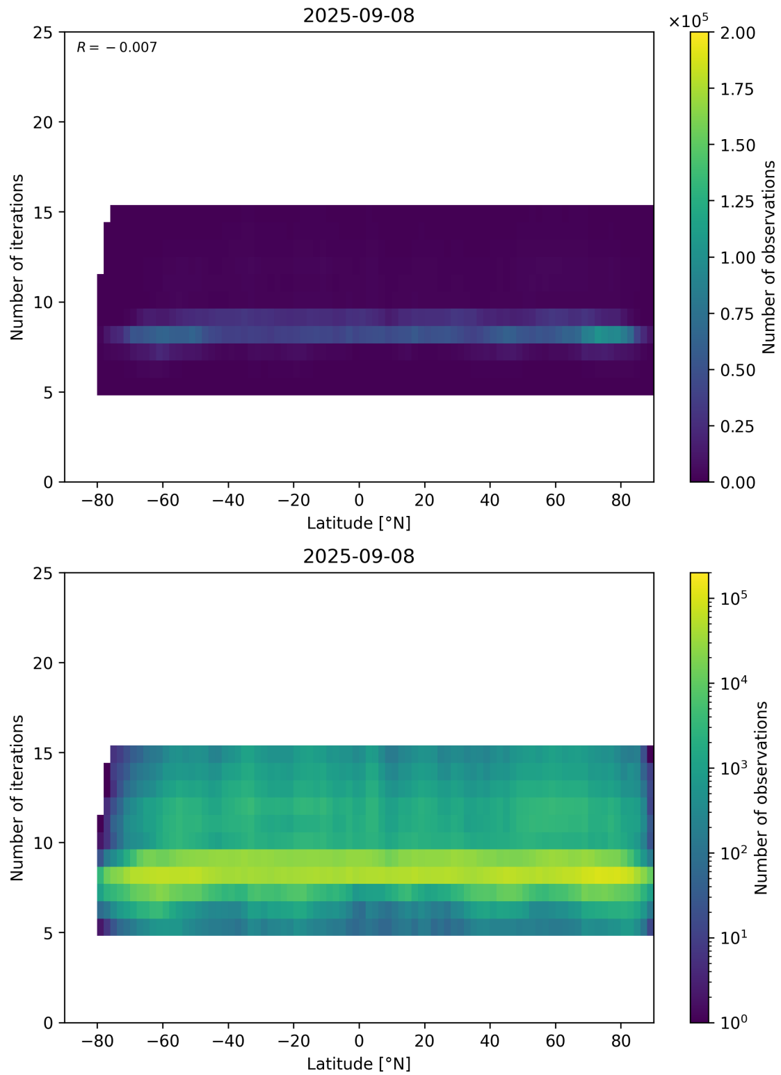
Figure 56: Scatter density plot of “Latitude” against “Number of iterations” for 2025-09-07 to 2025-09-09.
