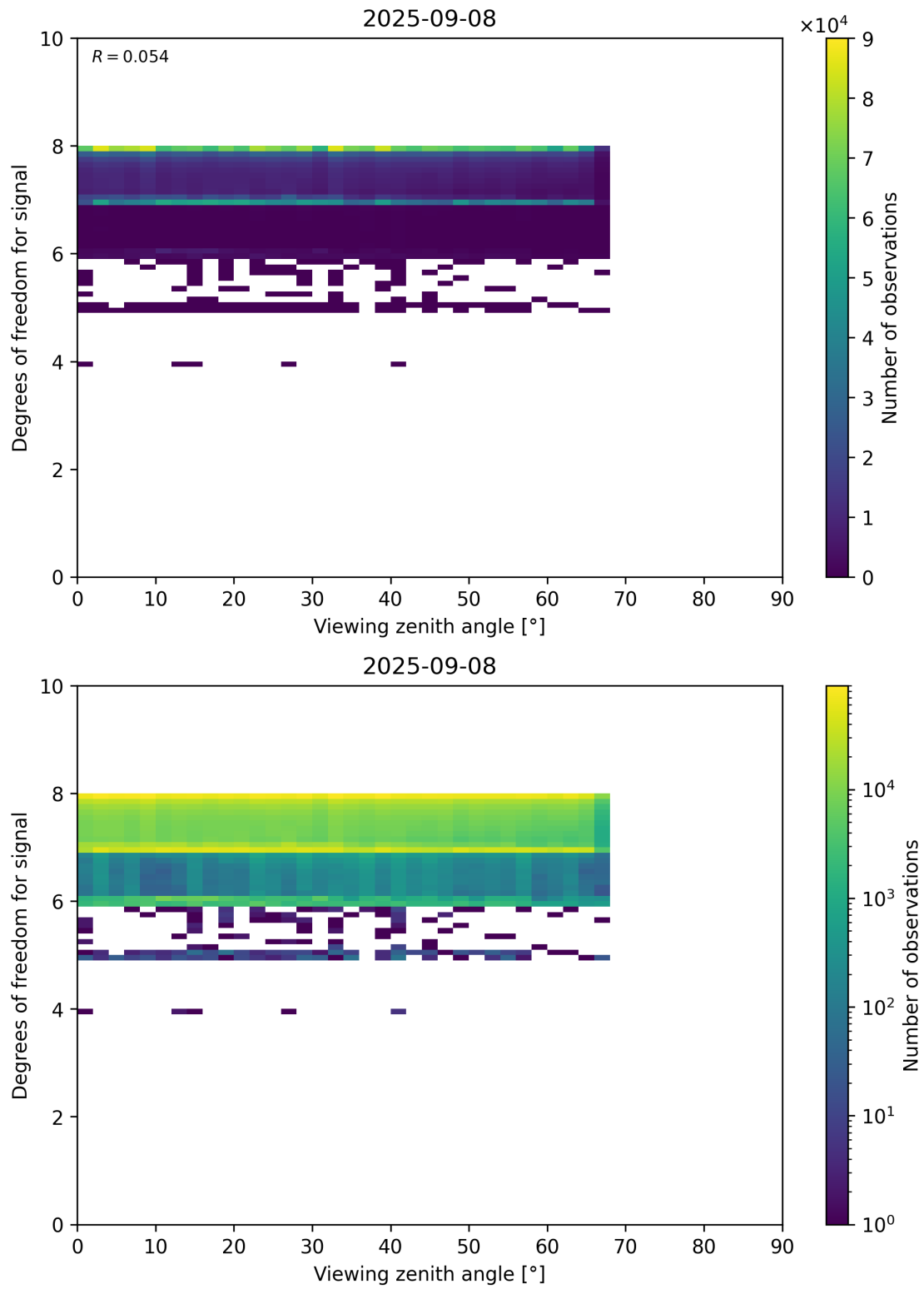
Figure 73: Scatter density plot of “Viewing zenith angle” against “Degrees of freedom for signal” for 2025-09-07 to 2025-09-09.
