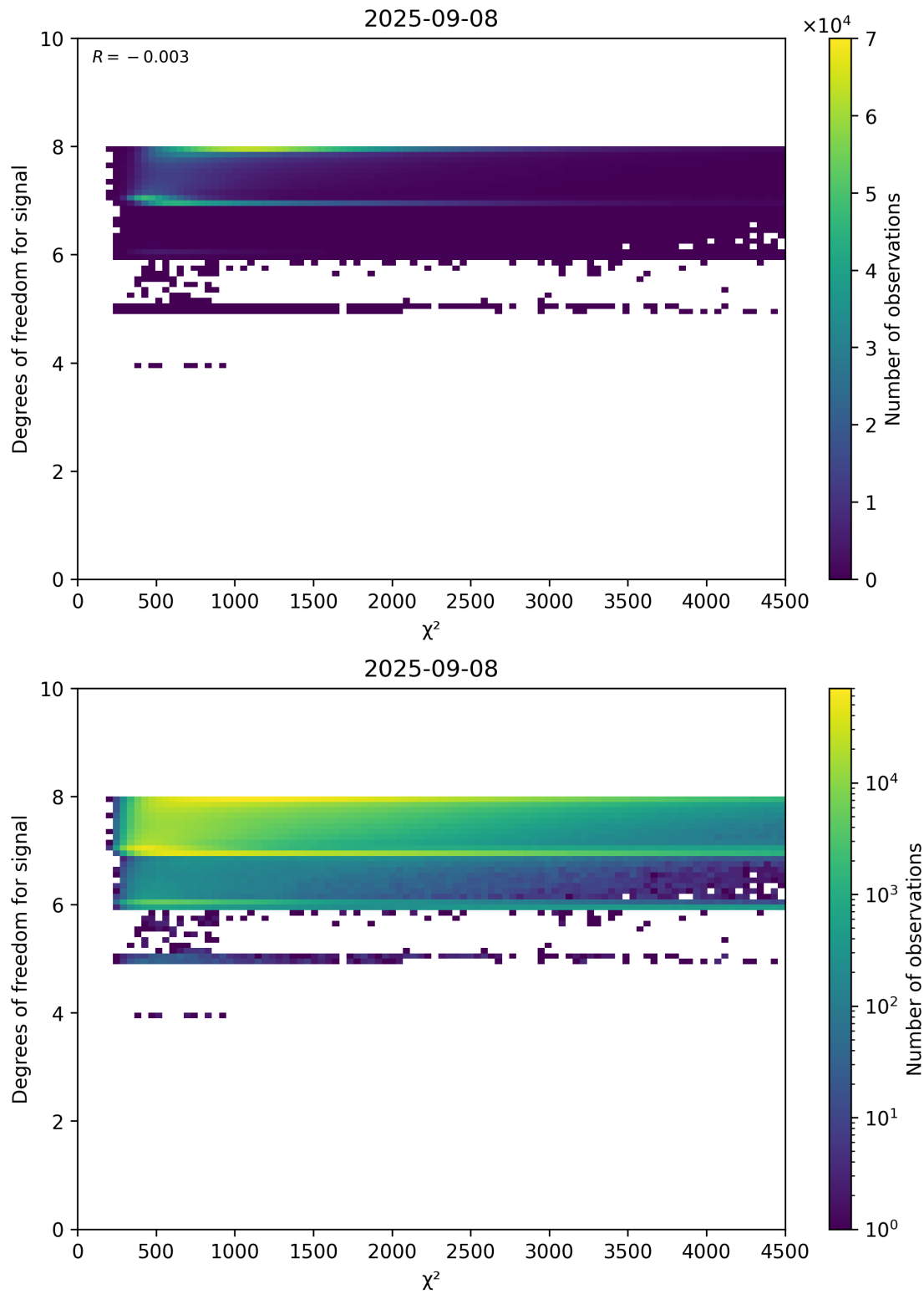
Figure 48: Scatter density plot of “ \chi^2 ” against “Degrees of freedom for signal” for 2025-09-07 to 2025-09-09.
