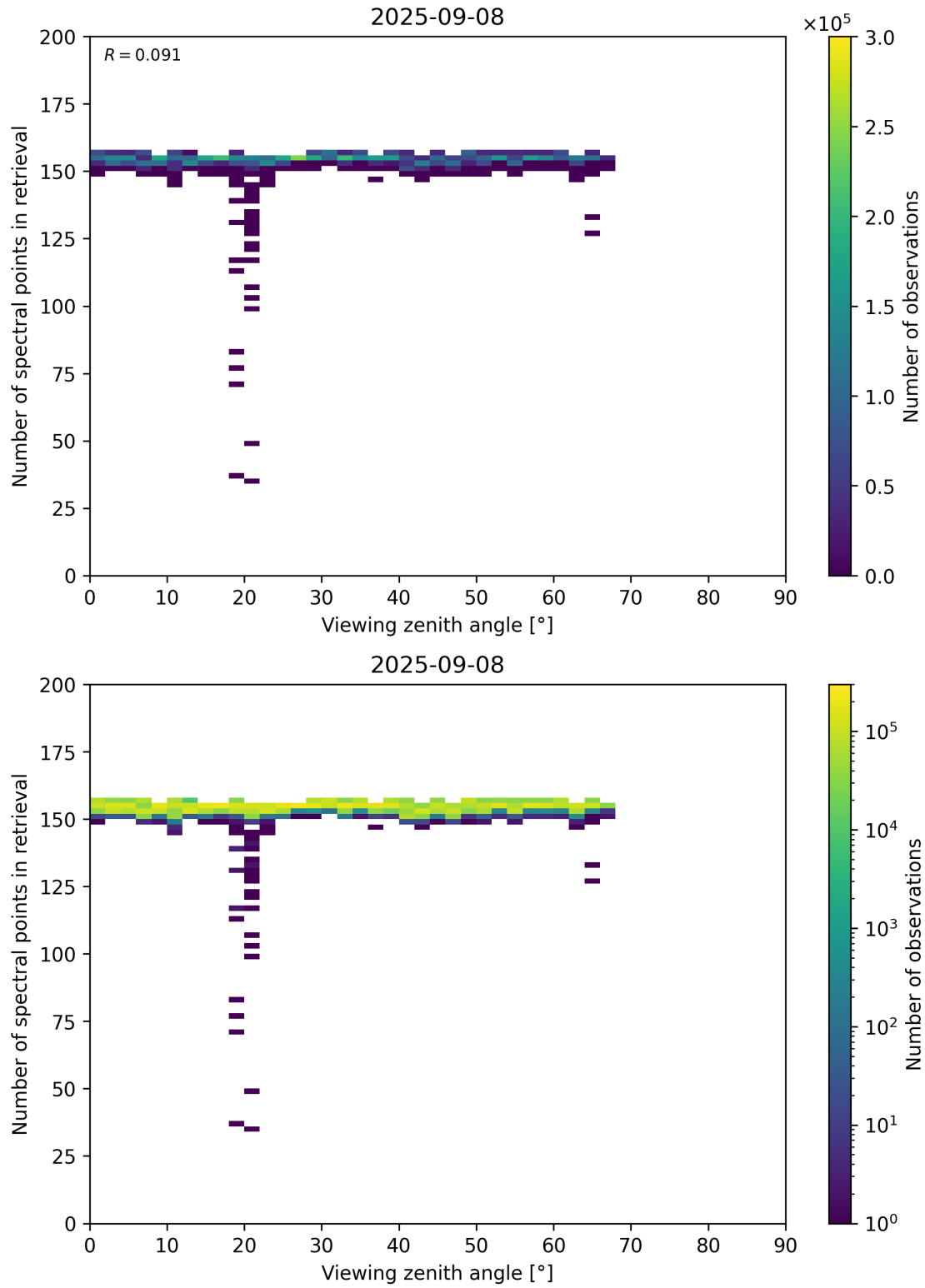
Figure 76: Scatter density plot of “Viewing zenith angle” against “Number of spectral points in retrieval” for 2025-09-07 to 2025-09-09.
