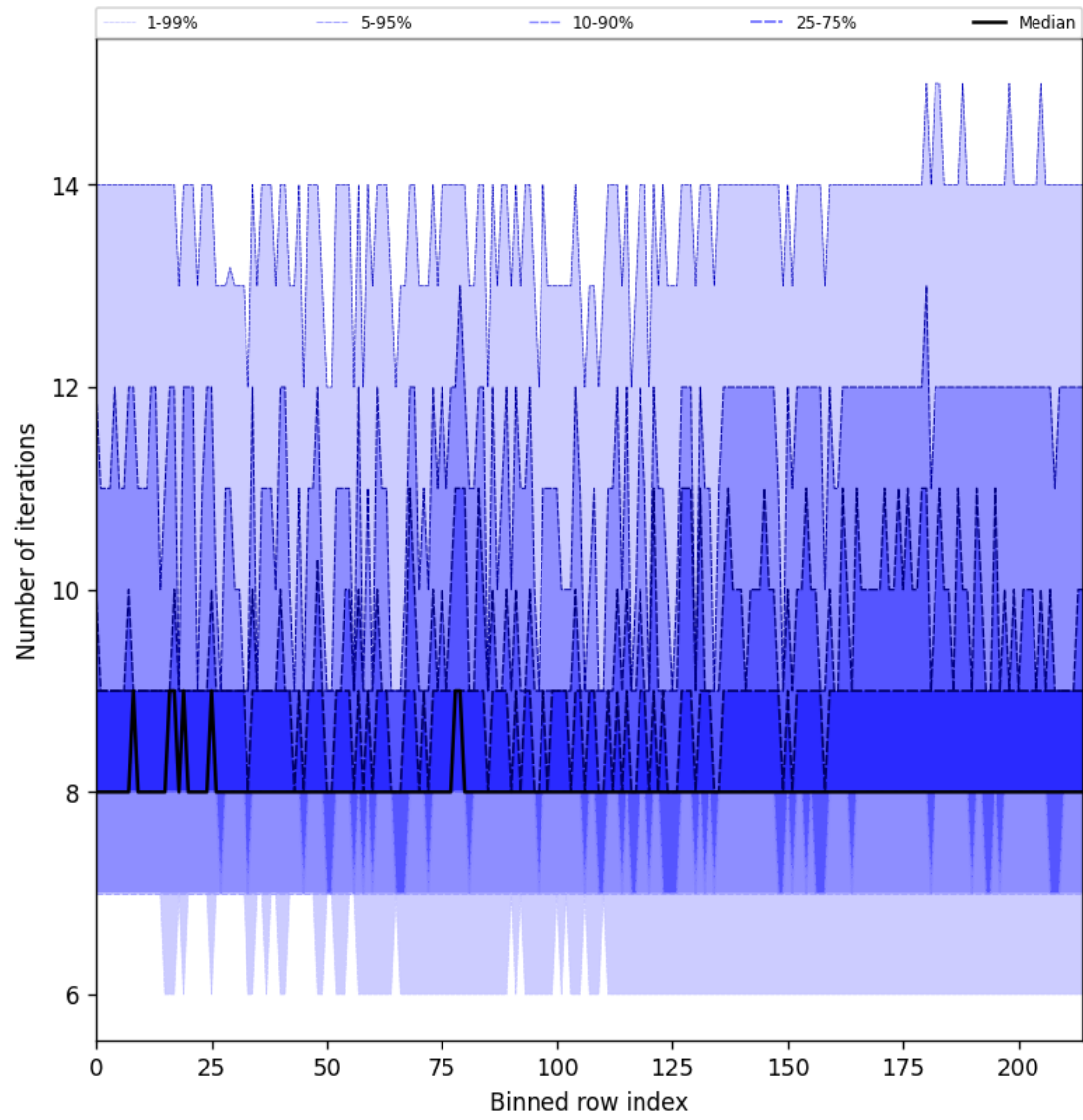
Figure 32: Along track statistics of “Number of iterations” for 2025-09-07 to 2025-09-09
