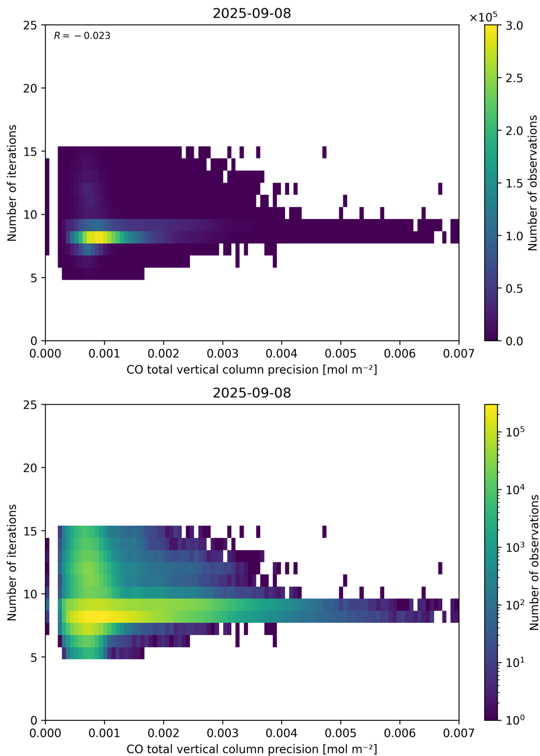
Figure 46: Scatter density plot of “CO total vertical column precision” against “Number of iterations” for 2025-09-07 to 2025-09-09.
