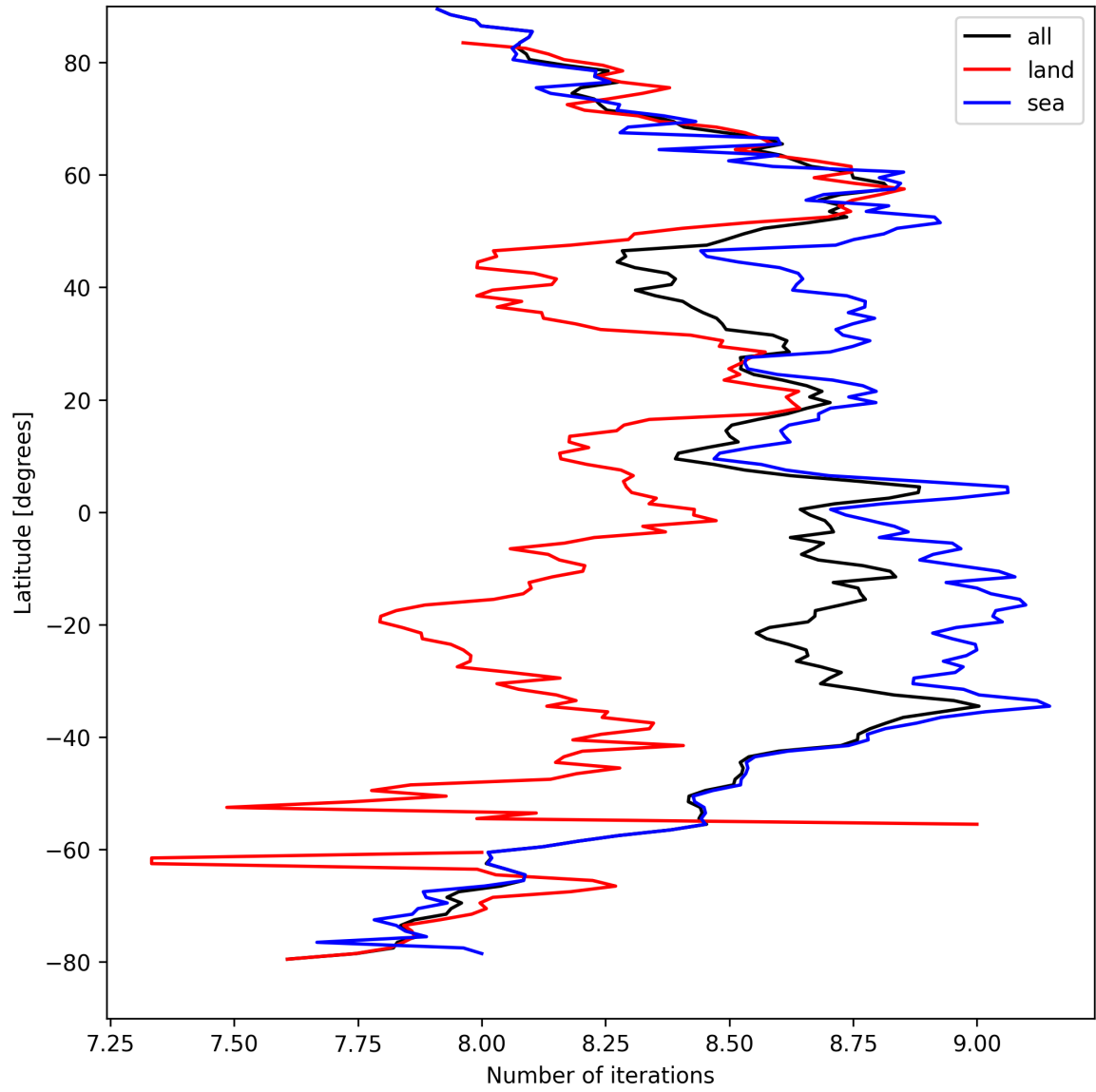
Figure 16: Zonal average of “Number of iterations” for 2025-09-07 to 2025-09-09.
