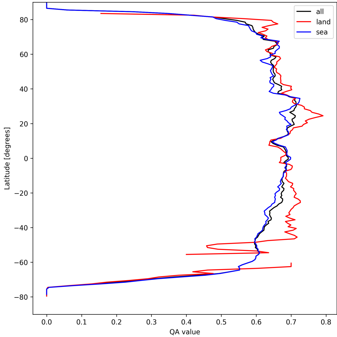
Figure 9: Zonal average of “QA value” for 2025-09-07 to 2025-09-09.
