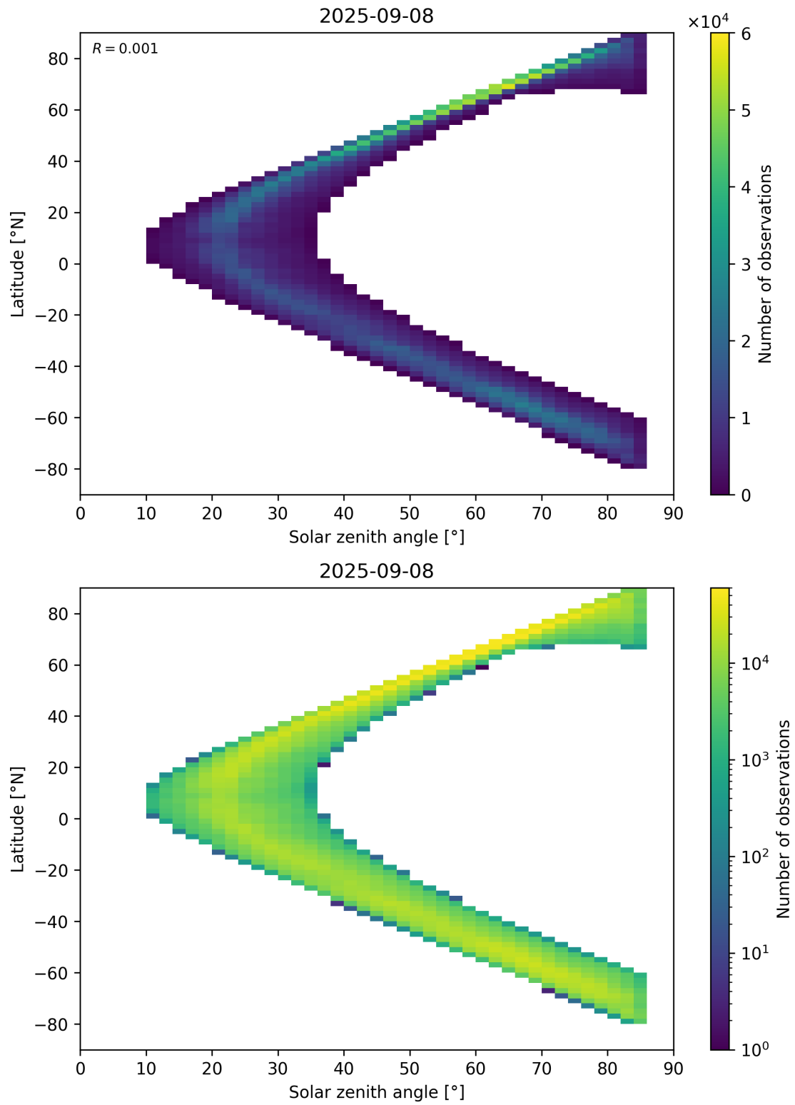
Figure 66: Scatter density plot of “Solar zenith angle” against “Latitude” for 2025-09-07 to 2025-09-09.
