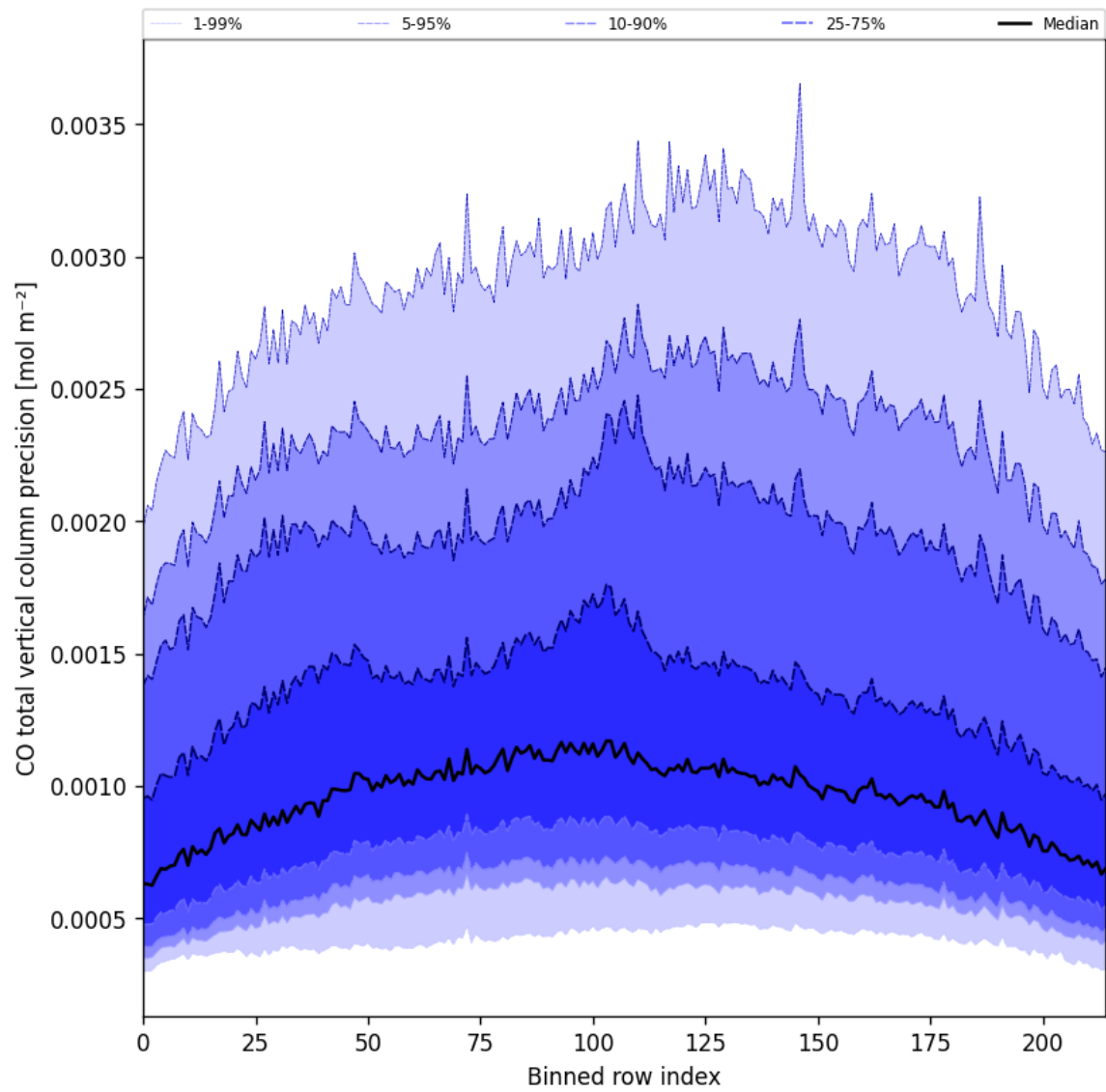
Figure 28: Along track statistics of “CO total vertical column precision” for 2025-09-07 to 2025-09-09
