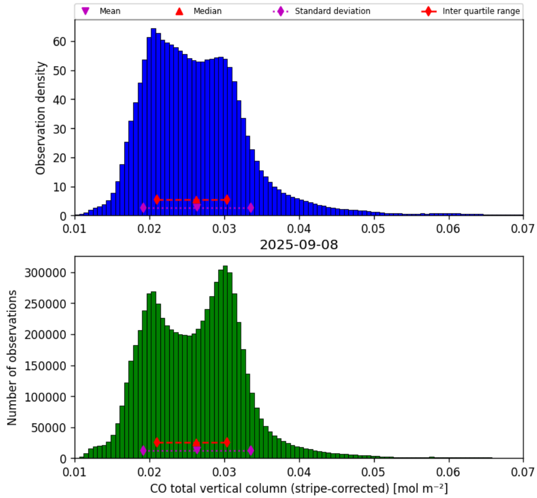
Figure 19: Histogram of “CO total vertical column (stripe-corrected)” for 2025-09-07 to 2025-09-09
