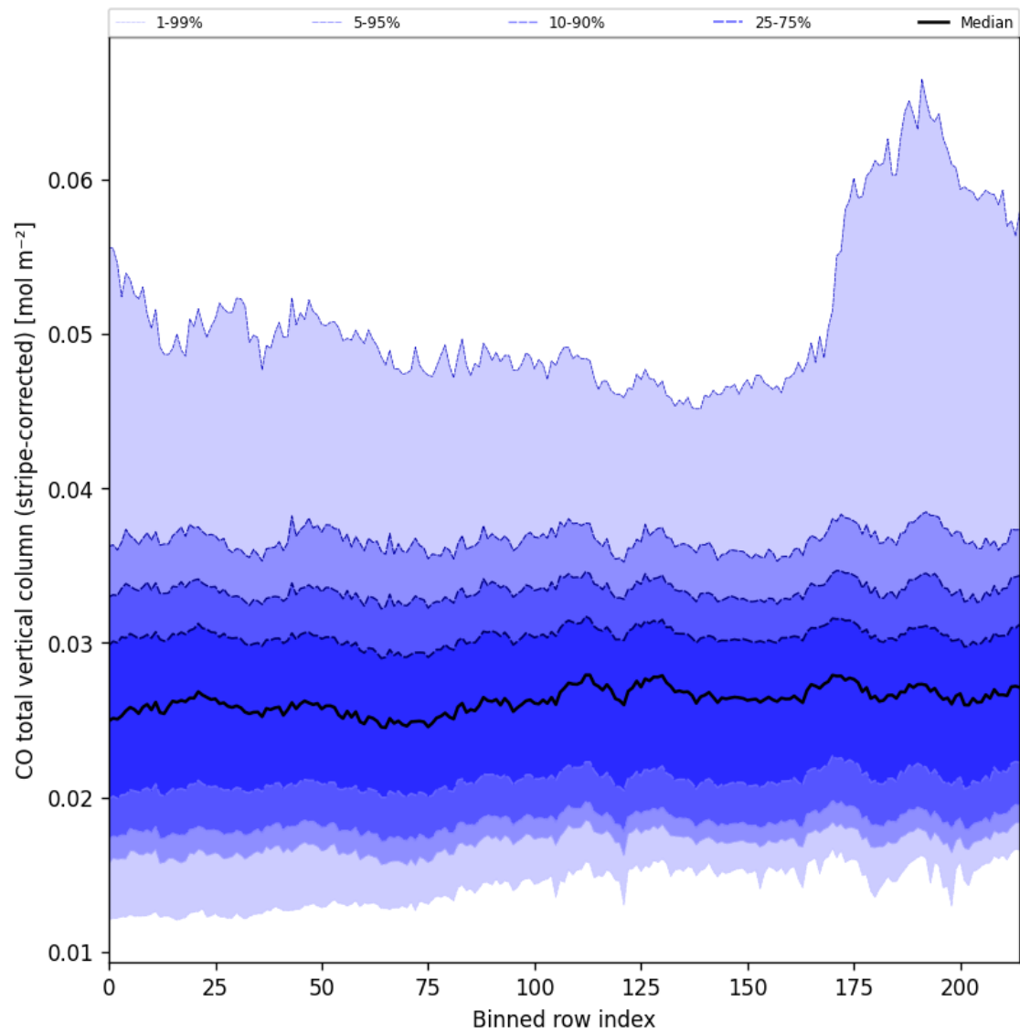
Figure 27: Along track statistics of “CO total vertical column (stripe-corrected)” for 2025-09-07 to 2025-09-09
