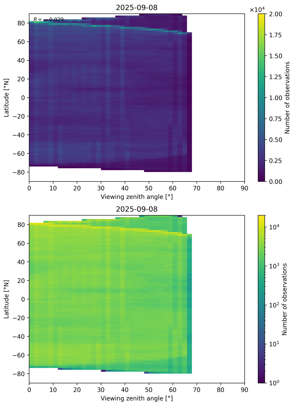
Figure 74: Scatter density plot of “Viewing zenith angle” against “Latitude” for 2025-09-07 to 2025-09-09.
