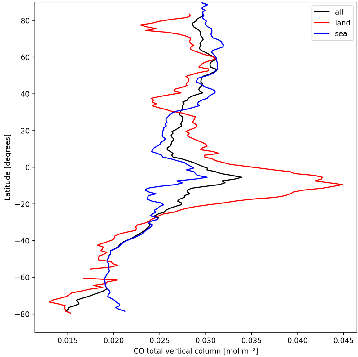
Figure 10: Zonal average of “CO total vertical column” for 2025-09-07 to 2025-09-09.
