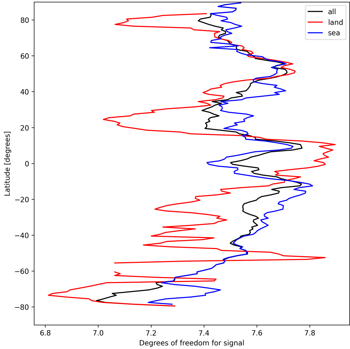
Figure 15: Zonal average of “Degrees of freedom for signal” for 2025-09-07 to 2025-09-09.
