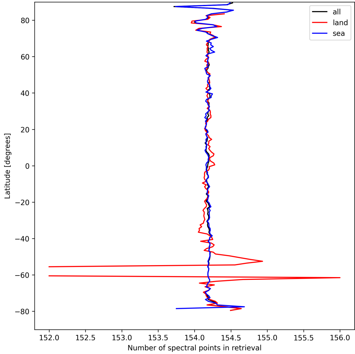
Figure 13: Zonal average of “Number of spectral points in retrieval” for 2025-09-07 to 2025-09-09.
