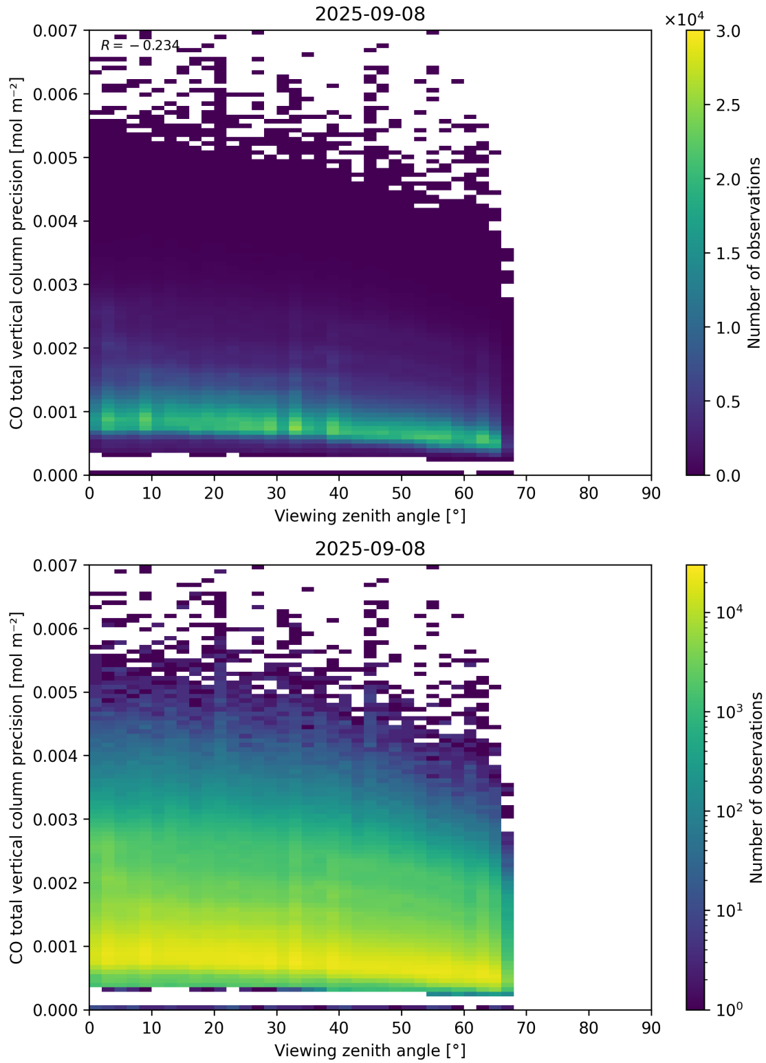
Figure 71: Scatter density plot of “Viewing zenith angle” against “CO total vertical column precision” for 2025-09-07 to 2025-09-09.
