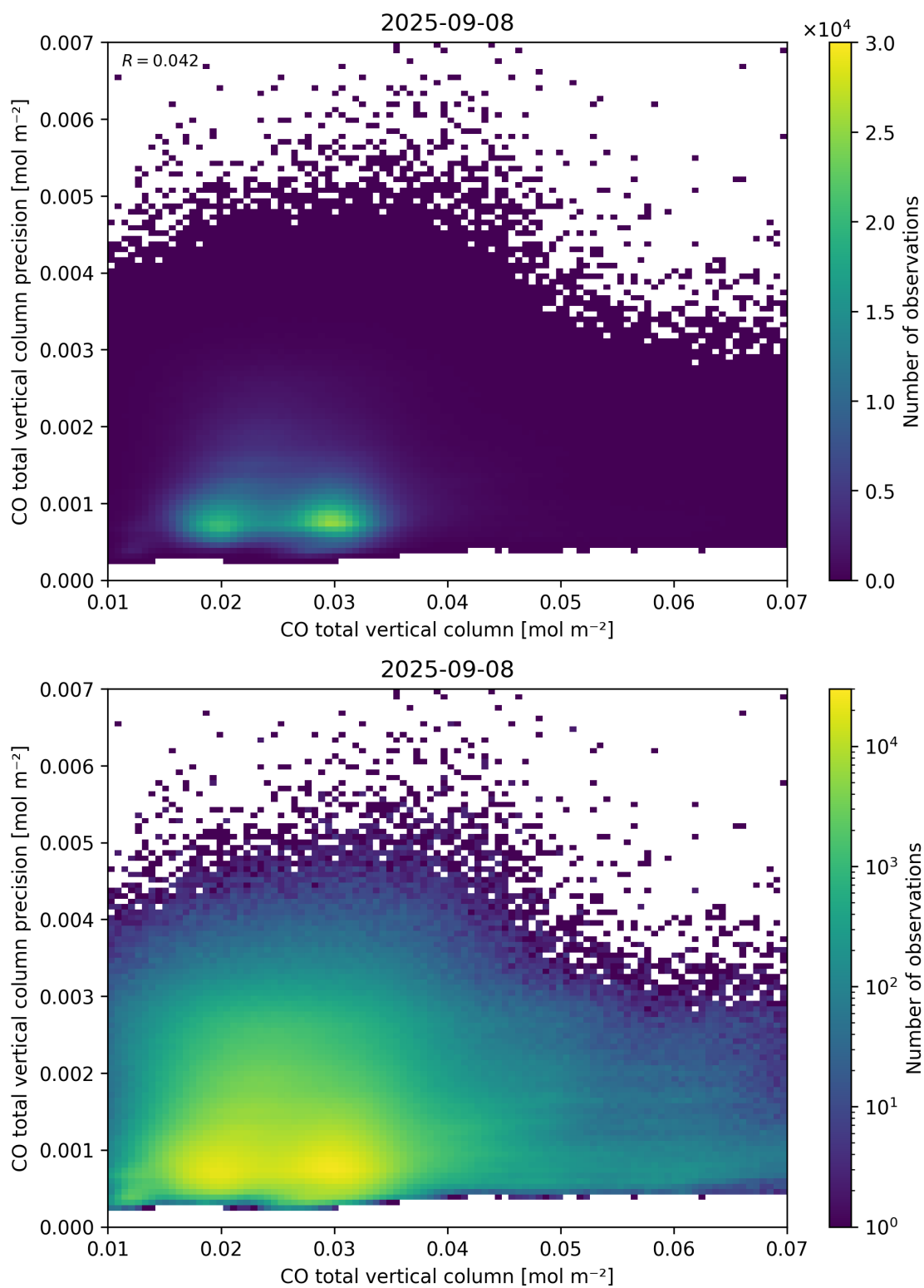
Figure 34: Scatter density plot of “CO total vertical column” against “CO total vertical column precision” for 2025-09-07 to 2025-09-09.
