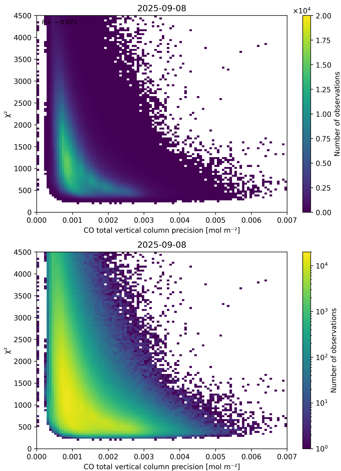
Figure 44: Scatter density plot of “CO total vertical column precision” against “ \chi^2 ” for 2025-09-07 to 2025-09-09.
