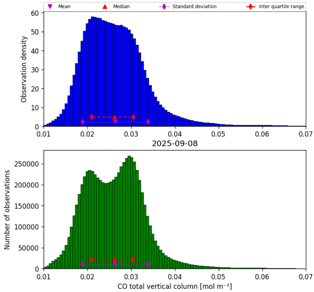
Figure 18: Histogram of “CO total vertical column” for 2025-09-07 to 2025-09-09
