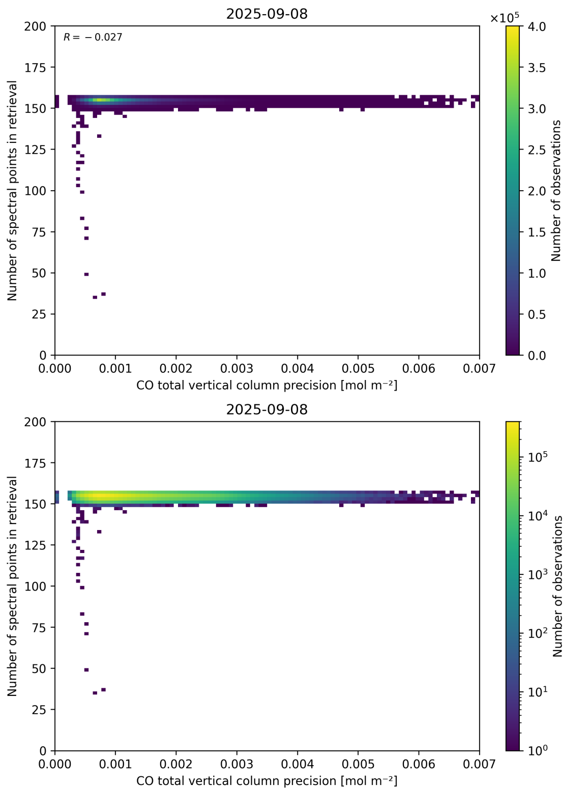
Figure 47: Scatter density plot of “CO total vertical column precision” against “Number of spectral points in retrieval” for 2025-09-07 to 2025-09-09.
