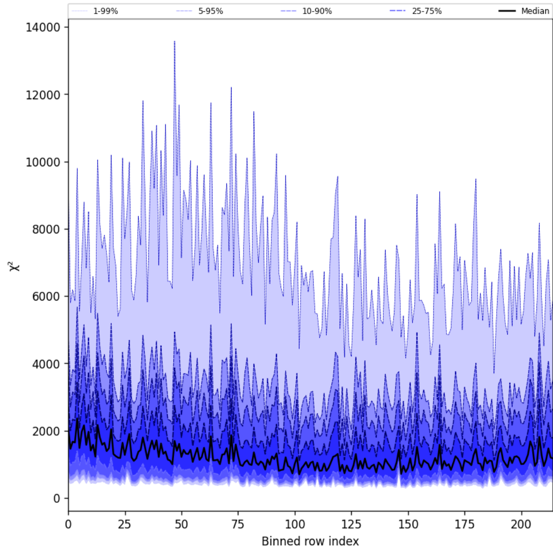
Figure 30: Along track statistics of “ \chi^2 ” for 2025-09-07 to 2025-09-09
