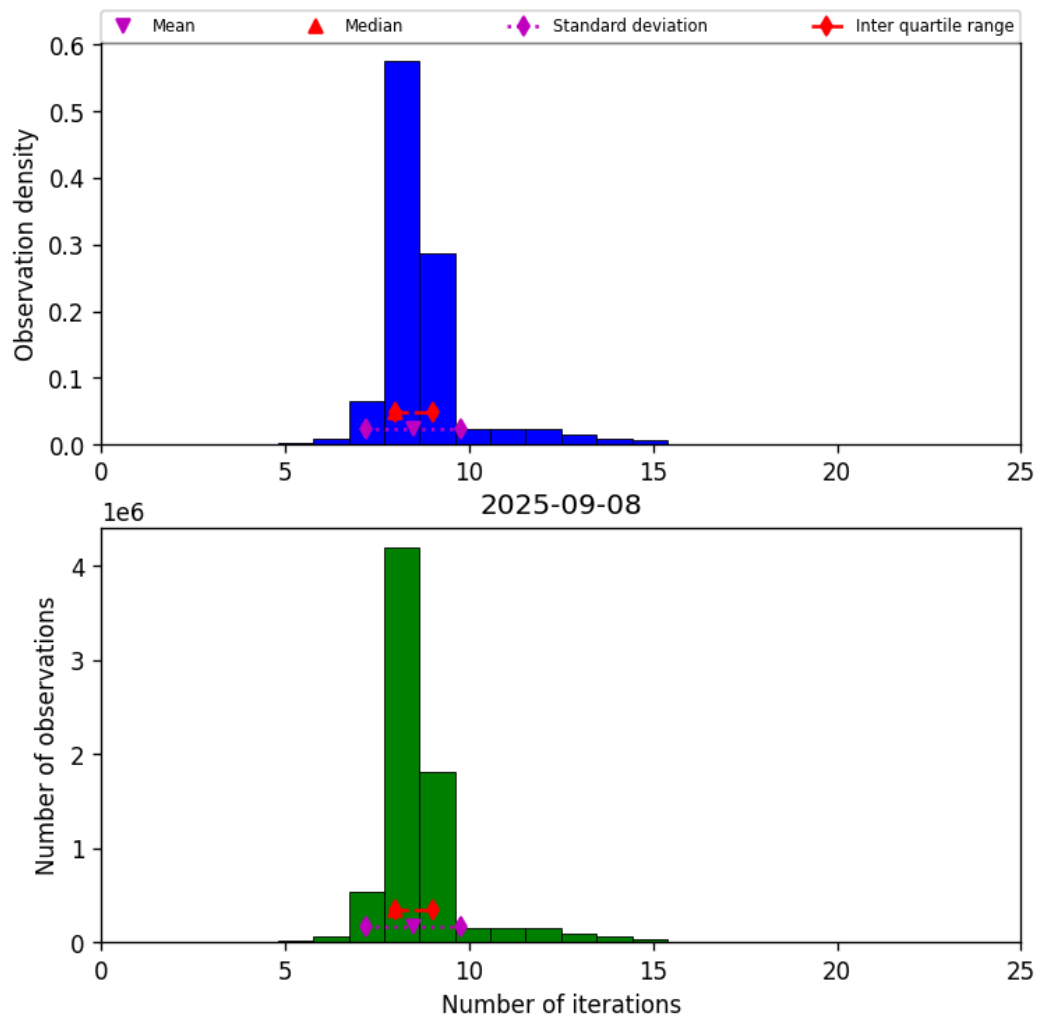
Figure 24: Histogram of “Number of iterations” for 2025-09-07 to 2025-09-09
