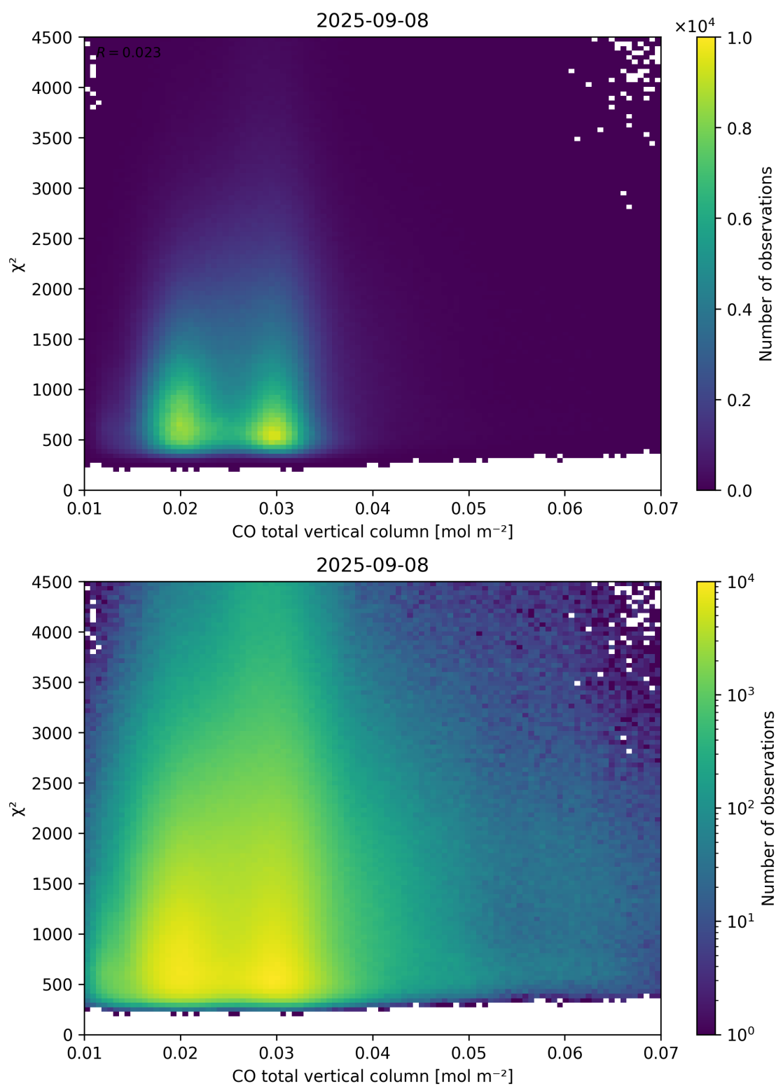
Figure 35: Scatter density plot of “CO total vertical column” against “ \chi^2 ” for 2025-09-07 to 2025-09-09.
