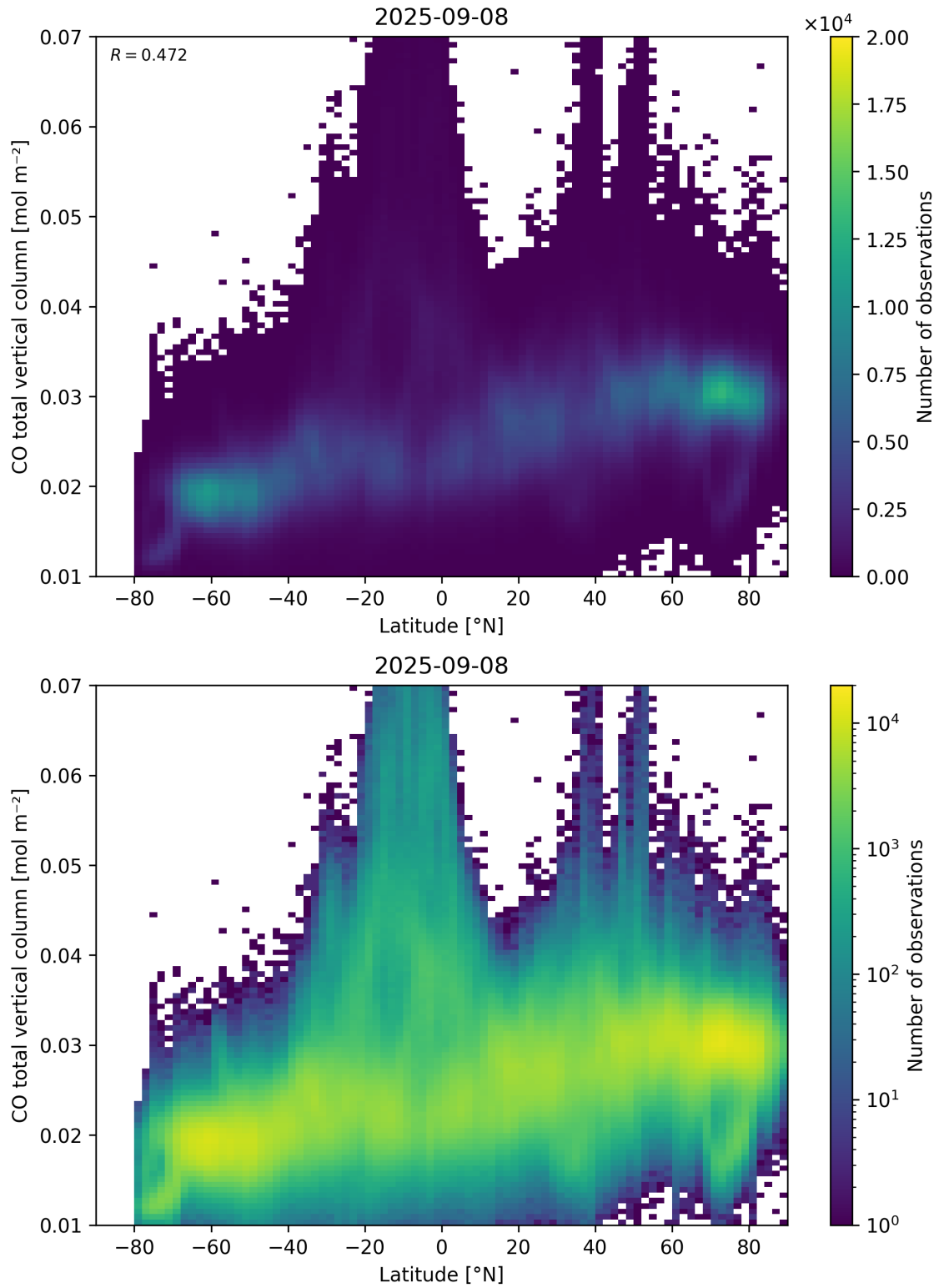
Figure 51: Scatter density plot of “Latitude” against “CO total vertical column” for 2025-09-07 to 2025-09-09.
