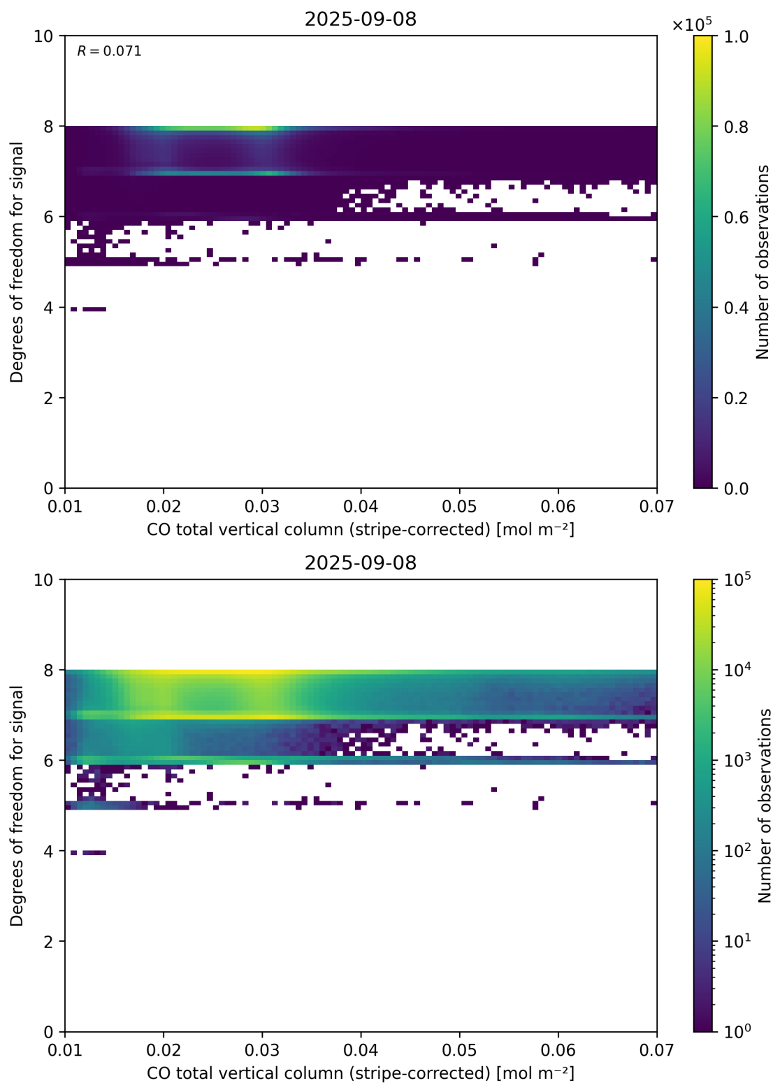
Figure 38: Scatter density plot of “CO total vertical column (stripe-corrected)” against “Degrees of freedom for signal” for 2025-09-07 to 2025-09-09.
