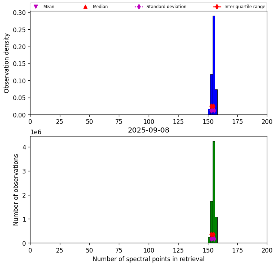
Figure 21: Histogram of “Number of spectral points in retrieval” for 2025-09-07 to 2025-09-09
