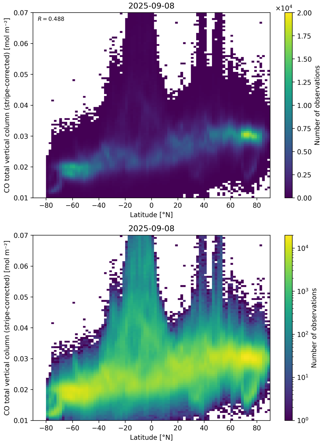
Figure 52: Scatter density plot of “Latitude” against “CO total vertical column (stripe-corrected)” for 2025-09-07 to 2025-09-09.
