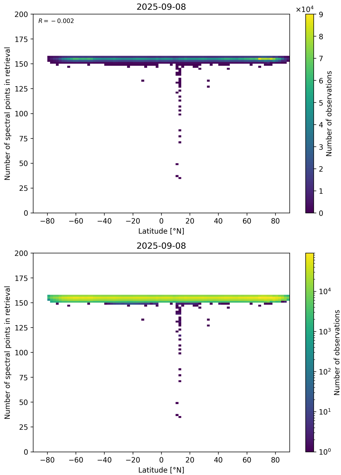
Figure 57: Scatter density plot of “Latitude” against “Number of spectral points in retrieval” for 2025-09-07 to 2025-09-09.
