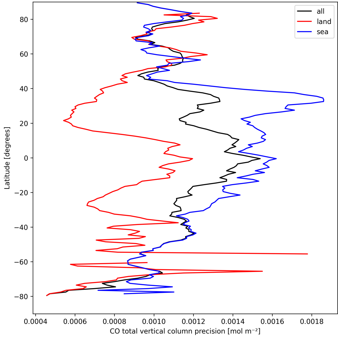
Figure 12: Zonal average of “CO total vertical column precision” for 2025-09-07 to 2025-09-09.
