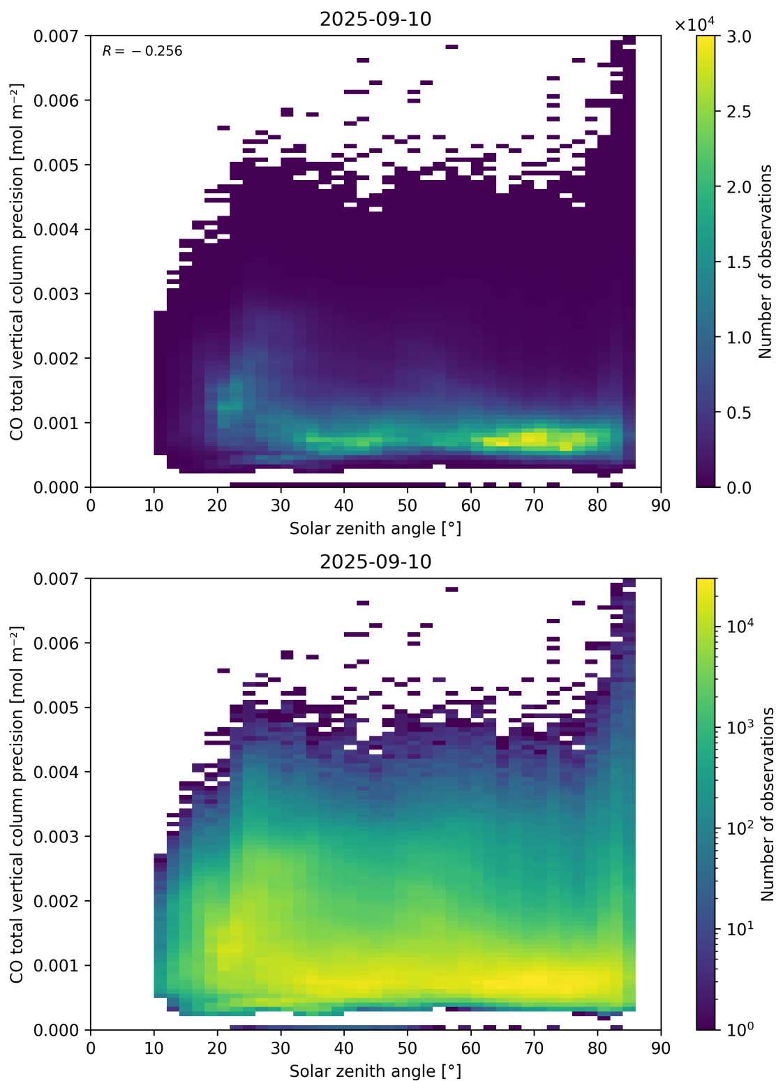
Figure 63: Scatter density plot of “Solar zenith angle” against “CO total vertical column precision” for 2025-09-10 to 2025-09-11.
