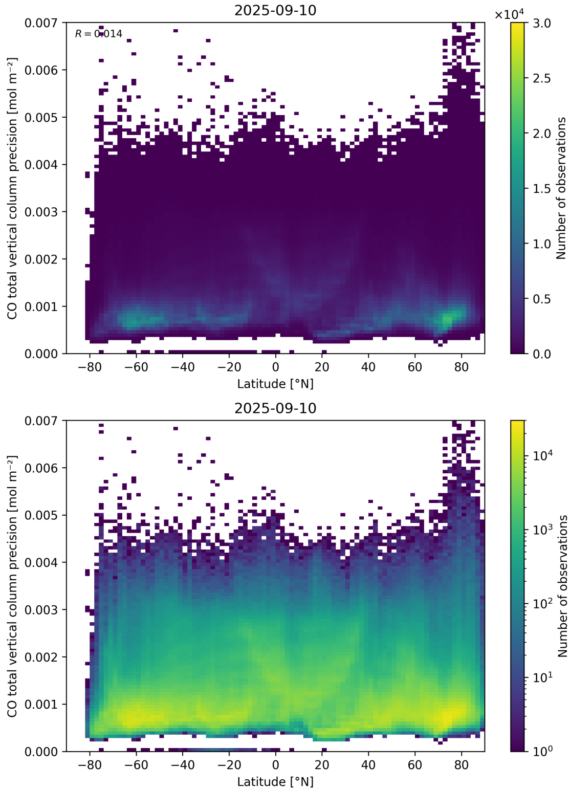
Figure 53: Scatter density plot of “Latitude” against “CO total vertical column precision” for 2025-09-10 to 2025-09-11.
