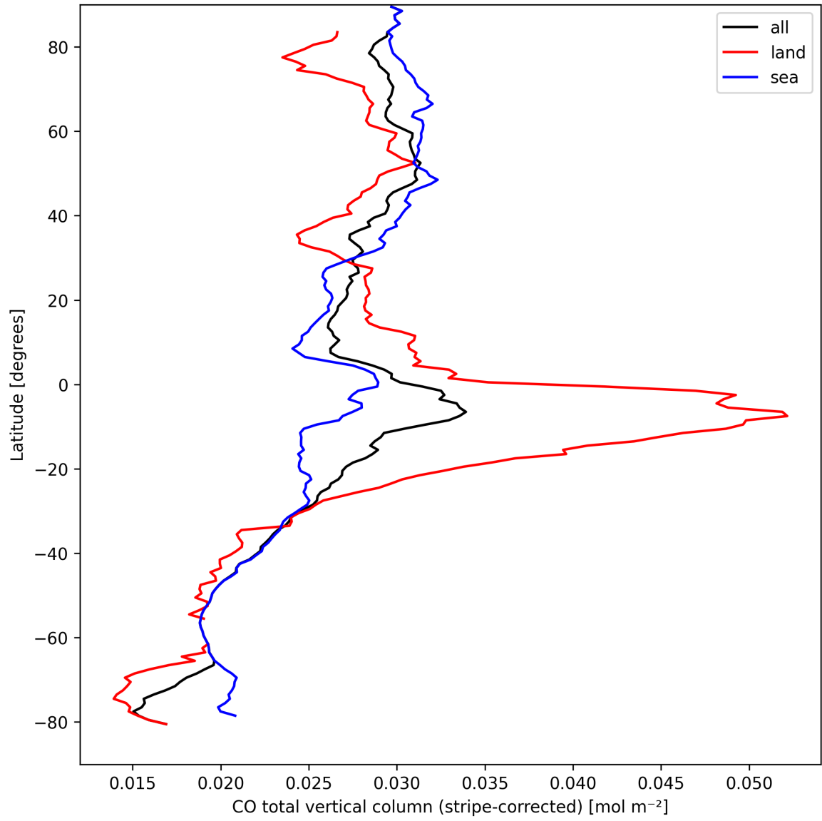
Figure 11: Zonal average of “CO total vertical column (stripe-corrected)” for 2025-09-10 to 2025-09-11.
