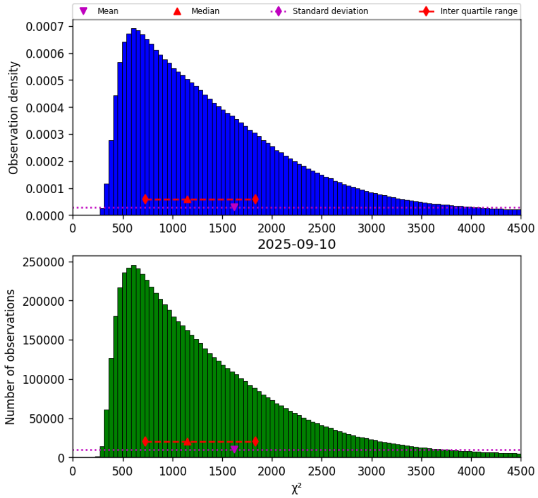
Figure 22: Histogram of “ \chi^2 ” for 2025-09-10 to 2025-09-11
