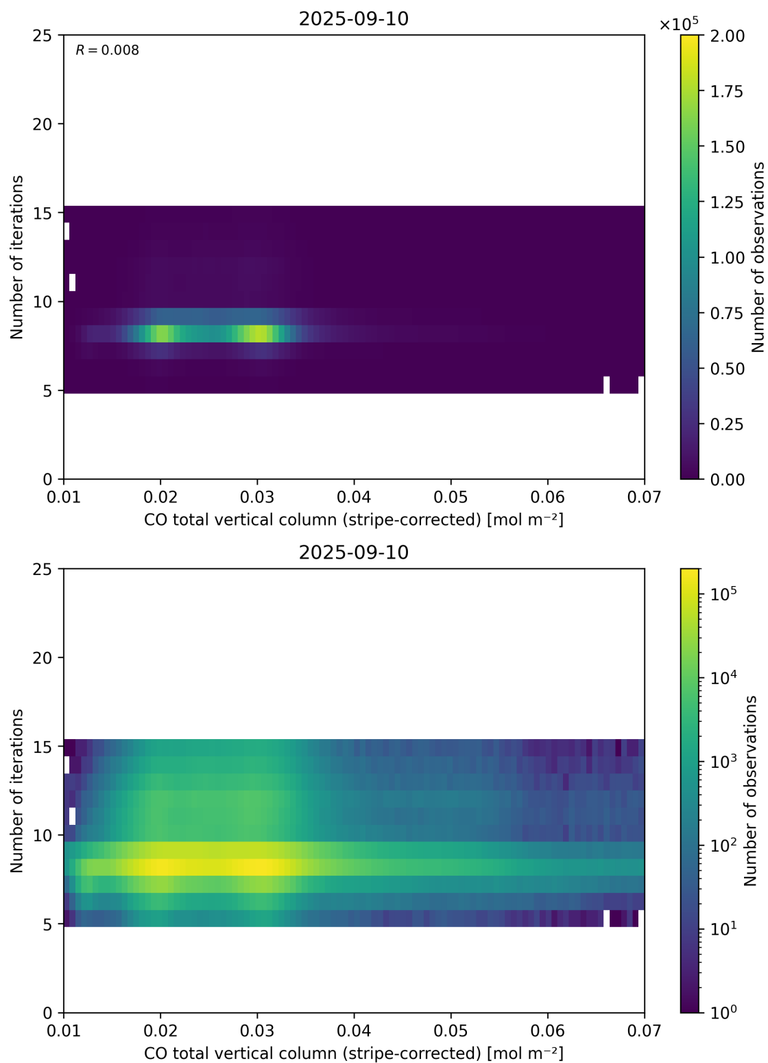
Figure 39: Scatter density plot of “CO total vertical column (stripe-corrected)” against “Number of iterations” for 2025-09-10 to 2025-09-11.
