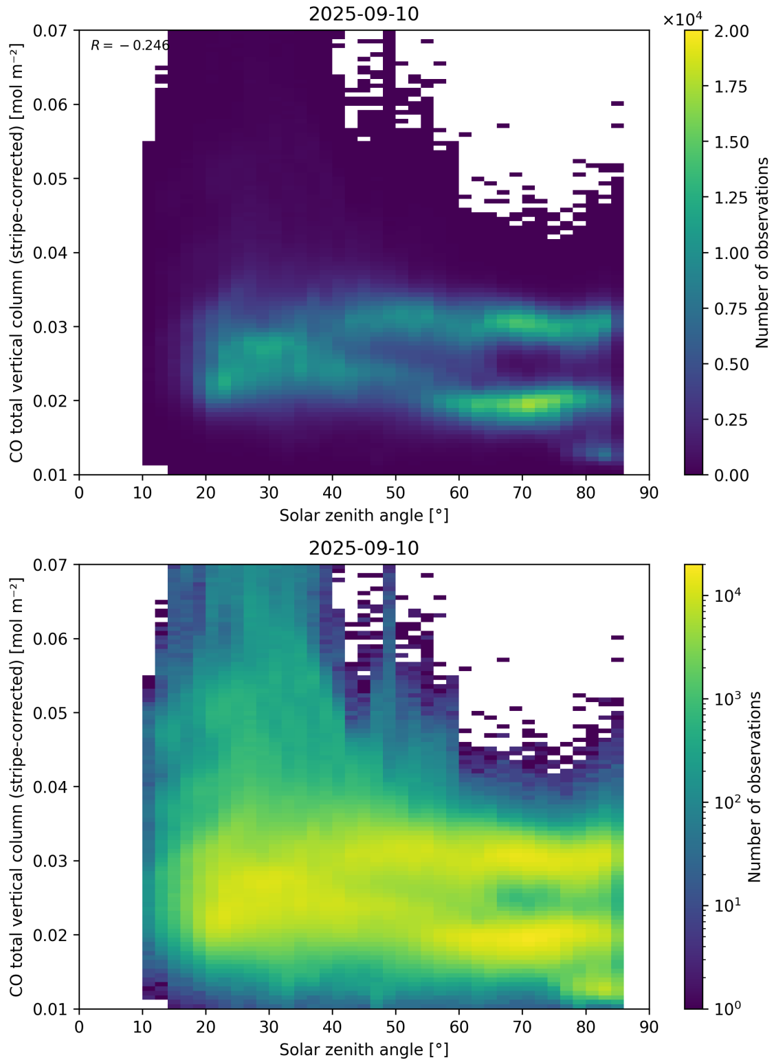
Figure 62: Scatter density plot of “Solar zenith angle” against “CO total vertical column (stripe-corrected)” for 2025-09-10 to 2025-09-11.
