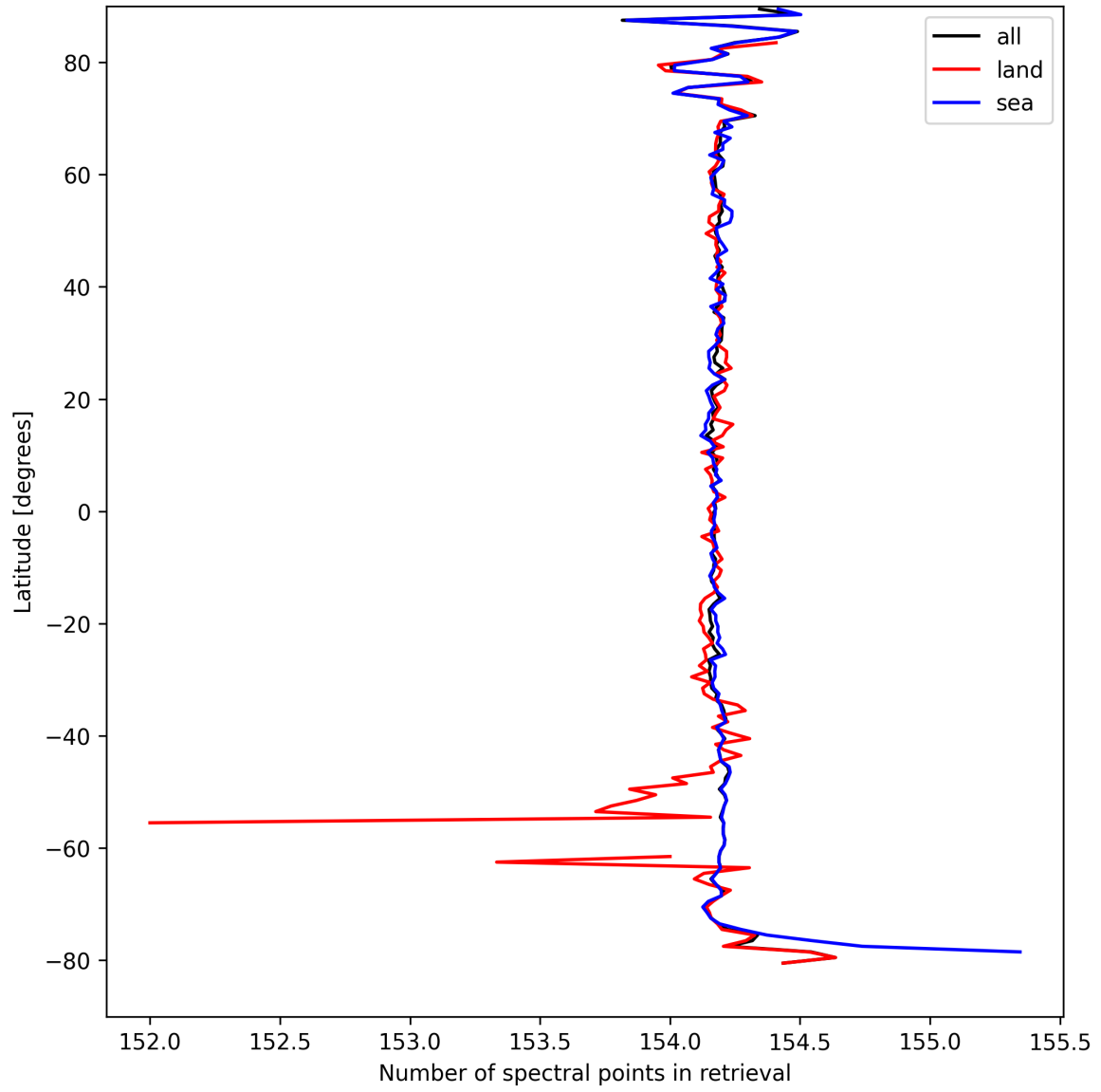
Figure 13: Zonal average of “Number of spectral points in retrieval” for 2025-09-10 to 2025-09-11.
