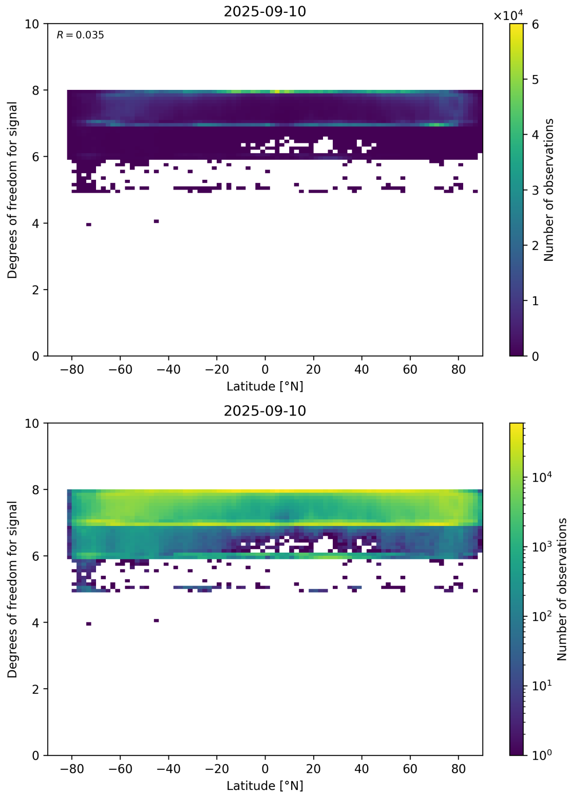
Figure 55: Scatter density plot of “Latitude” against “Degrees of freedom for signal” for 2025-09-10 to 2025-09-11.
