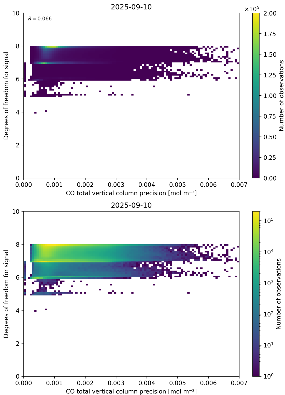
Figure 45: Scatter density plot of “CO total vertical column precision” against “Degrees of freedom for signal” for 2025-09-10 to 2025-09-11.
