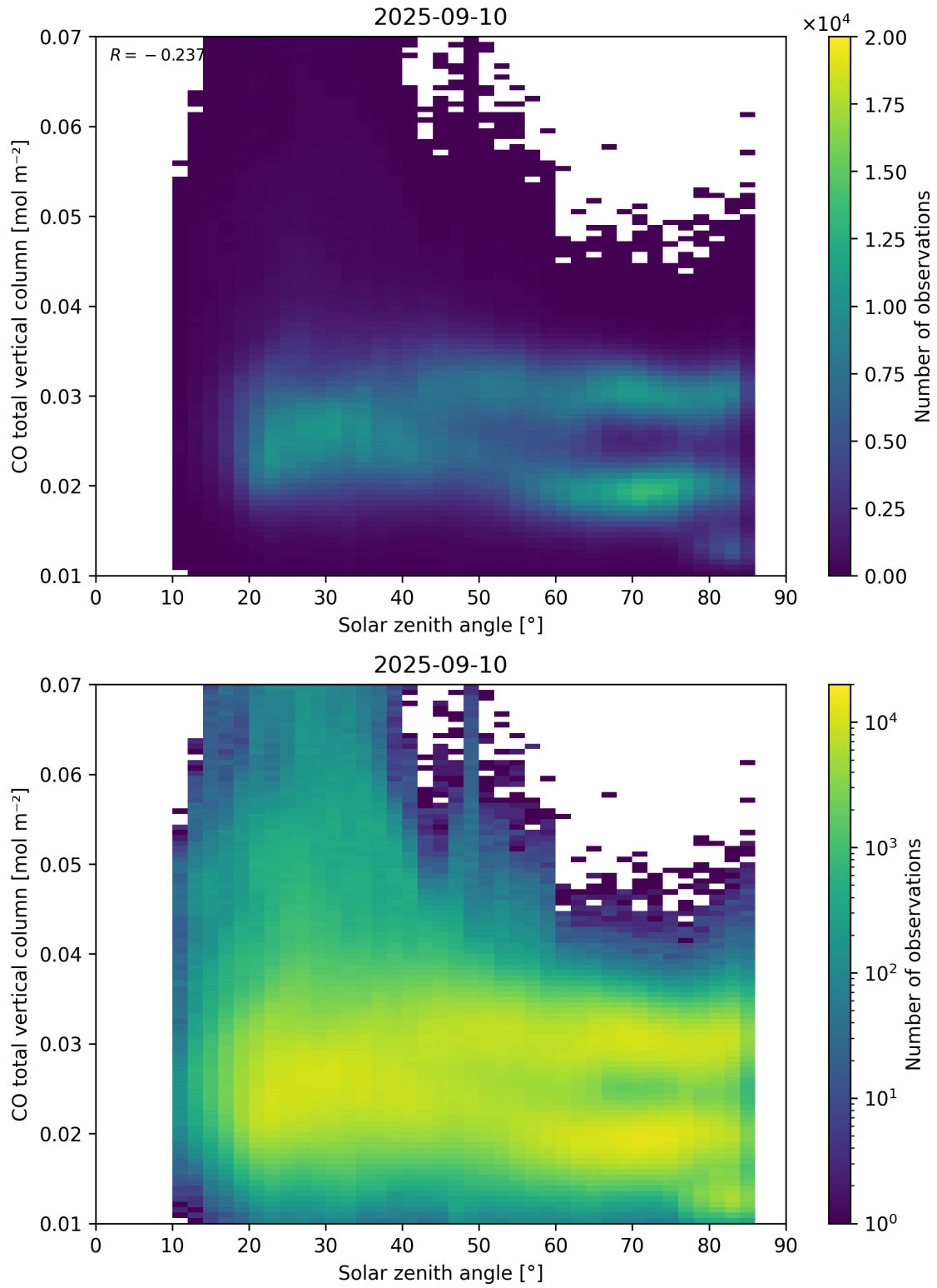
Figure 61: Scatter density plot of “Solar zenith angle” against “CO total vertical column” for 2025-09-10 to 2025-09-11.
