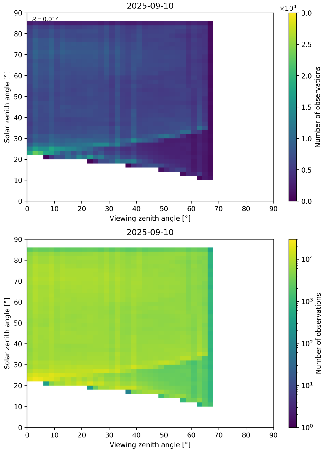
Figure 77: Scatter density plot of “Viewing zenith angle” against “Solar zenith angle” for 2025-09-10 to 2025-09-11.
