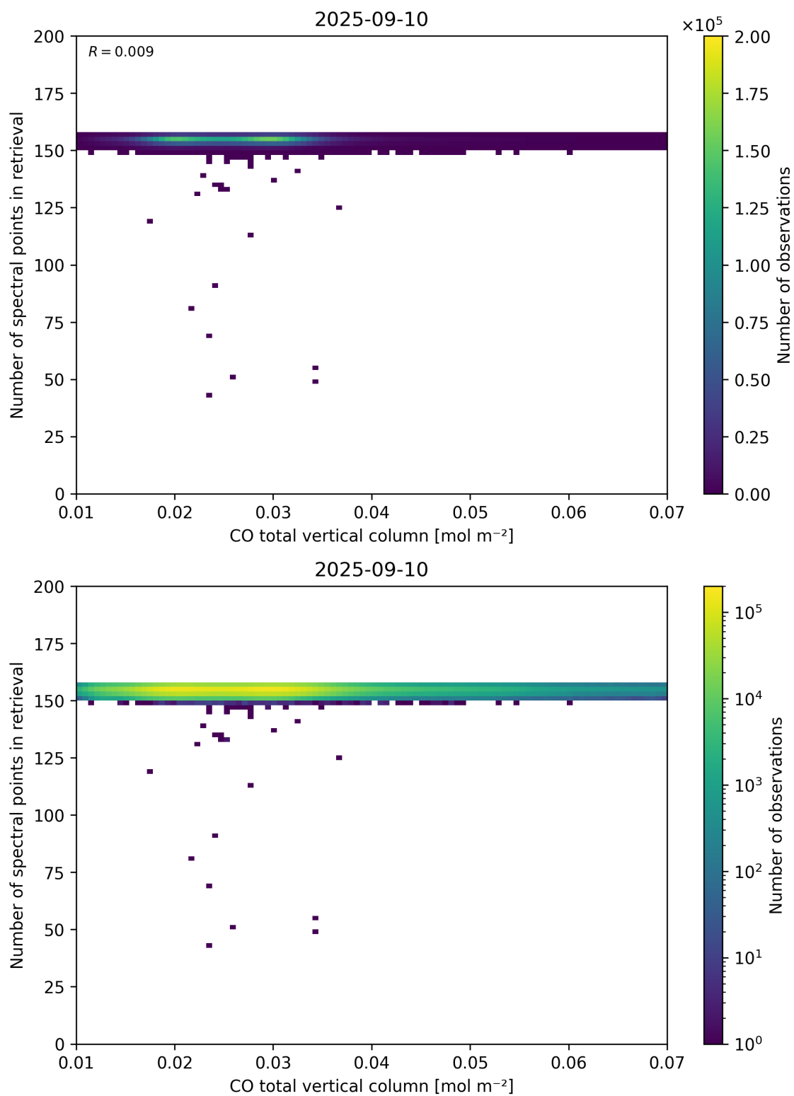
Figure 43: Scatter density plot of “CO total vertical column” against “Number of spectral points in retrieval” for 2025-09-10 to 2025-09-11.
