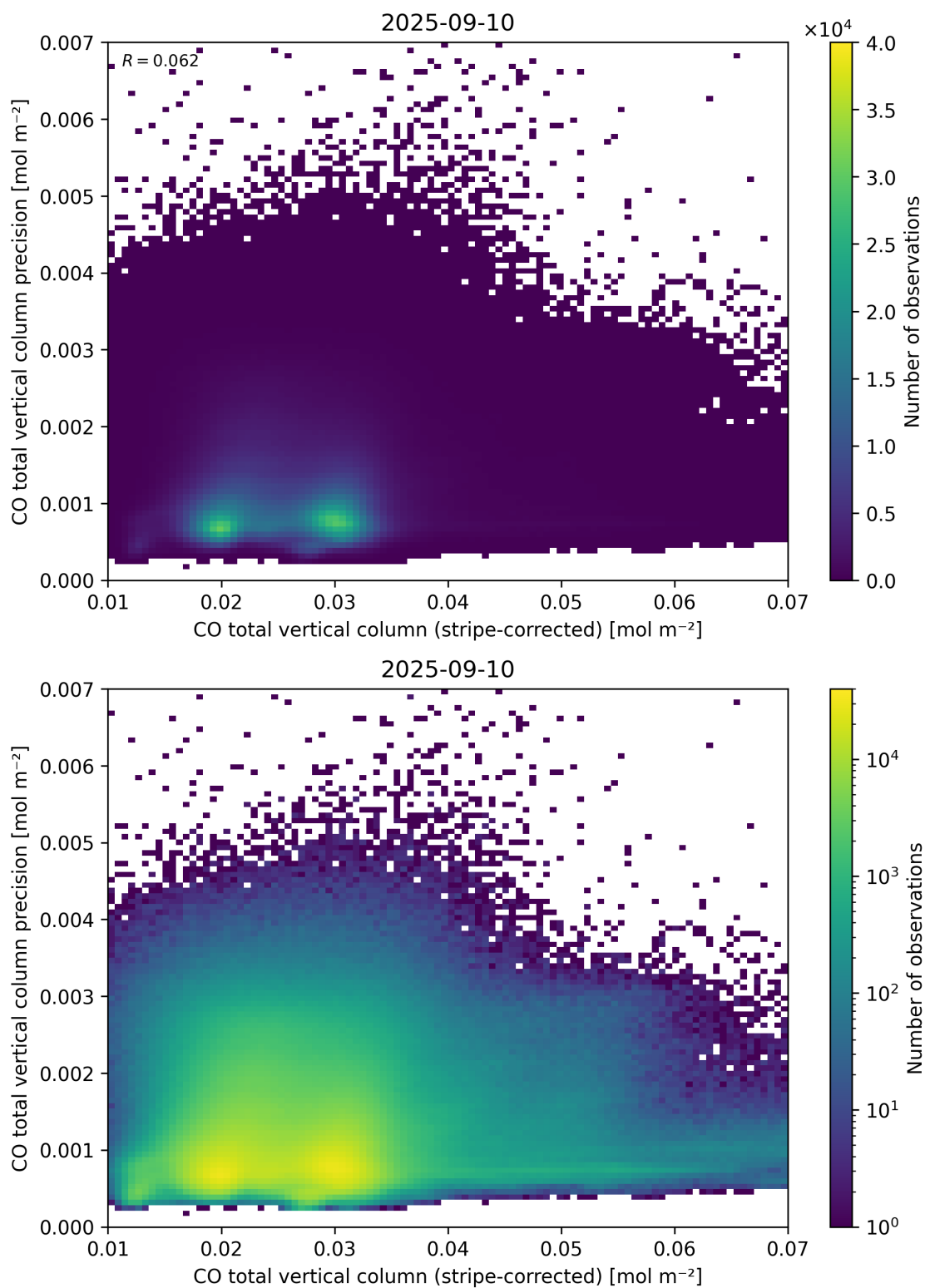
Figure 36: Scatter density plot of “CO total vertical column (stripe-corrected)” against “CO total vertical column precision” for 2025-09-10 to 2025-09-11.
