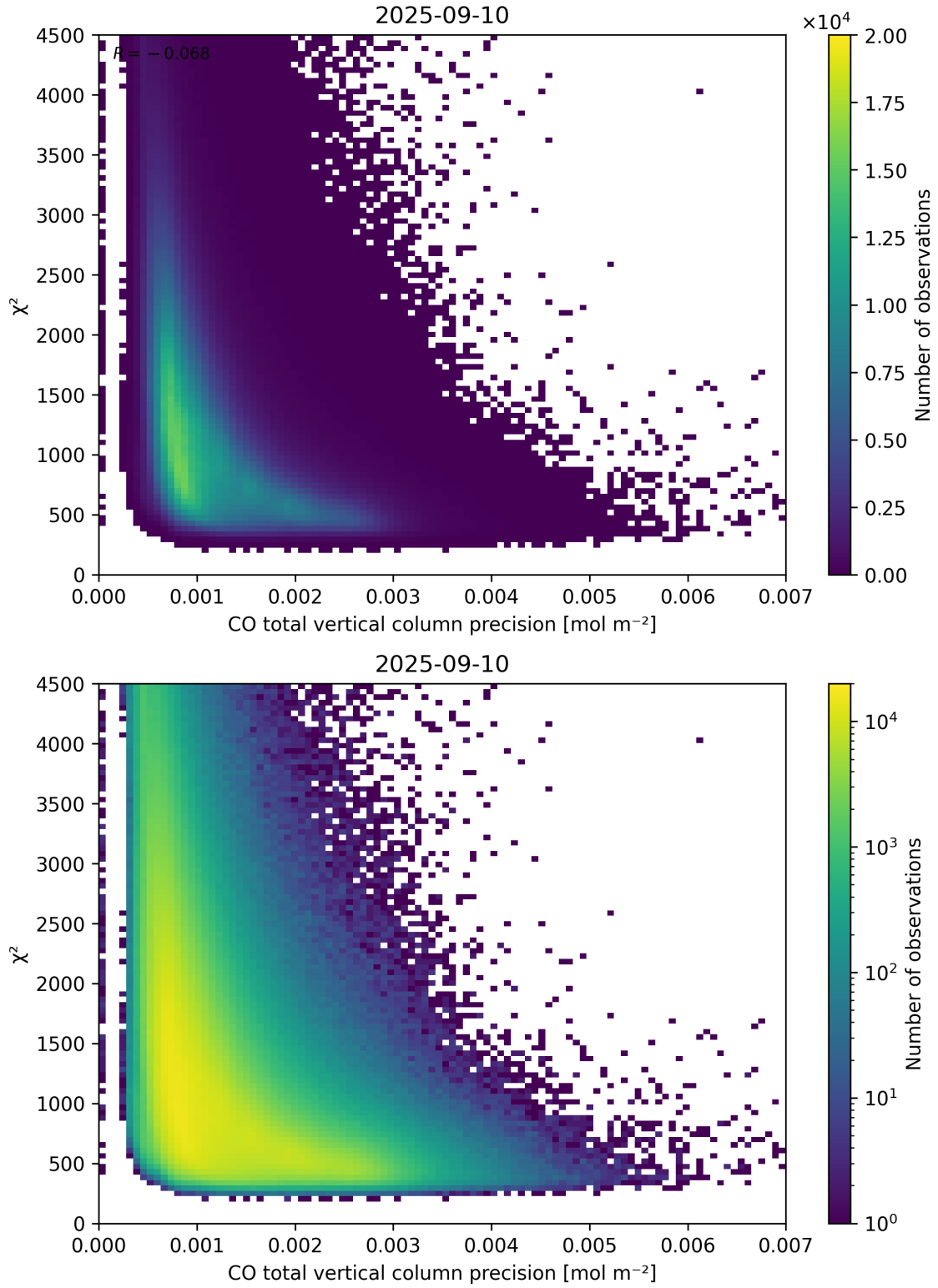
Figure 44: Scatter density plot of “CO total vertical column precision” against “ \chi^2 ” for 2025-09-10 to 2025-09-11.
