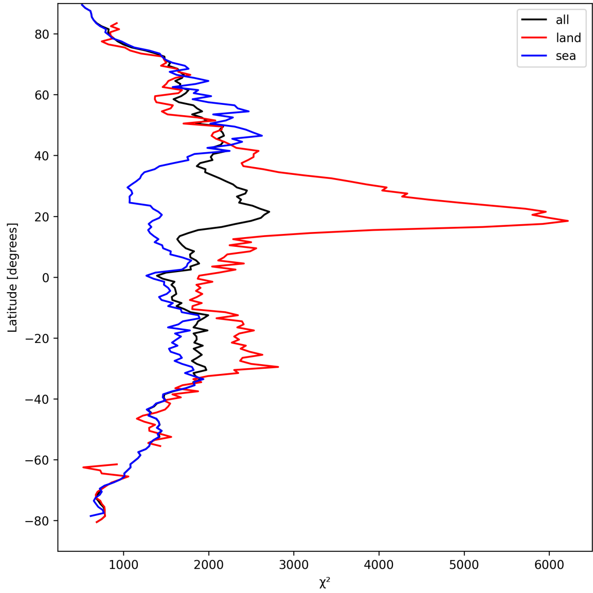
Figure 14: Zonal average of “ \chi^2 ” for 2025-09-10 to 2025-09-11.
