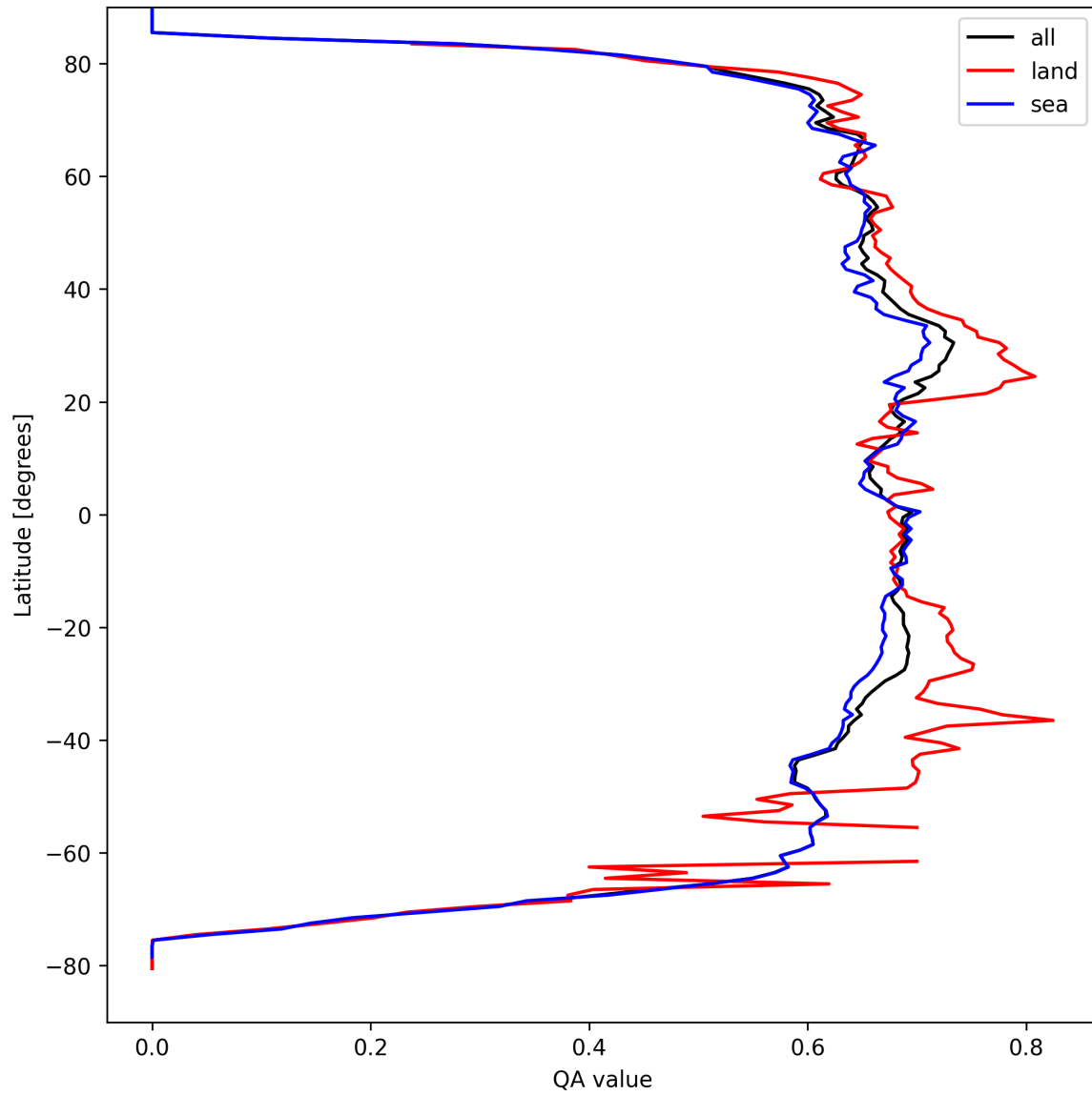
Figure 9: Zonal average of “QA value” for 2025-09-10 to 2025-09-11.
