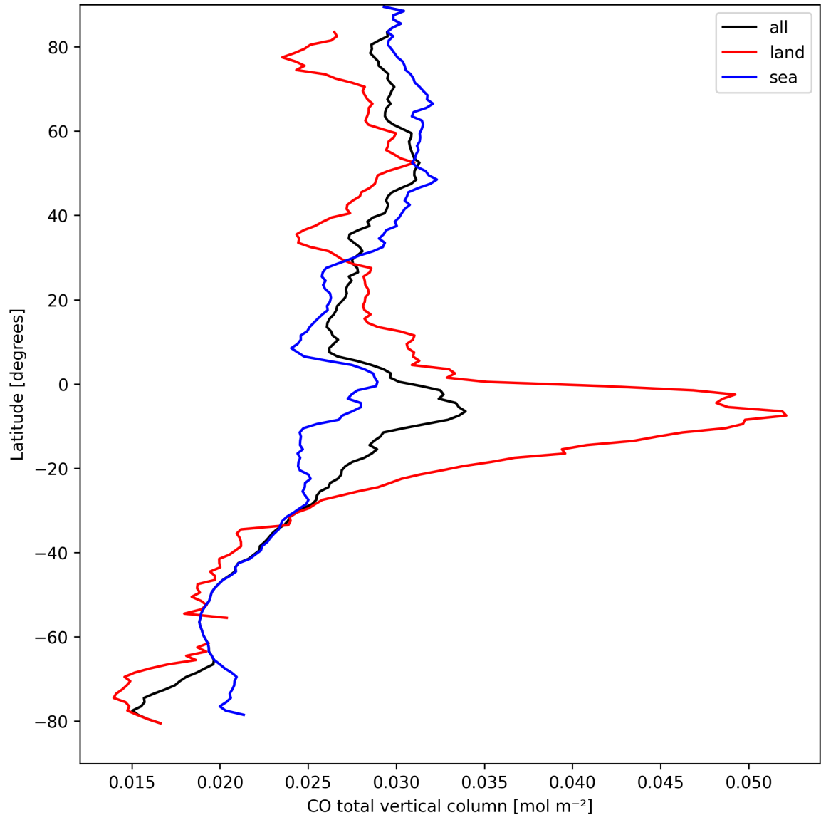
Figure 10: Zonal average of “CO total vertical column” for 2025-09-10 to 2025-09-11.
