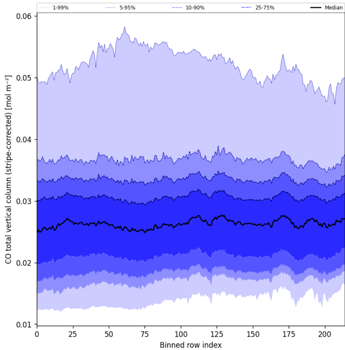
Figure 27: Along track statistics of “CO total vertical column (stripe-corrected)” for 2025-09-10 to 2025-09-11
