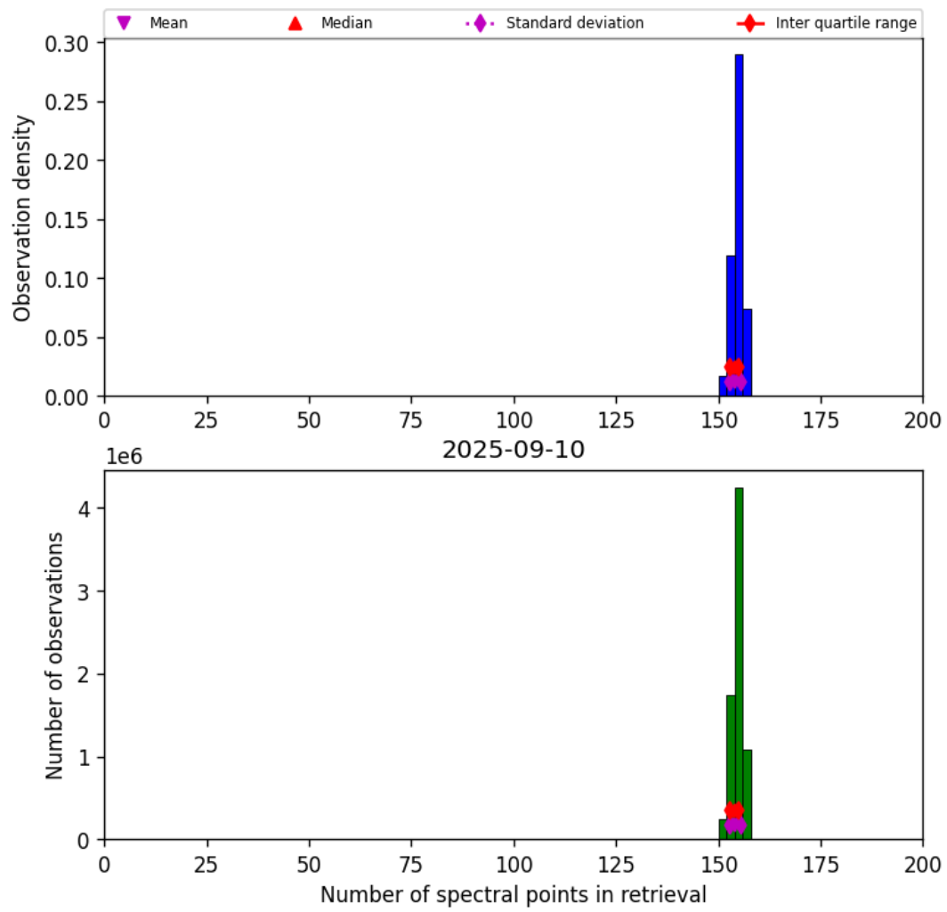
Figure 21: Histogram of “Number of spectral points in retrieval” for 2025-09-10 to 2025-09-11
