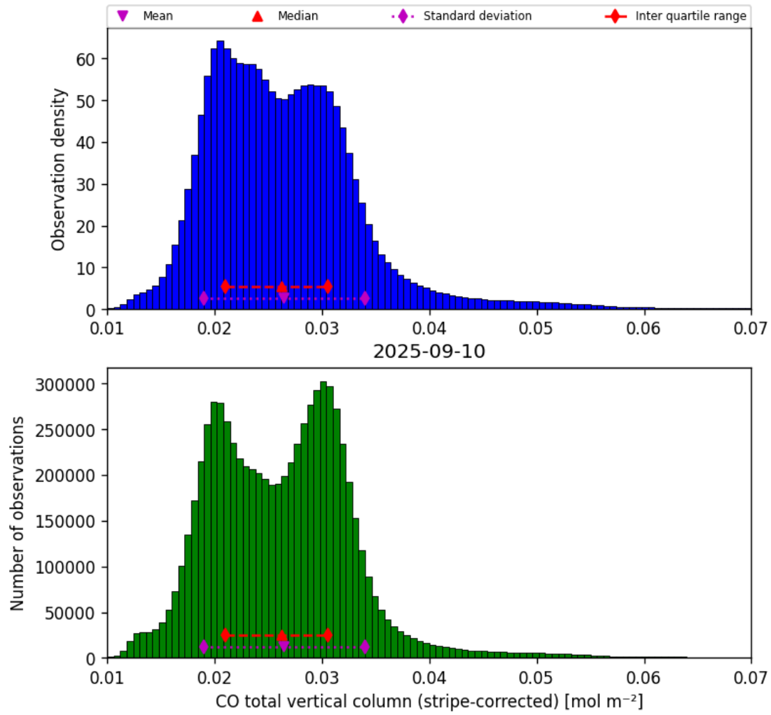
Figure 19: Histogram of “CO total vertical column (stripe-corrected)” for 2025-09-10 to 2025-09-11
