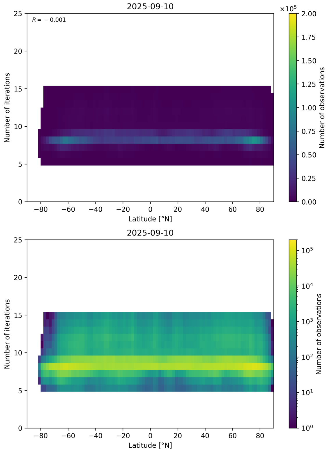
Figure 56: Scatter density plot of “Latitude” against “Number of iterations” for 2025-09-10 to 2025-09-11.
