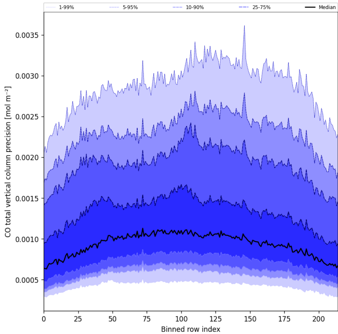
Figure 28: Along track statistics of “CO total vertical column precision” for 2025-09-10 to 2025-09-11
