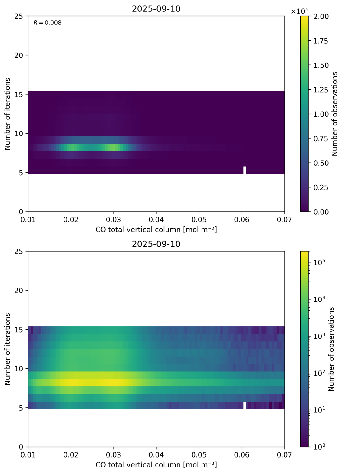
Figure 42: Scatter density plot of “CO total vertical column” against “Number of iterations” for 2025-09-10 to 2025-09-11.
