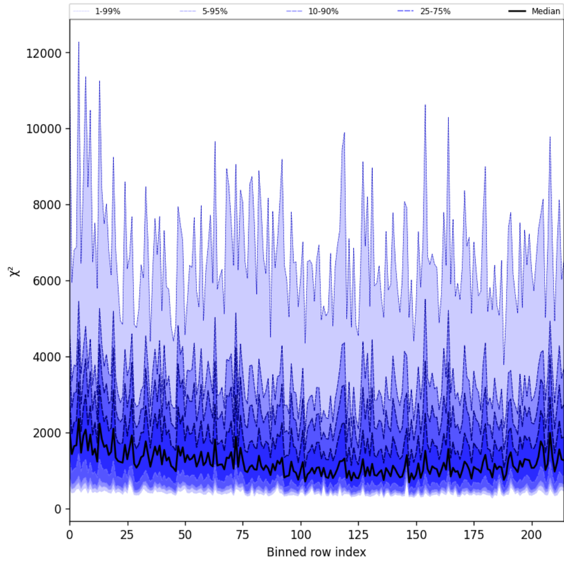
Figure 30: Along track statistics of “ \chi^2 ” for 2025-09-10 to 2025-09-11
