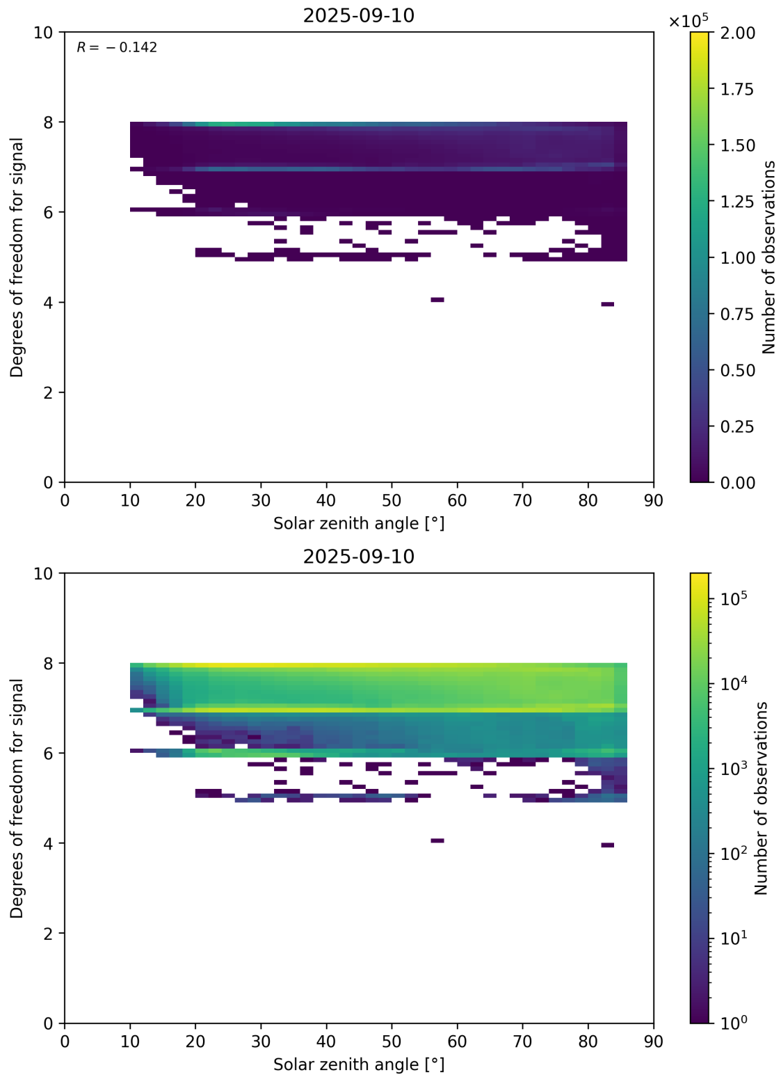
Figure 65: Scatter density plot of “Solar zenith angle” against “Degrees of freedom for signal” for 2025-09-10 to 2025-09-11.
