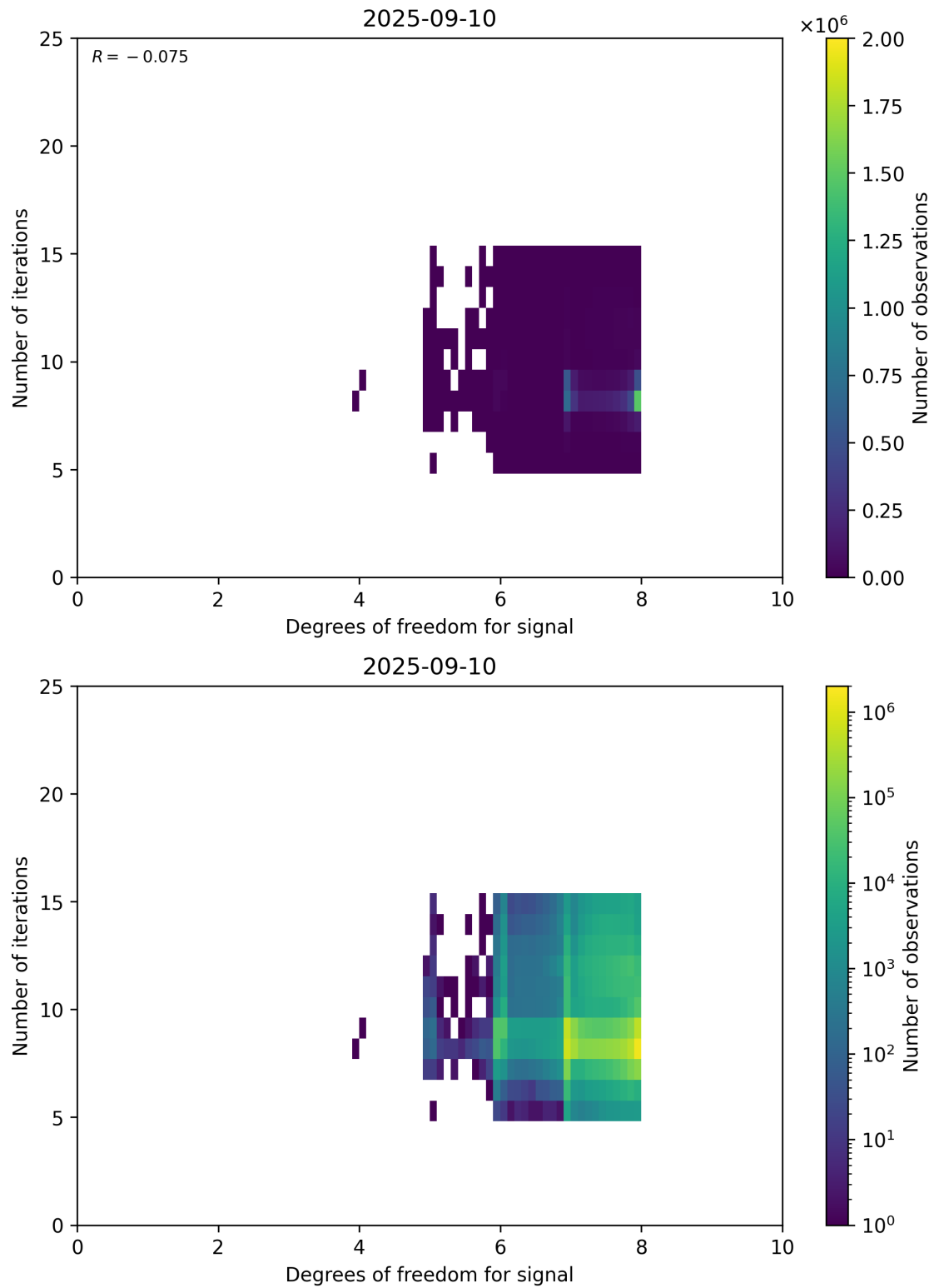
Figure 50: Scatter density plot of “Degrees of freedom for signal” against “Number of iterations” for 2025-09-10 to 2025-09-11.
