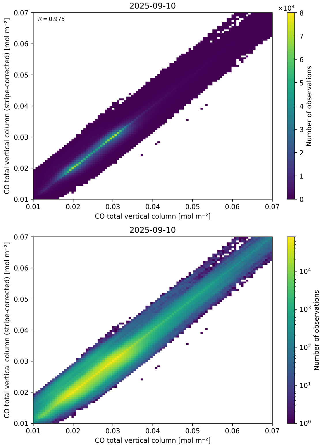
Figure 33: Scatter density plot of “CO total vertical column” against “CO total vertical column (stripe-corrected)” for 2025-09-10 to 2025-09-11.
