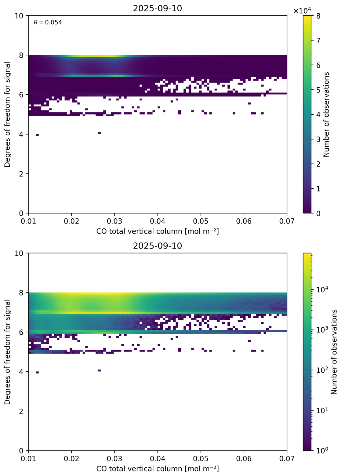
Figure 41: Scatter density plot of “CO total vertical column” against “Degrees of freedom for signal” for 2025-09-10 to 2025-09-11.
