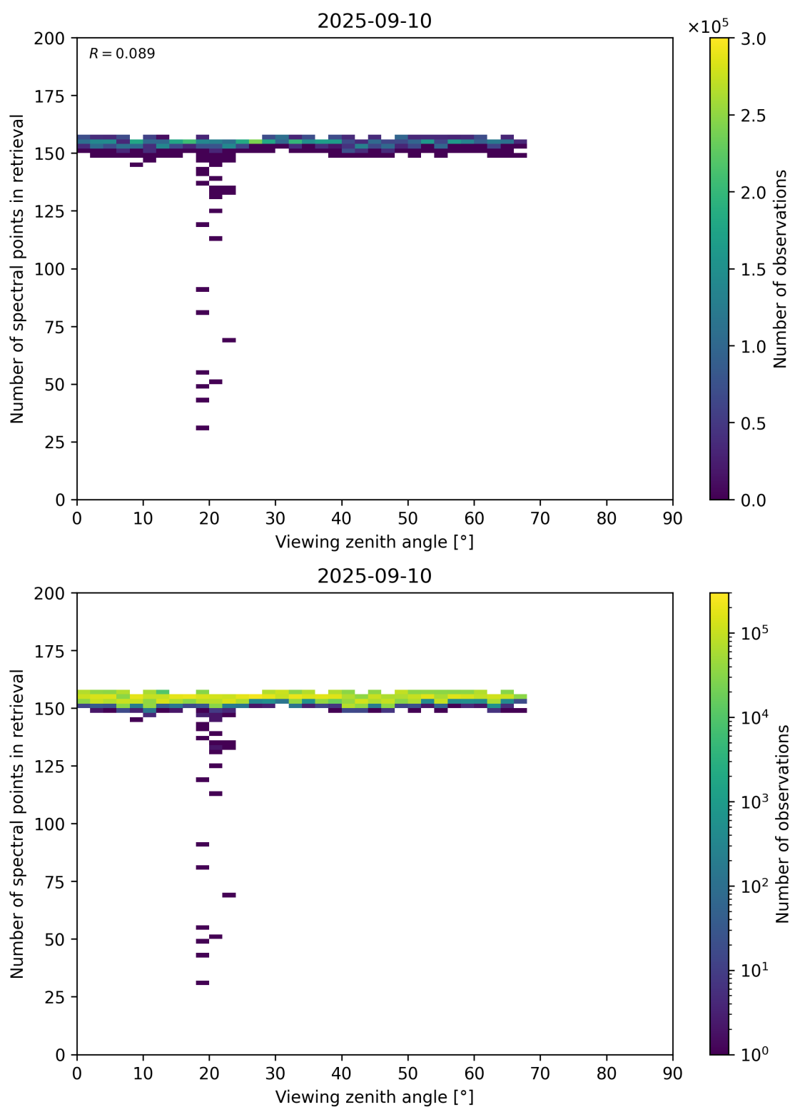
Figure 76: Scatter density plot of “Viewing zenith angle” against “Number of spectral points in retrieval” for 2025-09-10 to 2025-09-11.
