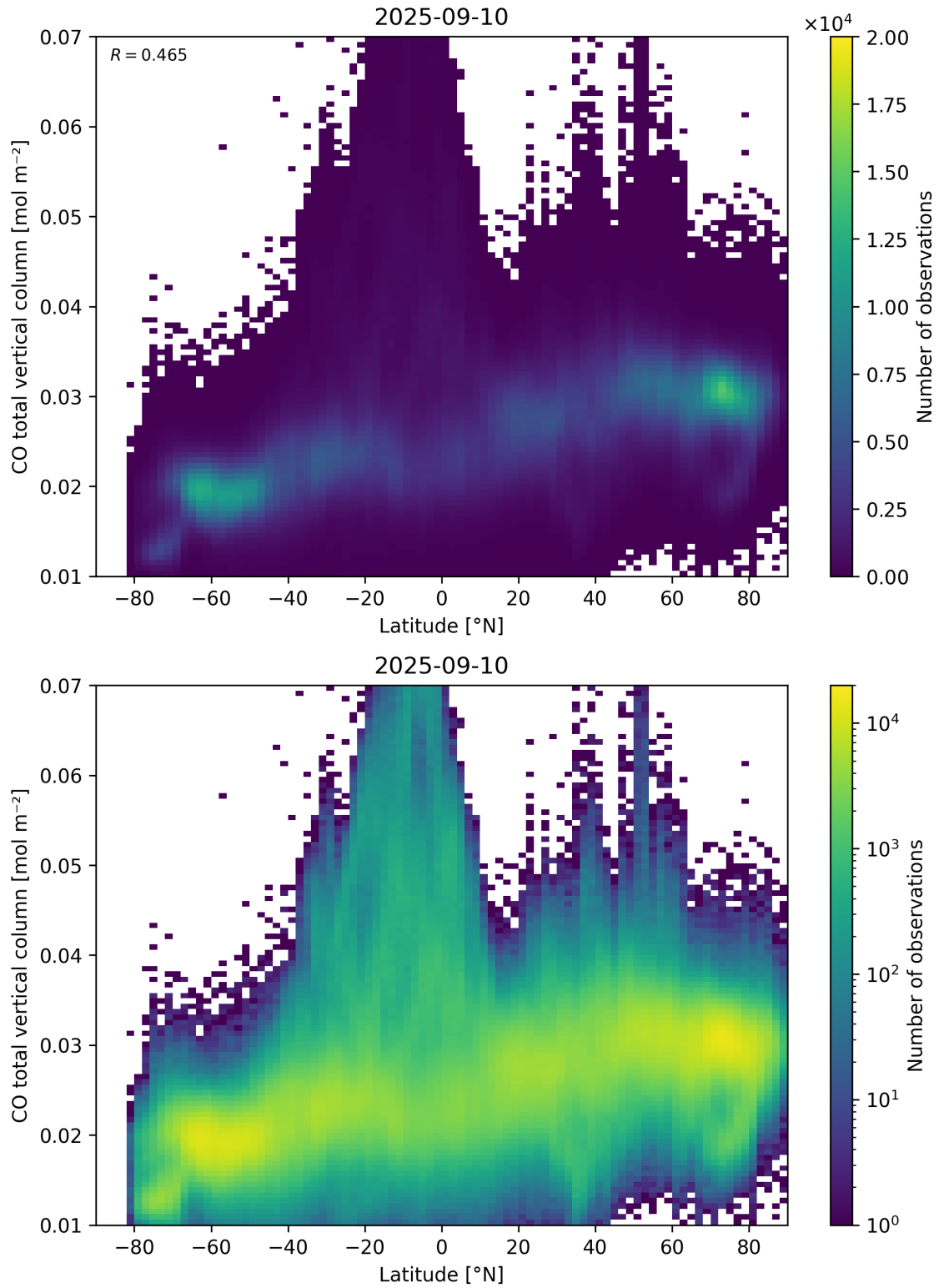
Figure 51: Scatter density plot of “Latitude” against “CO total vertical column” for 2025-09-10 to 2025-09-11.
