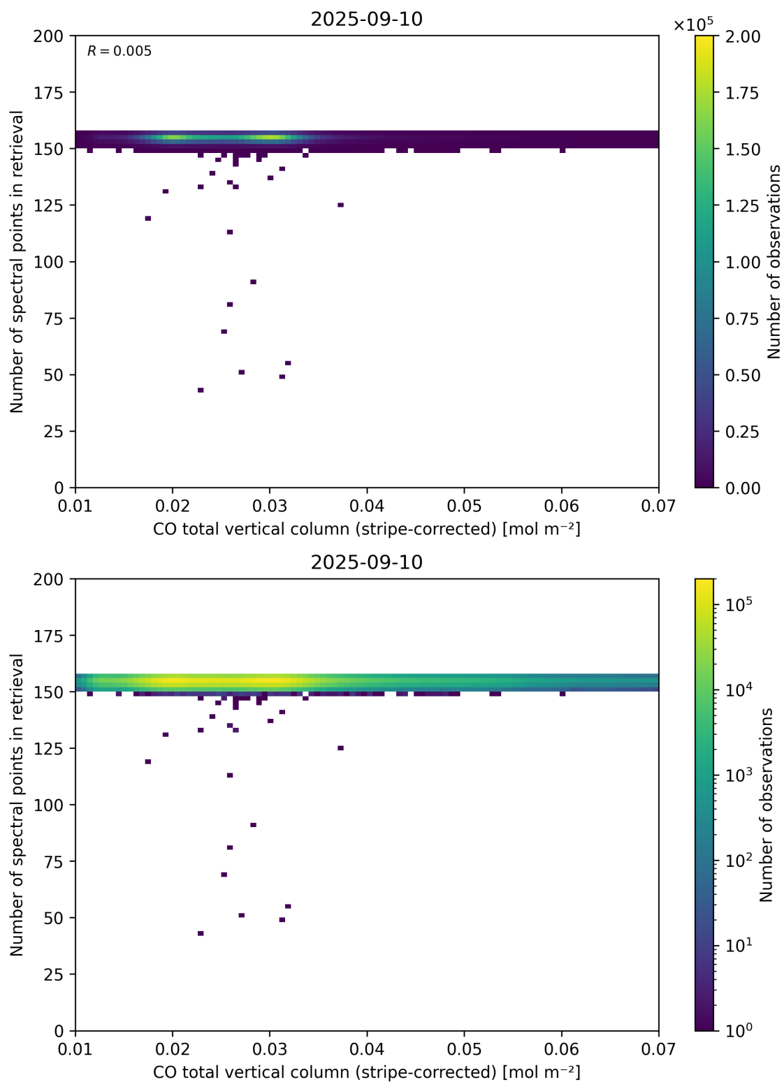
Figure 40: Scatter density plot of “CO total vertical column (stripe-corrected)” against “Number of spectral points in retrieval” for 2025-09-10 to 2025-09-11.
