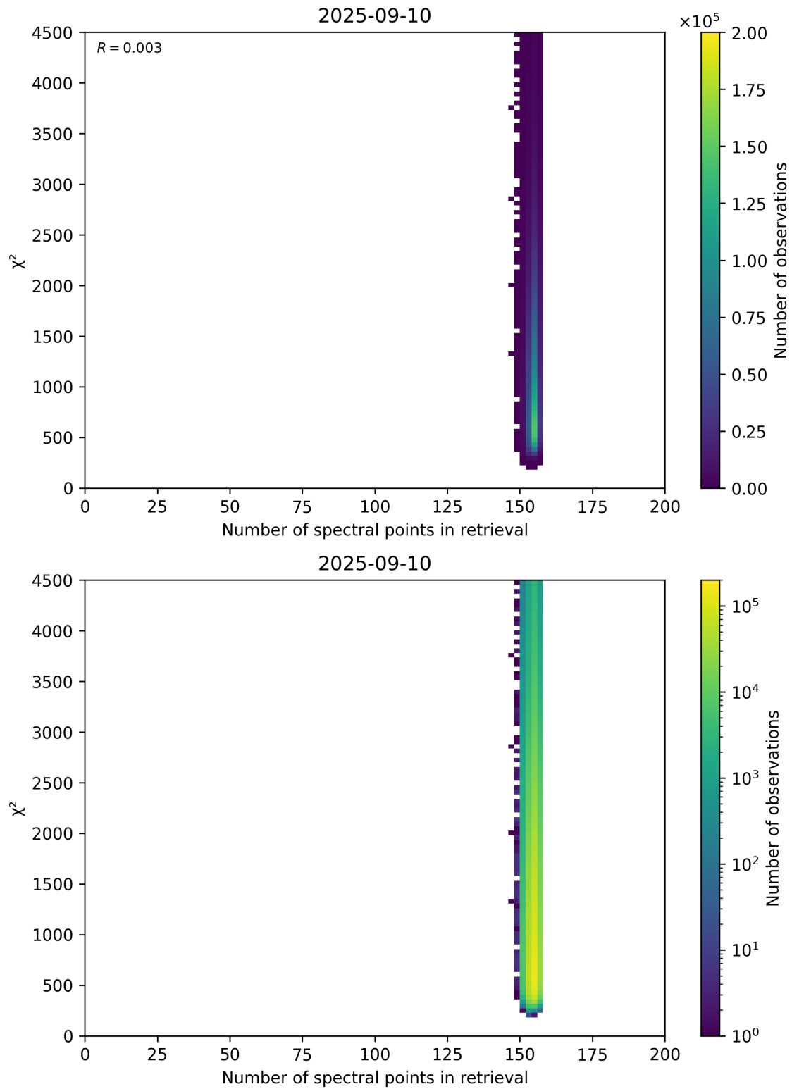
Figure 58: Scatter density plot of “Number of spectral points in retrieval” against “ \chi^2 ” for 2025-09-10 to 2025-09-11.
