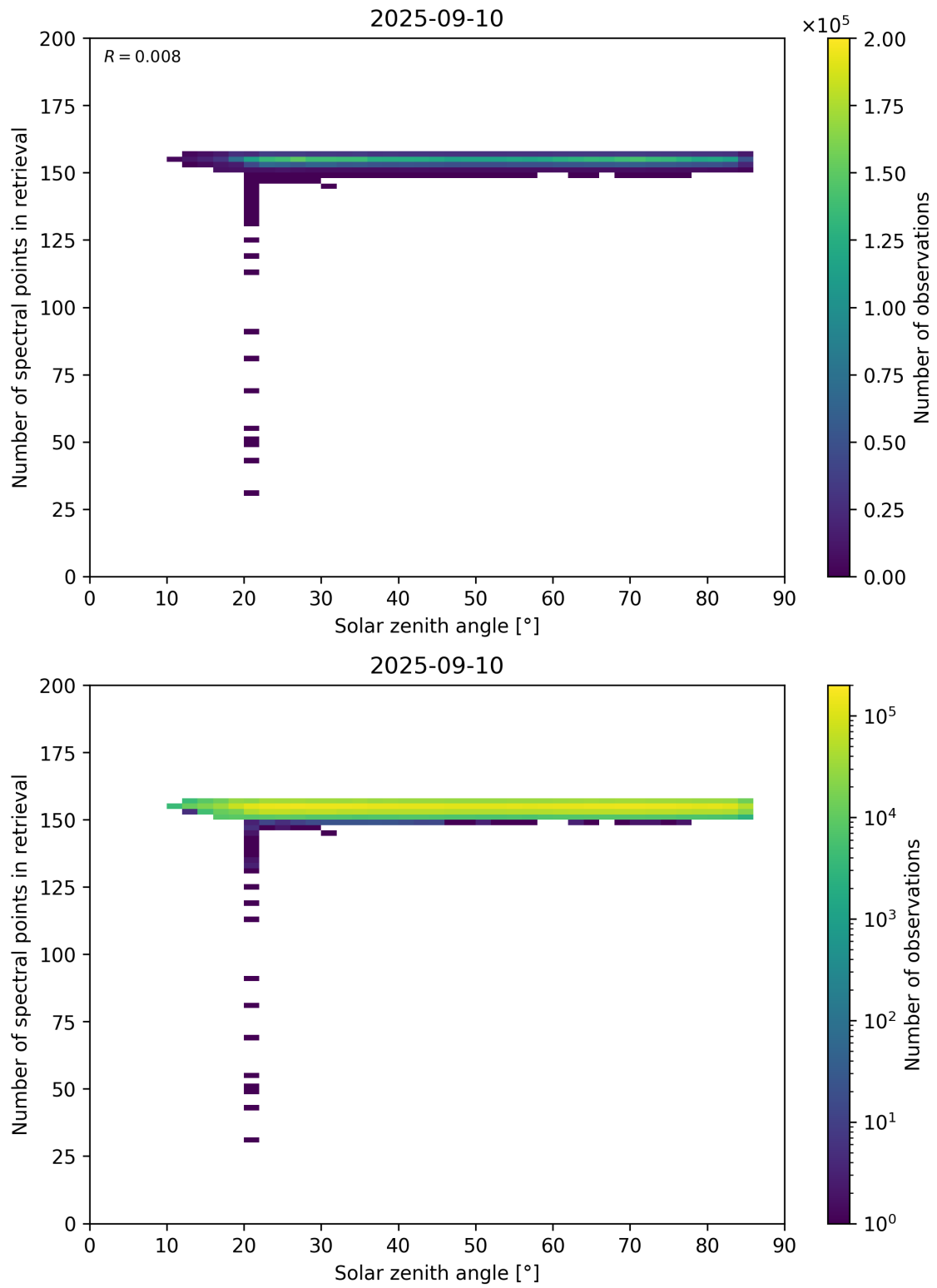
Figure 68: Scatter density plot of “Solar zenith angle” against “Number of spectral points in retrieval” for 2025-09-10 to 2025-09-11.
