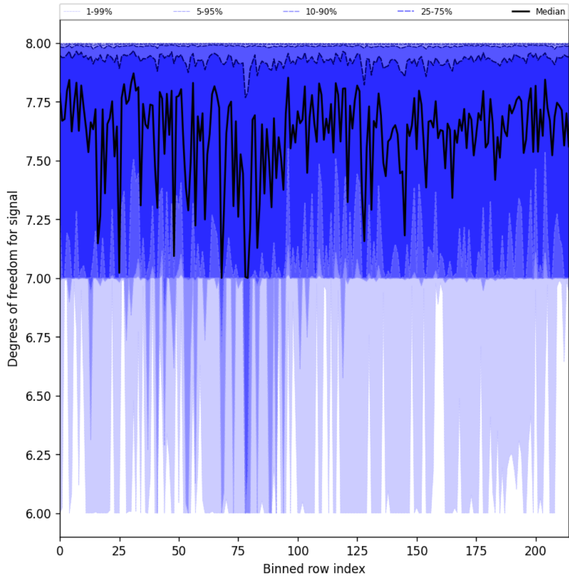
Figure 31: Along track statistics of “Degrees of freedom for signal” for 2025-09-10 to 2025-09-11
