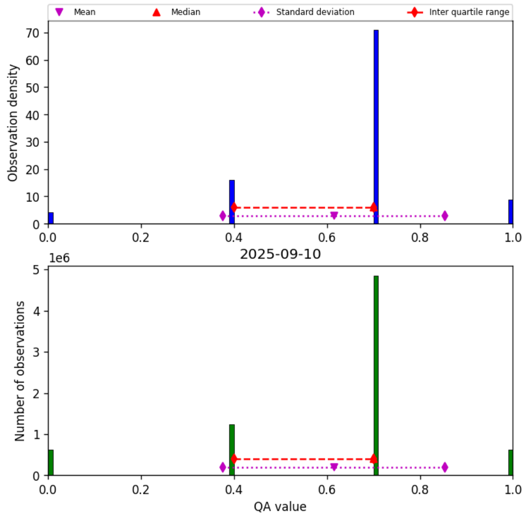
Figure 17: Histogram of “QA value” for 2025-09-10 to 2025-09-11
