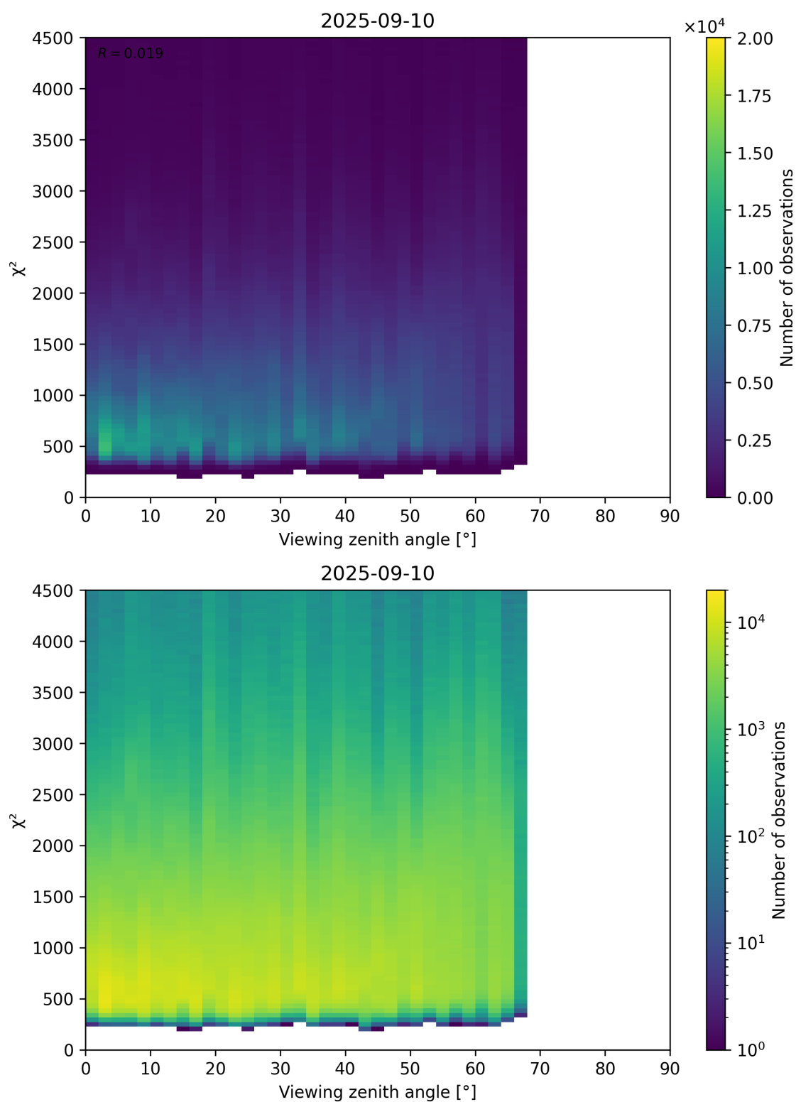
Figure 72: Scatter density plot of “Viewing zenith angle” against “ \chi^2 ” for 2025-09-10 to 2025-09-11.
