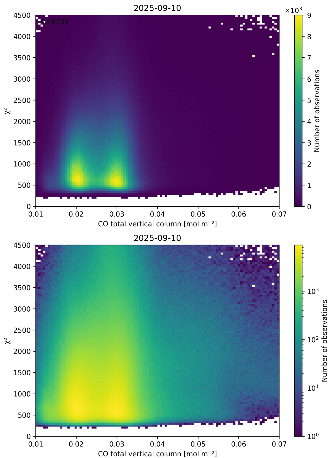
Figure 35: Scatter density plot of “CO total vertical column” against “ \chi^2 ” for 2025-09-10 to 2025-09-11.
