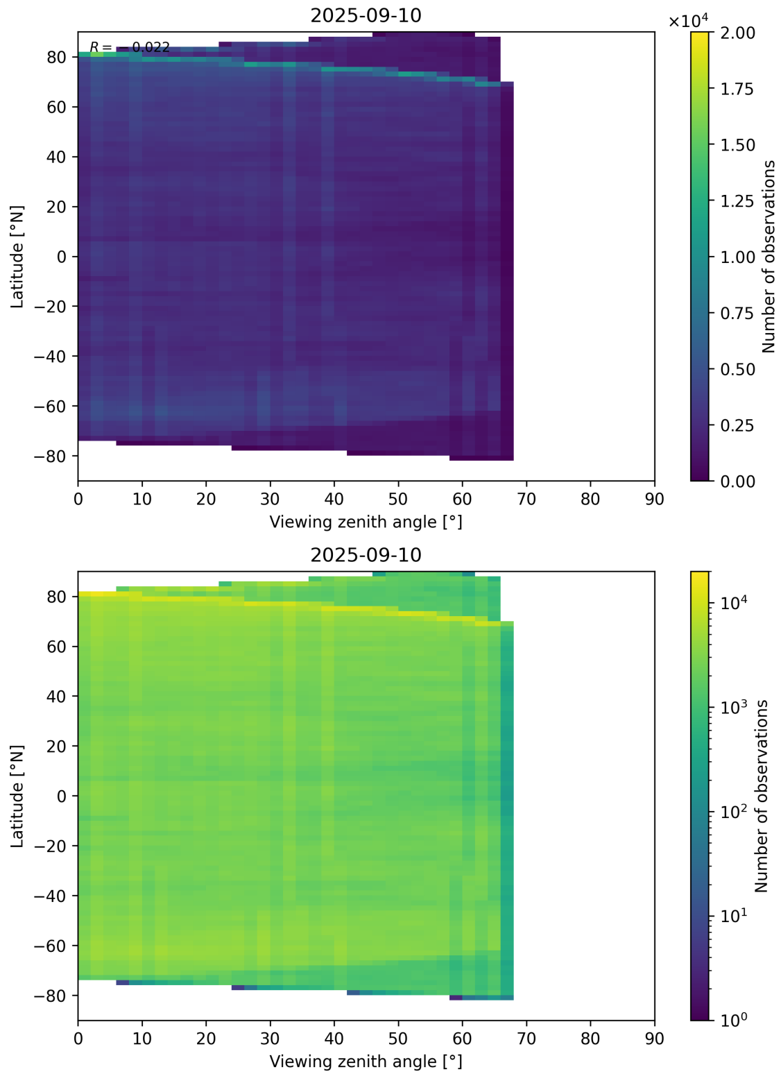
Figure 74: Scatter density plot of “Viewing zenith angle” against “Latitude” for 2025-09-10 to 2025-09-11.
