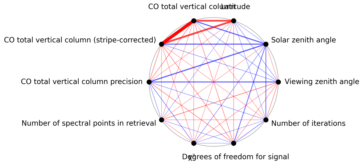
Figure 1: Map of correlation graph for 2025-09-10 to 2025-09-11.
