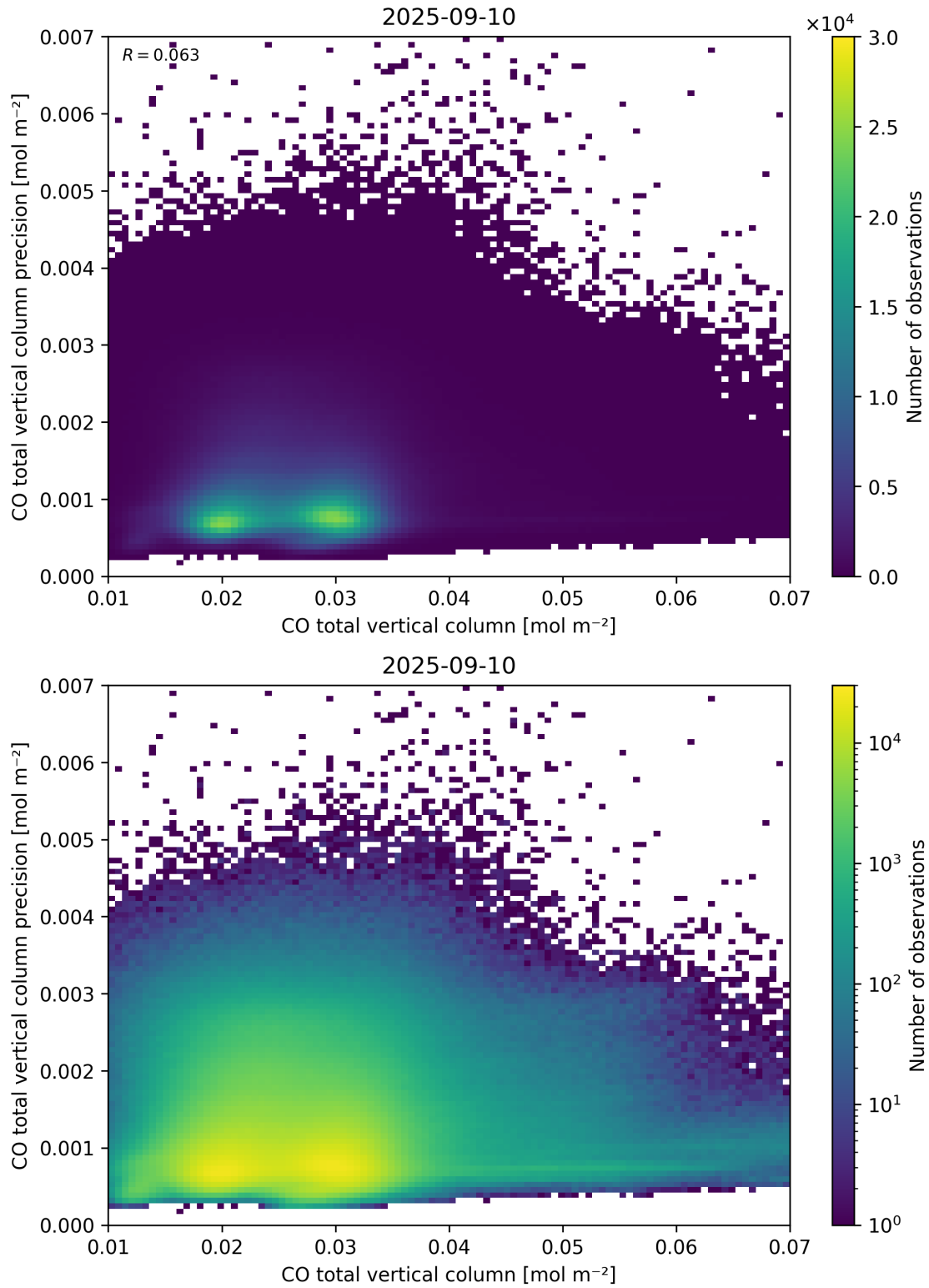
Figure 34: Scatter density plot of “CO total vertical column” against “CO total vertical column precision” for 2025-09-10 to 2025-09-11.
