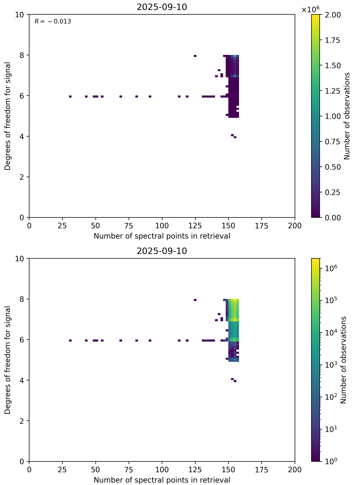
Figure 59: Scatter density plot of “Number of spectral points in retrieval” against “Degrees of freedom for signal” for 2025-09-10 to 2025-09-11.
