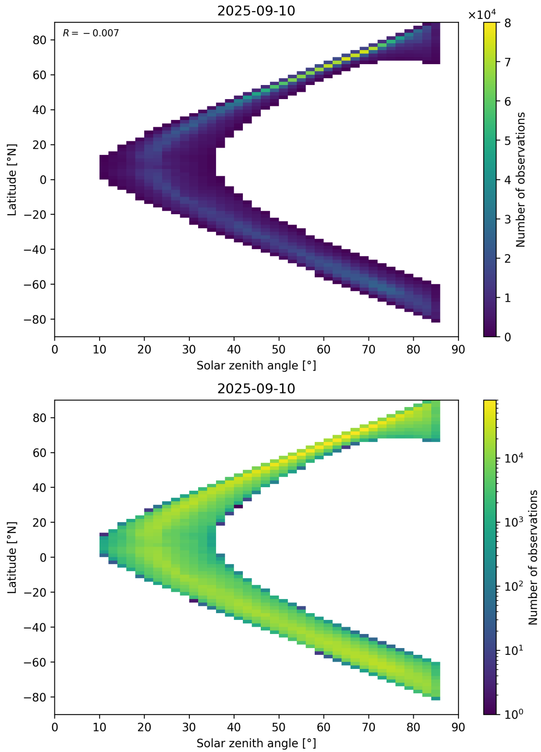
Figure 66: Scatter density plot of “Solar zenith angle” against “Latitude” for 2025-09-10 to 2025-09-11.
