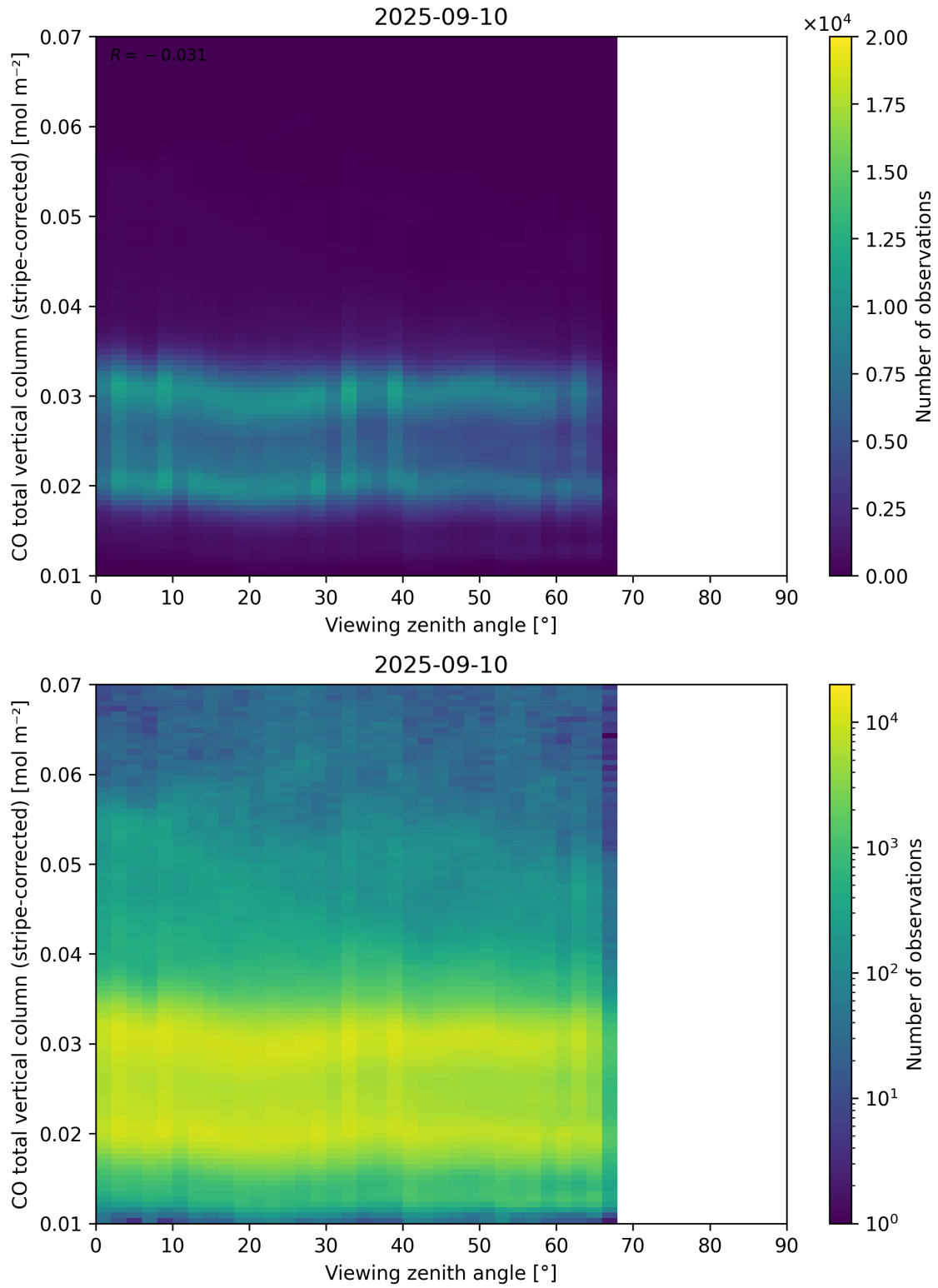
Figure 70: Scatter density plot of “Viewing zenith angle” against “CO total vertical column (stripe-corrected)” for 2025-09-10 to 2025-09-11.
