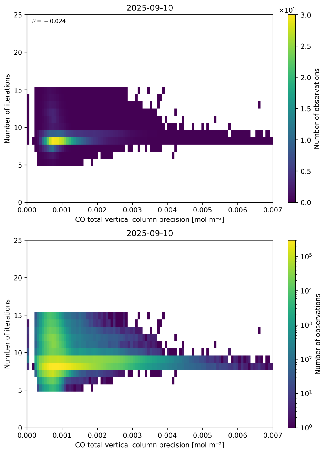
Figure 46: Scatter density plot of “CO total vertical column precision” against “Number of iterations” for 2025-09-10 to 2025-09-11.
