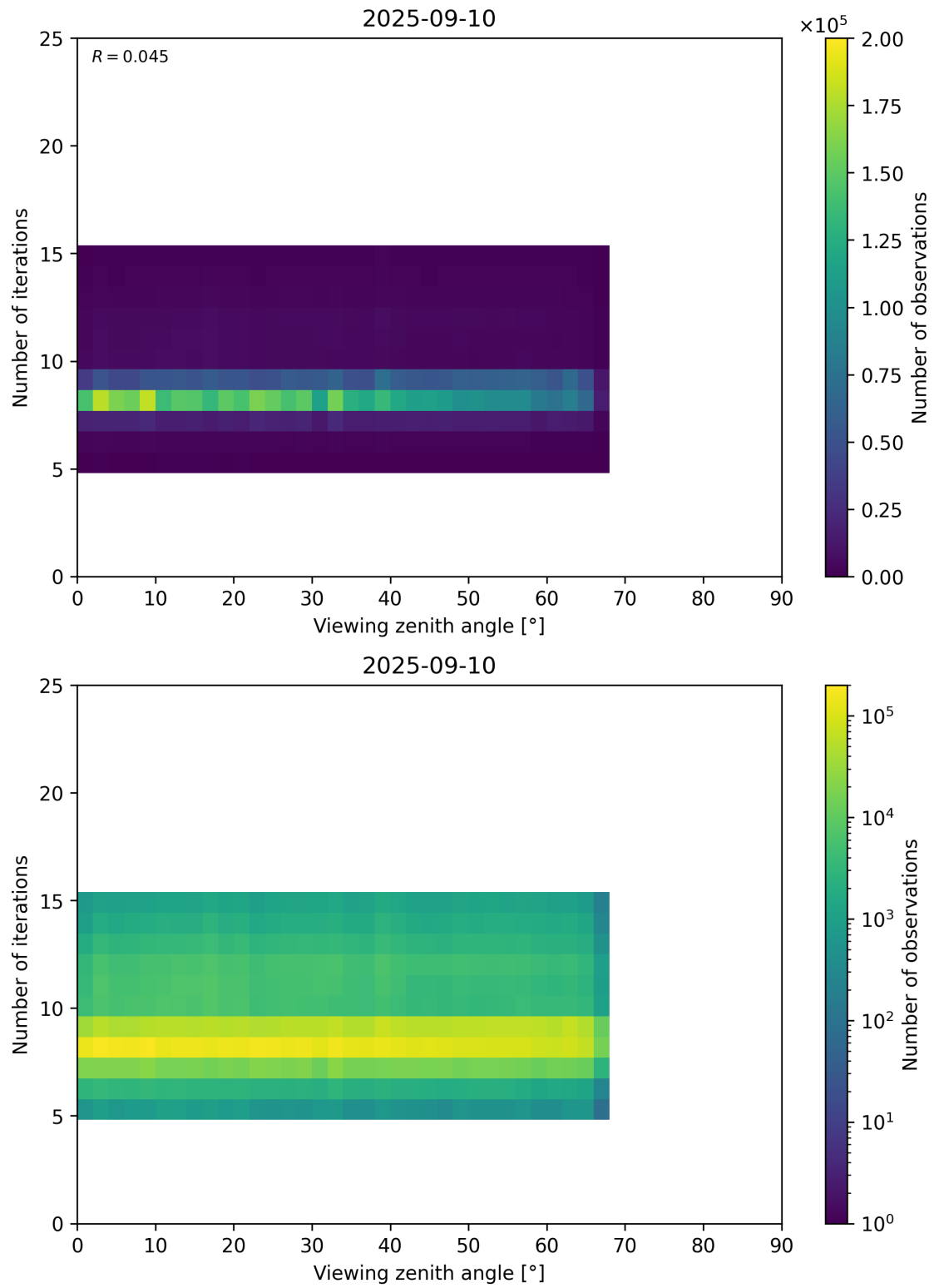
Figure 75: Scatter density plot of “Viewing zenith angle” against “Number of iterations” for 2025-09-10 to 2025-09-11.
