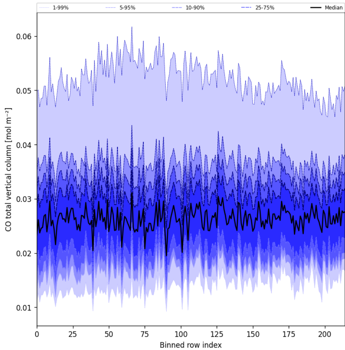
Figure 26: Along track statistics of “CO total vertical column” for 2025-09-10 to 2025-09-11
