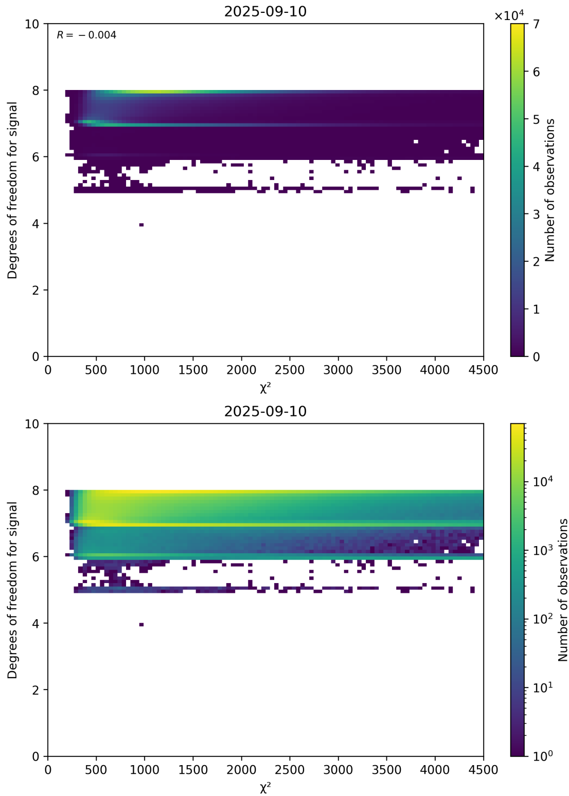
Figure 48: Scatter density plot of " \chi^2 " against "Degrees of freedom for signal" for 2025-09-10 to 2025-09-11.
