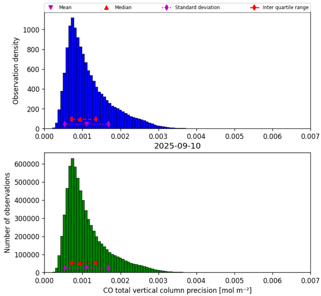
Figure 20: Histogram of “CO total vertical column precision” for 2025-09-10 to 2025-09-11
