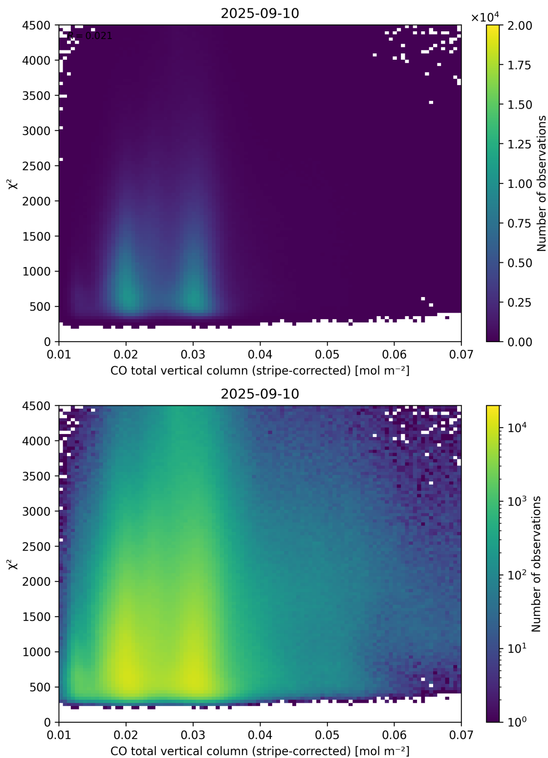
Figure 37: Scatter density plot of “CO total vertical column (stripe-corrected)” against “ \chi^2 ” for 2025-09-10 to 2025-09-11.
