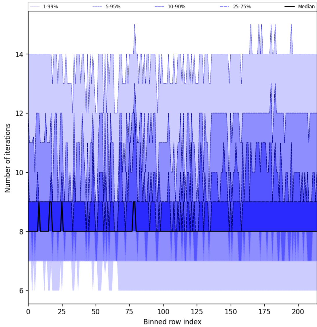
Figure 32: Along track statistics of “Number of iterations” for 2025-09-10 to 2025-09-11
