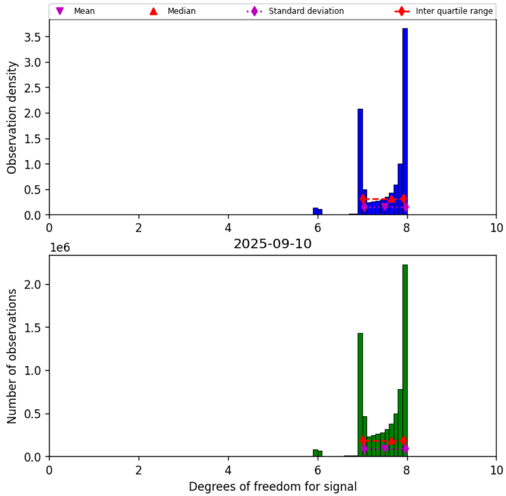
Figure 23: Histogram of “Degrees of freedom for signal” for 2025-09-10 to 2025-09-11
