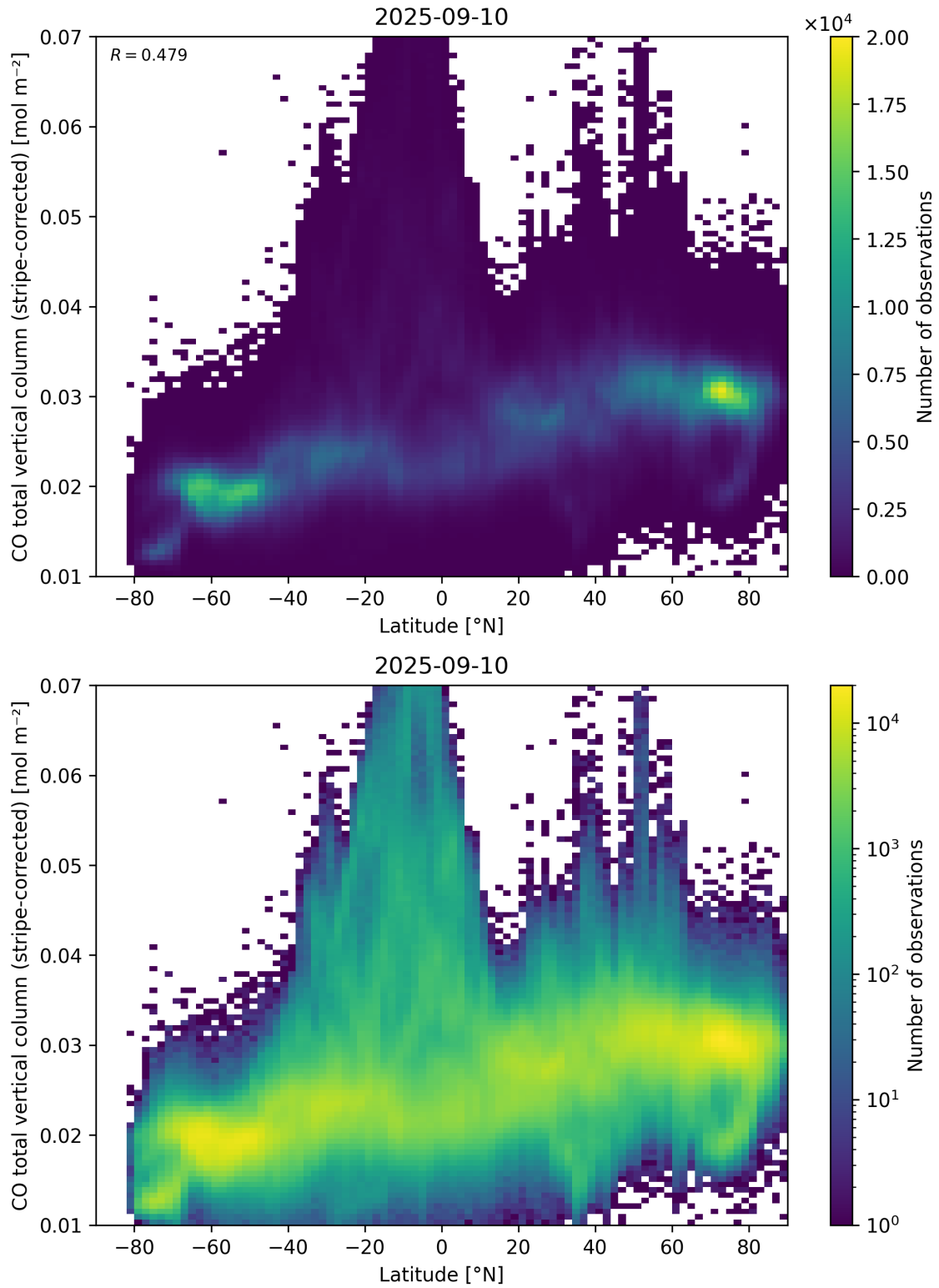
Figure 52: Scatter density plot of “Latitude” against “CO total vertical column (stripe-corrected)” for 2025-09-10 to 2025-09-11.
