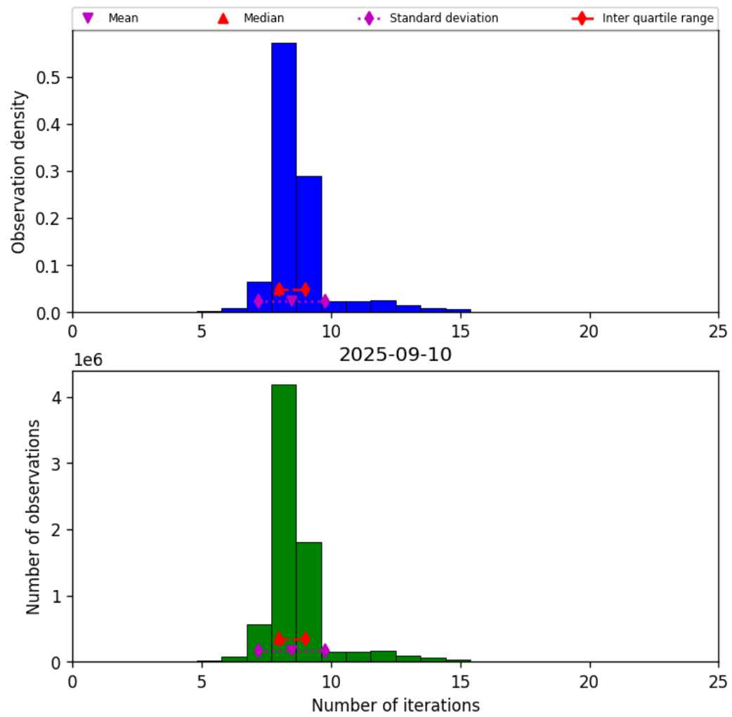
Figure 24: Histogram of “Number of iterations” for 2025-09-10 to 2025-09-11
