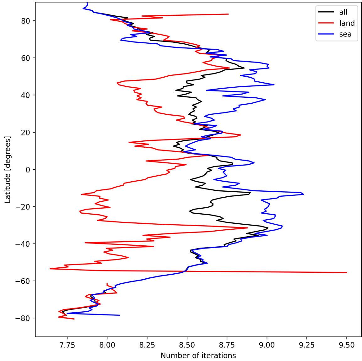
Figure 16: Zonal average of “Number of iterations” for 2025-09-10 to 2025-09-11.
