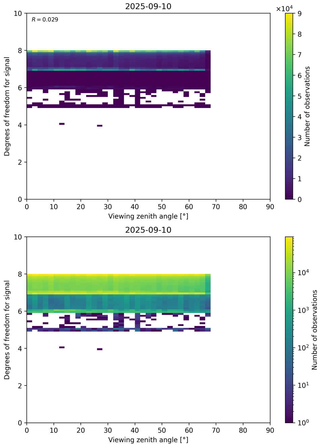
Figure 73: Scatter density plot of “Viewing zenith angle” against “Degrees of freedom for signal” for 2025-09-10 to 2025-09-11.
