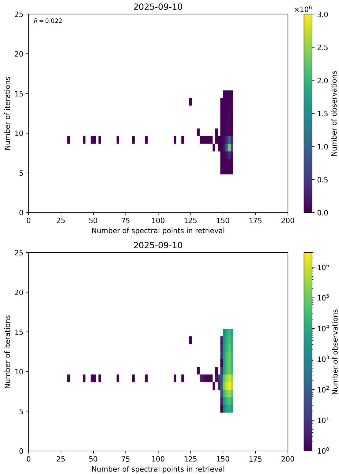
Figure 60: Scatter density plot of “Number of spectral points in retrieval” against “Number of iterations” for 2025-09-10 to 2025-09-11.
