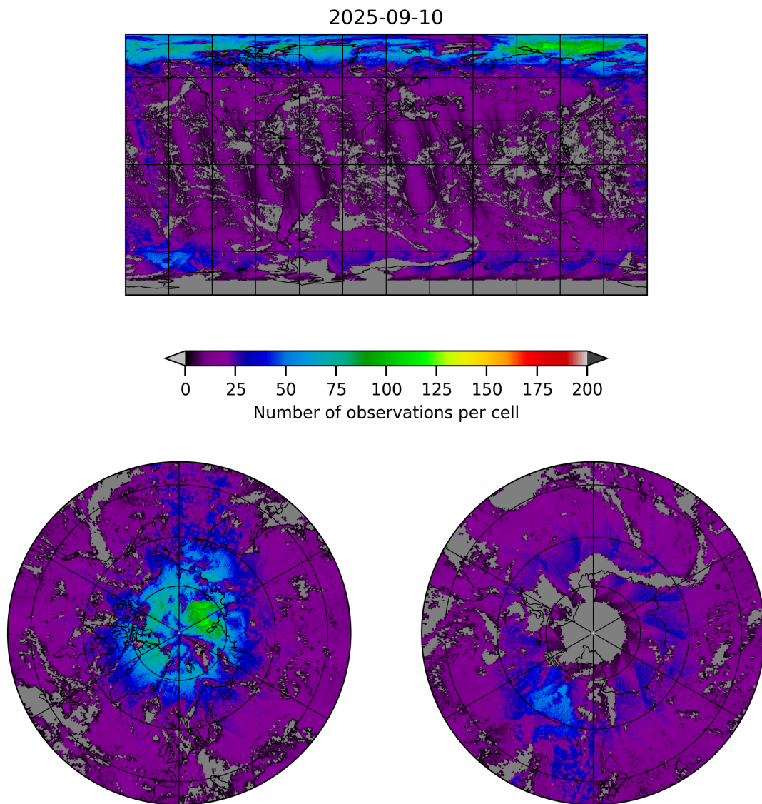
Figure 8: Map of the number of observations for 2025-09-10 to 2025-09-11
