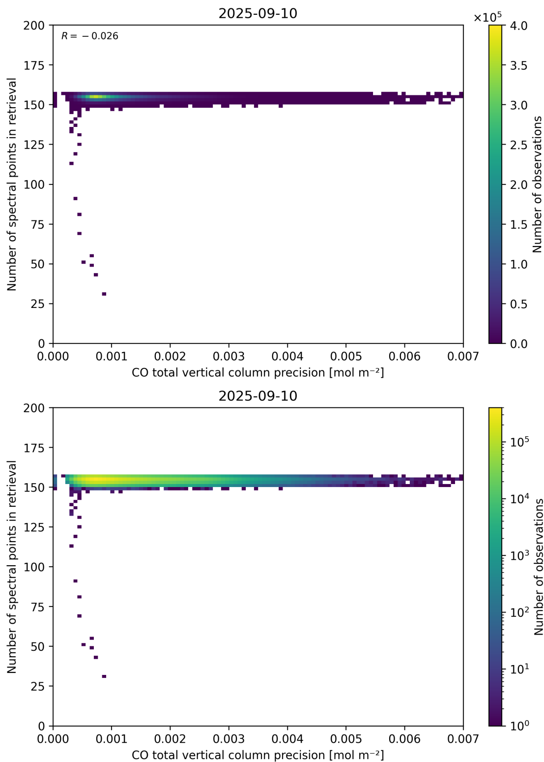
Figure 47: Scatter density plot of “CO total vertical column precision” against “Number of spectral points in retrieval” for 2025-09-10 to 2025-09-11.
