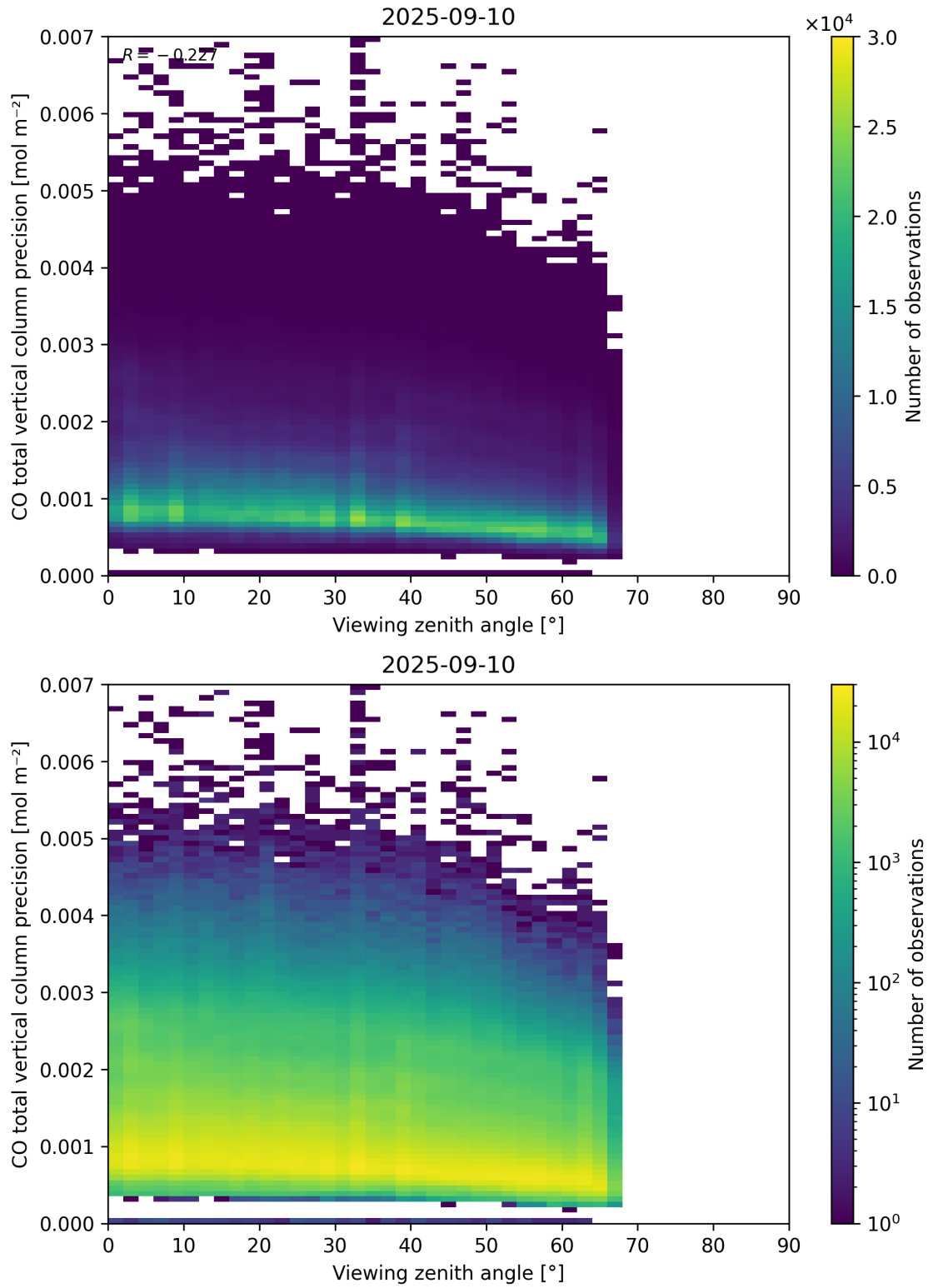
Figure 71: Scatter density plot of “Viewing zenith angle” against “CO total vertical column precision” for 2025-09-10 to 2025-09-11.
