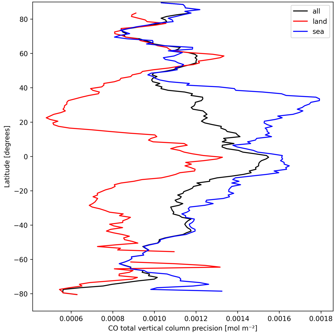
Figure 12: Zonal average of "CO total vertical column precision" for 2025-09-10 to 2025-09-11.
