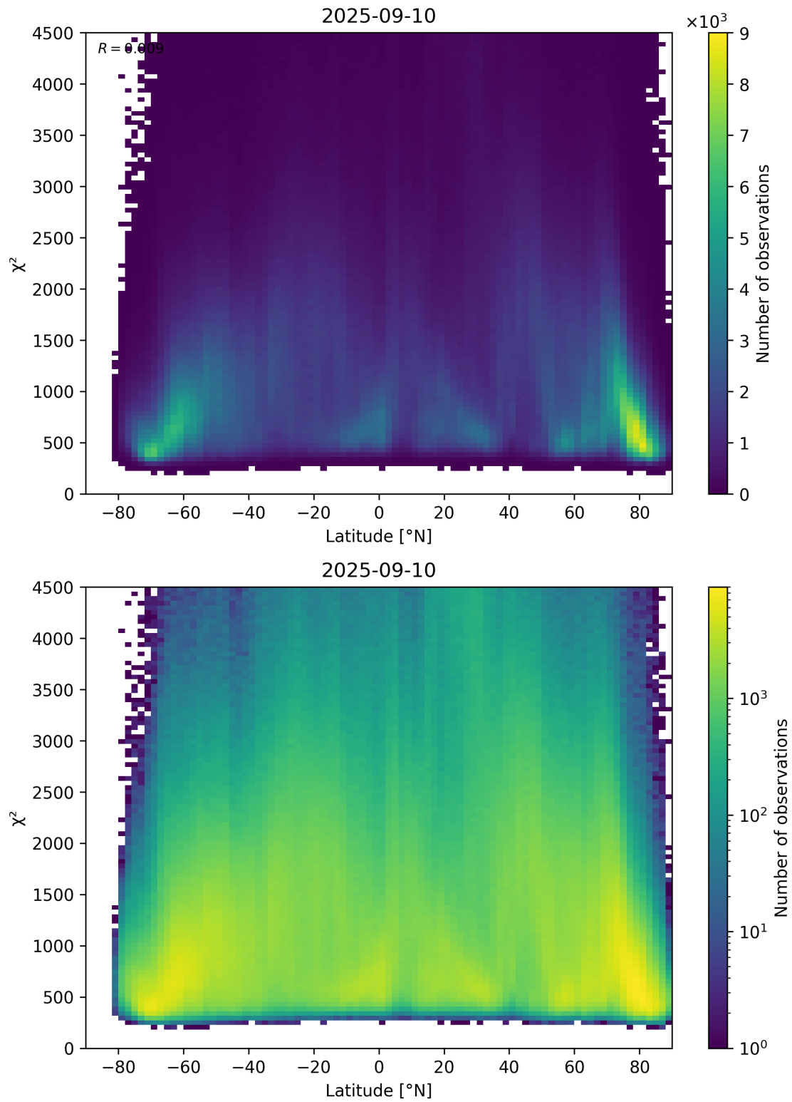
Figure 54: Scatter density plot of “Latitude” against “ \chi^2 ” for 2025-09-10 to 2025-09-11.
