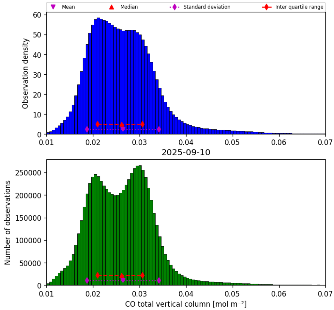
Figure 18: Histogram of “CO total vertical column” for 2025-09-10 to 2025-09-11
