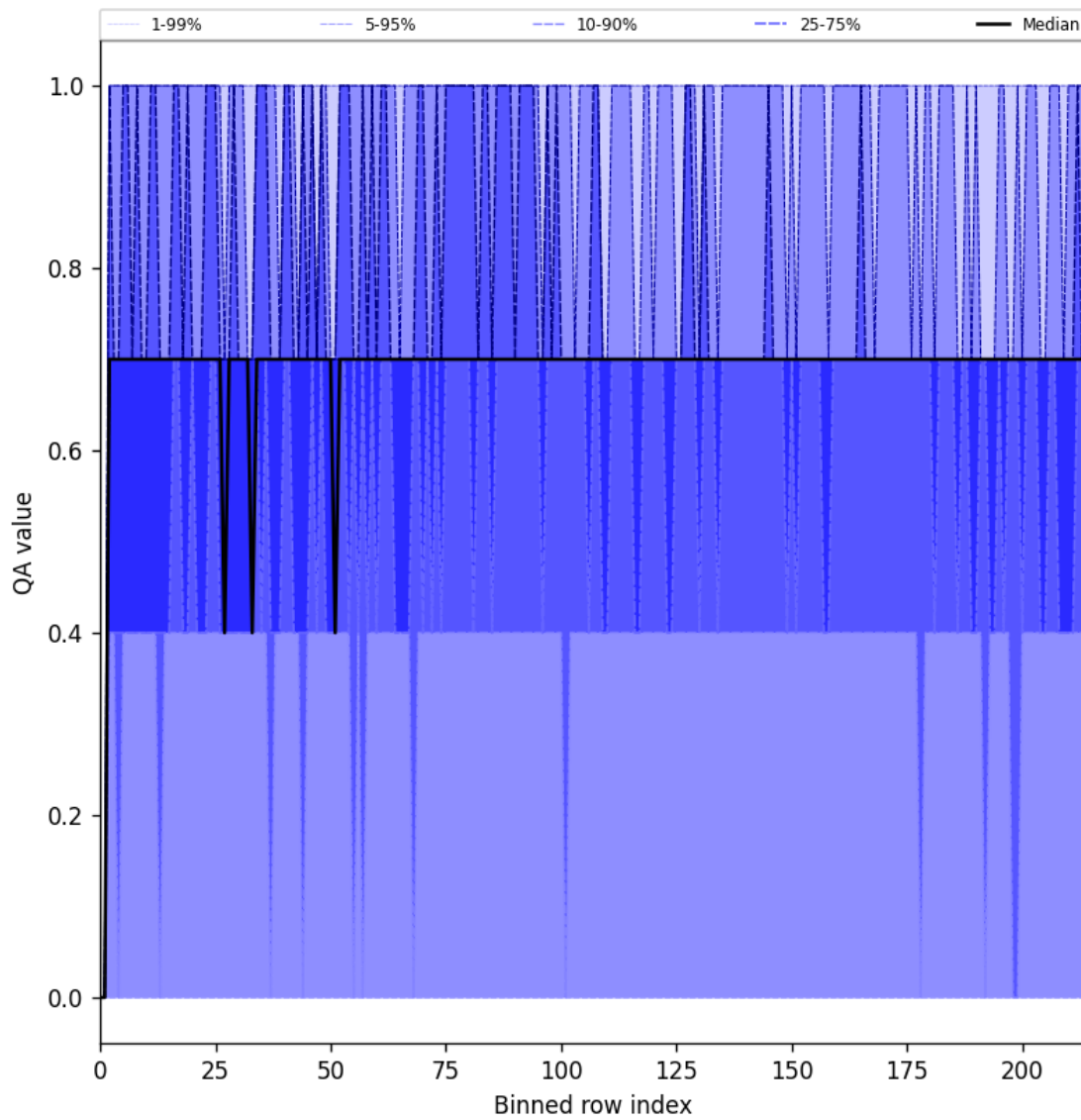
Figure 25: Along track statistics of “QA value” for 2025-09-10 to 2025-09-11
