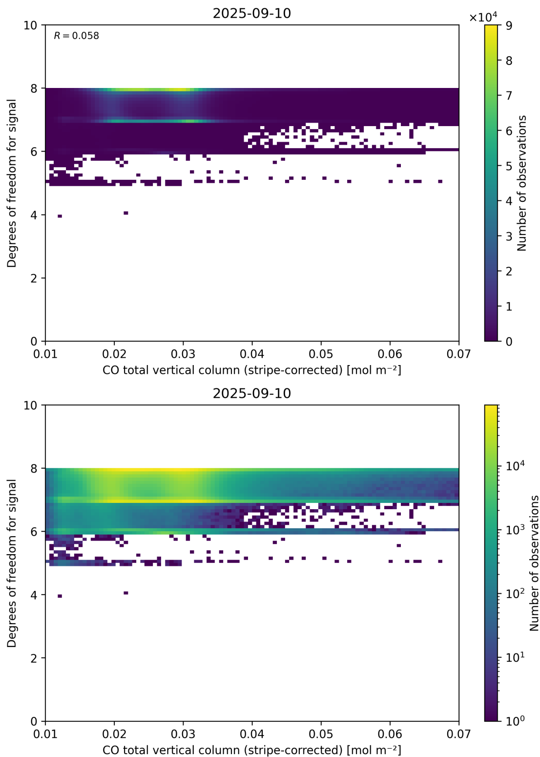
Figure 38: Scatter density plot of “CO total vertical column (stripe-corrected)” against “Degrees of freedom for signal” for 2025-09-10 to 2025-09-11.
