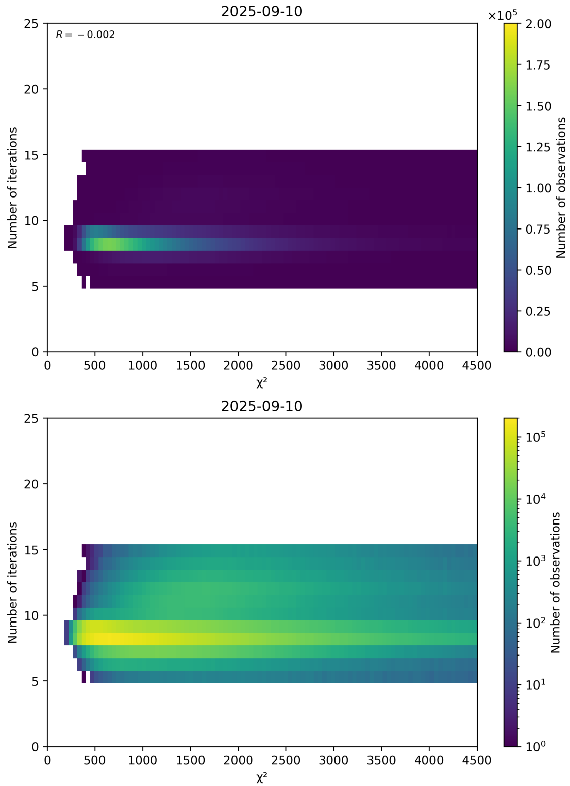
Figure 49: Scatter density plot of “ \chi^2 ” against “Number of iterations” for 2025-09-10 to 2025-09-11.
