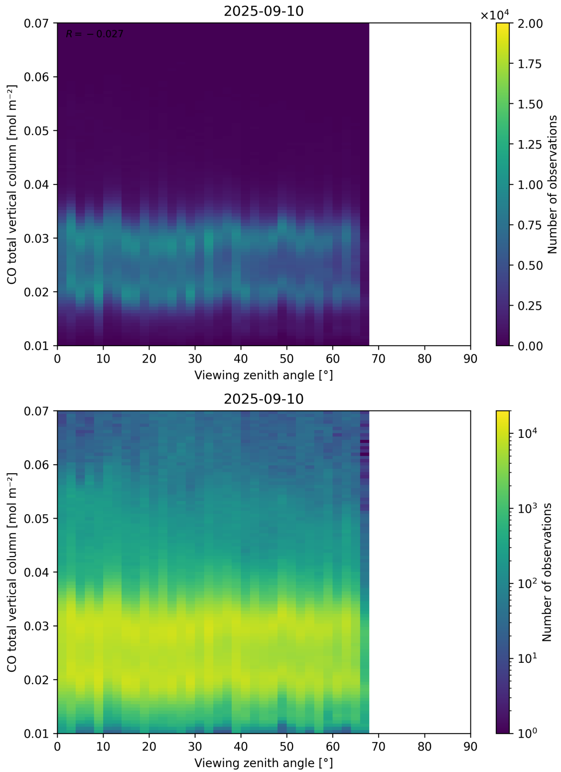
Figure 69: Scatter density plot of “Viewing zenith angle” against “CO total vertical column” for 2025-09-10 to 2025-09-11.
