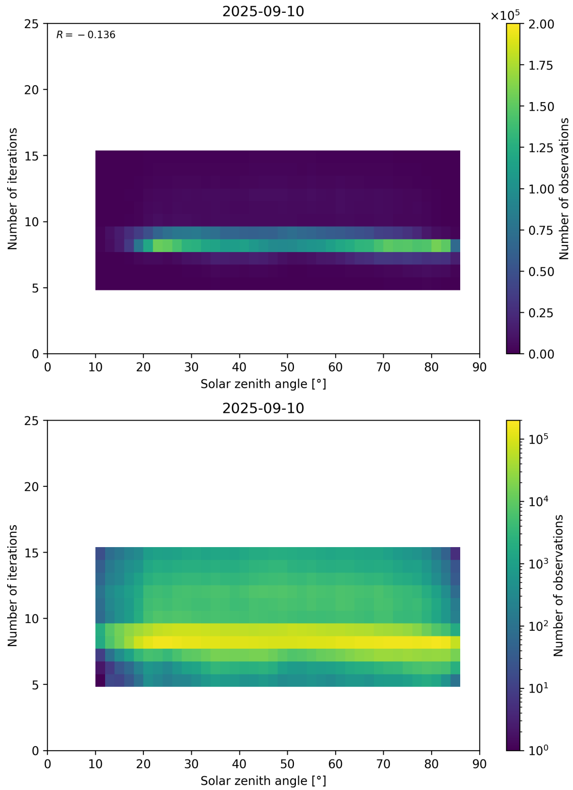
Figure 67: Scatter density plot of “Solar zenith angle” against “Number of iterations” for 2025-09-10 to 2025-09-11.
