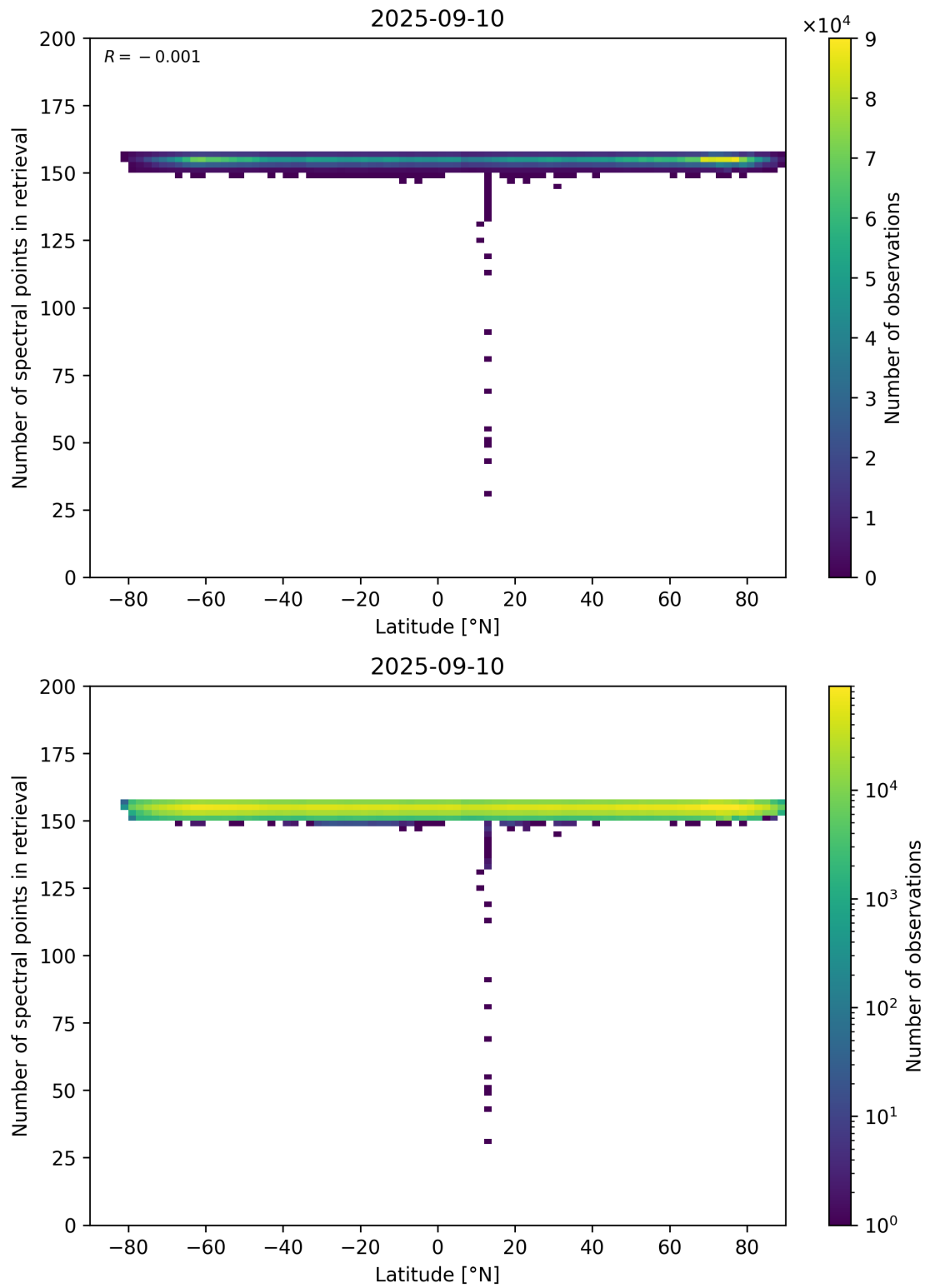
Figure 57: Scatter density plot of “Latitude” against “Number of spectral points in retrieval” for 2025-09-10 to 2025-09-11.
