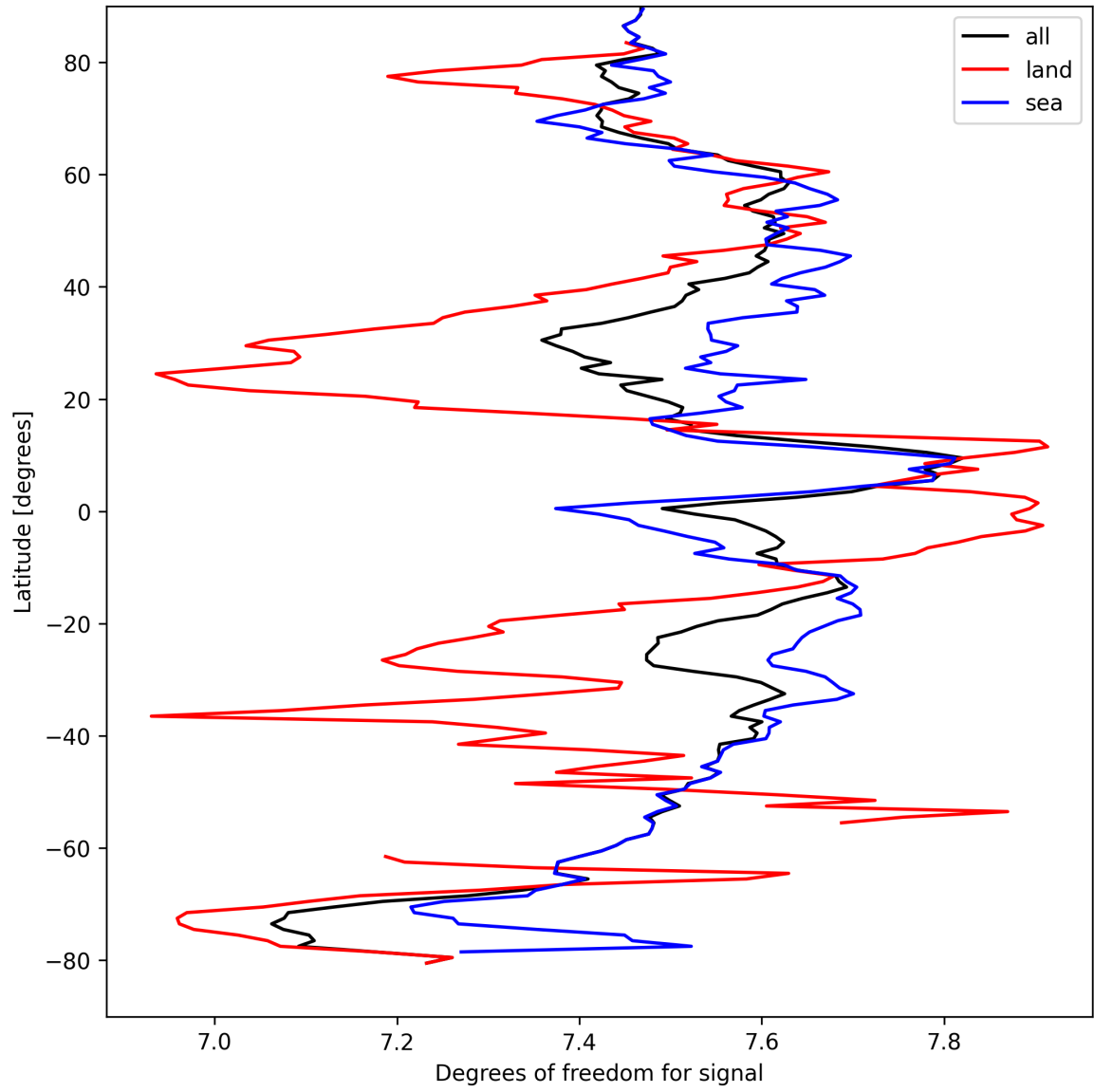
Figure 15: Zonal average of “Degrees of freedom for signal” for 2025-09-10 to 2025-09-11.
