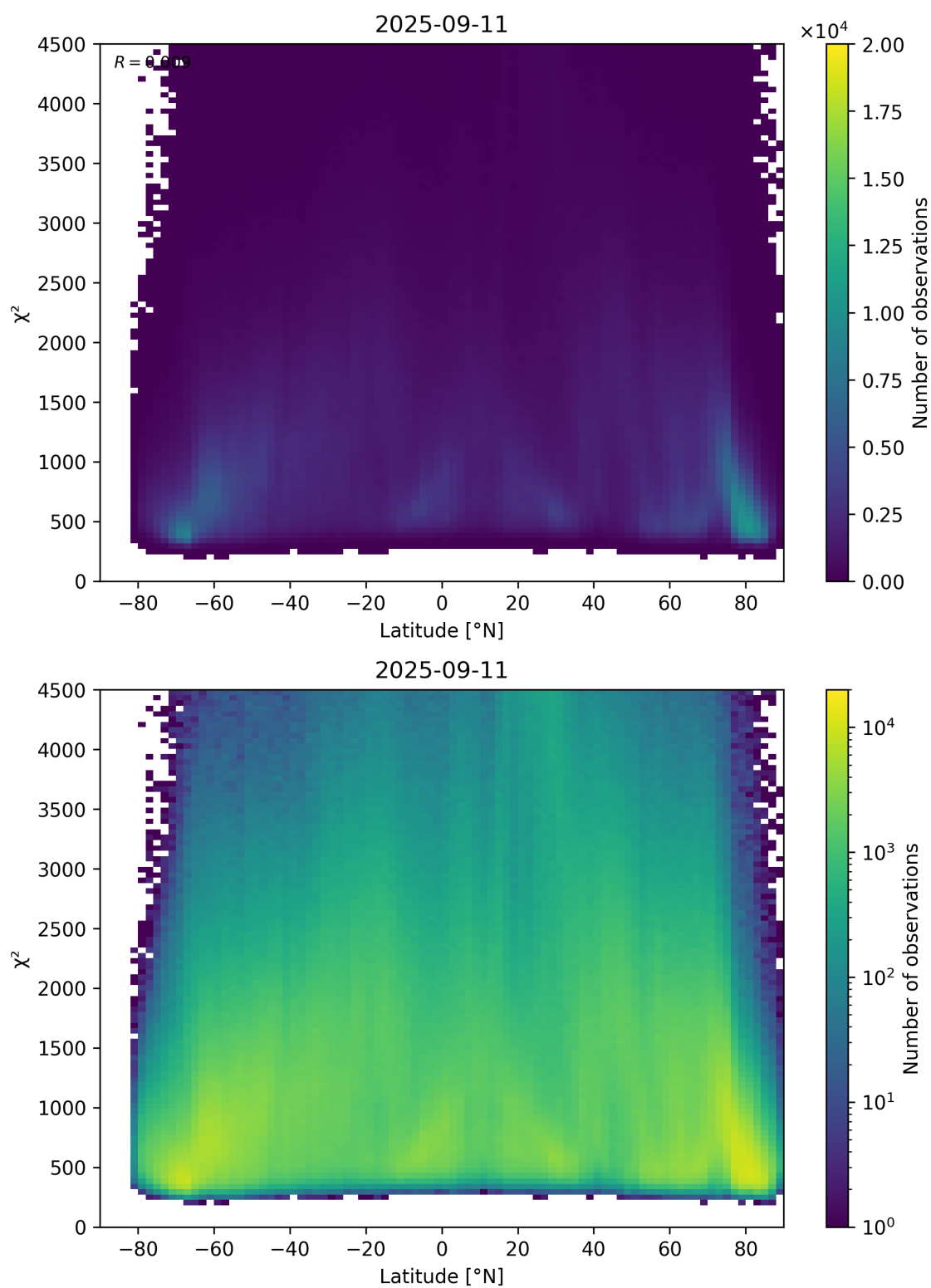
Figure 54: Scatter density plot of “Latitude” against “ \chi^2 ” for 2025-09-10 to 2025-09-12.
