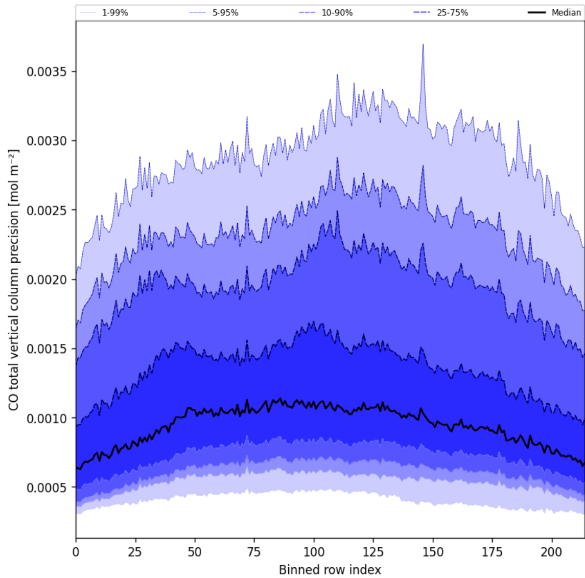
Figure 28: Along track statistics of “CO total vertical column precision” for 2025-09-10 to 2025-09-12
