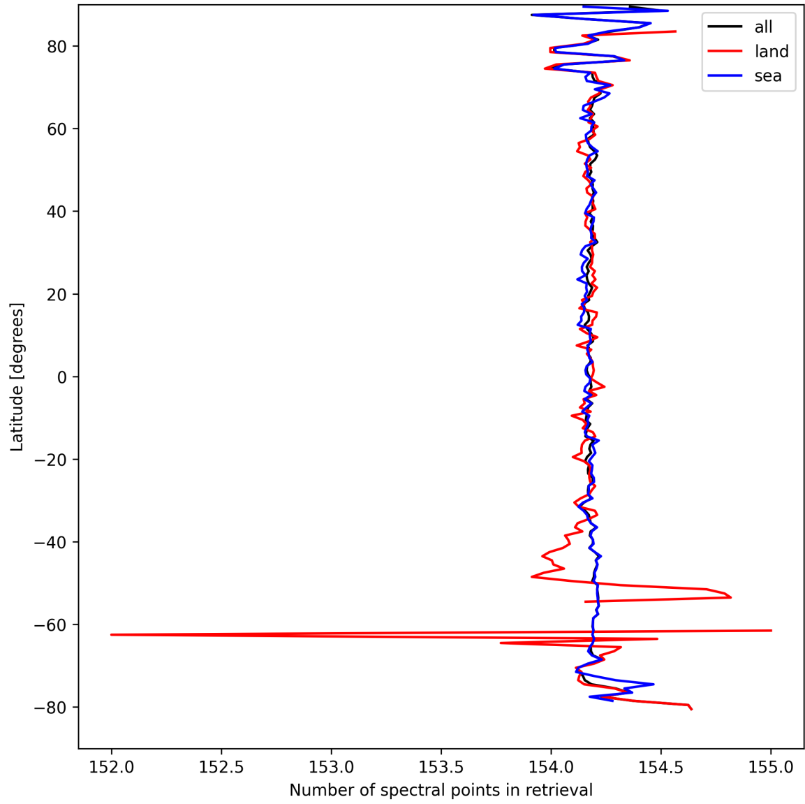
Figure 13: Zonal average of “Number of spectral points in retrieval” for 2025-09-10 to 2025-09-12.
