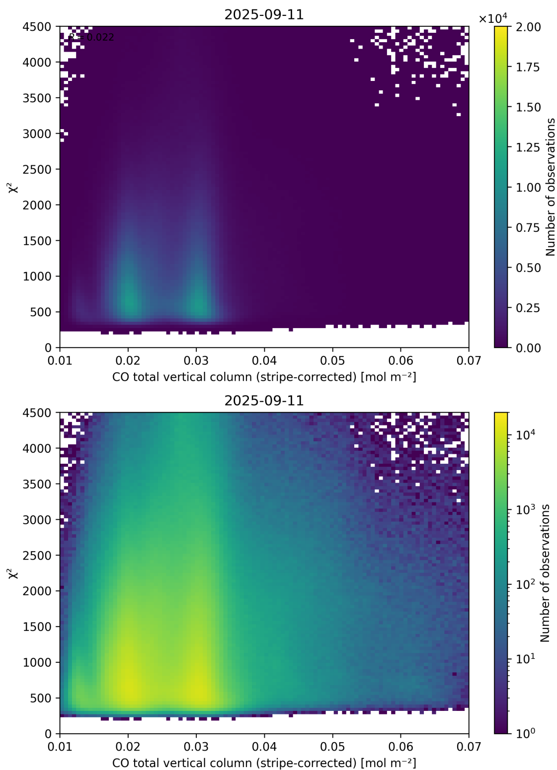
Figure 37: Scatter density plot of “CO total vertical column (stripe-corrected)” against “ \chi^2 ” for 2025-09-10 to 2025-09-12.
