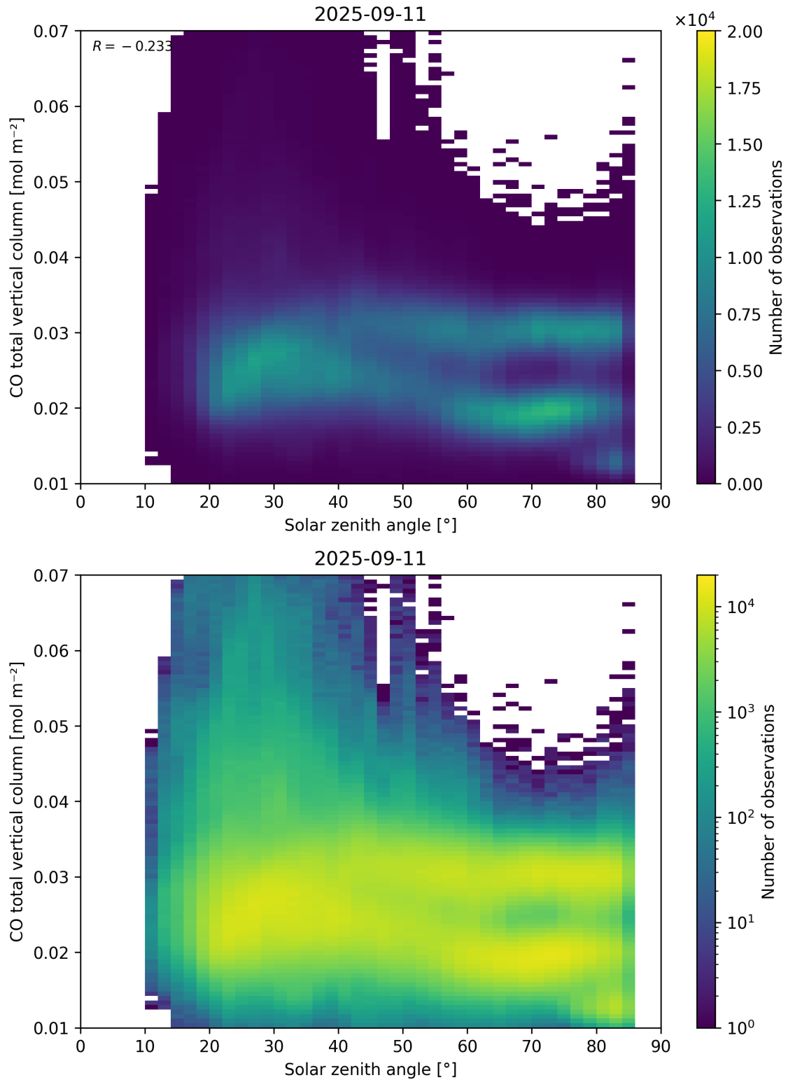
Figure 61: Scatter density plot of “Solar zenith angle” against “CO total vertical column” for 2025-09-10 to 2025-09-12.
