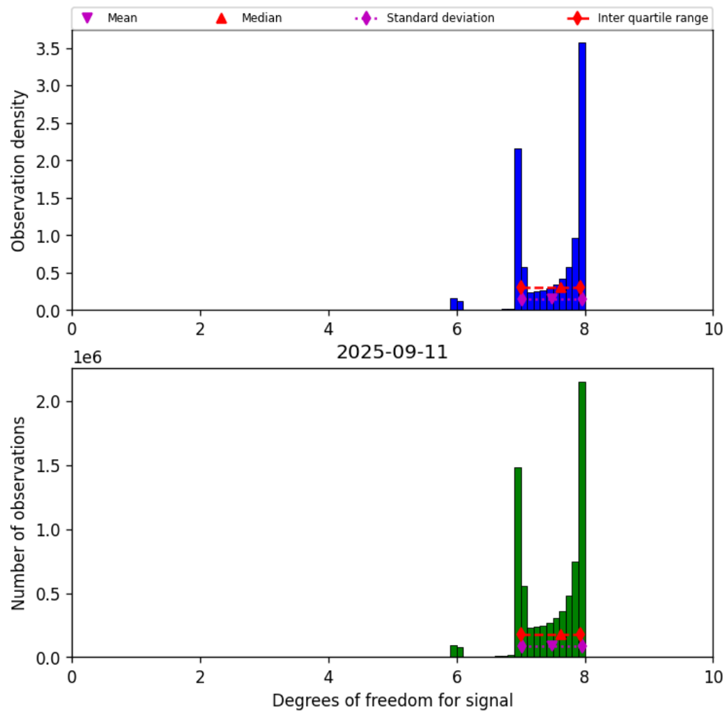
Figure 23: Histogram of “Degrees of freedom for signal” for 2025-09-10 to 2025-09-12
