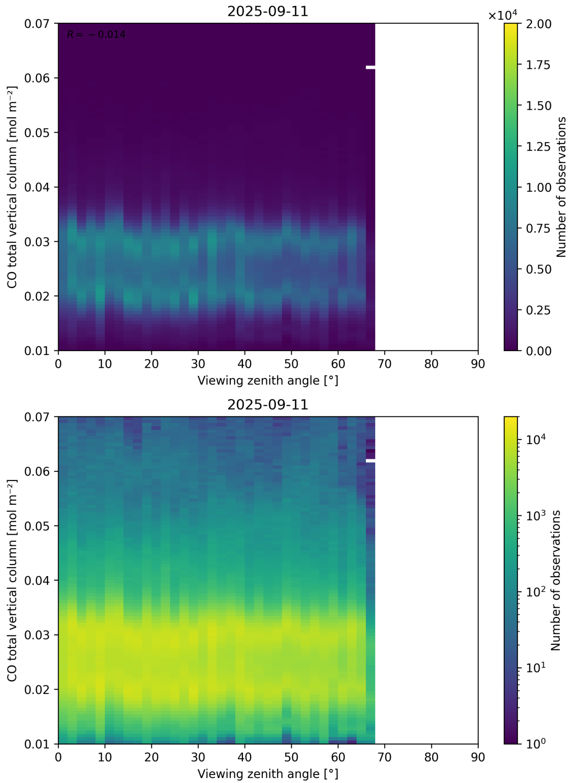
Figure 69: Scatter density plot of “Viewing zenith angle” against “CO total vertical column” for 2025-09-10 to 2025-09-12.
