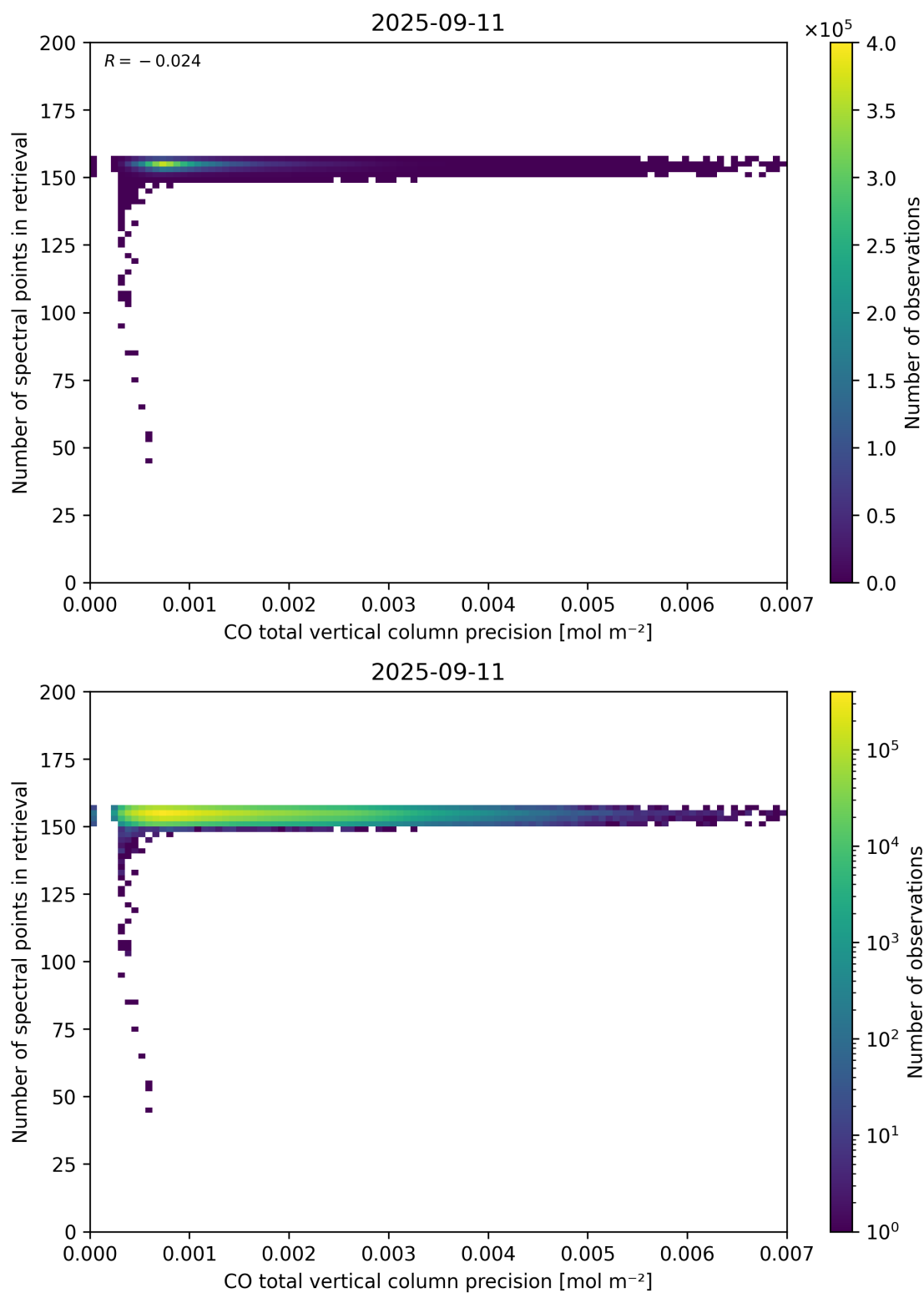
Figure 47: Scatter density plot of “CO total vertical column precision” against “Number of spectral points in retrieval” for 2025-09-10 to 2025-09-12.
