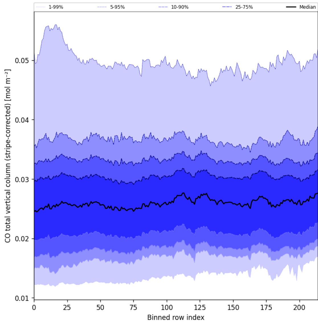
Figure 27: Along track statistics of “CO total vertical column (stripe-corrected)” for 2025-09-10 to 2025-09-12
