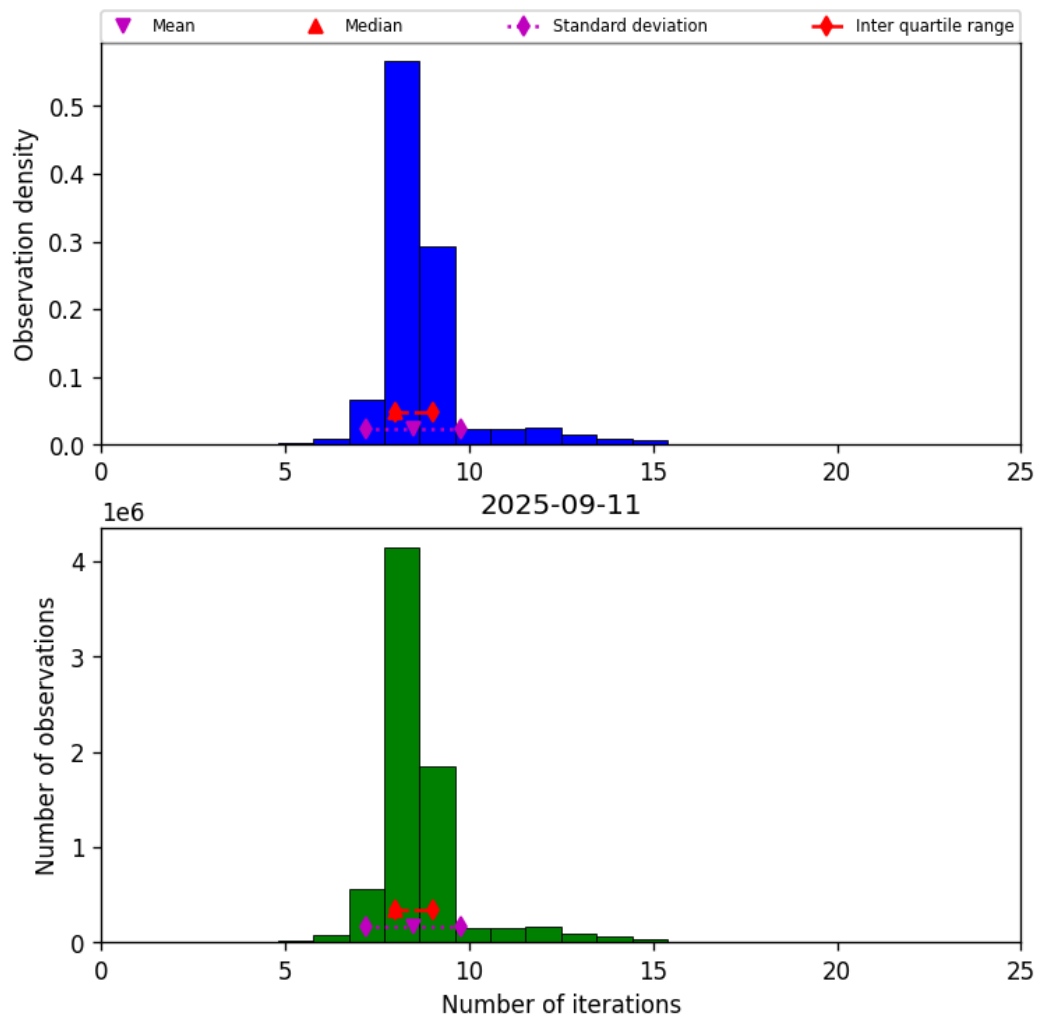
Figure 24: Histogram of “Number of iterations” for 2025-09-10 to 2025-09-12
