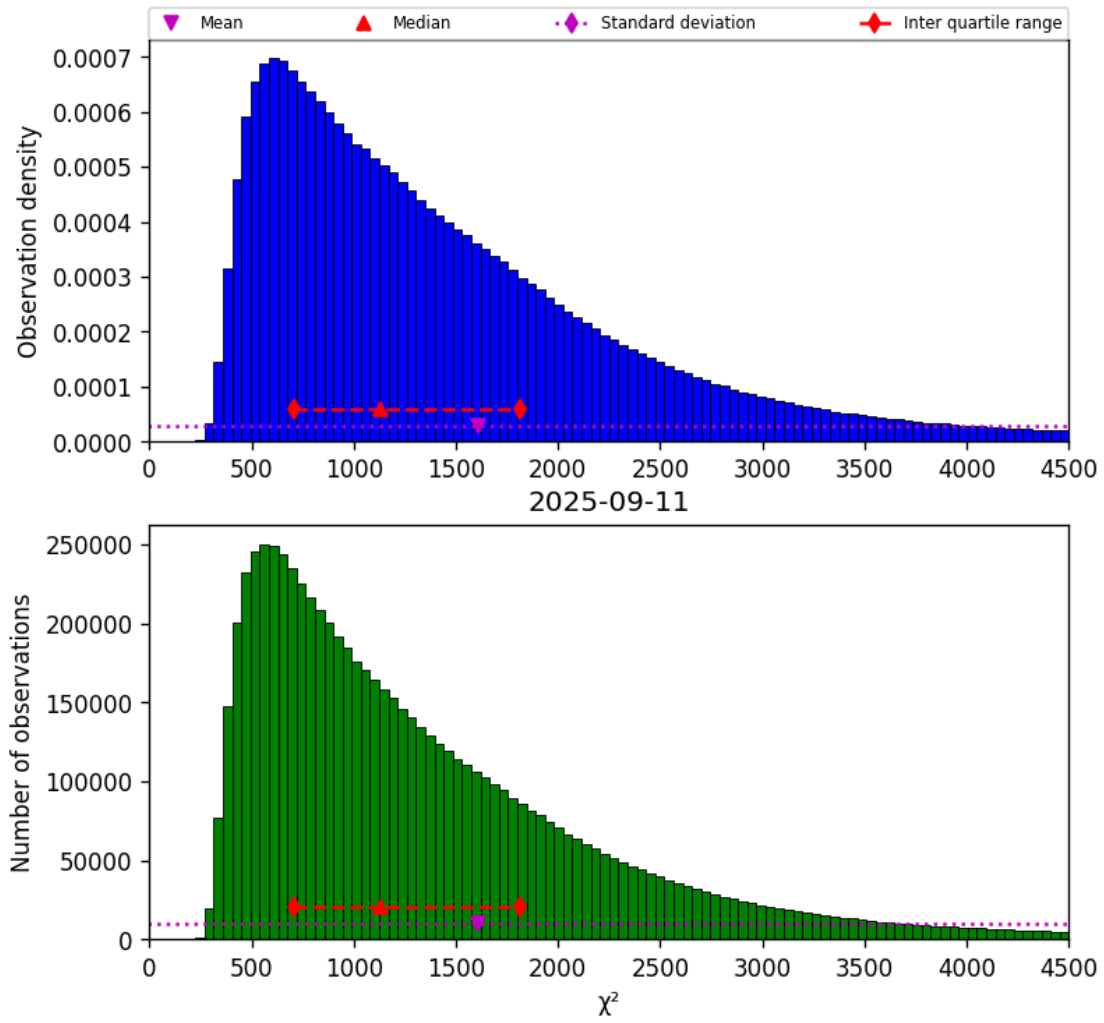
Figure 22: Histogram of “ \chi^2 ” for 2025-09-10 to 2025-09-12
