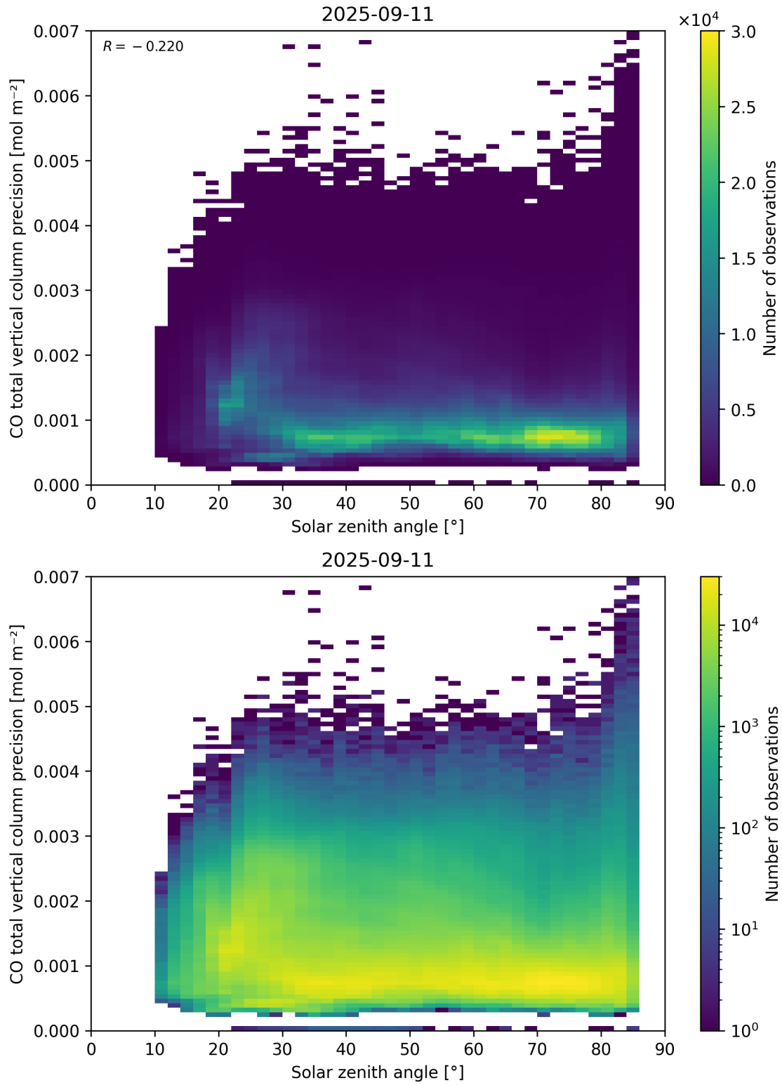
Figure 63: Scatter density plot of “Solar zenith angle” against “CO total vertical column precision” for 2025-09-10 to 2025-09-12.
