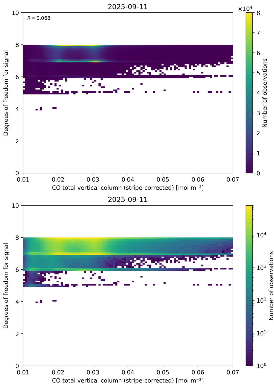
Figure 38: Scatter density plot of “CO total vertical column (stripe-corrected)” against “Degrees of freedom for signal” for 2025-09-10 to 2025-09-12.
