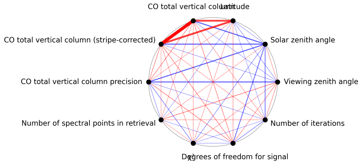
Figure 1: Map of correlation graph for 2025-09-10 to 2025-09-12.
