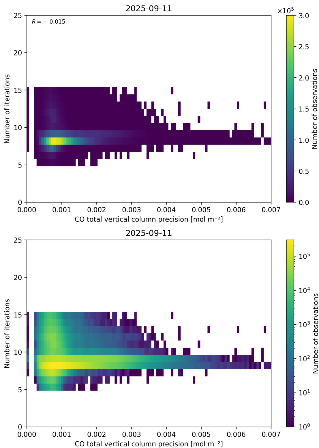
Figure 46: Scatter density plot of “CO total vertical column precision” against “Number of iterations” for 2025-09-10 to 2025-09-12.
