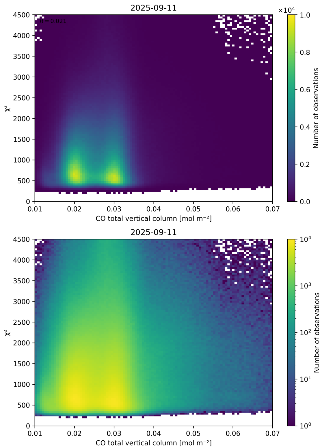
Figure 35: Scatter density plot of “CO total vertical column” against “ \chi^2 ” for 2025-09-10 to 2025-09-12.
