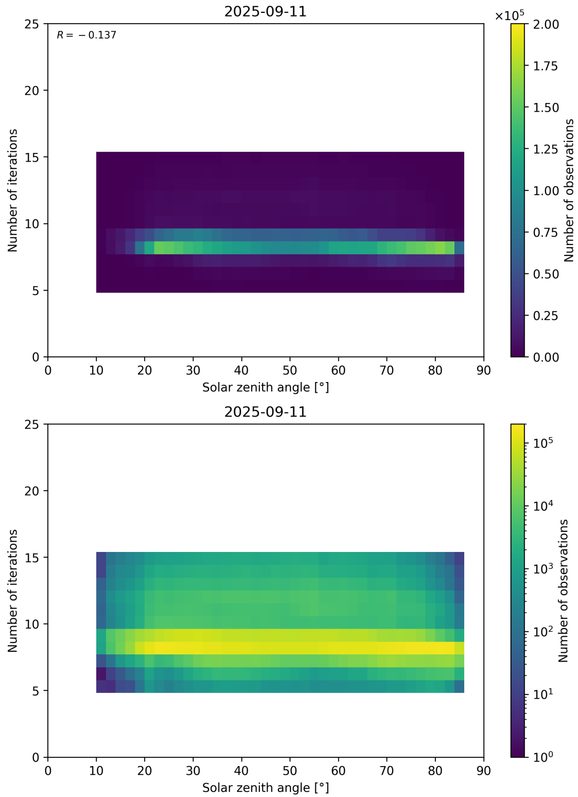
Figure 67: Scatter density plot of “Solar zenith angle” against “Number of iterations” for 2025-09-10 to 2025-09-12.
