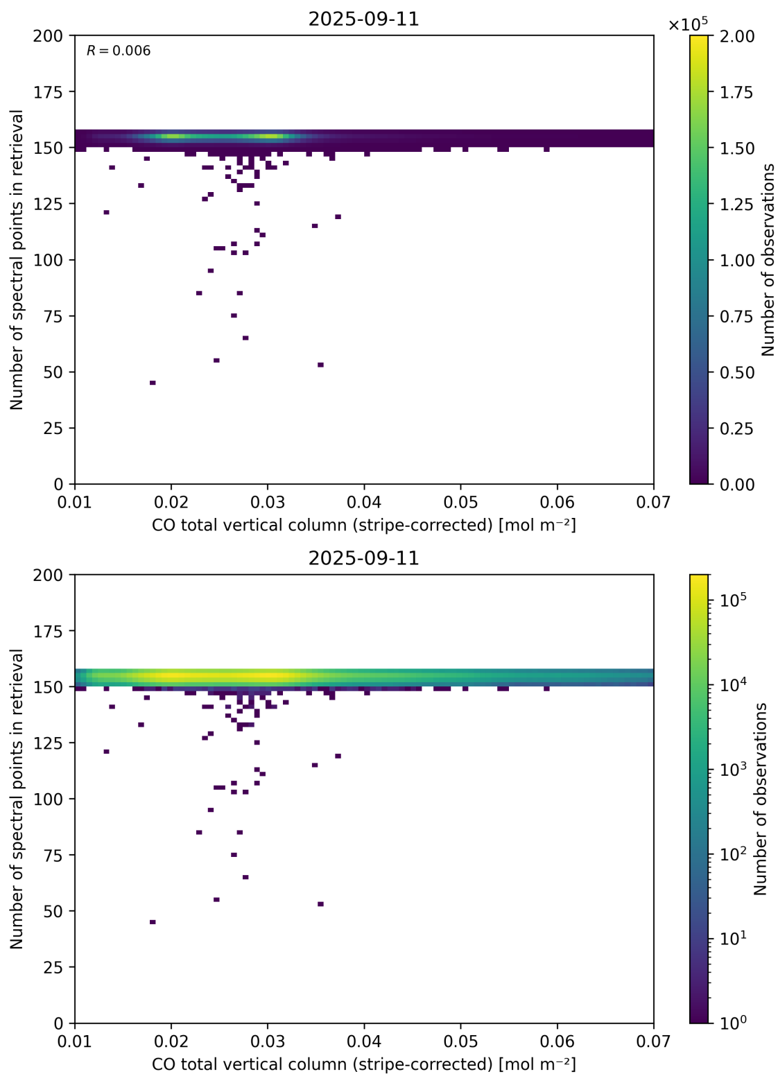
Figure 40: Scatter density plot of “CO total vertical column (stripe-corrected)” against “Number of spectral points in retrieval” for 2025-09-10 to 2025-09-12.
