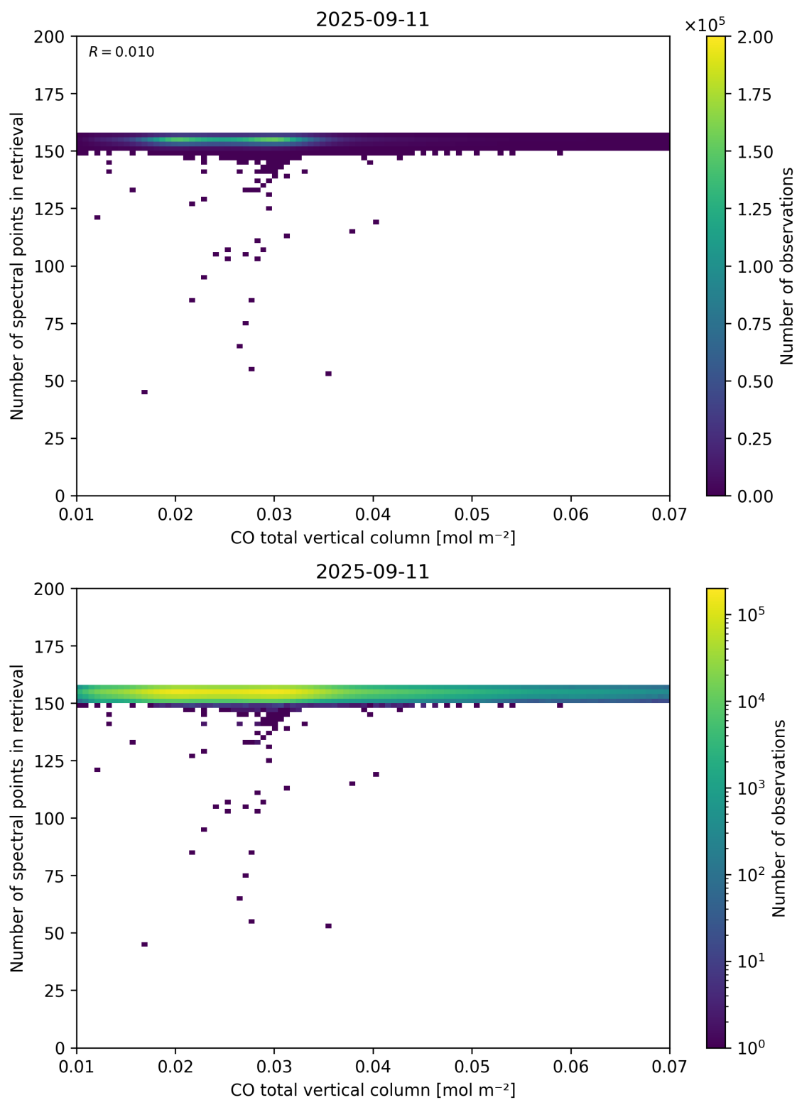
Figure 43: Scatter density plot of “CO total vertical column” against “Number of spectral points in retrieval” for 2025-09-10 to 2025-09-12.
