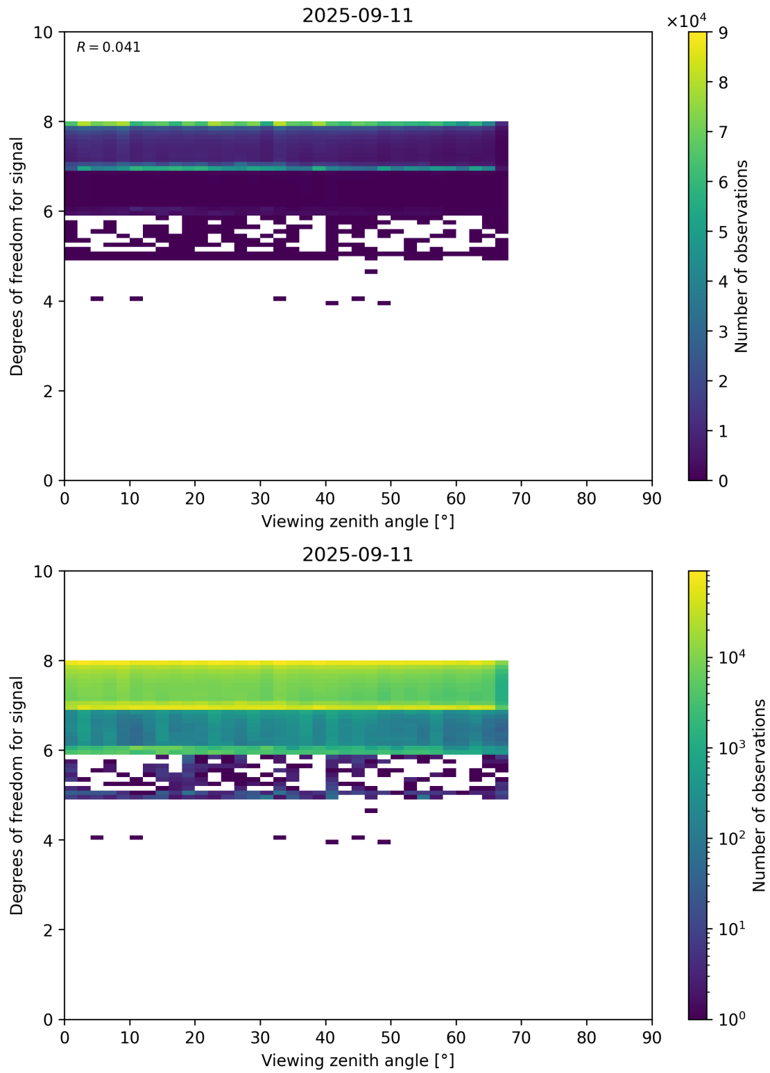
Figure 73: Scatter density plot of “Viewing zenith angle” against “Degrees of freedom for signal” for 2025-09-10 to 2025-09-12.
