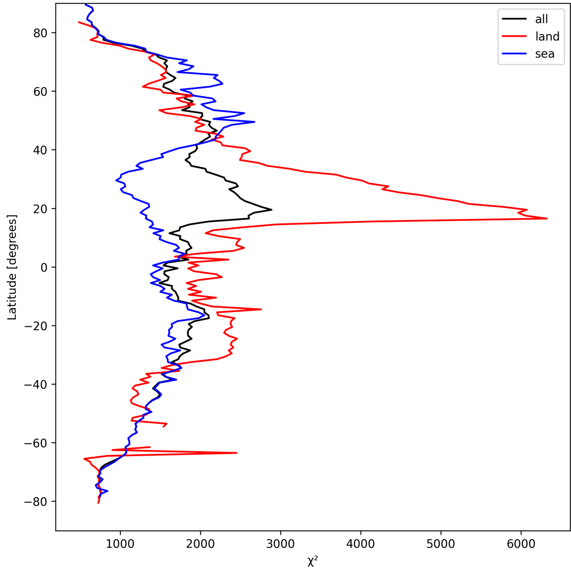
Figure 14: Zonal average of “ \chi^2 ” for 2025-09-10 to 2025-09-12.
