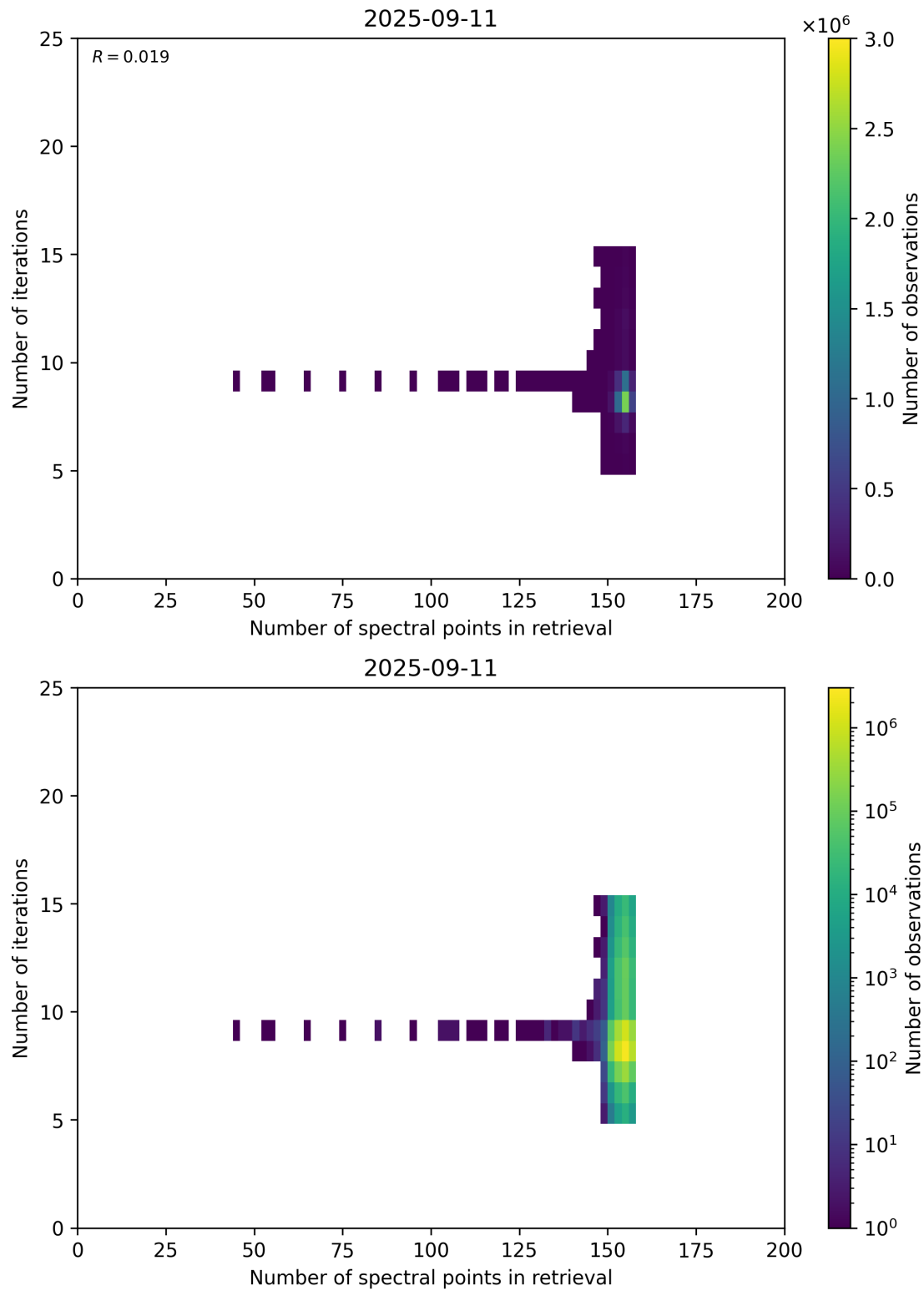
Figure 60: Scatter density plot of “Number of spectral points in retrieval” against “Number of iterations” for 2025-09-10 to 2025-09-12.
