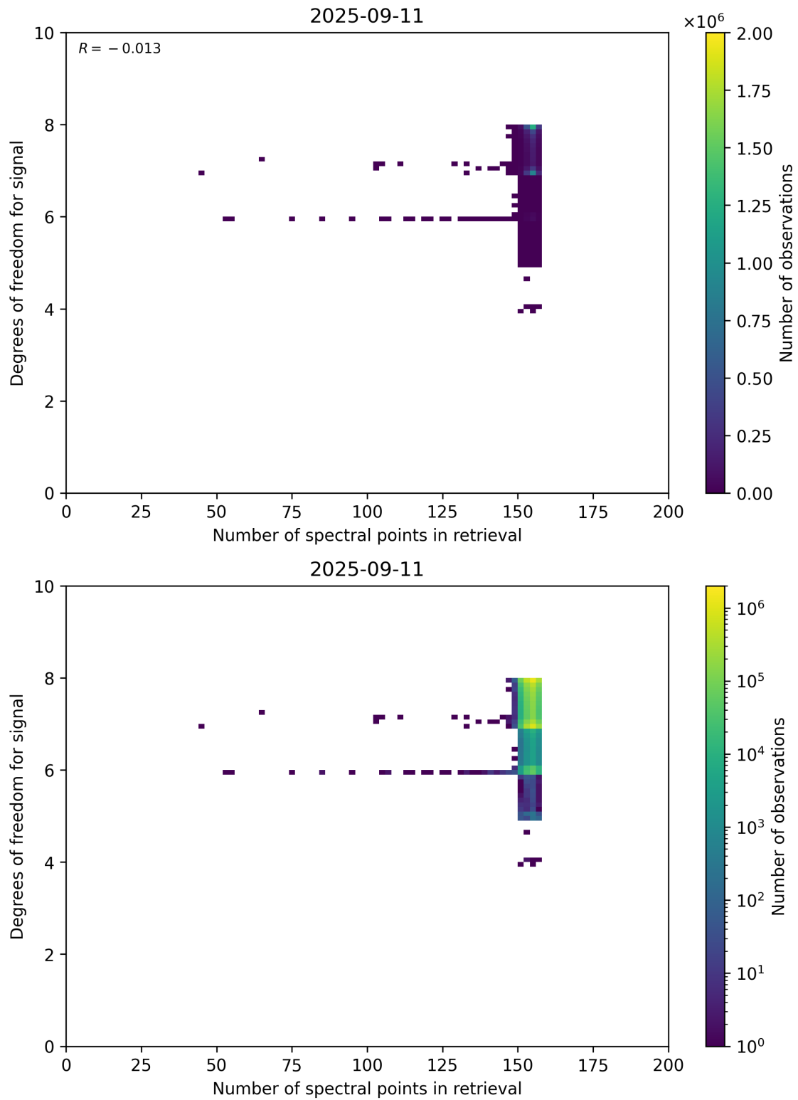
Figure 59: Scatter density plot of “Number of spectral points in retrieval” against “Degrees of freedom for signal” for 2025-09-10 to 2025-09-12.
