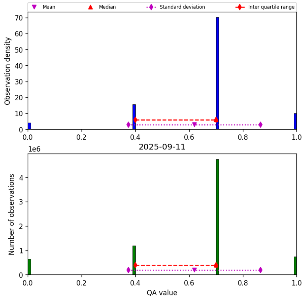
Figure 17: Histogram of “QA value” for 2025-09-10 to 2025-09-12
