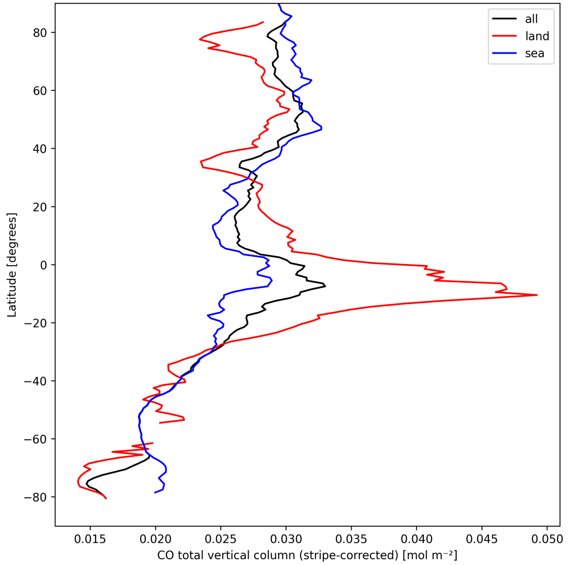
Figure 11: Zonal average of “CO total vertical column (stripe-corrected)” for 2025-09-10 to 2025-09-12.
