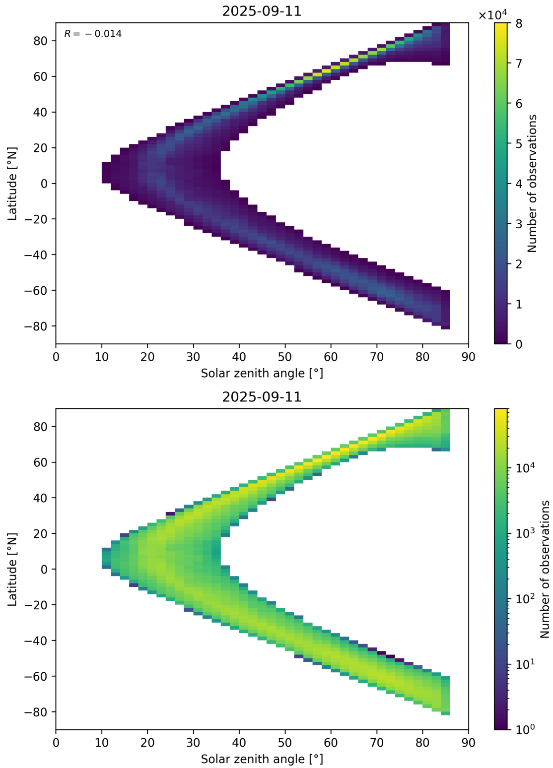
Figure 66: Scatter density plot of “Solar zenith angle” against “Latitude” for 2025-09-10 to 2025-09-12.
