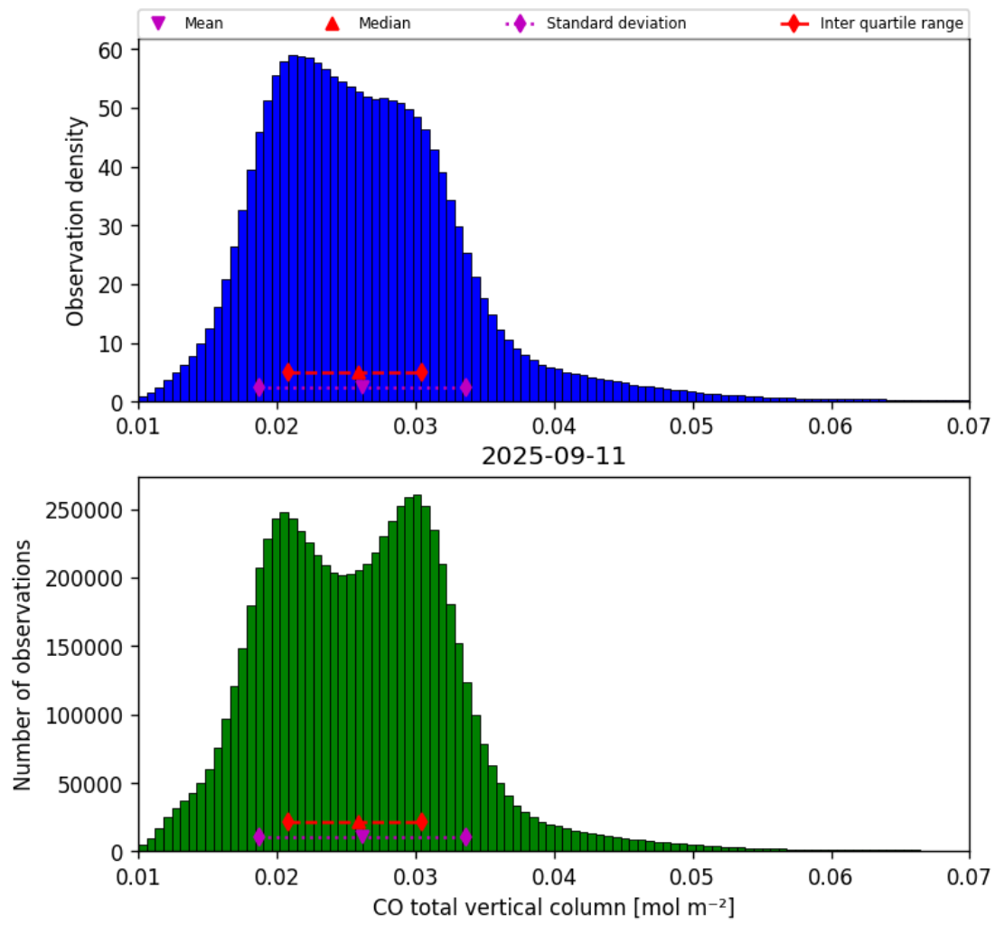
Figure 18: Histogram of “CO total vertical column” for 2025-09-10 to 2025-09-12
