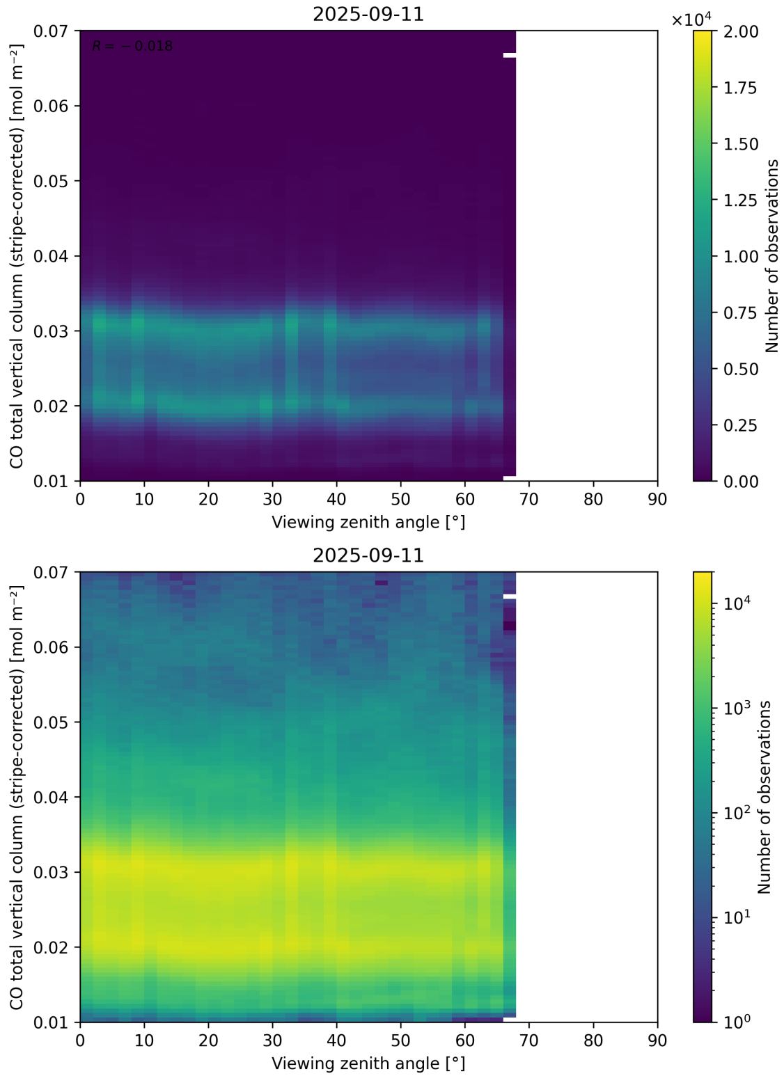
Figure 70: Scatter density plot of “Viewing zenith angle” against “CO total vertical column (stripe-corrected)” for 2025-09-10 to 2025-09-12.
