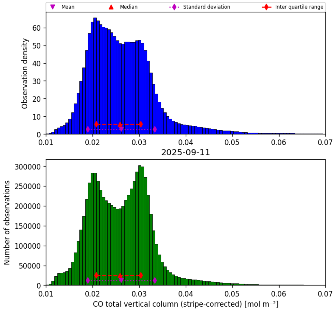
Figure 19: Histogram of “CO total vertical column (stripe-corrected)” for 2025-09-10 to 2025-09-12
