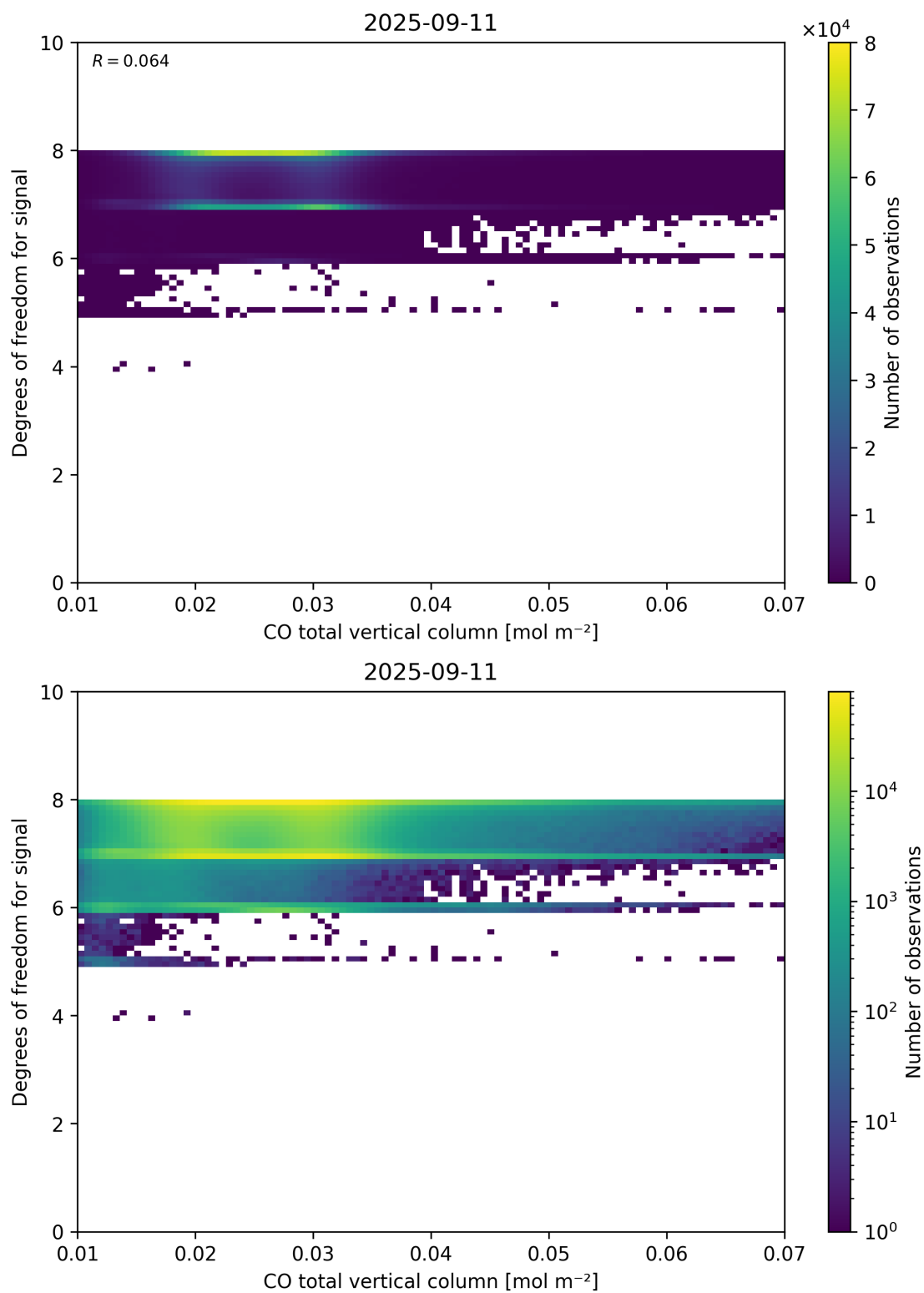
Figure 41: Scatter density plot of “CO total vertical column” against “Degrees of freedom for signal” for 2025-09-10 to 2025-09-12.
