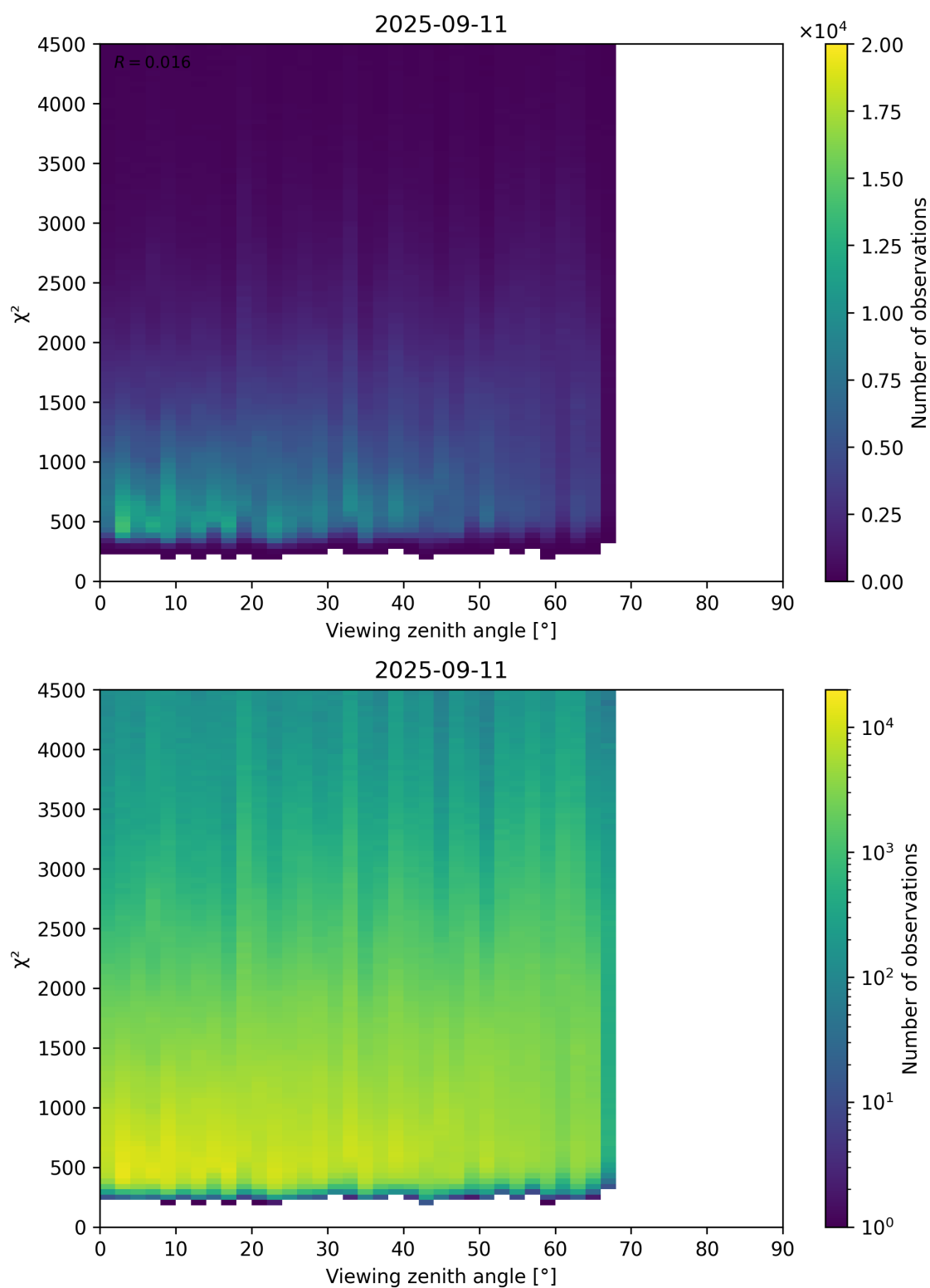
Figure 72: Scatter density plot of “Viewing zenith angle” against “ \chi^2 ” for 2025-09-10 to 2025-09-12.
