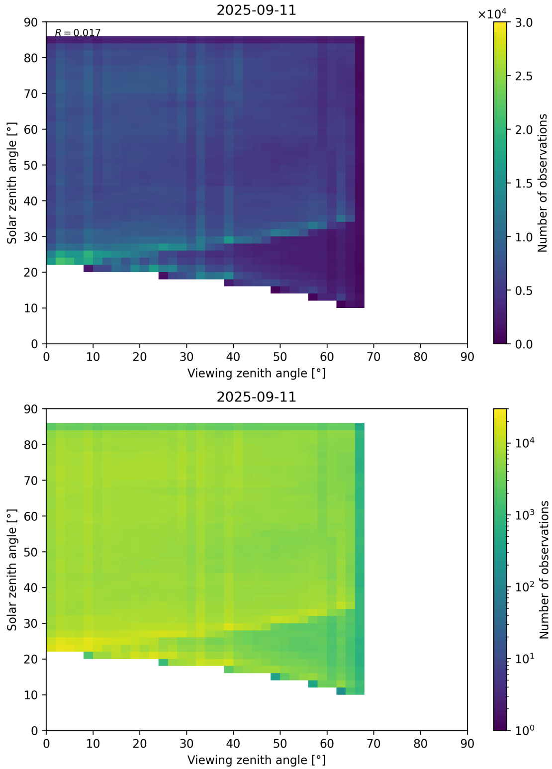
Figure 77: Scatter density plot of “Viewing zenith angle” against “Solar zenith angle” for 2025-09-10 to 2025-09-12.
