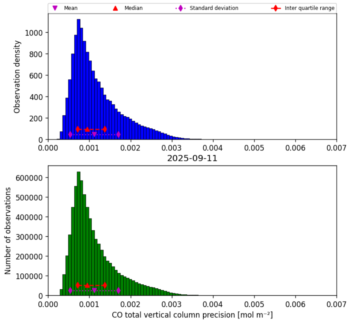
Figure 20: Histogram of “CO total vertical column precision” for 2025-09-10 to 2025-09-12
