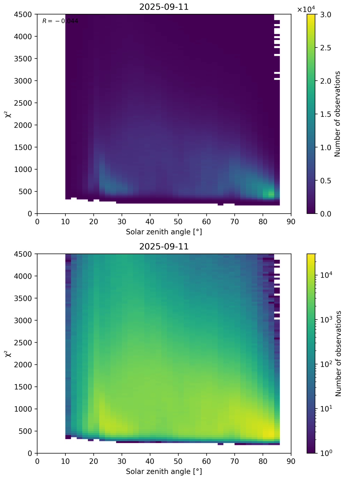
Figure 64: Scatter density plot of “Solar zenith angle” against “ \chi^2 ” for 2025-09-10 to 2025-09-12.
