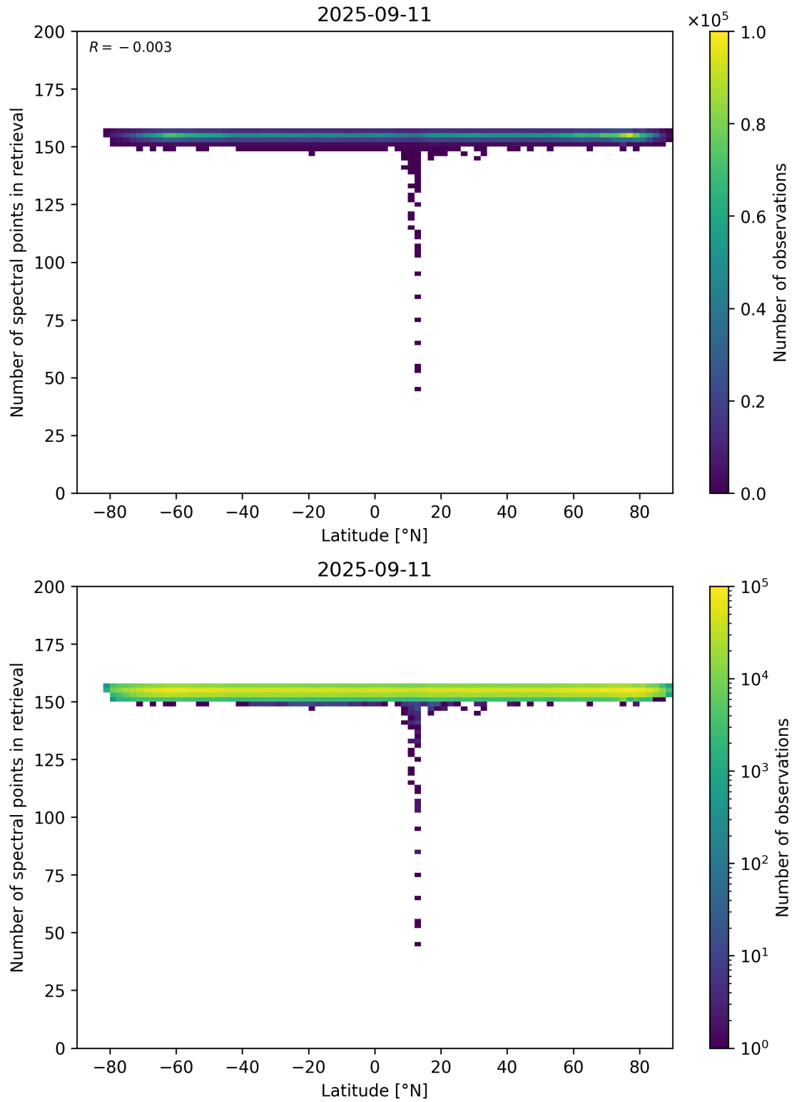
Figure 57: Scatter density plot of “Latitude” against “Number of spectral points in retrieval” for 2025-09-10 to 2025-09-12.
