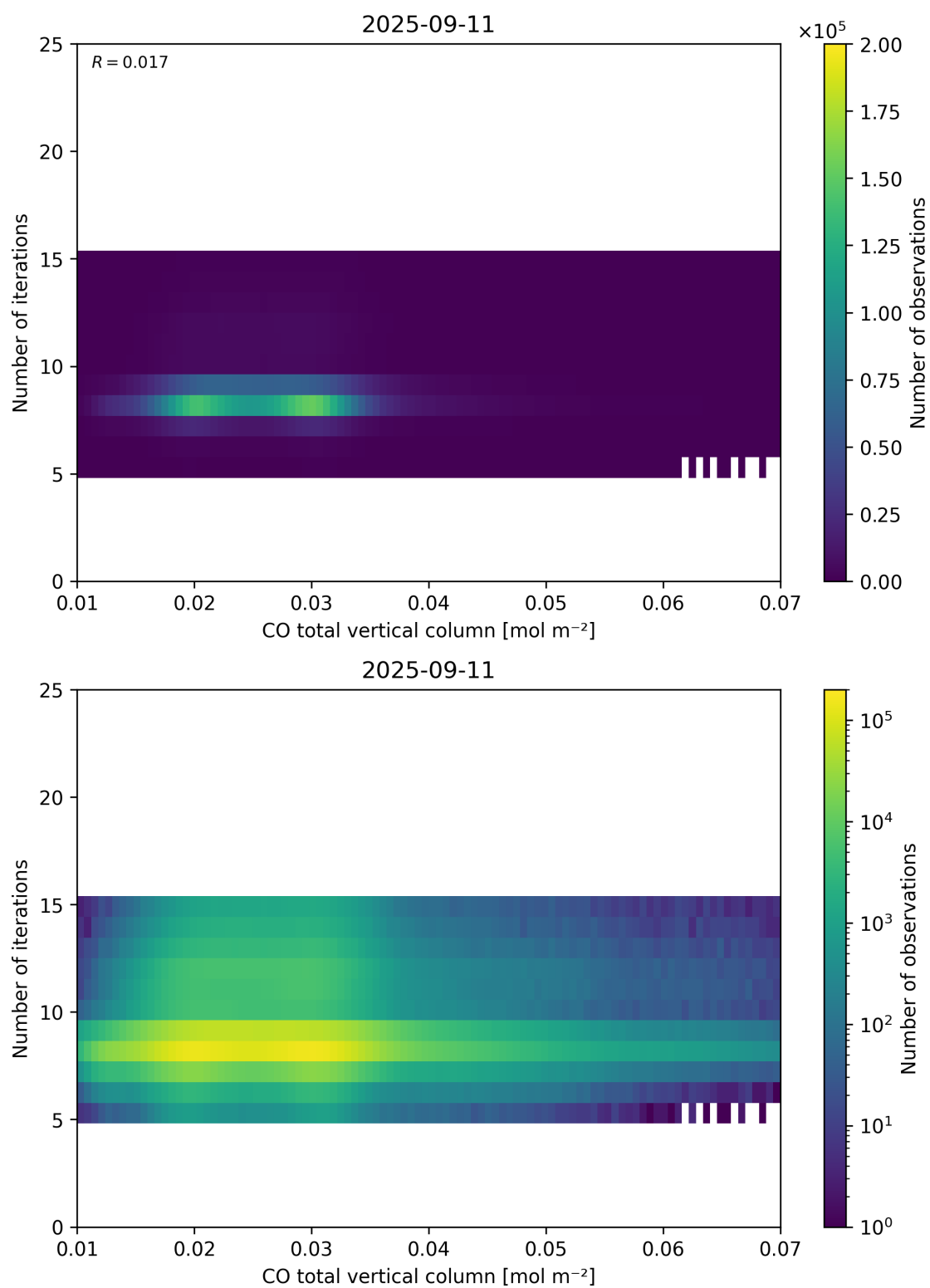
Figure 42: Scatter density plot of “CO total vertical column” against “Number of iterations” for 2025-09-10 to 2025-09-12.
