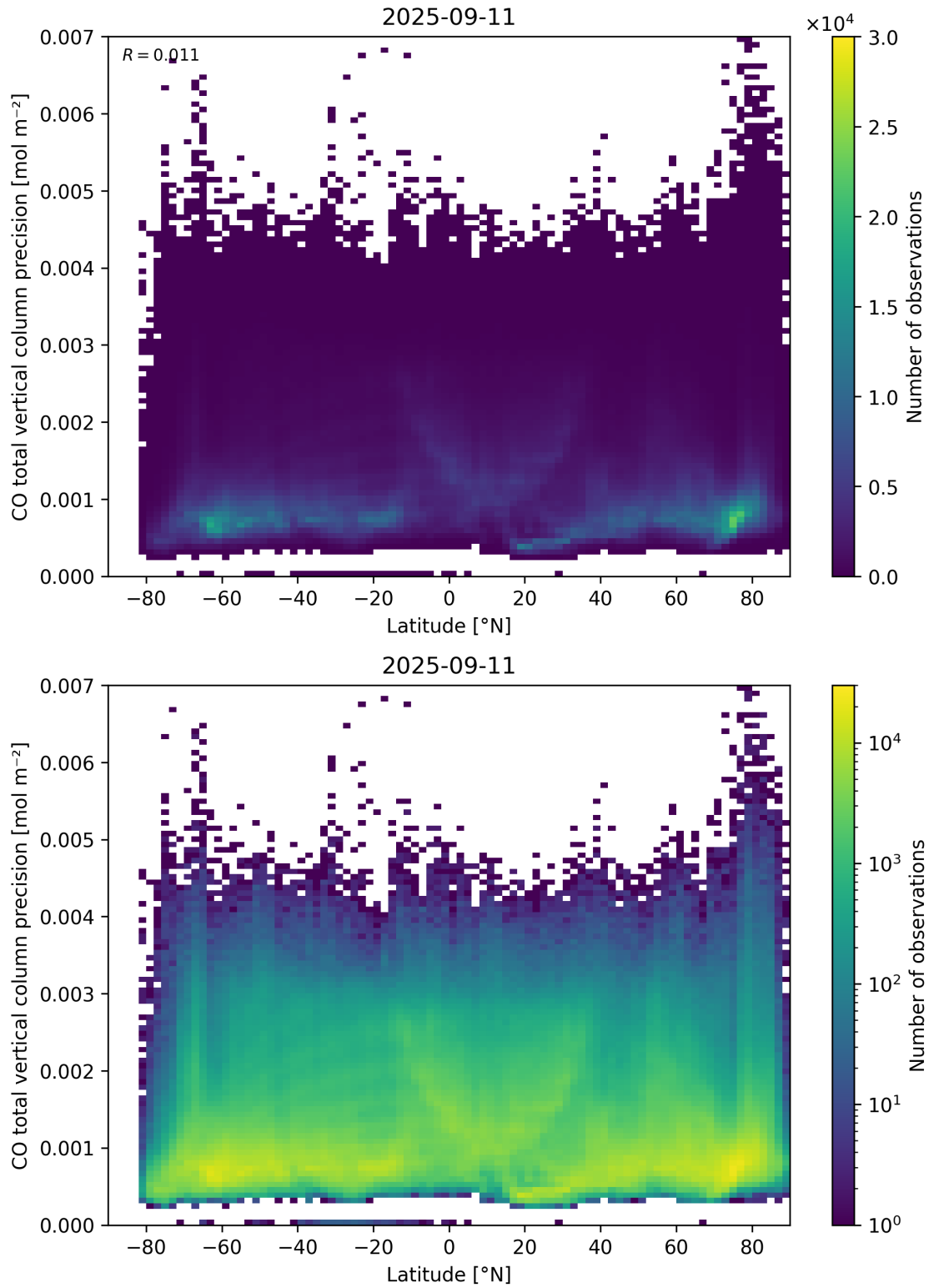
Figure 53: Scatter density plot of “Latitude” against “CO total vertical column precision” for 2025-09-10 to 2025-09-12.
