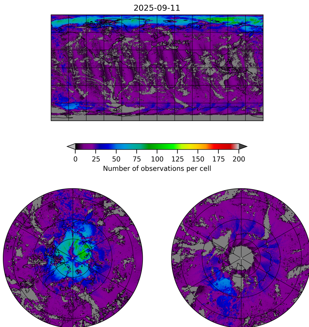
Figure 8: Map of the number of observations for 2025-09-10 to 2025-09-12
