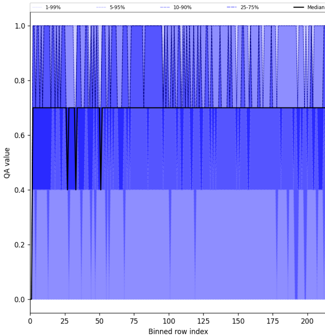
Figure 25: Along track statistics of “QA value” for 2025-09-10 to 2025-09-12
