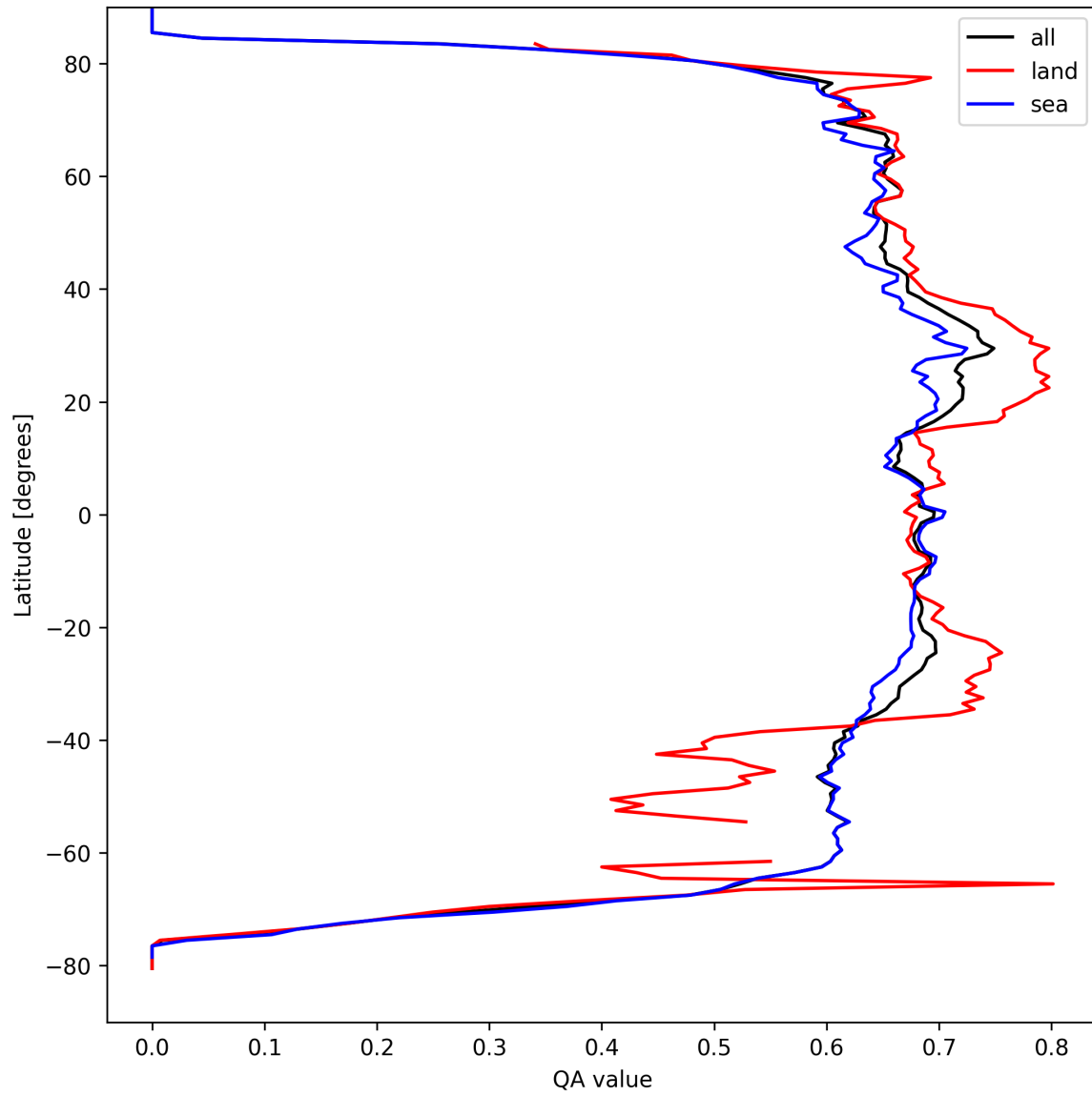
Figure 9: Zonal average of “QA value” for 2025-09-10 to 2025-09-12.
