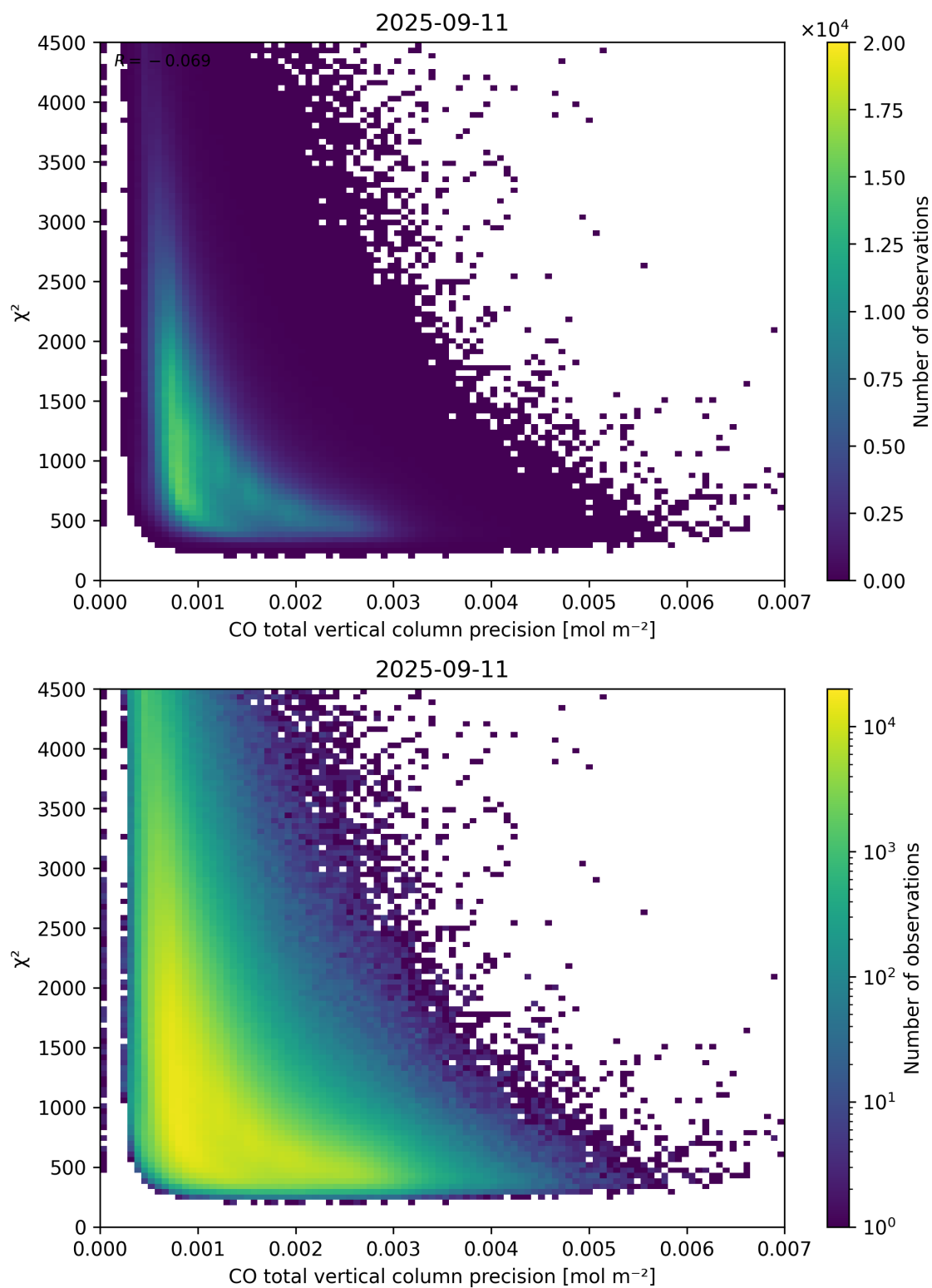
Figure 44: Scatter density plot of “CO total vertical column precision” against “ \chi^2 ” for 2025-09-10 to 2025-09-12.
