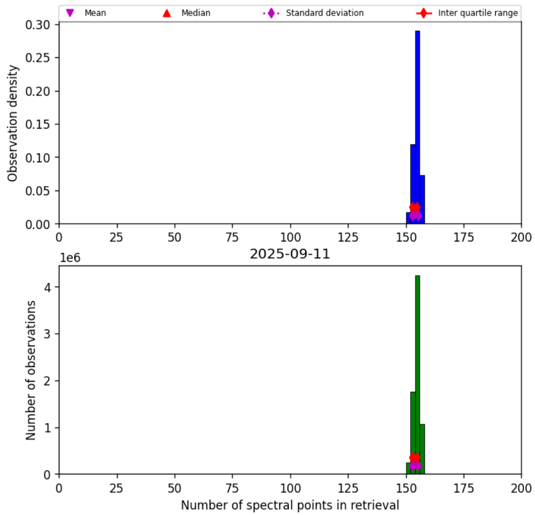
Figure 21: Histogram of “Number of spectral points in retrieval” for 2025-09-10 to 2025-09-12
