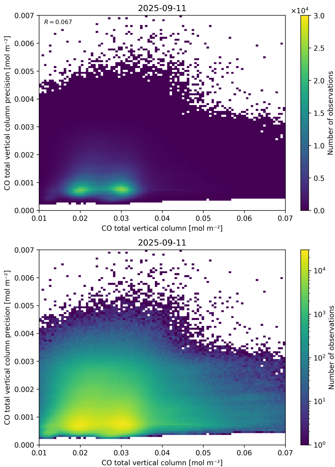
Figure 34: Scatter density plot of “CO total vertical column” against “CO total vertical column precision” for 2025-09-10 to 2025-09-12.
