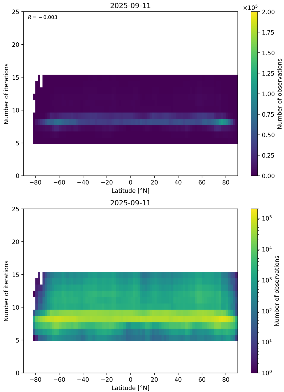
Figure 56: Scatter density plot of “Latitude” against “Number of iterations” for 2025-09-10 to 2025-09-12.
