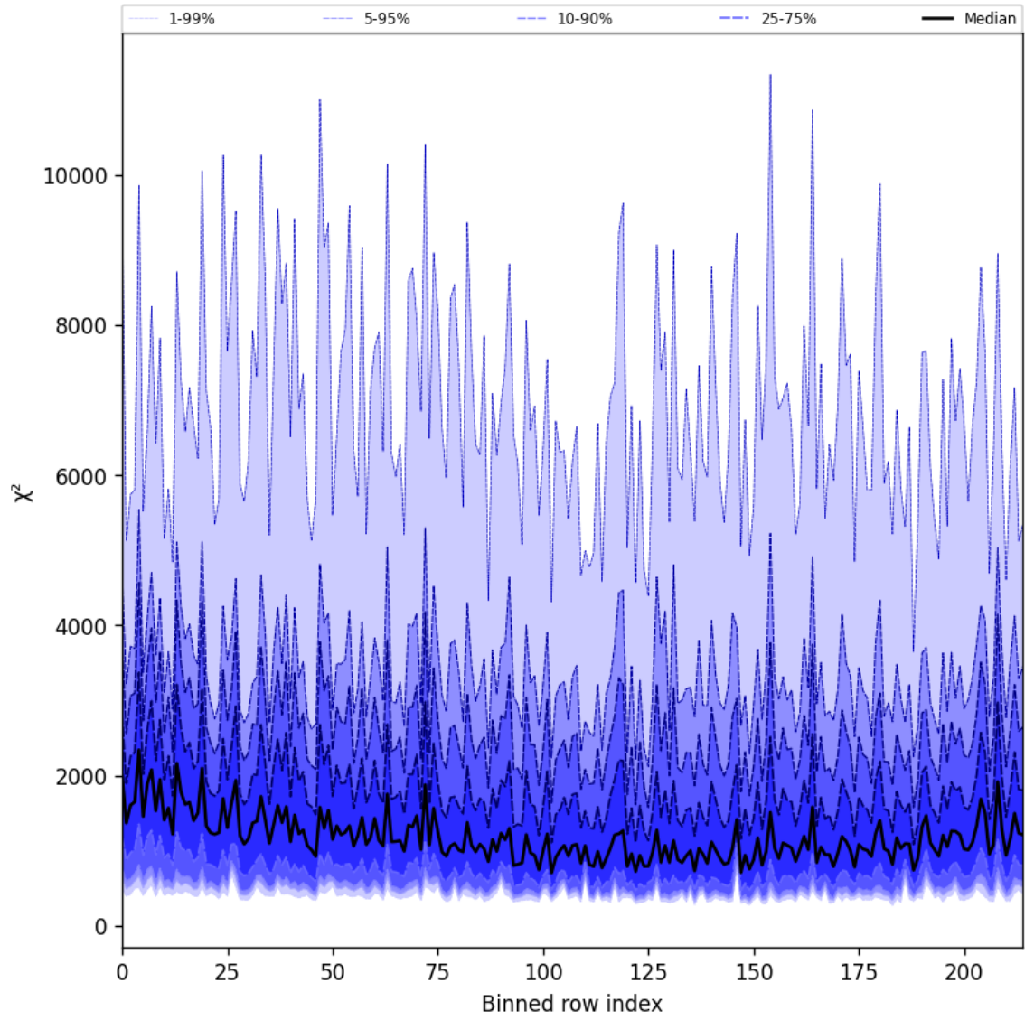
Figure 30: Along track statistics of “ \chi^2 ” for 2025-09-10 to 2025-09-12
