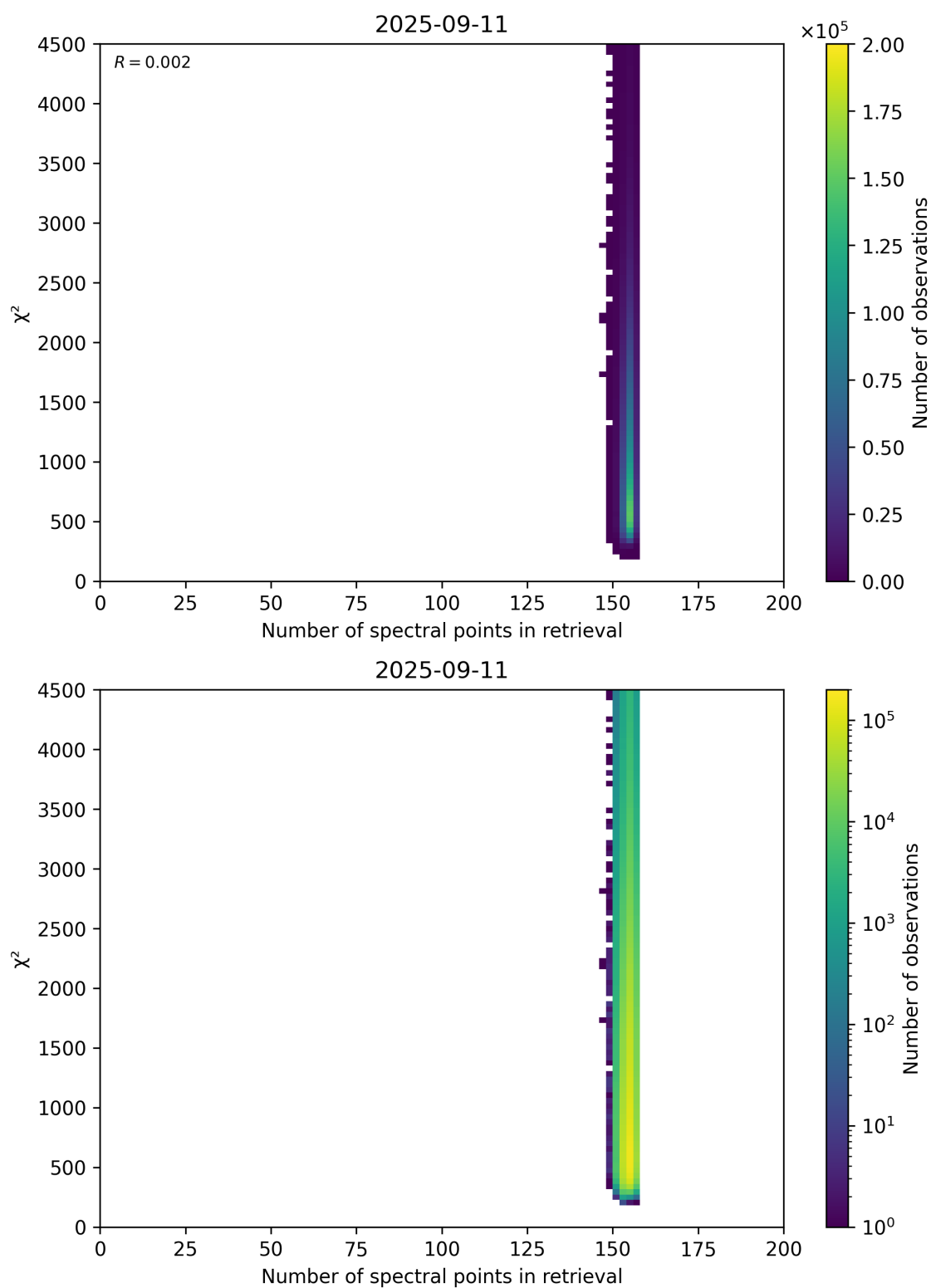
Figure 58: Scatter density plot of “Number of spectral points in retrieval” against “ \chi^2 ” for 2025-09-10 to 2025-09-12.
