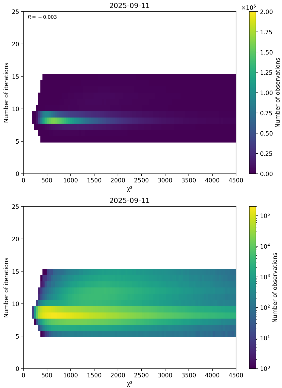
Figure 49: Scatter density plot of “ \chi^2 ” against “Number of iterations” for 2025-09-10 to 2025-09-12.
