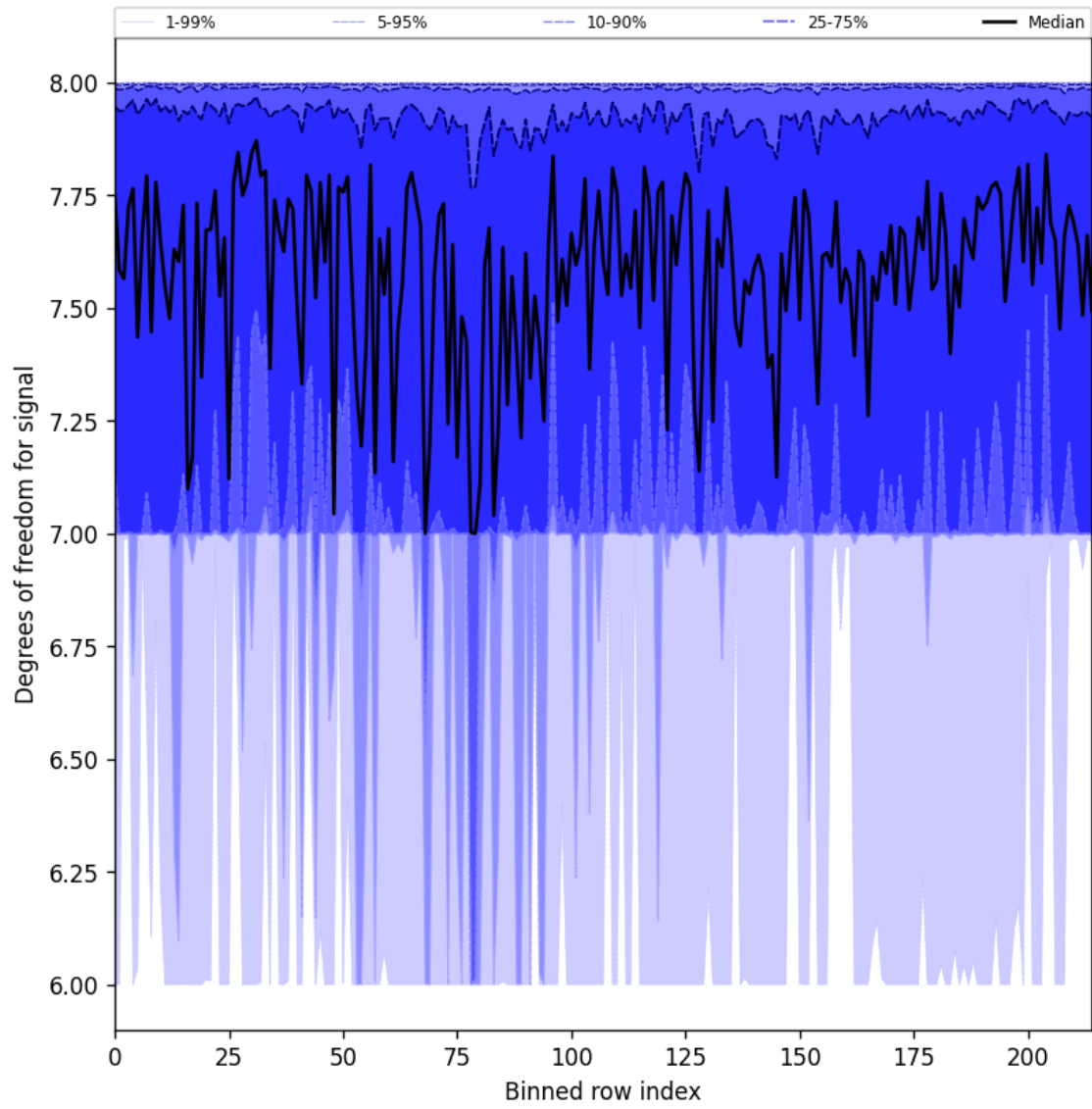
Figure 31: Along track statistics of “Degrees of freedom for signal” for 2025-09-10 to 2025-09-12
