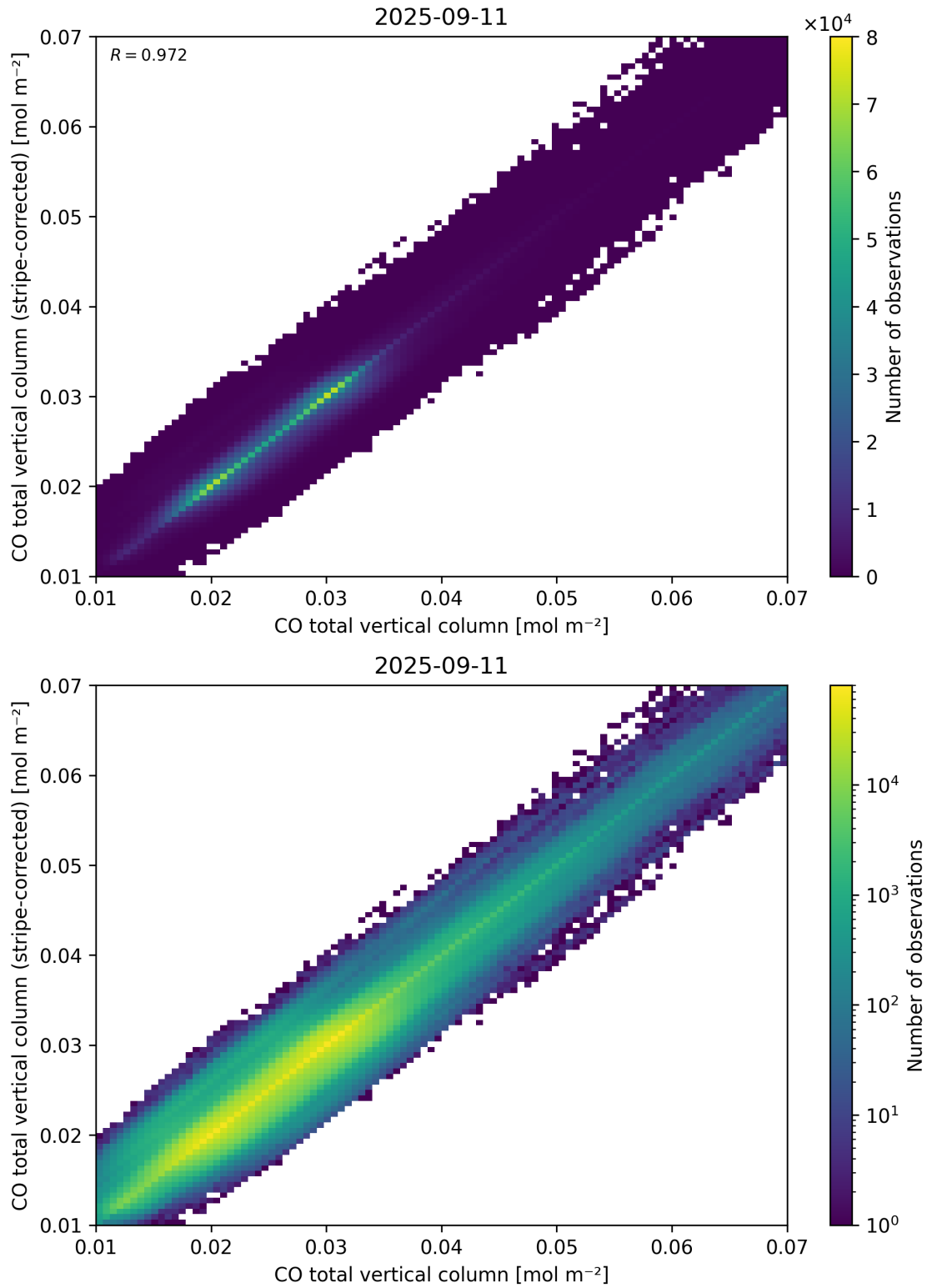
Figure 33: Scatter density plot of “CO total vertical column” against “CO total vertical column (stripe-corrected)” for 2025-09-10 to 2025-09-12.
