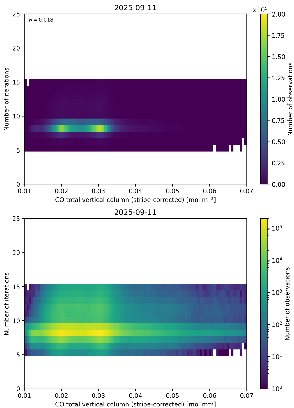
Figure 39: Scatter density plot of “CO total vertical column (stripe-corrected)” against “Number of iterations” for 2025-09-10 to 2025-09-12.
