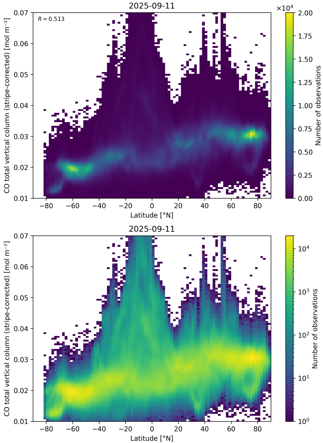
Figure 52: Scatter density plot of “Latitude” against “CO total vertical column (stripe-corrected)” for 2025-09-10 to 2025-09-12.
