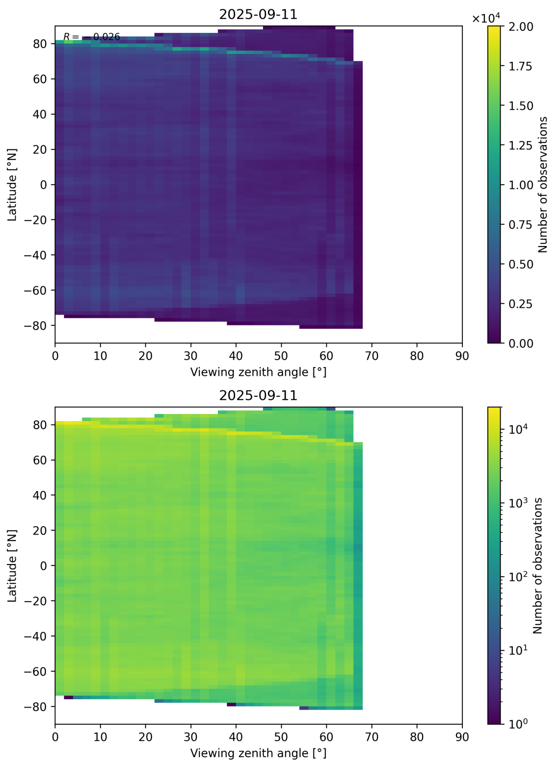
Figure 74: Scatter density plot of “Viewing zenith angle” against “Latitude” for 2025-09-10 to 2025-09-12.
