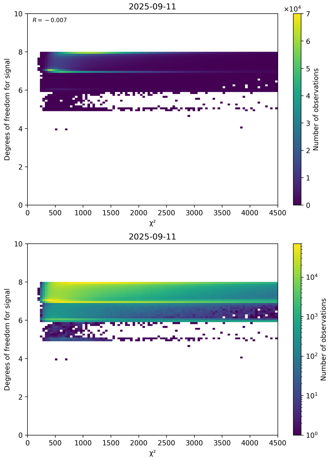
Figure 48: Scatter density plot of “ \chi^2 ” against “Degrees of freedom for signal” for 2025-09-10 to 2025-09-12.
