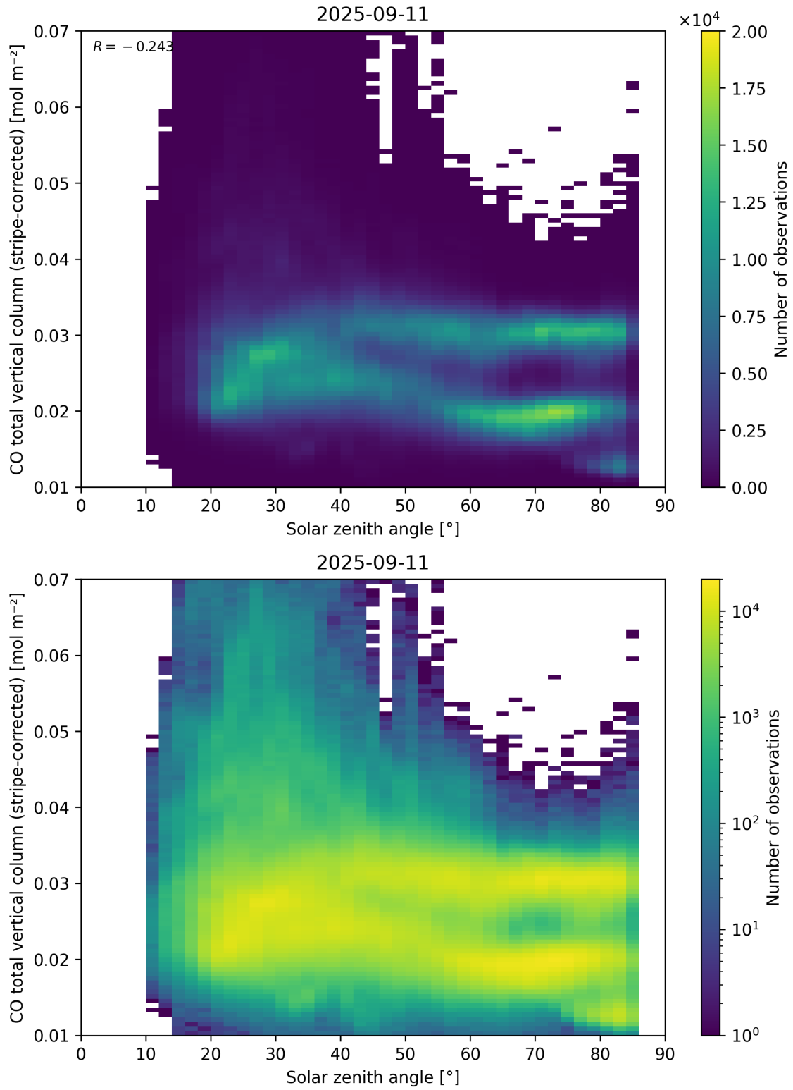
Figure 62: Scatter density plot of “Solar zenith angle” against “CO total vertical column (stripe-corrected)” for 2025-09-10 to 2025-09-12.
