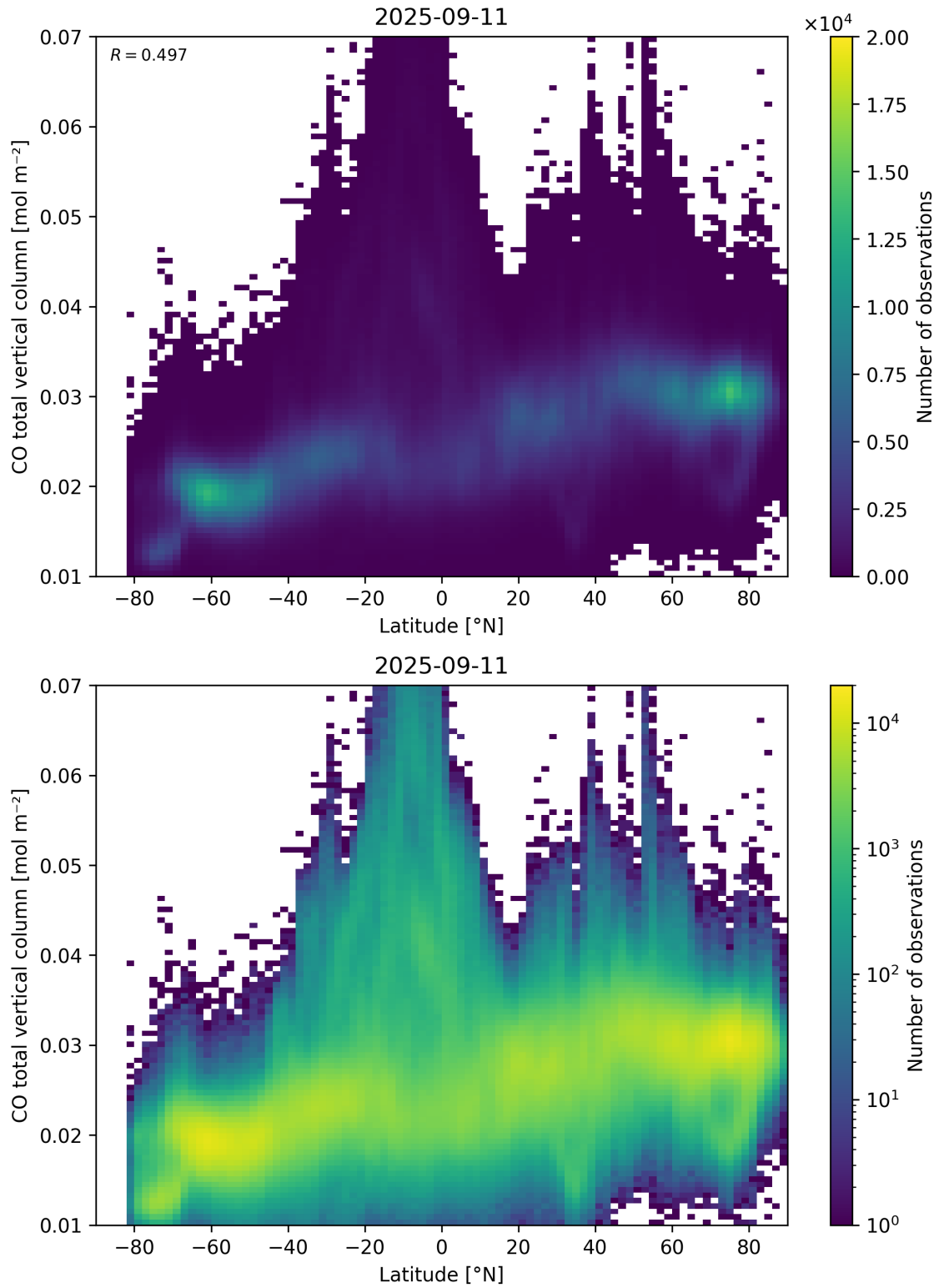
Figure 51: Scatter density plot of “Latitude” against “CO total vertical column” for 2025-09-10 to 2025-09-12.
