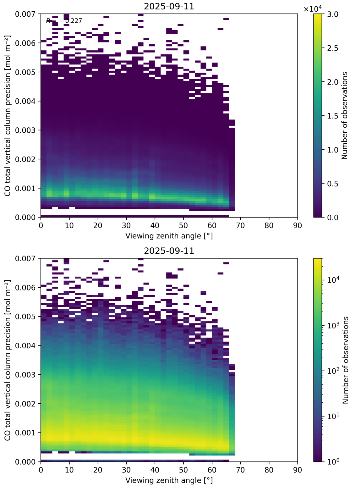
Figure 71: Scatter density plot of “Viewing zenith angle” against “CO total vertical column precision” for 2025-09-10 to 2025-09-12.
