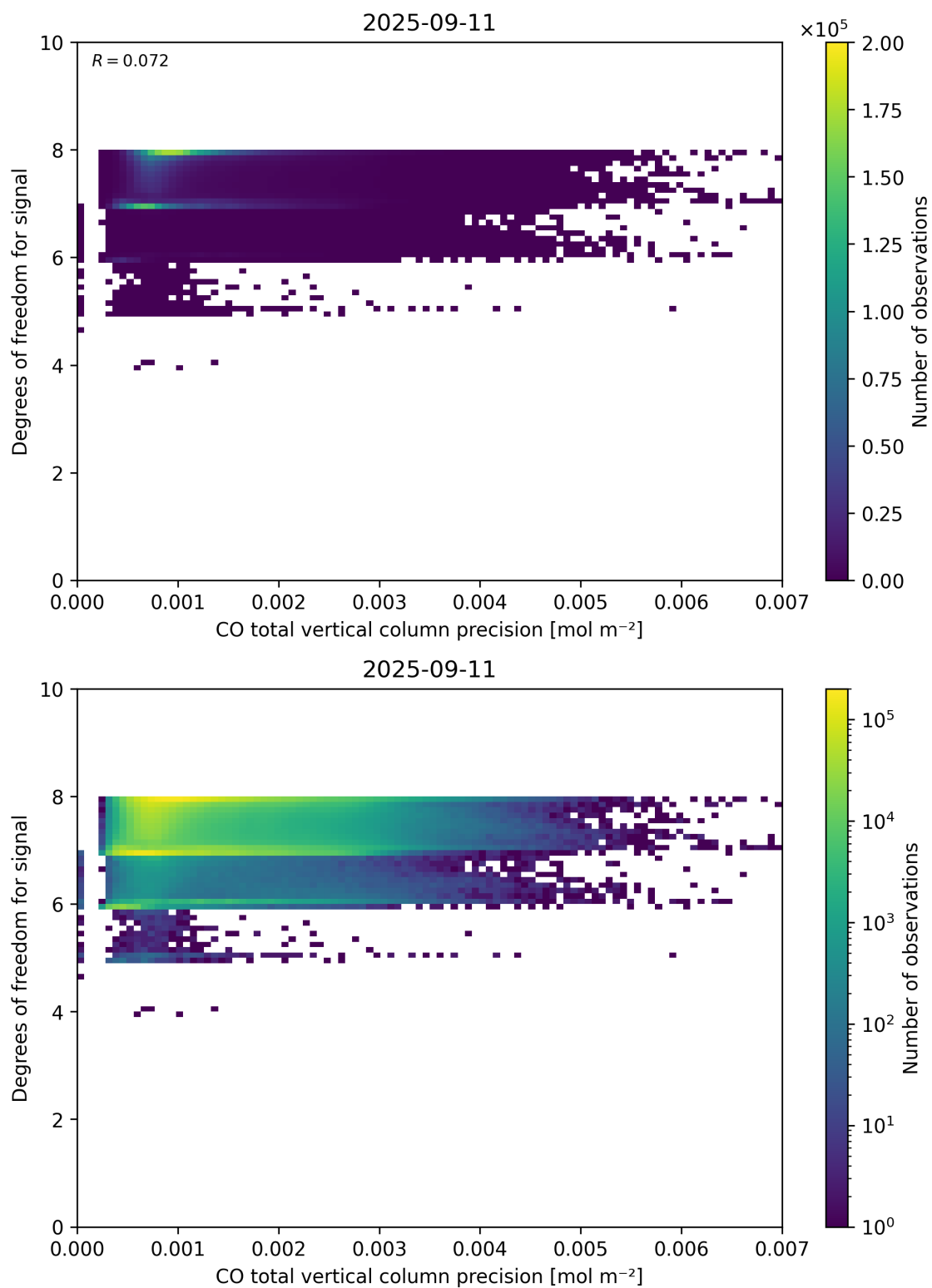
Figure 45: Scatter density plot of “CO total vertical column precision” against “Degrees of freedom for signal” for 2025-09-10 to 2025-09-12.
