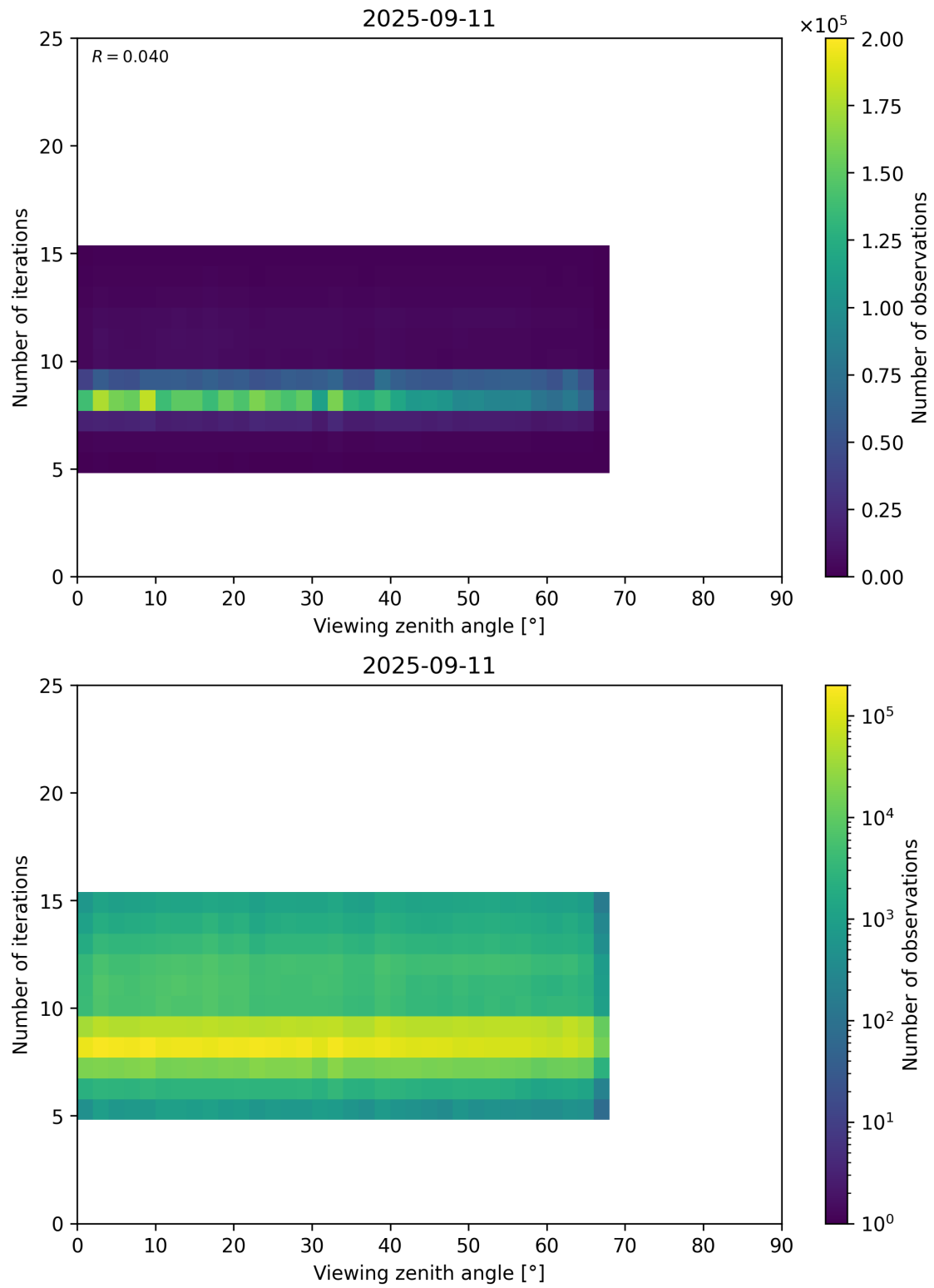
Figure 75: Scatter density plot of “Viewing zenith angle” against “Number of iterations” for 2025-09-10 to 2025-09-12.
