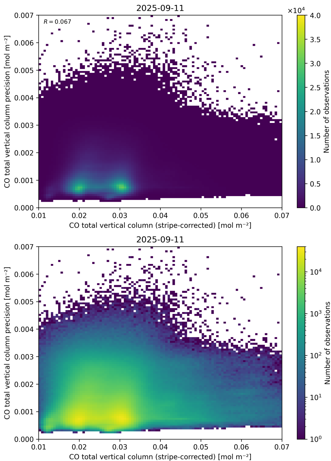
Figure 36: Scatter density plot of “CO total vertical column (stripe-corrected)” against “CO total vertical column precision” for 2025-09-10 to 2025-09-12.
