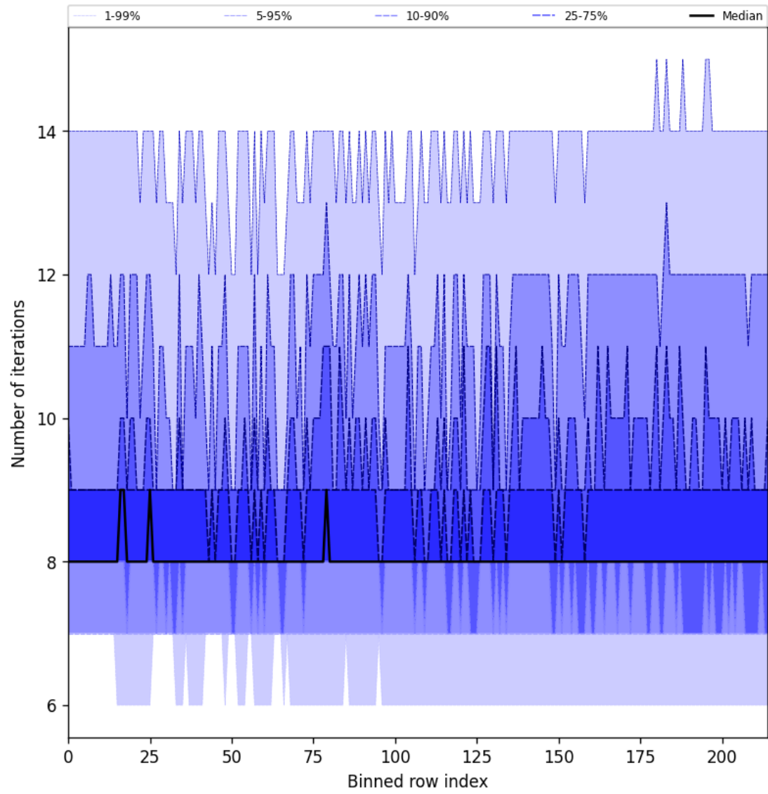
Figure 32: Along track statistics of “Number of iterations” for 2025-09-10 to 2025-09-12
