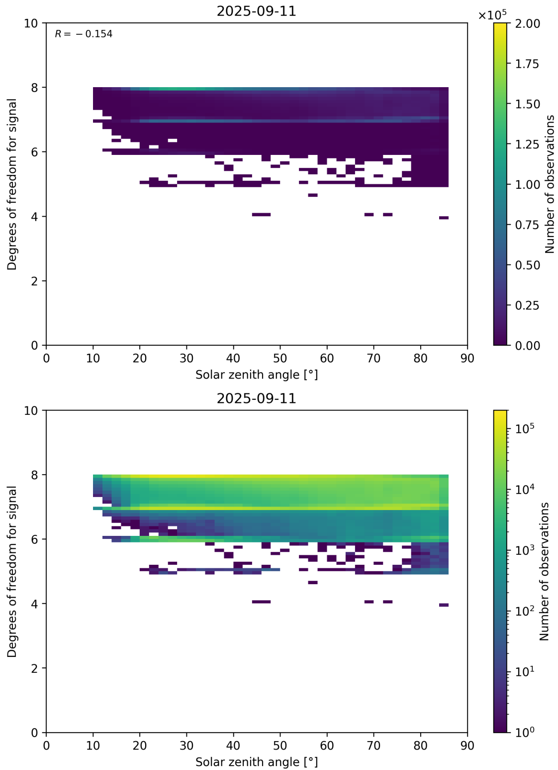
Figure 65: Scatter density plot of “Solar zenith angle” against “Degrees of freedom for signal” for 2025-09-10 to 2025-09-12.
