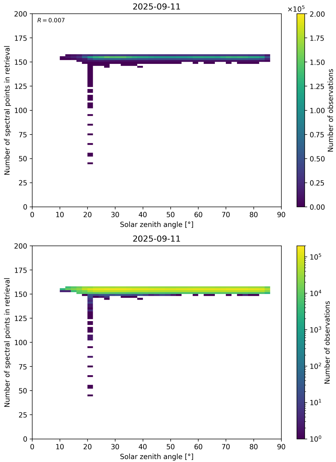
Figure 68: Scatter density plot of “Solar zenith angle” against “Number of spectral points in retrieval” for 2025-09-10 to 2025-09-12.
