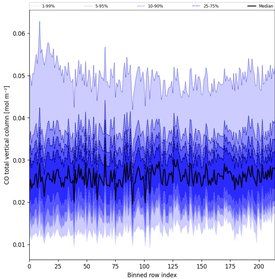
Figure 26: Along track statistics of "CO total vertical column" for 2025-09-10 to 2025-09-12
