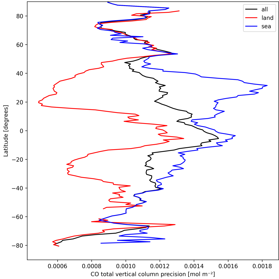
Figure 12: Zonal average of "CO total vertical column precision" for 2025-09-10 to 2025-09-12.
