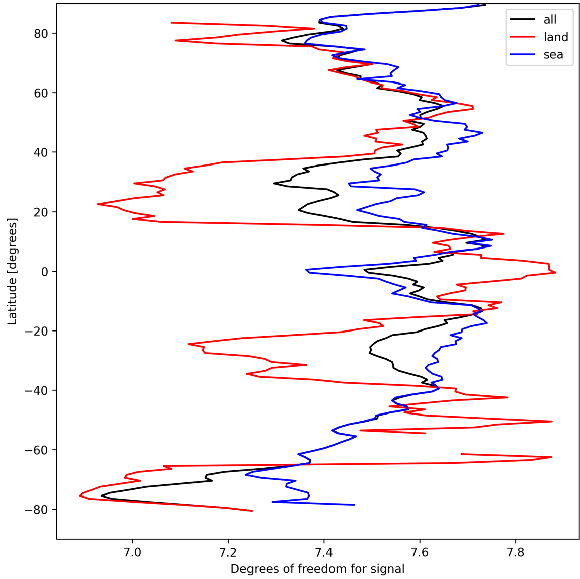
Figure 15: Zonal average of “Degrees of freedom for signal” for 2025-09-10 to 2025-09-12.
