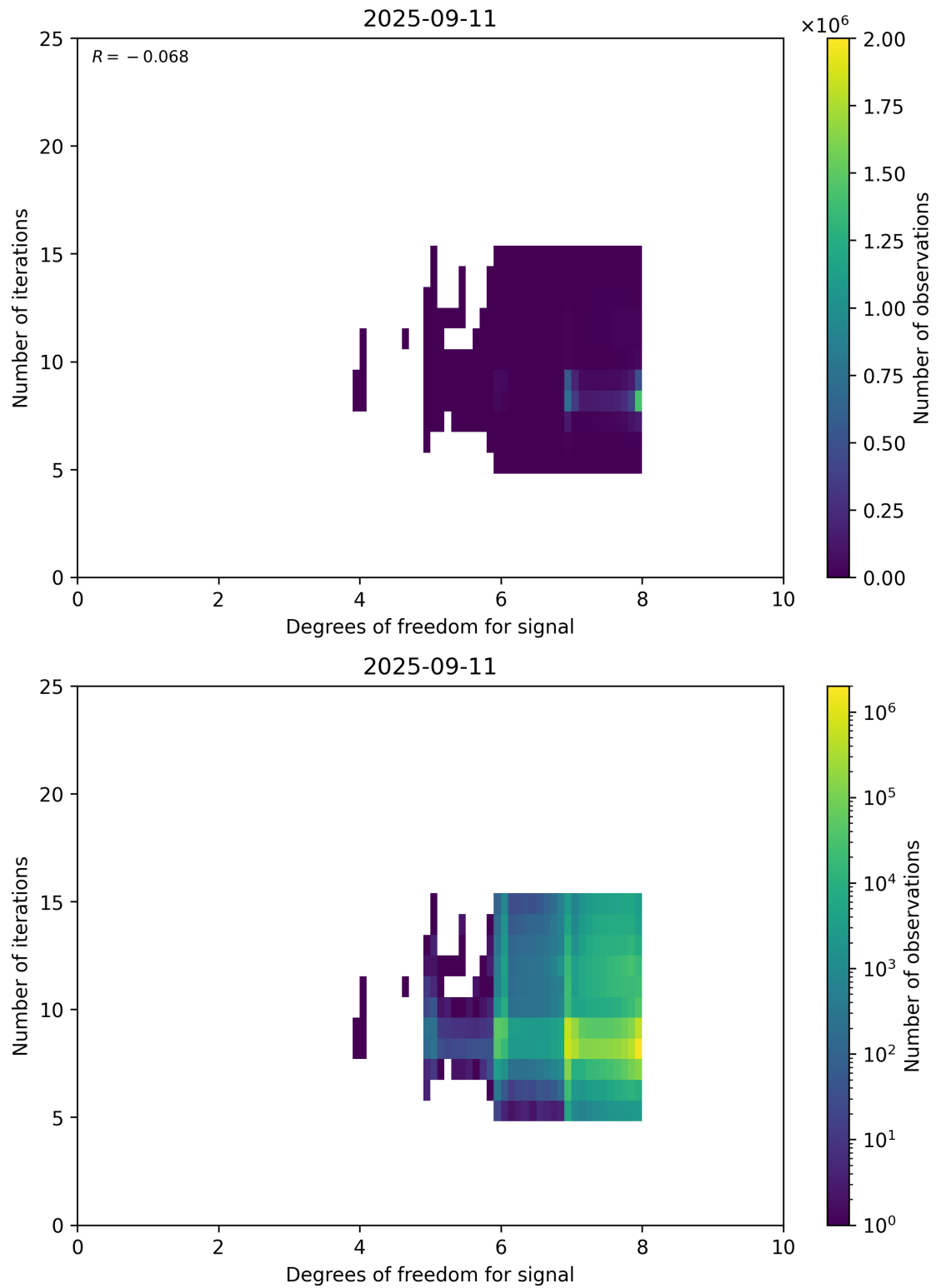
Figure 50: Scatter density plot of “Degrees of freedom for signal” against “Number of iterations” for 2025-09-10 to 2025-09-12.
