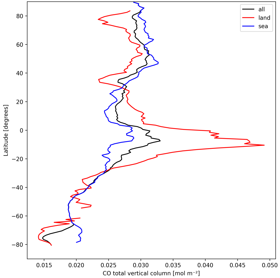
Figure 10: Zonal average of “CO total vertical column” for 2025-09-10 to 2025-09-12.
