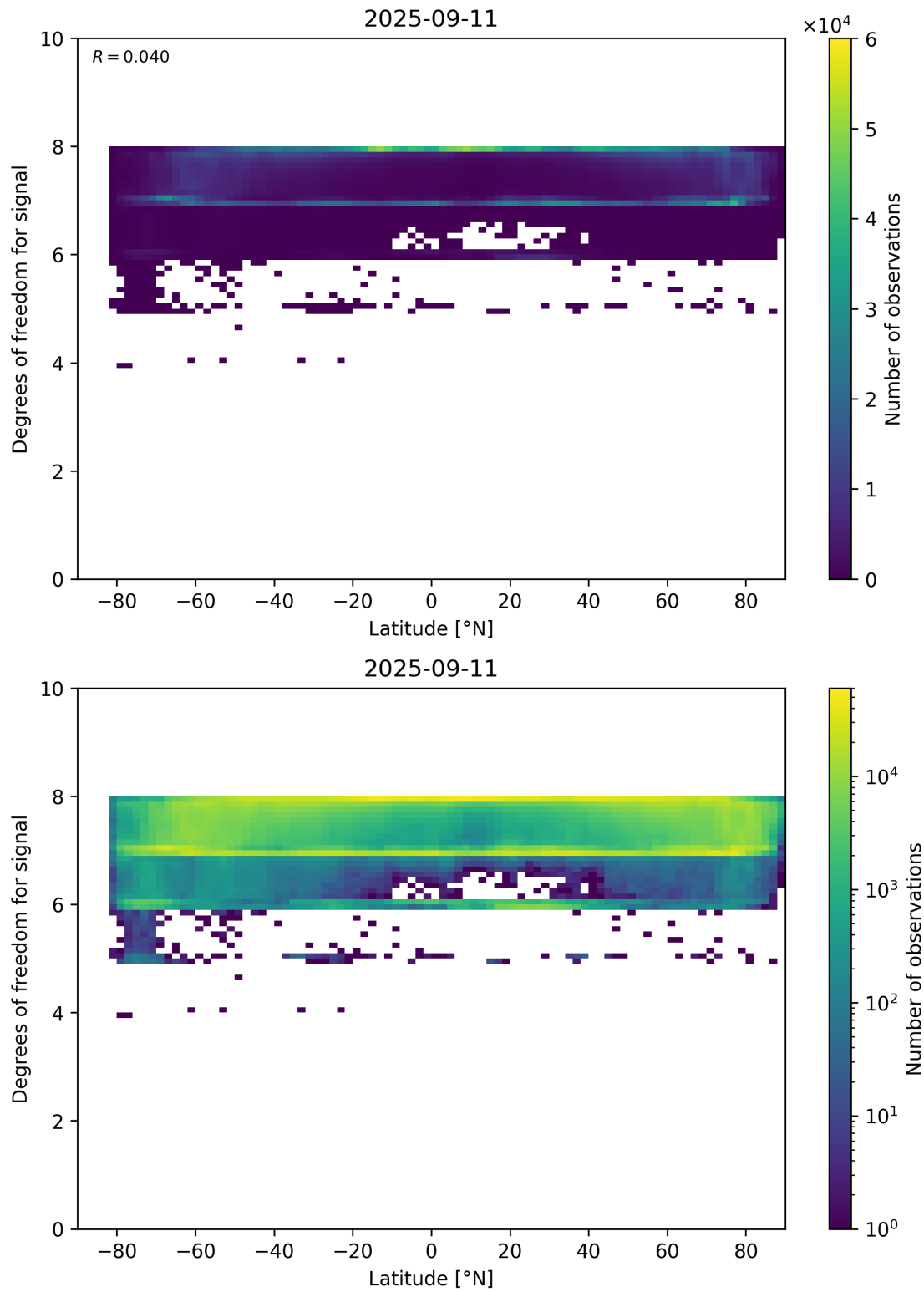
Figure 55: Scatter density plot of “Latitude” against “Degrees of freedom for signal” for 2025-09-10 to 2025-09-12.
