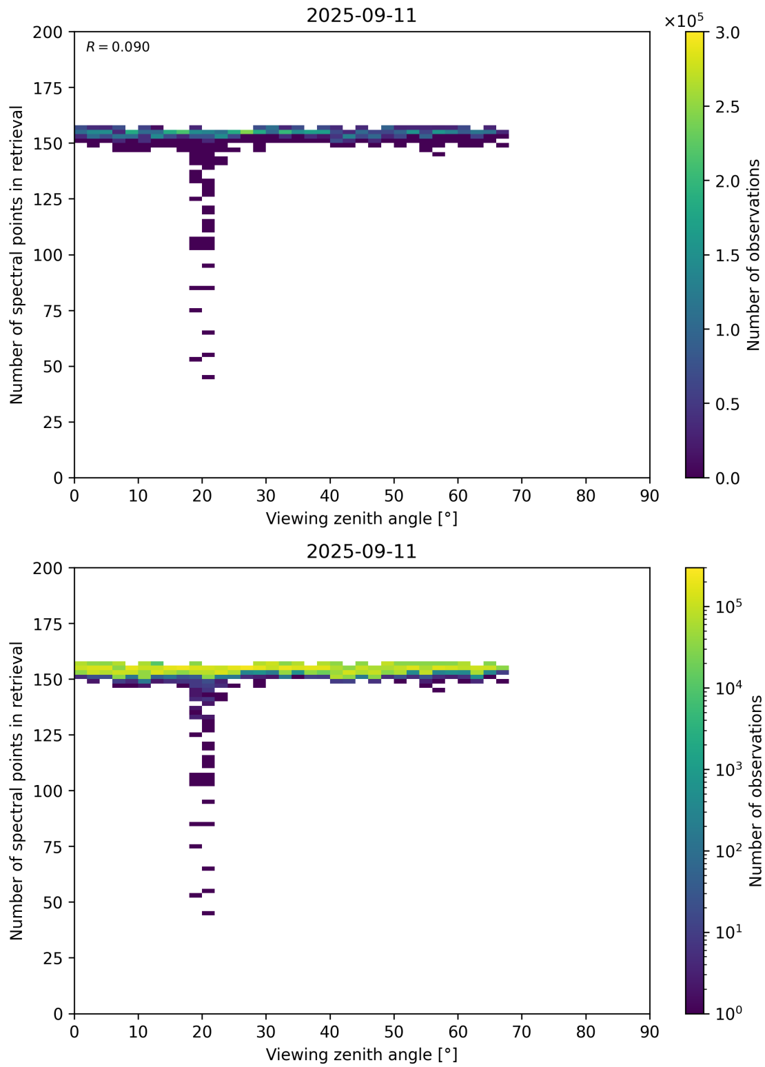
Figure 76: Scatter density plot of “Viewing zenith angle” against “Number of spectral points in retrieval” for 2025-09-10 to 2025-09-12.
