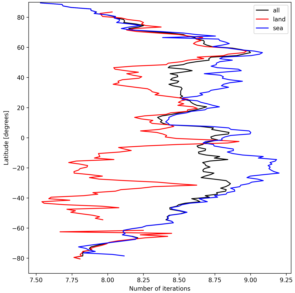
Figure 16: Zonal average of “Number of iterations” for 2025-09-10 to 2025-09-12.
