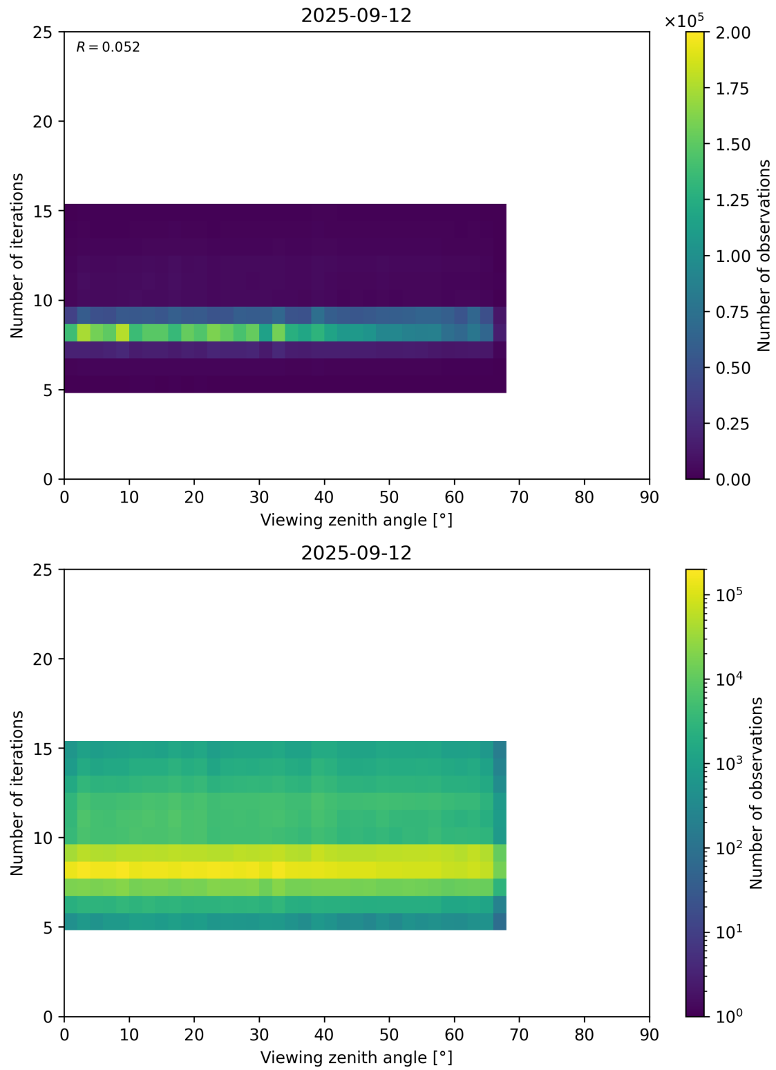
Figure 75: Scatter density plot of “Viewing zenith angle” against “Number of iterations” for 2025-09-11 to 2025-09-13.
