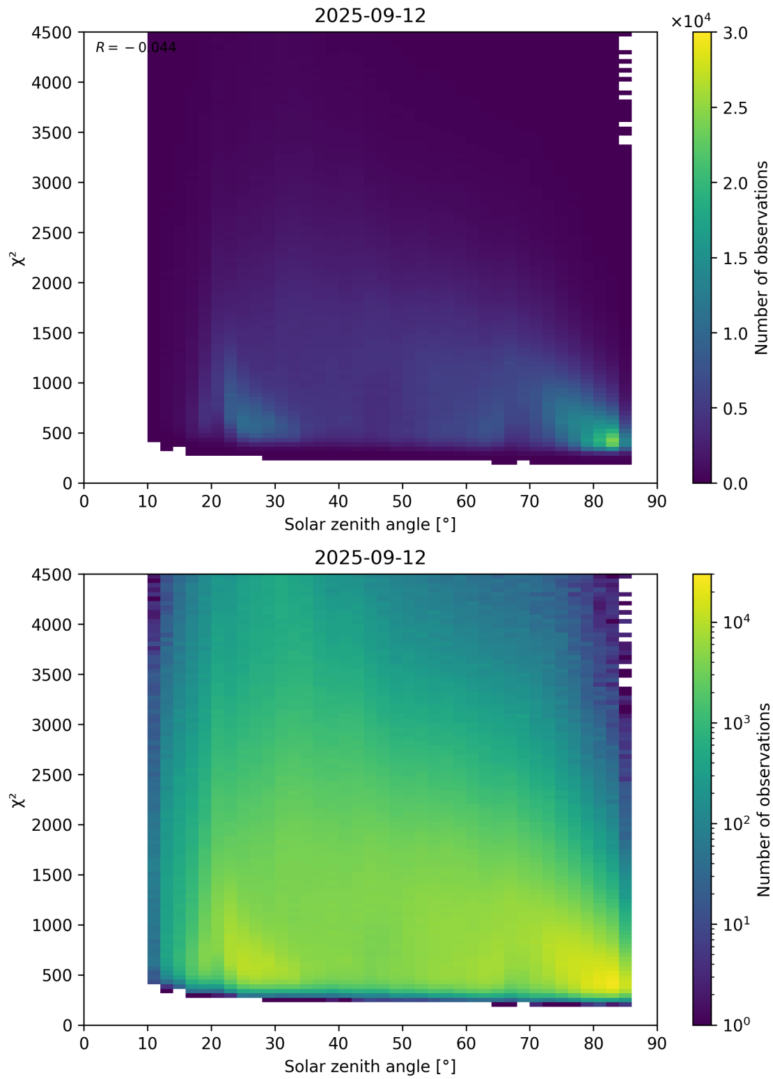
Figure 64: Scatter density plot of “Solar zenith angle” against “ \chi^2 ” for 2025-09-11 to 2025-09-13.
