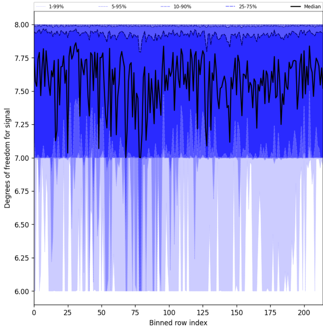
Figure 31: Along track statistics of “Degrees of freedom for signal” for 2025-09-11 to 2025-09-13
