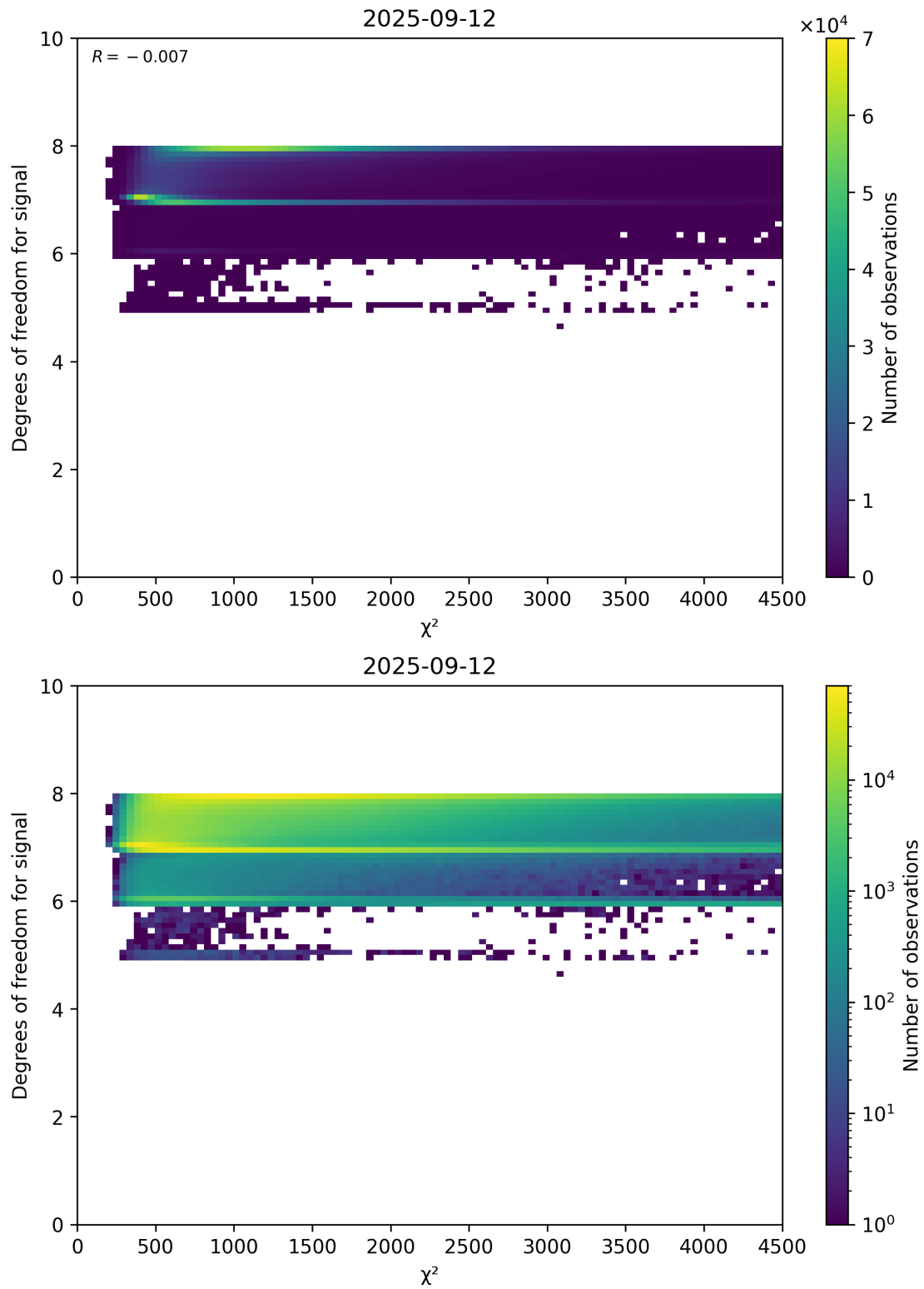
Figure 48: Scatter density plot of “ \chi^2 ” against “Degrees of freedom for signal” for 2025-09-11 to 2025-09-13.
