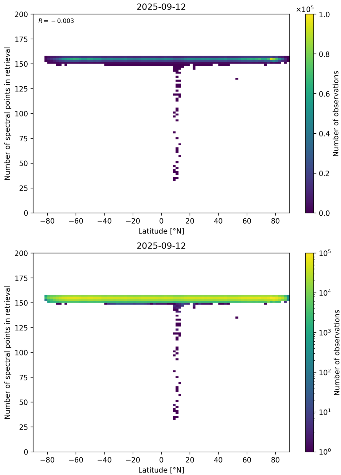
Figure 57: Scatter density plot of “Latitude” against “Number of spectral points in retrieval” for 2025-09-11 to 2025-09-13.
