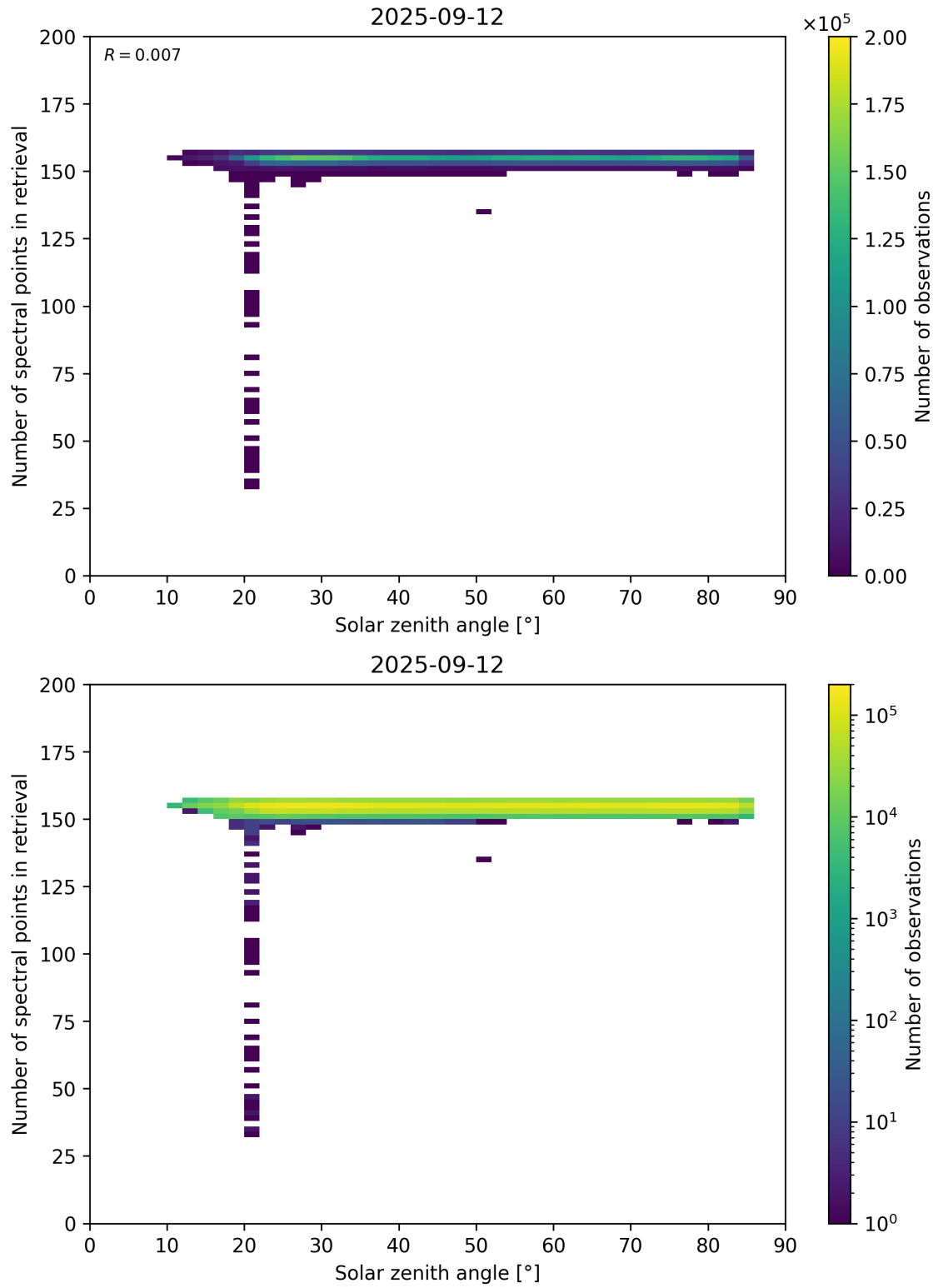
Figure 68: Scatter density plot of “Solar zenith angle” against “Number of spectral points in retrieval” for 2025-09-11 to 2025-09-13.
