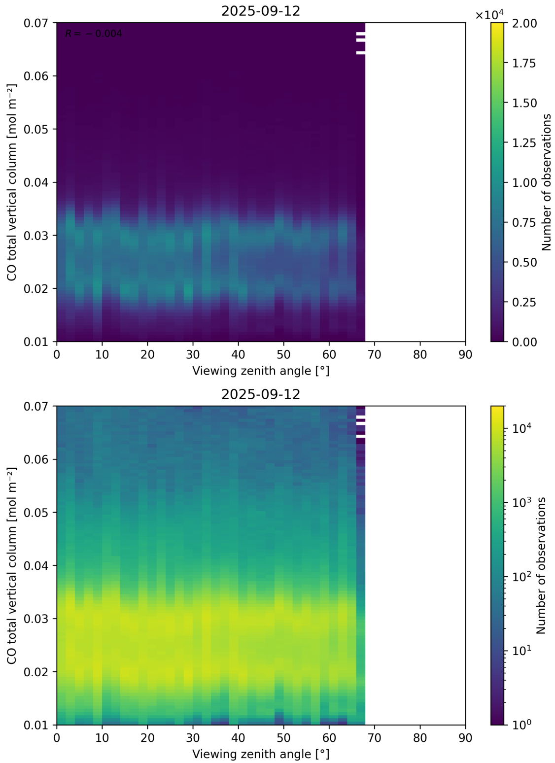
Figure 69: Scatter density plot of “Viewing zenith angle” against “CO total vertical column” for 2025-09-11 to 2025-09-13.
