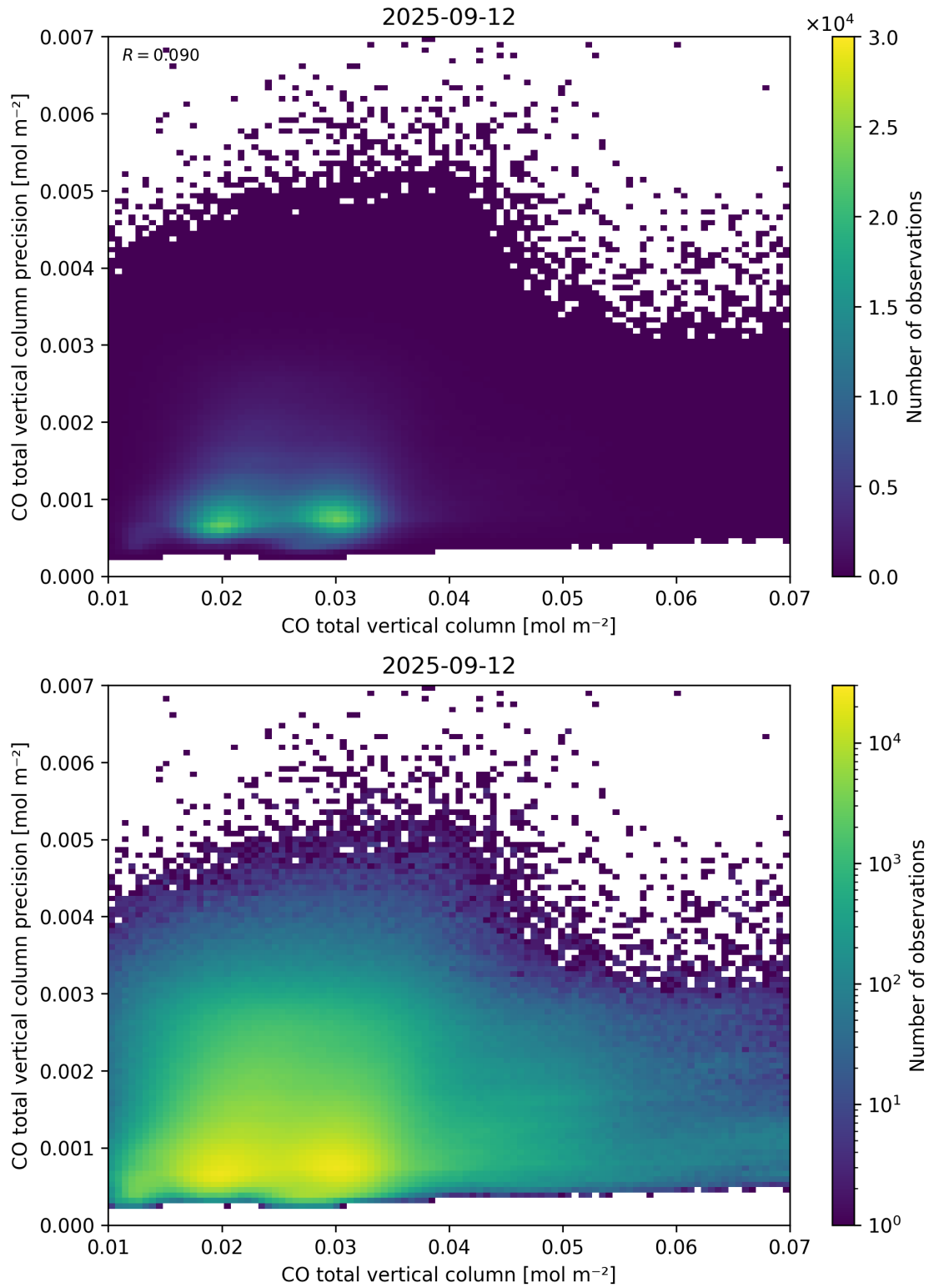
Figure 34: Scatter density plot of “CO total vertical column” against “CO total vertical column precision” for 2025-09-11 to 2025-09-13.
