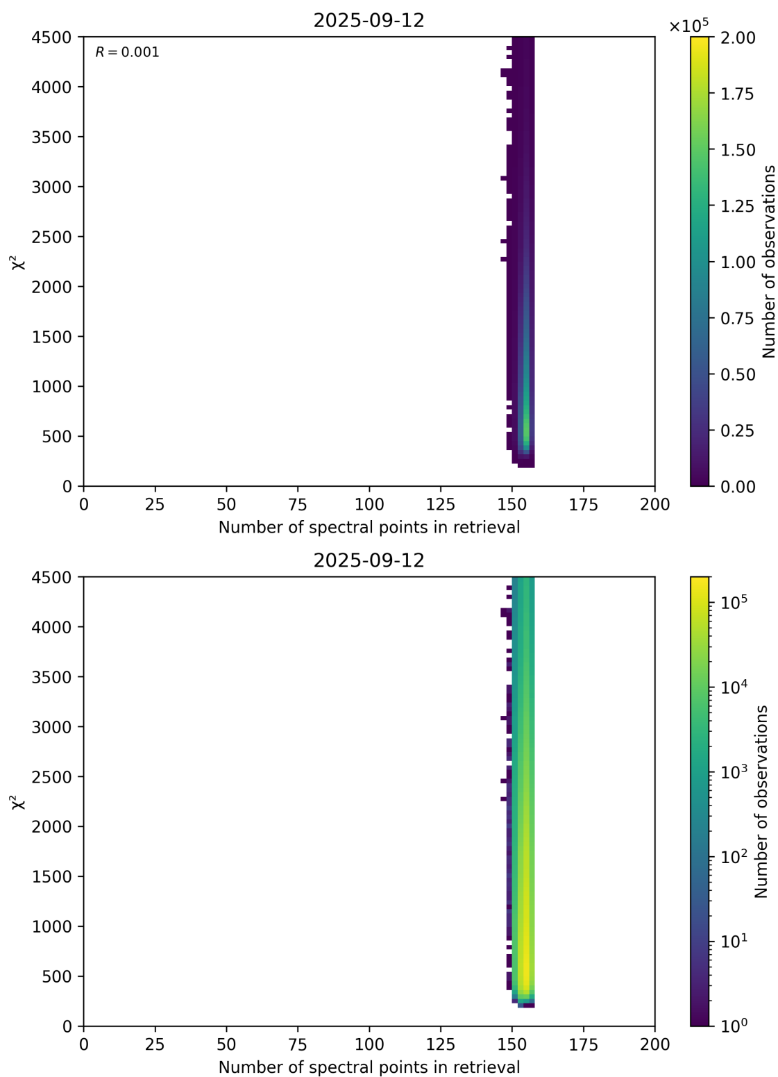
Figure 58: Scatter density plot of “Number of spectral points in retrieval” against “ \chi^2 ” for 2025-09-11 to 2025-09-13.
