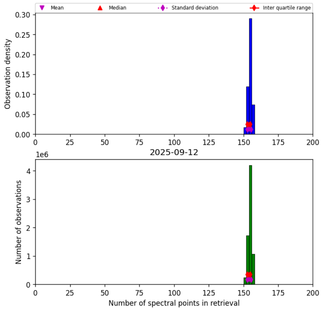
Figure 21: Histogram of “Number of spectral points in retrieval” for 2025-09-11 to 2025-09-13
