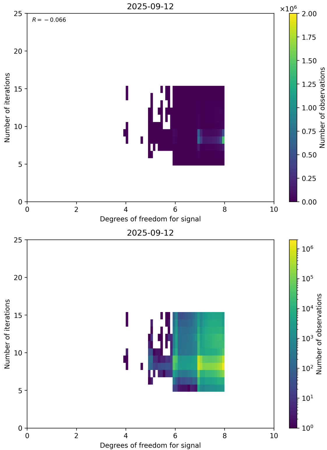
Figure 50: Scatter density plot of “Degrees of freedom for signal” against “Number of iterations” for 2025-09-11 to 2025-09-13.
