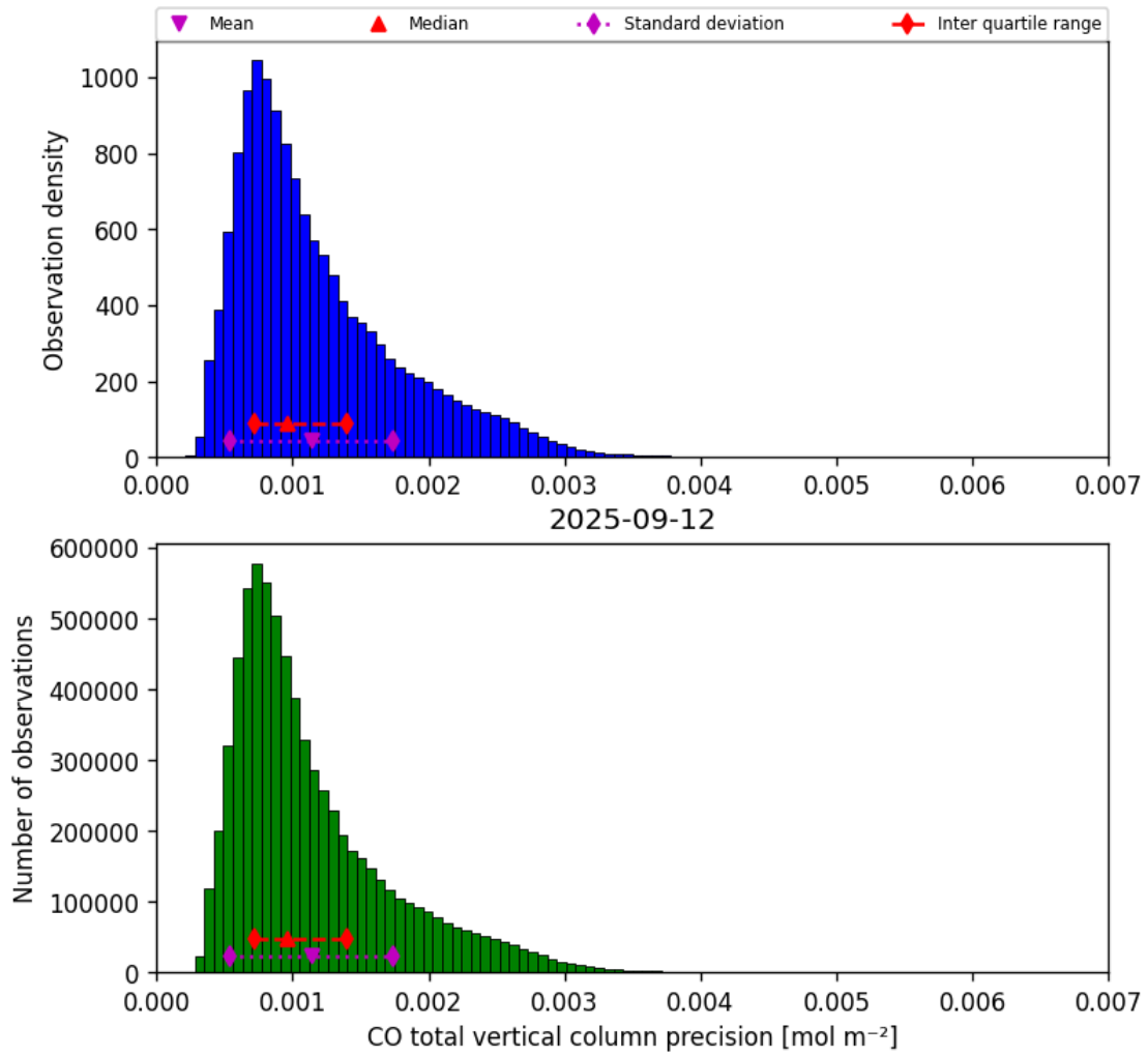
Figure 20: Histogram of “CO total vertical column precision” for 2025-09-11 to 2025-09-13
