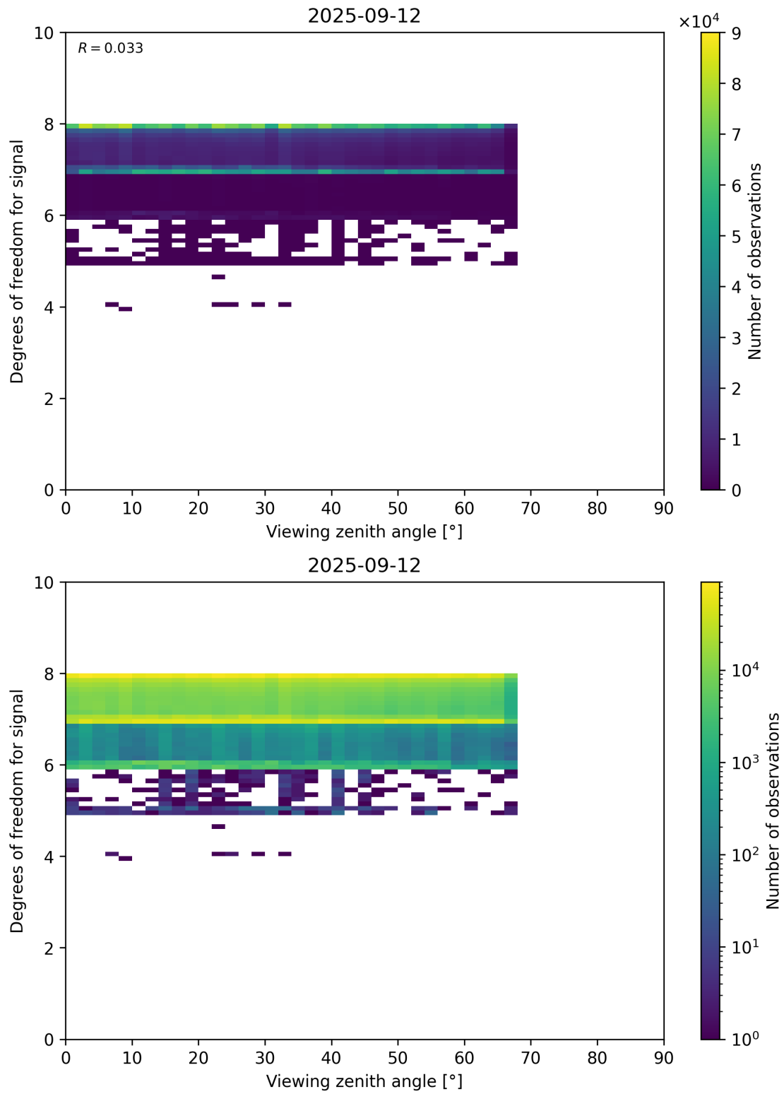
Figure 73: Scatter density plot of “Viewing zenith angle” against “Degrees of freedom for signal” for 2025-09-11 to 2025-09-13.
