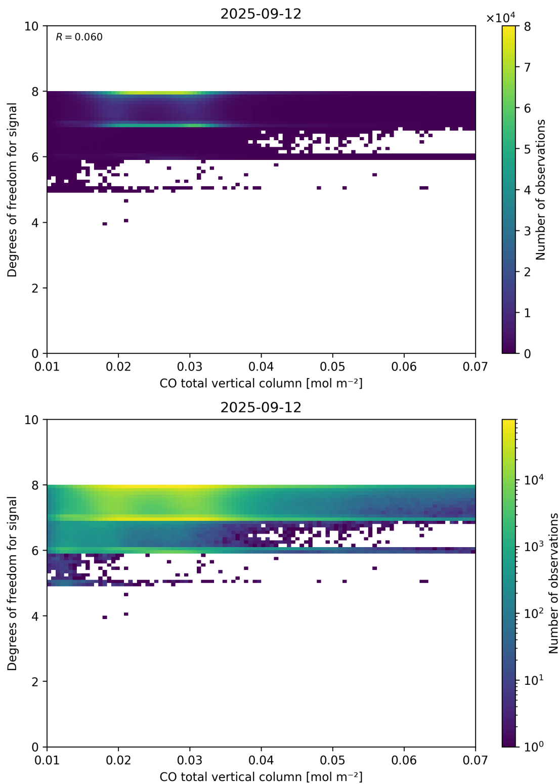
Figure 41: Scatter density plot of “CO total vertical column” against “Degrees of freedom for signal” for 2025-09-11 to 2025-09-13.
