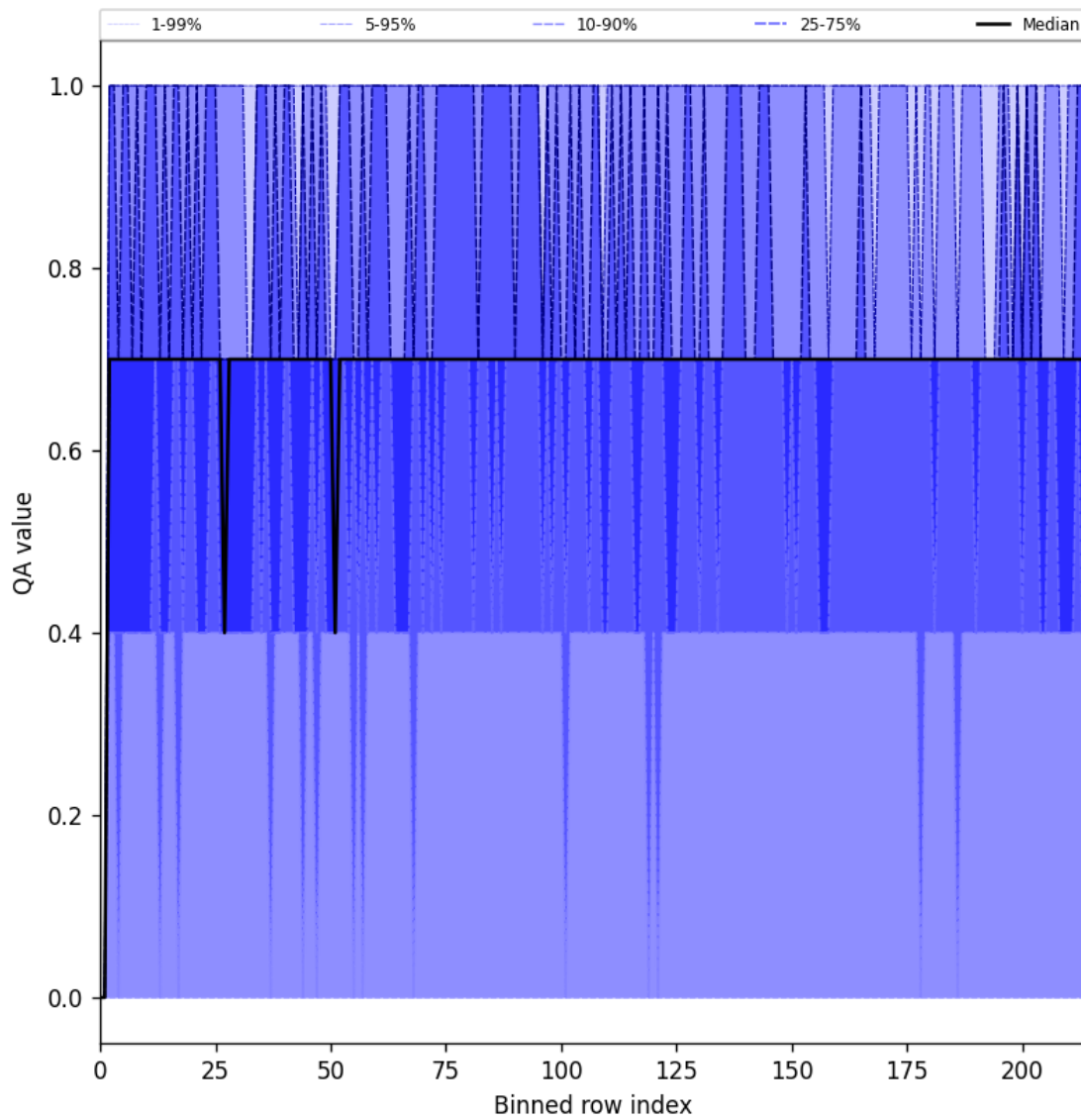
Figure 25: Along track statistics of “QA value” for 2025-09-11 to 2025-09-13
