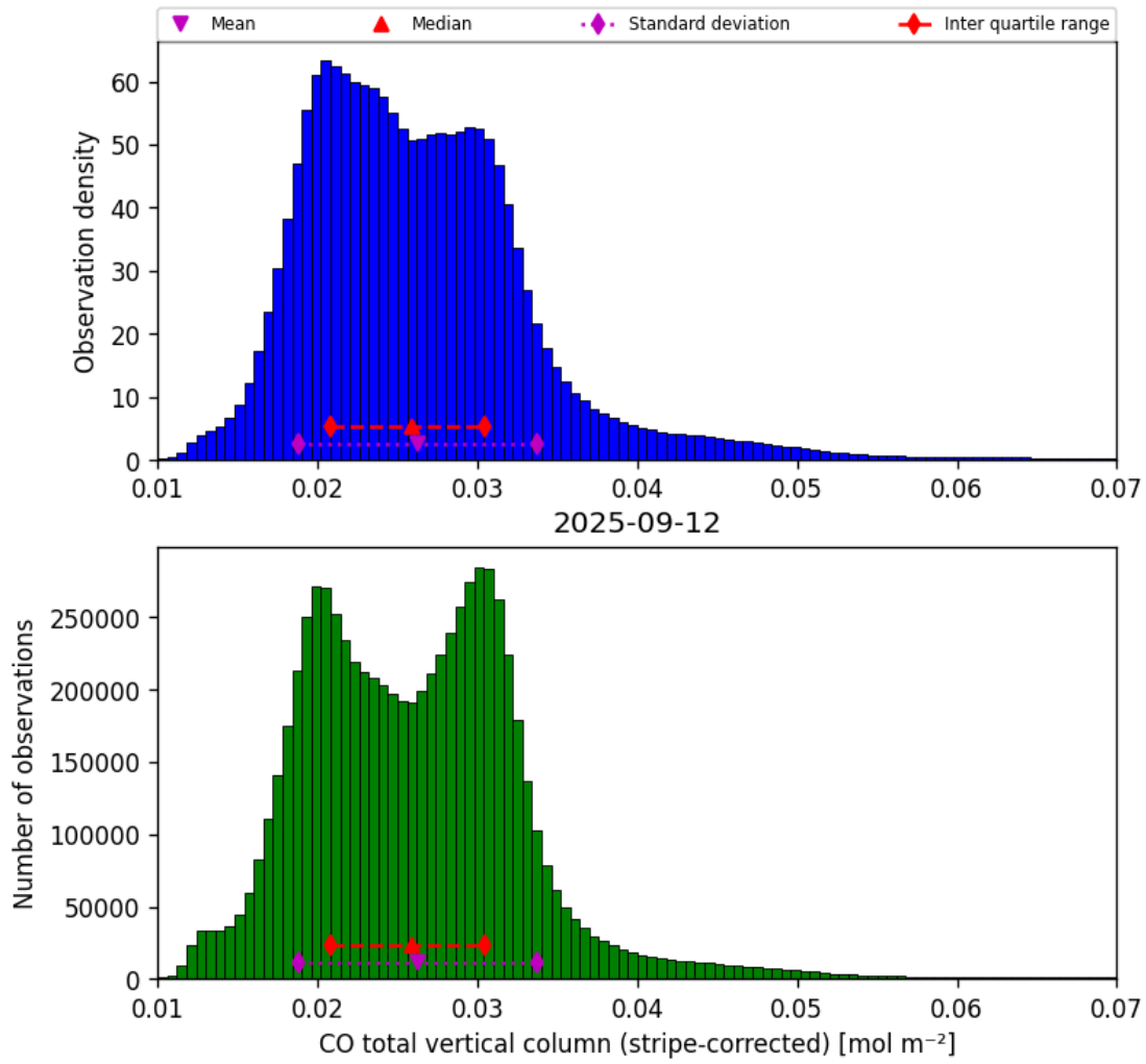
Figure 19: Histogram of “CO total vertical column (stripe-corrected)” for 2025-09-11 to 2025-09-13
