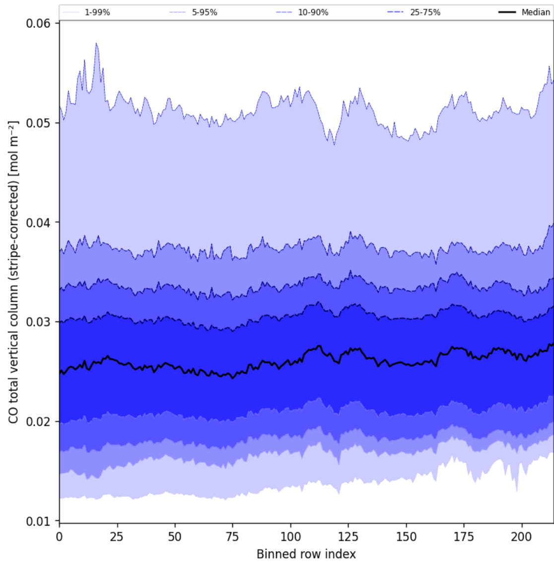
Figure 27: Along track statistics of “CO total vertical column (stripe-corrected)” for 2025-09-11 to 2025-09-13
