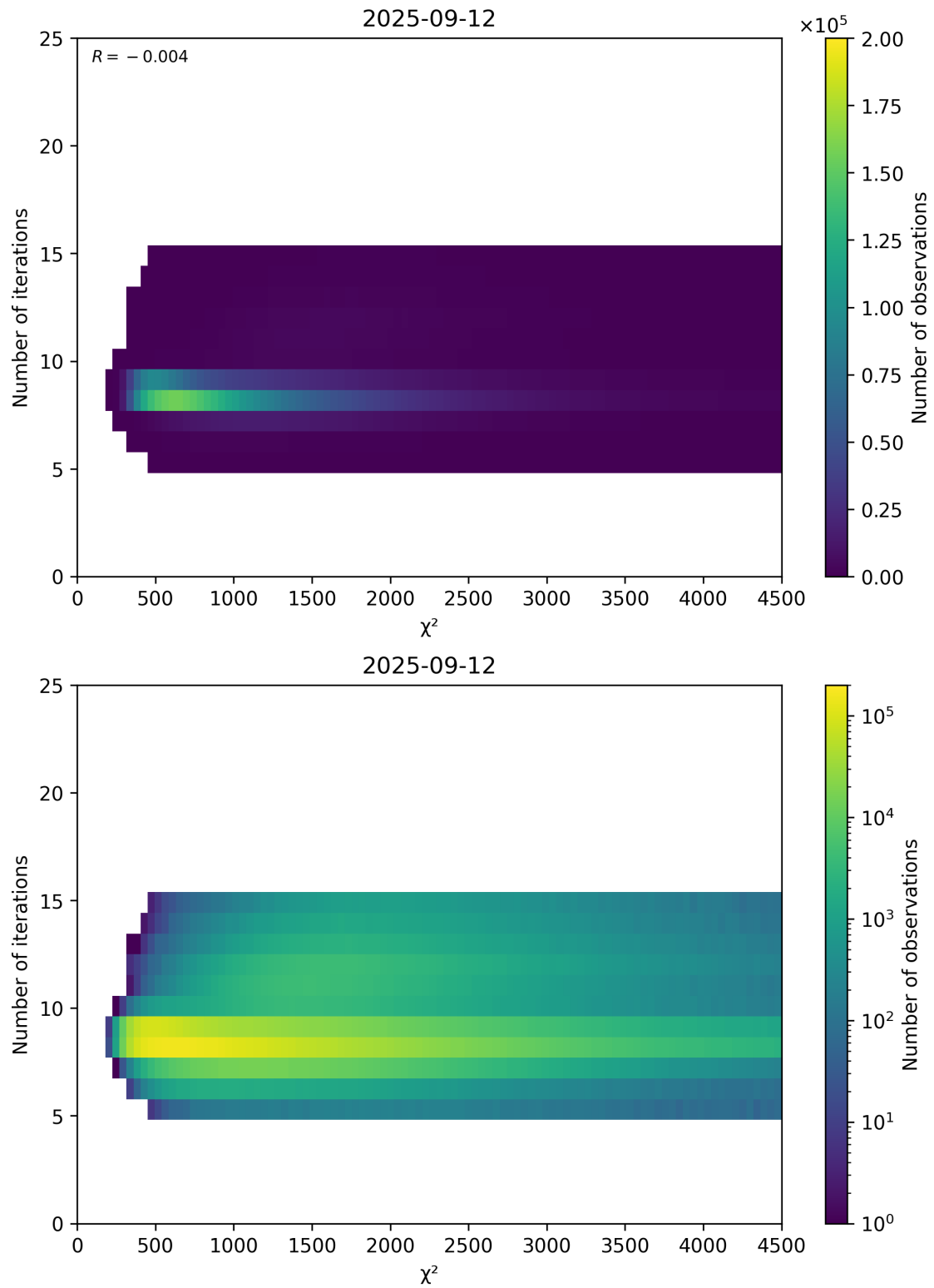
Figure 49: Scatter density plot of “ \chi^2 ” against “Number of iterations” for 2025-09-11 to 2025-09-13.
