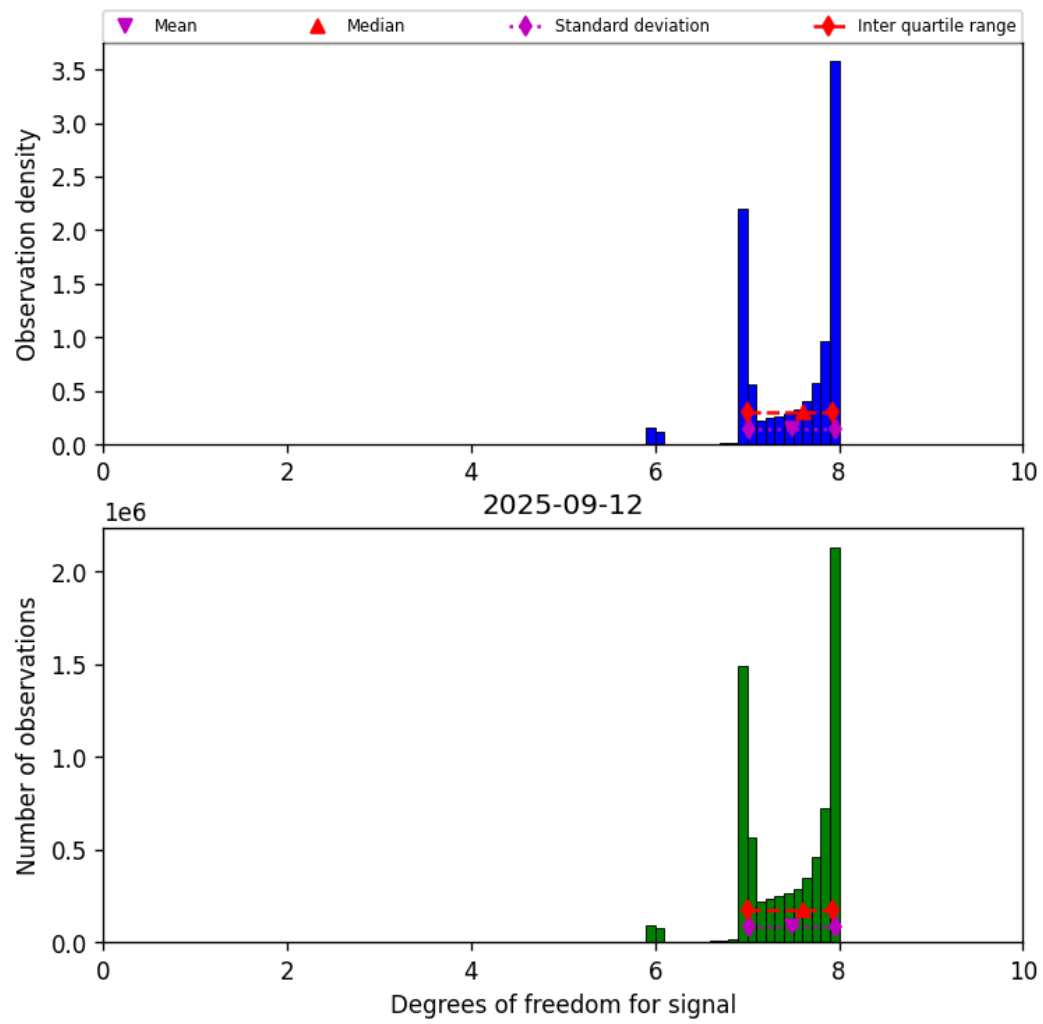
Figure 23: Histogram of “Degrees of freedom for signal” for 2025-09-11 to 2025-09-13
