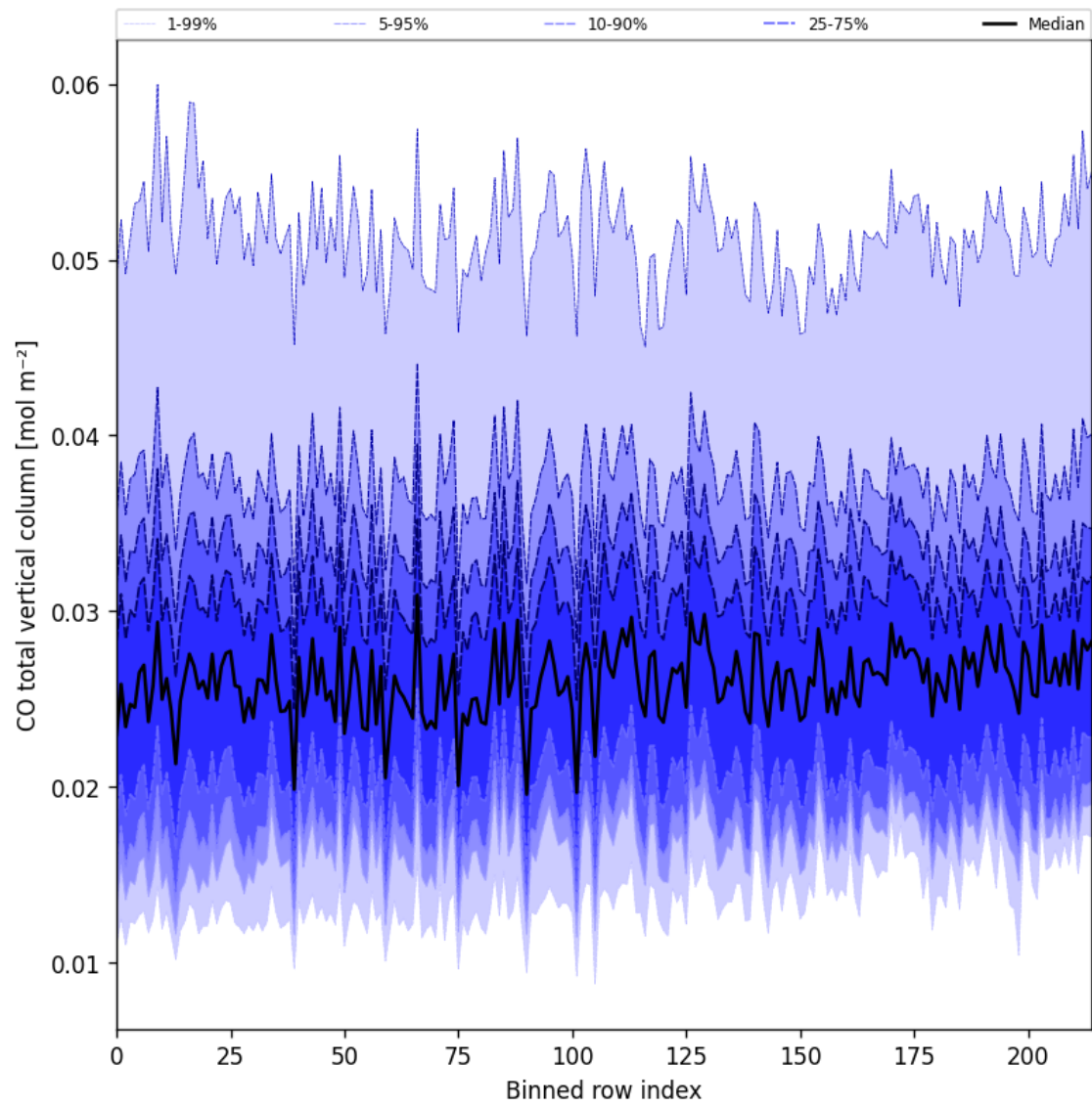
Figure 26: Along track statistics of “CO total vertical column” for 2025-09-11 to 2025-09-13
