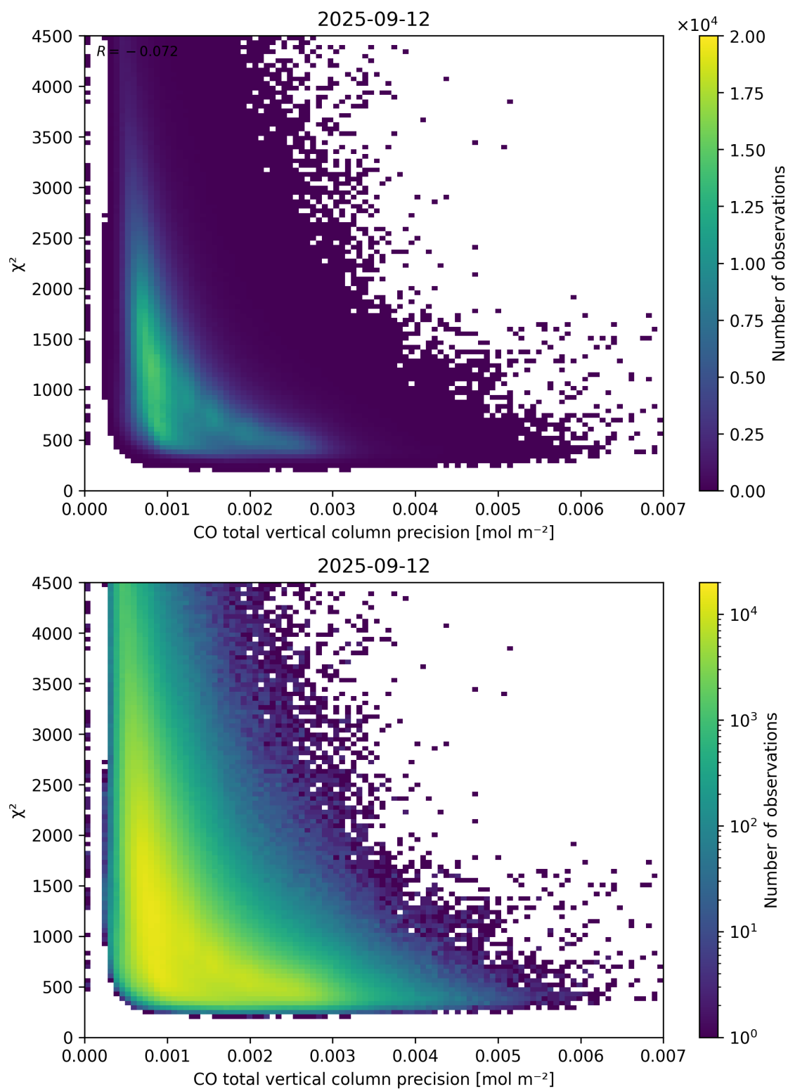
Figure 44: Scatter density plot of “CO total vertical column precision” against “ \chi^2 ” for 2025-09-11 to 2025-09-13.
