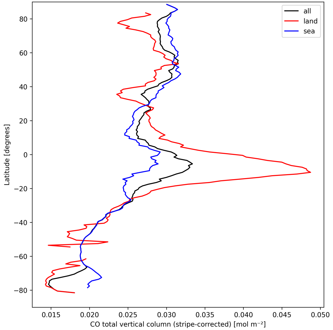
Figure 11: Zonal average of “CO total vertical column (stripe-corrected)” for 2025-09-11 to 2025-09-13.
