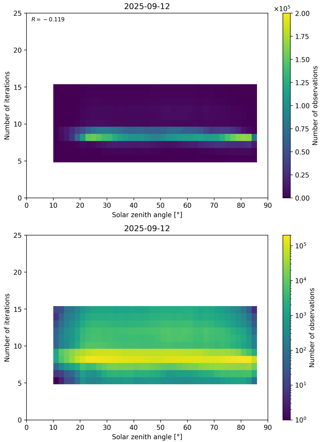
Figure 67: Scatter density plot of “Solar zenith angle” against “Number of iterations” for 2025-09-11 to 2025-09-13.
