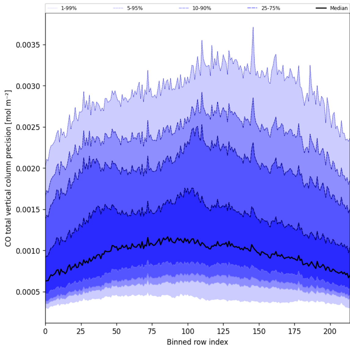
Figure 28: Along track statistics of “CO total vertical column precision” for 2025-09-11 to 2025-09-13
