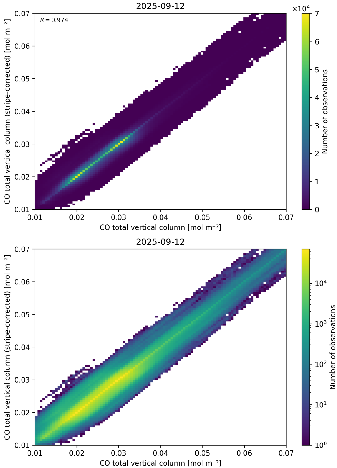
Figure 33: Scatter density plot of “CO total vertical column” against “CO total vertical column (stripe-corrected)” for 2025-09-11 to 2025-09-13.
