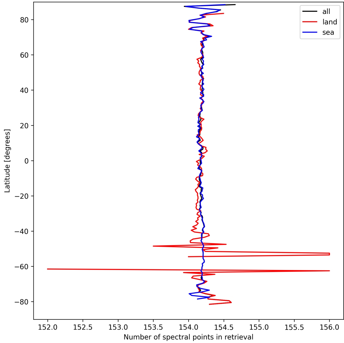
Figure 13: Zonal average of “Number of spectral points in retrieval” for 2025-09-11 to 2025-09-13.
