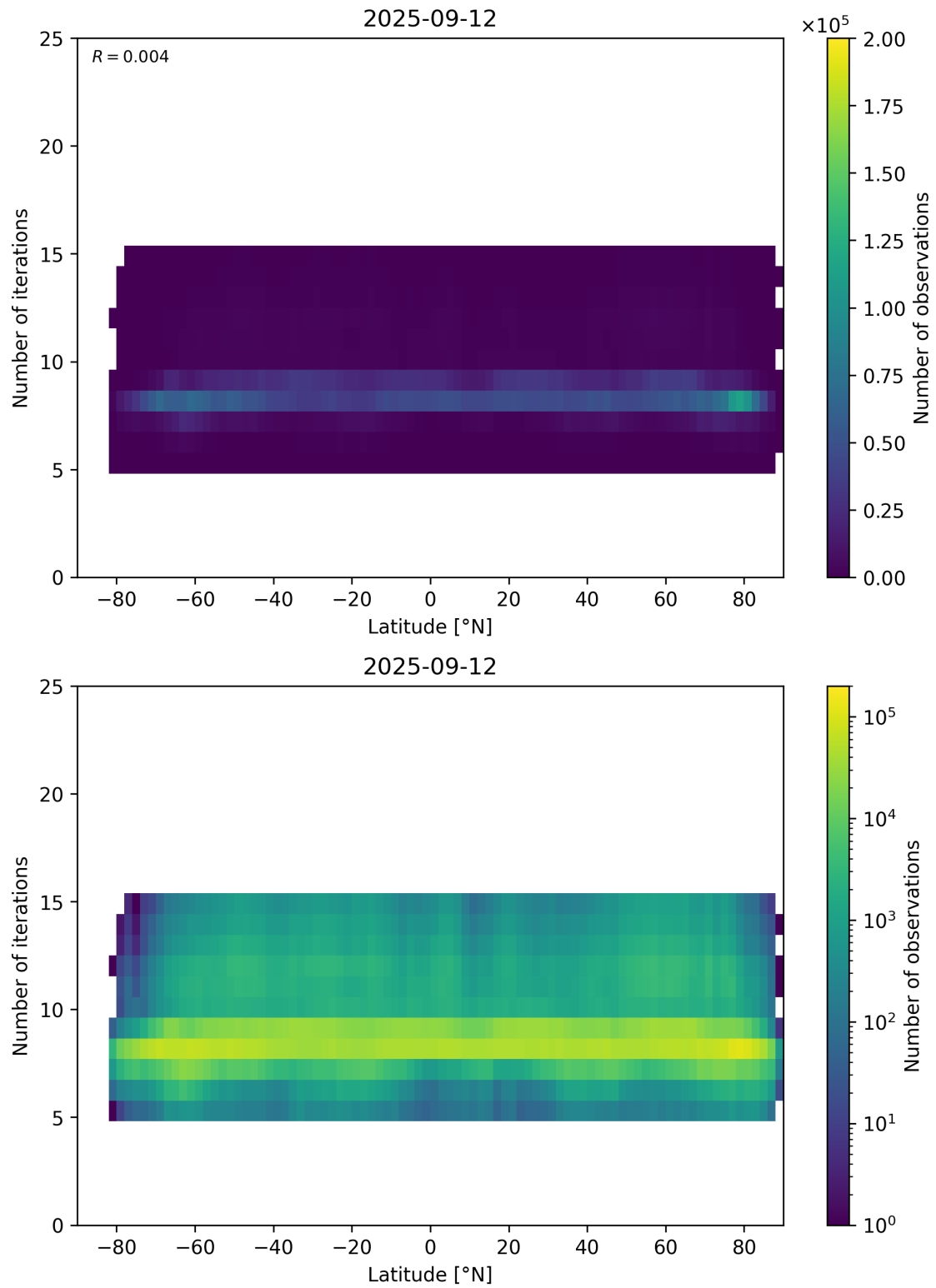
Figure 56: Scatter density plot of “Latitude” against “Number of iterations” for 2025-09-11 to 2025-09-13.
