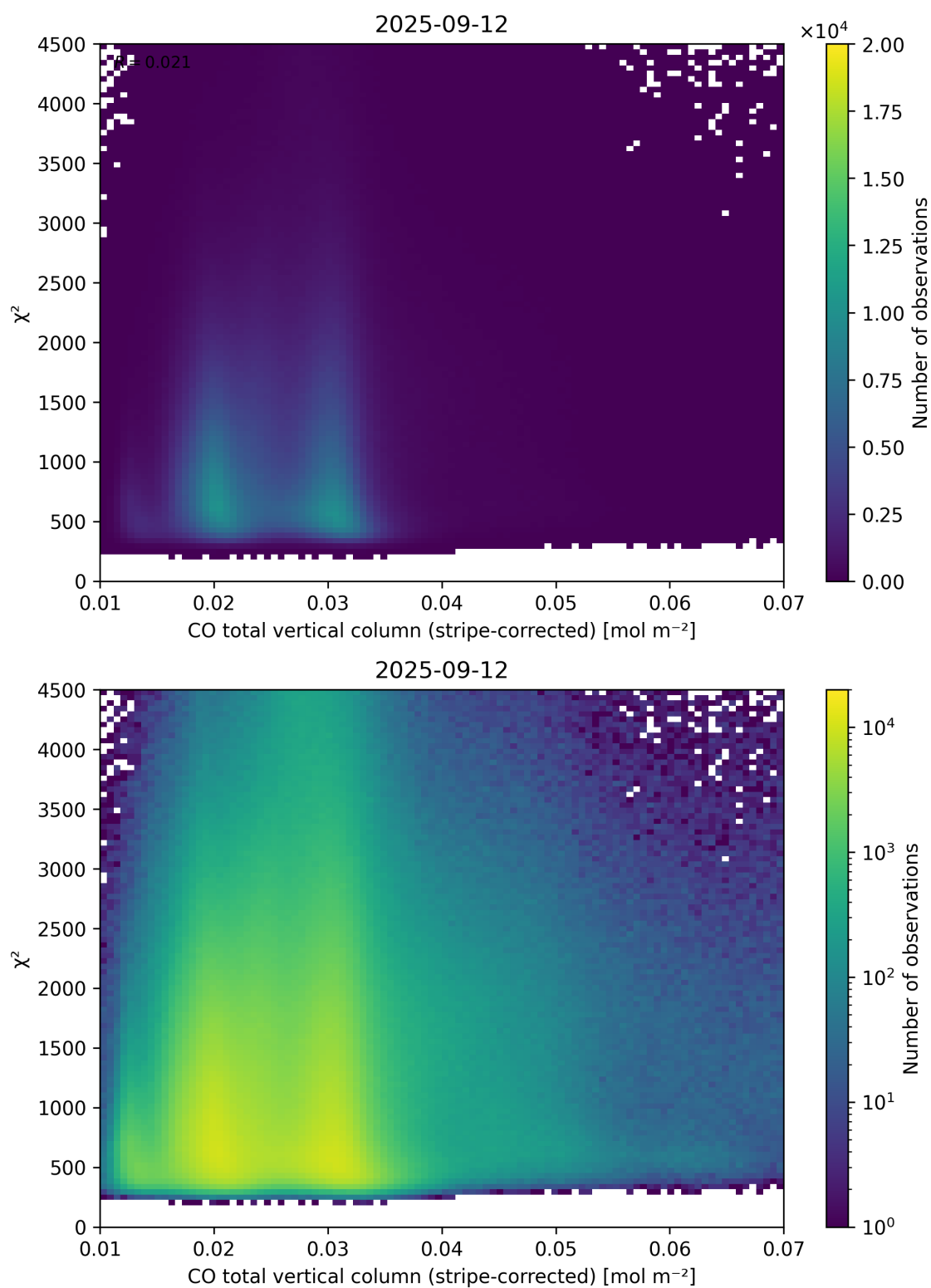
Figure 37: Scatter density plot of “CO total vertical column (stripe-corrected)” against “ \chi^2 ” for 2025-09-11 to 2025-09-13.
