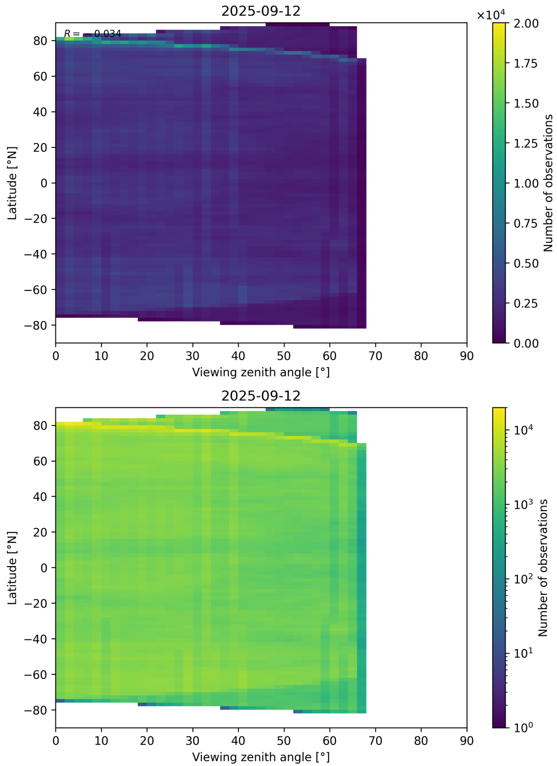
Figure 74: Scatter density plot of “Viewing zenith angle” against “Latitude” for 2025-09-11 to 2025-09-13.
