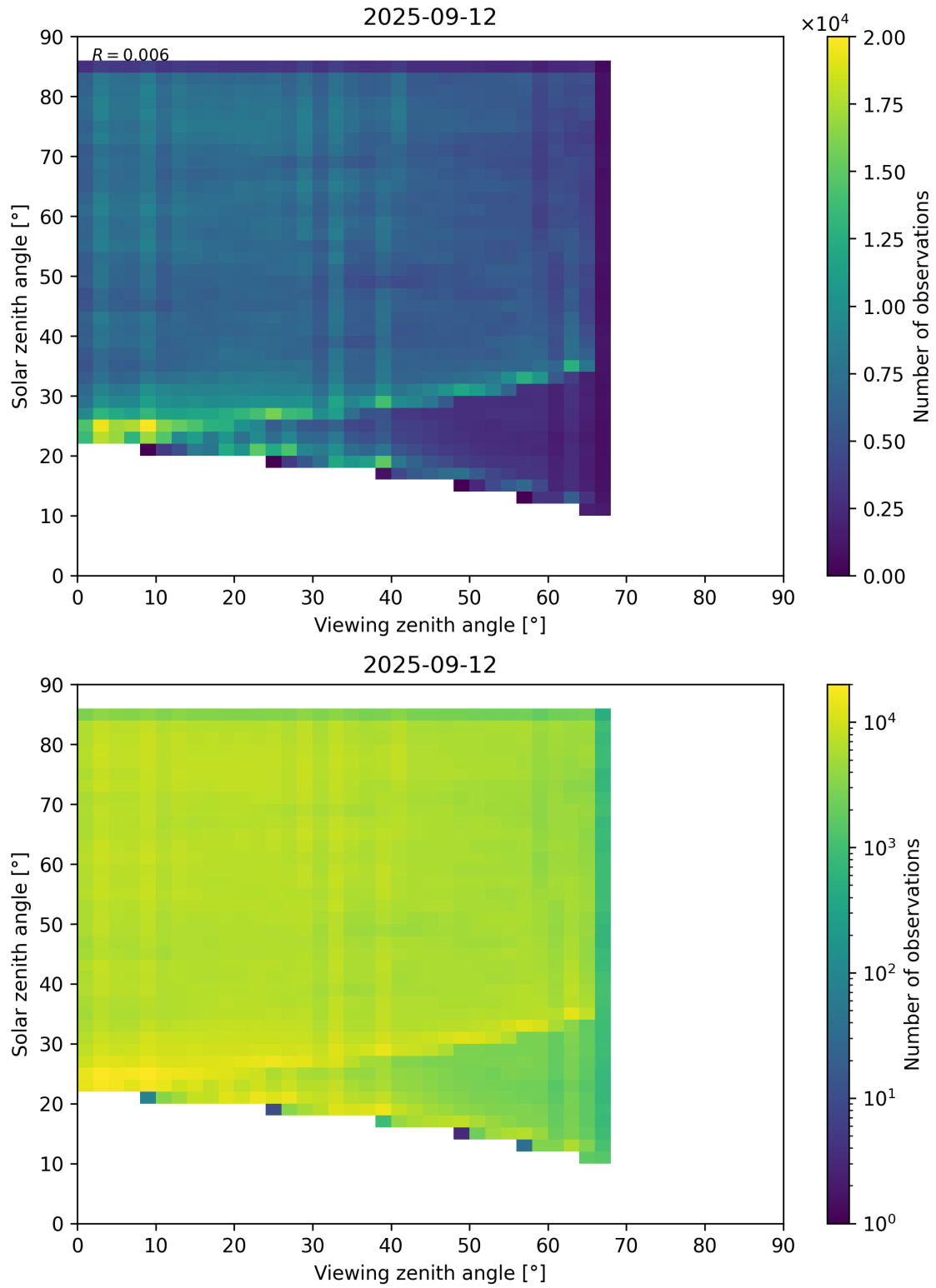
Figure 77: Scatter density plot of “Viewing zenith angle” against “Solar zenith angle” for 2025-09-11 to 2025-09-13.
