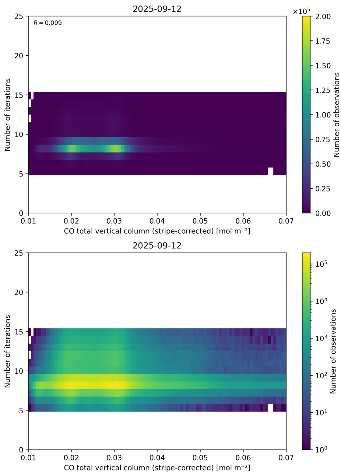
Figure 39: Scatter density plot of “CO total vertical column (stripe-corrected)” against “Number of iterations” for 2025-09-11 to 2025-09-13.
