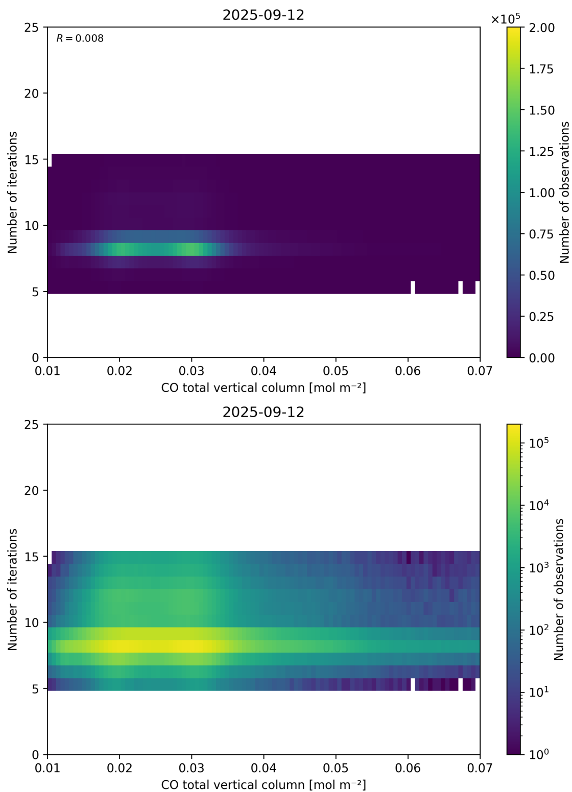
Figure 42: Scatter density plot of “CO total vertical column” against “Number of iterations” for 2025-09-11 to 2025-09-13.
