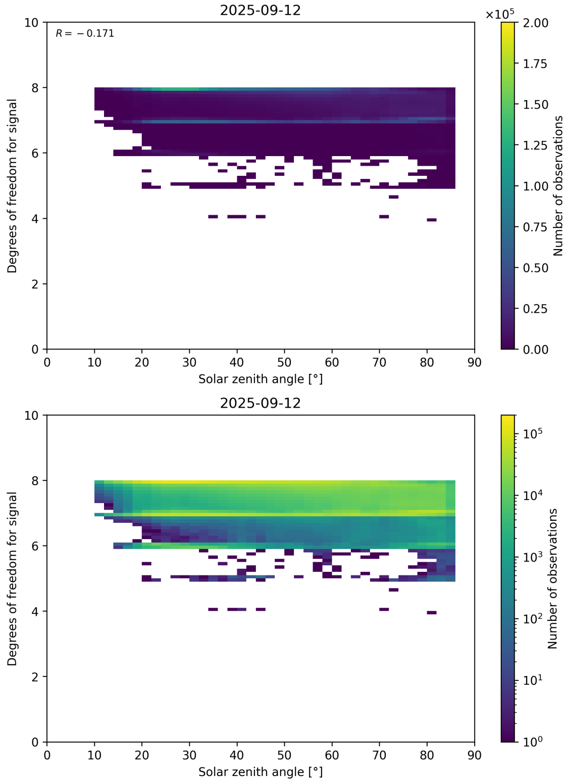
Figure 65: Scatter density plot of “Solar zenith angle” against “Degrees of freedom for signal” for 2025-09-11 to 2025-09-13.
