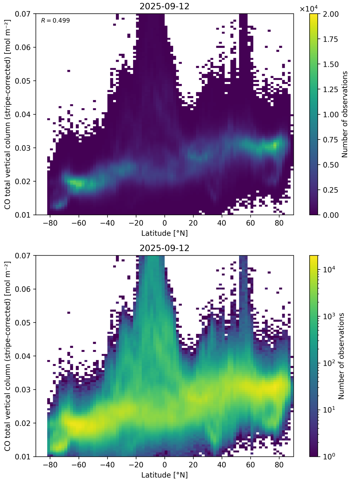
Figure 52: Scatter density plot of “Latitude” against “CO total vertical column (stripe-corrected)” for 2025-09-11 to 2025-09-13.
