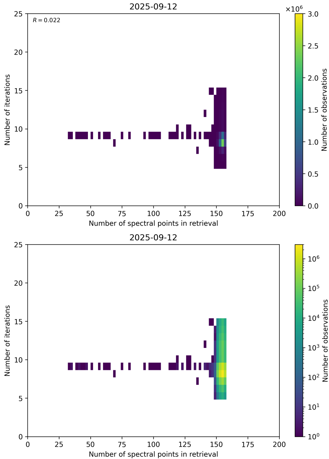
Figure 60: Scatter density plot of “Number of spectral points in retrieval” against “Number of iterations” for 2025-09-11 to 2025-09-13.
