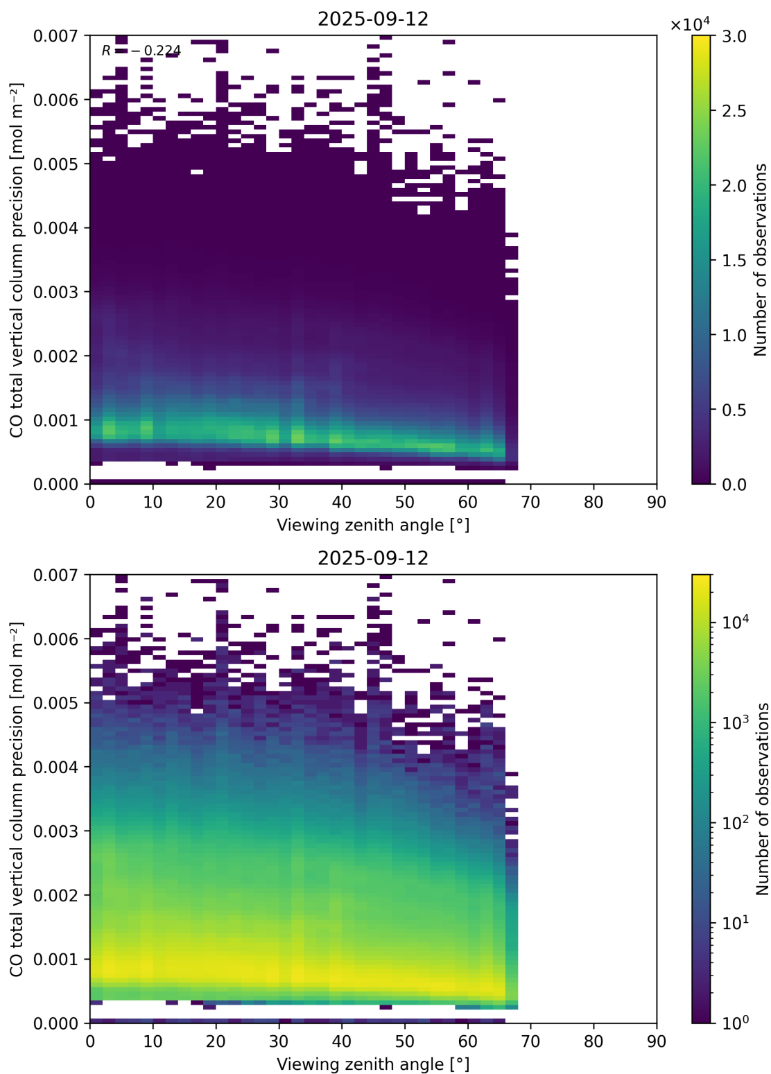
Figure 71: Scatter density plot of “Viewing zenith angle” against “CO total vertical column precision” for 2025-09-11 to 2025-09-13.
