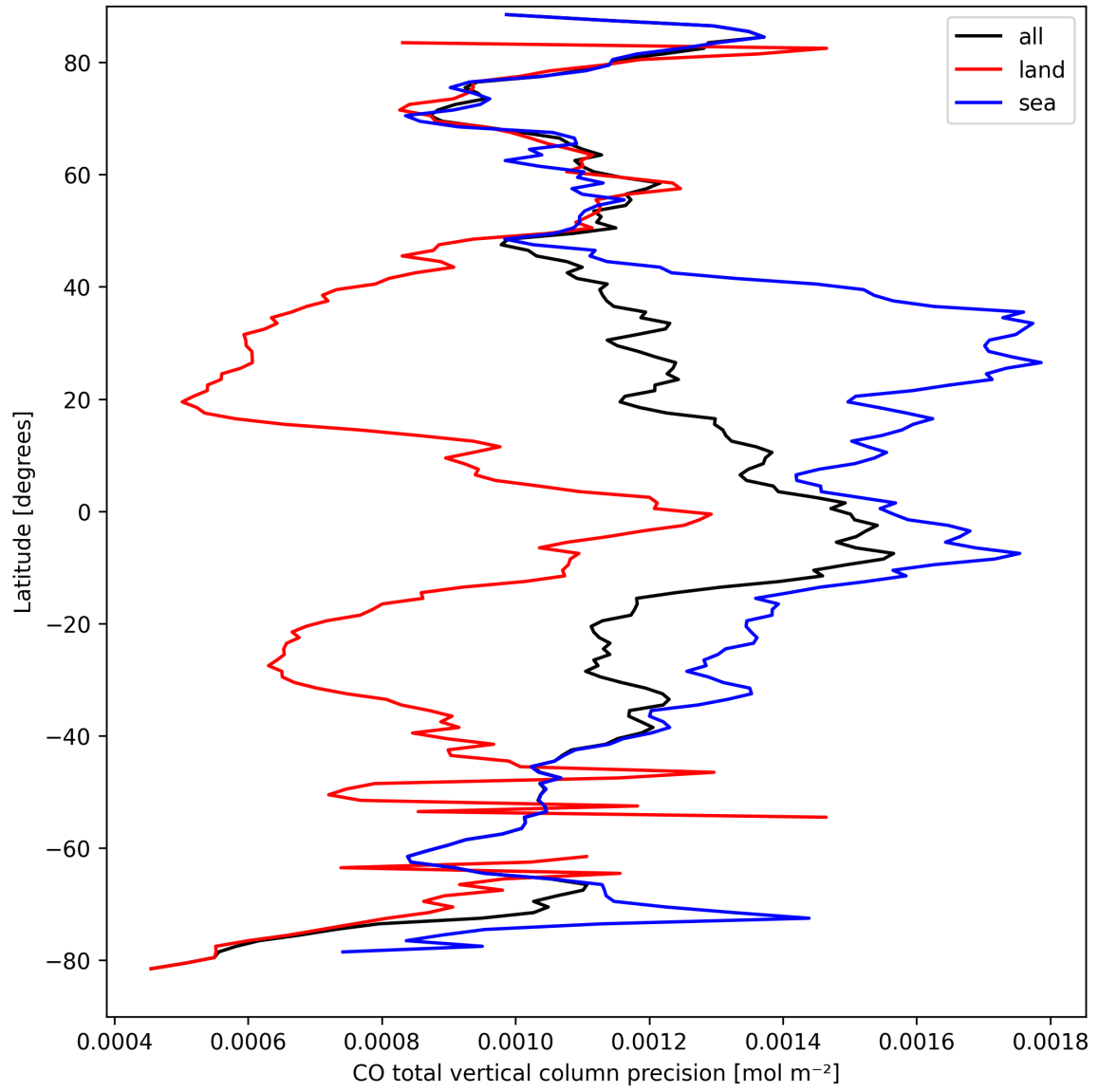
Figure 12: Zonal average of “CO total vertical column precision” for 2025-09-11 to 2025-09-13.
