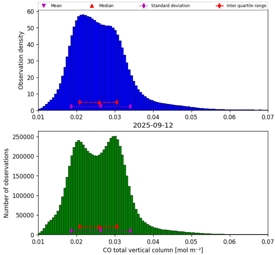
Figure 18: Histogram of “CO total vertical column” for 2025-09-11 to 2025-09-13
