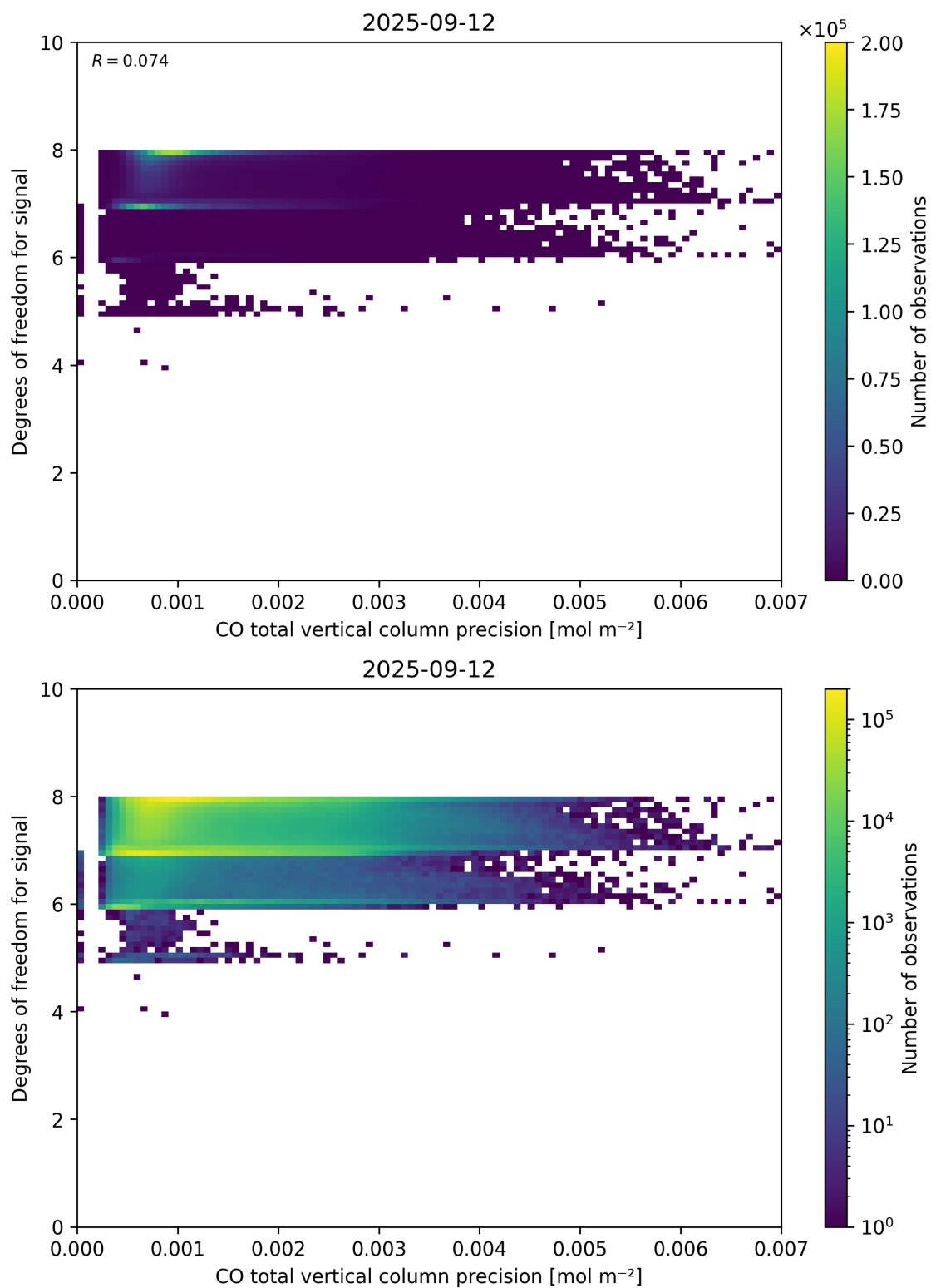
Figure 45: Scatter density plot of “CO total vertical column precision” against “Degrees of freedom for signal” for 2025-09-11 to 2025-09-13.
