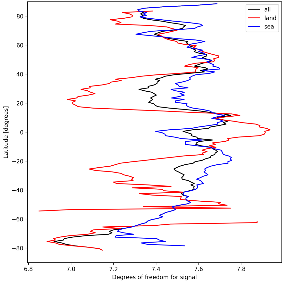
Figure 15: Zonal average of “Degrees of freedom for signal” for 2025-09-11 to 2025-09-13.
