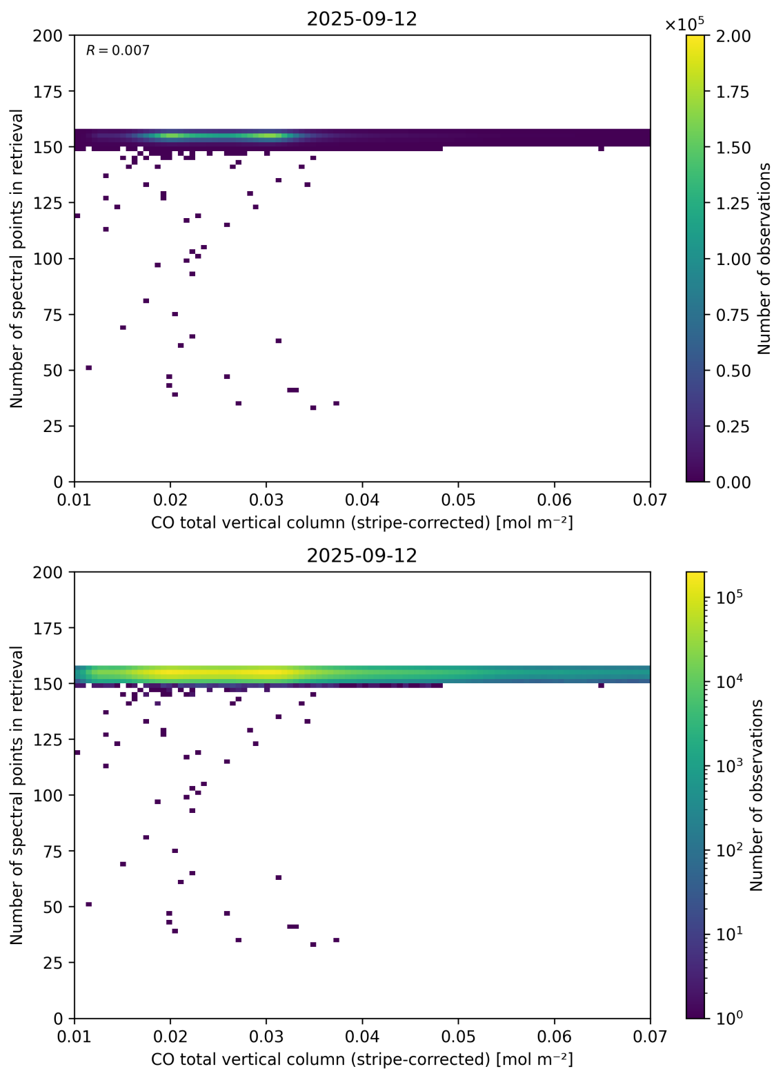
Figure 40: Scatter density plot of “CO total vertical column (stripe-corrected)” against “Number of spectral points in retrieval” for 2025-09-11 to 2025-09-13.
