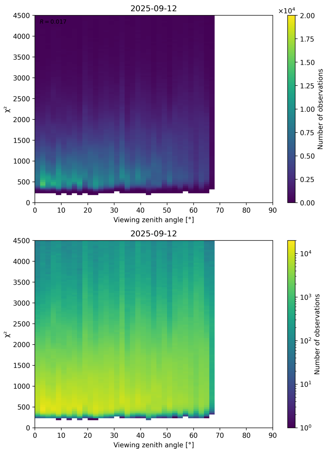
Figure 72: Scatter density plot of “Viewing zenith angle” against “ \chi^2 ” for 2025-09-11 to 2025-09-13.
