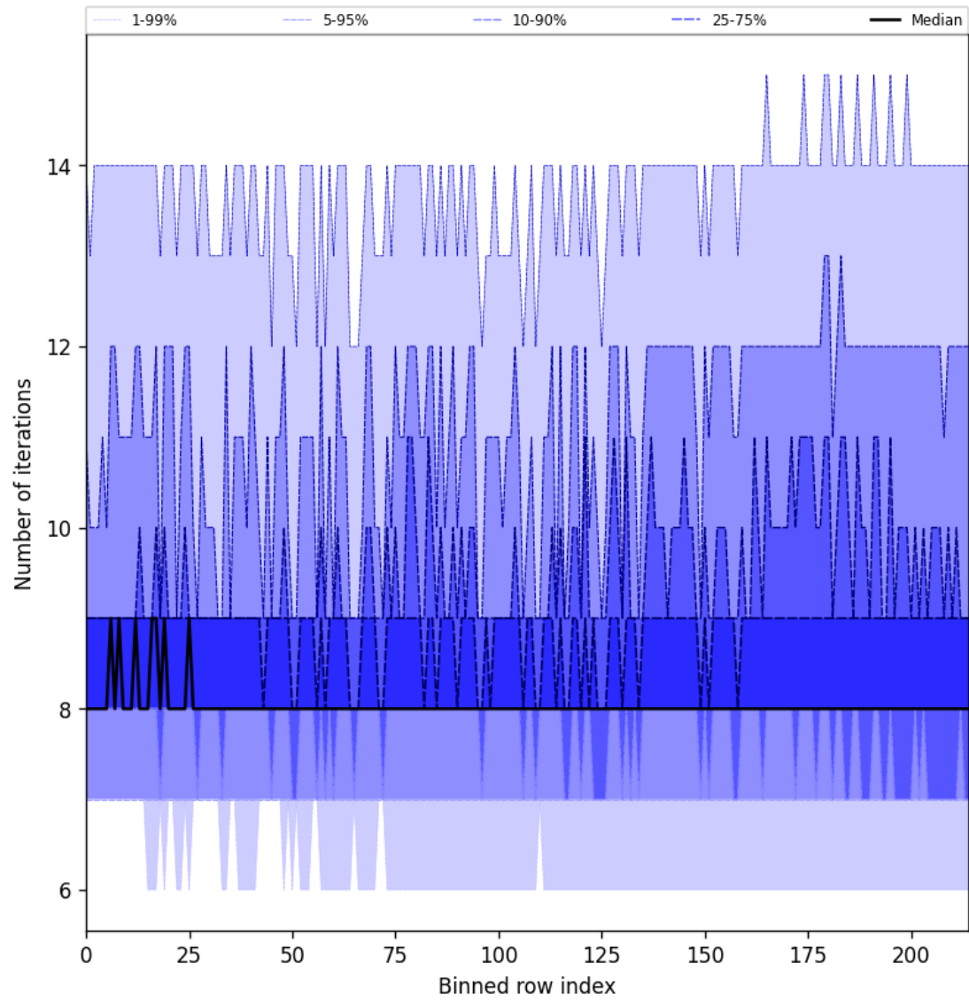
Figure 32: Along track statistics of “Number of iterations” for 2025-09-11 to 2025-09-13
