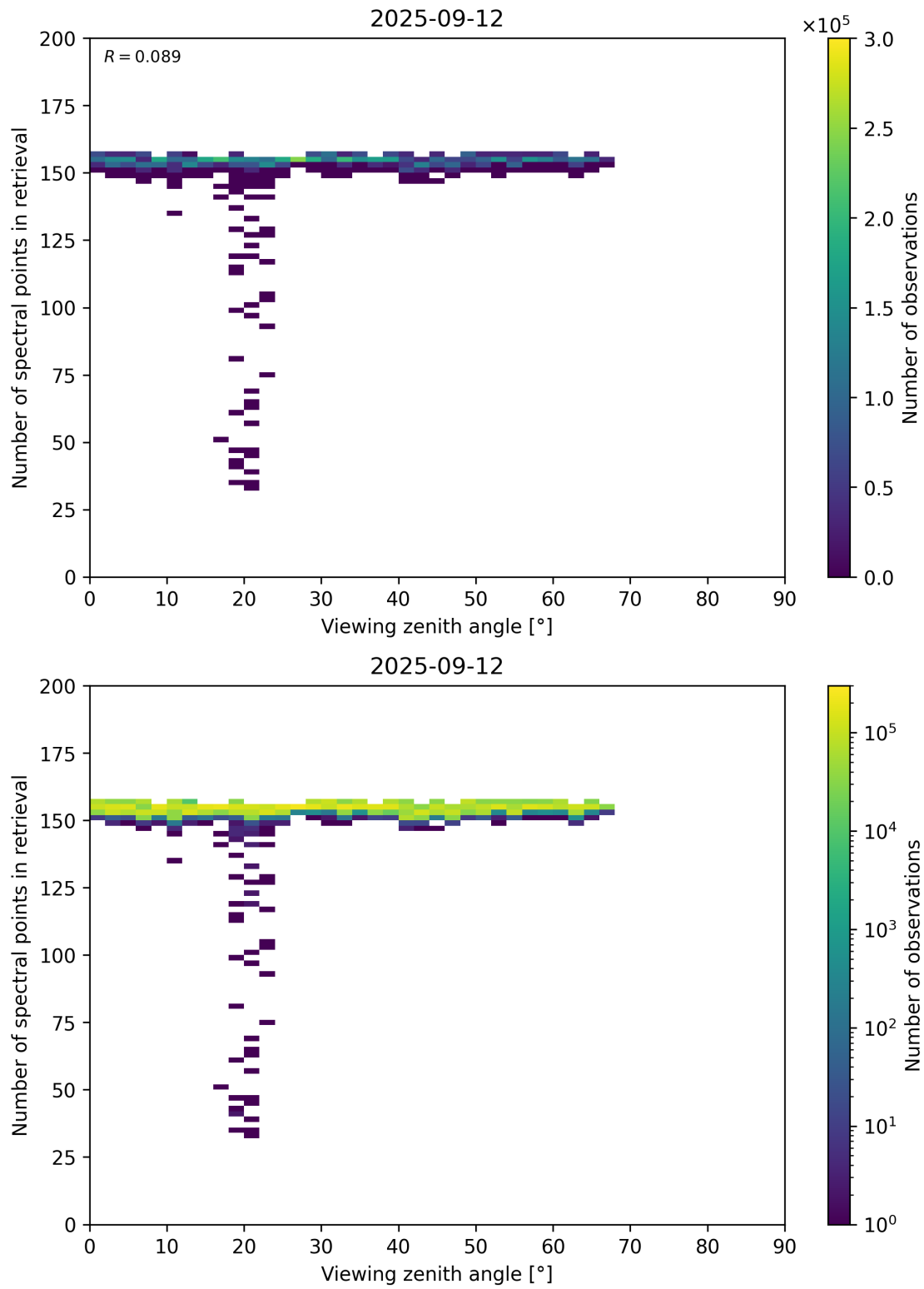
Figure 76: Scatter density plot of “Viewing zenith angle” against “Number of spectral points in retrieval” for 2025-09-11 to 2025-09-13.
