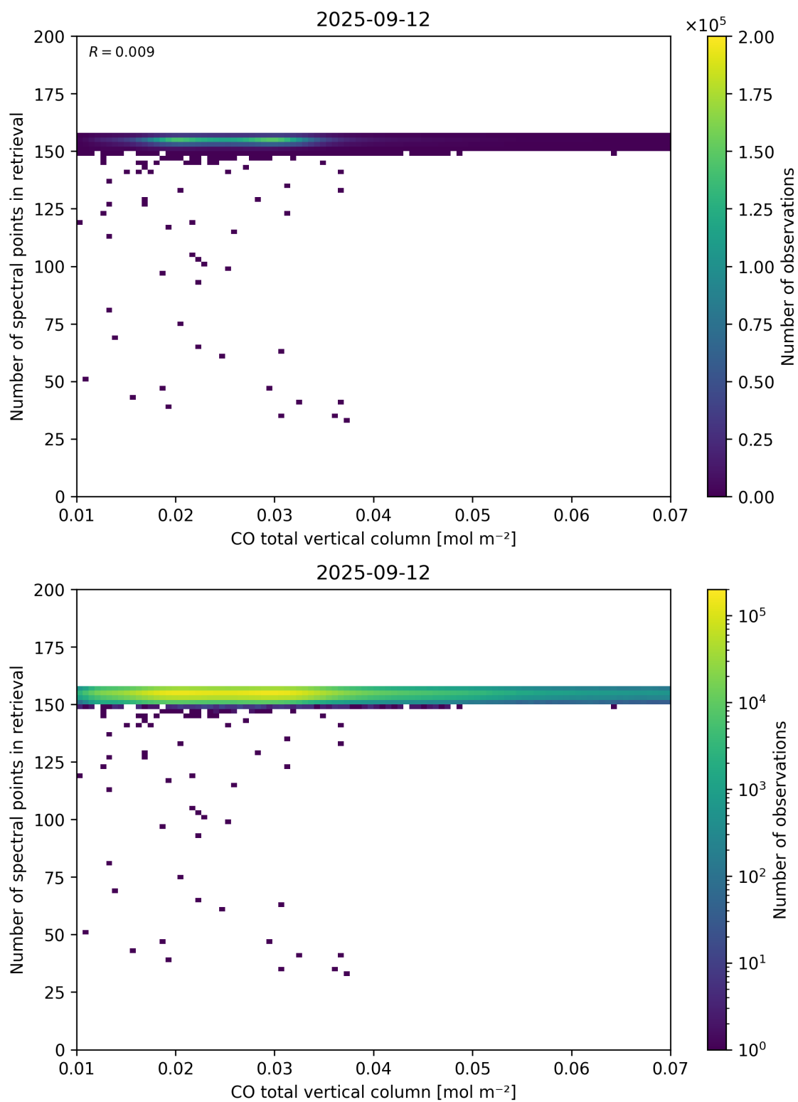
Figure 43: Scatter density plot of “CO total vertical column” against “Number of spectral points in retrieval” for 2025-09-11 to 2025-09-13.
