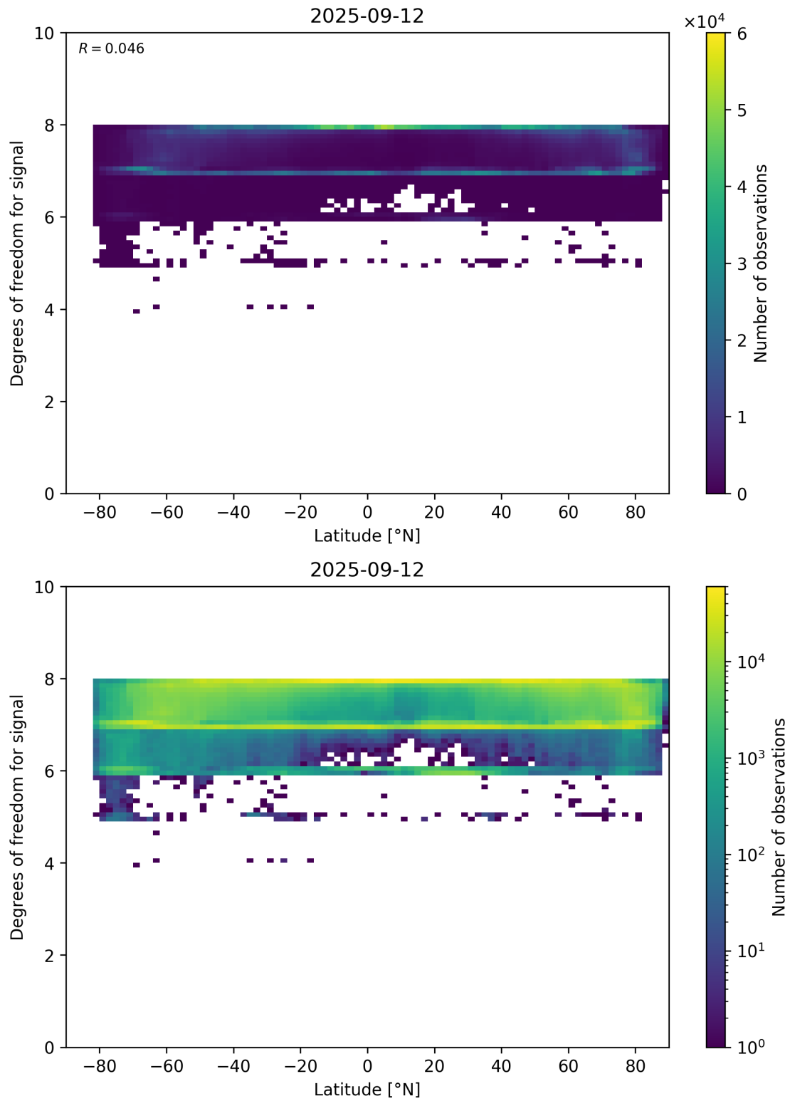
Figure 55: Scatter density plot of “Latitude” against “Degrees of freedom for signal” for 2025-09-11 to 2025-09-13.
