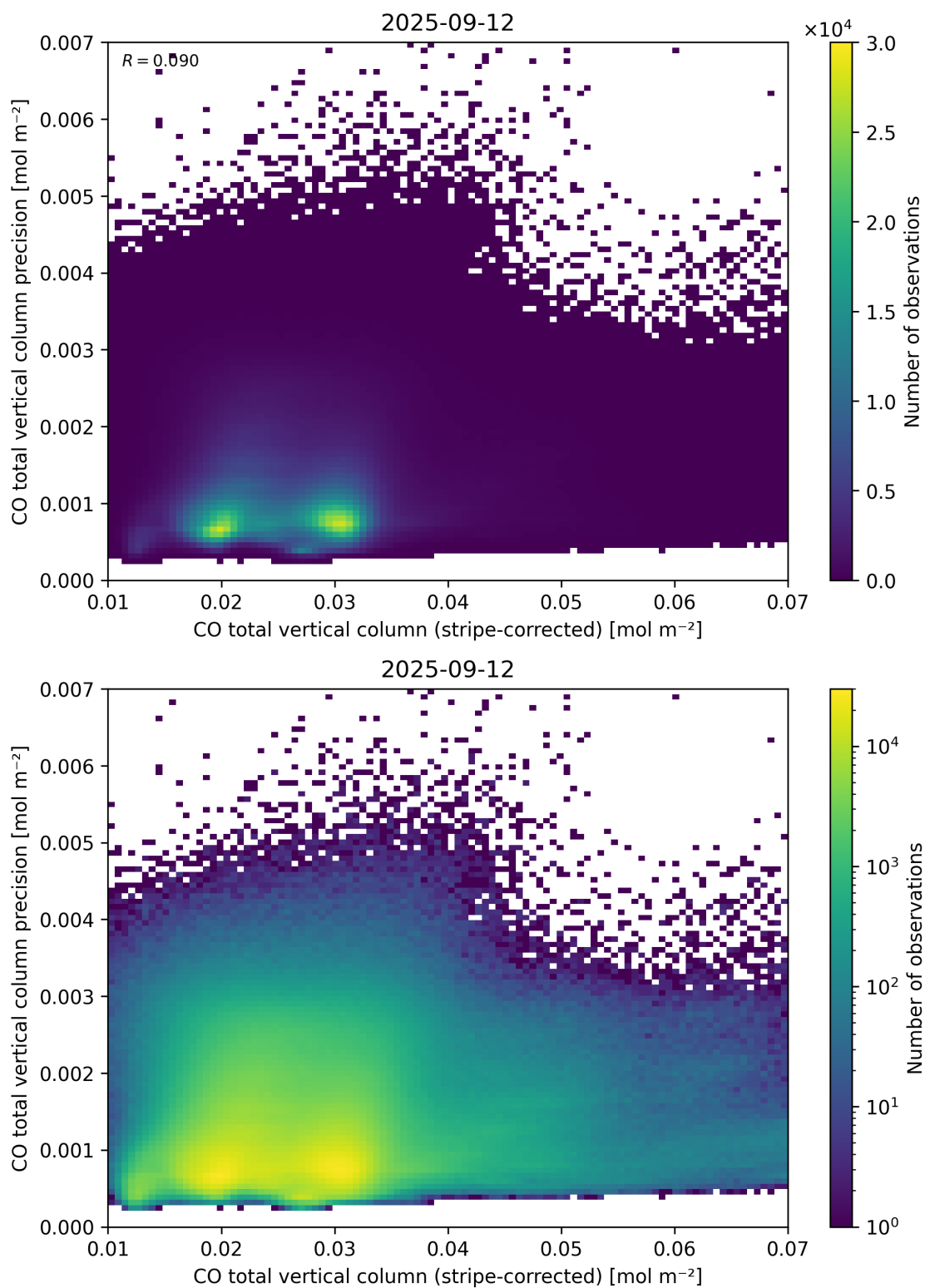
Figure 36: Scatter density plot of “CO total vertical column (stripe-corrected)” against “CO total vertical column precision” for 2025-09-11 to 2025-09-13.
