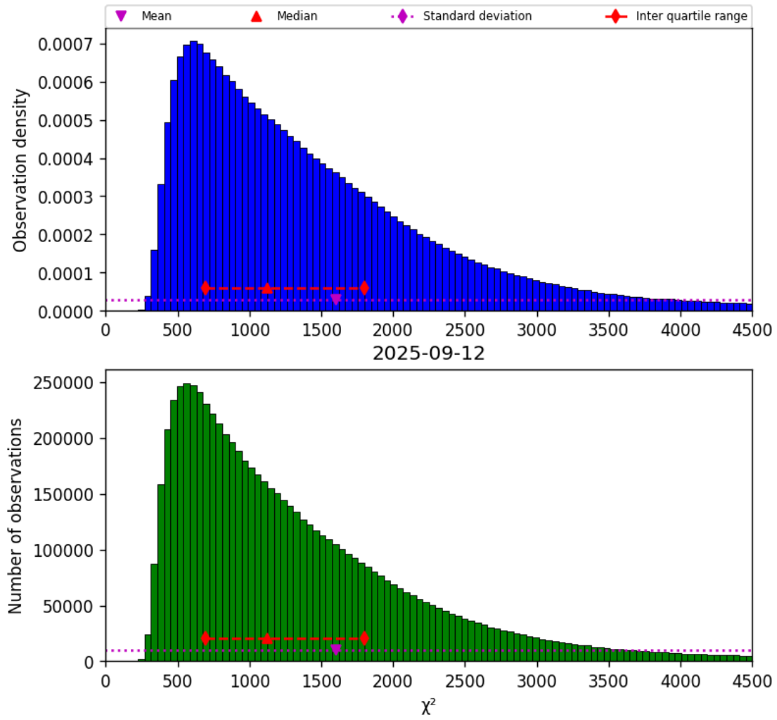
Figure 22: Histogram of “ \chi^2 ” for 2025-09-11 to 2025-09-13
