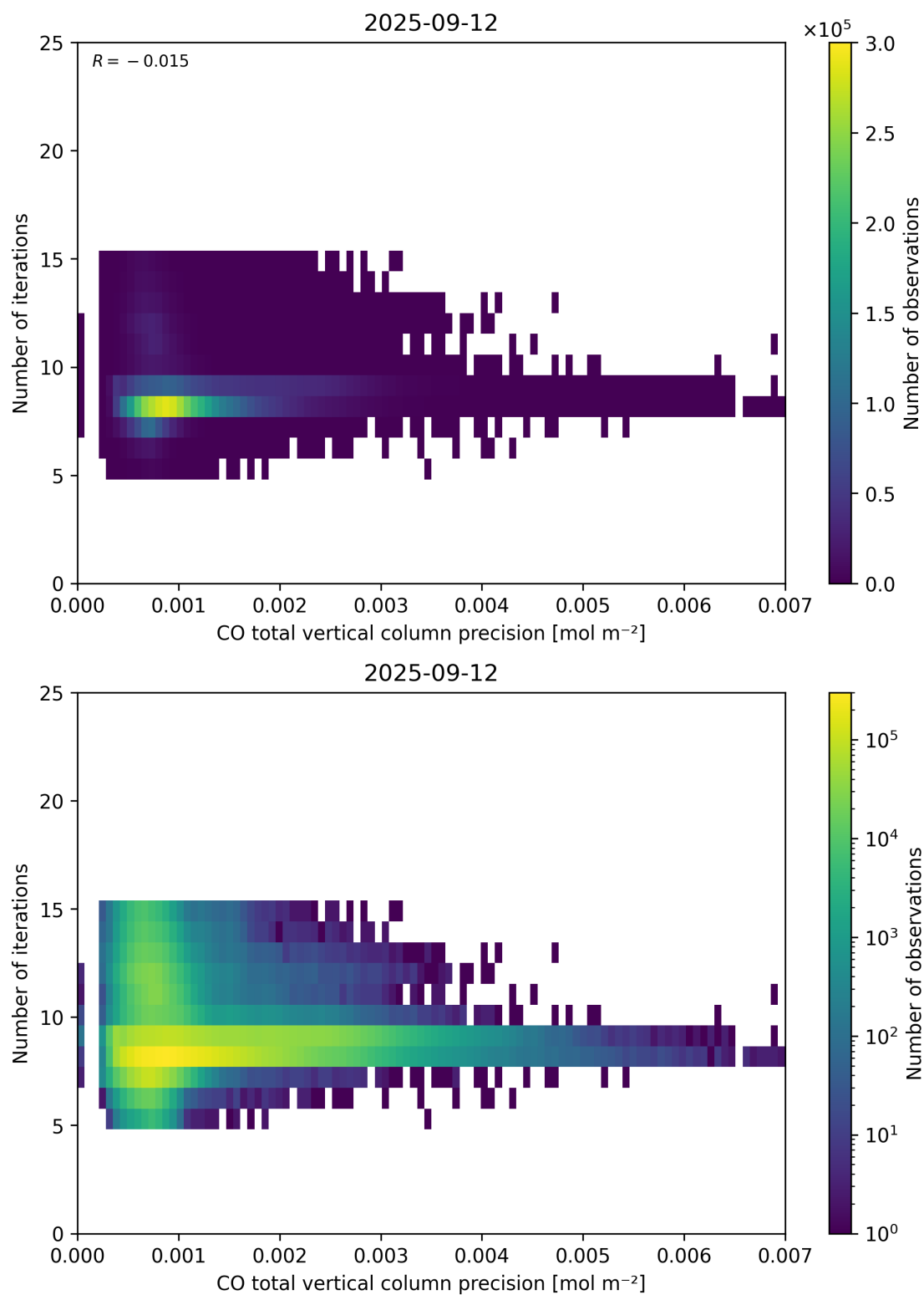
Figure 46: Scatter density plot of “CO total vertical column precision” against “Number of iterations” for 2025-09-11 to 2025-09-13.
