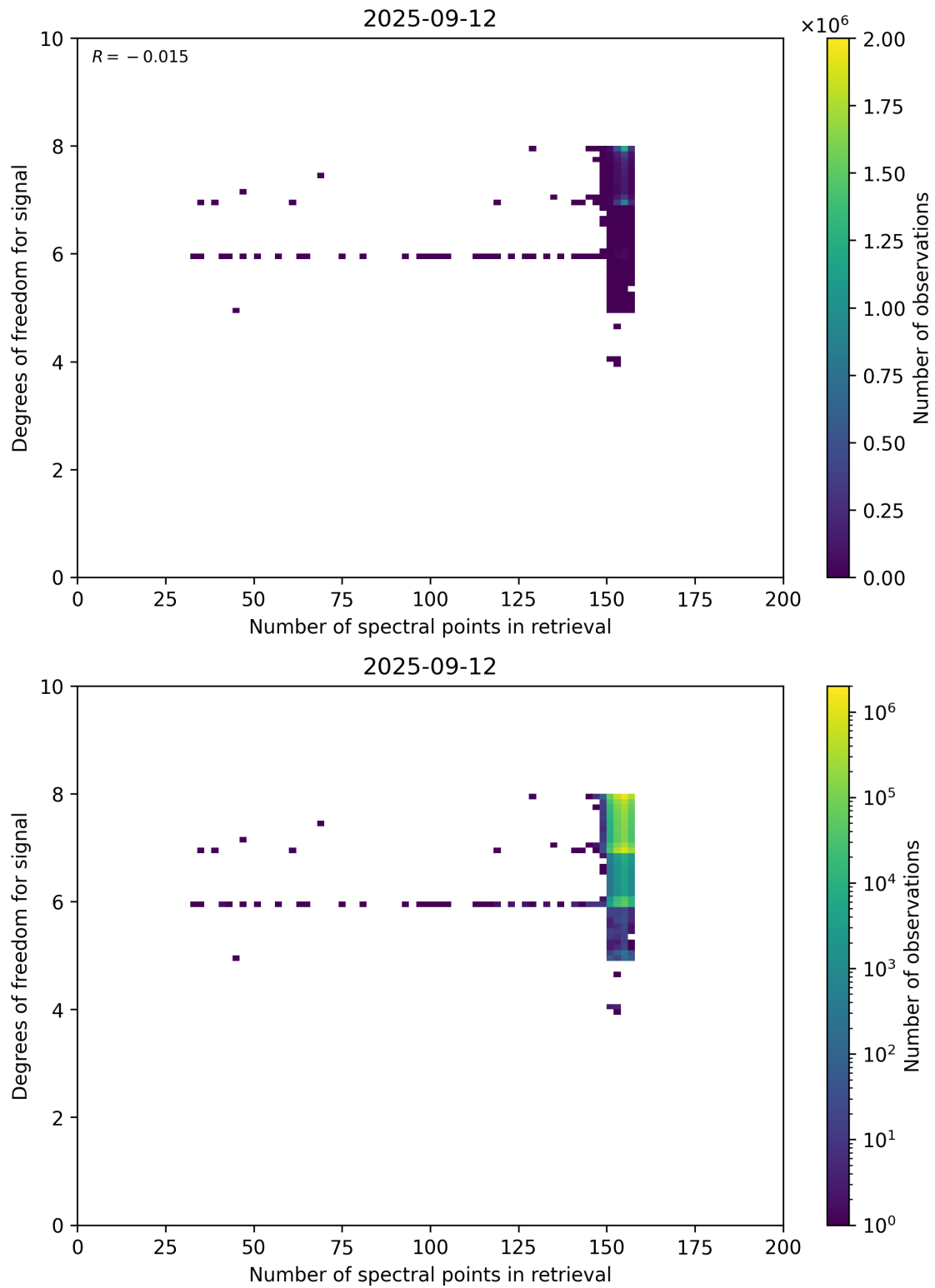
Figure 59: Scatter density plot of “Number of spectral points in retrieval” against “Degrees of freedom for signal” for 2025-09-11 to 2025-09-13.
