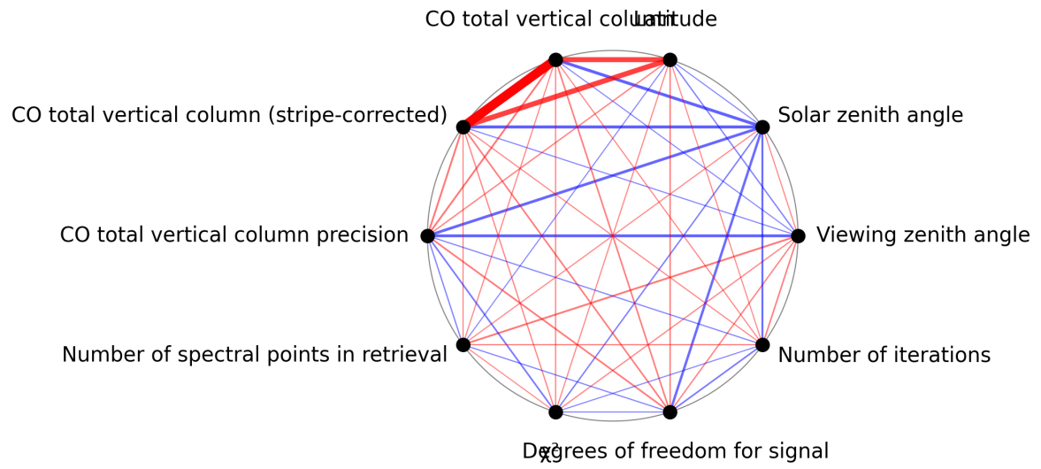
Figure 1: Map of correlation graph for 2025-09-11 to 2025-09-13.
