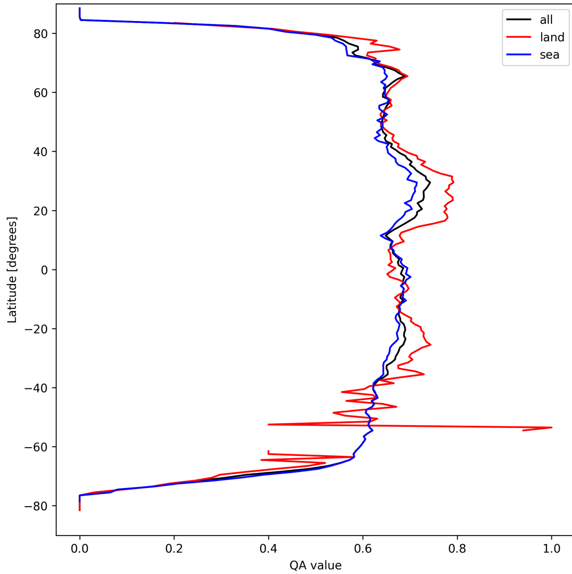
Figure 9: Zonal average of “QA value” for 2025-09-11 to 2025-09-13.
