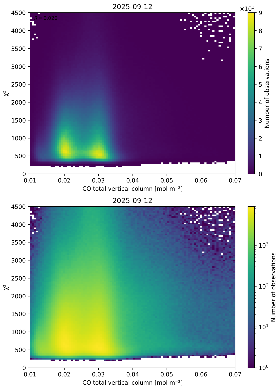
Figure 35: Scatter density plot of “CO total vertical column” against “ \chi^2 ” for 2025-09-11 to 2025-09-13.
