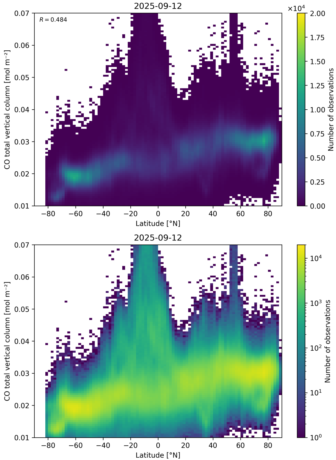
Figure 51: Scatter density plot of “Latitude” against “CO total vertical column” for 2025-09-11 to 2025-09-13.
