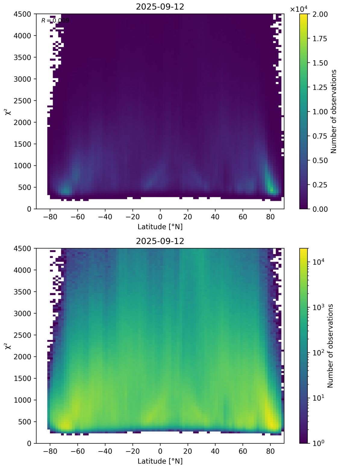
Figure 54: Scatter density plot of “Latitude” against “ \chi^2 ” for 2025-09-11 to 2025-09-13.
