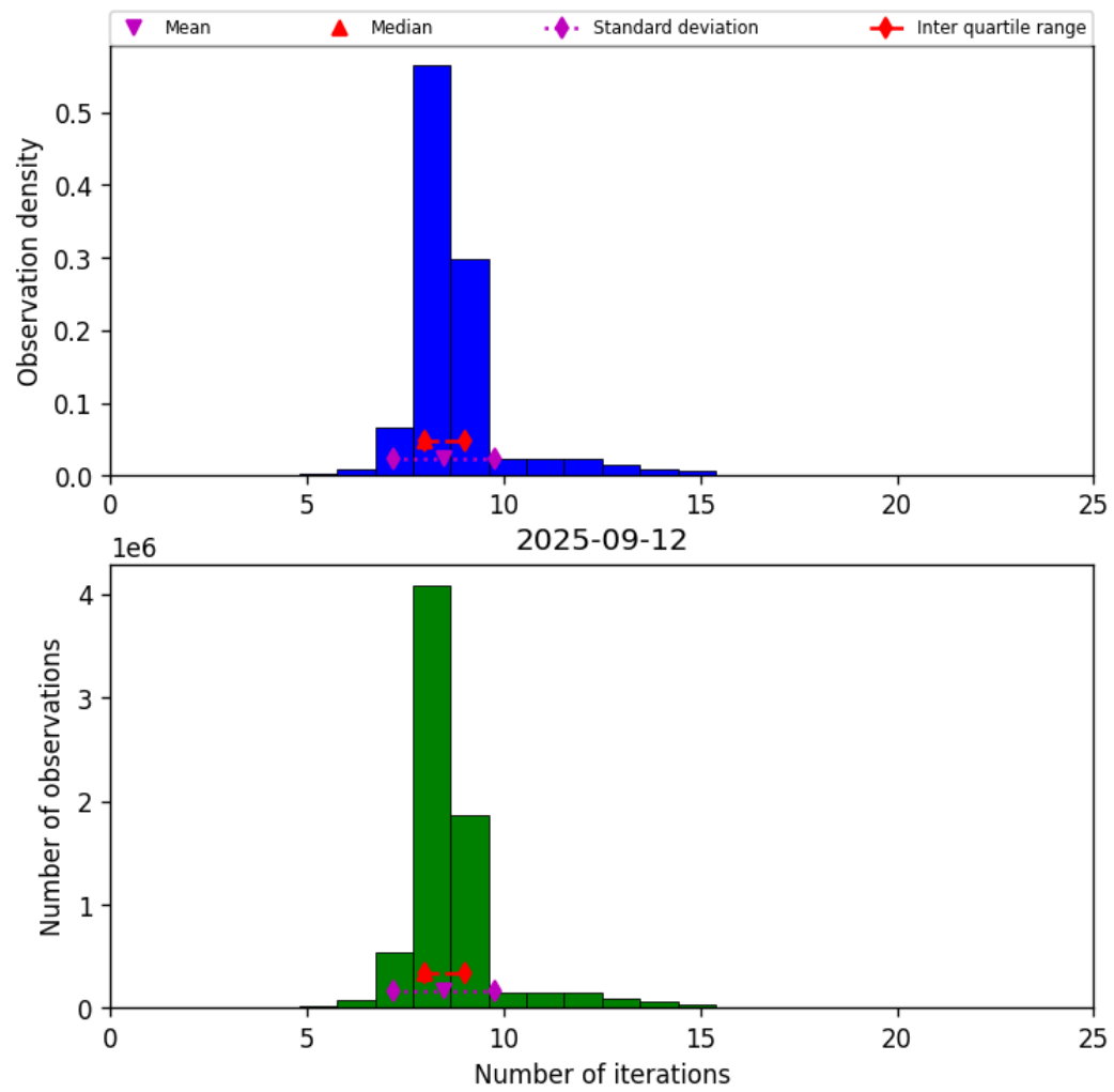
Figure 24: Histogram of “Number of iterations” for 2025-09-11 to 2025-09-13
