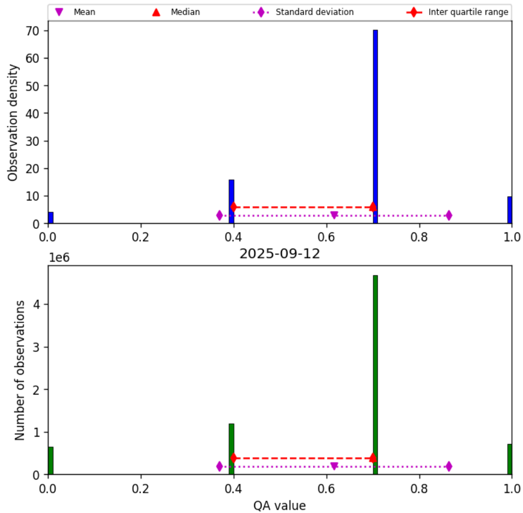
Figure 17: Histogram of “QA value” for 2025-09-11 to 2025-09-13
