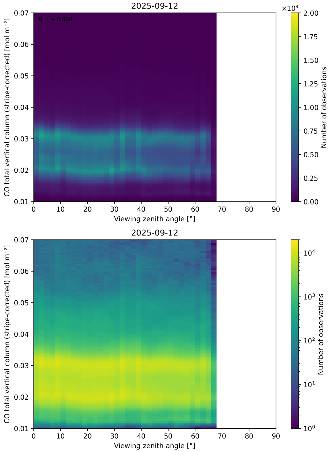
Figure 70: Scatter density plot of “Viewing zenith angle” against “CO total vertical column (stripe-corrected)” for 2025-09-11 to 2025-09-13.
