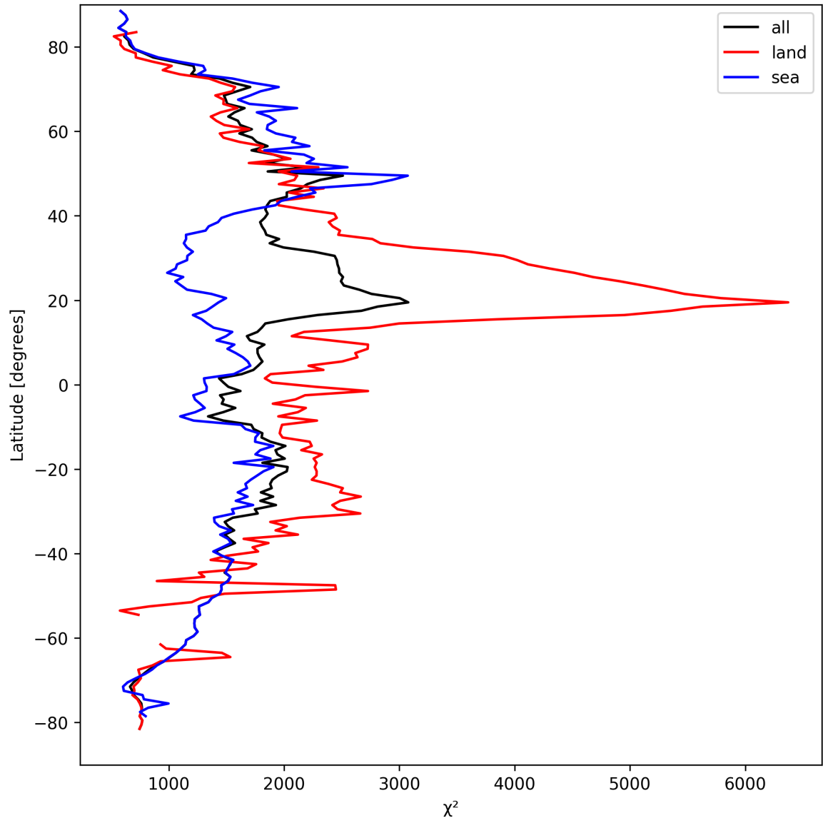
Figure 14: Zonal average of “ \chi^2 ” for 2025-09-11 to 2025-09-13.
