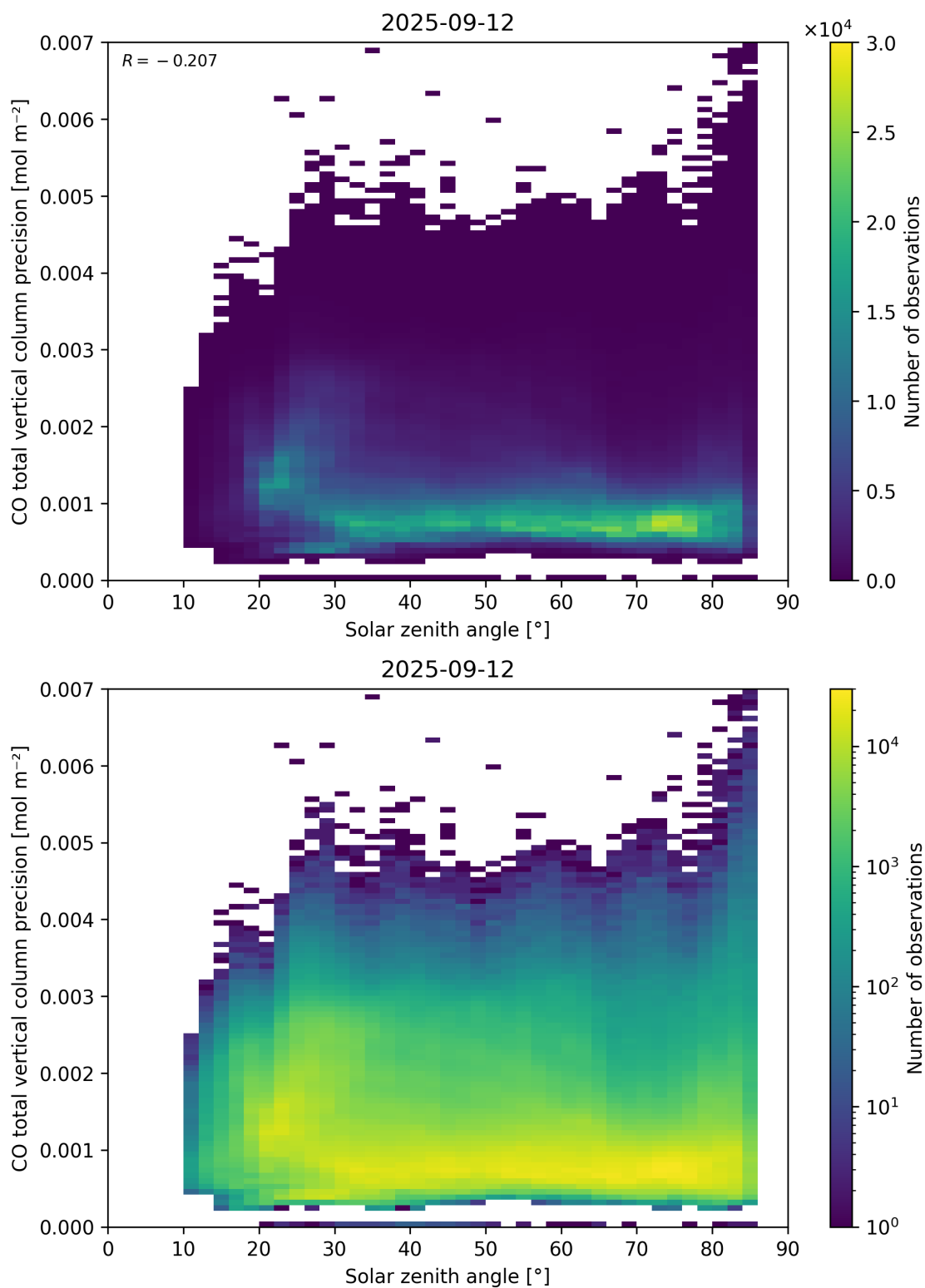
Figure 63: Scatter density plot of “Solar zenith angle” against “CO total vertical column precision” for 2025-09-11 to 2025-09-13.
