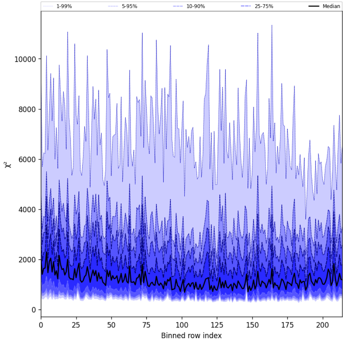
Figure 30: Along track statistics of “ \chi^2 ” for 2025-09-11 to 2025-09-13
