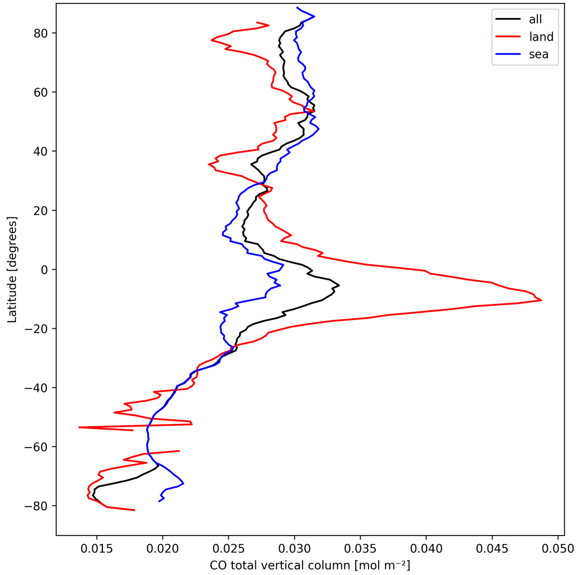
Figure 10: Zonal average of “CO total vertical column” for 2025-09-11 to 2025-09-13.
