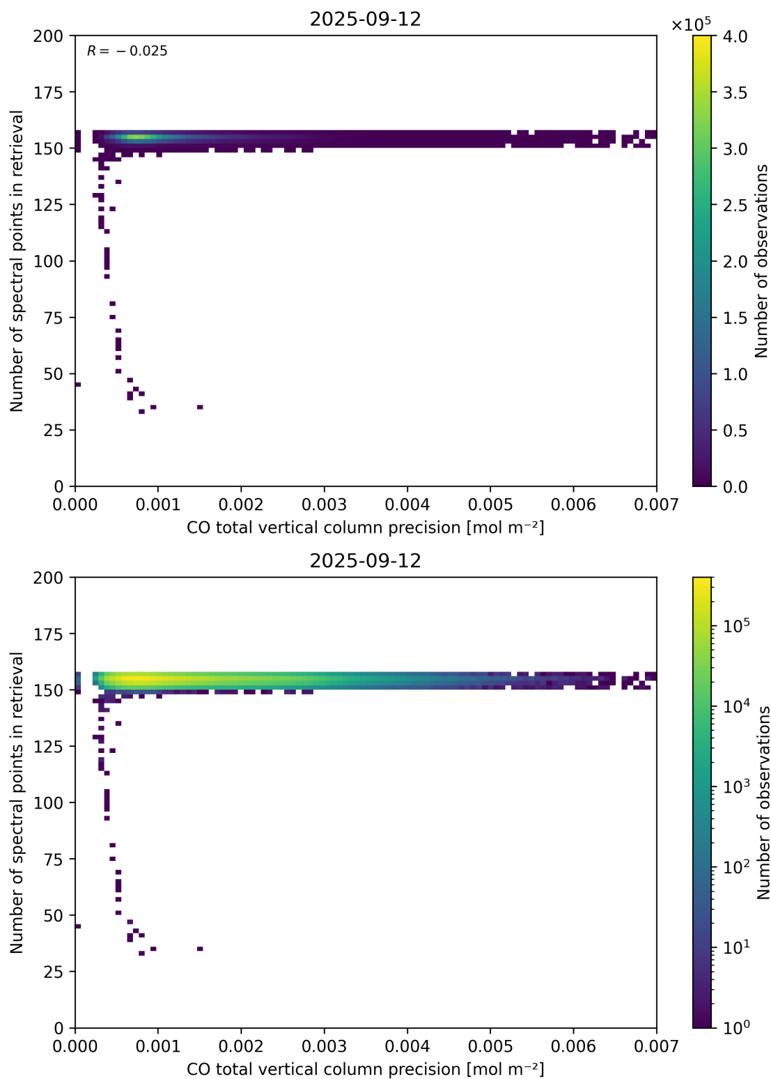
Figure 47: Scatter density plot of “CO total vertical column precision” against “Number of spectral points in retrieval” for 2025-09-11 to 2025-09-13.
