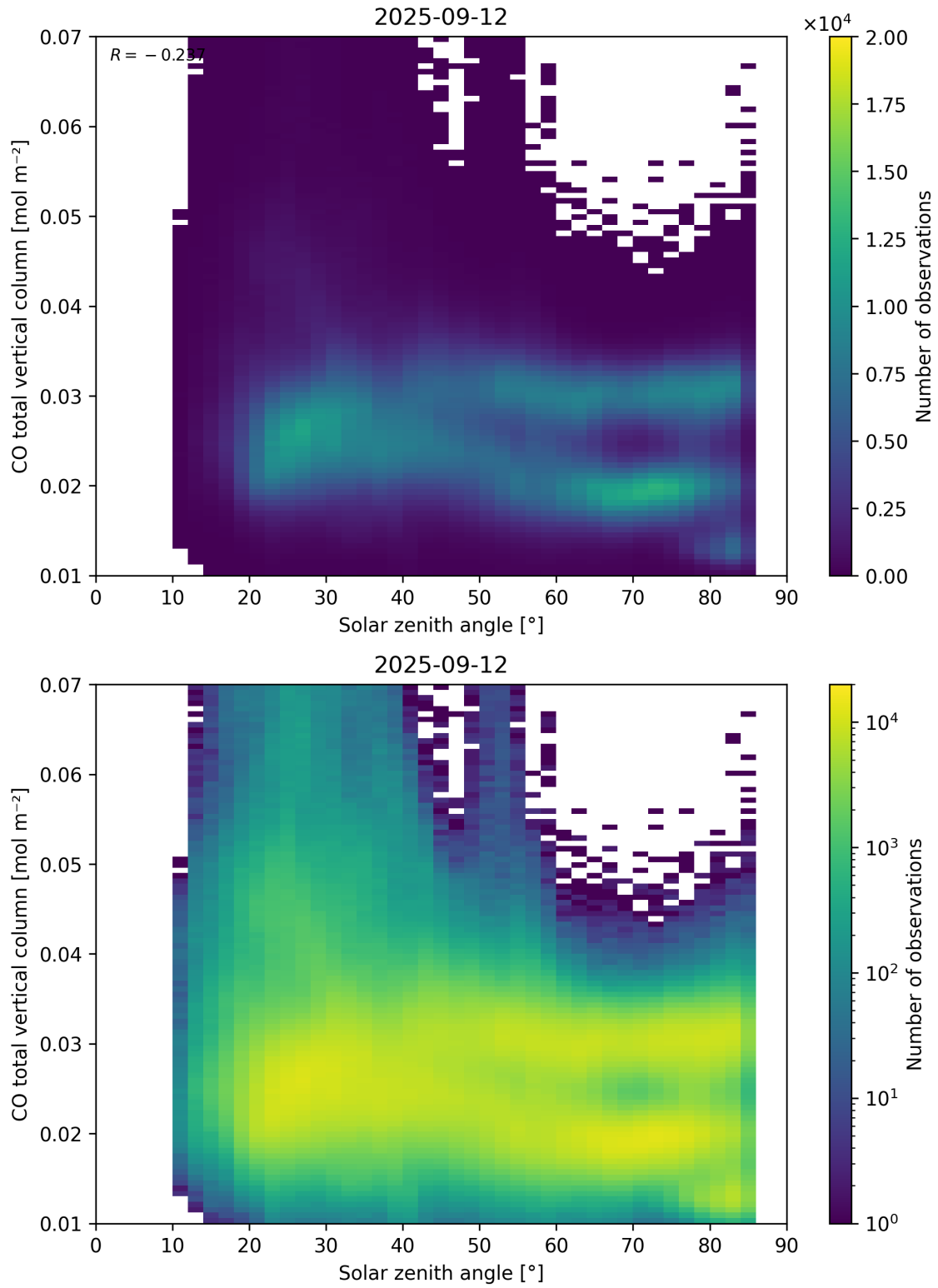
Figure 61: Scatter density plot of “Solar zenith angle” against “CO total vertical column” for 2025-09-11 to 2025-09-13.
