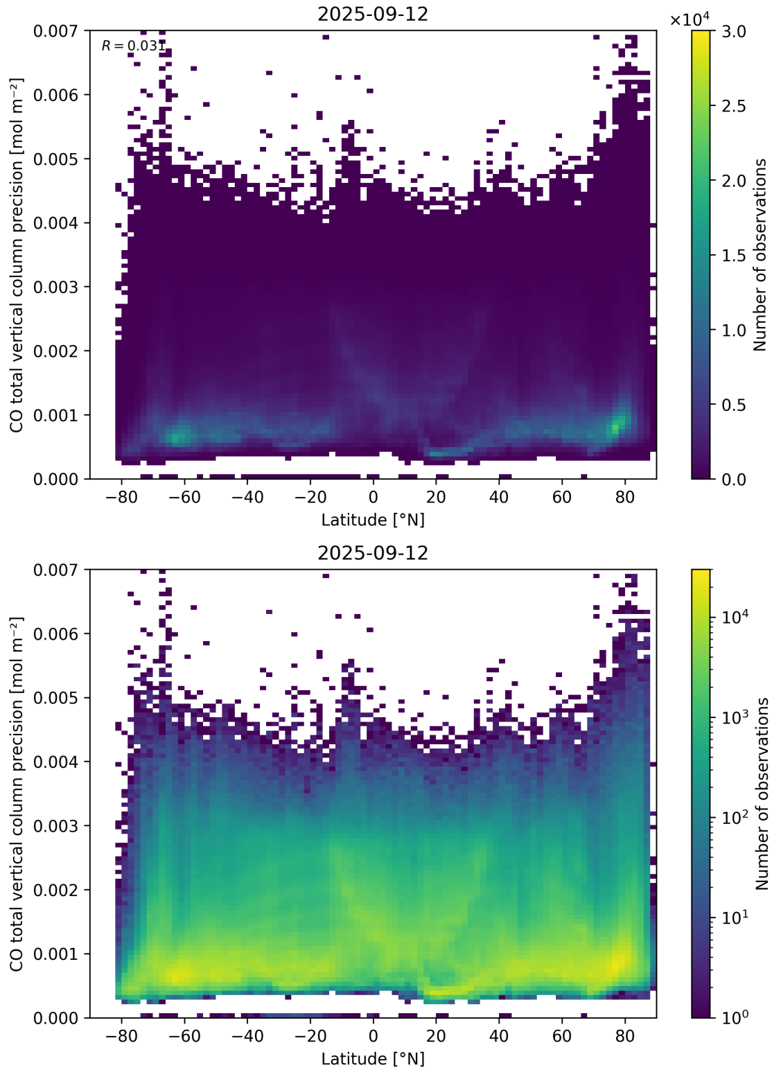
Figure 53: Scatter density plot of “Latitude” against “CO total vertical column precision” for 2025-09-11 to 2025-09-13.
