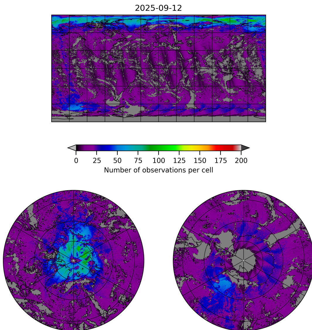
Figure 8: Map of the number of observations for 2025-09-11 to 2025-09-13
