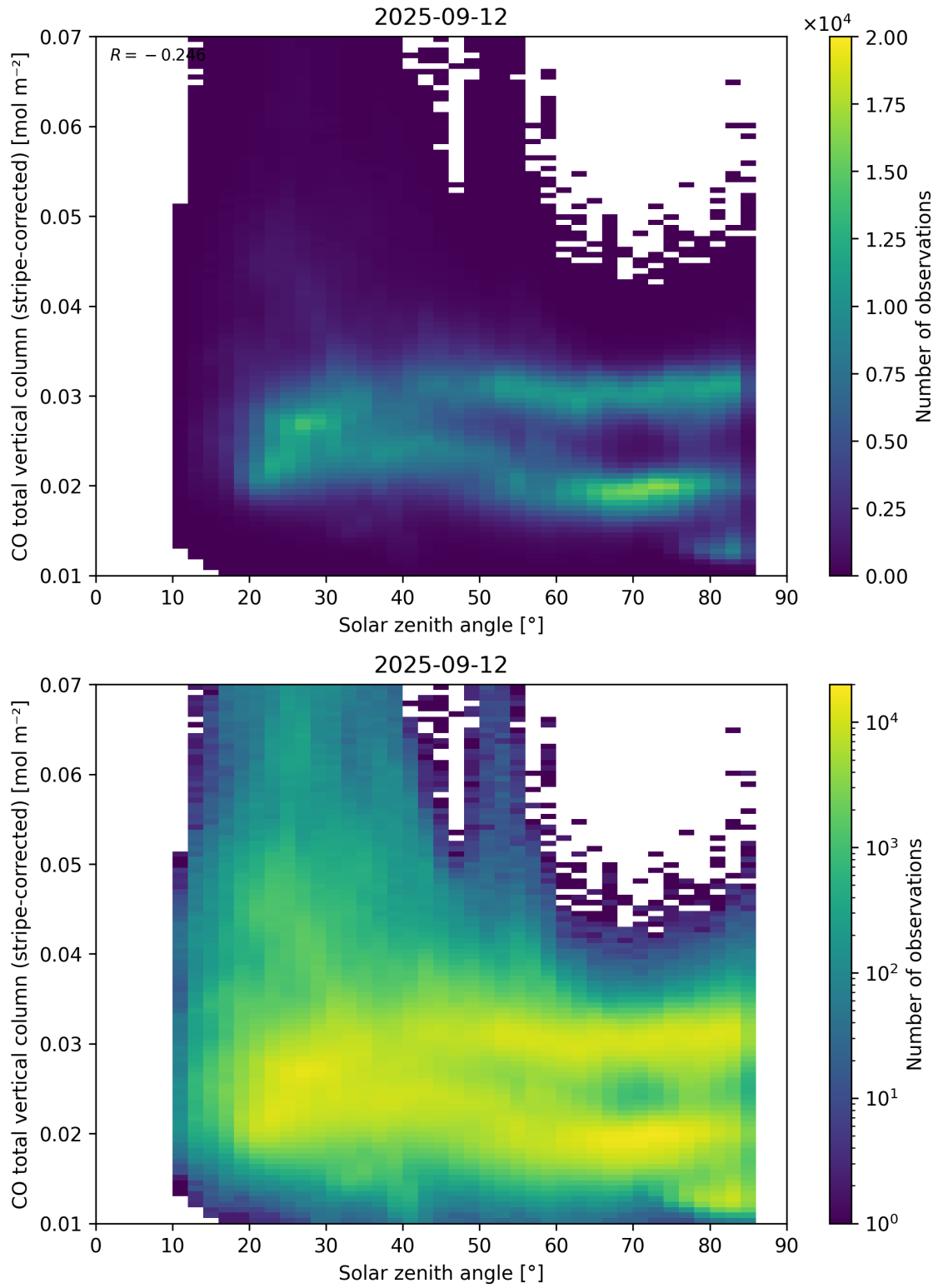
Figure 62: Scatter density plot of “Solar zenith angle” against “CO total vertical column (stripe-corrected)” for 2025-09-11 to 2025-09-13.
