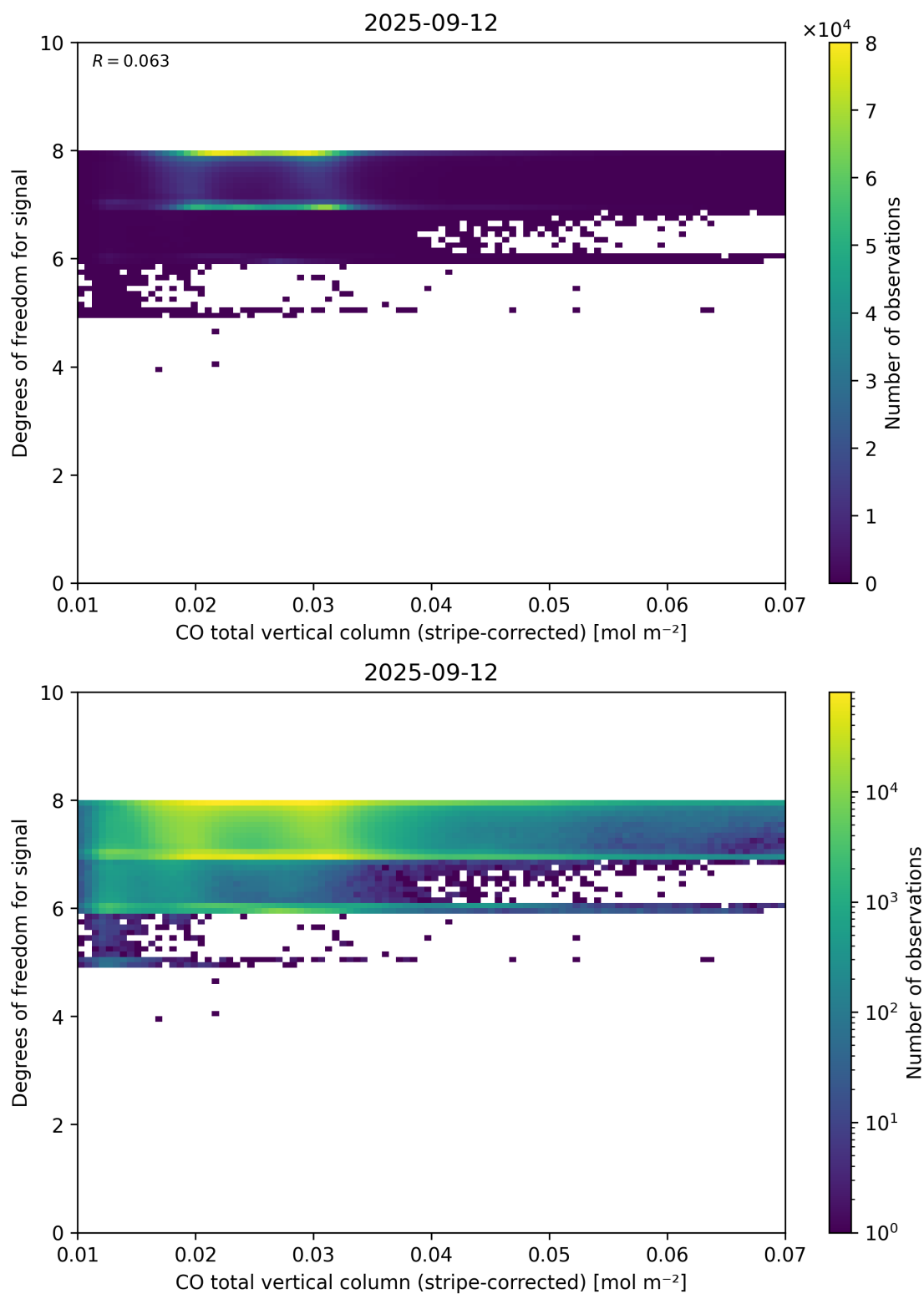
Figure 38: Scatter density plot of “CO total vertical column (stripe-corrected)” against “Degrees of freedom for signal” for 2025-09-11 to 2025-09-13.
