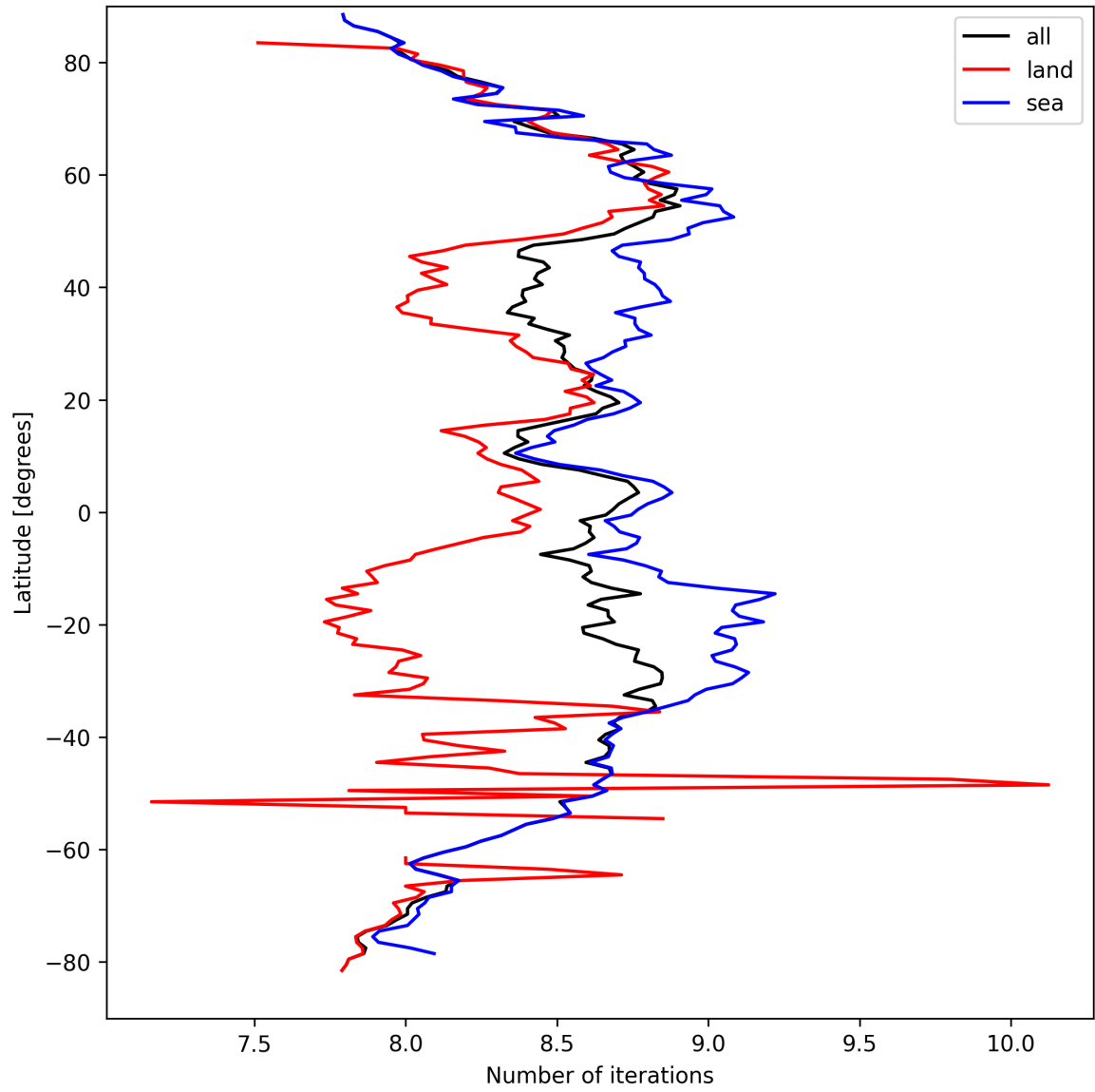
Figure 16: Zonal average of “Number of iterations” for 2025-09-11 to 2025-09-13.
