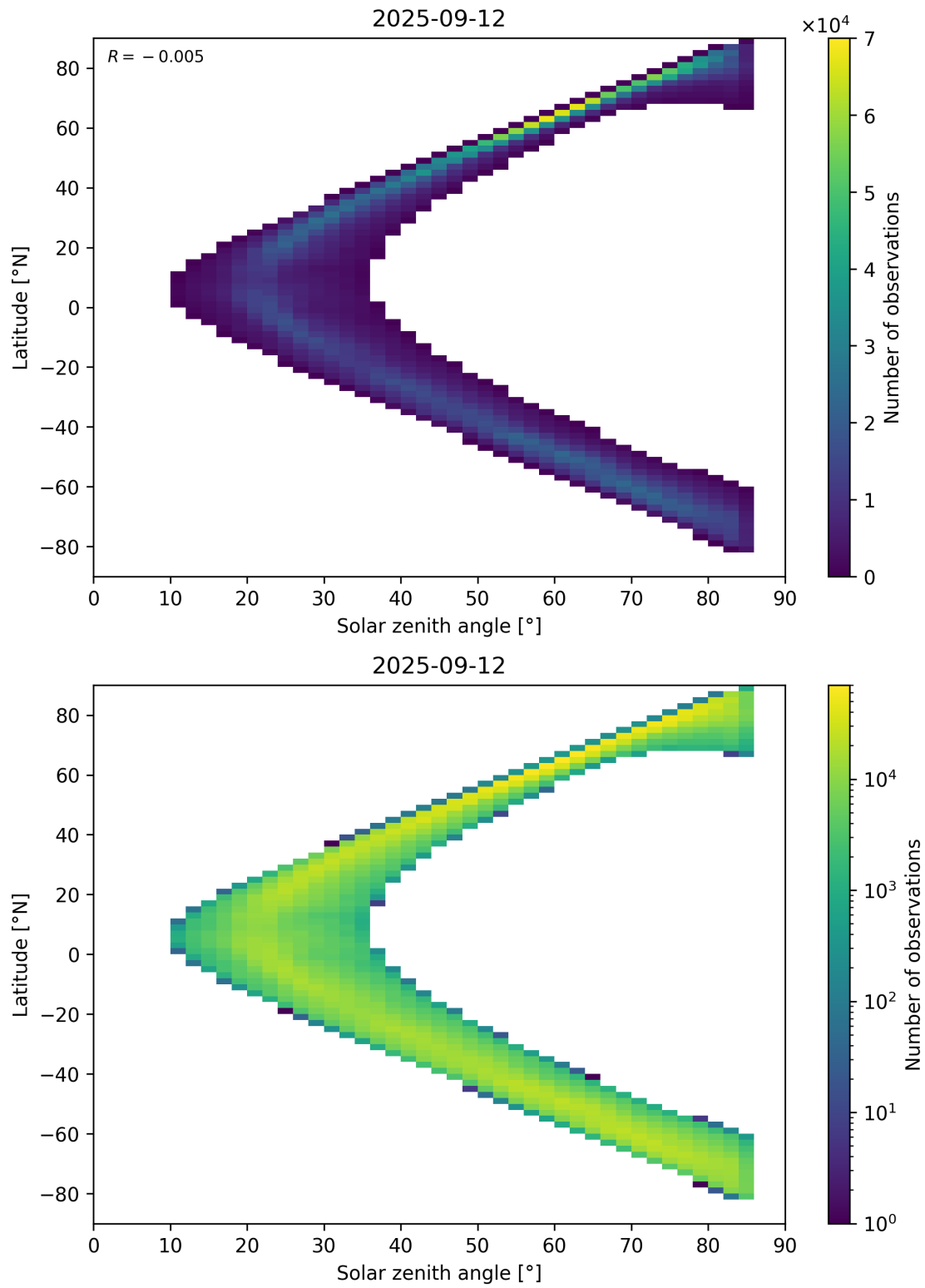
Figure 66: Scatter density plot of “Solar zenith angle” against “Latitude” for 2025-09-11 to 2025-09-13.
