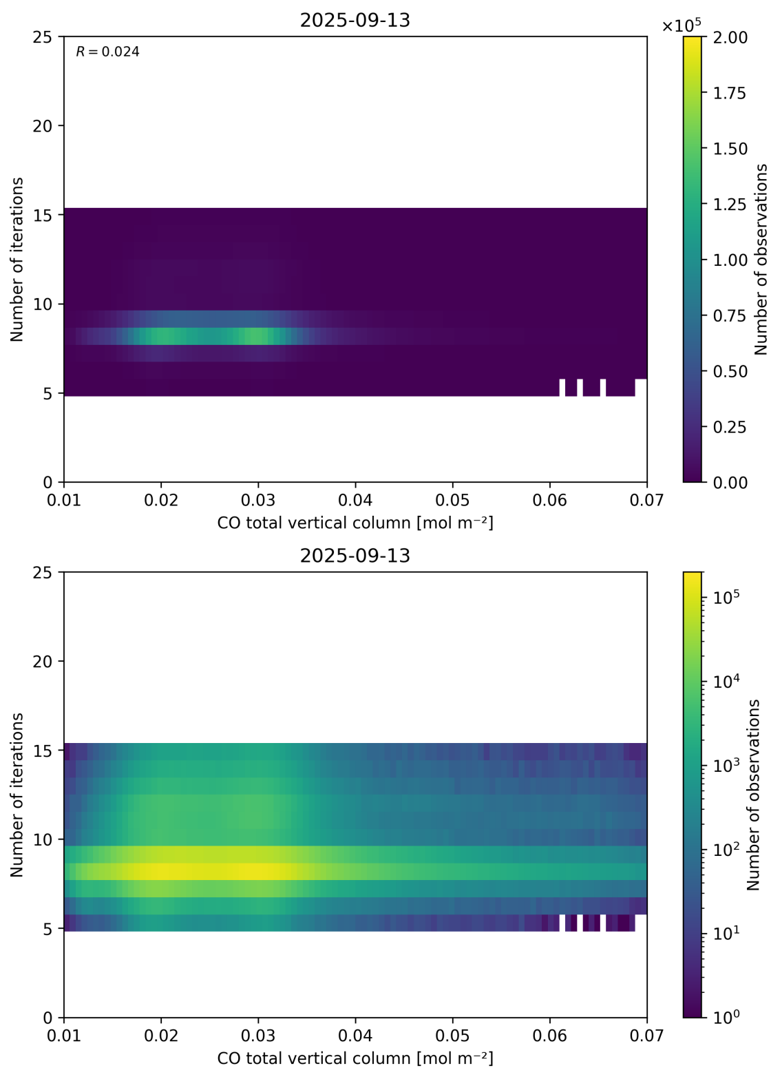
Figure 42: Scatter density plot of “CO total vertical column” against “Number of iterations” for 2025-09-12 to 2025-09-14.
