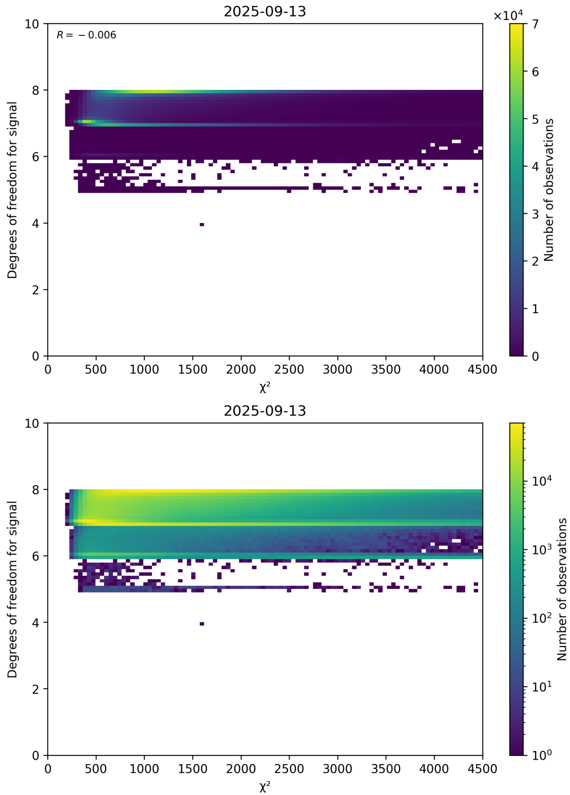
Figure 48: Scatter density plot of “ \chi^2 ” against “Degrees of freedom for signal” for 2025-09-12 to 2025-09-14.
