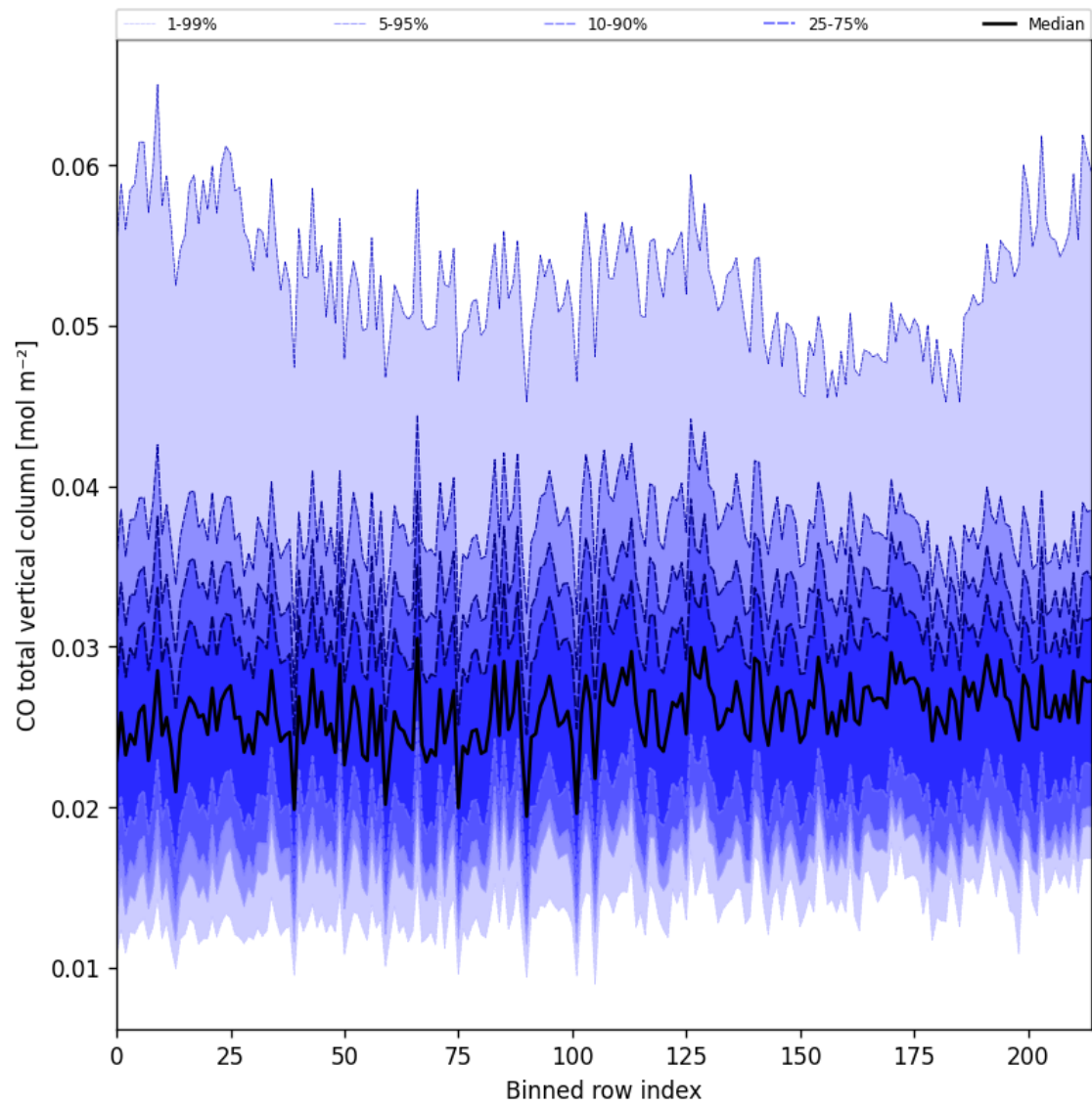
Figure 26: Along track statistics of “CO total vertical column” for 2025-09-12 to 2025-09-14
