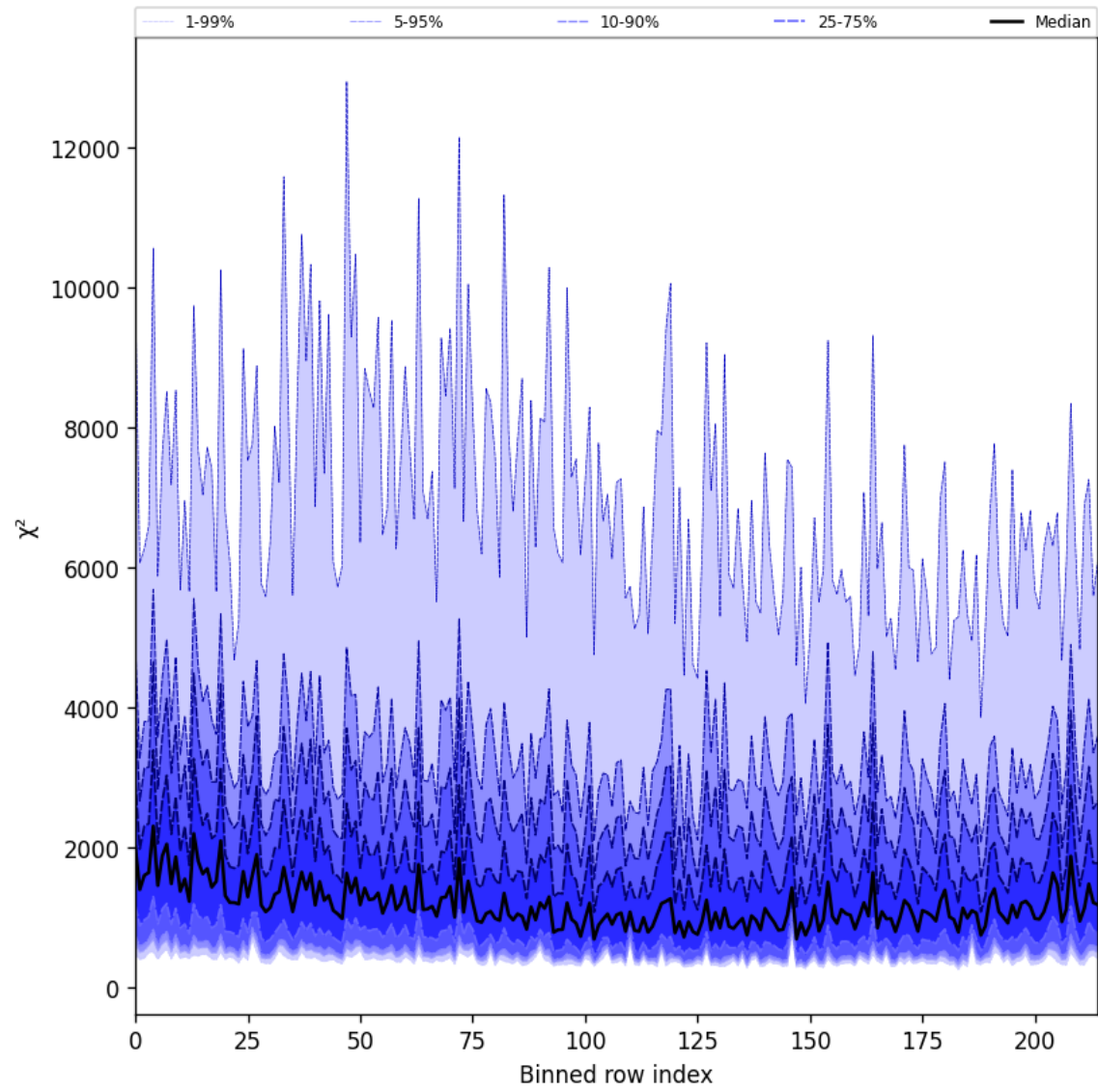
Figure 30: Along track statistics of “ \chi^2 ” for 2025-09-12 to 2025-09-14
