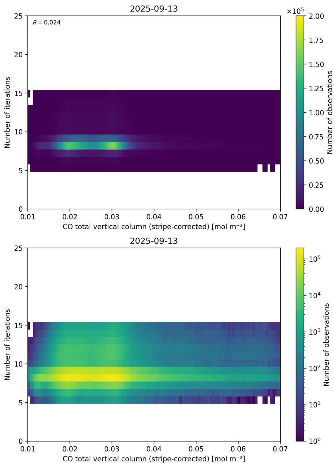
Figure 39: Scatter density plot of “CO total vertical column (stripe-corrected)” against “Number of iterations” for 2025-09-12 to 2025-09-14.
