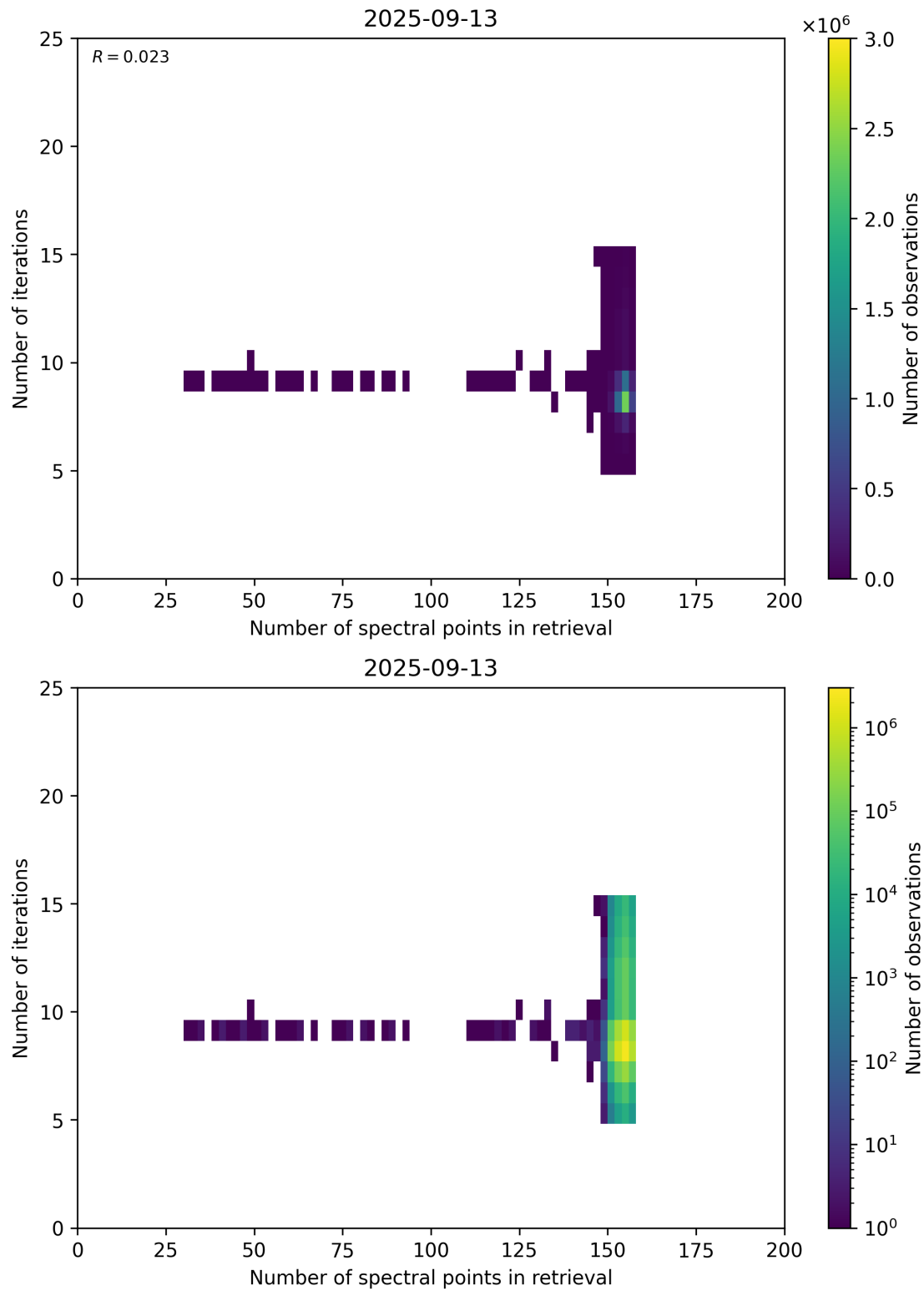
Figure 60: Scatter density plot of “Number of spectral points in retrieval” against “Number of iterations” for 2025-09-12 to 2025-09-14.
