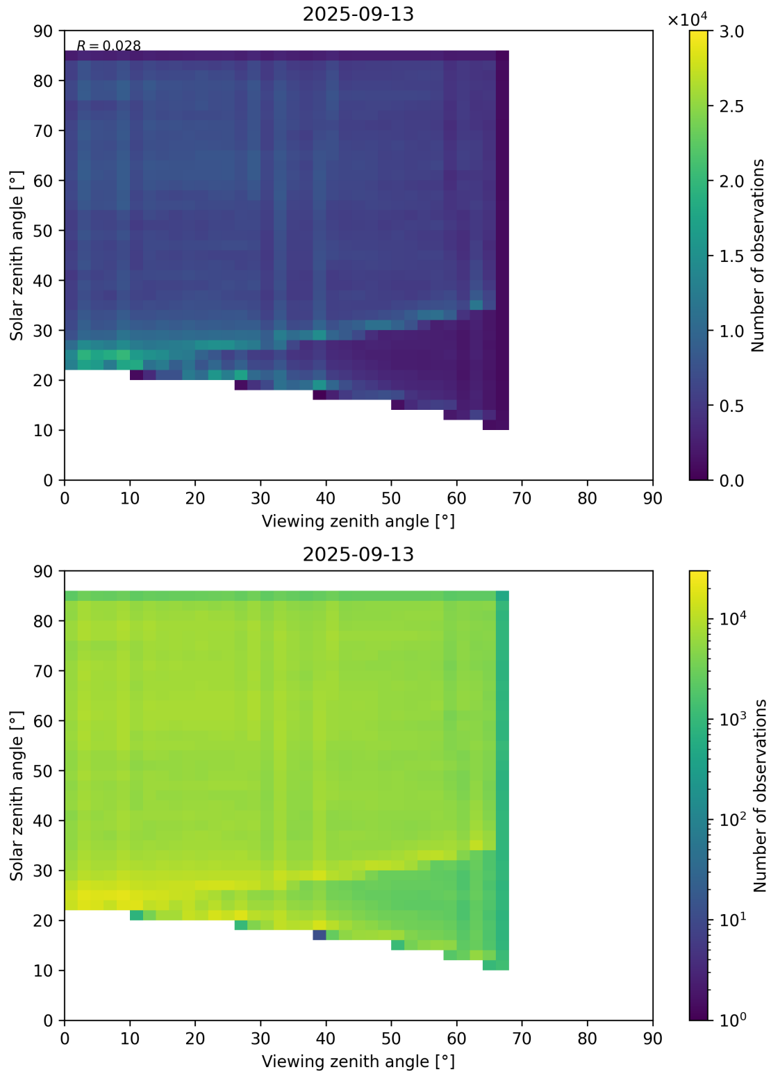
Figure 77: Scatter density plot of “Viewing zenith angle” against “Solar zenith angle” for 2025-09-12 to 2025-09-14.
