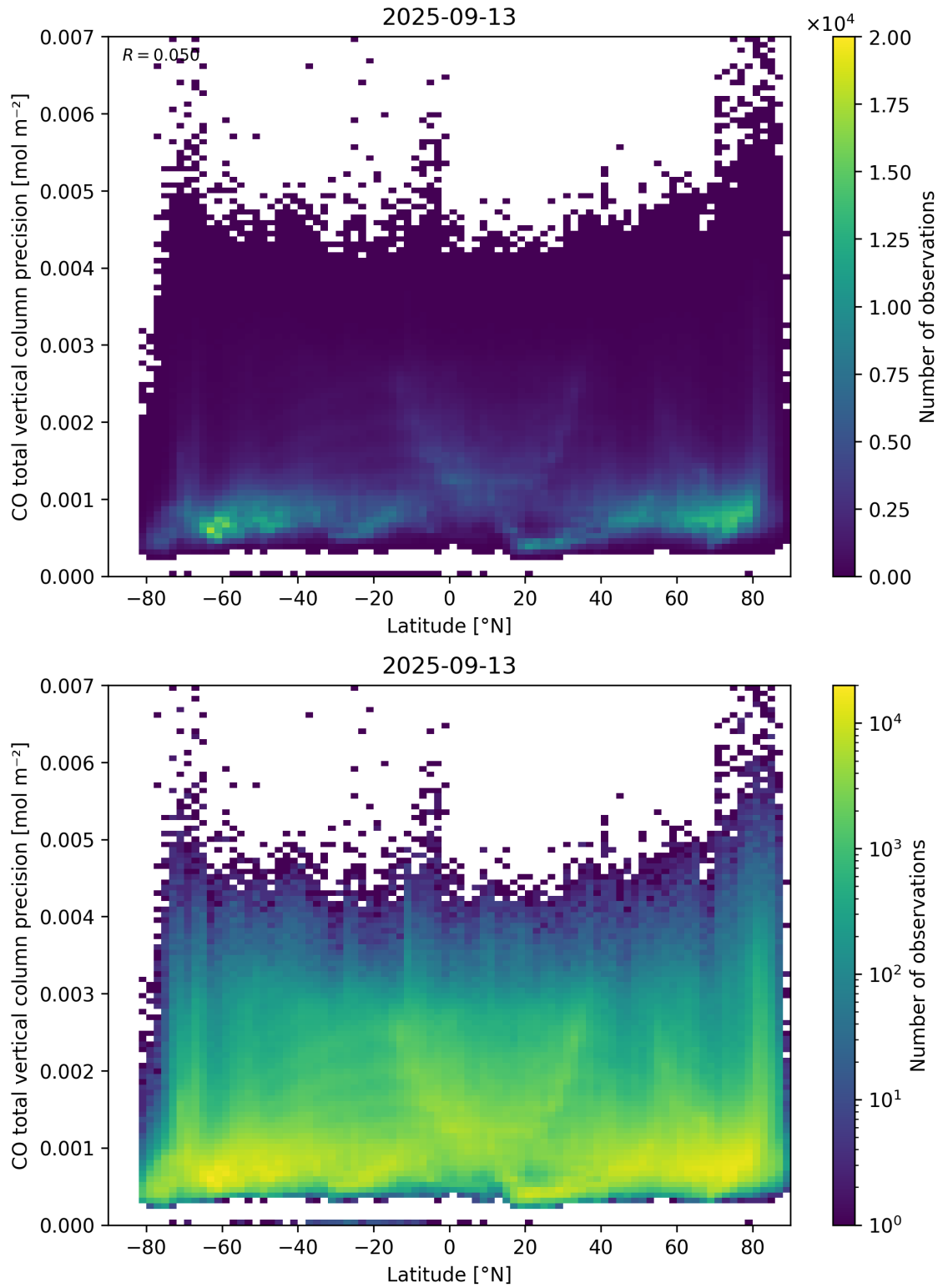
Figure 53: Scatter density plot of “Latitude” against “CO total vertical column precision” for 2025-09-12 to 2025-09-14.
