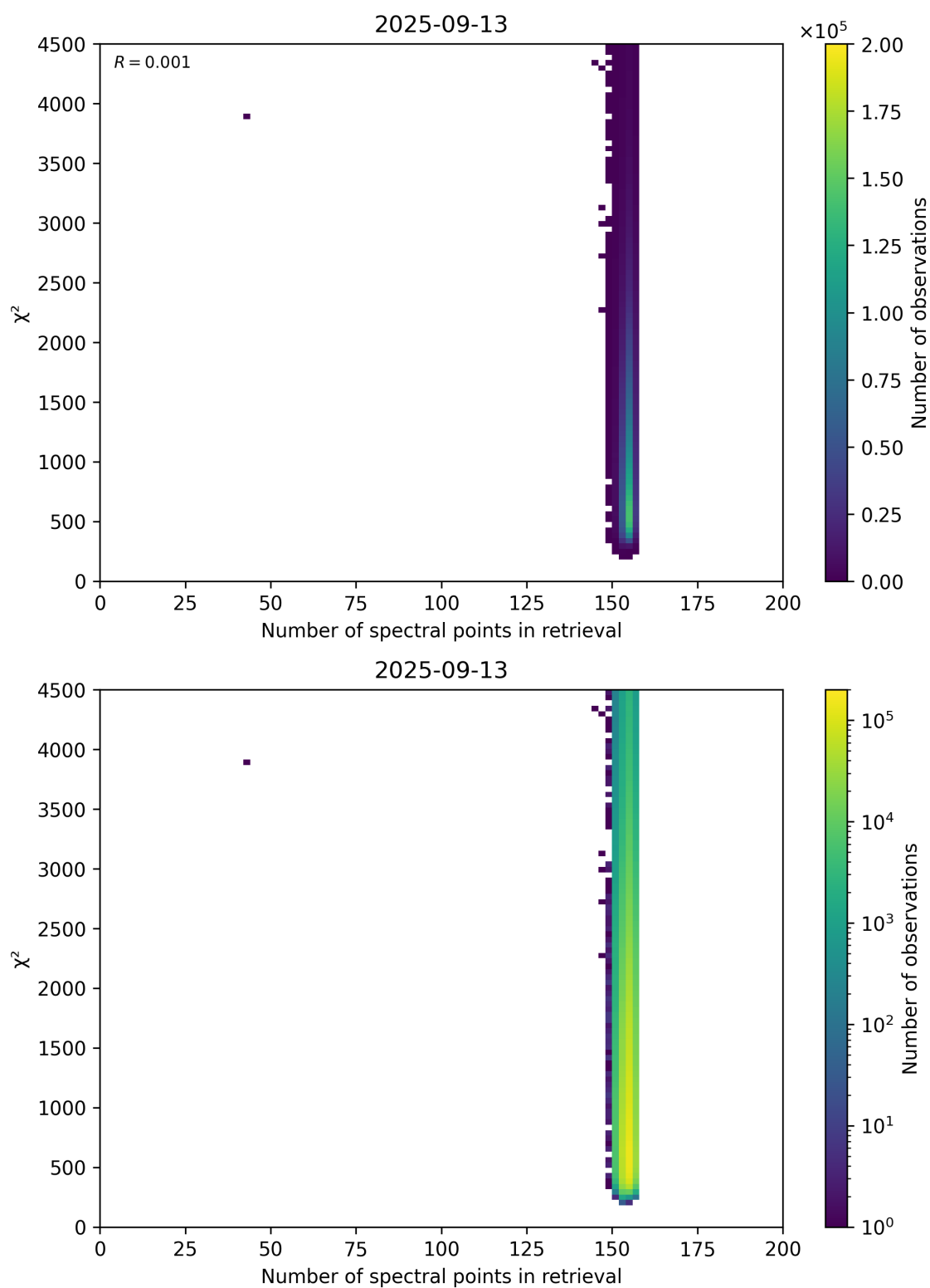
Figure 58: Scatter density plot of “Number of spectral points in retrieval” against “ \chi^2 ” for 2025-09-12 to 2025-09-14.
