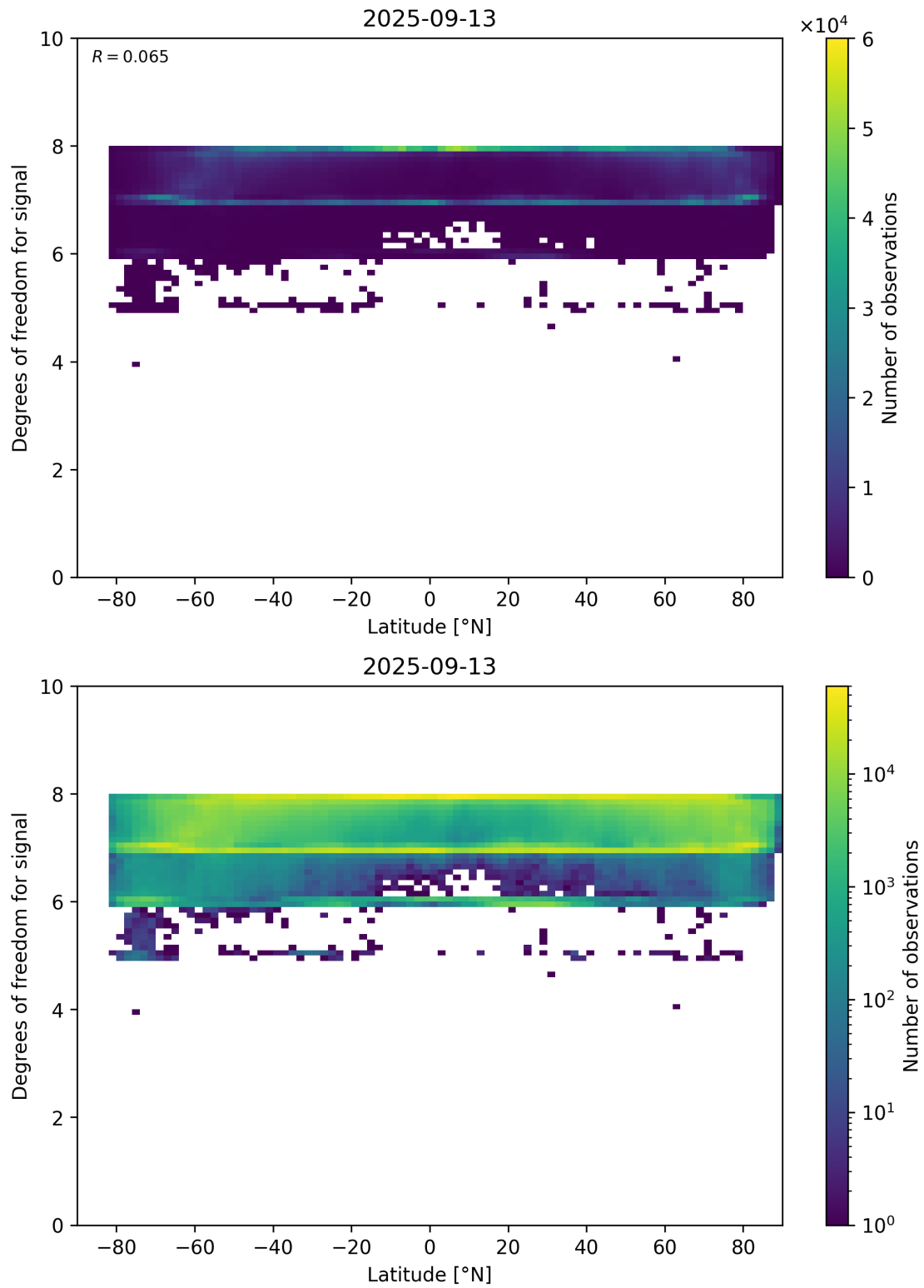
Figure 55: Scatter density plot of “Latitude” against “Degrees of freedom for signal” for 2025-09-12 to 2025-09-14.
