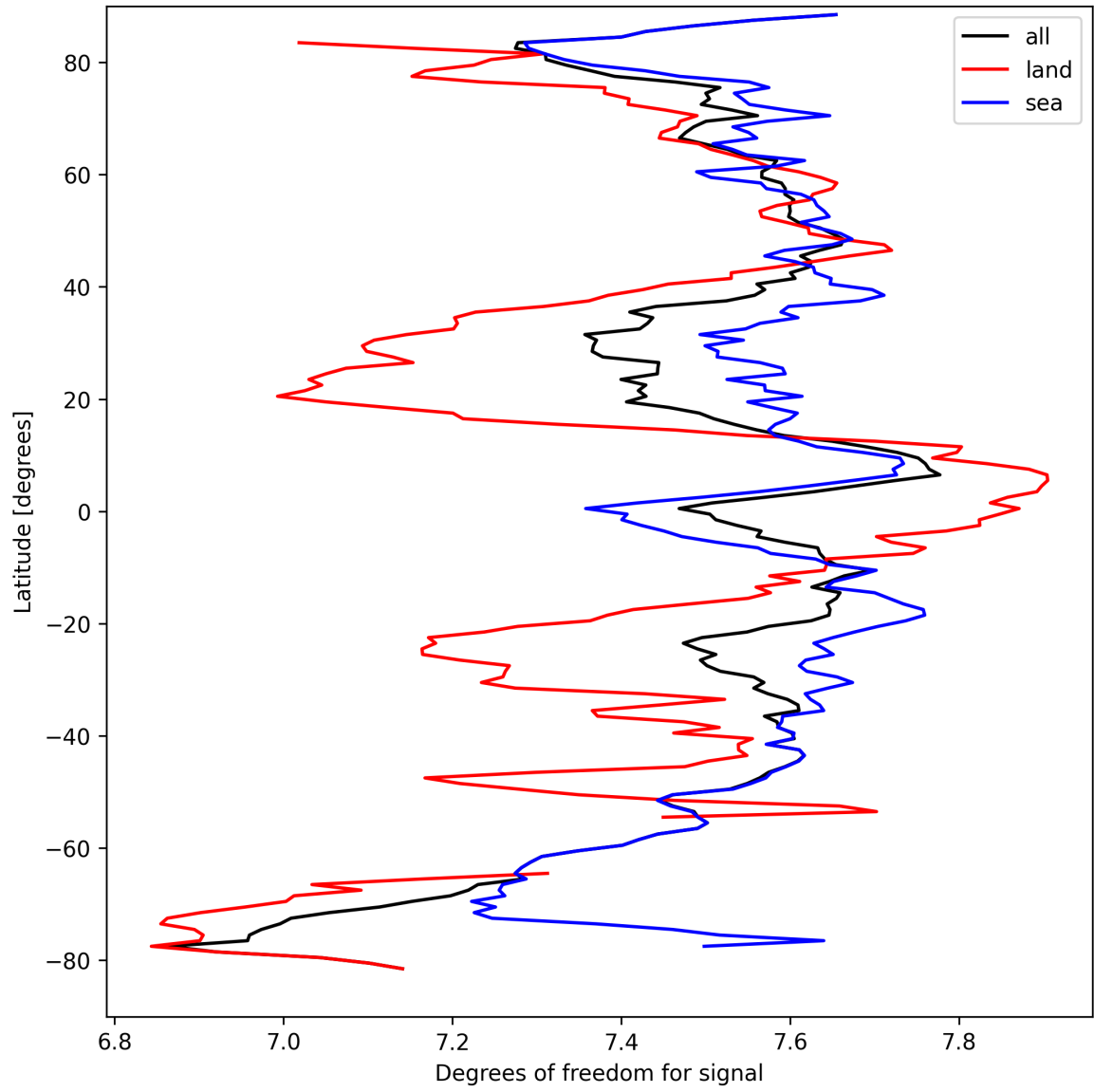
Figure 15: Zonal average of “Degrees of freedom for signal” for 2025-09-12 to 2025-09-14.
