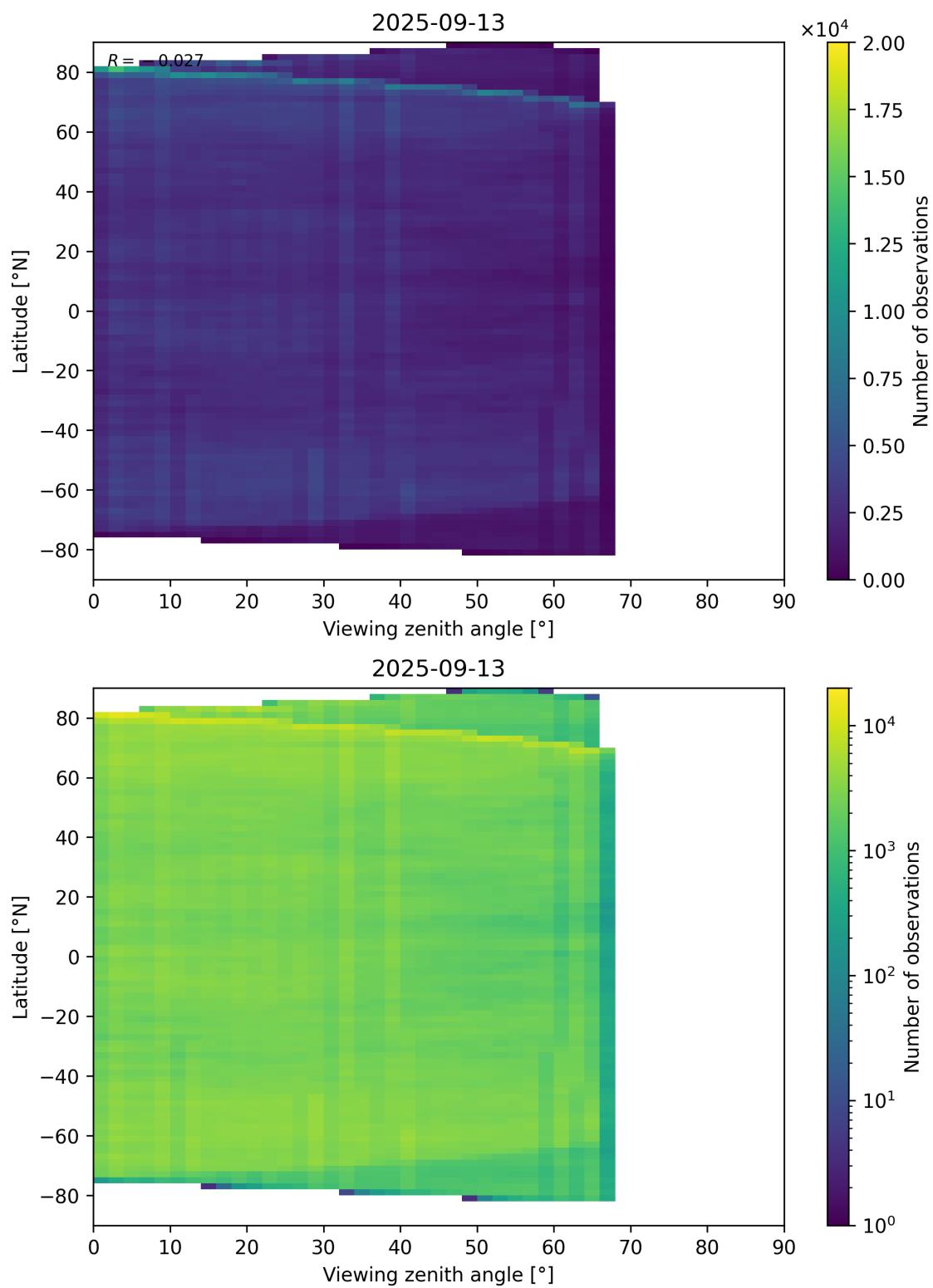
Figure 74: Scatter density plot of “Viewing zenith angle” against “Latitude” for 2025-09-12 to 2025-09-14.
