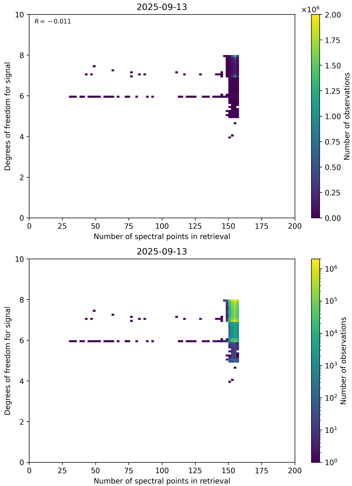
Figure 59: Scatter density plot of “Number of spectral points in retrieval” against “Degrees of freedom for signal” for 2025-09-12 to 2025-09-14.
