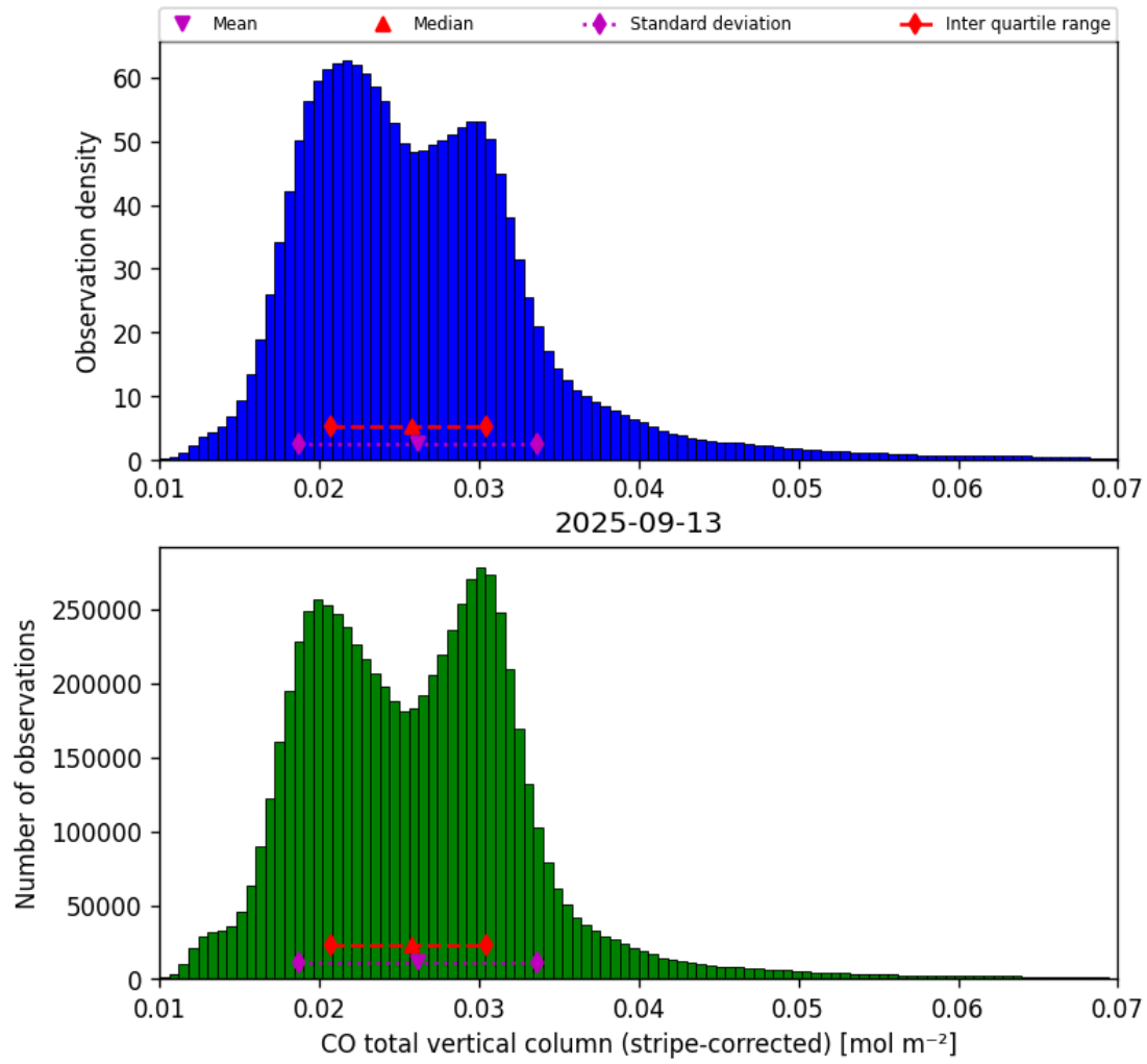
Figure 19: Histogram of “CO total vertical column (stripe-corrected)” for 2025-09-12 to 2025-09-14
