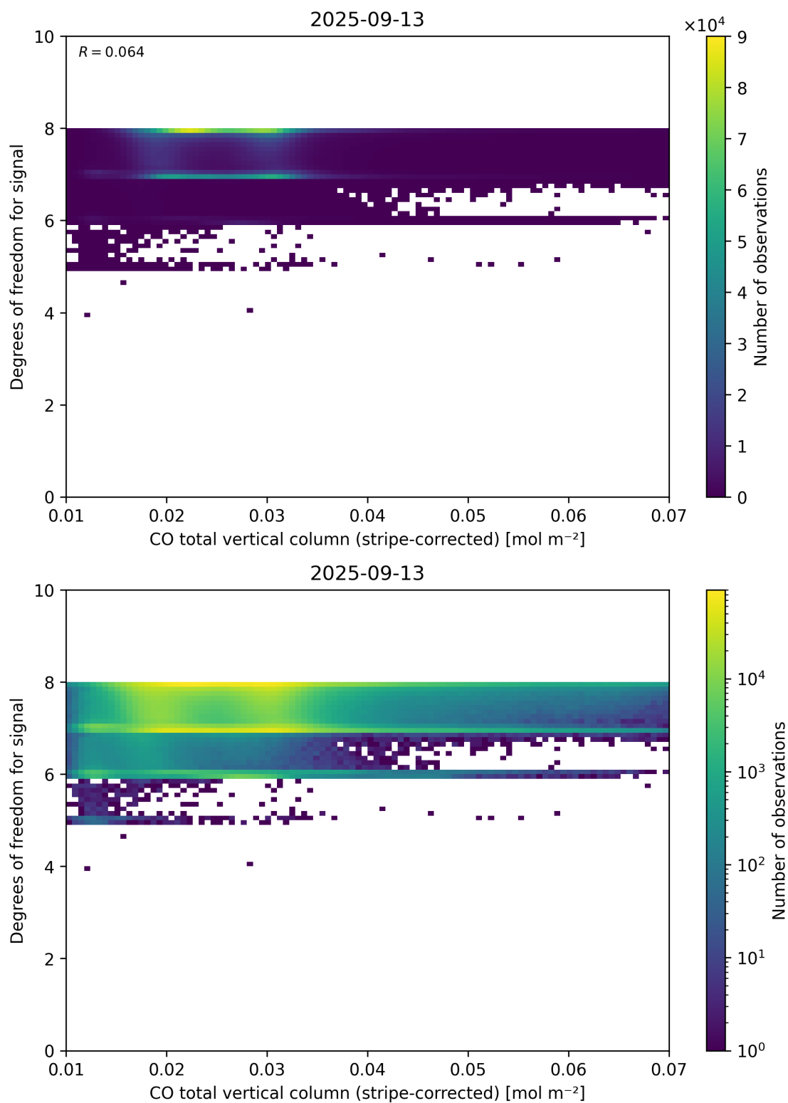
Figure 38: Scatter density plot of “CO total vertical column (stripe-corrected)” against “Degrees of freedom for signal” for 2025-09-12 to 2025-09-14.
