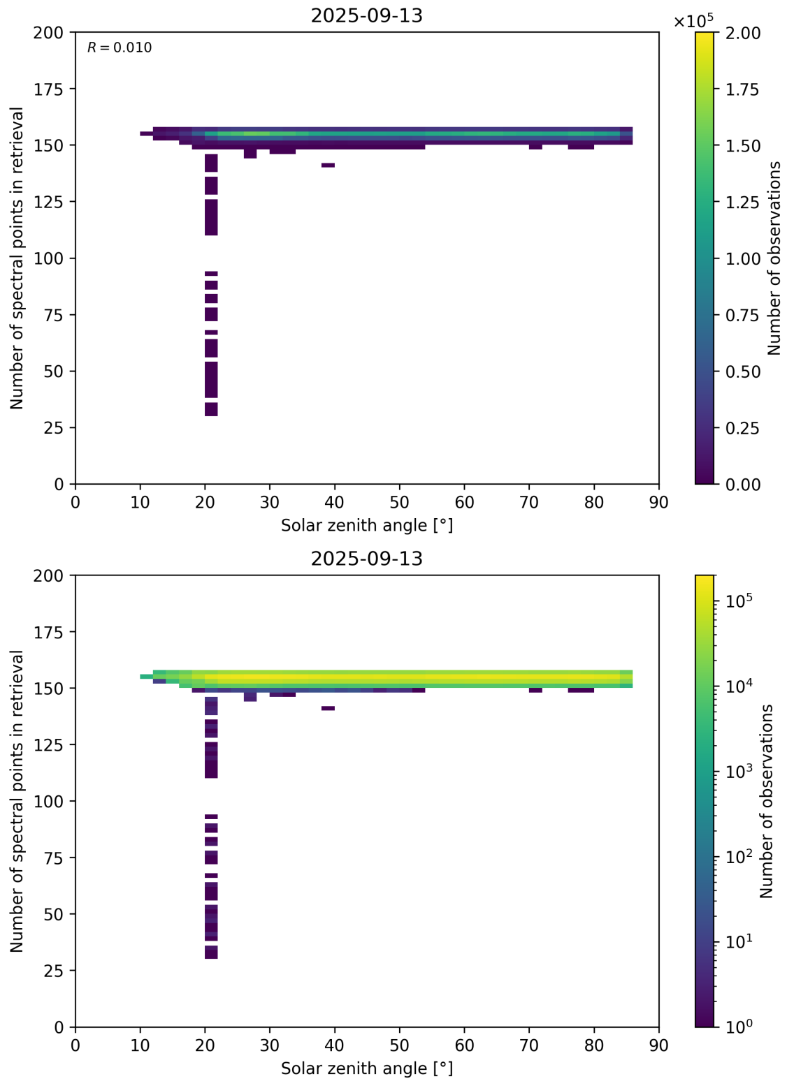
Figure 68: Scatter density plot of “Solar zenith angle” against “Number of spectral points in retrieval” for 2025-09-12 to 2025-09-14.
