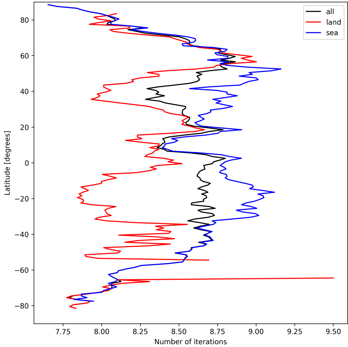
Figure 16: Zonal average of “Number of iterations” for 2025-09-12 to 2025-09-14.
