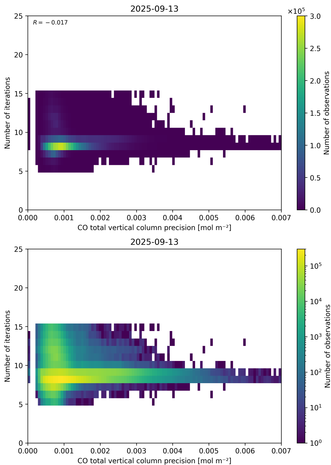
Figure 46: Scatter density plot of “CO total vertical column precision” against “Number of iterations” for 2025-09-12 to 2025-09-14.
