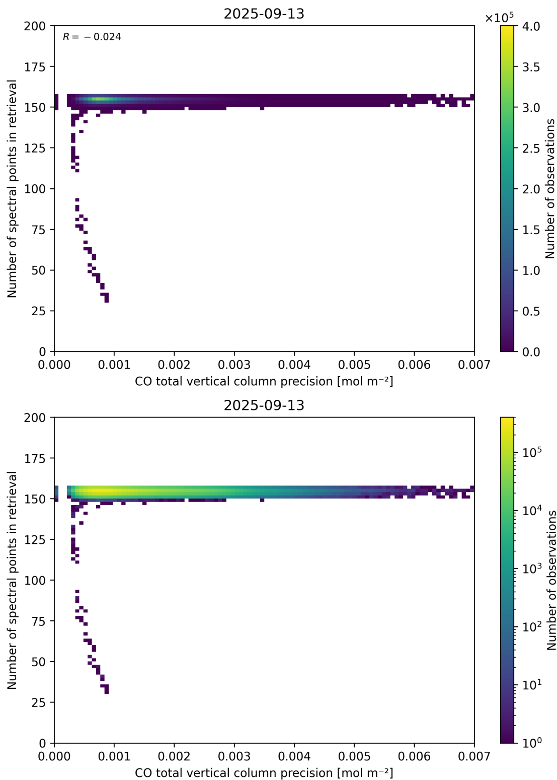
Figure 47: Scatter density plot of “CO total vertical column precision” against “Number of spectral points in retrieval” for 2025-09-12 to 2025-09-14.
