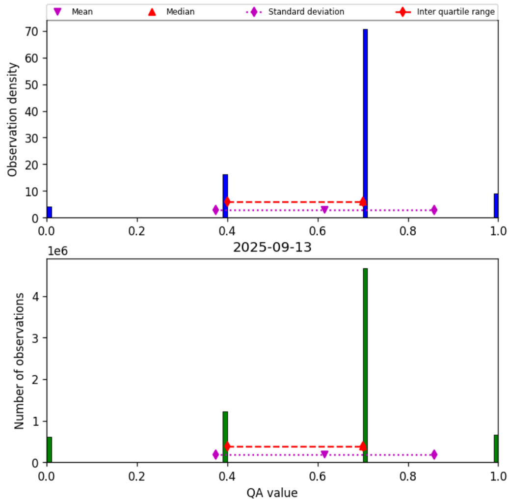
Figure 17: Histogram of “QA value” for 2025-09-12 to 2025-09-14
