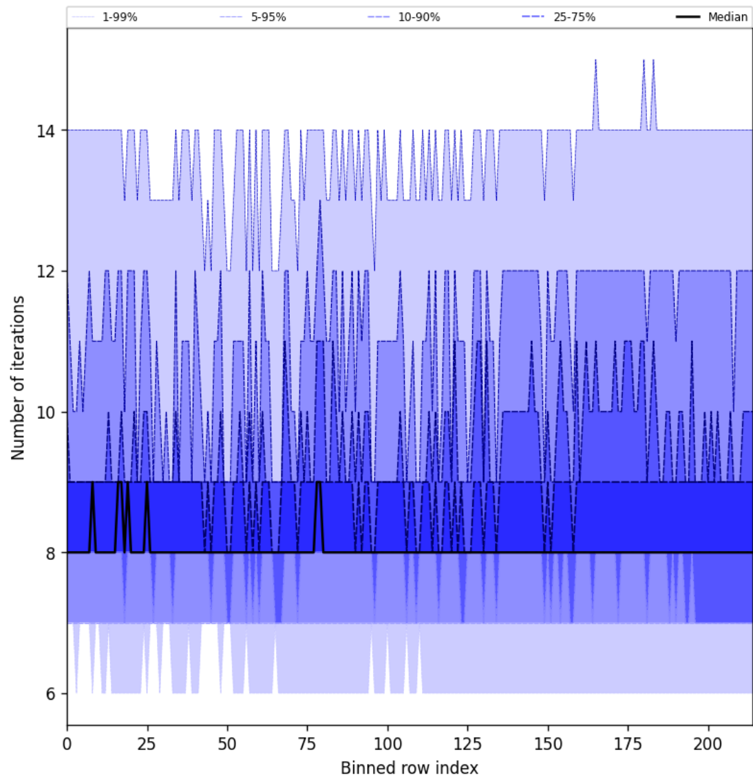
Figure 32: Along track statistics of “Number of iterations” for 2025-09-12 to 2025-09-14
