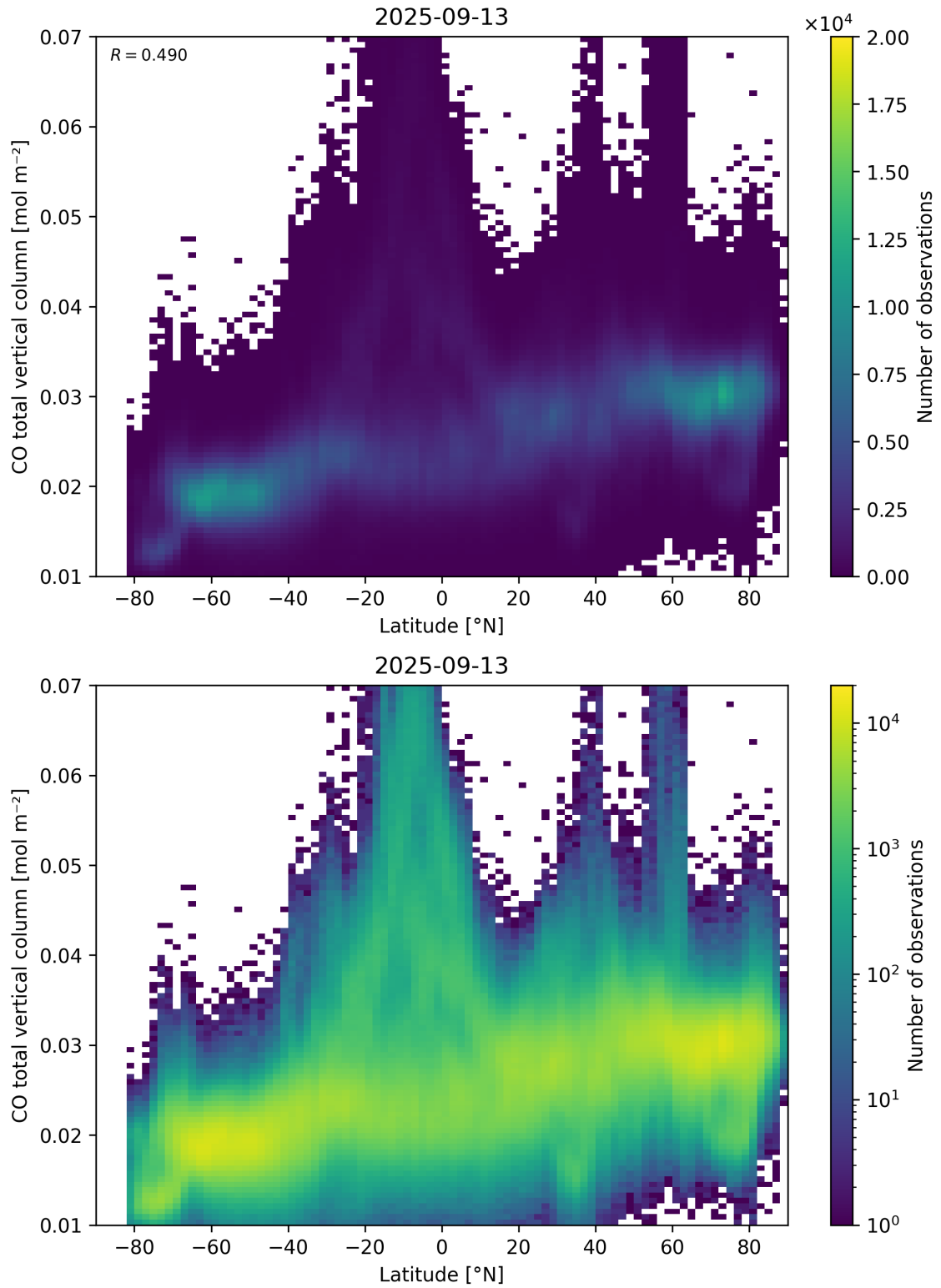
Figure 51: Scatter density plot of “Latitude” against “CO total vertical column” for 2025-09-12 to 2025-09-14.
