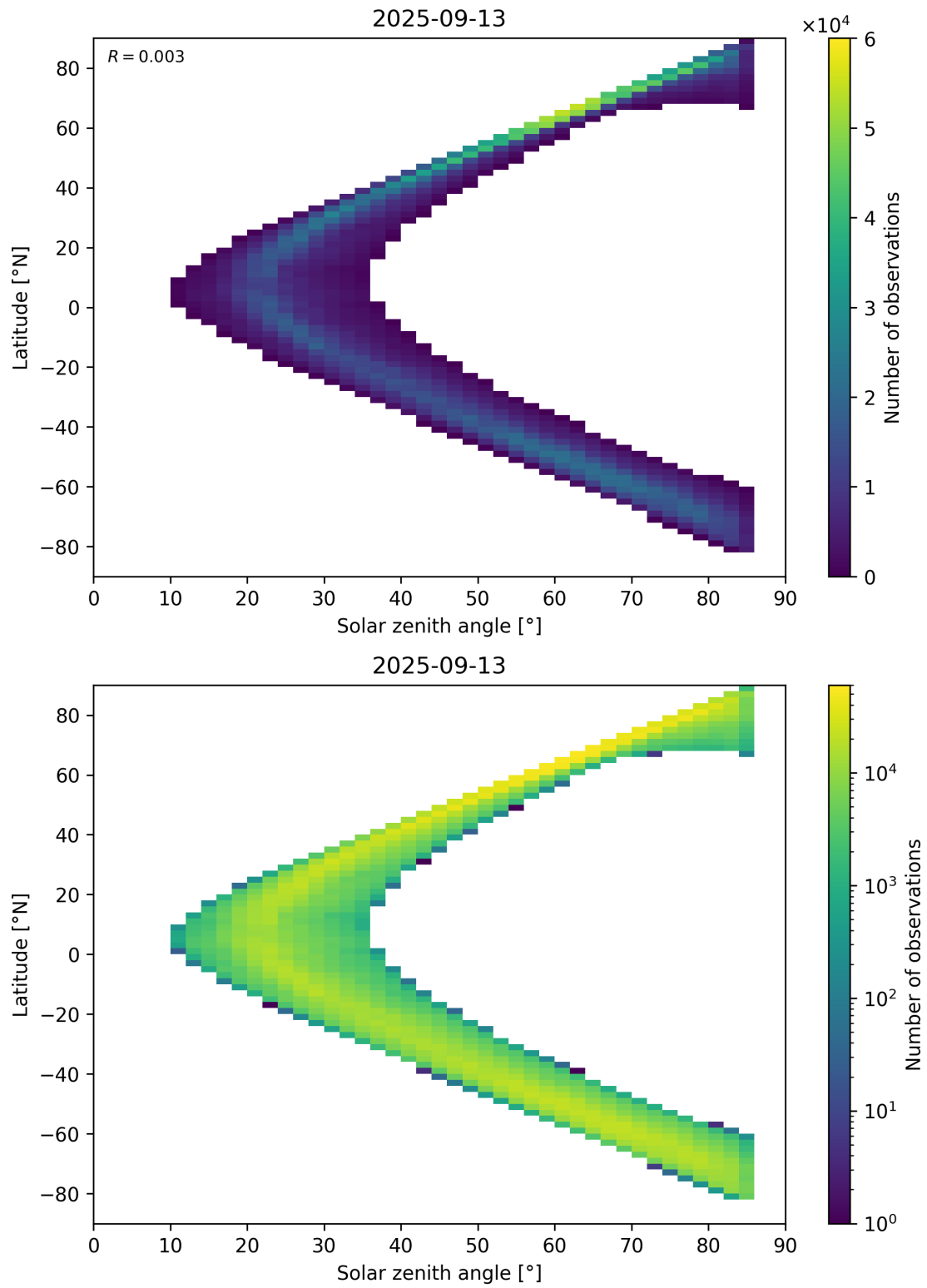
Figure 66: Scatter density plot of “Solar zenith angle” against “Latitude” for 2025-09-12 to 2025-09-14.
