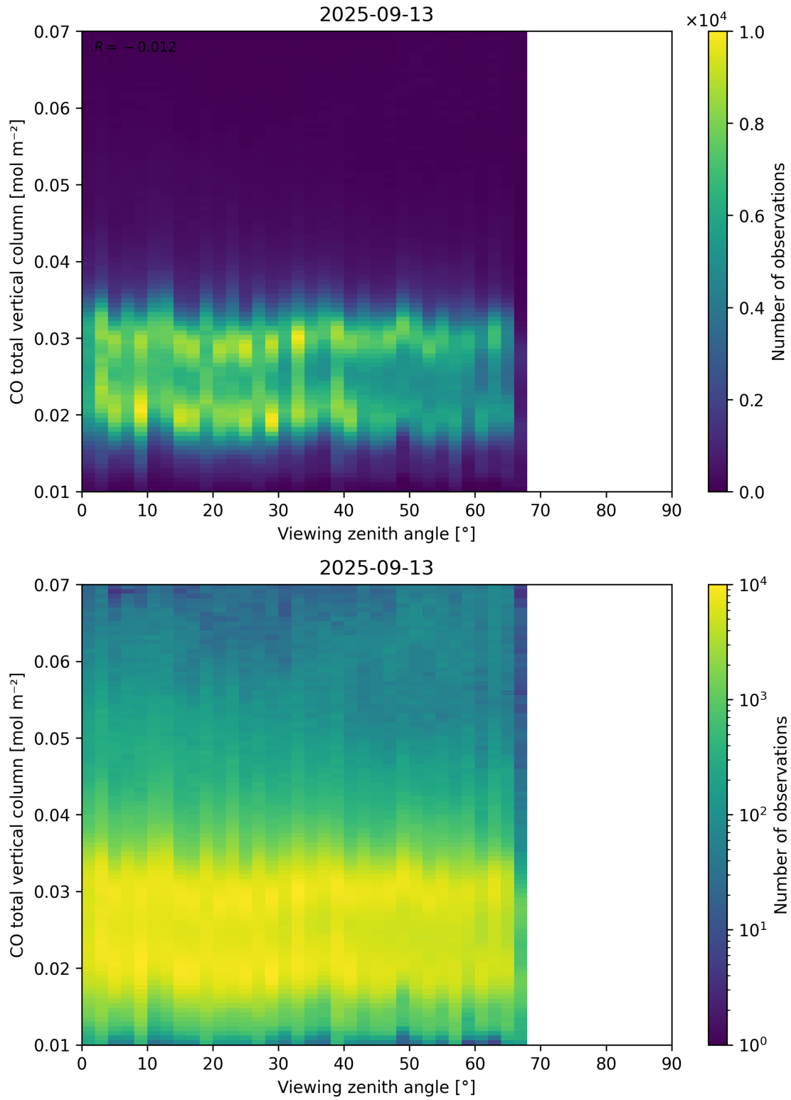
Figure 69: Scatter density plot of “Viewing zenith angle” against “CO total vertical column” for 2025-09-12 to 2025-09-14.
