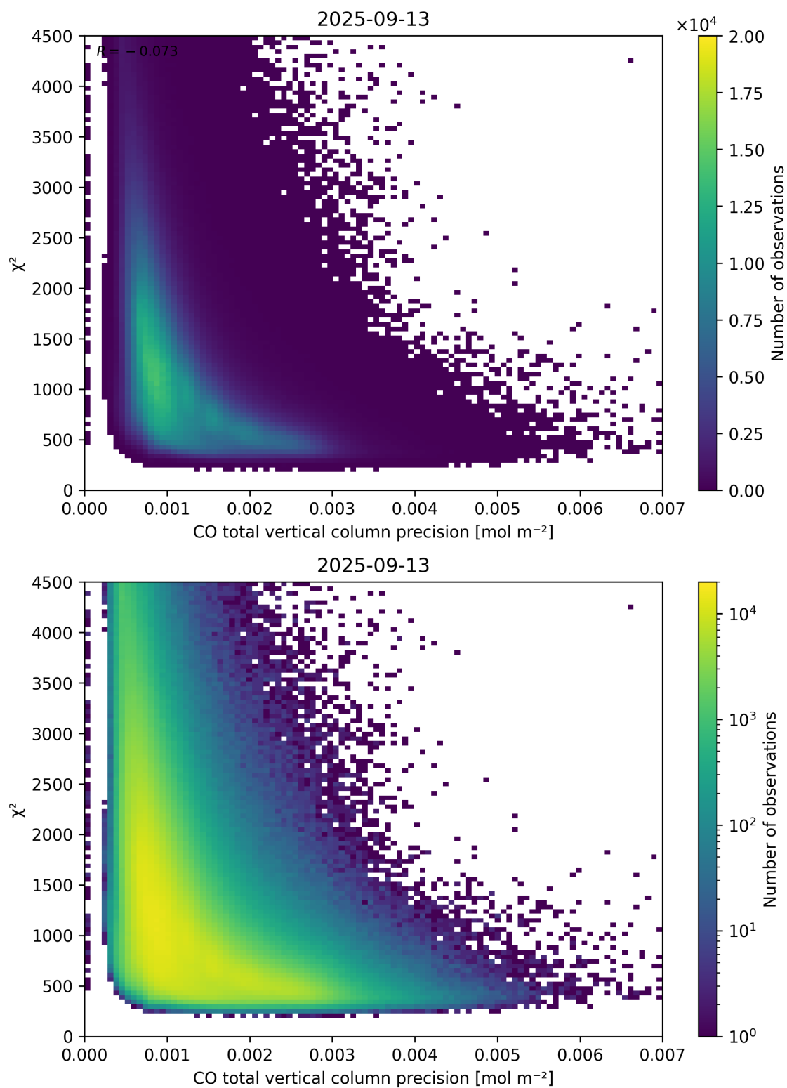
Figure 44: Scatter density plot of “CO total vertical column precision” against “ \chi^2 ” for 2025-09-12 to 2025-09-14.
