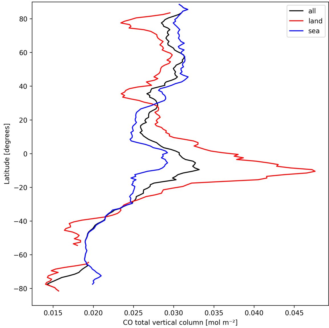
Figure 10: Zonal average of “CO total vertical column” for 2025-09-12 to 2025-09-14.
