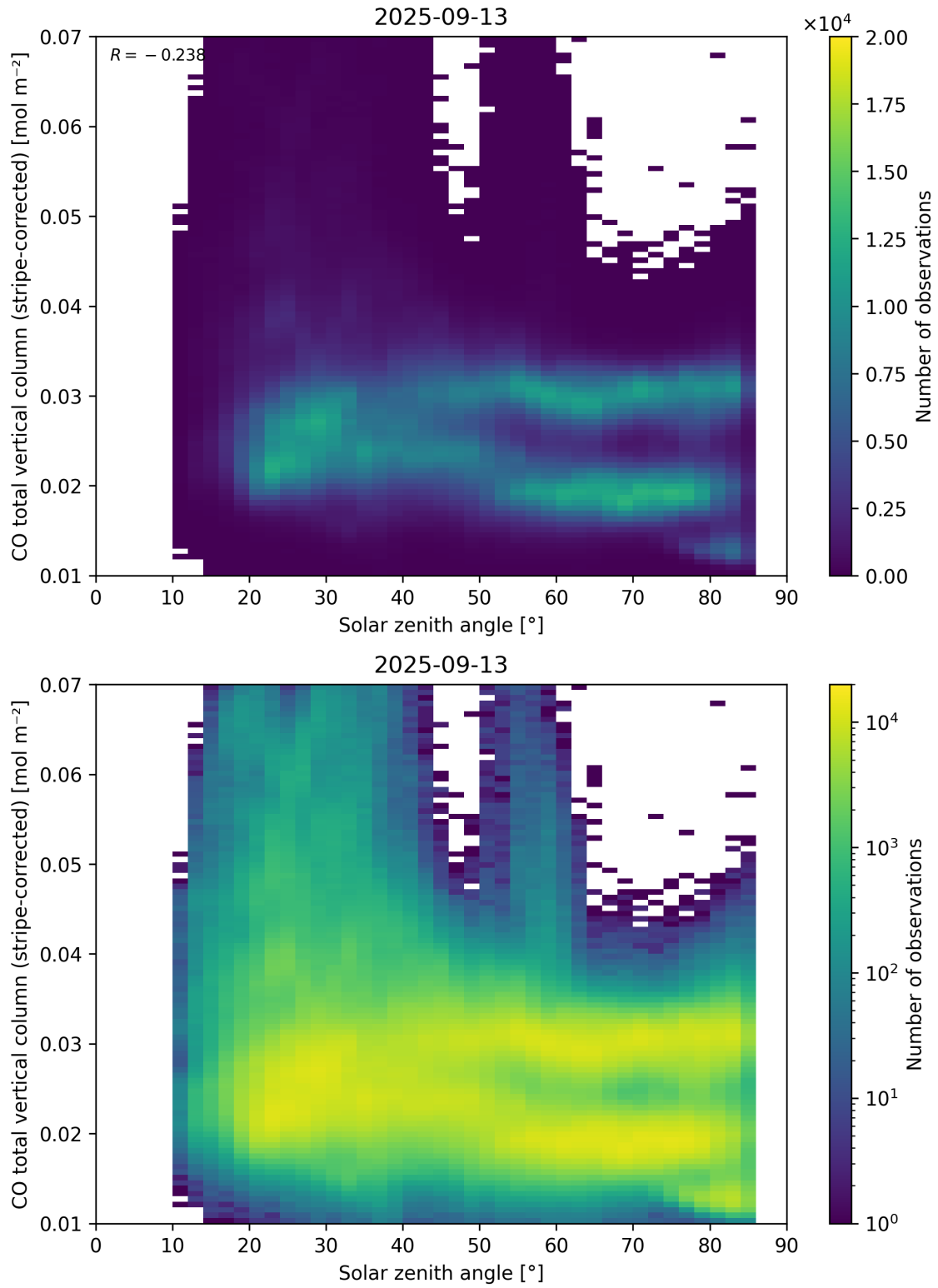
Figure 62: Scatter density plot of “Solar zenith angle” against “CO total vertical column (stripe-corrected)” for 2025-09-12 to 2025-09-14.
