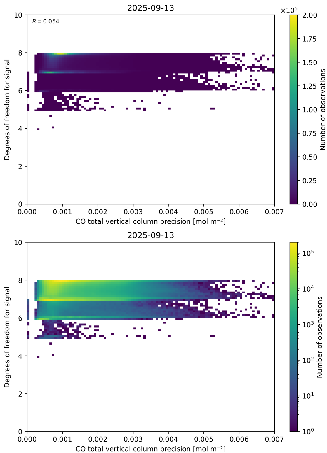
Figure 45: Scatter density plot of “CO total vertical column precision” against “Degrees of freedom for signal” for 2025-09-12 to 2025-09-14.
