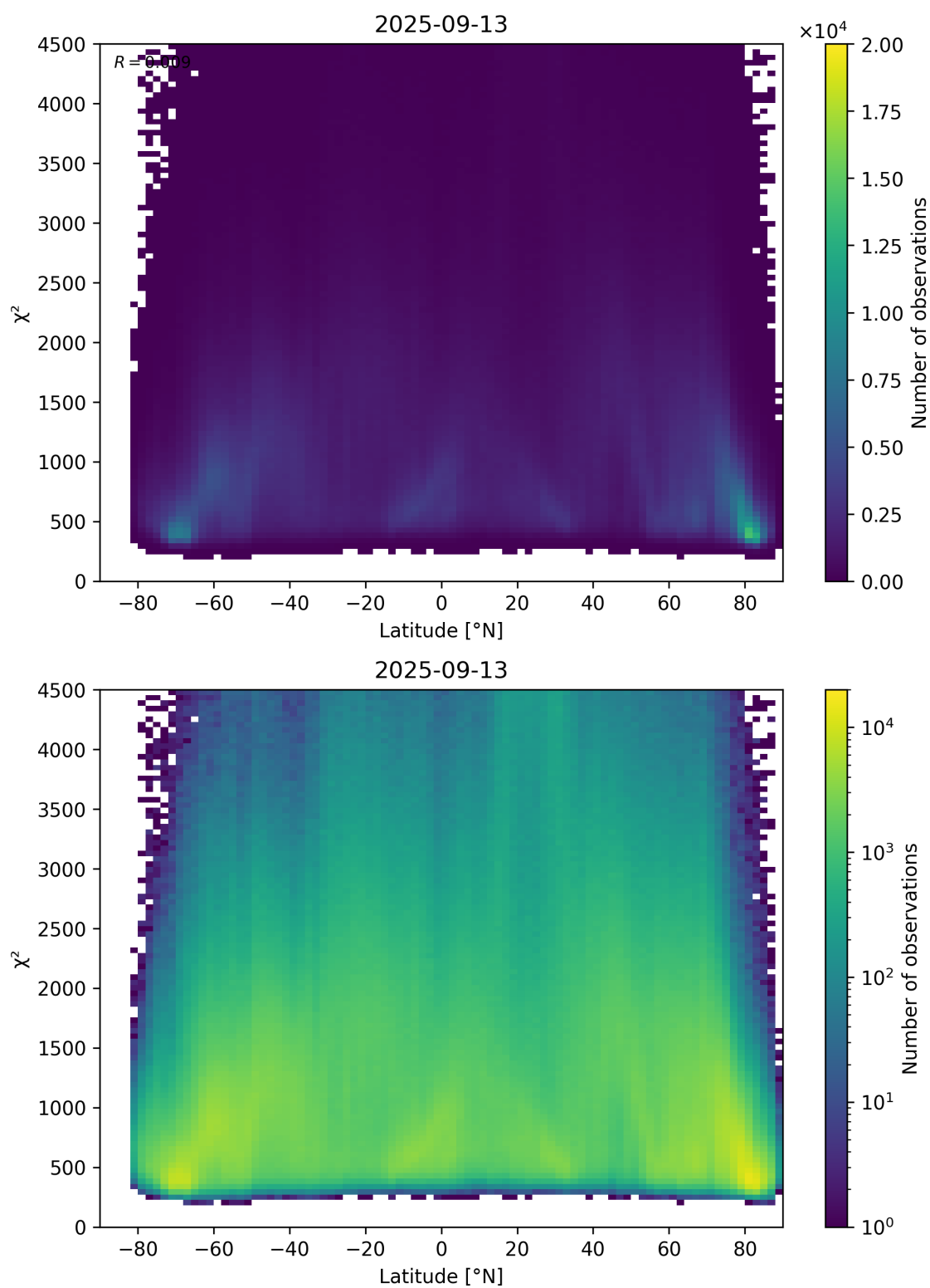
Figure 54: Scatter density plot of “Latitude” against “ \chi^2 ” for 2025-09-12 to 2025-09-14.
