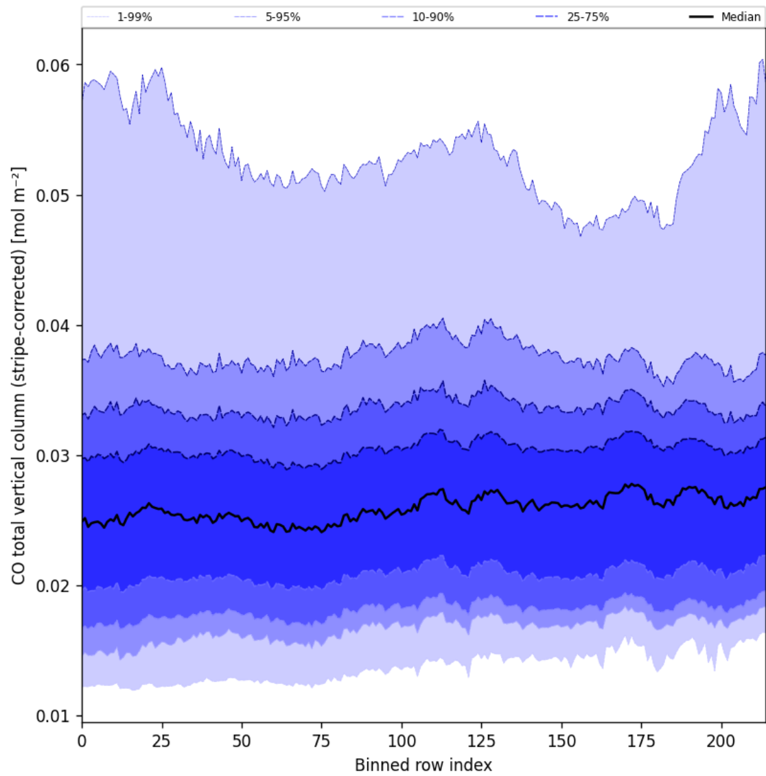
Figure 27: Along track statistics of “CO total vertical column (stripe-corrected)” for 2025-09-12 to 2025-09-14
