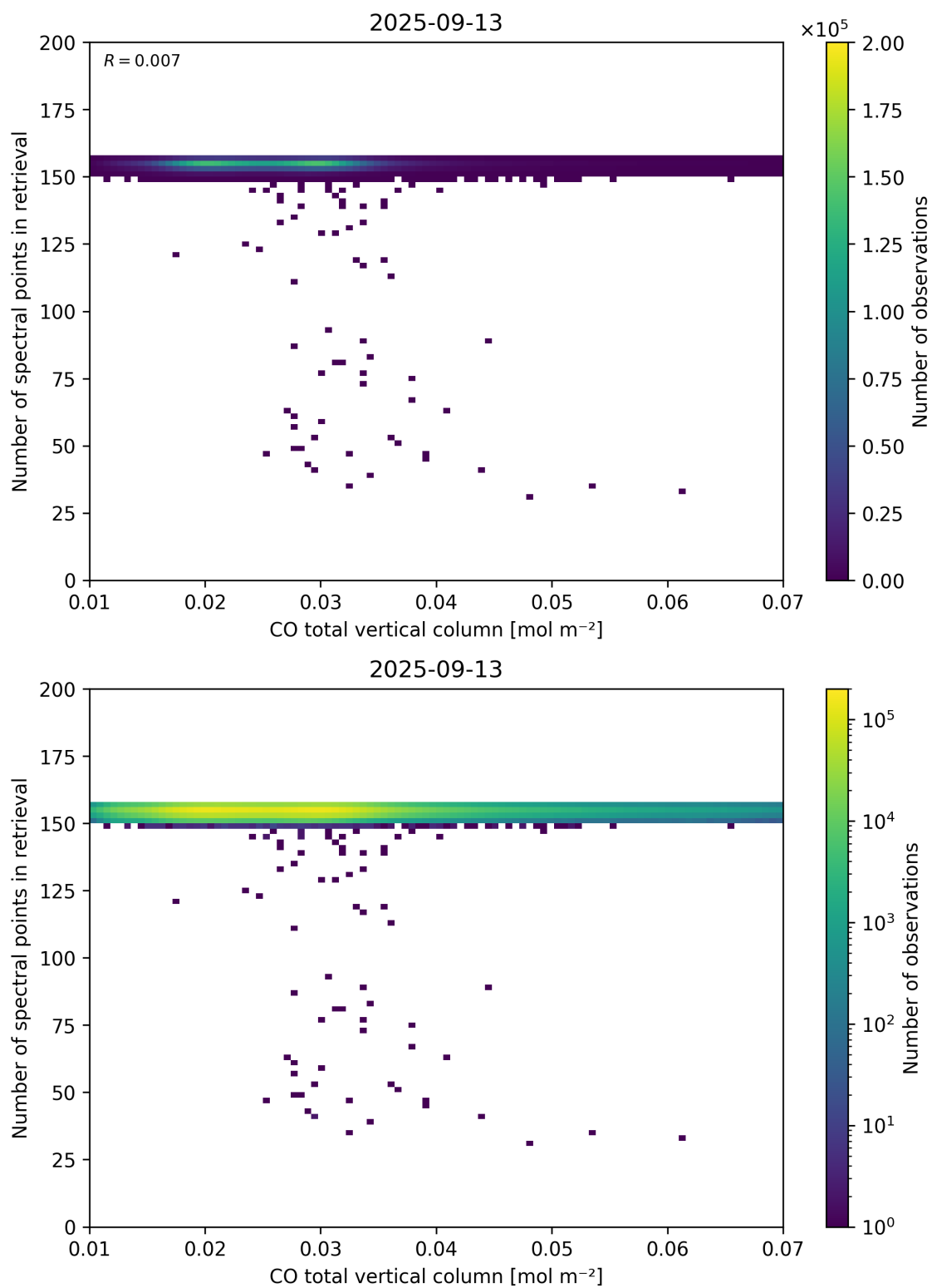
Figure 43: Scatter density plot of “CO total vertical column” against “Number of spectral points in retrieval” for 2025-09-12 to 2025-09-14.
