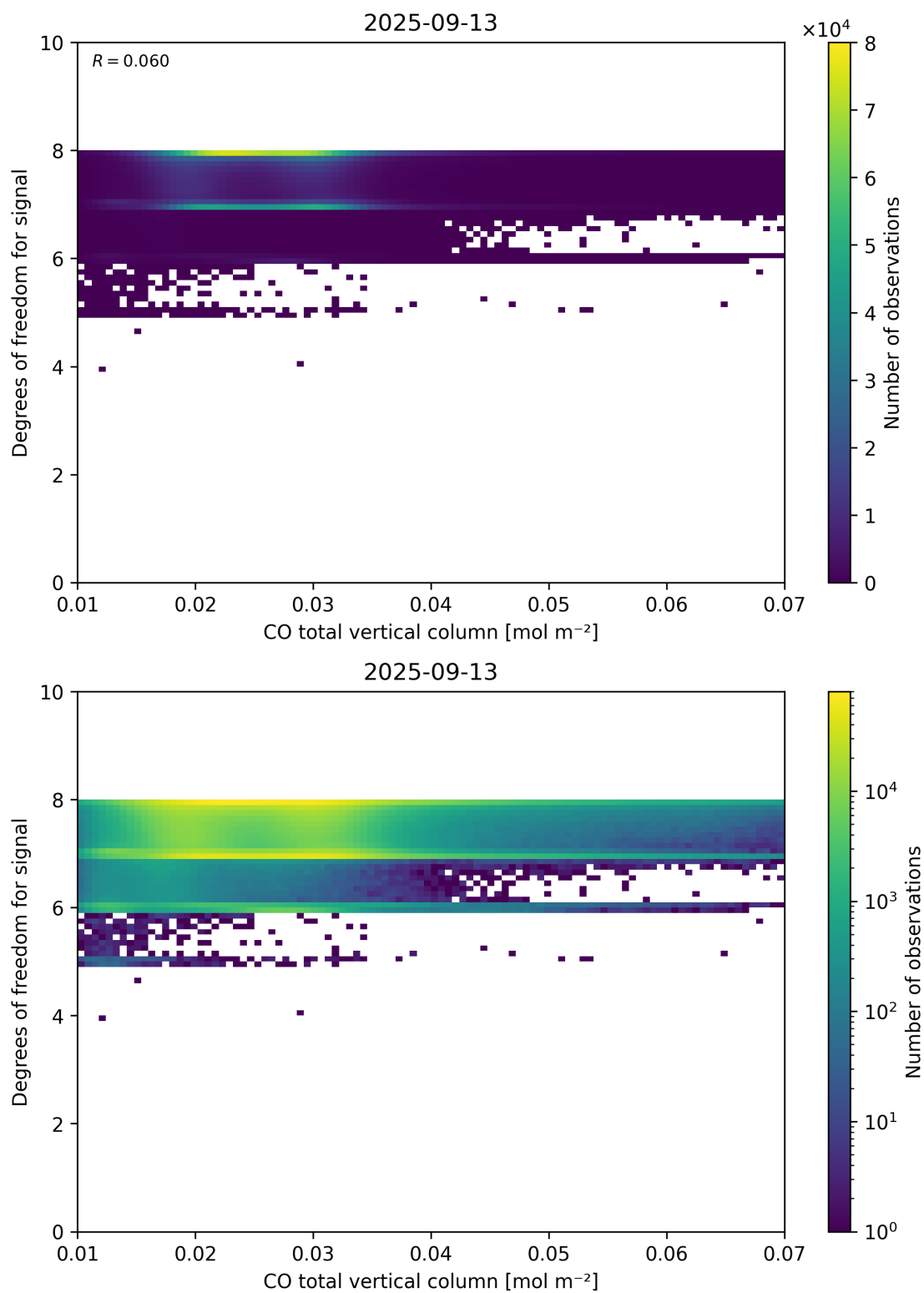
Figure 41: Scatter density plot of “CO total vertical column” against “Degrees of freedom for signal” for 2025-09-12 to 2025-09-14.
