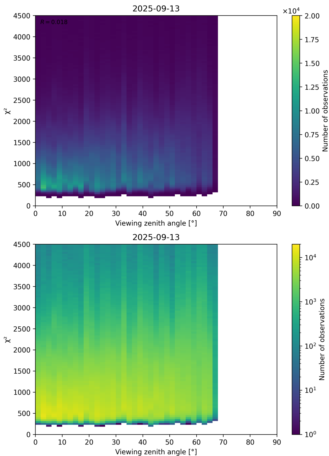
Figure 72: Scatter density plot of “Viewing zenith angle” against “ \chi^2 ” for 2025-09-12 to 2025-09-14.
