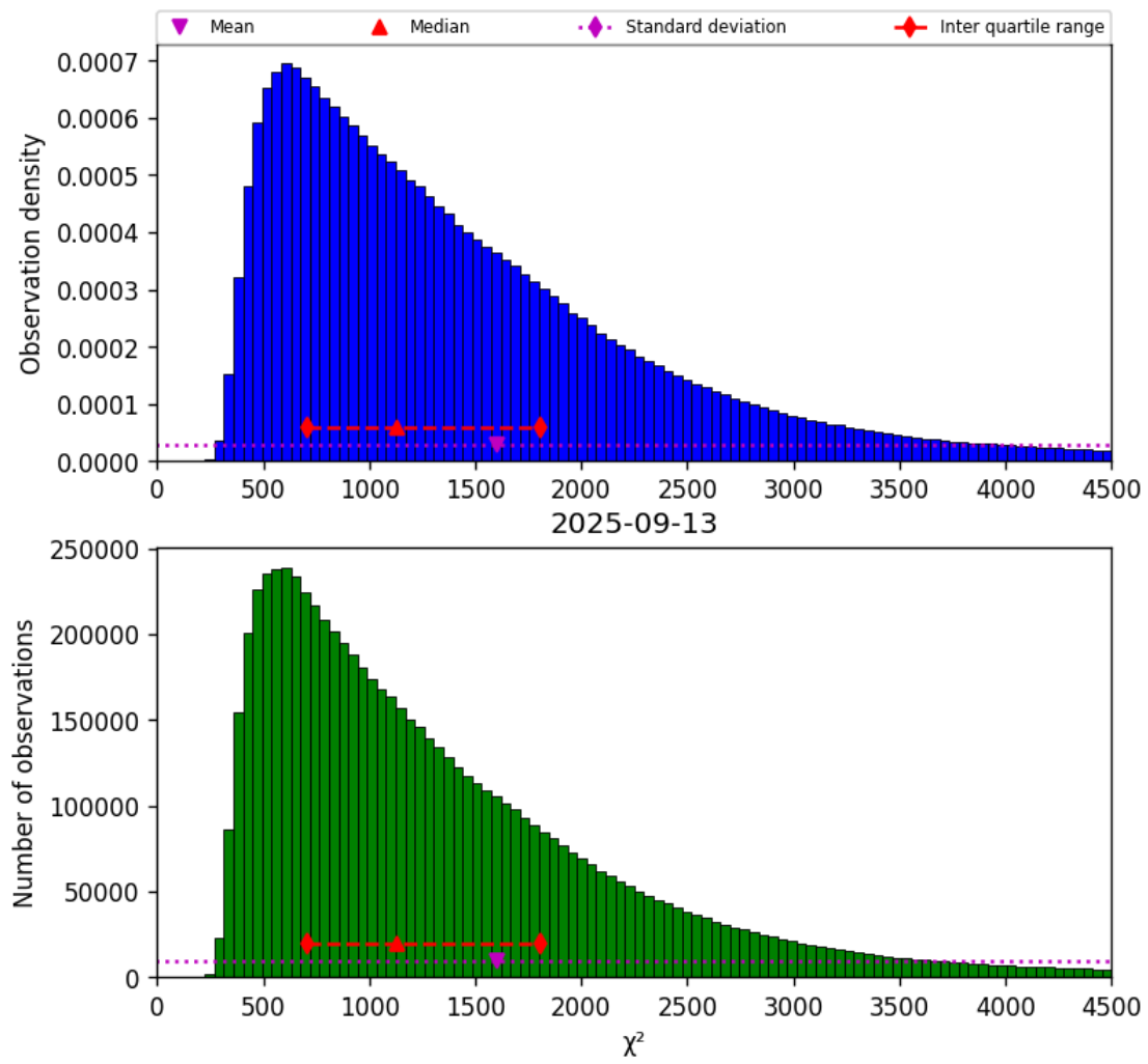
Figure 22: Histogram of “ \chi^2 ” for 2025-09-12 to 2025-09-14
