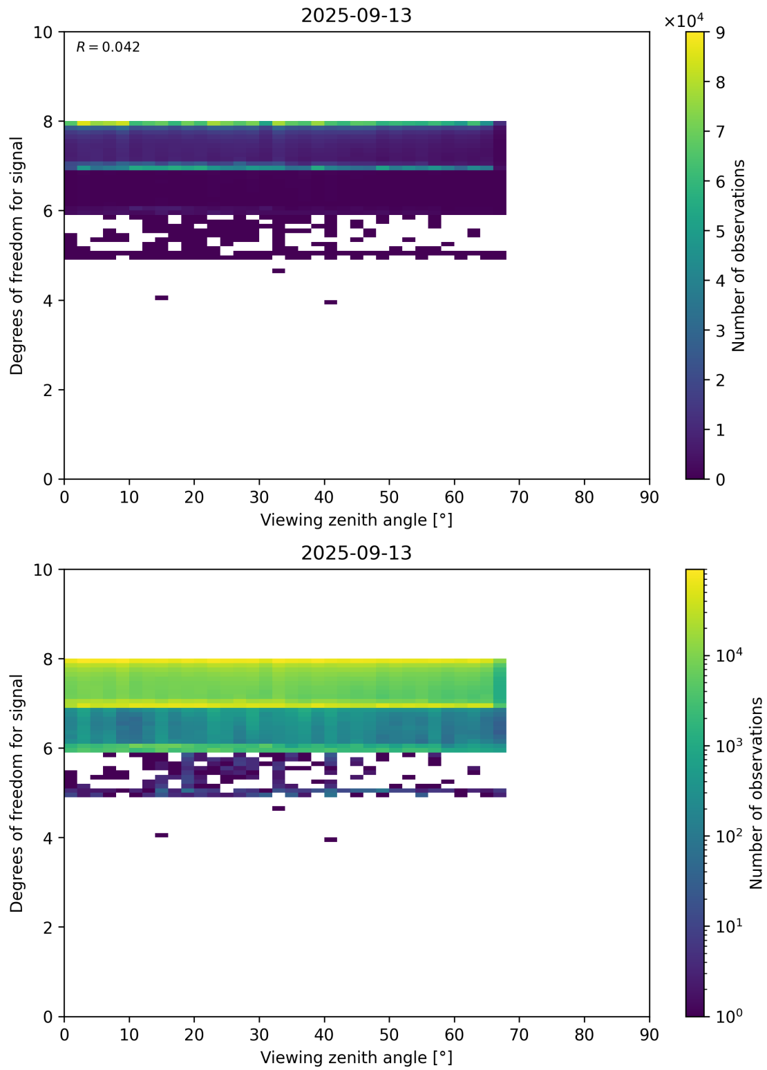
Figure 73: Scatter density plot of “Viewing zenith angle” against “Degrees of freedom for signal” for 2025-09-12 to 2025-09-14.
