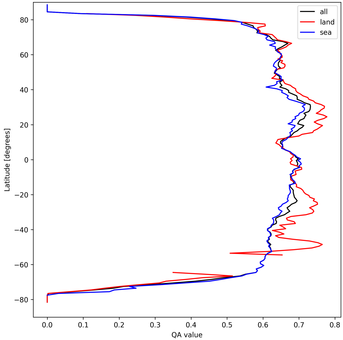
Figure 9: Zonal average of “QA value” for 2025-09-12 to 2025-09-14.
