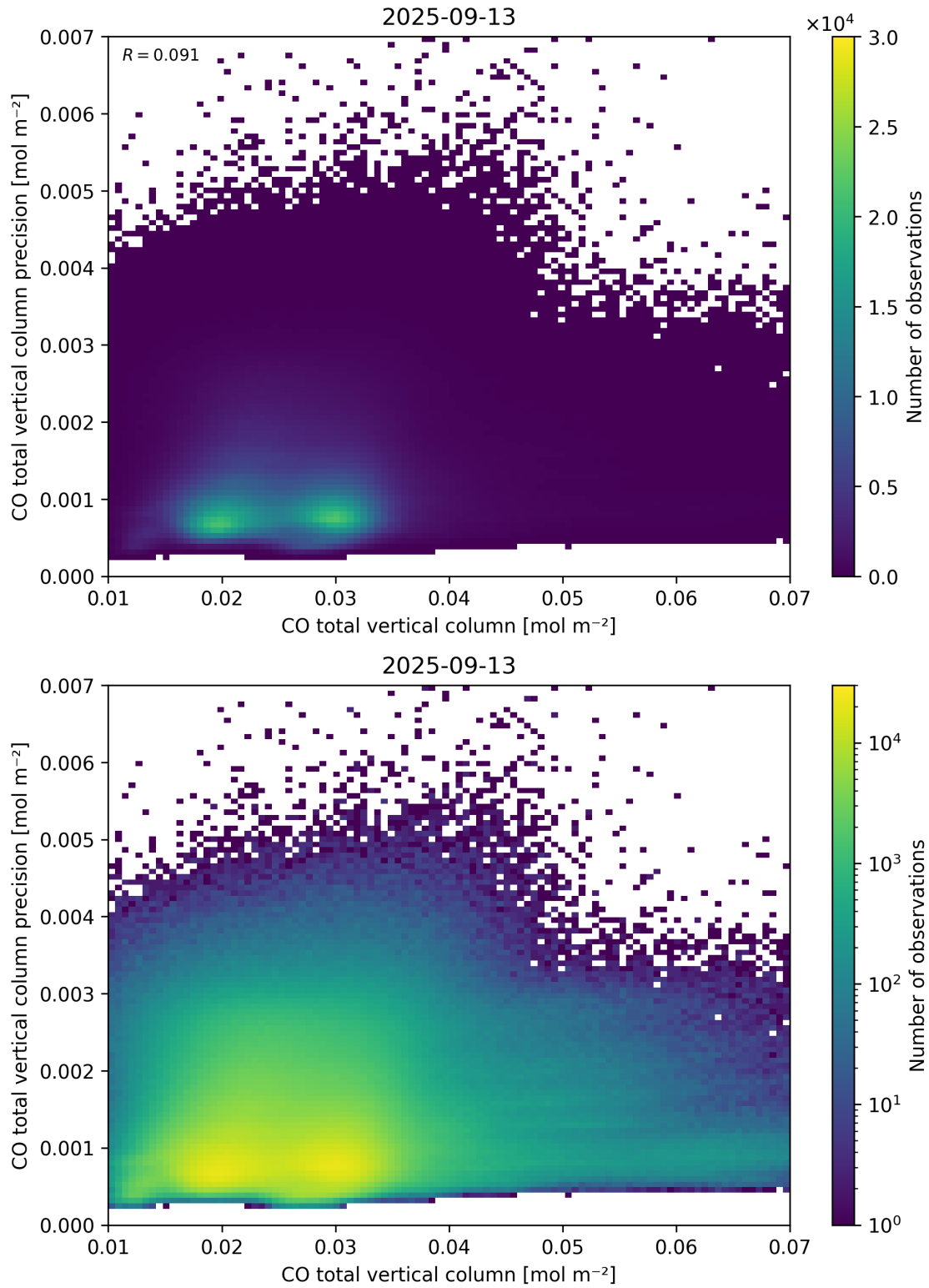
Figure 34: Scatter density plot of “CO total vertical column” against “CO total vertical column precision” for 2025-09-12 to 2025-09-14.
