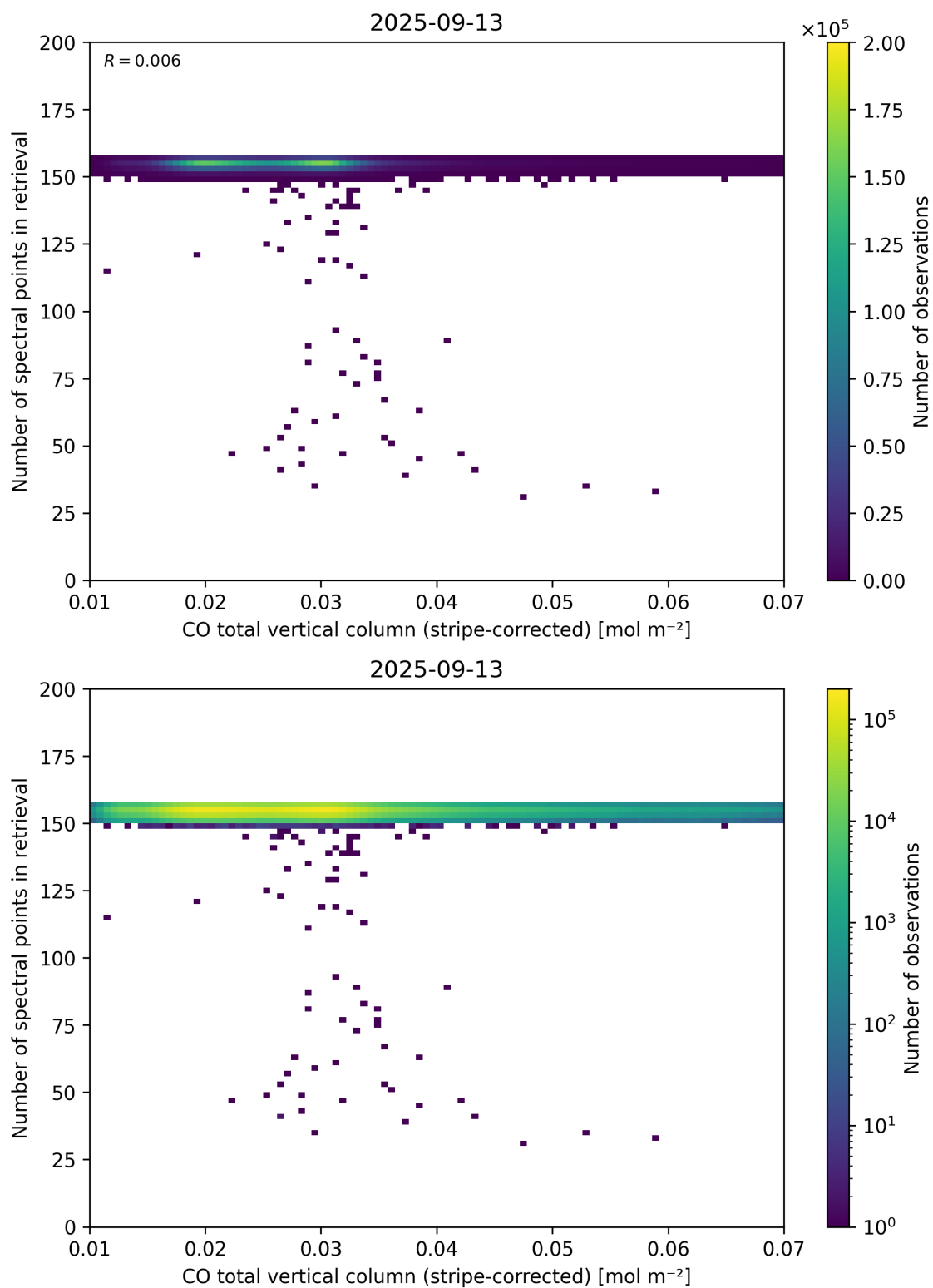
Figure 40: Scatter density plot of “CO total vertical column (stripe-corrected)” against “Number of spectral points in retrieval” for 2025-09-12 to 2025-09-14.
