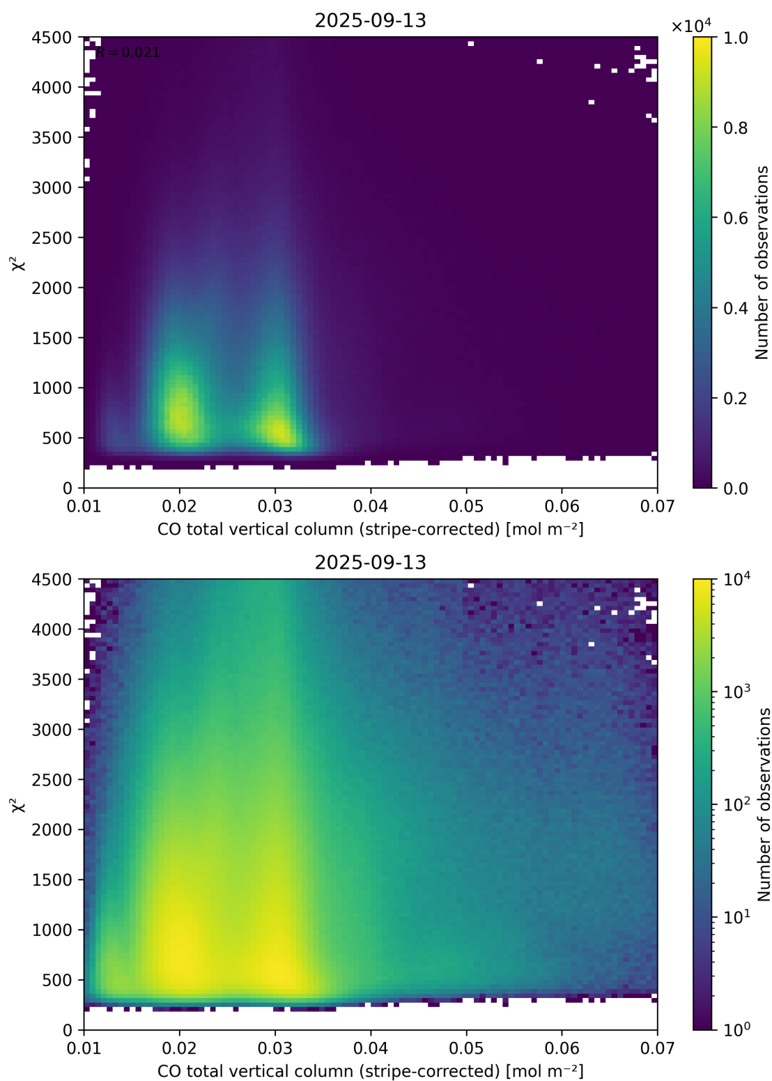
Figure 37: Scatter density plot of “CO total vertical column (stripe-corrected)” against “ \chi^2 ” for 2025-09-12 to 2025-09-14.
