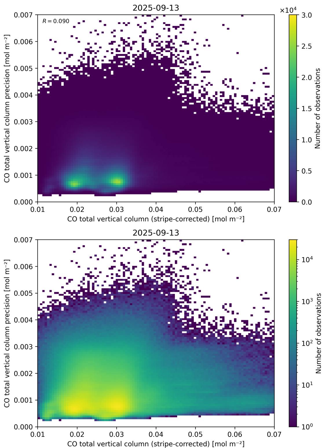
Figure 36: Scatter density plot of “CO total vertical column (stripe-corrected)” against “CO total vertical column precision” for 2025-09-12 to 2025-09-14.
