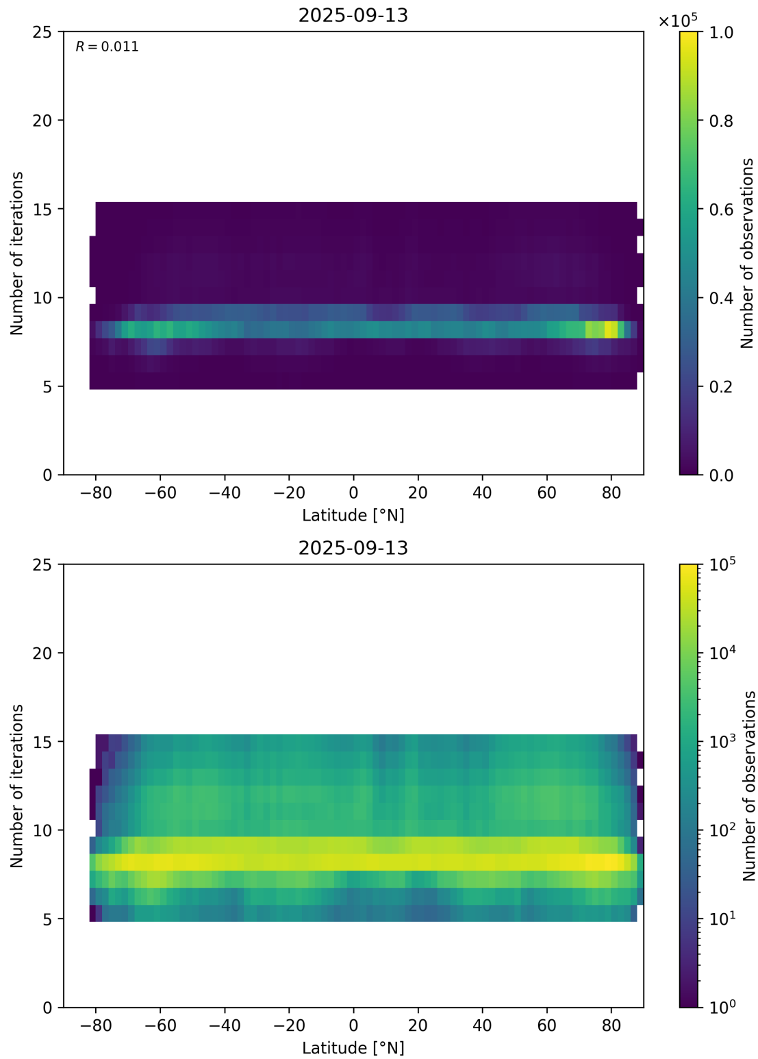
Figure 56: Scatter density plot of “Latitude” against “Number of iterations” for 2025-09-12 to 2025-09-14.
