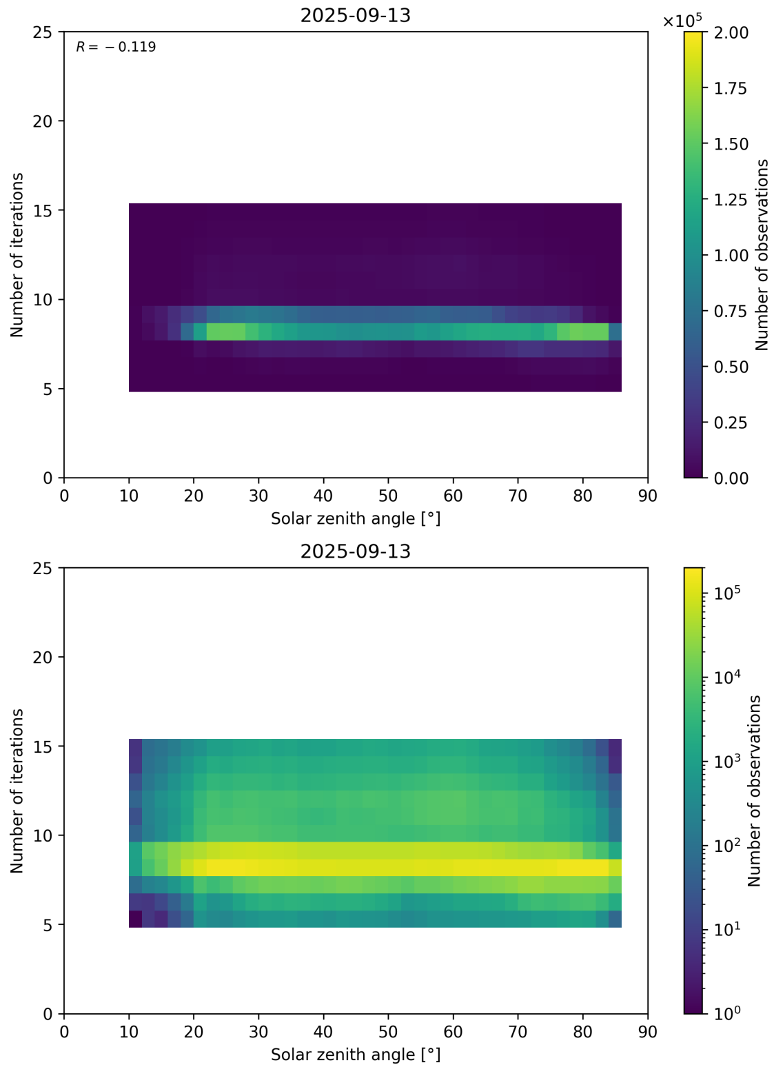
Figure 67: Scatter density plot of “Solar zenith angle” against “Number of iterations” for 2025-09-12 to 2025-09-14.
