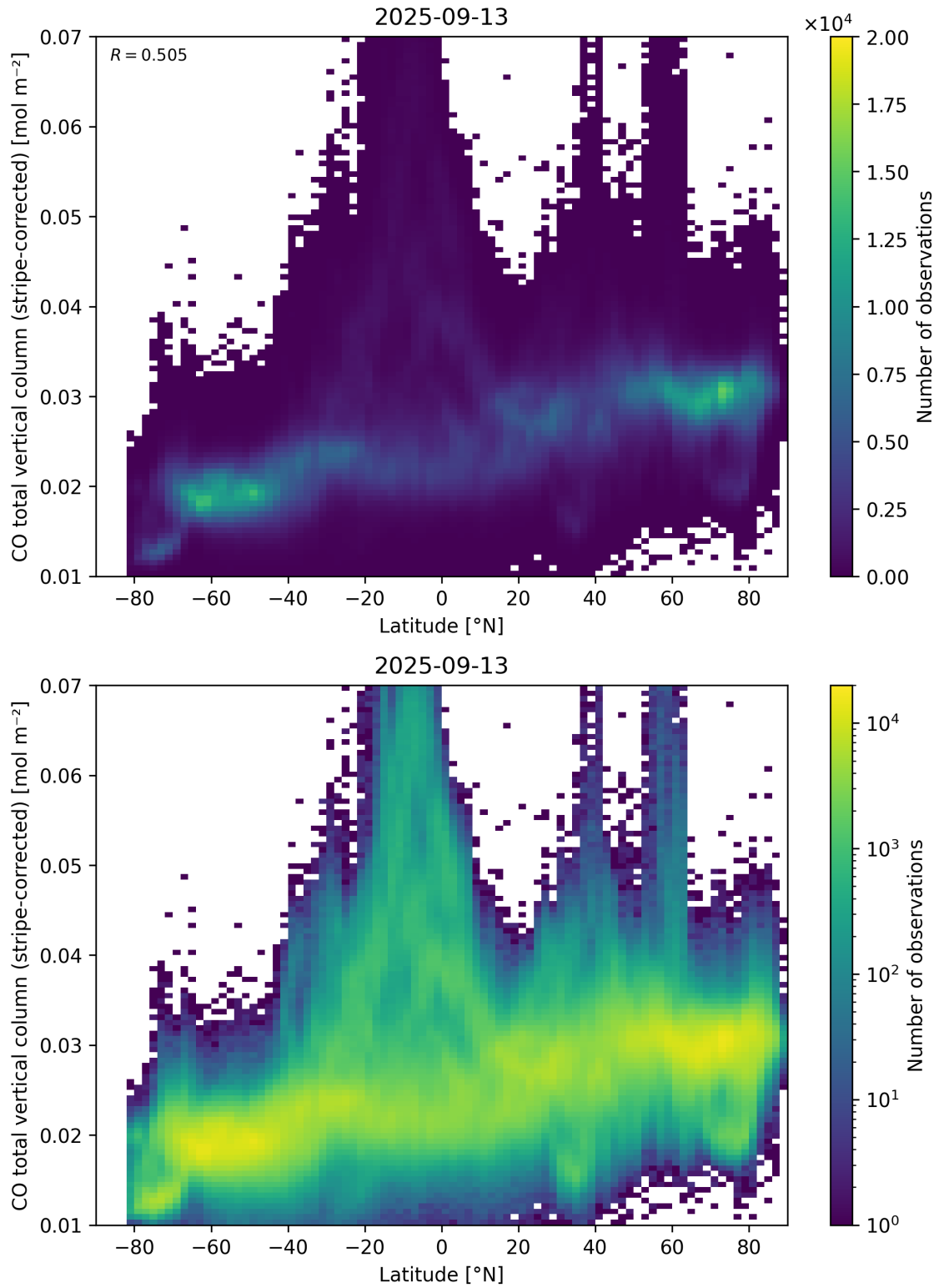
Figure 52: Scatter density plot of “Latitude” against “CO total vertical column (stripe-corrected)” for 2025-09-12 to 2025-09-14.
