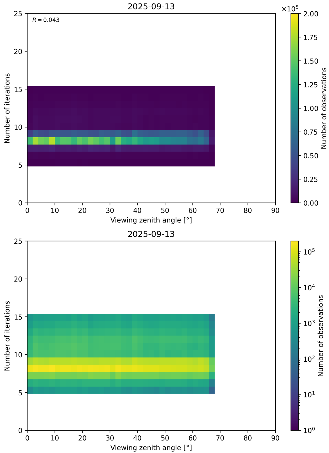
Figure 75: Scatter density plot of “Viewing zenith angle” against “Number of iterations” for 2025-09-12 to 2025-09-14.
