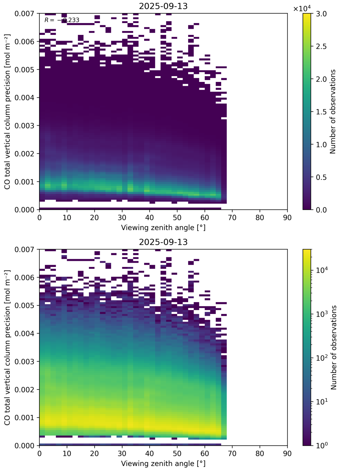
Figure 71: Scatter density plot of “Viewing zenith angle” against “CO total vertical column precision” for 2025-09-12 to 2025-09-14.
