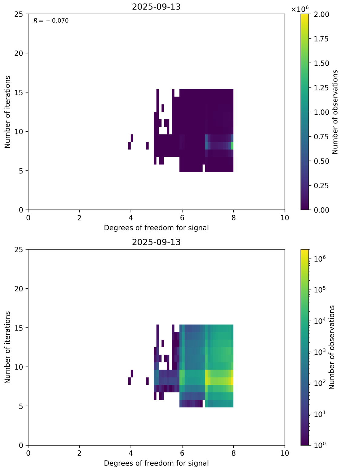
Figure 50: Scatter density plot of “Degrees of freedom for signal” against “Number of iterations” for 2025-09-12 to 2025-09-14.
