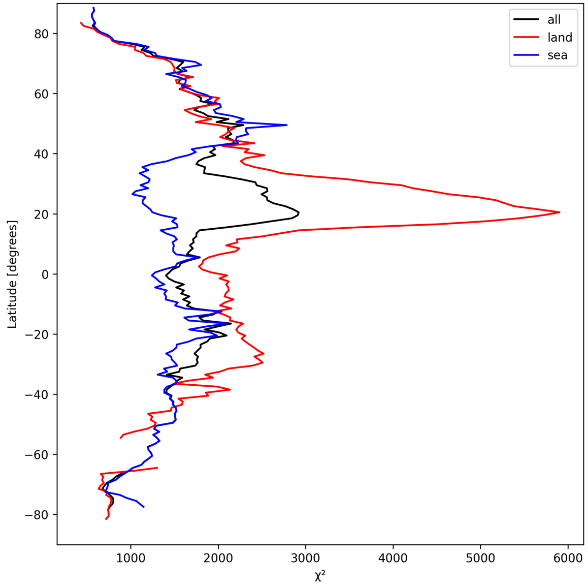
Figure 14: Zonal average of “ \chi^2 ” for 2025-09-12 to 2025-09-14.
