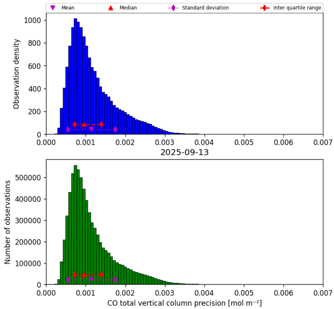
Figure 20: Histogram of “CO total vertical column precision” for 2025-09-12 to 2025-09-14
