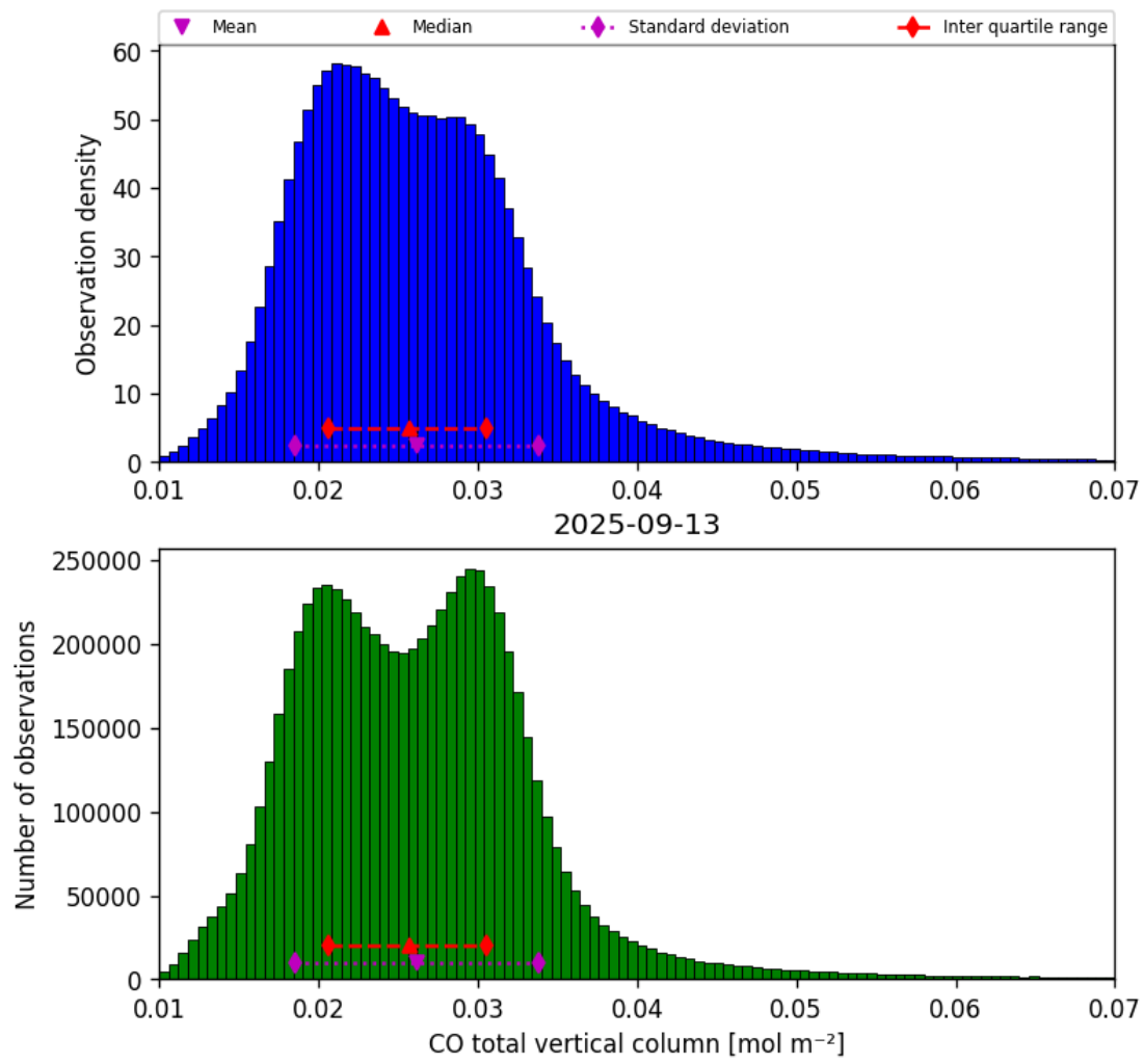
Figure 18: Histogram of “CO total vertical column” for 2025-09-12 to 2025-09-14
