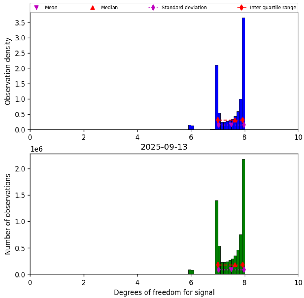
Figure 23: Histogram of “Degrees of freedom for signal” for 2025-09-12 to 2025-09-14
