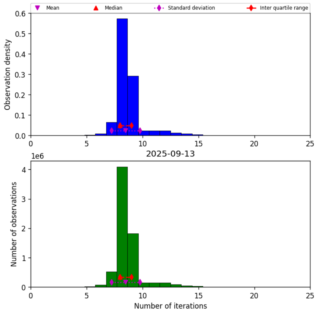
Figure 24: Histogram of “Number of iterations” for 2025-09-12 to 2025-09-14
