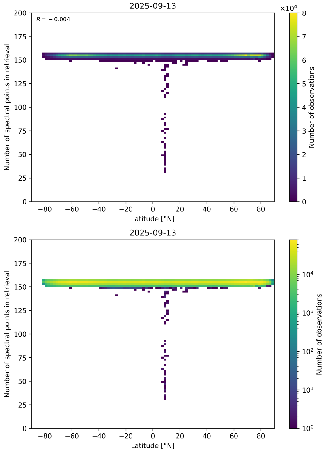
Figure 57: Scatter density plot of “Latitude” against “Number of spectral points in retrieval” for 2025-09-12 to 2025-09-14.
