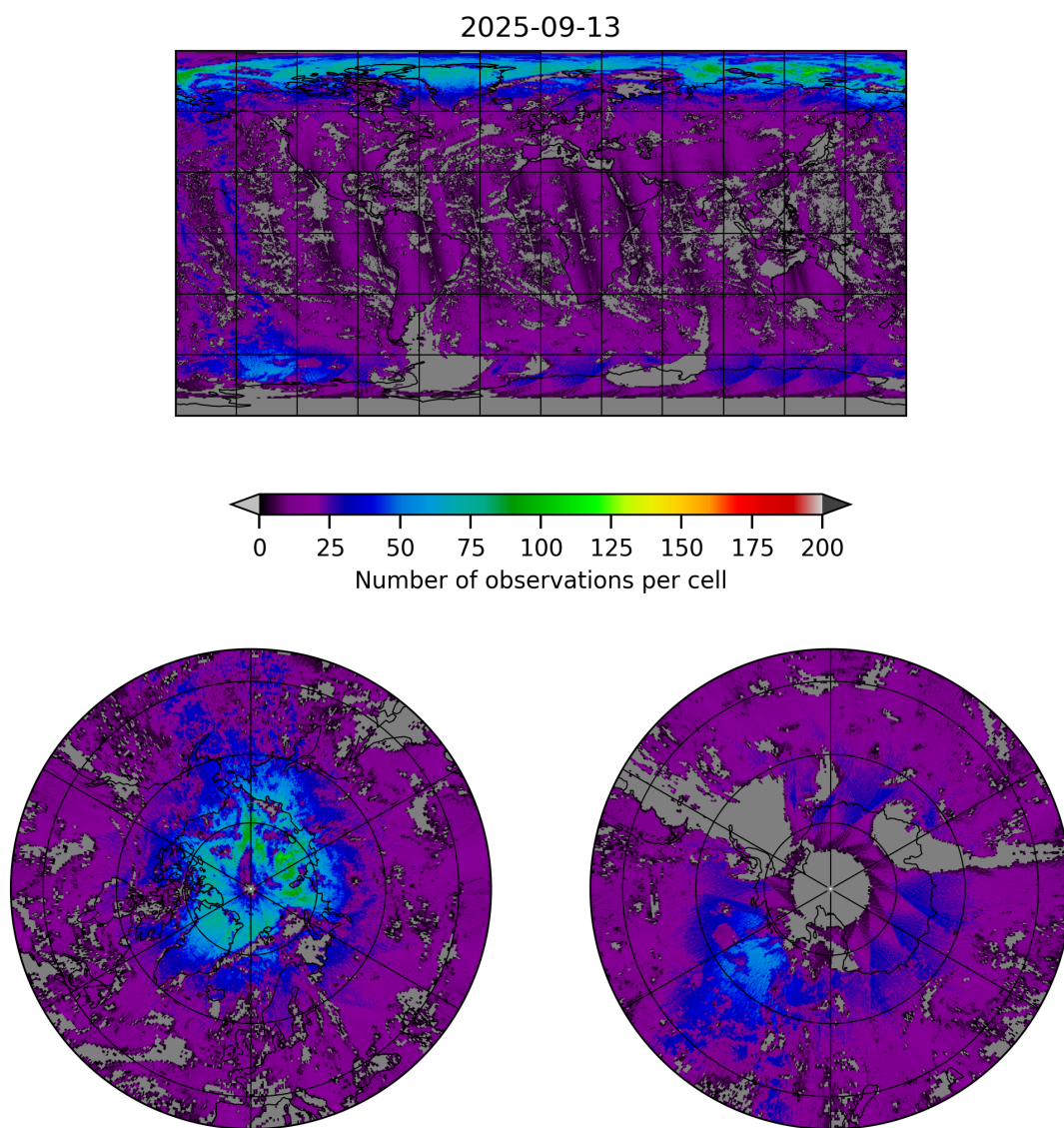
Figure 8: Map of the number of observations for 2025-09-12 to 2025-09-14
