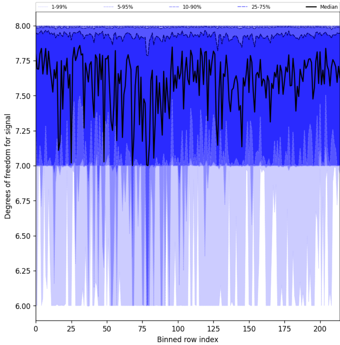
Figure 31: Along track statistics of “Degrees of freedom for signal” for 2025-09-12 to 2025-09-14
