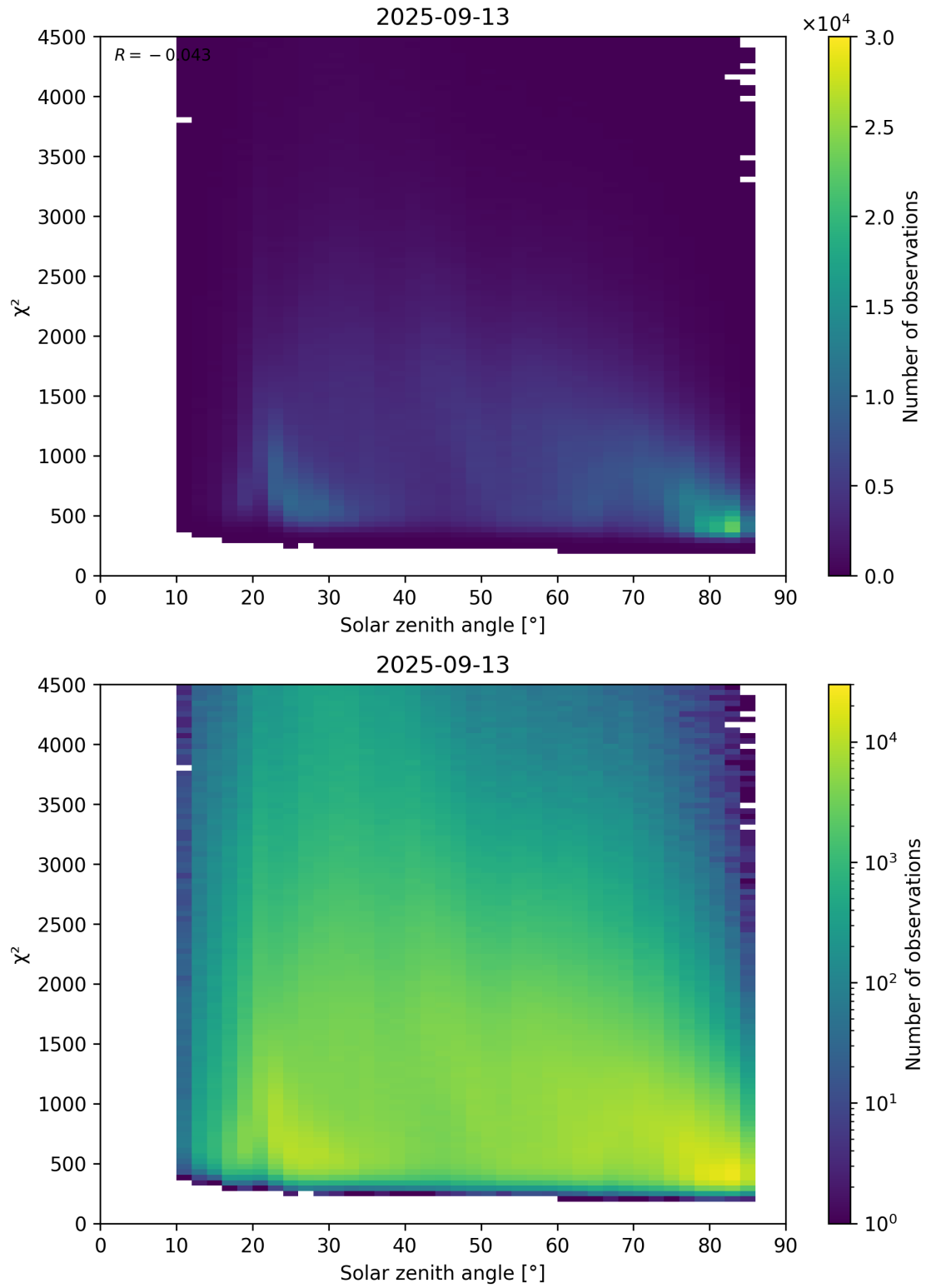
Figure 64: Scatter density plot of “Solar zenith angle” against “ \chi^2 ” for 2025-09-12 to 2025-09-14.
