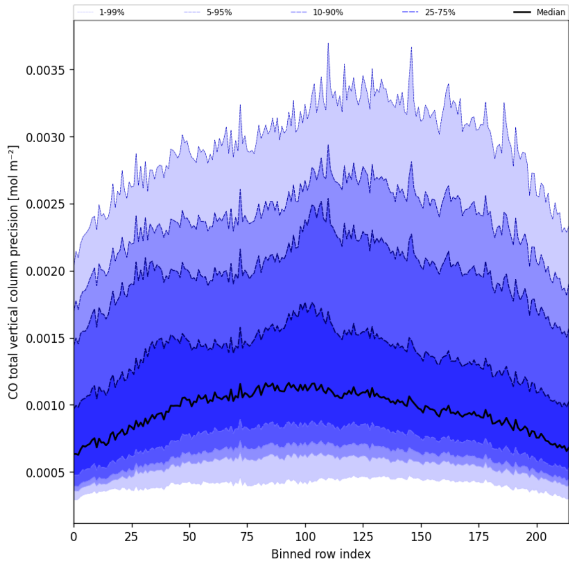
Figure 28: Along track statistics of “CO total vertical column precision” for 2025-09-12 to 2025-09-14
