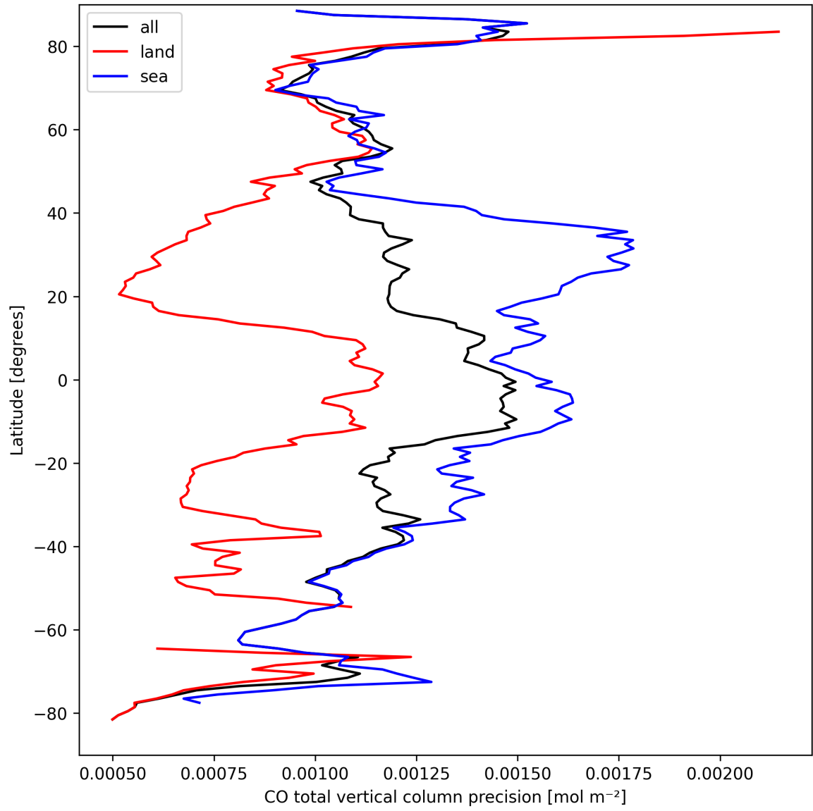
Figure 12: Zonal average of “CO total vertical column precision” for 2025-09-12 to 2025-09-14.
