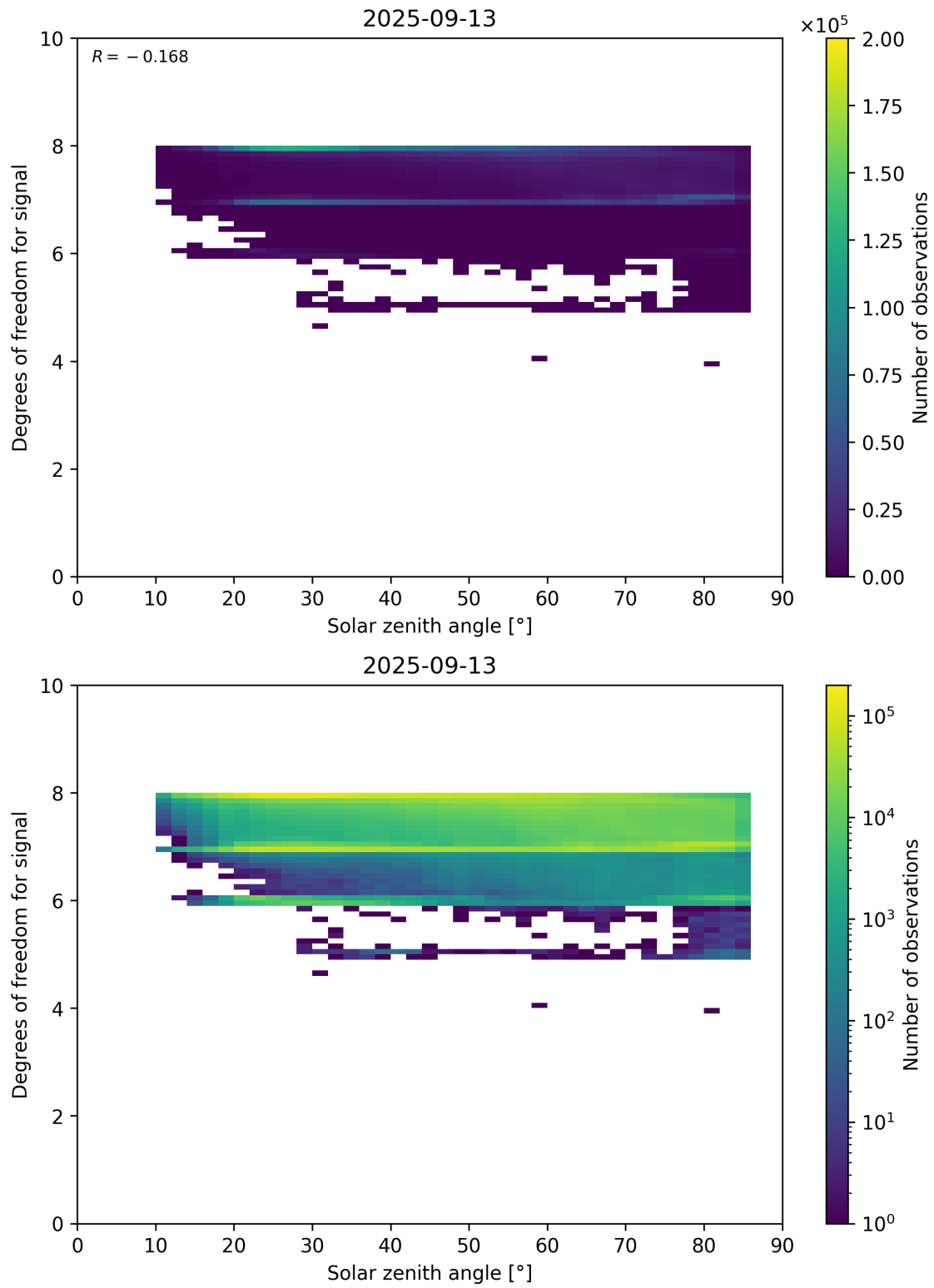
Figure 65: Scatter density plot of “Solar zenith angle” against “Degrees of freedom for signal” for 2025-09-12 to 2025-09-14.
