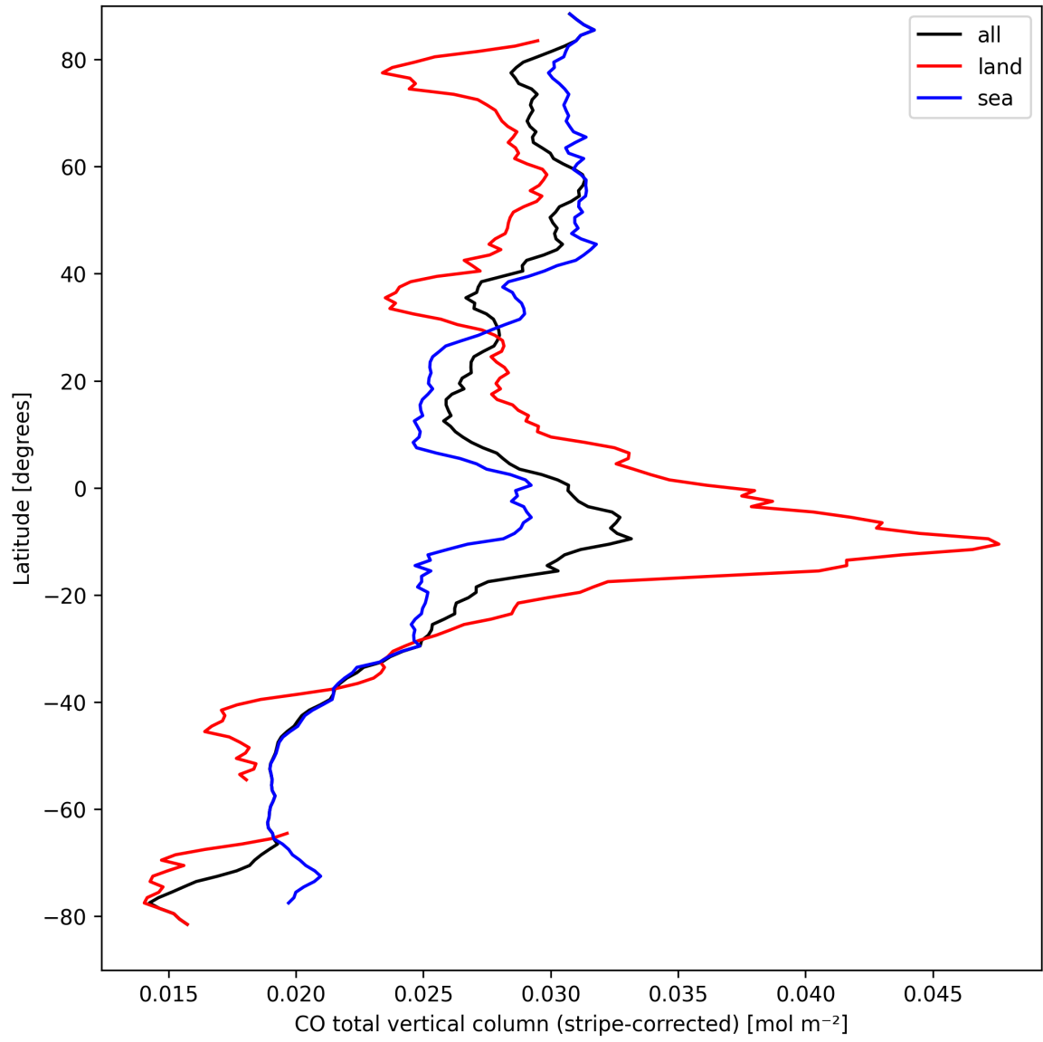
Figure 11: Zonal average of “CO total vertical column (stripe-corrected)” for 2025-09-12 to 2025-09-14.
