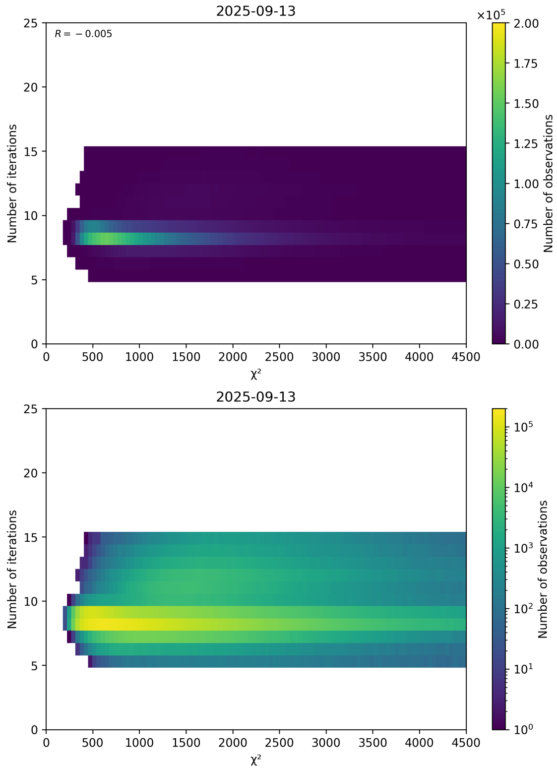
Figure 49: Scatter density plot of “ \chi^2 ” against “Number of iterations” for 2025-09-12 to 2025-09-14.
