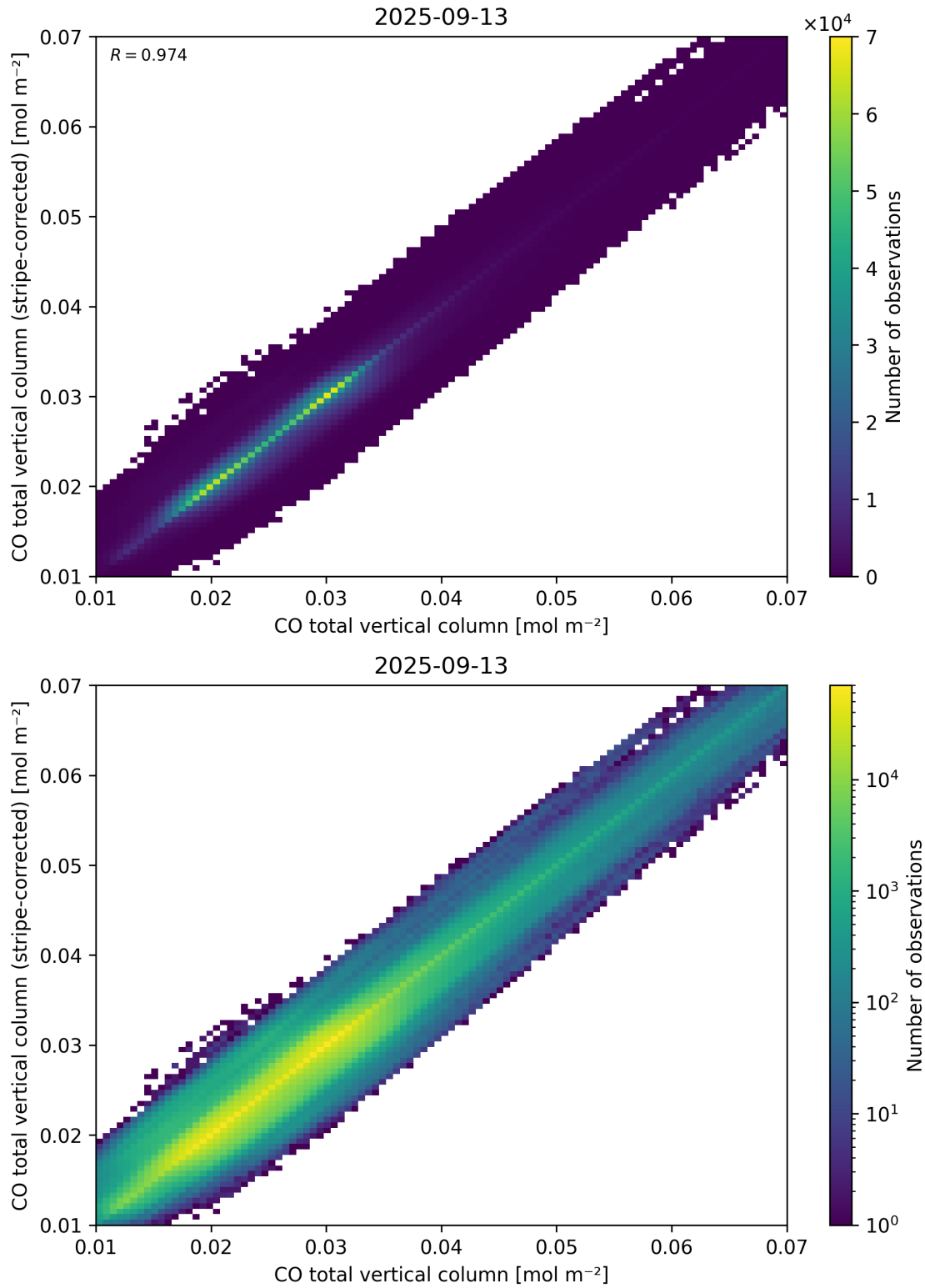
Figure 33: Scatter density plot of “CO total vertical column” against “CO total vertical column (stripe-corrected)” for 2025-09-12 to 2025-09-14.
