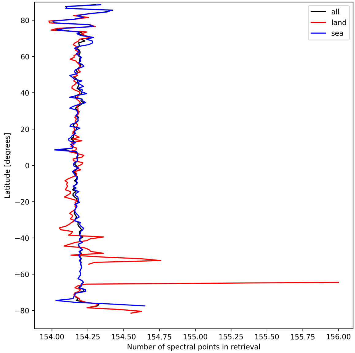
Figure 13: Zonal average of “Number of spectral points in retrieval” for 2025-09-12 to 2025-09-14.
