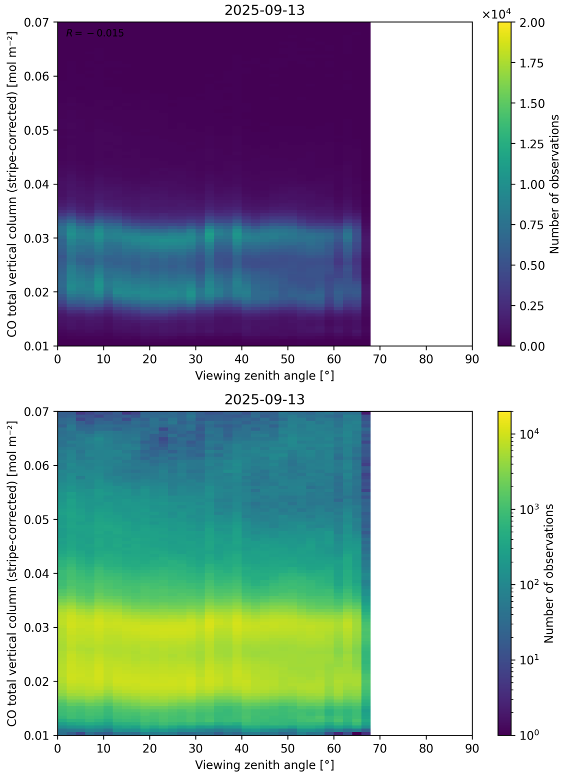
Figure 70: Scatter density plot of “Viewing zenith angle” against “CO total vertical column (stripe-corrected)” for 2025-09-12 to 2025-09-14.
