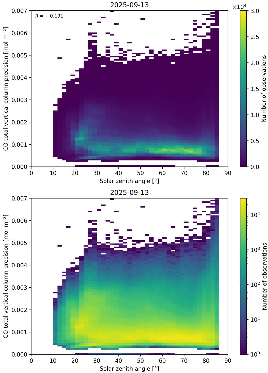
Figure 63: Scatter density plot of “Solar zenith angle” against “CO total vertical column precision” for 2025-09-12 to 2025-09-14.
