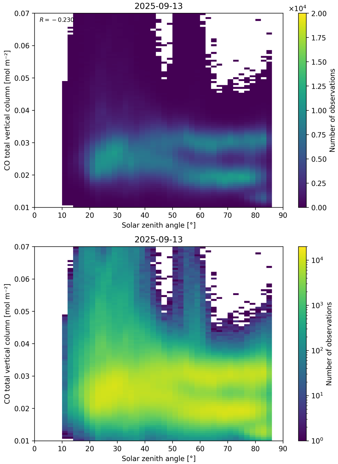
Figure 61: Scatter density plot of “Solar zenith angle” against “CO total vertical column” for 2025-09-12 to 2025-09-14.
