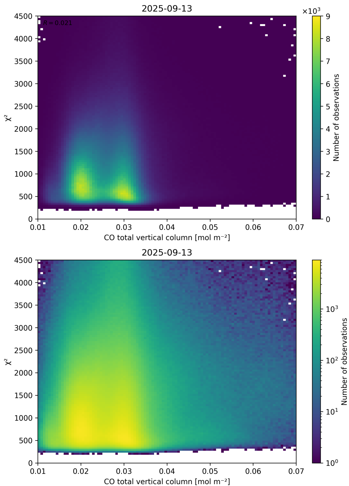
Figure 35: Scatter density plot of “CO total vertical column” against “ \chi^2 ” for 2025-09-12 to 2025-09-14.
