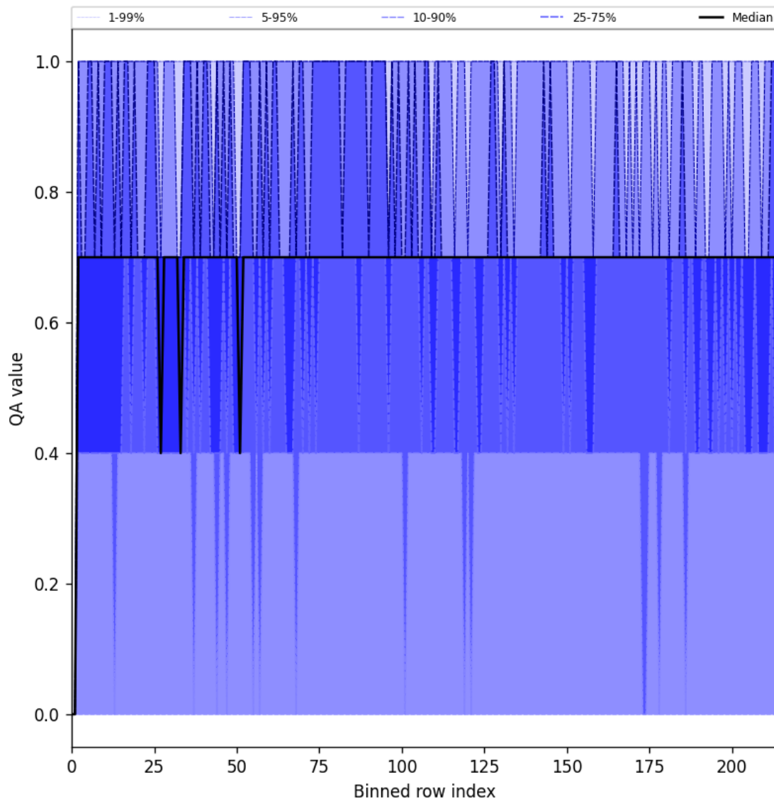
Figure 25: Along track statistics of “QA value” for 2025-09-12 to 2025-09-14
