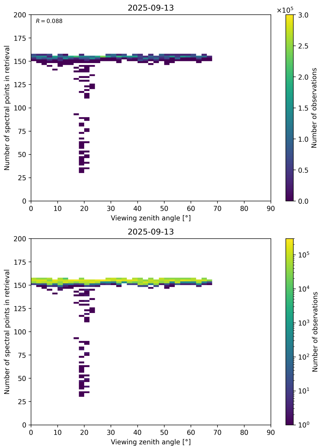
Figure 76: Scatter density plot of “Viewing zenith angle” against “Number of spectral points in retrieval” for 2025-09-12 to 2025-09-14.
