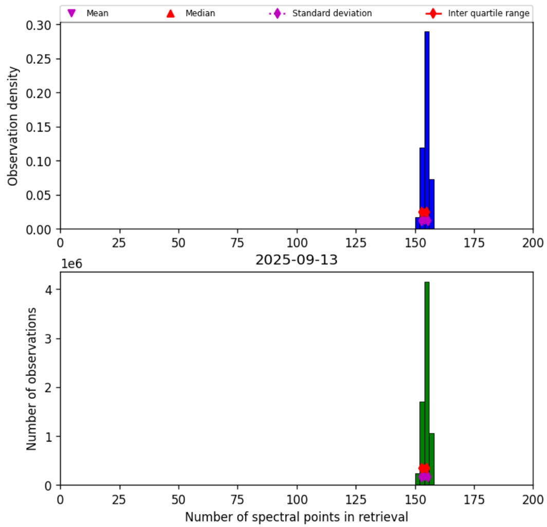
Figure 21: Histogram of “Number of spectral points in retrieval” for 2025-09-12 to 2025-09-14
