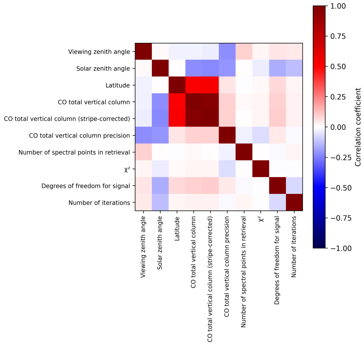
Figure 2: Map of correlation matrix for 2025-09-13 to 2025-09-15.
