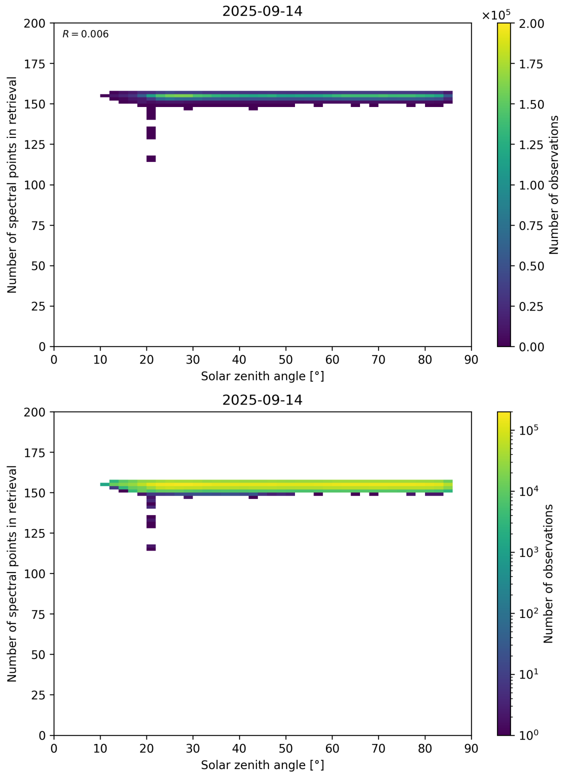
Figure 68: Scatter density plot of “Solar zenith angle” against “Number of spectral points in retrieval” for 2025-09-13 to 2025-09-15.
