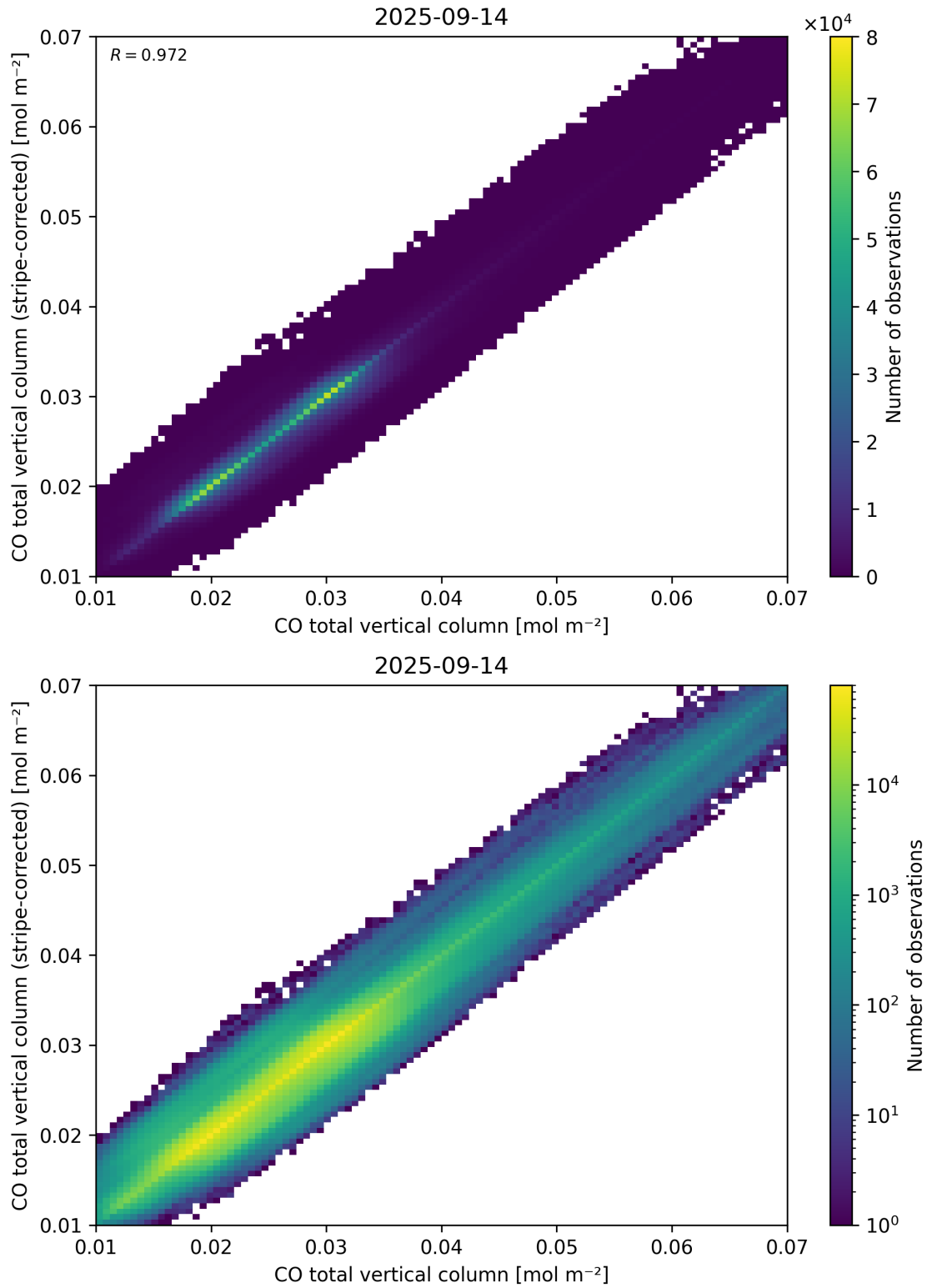
Figure 33: Scatter density plot of “CO total vertical column” against “CO total vertical column (stripe-corrected)” for 2025-09-13 to 2025-09-15.
