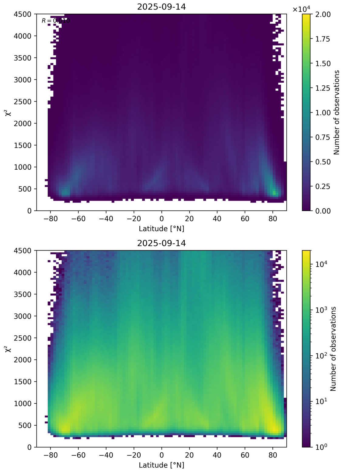
Figure 54: Scatter density plot of “Latitude” against “ \chi^2 ” for 2025-09-13 to 2025-09-15.
