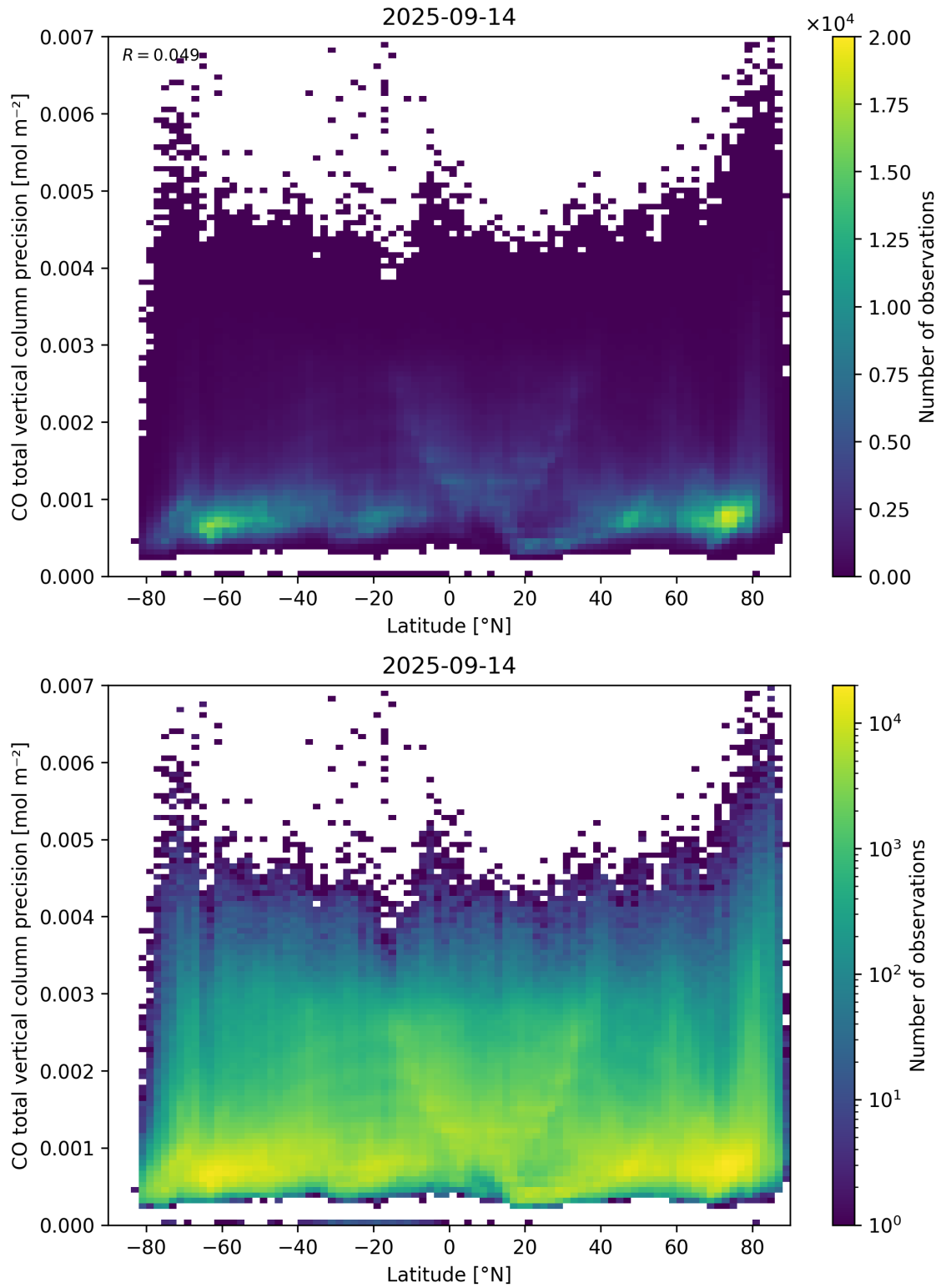
Figure 53: Scatter density plot of “Latitude” against “CO total vertical column precision” for 2025-09-13 to 2025-09-15.
