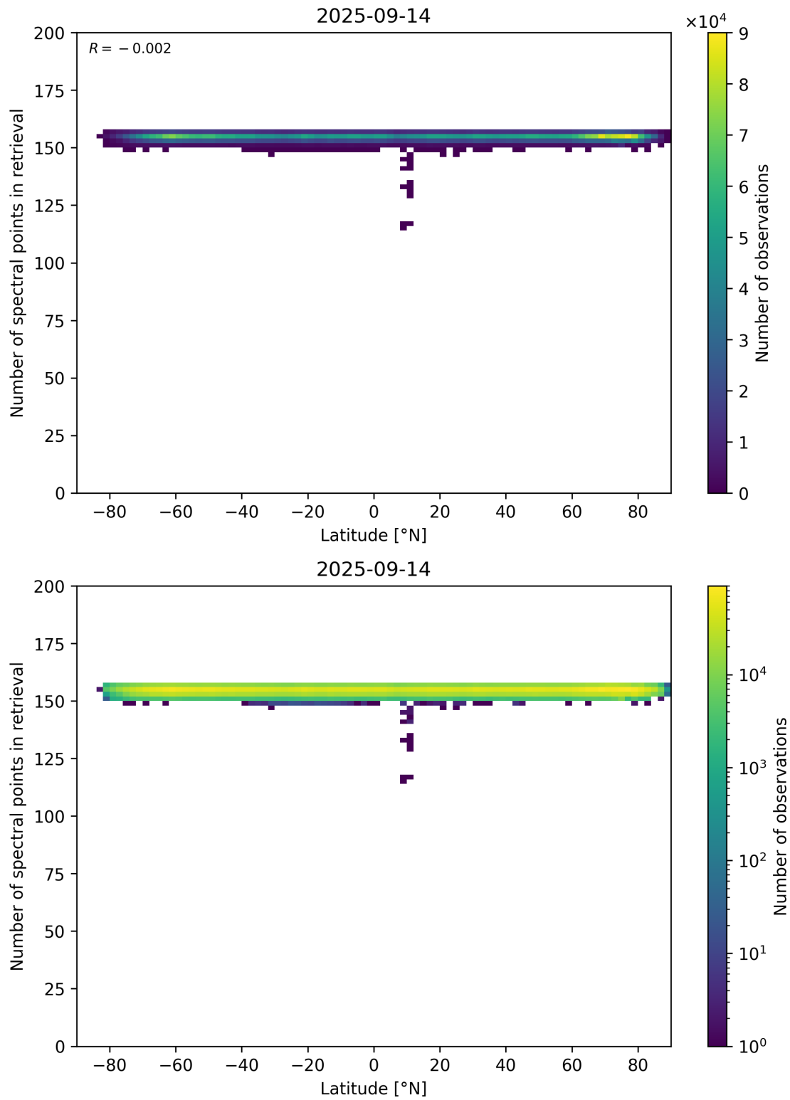
Figure 57: Scatter density plot of “Latitude” against “Number of spectral points in retrieval” for 2025-09-13 to 2025-09-15.
