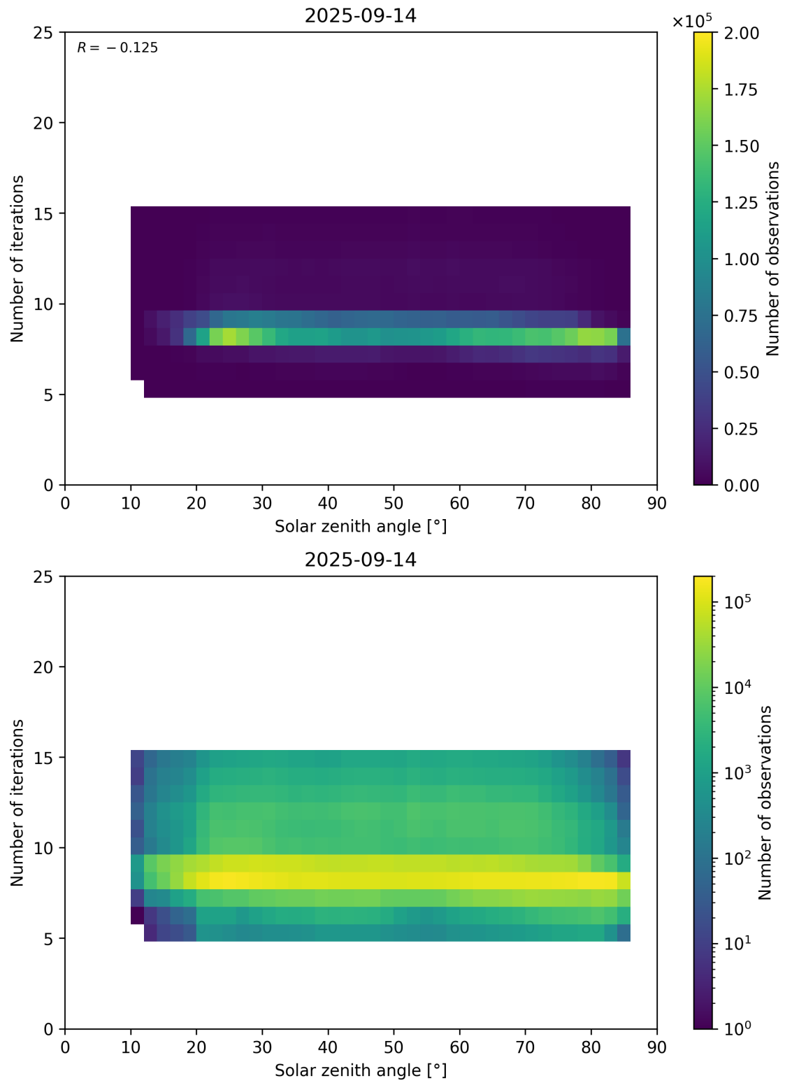
Figure 67: Scatter density plot of “Solar zenith angle” against “Number of iterations” for 2025-09-13 to 2025-09-15.
