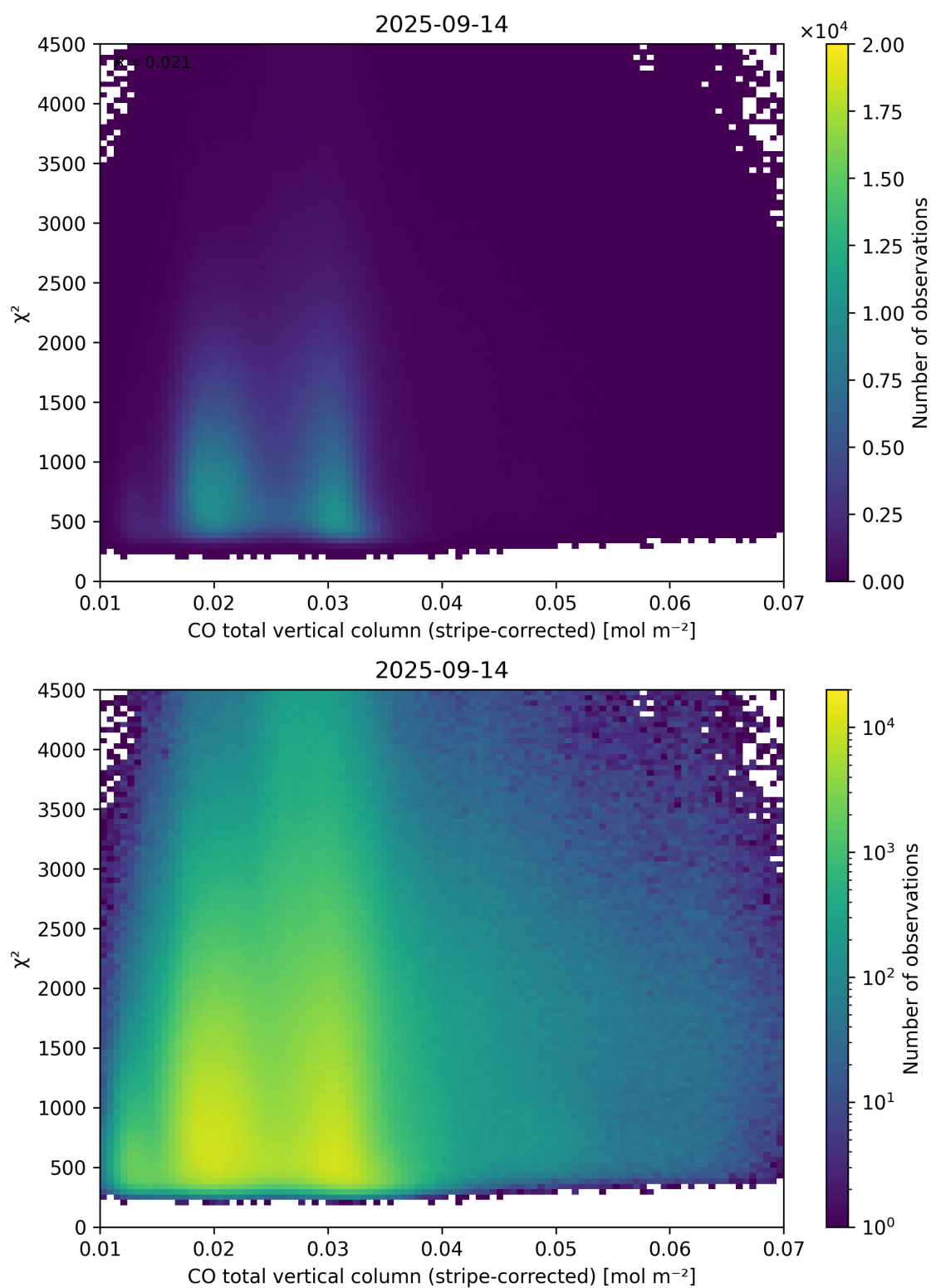
Figure 37: Scatter density plot of “CO total vertical column (stripe-corrected)” against “ \chi^2 ” for 2025-09-13 to 2025-09-15.
