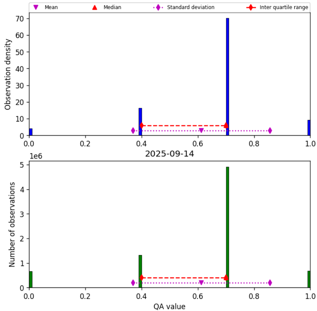
Figure 17: Histogram of “QA value” for 2025-09-13 to 2025-09-15
