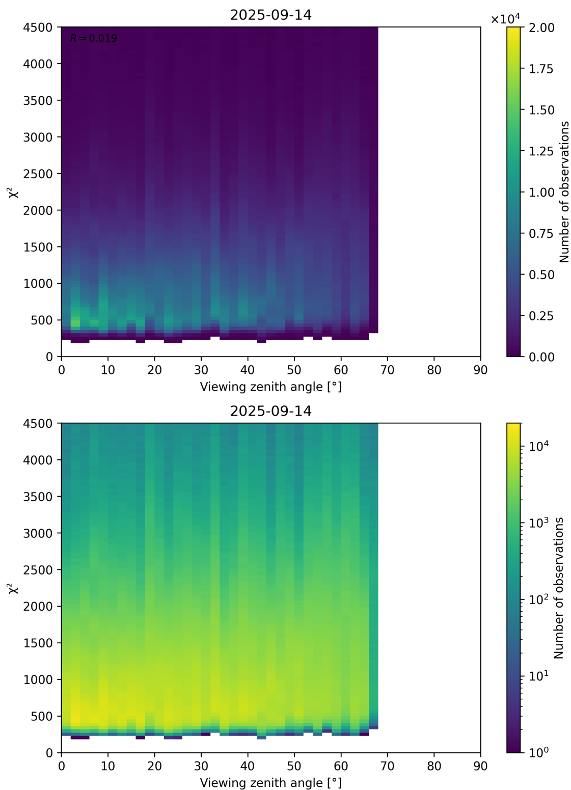
Figure 72: Scatter density plot of “Viewing zenith angle” against “ \chi^2 ” for 2025-09-13 to 2025-09-15.
