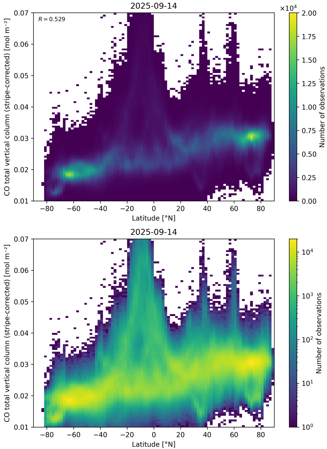
Figure 52: Scatter density plot of “Latitude” against “CO total vertical column (stripe-corrected)” for 2025-09-13 to 2025-09-15.
