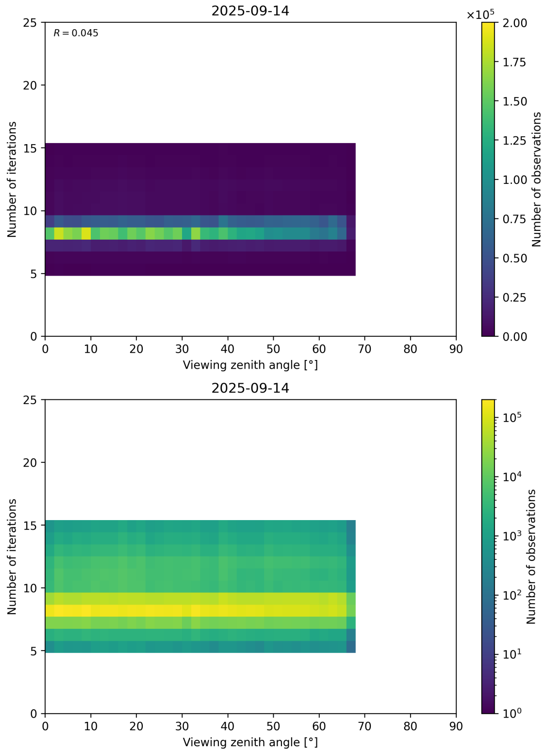
Figure 75: Scatter density plot of “Viewing zenith angle” against “Number of iterations” for 2025-09-13 to 2025-09-15.
