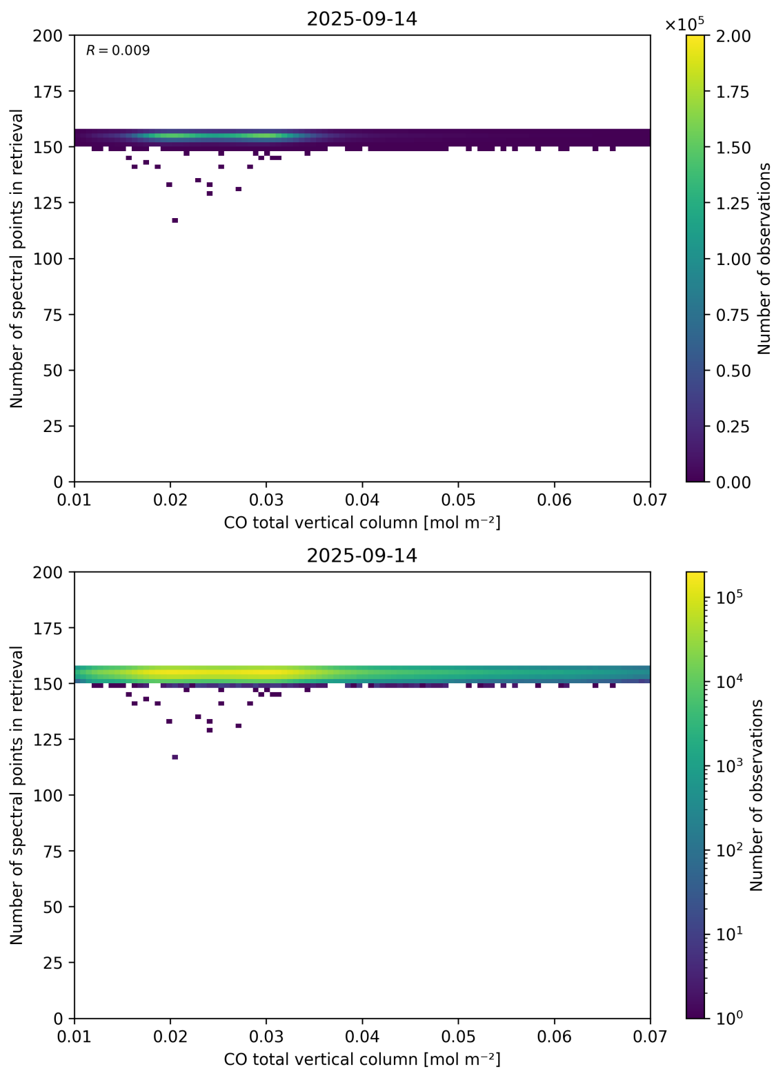
Figure 43: Scatter density plot of “CO total vertical column” against “Number of spectral points in retrieval” for 2025-09-13 to 2025-09-15.
