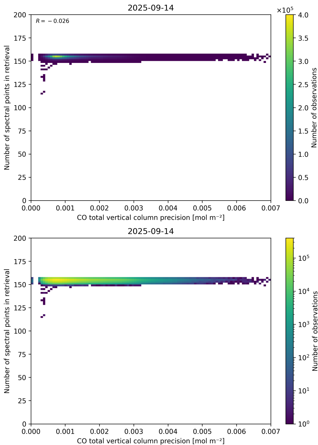
Figure 47: Scatter density plot of “CO total vertical column precision” against “Number of spectral points in retrieval” for 2025-09-13 to 2025-09-15.
