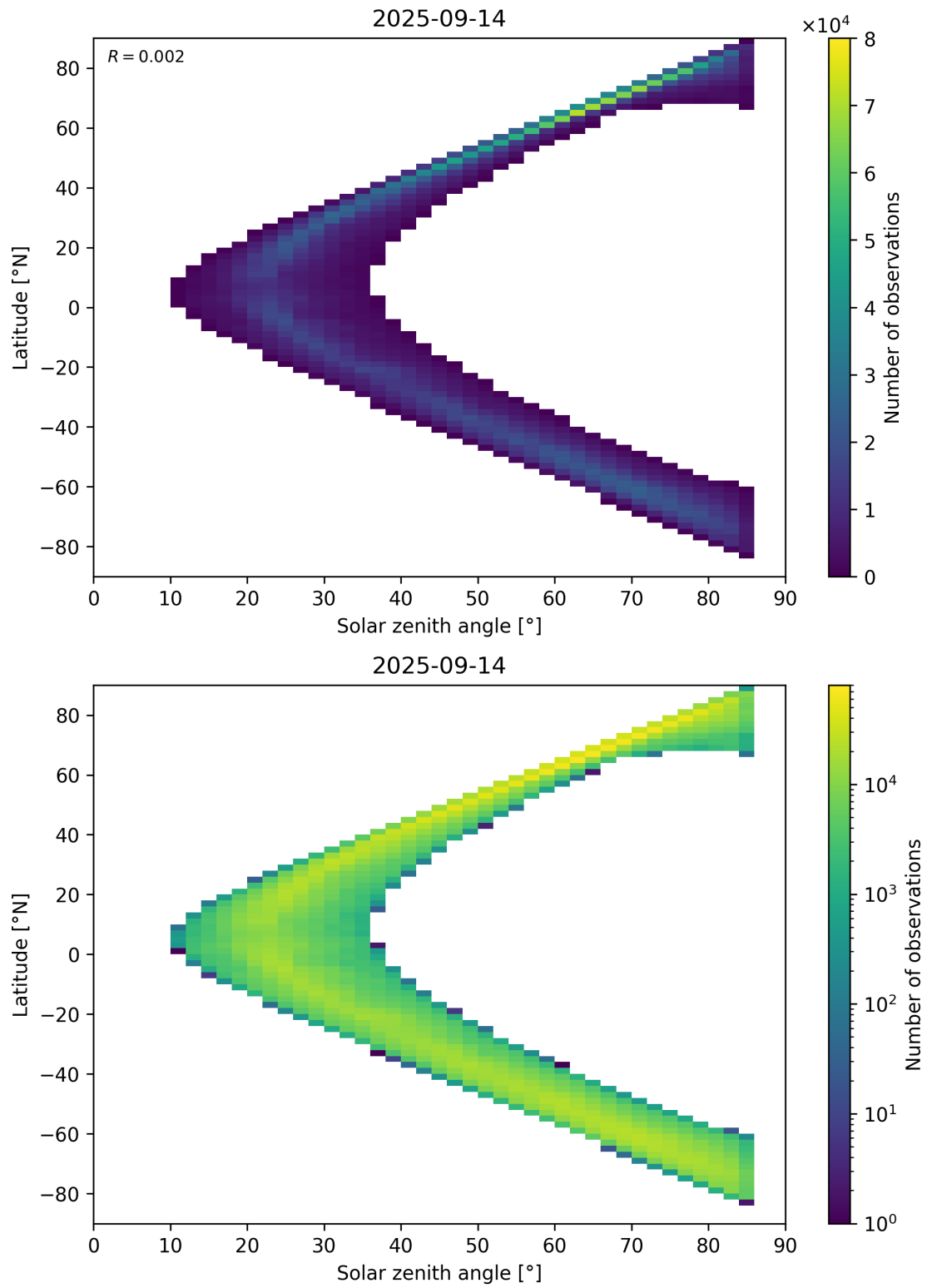
Figure 66: Scatter density plot of “Solar zenith angle” against “Latitude” for 2025-09-13 to 2025-09-15.
