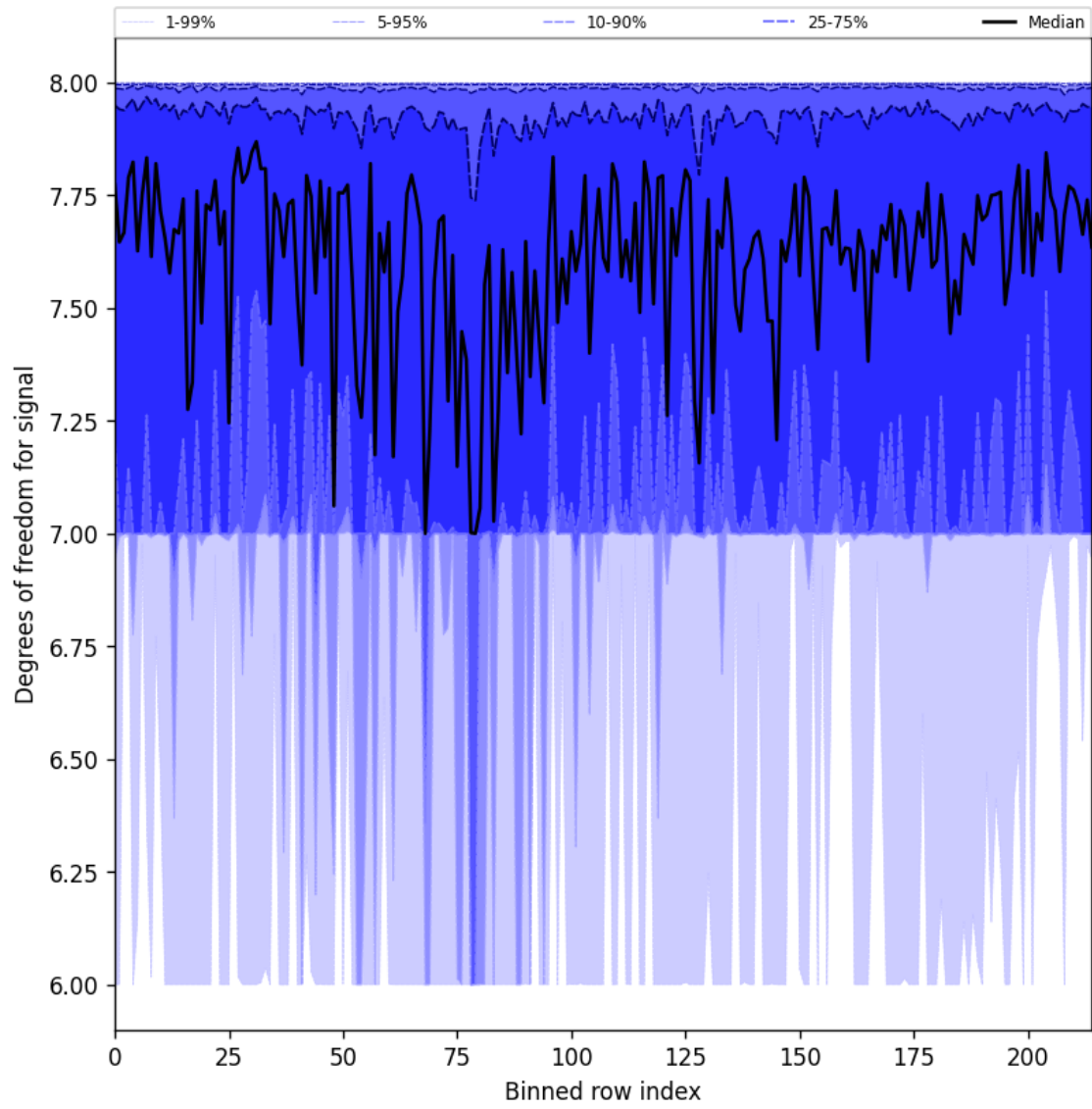
Figure 31: Along track statistics of “Degrees of freedom for signal” for 2025-09-13 to 2025-09-15
