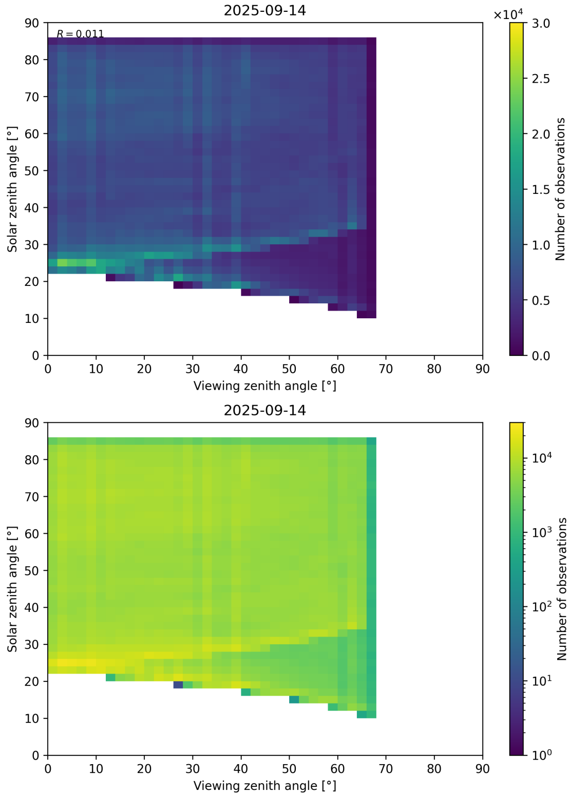
Figure 77: Scatter density plot of “Viewing zenith angle” against “Solar zenith angle” for 2025-09-13 to 2025-09-15.
