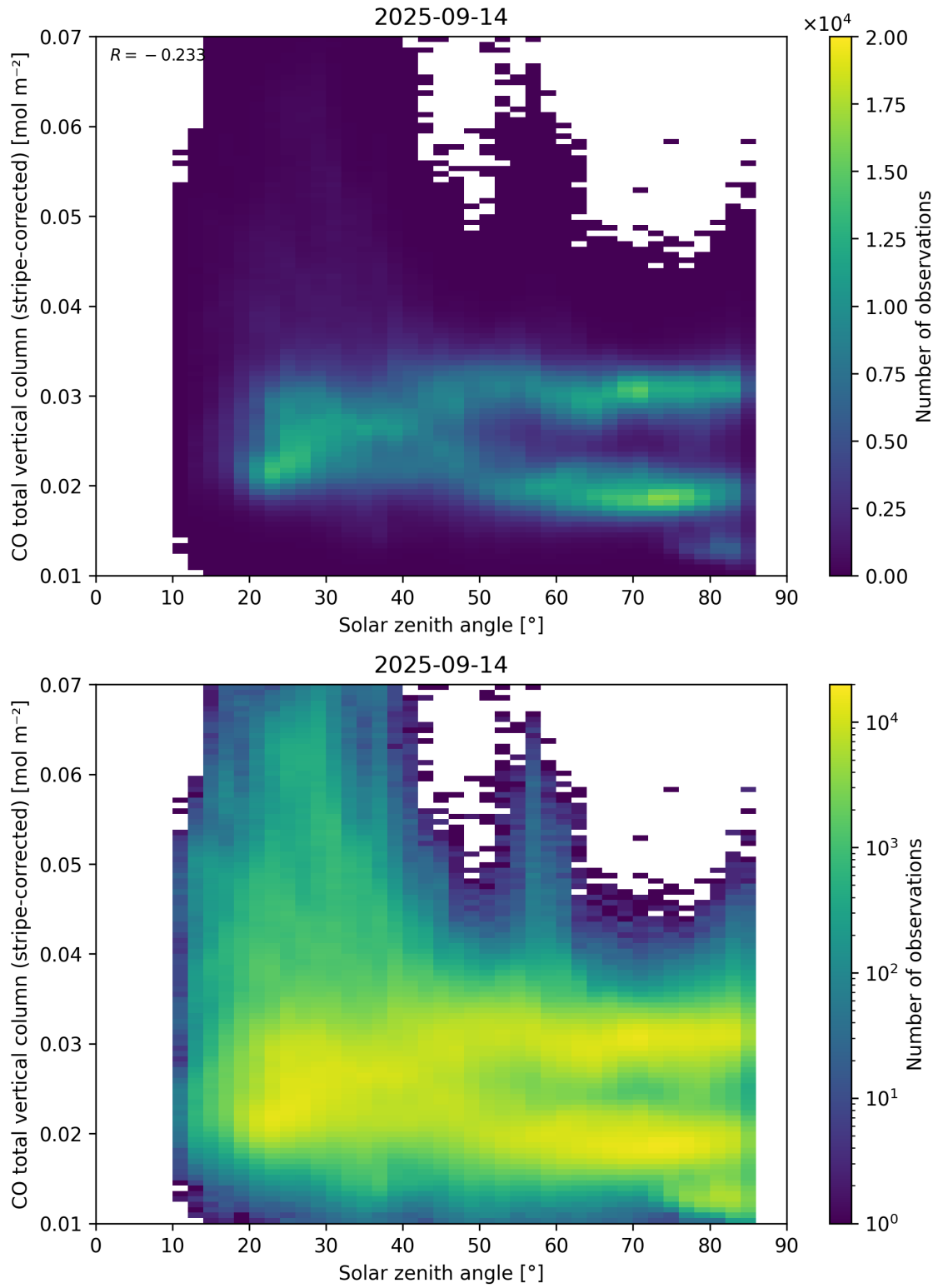
Figure 62: Scatter density plot of “Solar zenith angle” against “CO total vertical column (stripe-corrected)” for 2025-09-13 to 2025-09-15.
