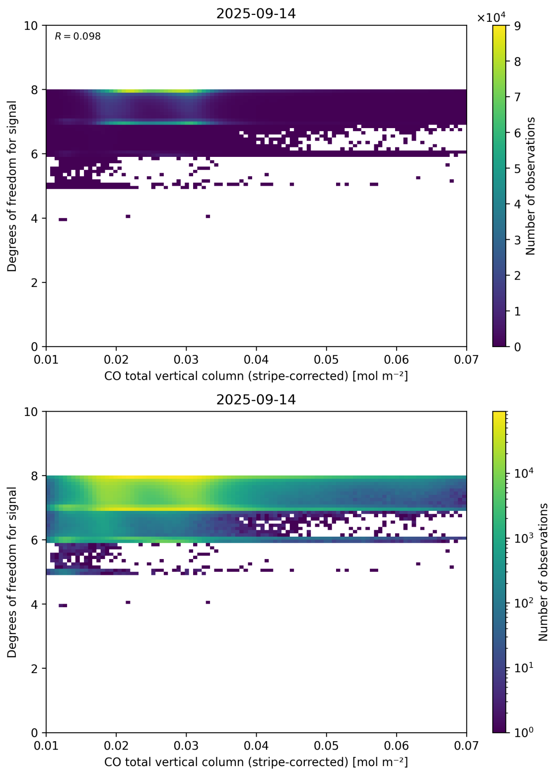
Figure 38: Scatter density plot of “CO total vertical column (stripe-corrected)” against “Degrees of freedom for signal” for 2025-09-13 to 2025-09-15.
