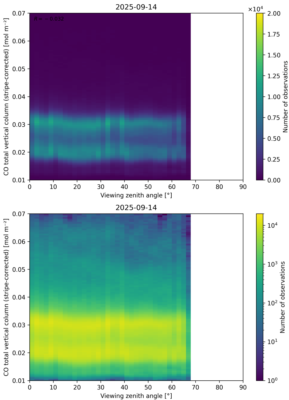
Figure 70: Scatter density plot of “Viewing zenith angle” against “CO total vertical column (stripe-corrected)” for 2025-09-13 to 2025-09-15.
