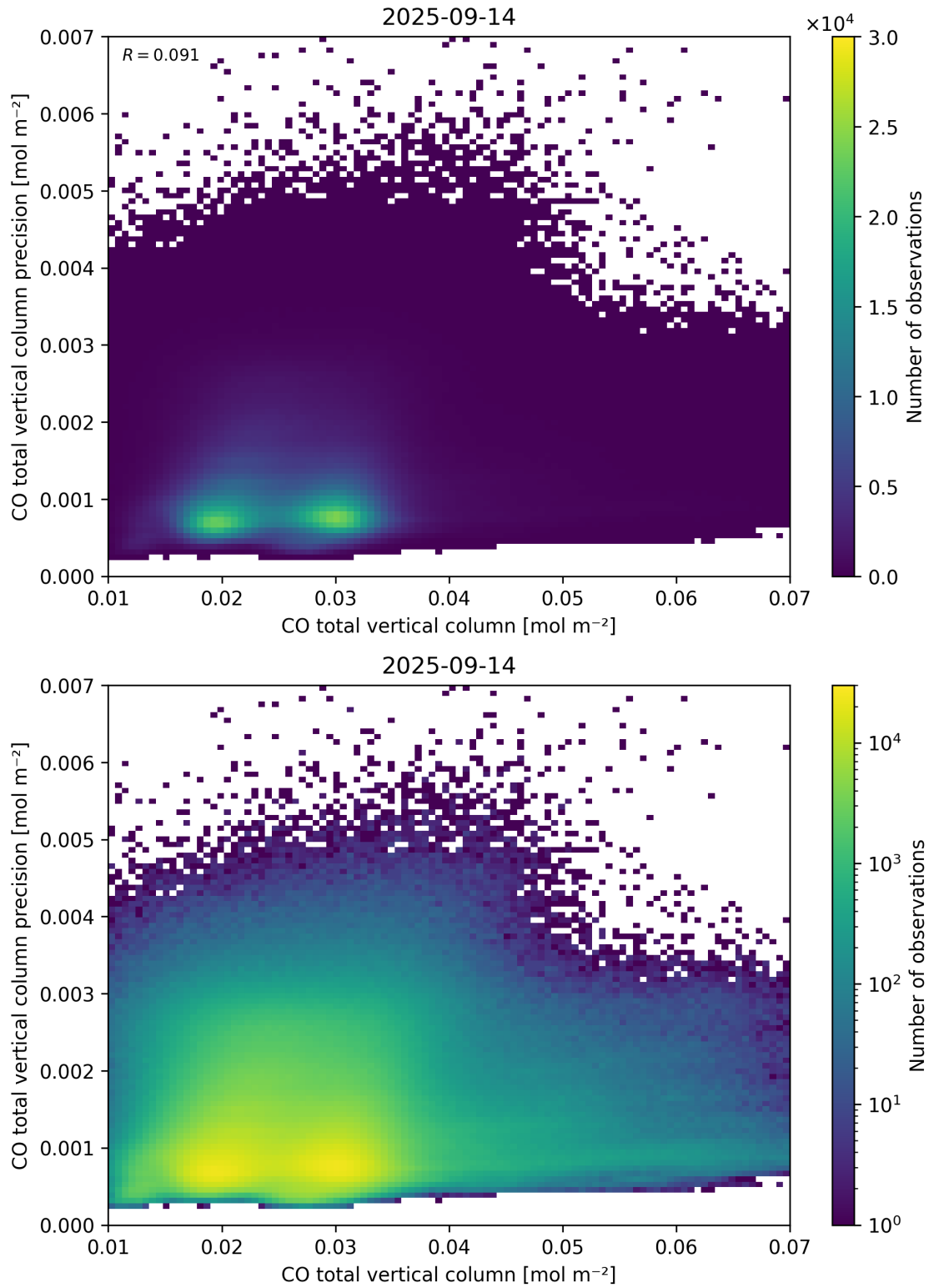
Figure 34: Scatter density plot of “CO total vertical column” against “CO total vertical column precision” for 2025-09-13 to 2025-09-15.
