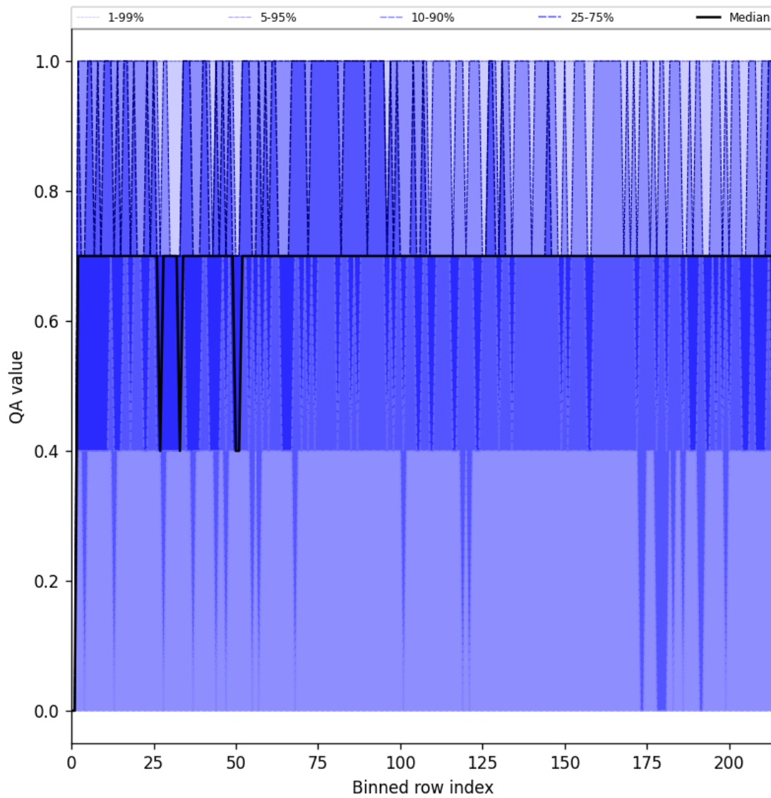
Figure 25: Along track statistics of “QA value” for 2025-09-13 to 2025-09-15
