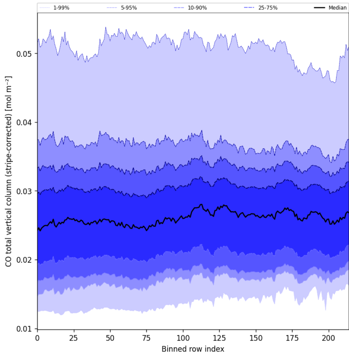
Figure 27: Along track statistics of “CO total vertical column (stripe-corrected)” for 2025-09-13 to 2025-09-15
