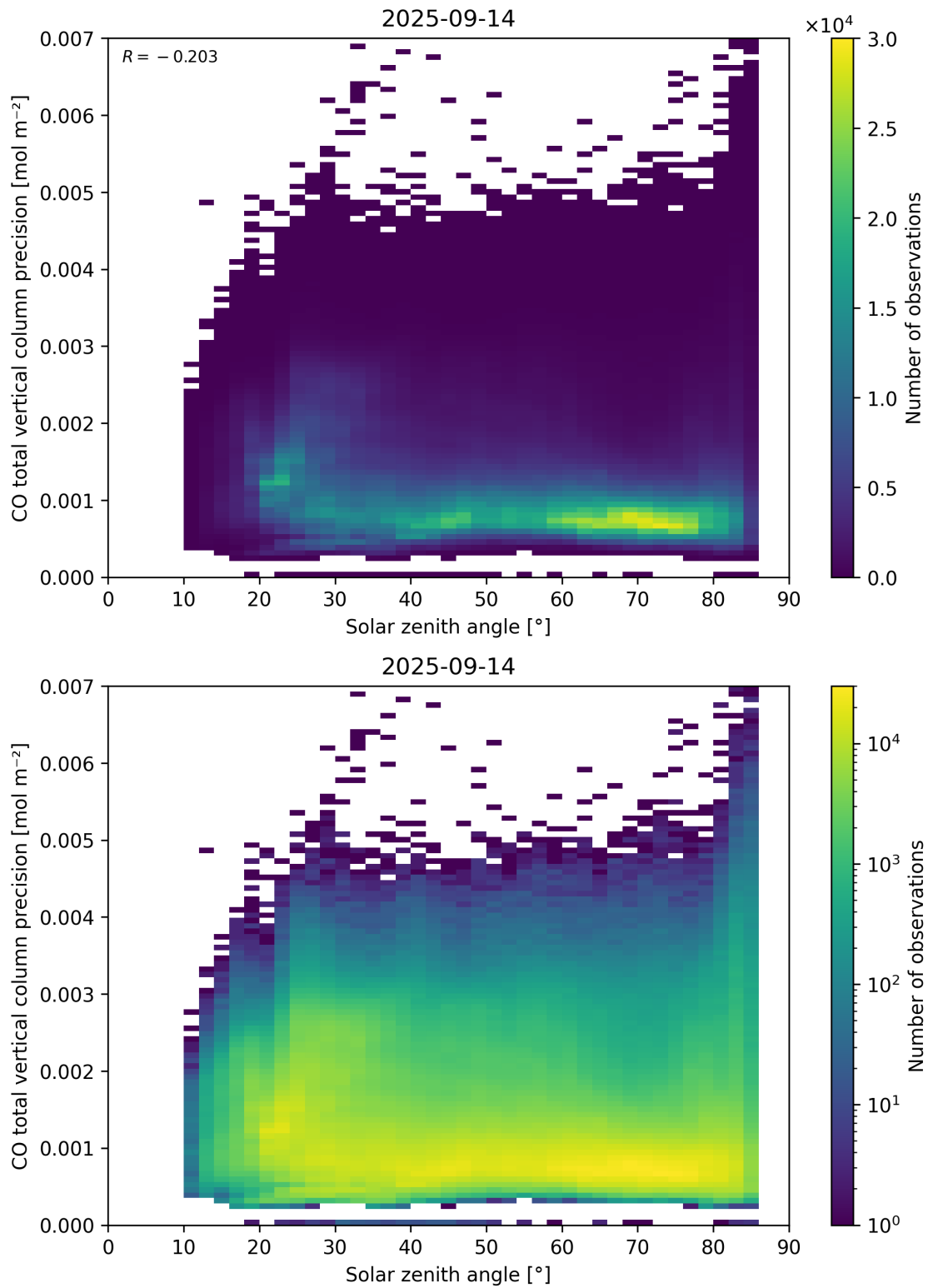
Figure 63: Scatter density plot of “Solar zenith angle” against “CO total vertical column precision” for 2025-09-13 to 2025-09-15.
