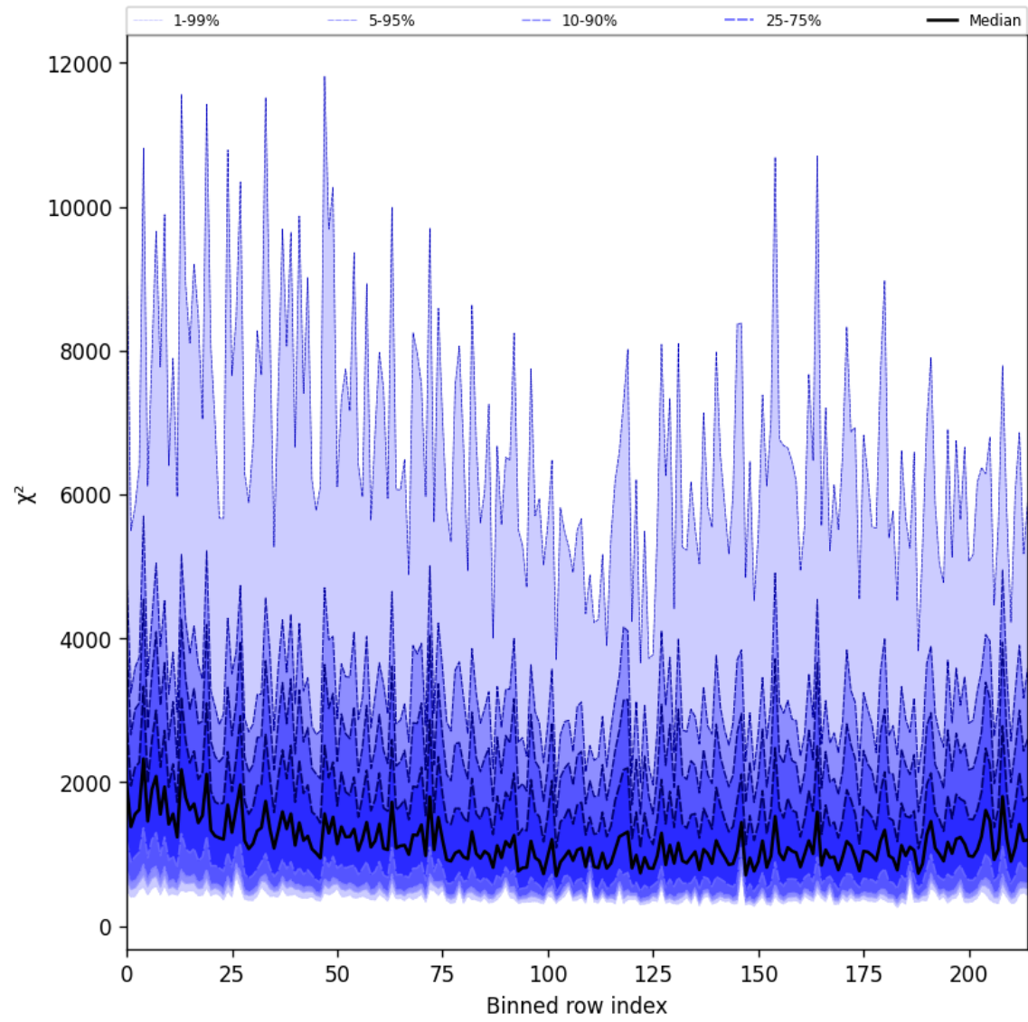
Figure 30: Along track statistics of “ \chi^2 ” for 2025-09-13 to 2025-09-15
