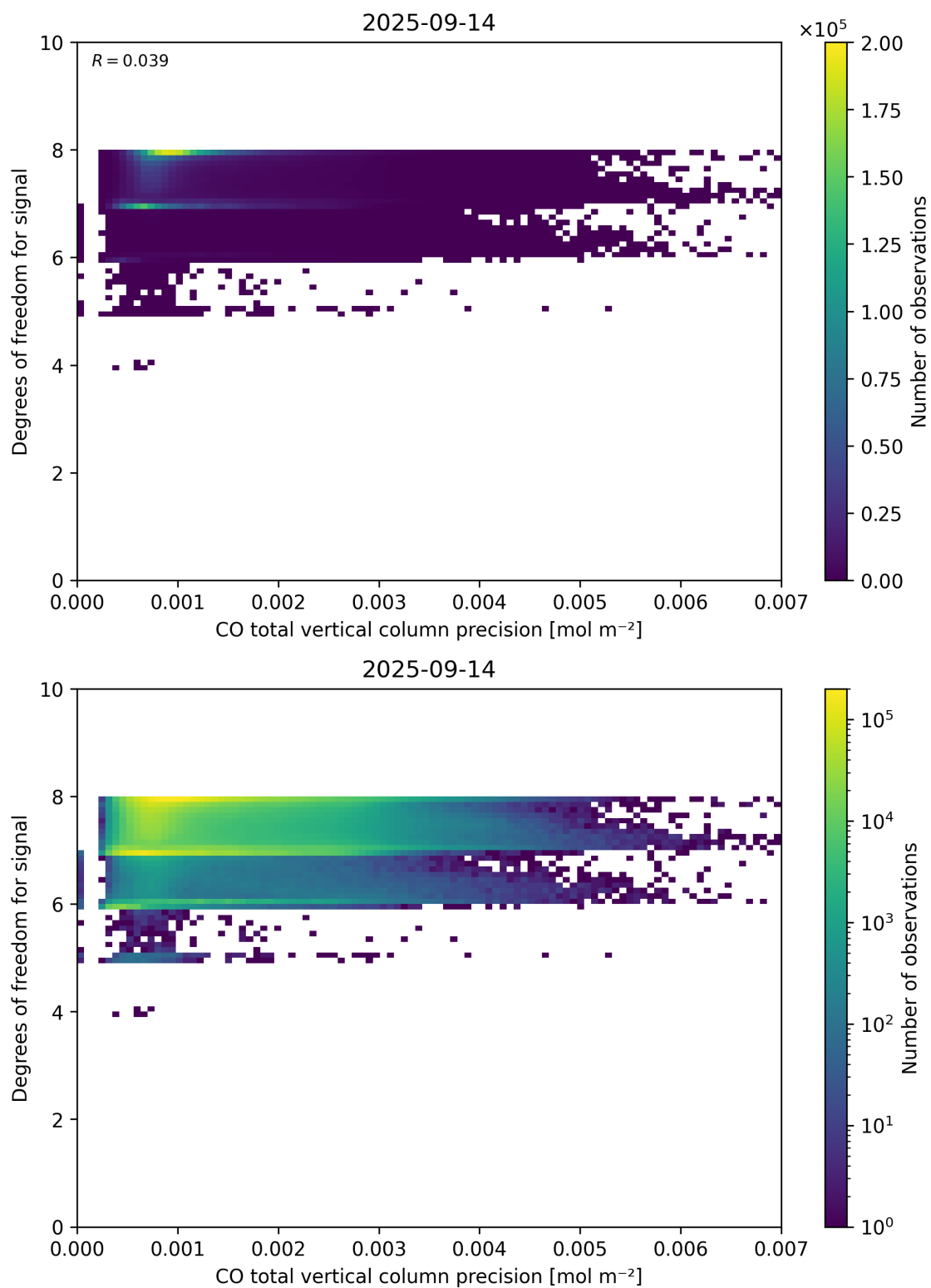
Figure 45: Scatter density plot of “CO total vertical column precision” against “Degrees of freedom for signal” for 2025-09-13 to 2025-09-15.
