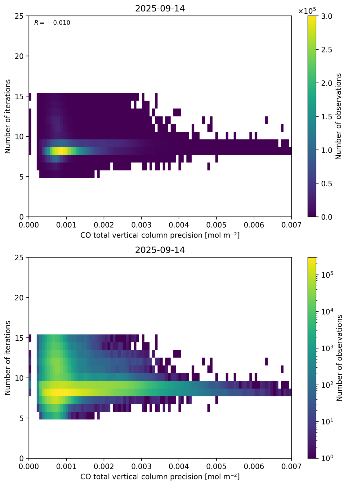
Figure 46: Scatter density plot of “CO total vertical column precision” against “Number of iterations” for 2025-09-13 to 2025-09-15.
