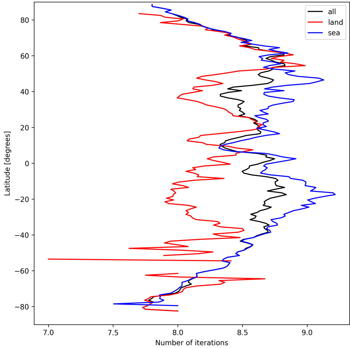
Figure 16: Zonal average of “Number of iterations” for 2025-09-13 to 2025-09-15.
