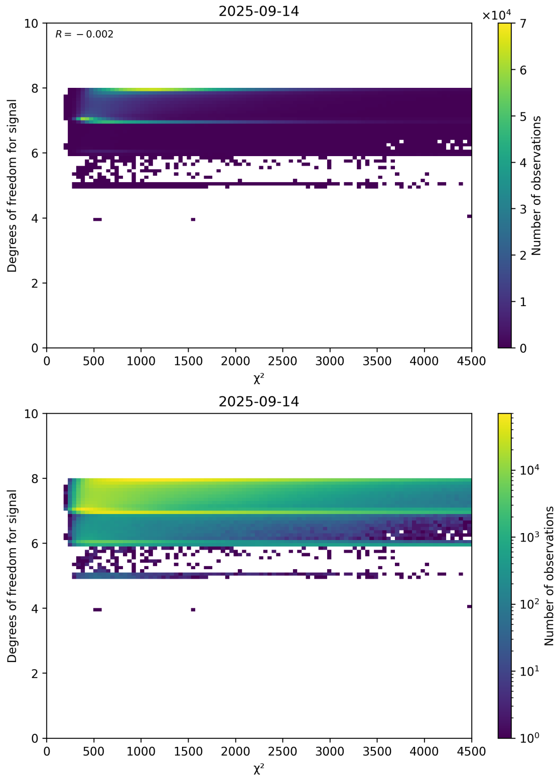
Figure 48: Scatter density plot of “ \chi^2 ” against “Degrees of freedom for signal” for 2025-09-13 to 2025-09-15.
