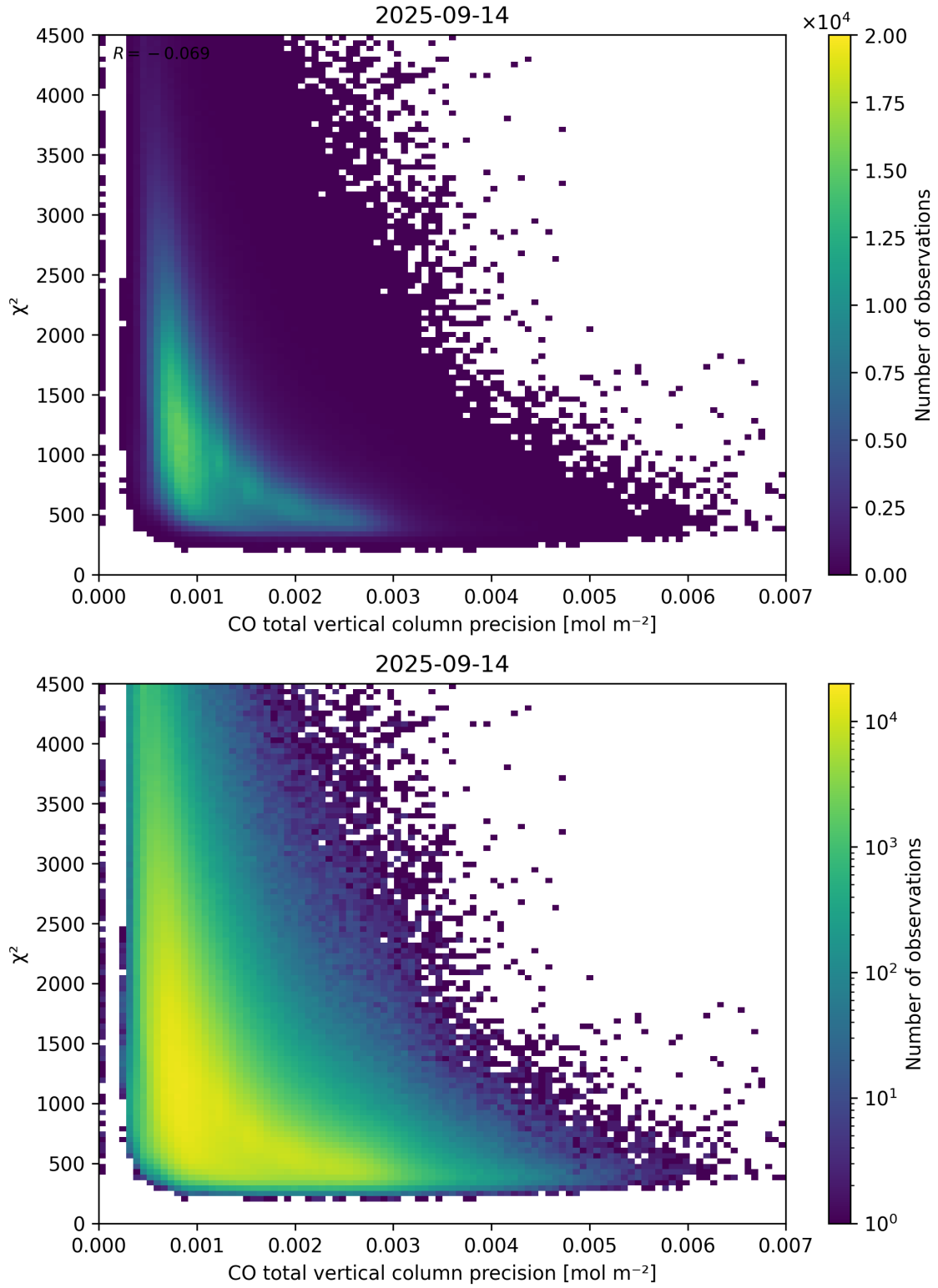
Figure 44: Scatter density plot of “CO total vertical column precision” against “ \chi^2 ” for 2025-09-13 to 2025-09-15.
