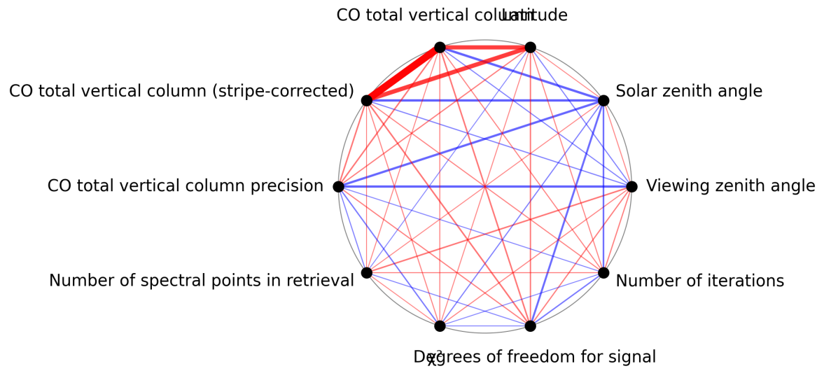
Figure 1: Map of correlation graph for 2025-09-13 to 2025-09-15.
