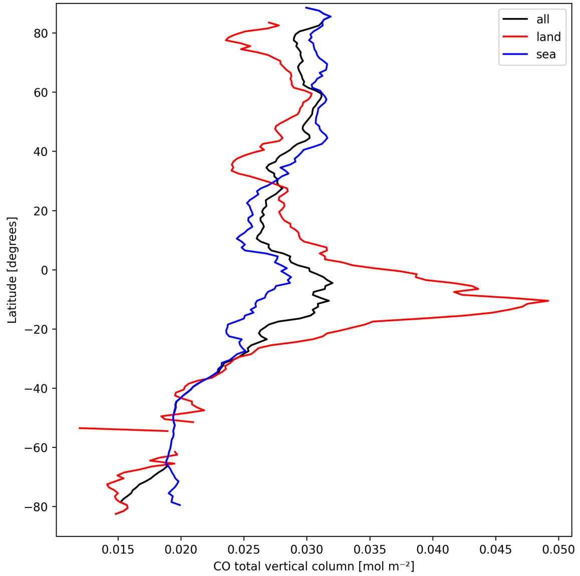
Figure 10: Zonal average of “CO total vertical column” for 2025-09-13 to 2025-09-15.
