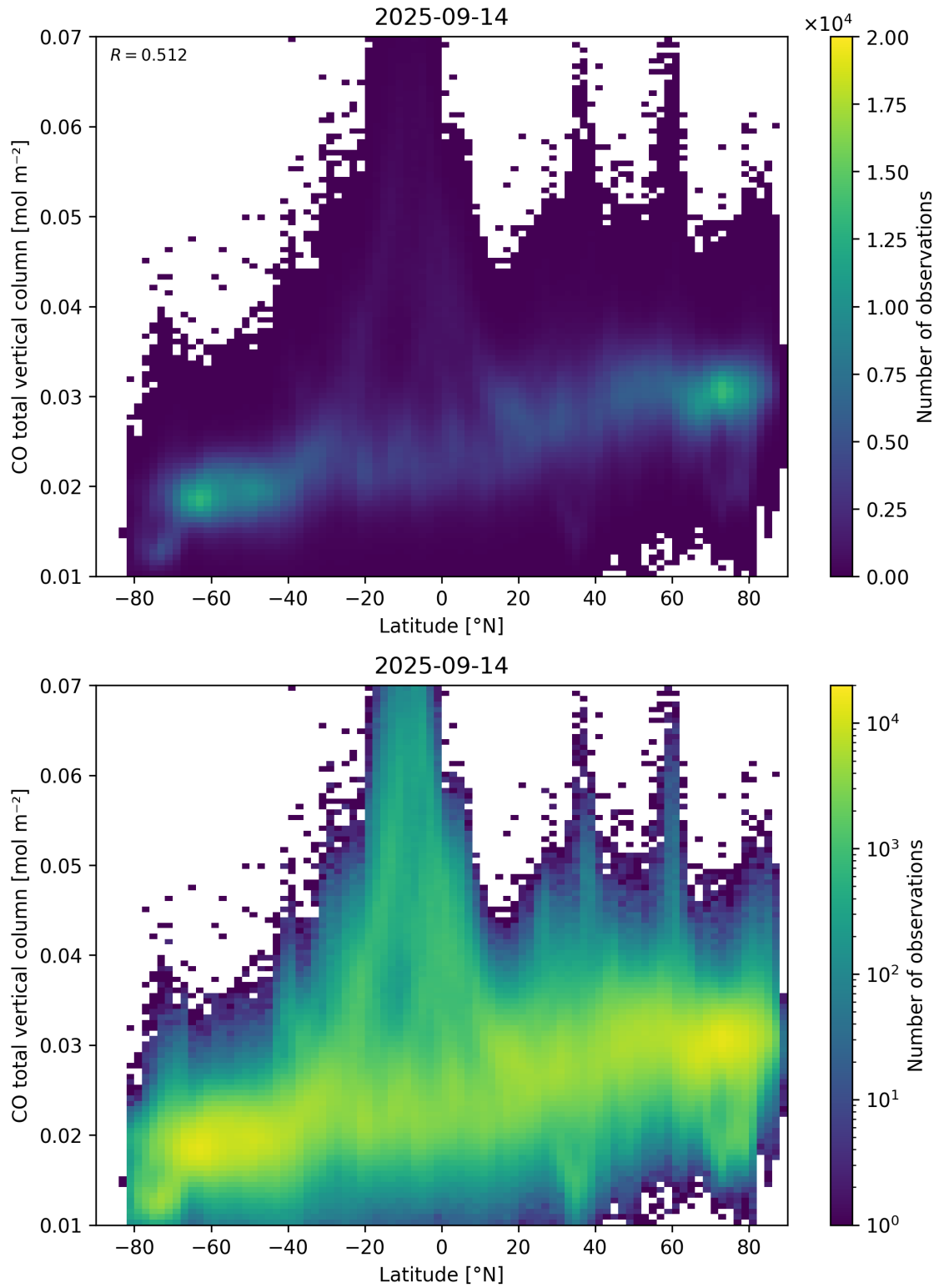
Figure 51: Scatter density plot of “Latitude” against “CO total vertical column” for 2025-09-13 to 2025-09-15.
