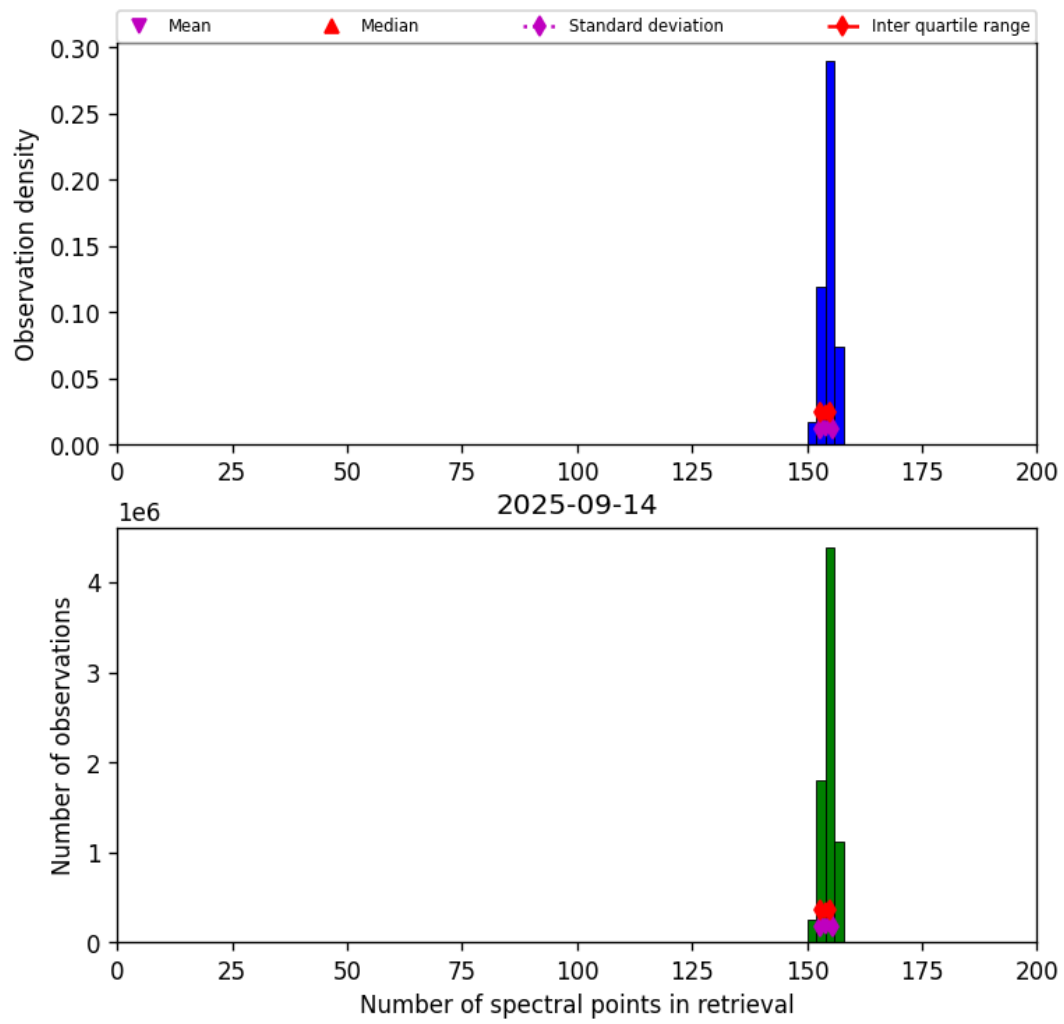
Figure 21: Histogram of “Number of spectral points in retrieval” for 2025-09-13 to 2025-09-15
