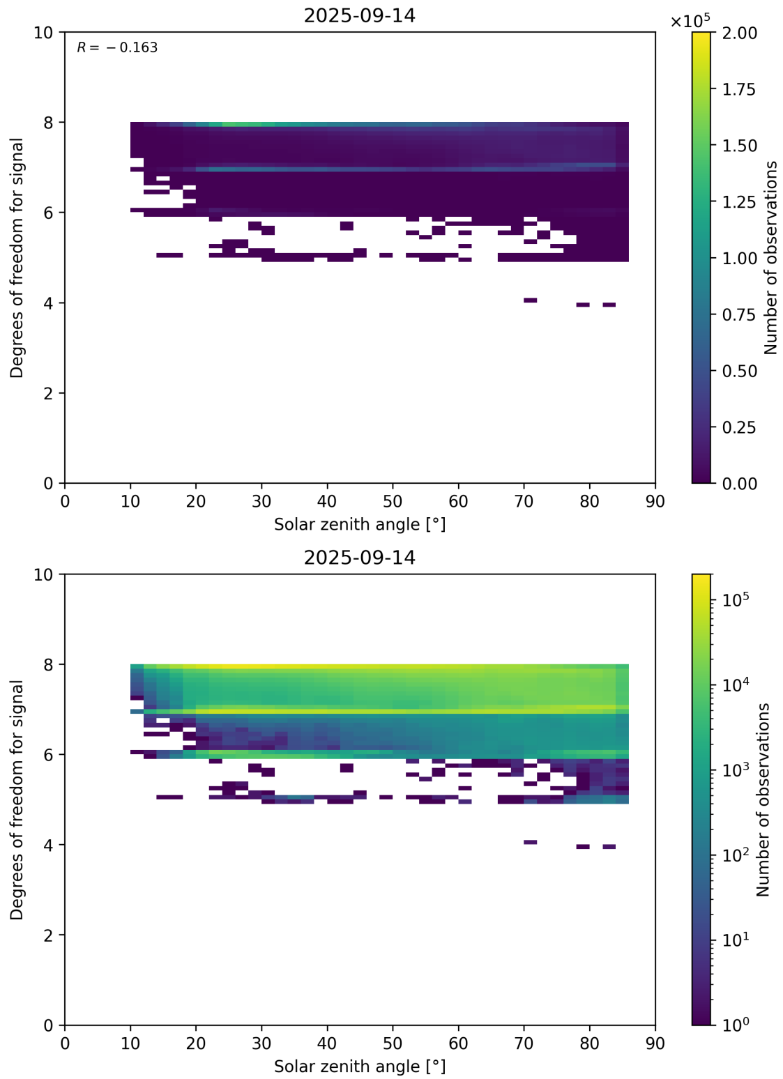
Figure 65: Scatter density plot of “Solar zenith angle” against “Degrees of freedom for signal” for 2025-09-13 to 2025-09-15.
