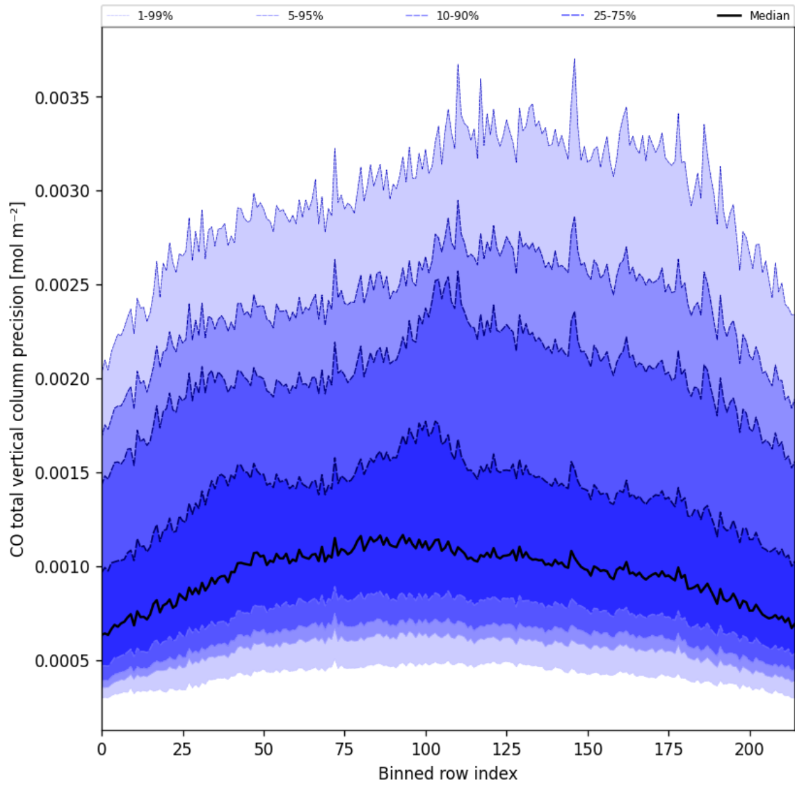
Figure 28: Along track statistics of “CO total vertical column precision” for 2025-09-13 to 2025-09-15
