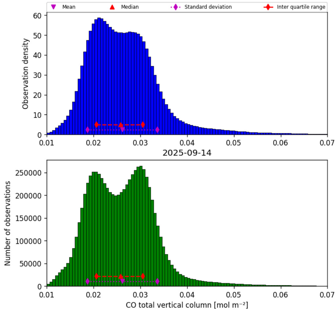
Figure 18: Histogram of “CO total vertical column” for 2025-09-13 to 2025-09-15
