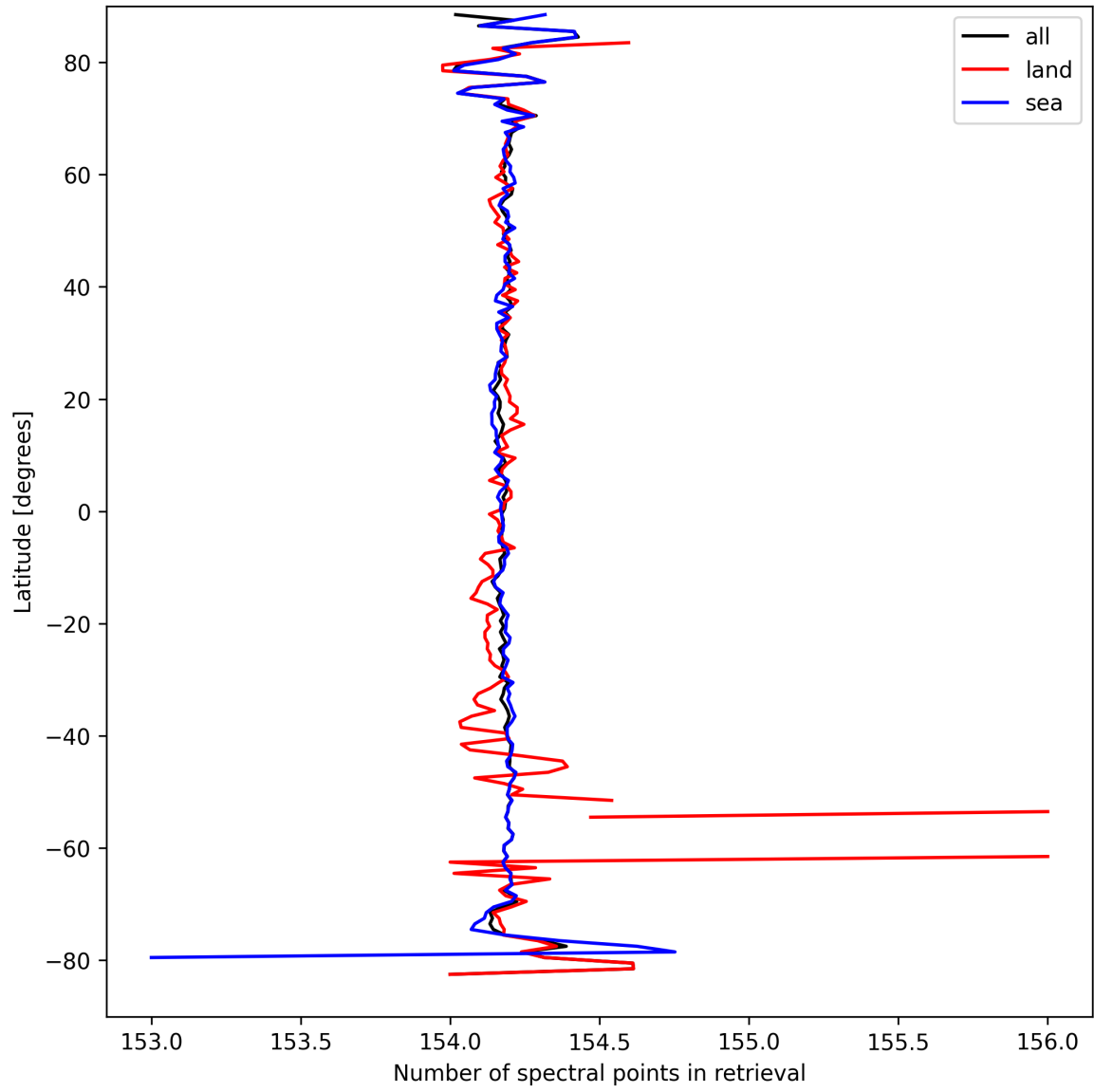
Figure 13: Zonal average of “Number of spectral points in retrieval” for 2025-09-13 to 2025-09-15.
