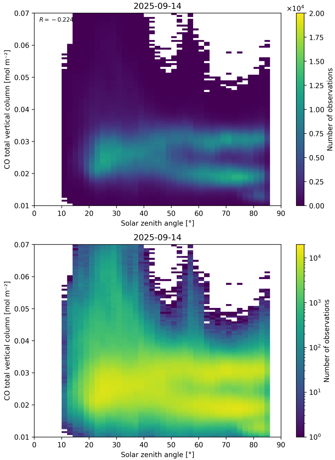
Figure 61: Scatter density plot of “Solar zenith angle” against “CO total vertical column” for 2025-09-13 to 2025-09-15.
