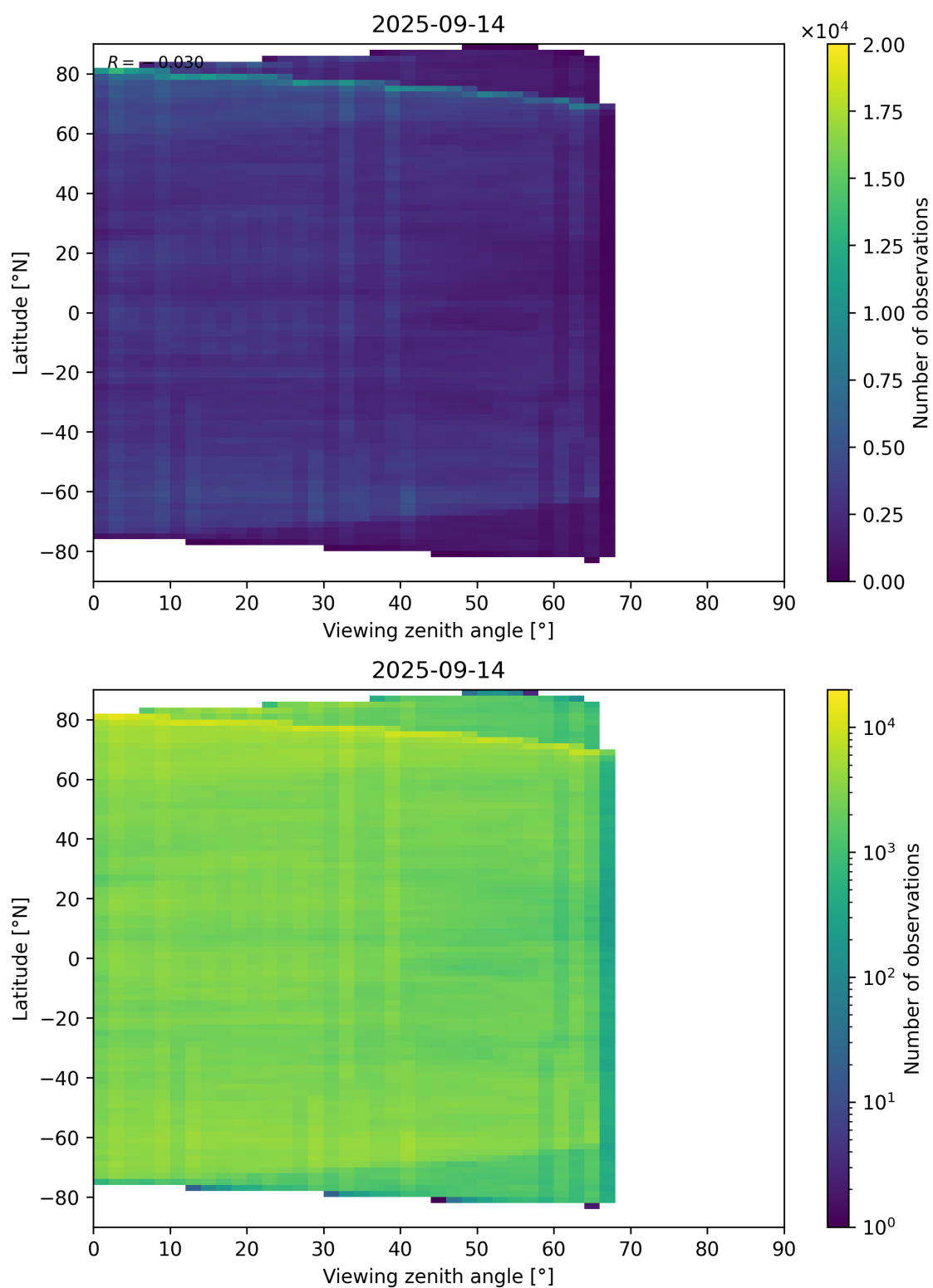
Figure 74: Scatter density plot of “Viewing zenith angle” against “Latitude” for 2025-09-13 to 2025-09-15.
