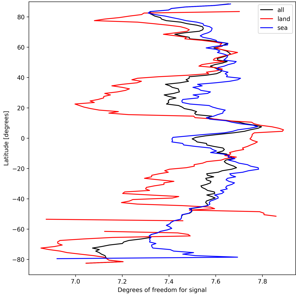
Figure 15: Zonal average of “Degrees of freedom for signal” for 2025-09-13 to 2025-09-15.
