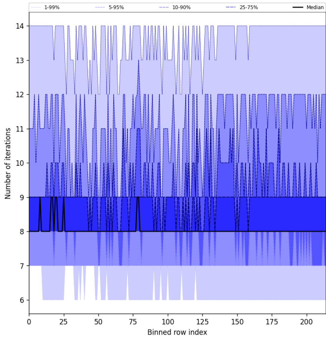
Figure 32: Along track statistics of “Number of iterations” for 2025-09-13 to 2025-09-15
