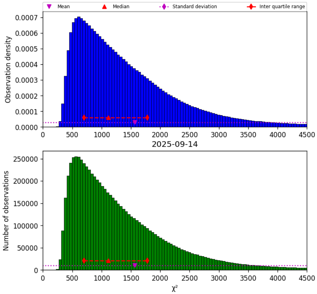
Figure 22: Histogram of “ \chi^2 ” for 2025-09-13 to 2025-09-15
