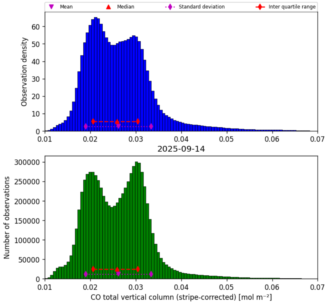
Figure 19: Histogram of “CO total vertical column (stripe-corrected)” for 2025-09-13 to 2025-09-15
