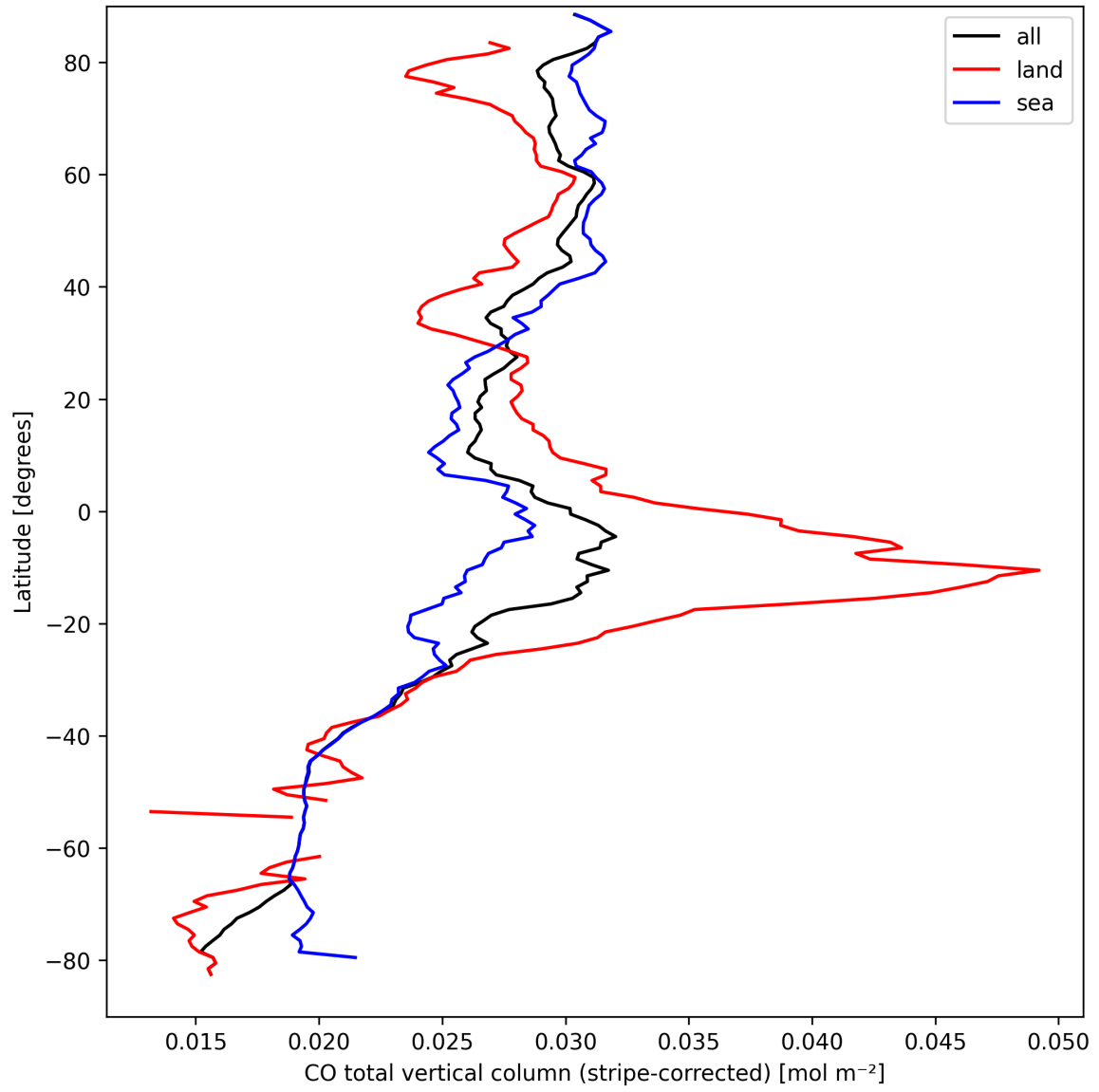
Figure 11: Zonal average of “CO total vertical column (stripe-corrected)” for 2025-09-13 to 2025-09-15.
