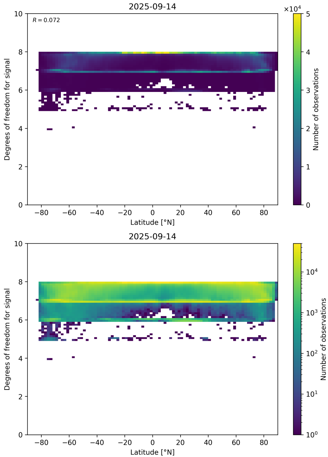
Figure 55: Scatter density plot of “Latitude” against “Degrees of freedom for signal” for 2025-09-13 to 2025-09-15.
