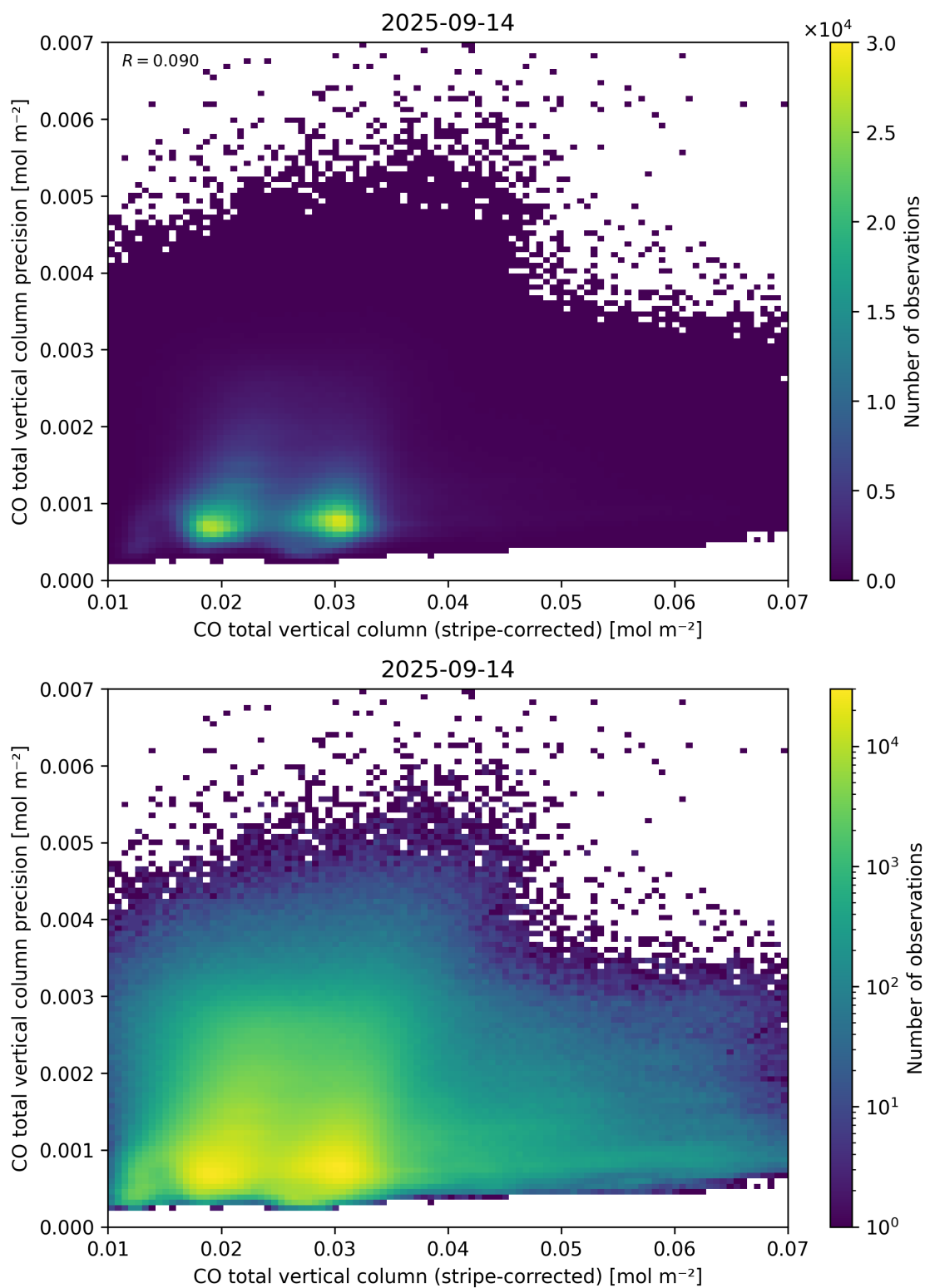
Figure 36: Scatter density plot of “CO total vertical column (stripe-corrected)” against “CO total vertical column precision” for 2025-09-13 to 2025-09-15.
