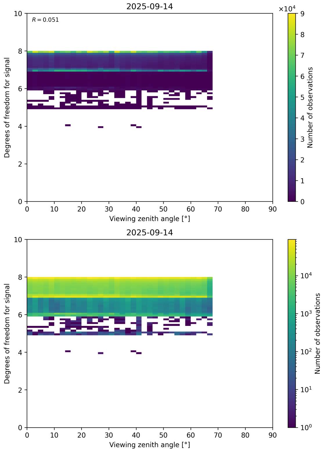
Figure 73: Scatter density plot of “Viewing zenith angle” against “Degrees of freedom for signal” for 2025-09-13 to 2025-09-15.
