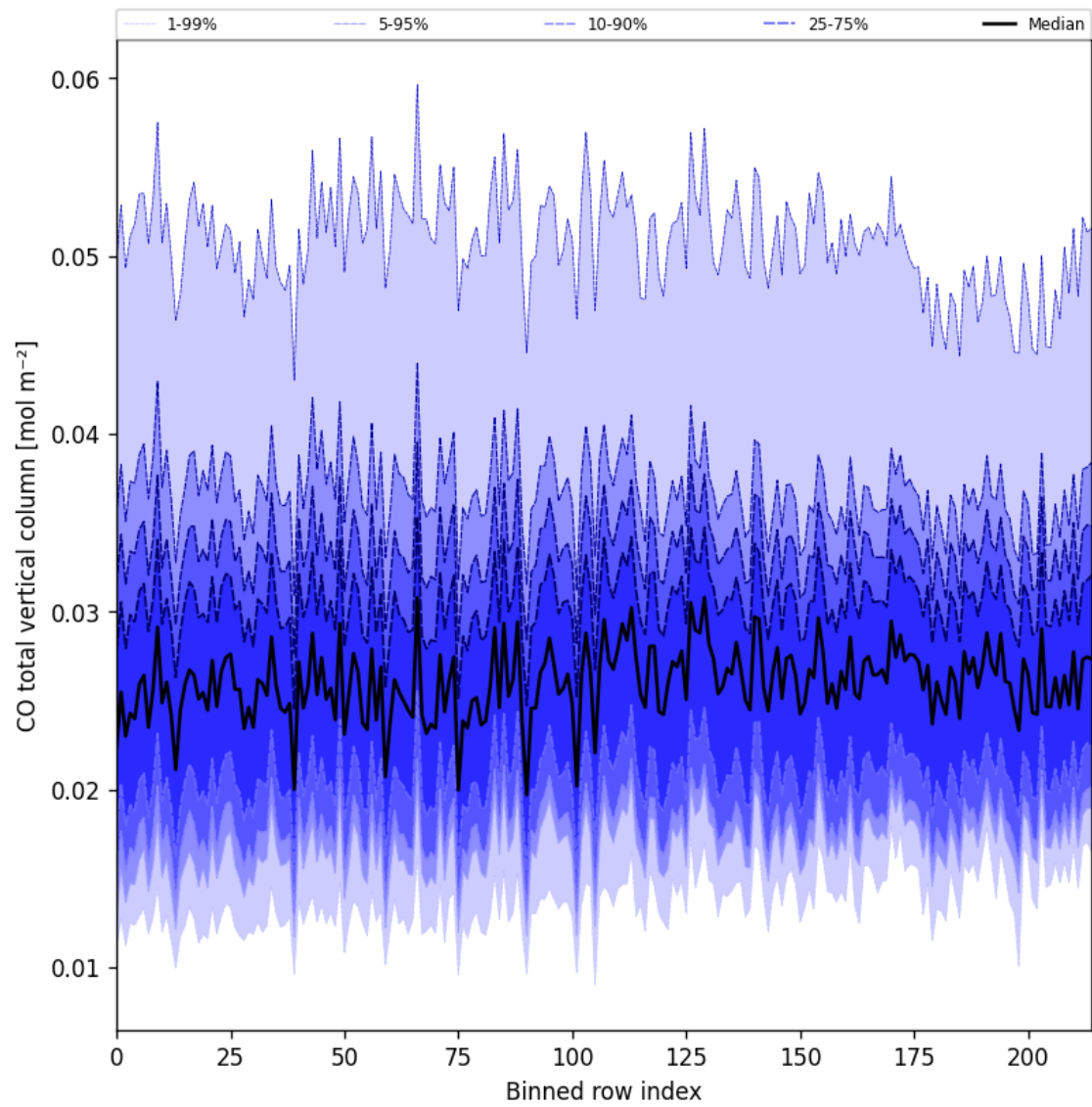
Figure 26: Along track statistics of “CO total vertical column” for 2025-09-13 to 2025-09-15
