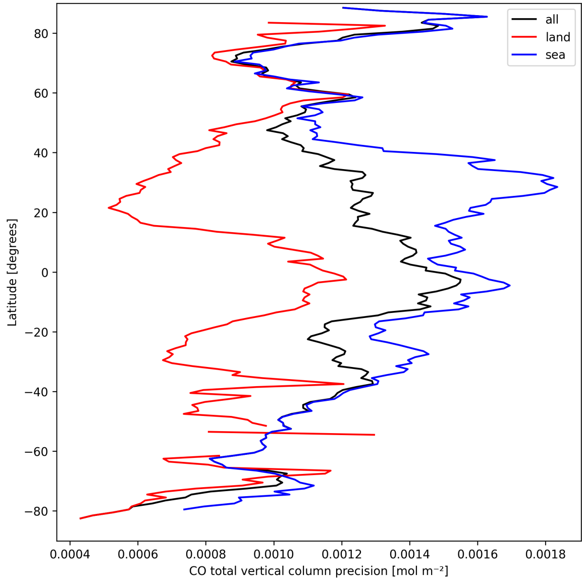
Figure 12: Zonal average of “CO total vertical column precision” for 2025-09-13 to 2025-09-15.
