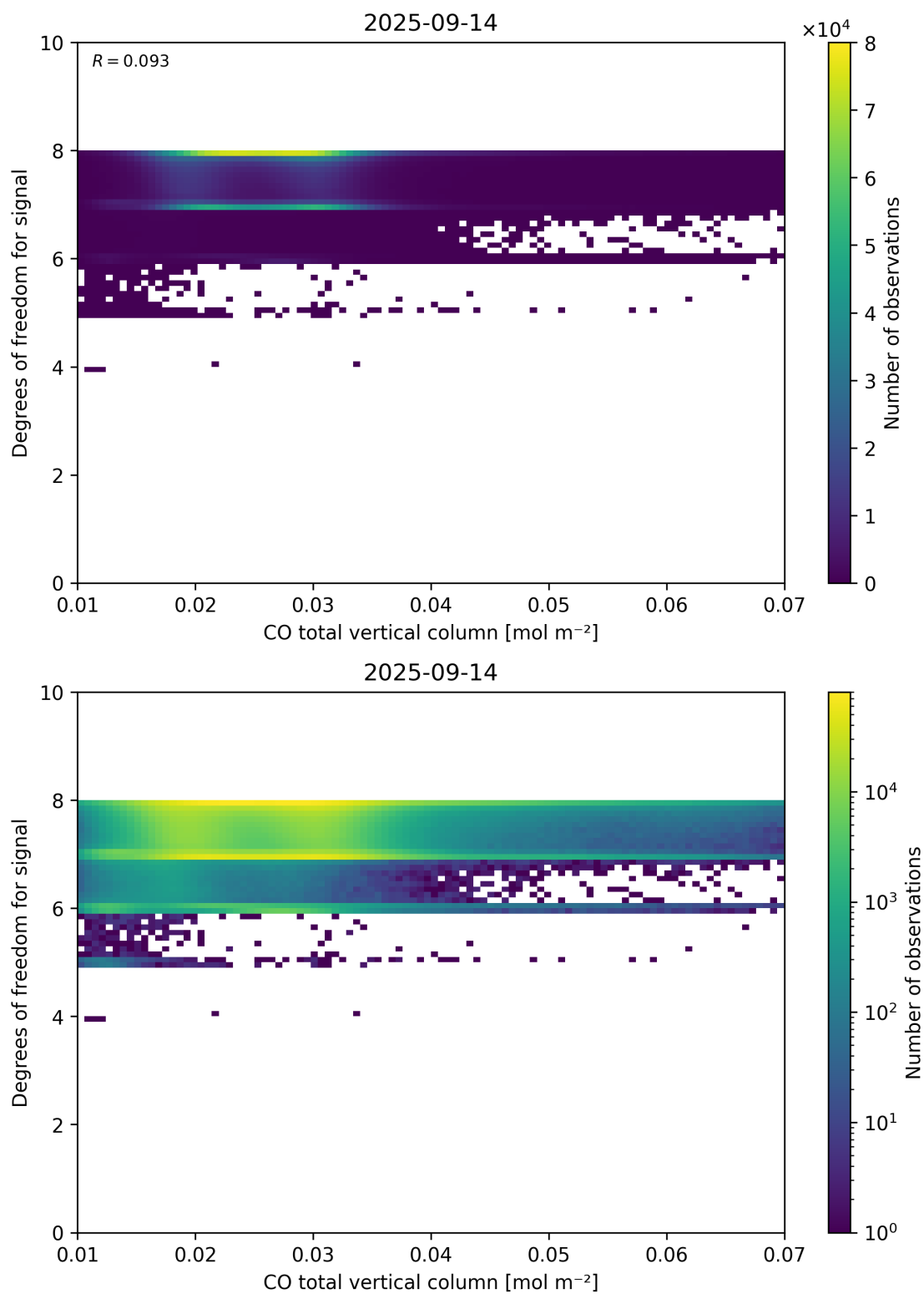
Figure 41: Scatter density plot of “CO total vertical column” against “Degrees of freedom for signal” for 2025-09-13 to 2025-09-15.
