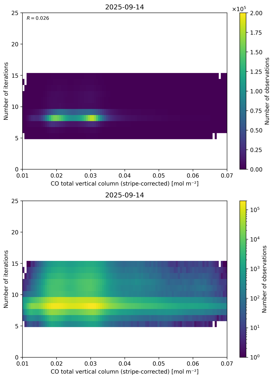
Figure 39: Scatter density plot of “CO total vertical column (stripe-corrected)” against “Number of iterations” for 2025-09-13 to 2025-09-15.
