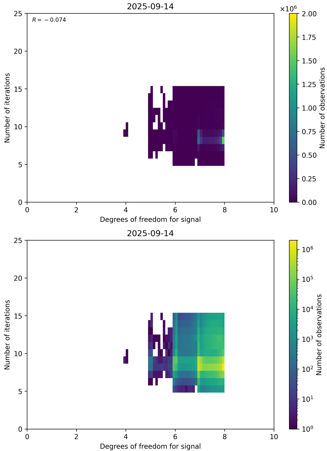
Figure 50: Scatter density plot of “Degrees of freedom for signal” against “Number of iterations” for 2025-09-13 to 2025-09-15.
