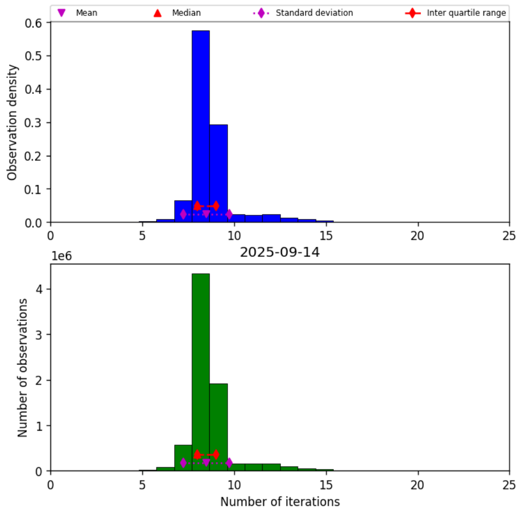
Figure 24: Histogram of “Number of iterations” for 2025-09-13 to 2025-09-15
