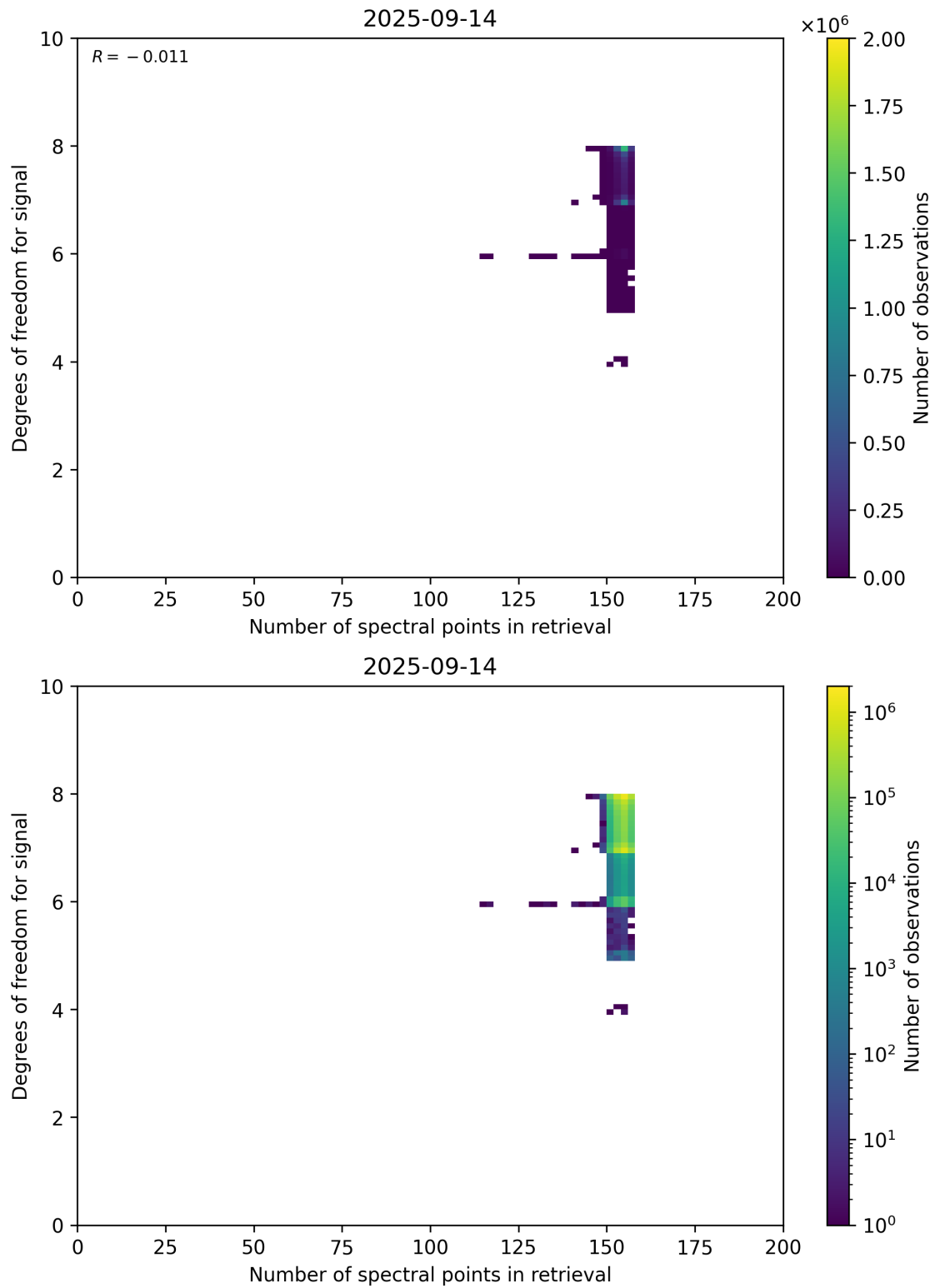
Figure 59: Scatter density plot of “Number of spectral points in retrieval” against “Degrees of freedom for signal” for 2025-09-13 to 2025-09-15.
