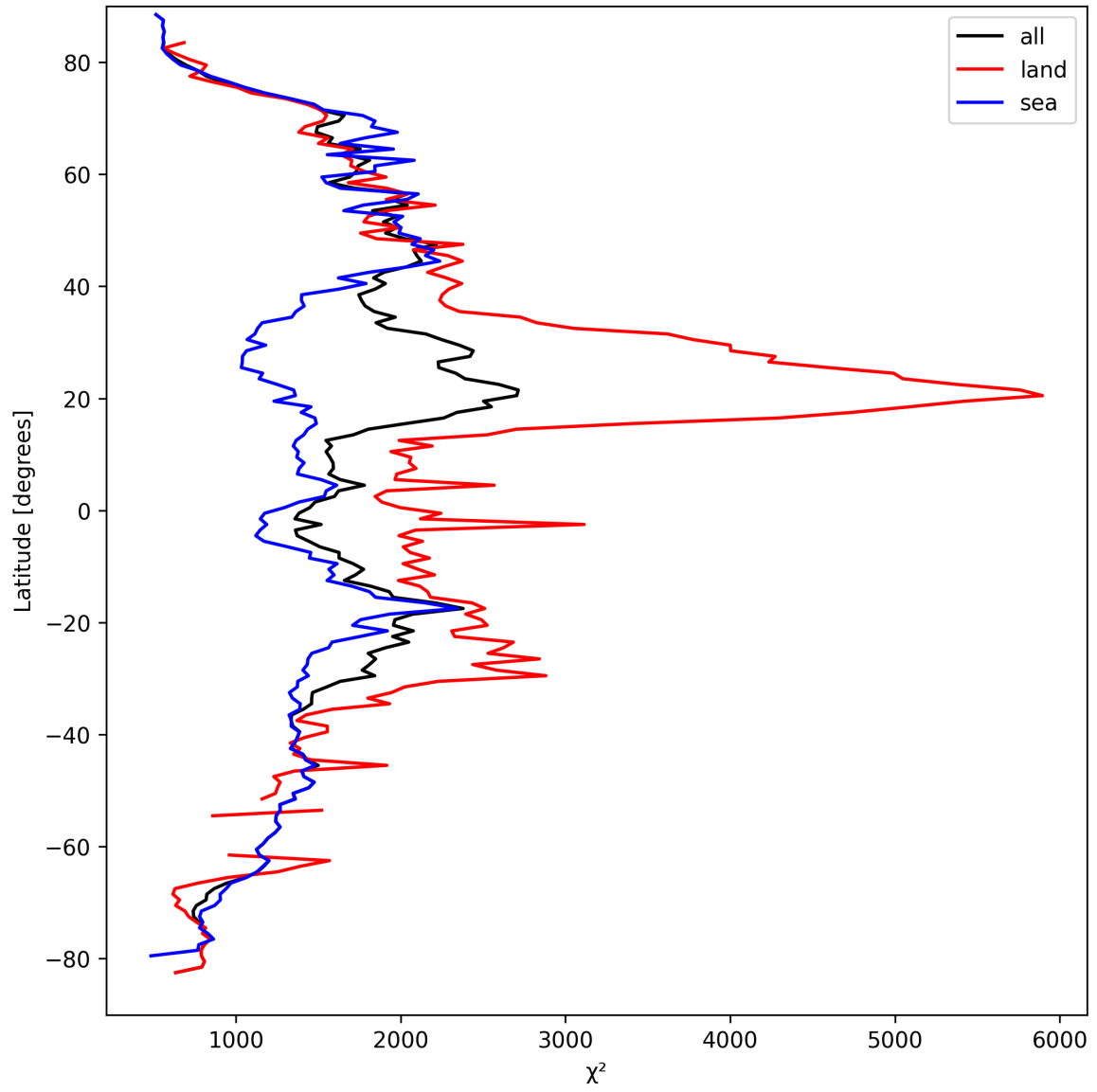
Figure 14: Zonal average of “ \chi^2 ” for 2025-09-13 to 2025-09-15.
