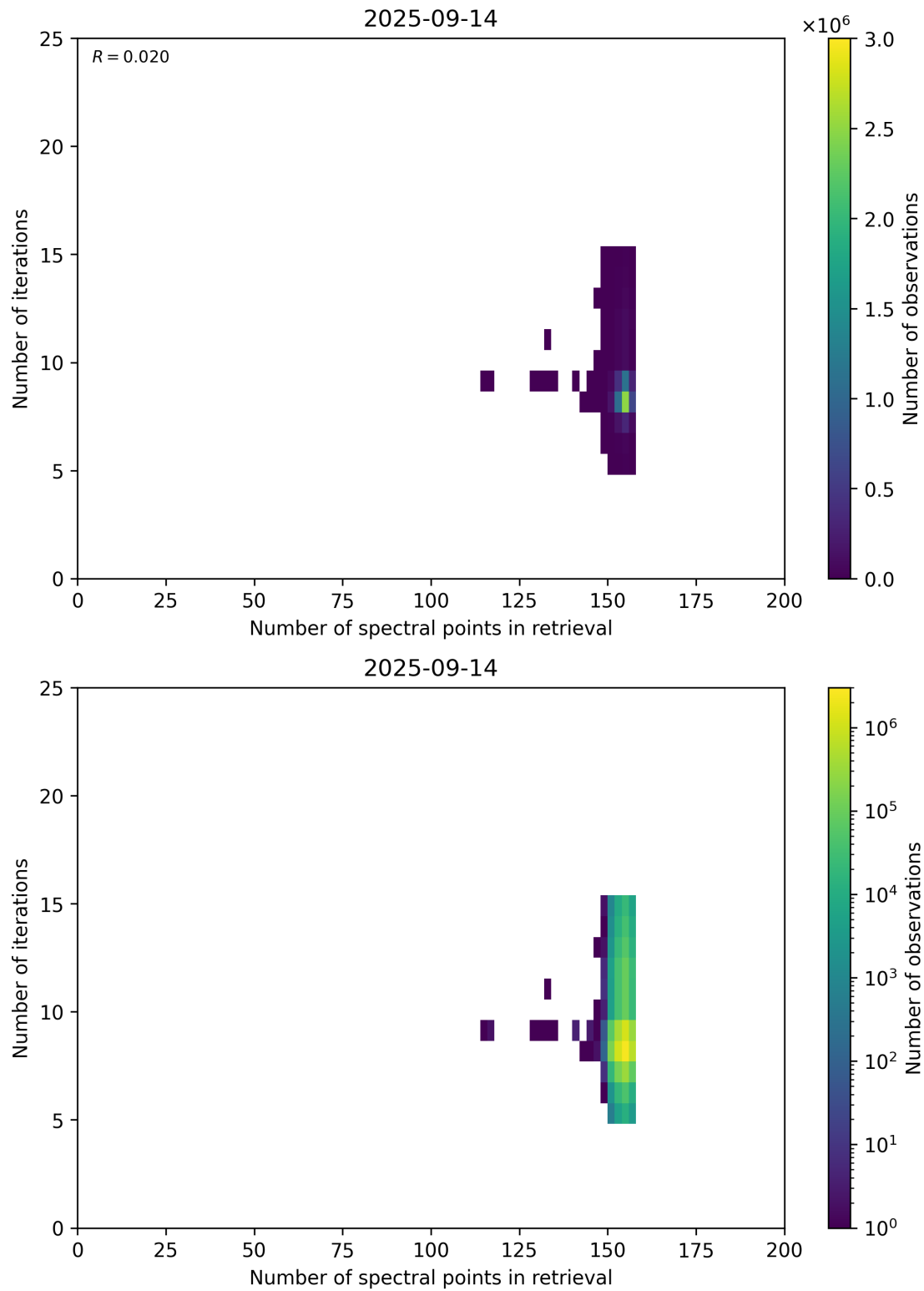
Figure 60: Scatter density plot of “Number of spectral points in retrieval” against “Number of iterations” for 2025-09-13 to 2025-09-15.
