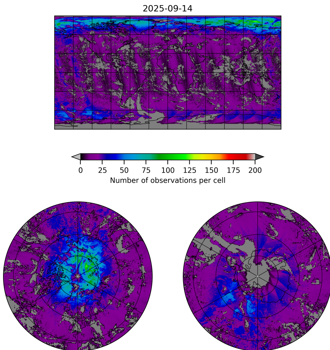
Figure 8: Map of the number of observations for 2025-09-13 to 2025-09-15
