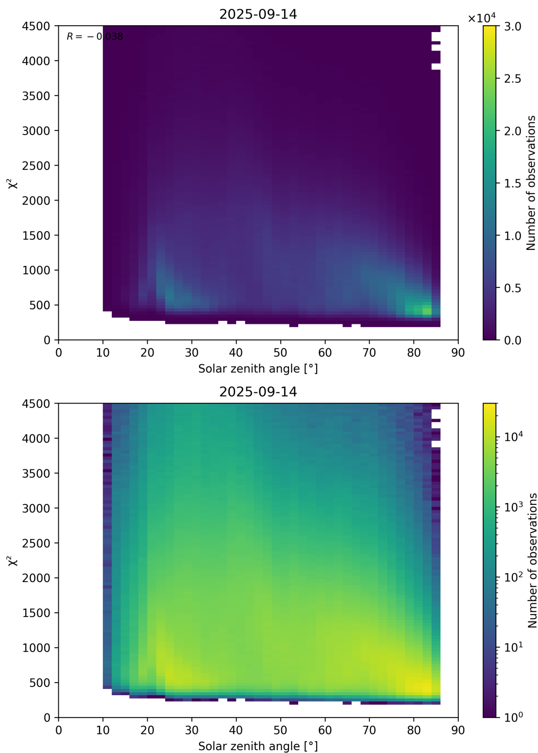
Figure 64: Scatter density plot of “Solar zenith angle” against “ \chi^2 ” for 2025-09-13 to 2025-09-15.
