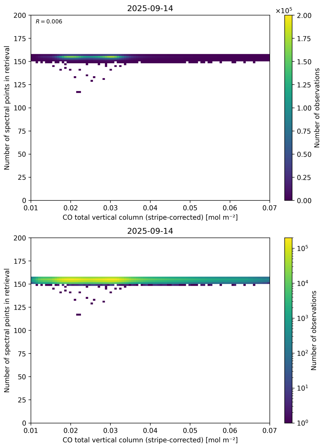
Figure 40: Scatter density plot of “CO total vertical column (stripe-corrected)” against “Number of spectral points in retrieval” for 2025-09-13 to 2025-09-15.
