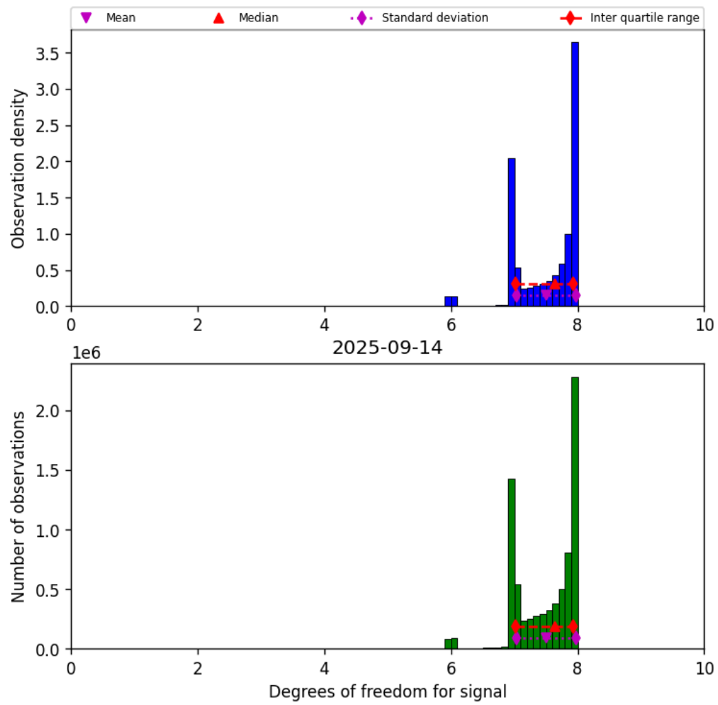
Figure 23: Histogram of “Degrees of freedom for signal” for 2025-09-13 to 2025-09-15
