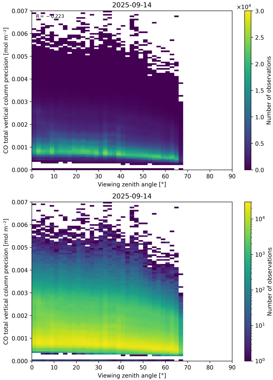
Figure 71: Scatter density plot of “Viewing zenith angle” against “CO total vertical column precision” for 2025-09-13 to 2025-09-15.
