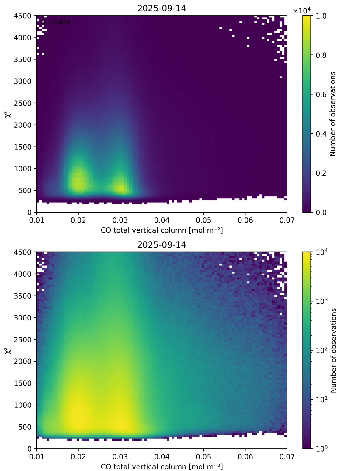
Figure 35: Scatter density plot of “CO total vertical column” against “ \chi^2 ” for 2025-09-13 to 2025-09-15.
