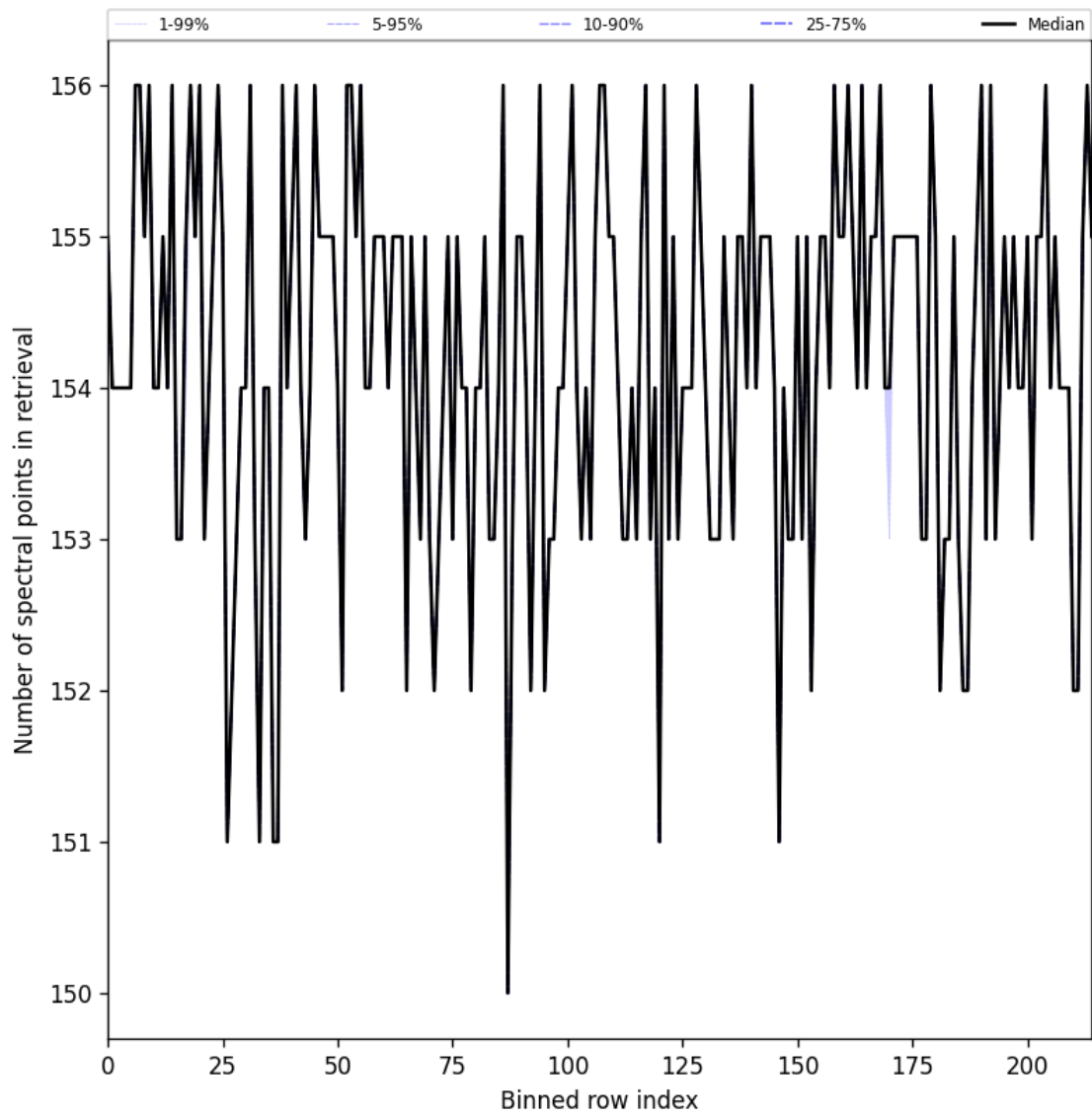
Figure 29: Along track statistics of “Number of spectral points in retrieval” for 2025-09-13 to 2025-09-15
