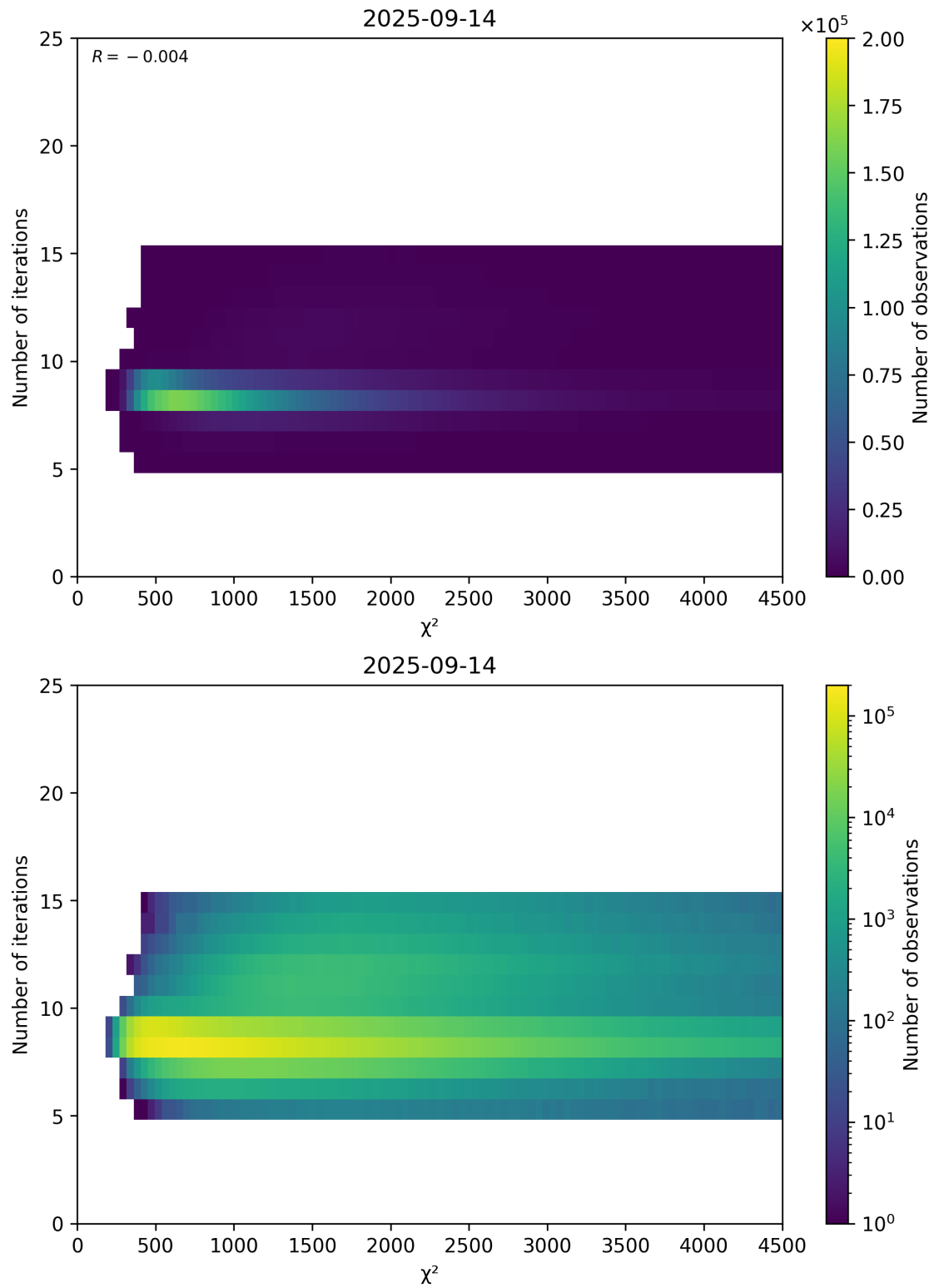
Figure 49: Scatter density plot of “ \chi^2 ” against “Number of iterations” for 2025-09-13 to 2025-09-15.
