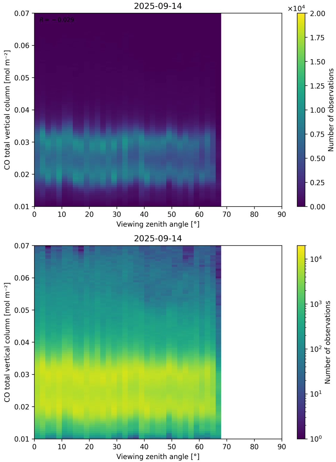
Figure 69: Scatter density plot of “Viewing zenith angle” against “CO total vertical column” for 2025-09-13 to 2025-09-15.
