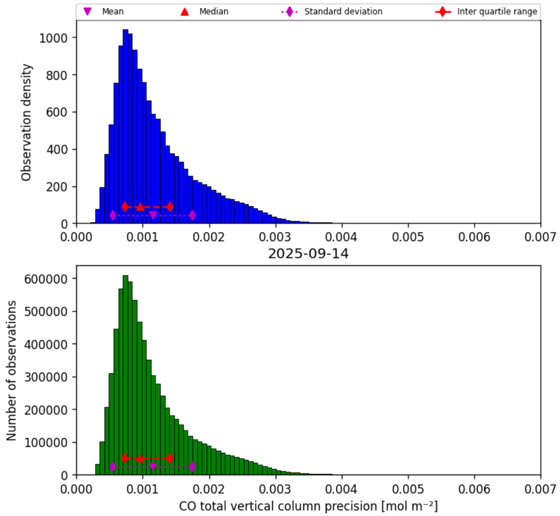
Figure 20: Histogram of “CO total vertical column precision” for 2025-09-13 to 2025-09-15
