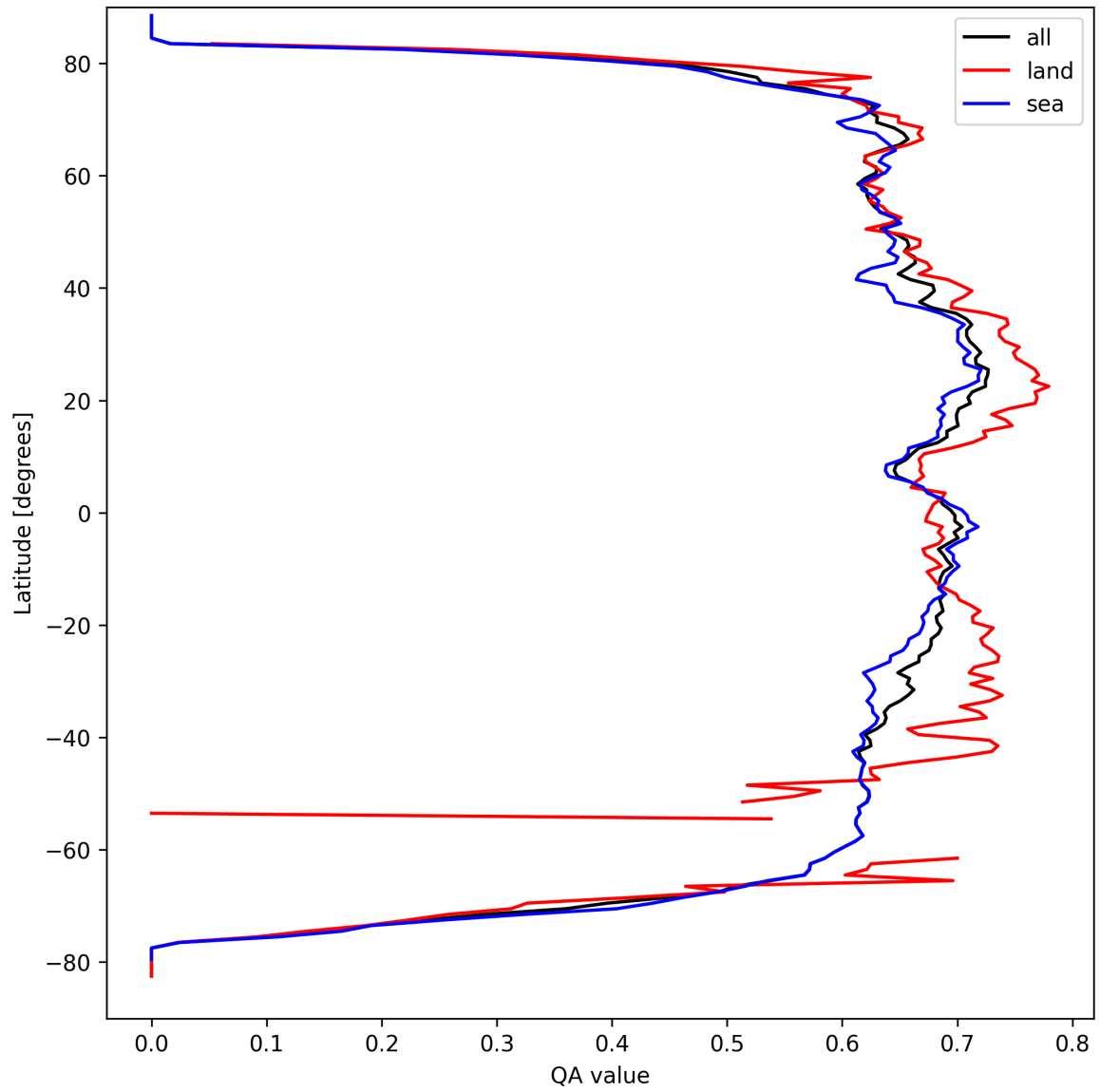
Figure 9: Zonal average of “QA value” for 2025-09-13 to 2025-09-15.
