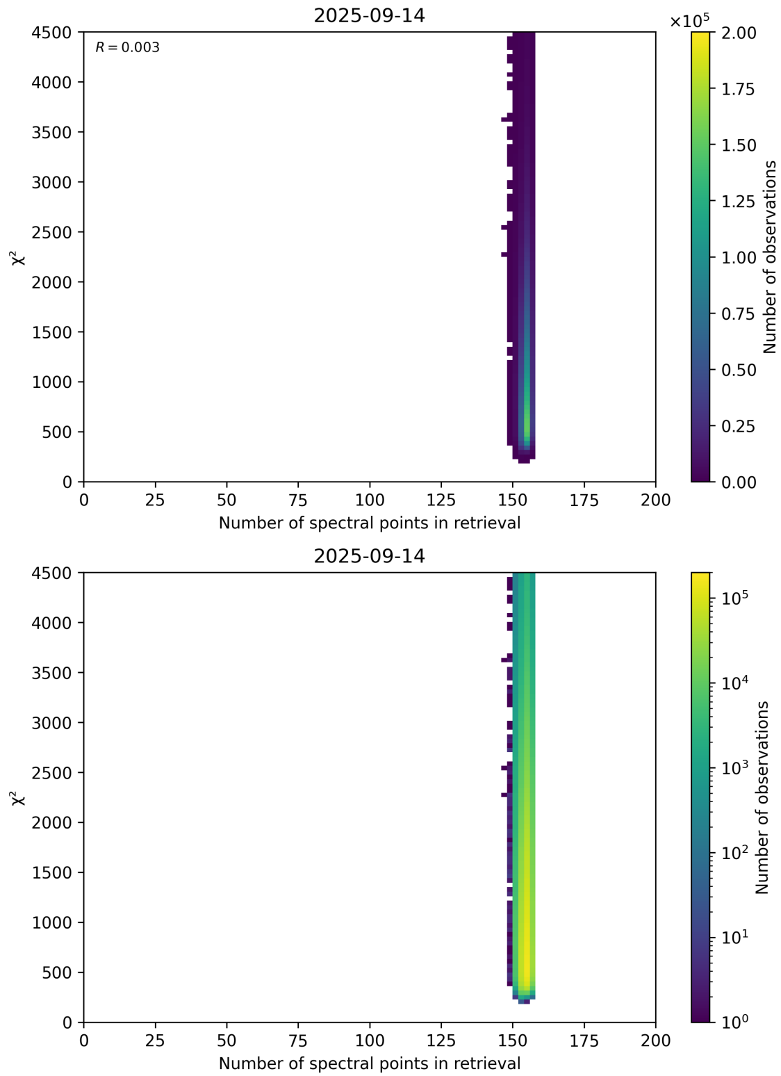
Figure 58: Scatter density plot of “Number of spectral points in retrieval” against “ \chi^2 ” for 2025-09-13 to 2025-09-15.
