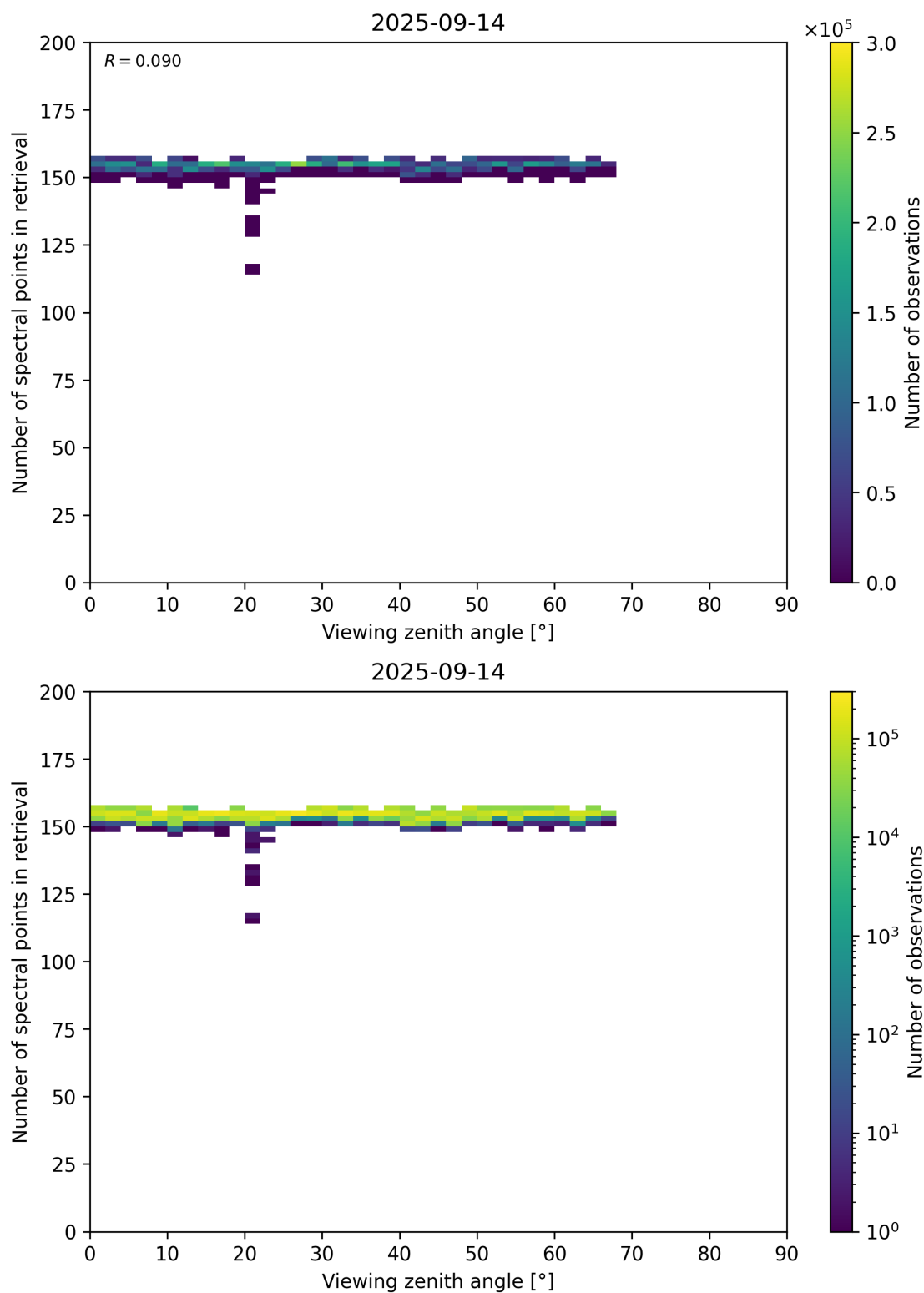
Figure 76: Scatter density plot of “Viewing zenith angle” against “Number of spectral points in retrieval” for 2025-09-13 to 2025-09-15.
