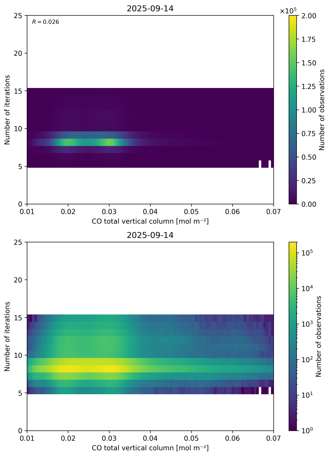
Figure 42: Scatter density plot of “CO total vertical column” against “Number of iterations” for 2025-09-13 to 2025-09-15.
