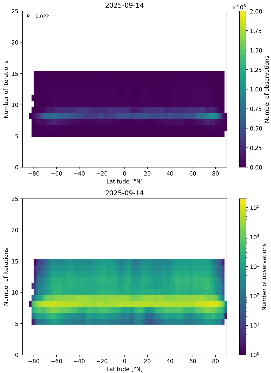
Figure 56: Scatter density plot of “Latitude” against “Number of iterations” for 2025-09-13 to 2025-09-15.
