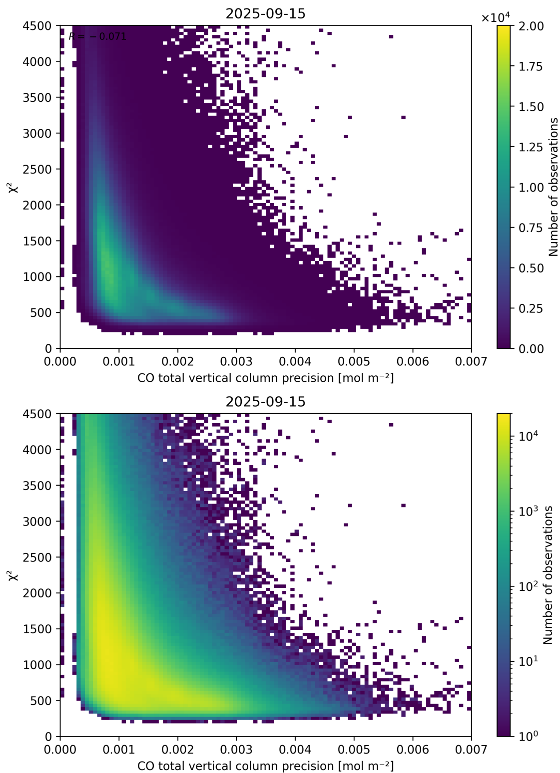
Figure 44: Scatter density plot of “CO total vertical column precision” against “ \chi^2 ” for 2025-09-15 to 2025-09-16.
