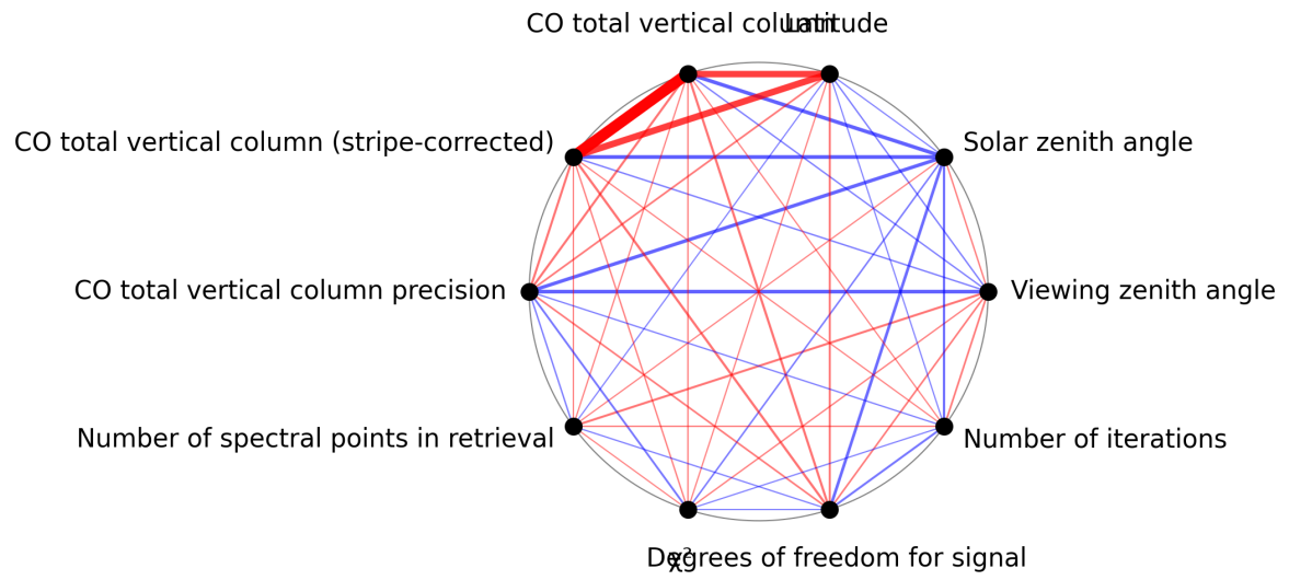
Figure 1: Map of correlation graph for 2025-09-15 to 2025-09-16.
