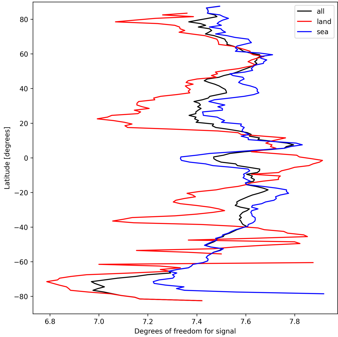
Figure 15: Zonal average of “Degrees of freedom for signal” for 2025-09-15 to 2025-09-16.
