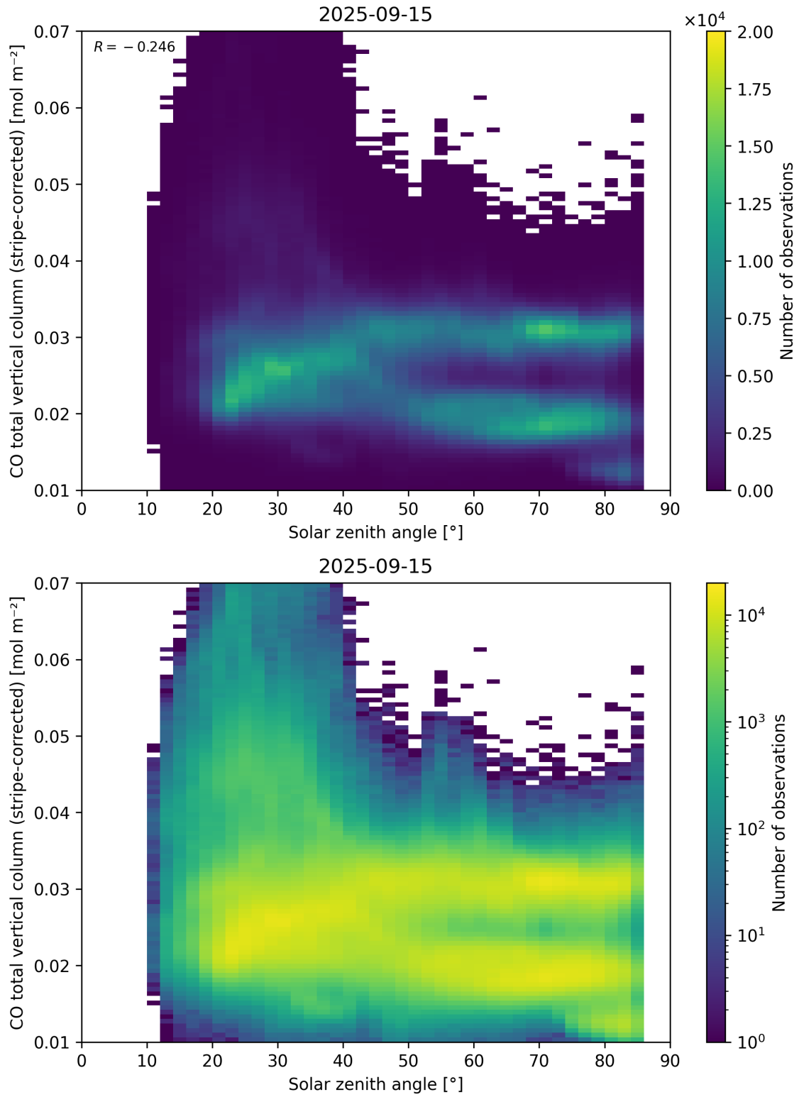
Figure 62: Scatter density plot of “Solar zenith angle” against “CO total vertical column (stripe-corrected)” for 2025-09-15 to 2025-09-16.
