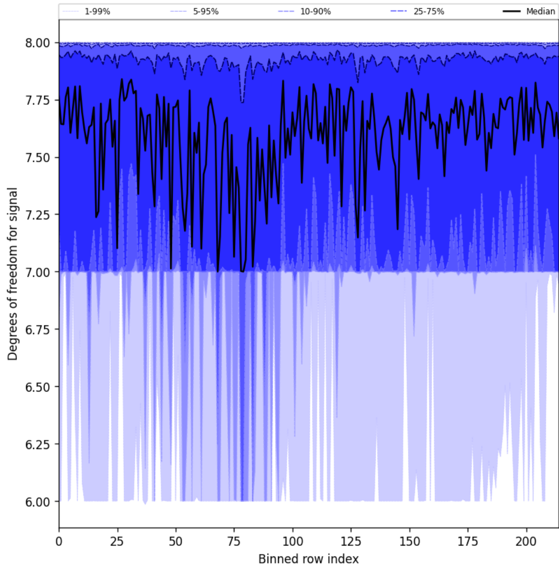
Figure 31: Along track statistics of “Degrees of freedom for signal” for 2025-09-15 to 2025-09-16
