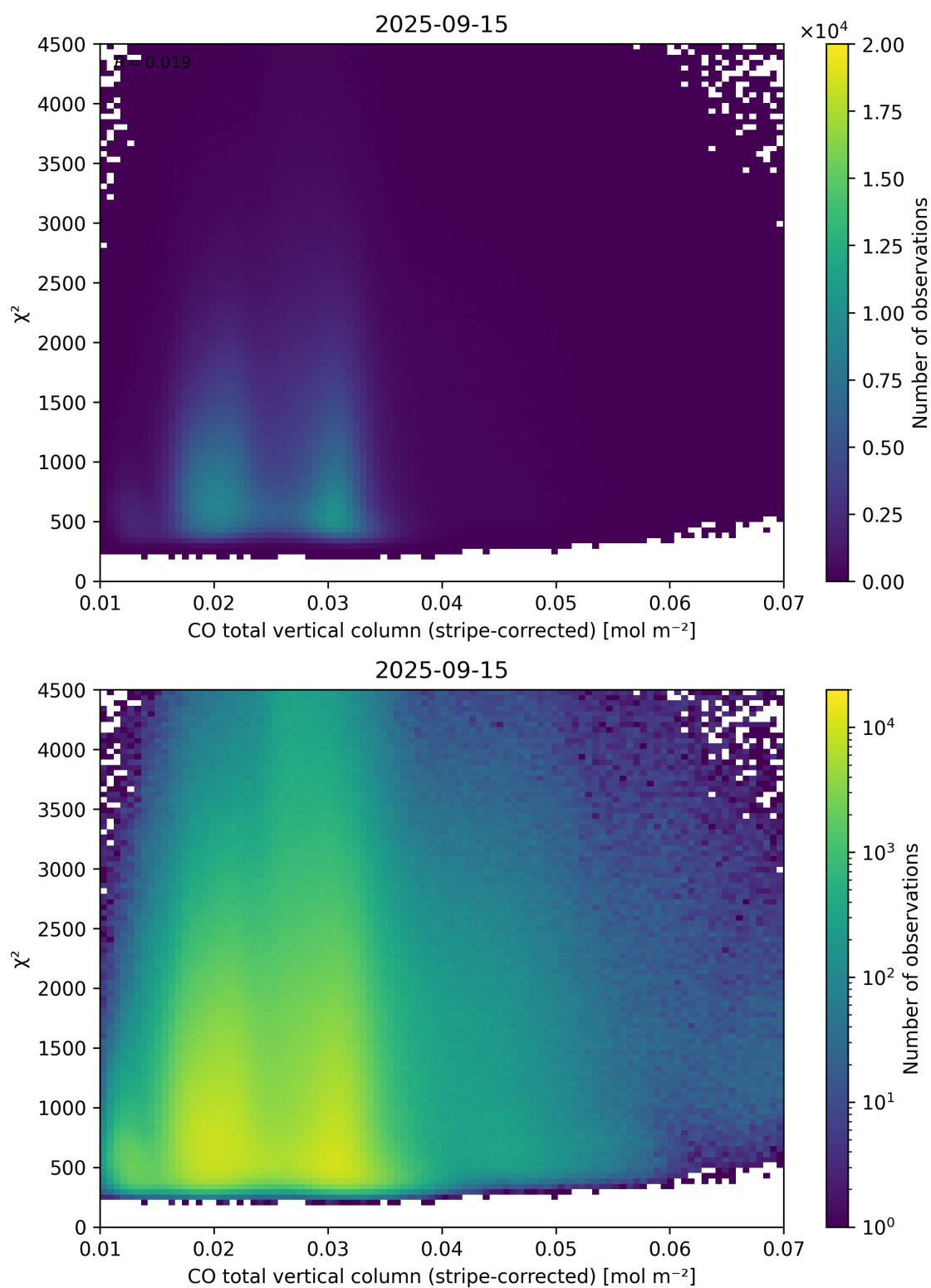
Figure 37: Scatter density plot of “CO total vertical column (stripe-corrected)” against “ \chi^2 ” for 2025-09-15 to 2025-09-16.
