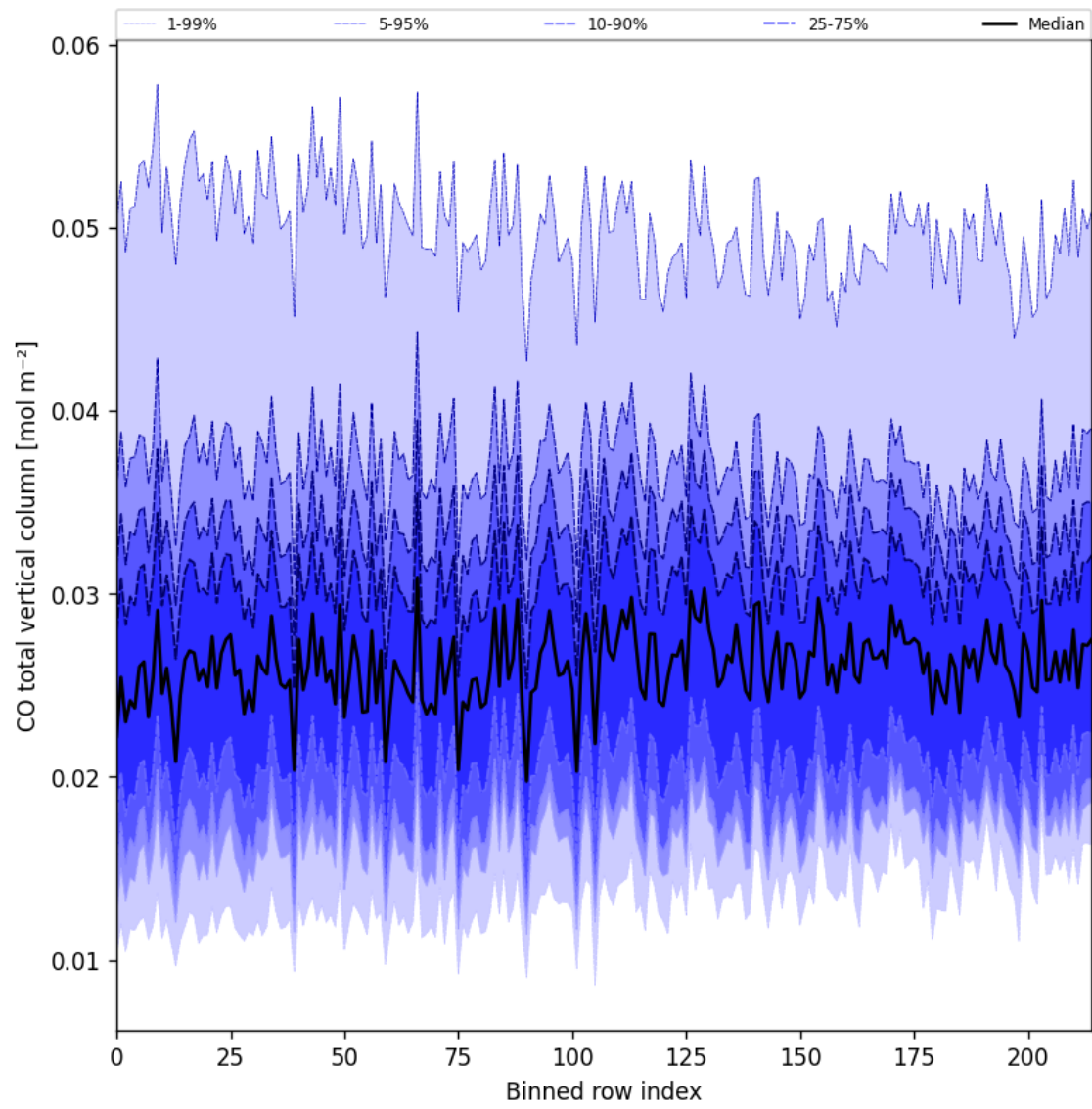
Figure 26: Along track statistics of “CO total vertical column” for 2025-09-15 to 2025-09-16
