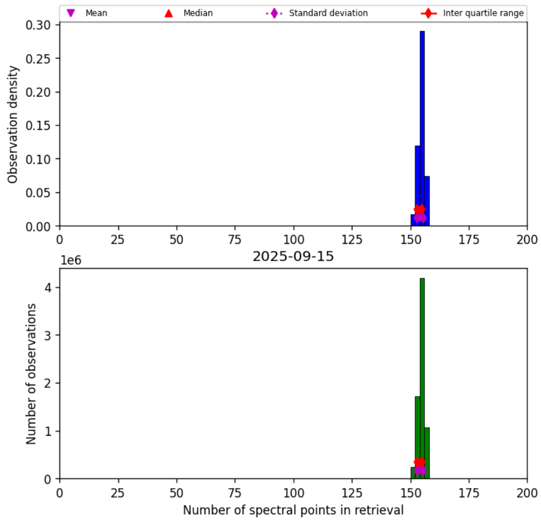
Figure 21: Histogram of “Number of spectral points in retrieval” for 2025-09-15 to 2025-09-16
