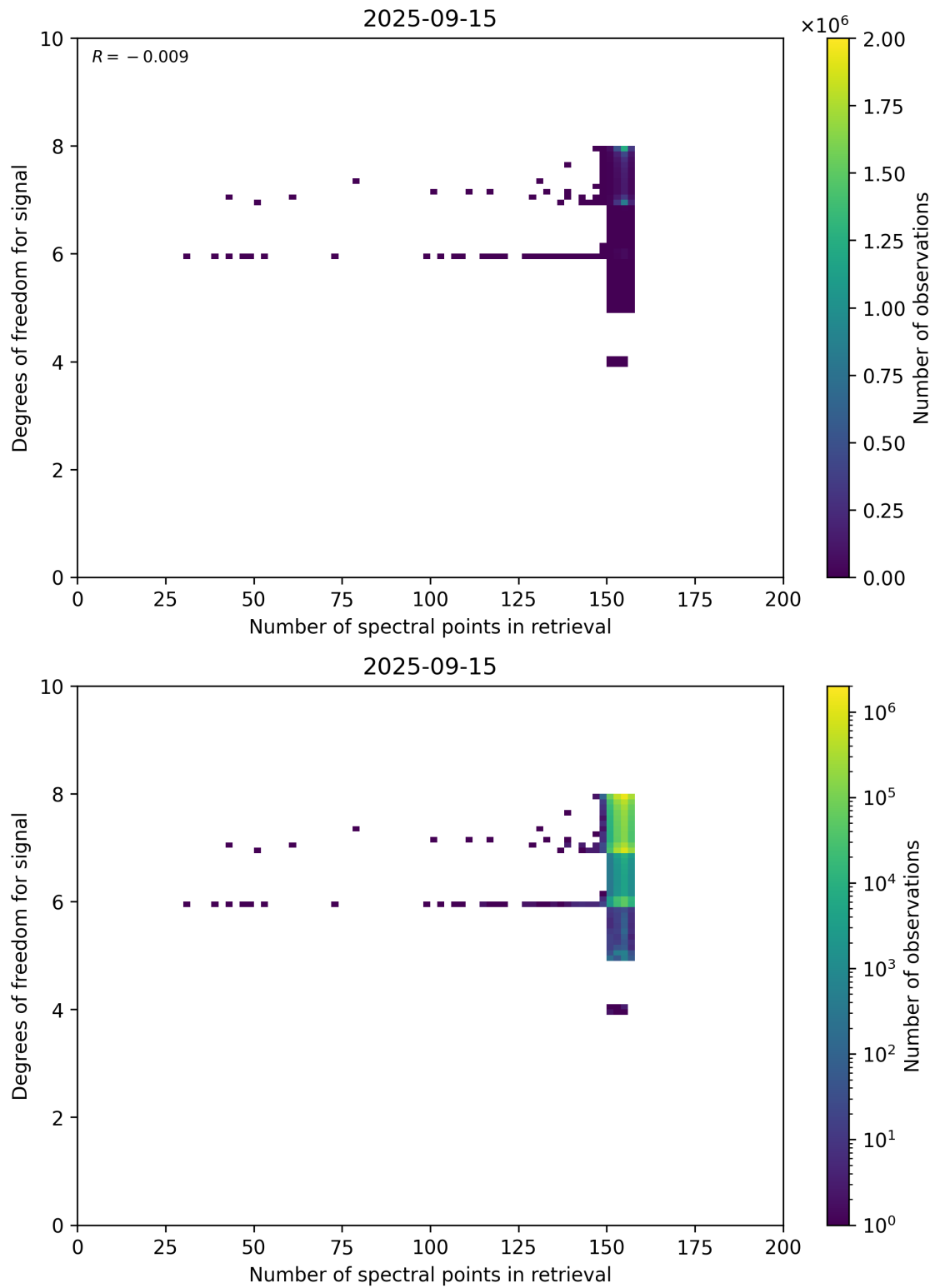
Figure 59: Scatter density plot of “Number of spectral points in retrieval” against “Degrees of freedom for signal” for 2025-09-15 to 2025-09-16.
