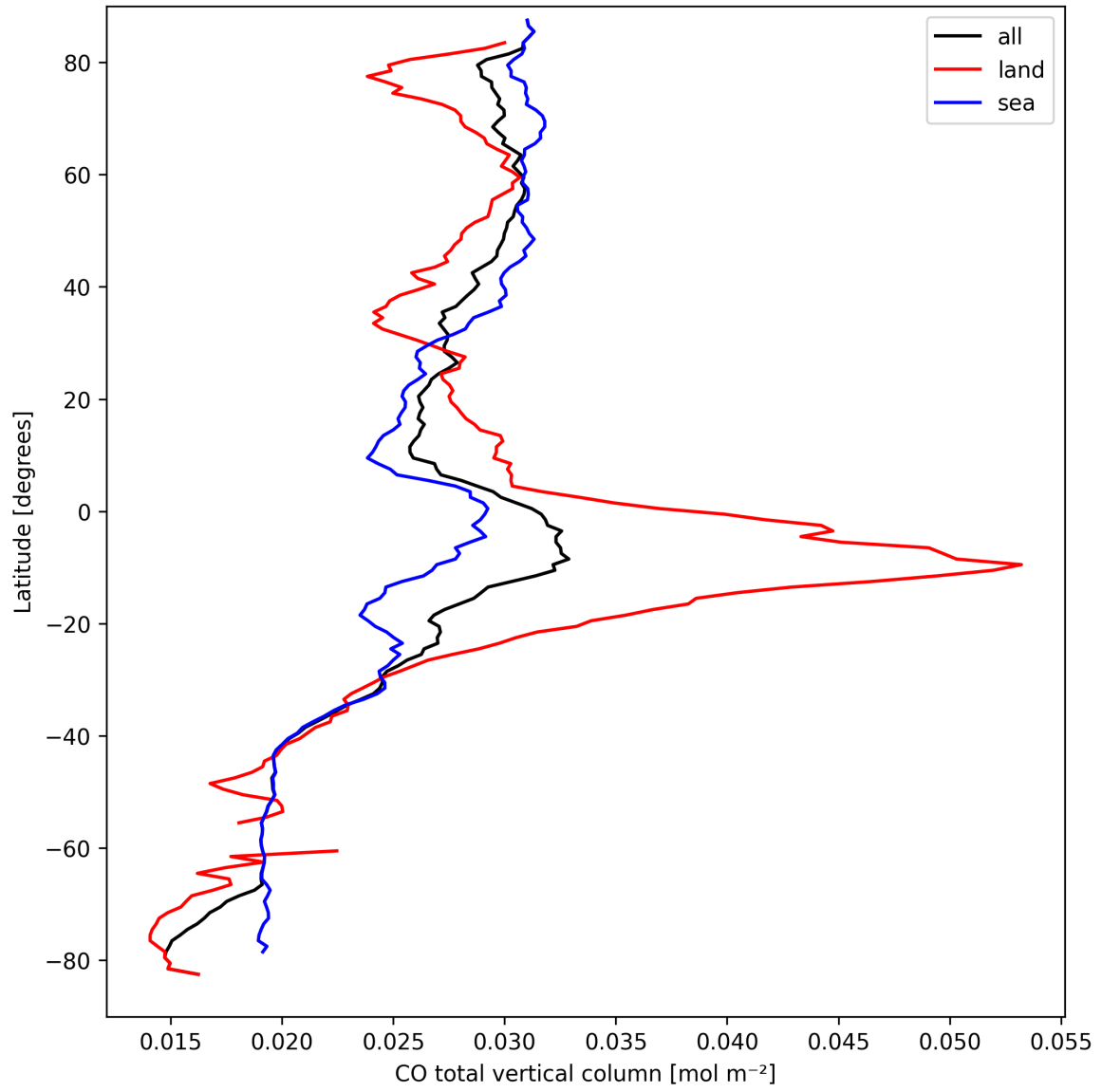
Figure 10: Zonal average of “CO total vertical column” for 2025-09-15 to 2025-09-16.
