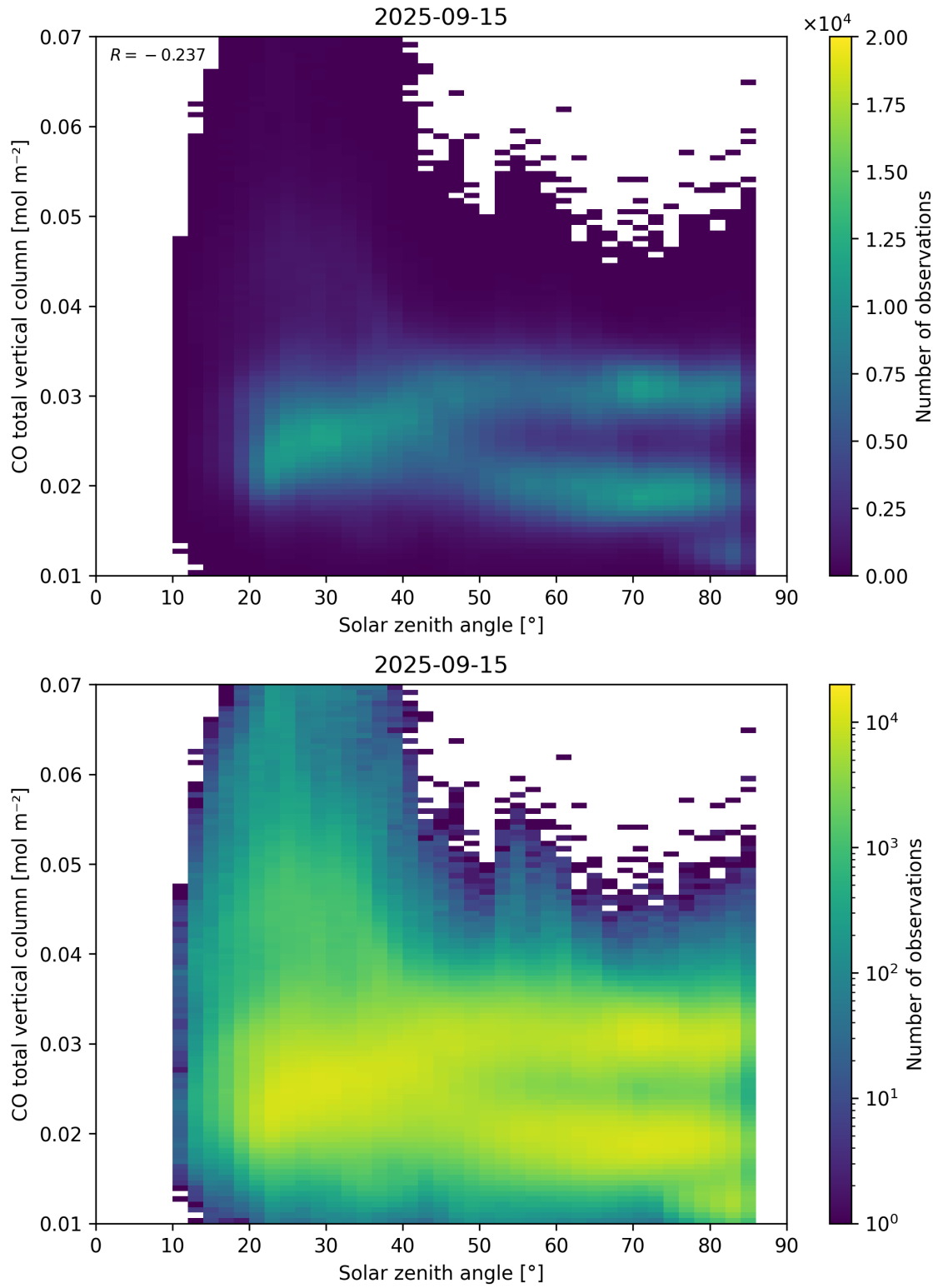
Figure 61: Scatter density plot of “Solar zenith angle” against “CO total vertical column” for 2025-09-15 to 2025-09-16.
