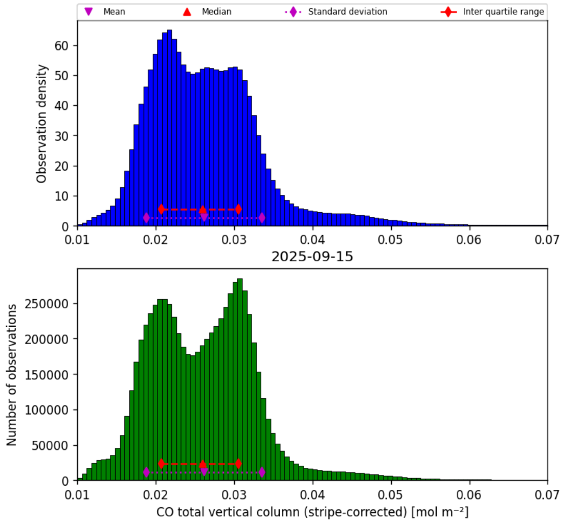
Figure 19: Histogram of “CO total vertical column (stripe-corrected)” for 2025-09-15 to 2025-09-16
