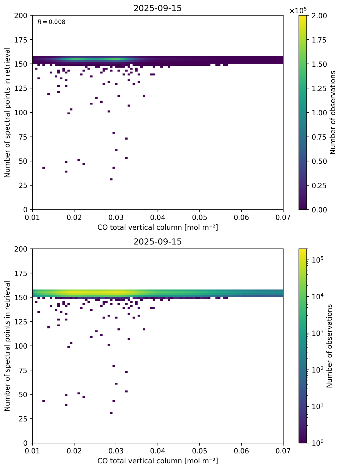
Figure 43: Scatter density plot of “CO total vertical column” against “Number of spectral points in retrieval” for 2025-09-15 to 2025-09-16.
