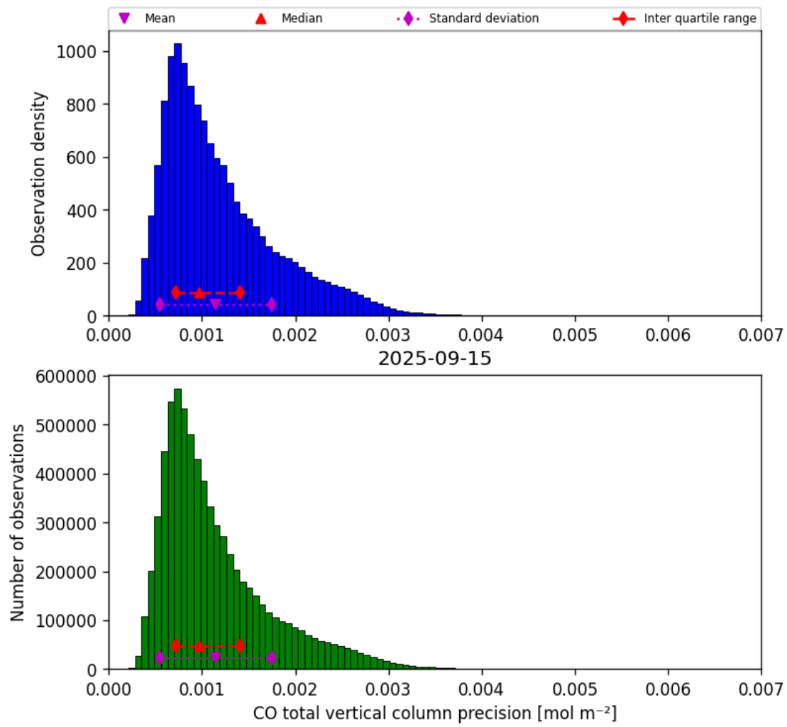
Figure 20: Histogram of “CO total vertical column precision” for 2025-09-15 to 2025-09-16
