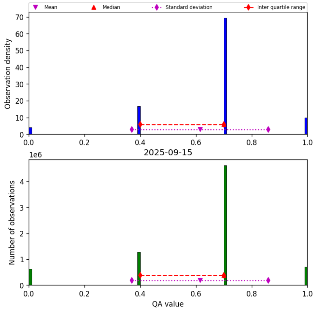
Figure 17: Histogram of “QA value” for 2025-09-15 to 2025-09-16
