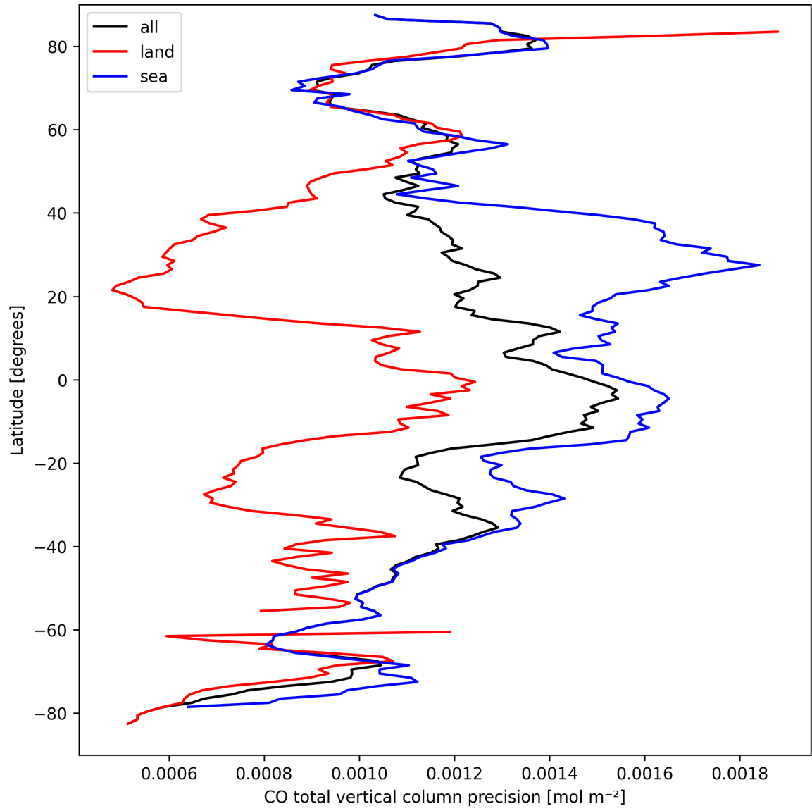
Figure 12: Zonal average of “CO total vertical column precision” for 2025-09-15 to 2025-09-16.
