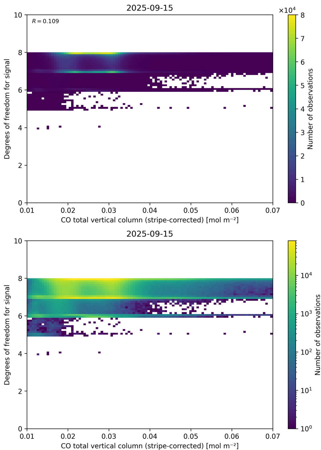
Figure 38: Scatter density plot of “CO total vertical column (stripe-corrected)” against “Degrees of freedom for signal” for 2025-09-15 to 2025-09-16.
