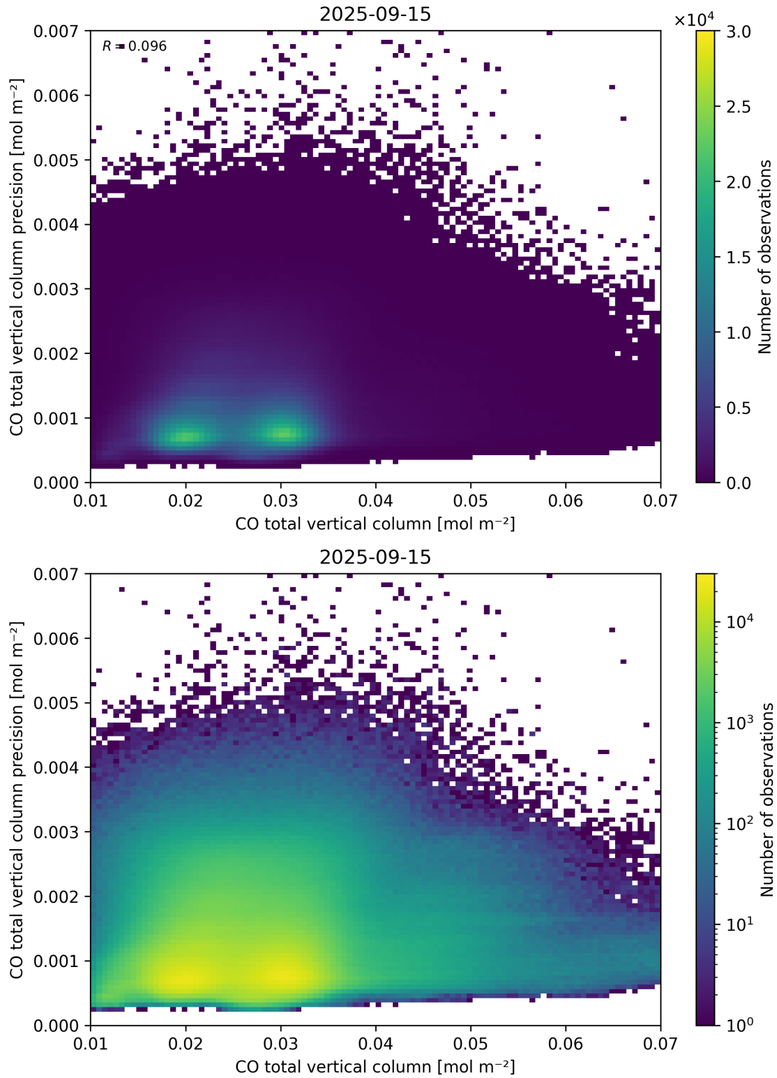
Figure 34: Scatter density plot of “CO total vertical column” against “CO total vertical column precision” for 2025-09-15 to 2025-09-16.
