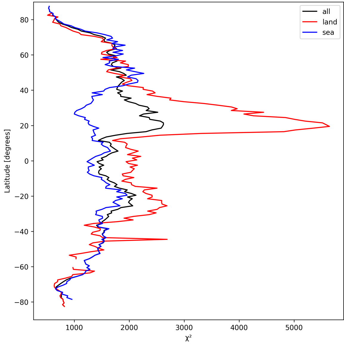
Figure 14: Zonal average of “ \chi^2 ” for 2025-09-15 to 2025-09-16.
