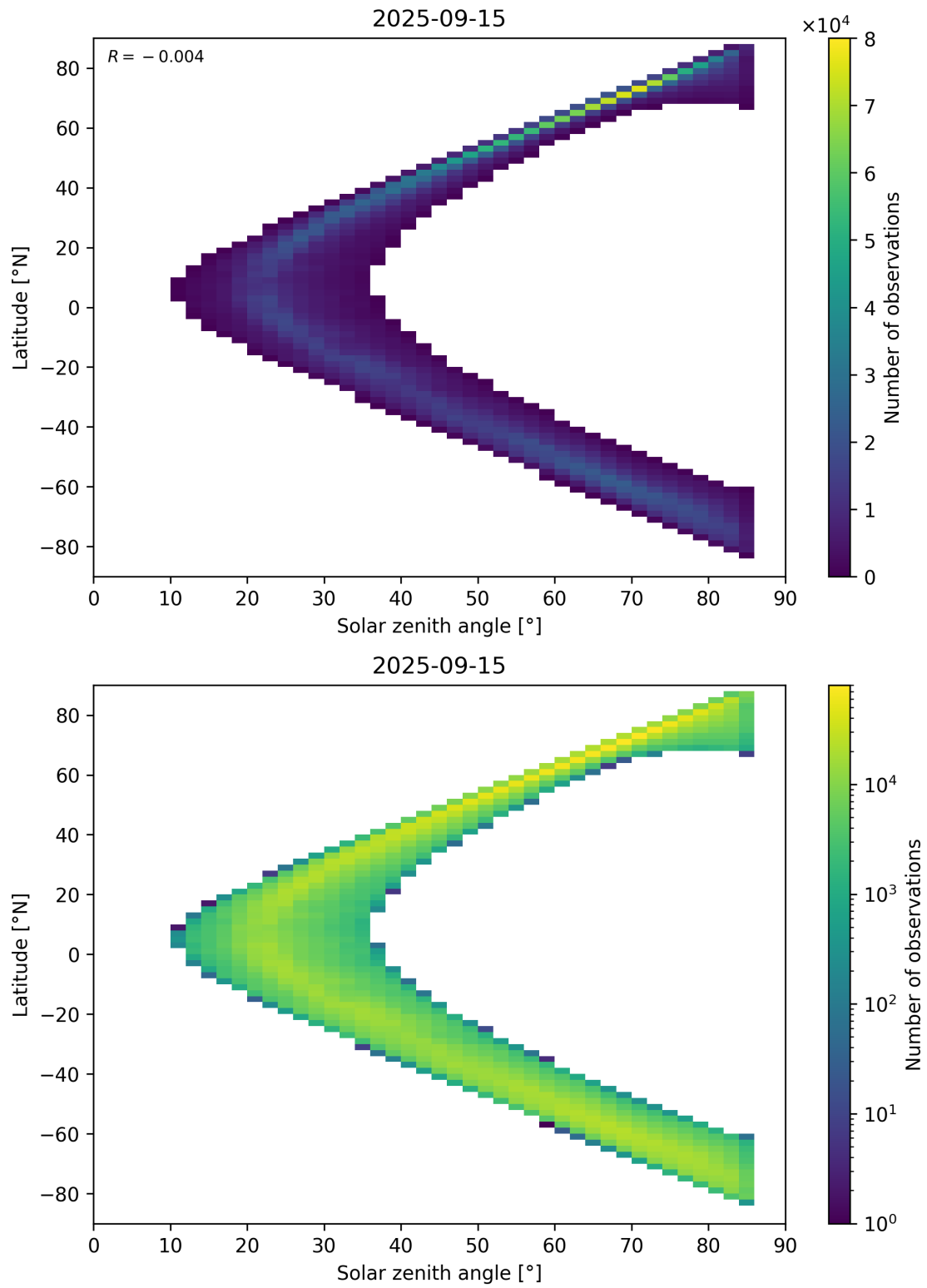
Figure 66: Scatter density plot of “Solar zenith angle” against “Latitude” for 2025-09-15 to 2025-09-16.
