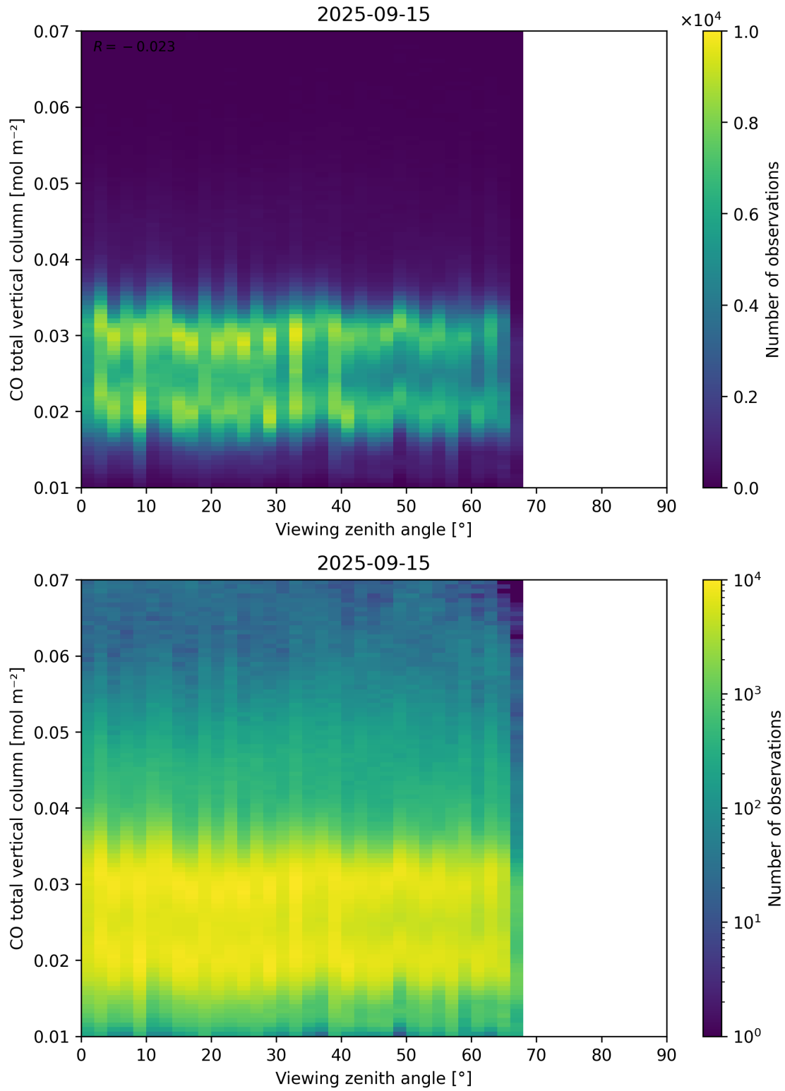
Figure 69: Scatter density plot of “Viewing zenith angle” against “CO total vertical column” for 2025-09-15 to 2025-09-16.
