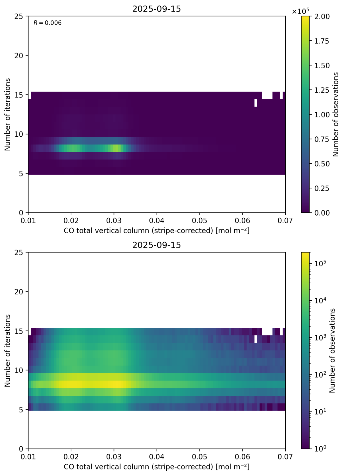
Figure 39: Scatter density plot of “CO total vertical column (stripe-corrected)” against “Number of iterations” for 2025-09-15 to 2025-09-16.
