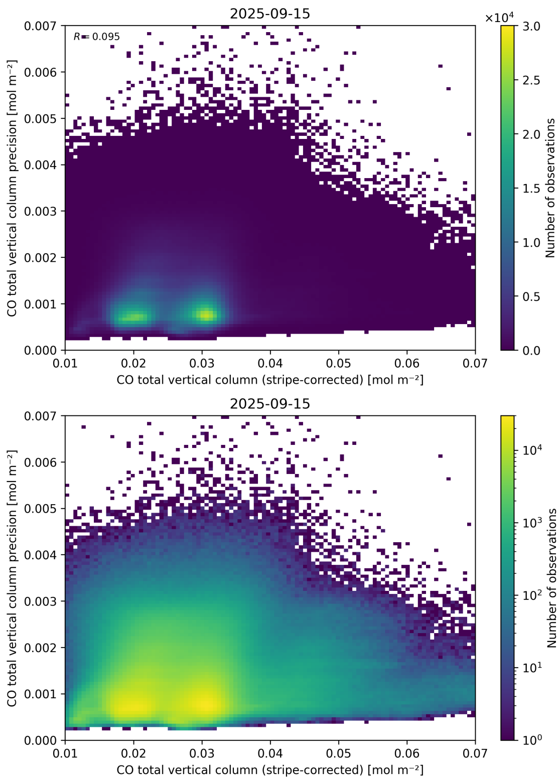
Figure 36: Scatter density plot of “CO total vertical column (stripe-corrected)” against “CO total vertical column precision” for 2025-09-15 to 2025-09-16.
