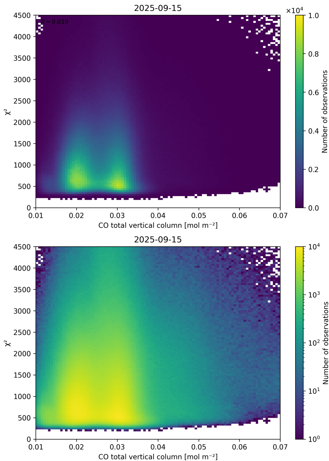
Figure 35: Scatter density plot of “CO total vertical column” against “ \chi^2 ” for 2025-09-15 to 2025-09-16.
