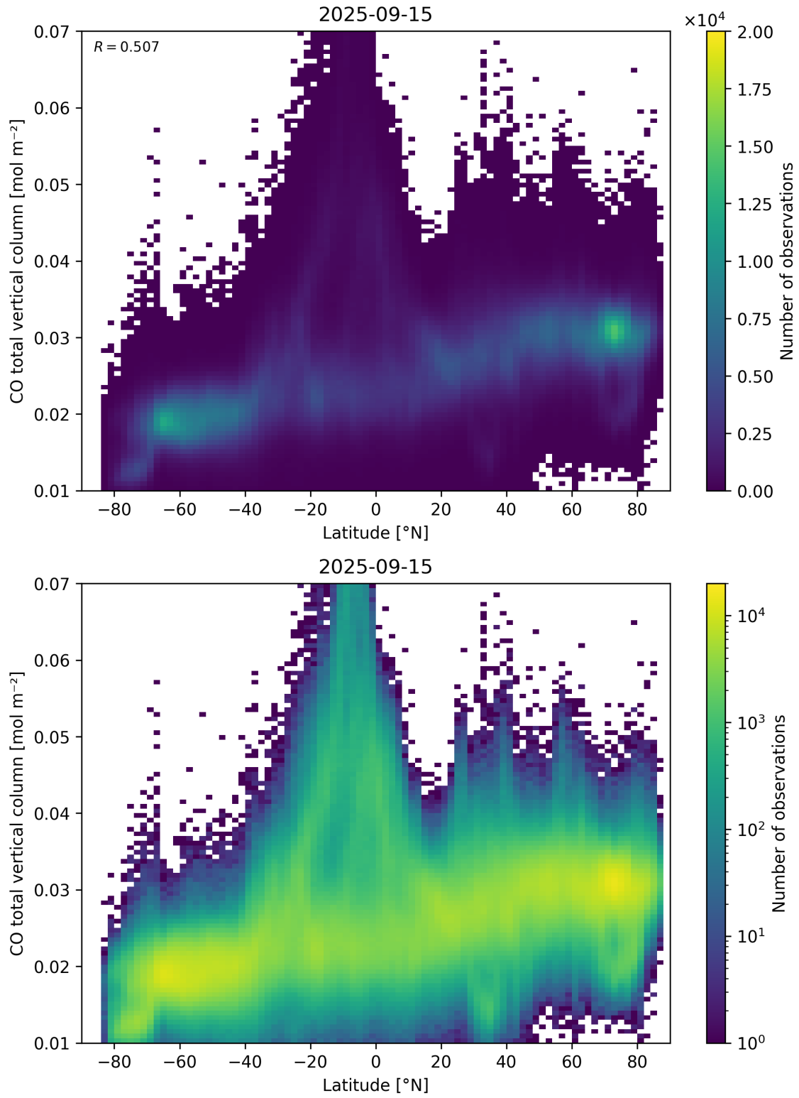
Figure 51: Scatter density plot of “Latitude” against “CO total vertical column” for 2025-09-15 to 2025-09-16.
