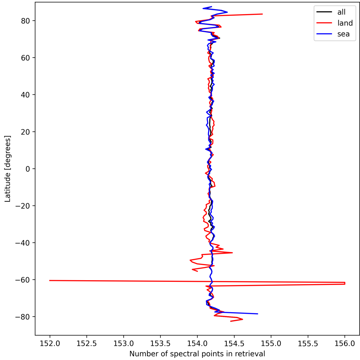
Figure 13: Zonal average of “Number of spectral points in retrieval” for 2025-09-15 to 2025-09-16.
