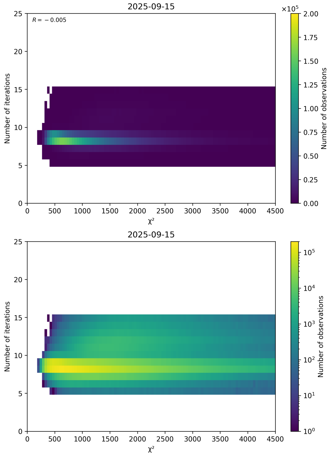
Figure 49: Scatter density plot of “ \chi^2 ” against “Number of iterations” for 2025-09-15 to 2025-09-16.
