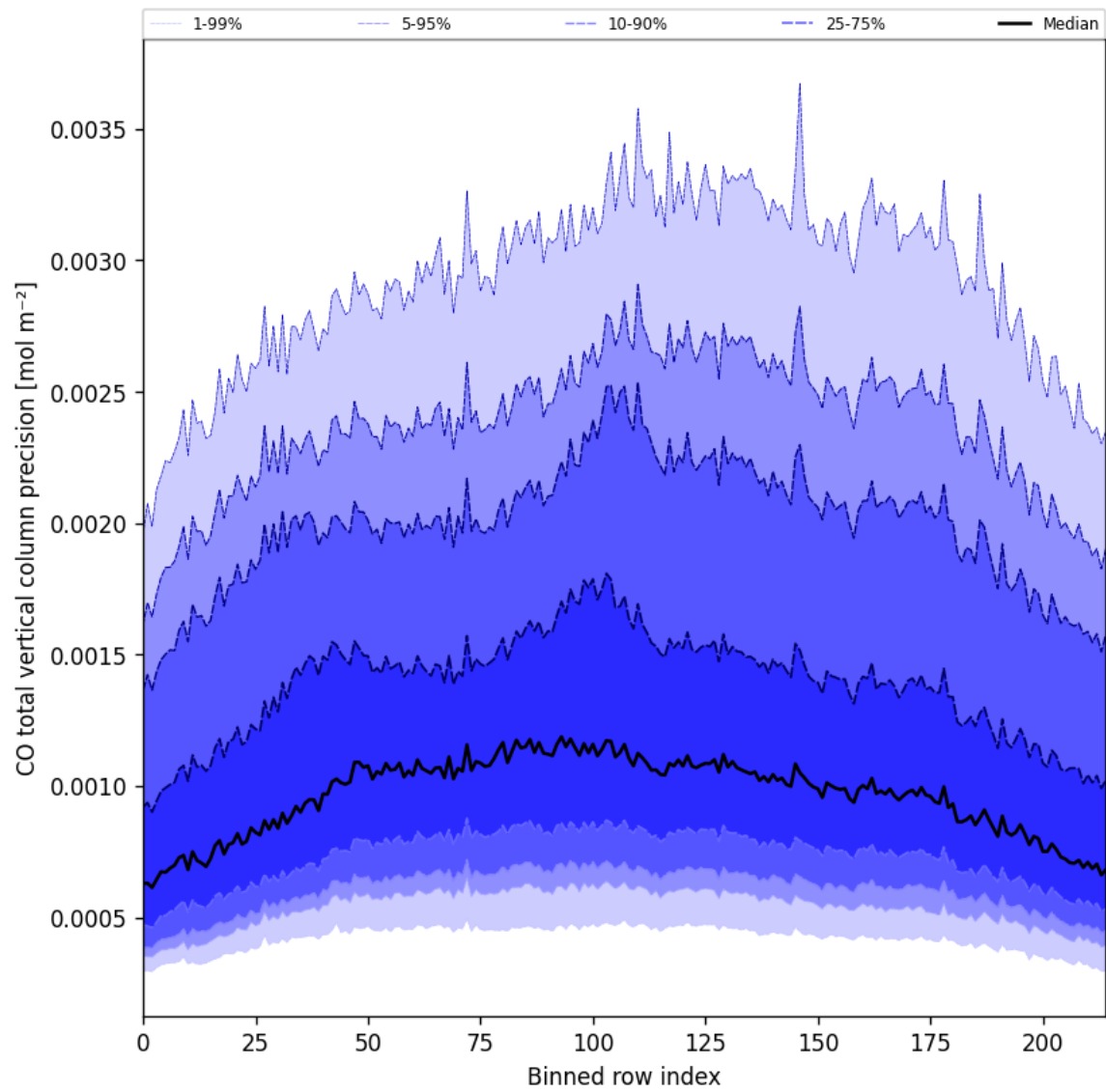
Figure 28: Along track statistics of “CO total vertical column precision” for 2025-09-15 to 2025-09-16
