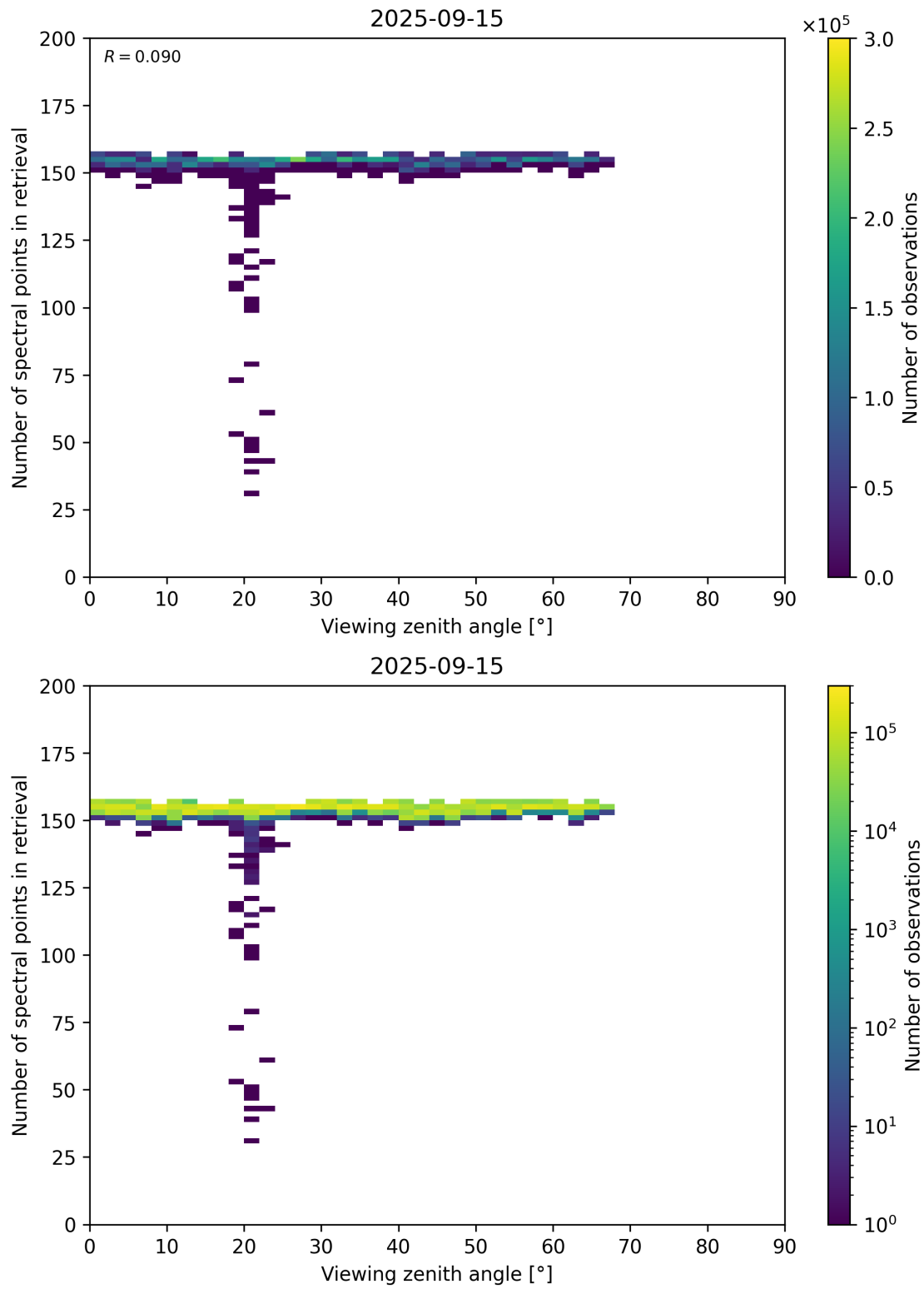
Figure 76: Scatter density plot of “Viewing zenith angle” against “Number of spectral points in retrieval” for 2025-09-15 to 2025-09-16.
