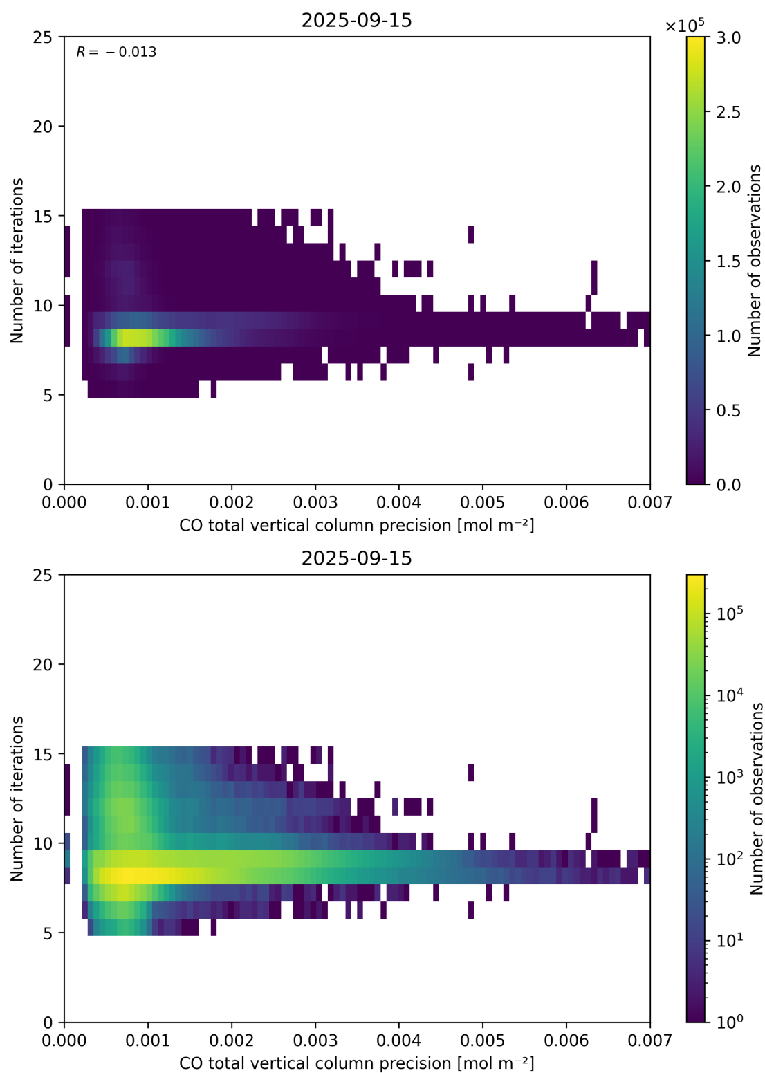
Figure 46: Scatter density plot of “CO total vertical column precision” against “Number of iterations” for 2025-09-15 to 2025-09-16.
