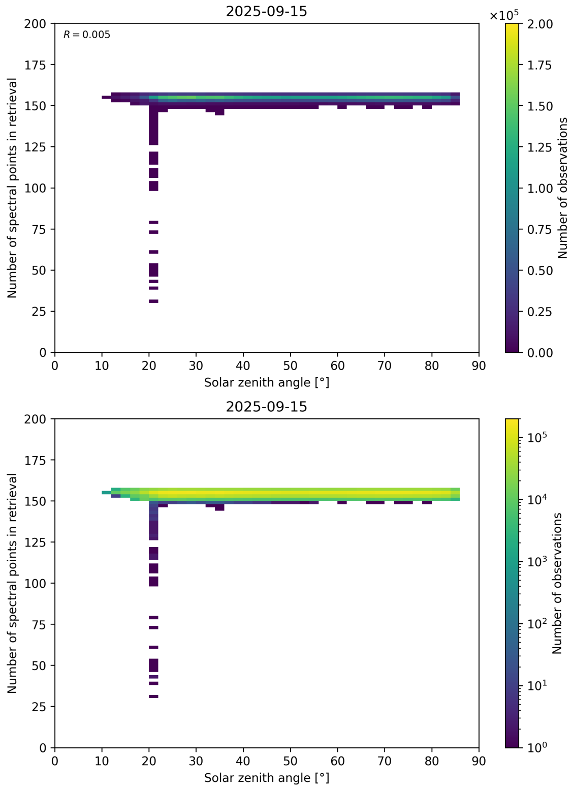
Figure 68: Scatter density plot of “Solar zenith angle” against “Number of spectral points in retrieval” for 2025-09-15 to 2025-09-16.
