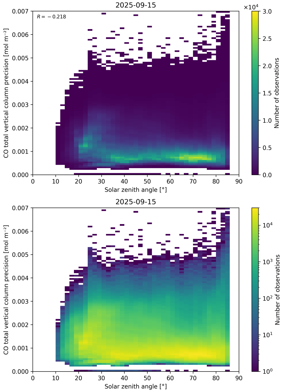
Figure 63: Scatter density plot of “Solar zenith angle” against “CO total vertical column precision” for 2025-09-15 to 2025-09-16.
