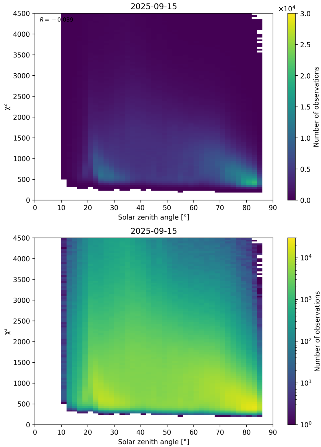
Figure 64: Scatter density plot of “Solar zenith angle” against “ \chi^2 ” for 2025-09-15 to 2025-09-16.
