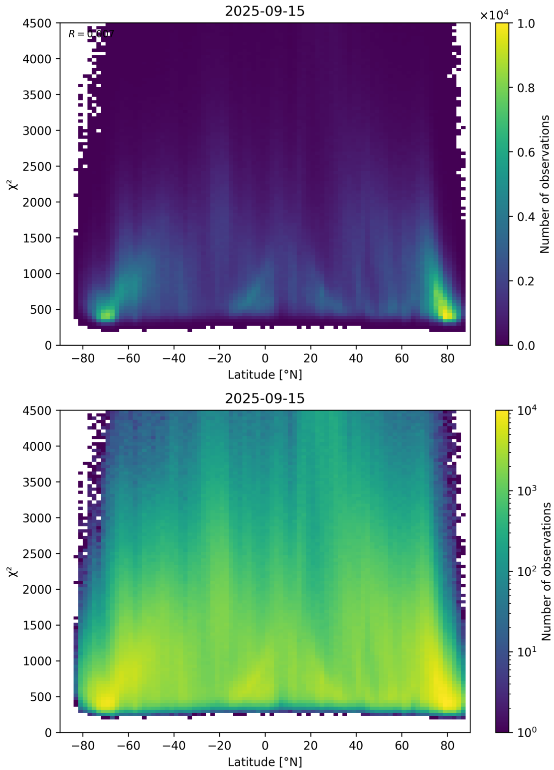
Figure 54: Scatter density plot of “Latitude” against “ \chi^2 ” for 2025-09-15 to 2025-09-16.
