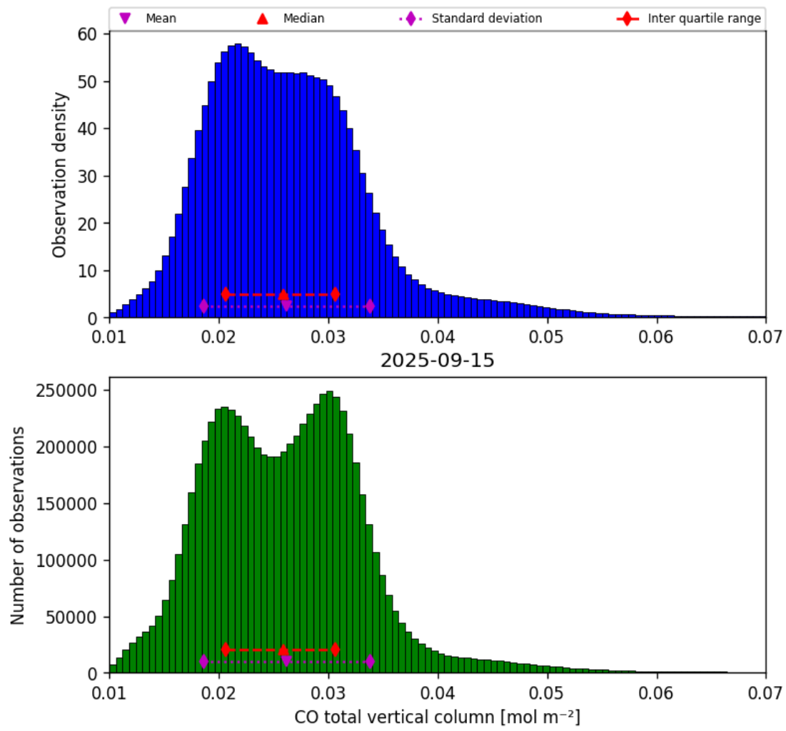
Figure 18: Histogram of “CO total vertical column” for 2025-09-15 to 2025-09-16
