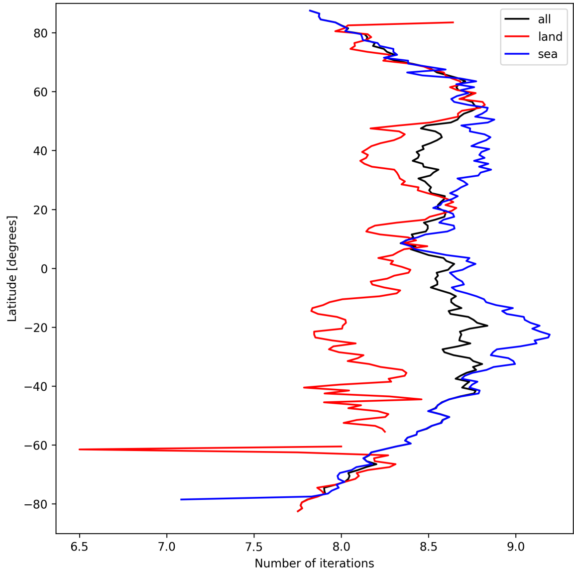
Figure 16: Zonal average of “Number of iterations” for 2025-09-15 to 2025-09-16.
