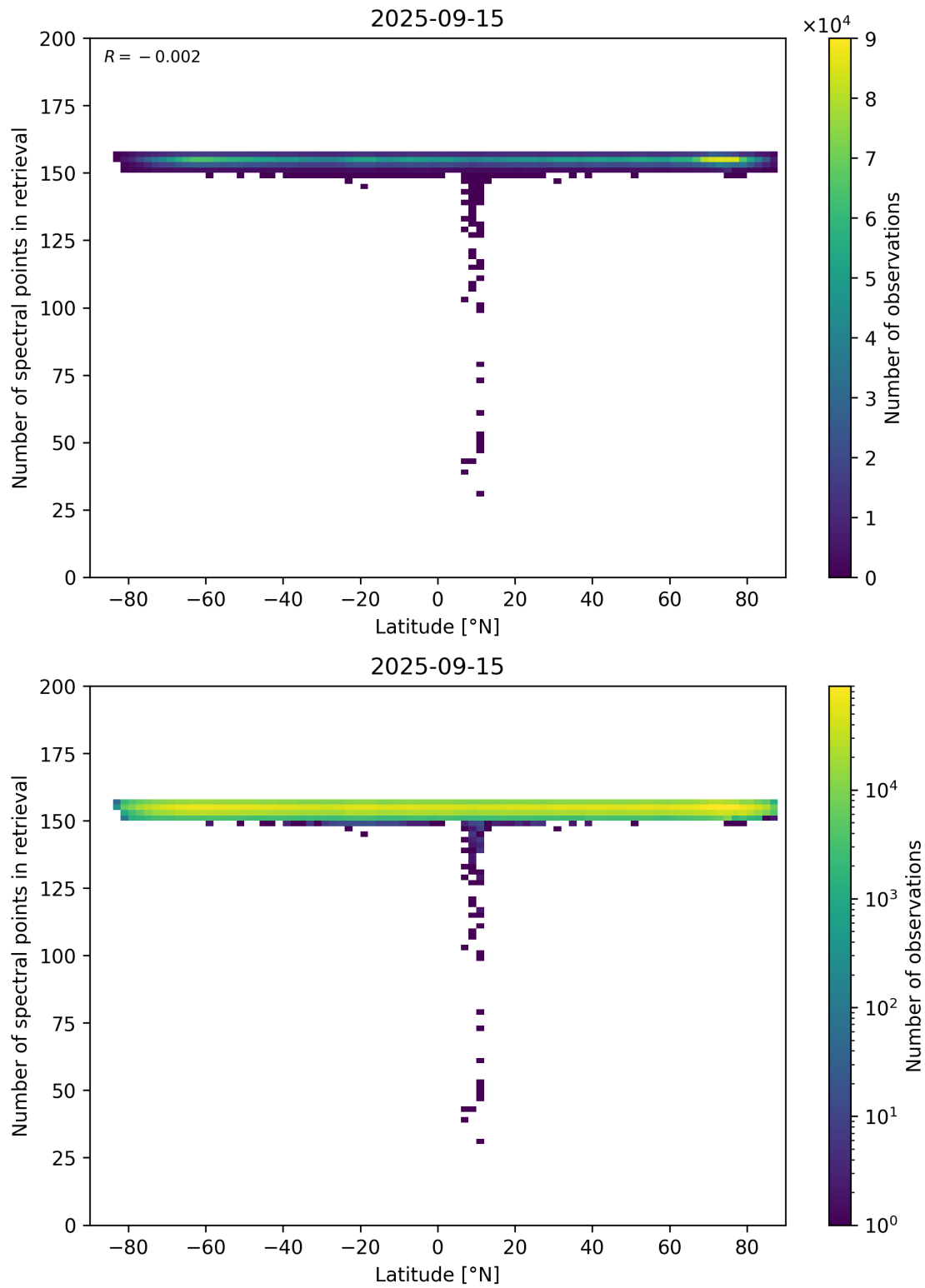
Figure 57: Scatter density plot of “Latitude” against “Number of spectral points in retrieval” for 2025-09-15 to 2025-09-16.
