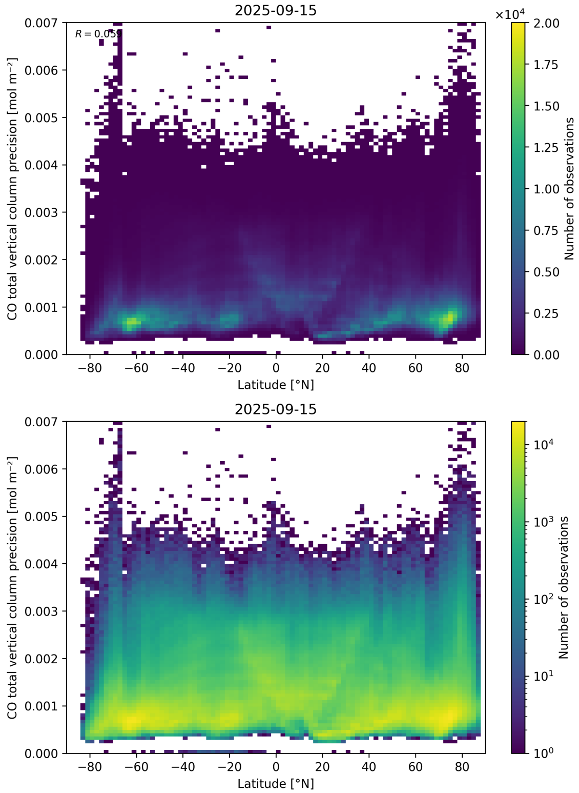
Figure 53: Scatter density plot of “Latitude” against “CO total vertical column precision” for 2025-09-15 to 2025-09-16.
