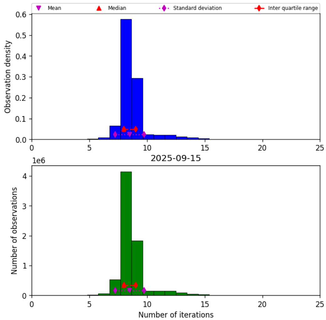
Figure 24: Histogram of “Number of iterations” for 2025-09-15 to 2025-09-16
