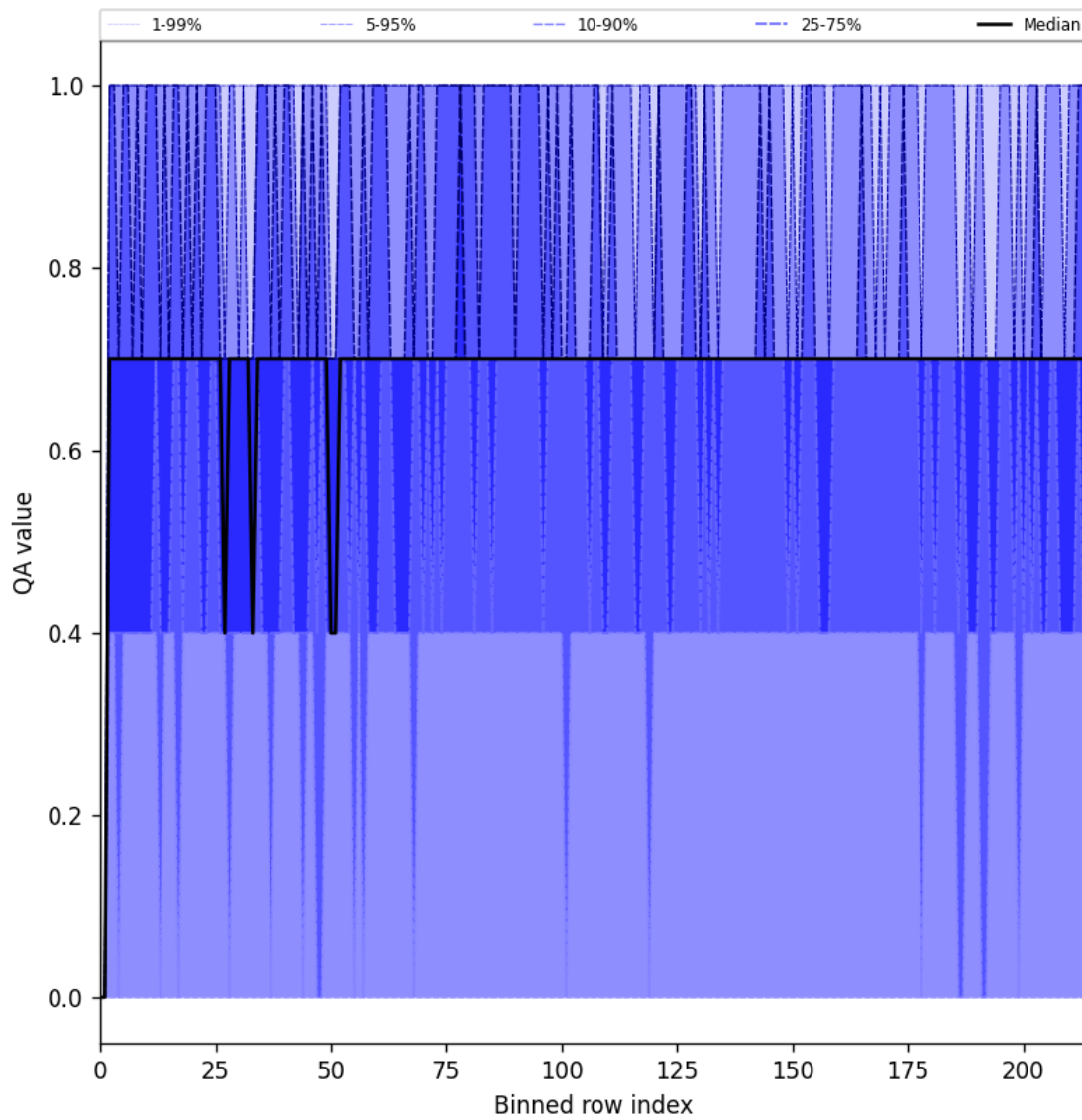
Figure 25: Along track statistics of “QA value” for 2025-09-15 to 2025-09-16
