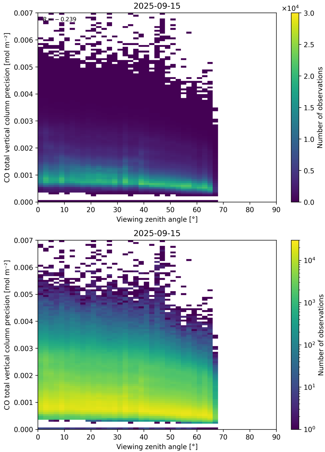
Figure 71: Scatter density plot of “Viewing zenith angle” against “CO total vertical column precision” for 2025-09-15 to 2025-09-16.
