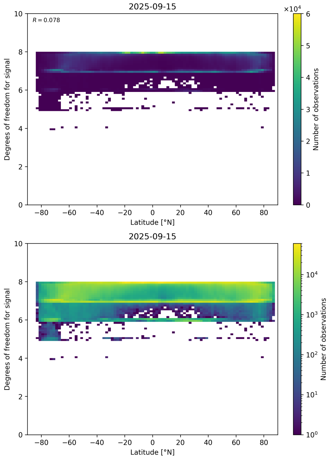
Figure 55: Scatter density plot of “Latitude” against “Degrees of freedom for signal” for 2025-09-15 to 2025-09-16.
