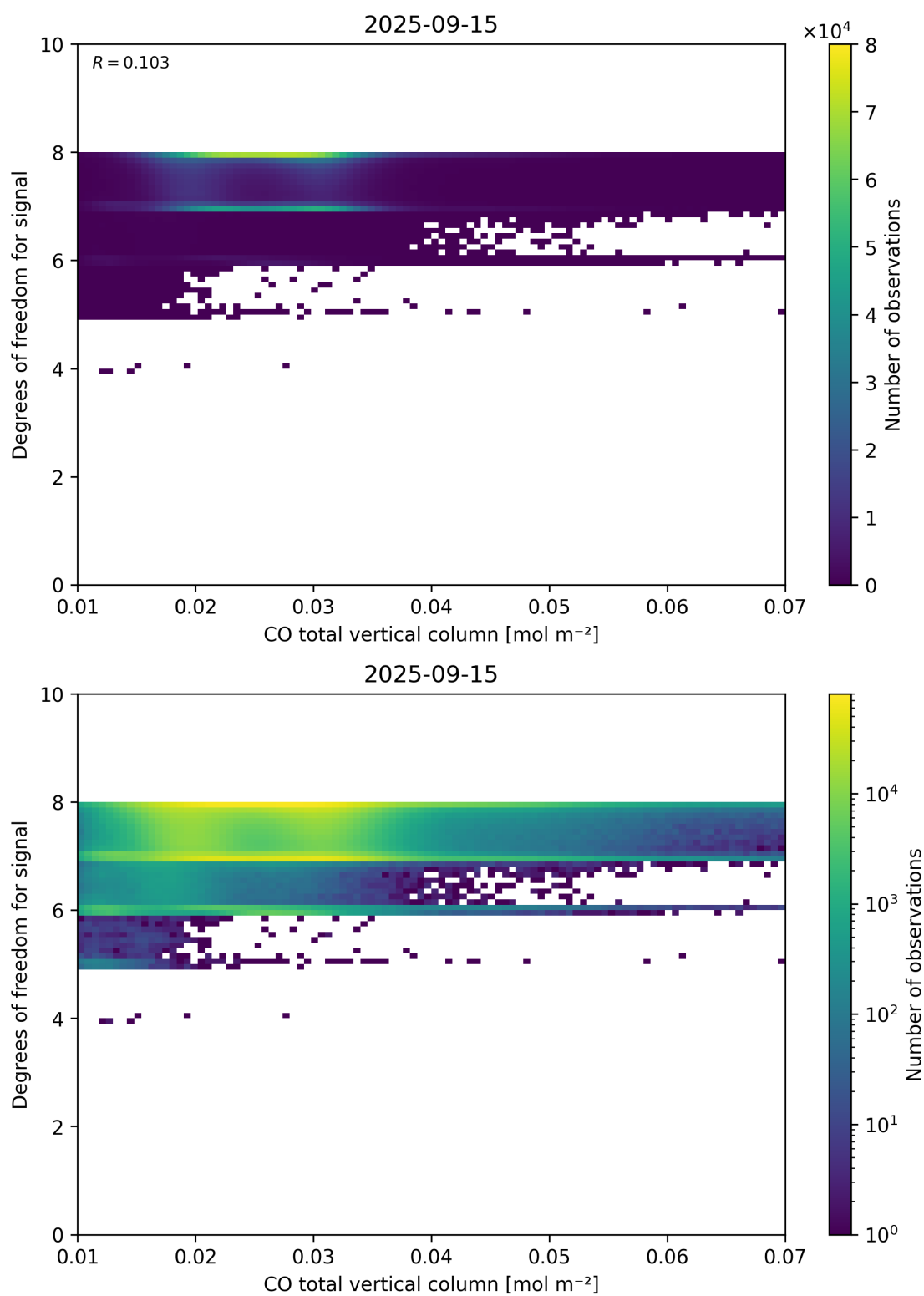
Figure 41: Scatter density plot of “CO total vertical column” against “Degrees of freedom for signal” for 2025-09-15 to 2025-09-16.
