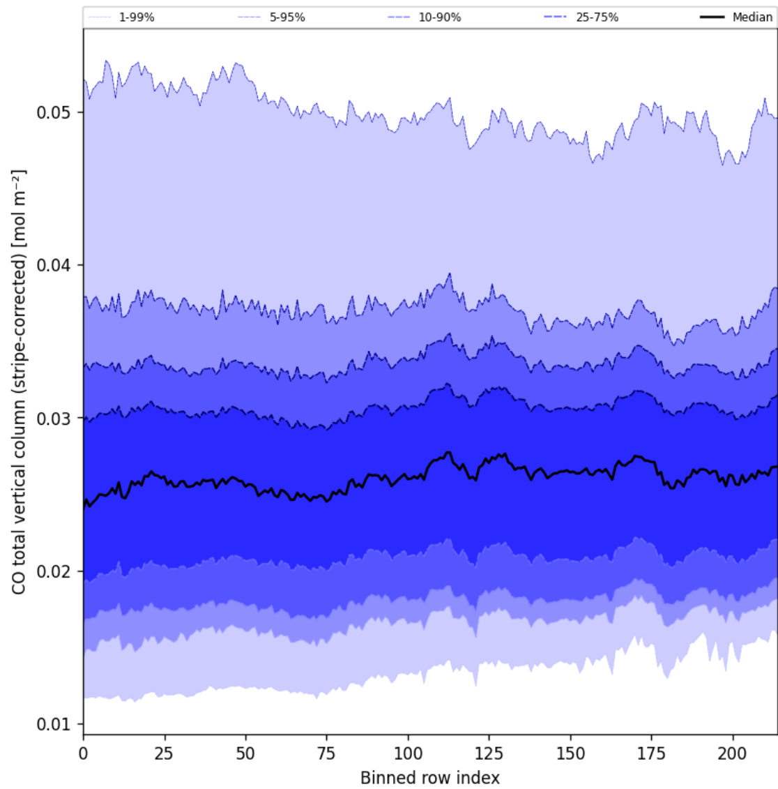
Figure 27: Along track statistics of “CO total vertical column (stripe-corrected)” for 2025-09-15 to 2025-09-16
