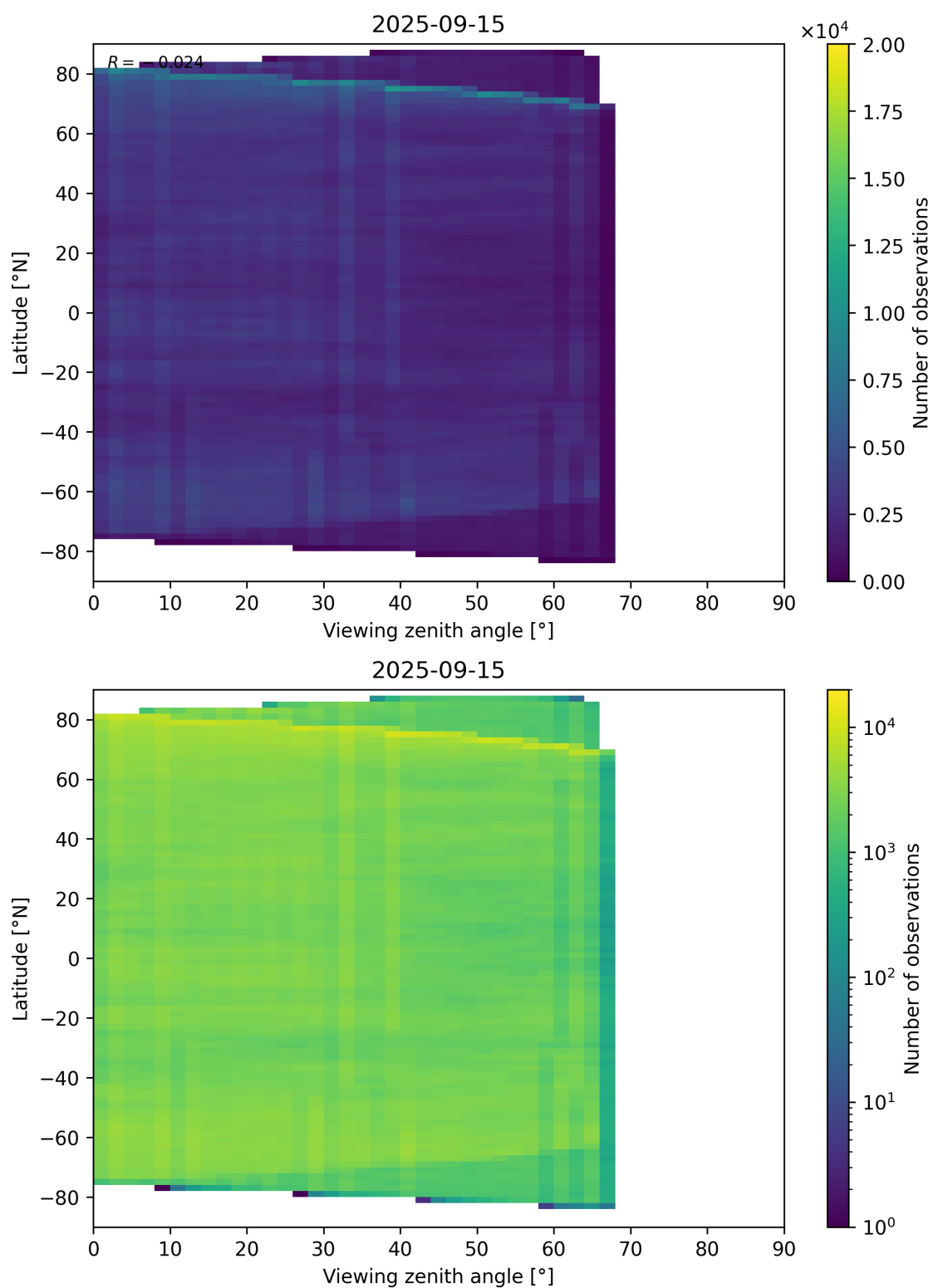
Figure 74: Scatter density plot of “Viewing zenith angle” against “Latitude” for 2025-09-15 to 2025-09-16.
