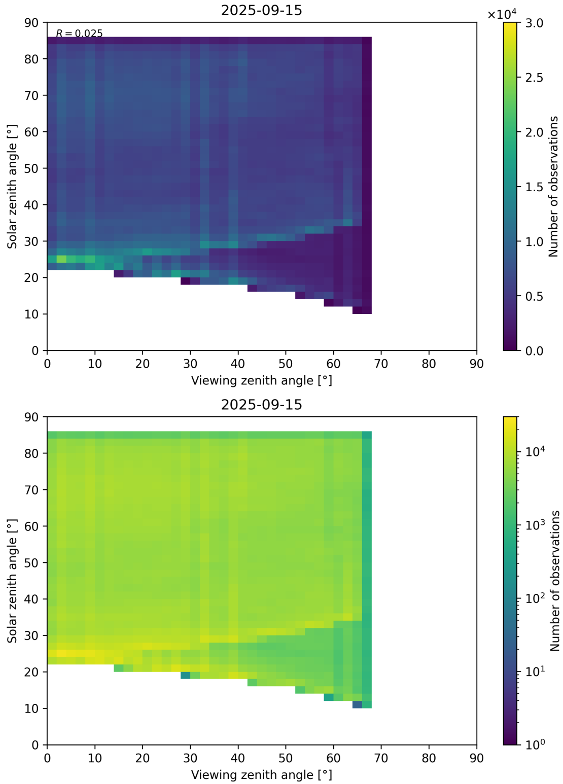
Figure 77: Scatter density plot of “Viewing zenith angle” against “Solar zenith angle” for 2025-09-15 to 2025-09-16.
