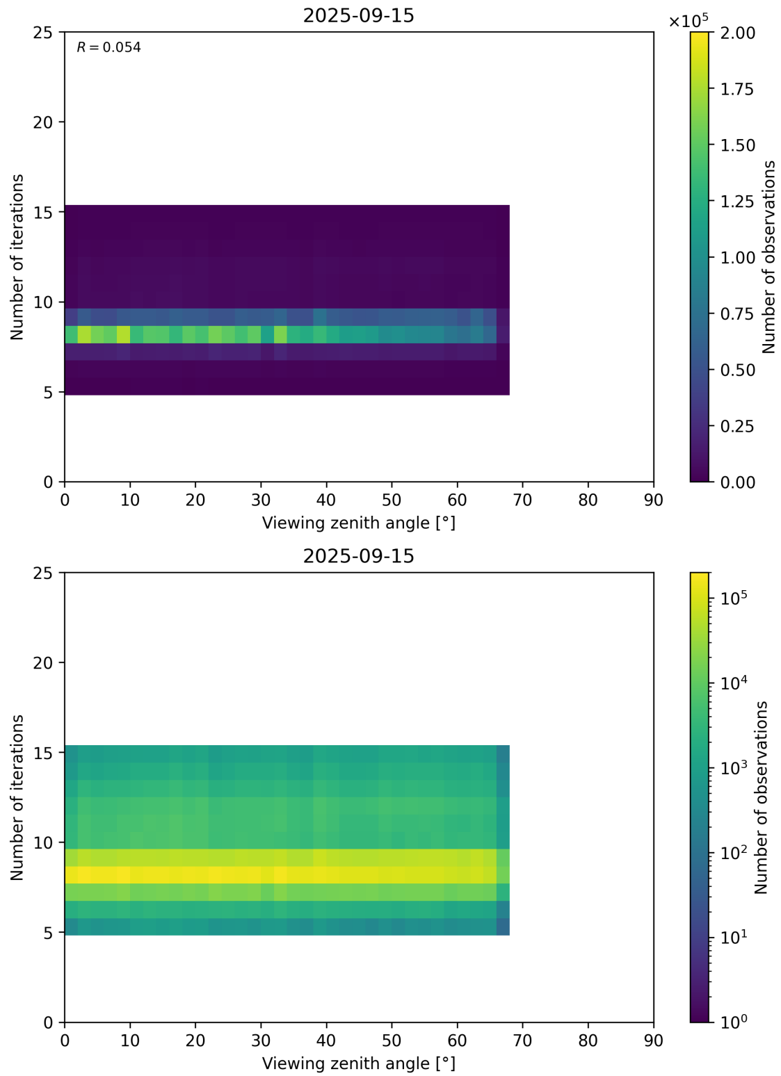
Figure 75: Scatter density plot of “Viewing zenith angle” against “Number of iterations” for 2025-09-15 to 2025-09-16.
