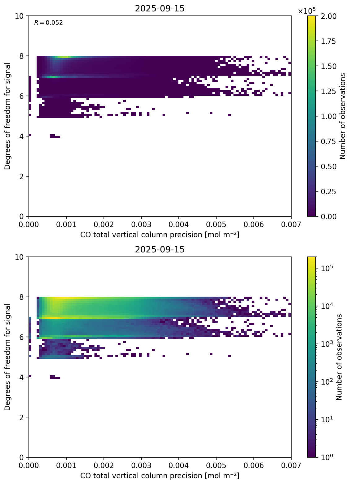
Figure 45: Scatter density plot of “CO total vertical column precision” against “Degrees of freedom for signal” for 2025-09-15 to 2025-09-16.
