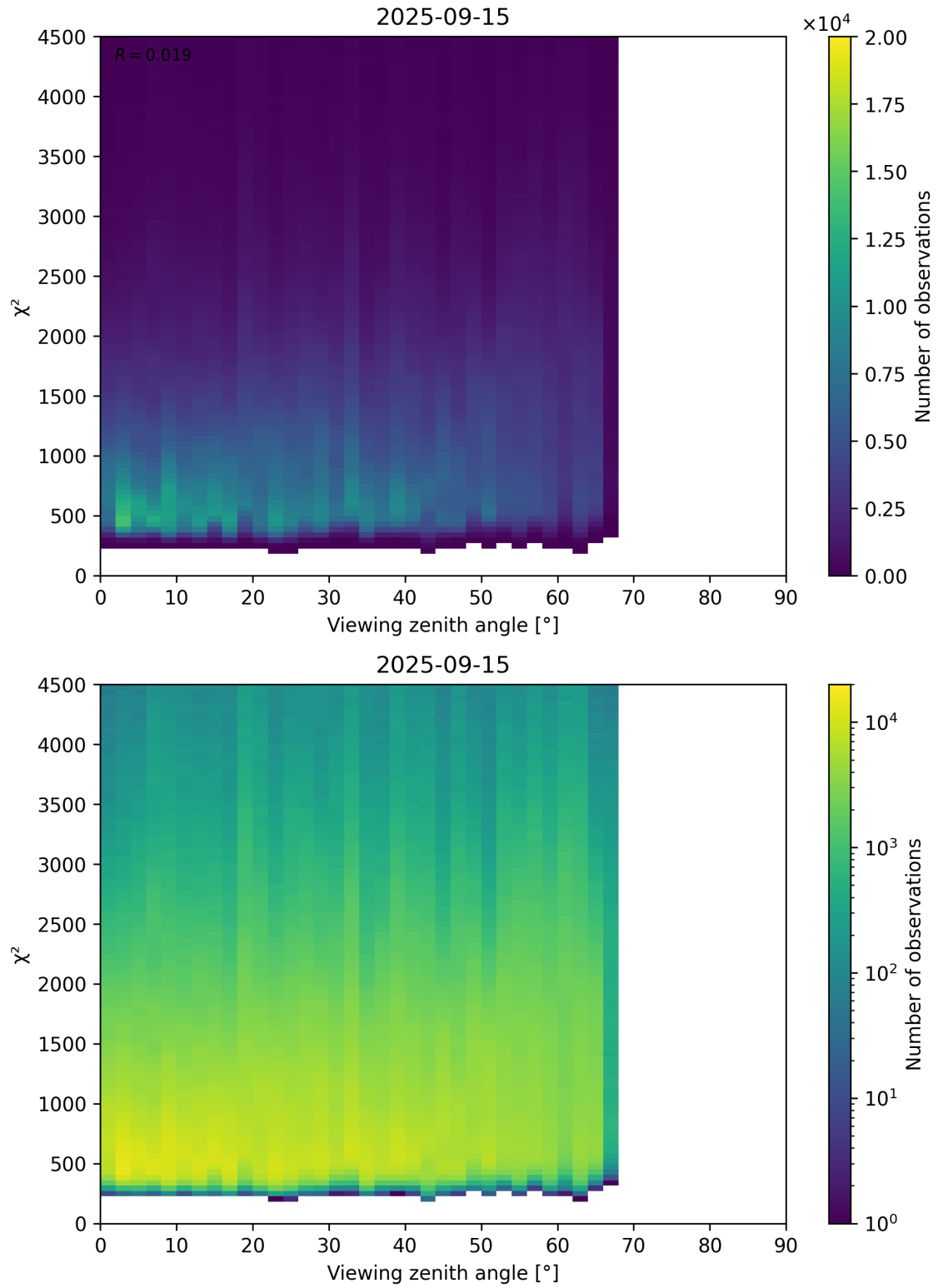
Figure 72: Scatter density plot of “Viewing zenith angle” against “ \chi^2 ” for 2025-09-15 to 2025-09-16.
