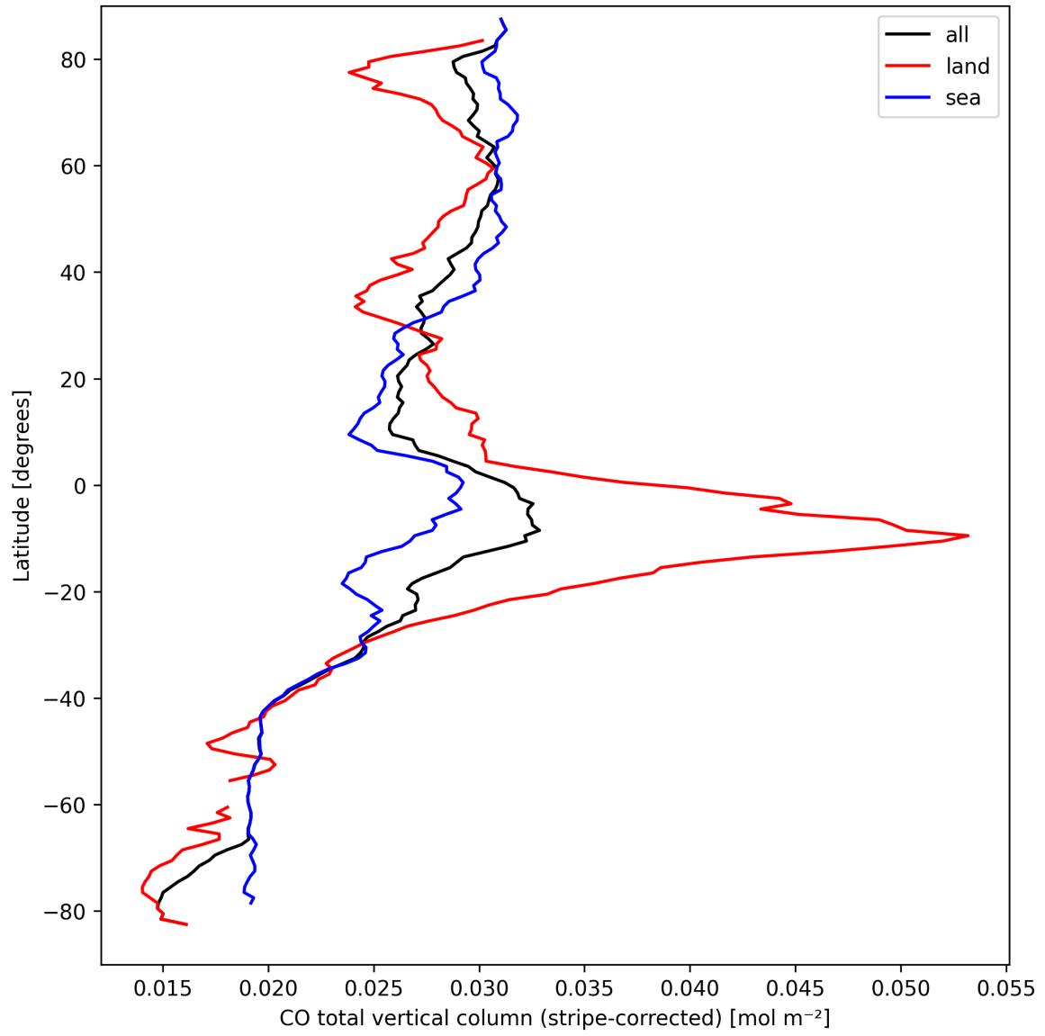
Figure 11: Zonal average of “CO total vertical column (stripe-corrected)” for 2025-09-15 to 2025-09-16.
