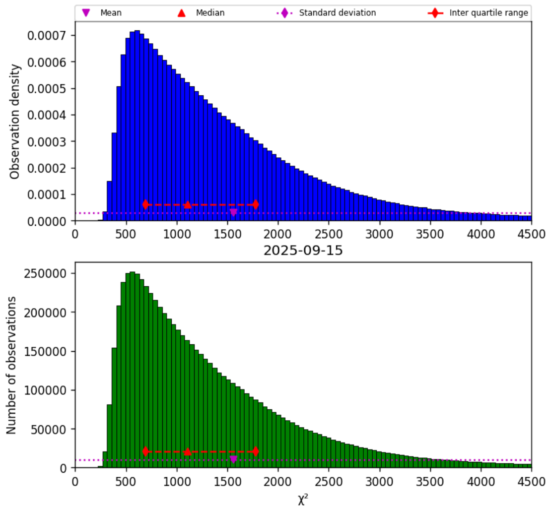
Figure 22: Histogram of “ \chi^2 ” for 2025-09-15 to 2025-09-16
