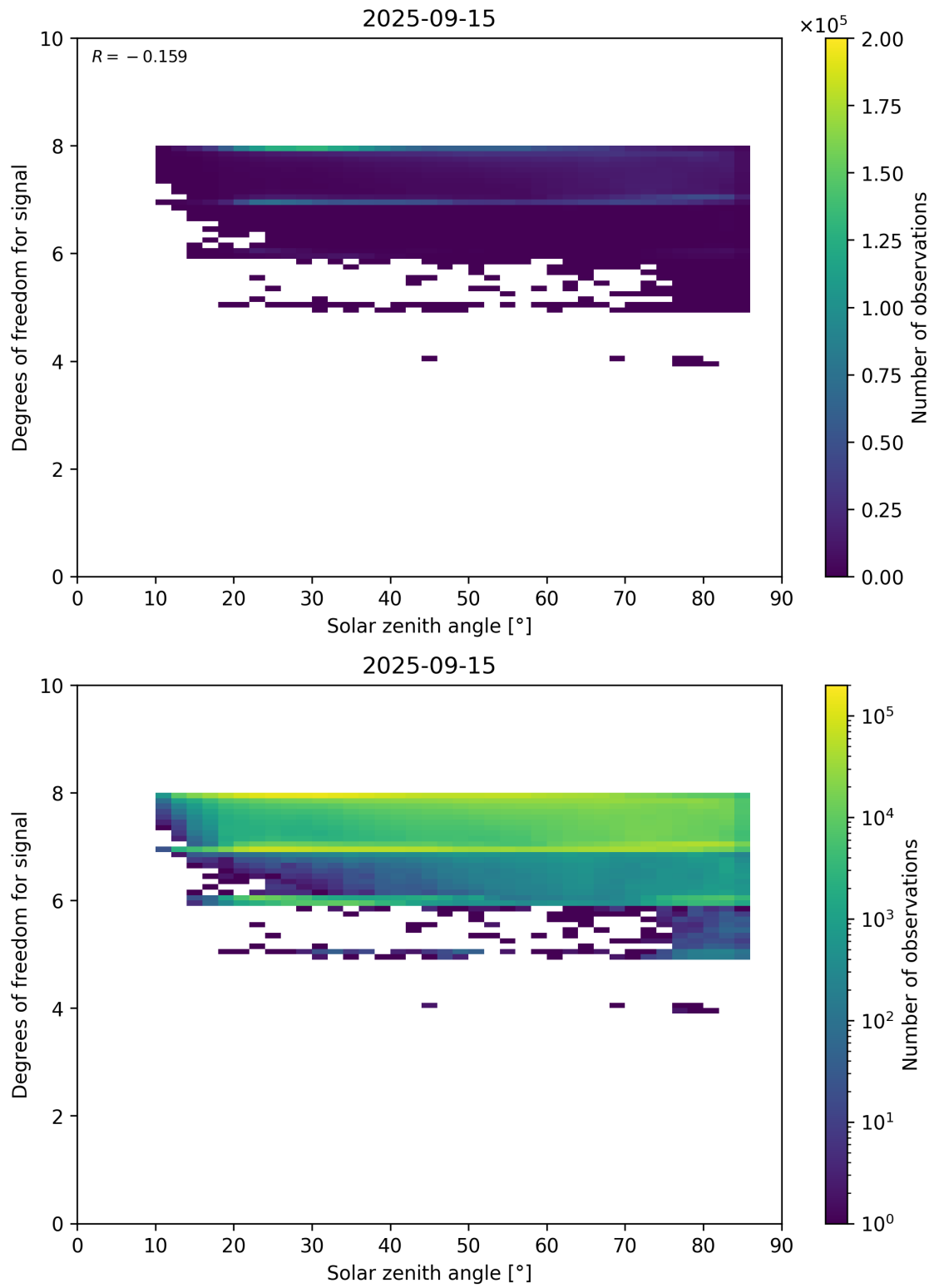
Figure 65: Scatter density plot of “Solar zenith angle” against “Degrees of freedom for signal” for 2025-09-15 to 2025-09-16.
