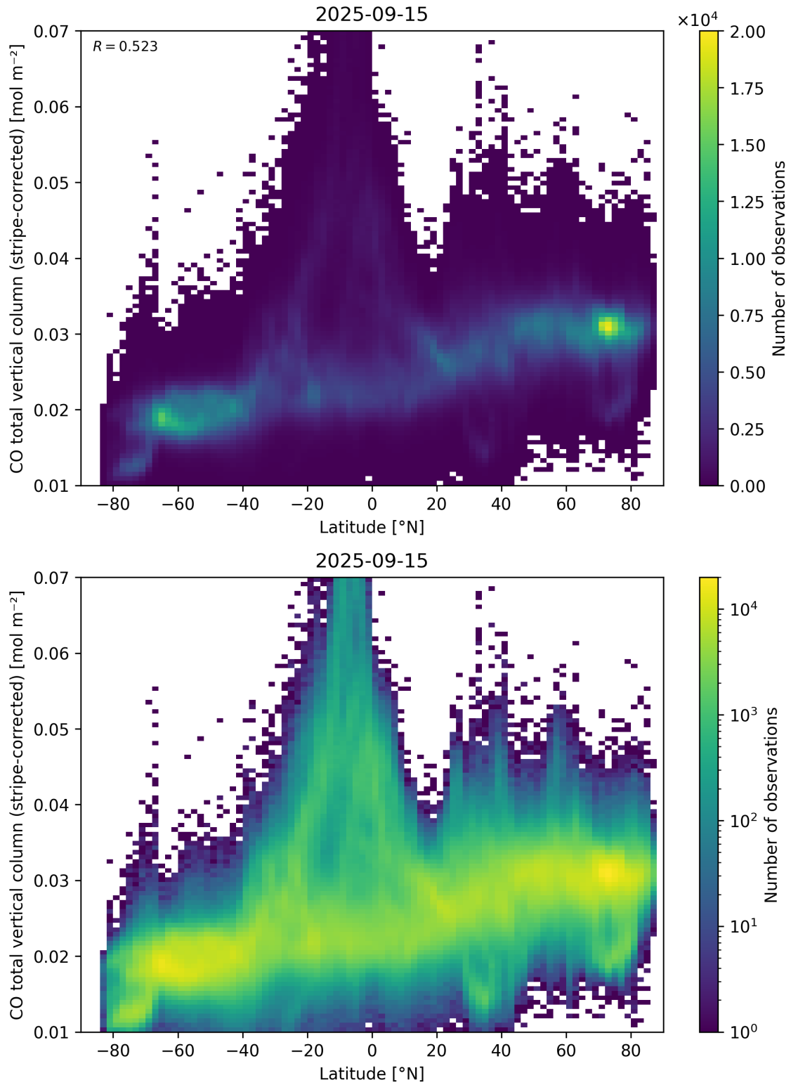
Figure 52: Scatter density plot of “Latitude” against “CO total vertical column (stripe-corrected)” for 2025-09-15 to 2025-09-16.
