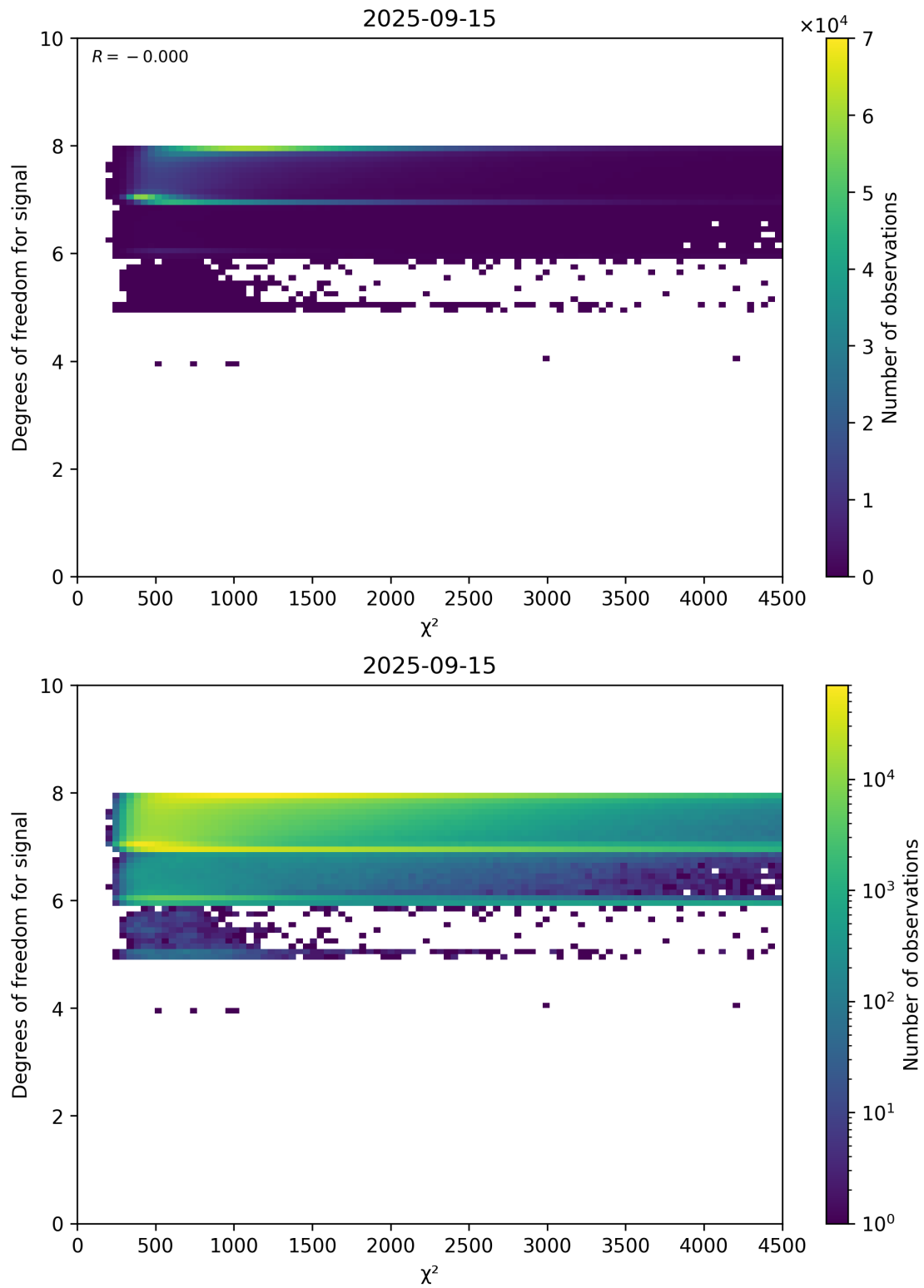
Figure 48: Scatter density plot of " \chi^2 " against "Degrees of freedom for signal" for 2025-09-15 to 2025-09-16.
