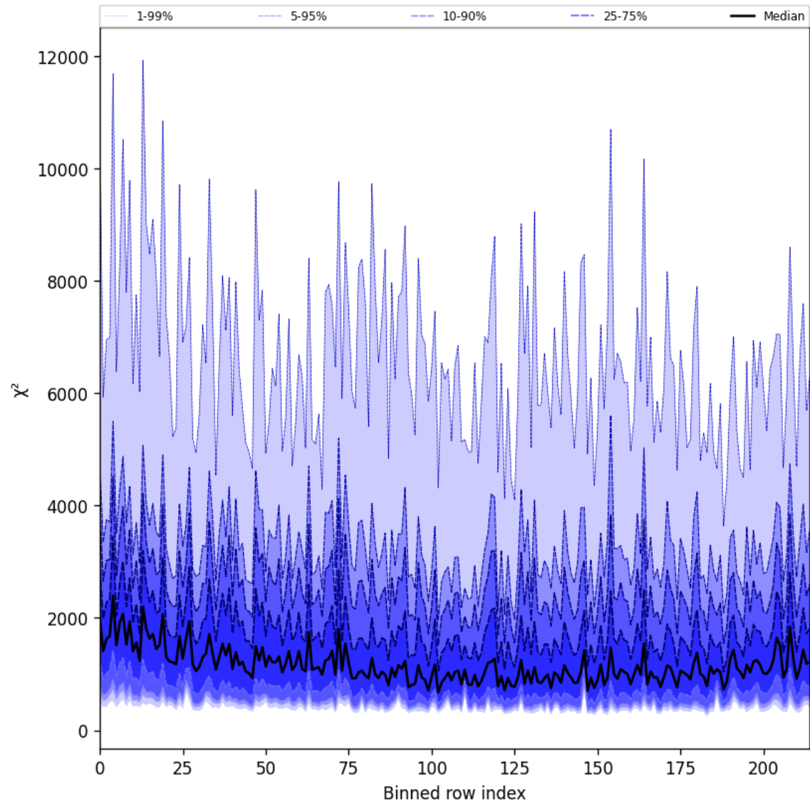
Figure 30: Along track statistics of “ \chi^2 ” for 2025-09-15 to 2025-09-16
