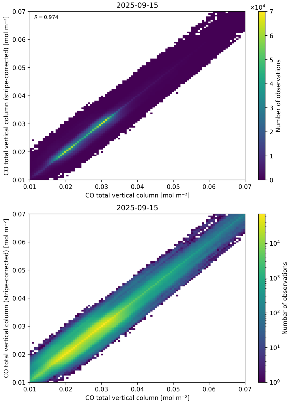
Figure 33: Scatter density plot of “CO total vertical column” against “CO total vertical column (stripe-corrected)” for 2025-09-15 to 2025-09-16.
