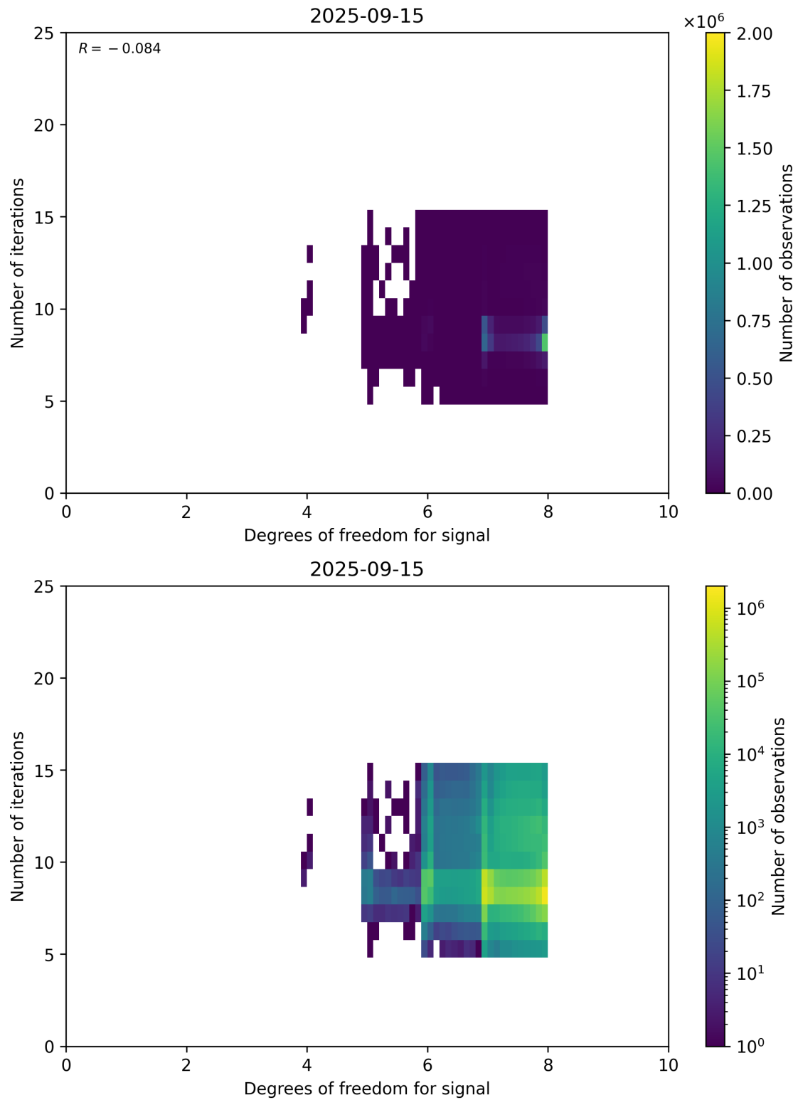
Figure 50: Scatter density plot of “Degrees of freedom for signal” against “Number of iterations” for 2025-09-15 to 2025-09-16.
