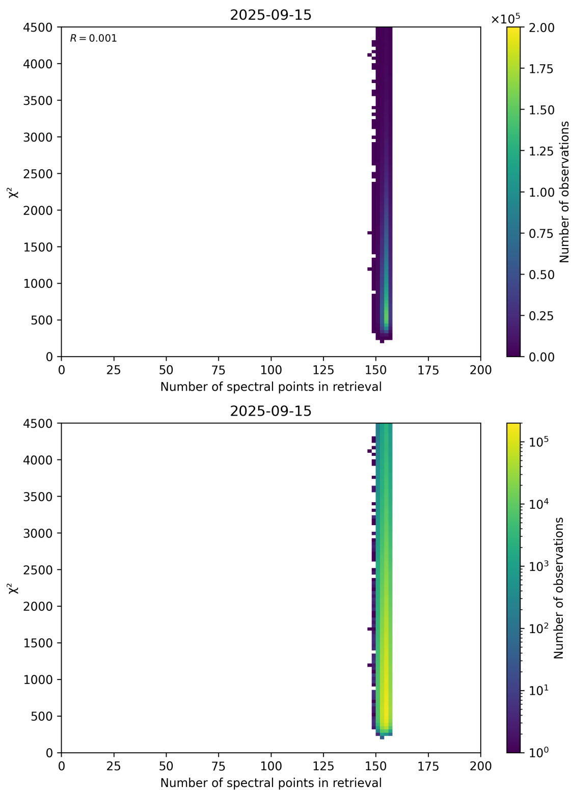
Figure 58: Scatter density plot of “Number of spectral points in retrieval” against “ \chi^2 ” for 2025-09-15 to 2025-09-16.
