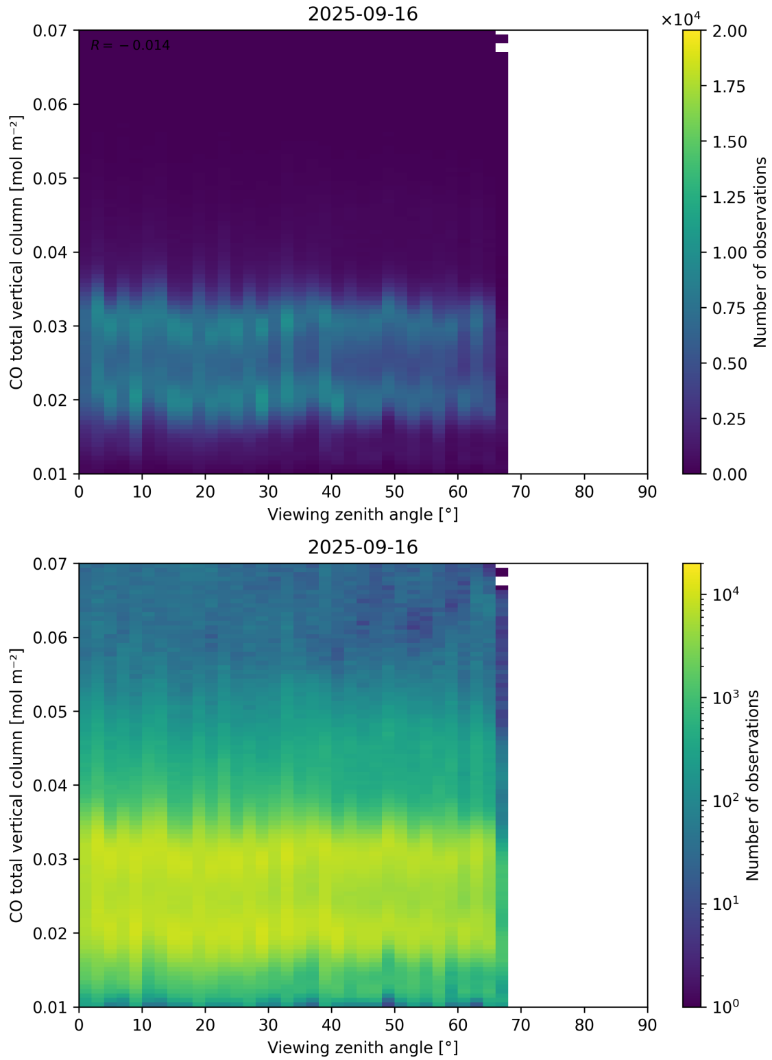
Figure 69: Scatter density plot of “Viewing zenith angle” against “CO total vertical column” for 2025-09-15 to 2025-09-17.
