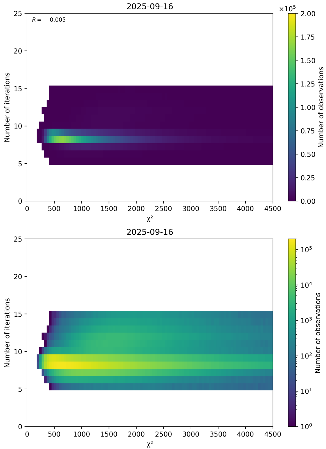
Figure 49: Scatter density plot of “ \chi^2 ” against “Number of iterations” for 2025-09-15 to 2025-09-17.
