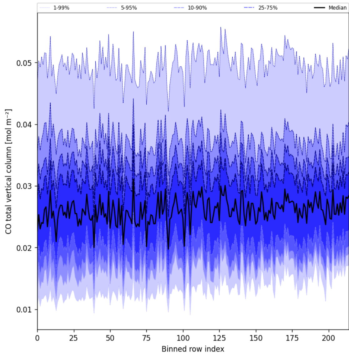
Figure 26: Along track statistics of “CO total vertical column” for 2025-09-15 to 2025-09-17
