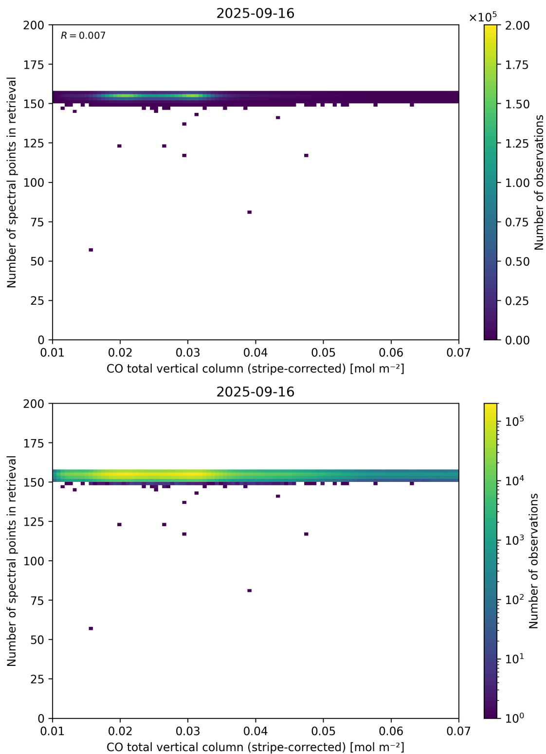
Figure 40: Scatter density plot of “CO total vertical column (stripe-corrected)” against “Number of spectral points in retrieval” for 2025-09-15 to 2025-09-17.
