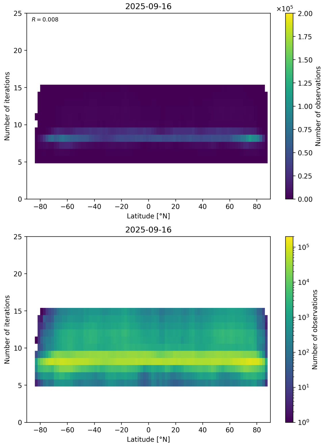
Figure 56: Scatter density plot of “Latitude” against “Number of iterations” for 2025-09-15 to 2025-09-17.
