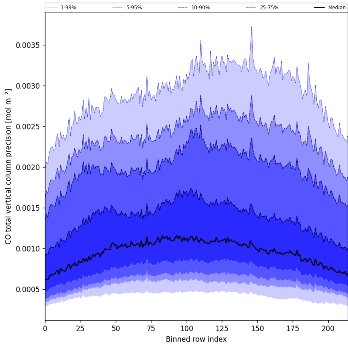
Figure 28: Along track statistics of “CO total vertical column precision” for 2025-09-15 to 2025-09-17
