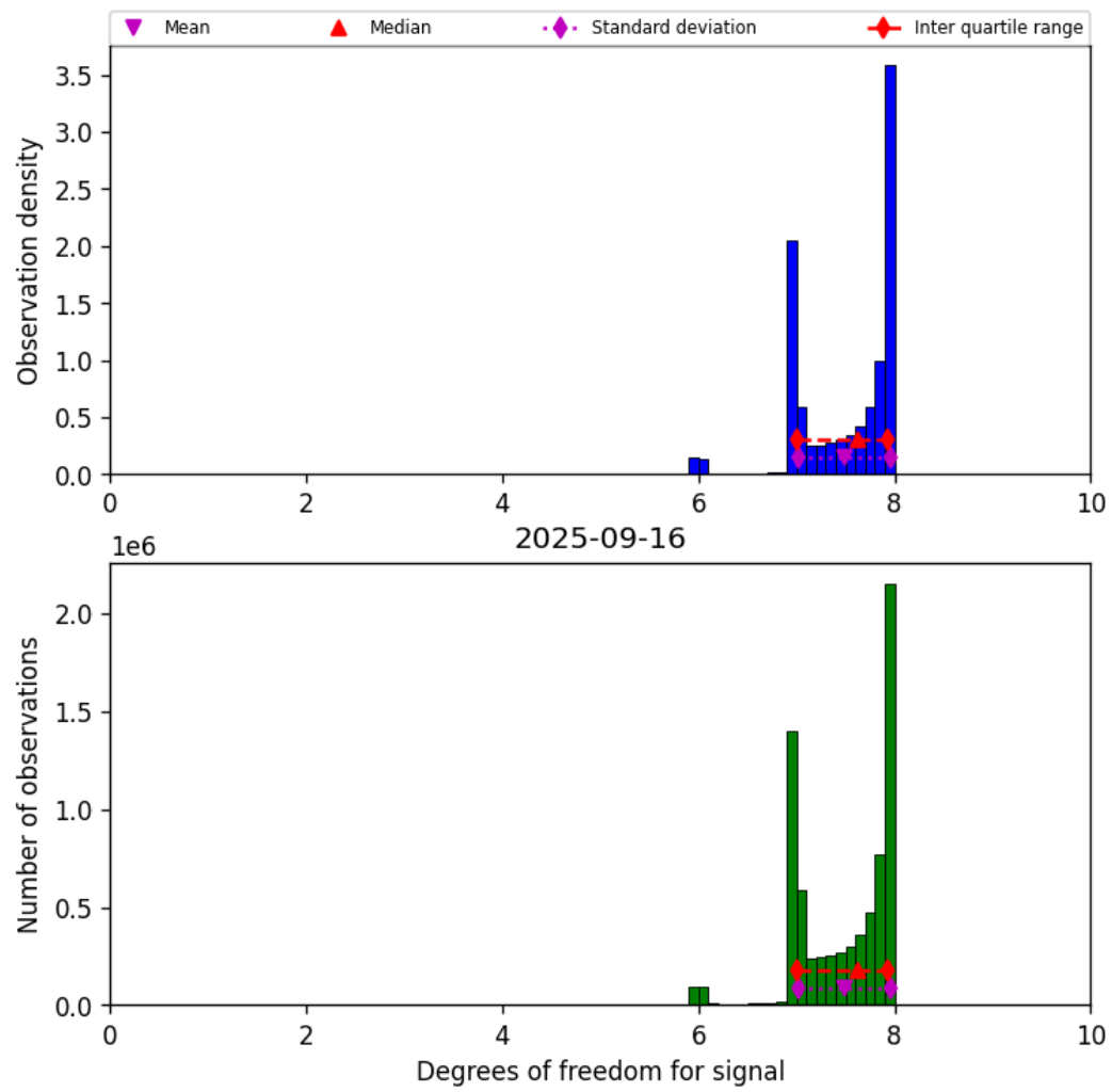
Figure 23: Histogram of “Degrees of freedom for signal” for 2025-09-15 to 2025-09-17
