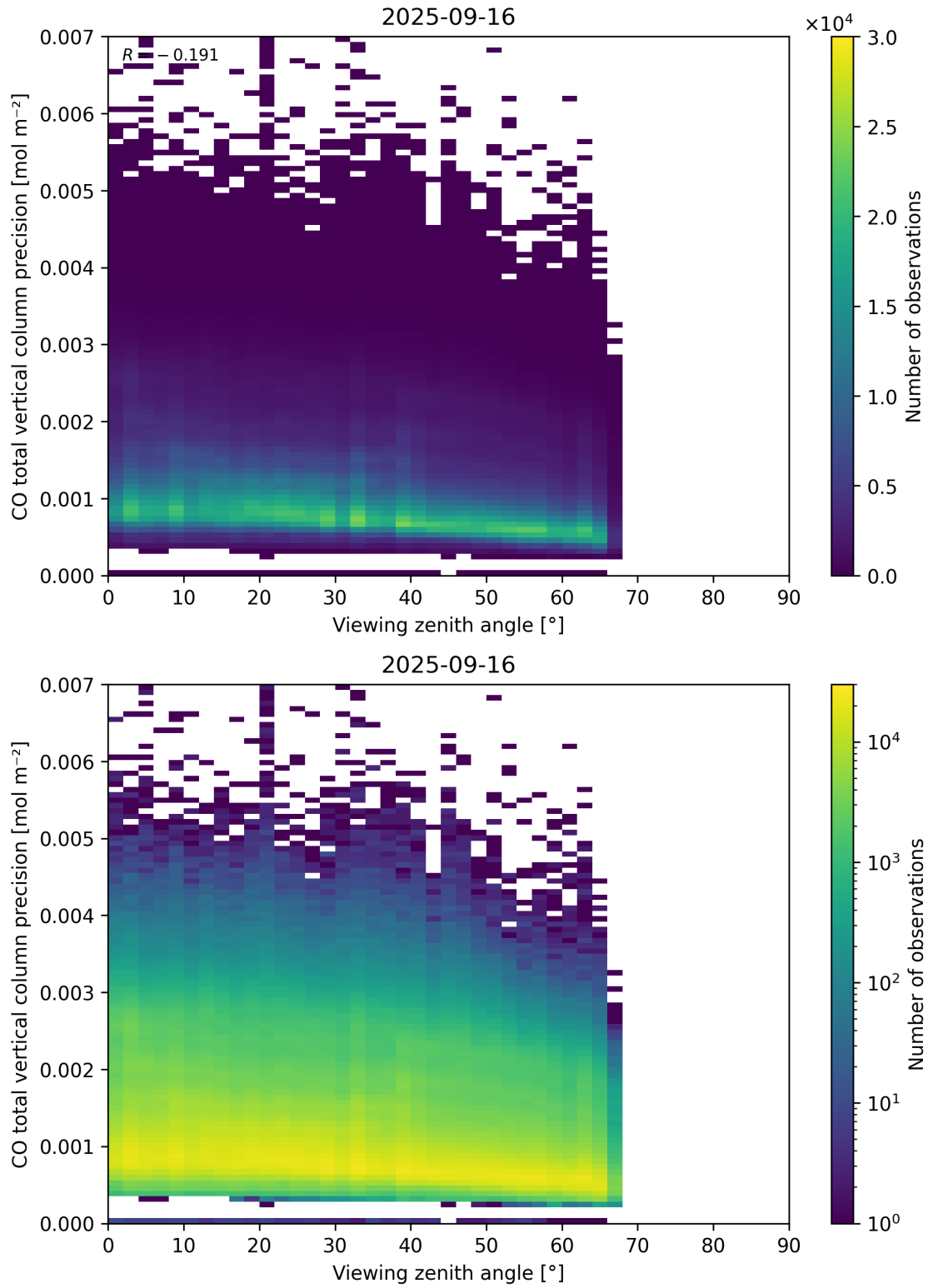
Figure 71: Scatter density plot of “Viewing zenith angle” against “CO total vertical column precision” for 2025-09-15 to 2025-09-17.
