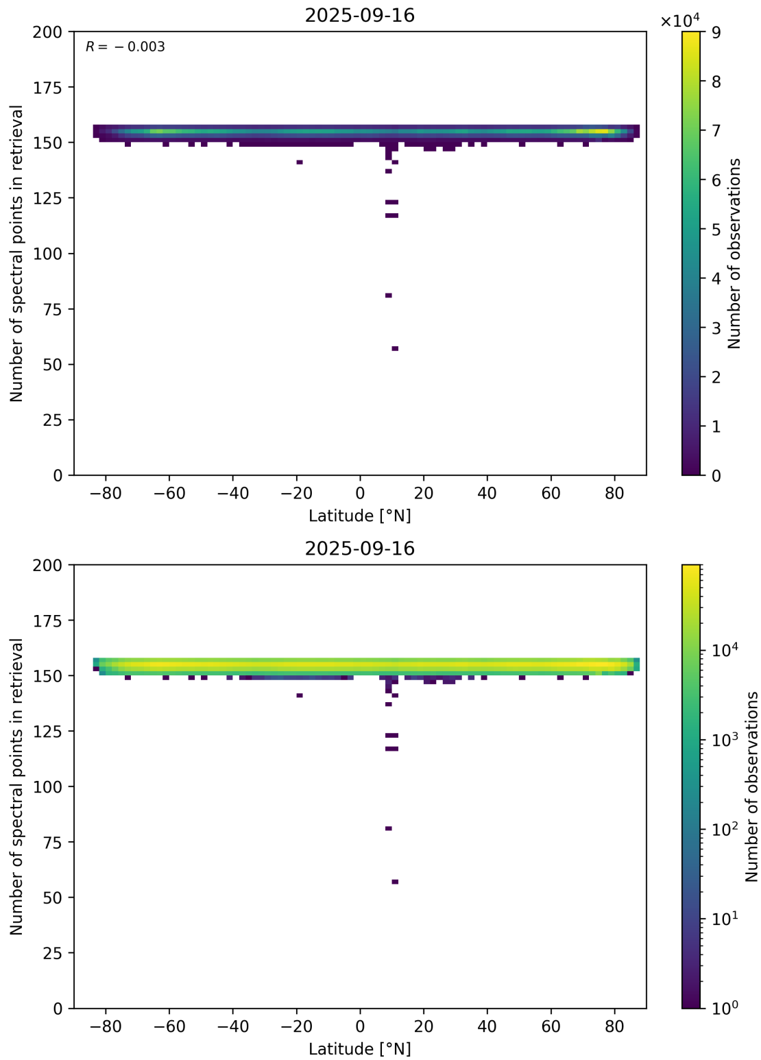
Figure 57: Scatter density plot of “Latitude” against “Number of spectral points in retrieval” for 2025-09-15 to 2025-09-17.
