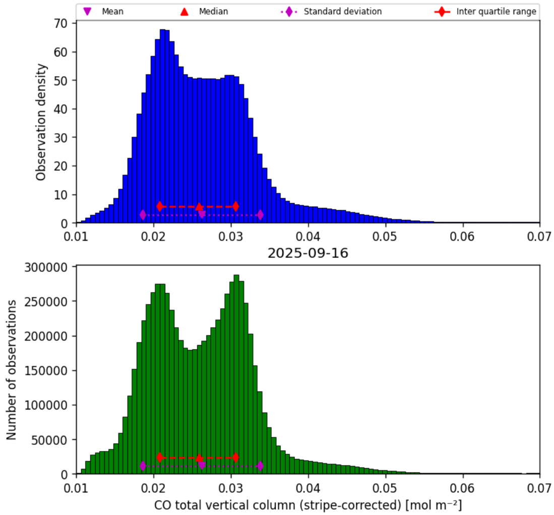
Figure 19: Histogram of “CO total vertical column (stripe-corrected)” for 2025-09-15 to 2025-09-17
