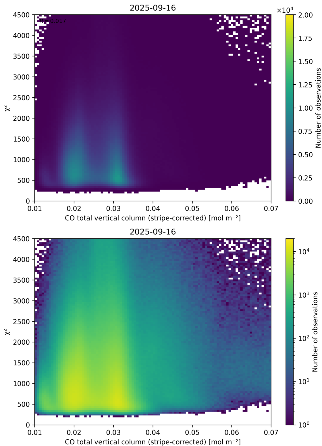
Figure 37: Scatter density plot of “CO total vertical column (stripe-corrected)” against “ \chi^2 ” for 2025-09-15 to 2025-09-17.
