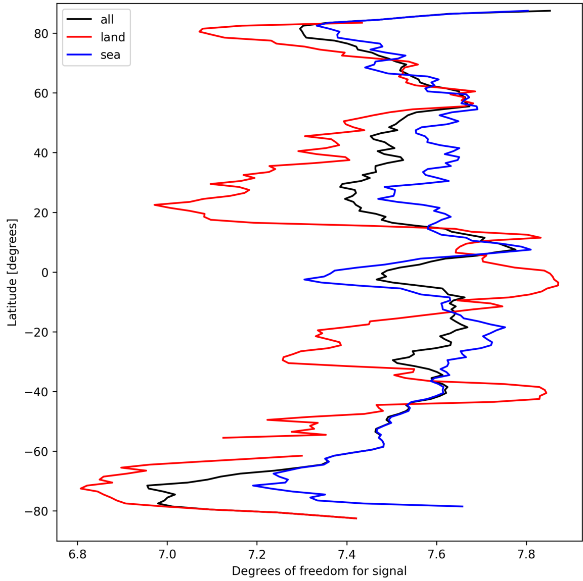
Figure 15: Zonal average of “Degrees of freedom for signal” for 2025-09-15 to 2025-09-17.
