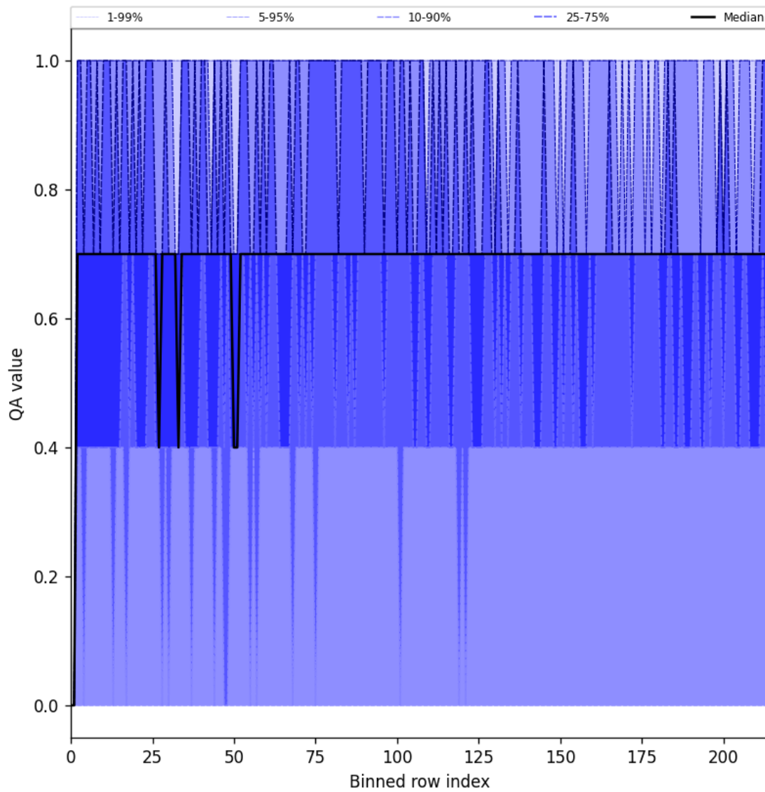
Figure 25: Along track statistics of “QA value” for 2025-09-15 to 2025-09-17
