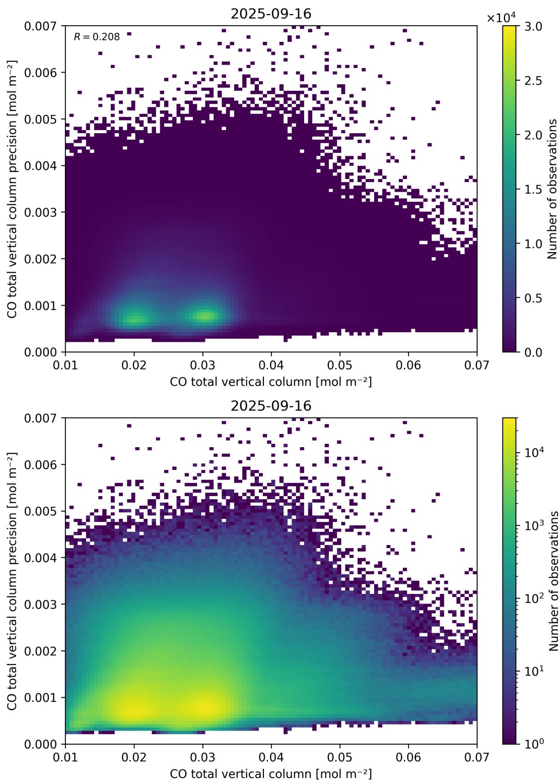
Figure 34: Scatter density plot of “CO total vertical column” against “CO total vertical column precision” for 2025-09-15 to 2025-09-17.
