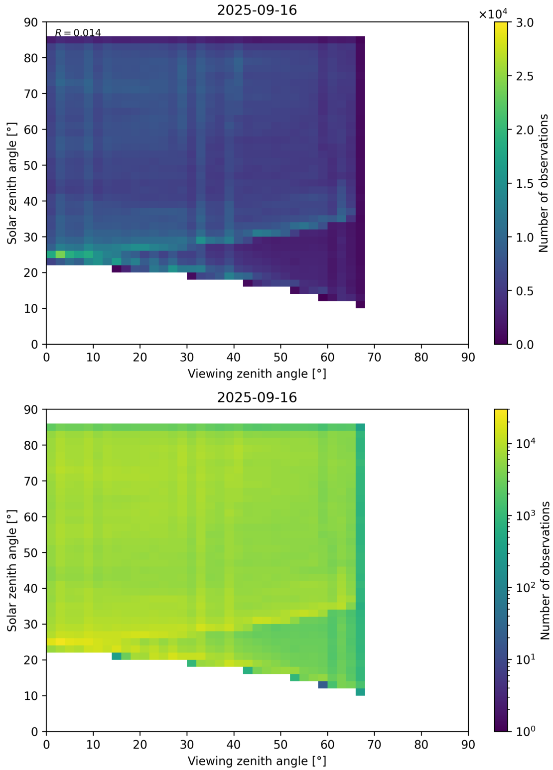
Figure 77: Scatter density plot of “Viewing zenith angle” against “Solar zenith angle” for 2025-09-15 to 2025-09-17.
