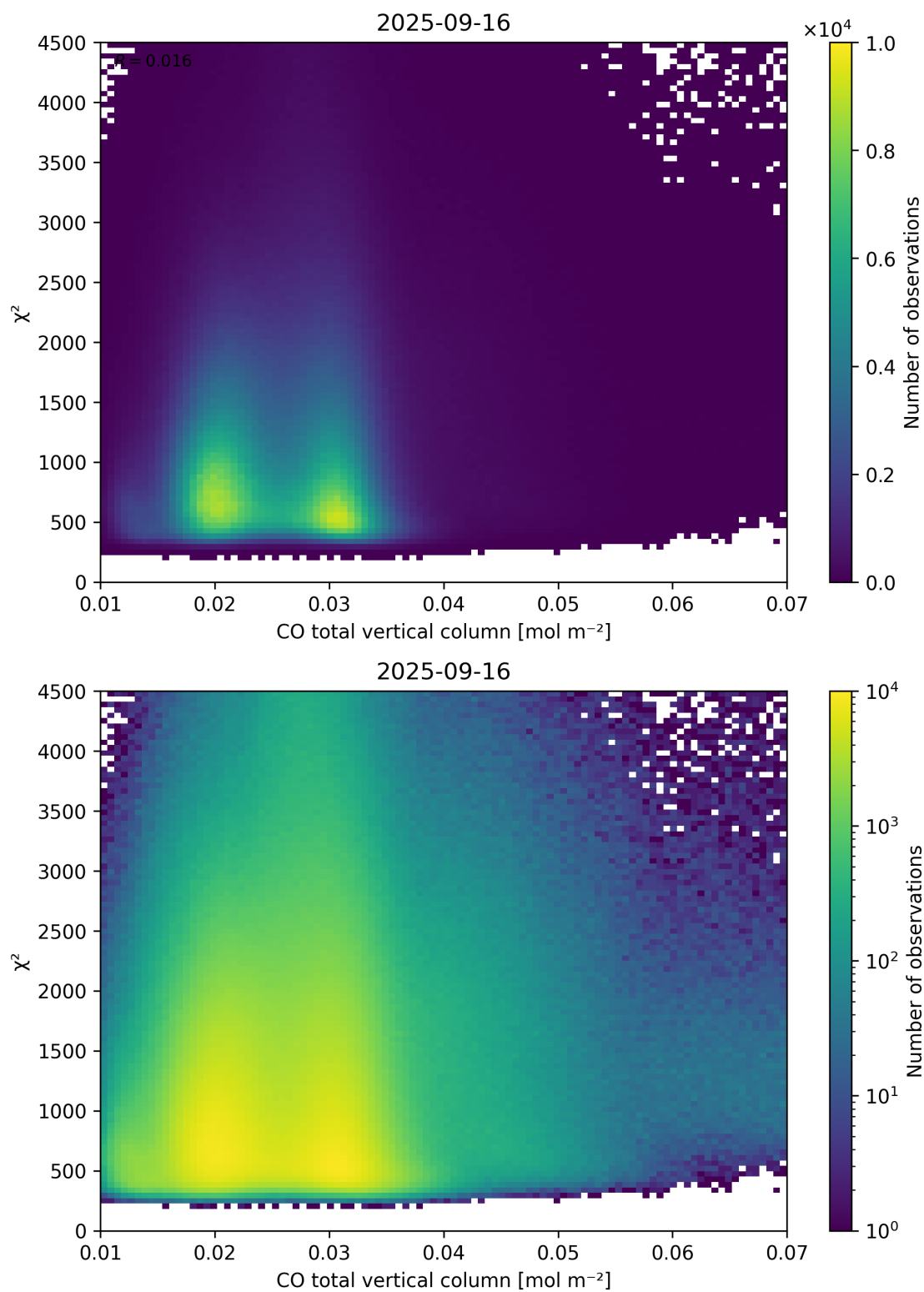
Figure 35: Scatter density plot of “CO total vertical column” against “ \chi^2 ” for 2025-09-15 to 2025-09-17.
