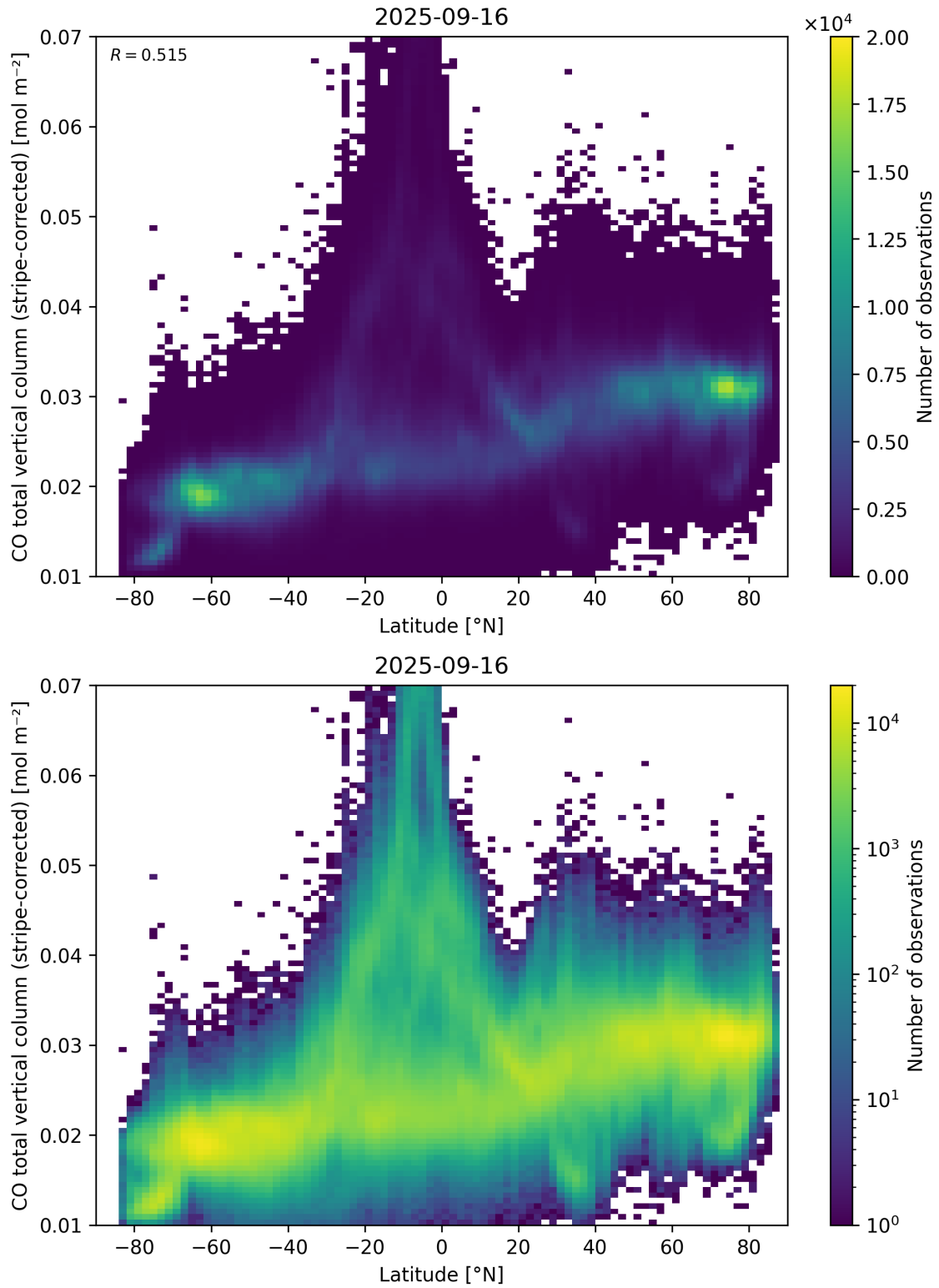
Figure 52: Scatter density plot of “Latitude” against “CO total vertical column (stripe-corrected)” for 2025-09-15 to 2025-09-17.
