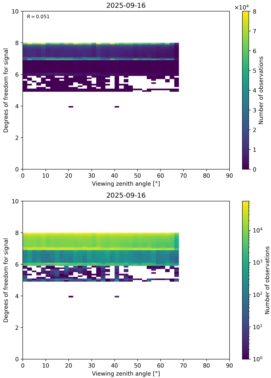
Figure 73: Scatter density plot of “Viewing zenith angle” against “Degrees of freedom for signal” for 2025-09-15 to 2025-09-17.
