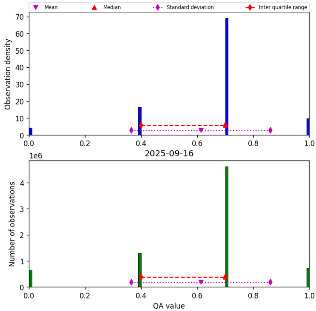
Figure 17: Histogram of “QA value” for 2025-09-15 to 2025-09-17
