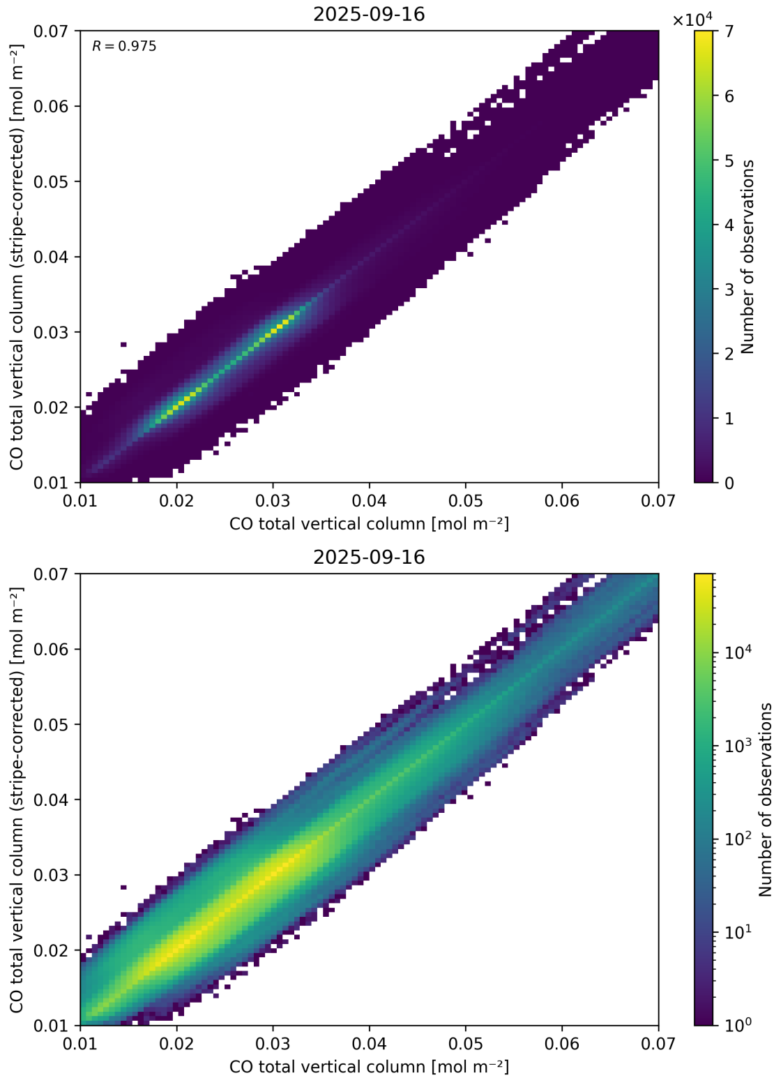
Figure 33: Scatter density plot of “CO total vertical column” against “CO total vertical column (stripe-corrected)” for 2025-09-15 to 2025-09-17.
