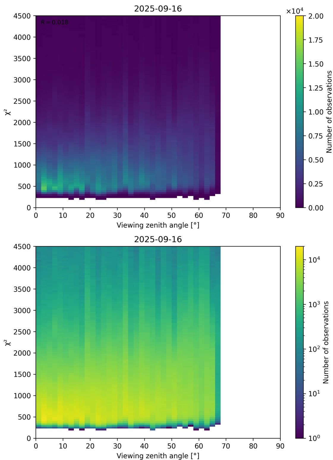
Figure 72: Scatter density plot of “Viewing zenith angle” against “ \chi^2 ” for 2025-09-15 to 2025-09-17.
