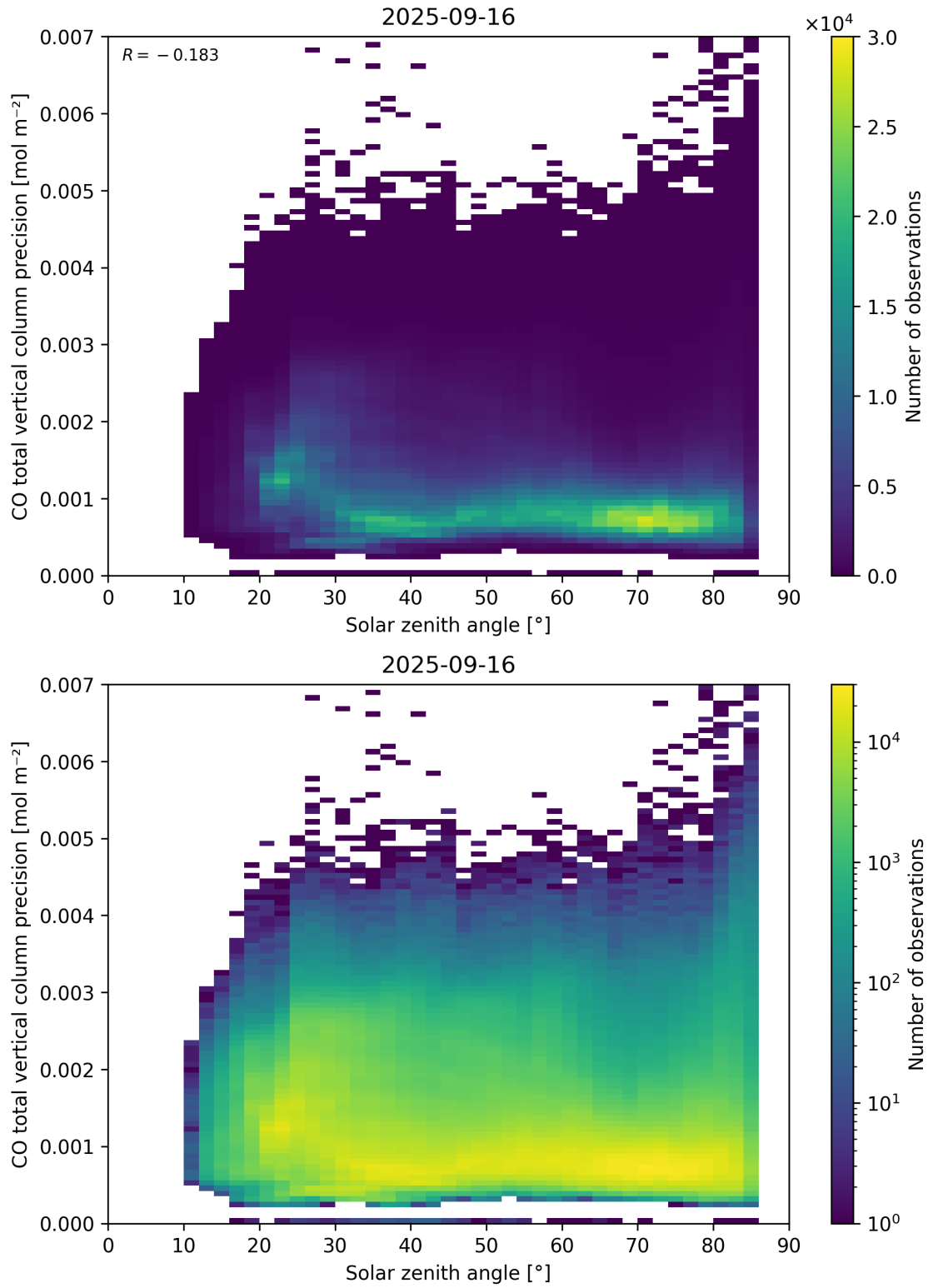
Figure 63: Scatter density plot of “Solar zenith angle” against “CO total vertical column precision” for 2025-09-15 to 2025-09-17.
