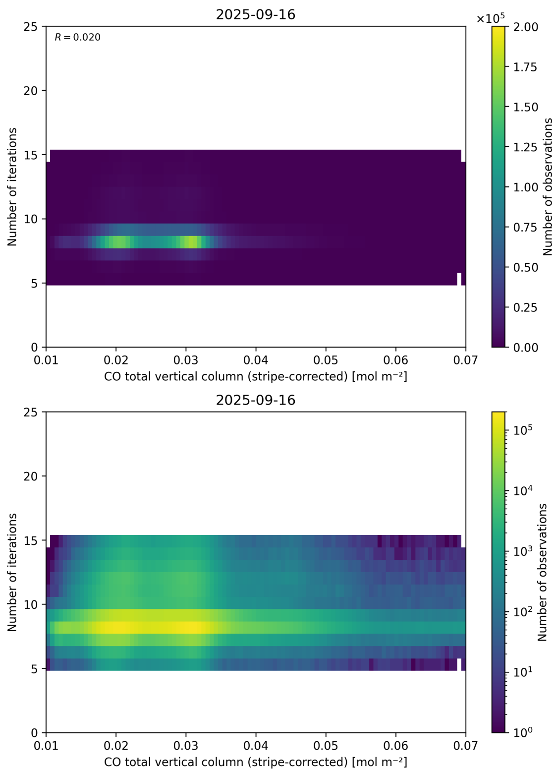
Figure 39: Scatter density plot of “CO total vertical column (stripe-corrected)” against “Number of iterations” for 2025-09-15 to 2025-09-17.
