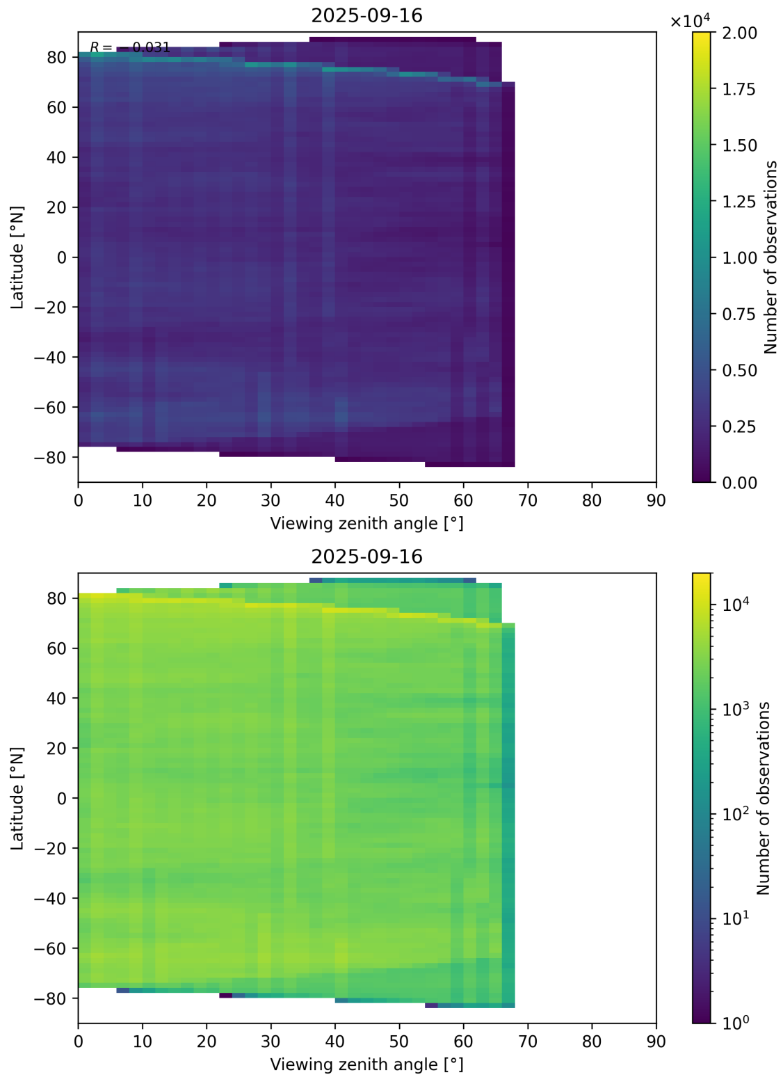
Figure 74: Scatter density plot of “Viewing zenith angle” against “Latitude” for 2025-09-15 to 2025-09-17.
