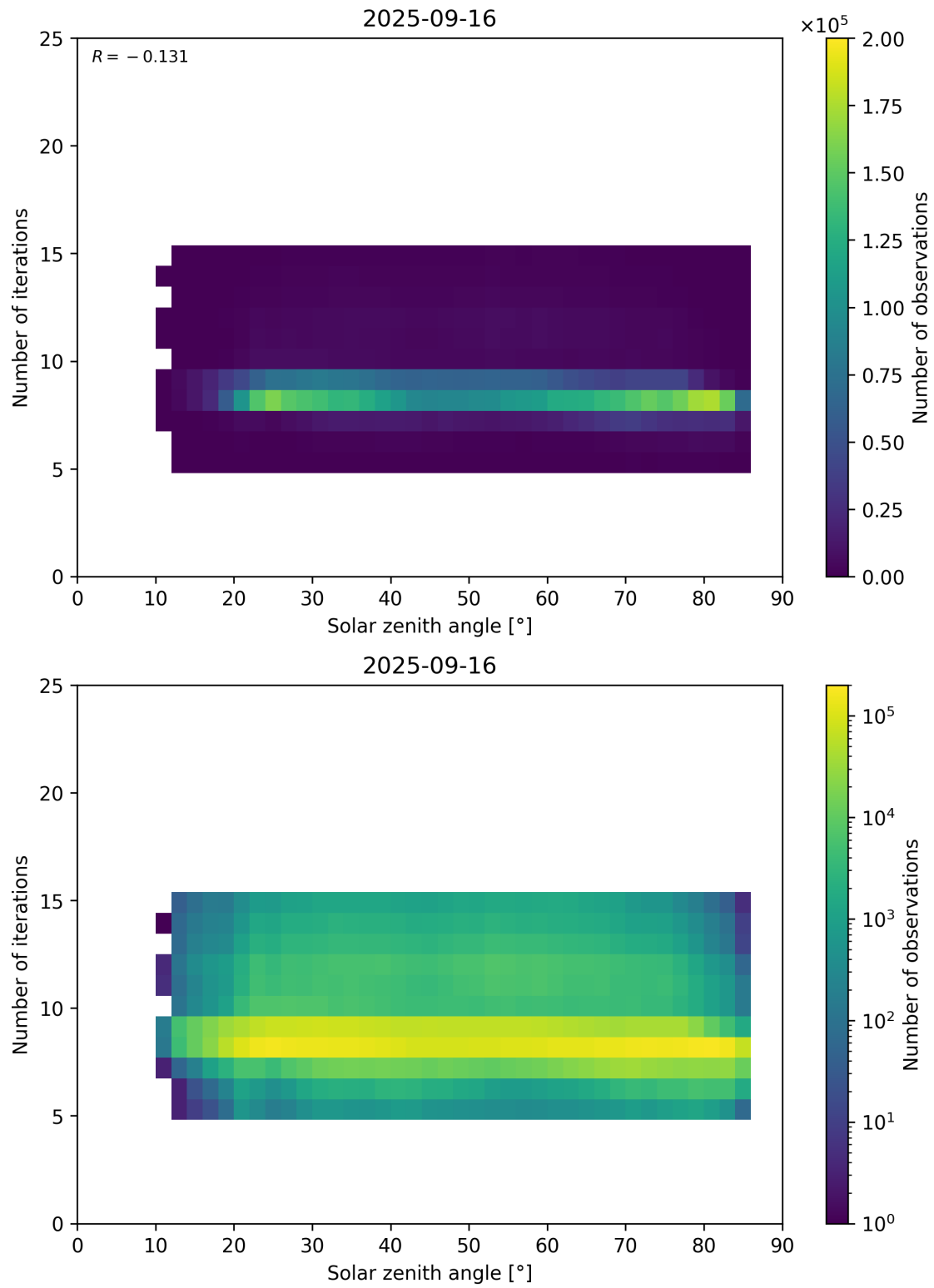
Figure 67: Scatter density plot of “Solar zenith angle” against “Number of iterations” for 2025-09-15 to 2025-09-17.
