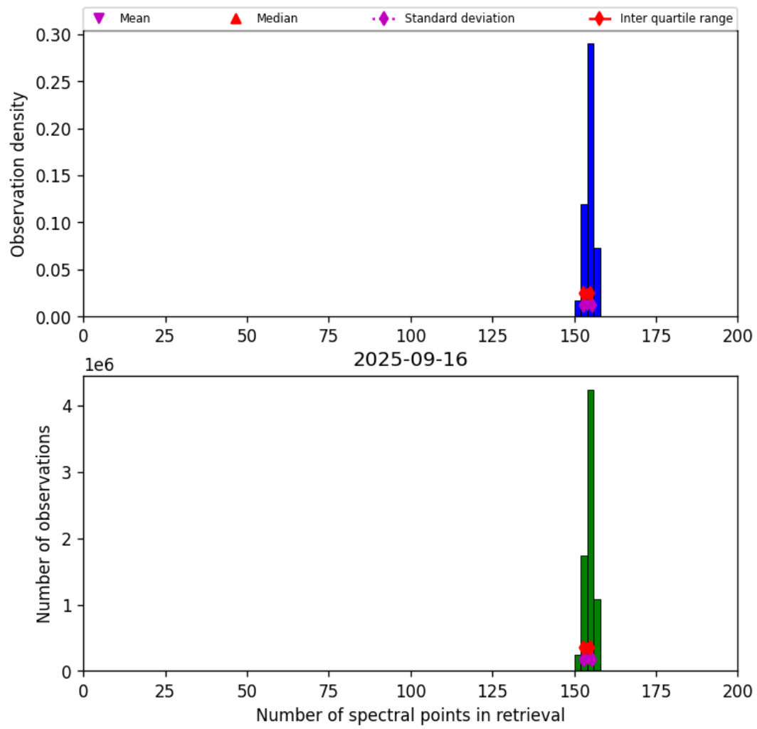
Figure 21: Histogram of “Number of spectral points in retrieval” for 2025-09-15 to 2025-09-17
