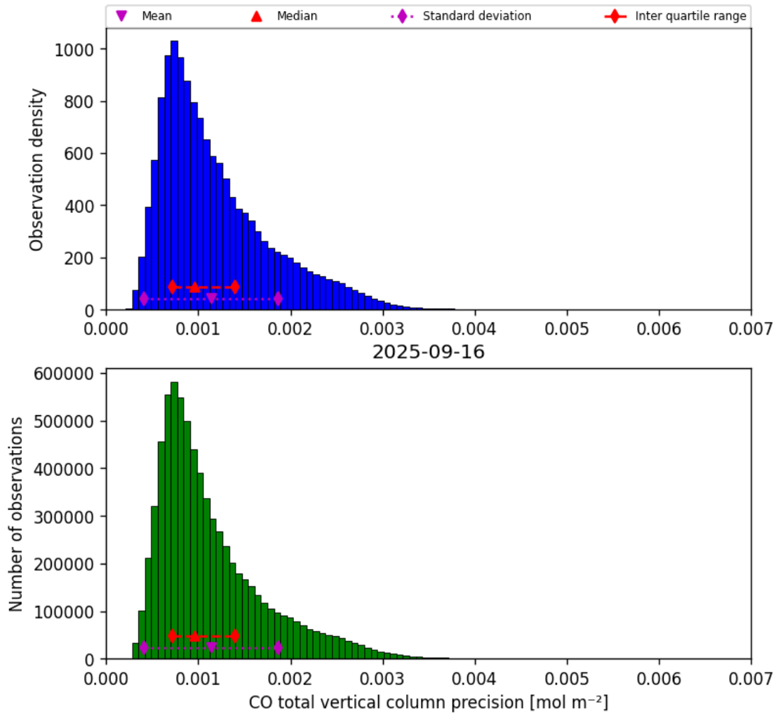
Figure 20: Histogram of “CO total vertical column precision” for 2025-09-15 to 2025-09-17
