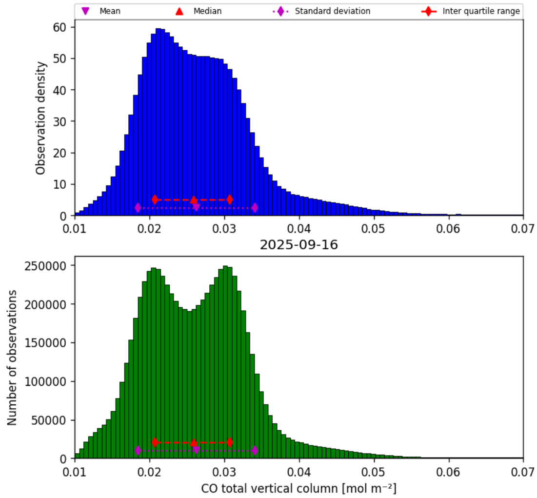
Figure 18: Histogram of “CO total vertical column” for 2025-09-15 to 2025-09-17
