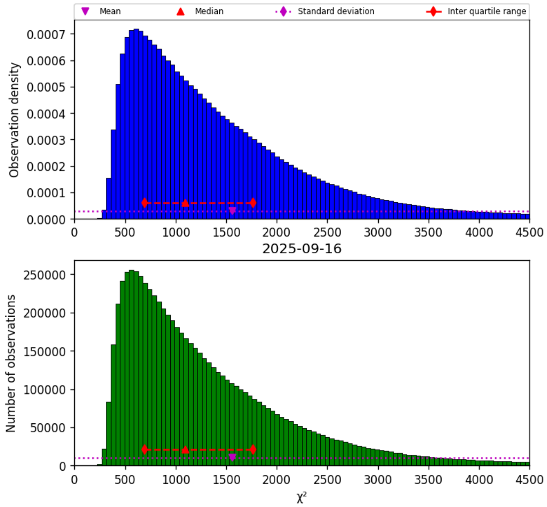
Figure 22: Histogram of “ \chi^2 ” for 2025-09-15 to 2025-09-17
