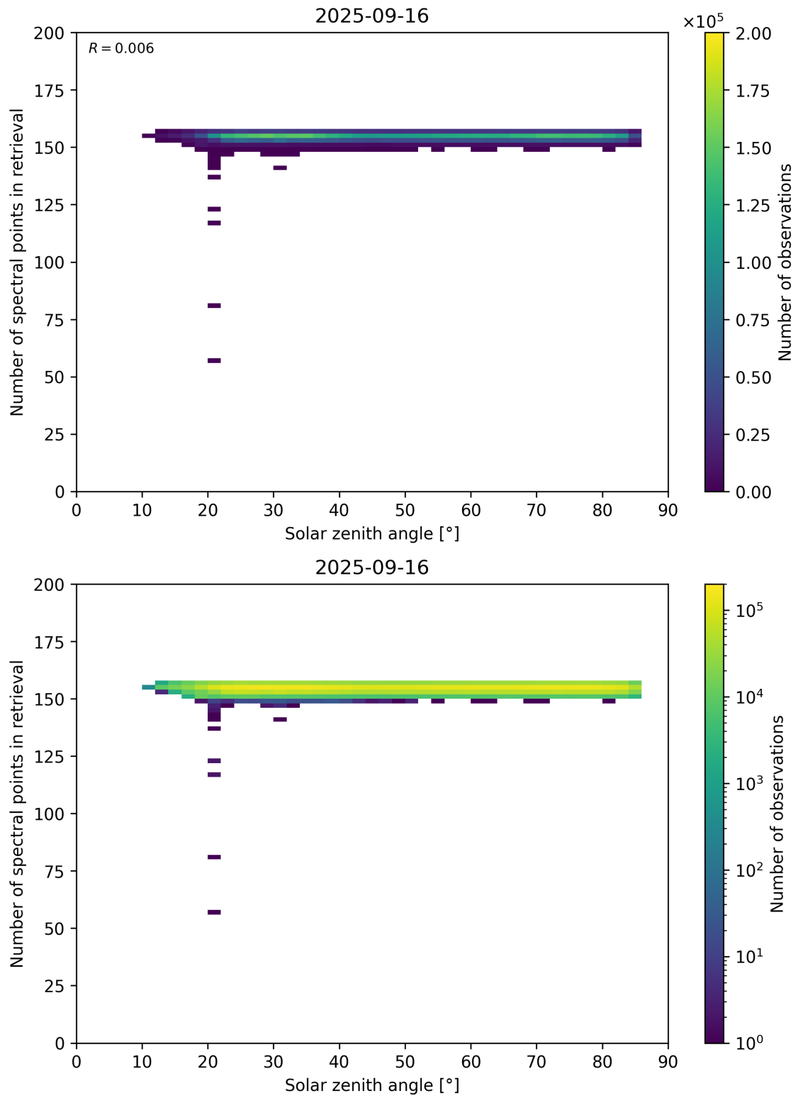
Figure 68: Scatter density plot of “Solar zenith angle” against “Number of spectral points in retrieval” for 2025-09-15 to 2025-09-17.
