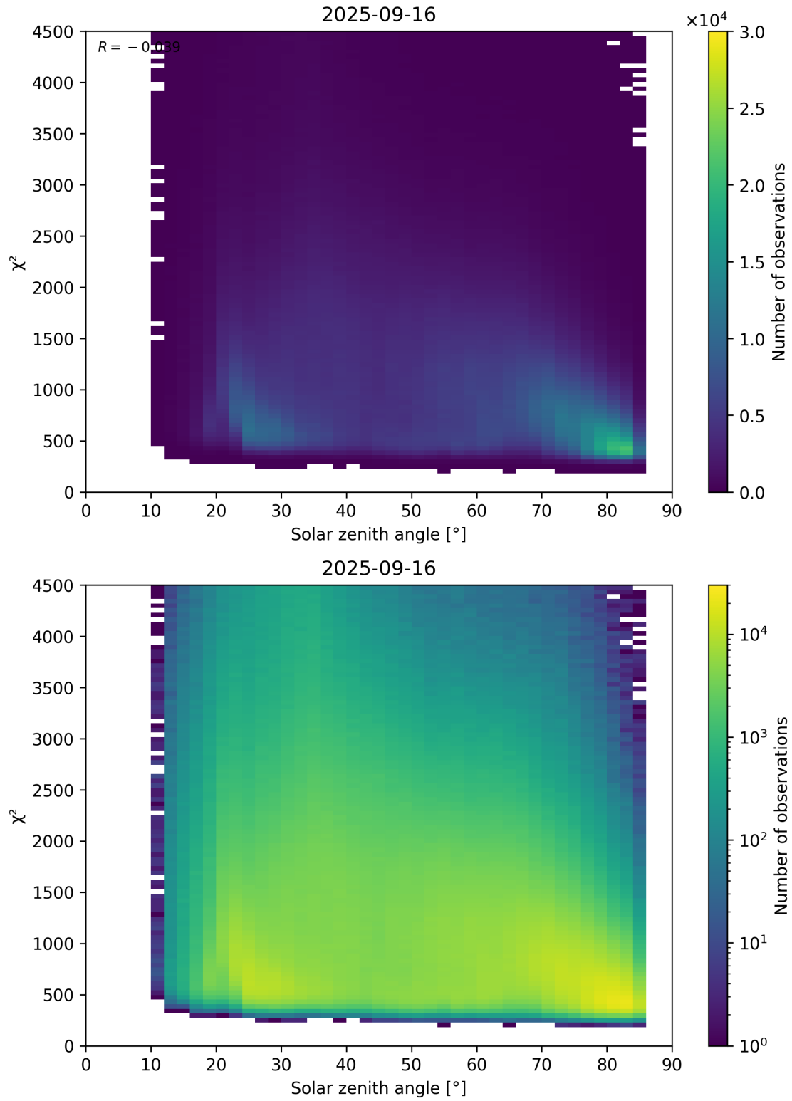
Figure 64: Scatter density plot of “Solar zenith angle” against “ \chi^2 ” for 2025-09-15 to 2025-09-17.
