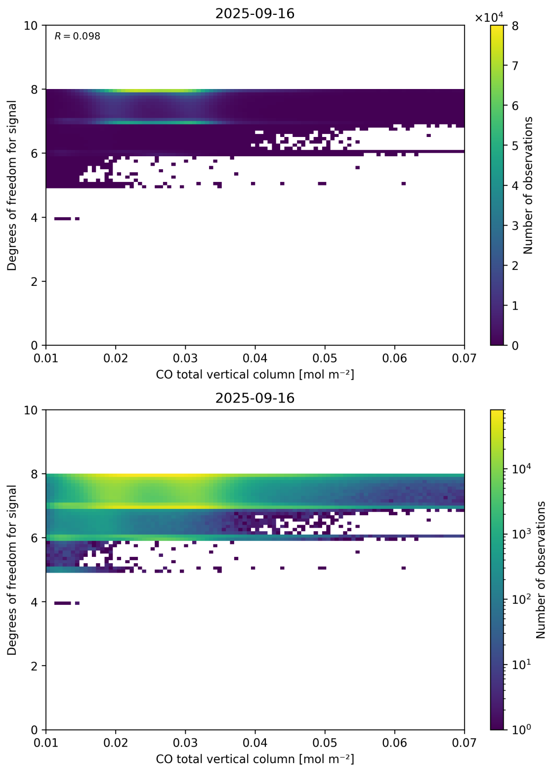
Figure 41: Scatter density plot of “CO total vertical column” against “Degrees of freedom for signal” for 2025-09-15 to 2025-09-17.
