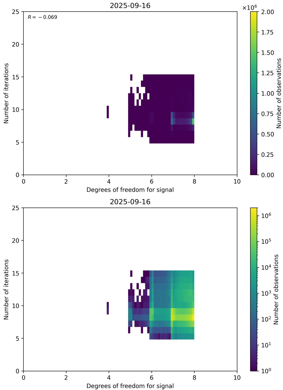
Figure 50: Scatter density plot of “Degrees of freedom for signal” against “Number of iterations” for 2025-09-15 to 2025-09-17.
