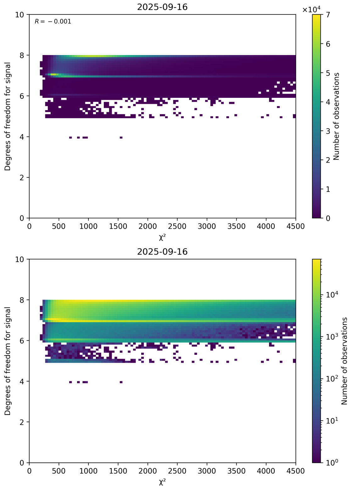
Figure 48: Scatter density plot of “ \chi^2 ” against “Degrees of freedom for signal” for 2025-09-15 to 2025-09-17.
