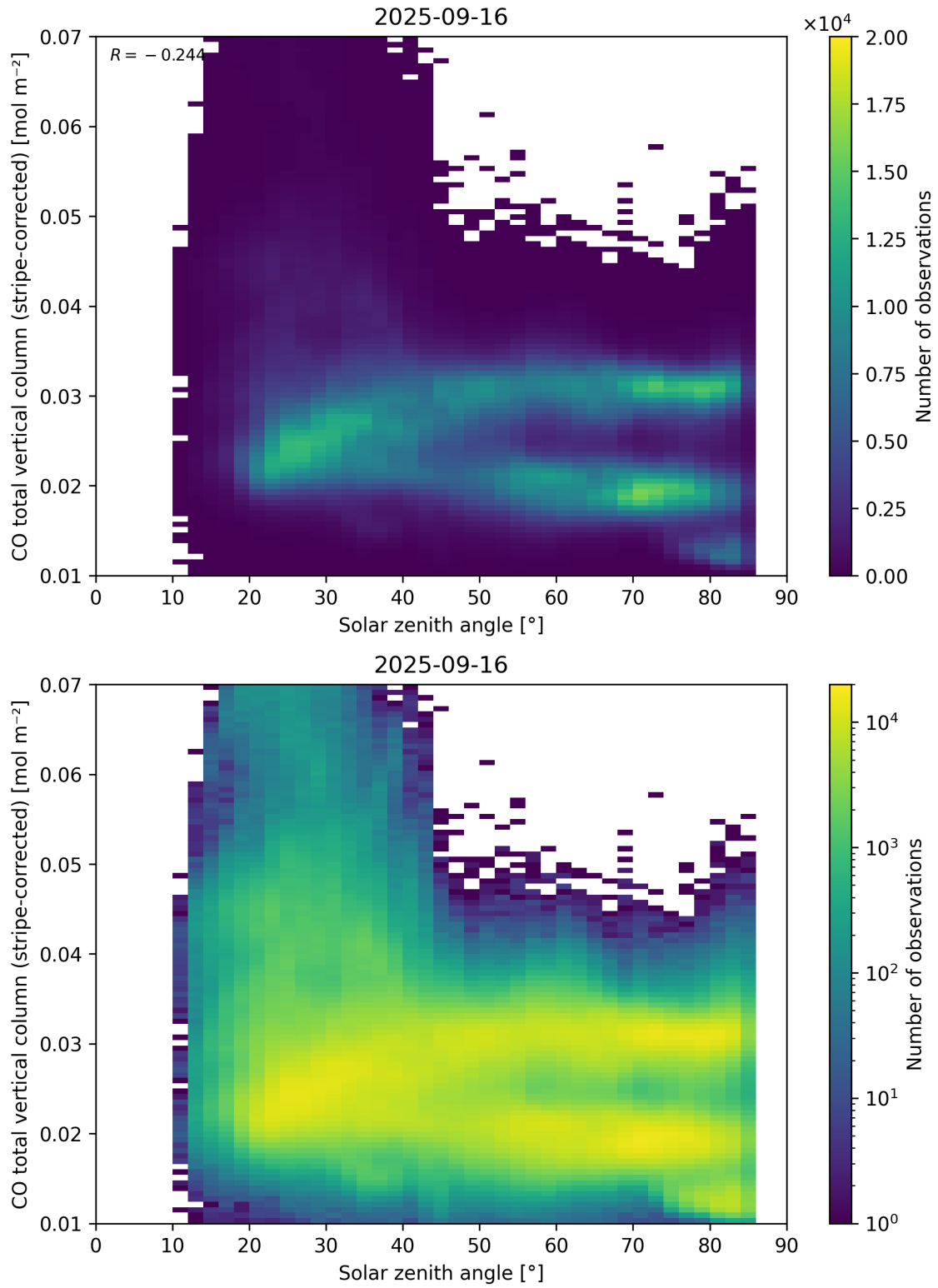
Figure 62: Scatter density plot of “Solar zenith angle” against “CO total vertical column (stripe-corrected)” for 2025-09-15 to 2025-09-17.
