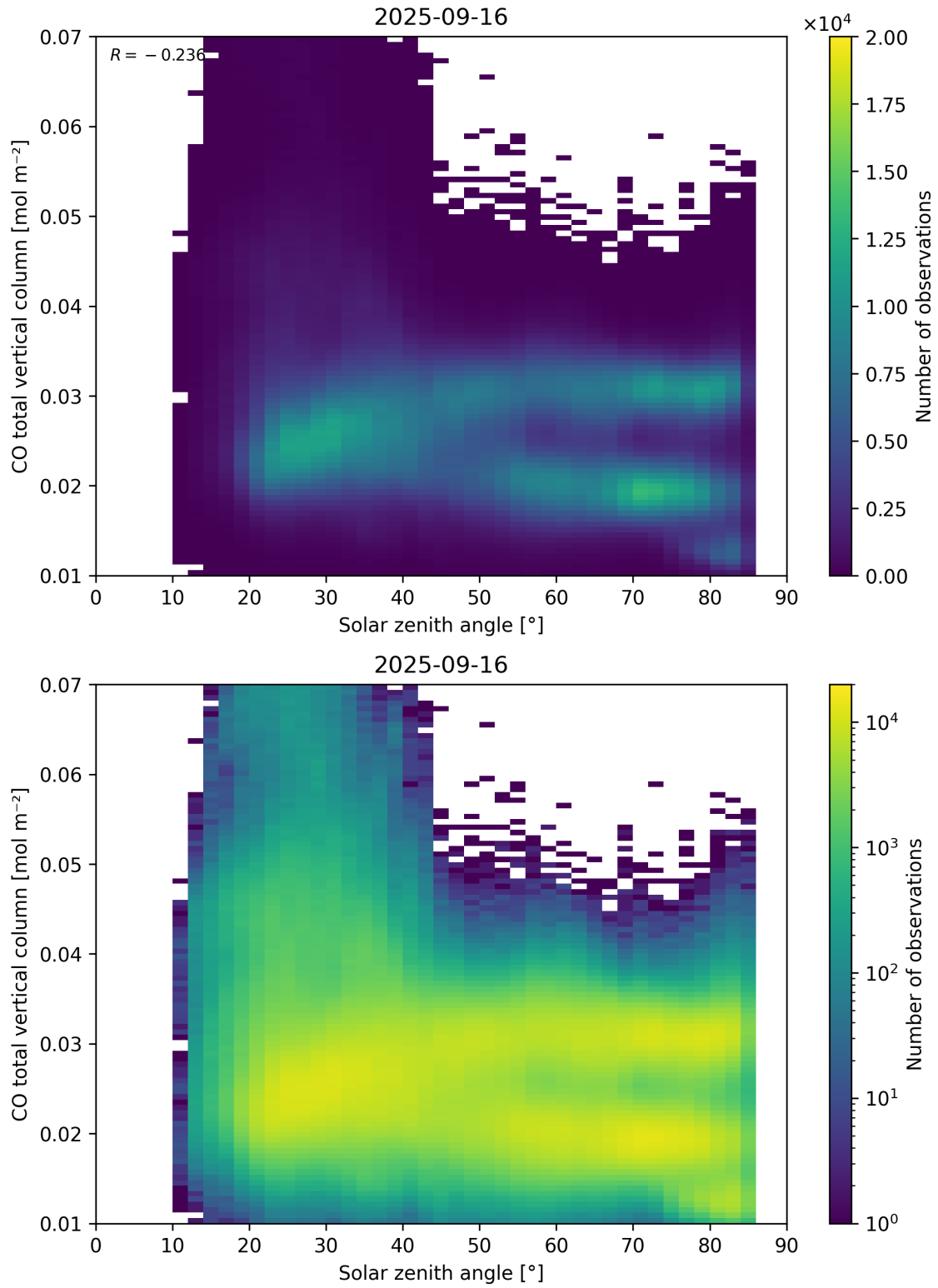
Figure 61: Scatter density plot of “Solar zenith angle” against “CO total vertical column” for 2025-09-15 to 2025-09-17.
