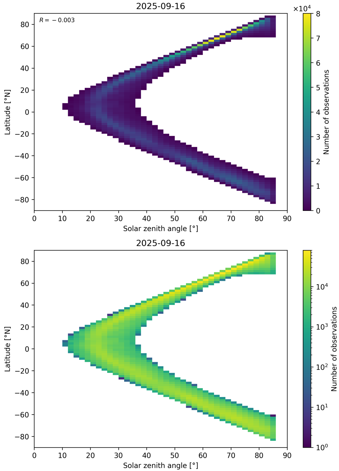
Figure 66: Scatter density plot of “Solar zenith angle” against “Latitude” for 2025-09-15 to 2025-09-17.
