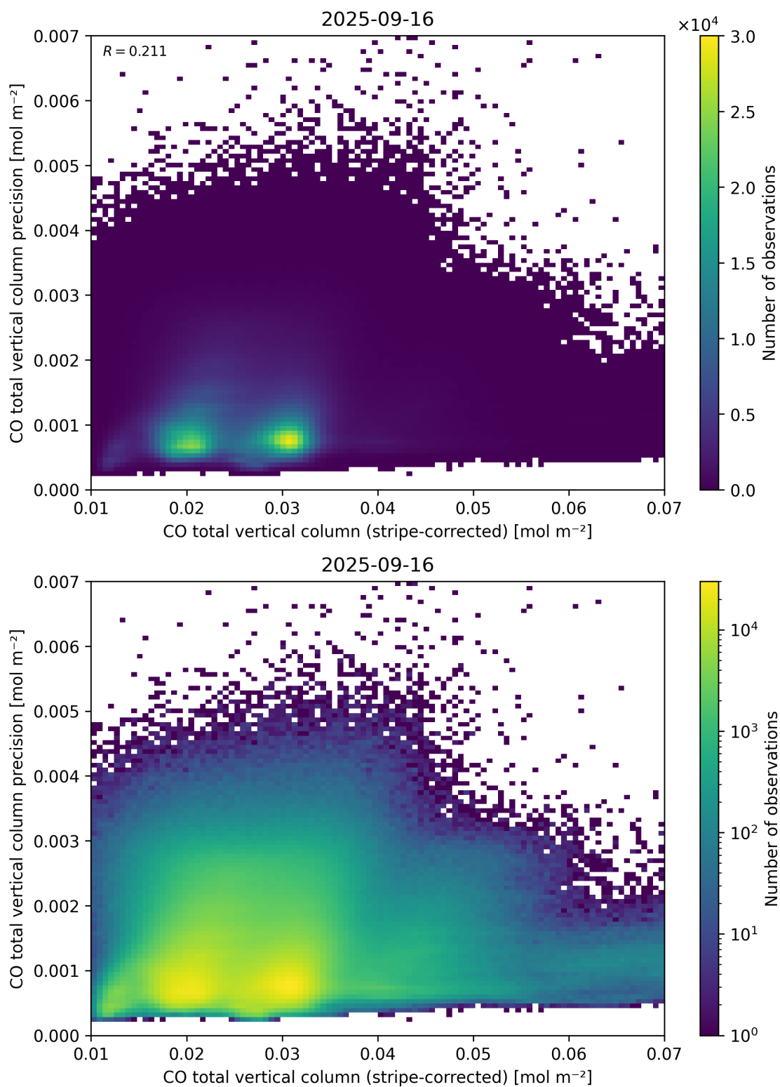
Figure 36: Scatter density plot of “CO total vertical column (stripe-corrected)” against “CO total vertical column precision” for 2025-09-15 to 2025-09-17.
