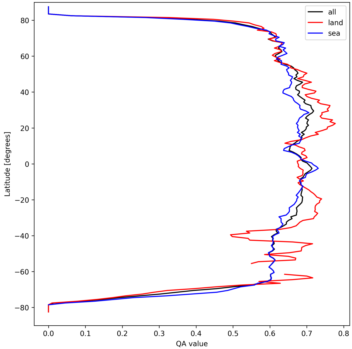
Figure 9: Zonal average of “QA value” for 2025-09-15 to 2025-09-17.
