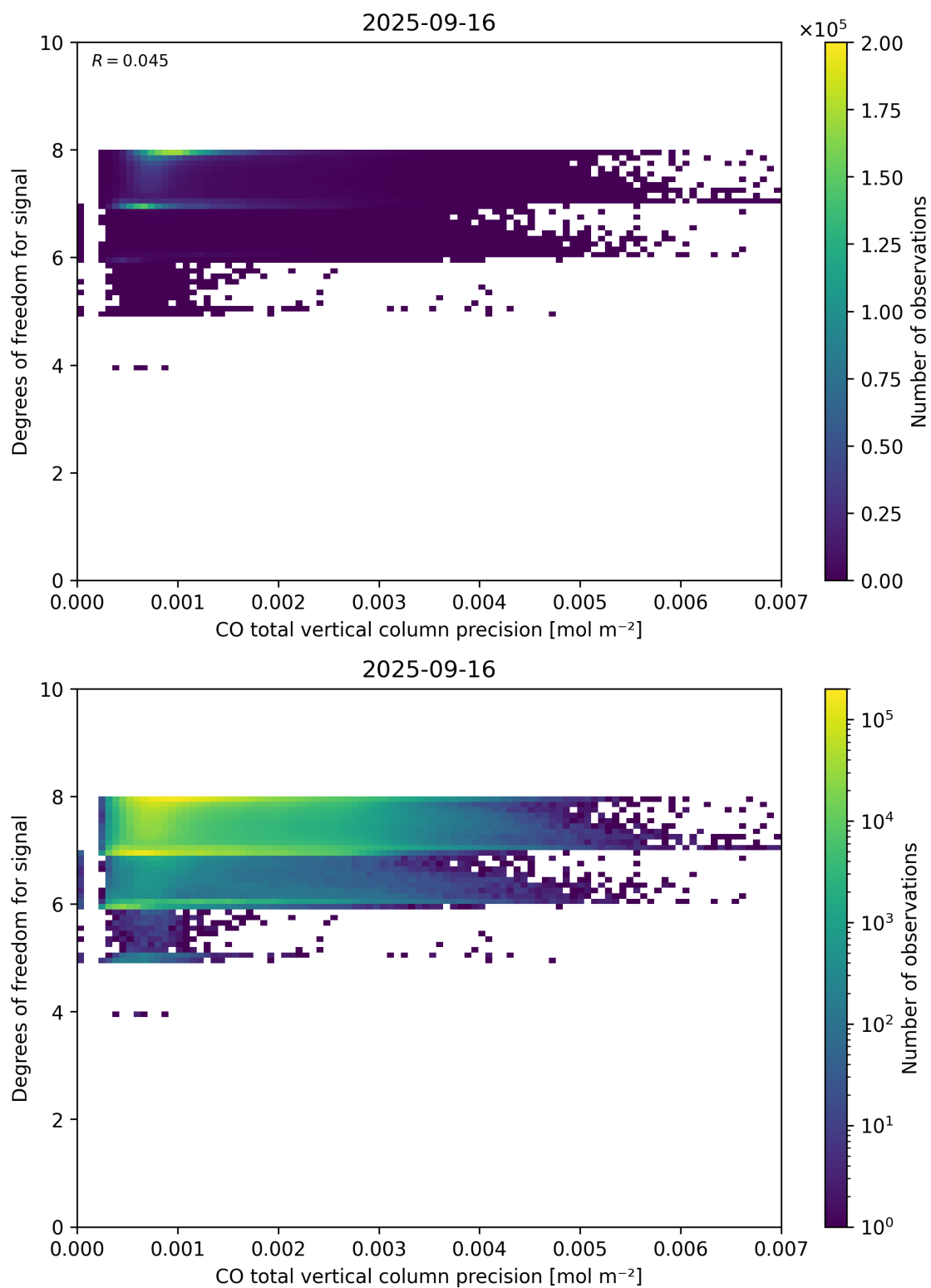
Figure 45: Scatter density plot of “CO total vertical column precision” against “Degrees of freedom for signal” for 2025-09-15 to 2025-09-17.
