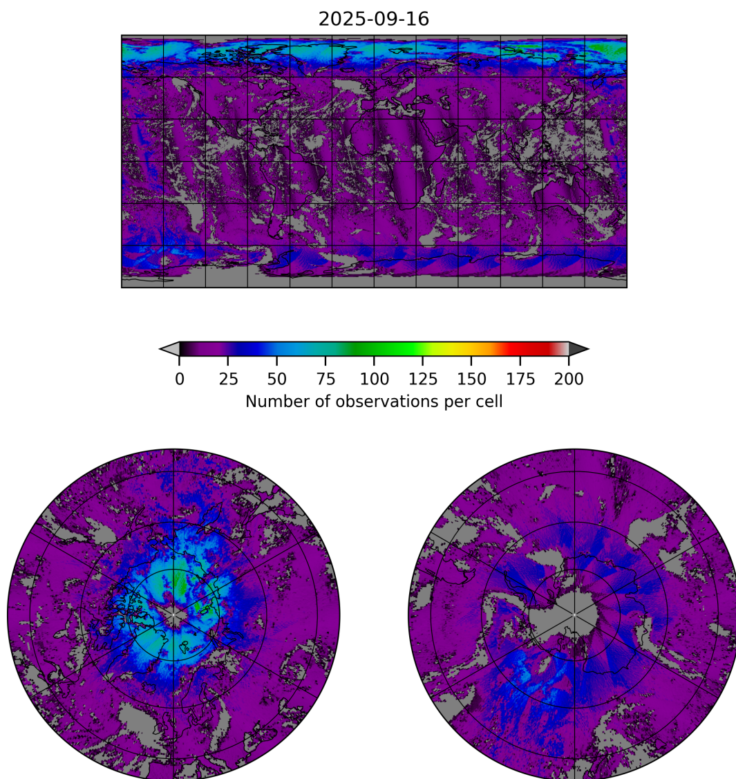
Figure 8: Map of the number of observations for 2025-09-15 to 2025-09-17
