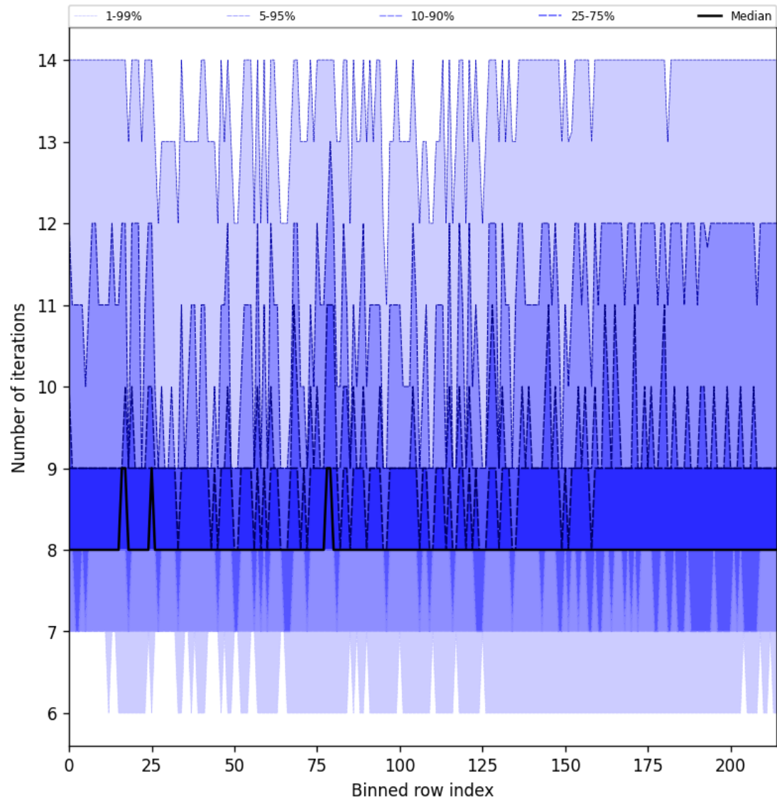
Figure 32: Along track statistics of “Number of iterations” for 2025-09-15 to 2025-09-17
