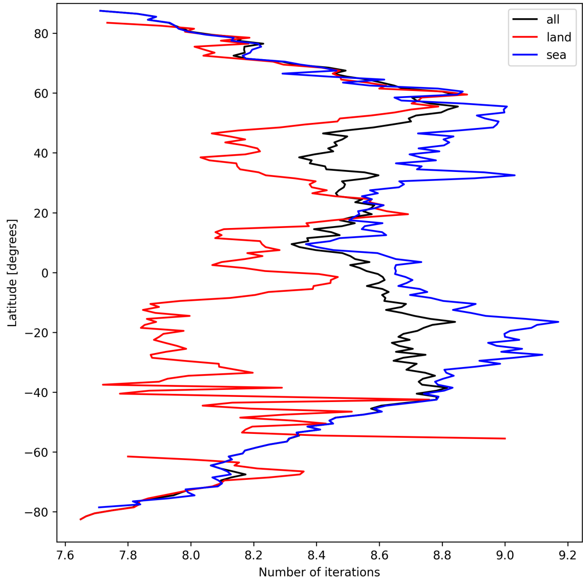
Figure 16: Zonal average of “Number of iterations” for 2025-09-15 to 2025-09-17.
