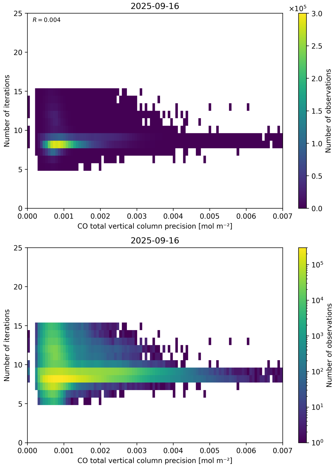
Figure 46: Scatter density plot of “CO total vertical column precision” against “Number of iterations” for 2025-09-15 to 2025-09-17.
