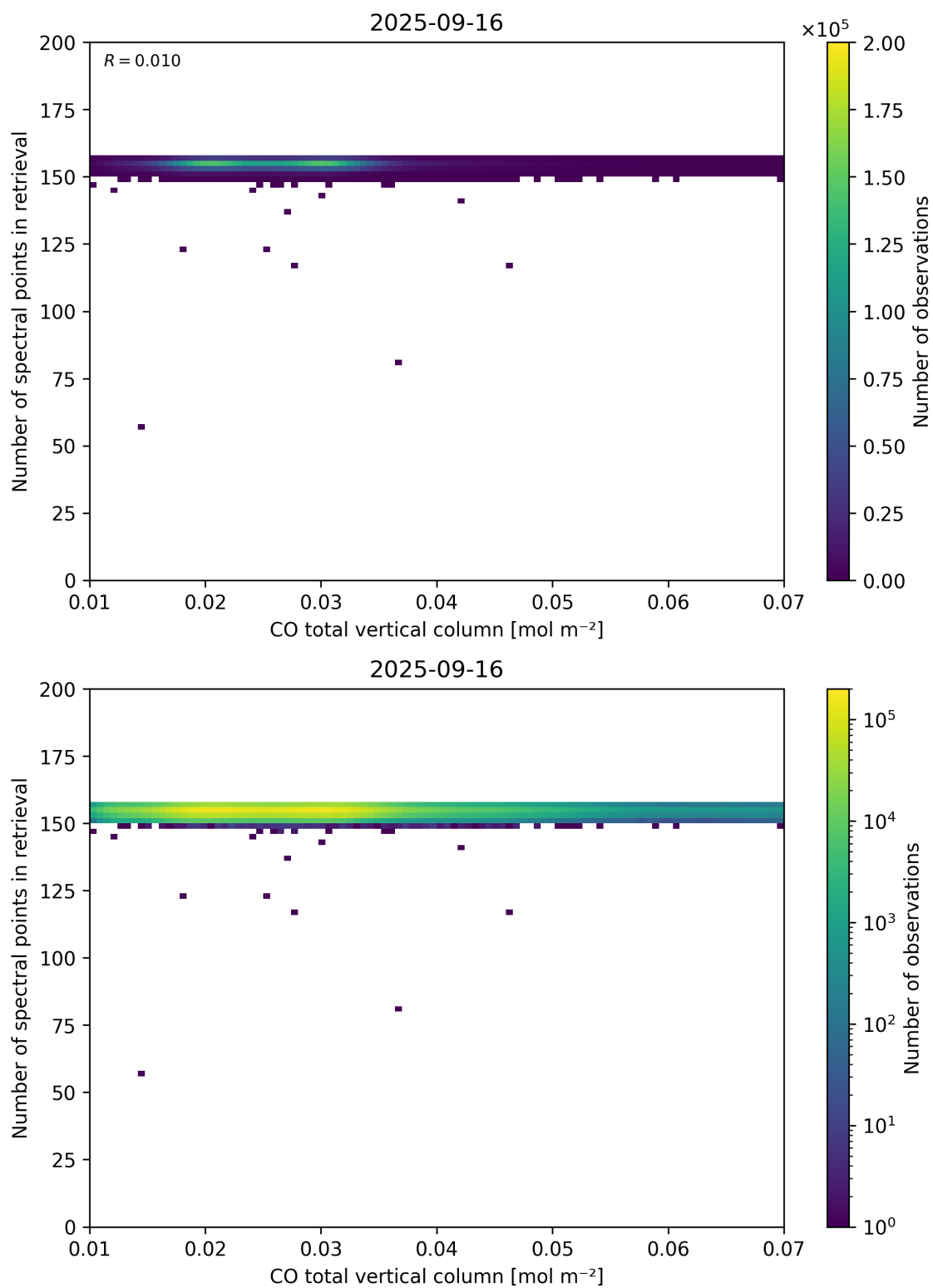
Figure 43: Scatter density plot of “CO total vertical column” against “Number of spectral points in retrieval” for 2025-09-15 to 2025-09-17.
