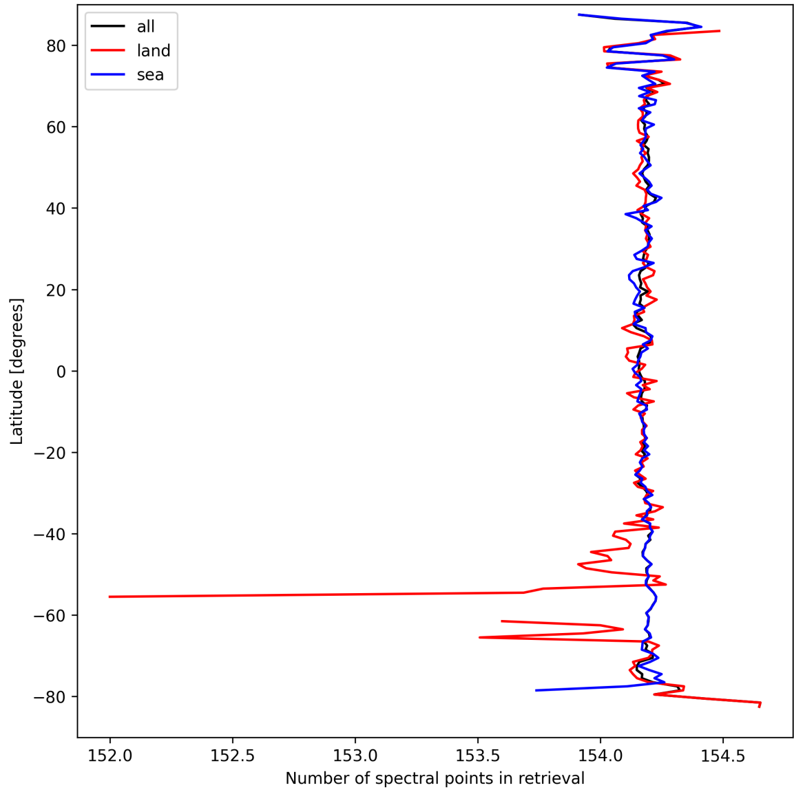
Figure 13: Zonal average of “Number of spectral points in retrieval” for 2025-09-15 to 2025-09-17.
