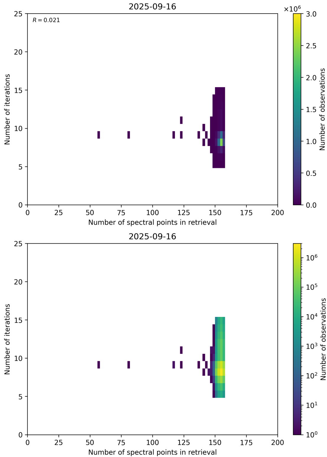
Figure 60: Scatter density plot of “Number of spectral points in retrieval” against “Number of iterations” for 2025-09-15 to 2025-09-17.
