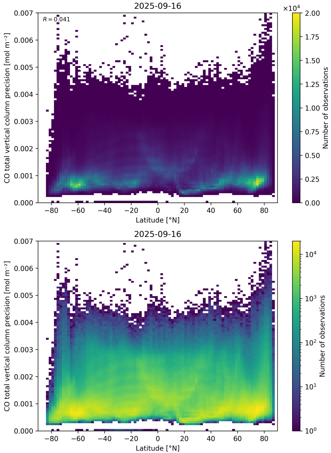
Figure 53: Scatter density plot of “Latitude” against “CO total vertical column precision” for 2025-09-15 to 2025-09-17.
