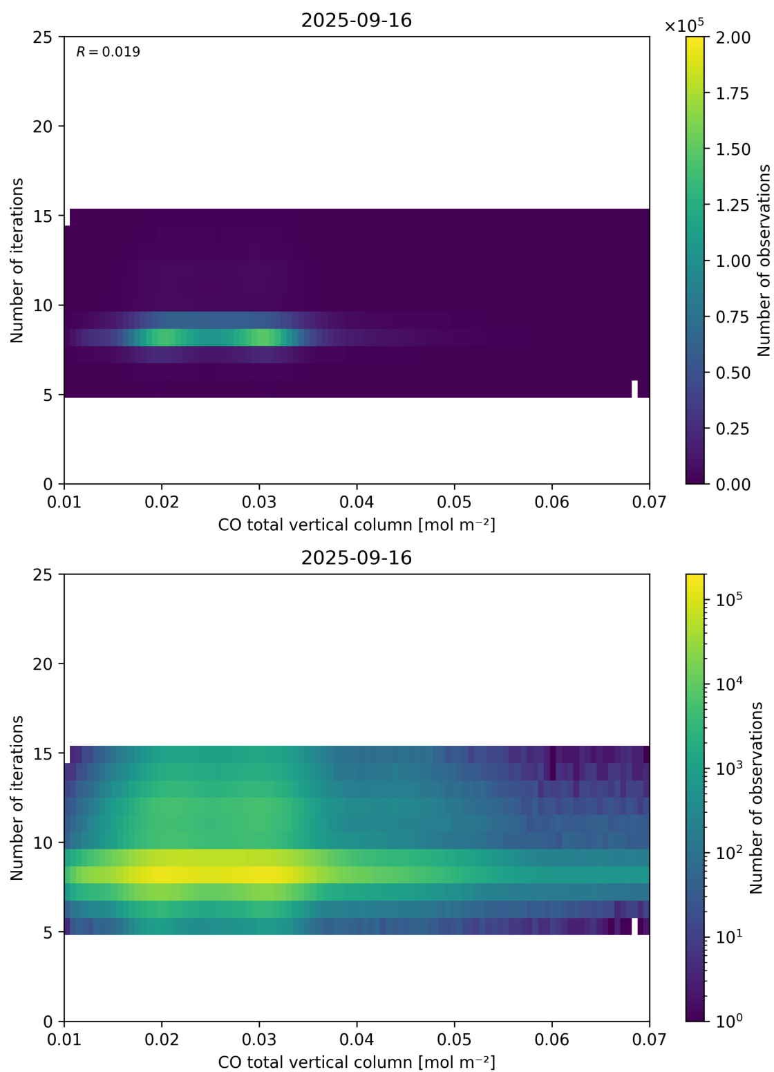
Figure 42: Scatter density plot of “CO total vertical column” against “Number of iterations” for 2025-09-15 to 2025-09-17.
