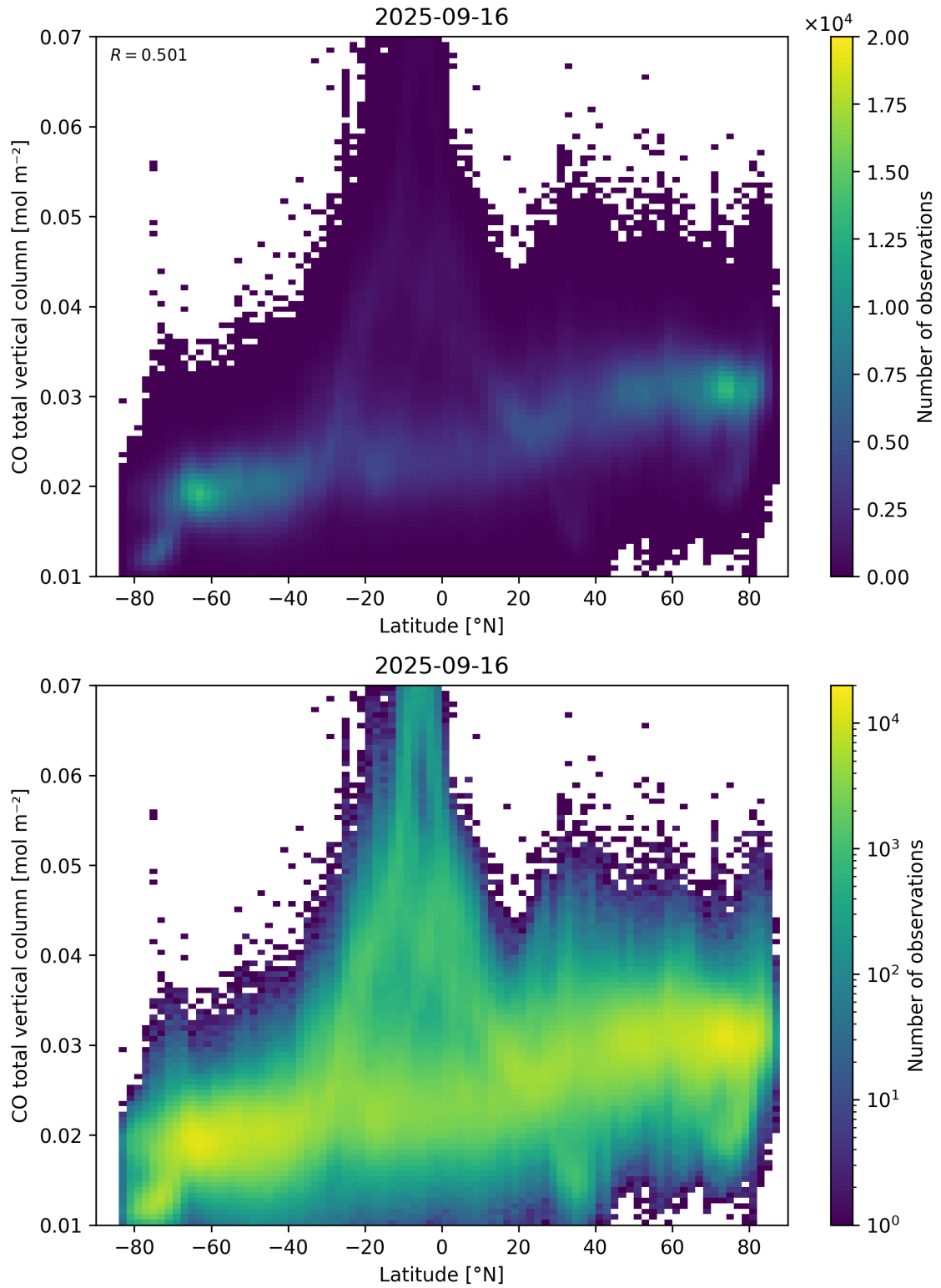
Figure 51: Scatter density plot of “Latitude” against “CO total vertical column” for 2025-09-15 to 2025-09-17.
