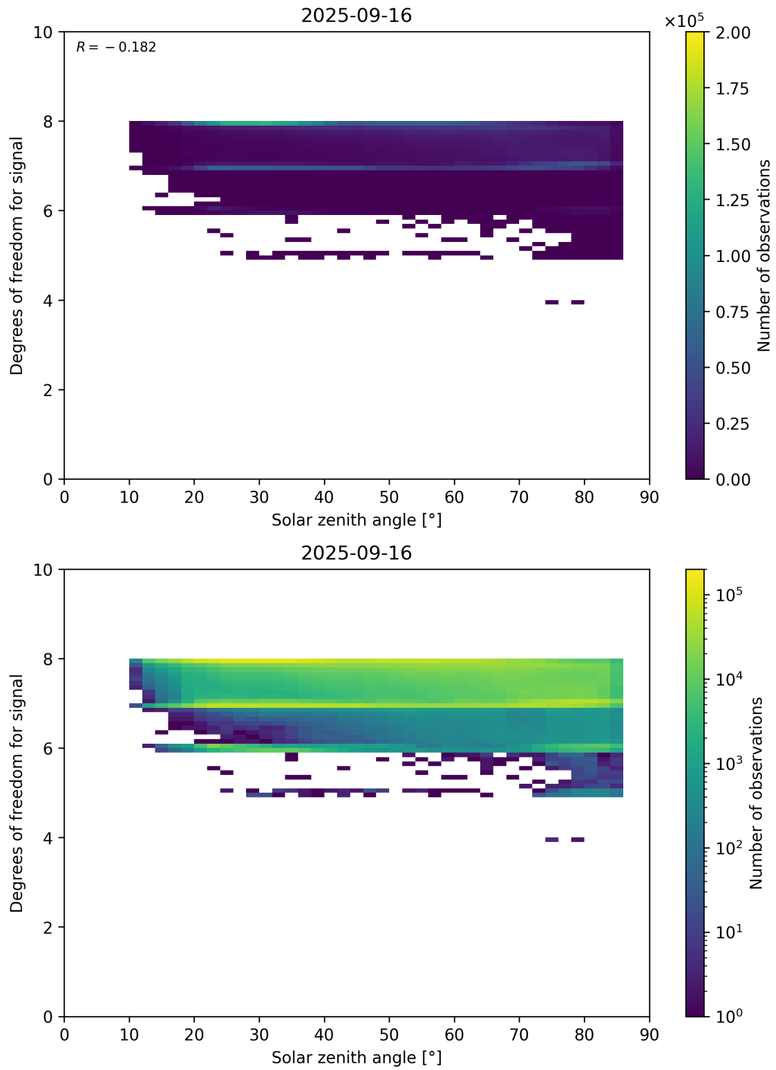
Figure 65: Scatter density plot of “Solar zenith angle” against “Degrees of freedom for signal” for 2025-09-15 to 2025-09-17.
