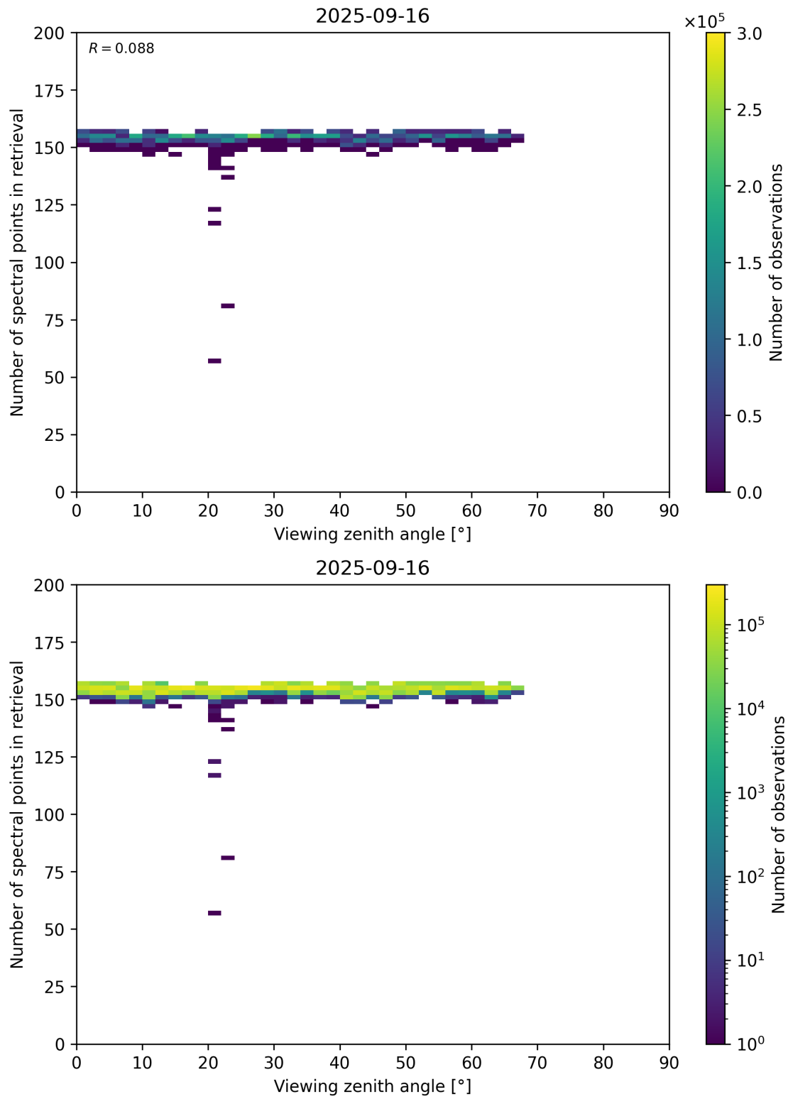
Figure 76: Scatter density plot of “Viewing zenith angle” against “Number of spectral points in retrieval” for 2025-09-15 to 2025-09-17.
