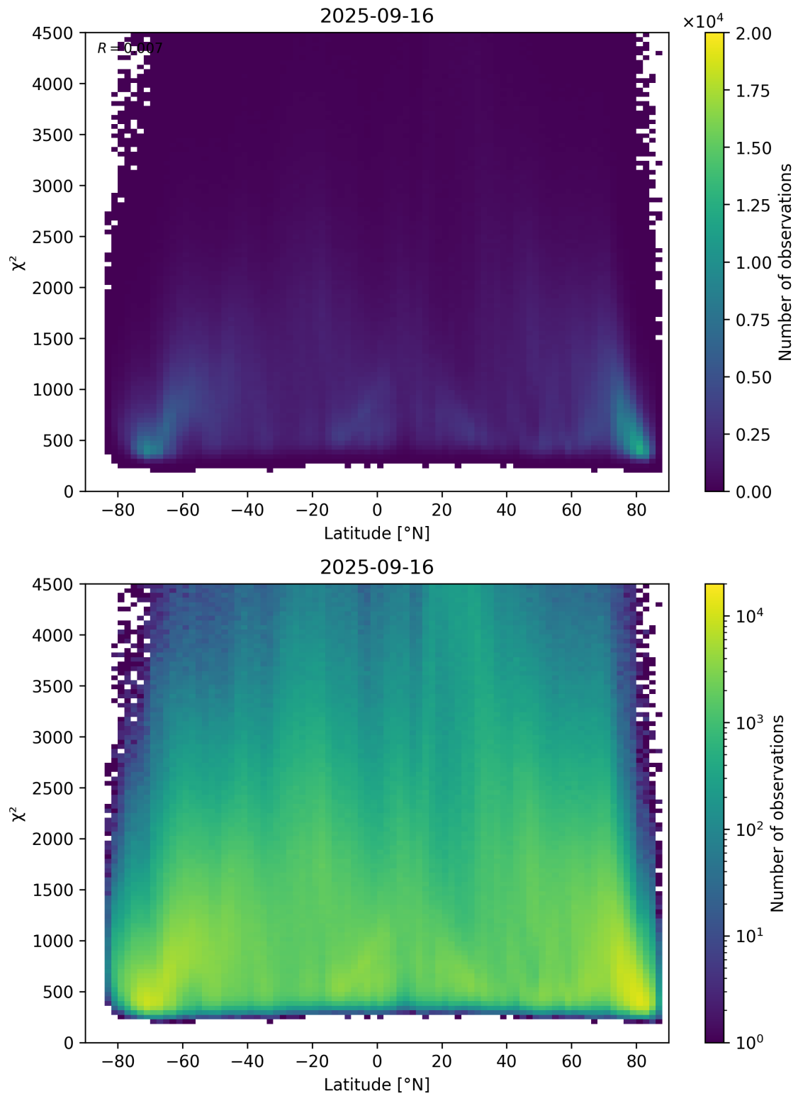
Figure 54: Scatter density plot of “Latitude” against “ \chi^2 ” for 2025-09-15 to 2025-09-17.
