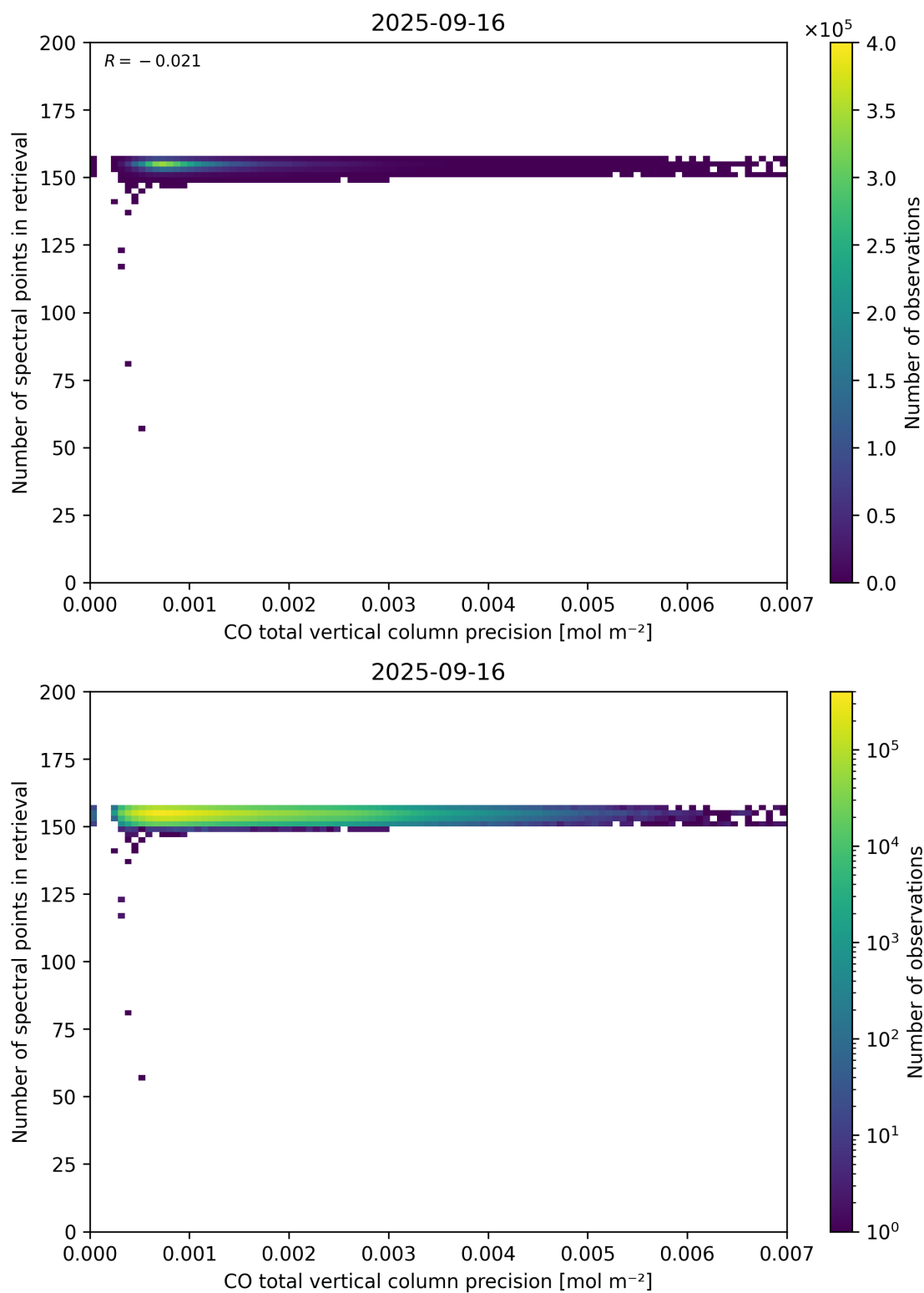
Figure 47: Scatter density plot of “CO total vertical column precision” against “Number of spectral points in retrieval” for 2025-09-15 to 2025-09-17.
