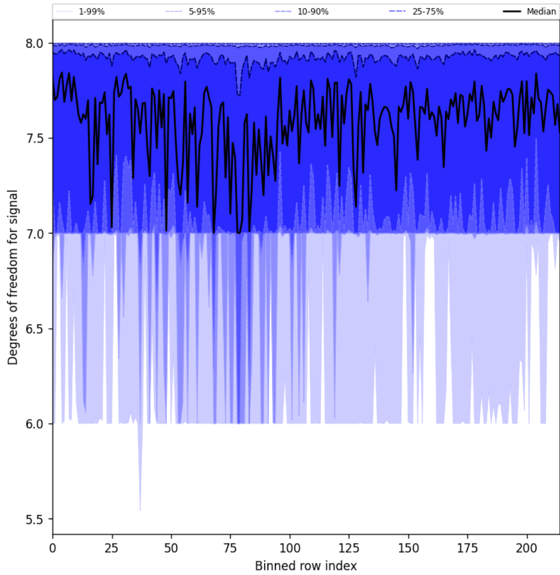
Figure 31: Along track statistics of “Degrees of freedom for signal” for 2025-09-15 to 2025-09-17
