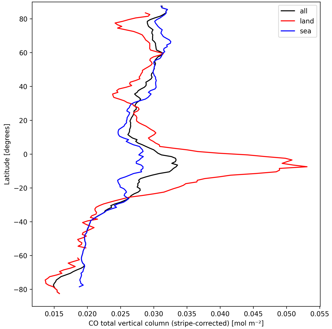
Figure 11: Zonal average of “CO total vertical column (stripe-corrected)” for 2025-09-15 to 2025-09-17.
