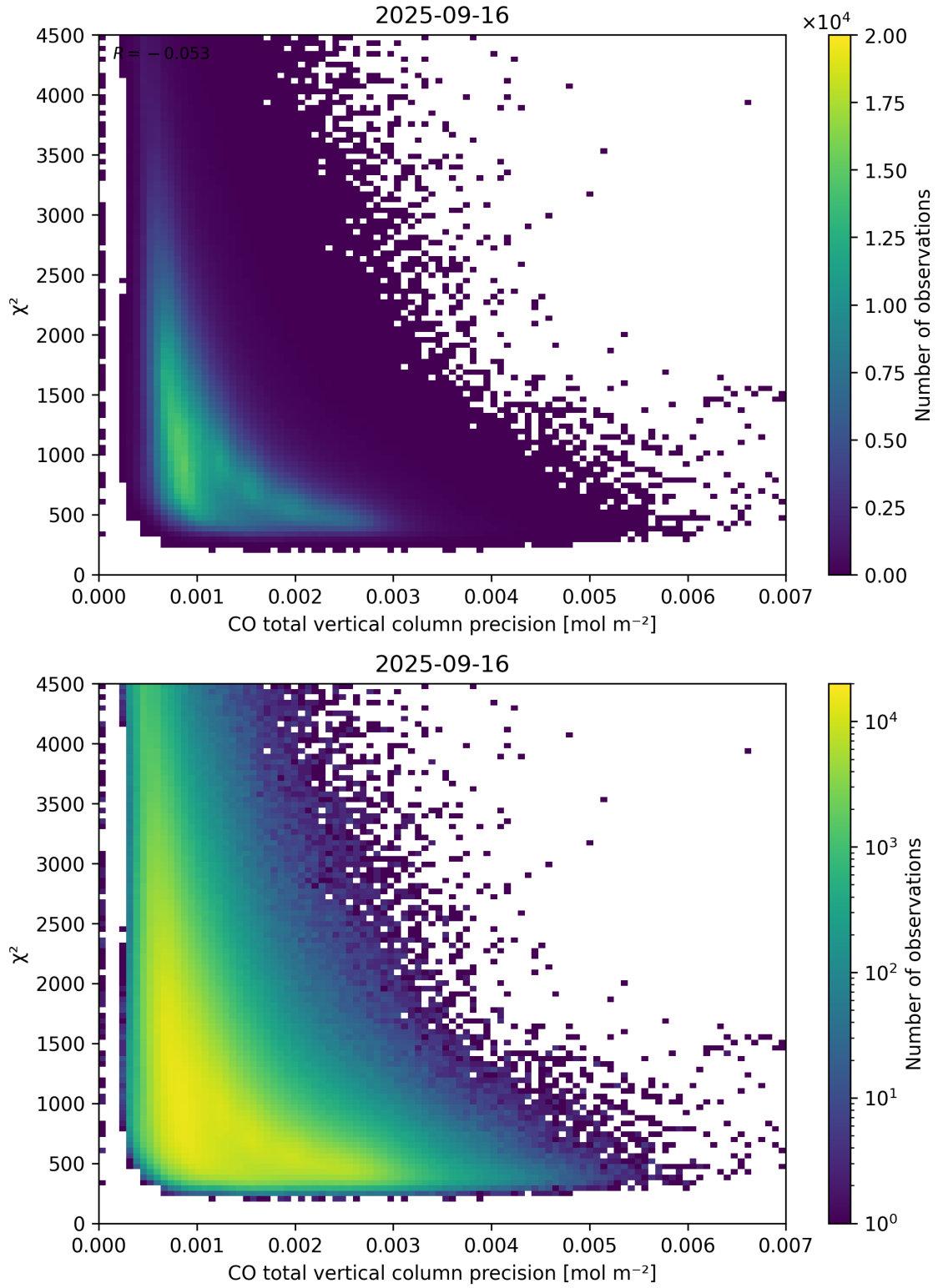
Figure 44: Scatter density plot of “CO total vertical column precision” against “ \chi^2 ” for 2025-09-15 to 2025-09-17.
