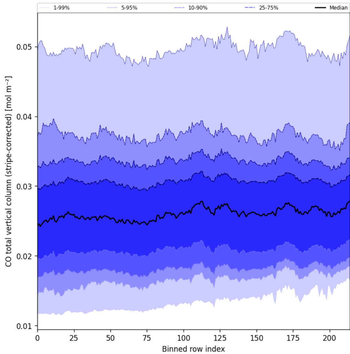
Figure 27: Along track statistics of “CO total vertical column (stripe-corrected)” for 2025-09-15 to 2025-09-17
