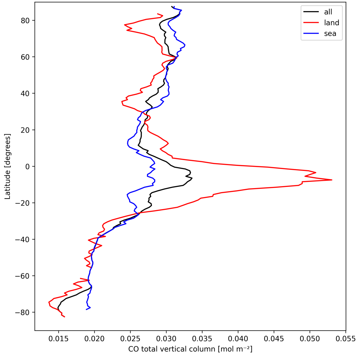
Figure 10: Zonal average of “CO total vertical column” for 2025-09-15 to 2025-09-17.
