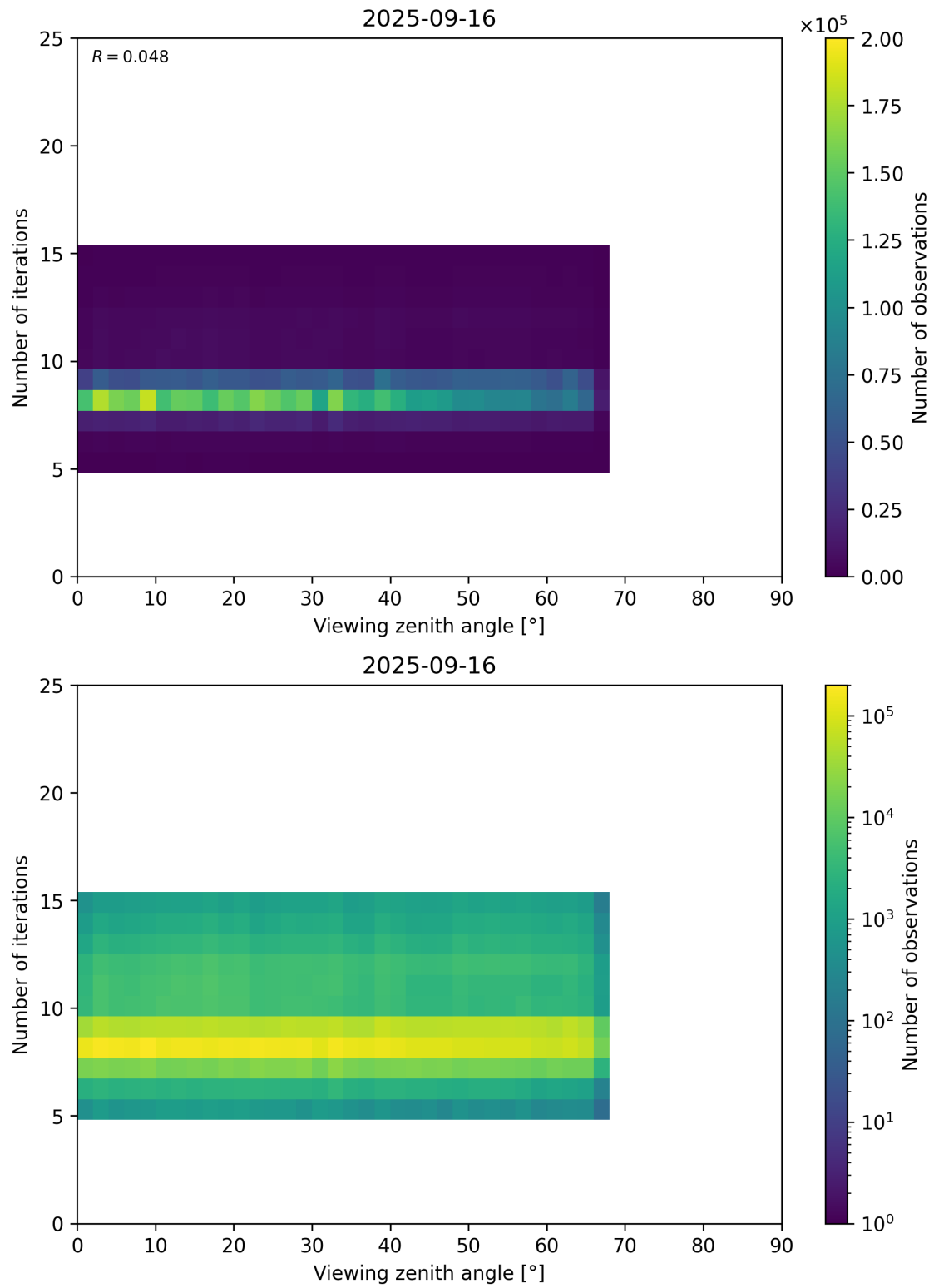
Figure 75: Scatter density plot of “Viewing zenith angle” against “Number of iterations” for 2025-09-15 to 2025-09-17.
