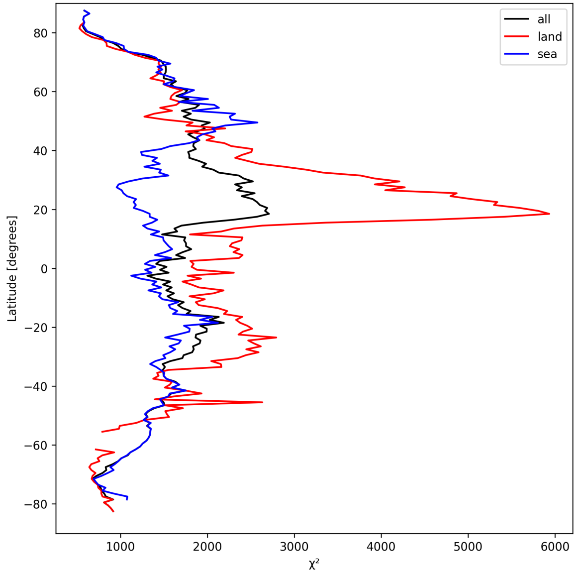
Figure 14: Zonal average of “ \chi^2 ” for 2025-09-15 to 2025-09-17.
