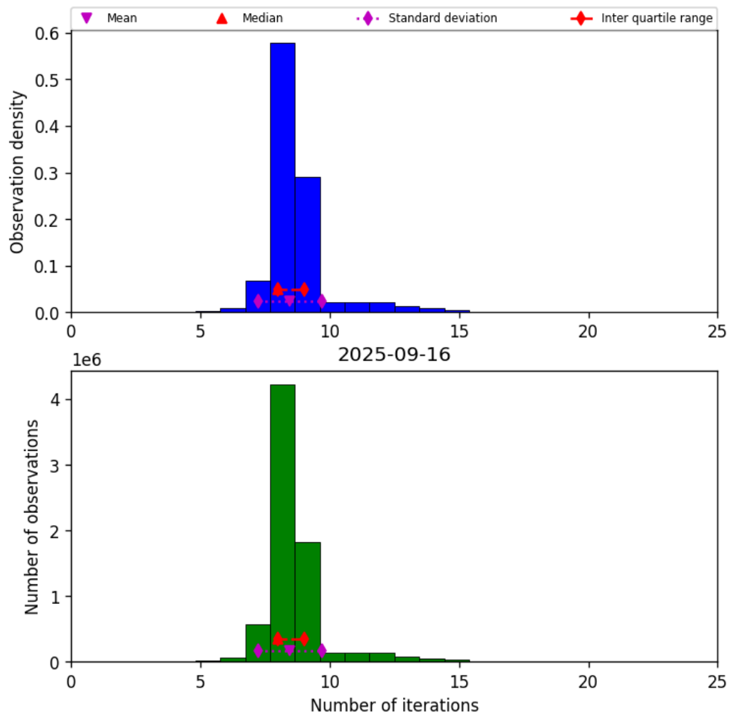
Figure 24: Histogram of “Number of iterations” for 2025-09-15 to 2025-09-17
