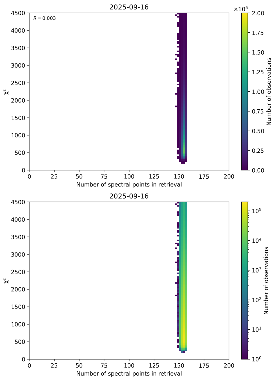
Figure 58: Scatter density plot of “Number of spectral points in retrieval” against “ \chi^2 ” for 2025-09-15 to 2025-09-17.
