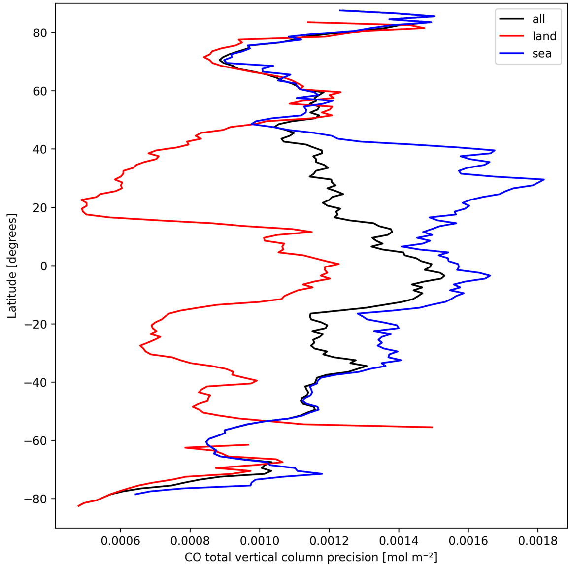
Figure 12: Zonal average of “CO total vertical column precision” for 2025-09-15 to 2025-09-17.
