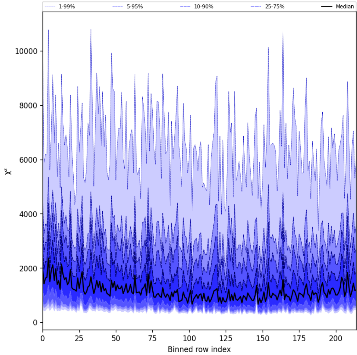
Figure 30: Along track statistics of “ \chi^2 ” for 2025-09-15 to 2025-09-17
