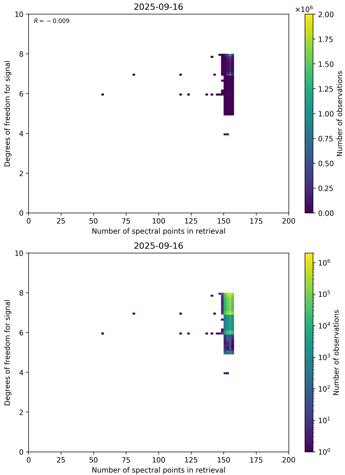
Figure 59: Scatter density plot of “Number of spectral points in retrieval” against “Degrees of freedom for signal” for 2025-09-15 to 2025-09-17.
