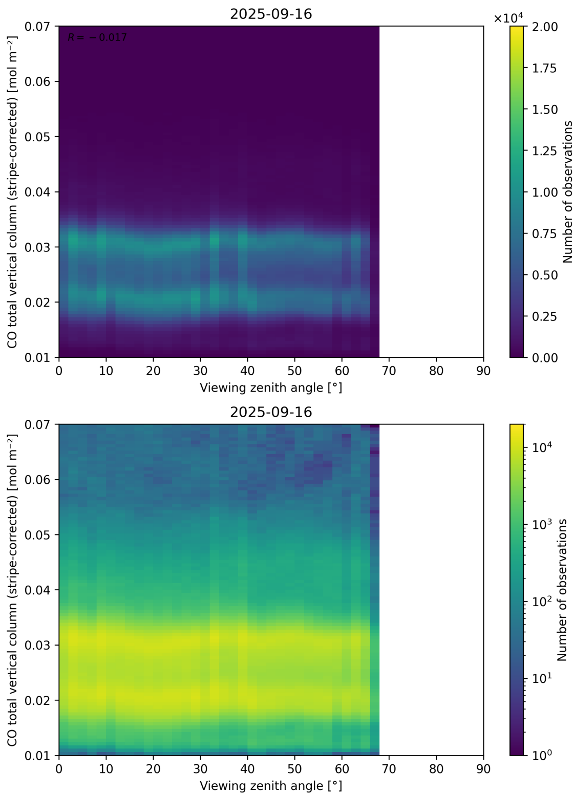
Figure 70: Scatter density plot of “Viewing zenith angle” against “CO total vertical column (stripe-corrected)” for 2025-09-15 to 2025-09-17.
