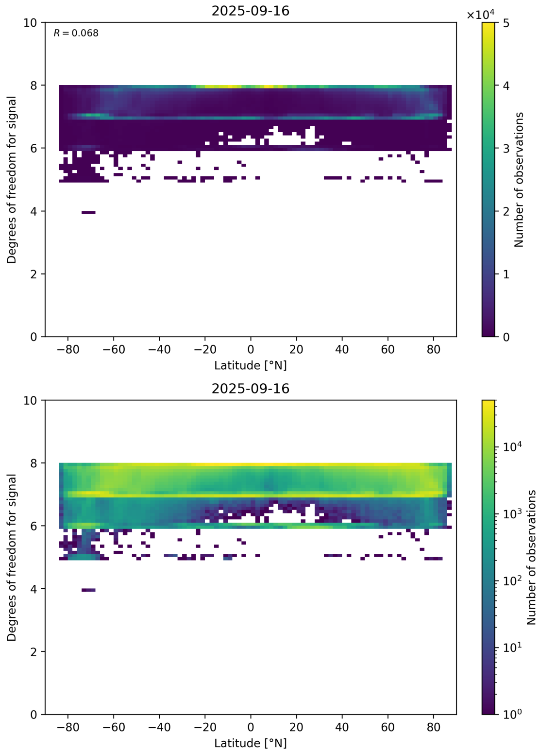
Figure 55: Scatter density plot of “Latitude” against “Degrees of freedom for signal” for 2025-09-15 to 2025-09-17.
