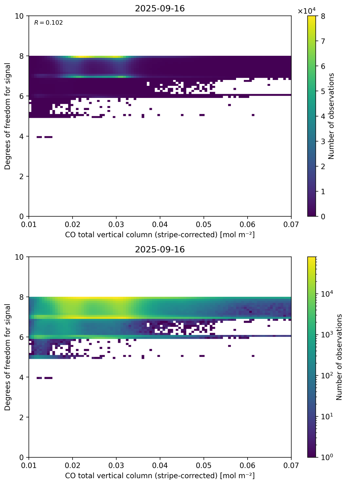
Figure 38: Scatter density plot of “CO total vertical column (stripe-corrected)” against “Degrees of freedom for signal” for 2025-09-15 to 2025-09-17.
