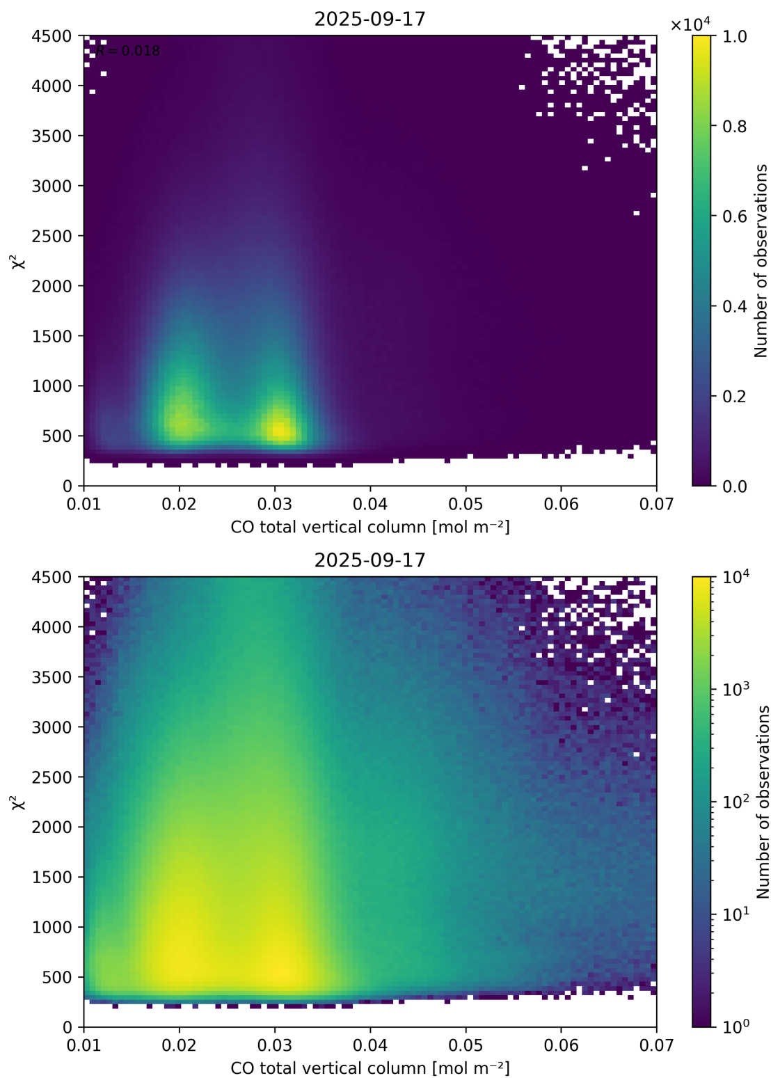
Figure 35: Scatter density plot of “CO total vertical column” against “ \chi^2 ” for 2025-09-16 to 2025-09-18.
