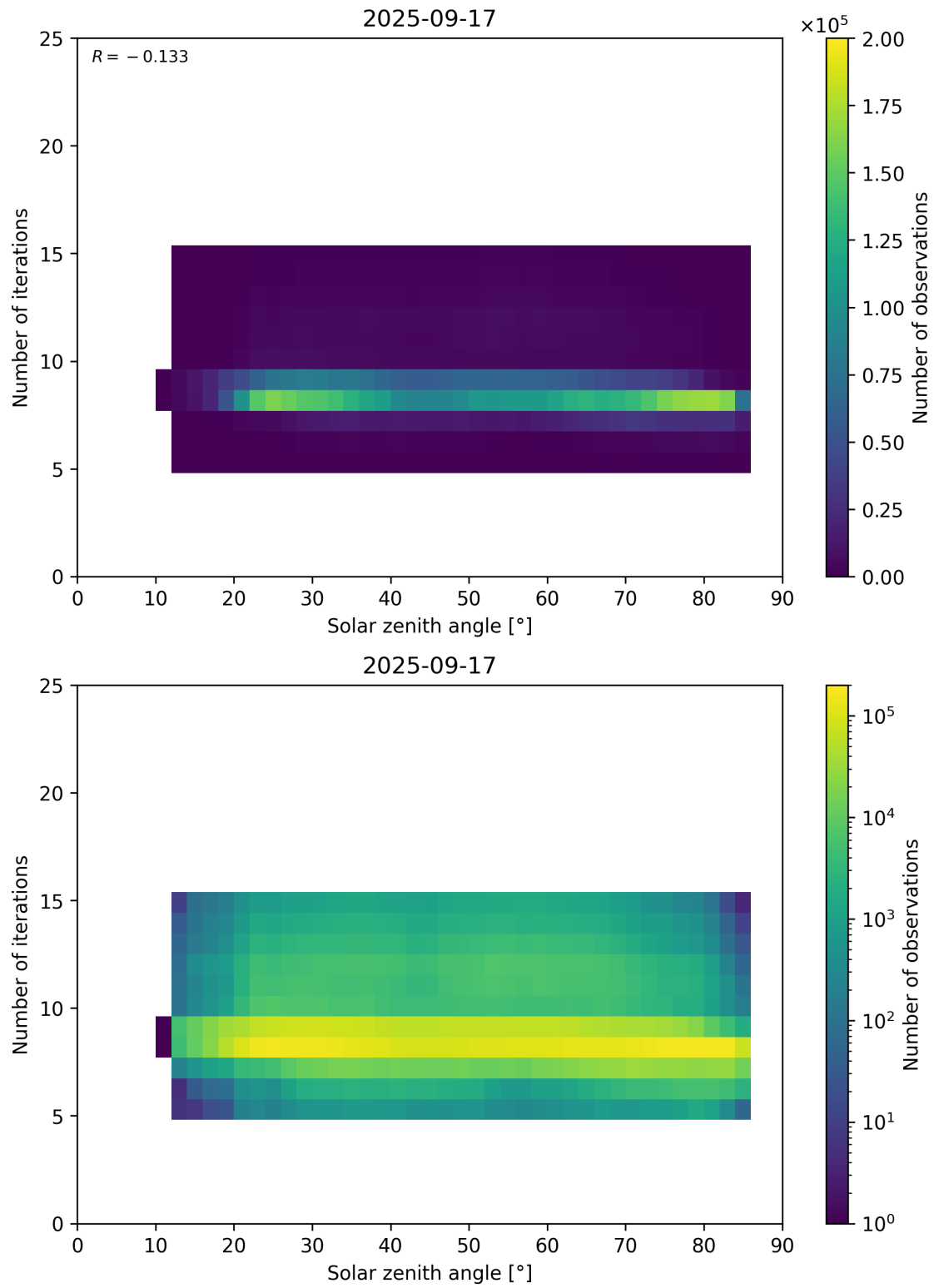
Figure 67: Scatter density plot of “Solar zenith angle” against “Number of iterations” for 2025-09-16 to 2025-09-18.
