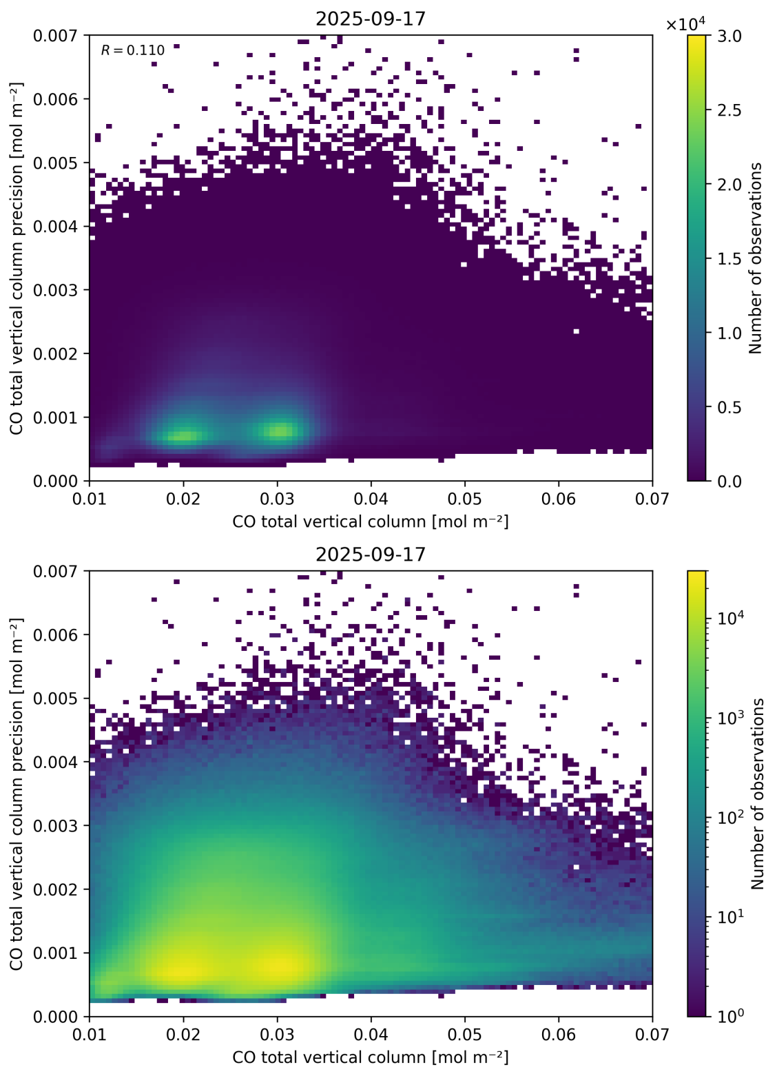
Figure 34: Scatter density plot of “CO total vertical column” against “CO total vertical column precision” for 2025-09-16 to 2025-09-18.
