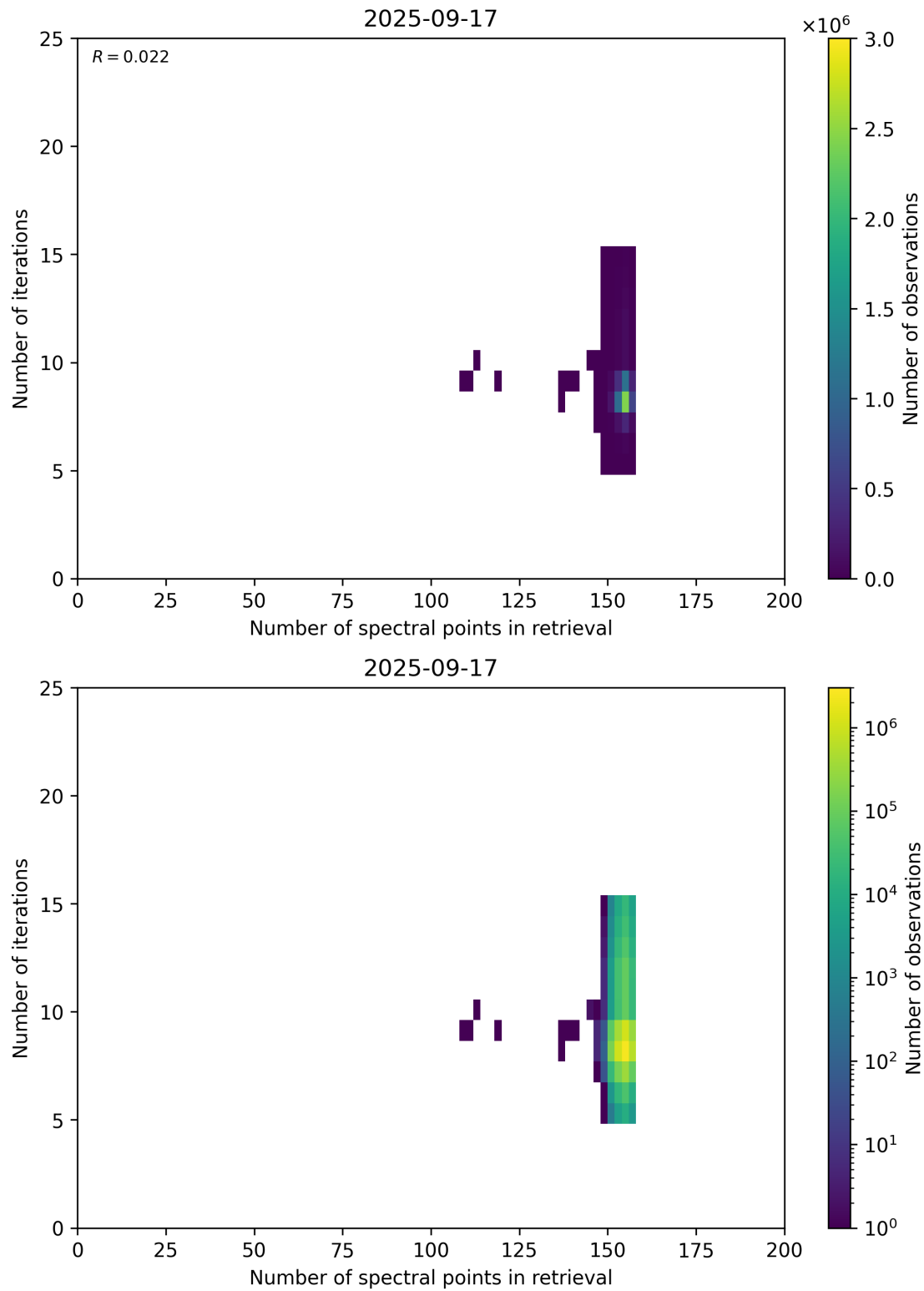
Figure 60: Scatter density plot of “Number of spectral points in retrieval” against “Number of iterations” for 2025-09-16 to 2025-09-18.
