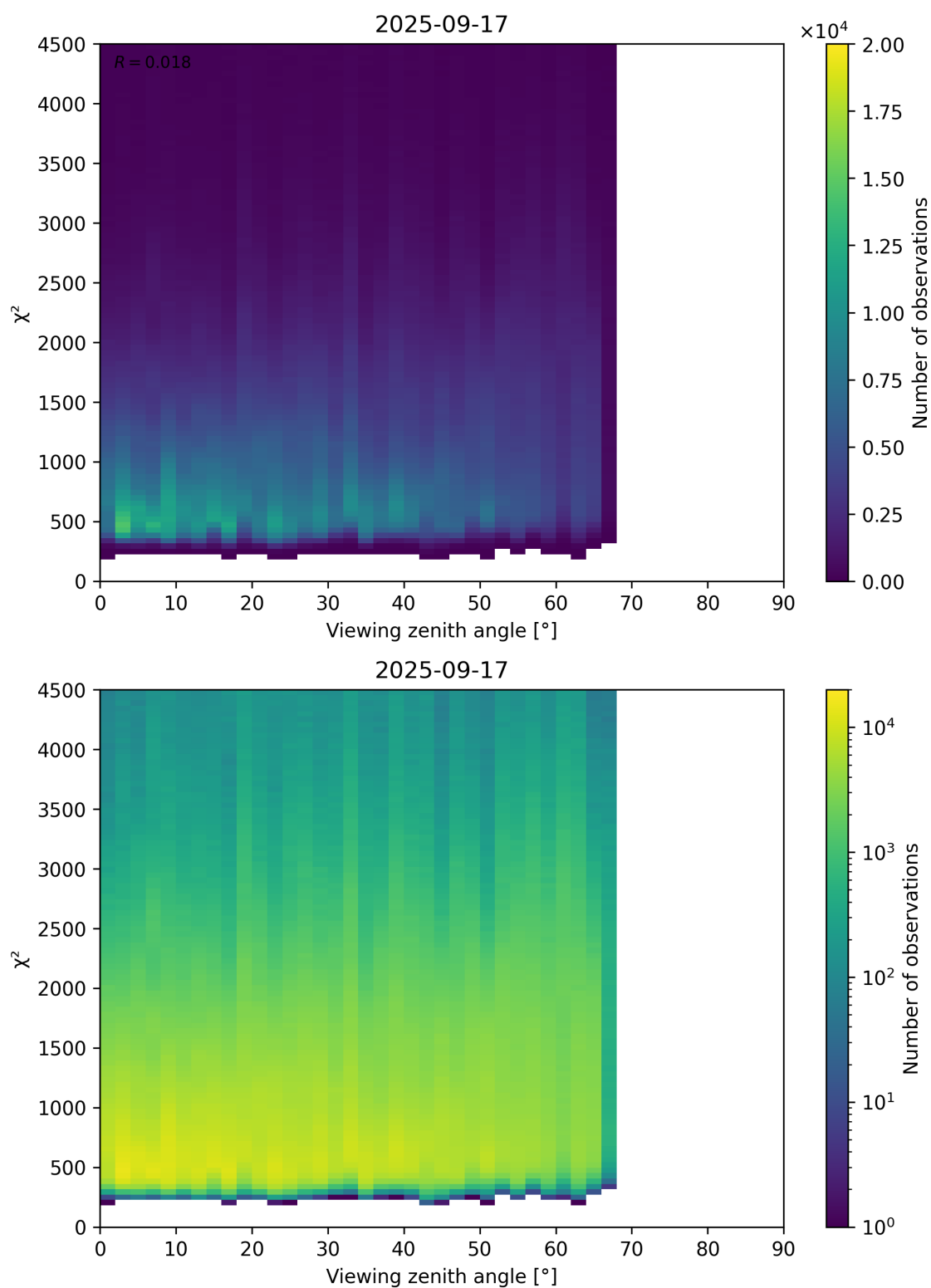
Figure 72: Scatter density plot of “Viewing zenith angle” against “ \chi^2 ” for 2025-09-16 to 2025-09-18.
