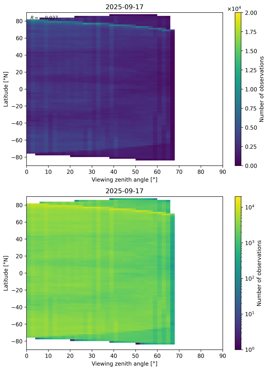
Figure 74: Scatter density plot of “Viewing zenith angle” against “Latitude” for 2025-09-16 to 2025-09-18.
