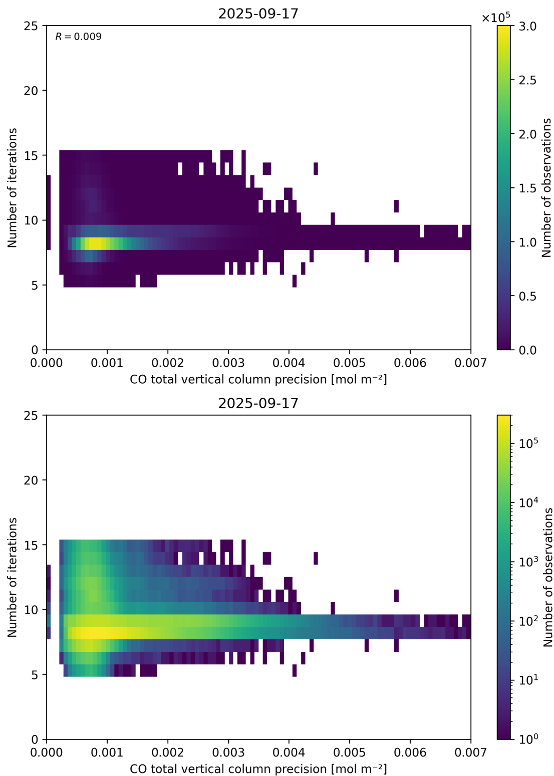
Figure 46: Scatter density plot of “CO total vertical column precision” against “Number of iterations” for 2025-09-16 to 2025-09-18.
