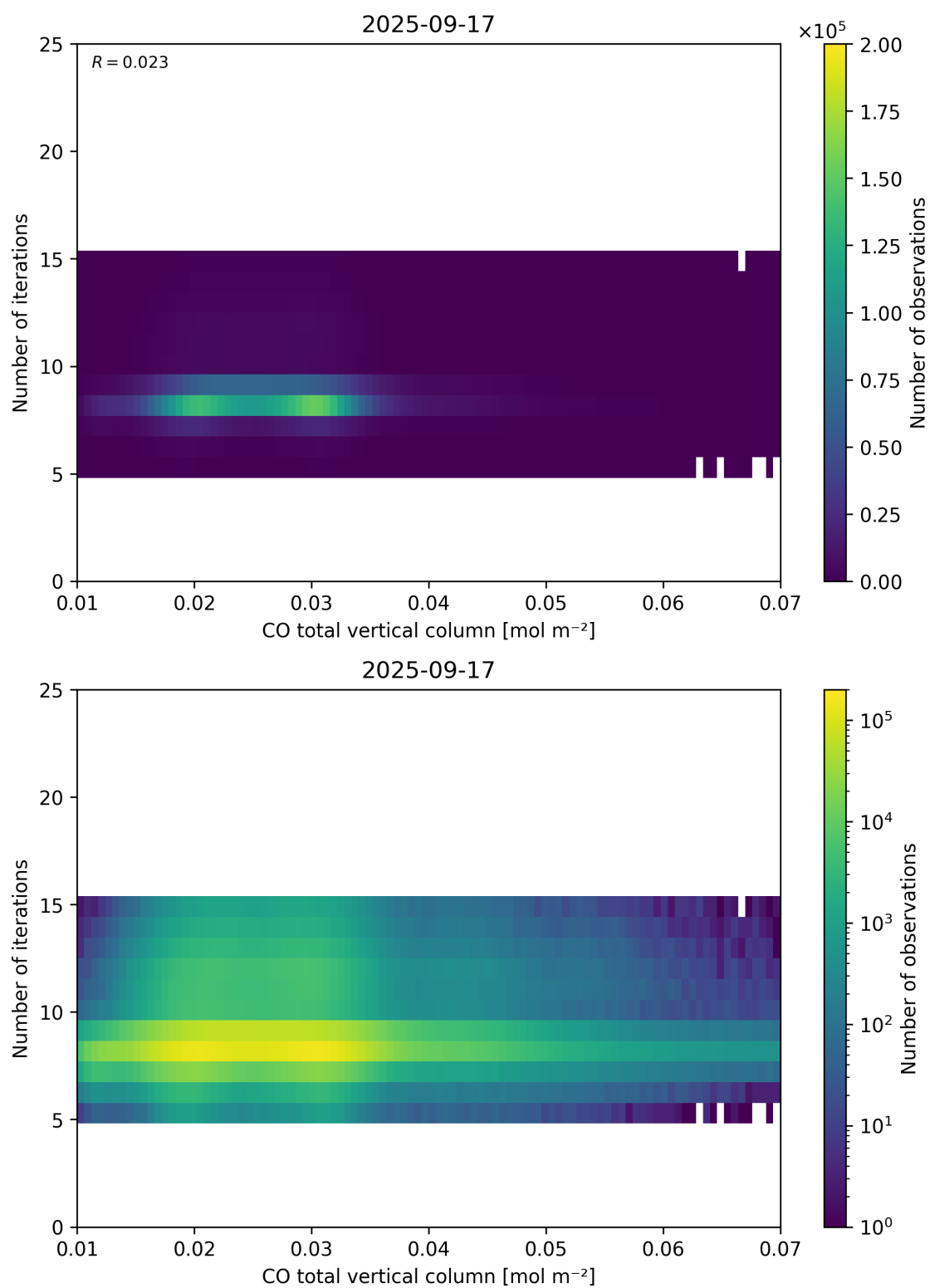
Figure 42: Scatter density plot of “CO total vertical column” against “Number of iterations” for 2025-09-16 to 2025-09-18.
