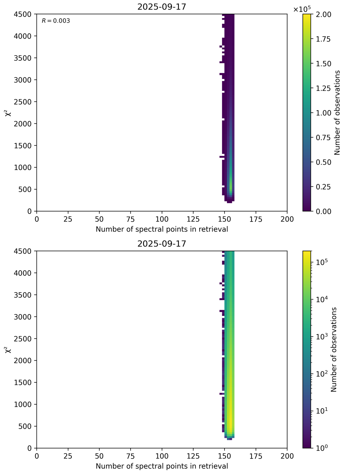
Figure 58: Scatter density plot of “Number of spectral points in retrieval” against “ \chi^2 ” for 2025-09-16 to 2025-09-18.
