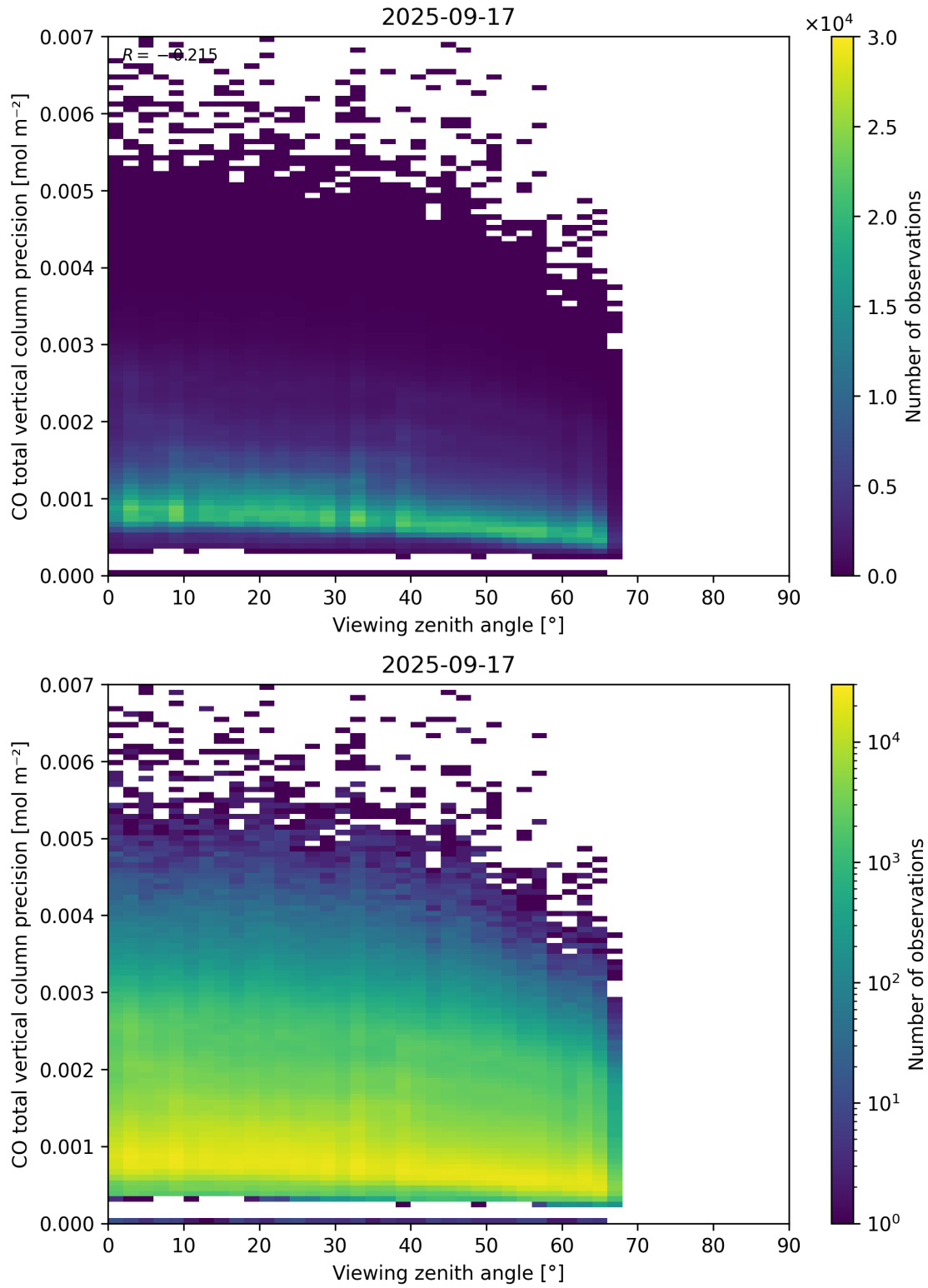
Figure 71: Scatter density plot of “Viewing zenith angle” against “CO total vertical column precision” for 2025-09-16 to 2025-09-18.
