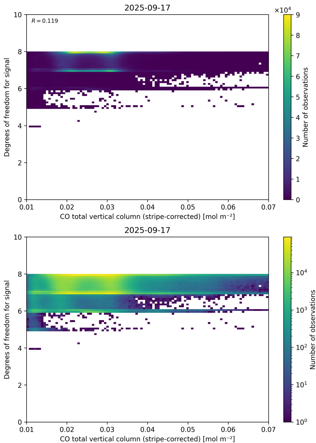
Figure 38: Scatter density plot of “CO total vertical column (stripe-corrected)” against “Degrees of freedom for signal” for 2025-09-16 to 2025-09-18.
