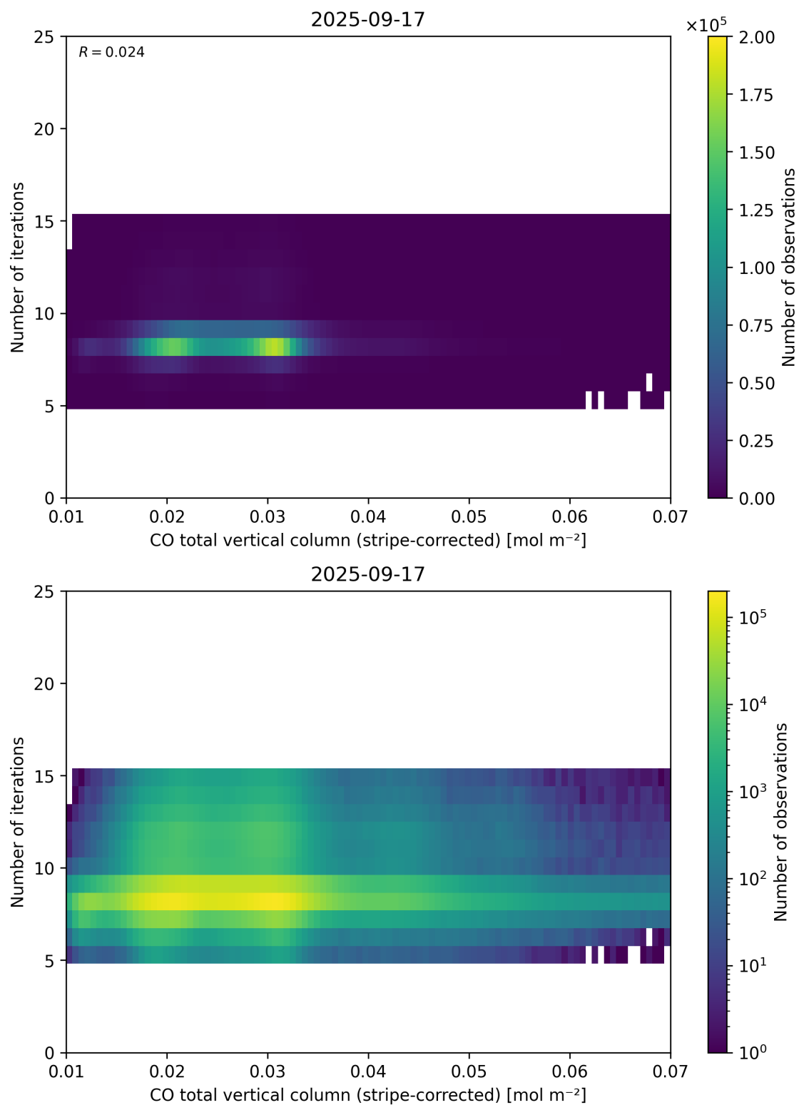
Figure 39: Scatter density plot of “CO total vertical column (stripe-corrected)” against “Number of iterations” for 2025-09-16 to 2025-09-18.
