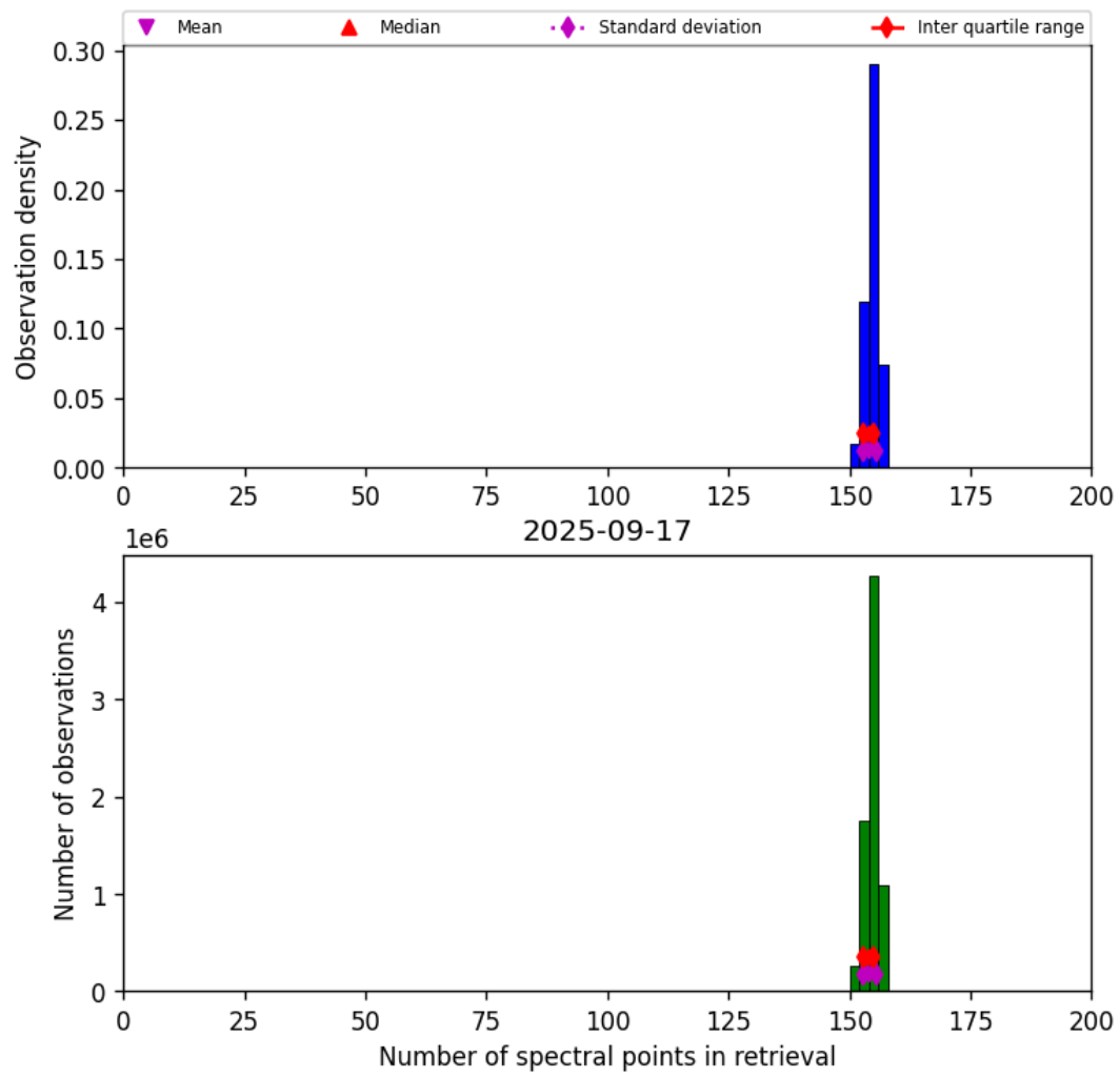
Figure 21: Histogram of “Number of spectral points in retrieval” for 2025-09-16 to 2025-09-18
