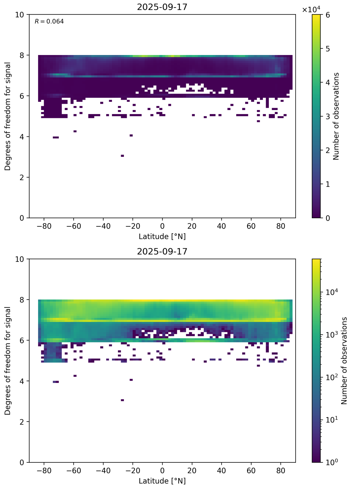
Figure 55: Scatter density plot of “Latitude” against “Degrees of freedom for signal” for 2025-09-16 to 2025-09-18.
