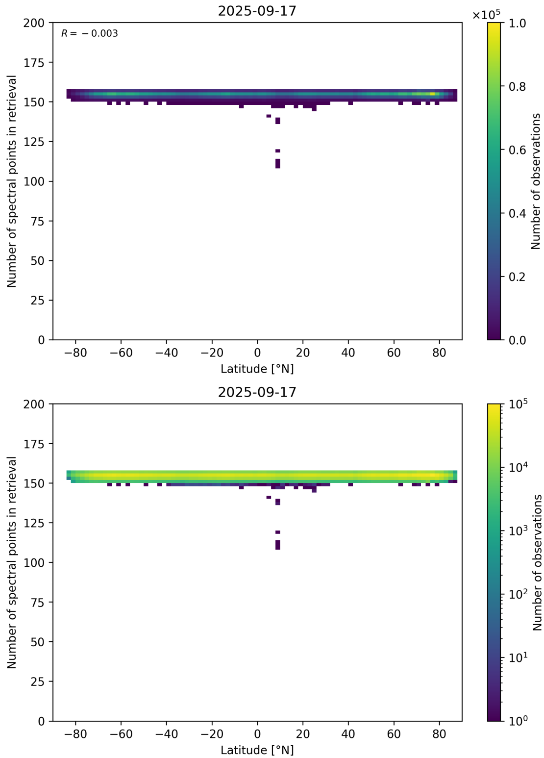
Figure 57: Scatter density plot of “Latitude” against “Number of spectral points in retrieval” for 2025-09-16 to 2025-09-18.
