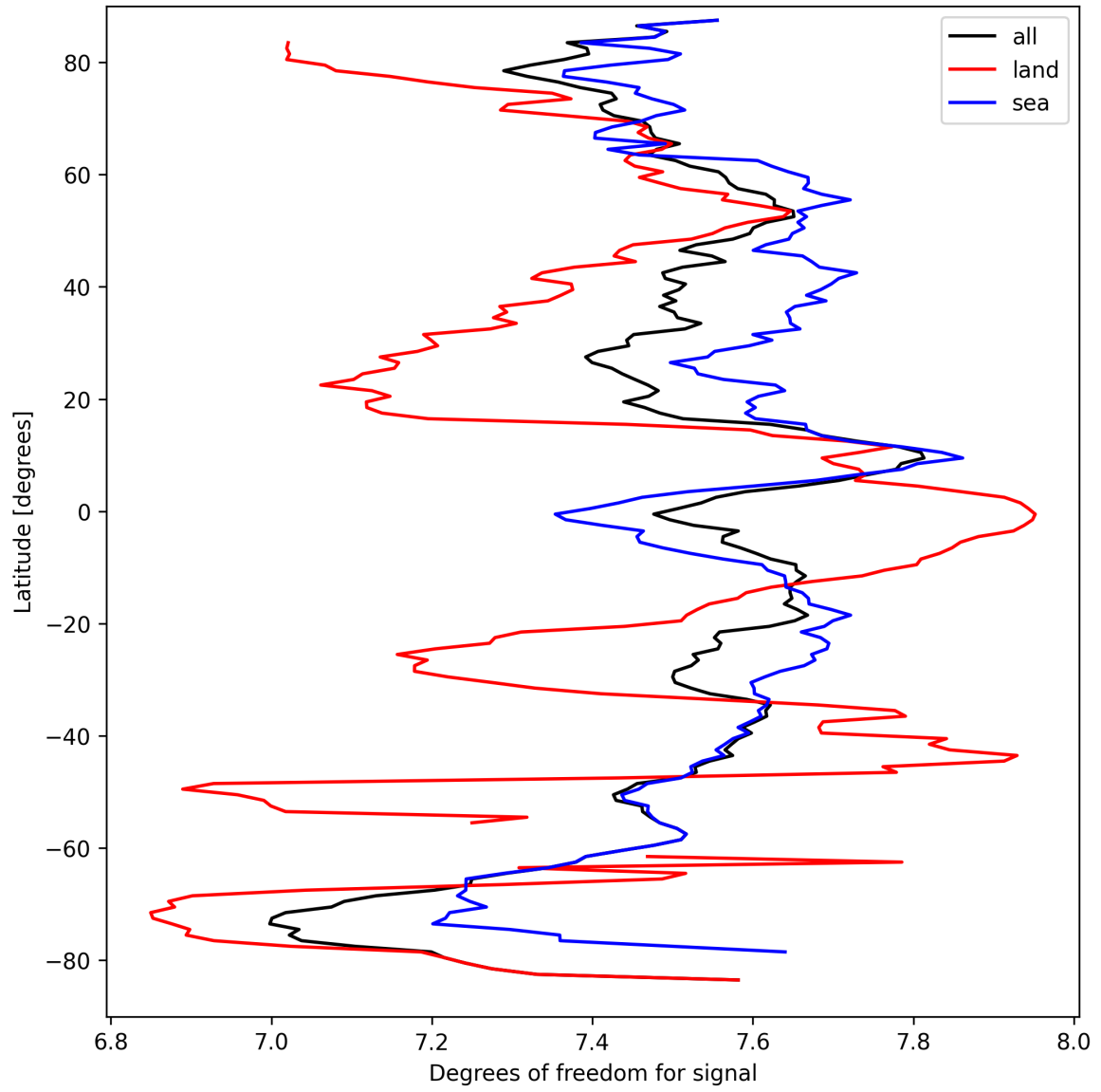
Figure 15: Zonal average of “Degrees of freedom for signal” for 2025-09-16 to 2025-09-18.
