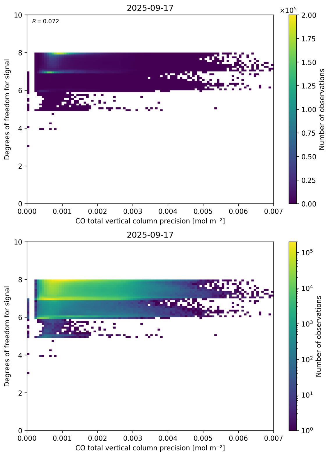
Figure 45: Scatter density plot of “CO total vertical column precision” against “Degrees of freedom for signal” for 2025-09-16 to 2025-09-18.
