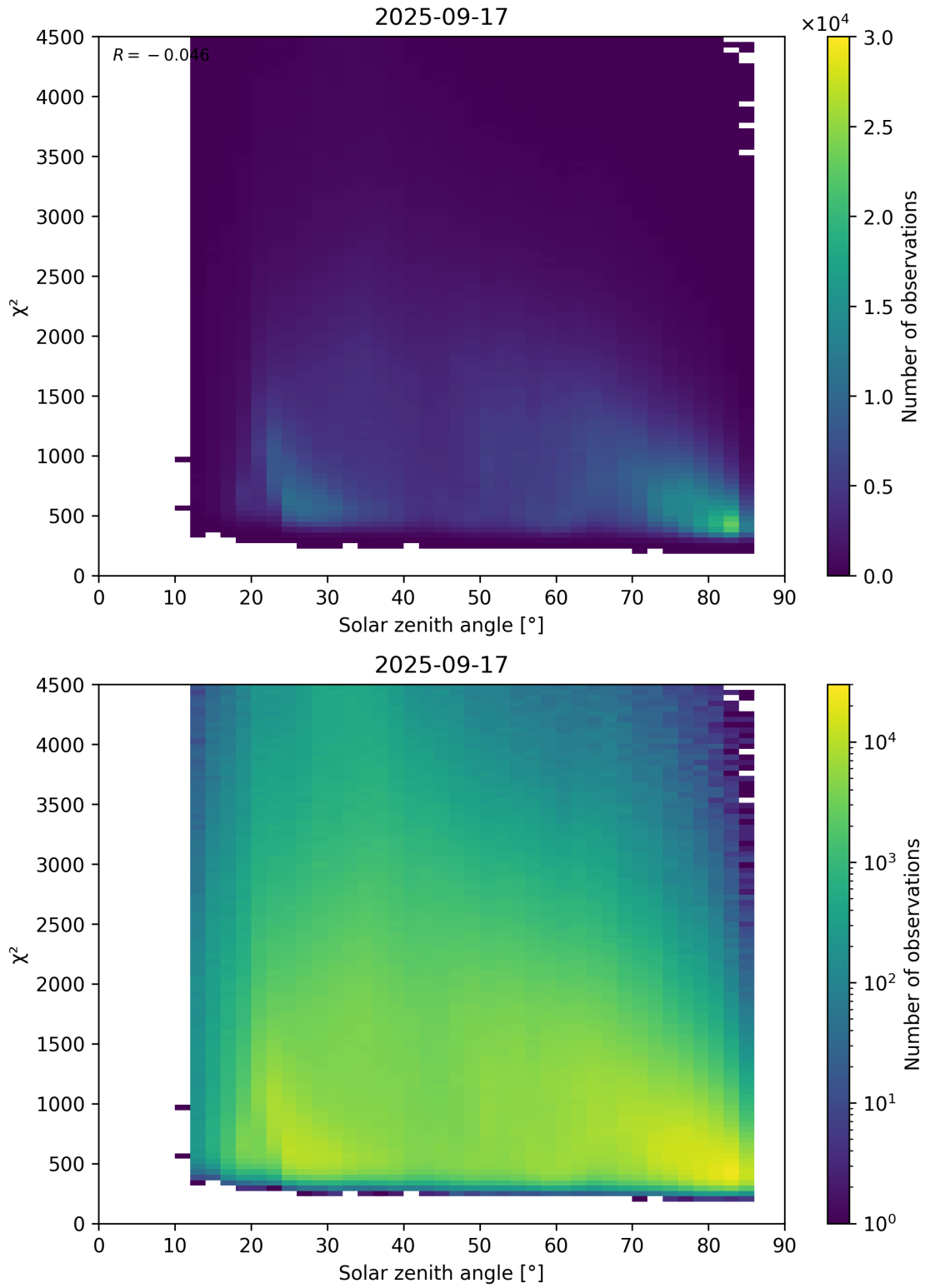
Figure 64: Scatter density plot of “Solar zenith angle” against “ \chi^2 ” for 2025-09-16 to 2025-09-18.
