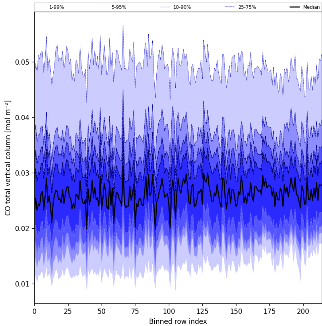
Figure 26: Along track statistics of “CO total vertical column” for 2025-09-16 to 2025-09-18
