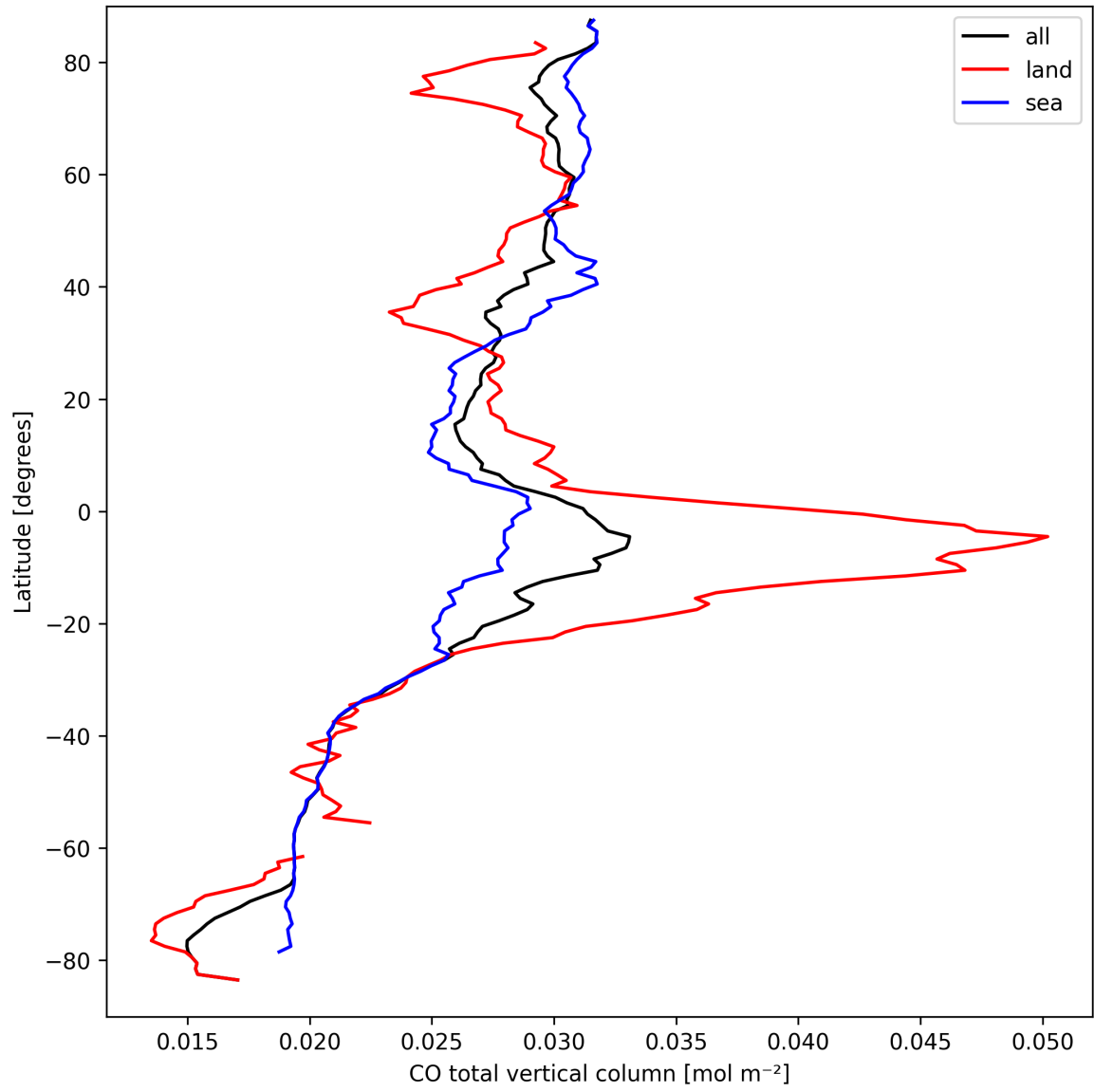
Figure 10: Zonal average of “CO total vertical column” for 2025-09-16 to 2025-09-18.
