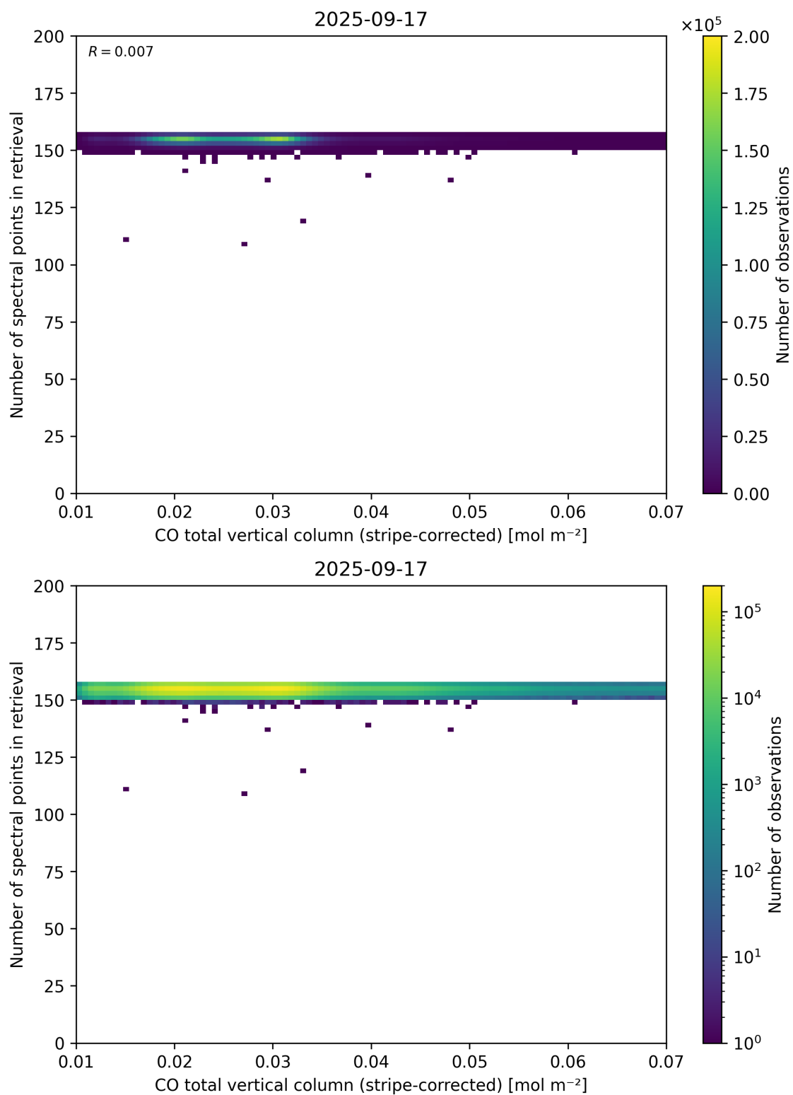
Figure 40: Scatter density plot of “CO total vertical column (stripe-corrected)” against “Number of spectral points in retrieval” for 2025-09-16 to 2025-09-18.
