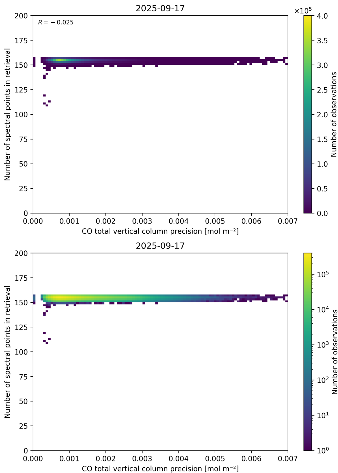
Figure 47: Scatter density plot of “CO total vertical column precision” against “Number of spectral points in retrieval” for 2025-09-16 to 2025-09-18.
