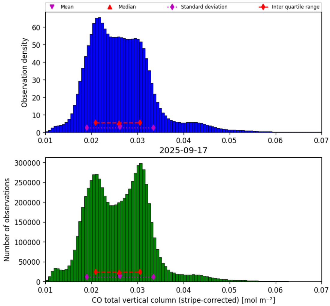
Figure 19: Histogram of “CO total vertical column (stripe-corrected)” for 2025-09-16 to 2025-09-18
