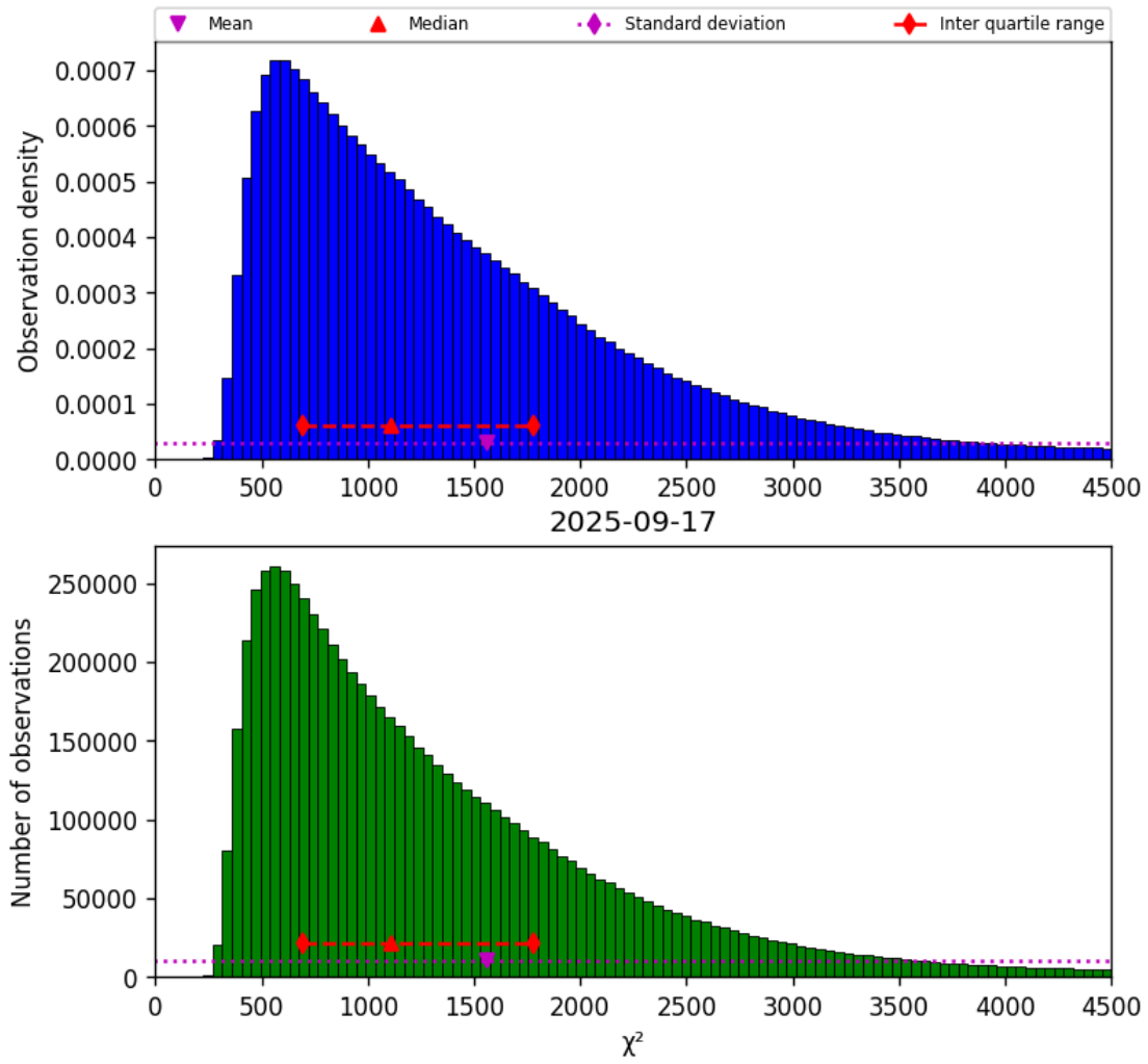
Figure 22: Histogram of “ \chi^2 ” for 2025-09-16 to 2025-09-18
