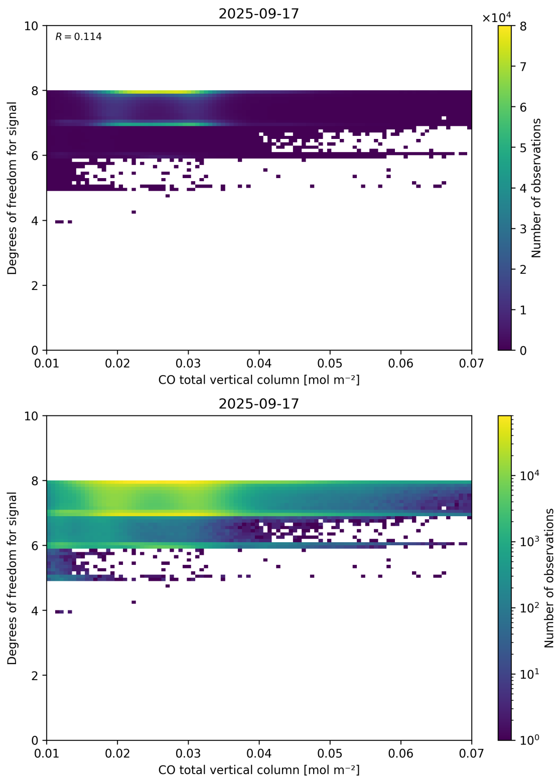
Figure 41: Scatter density plot of “CO total vertical column” against “Degrees of freedom for signal” for 2025-09-16 to 2025-09-18.
