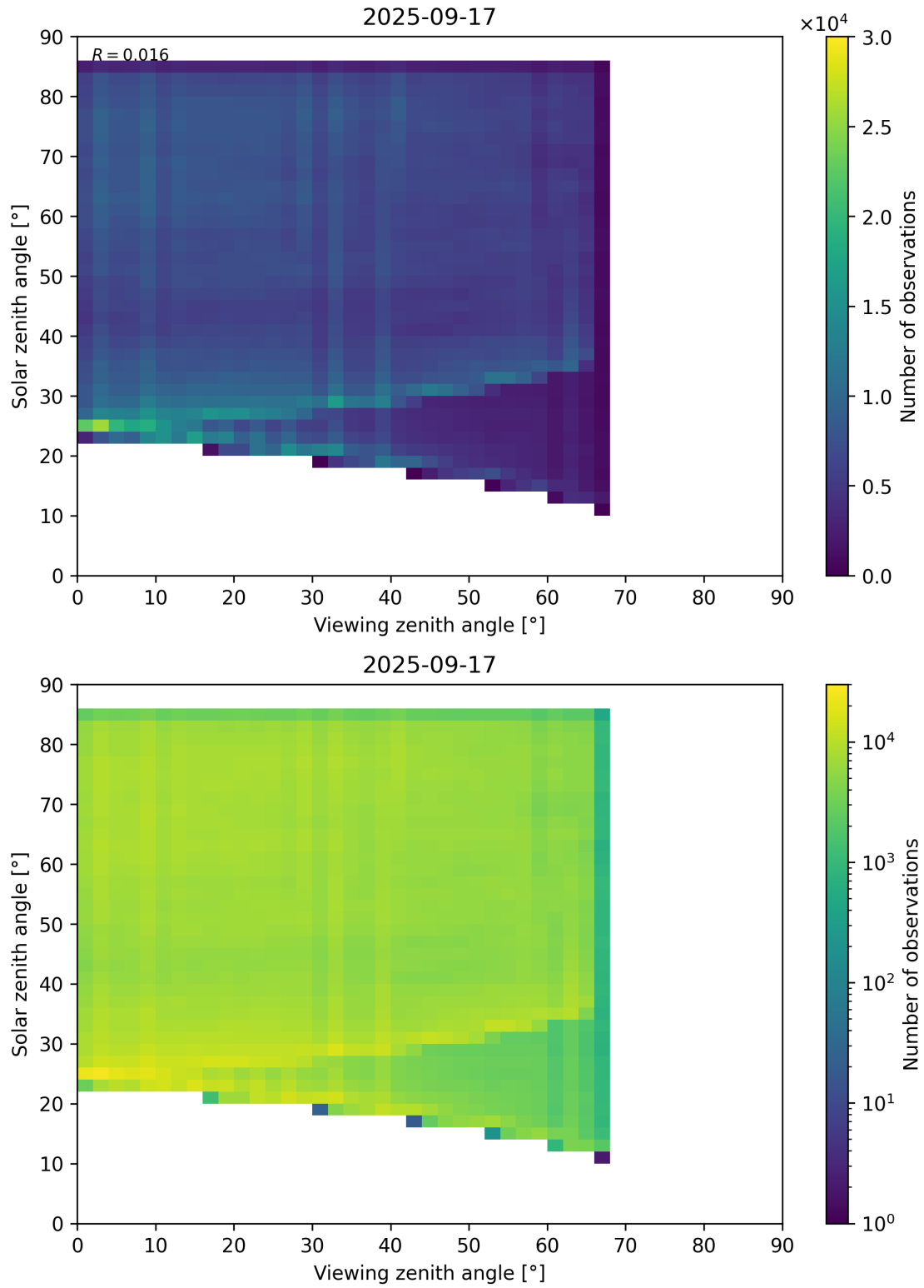
Figure 77: Scatter density plot of “Viewing zenith angle” against “Solar zenith angle” for 2025-09-16 to 2025-09-18.
