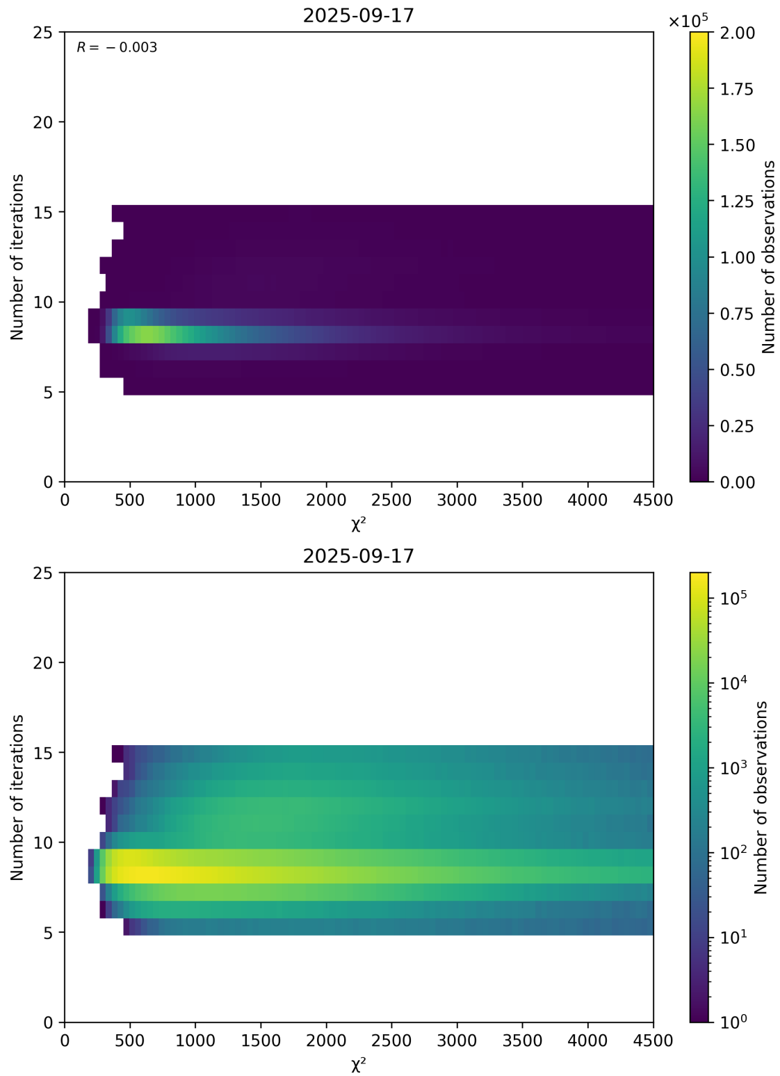
Figure 49: Scatter density plot of “ \chi^2 ” against “Number of iterations” for 2025-09-16 to 2025-09-18.
