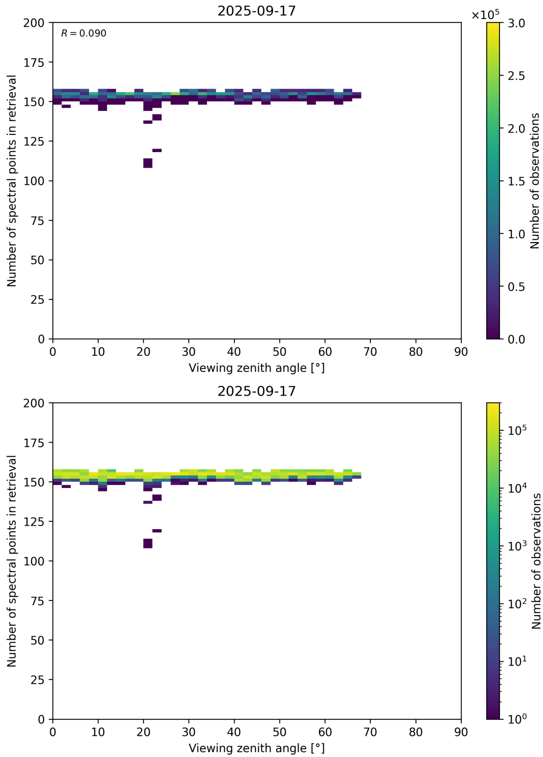
Figure 76: Scatter density plot of “Viewing zenith angle” against “Number of spectral points in retrieval” for 2025-09-16 to 2025-09-18.
