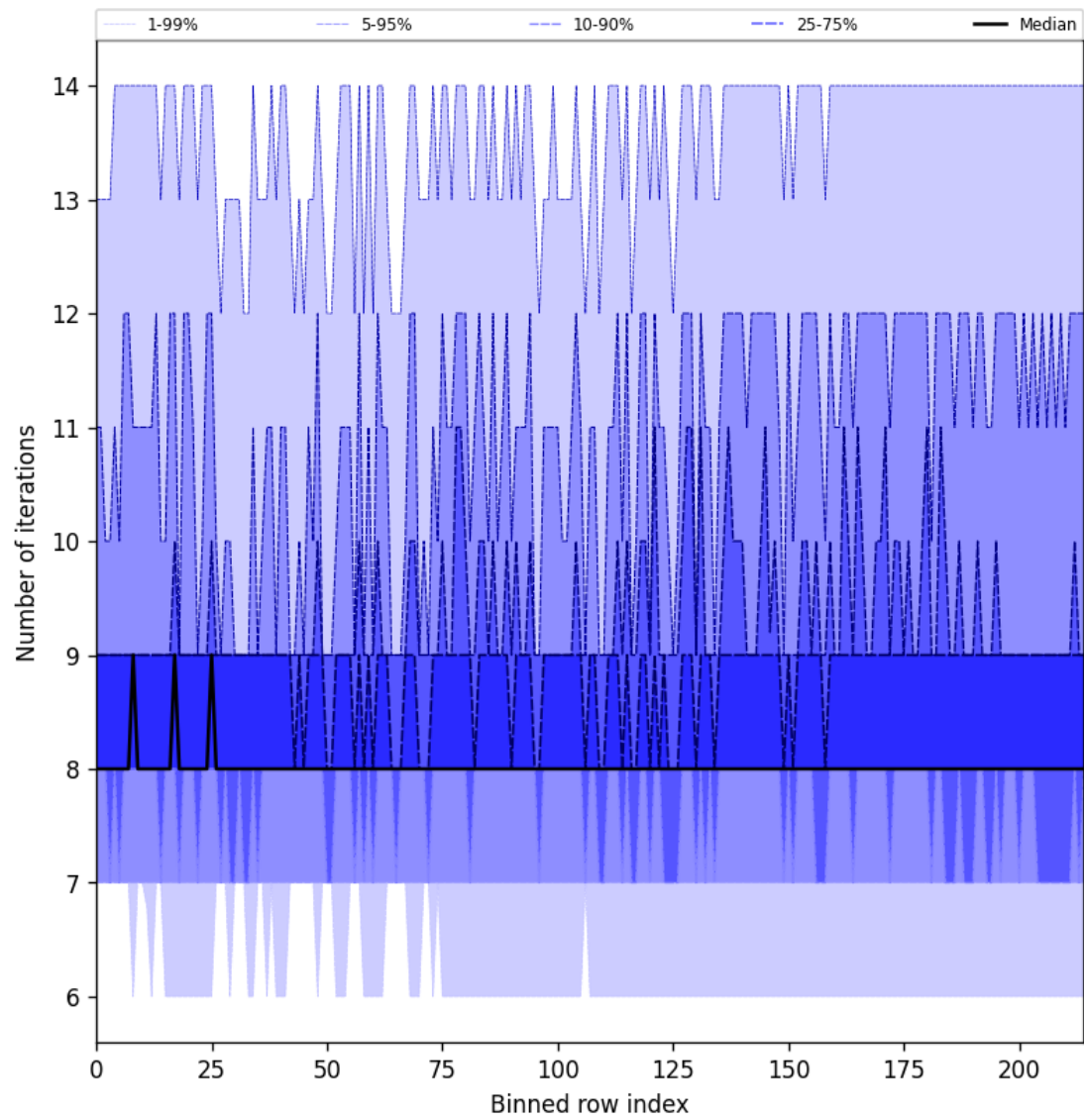
Figure 32: Along track statistics of “Number of iterations” for 2025-09-16 to 2025-09-18
