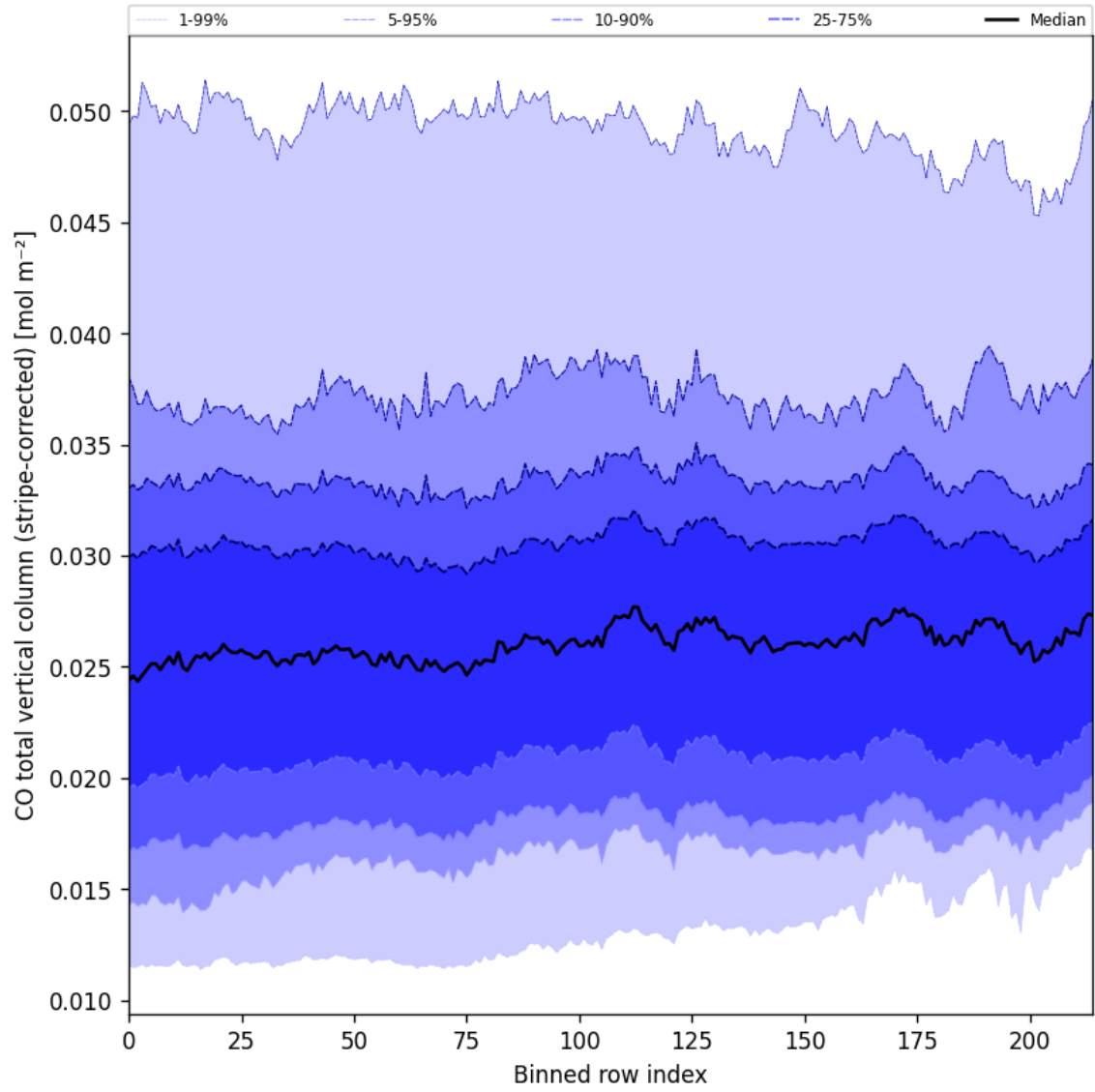
Figure 27: Along track statistics of “CO total vertical column (stripe-corrected)” for 2025-09-16 to 2025-09-18
