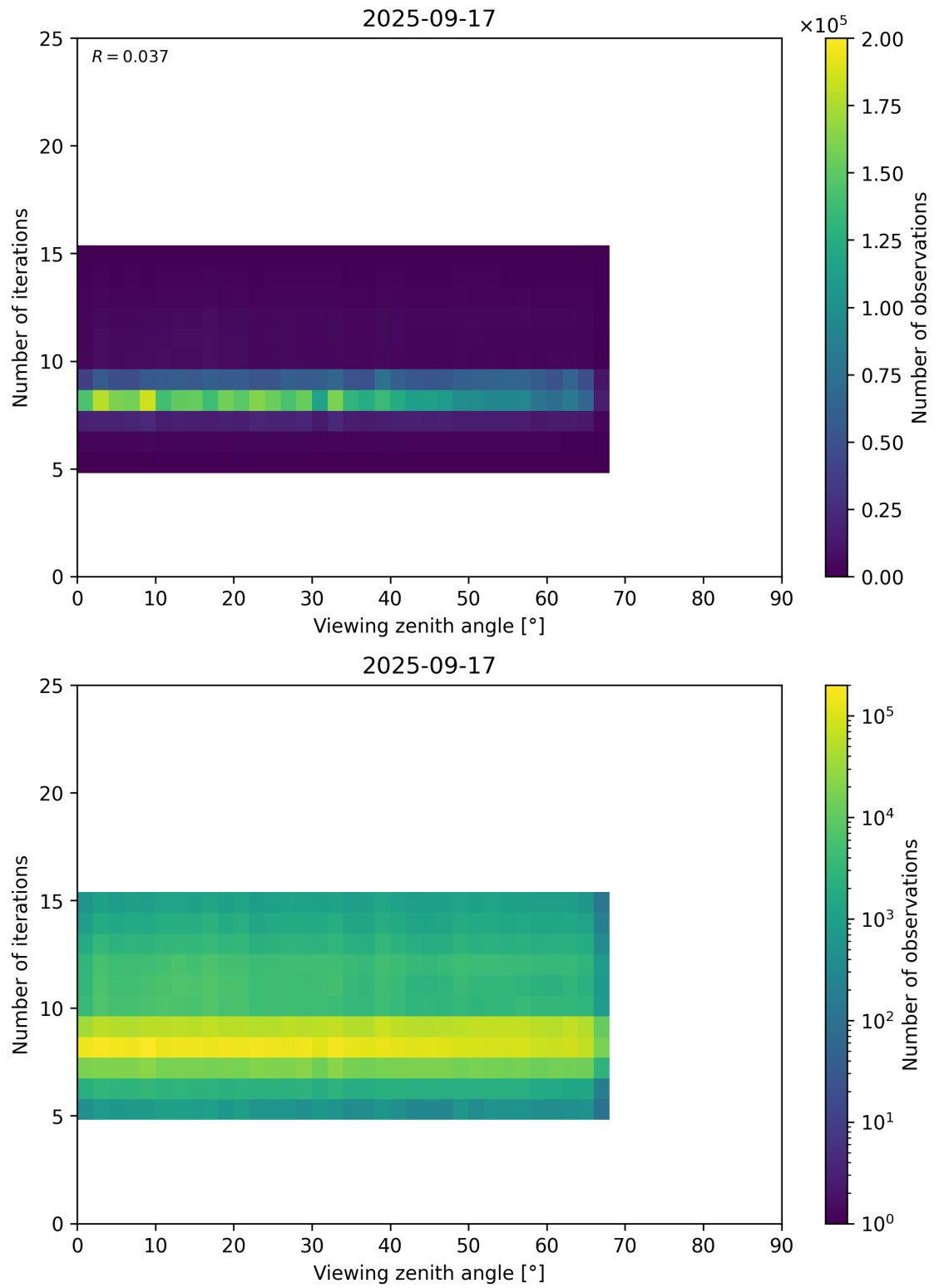
Figure 75: Scatter density plot of “Viewing zenith angle” against “Number of iterations” for 2025-09-16 to 2025-09-18.
