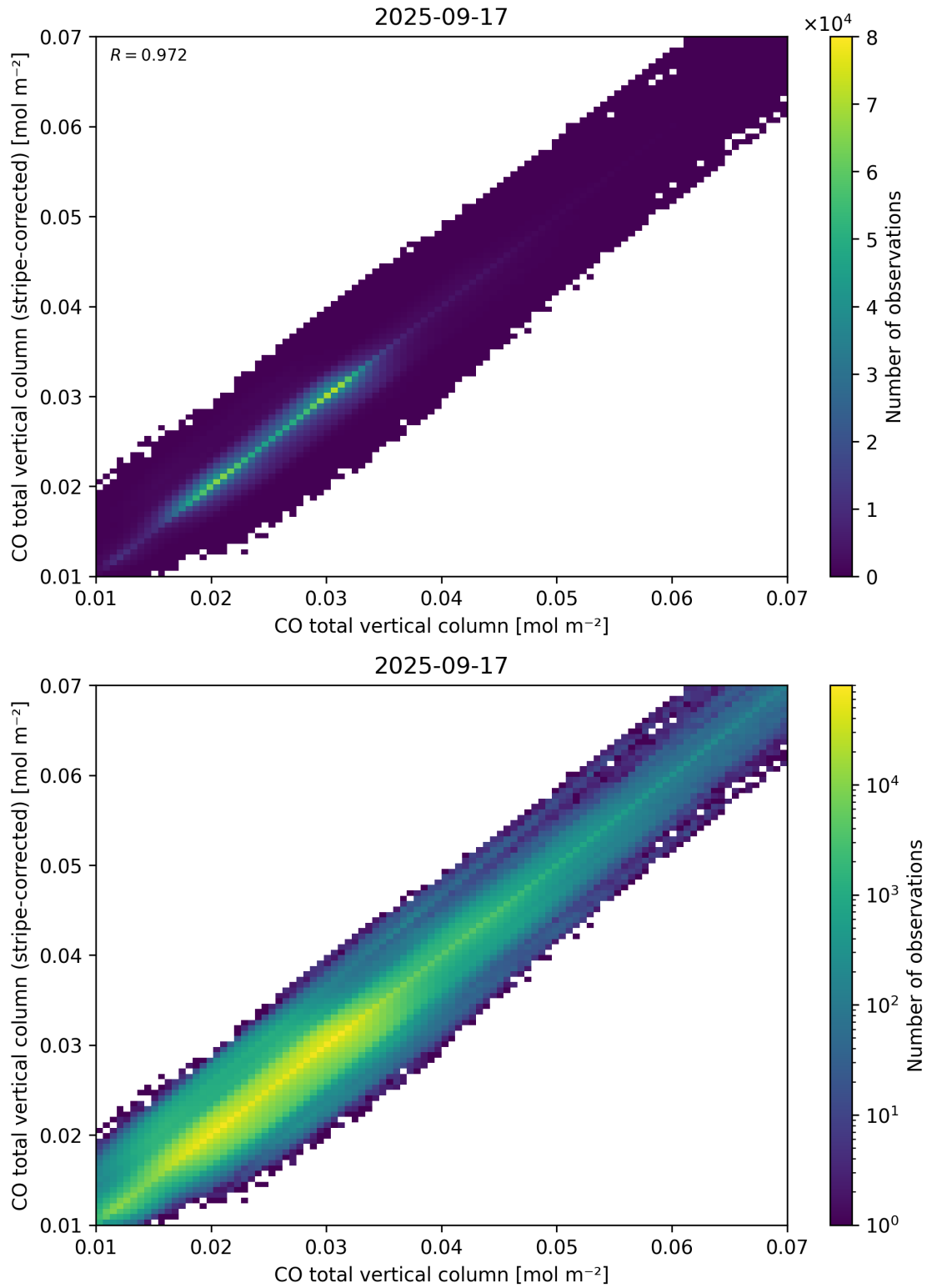
Figure 33: Scatter density plot of “CO total vertical column” against “CO total vertical column (stripe-corrected)” for 2025-09-16 to 2025-09-18.
