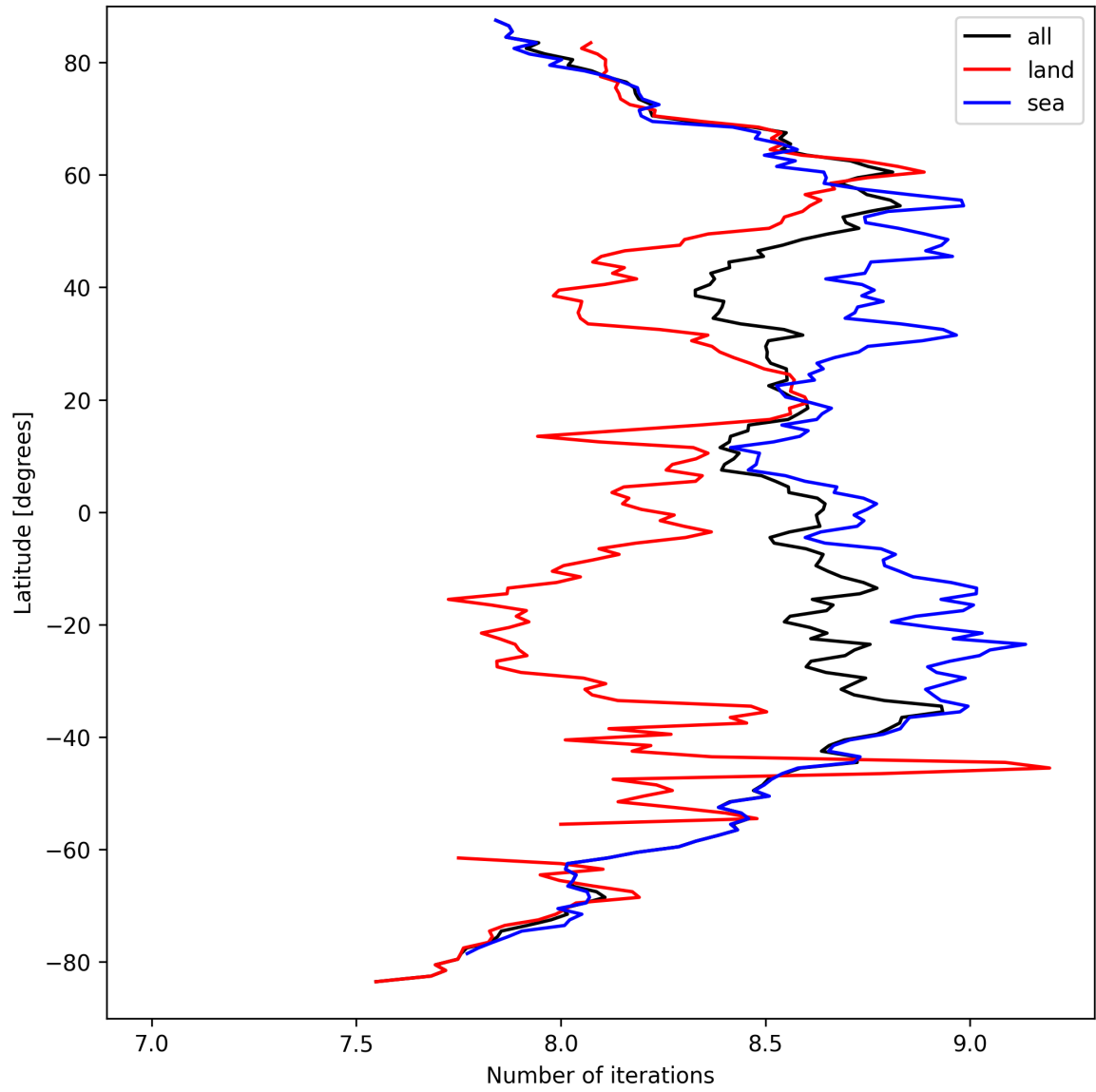
Figure 16: Zonal average of “Number of iterations” for 2025-09-16 to 2025-09-18.
