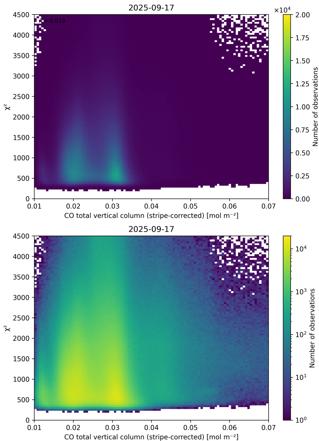
Figure 37: Scatter density plot of “CO total vertical column (stripe-corrected)” against “ \chi^2 ” for 2025-09-16 to 2025-09-18.
