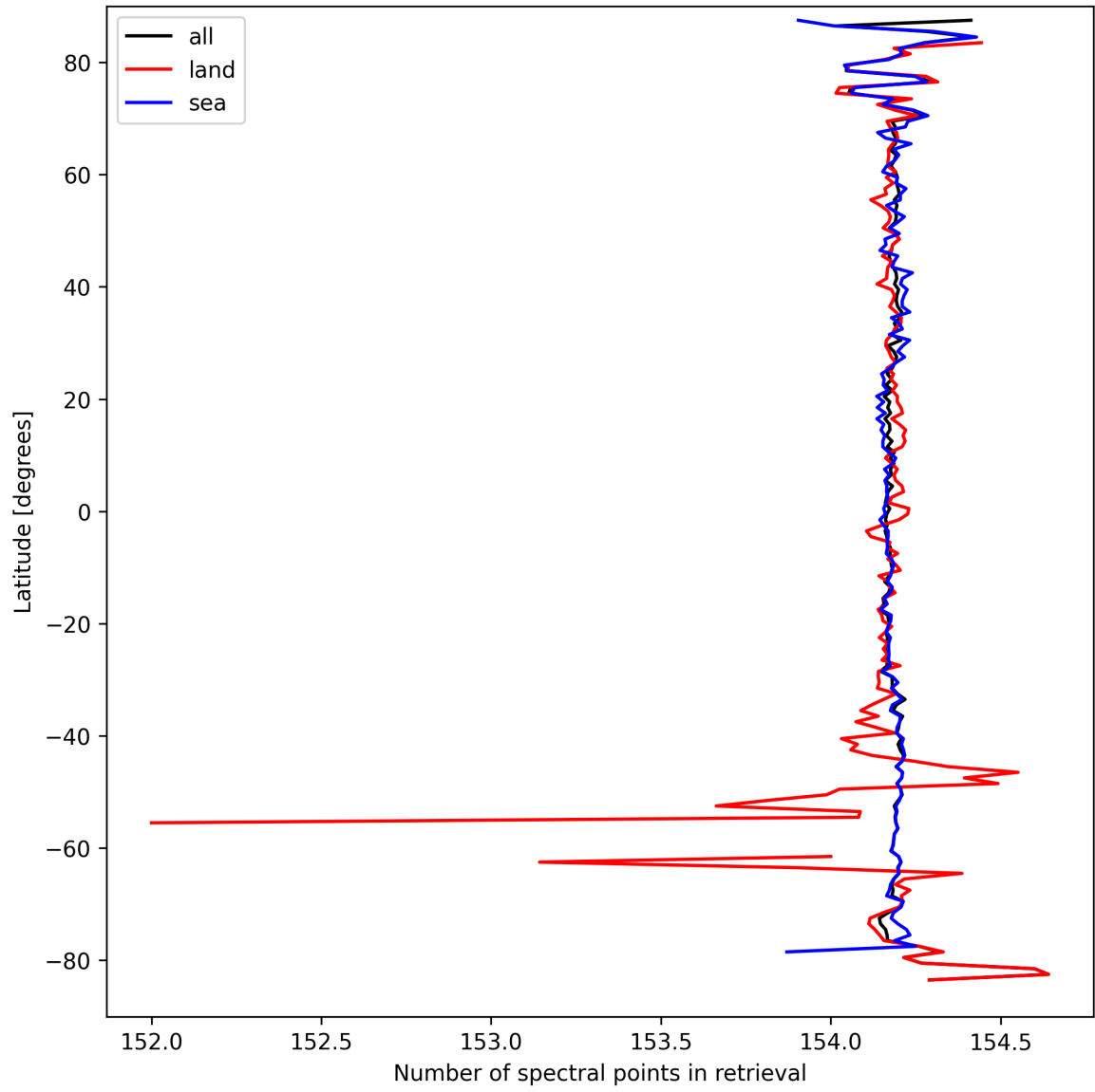
Figure 13: Zonal average of “Number of spectral points in retrieval” for 2025-09-16 to 2025-09-18.
