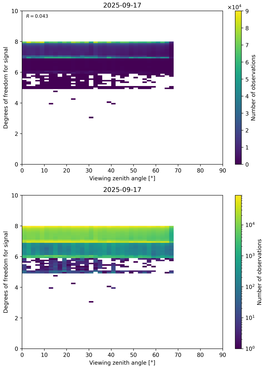
Figure 73: Scatter density plot of “Viewing zenith angle” against “Degrees of freedom for signal” for 2025-09-16 to 2025-09-18.
