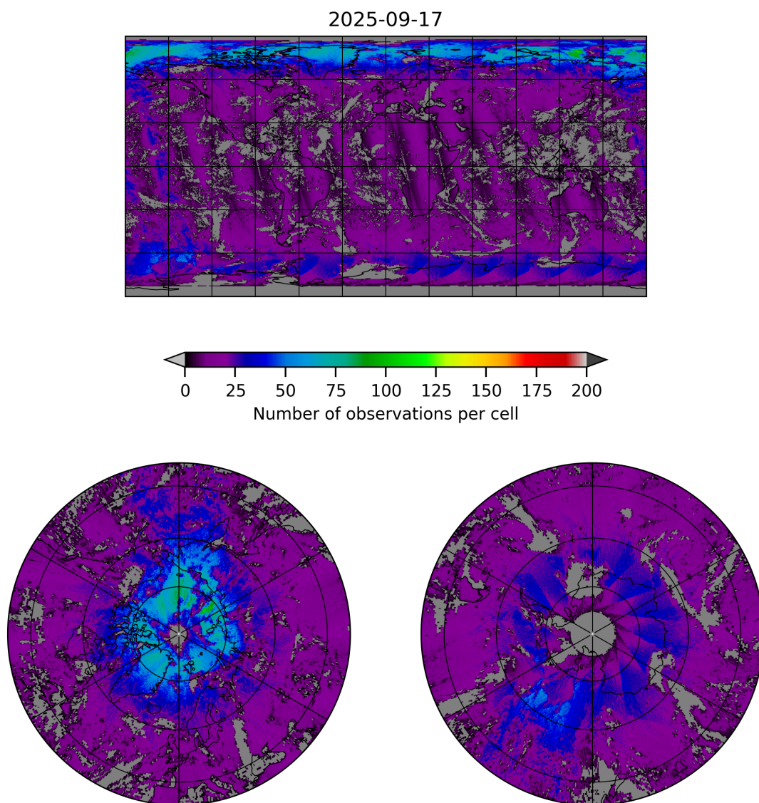
Figure 8: Map of the number of observations for 2025-09-16 to 2025-09-18
