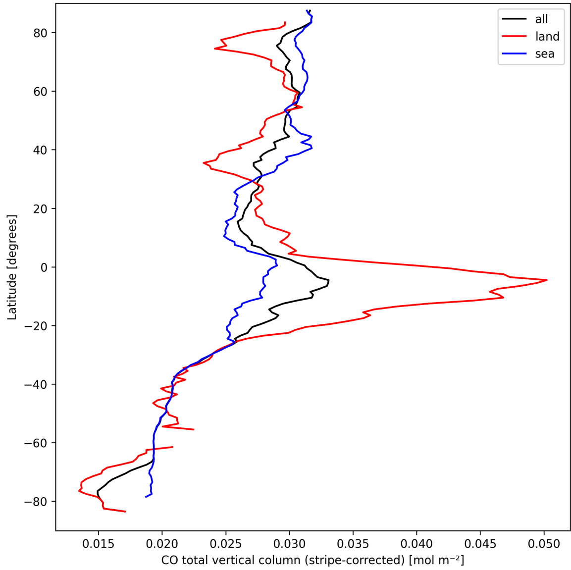
Figure 11: Zonal average of “CO total vertical column (stripe-corrected)” for 2025-09-16 to 2025-09-18.
