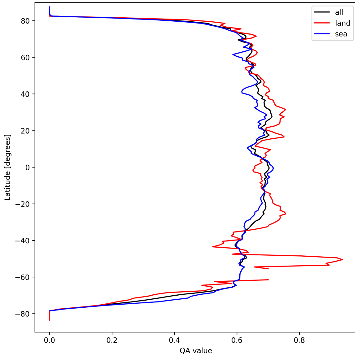
Figure 9: Zonal average of “QA value” for 2025-09-16 to 2025-09-18.
