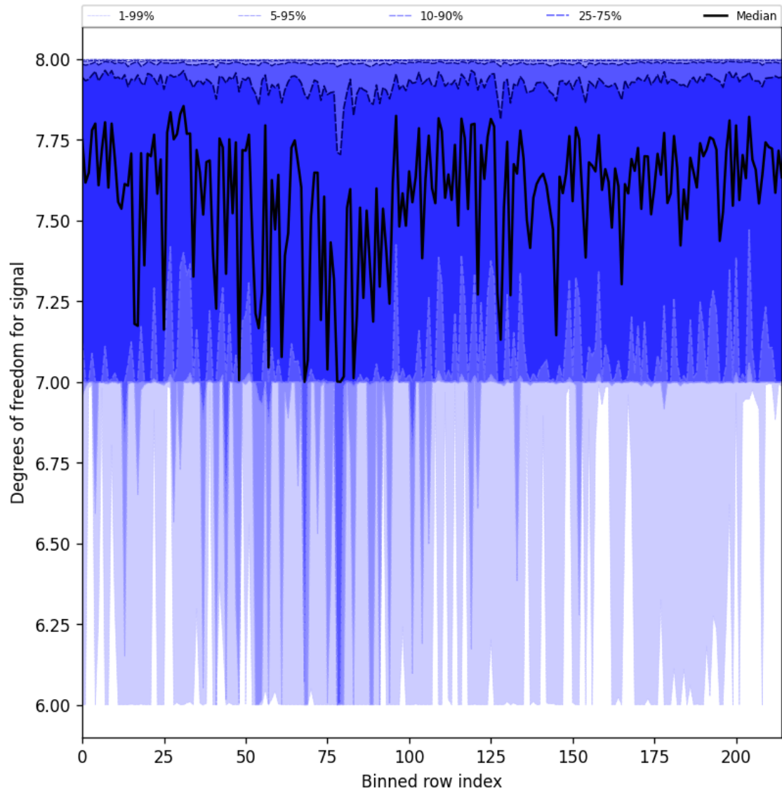
Figure 31: Along track statistics of “Degrees of freedom for signal” for 2025-09-16 to 2025-09-18
