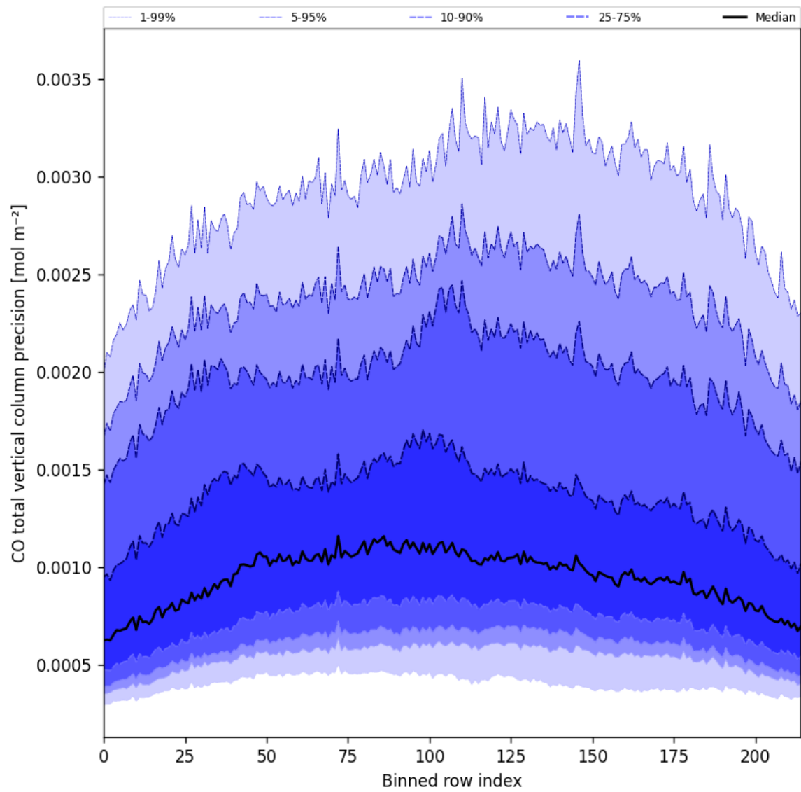
Figure 28: Along track statistics of “CO total vertical column precision” for 2025-09-16 to 2025-09-18
