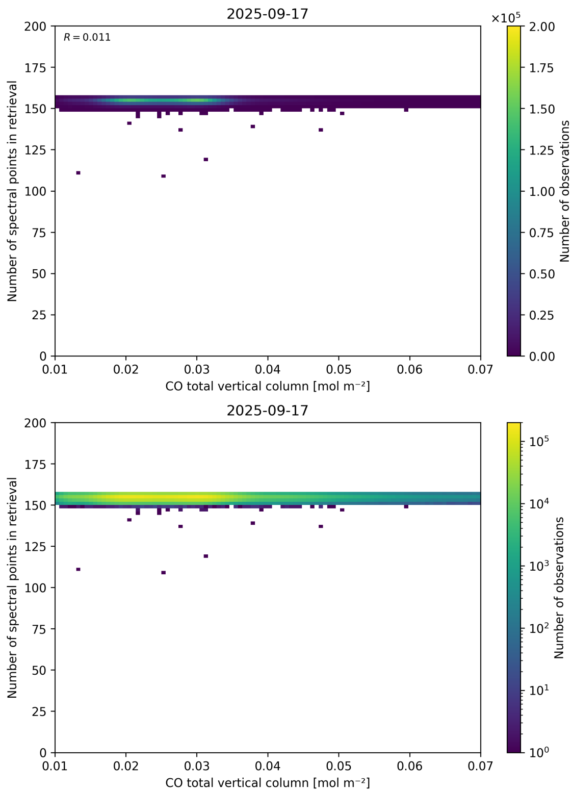
Figure 43: Scatter density plot of “CO total vertical column” against “Number of spectral points in retrieval” for 2025-09-16 to 2025-09-18.
