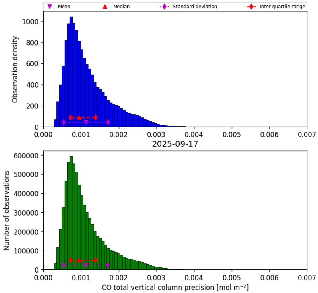
Figure 20: Histogram of “CO total vertical column precision” for 2025-09-16 to 2025-09-18
