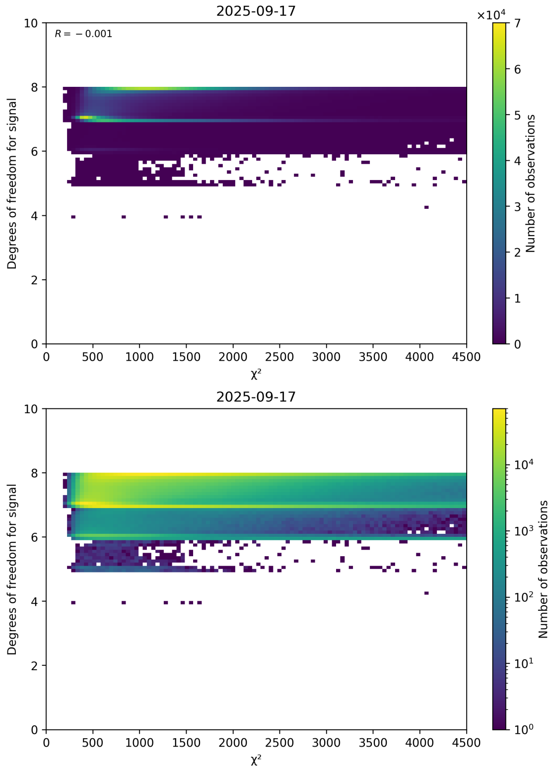
Figure 48: Scatter density plot of “ \chi^2 ” against “Degrees of freedom for signal” for 2025-09-16 to 2025-09-18.
