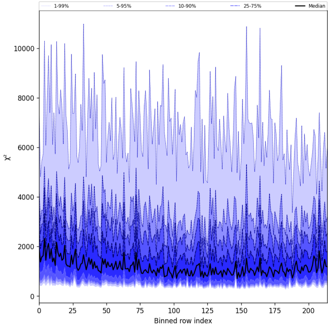
Figure 30: Along track statistics of “ \chi^2 ” for 2025-09-16 to 2025-09-18
