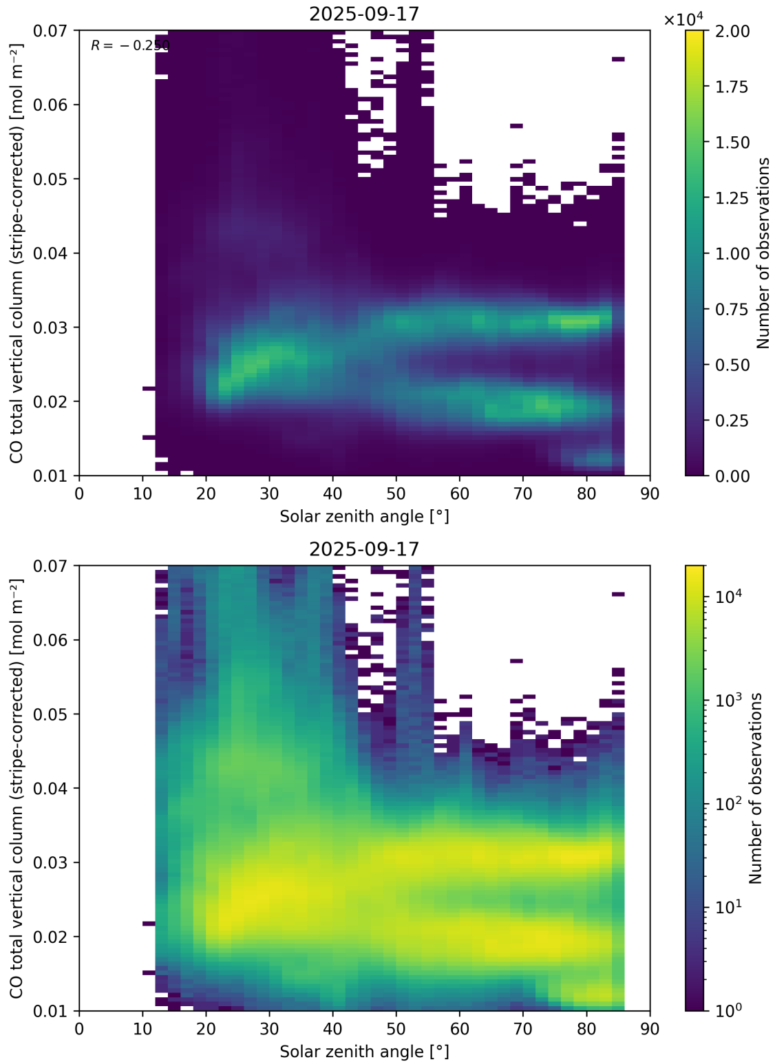
Figure 62: Scatter density plot of “Solar zenith angle” against “CO total vertical column (stripe-corrected)” for 2025-09-16 to 2025-09-18.
