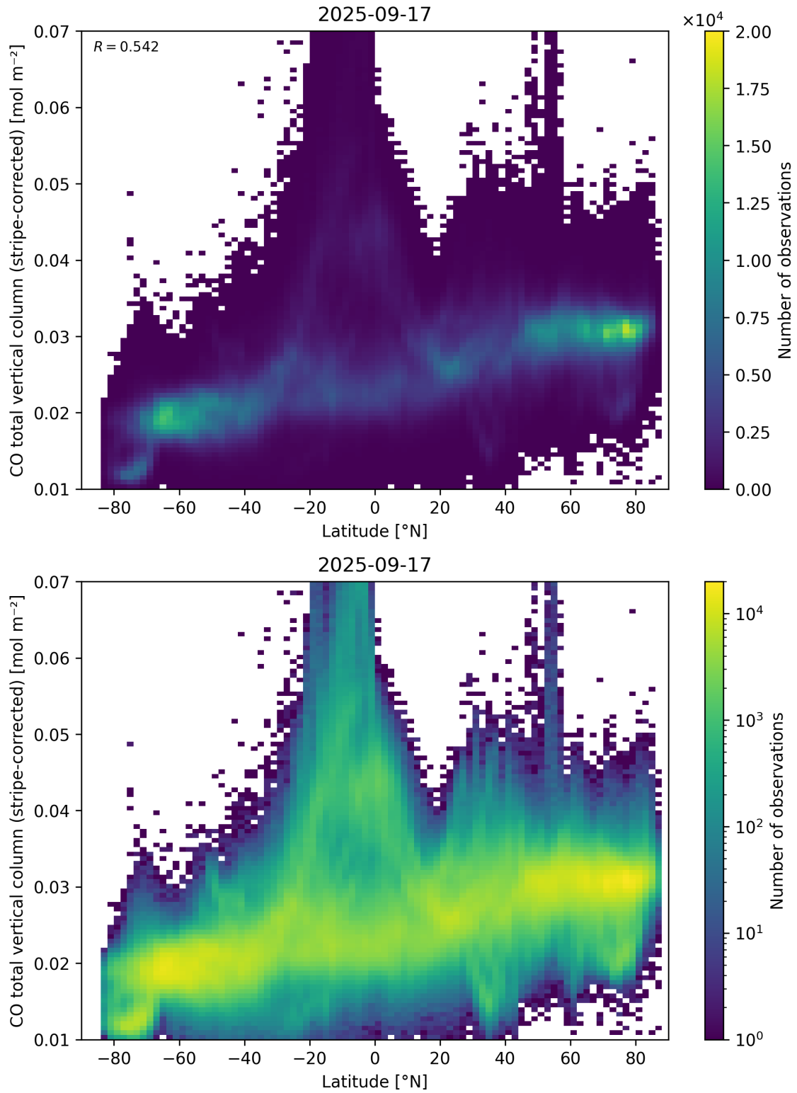
Figure 52: Scatter density plot of “Latitude” against “CO total vertical column (stripe-corrected)” for 2025-09-16 to 2025-09-18.
