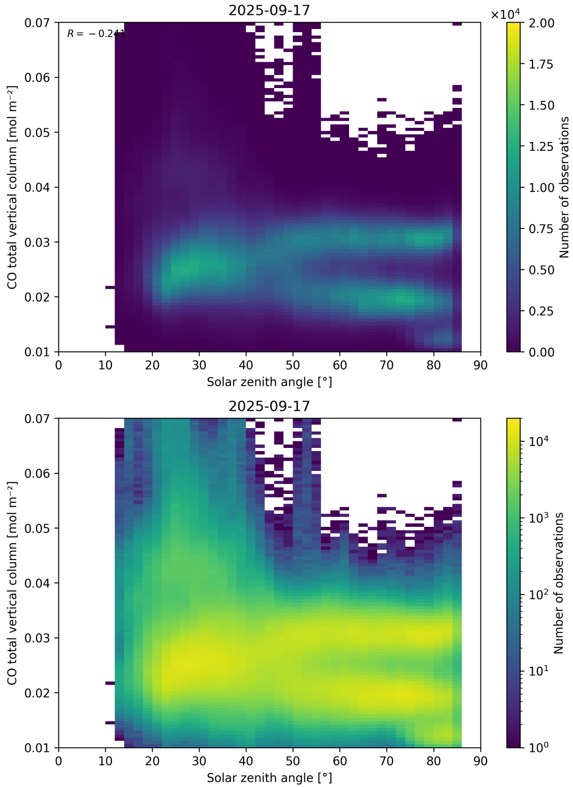
Figure 61: Scatter density plot of “Solar zenith angle” against “CO total vertical column” for 2025-09-16 to 2025-09-18.
