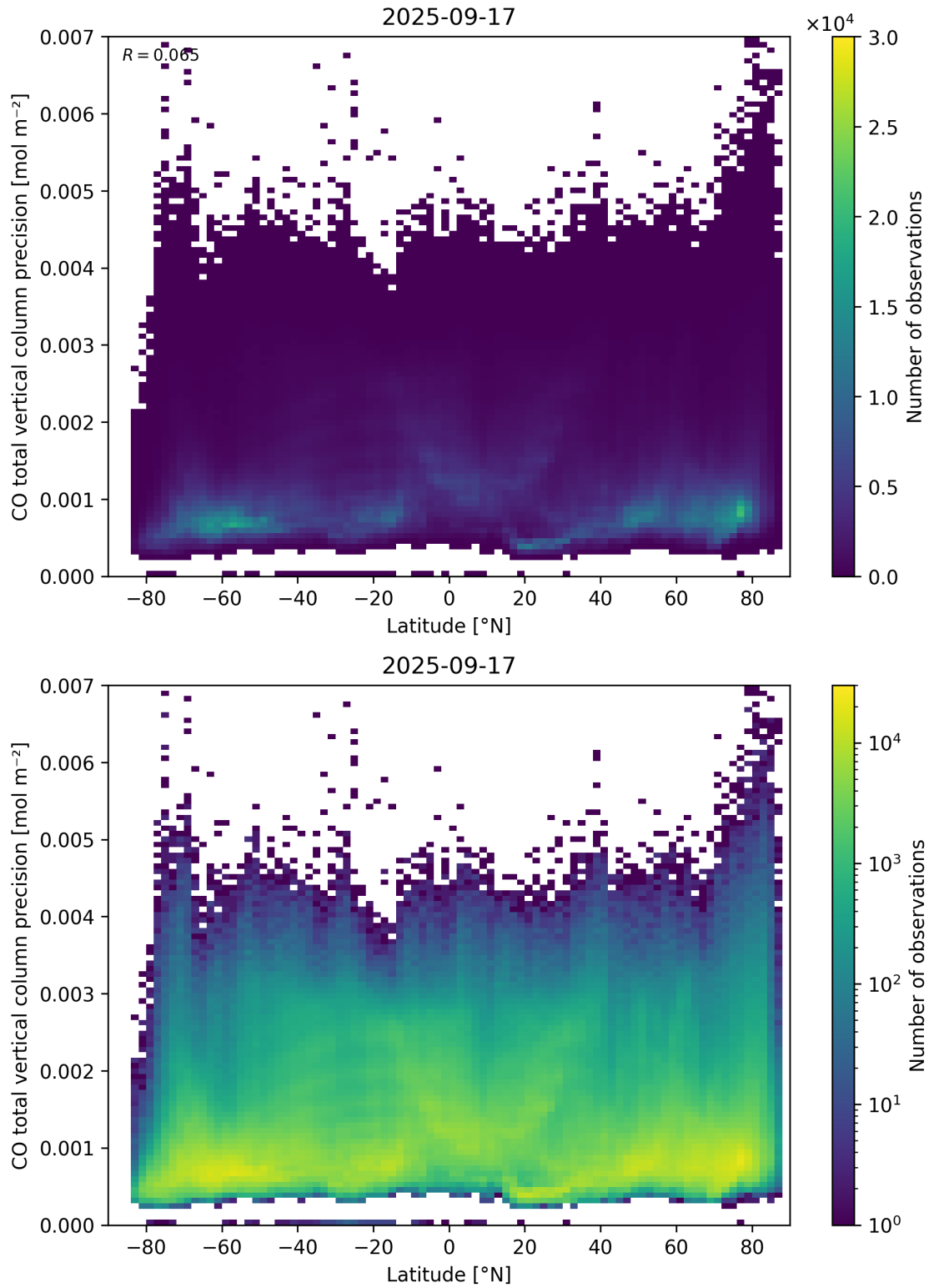
Figure 53: Scatter density plot of “Latitude” against “CO total vertical column precision” for 2025-09-16 to 2025-09-18.
