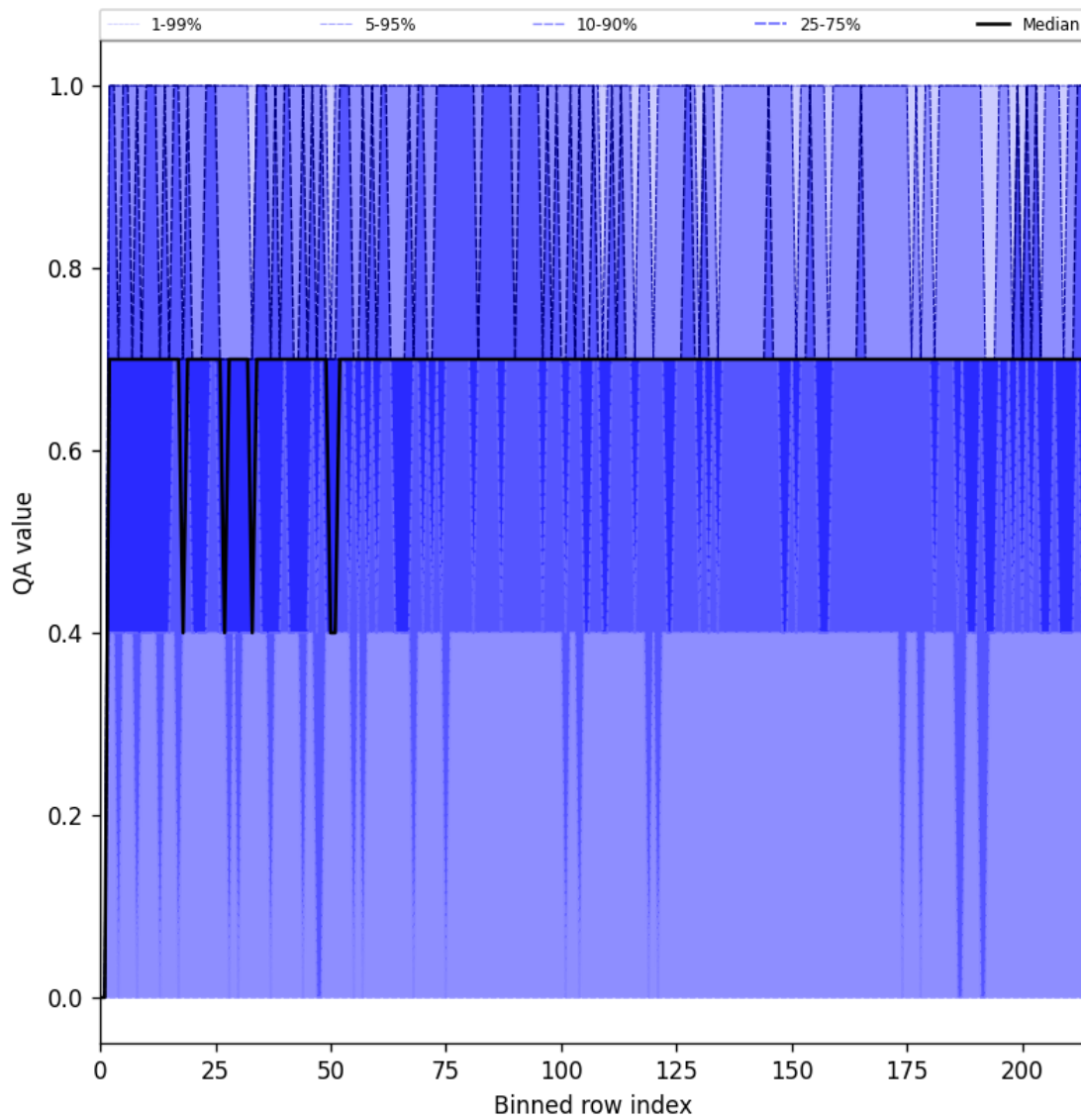
Figure 25: Along track statistics of “QA value” for 2025-09-16 to 2025-09-18
