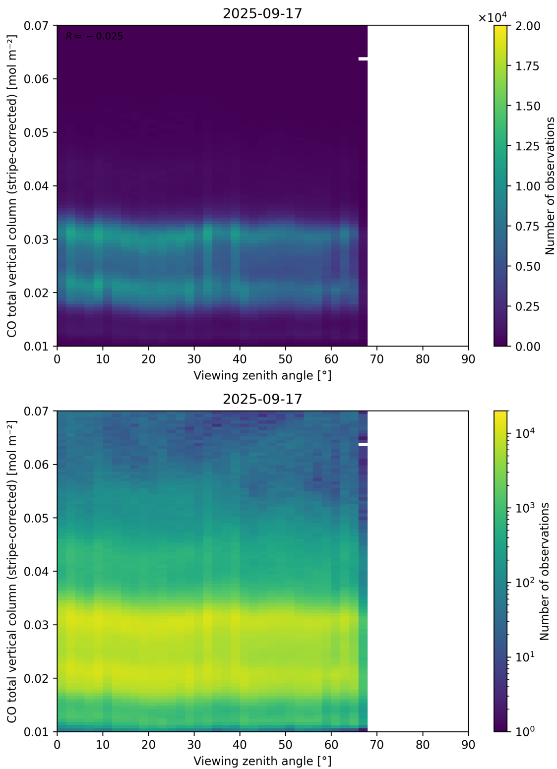
Figure 70: Scatter density plot of “Viewing zenith angle” against “CO total vertical column (stripe-corrected)” for 2025-09-16 to 2025-09-18.
