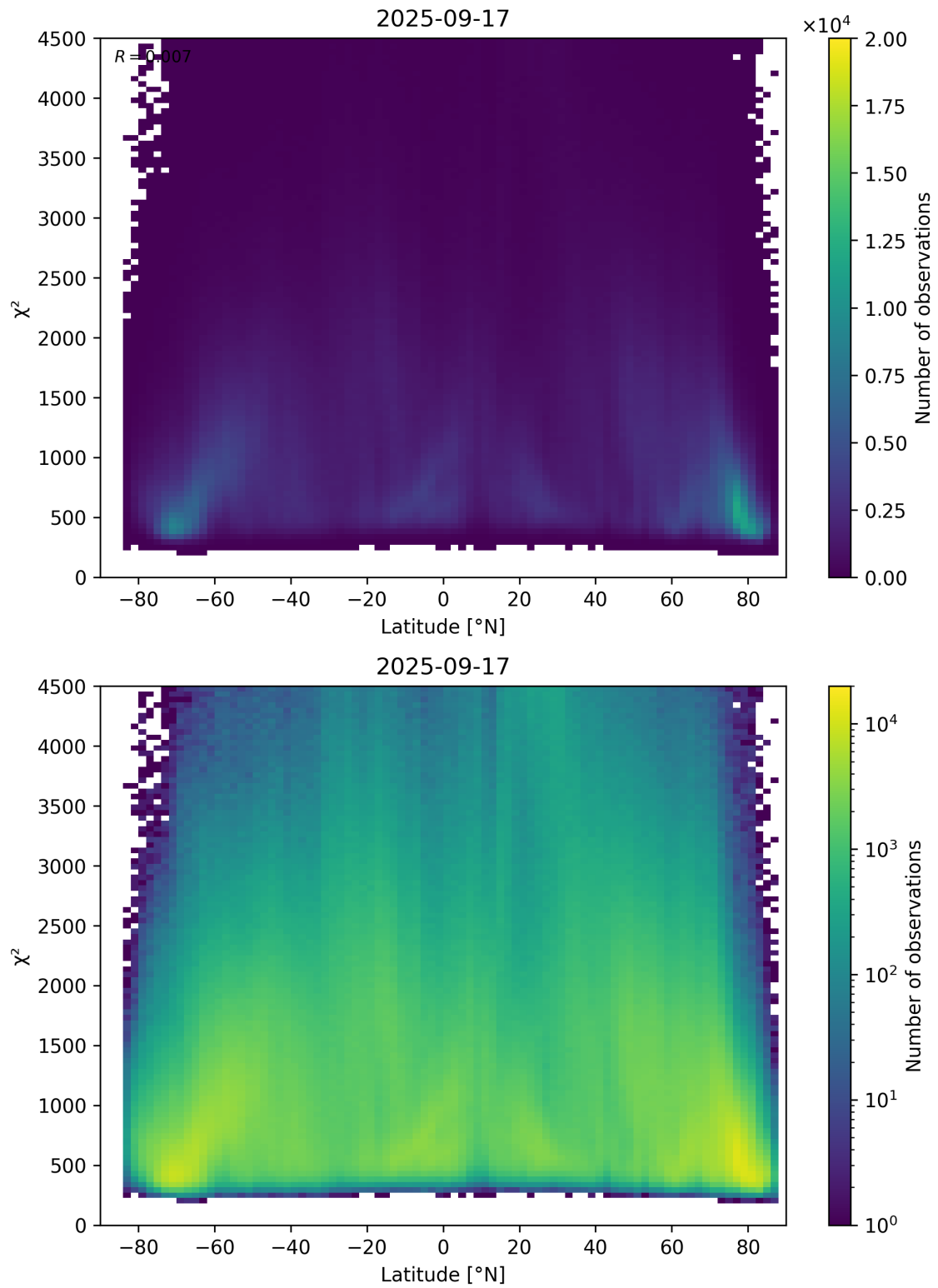
Figure 54: Scatter density plot of “Latitude” against “ \chi^2 ” for 2025-09-16 to 2025-09-18.
