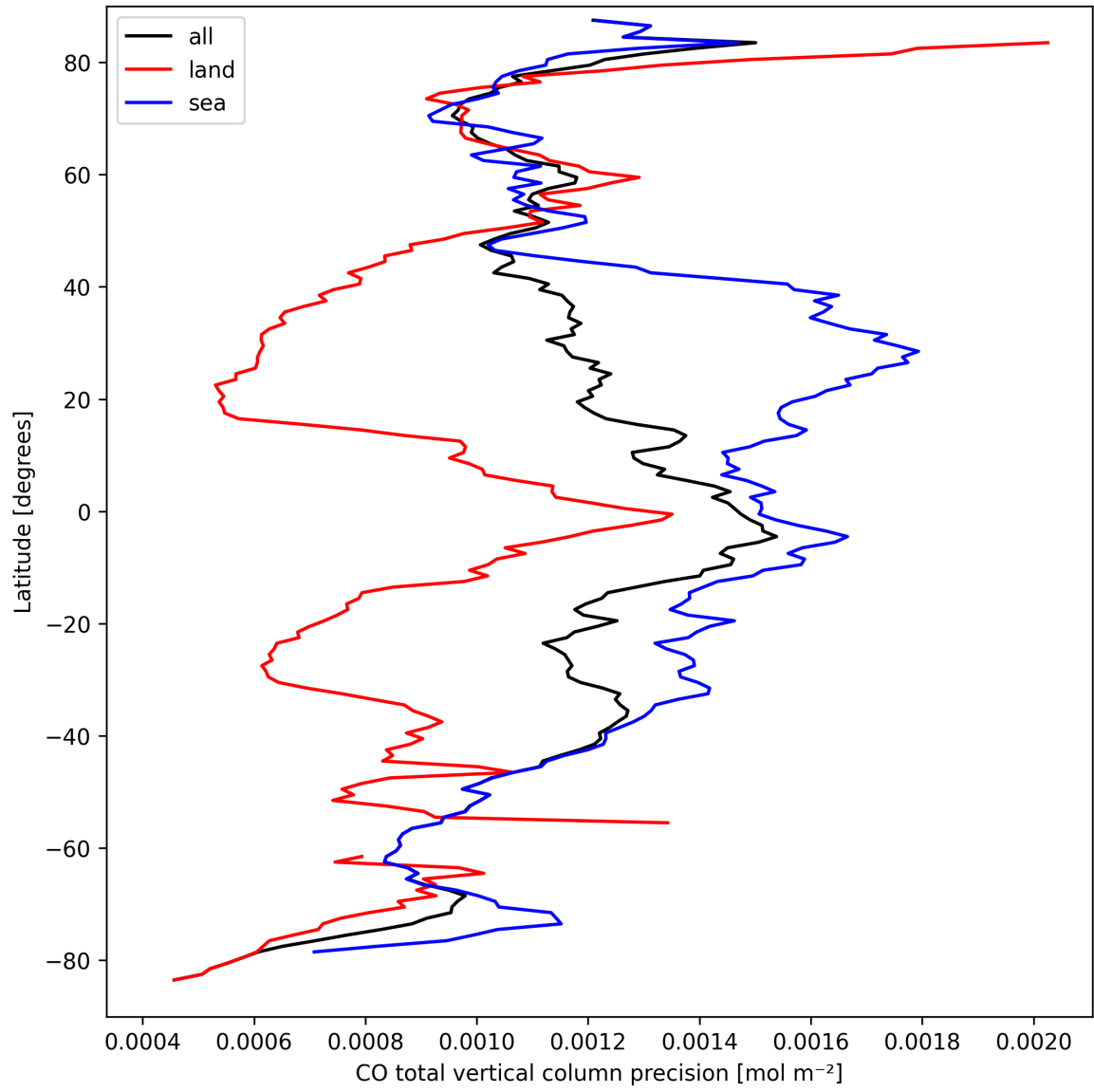
Figure 12: Zonal average of “CO total vertical column precision” for 2025-09-16 to 2025-09-18.
