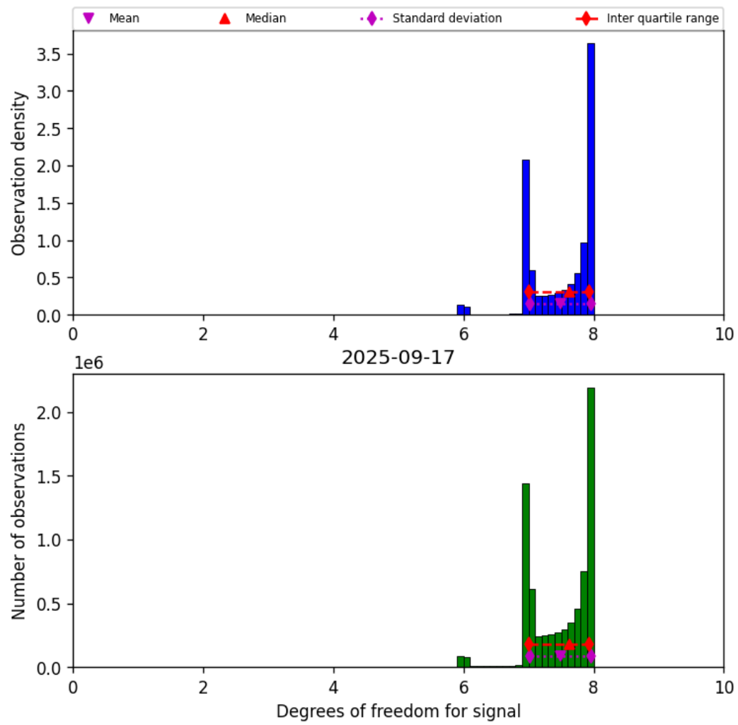
Figure 23: Histogram of “Degrees of freedom for signal” for 2025-09-16 to 2025-09-18
