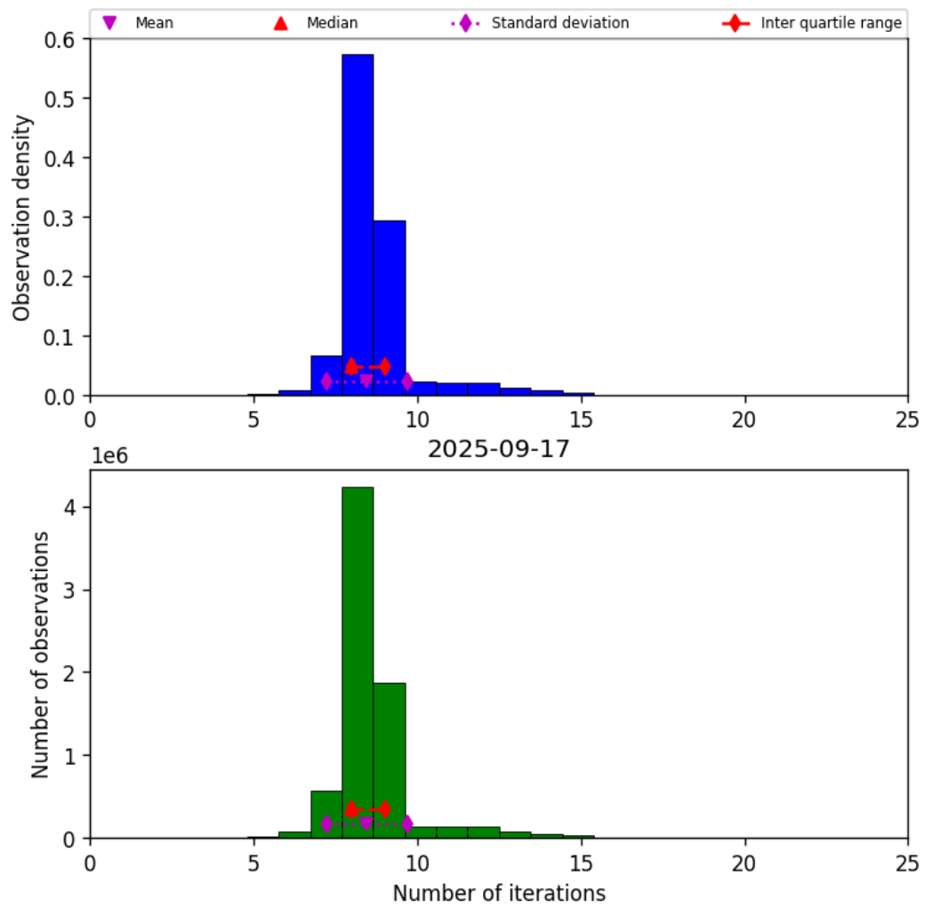
Figure 24: Histogram of “Number of iterations” for 2025-09-16 to 2025-09-18
