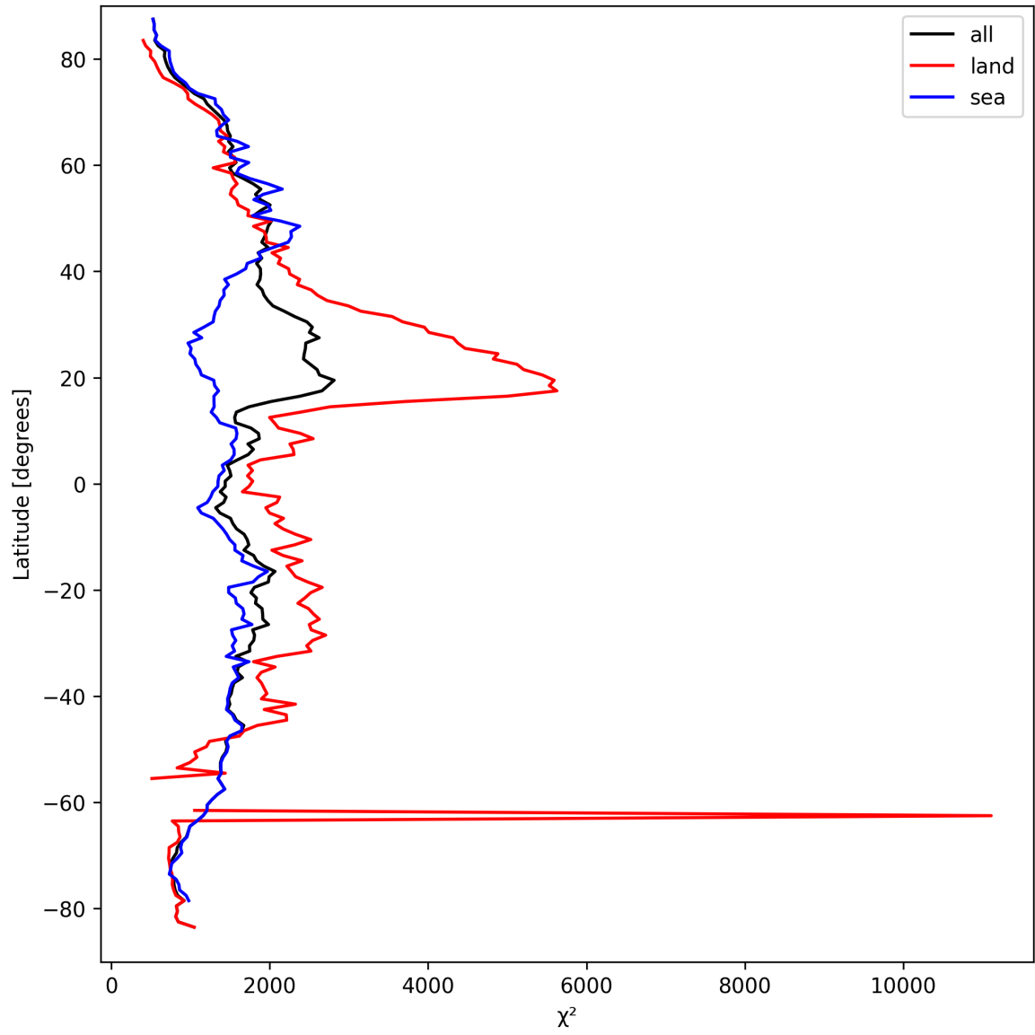
Figure 14: Zonal average of “ \chi^2 ” for 2025-09-16 to 2025-09-18.
