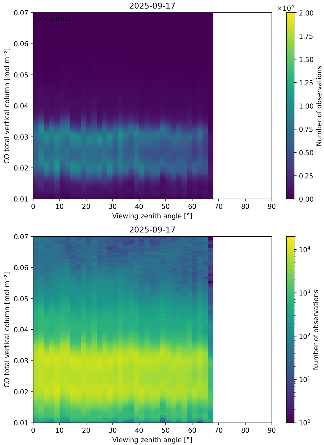
Figure 69: Scatter density plot of “Viewing zenith angle” against “CO total vertical column” for 2025-09-16 to 2025-09-18.
