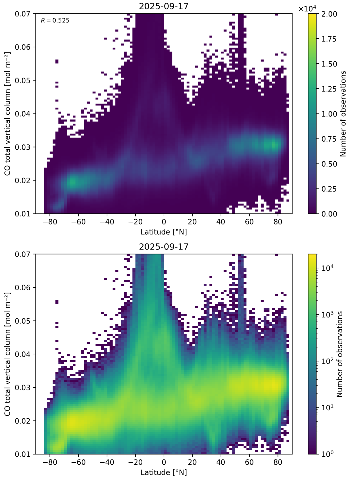
Figure 51: Scatter density plot of “Latitude” against “CO total vertical column” for 2025-09-16 to 2025-09-18.
