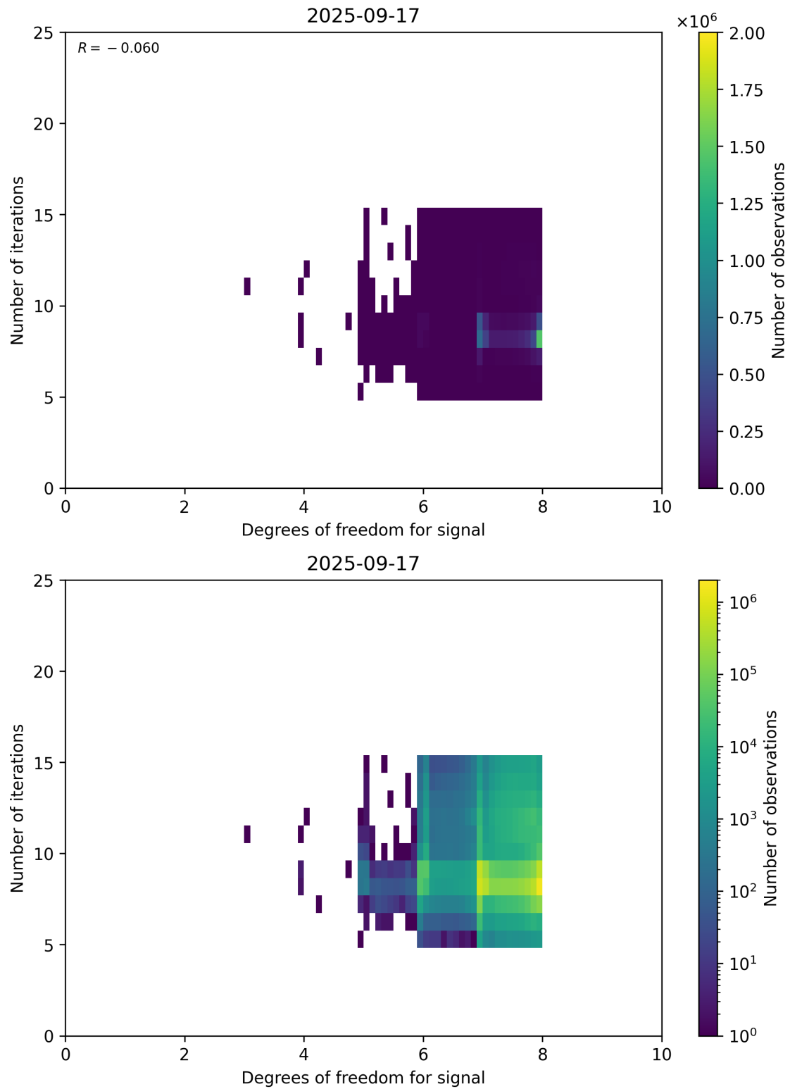
Figure 50: Scatter density plot of “Degrees of freedom for signal” against “Number of iterations” for 2025-09-16 to 2025-09-18.
