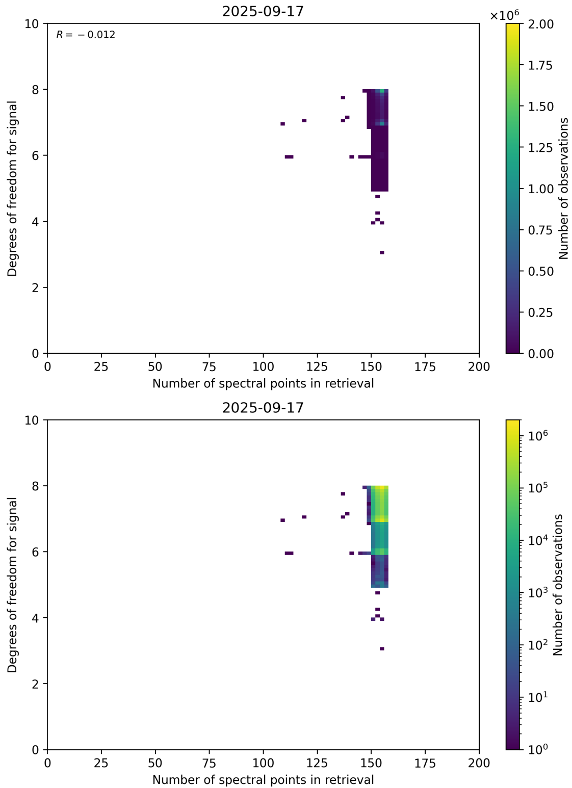
Figure 59: Scatter density plot of “Number of spectral points in retrieval” against “Degrees of freedom for signal” for 2025-09-16 to 2025-09-18.
