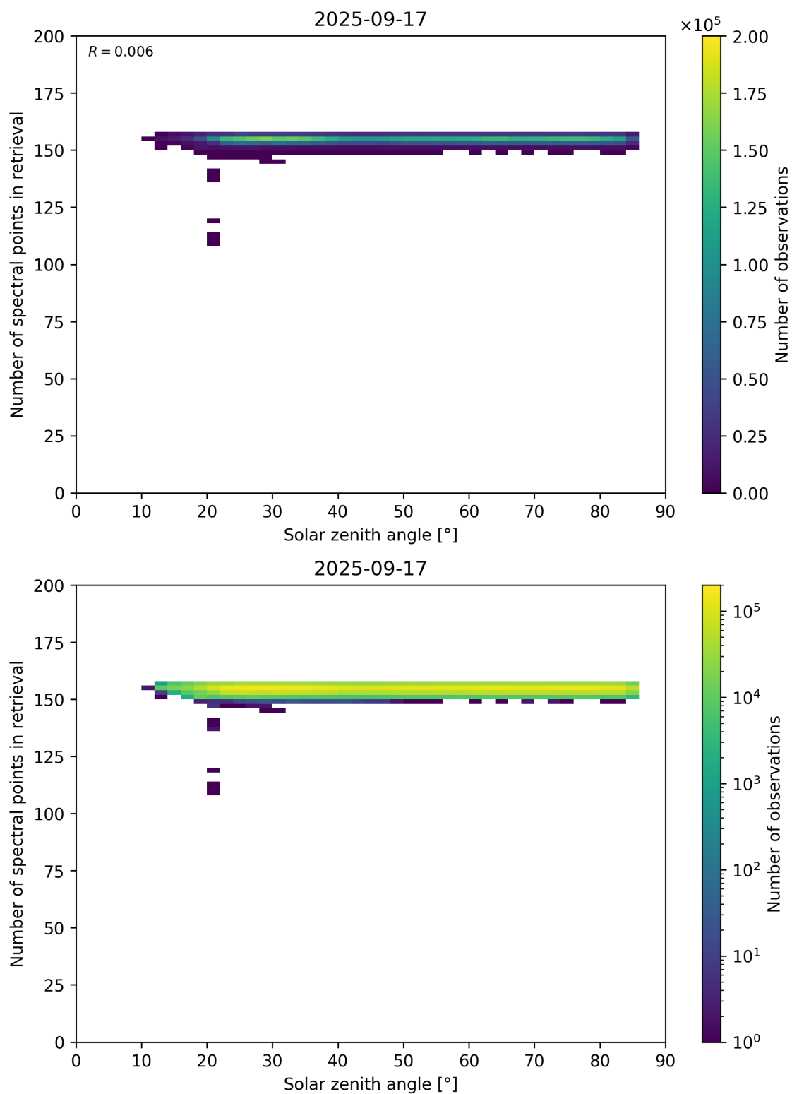
Figure 68: Scatter density plot of “Solar zenith angle” against “Number of spectral points in retrieval” for 2025-09-16 to 2025-09-18.
