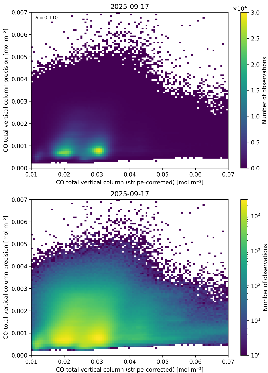
Figure 36: Scatter density plot of “CO total vertical column (stripe-corrected)” against “CO total vertical column precision” for 2025-09-16 to 2025-09-18.
