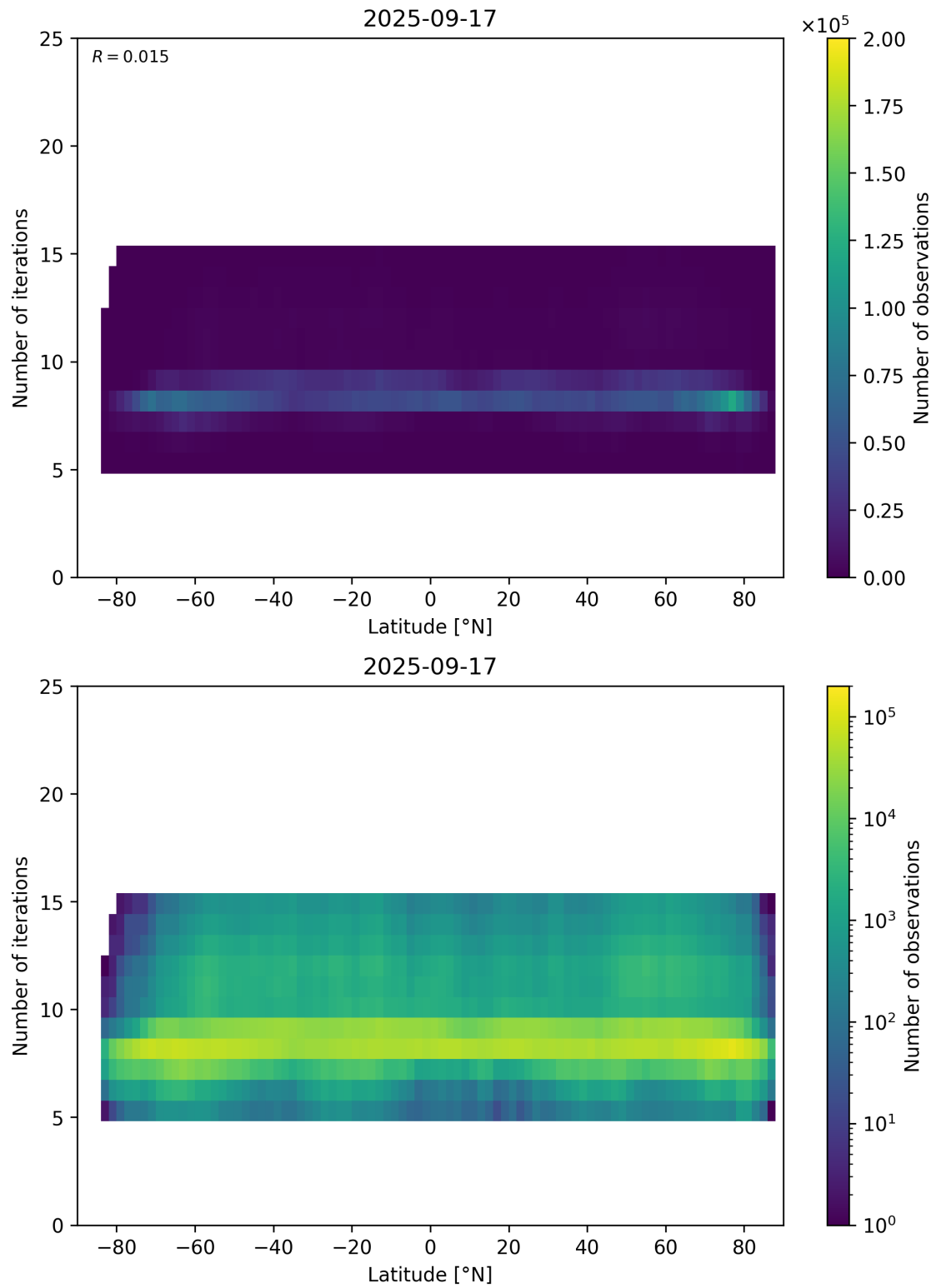
Figure 56: Scatter density plot of “Latitude” against “Number of iterations” for 2025-09-16 to 2025-09-18.
