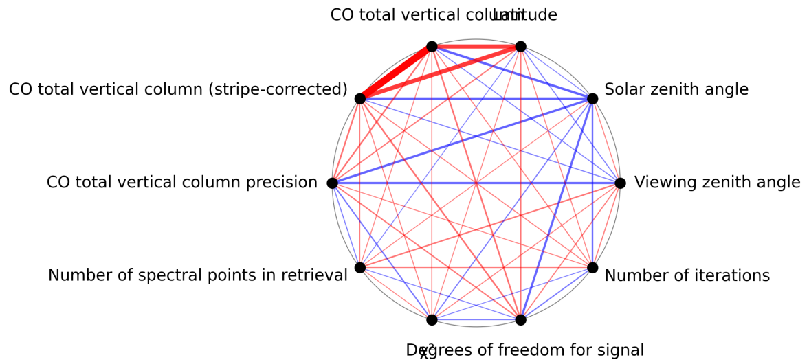
Figure 1: Map of correlation graph for 2025-09-16 to 2025-09-18.
