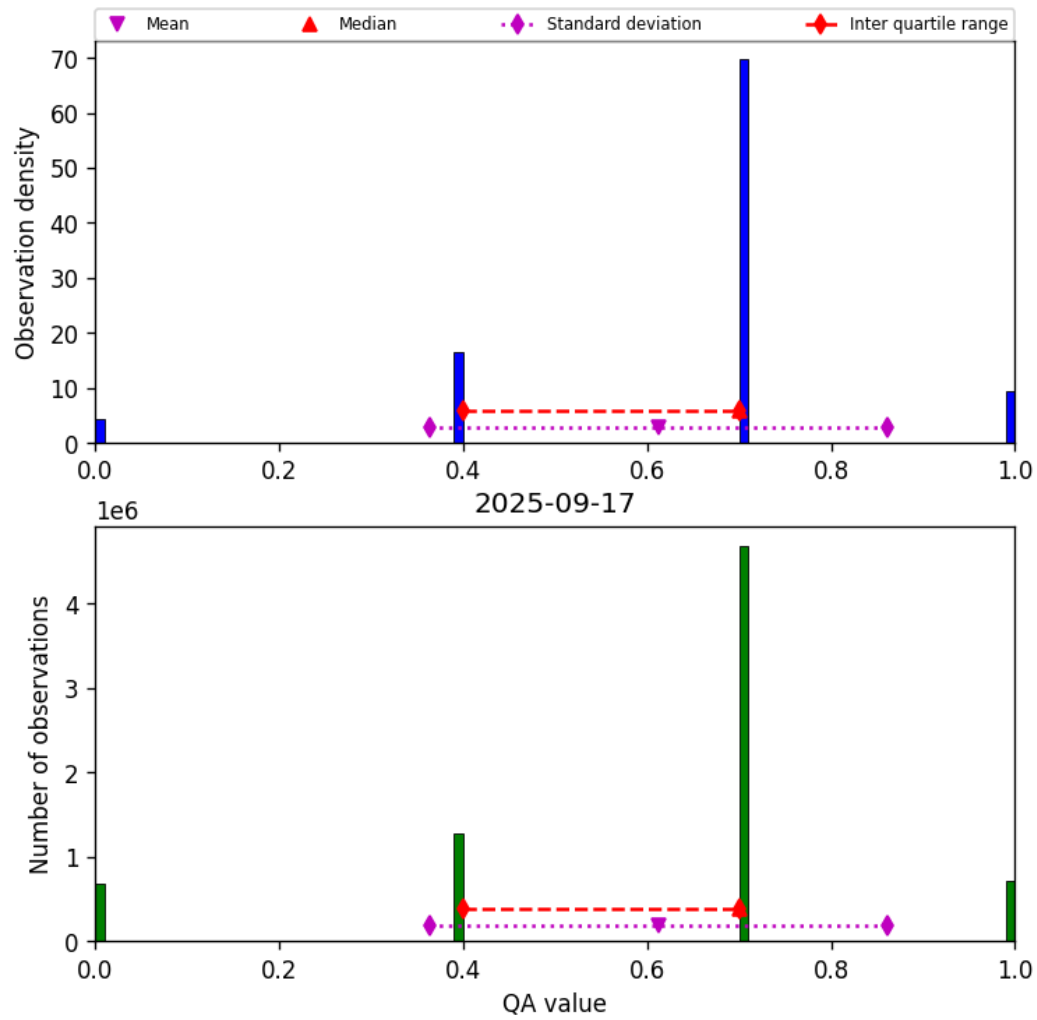
Figure 17: Histogram of “QA value” for 2025-09-16 to 2025-09-18
