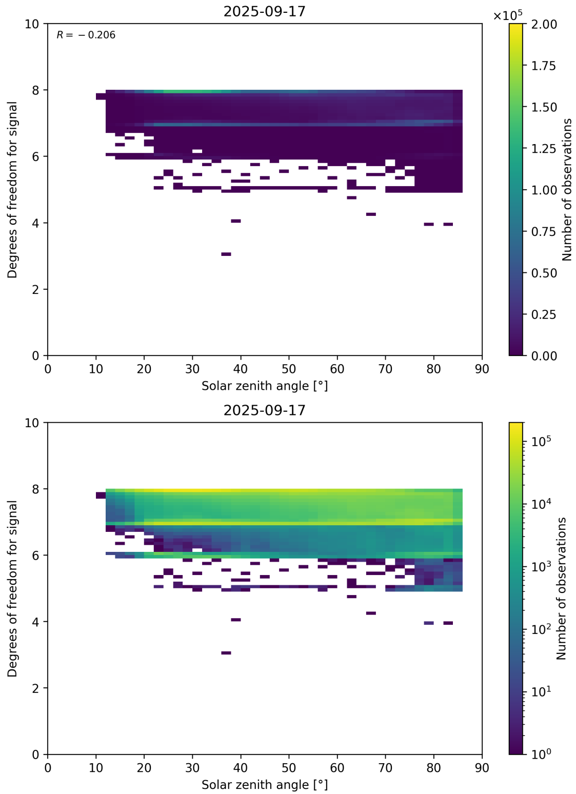
Figure 65: Scatter density plot of “Solar zenith angle” against “Degrees of freedom for signal” for 2025-09-16 to 2025-09-18.
