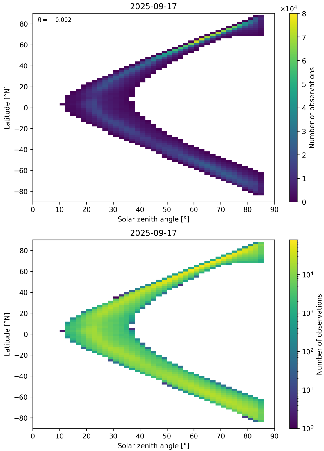
Figure 66: Scatter density plot of “Solar zenith angle” against “Latitude” for 2025-09-16 to 2025-09-18.
