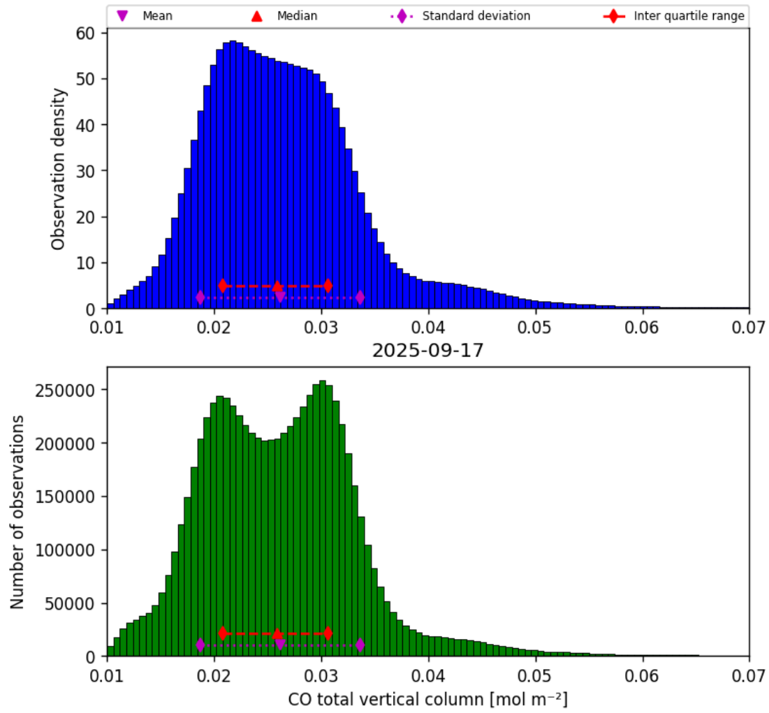
Figure 18: Histogram of “CO total vertical column” for 2025-09-16 to 2025-09-18
