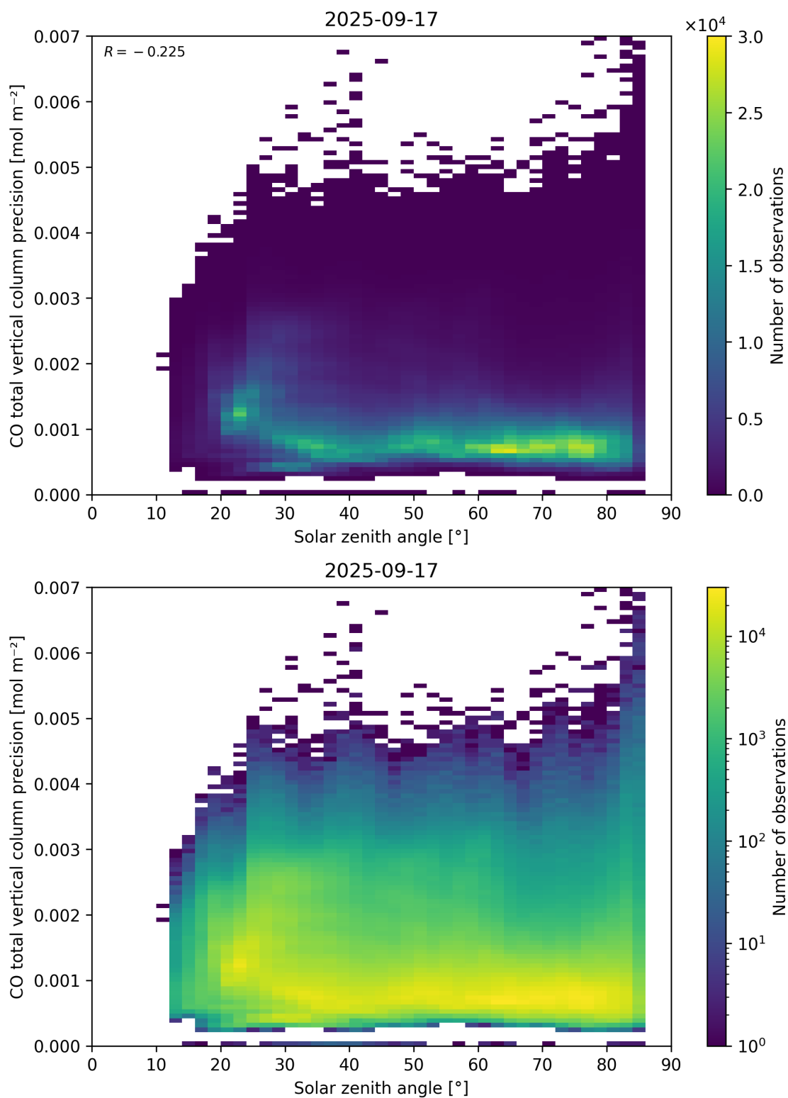
Figure 63: Scatter density plot of “Solar zenith angle” against “CO total vertical column precision” for 2025-09-16 to 2025-09-18.
