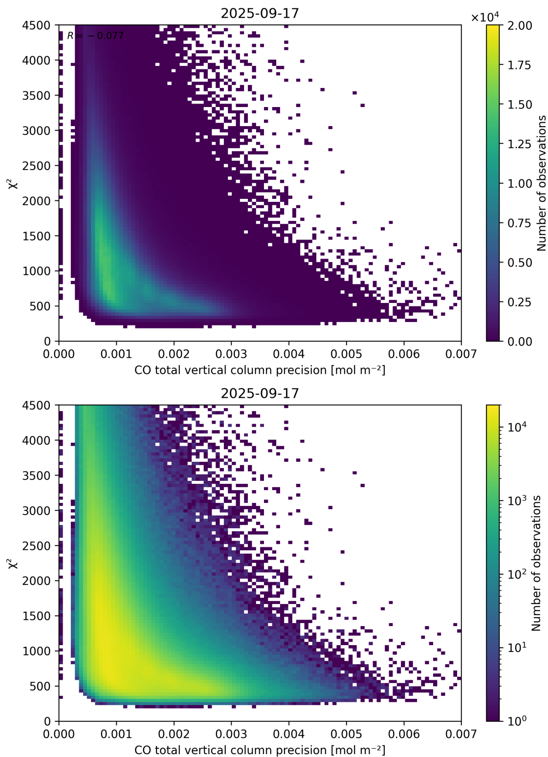
Figure 44: Scatter density plot of “CO total vertical column precision” against “ \chi^2 ” for 2025-09-16 to 2025-09-18.
