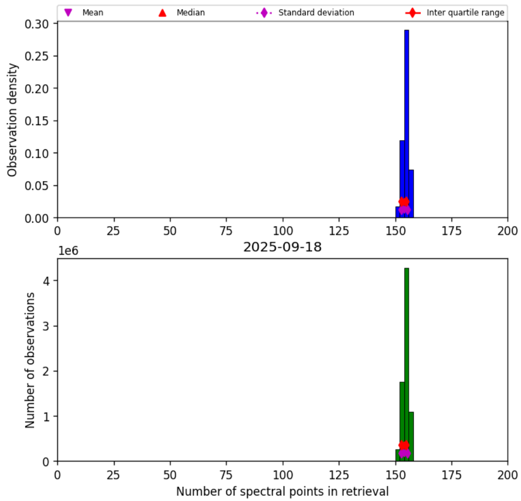
Figure 21: Histogram of “Number of spectral points in retrieval” for 2025-09-17 to 2025-09-19
