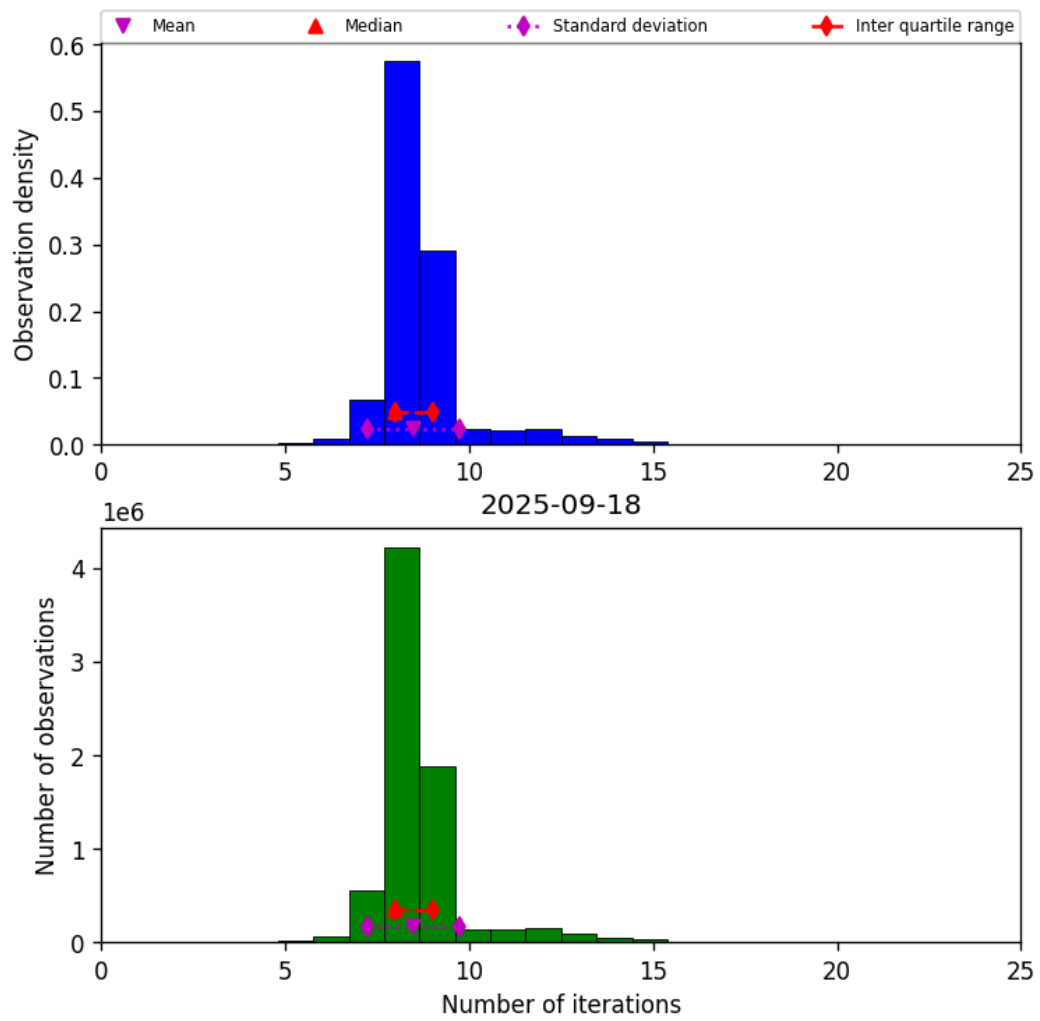
Figure 24: Histogram of “Number of iterations” for 2025-09-17 to 2025-09-19
