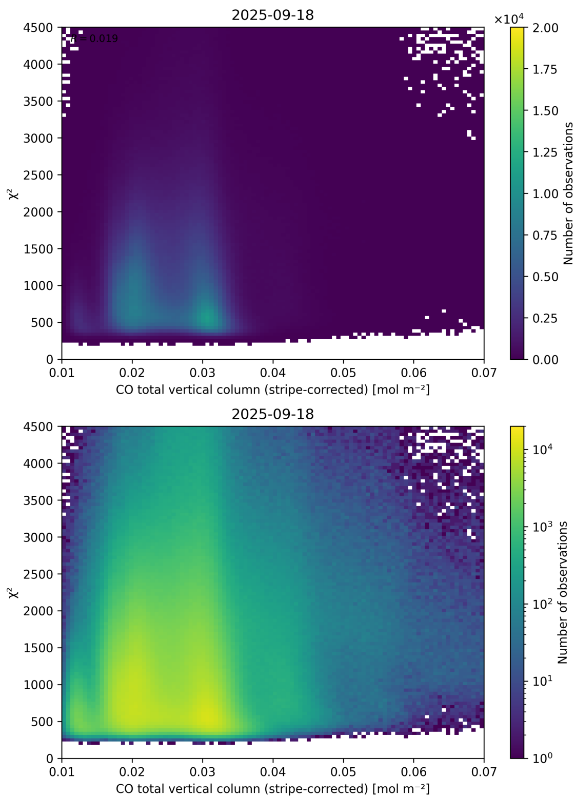
Figure 37: Scatter density plot of “CO total vertical column (stripe-corrected)” against “ \chi^2 ” for 2025-09-17 to 2025-09-19.
