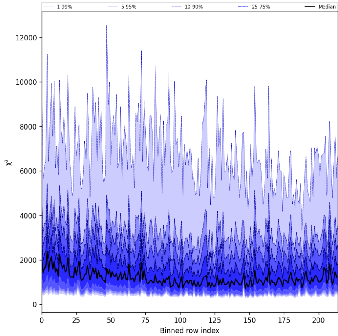
Figure 30: Along track statistics of “ \chi^2 ” for 2025-09-17 to 2025-09-19
