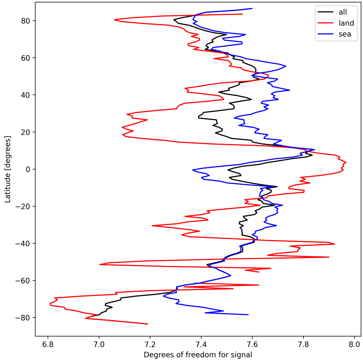
Figure 15: Zonal average of “Degrees of freedom for signal” for 2025-09-17 to 2025-09-19.
