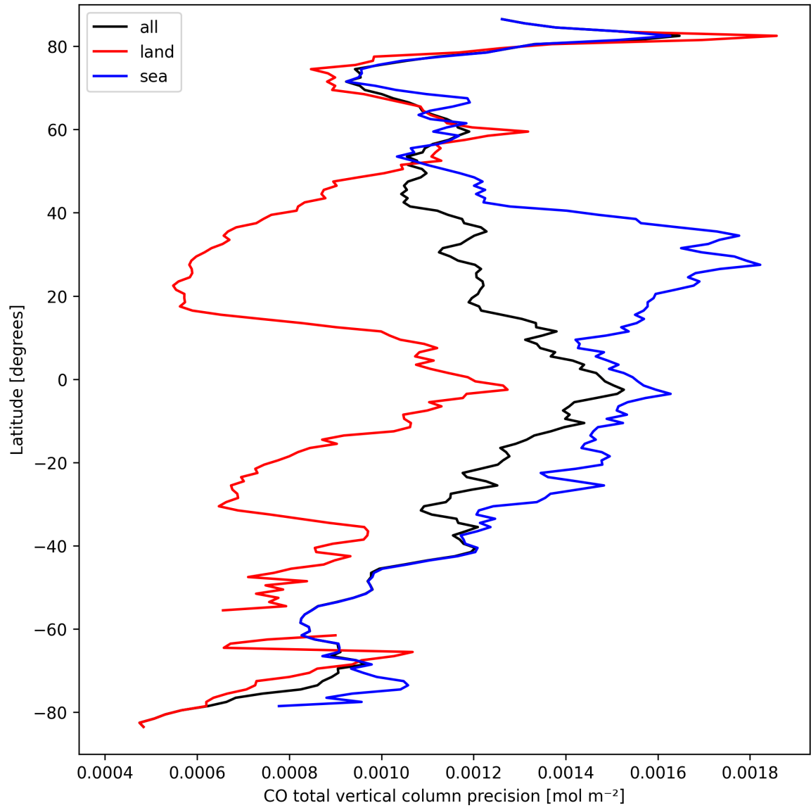
Figure 12: Zonal average of “CO total vertical column precision” for 2025-09-17 to 2025-09-19.
