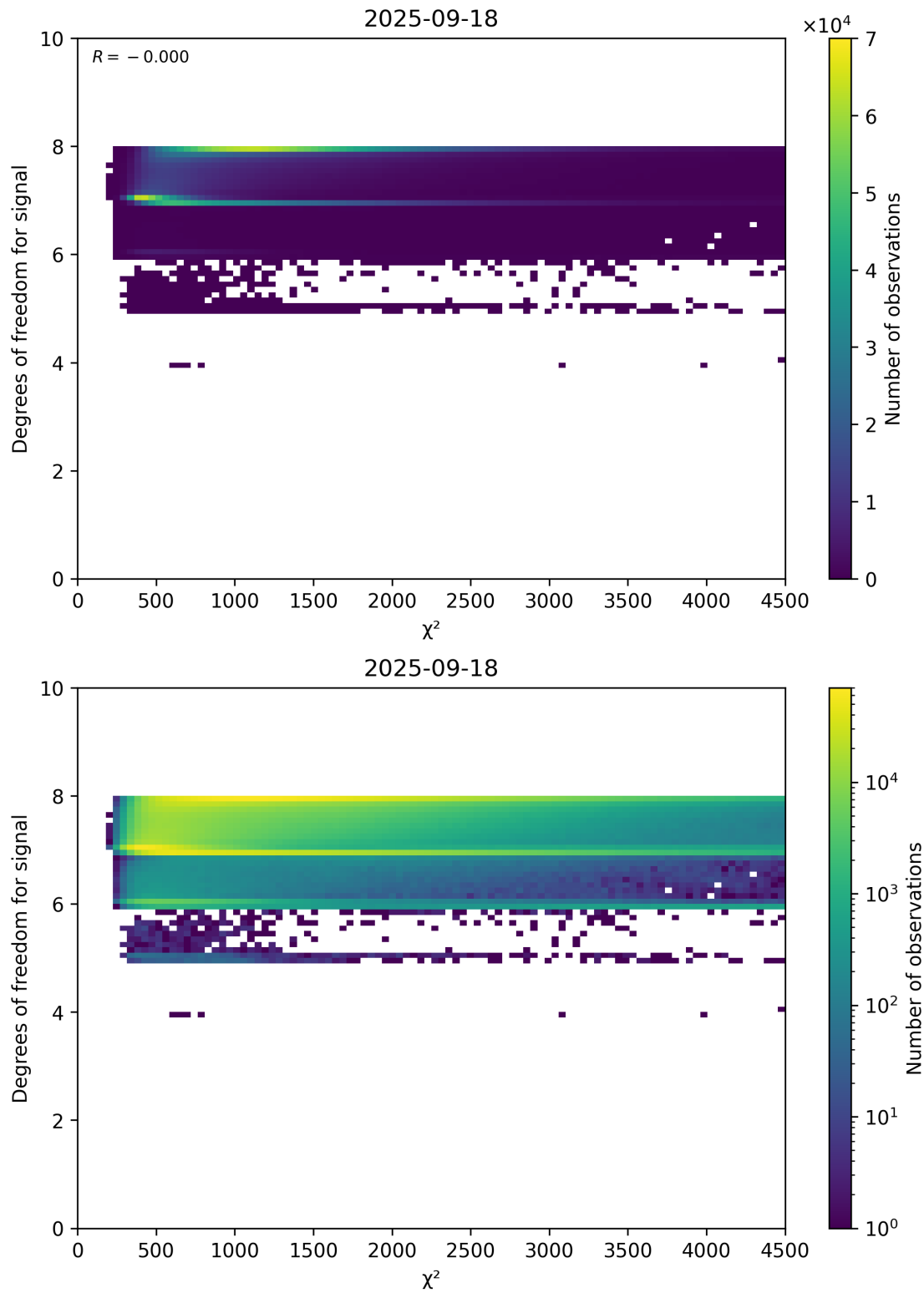
Figure 48: Scatter density plot of “ \chi^2 ” against “Degrees of freedom for signal” for 2025-09-17 to 2025-09-19.
