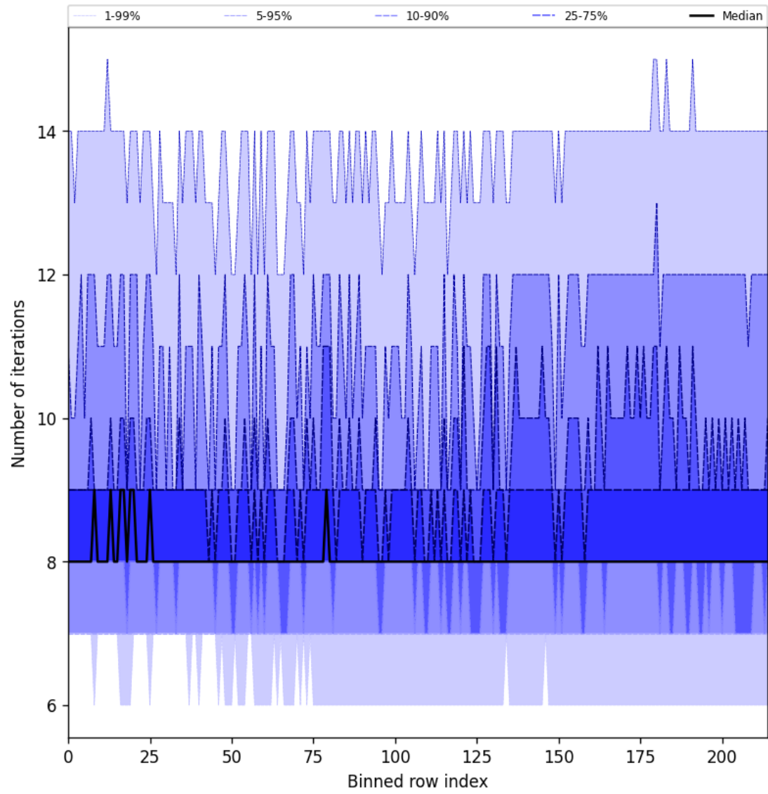
Figure 32: Along track statistics of “Number of iterations” for 2025-09-17 to 2025-09-19
