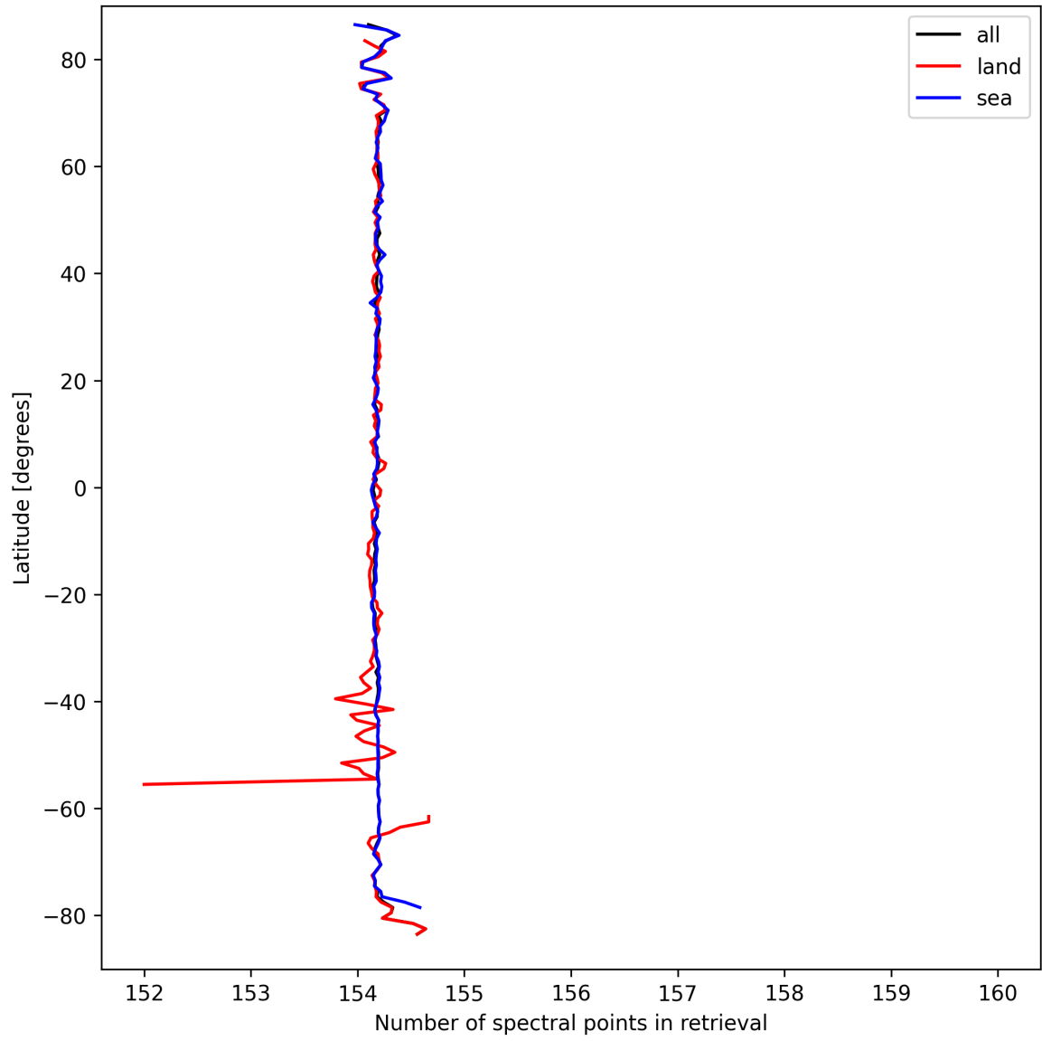
Figure 13: Zonal average of “Number of spectral points in retrieval” for 2025-09-17 to 2025-09-19.
