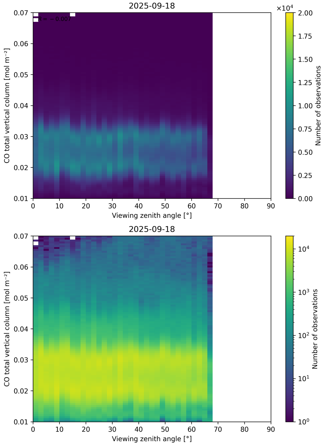
Figure 69: Scatter density plot of “Viewing zenith angle” against “CO total vertical column” for 2025-09-17 to 2025-09-19.
