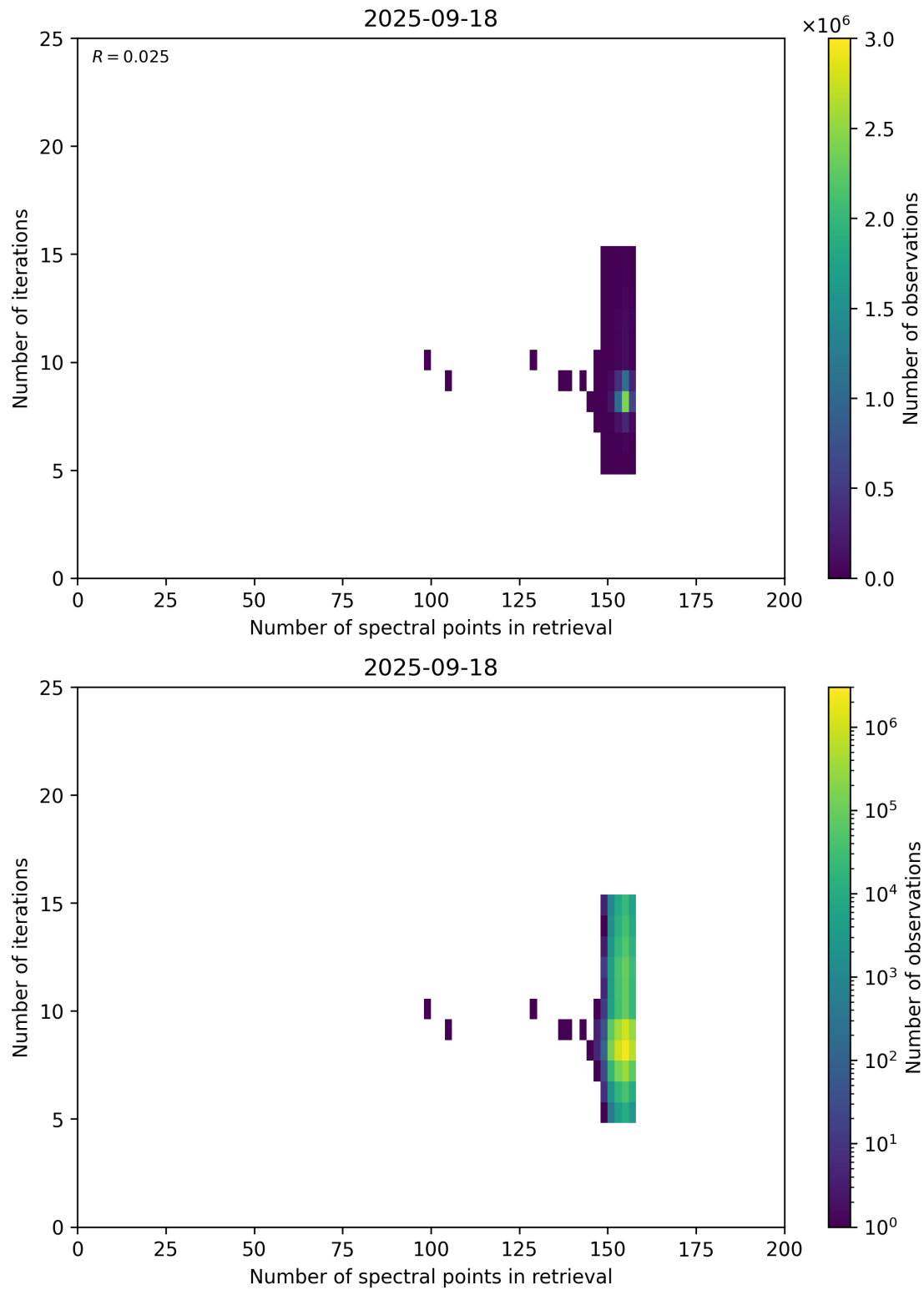
Figure 60: Scatter density plot of “Number of spectral points in retrieval” against “Number of iterations” for 2025-09-17 to 2025-09-19.
