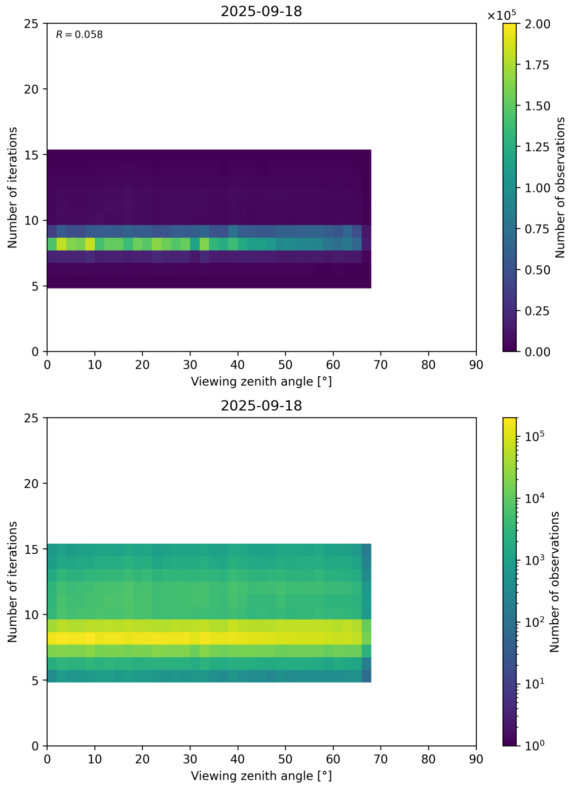
Figure 75: Scatter density plot of “Viewing zenith angle” against “Number of iterations” for 2025-09-17 to 2025-09-19.
