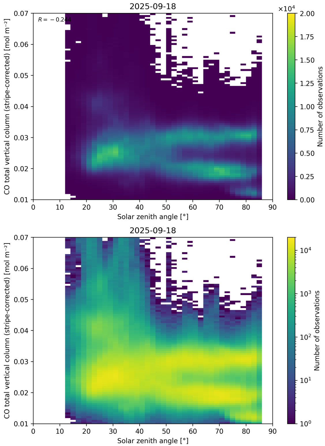
Figure 62: Scatter density plot of “Solar zenith angle” against “CO total vertical column (stripe-corrected)” for 2025-09-17 to 2025-09-19.
