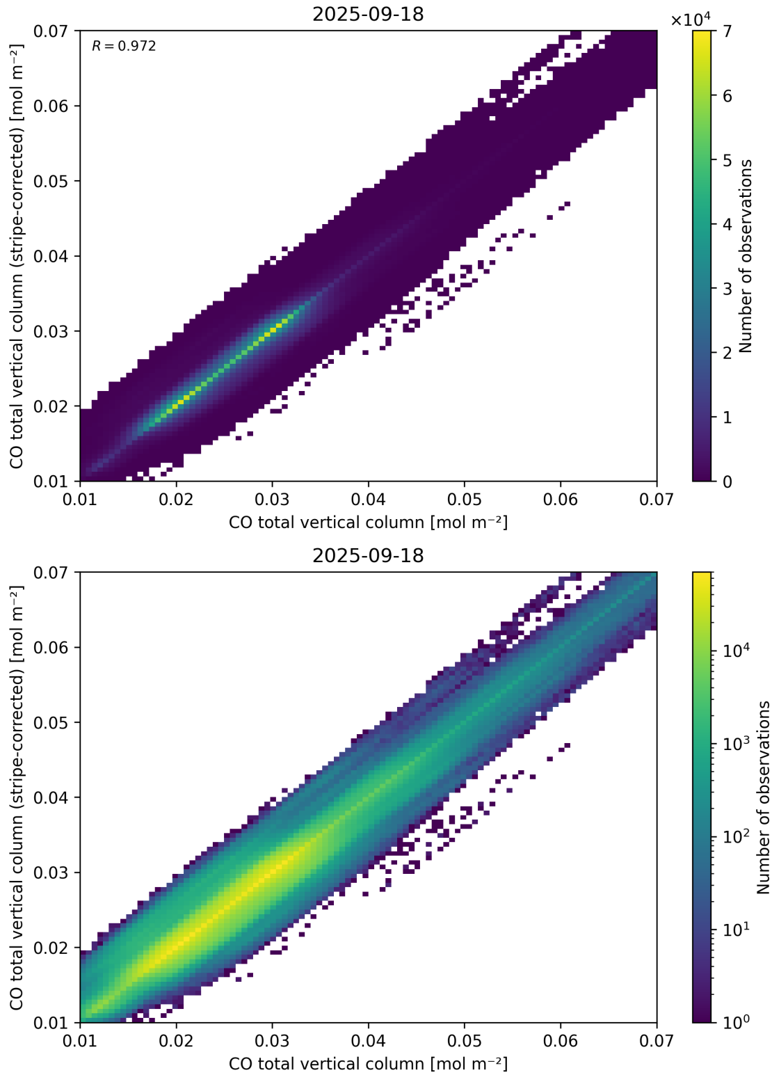
Figure 33: Scatter density plot of “CO total vertical column” against “CO total vertical column (stripe-corrected)” for 2025-09-17 to 2025-09-19.
