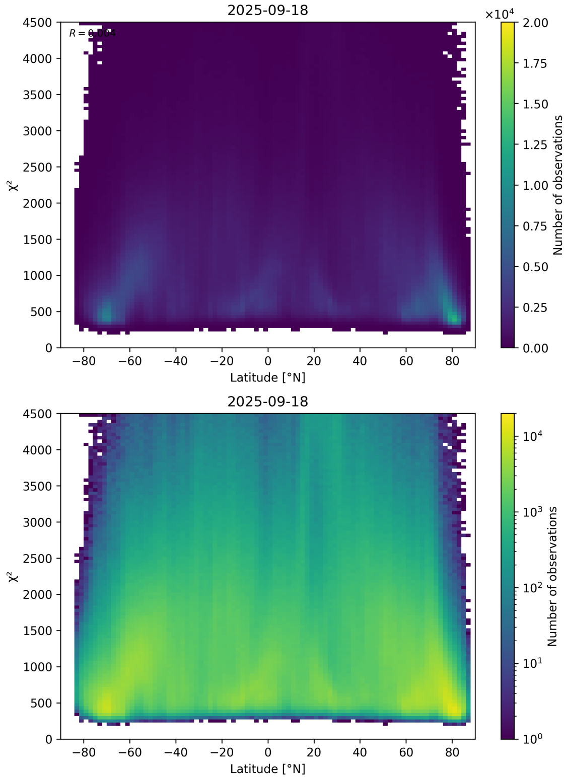
Figure 54: Scatter density plot of “Latitude” against “ \chi^2 ” for 2025-09-17 to 2025-09-19.
