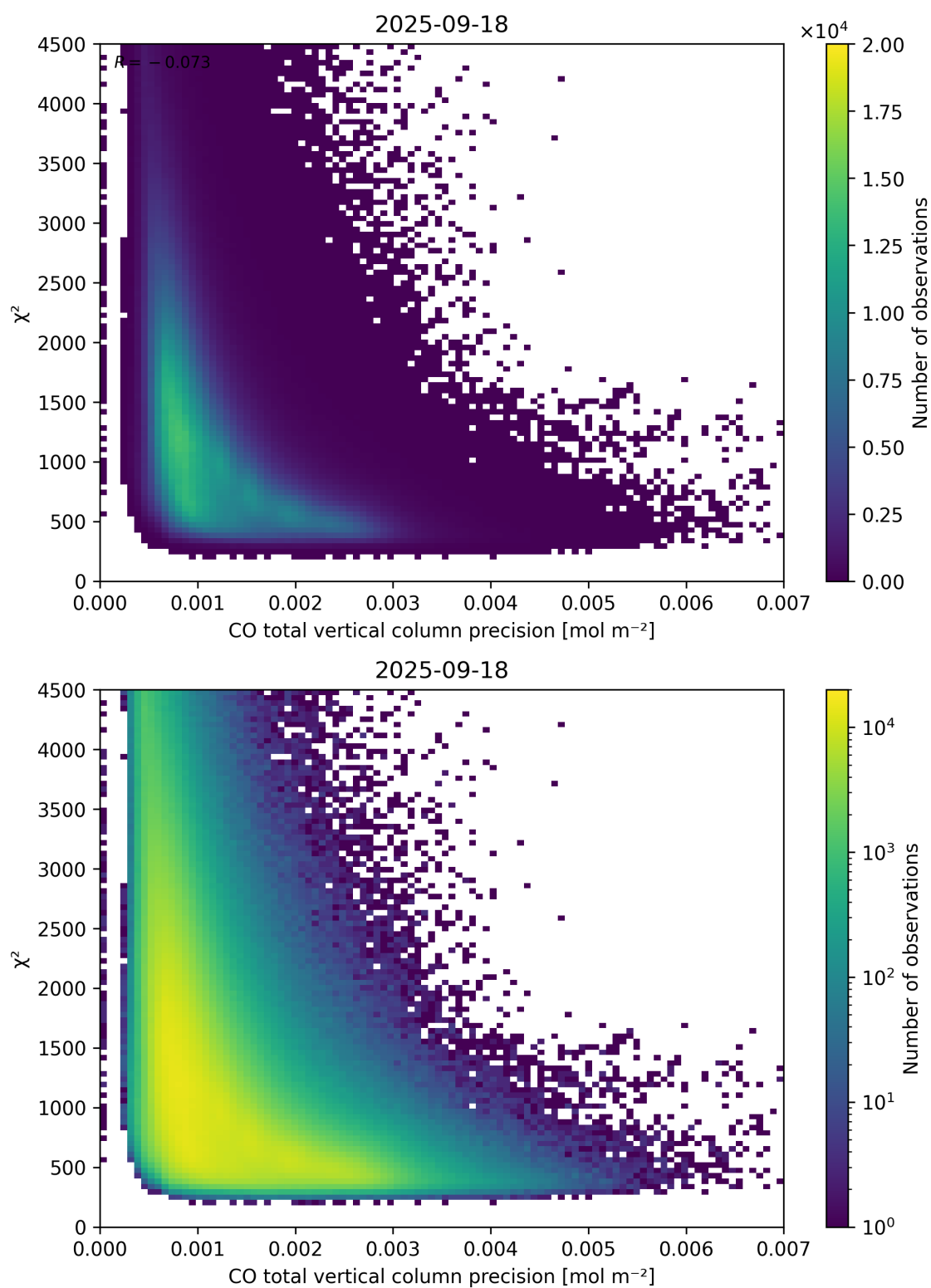
Figure 44: Scatter density plot of “CO total vertical column precision” against “ \chi^2 ” for 2025-09-17 to 2025-09-19.
