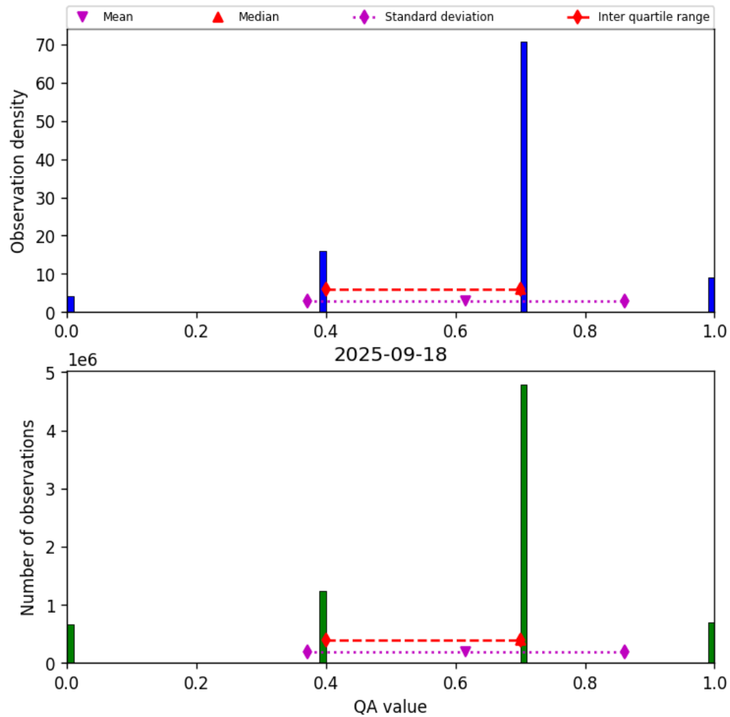
Figure 17: Histogram of “QA value” for 2025-09-17 to 2025-09-19
