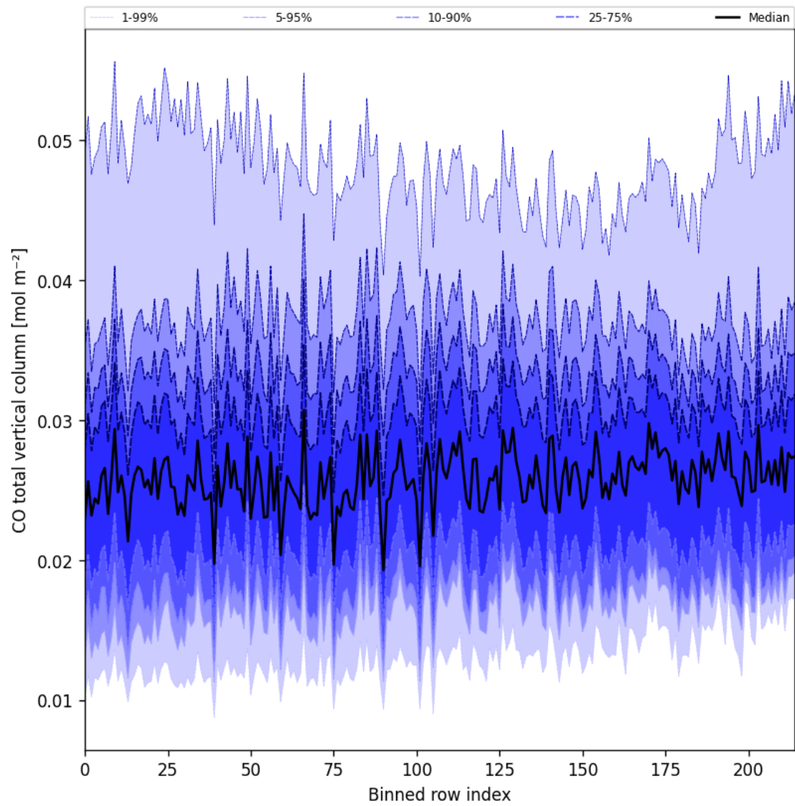
Figure 26: Along track statistics of “CO total vertical column” for 2025-09-17 to 2025-09-19
