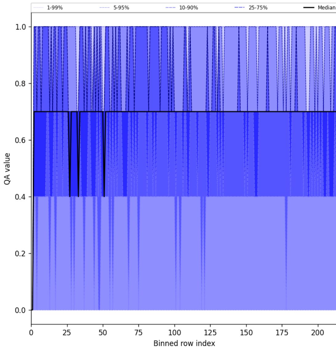
Figure 25: Along track statistics of “QA value” for 2025-09-17 to 2025-09-19
