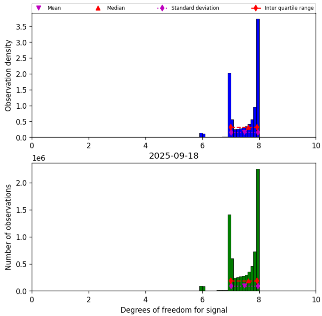
Figure 23: Histogram of “Degrees of freedom for signal” for 2025-09-17 to 2025-09-19
