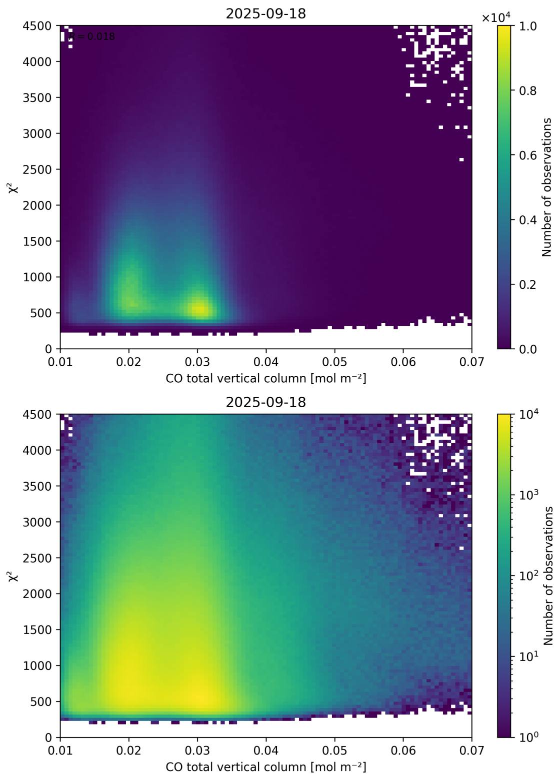
Figure 35: Scatter density plot of “CO total vertical column” against “ \chi^2 ” for 2025-09-17 to 2025-09-19.
