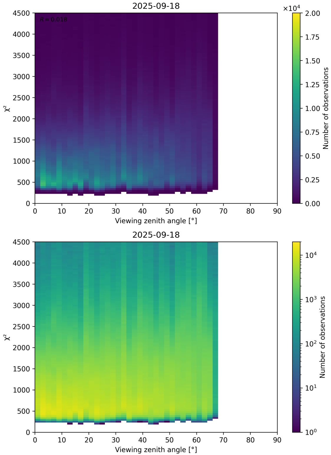
Figure 72: Scatter density plot of “Viewing zenith angle” against “ \chi^2 ” for 2025-09-17 to 2025-09-19.
