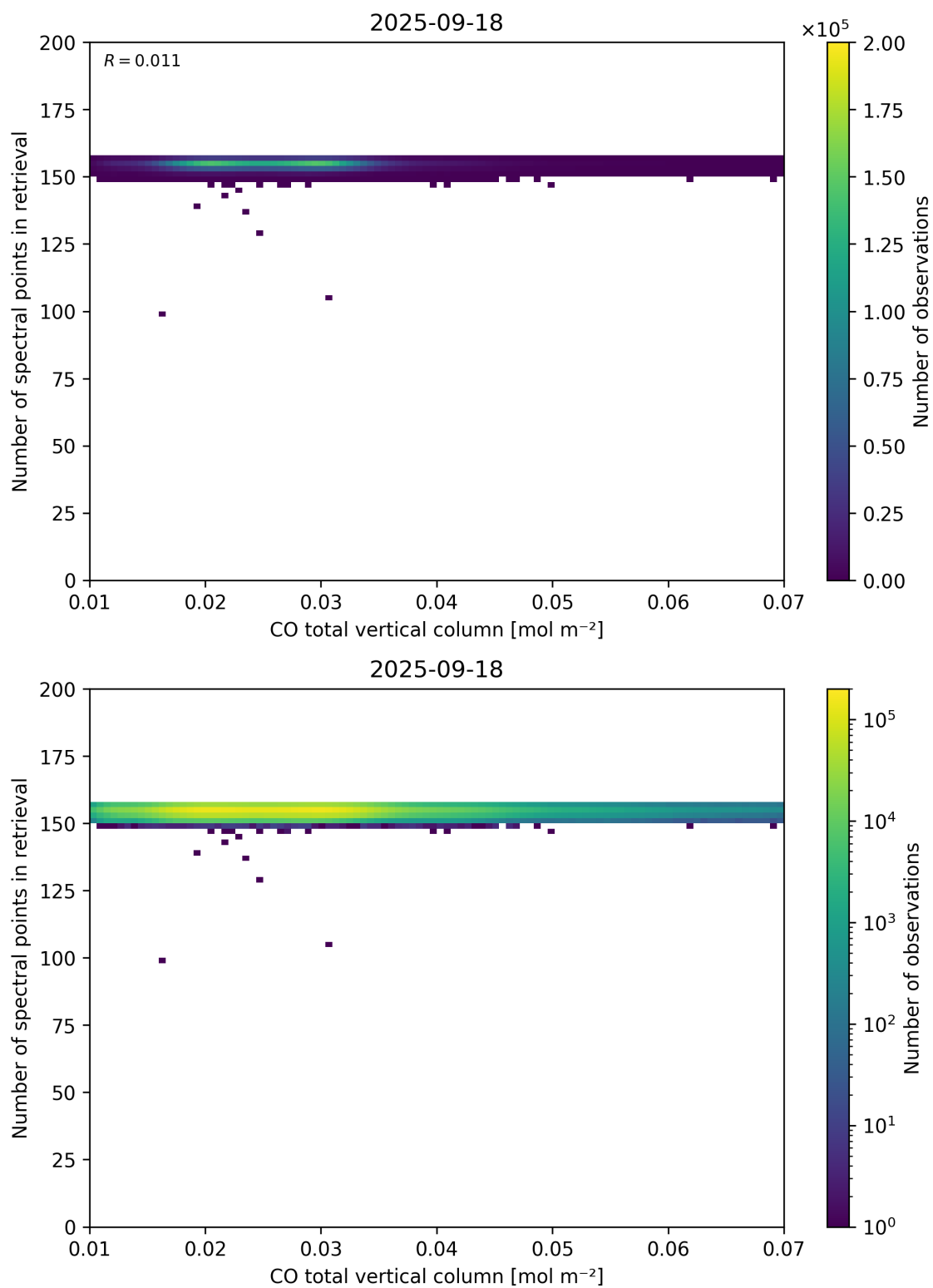
Figure 43: Scatter density plot of “CO total vertical column” against “Number of spectral points in retrieval” for 2025-09-17 to 2025-09-19.
