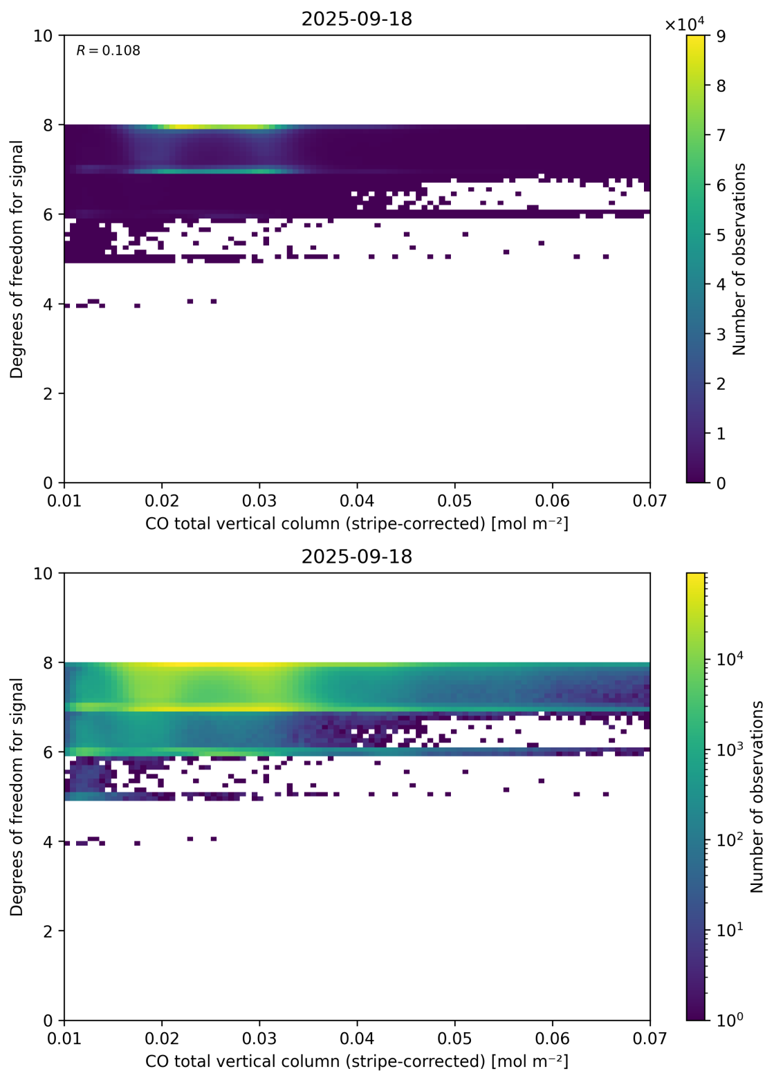
Figure 38: Scatter density plot of “CO total vertical column (stripe-corrected)” against “Degrees of freedom for signal” for 2025-09-17 to 2025-09-19.
