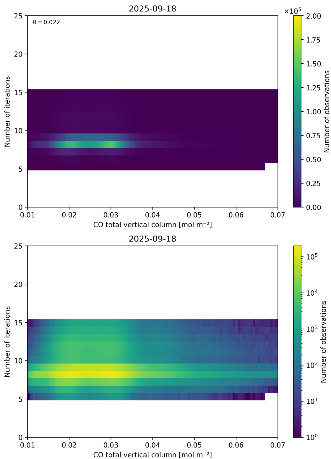
Figure 42: Scatter density plot of “CO total vertical column” against “Number of iterations” for 2025-09-17 to 2025-09-19.
