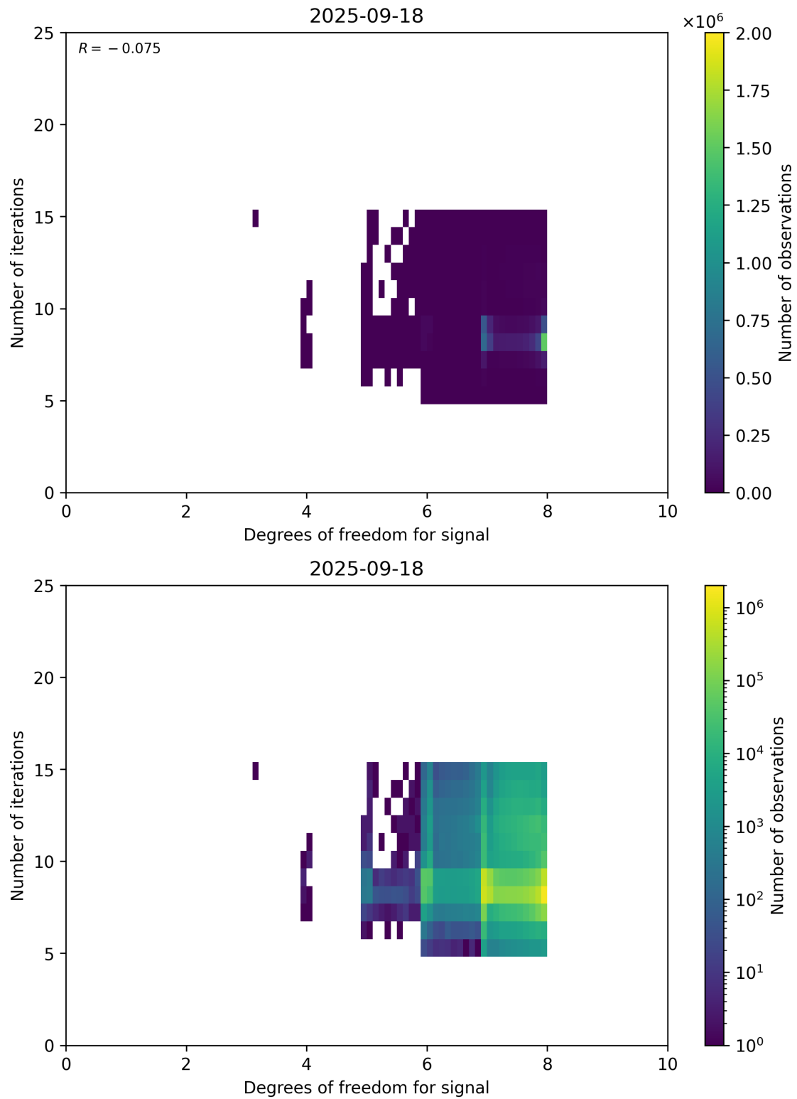
Figure 50: Scatter density plot of “Degrees of freedom for signal” against “Number of iterations” for 2025-09-17 to 2025-09-19.
