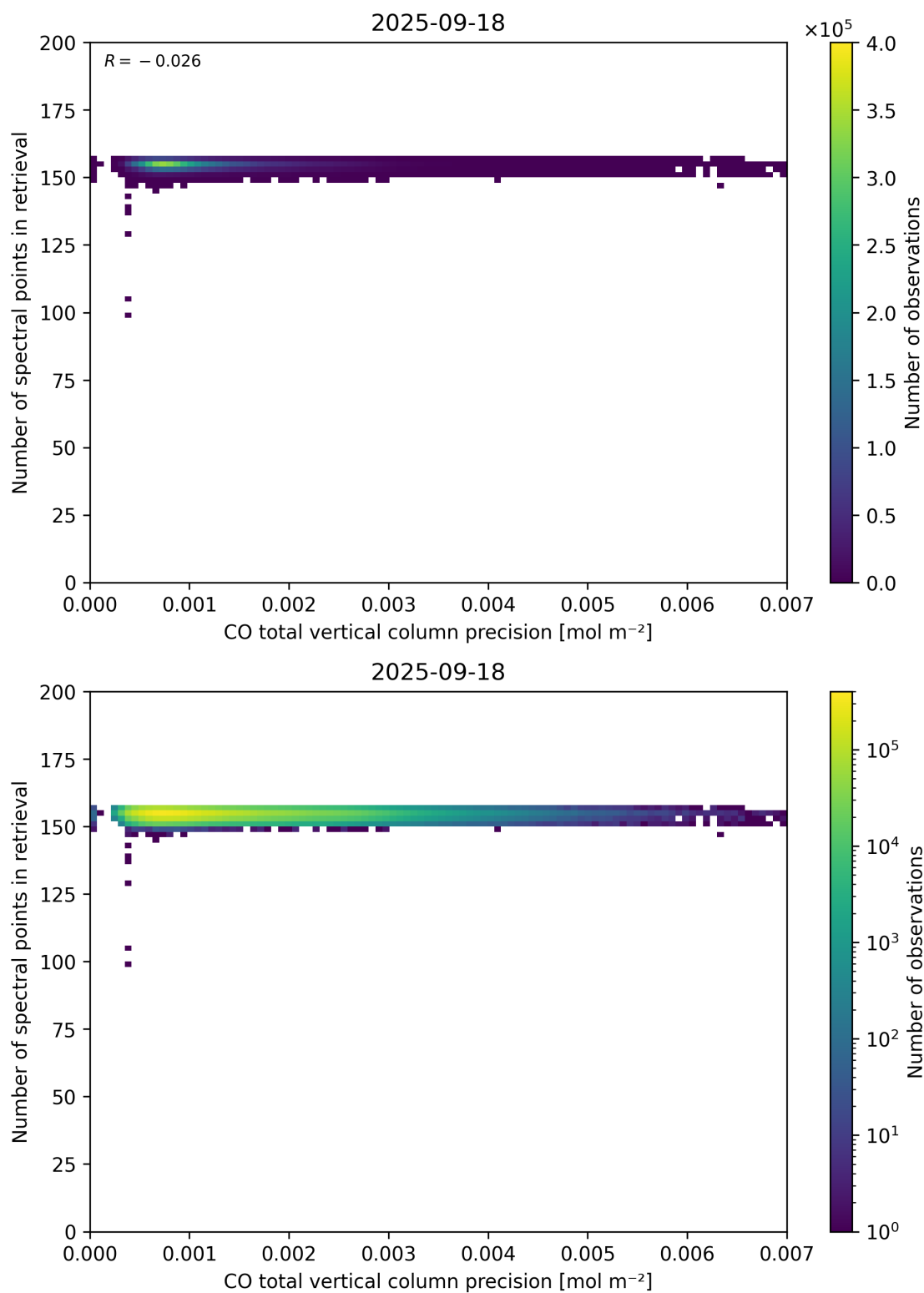
Figure 47: Scatter density plot of “CO total vertical column precision” against “Number of spectral points in retrieval” for 2025-09-17 to 2025-09-19.
