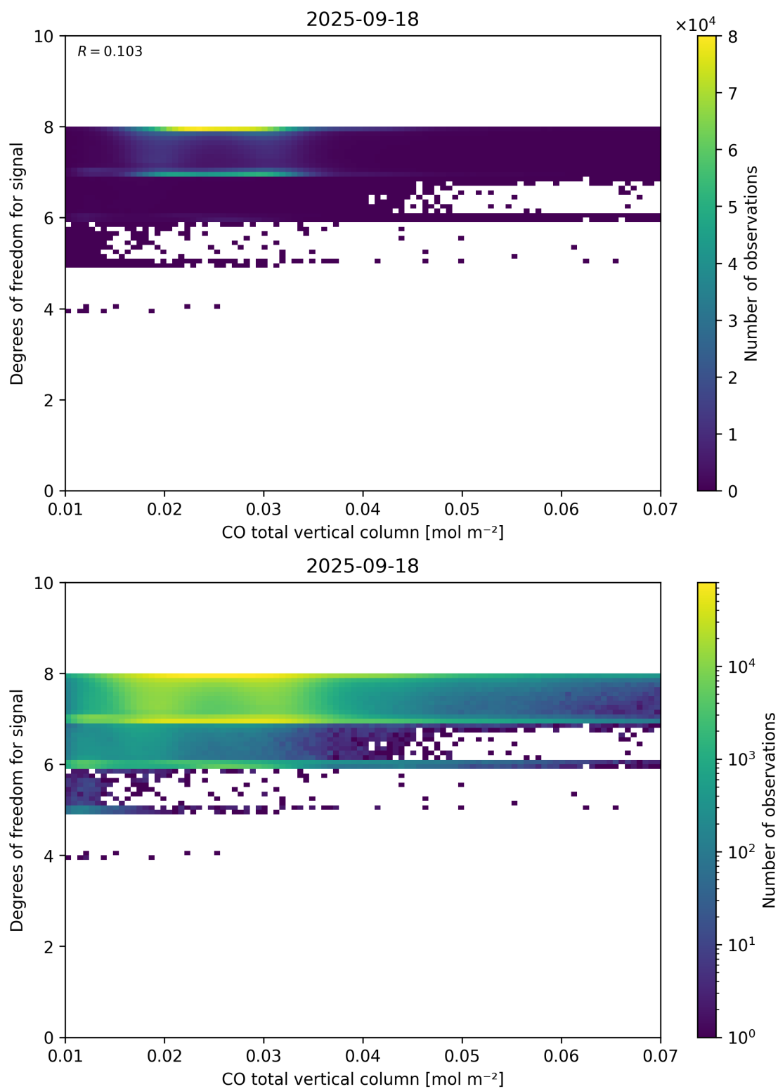
Figure 41: Scatter density plot of “CO total vertical column” against “Degrees of freedom for signal” for 2025-09-17 to 2025-09-19.
