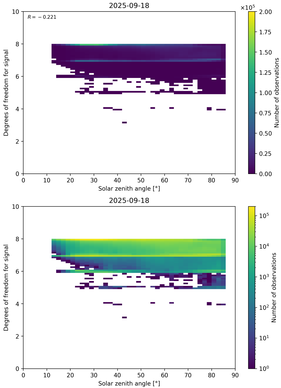
Figure 65: Scatter density plot of “Solar zenith angle” against “Degrees of freedom for signal” for 2025-09-17 to 2025-09-19.
