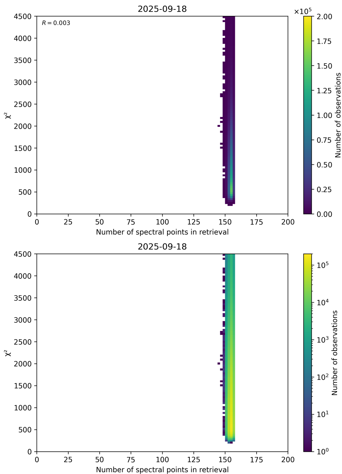
Figure 58: Scatter density plot of “Number of spectral points in retrieval” against “ \chi^2 ” for 2025-09-17 to 2025-09-19.
