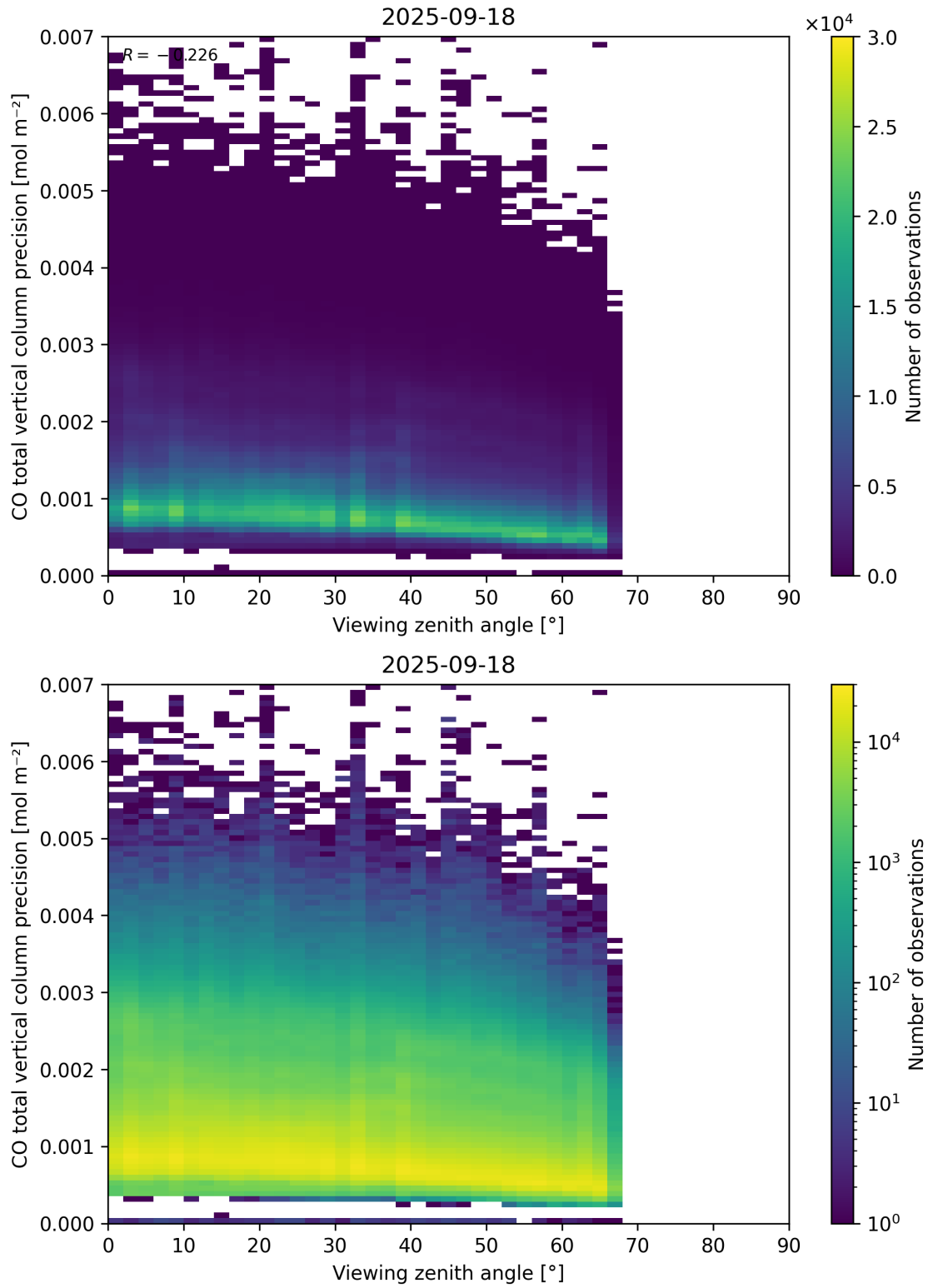
Figure 71: Scatter density plot of “Viewing zenith angle” against “CO total vertical column precision” for 2025-09-17 to 2025-09-19.
