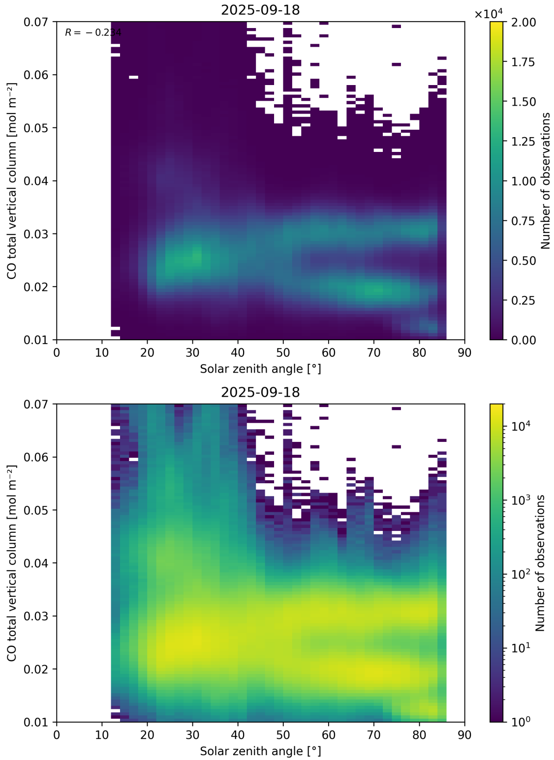
Figure 61: Scatter density plot of “Solar zenith angle” against “CO total vertical column” for 2025-09-17 to 2025-09-19.
