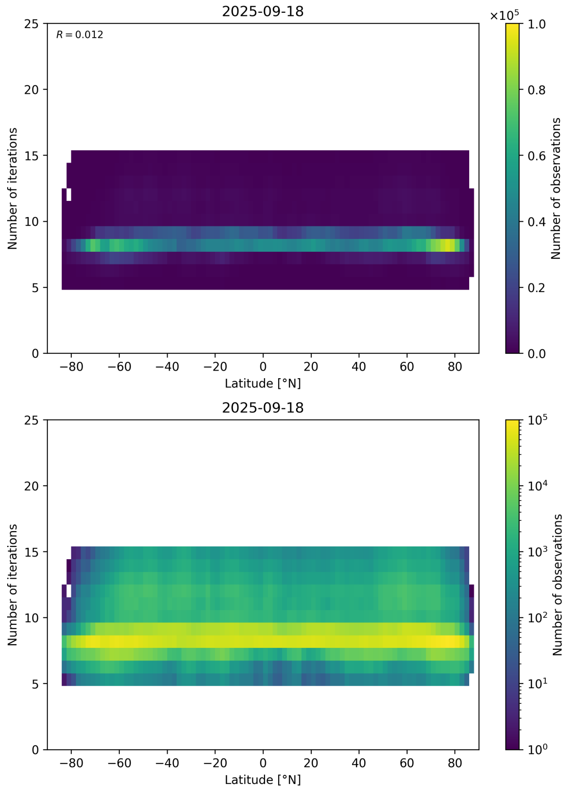
Figure 56: Scatter density plot of “Latitude” against “Number of iterations” for 2025-09-17 to 2025-09-19.
