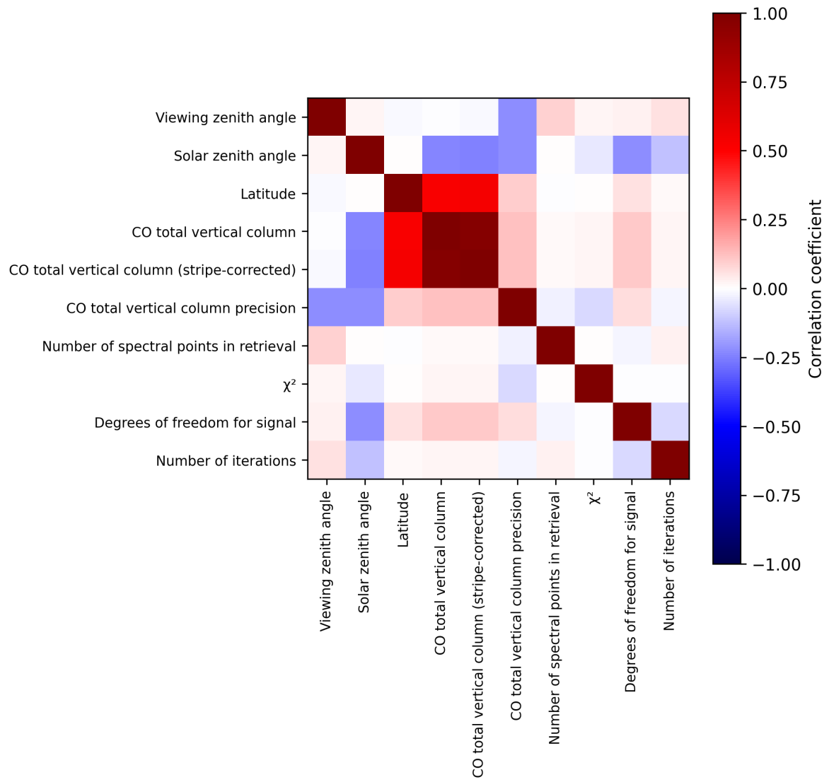
Figure 2: Map of correlation matrix for 2025-09-17 to 2025-09-19.
