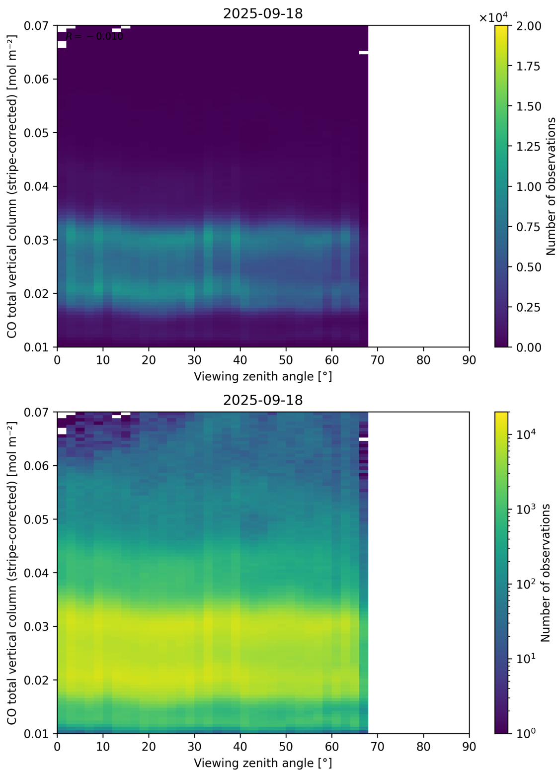
Figure 70: Scatter density plot of “Viewing zenith angle” against “CO total vertical column (stripe-corrected)” for 2025-09-17 to 2025-09-19.
