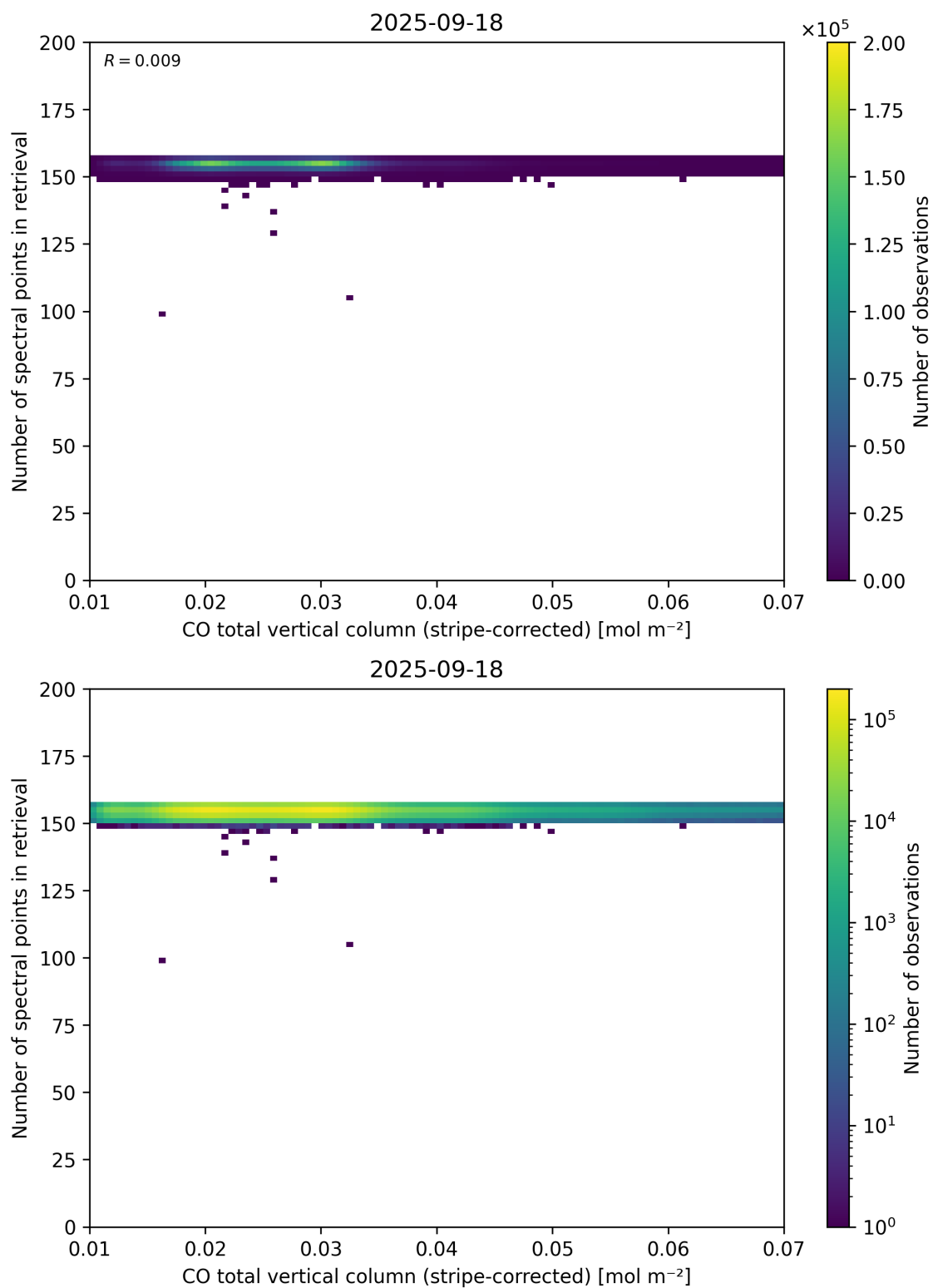
Figure 40: Scatter density plot of “CO total vertical column (stripe-corrected)” against “Number of spectral points in retrieval” for 2025-09-17 to 2025-09-19.
