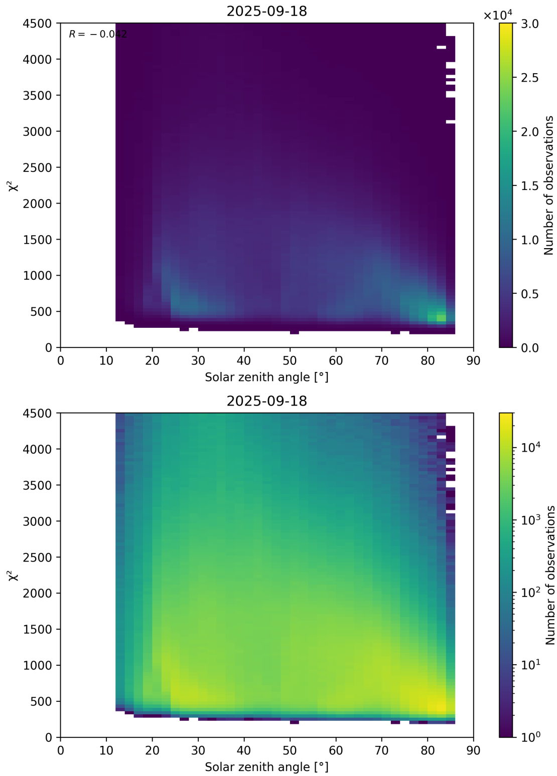
Figure 64: Scatter density plot of “Solar zenith angle” against “ \chi^2 ” for 2025-09-17 to 2025-09-19.
