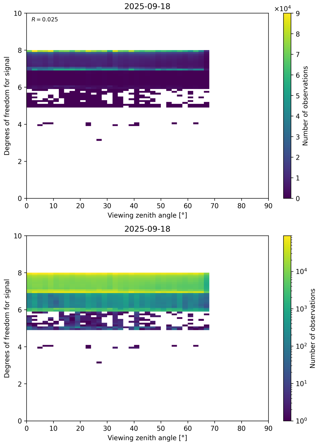
Figure 73: Scatter density plot of “Viewing zenith angle” against “Degrees of freedom for signal” for 2025-09-17 to 2025-09-19.
