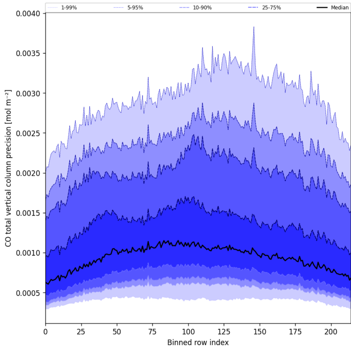
Figure 28: Along track statistics of “CO total vertical column precision” for 2025-09-17 to 2025-09-19
