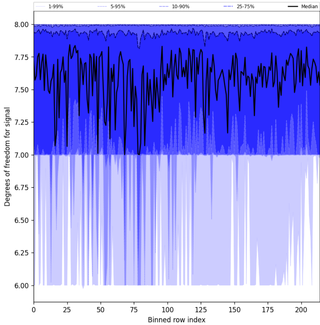
Figure 31: Along track statistics of “Degrees of freedom for signal” for 2025-09-17 to 2025-09-19
