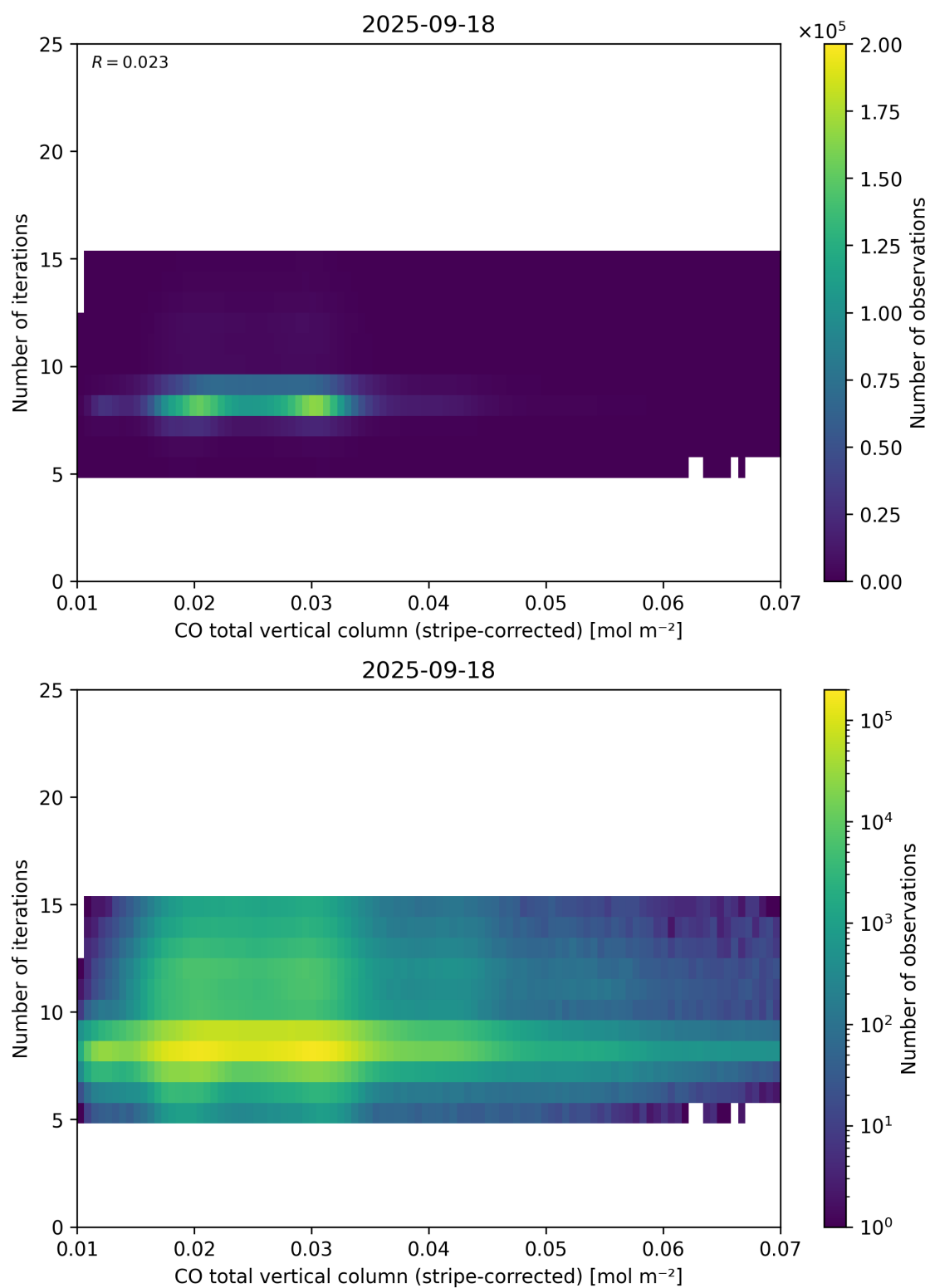
Figure 39: Scatter density plot of “CO total vertical column (stripe-corrected)” against “Number of iterations” for 2025-09-17 to 2025-09-19.
