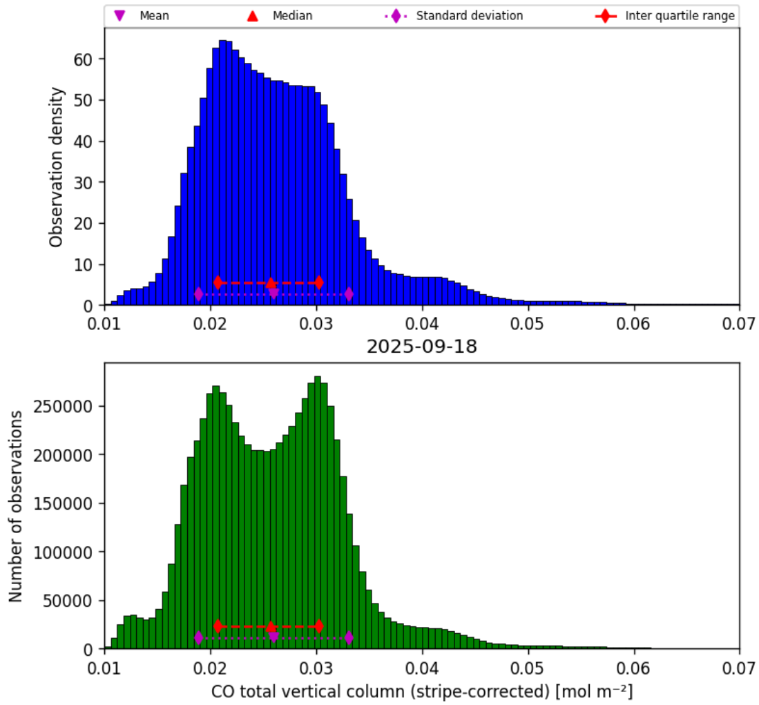
Figure 19: Histogram of “CO total vertical column (stripe-corrected)” for 2025-09-17 to 2025-09-19
