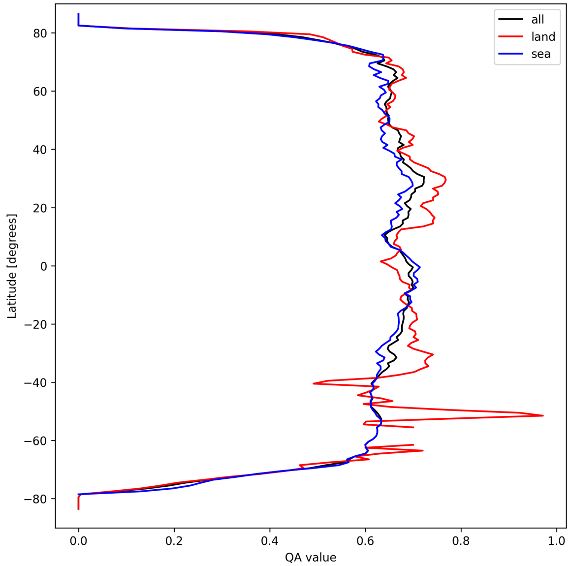
Figure 9: Zonal average of “QA value” for 2025-09-17 to 2025-09-19.
