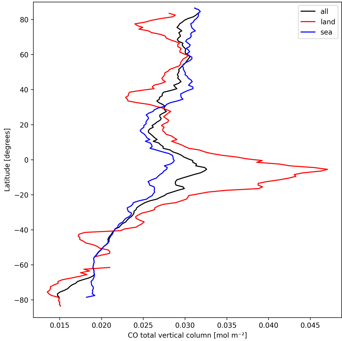
Figure 10: Zonal average of “CO total vertical column” for 2025-09-17 to 2025-09-19.
