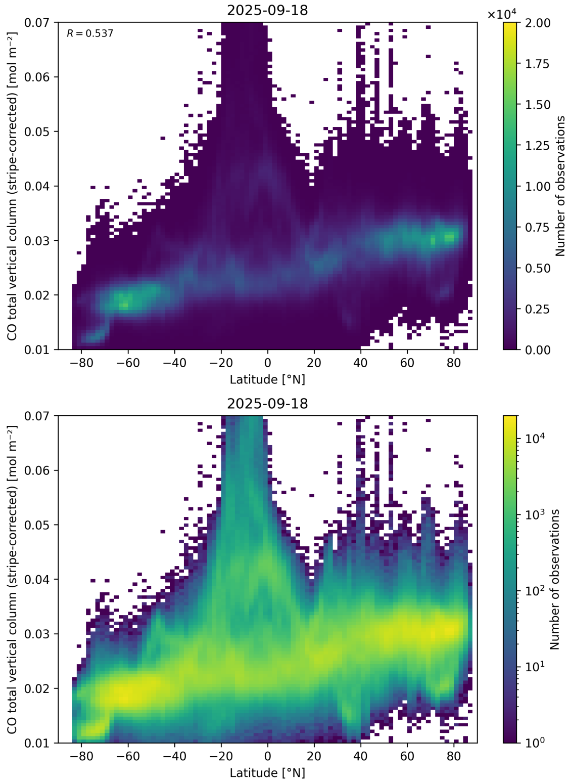
Figure 52: Scatter density plot of “Latitude” against “CO total vertical column (stripe-corrected)” for 2025-09-17 to 2025-09-19.
