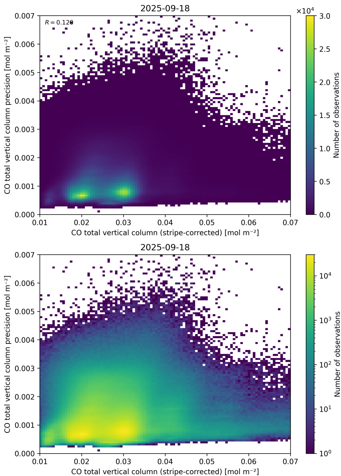
Figure 36: Scatter density plot of “CO total vertical column (stripe-corrected)” against “CO total vertical column precision” for 2025-09-17 to 2025-09-19.
