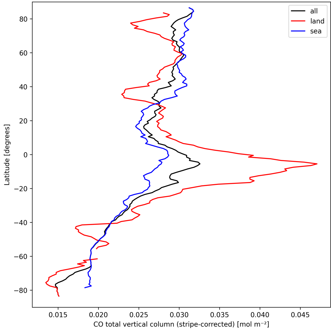
Figure 11: Zonal average of “CO total vertical column (stripe-corrected)” for 2025-09-17 to 2025-09-19.
