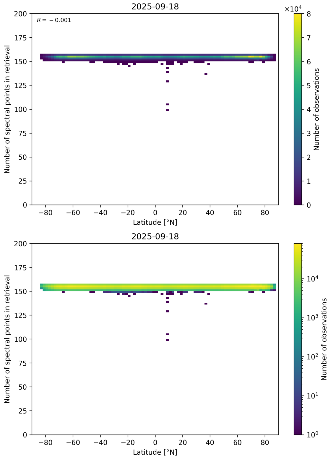
Figure 57: Scatter density plot of “Latitude” against “Number of spectral points in retrieval” for 2025-09-17 to 2025-09-19.
