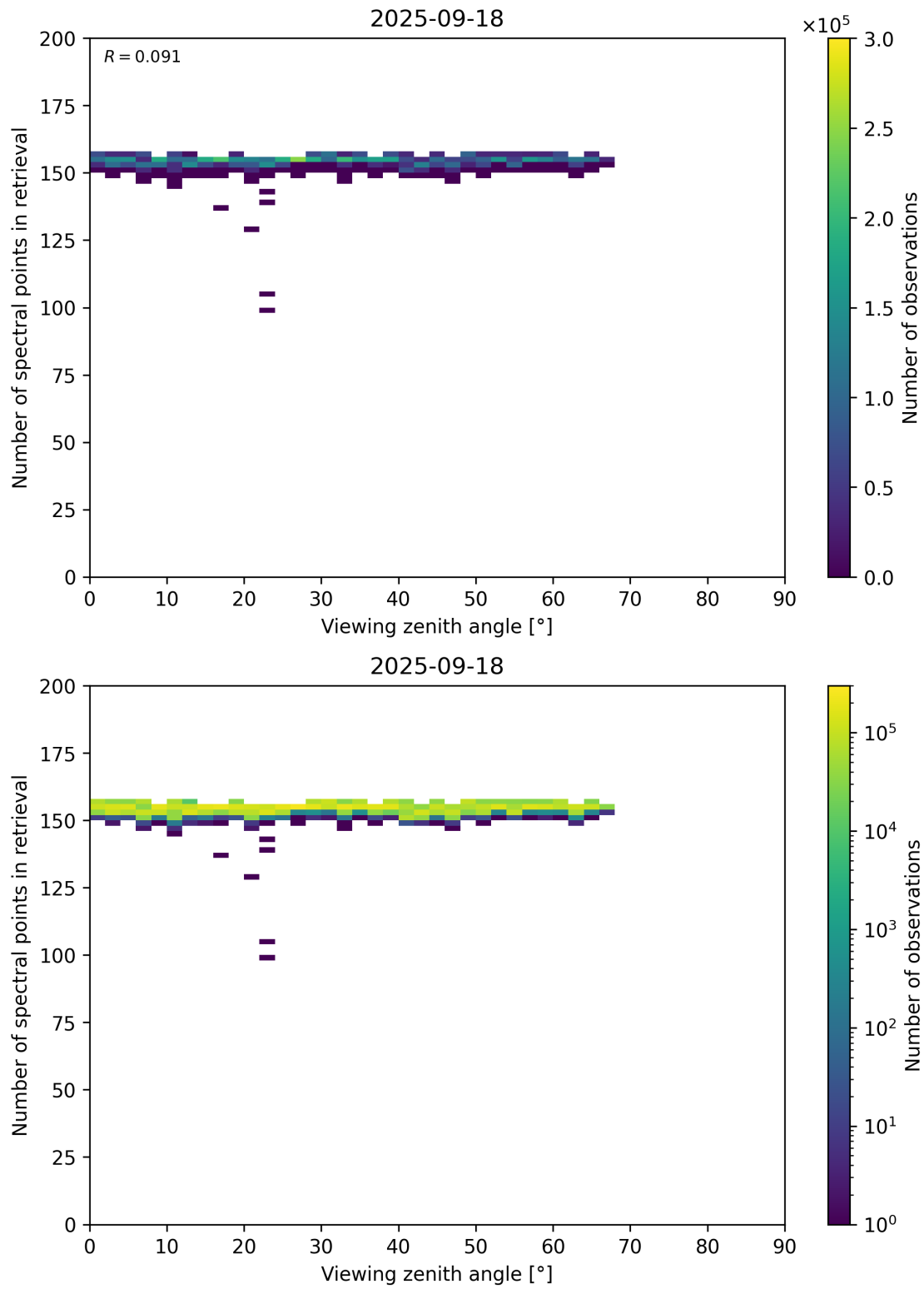
Figure 76: Scatter density plot of “Viewing zenith angle” against “Number of spectral points in retrieval” for 2025-09-17 to 2025-09-19.
