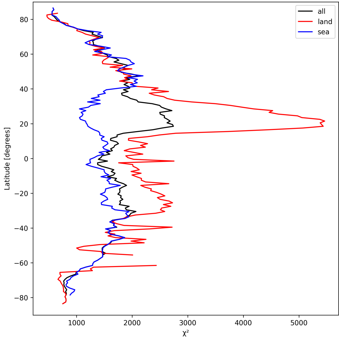
Figure 14: Zonal average of “ \chi^2 ” for 2025-09-17 to 2025-09-19.
