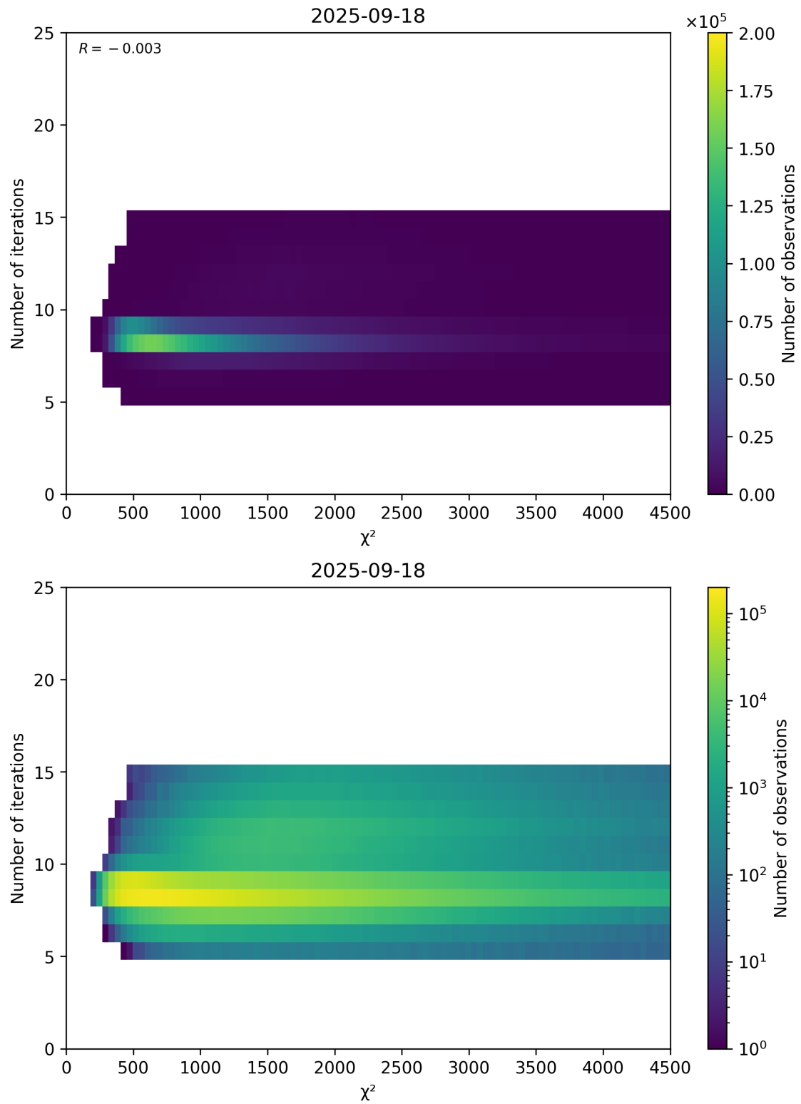
Figure 49: Scatter density plot of “ \chi^2 ” against “Number of iterations” for 2025-09-17 to 2025-09-19.
