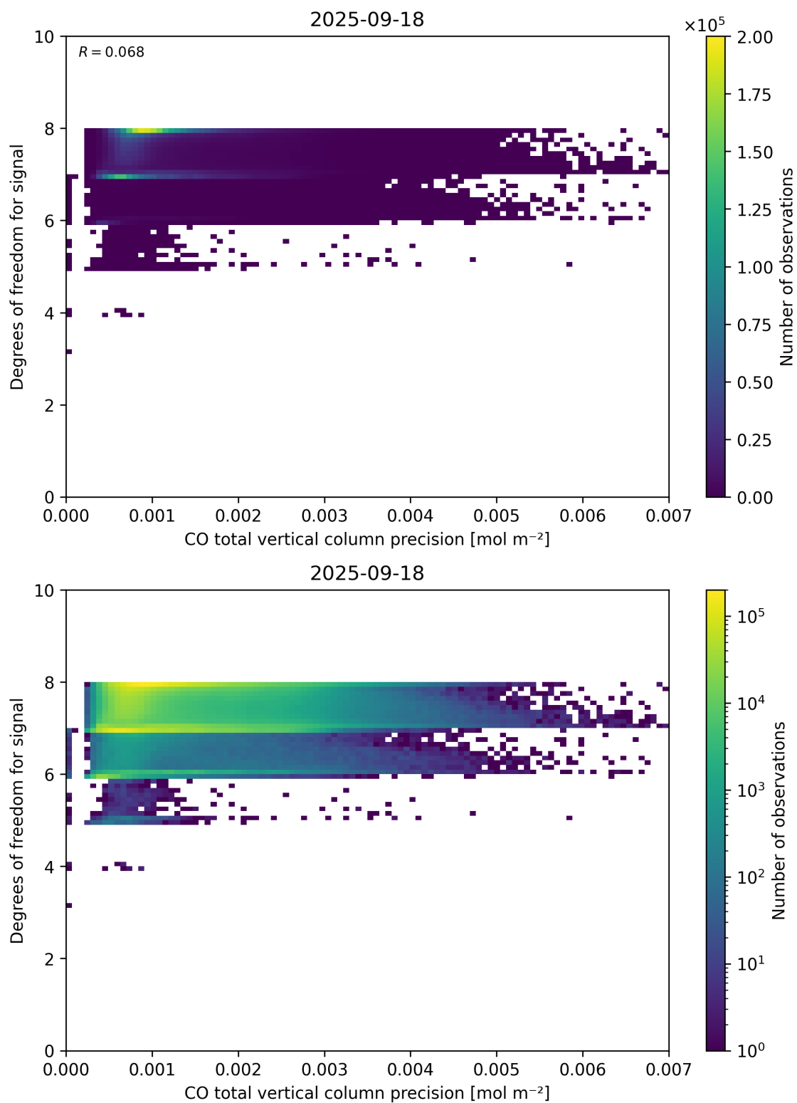
Figure 45: Scatter density plot of “CO total vertical column precision” against “Degrees of freedom for signal” for 2025-09-17 to 2025-09-19.
