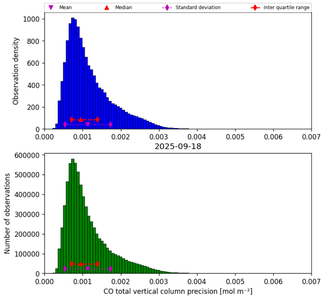
Figure 20: Histogram of “CO total vertical column precision” for 2025-09-17 to 2025-09-19
