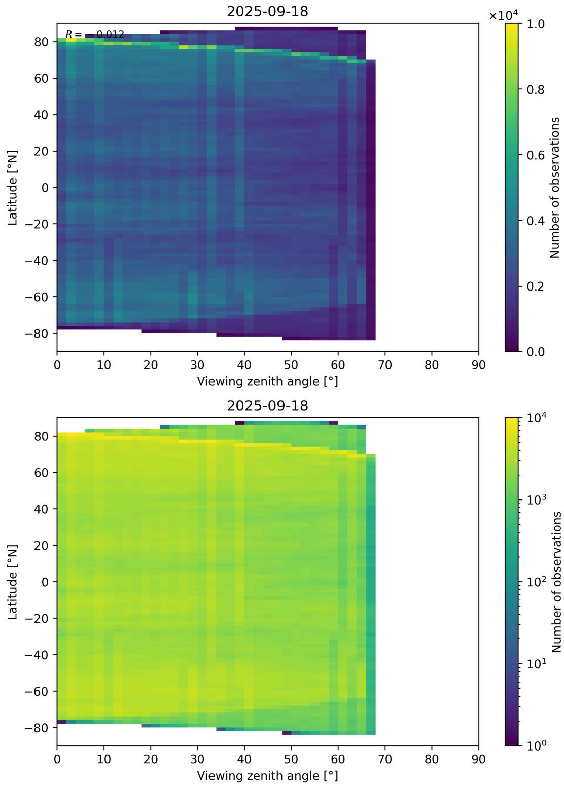
Figure 74: Scatter density plot of “Viewing zenith angle” against “Latitude” for 2025-09-17 to 2025-09-19.
