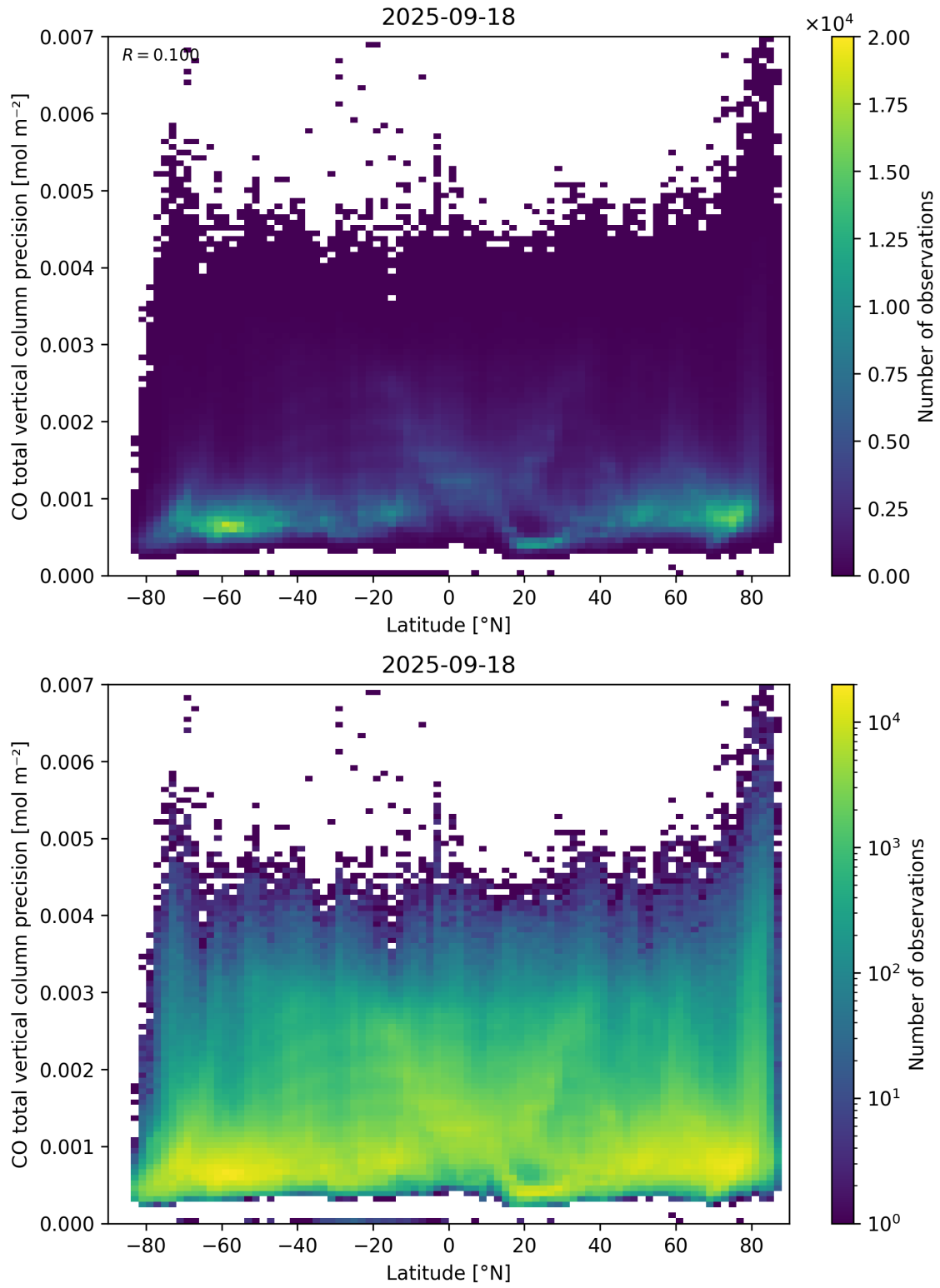
Figure 53: Scatter density plot of “Latitude” against “CO total vertical column precision” for 2025-09-17 to 2025-09-19.
