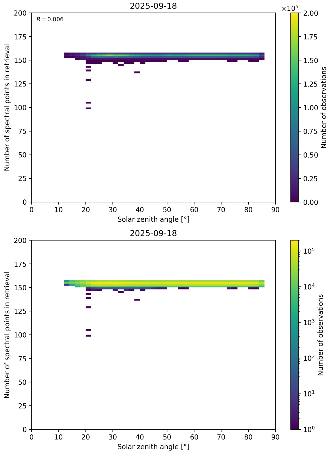
Figure 68: Scatter density plot of “Solar zenith angle” against “Number of spectral points in retrieval” for 2025-09-17 to 2025-09-19.
