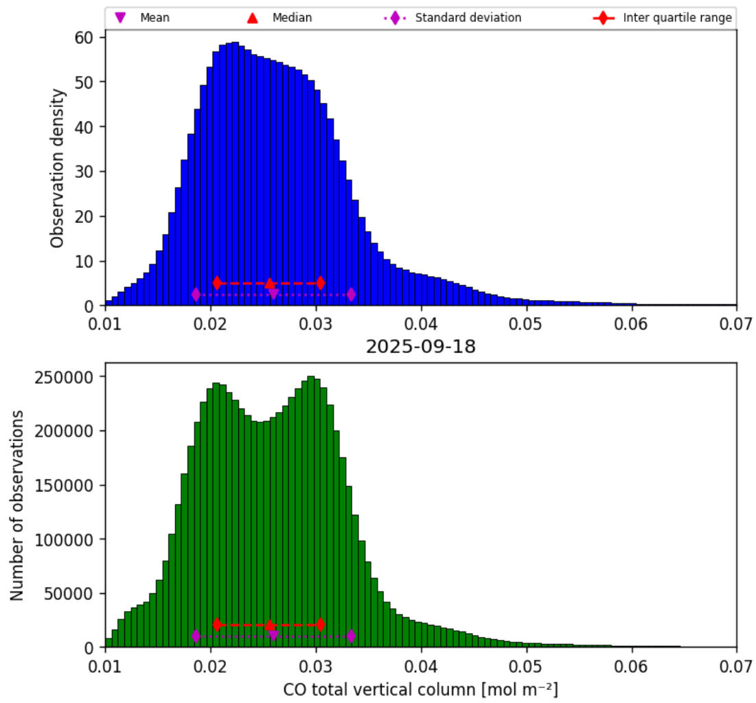
Figure 18: Histogram of “CO total vertical column” for 2025-09-17 to 2025-09-19
