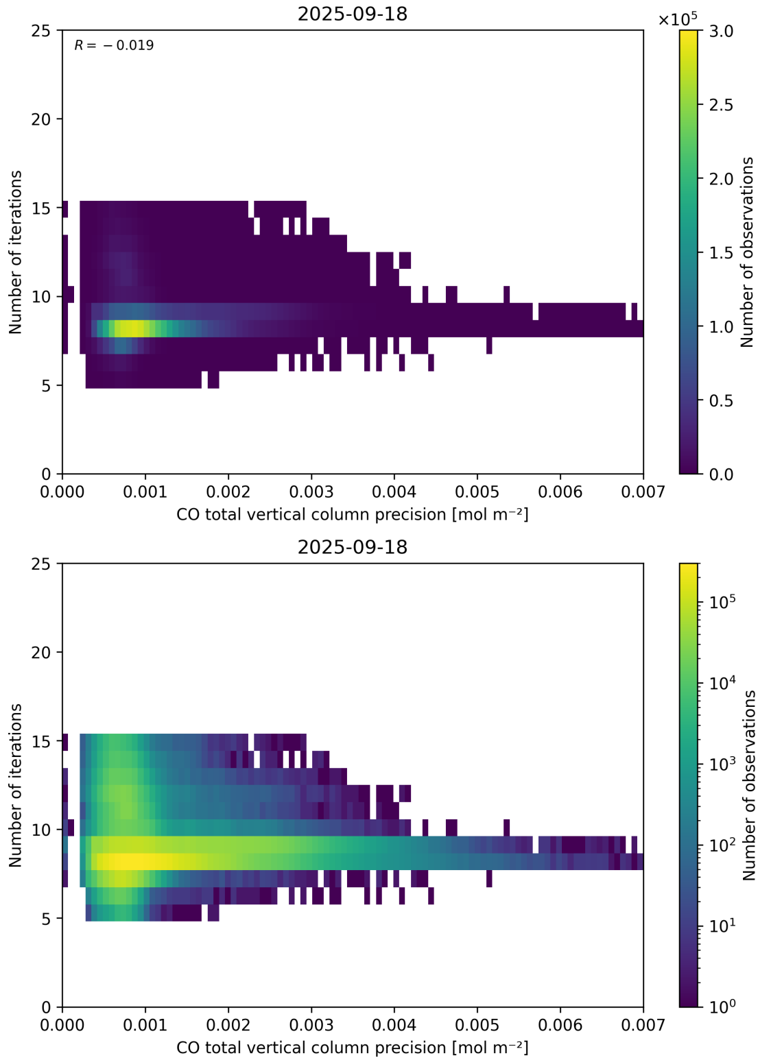
Figure 46: Scatter density plot of “CO total vertical column precision” against “Number of iterations” for 2025-09-17 to 2025-09-19.
