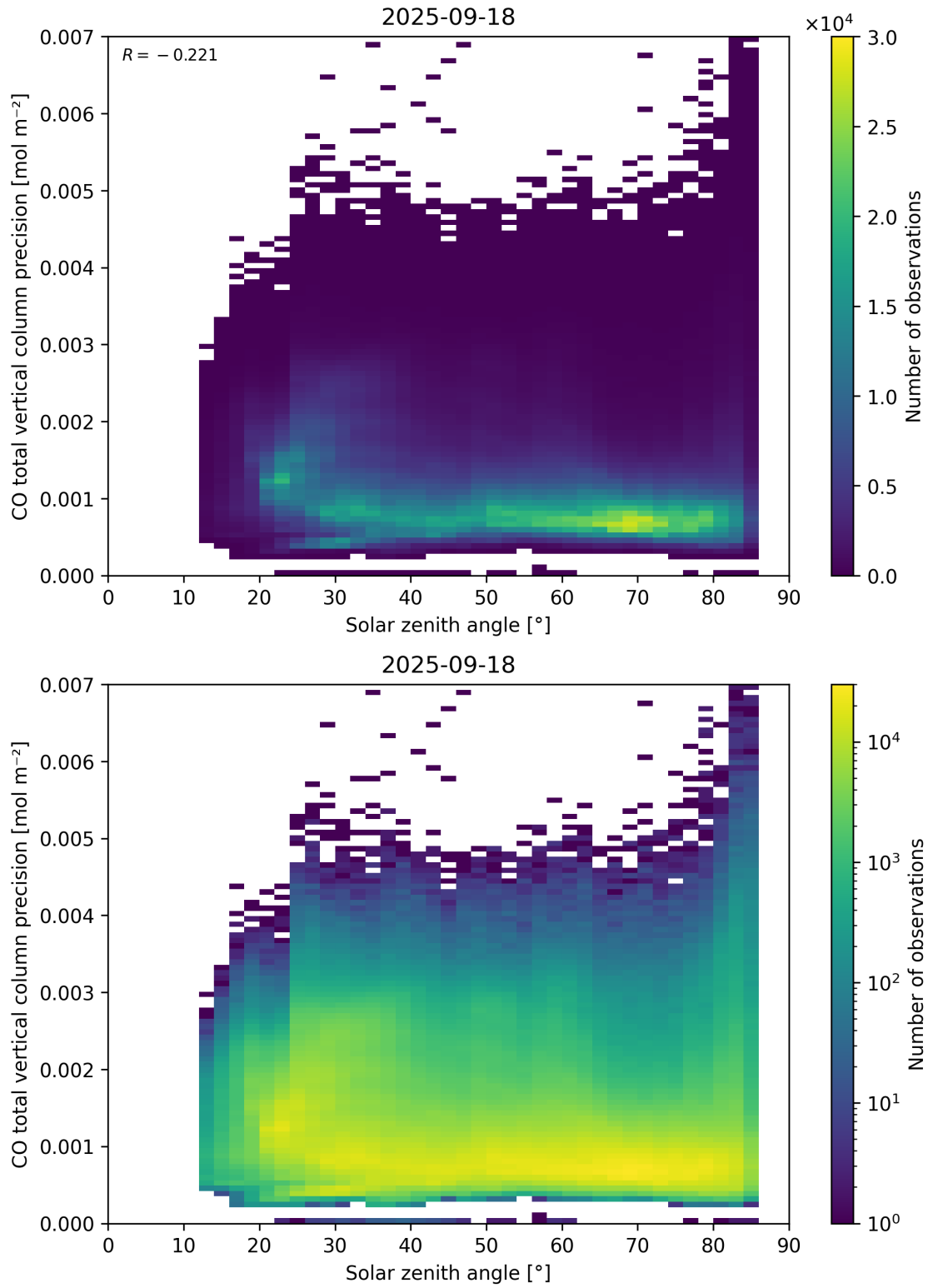
Figure 63: Scatter density plot of “Solar zenith angle” against “CO total vertical column precision” for 2025-09-17 to 2025-09-19.
