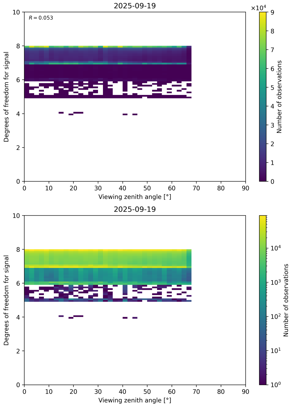
Figure 73: Scatter density plot of “Viewing zenith angle” against “Degrees of freedom for signal” for 2025-09-18 to 2025-09-20.
