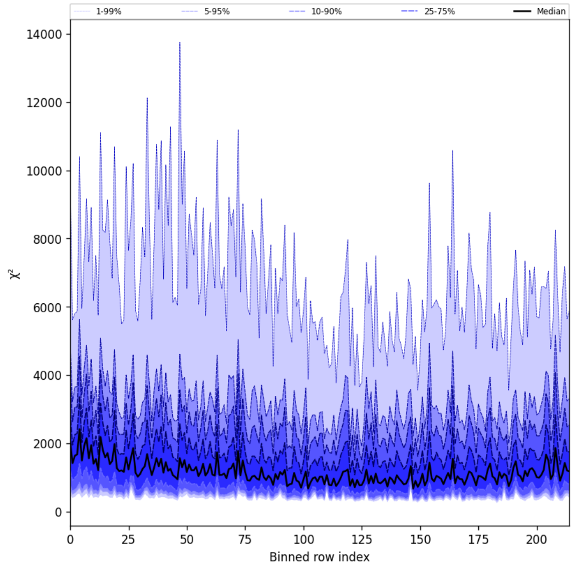
Figure 30: Along track statistics of “ \chi^2 ” for 2025-09-18 to 2025-09-20
