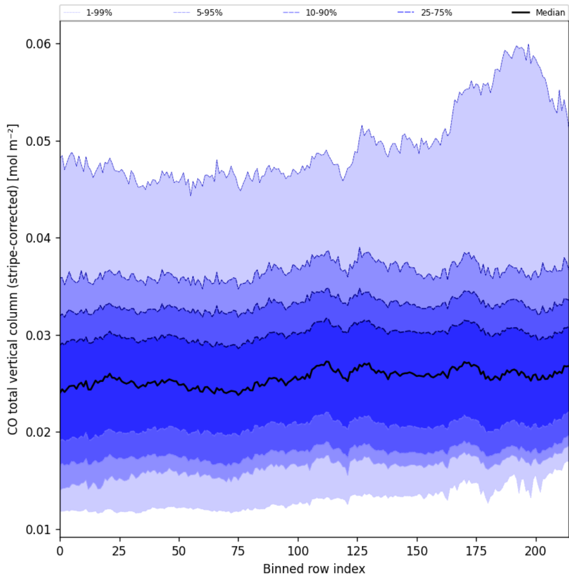
Figure 27: Along track statistics of “CO total vertical column (stripe-corrected)” for 2025-09-18 to 2025-09-20
