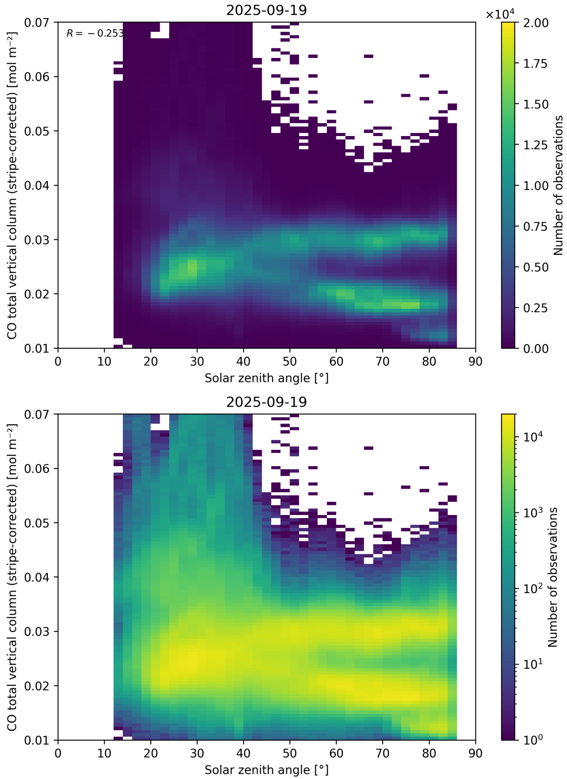
Figure 62: Scatter density plot of “Solar zenith angle” against “CO total vertical column (stripe-corrected)” for 2025-09-18 to 2025-09-20.
