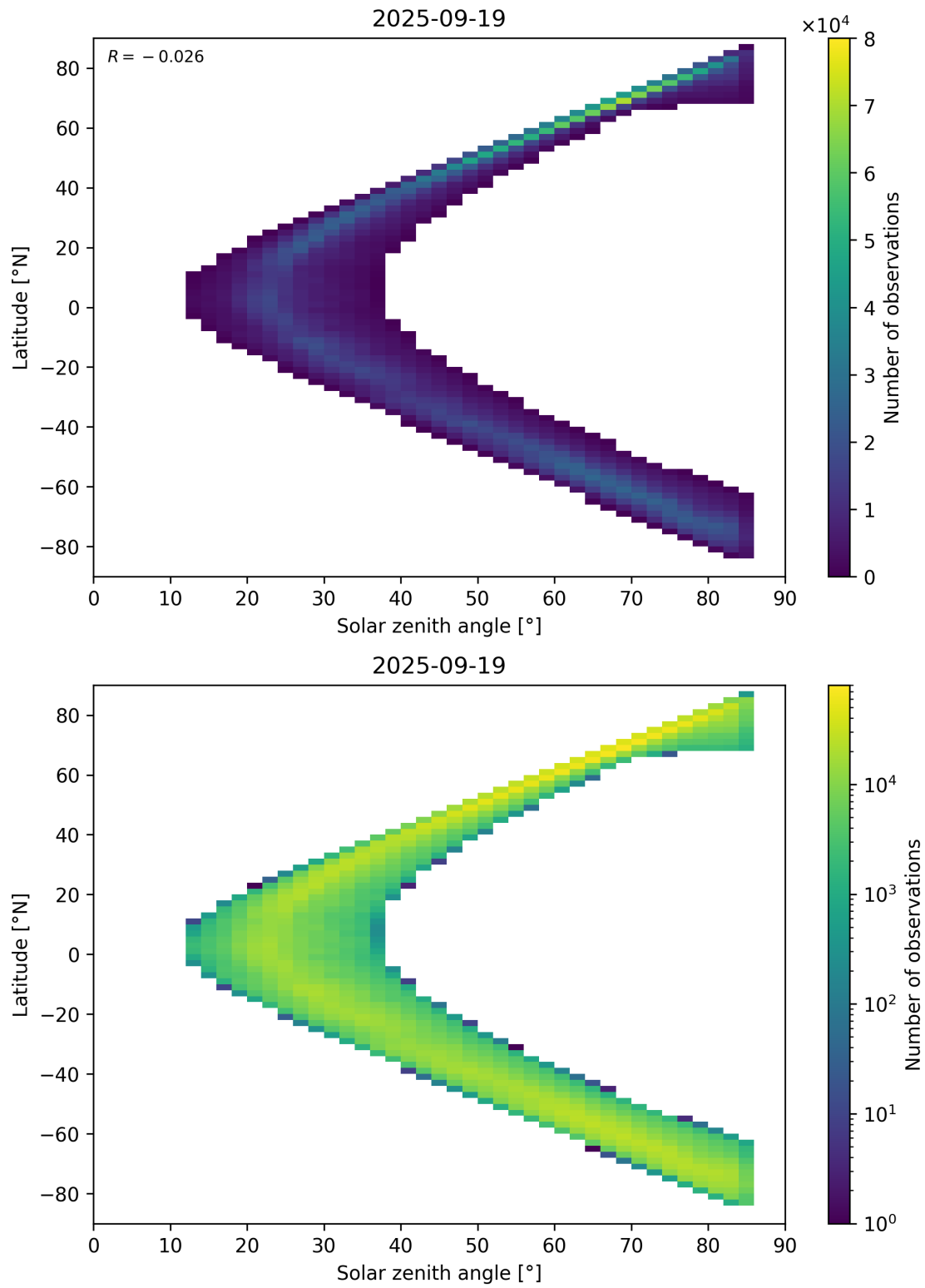
Figure 66: Scatter density plot of “Solar zenith angle” against “Latitude” for 2025-09-18 to 2025-09-20.
