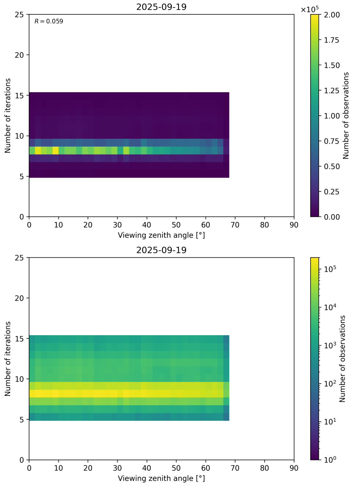
Figure 75: Scatter density plot of “Viewing zenith angle” against “Number of iterations” for 2025-09-18 to 2025-09-20.
