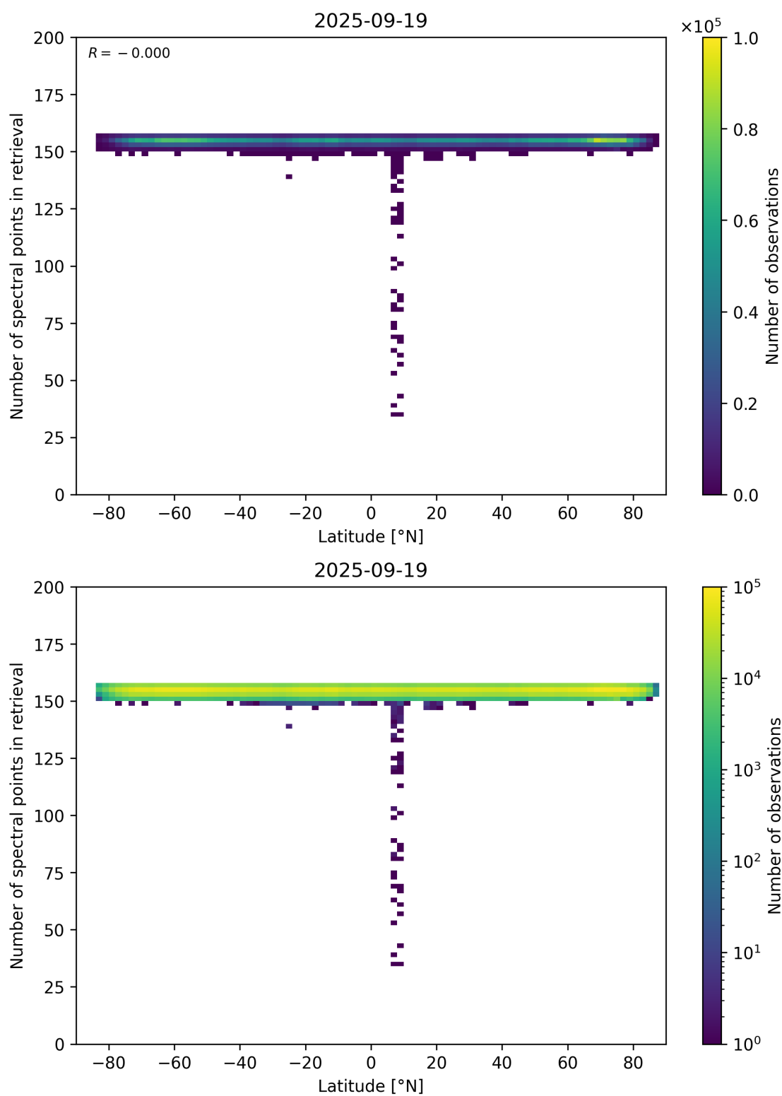
Figure 57: Scatter density plot of “Latitude” against “Number of spectral points in retrieval” for 2025-09-18 to 2025-09-20.
