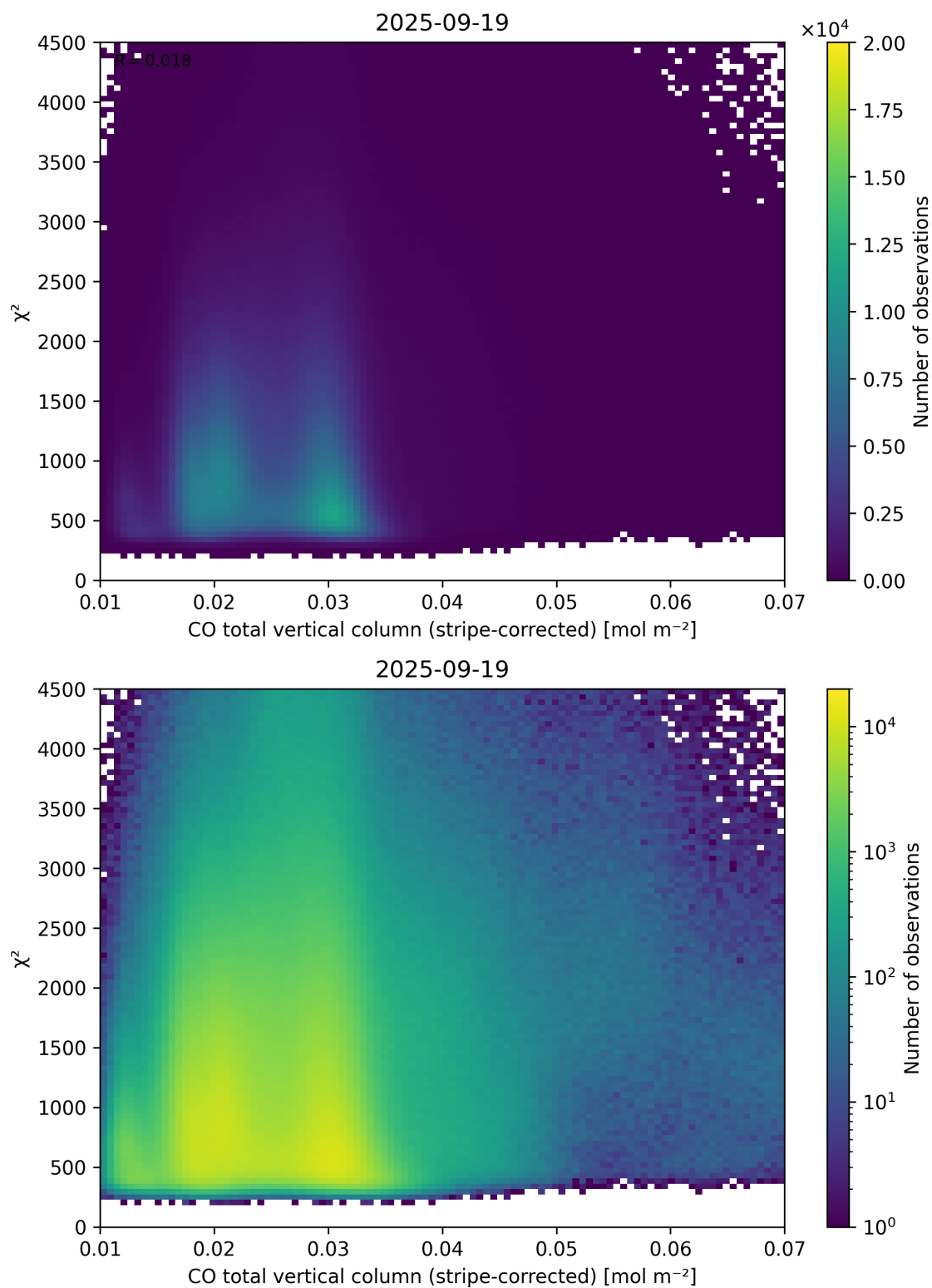
Figure 37: Scatter density plot of “CO total vertical column (stripe-corrected)” against “ \chi^2 ” for 2025-09-18 to 2025-09-20.
