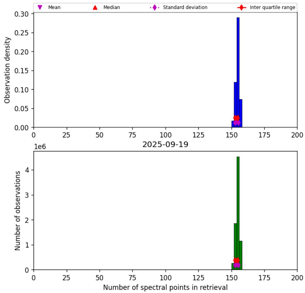
Figure 21: Histogram of “Number of spectral points in retrieval” for 2025-09-18 to 2025-09-20
