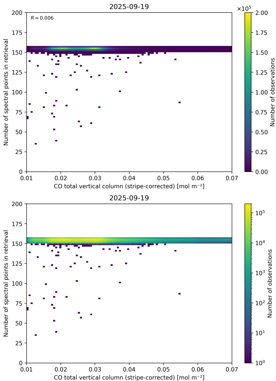
Figure 40: Scatter density plot of “CO total vertical column (stripe-corrected)” against “Number of spectral points in retrieval” for 2025-09-18 to 2025-09-20.
