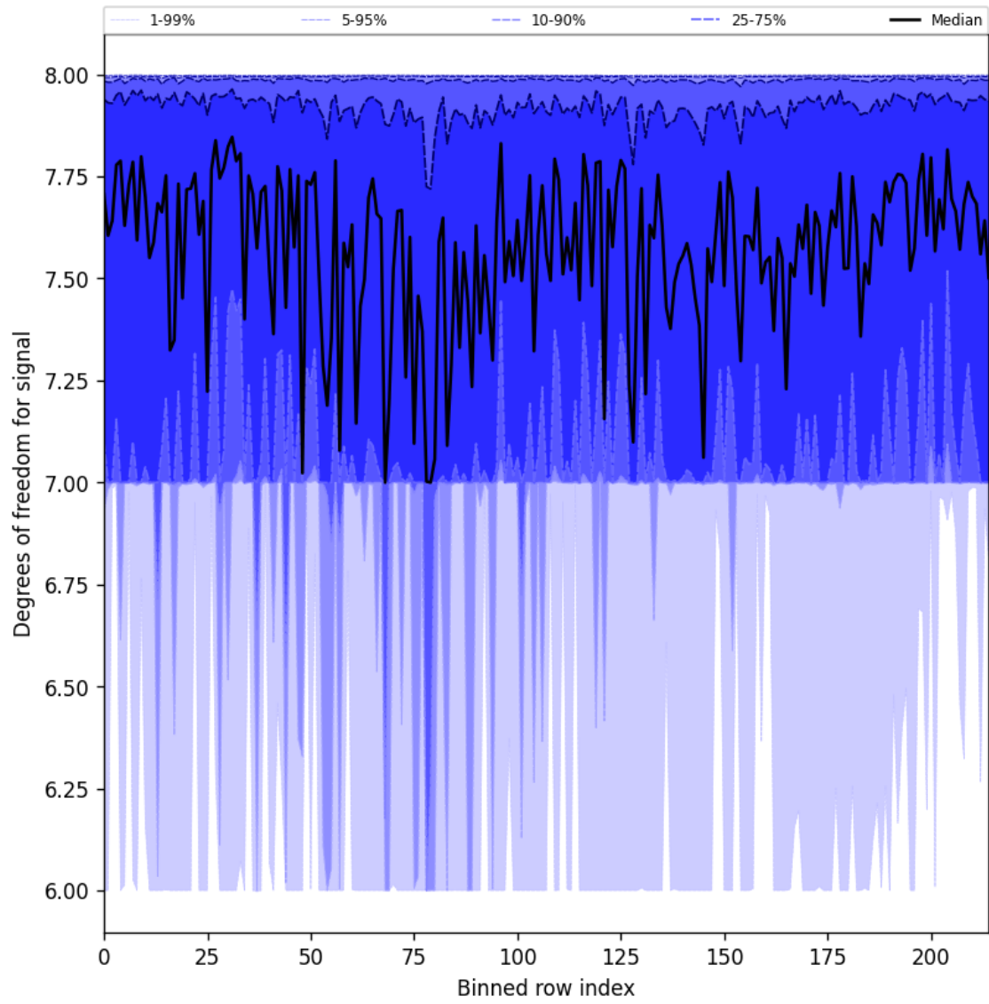
Figure 31: Along track statistics of “Degrees of freedom for signal” for 2025-09-18 to 2025-09-20
