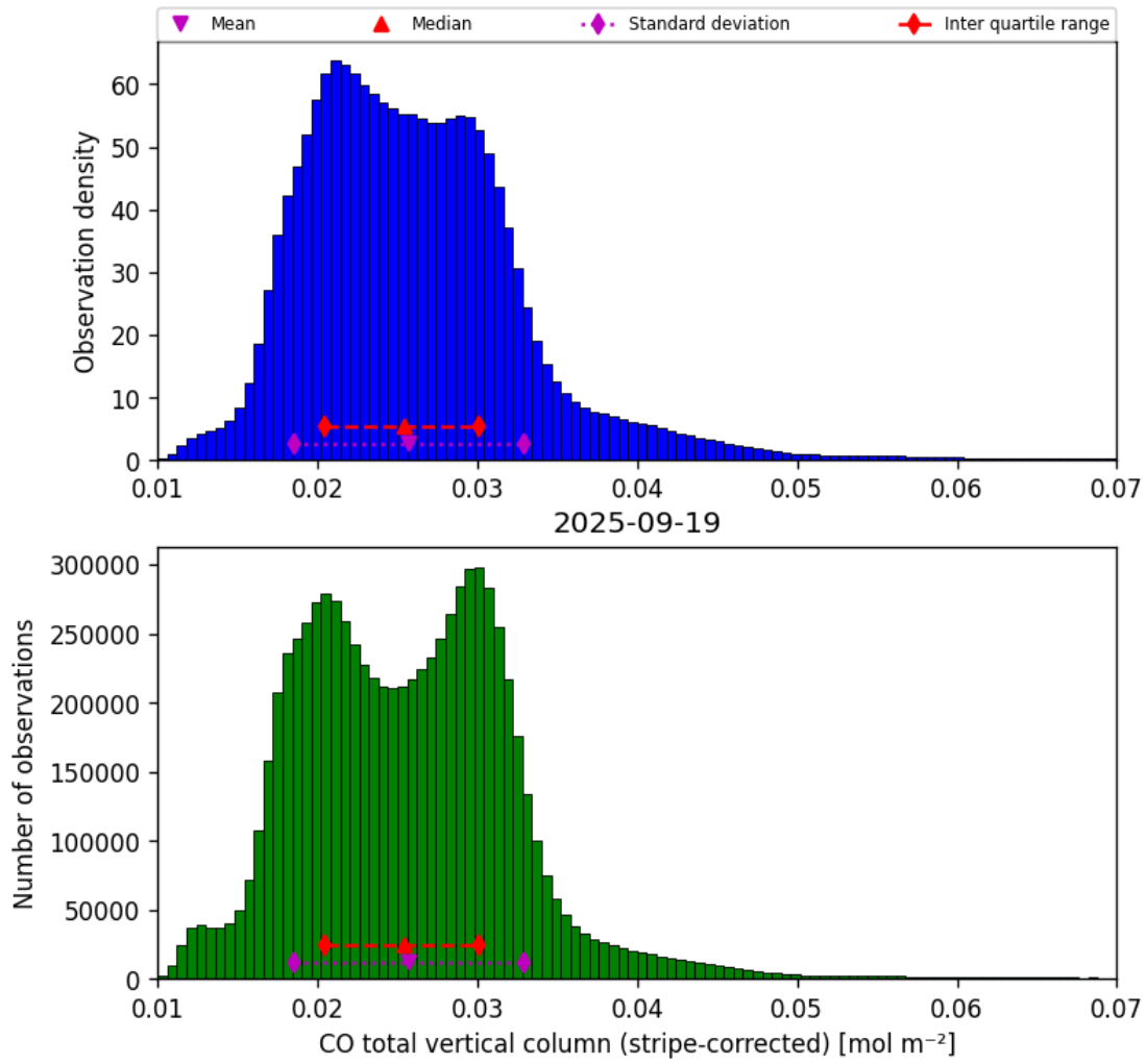
Figure 19: Histogram of “CO total vertical column (stripe-corrected)” for 2025-09-18 to 2025-09-20
