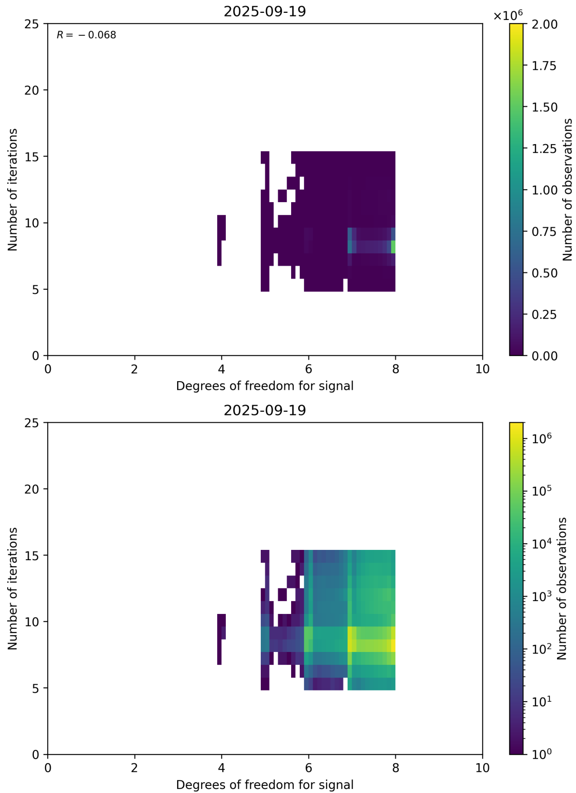
Figure 50: Scatter density plot of “Degrees of freedom for signal” against “Number of iterations” for 2025-09-18 to 2025-09-20.
