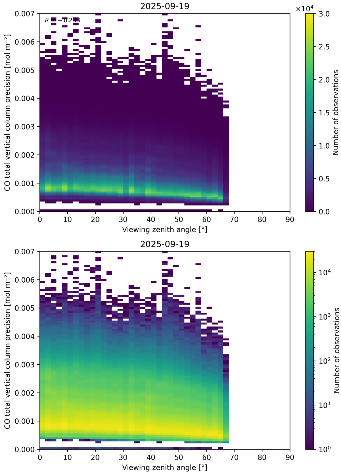
Figure 71: Scatter density plot of “Viewing zenith angle” against “CO total vertical column precision” for 2025-09-18 to 2025-09-20.
