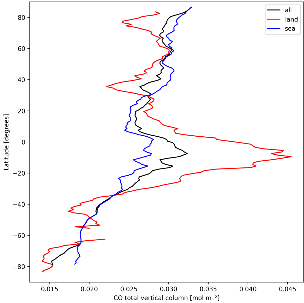
Figure 10: Zonal average of “CO total vertical column” for 2025-09-18 to 2025-09-20.
