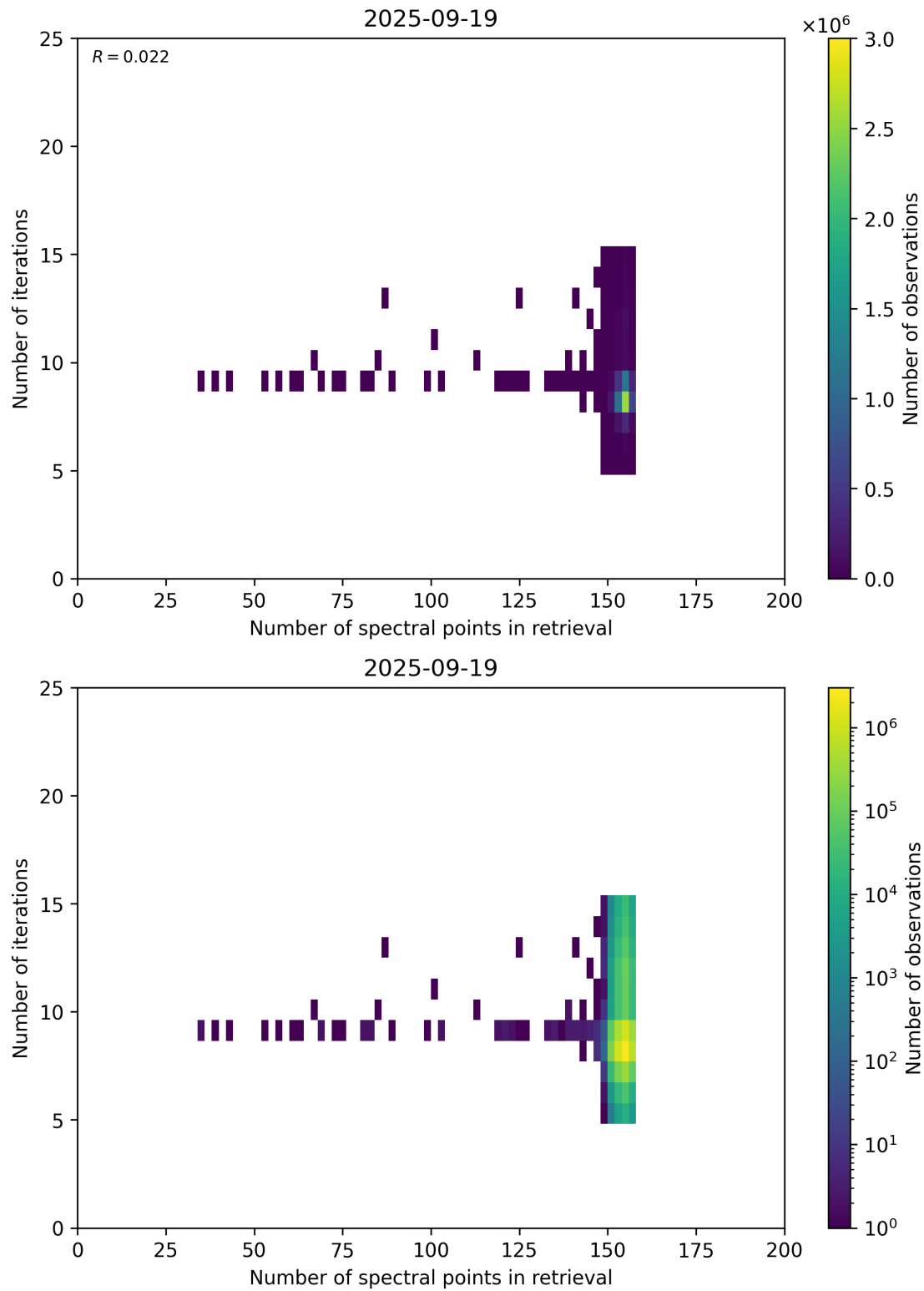
Figure 60: Scatter density plot of “Number of spectral points in retrieval” against “Number of iterations” for 2025-09-18 to 2025-09-20.
