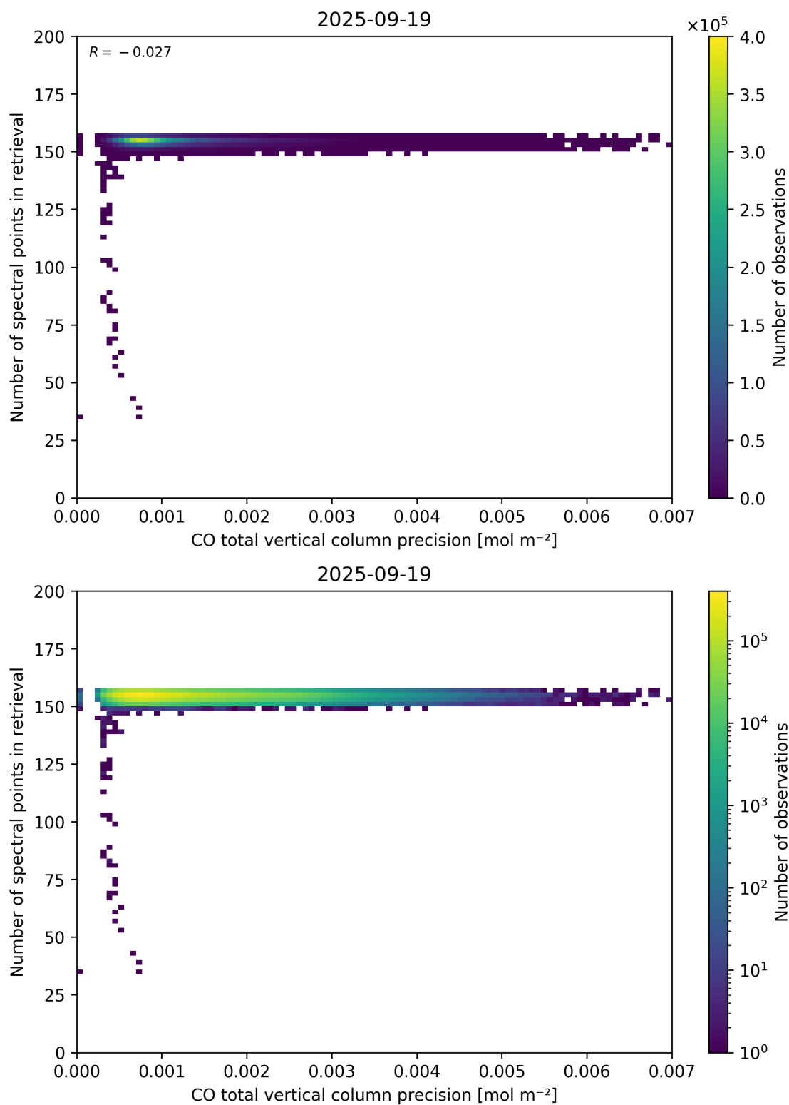
Figure 47: Scatter density plot of “CO total vertical column precision” against “Number of spectral points in retrieval” for 2025-09-18 to 2025-09-20.
