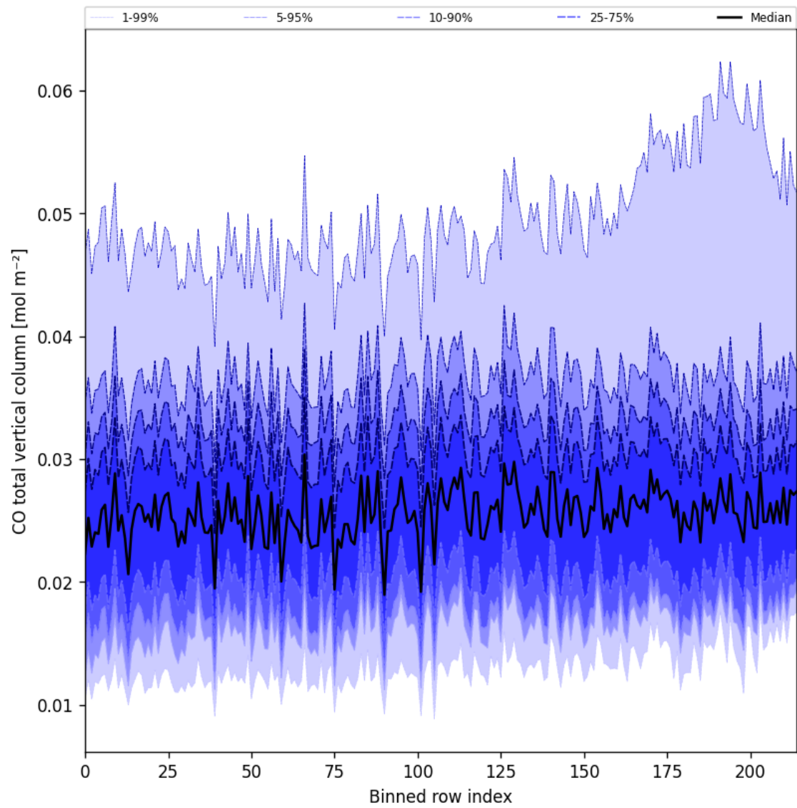
Figure 26: Along track statistics of “CO total vertical column” for 2025-09-18 to 2025-09-20
