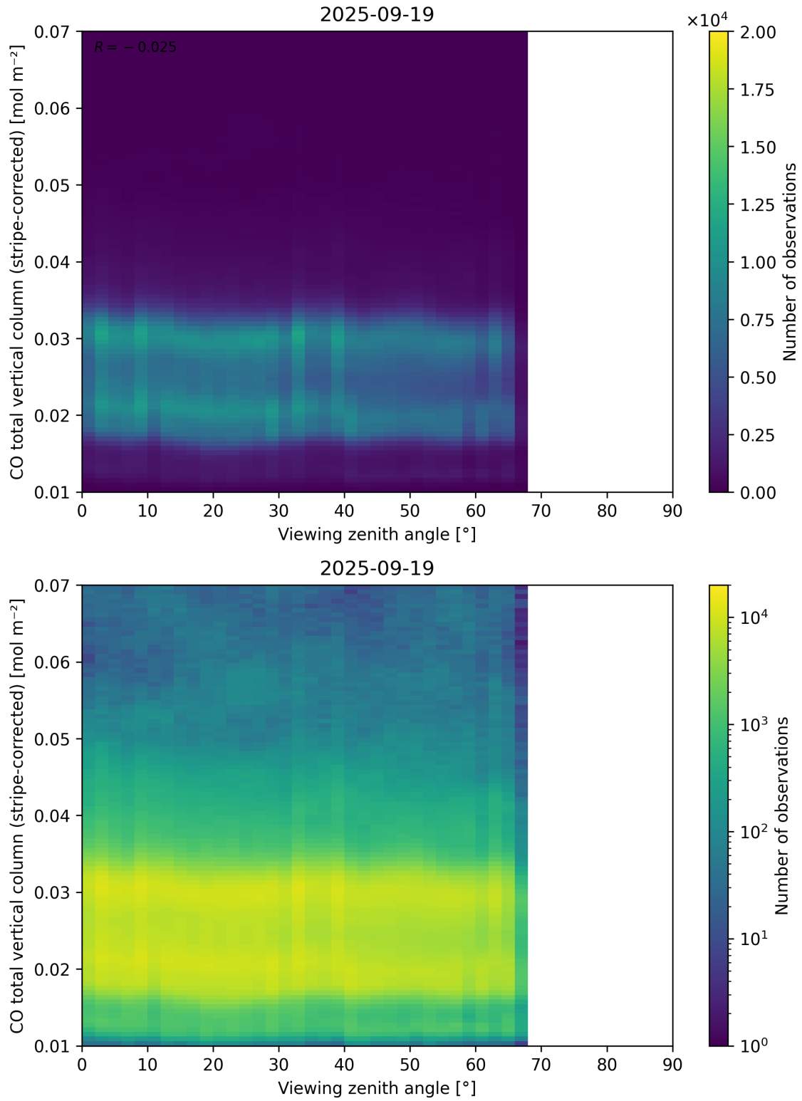
Figure 70: Scatter density plot of “Viewing zenith angle” against “CO total vertical column (stripe-corrected)” for 2025-09-18 to 2025-09-20.
