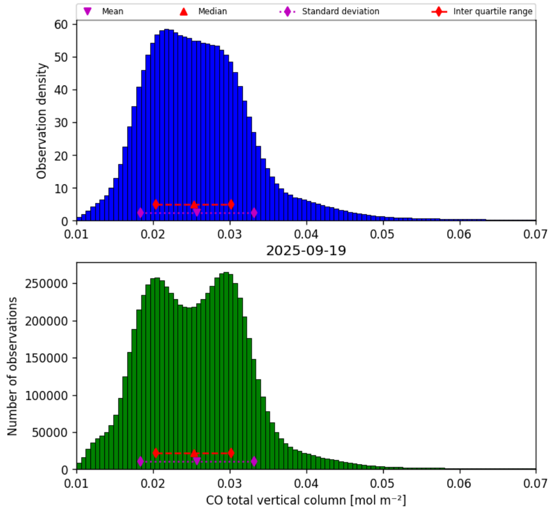
Figure 18: Histogram of “CO total vertical column” for 2025-09-18 to 2025-09-20
