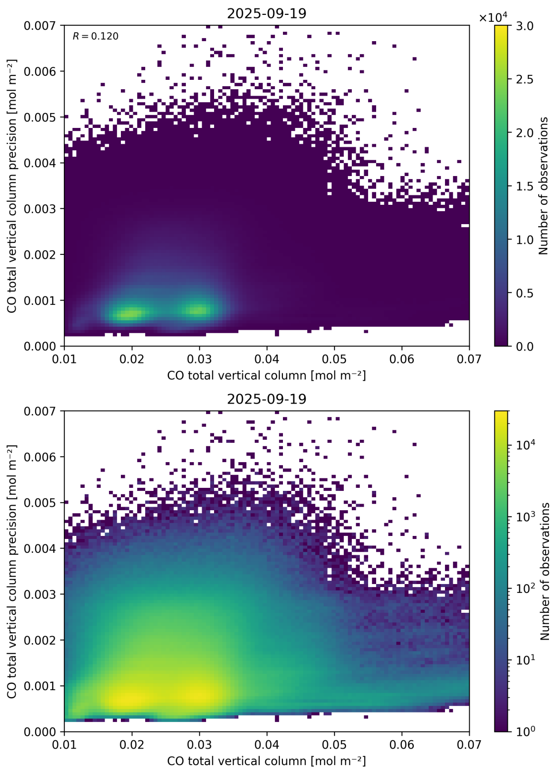
Figure 34: Scatter density plot of “CO total vertical column” against “CO total vertical column precision” for 2025-09-18 to 2025-09-20.
