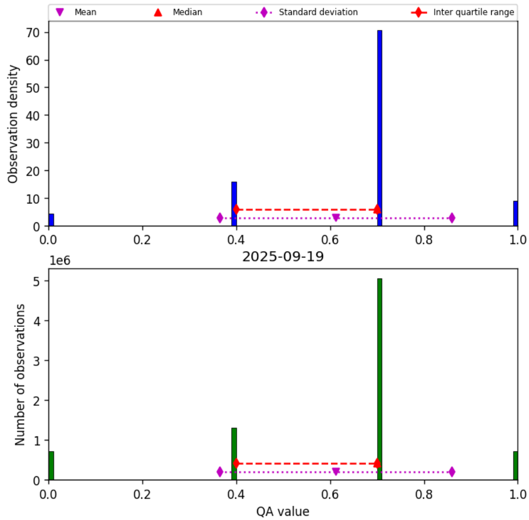
Figure 17: Histogram of “QA value” for 2025-09-18 to 2025-09-20
