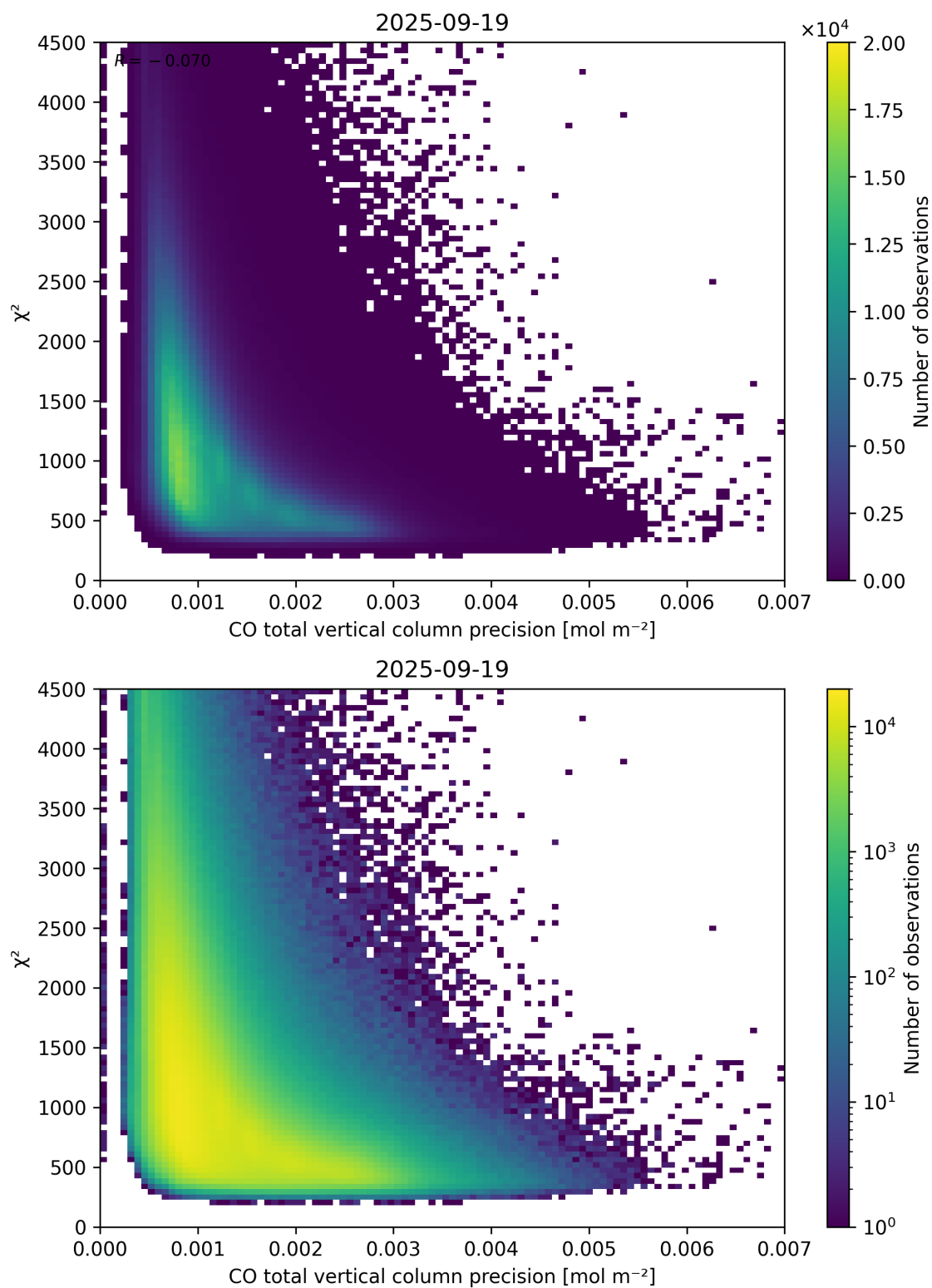
Figure 44: Scatter density plot of “CO total vertical column precision” against “ \chi^2 ” for 2025-09-18 to 2025-09-20.
