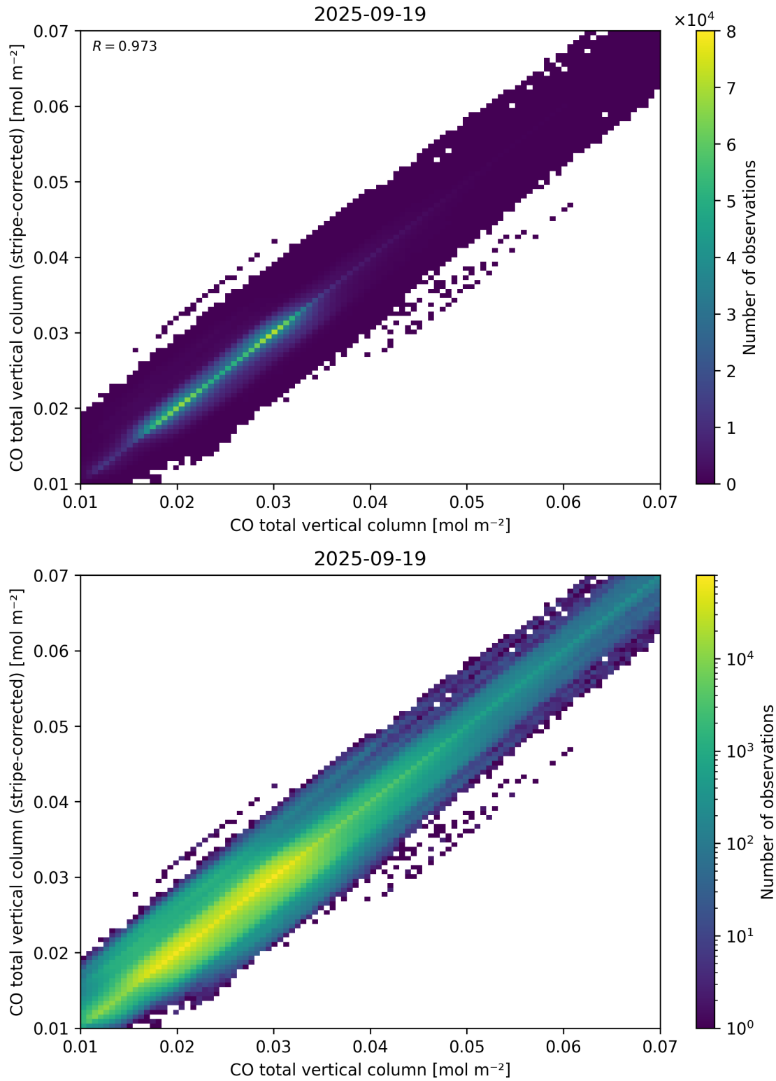
Figure 33: Scatter density plot of “CO total vertical column” against “CO total vertical column (stripe-corrected)” for 2025-09-18 to 2025-09-20.
