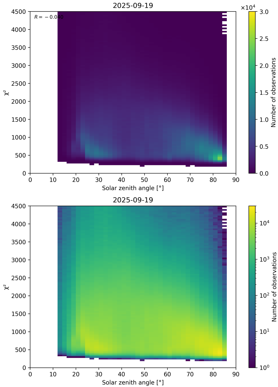
Figure 64: Scatter density plot of “Solar zenith angle” against “ \chi^2 ” for 2025-09-18 to 2025-09-20.
