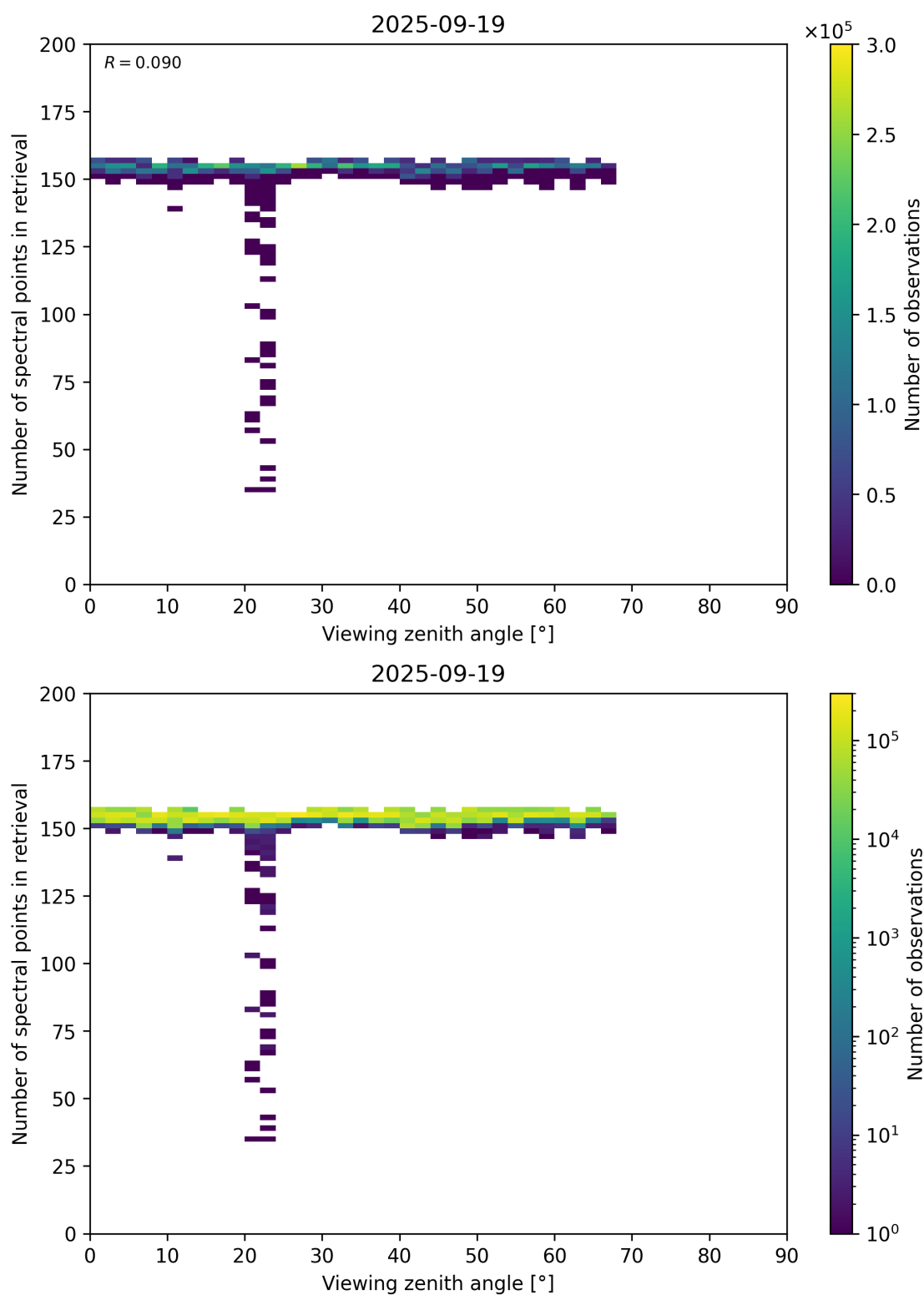
Figure 76: Scatter density plot of “Viewing zenith angle” against “Number of spectral points in retrieval” for 2025-09-18 to 2025-09-20.
