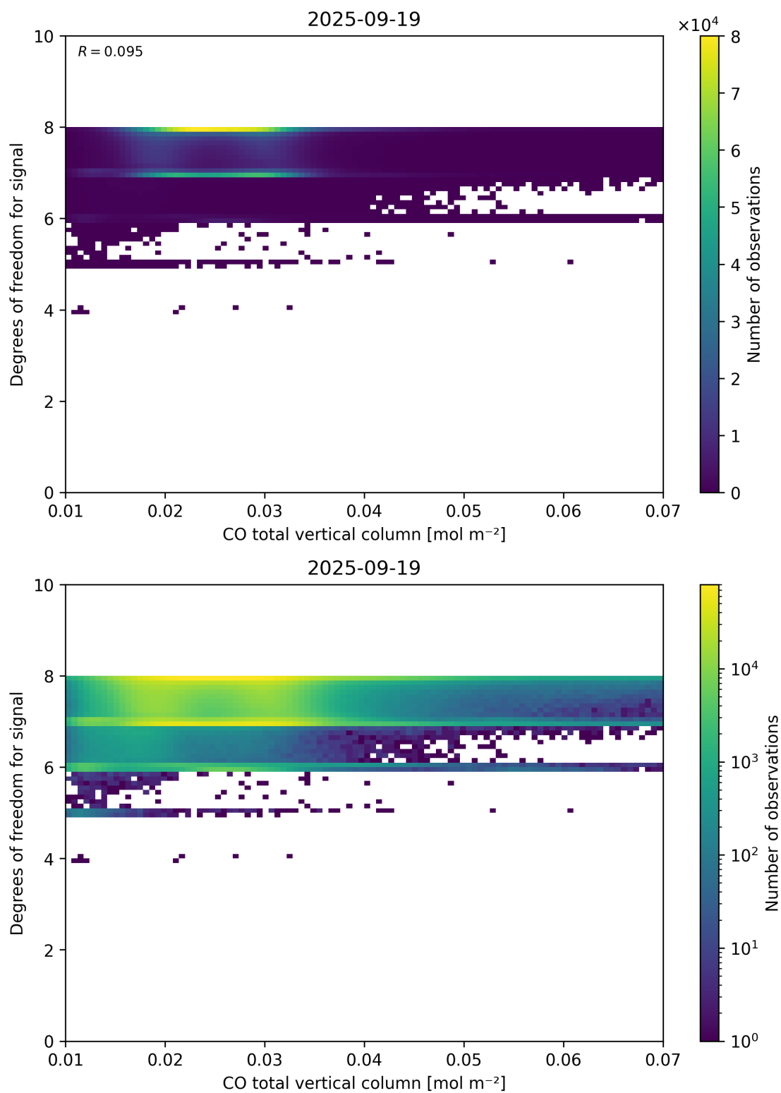
Figure 41: Scatter density plot of “CO total vertical column” against “Degrees of freedom for signal” for 2025-09-18 to 2025-09-20.
