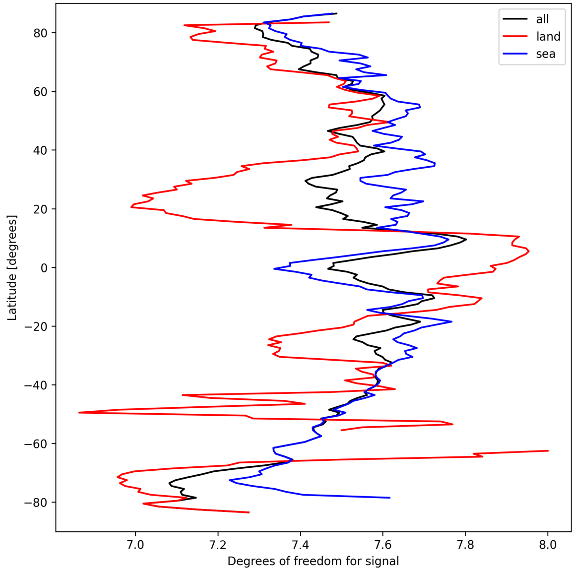
Figure 15: Zonal average of “Degrees of freedom for signal” for 2025-09-18 to 2025-09-20.
