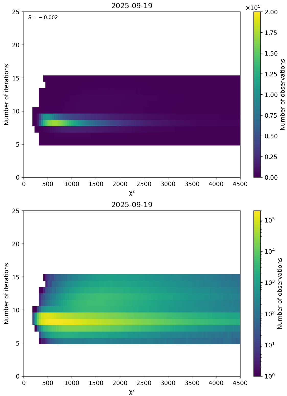
Figure 49: Scatter density plot of “ \chi^2 ” against “Number of iterations” for 2025-09-18 to 2025-09-20.
