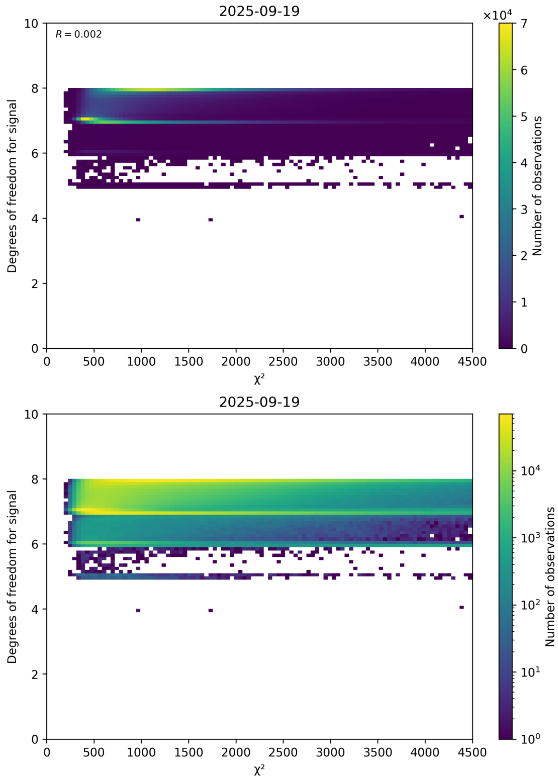
Figure 48: Scatter density plot of “ \chi^2 ” against “Degrees of freedom for signal” for 2025-09-18 to 2025-09-20.
