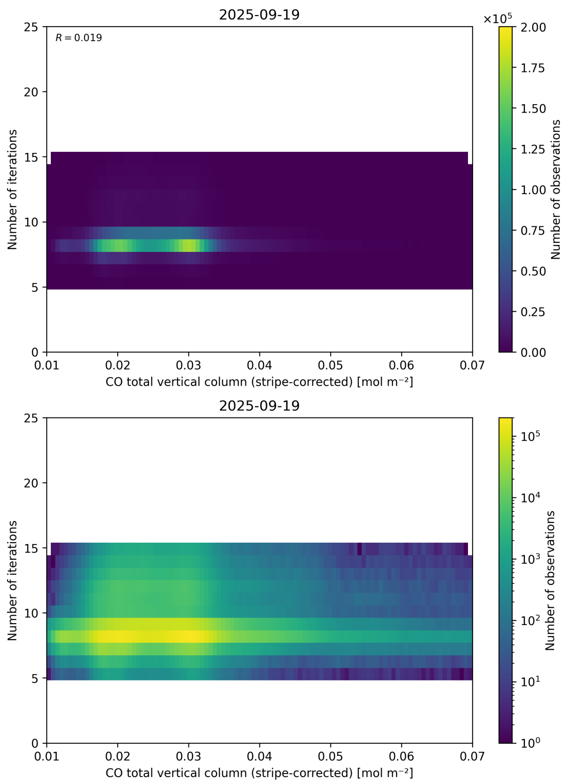
Figure 39: Scatter density plot of “CO total vertical column (stripe-corrected)” against “Number of iterations” for 2025-09-18 to 2025-09-20.
