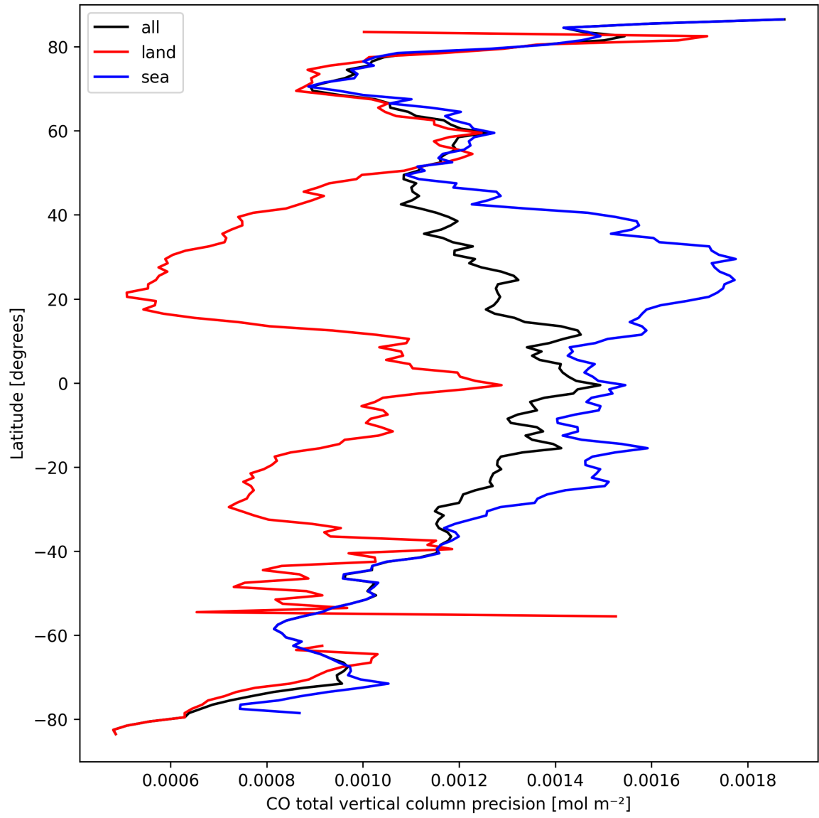
Figure 12: Zonal average of “CO total vertical column precision” for 2025-09-18 to 2025-09-20.
