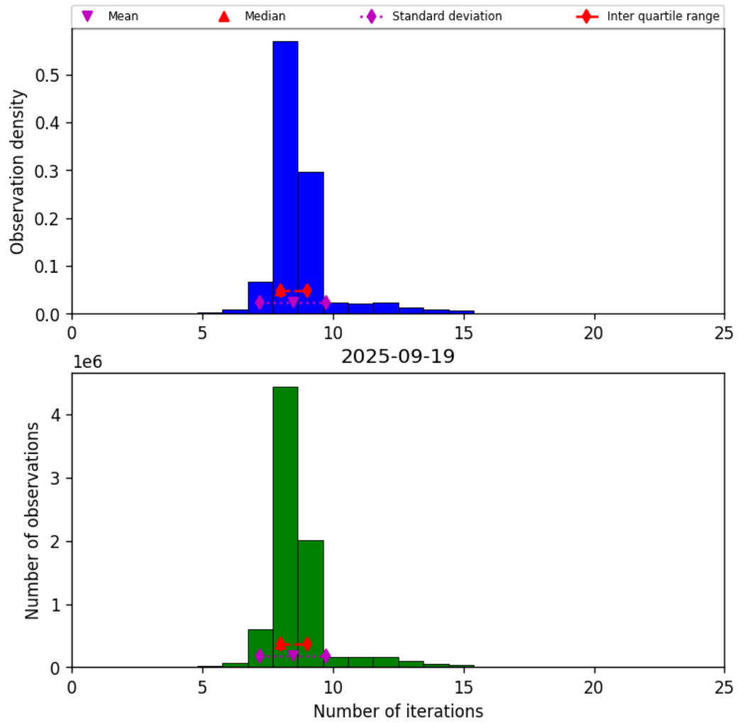
Figure 24: Histogram of “Number of iterations” for 2025-09-18 to 2025-09-20
