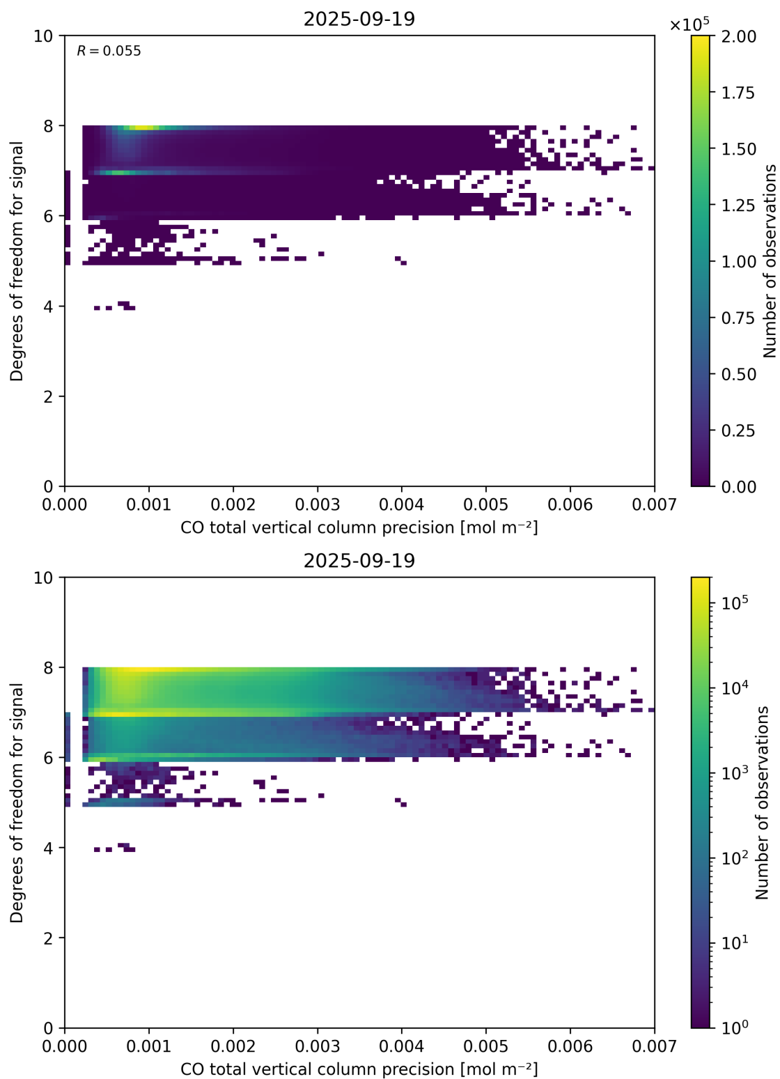
Figure 45: Scatter density plot of “CO total vertical column precision” against “Degrees of freedom for signal” for 2025-09-18 to 2025-09-20.
