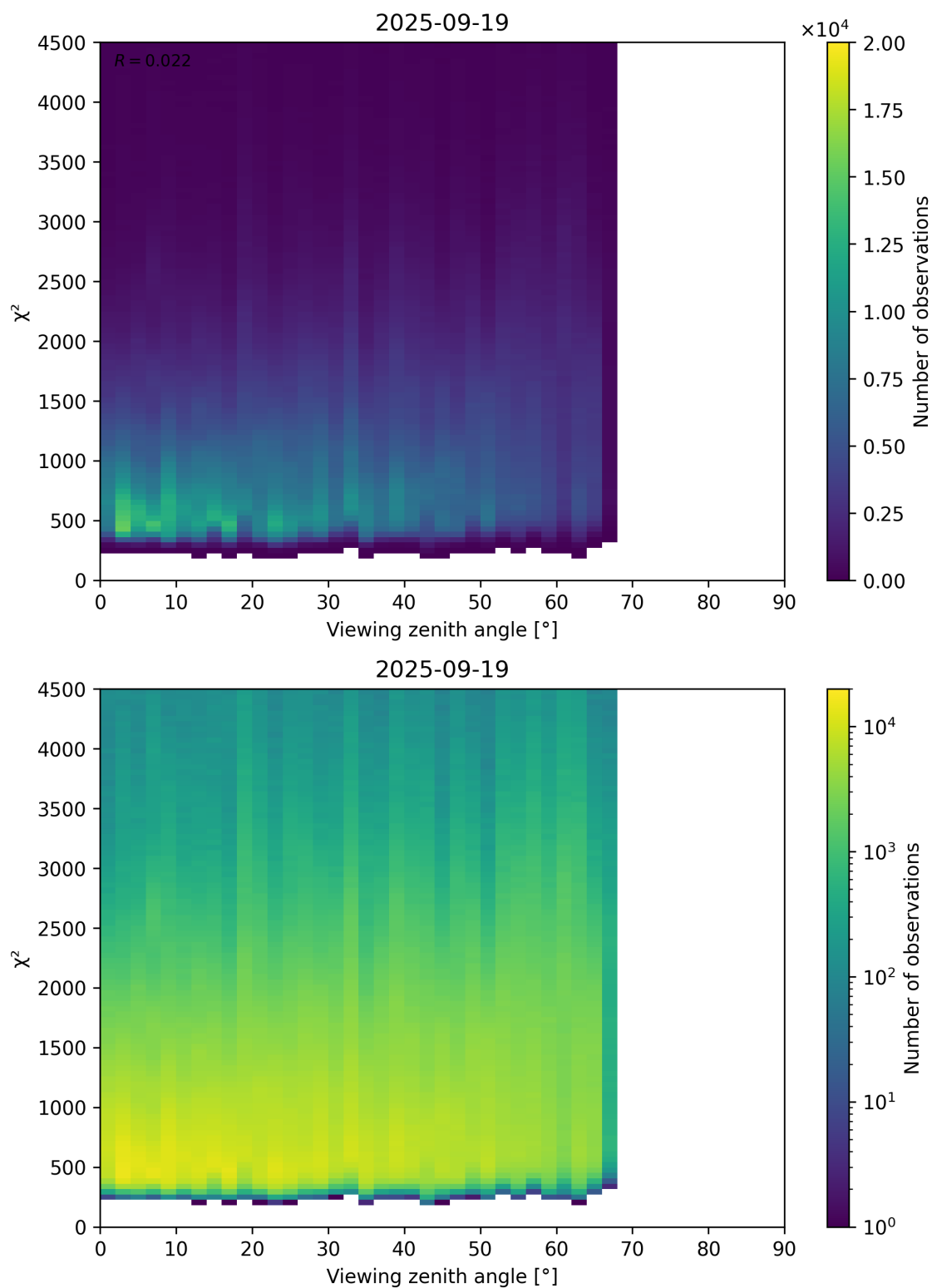
Figure 72: Scatter density plot of “Viewing zenith angle” against “ \chi^2 ” for 2025-09-18 to 2025-09-20.
