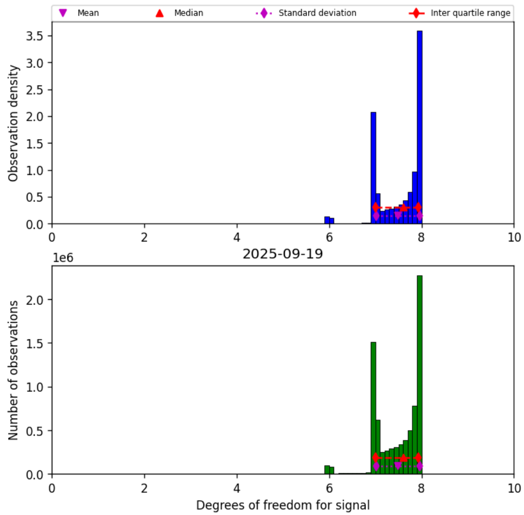
Figure 23: Histogram of “Degrees of freedom for signal” for 2025-09-18 to 2025-09-20
