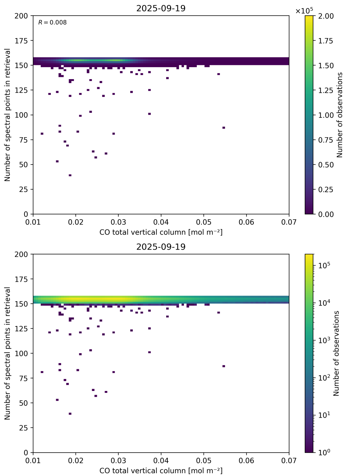
Figure 43: Scatter density plot of “CO total vertical column” against “Number of spectral points in retrieval” for 2025-09-18 to 2025-09-20.
