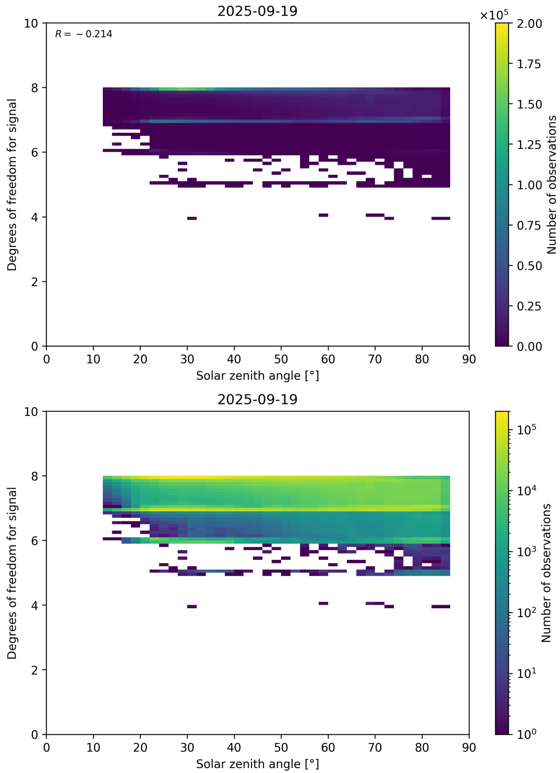
Figure 65: Scatter density plot of “Solar zenith angle” against “Degrees of freedom for signal” for 2025-09-18 to 2025-09-20.
