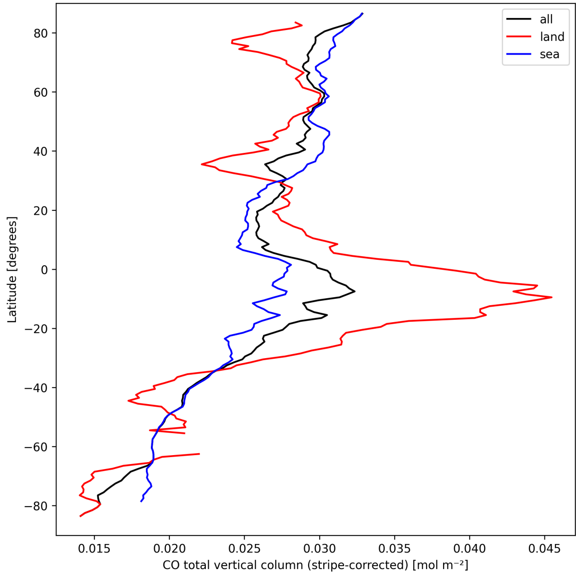
Figure 11: Zonal average of “CO total vertical column (stripe-corrected)” for 2025-09-18 to 2025-09-20.
