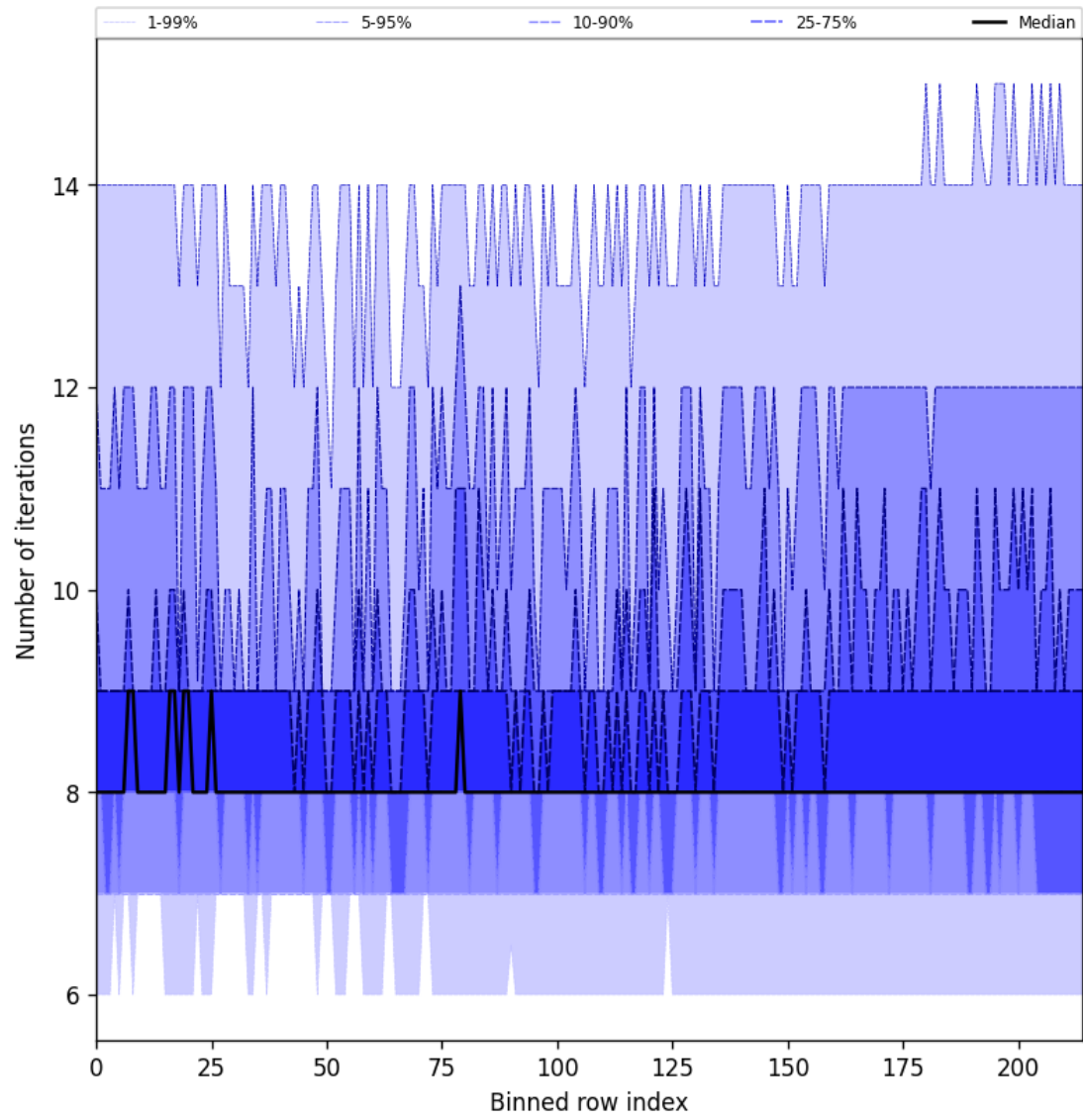
Figure 32: Along track statistics of “Number of iterations” for 2025-09-18 to 2025-09-20
