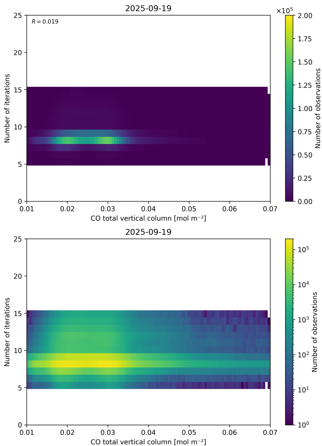
Figure 42: Scatter density plot of “CO total vertical column” against “Number of iterations” for 2025-09-18 to 2025-09-20.
