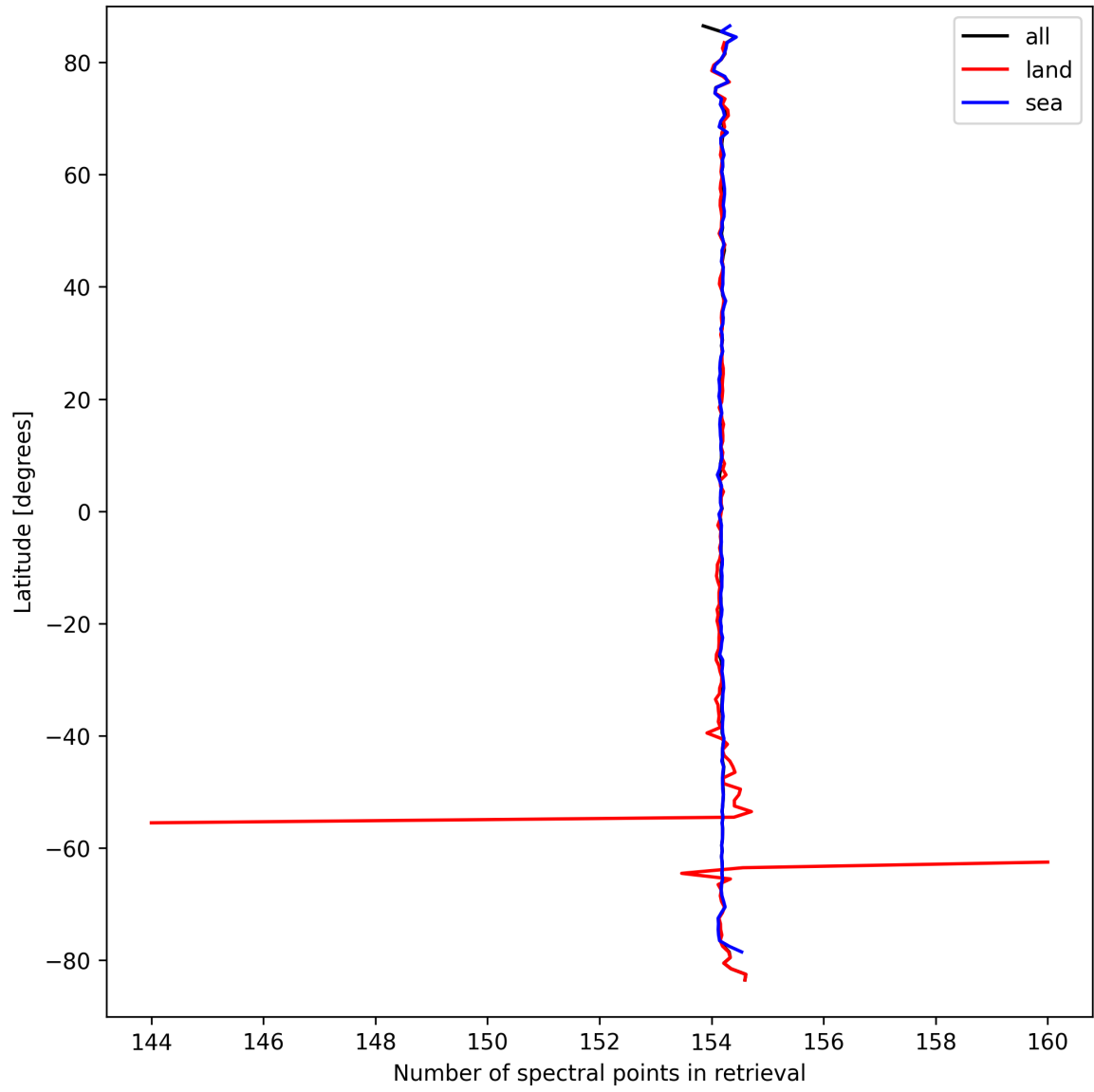
Figure 13: Zonal average of “Number of spectral points in retrieval” for 2025-09-18 to 2025-09-20.
