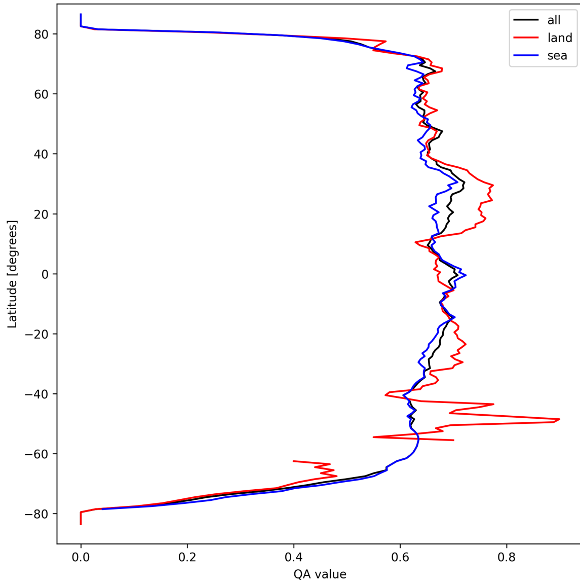
Figure 9: Zonal average of “QA value” for 2025-09-18 to 2025-09-20.
