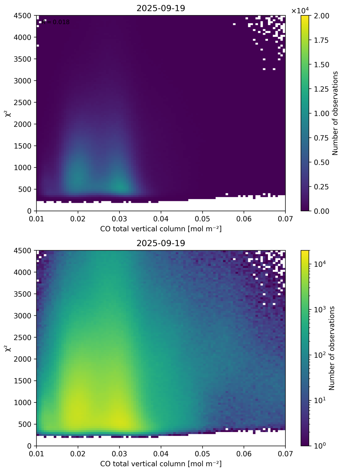
Figure 35: Scatter density plot of “CO total vertical column” against “ \chi^2 ” for 2025-09-18 to 2025-09-20.
