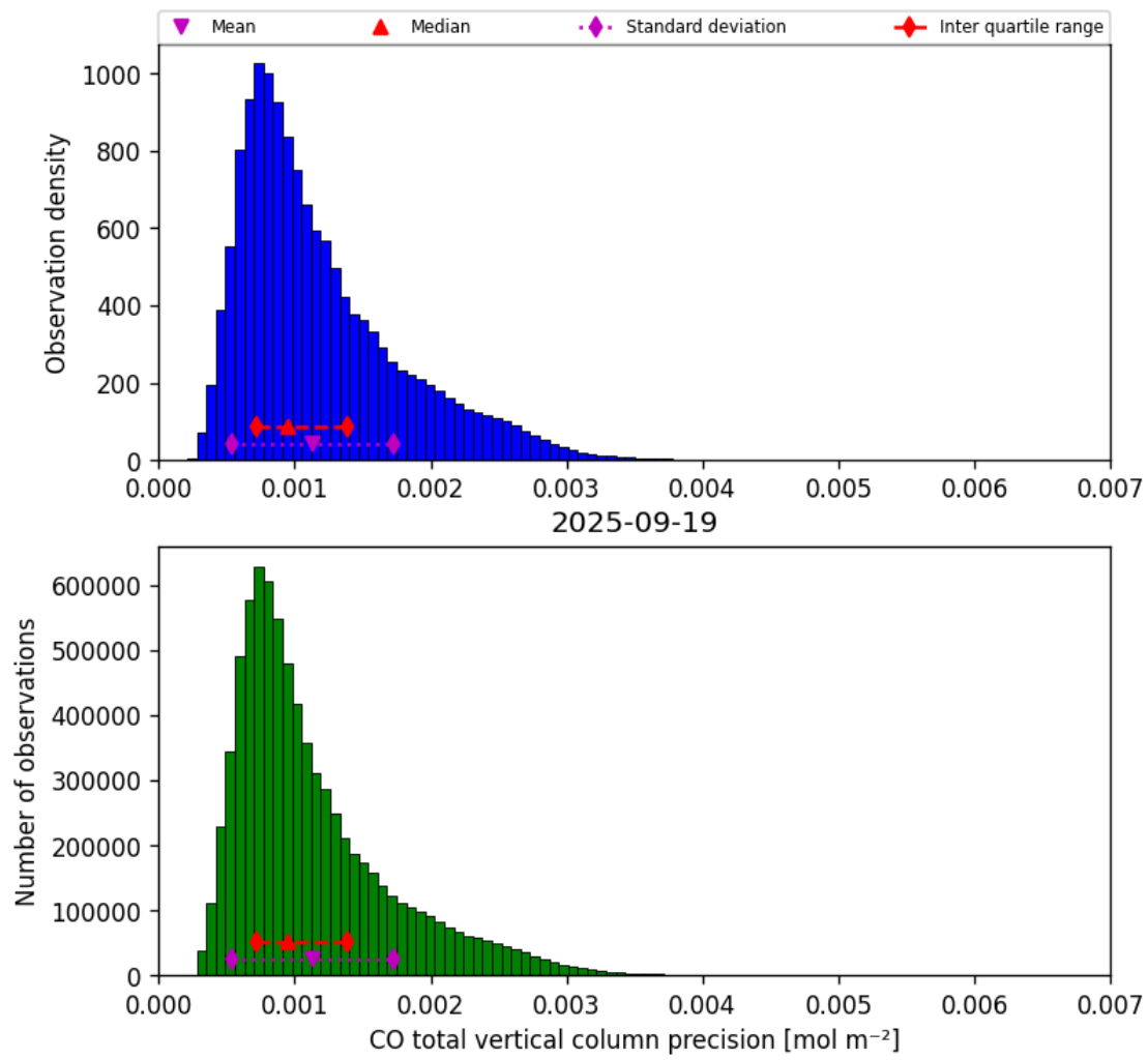
Figure 20: Histogram of “CO total vertical column precision” for 2025-09-18 to 2025-09-20
