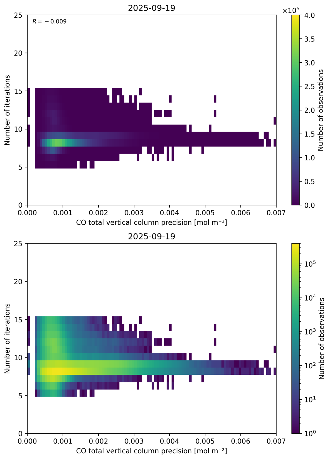
Figure 46: Scatter density plot of “CO total vertical column precision” against “Number of iterations” for 2025-09-18 to 2025-09-20.
