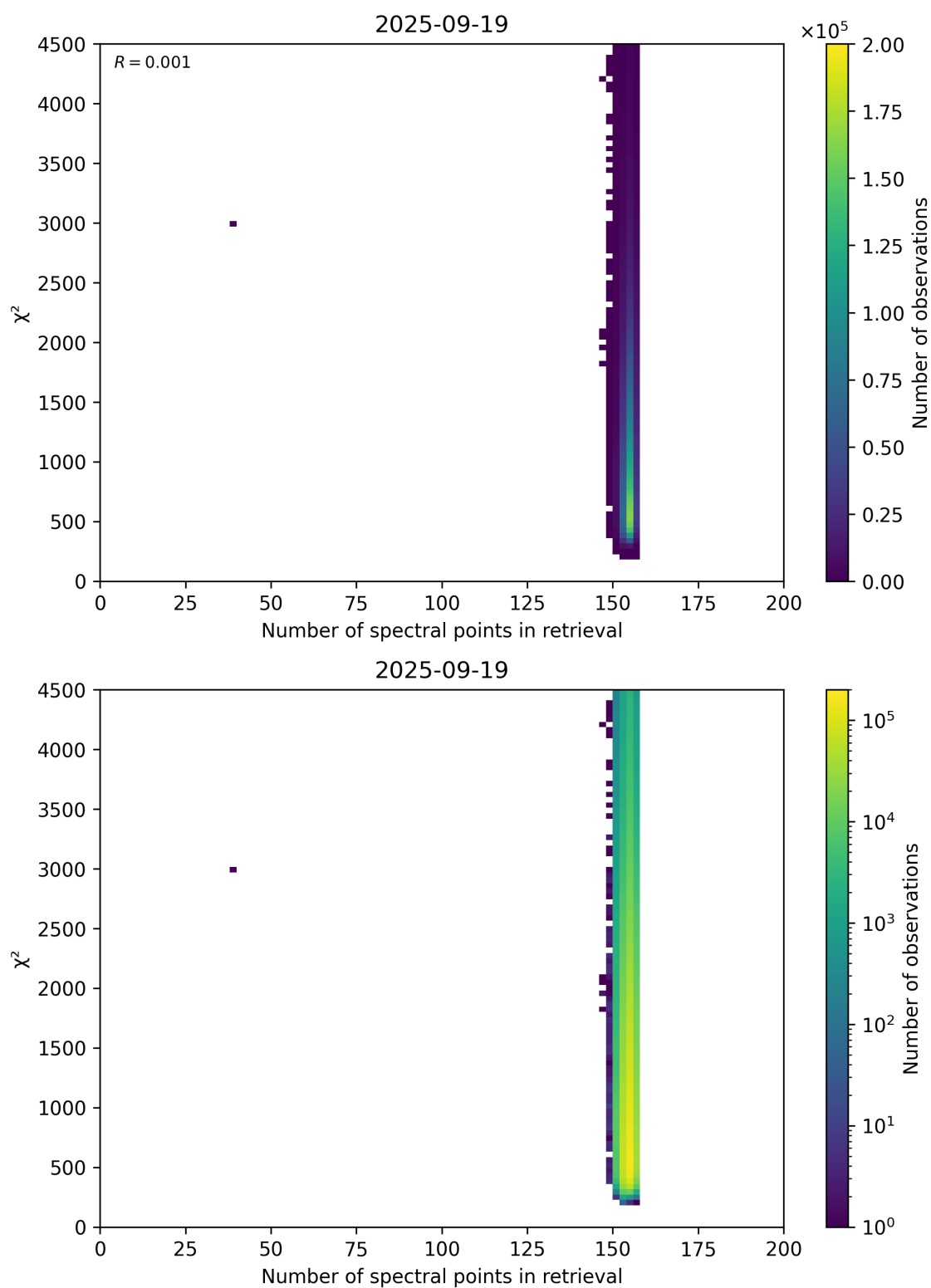
Figure 58: Scatter density plot of “Number of spectral points in retrieval” against “ \chi^2 ” for 2025-09-18 to 2025-09-20.
