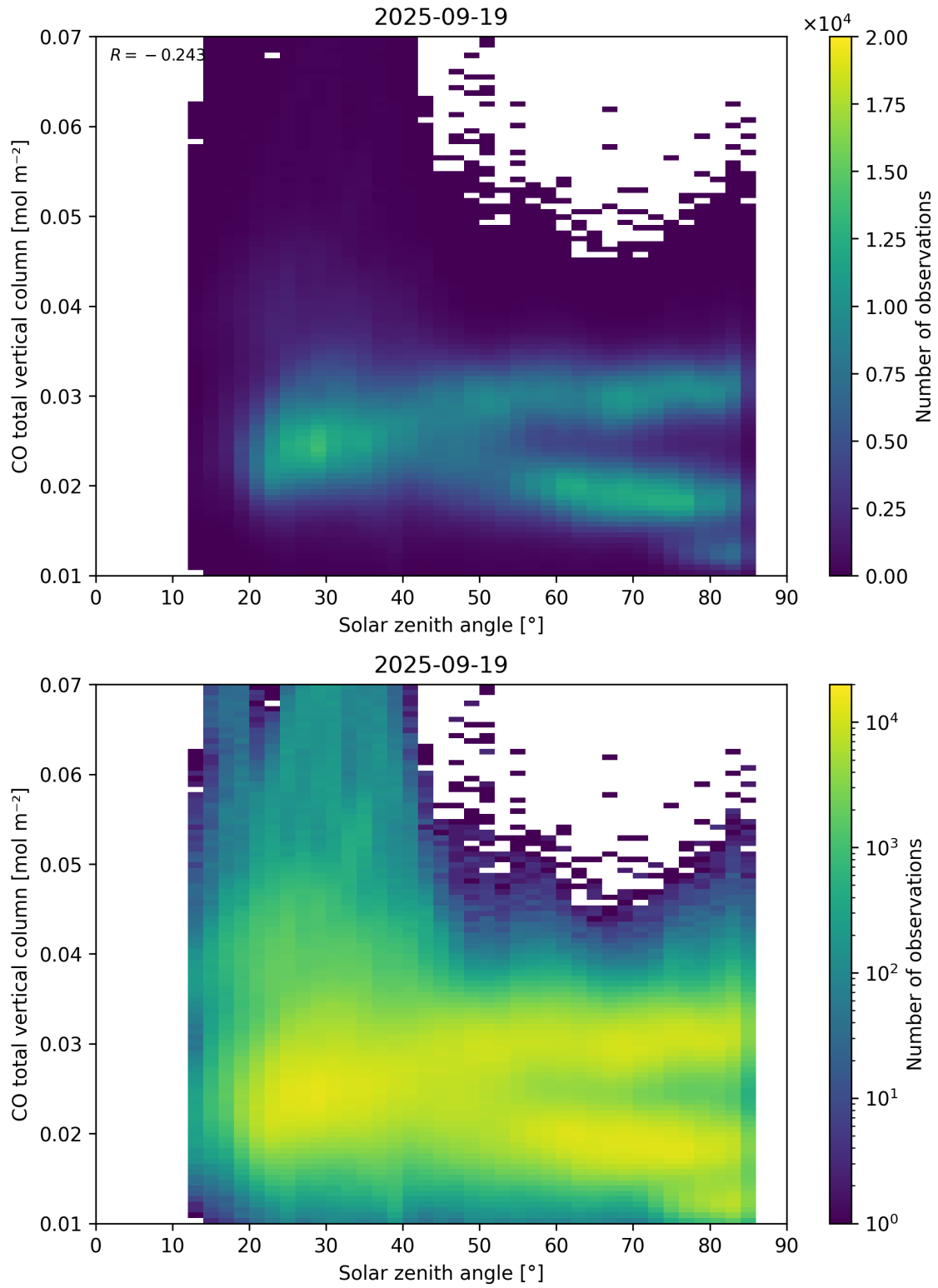
Figure 61: Scatter density plot of “Solar zenith angle” against “CO total vertical column” for 2025-09-18 to 2025-09-20.
