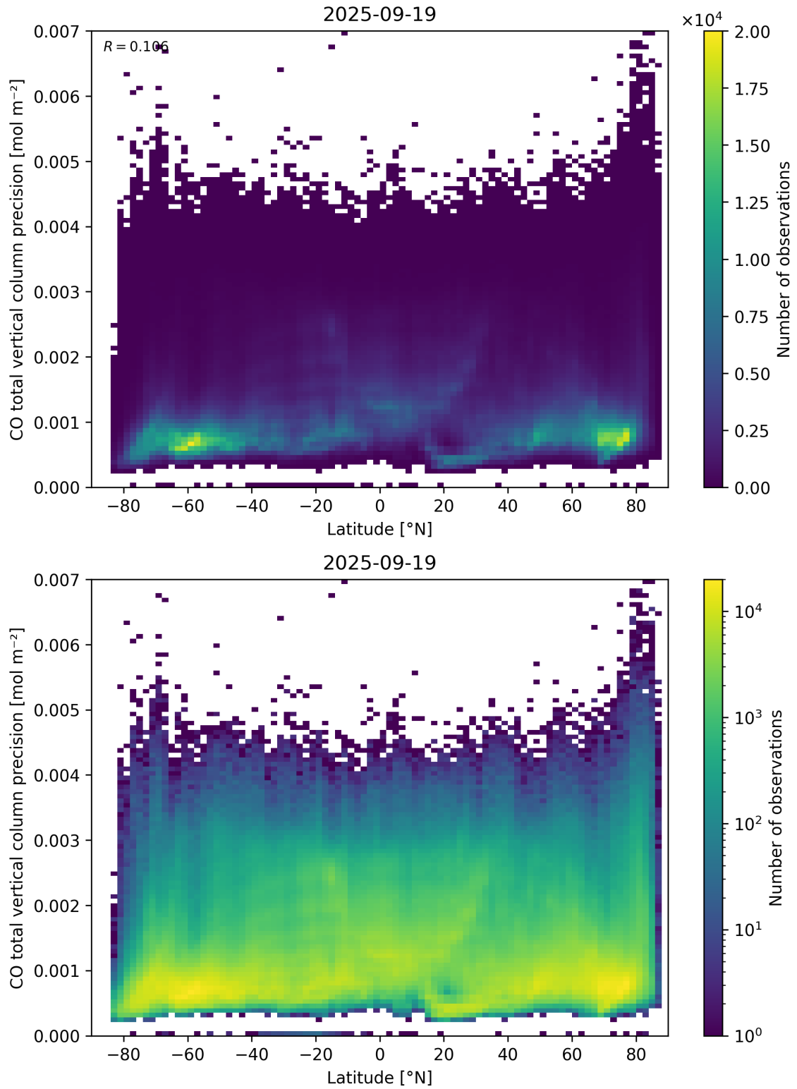
Figure 53: Scatter density plot of “Latitude” against “CO total vertical column precision” for 2025-09-18 to 2025-09-20.
