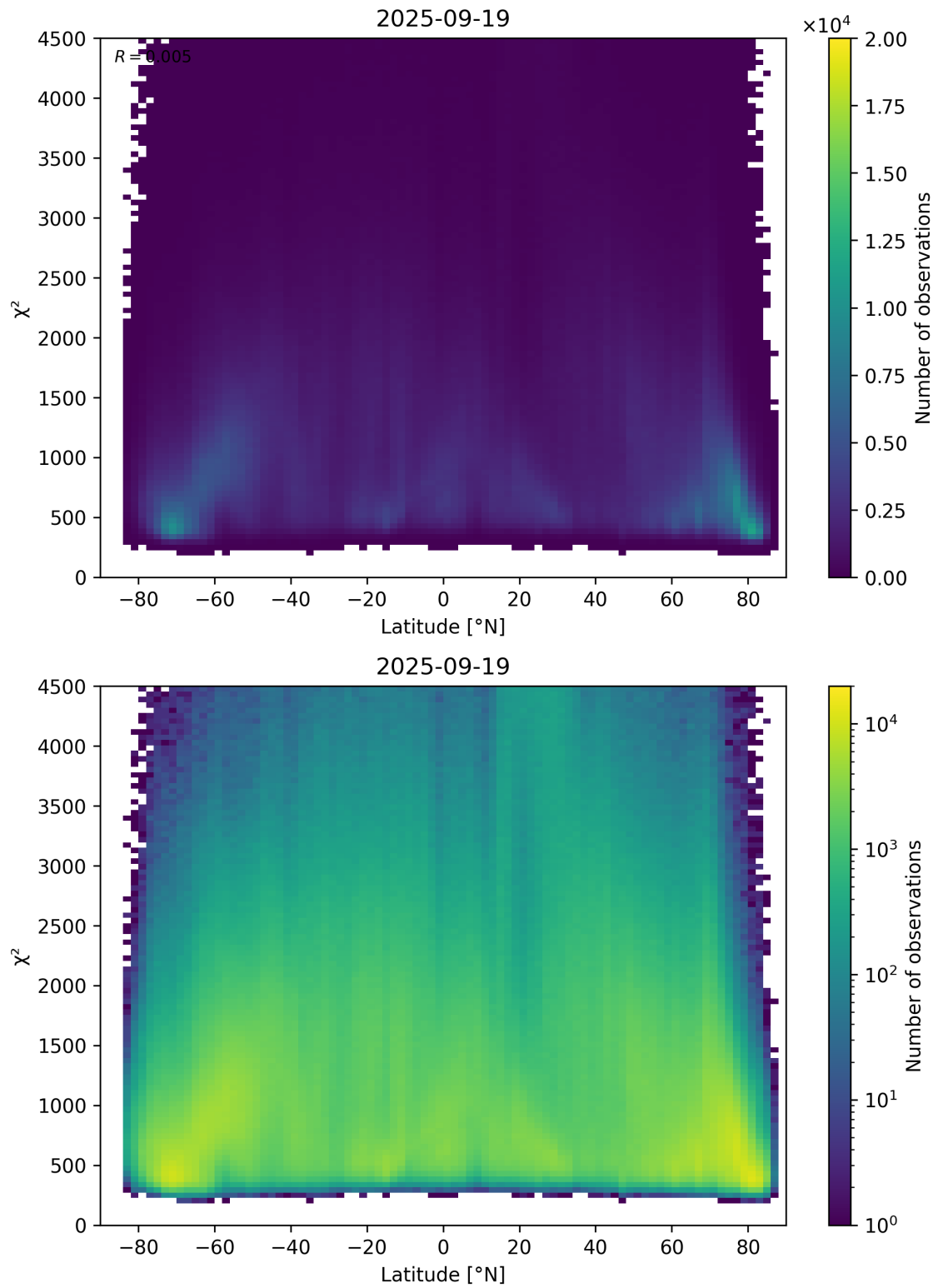
Figure 54: Scatter density plot of “Latitude” against “ \chi^2 ” for 2025-09-18 to 2025-09-20.
