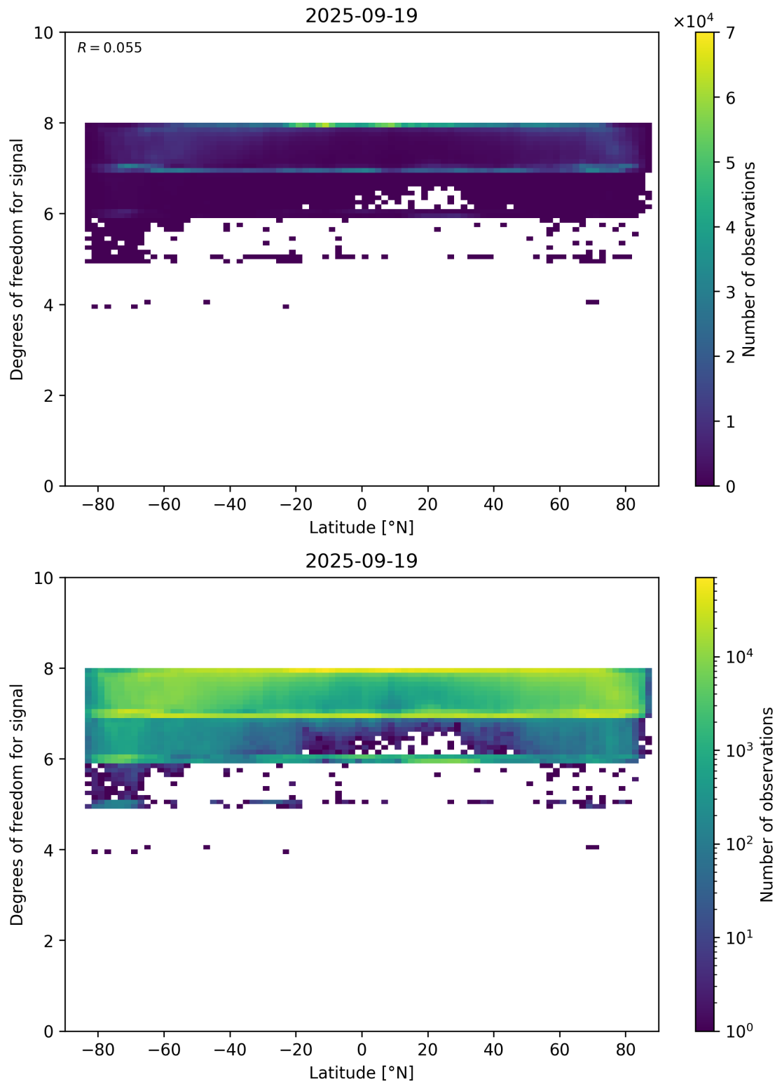
Figure 55: Scatter density plot of “Latitude” against “Degrees of freedom for signal” for 2025-09-18 to 2025-09-20.
