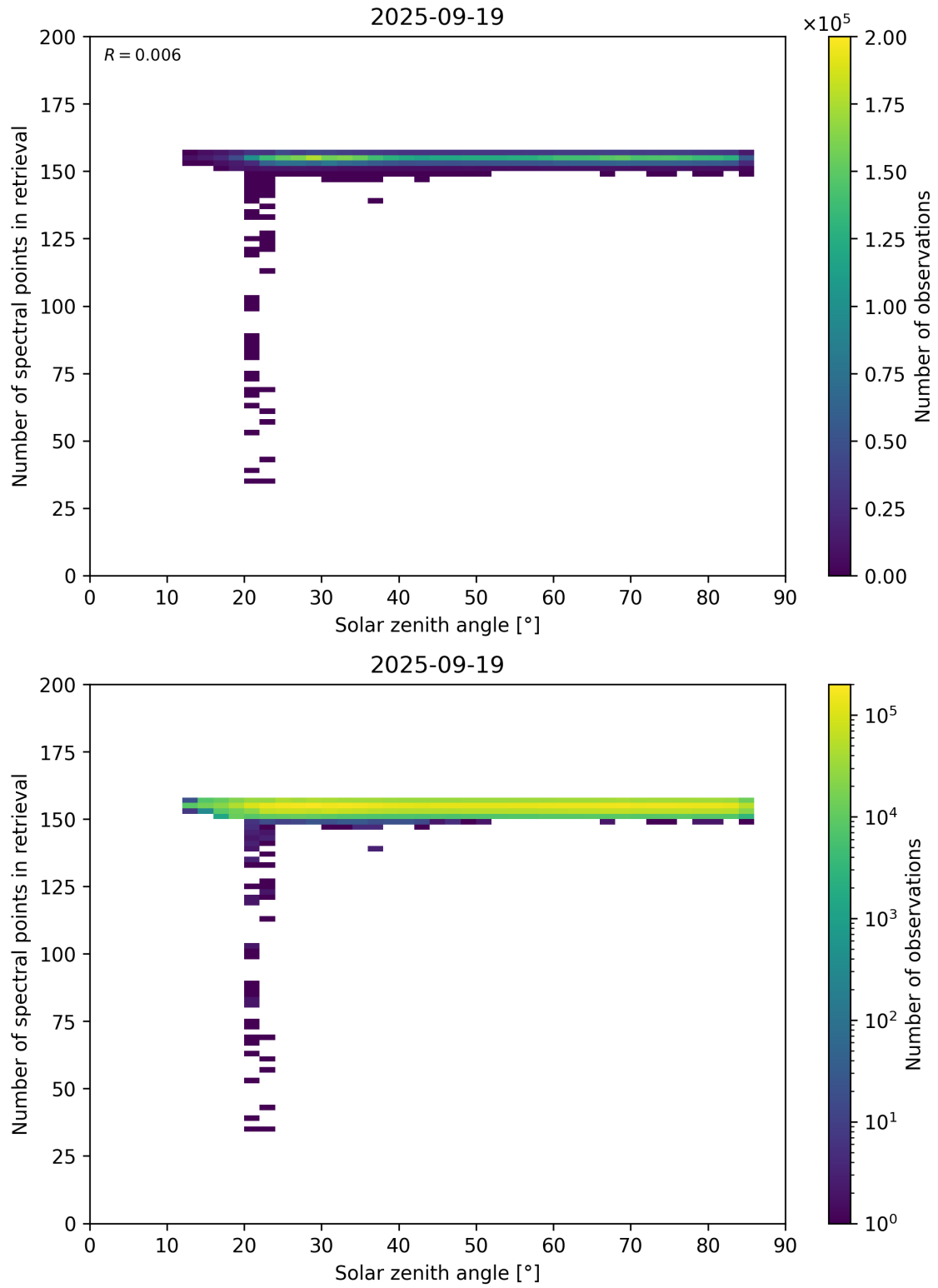
Figure 68: Scatter density plot of “Solar zenith angle” against “Number of spectral points in retrieval” for 2025-09-18 to 2025-09-20.
