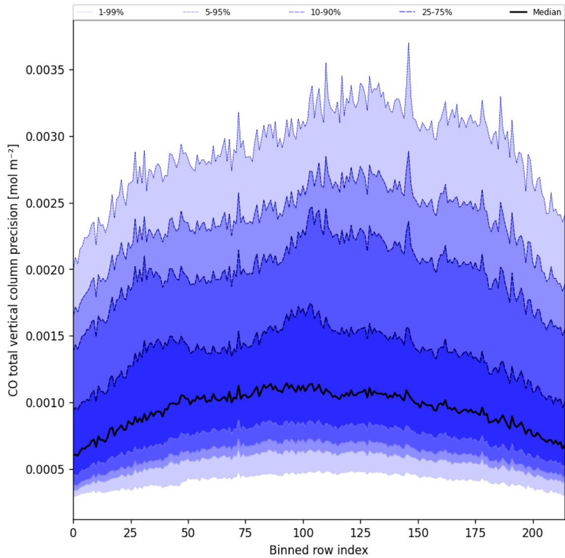
Figure 28: Along track statistics of “CO total vertical column precision” for 2025-09-18 to 2025-09-20
