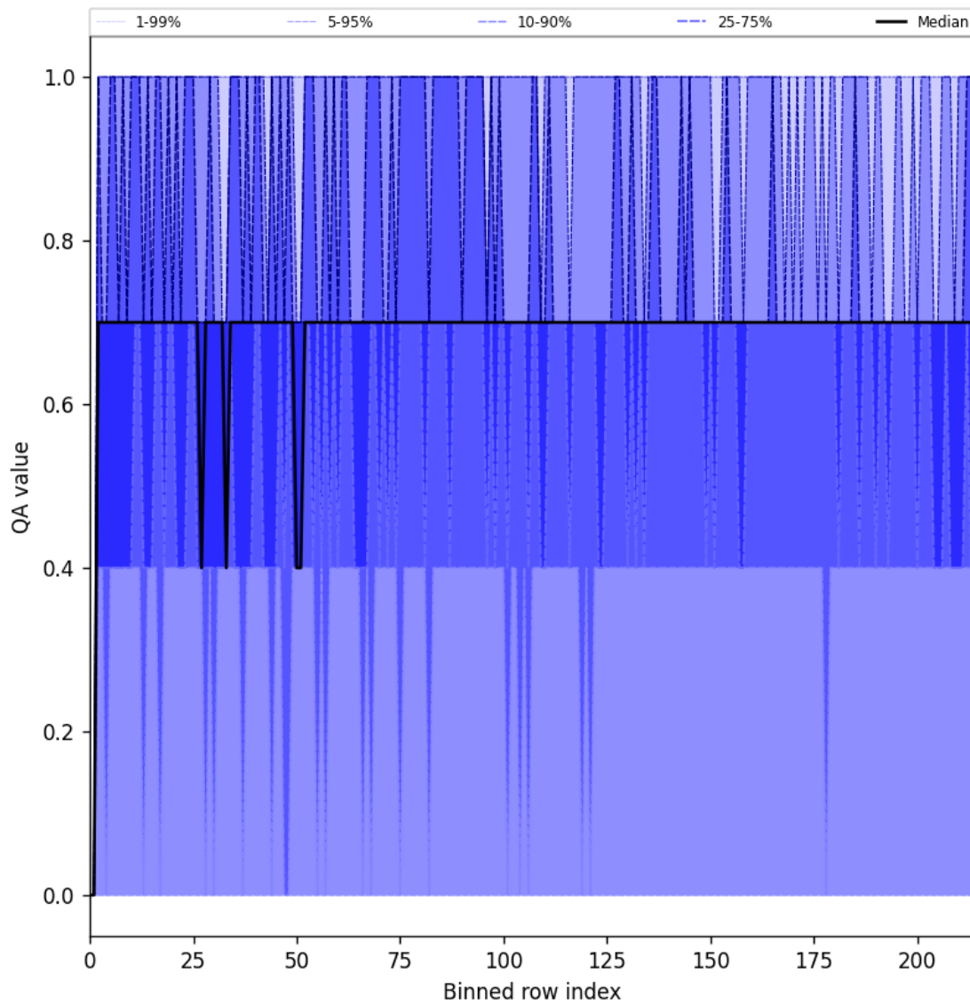
Figure 25: Along track statistics of “QA value” for 2025-09-18 to 2025-09-20
