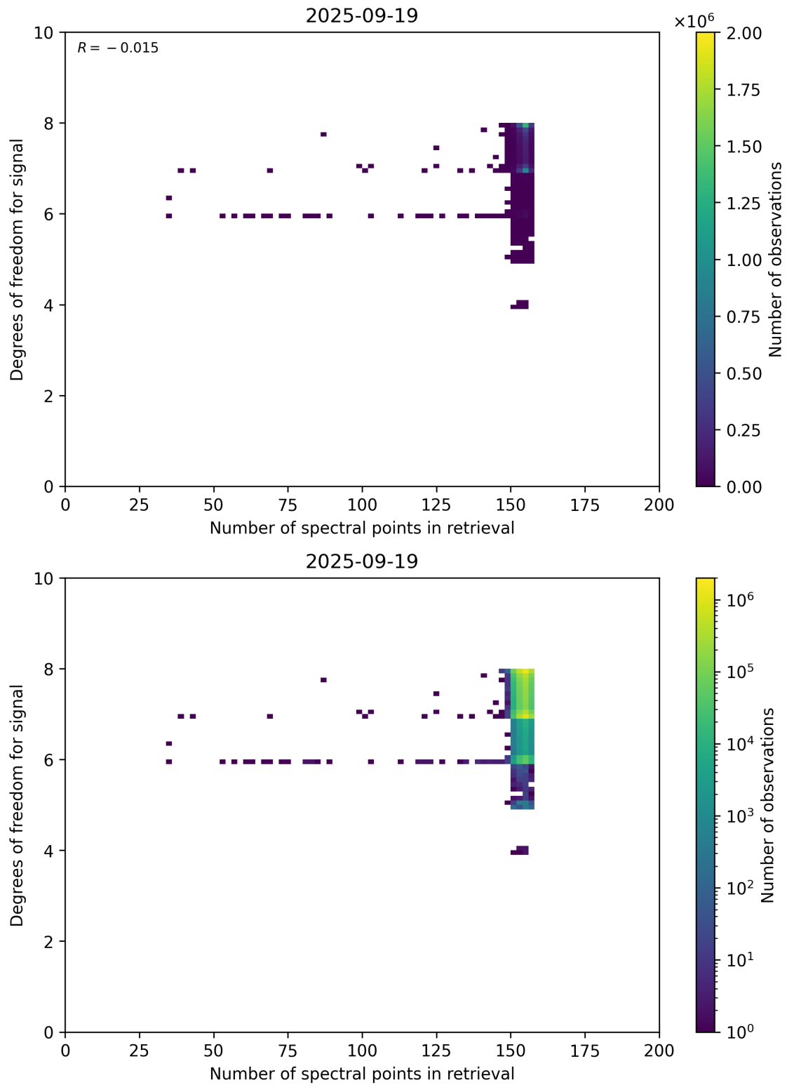
Figure 59: Scatter density plot of “Number of spectral points in retrieval” against “Degrees of freedom for signal” for 2025-09-18 to 2025-09-20.
