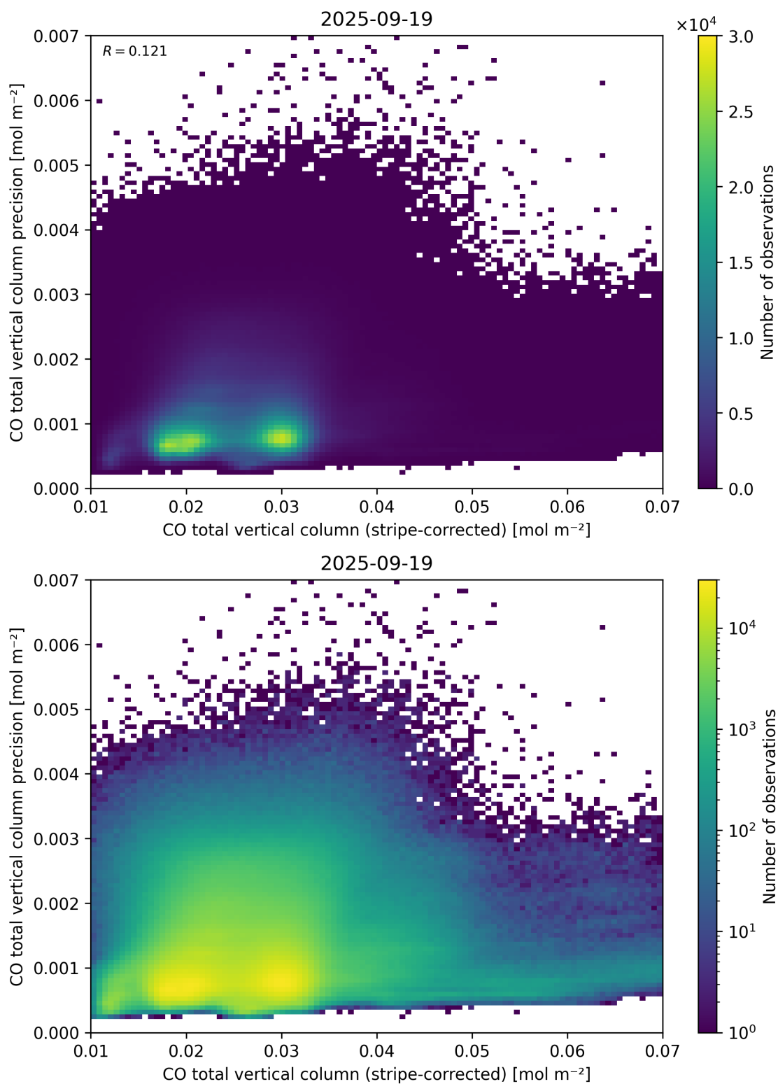
Figure 36: Scatter density plot of “CO total vertical column (stripe-corrected)” against “CO total vertical column precision” for 2025-09-18 to 2025-09-20.
