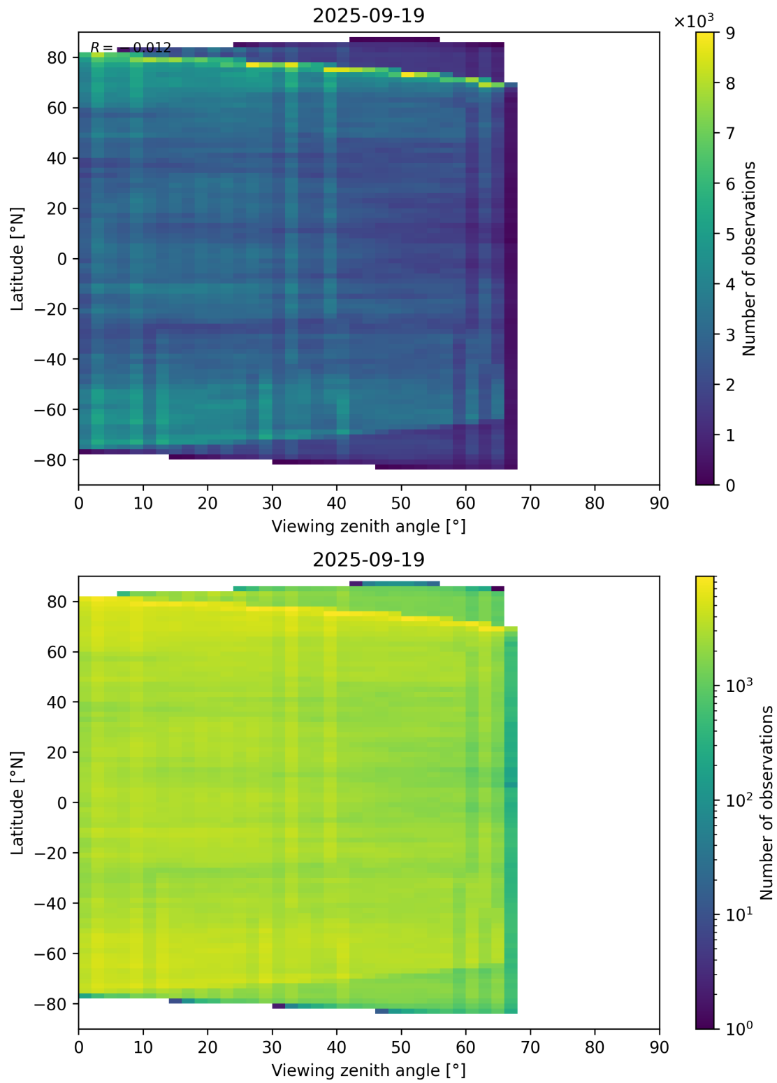
Figure 74: Scatter density plot of “Viewing zenith angle” against “Latitude” for 2025-09-18 to 2025-09-20.
