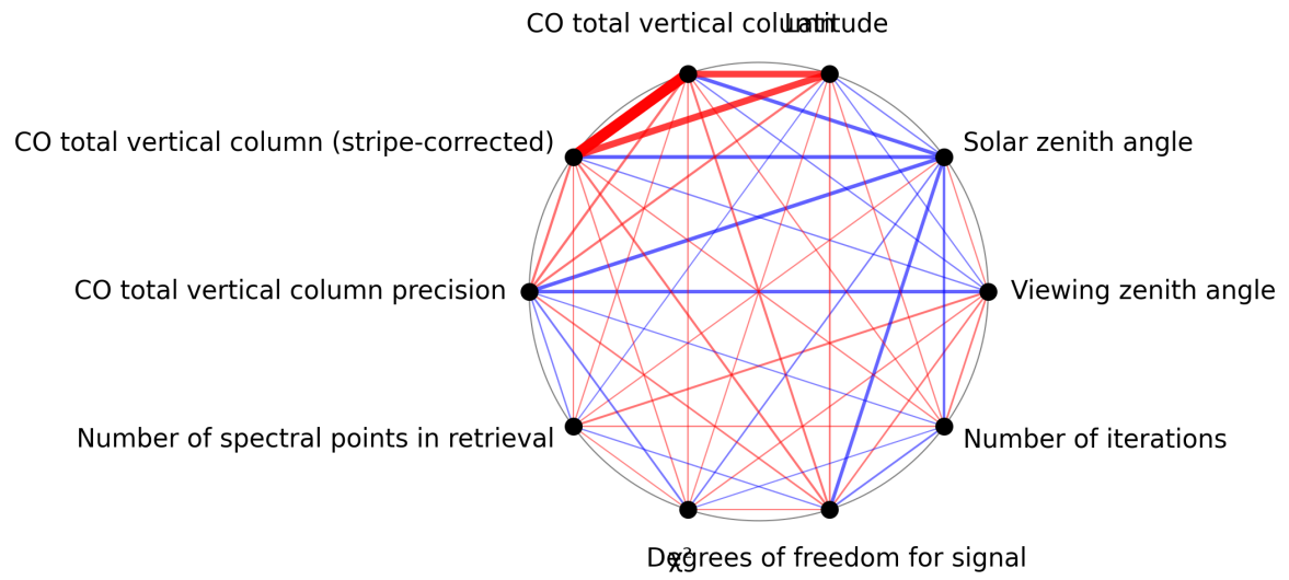
Figure 1: Map of correlation graph for 2025-09-18 to 2025-09-20.
