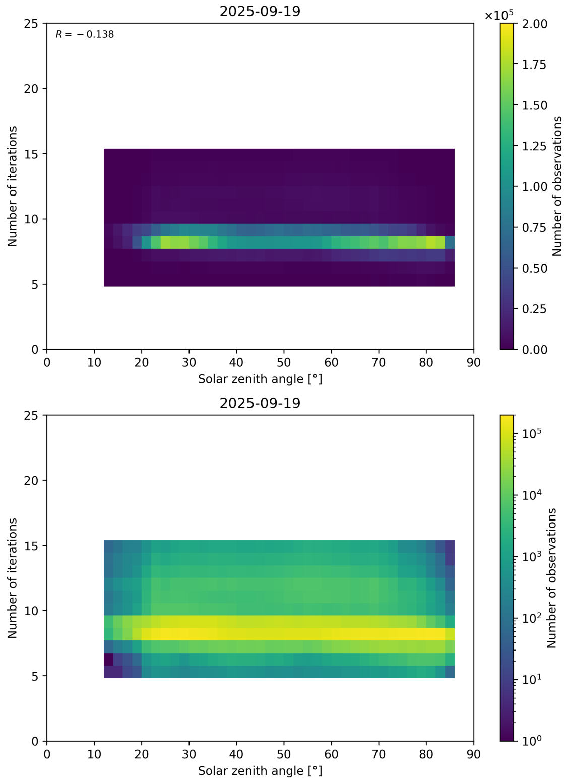
Figure 67: Scatter density plot of “Solar zenith angle” against “Number of iterations” for 2025-09-18 to 2025-09-20.
