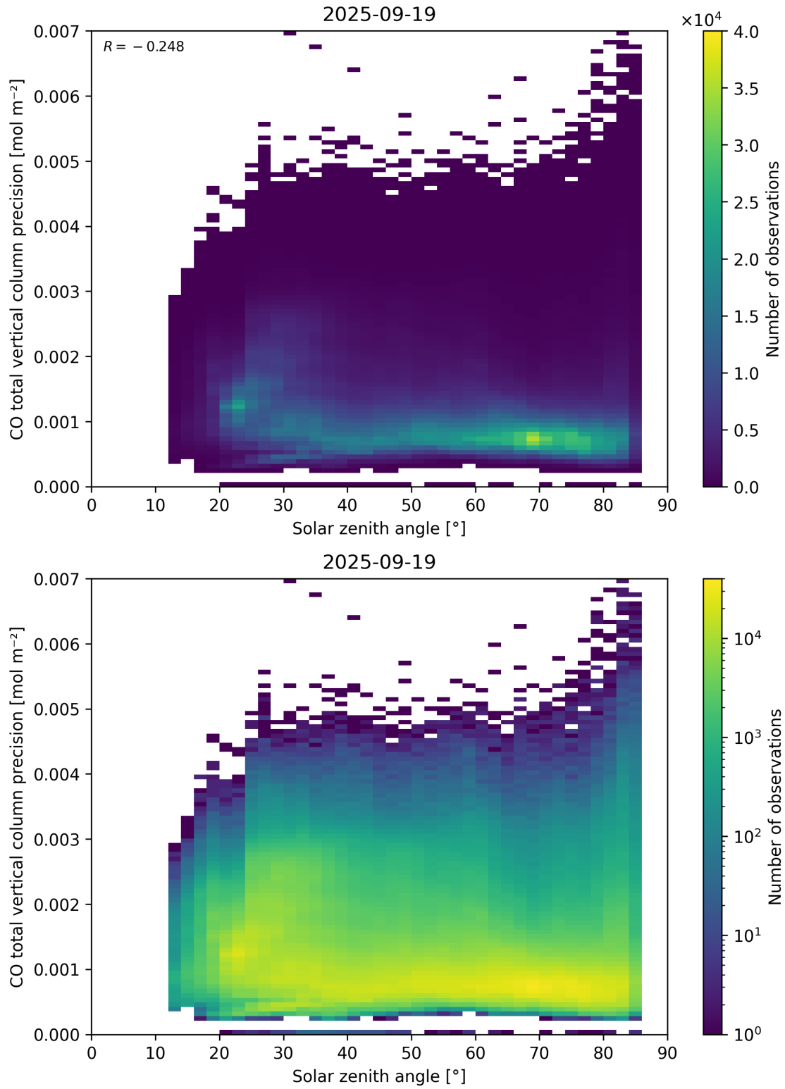
Figure 63: Scatter density plot of “Solar zenith angle” against “CO total vertical column precision” for 2025-09-18 to 2025-09-20.
