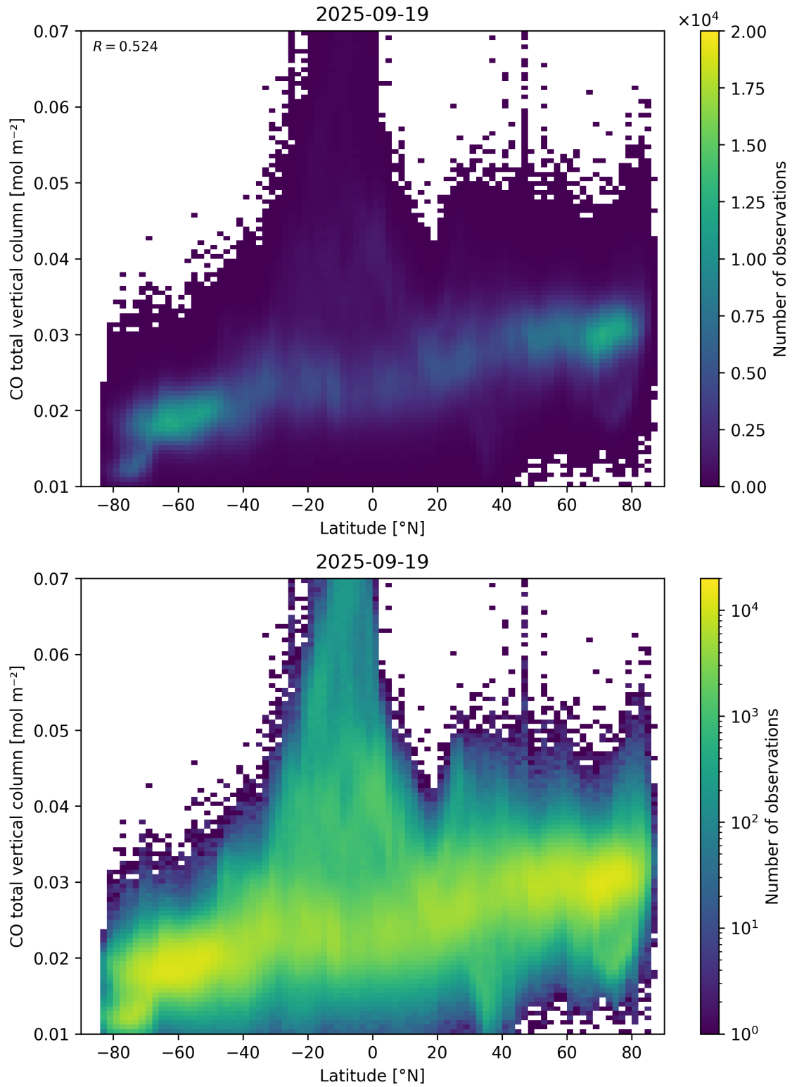
Figure 51: Scatter density plot of “Latitude” against “CO total vertical column” for 2025-09-18 to 2025-09-20.
