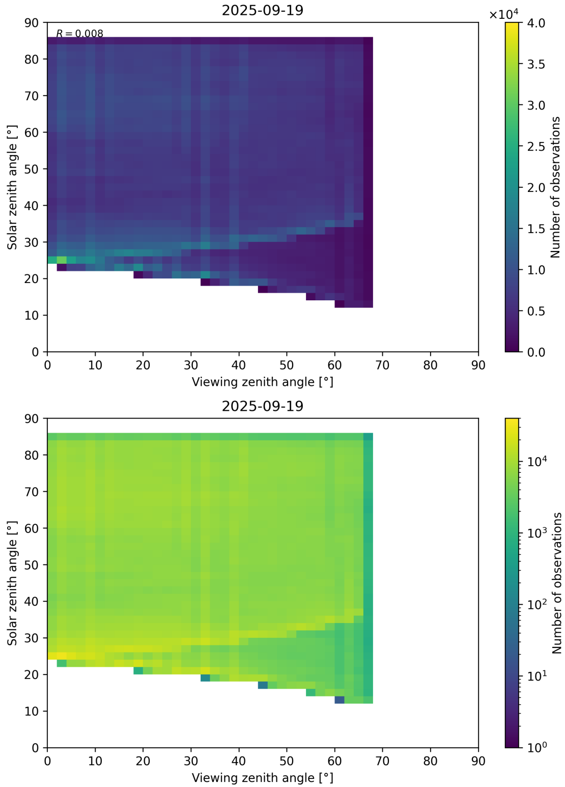
Figure 77: Scatter density plot of “Viewing zenith angle” against “Solar zenith angle” for 2025-09-18 to 2025-09-20.
