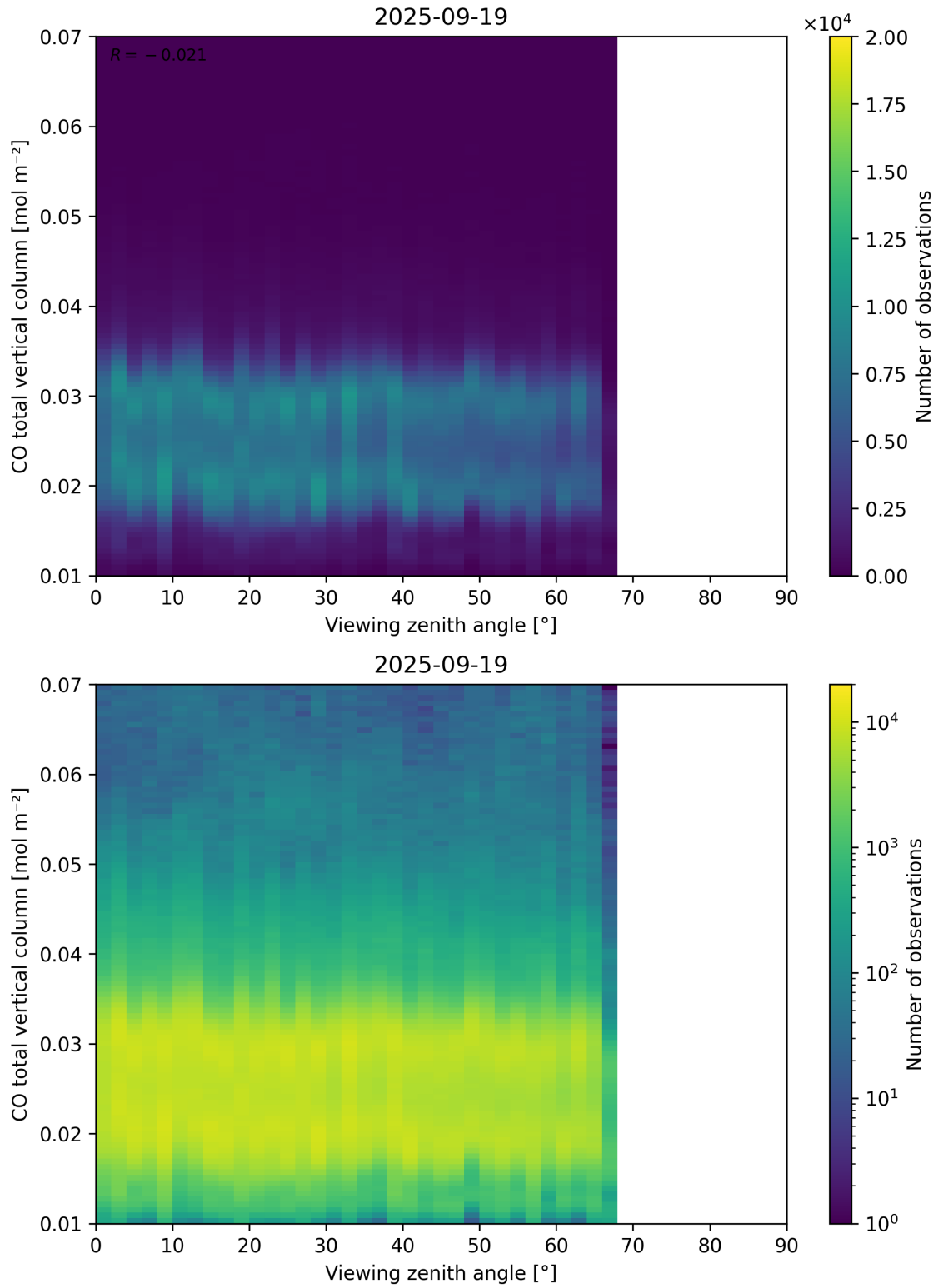
Figure 69: Scatter density plot of “Viewing zenith angle” against “CO total vertical column” for 2025-09-18 to 2025-09-20.
