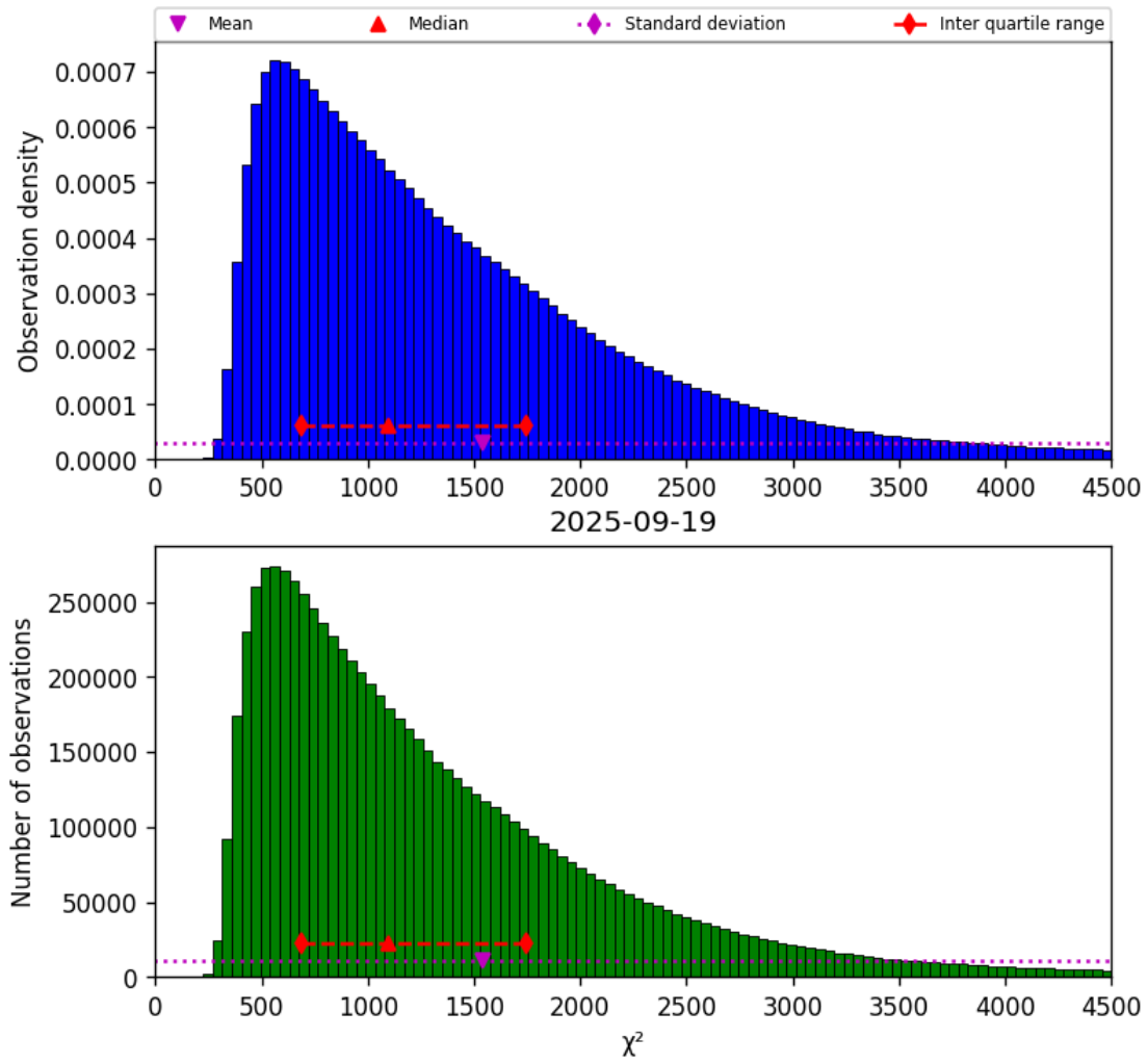
Figure 22: Histogram of “ \chi^2 ” for 2025-09-18 to 2025-09-20
