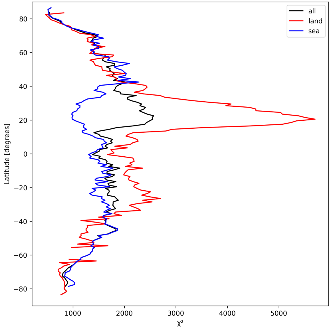
Figure 14: Zonal average of “ \chi^2 ” for 2025-09-18 to 2025-09-20.
