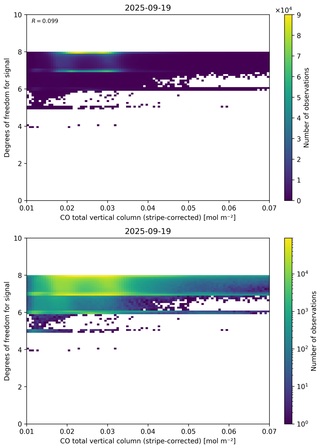
Figure 38: Scatter density plot of “CO total vertical column (stripe-corrected)” against “Degrees of freedom for signal” for 2025-09-18 to 2025-09-20.
