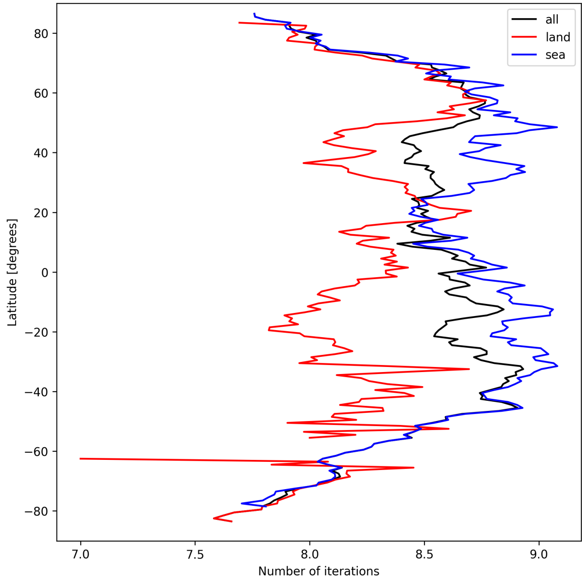
Figure 16: Zonal average of “Number of iterations” for 2025-09-18 to 2025-09-20.
