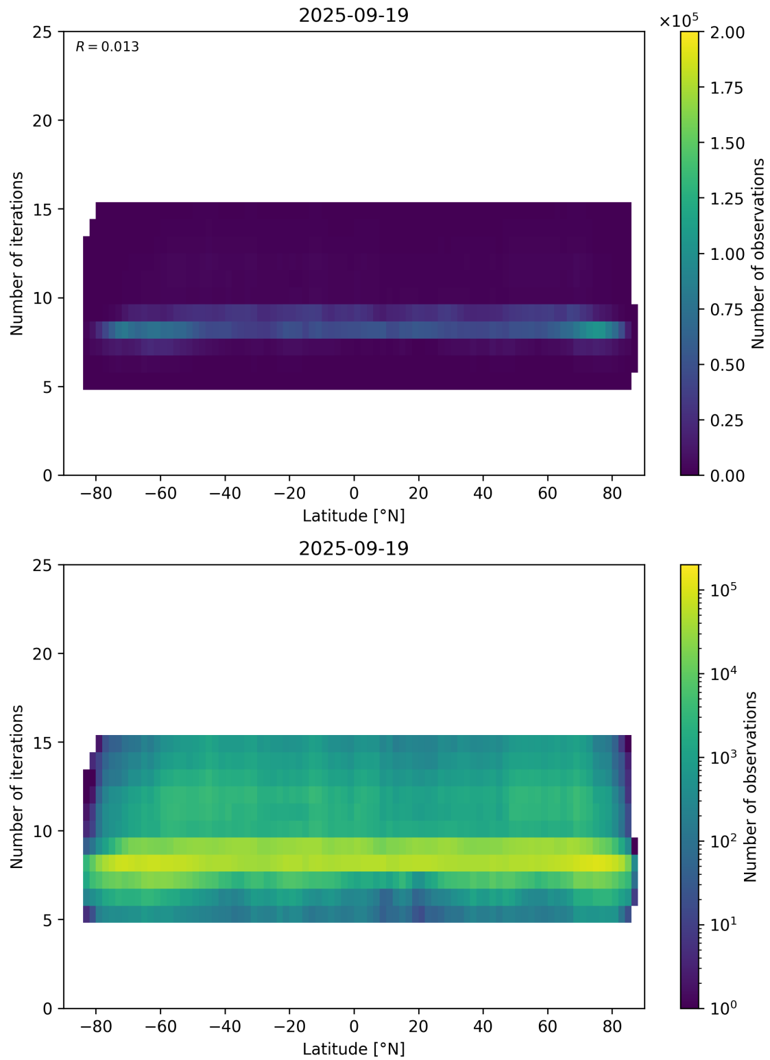
Figure 56: Scatter density plot of “Latitude” against “Number of iterations” for 2025-09-18 to 2025-09-20.
