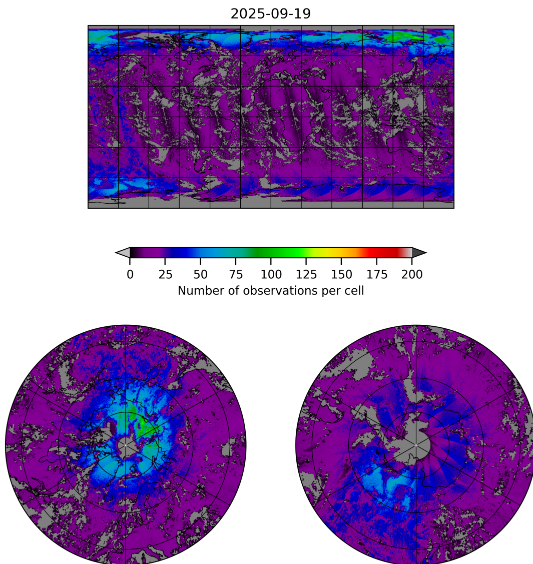
Figure 8: Map of the number of observations for 2025-09-18 to 2025-09-20
