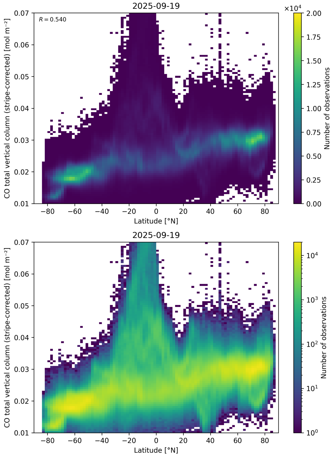
Figure 52: Scatter density plot of “Latitude” against “CO total vertical column (stripe-corrected)” for 2025-09-18 to 2025-09-20.
