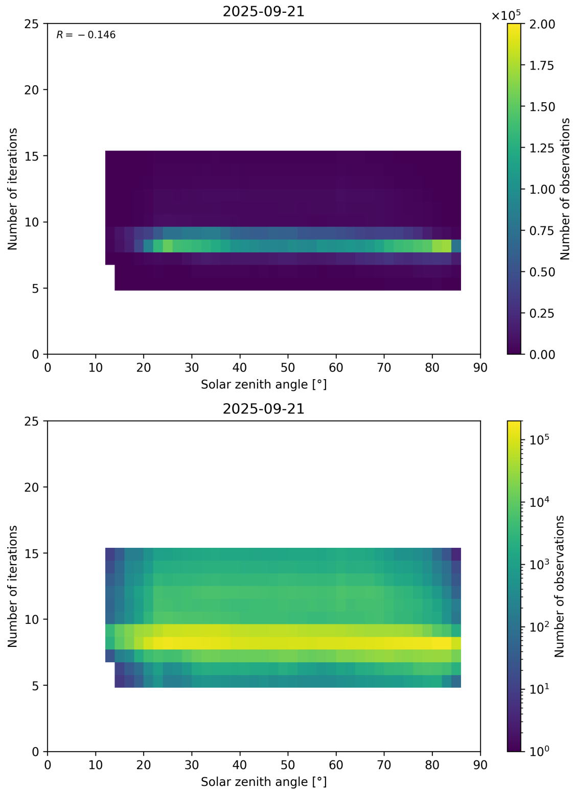
Figure 67: Scatter density plot of “Solar zenith angle” against “Number of iterations” for 2025-09-20 to 2025-09-22.
