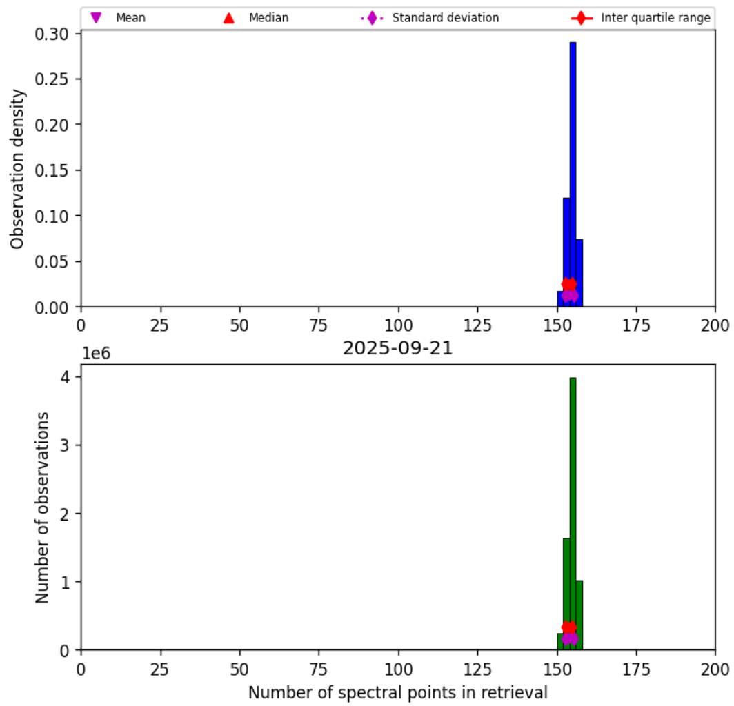
Figure 21: Histogram of “Number of spectral points in retrieval” for 2025-09-20 to 2025-09-22
