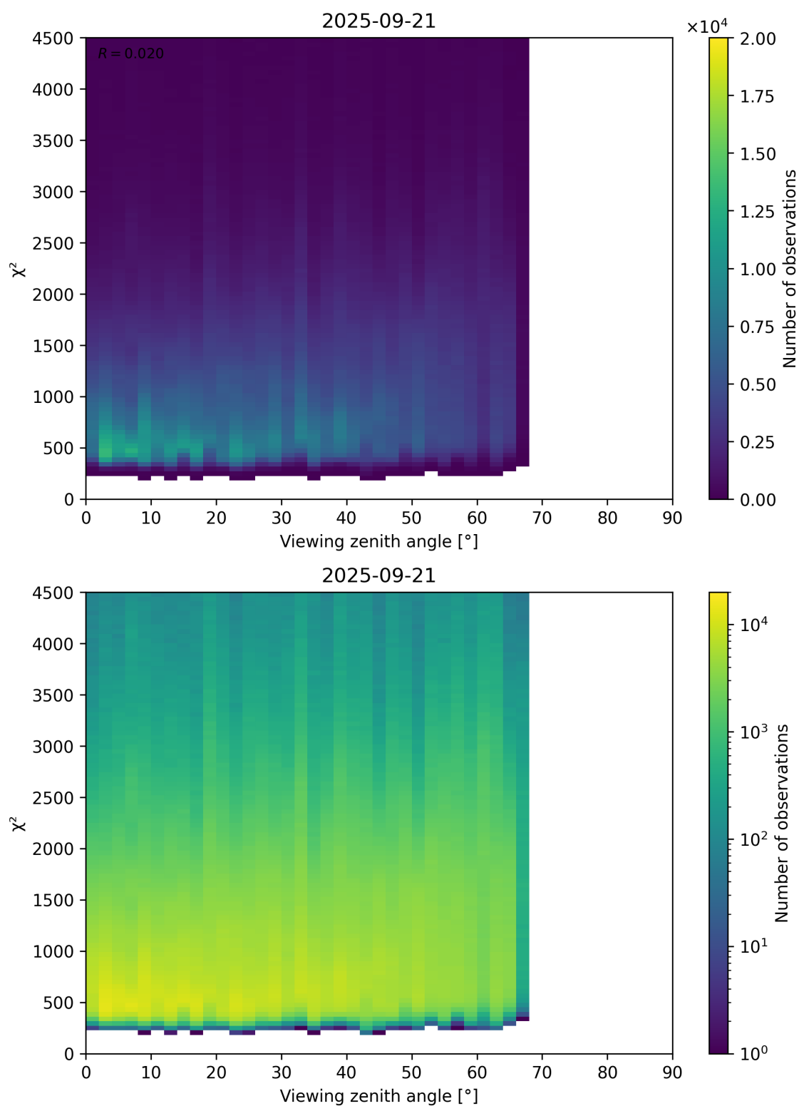
Figure 72: Scatter density plot of “Viewing zenith angle” against “ \chi^2 ” for 2025-09-20 to 2025-09-22.
