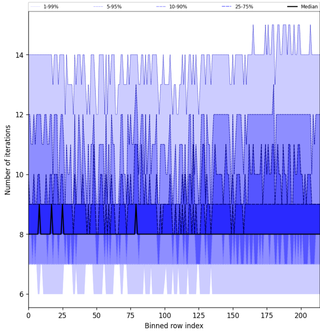
Figure 32: Along track statistics of “Number of iterations” for 2025-09-20 to 2025-09-22
