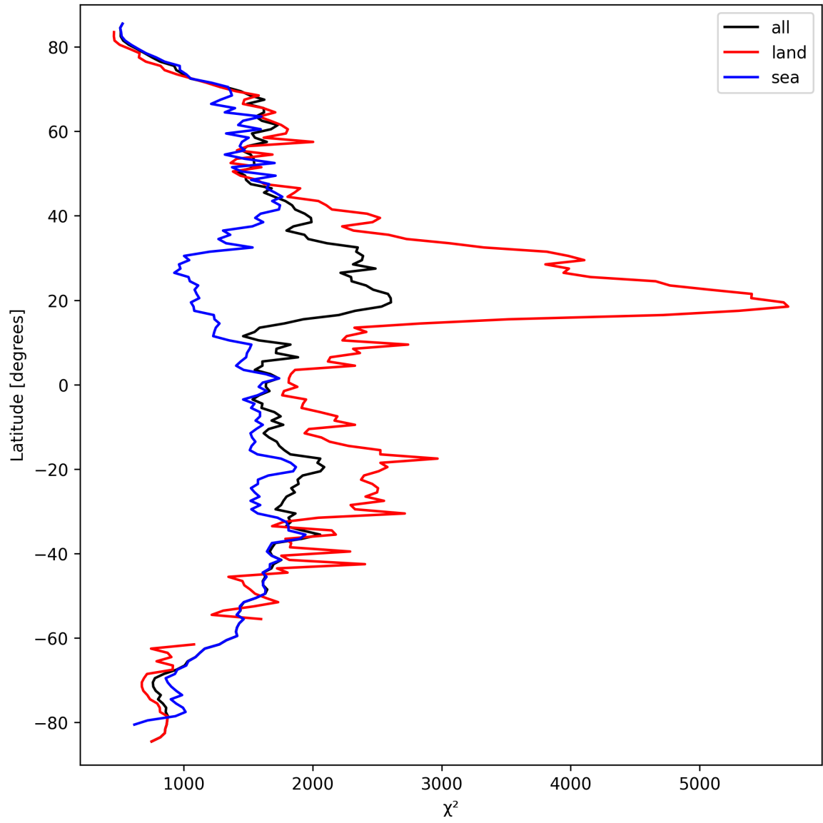
Figure 14: Zonal average of “ \chi^2 ” for 2025-09-20 to 2025-09-22.
