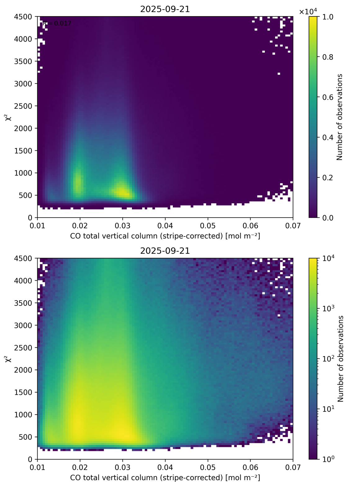
Figure 37: Scatter density plot of “CO total vertical column (stripe-corrected)” against “ \chi^2 ” for 2025-09-20 to 2025-09-22.
