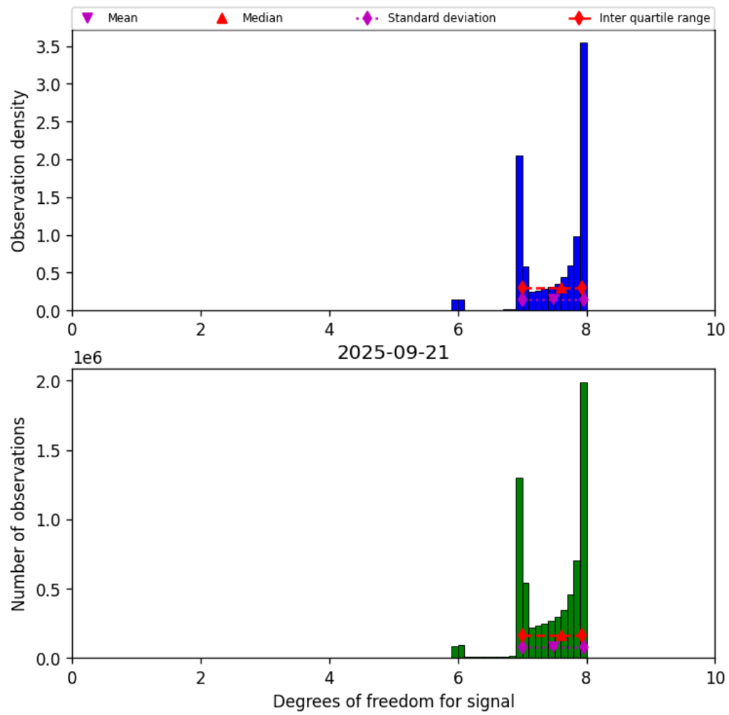
Figure 23: Histogram of “Degrees of freedom for signal” for 2025-09-20 to 2025-09-22
