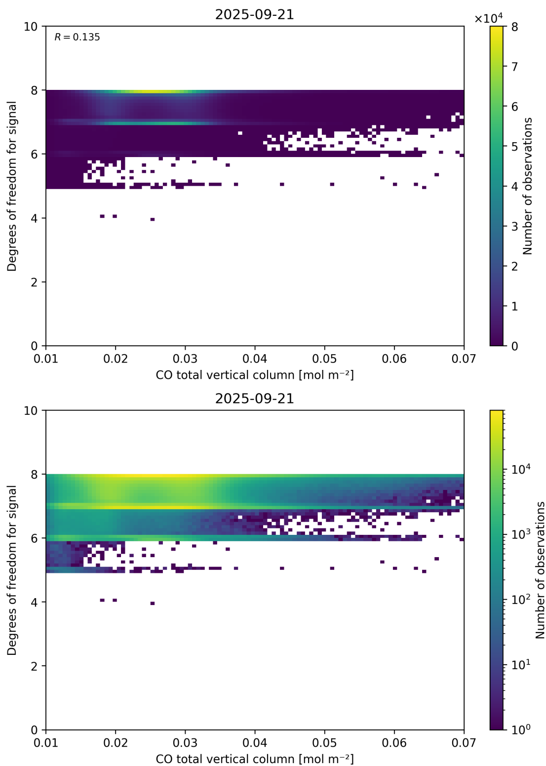
Figure 41: Scatter density plot of “CO total vertical column” against “Degrees of freedom for signal” for 2025-09-20 to 2025-09-22.
