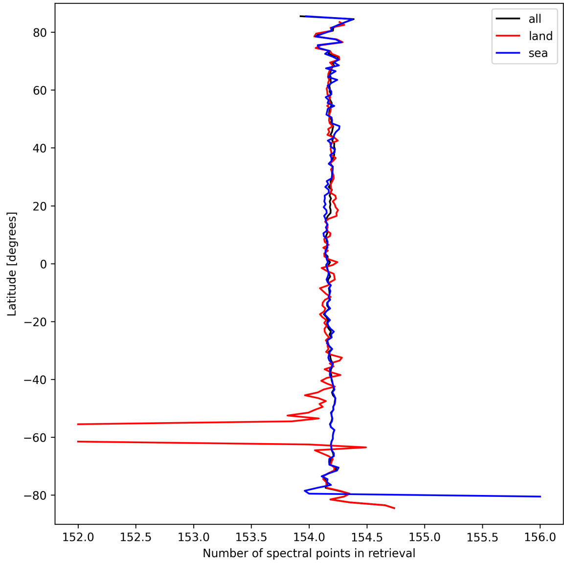
Figure 13: Zonal average of “Number of spectral points in retrieval” for 2025-09-20 to 2025-09-22.
