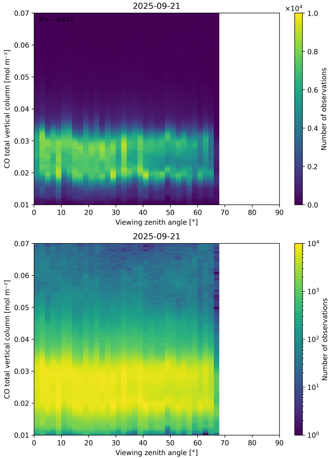
Figure 69: Scatter density plot of “Viewing zenith angle” against “CO total vertical column” for 2025-09-20 to 2025-09-22.
