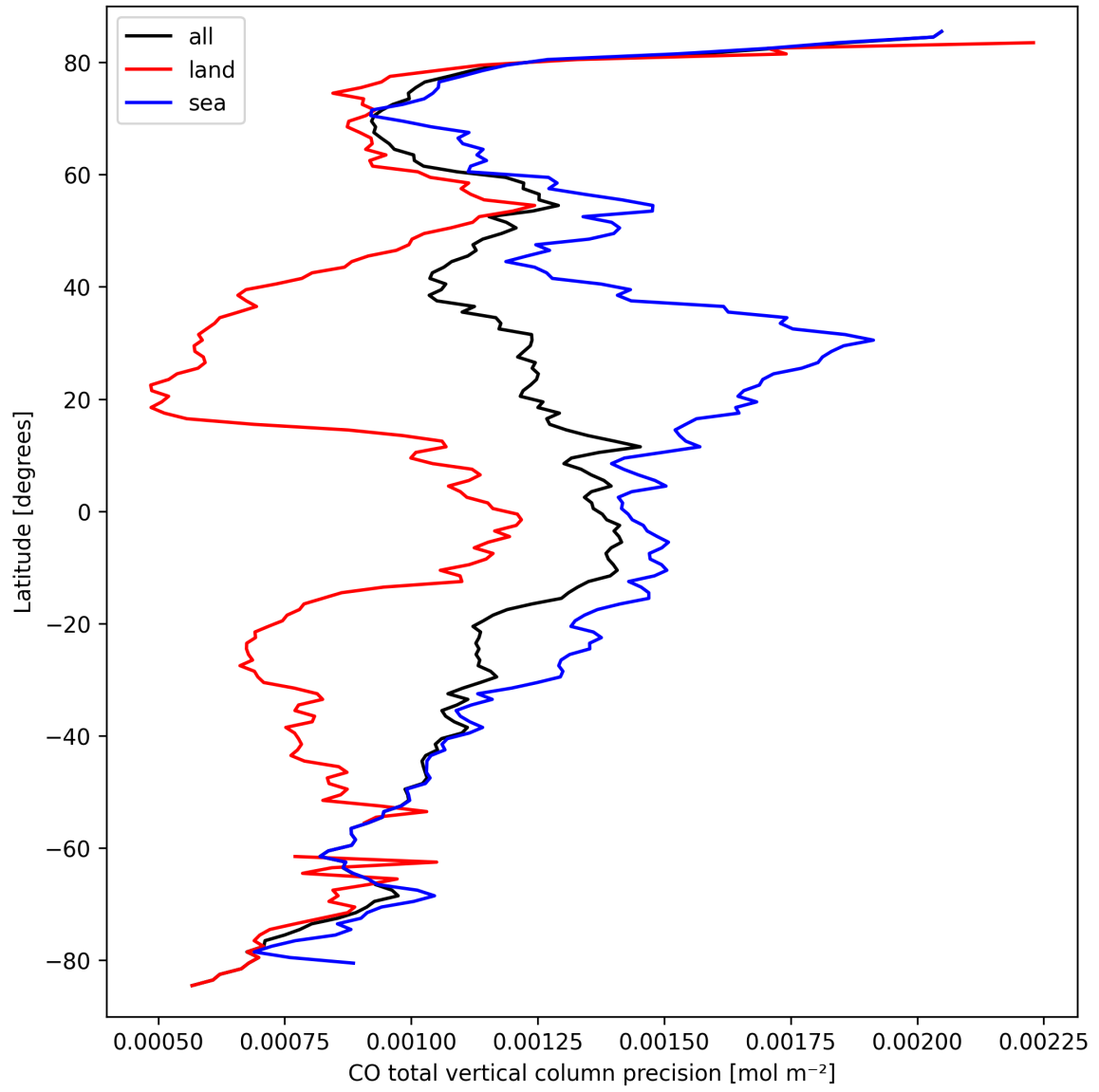
Figure 12: Zonal average of “CO total vertical column precision” for 2025-09-20 to 2025-09-22.
