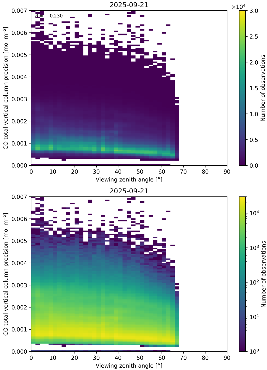
Figure 71: Scatter density plot of “Viewing zenith angle” against “CO total vertical column precision” for 2025-09-20 to 2025-09-22.
