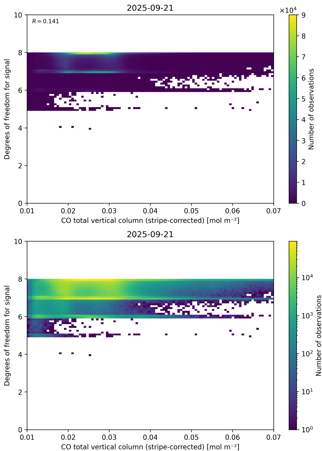
Figure 38: Scatter density plot of “CO total vertical column (stripe-corrected)” against “Degrees of freedom for signal” for 2025-09-20 to 2025-09-22.
