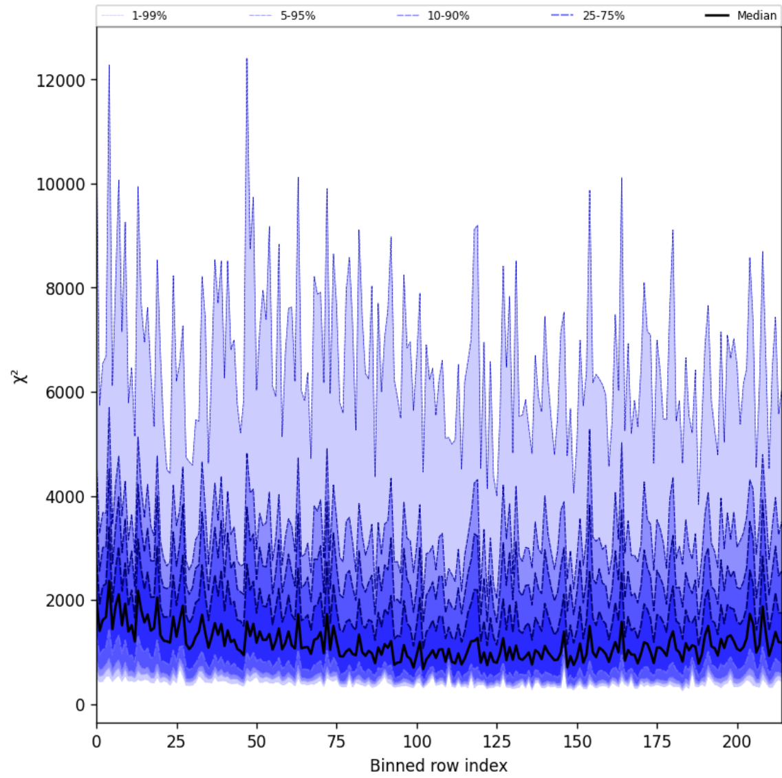
Figure 30: Along track statistics of “ \chi^2 ” for 2025-09-20 to 2025-09-22
