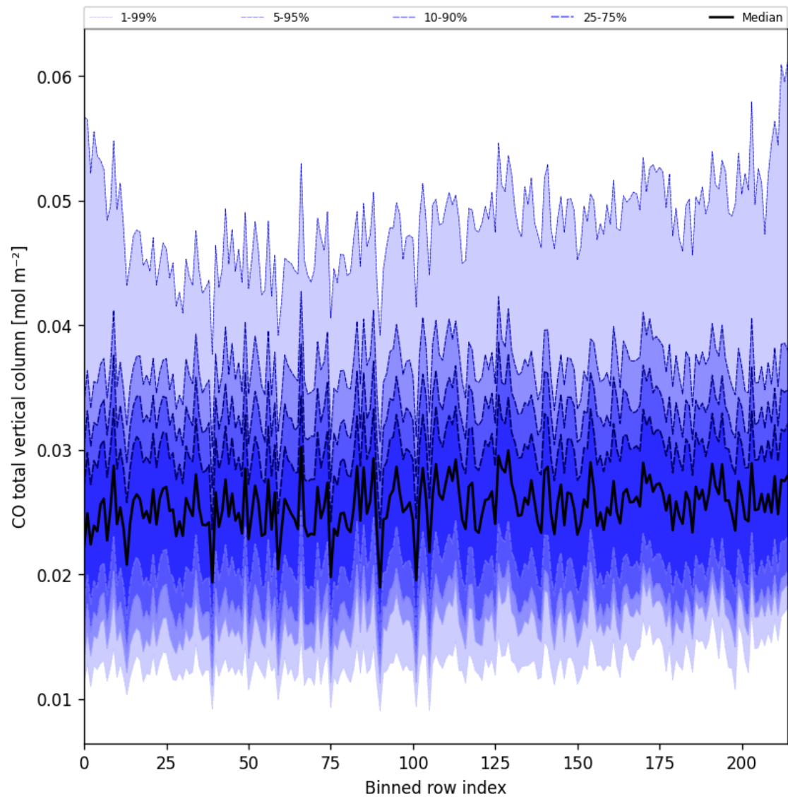
Figure 26: Along track statistics of “CO total vertical column” for 2025-09-20 to 2025-09-22
