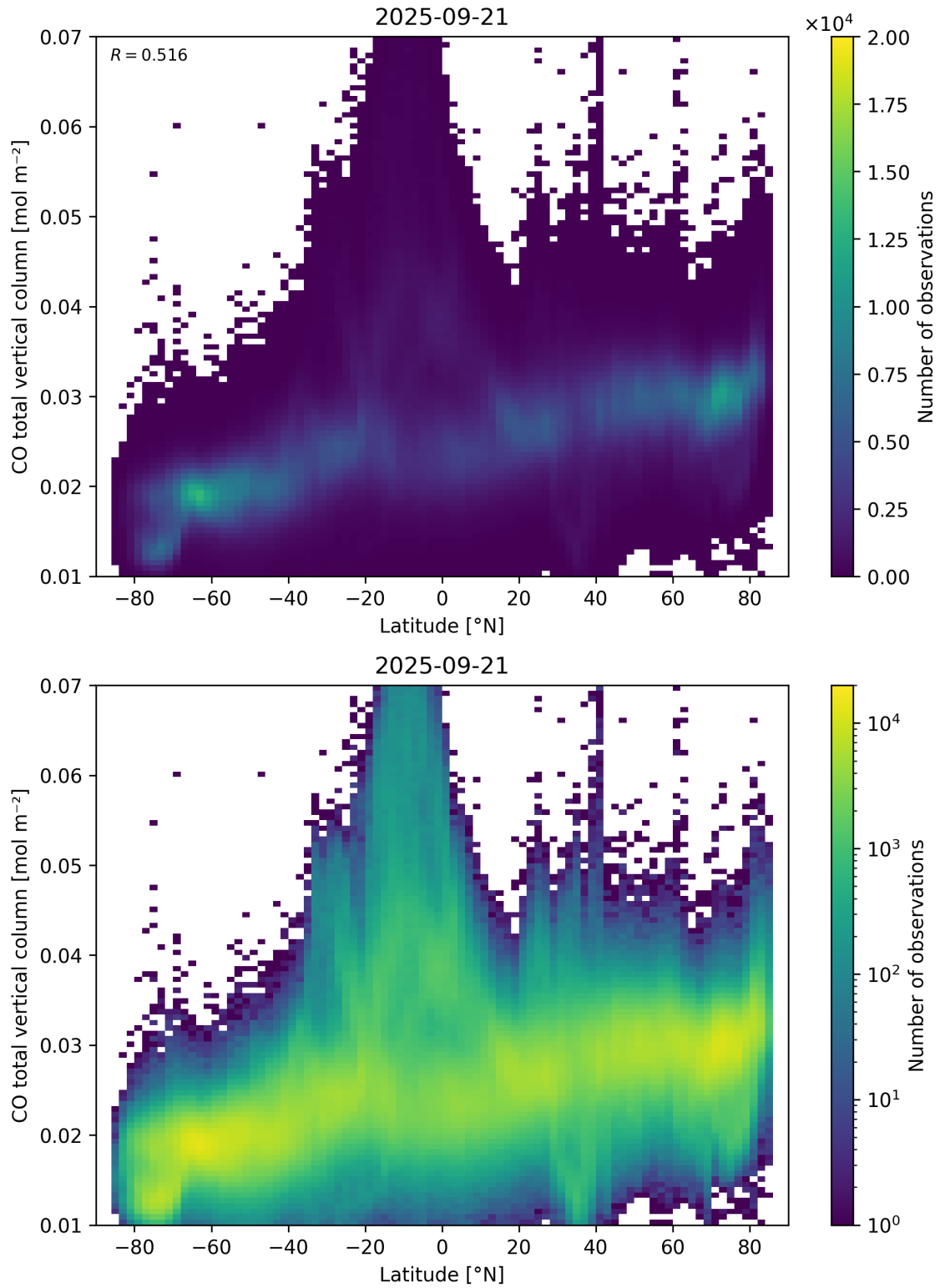
Figure 51: Scatter density plot of “Latitude” against “CO total vertical column” for 2025-09-20 to 2025-09-22.
