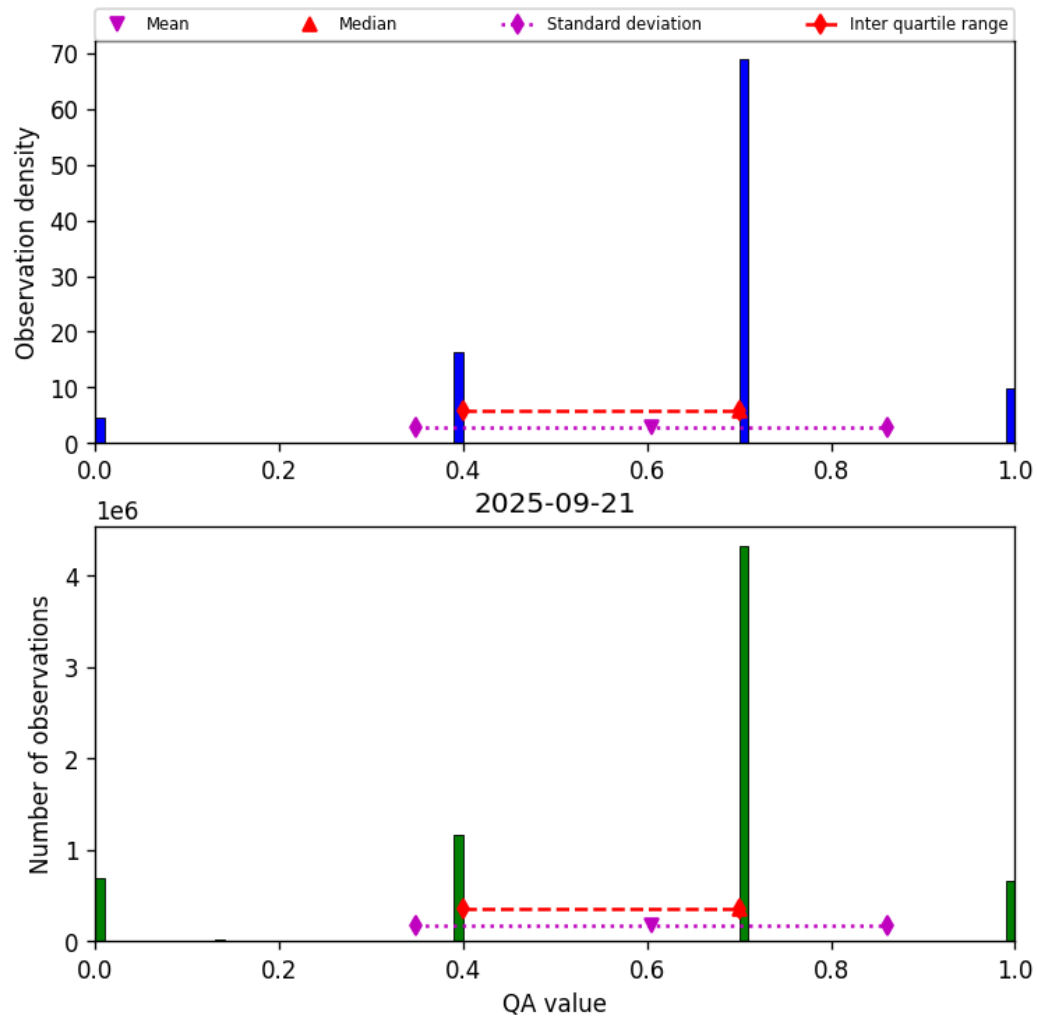
Figure 17: Histogram of “QA value” for 2025-09-20 to 2025-09-22
