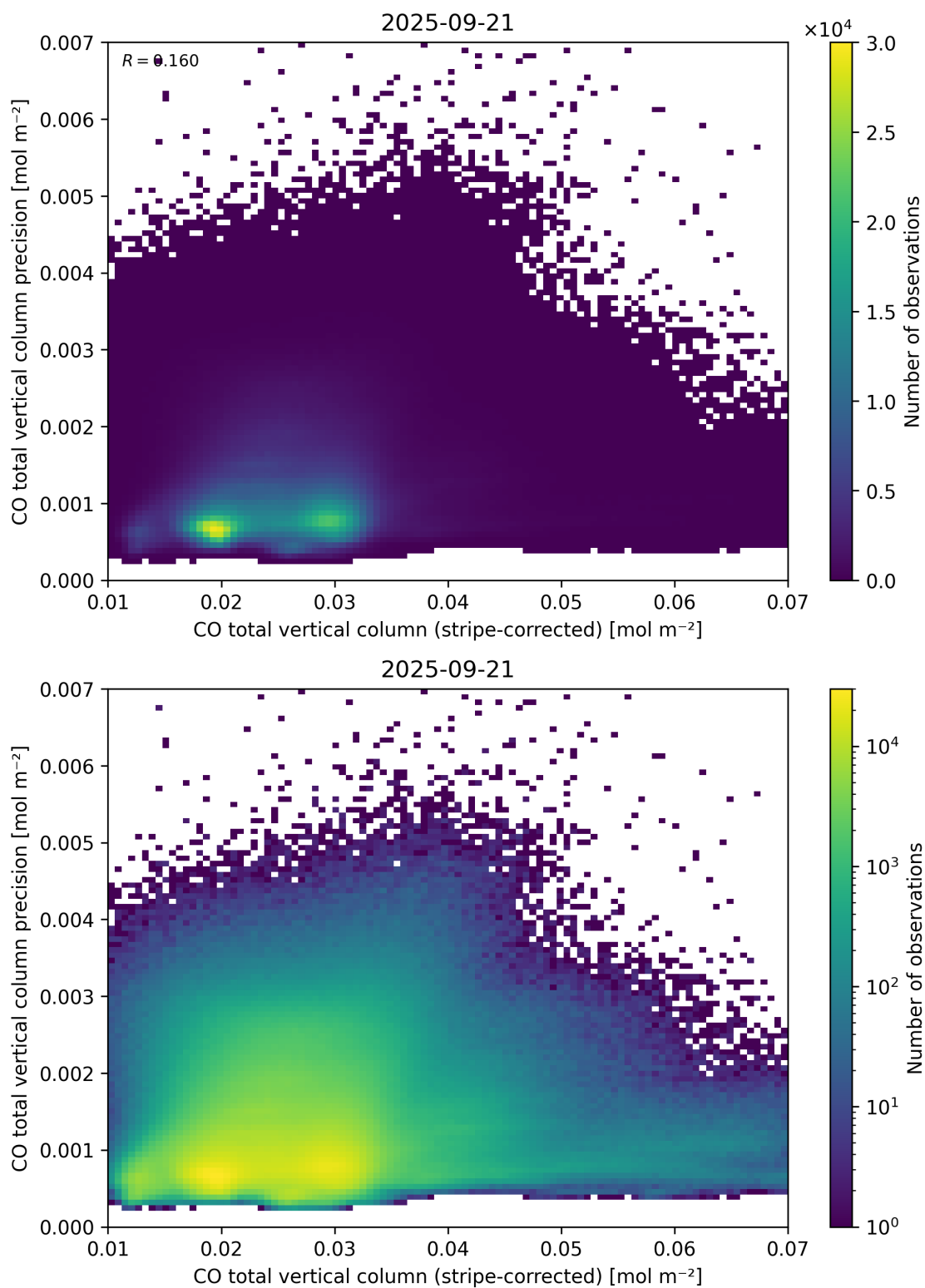
Figure 36: Scatter density plot of “CO total vertical column (stripe-corrected)” against “CO total vertical column precision” for 2025-09-20 to 2025-09-22.
