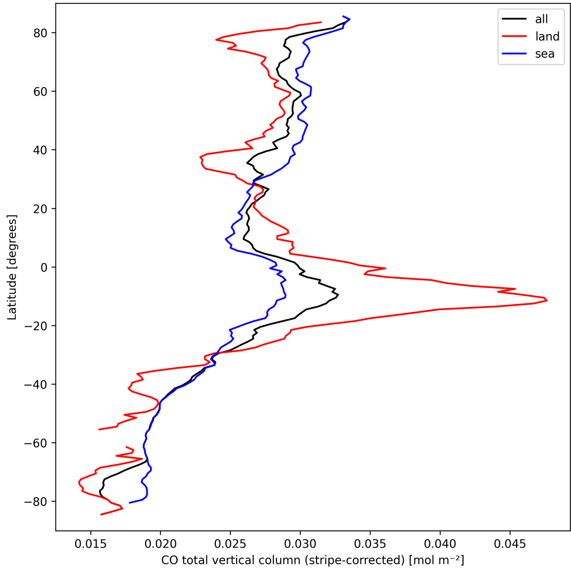
Figure 11: Zonal average of “CO total vertical column (stripe-corrected)” for 2025-09-20 to 2025-09-22.
