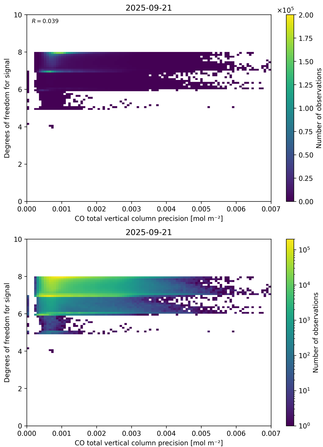
Figure 45: Scatter density plot of “CO total vertical column precision” against “Degrees of freedom for signal” for 2025-09-20 to 2025-09-22.
