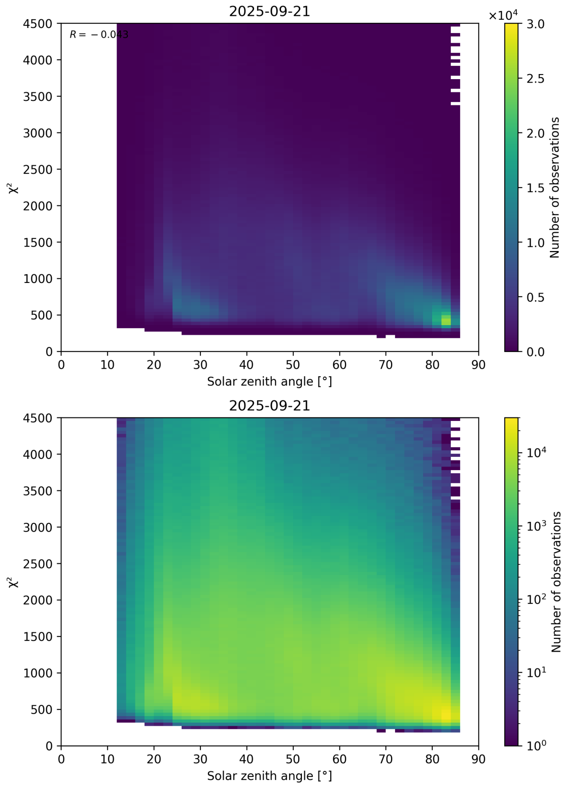
Figure 64: Scatter density plot of “Solar zenith angle” against “ \chi^2 ” for 2025-09-20 to 2025-09-22.
