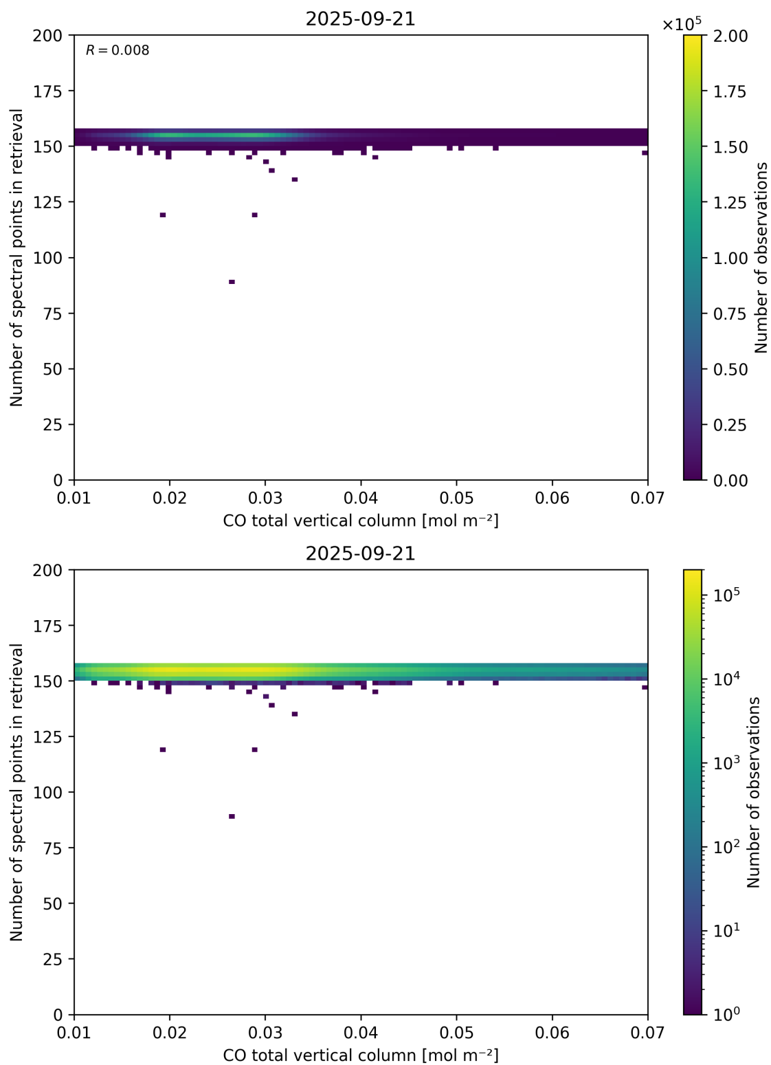
Figure 43: Scatter density plot of “CO total vertical column” against “Number of spectral points in retrieval” for 2025-09-20 to 2025-09-22.
