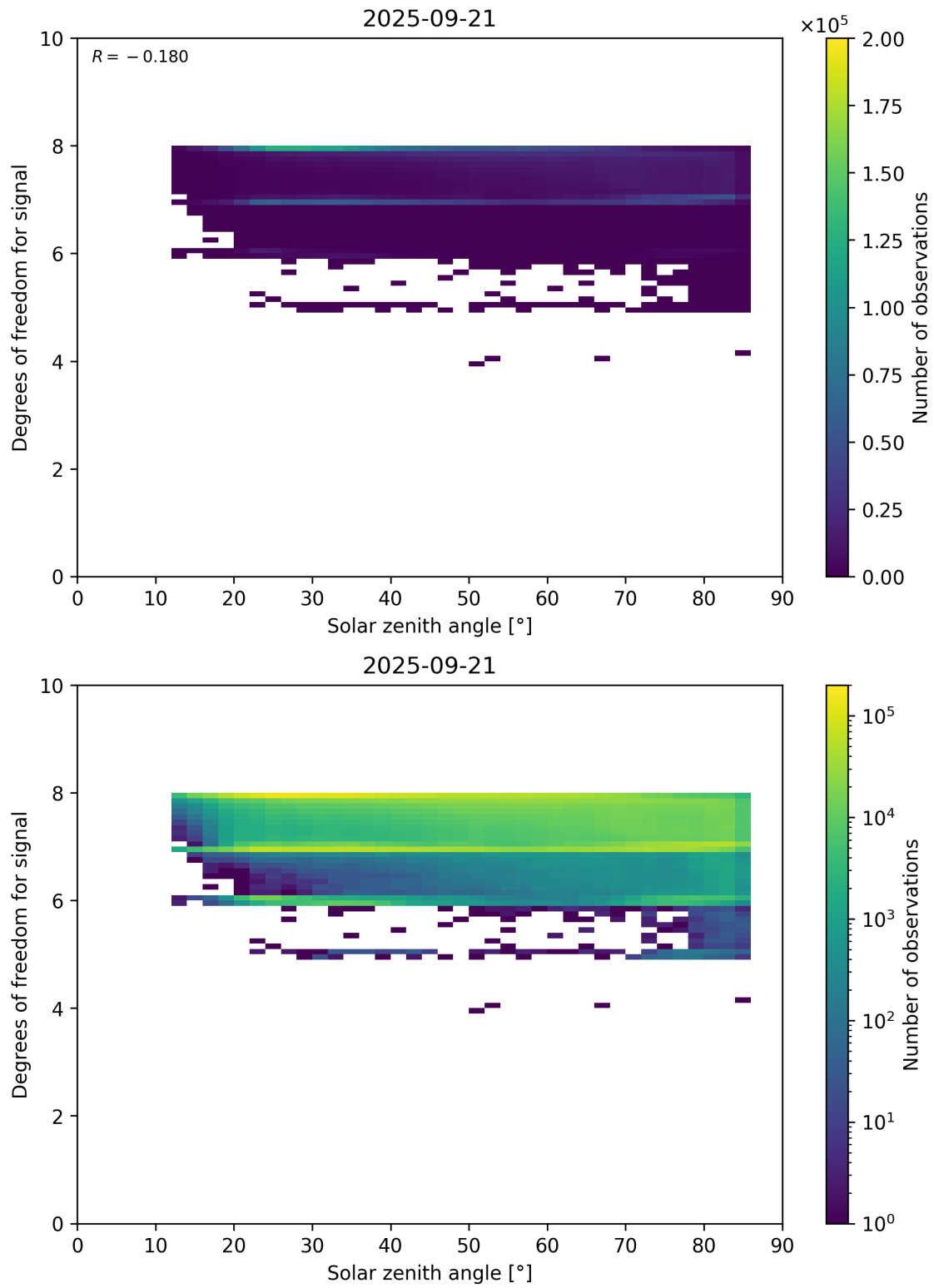
Figure 65: Scatter density plot of “Solar zenith angle” against “Degrees of freedom for signal” for 2025-09-20 to 2025-09-22.
