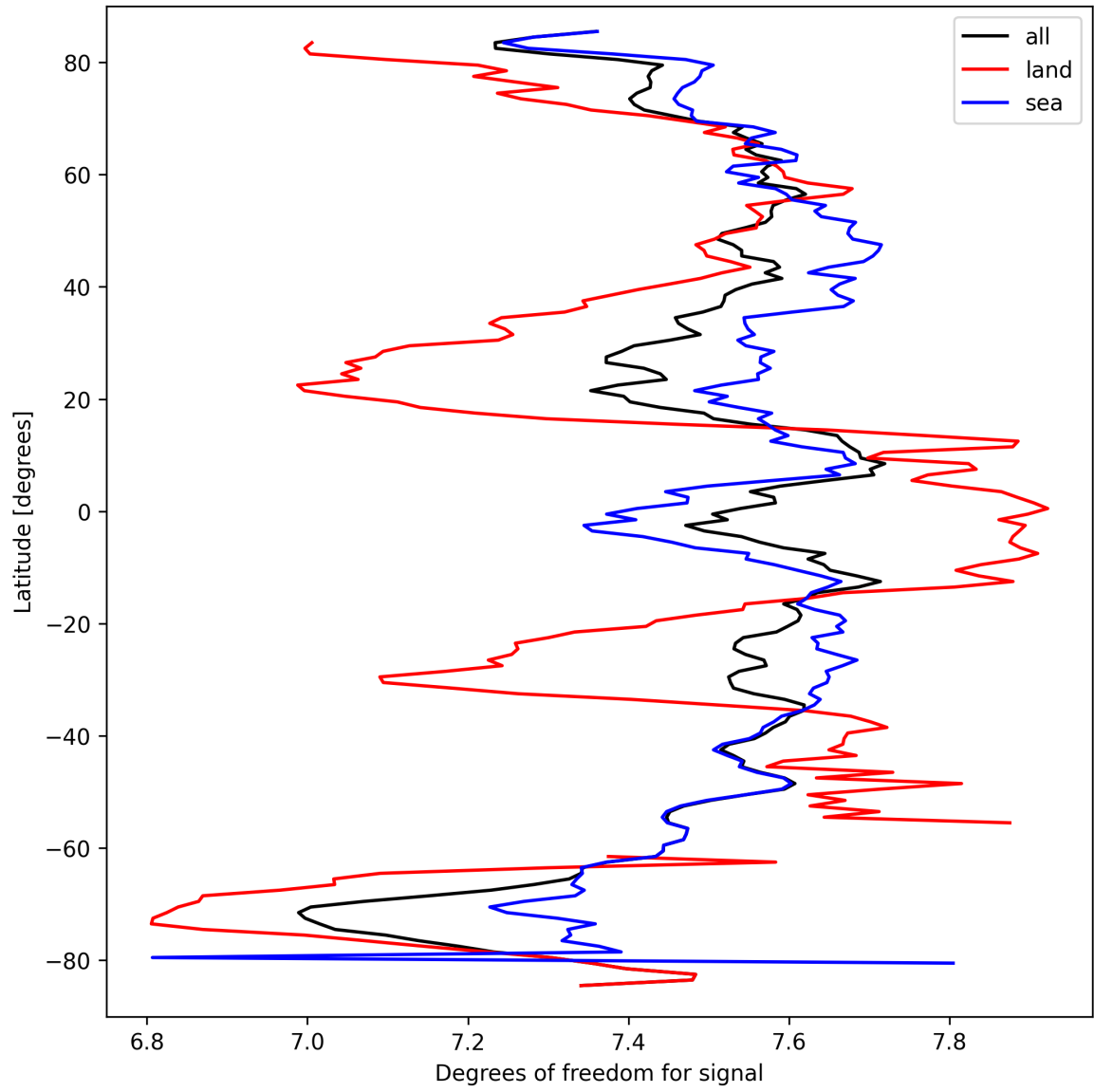
Figure 15: Zonal average of “Degrees of freedom for signal” for 2025-09-20 to 2025-09-22.
