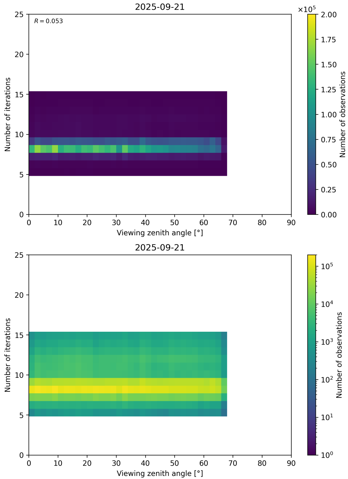
Figure 75: Scatter density plot of “Viewing zenith angle” against “Number of iterations” for 2025-09-20 to 2025-09-22.
