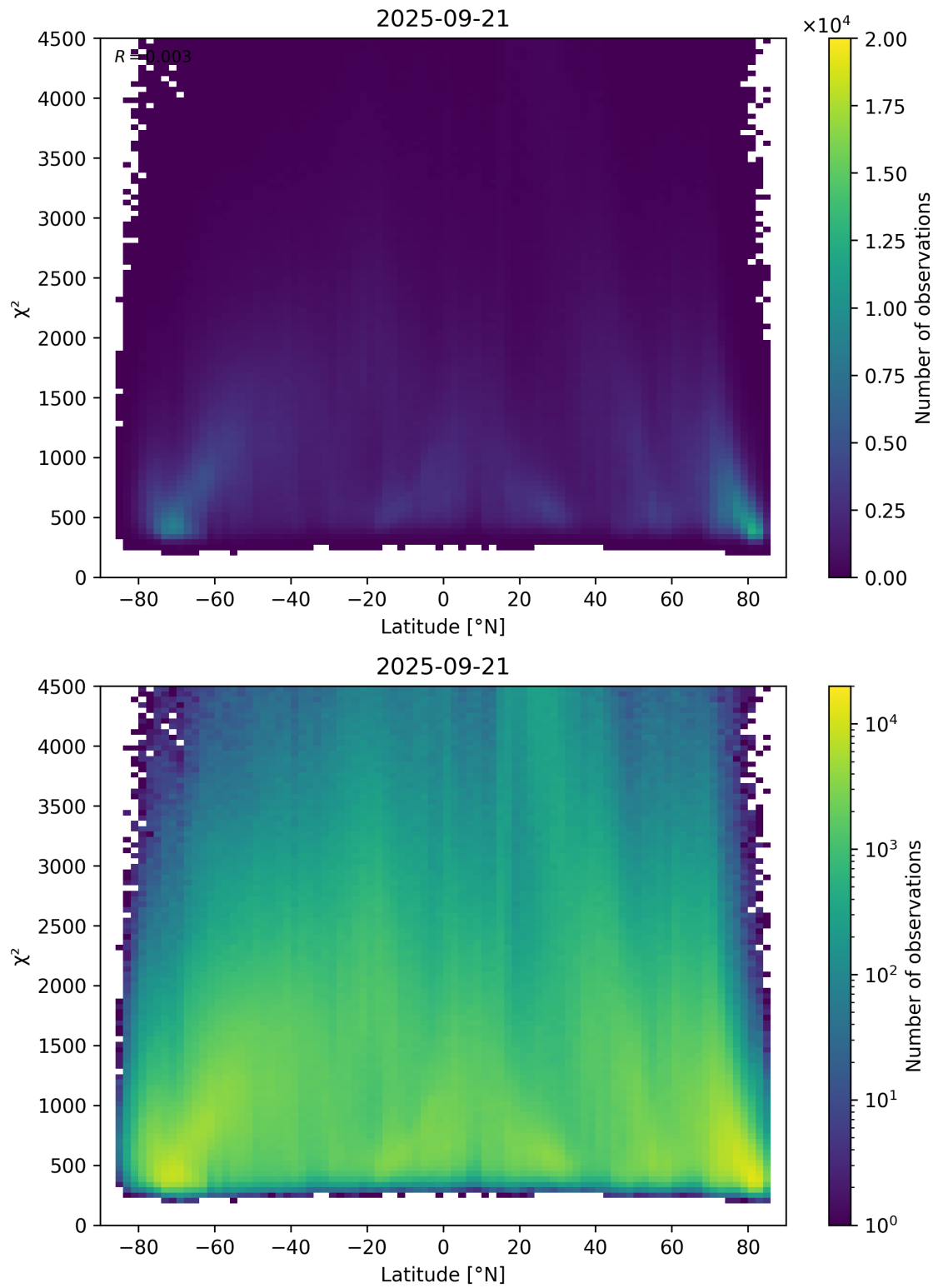
Figure 54: Scatter density plot of “Latitude” against “ \chi^2 ” for 2025-09-20 to 2025-09-22.
