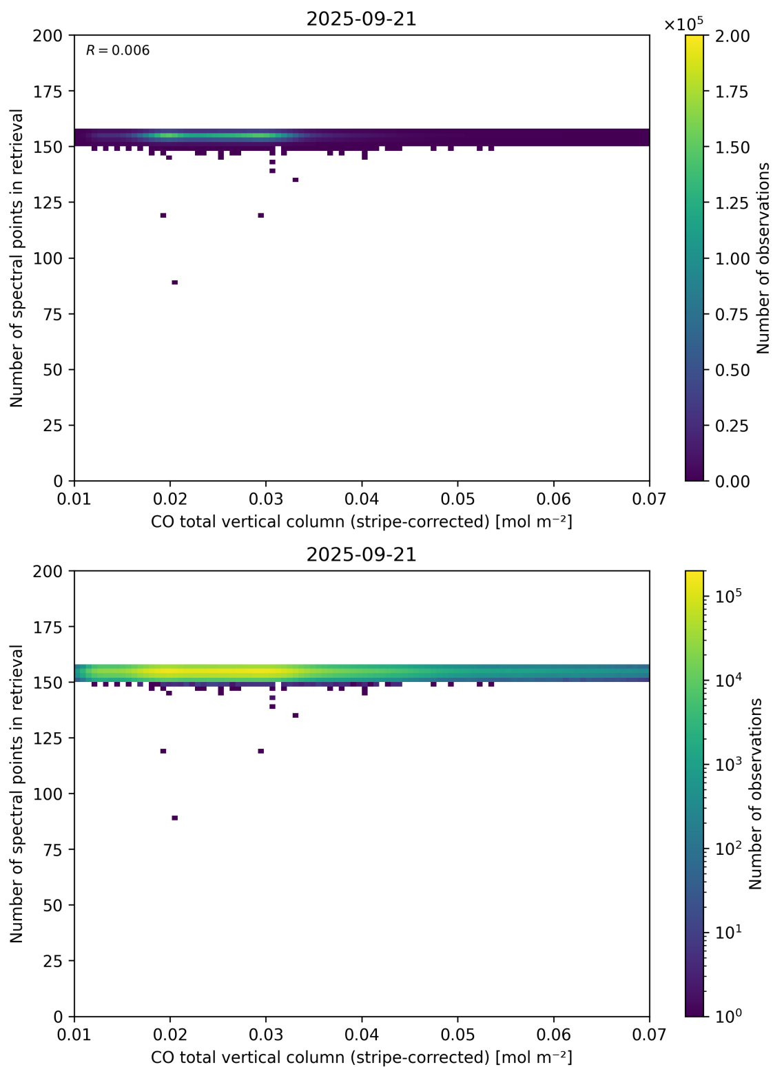
Figure 40: Scatter density plot of “CO total vertical column (stripe-corrected)” against “Number of spectral points in retrieval” for 2025-09-20 to 2025-09-22.
