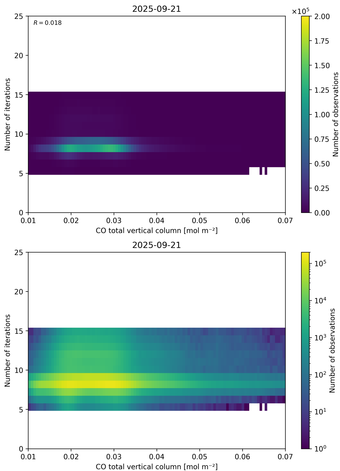
Figure 42: Scatter density plot of “CO total vertical column” against “Number of iterations” for 2025-09-20 to 2025-09-22.
