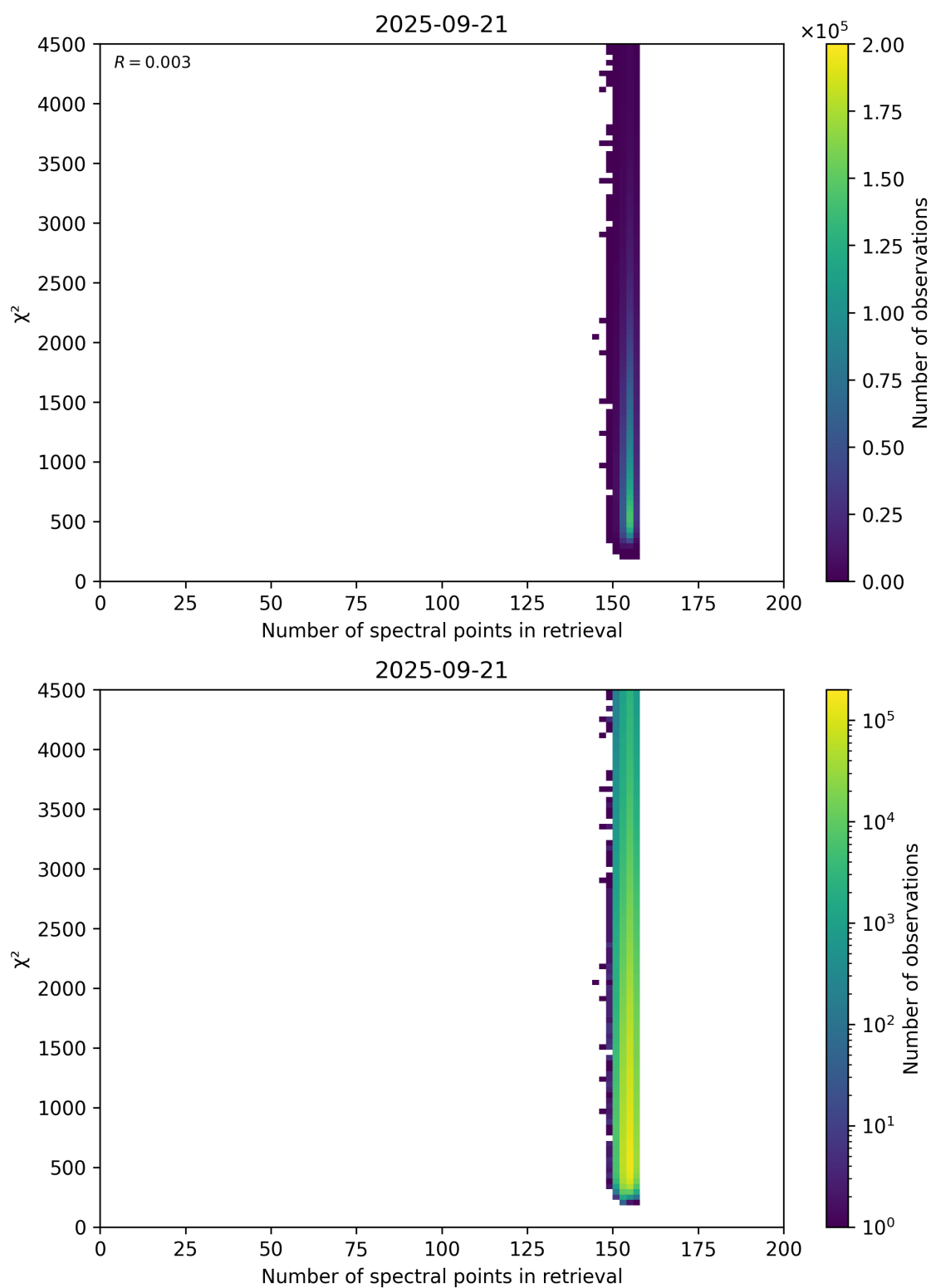
Figure 58: Scatter density plot of “Number of spectral points in retrieval” against “ \chi^2 ” for 2025-09-20 to 2025-09-22.
