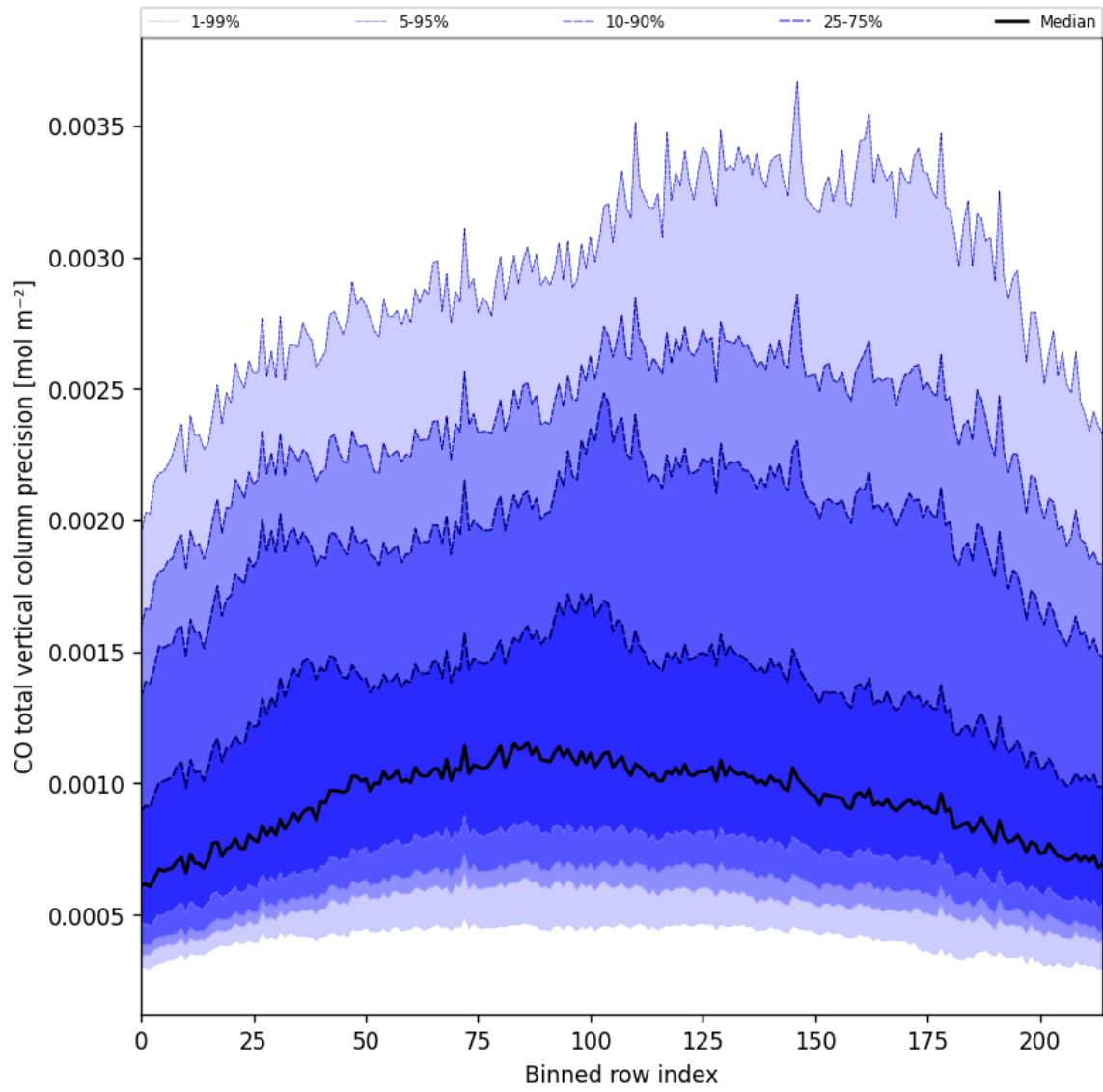
Figure 28: Along track statistics of “CO total vertical column precision” for 2025-09-20 to 2025-09-22
