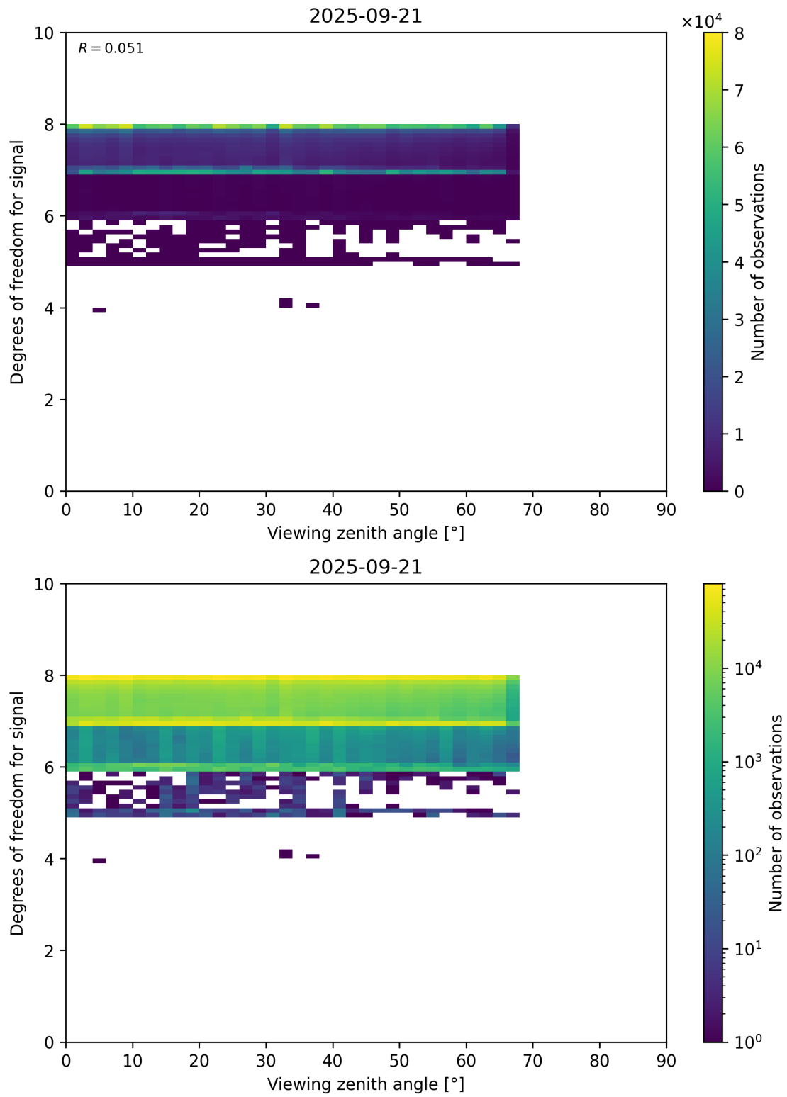
Figure 73: Scatter density plot of “Viewing zenith angle” against “Degrees of freedom for signal” for 2025-09-20 to 2025-09-22.
