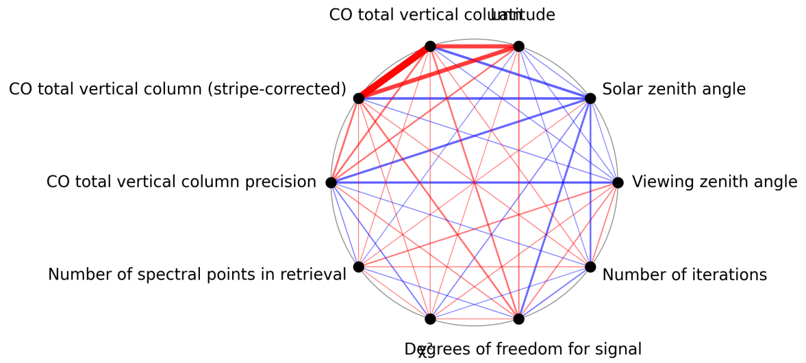
Figure 1: Map of correlation graph for 2025-09-20 to 2025-09-22.
