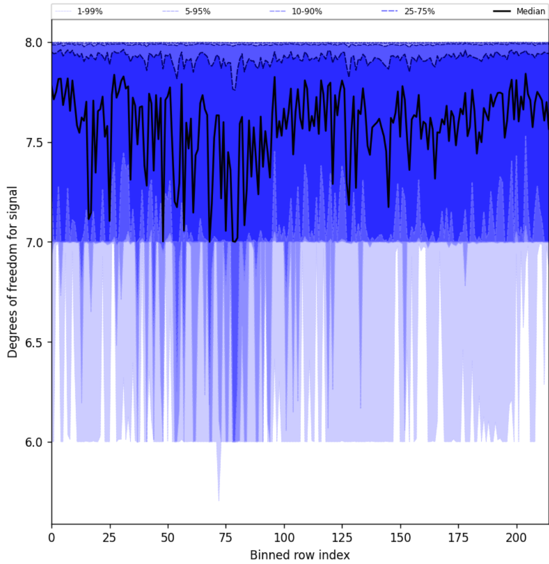
Figure 31: Along track statistics of “Degrees of freedom for signal” for 2025-09-20 to 2025-09-22
