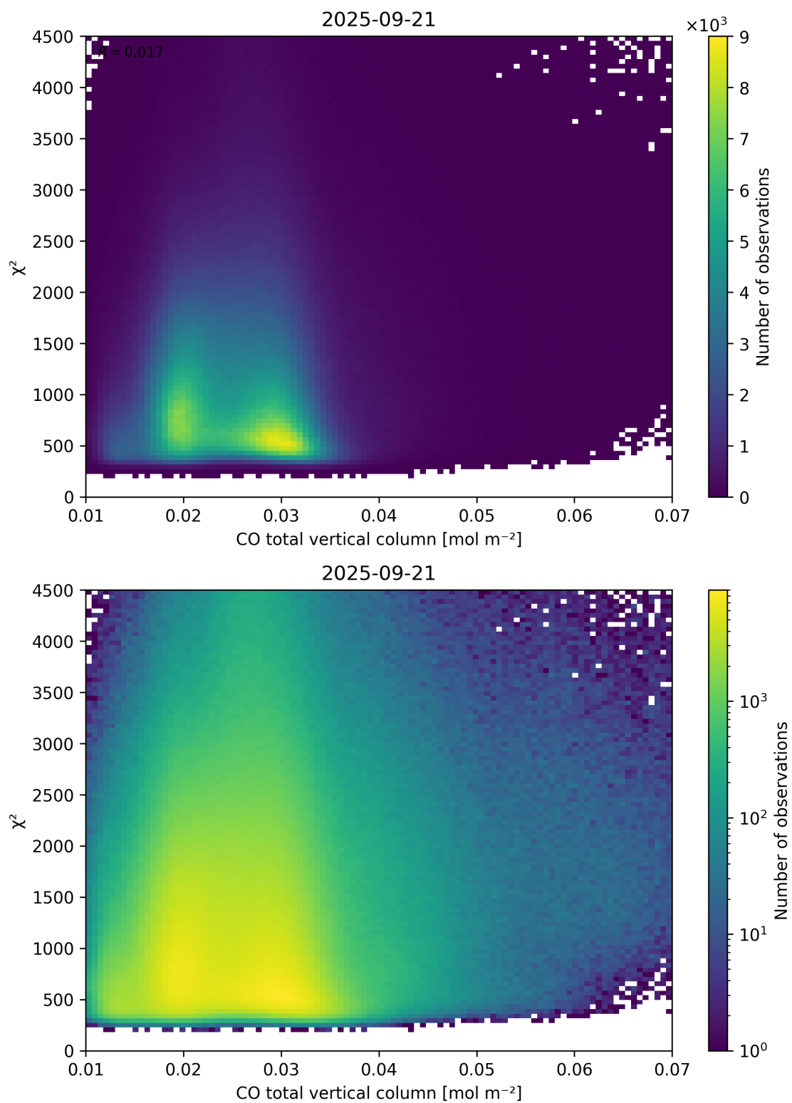
Figure 35: Scatter density plot of “CO total vertical column” against “ \chi^2 ” for 2025-09-20 to 2025-09-22.
