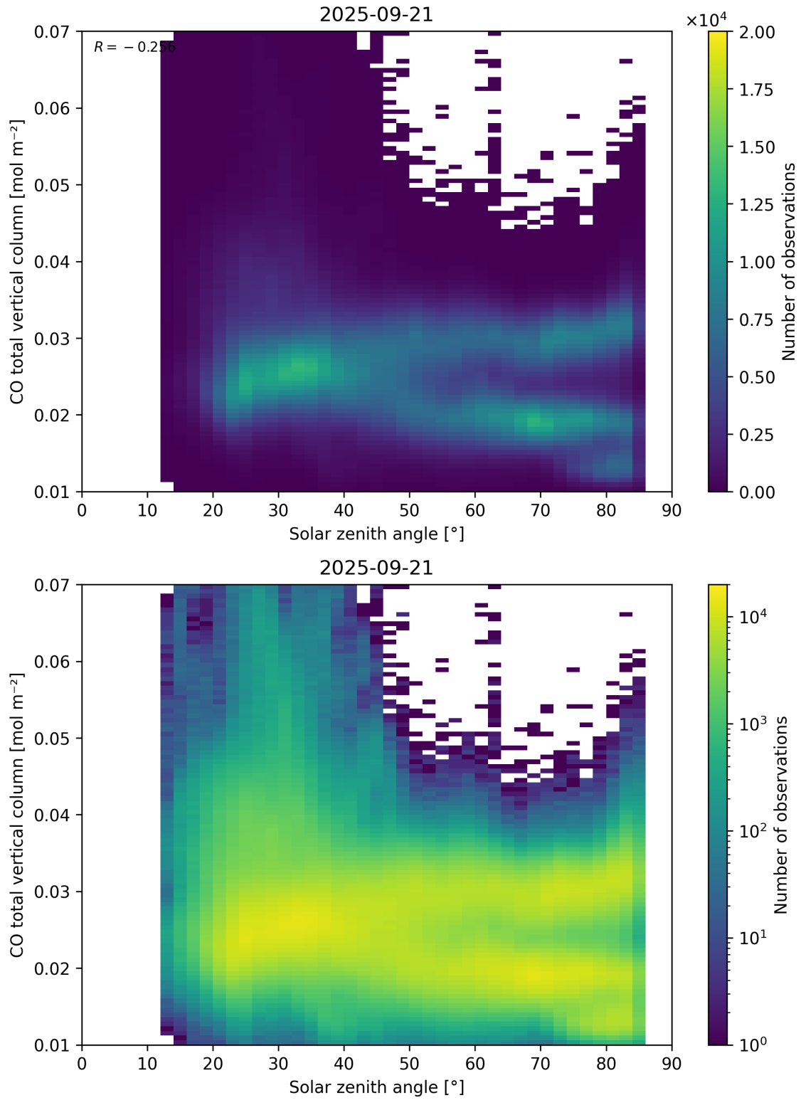
Figure 61: Scatter density plot of “Solar zenith angle” against “CO total vertical column” for 2025-09-20 to 2025-09-22.
