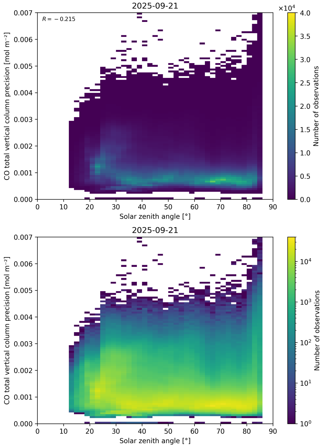
Figure 63: Scatter density plot of “Solar zenith angle” against “CO total vertical column precision” for 2025-09-20 to 2025-09-22.
