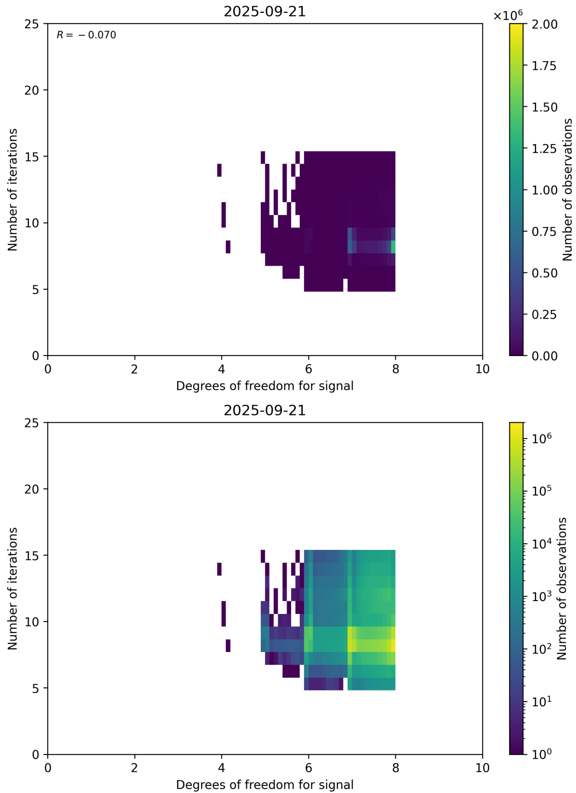
Figure 50: Scatter density plot of “Degrees of freedom for signal” against “Number of iterations” for 2025-09-20 to 2025-09-22.
