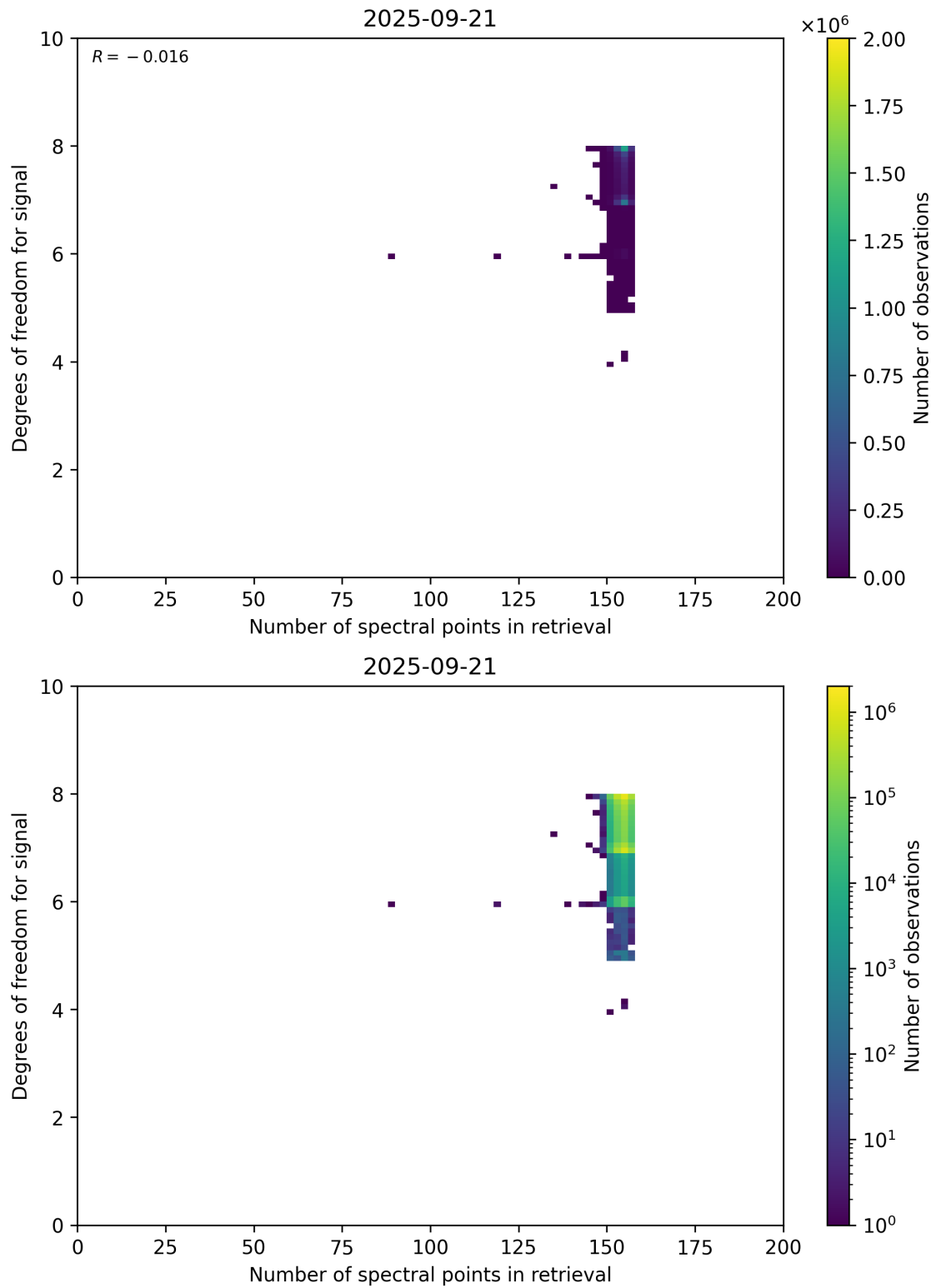
Figure 59: Scatter density plot of “Number of spectral points in retrieval” against “Degrees of freedom for signal” for 2025-09-20 to 2025-09-22.
