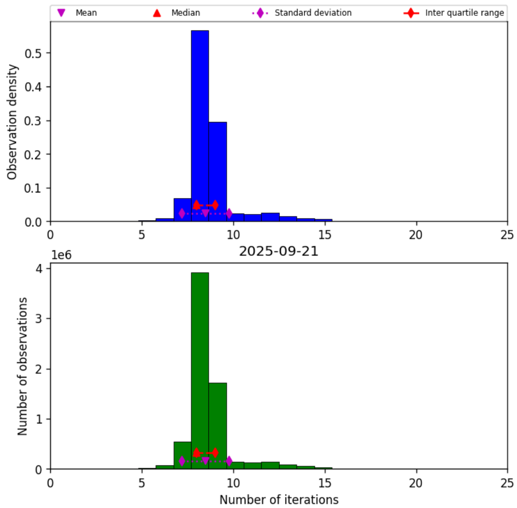
Figure 24: Histogram of “Number of iterations” for 2025-09-20 to 2025-09-22
