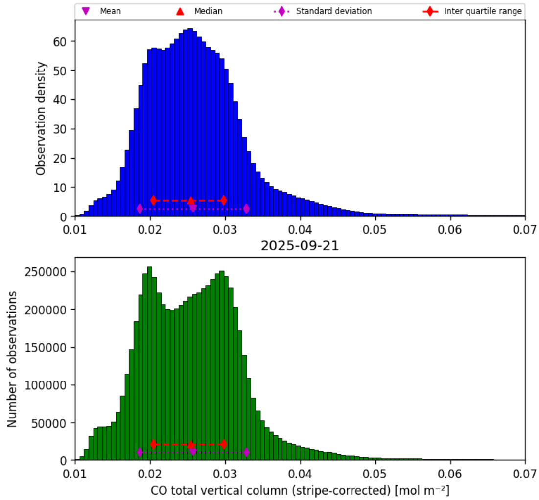
Figure 19: Histogram of “CO total vertical column (stripe-corrected)” for 2025-09-20 to 2025-09-22
