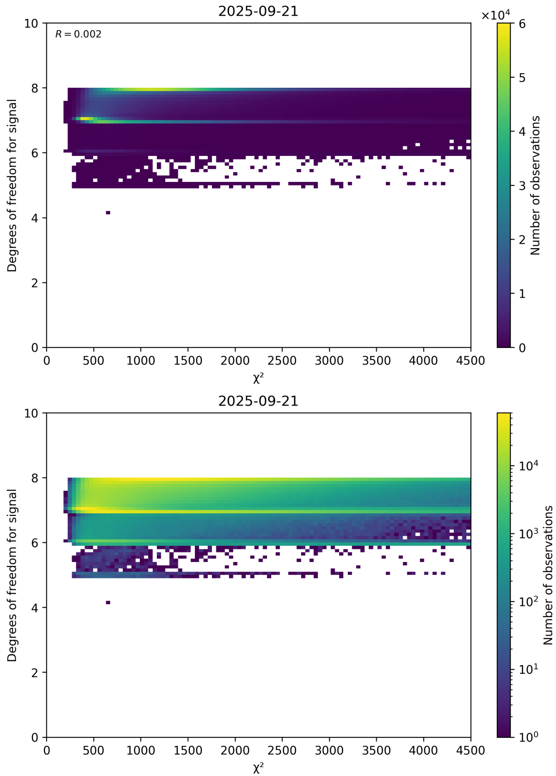
Figure 48: Scatter density plot of “ \chi^2 ” against “Degrees of freedom for signal” for 2025-09-20 to 2025-09-22.
