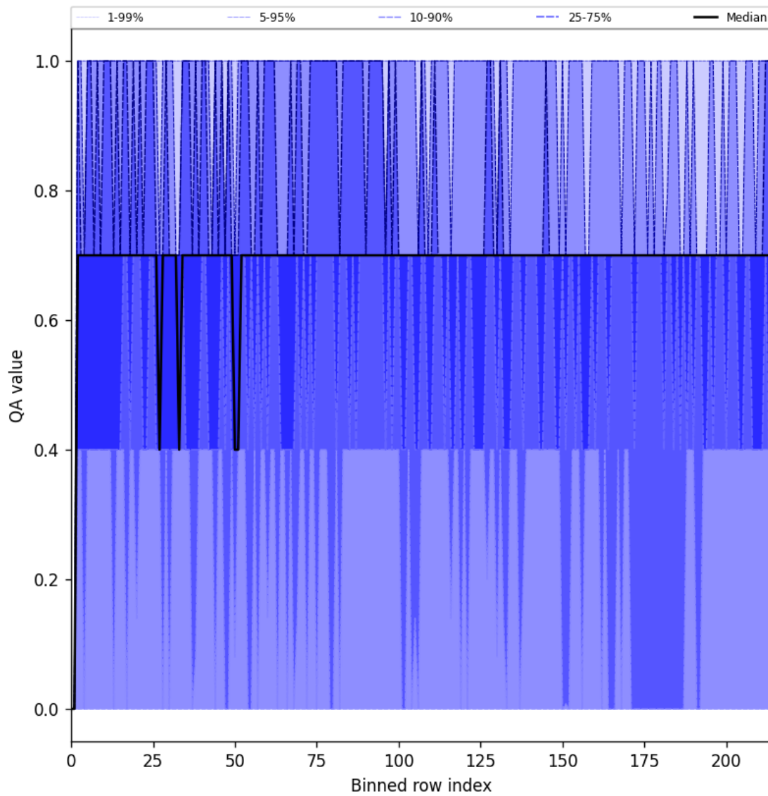
Figure 25: Along track statistics of “QA value” for 2025-09-20 to 2025-09-22
