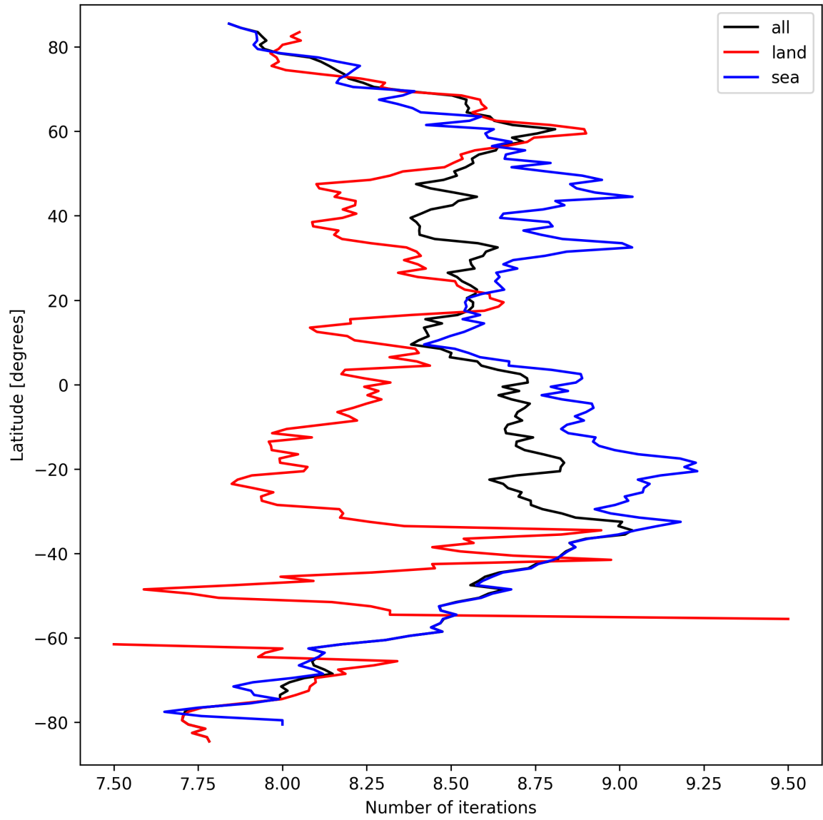
Figure 16: Zonal average of “Number of iterations” for 2025-09-20 to 2025-09-22.
