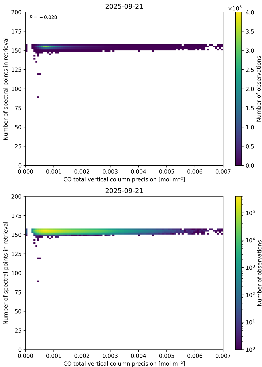
Figure 47: Scatter density plot of “CO total vertical column precision” against “Number of spectral points in retrieval” for 2025-09-20 to 2025-09-22.
