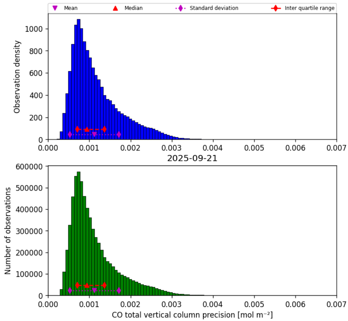
Figure 20: Histogram of “CO total vertical column precision” for 2025-09-20 to 2025-09-22
