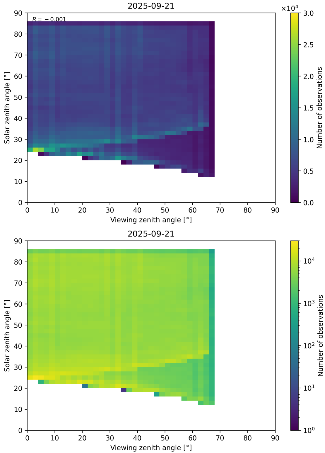
Figure 77: Scatter density plot of “Viewing zenith angle” against “Solar zenith angle” for 2025-09-20 to 2025-09-22.
