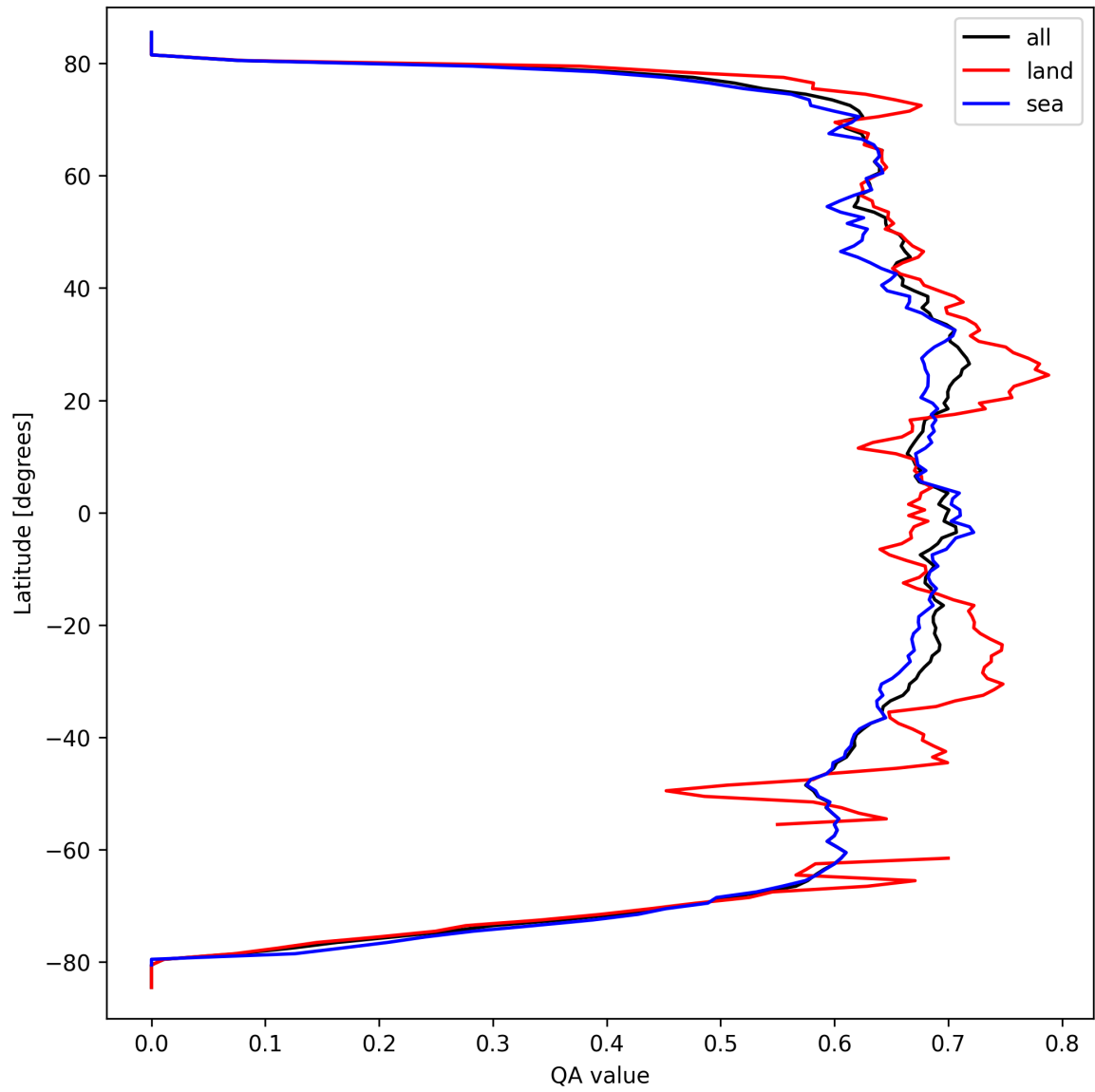
Figure 9: Zonal average of “QA value” for 2025-09-20 to 2025-09-22.
