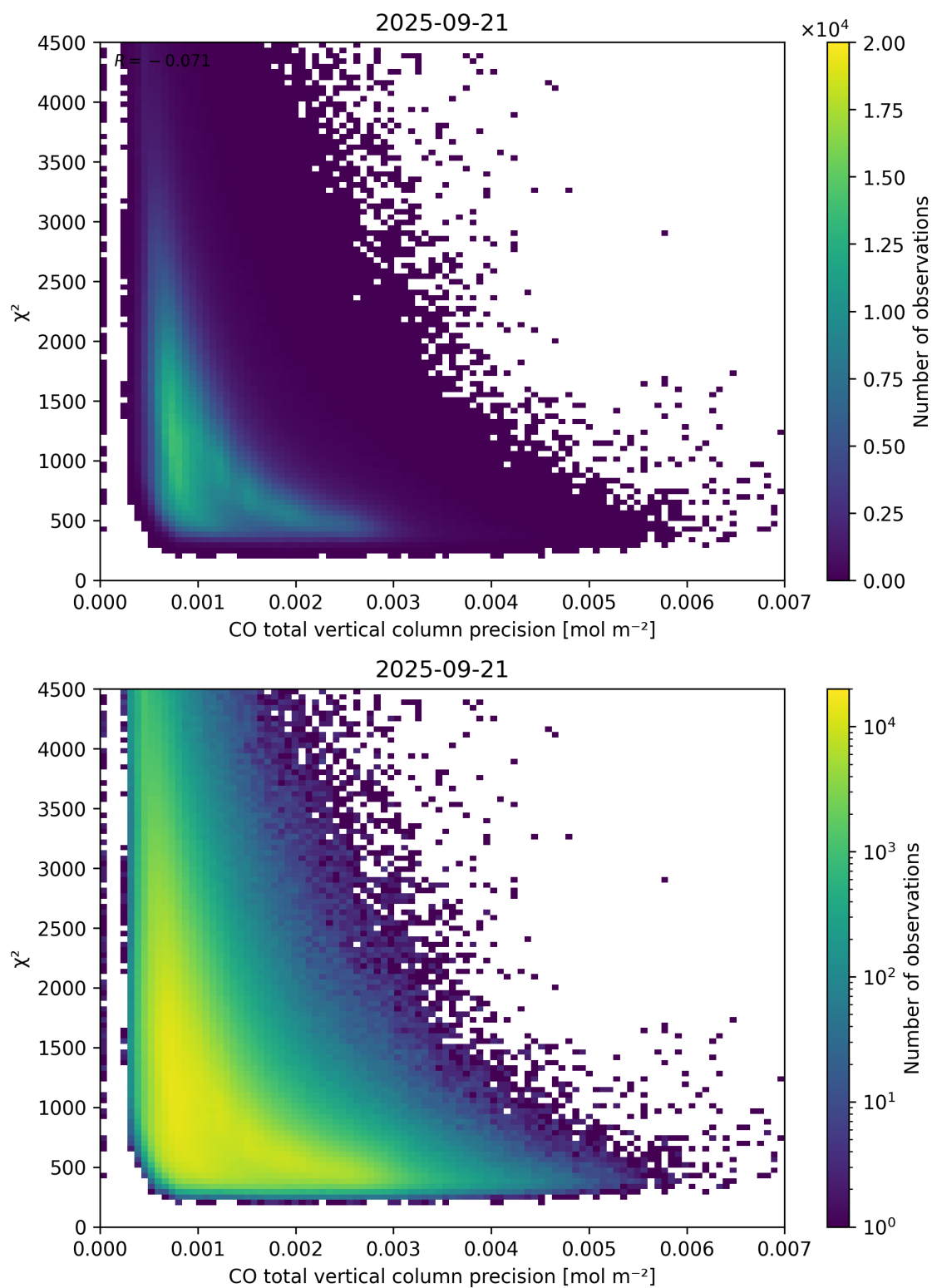
Figure 44: Scatter density plot of “CO total vertical column precision” against “ \chi^2 ” for 2025-09-20 to 2025-09-22.
