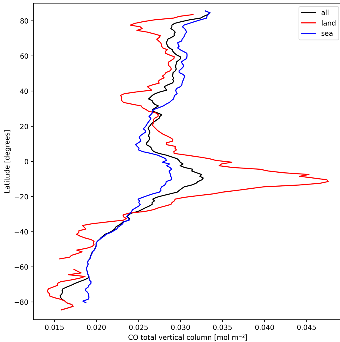
Figure 10: Zonal average of “CO total vertical column” for 2025-09-20 to 2025-09-22.
