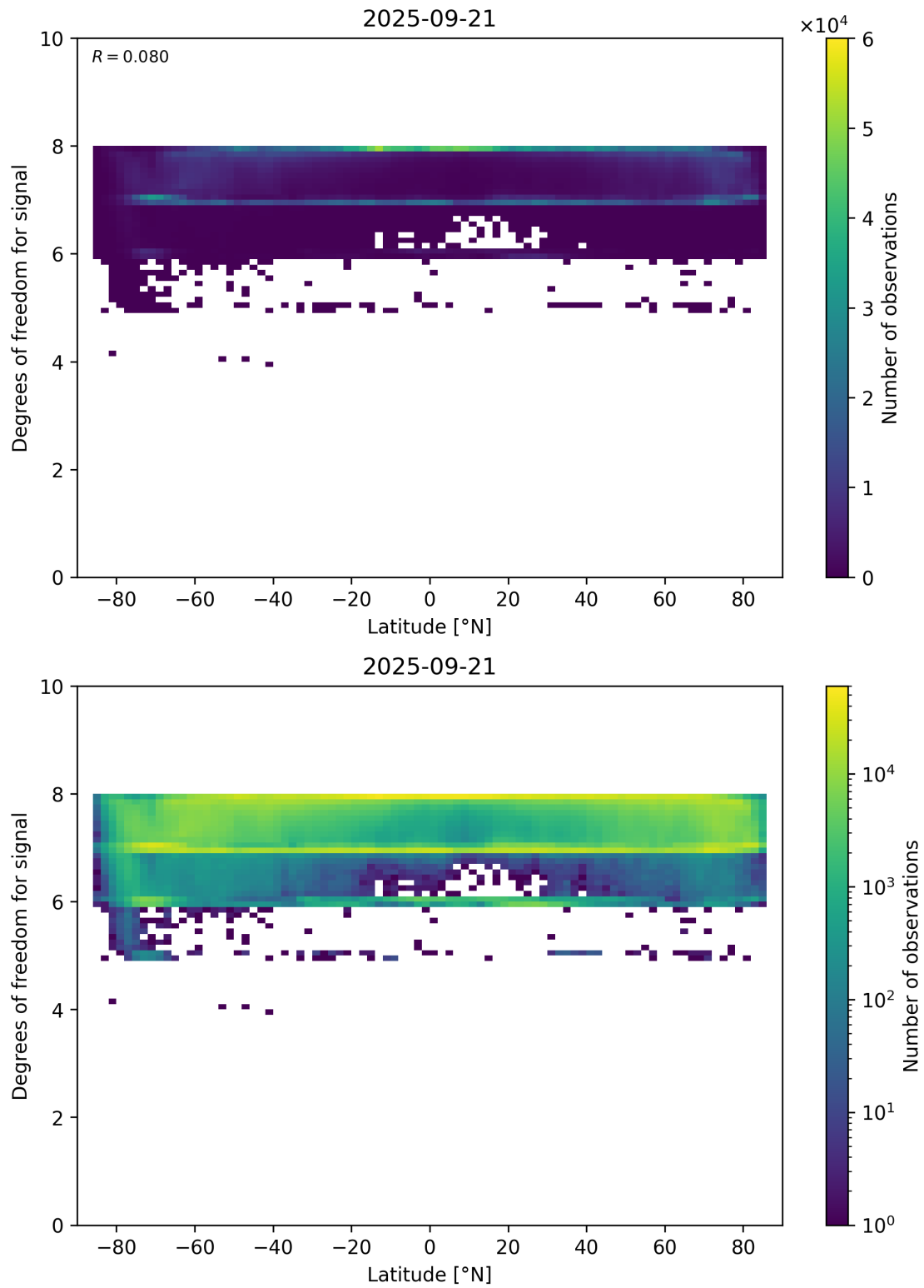
Figure 55: Scatter density plot of “Latitude” against “Degrees of freedom for signal” for 2025-09-20 to 2025-09-22.
