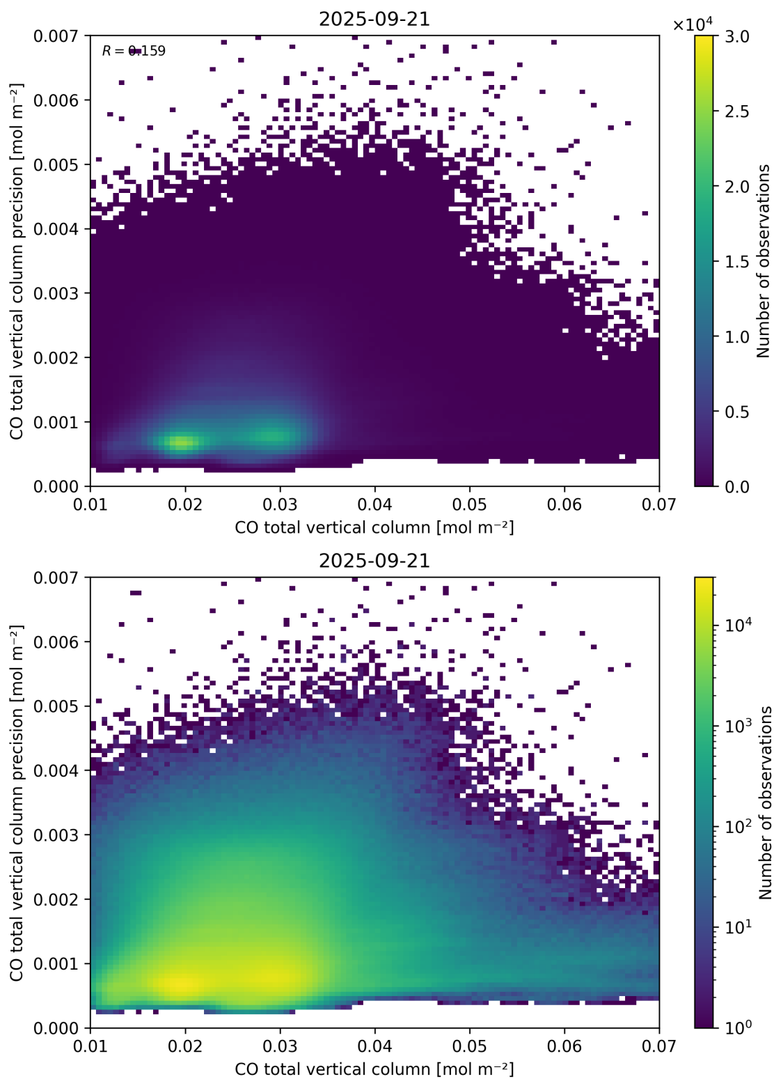
Figure 34: Scatter density plot of “CO total vertical column” against “CO total vertical column precision” for 2025-09-20 to 2025-09-22.
