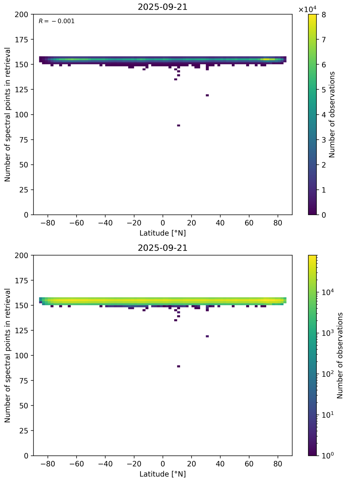
Figure 57: Scatter density plot of “Latitude” against “Number of spectral points in retrieval” for 2025-09-20 to 2025-09-22.
