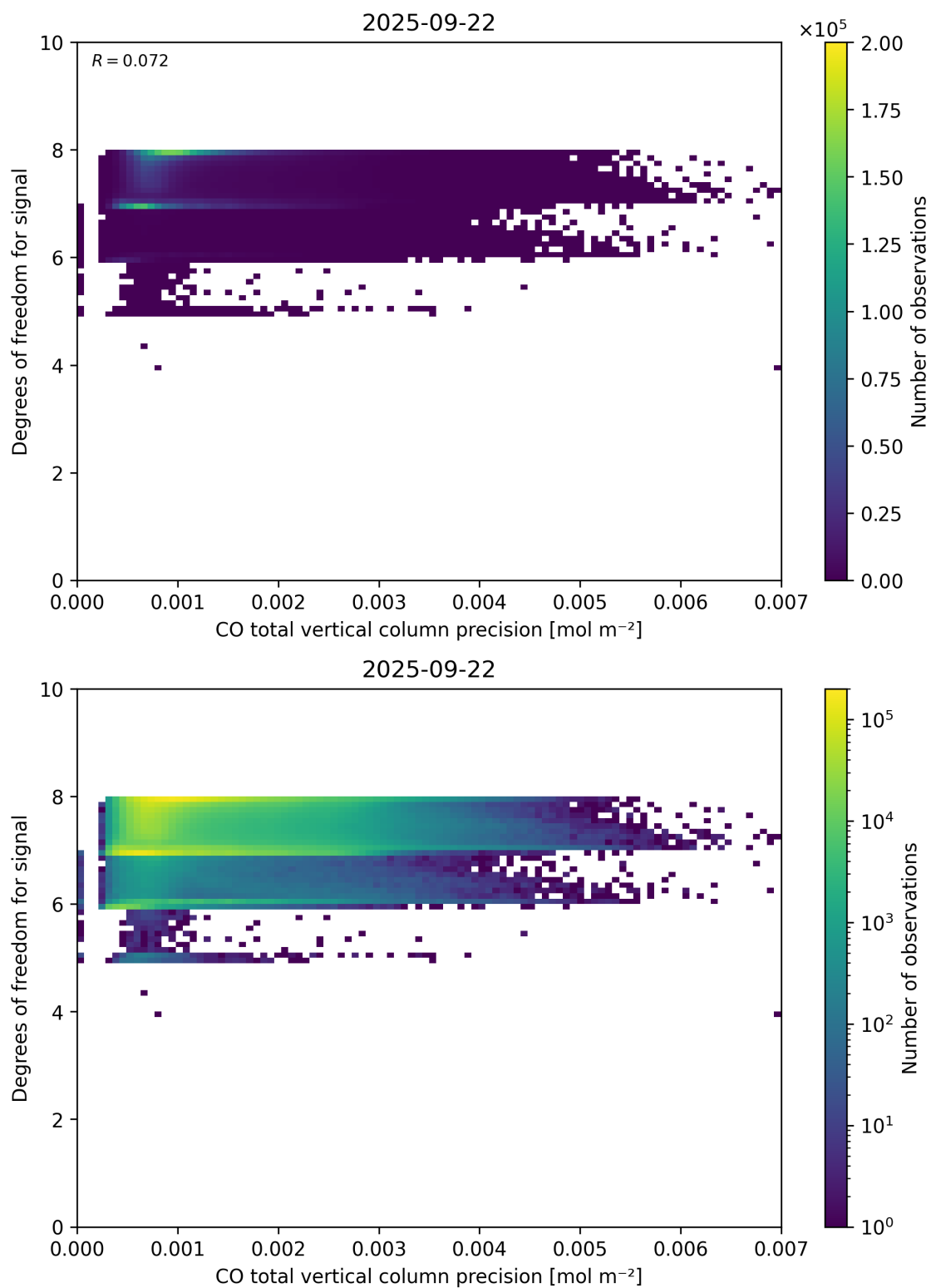
Figure 45: Scatter density plot of “CO total vertical column precision” against “Degrees of freedom for signal” for 2025-09-22 to 2025-09-23.
