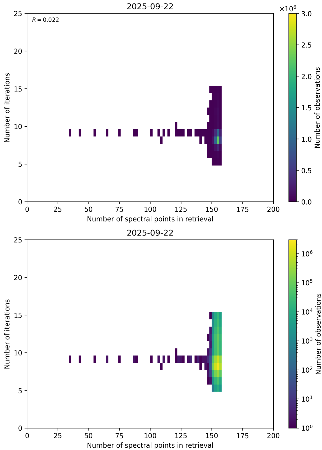
Figure 60: Scatter density plot of “Number of spectral points in retrieval” against “Number of iterations” for 2025-09-22 to 2025-09-23.
