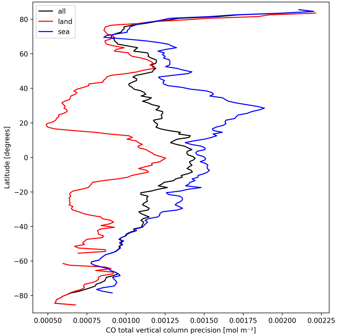
Figure 12: Zonal average of “CO total vertical column precision” for 2025-09-22 to 2025-09-23.
