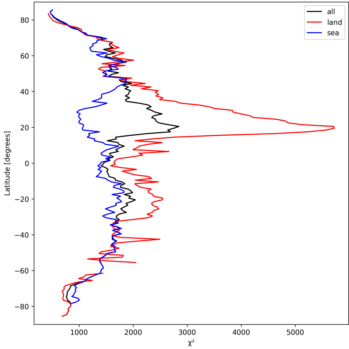
Figure 14: Zonal average of “ \chi^2 ” for 2025-09-22 to 2025-09-23.
