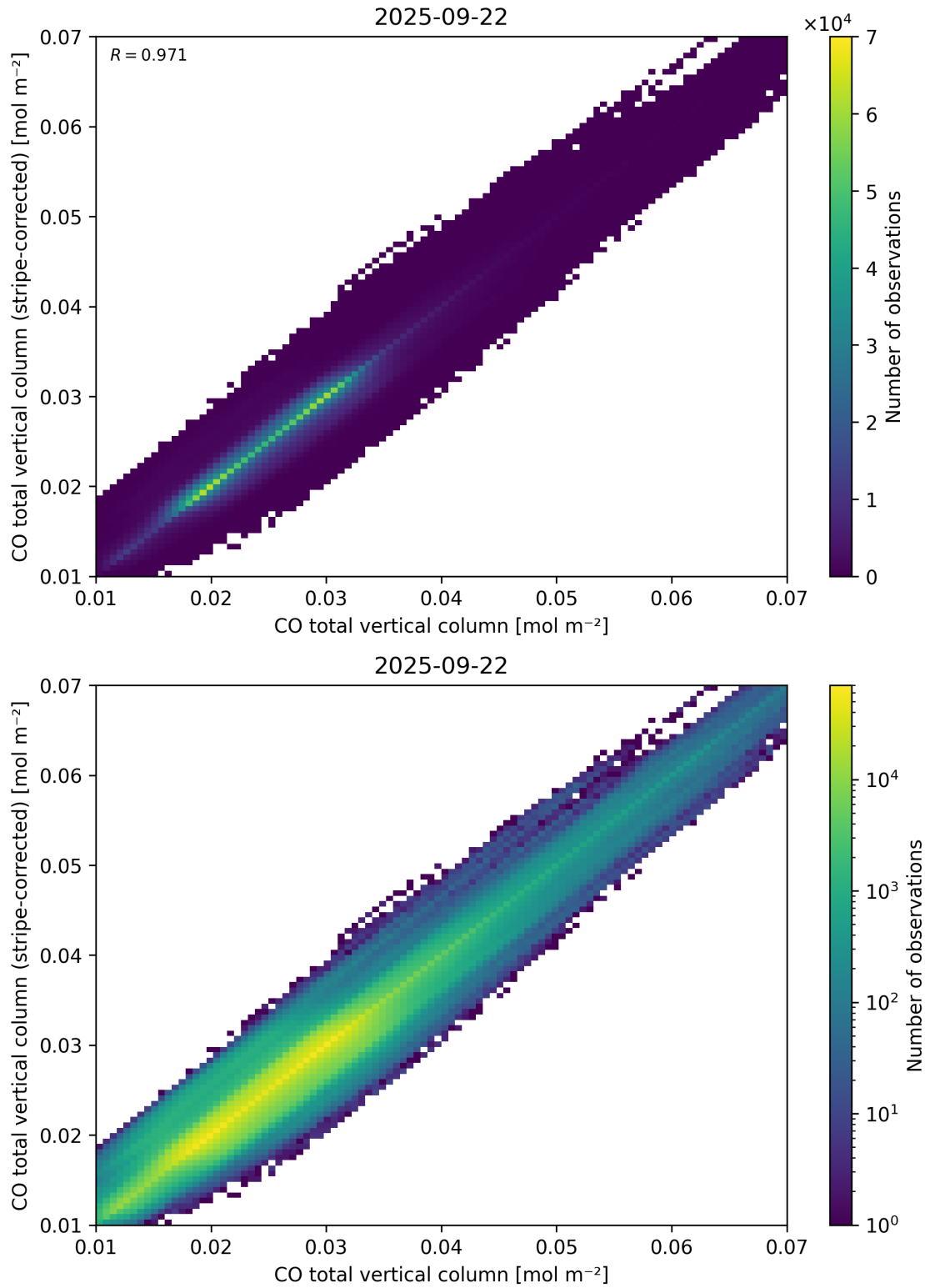
Figure 33: Scatter density plot of “CO total vertical column” against “CO total vertical column (stripe-corrected)” for 2025-09-22 to 2025-09-23.
