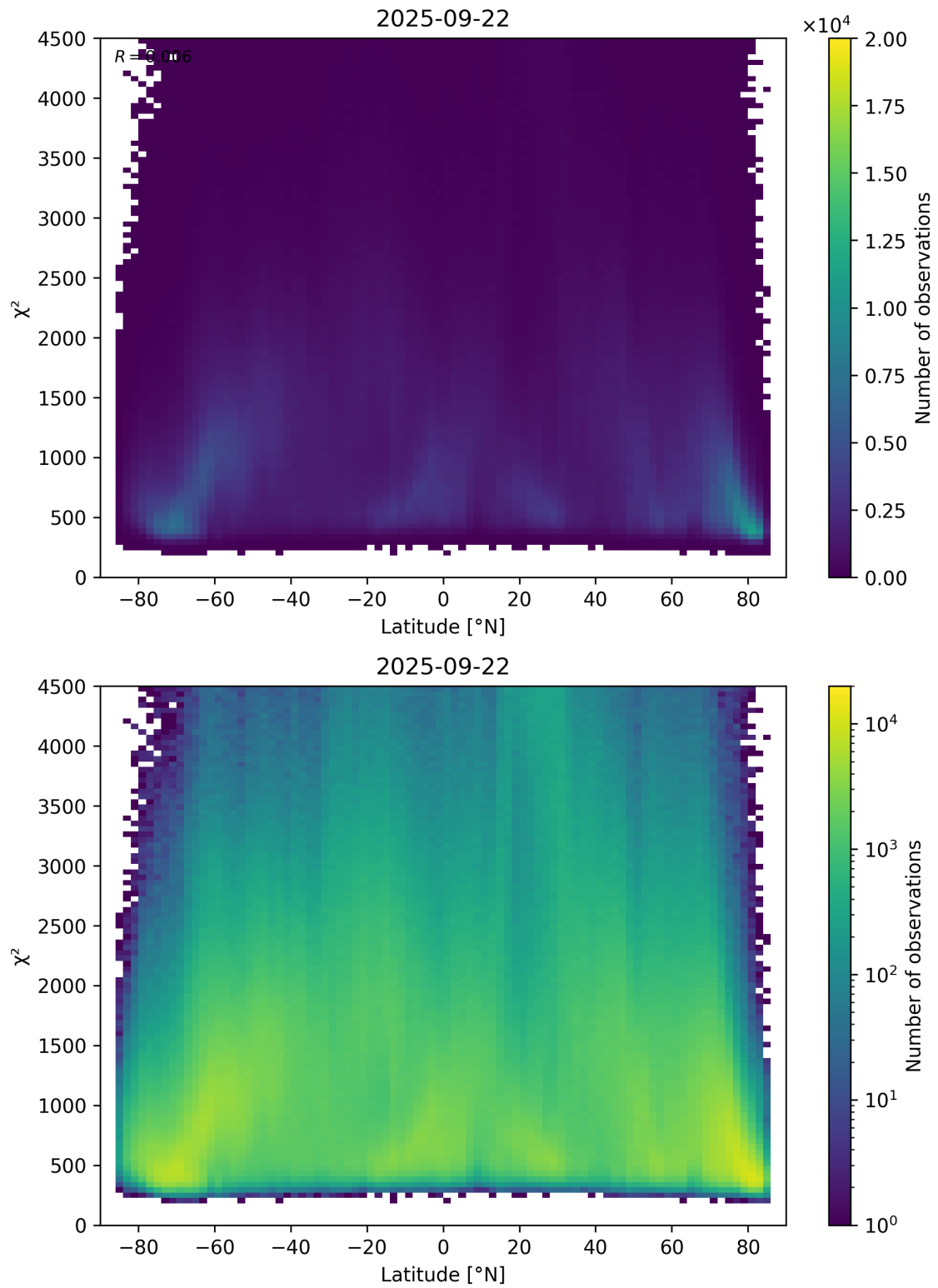
Figure 54: Scatter density plot of “Latitude” against “ \chi^2 ” for 2025-09-22 to 2025-09-23.
