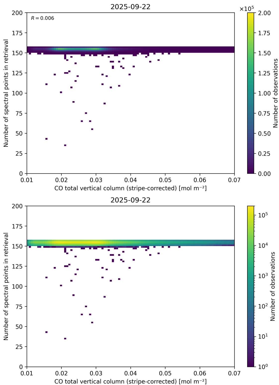
Figure 40: Scatter density plot of “CO total vertical column (stripe-corrected)” against “Number of spectral points in retrieval” for 2025-09-22 to 2025-09-23.
