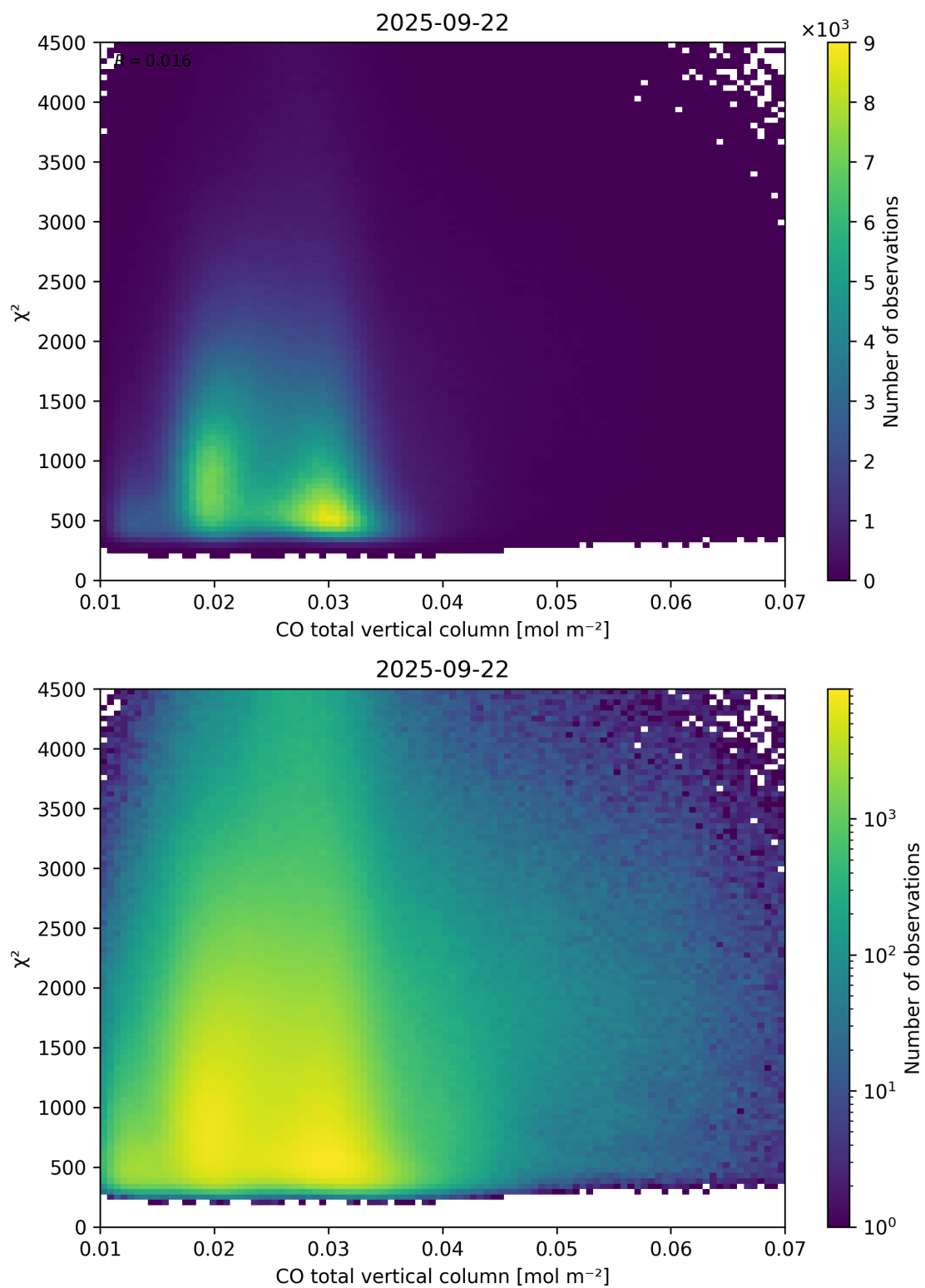
Figure 35: Scatter density plot of “CO total vertical column” against “ \chi^2 ” for 2025-09-22 to 2025-09-23.
