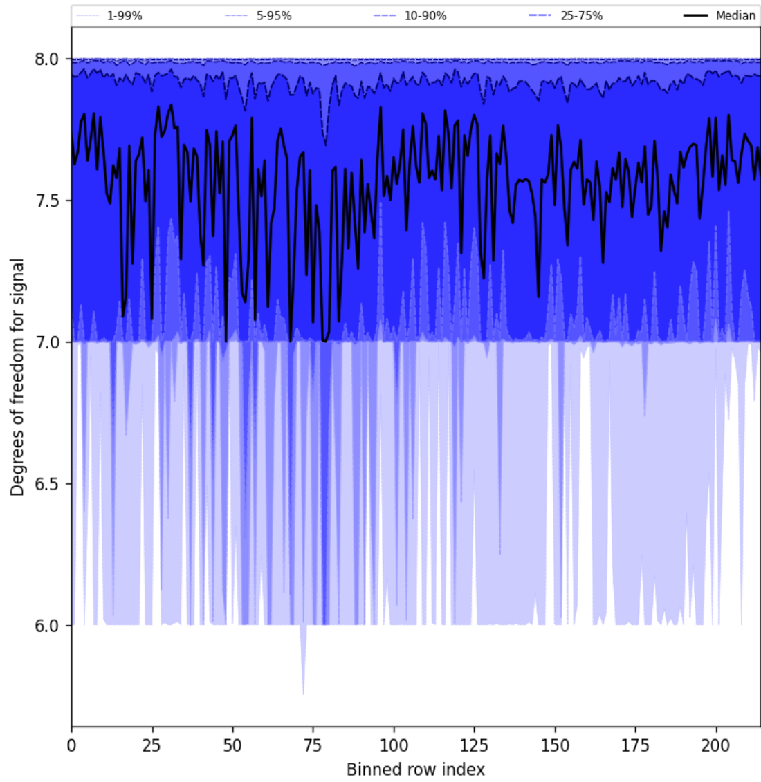
Figure 31: Along track statistics of “Degrees of freedom for signal” for 2025-09-22 to 2025-09-23
