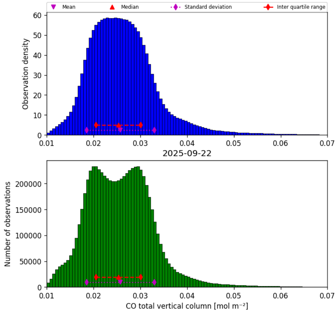
Figure 18: Histogram of “CO total vertical column” for 2025-09-22 to 2025-09-23
