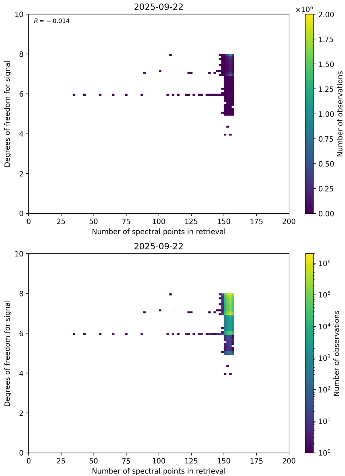
Figure 59: Scatter density plot of “Number of spectral points in retrieval” against “Degrees of freedom for signal” for 2025-09-22 to 2025-09-23.
