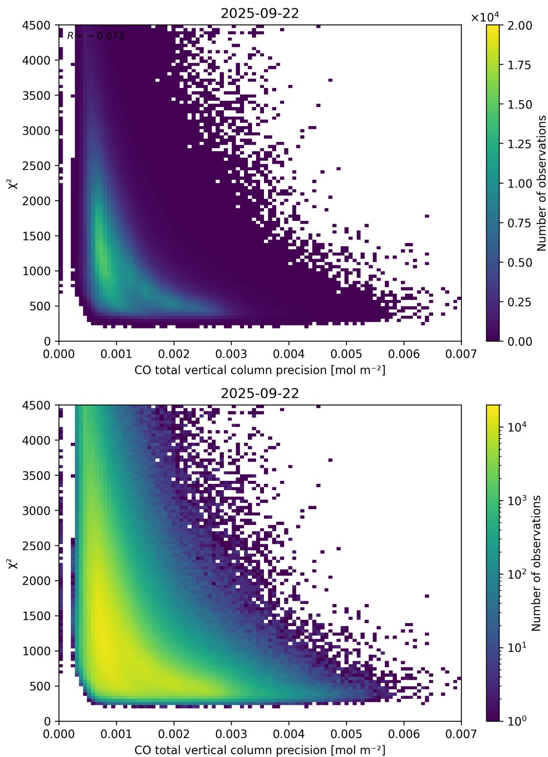
Figure 44: Scatter density plot of “CO total vertical column precision” against “ \chi^2 ” for 2025-09-22 to 2025-09-23.
