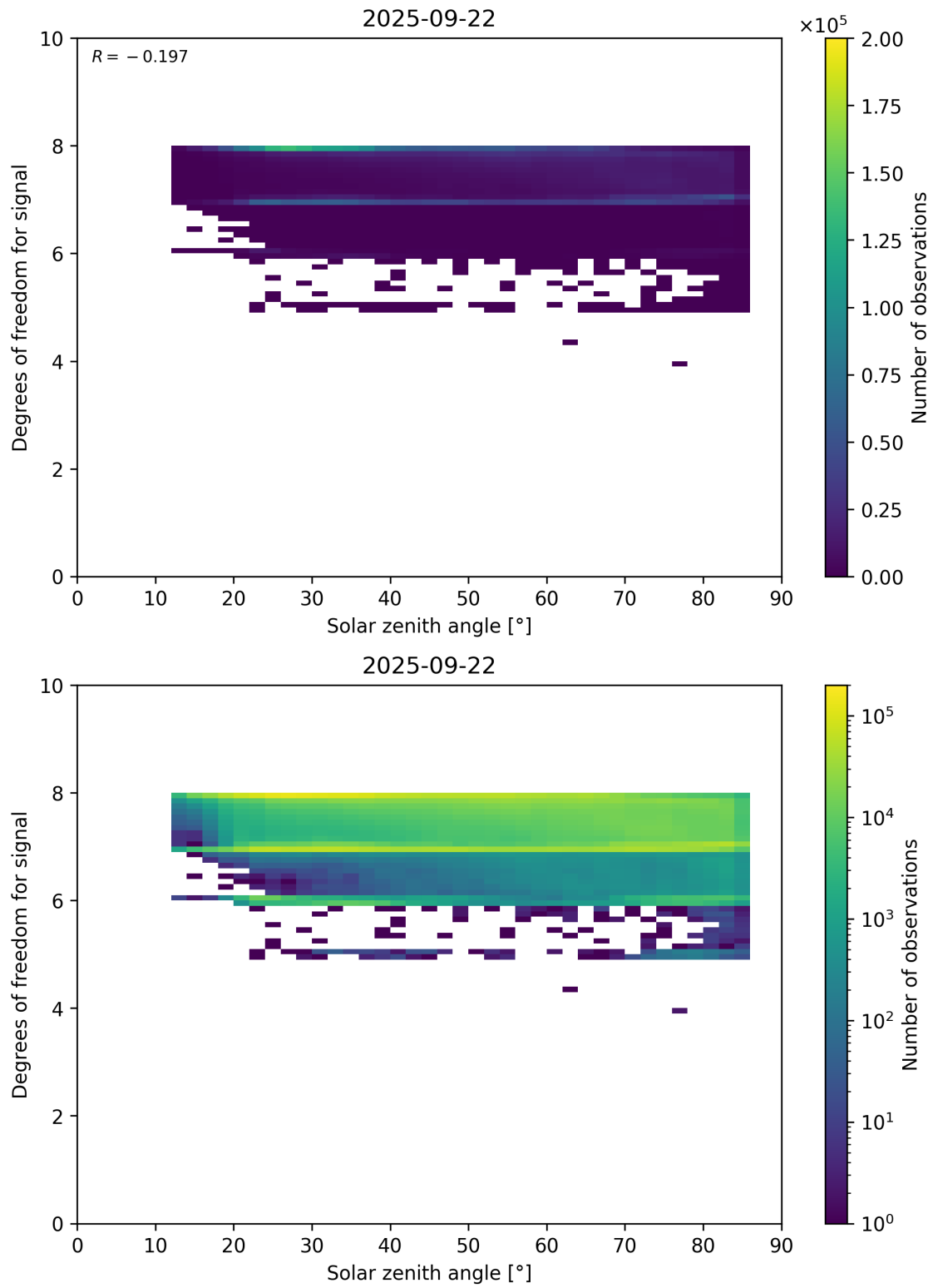
Figure 65: Scatter density plot of “Solar zenith angle” against “Degrees of freedom for signal” for 2025-09-22 to 2025-09-23.
