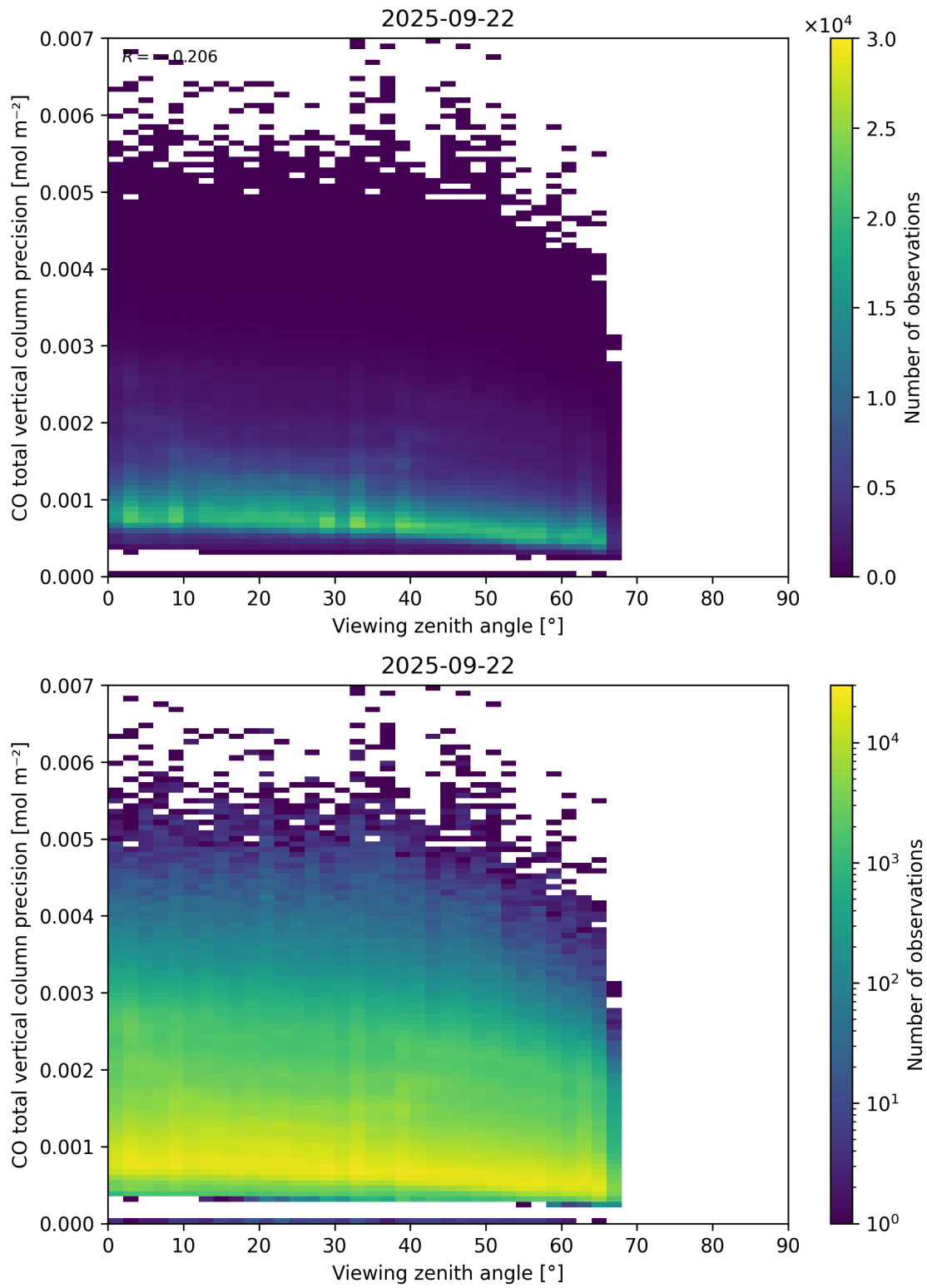
Figure 71: Scatter density plot of “Viewing zenith angle” against “CO total vertical column precision” for 2025-09-22 to 2025-09-23.
