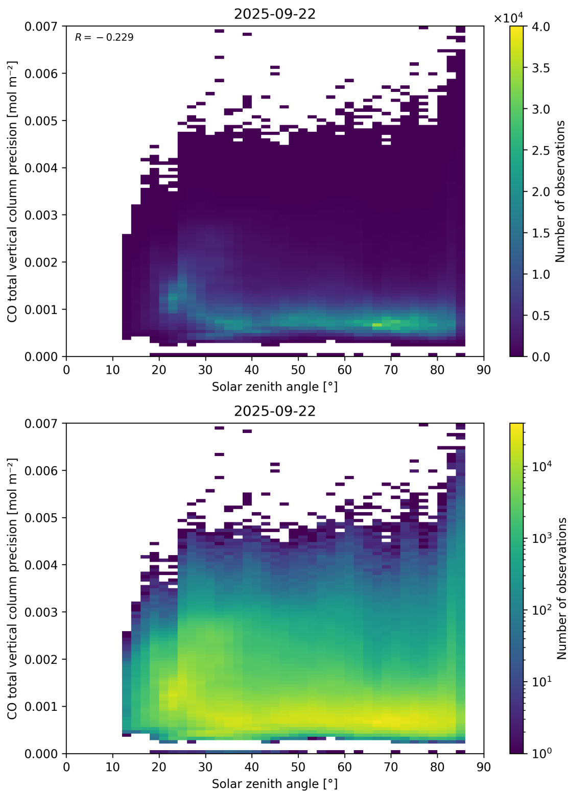
Figure 63: Scatter density plot of “Solar zenith angle” against “CO total vertical column precision” for 2025-09-22 to 2025-09-23.
