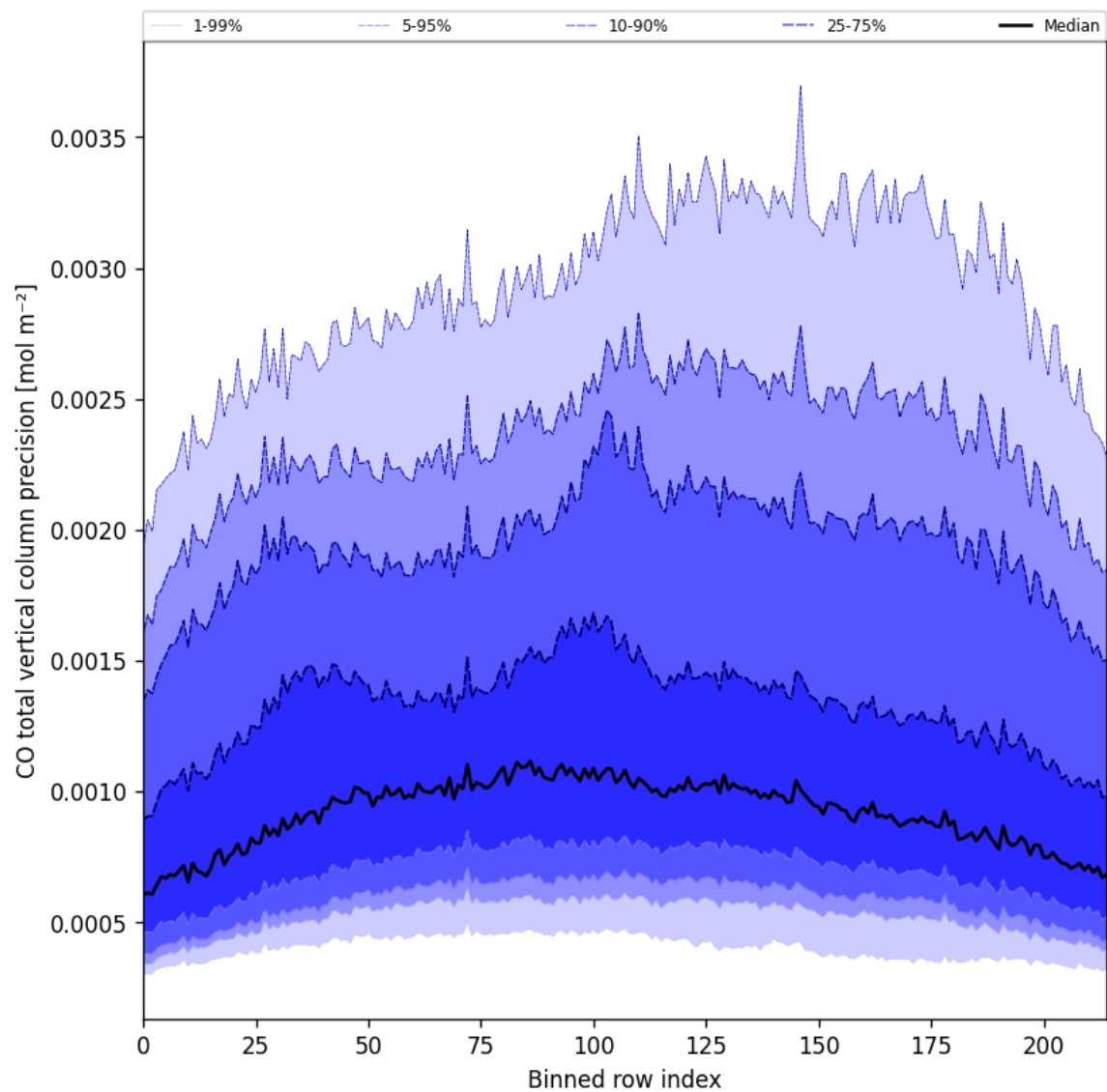
Figure 28: Along track statistics of “CO total vertical column precision” for 2025-09-22 to 2025-09-23
