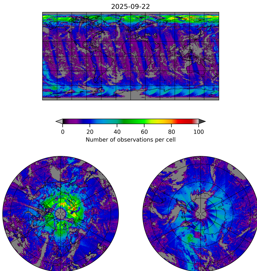
Figure 8: Map of the number of observations for 2025-09-22 to 2025-09-23
