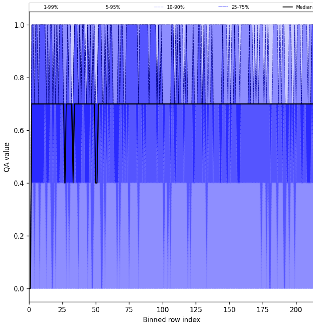
Figure 25: Along track statistics of “QA value” for 2025-09-22 to 2025-09-23
