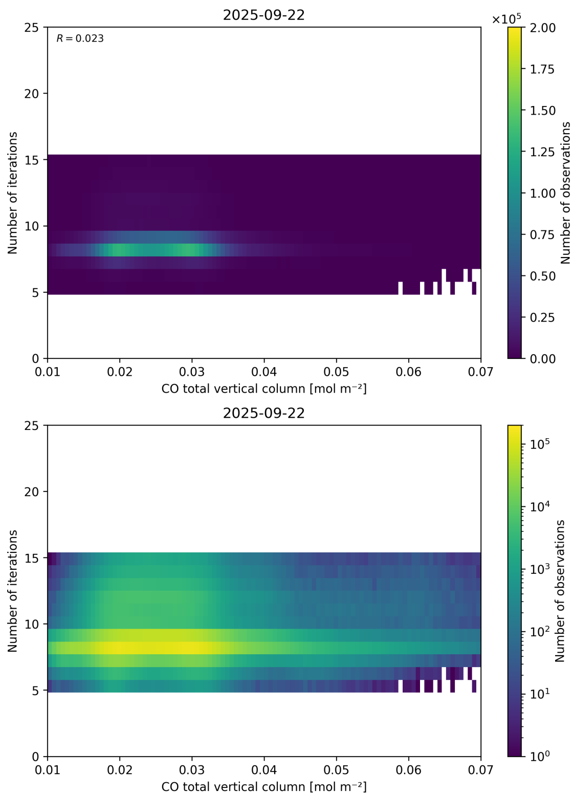
Figure 42: Scatter density plot of “CO total vertical column” against “Number of iterations” for 2025-09-22 to 2025-09-23.
