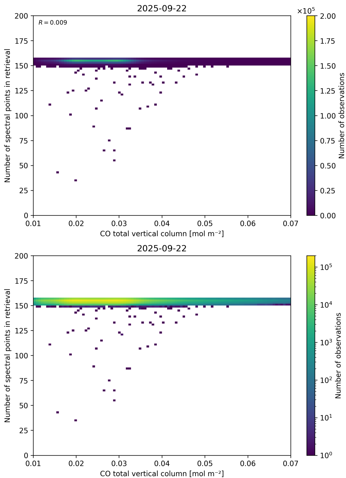
Figure 43: Scatter density plot of “CO total vertical column” against “Number of spectral points in retrieval” for 2025-09-22 to 2025-09-23.
