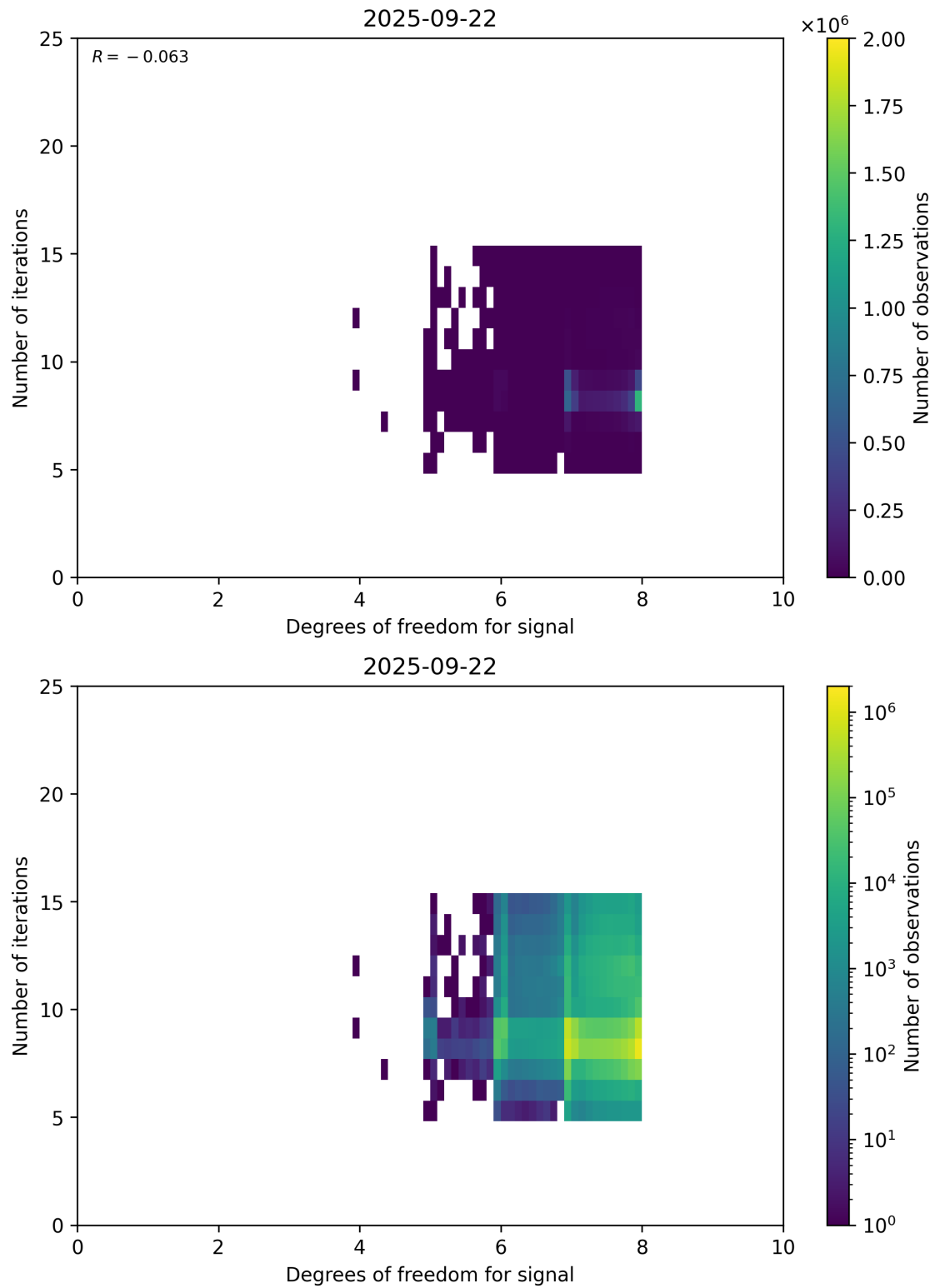
Figure 50: Scatter density plot of “Degrees of freedom for signal” against “Number of iterations” for 2025-09-22 to 2025-09-23.
