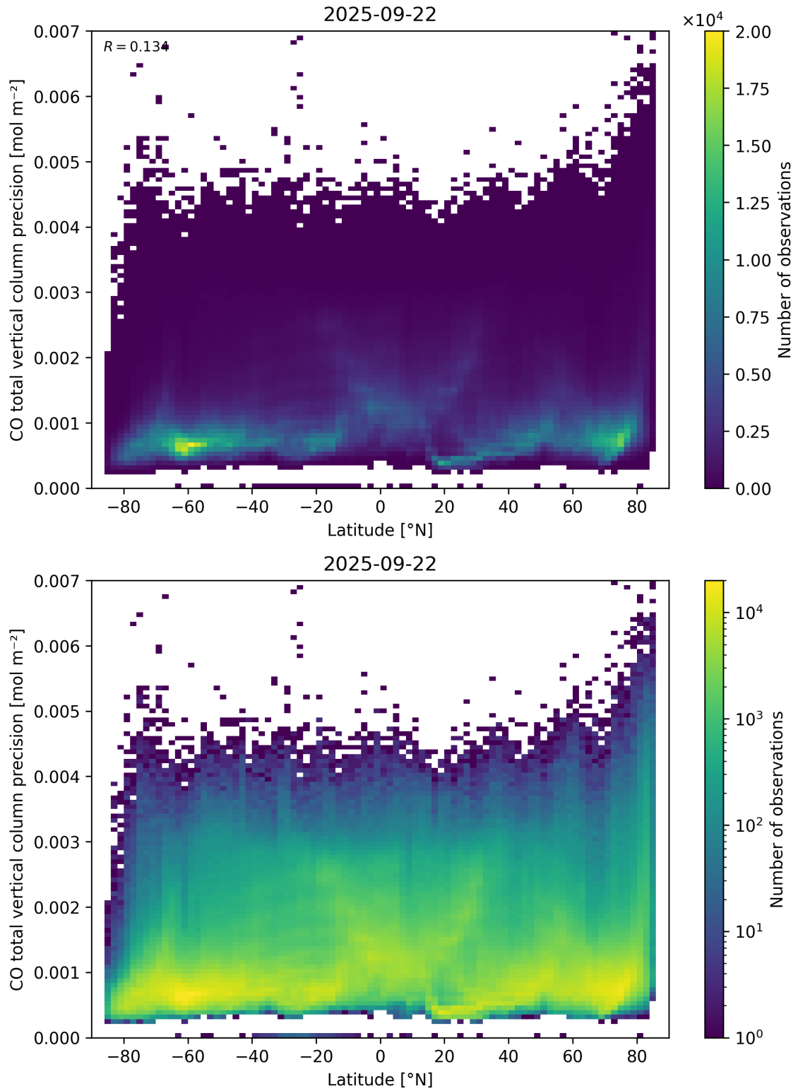
Figure 53: Scatter density plot of “Latitude” against “CO total vertical column precision” for 2025-09-22 to 2025-09-23.
