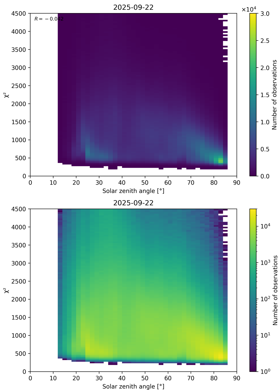
Figure 64: Scatter density plot of “Solar zenith angle” against “ \chi^2 ” for 2025-09-22 to 2025-09-23.
