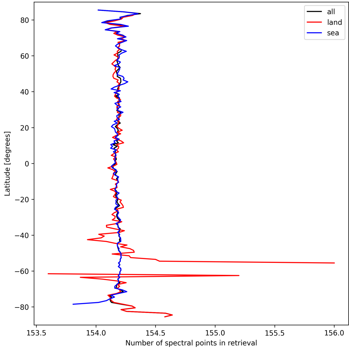
Figure 13: Zonal average of “Number of spectral points in retrieval” for 2025-09-22 to 2025-09-23.
