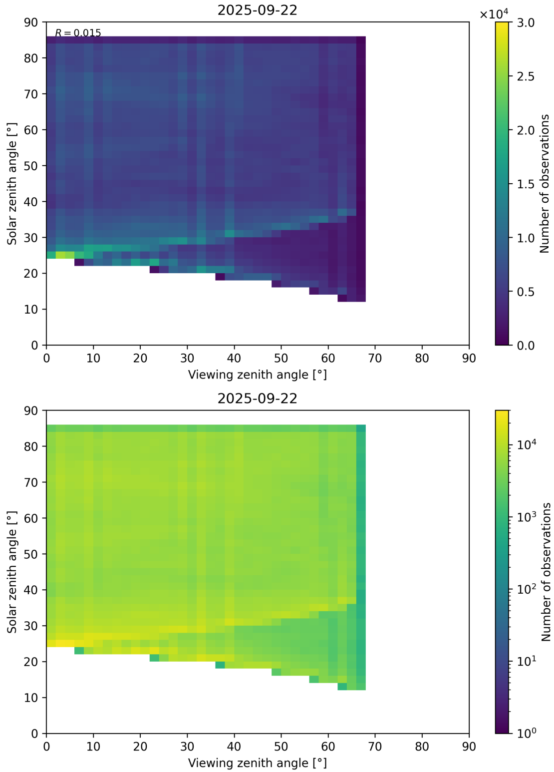
Figure 77: Scatter density plot of “Viewing zenith angle” against “Solar zenith angle” for 2025-09-22 to 2025-09-23.
