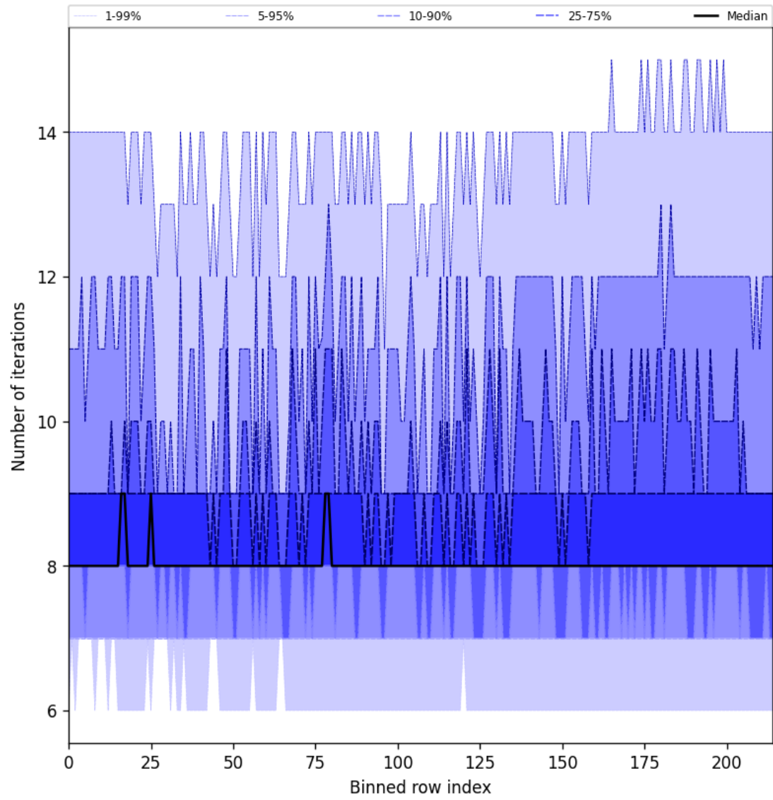
Figure 32: Along track statistics of “Number of iterations” for 2025-09-22 to 2025-09-23
