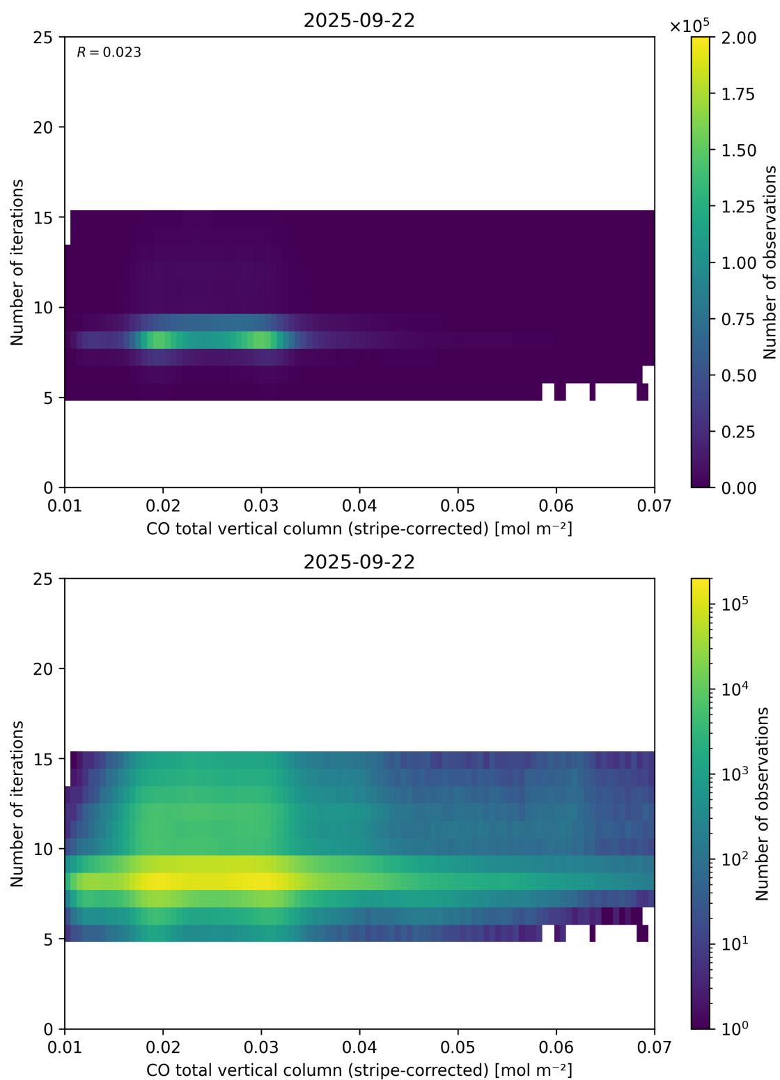
Figure 39: Scatter density plot of “CO total vertical column (stripe-corrected)” against “Number of iterations” for 2025-09-22 to 2025-09-23.
