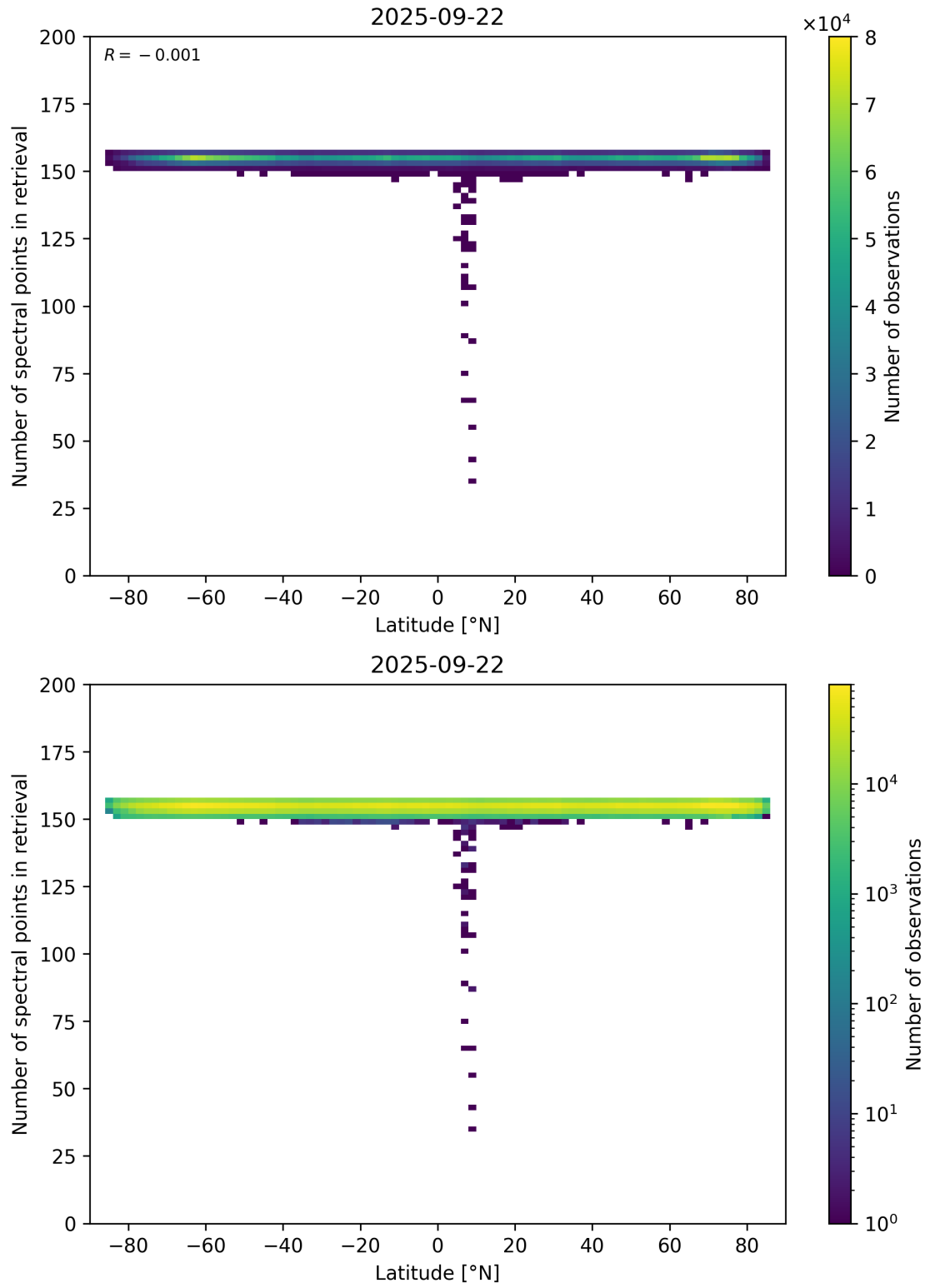
Figure 57: Scatter density plot of “Latitude” against “Number of spectral points in retrieval” for 2025-09-22 to 2025-09-23.
