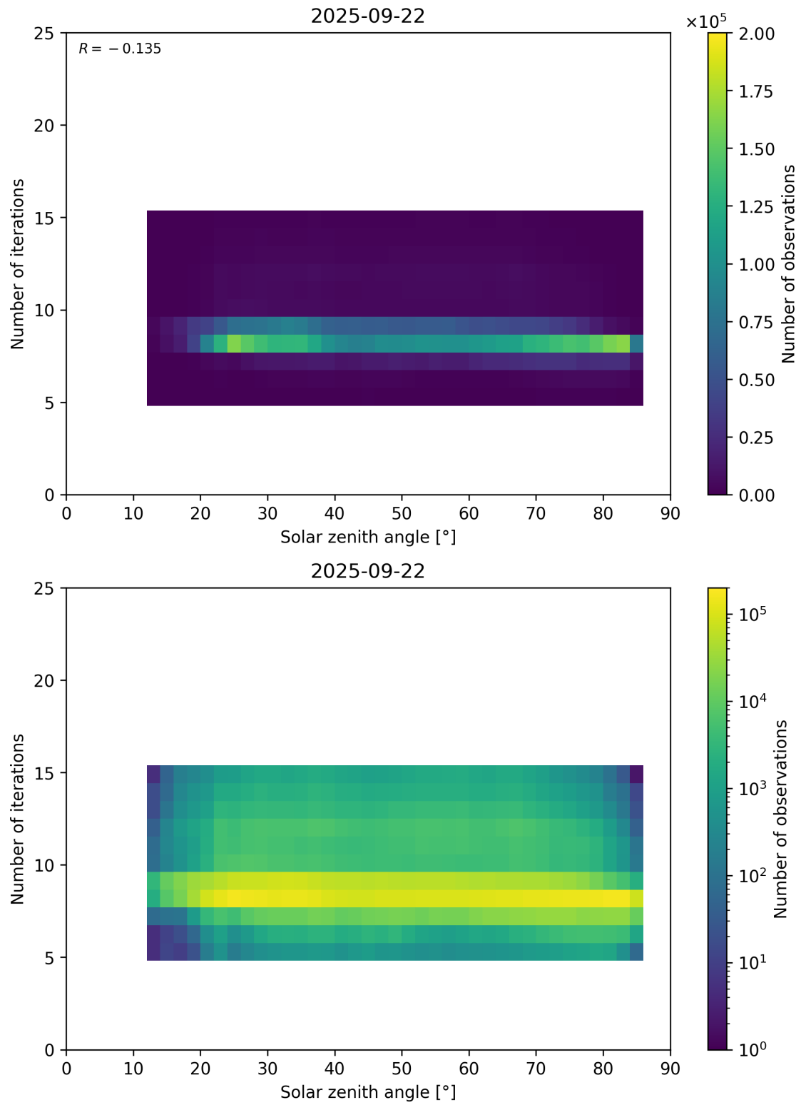
Figure 67: Scatter density plot of “Solar zenith angle” against “Number of iterations” for 2025-09-22 to 2025-09-23.
