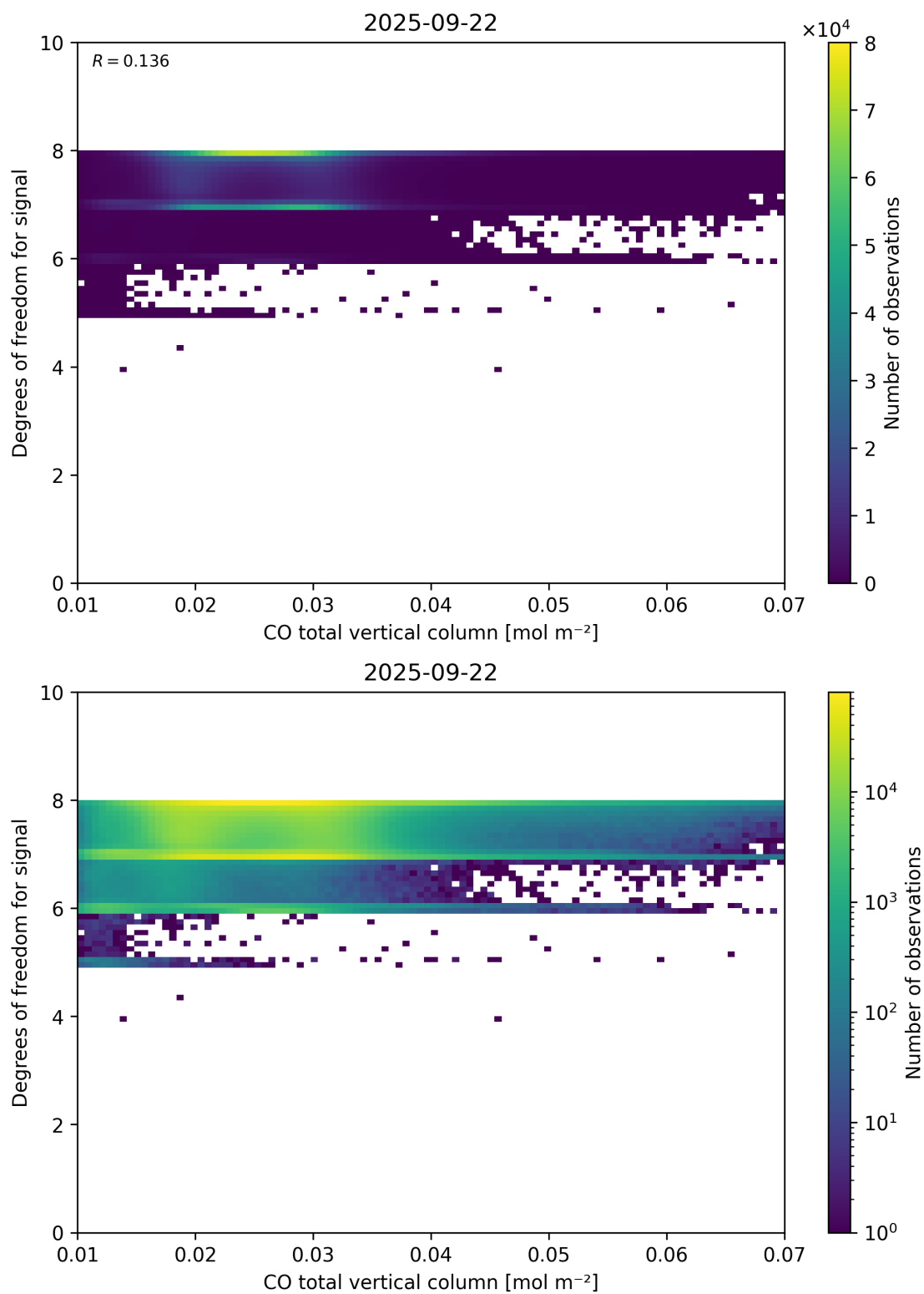
Figure 41: Scatter density plot of “CO total vertical column” against “Degrees of freedom for signal” for 2025-09-22 to 2025-09-23.
