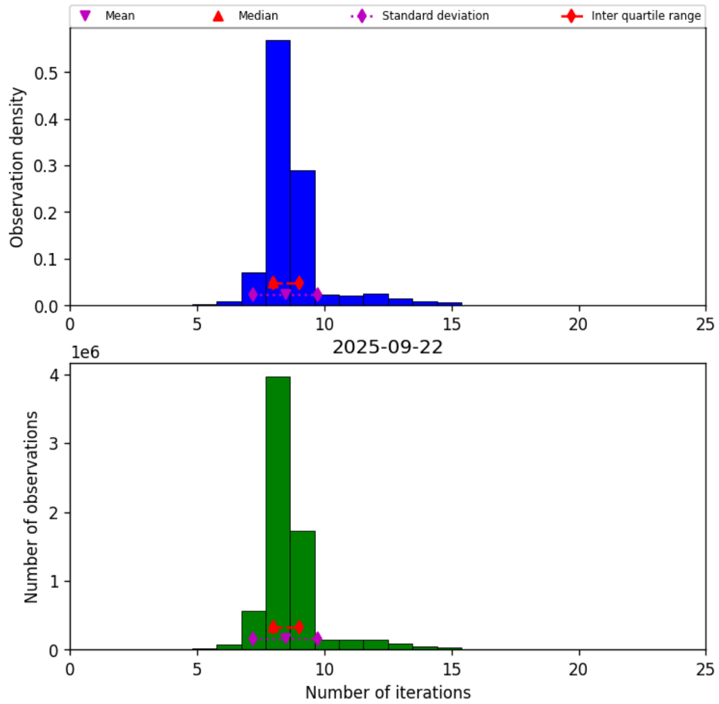
Figure 24: Histogram of “Number of iterations” for 2025-09-22 to 2025-09-23
