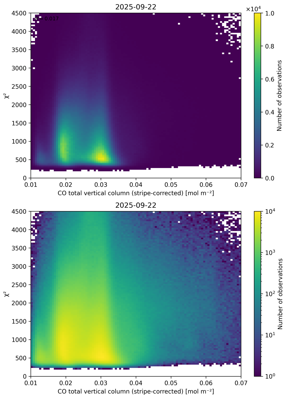
Figure 37: Scatter density plot of “CO total vertical column (stripe-corrected)” against “ \chi^2 ” for 2025-09-22 to 2025-09-23.
