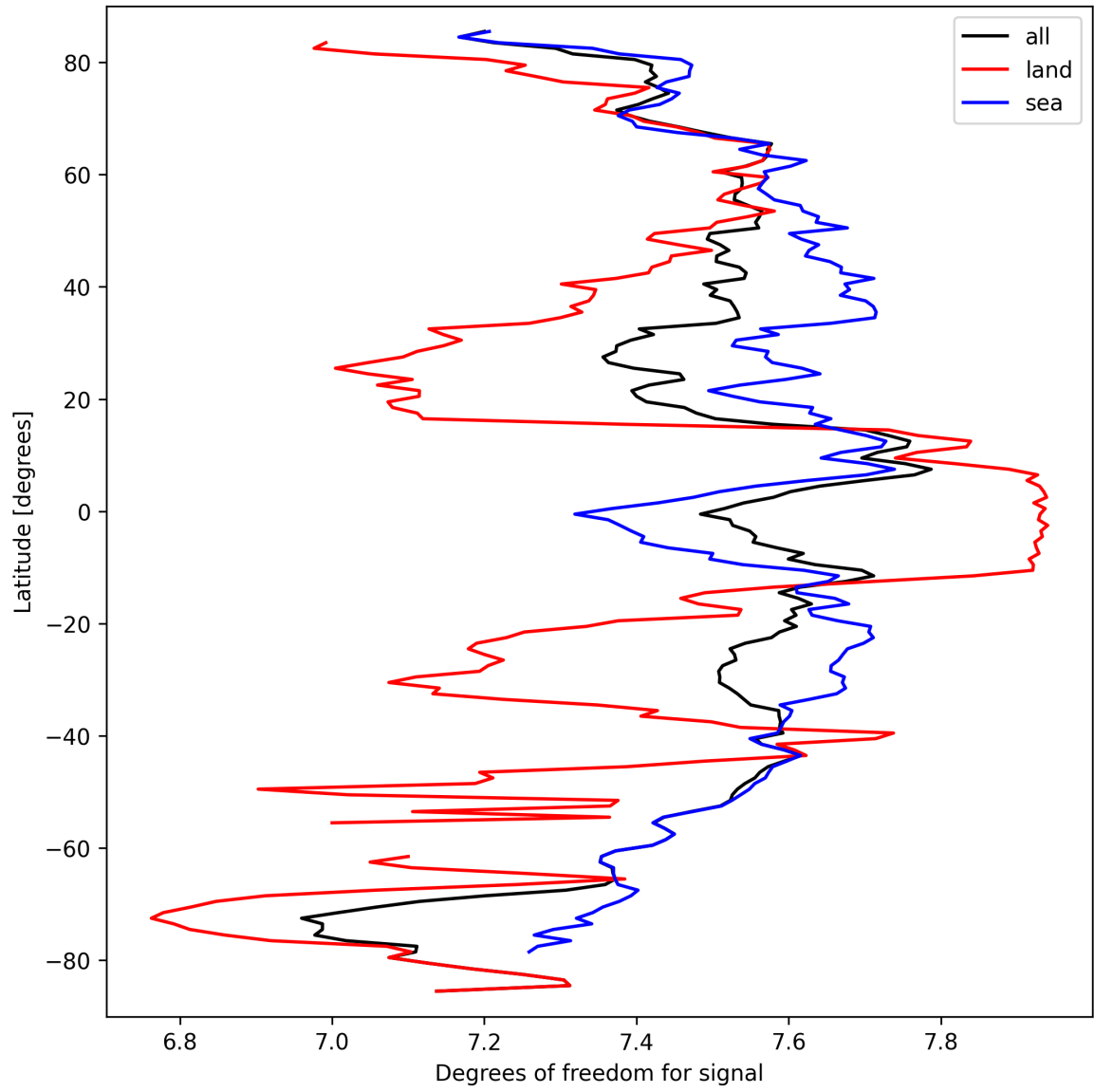
Figure 15: Zonal average of “Degrees of freedom for signal” for 2025-09-22 to 2025-09-23.
