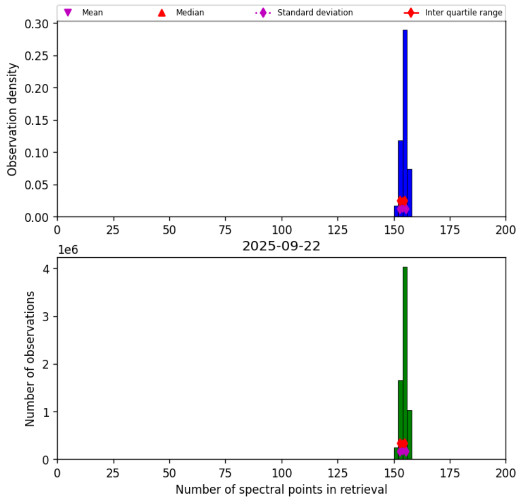
Figure 21: Histogram of “Number of spectral points in retrieval” for 2025-09-22 to 2025-09-23
