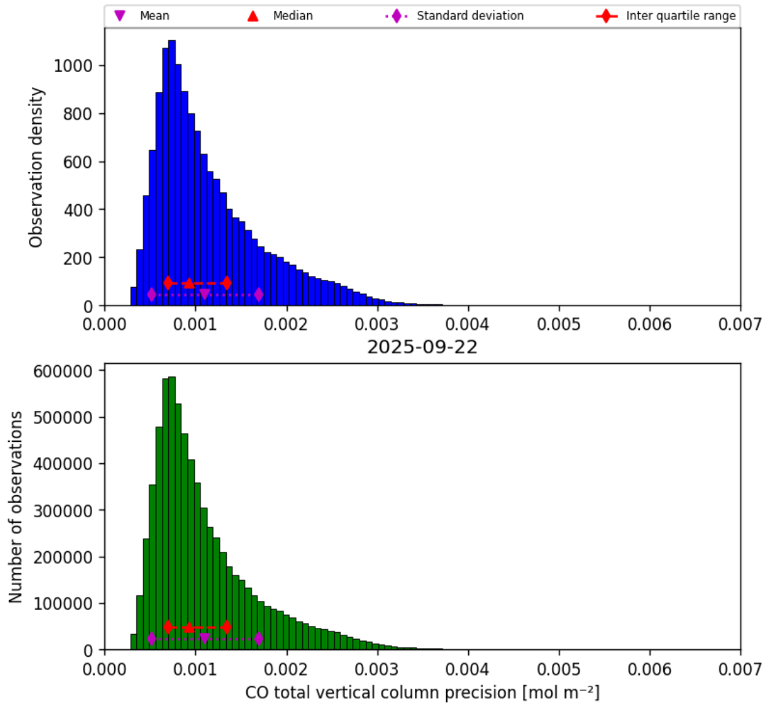
Figure 20: Histogram of “CO total vertical column precision” for 2025-09-22 to 2025-09-23
