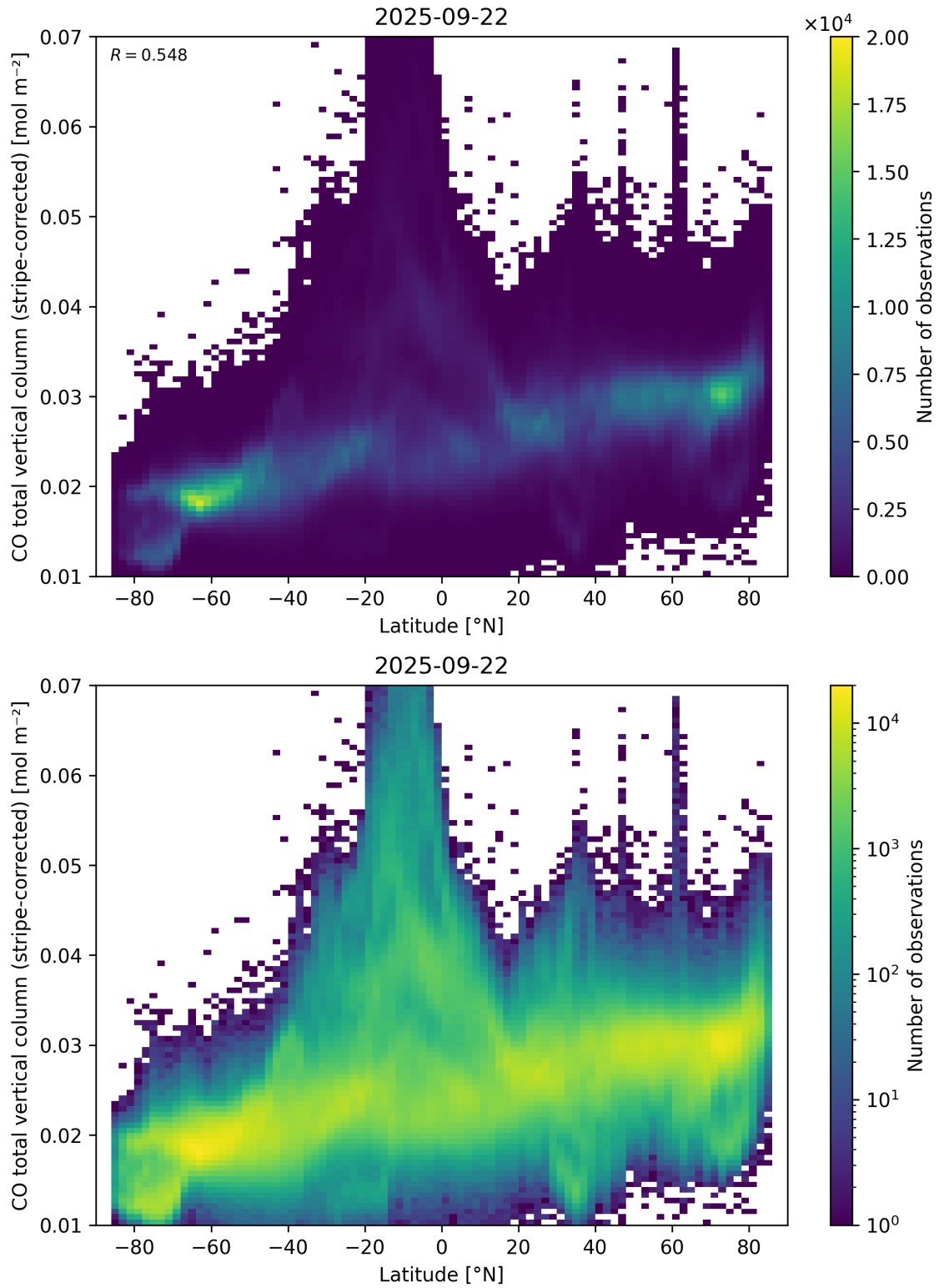
Figure 52: Scatter density plot of “Latitude” against “CO total vertical column (stripe-corrected)” for 2025-09-22 to 2025-09-23.
