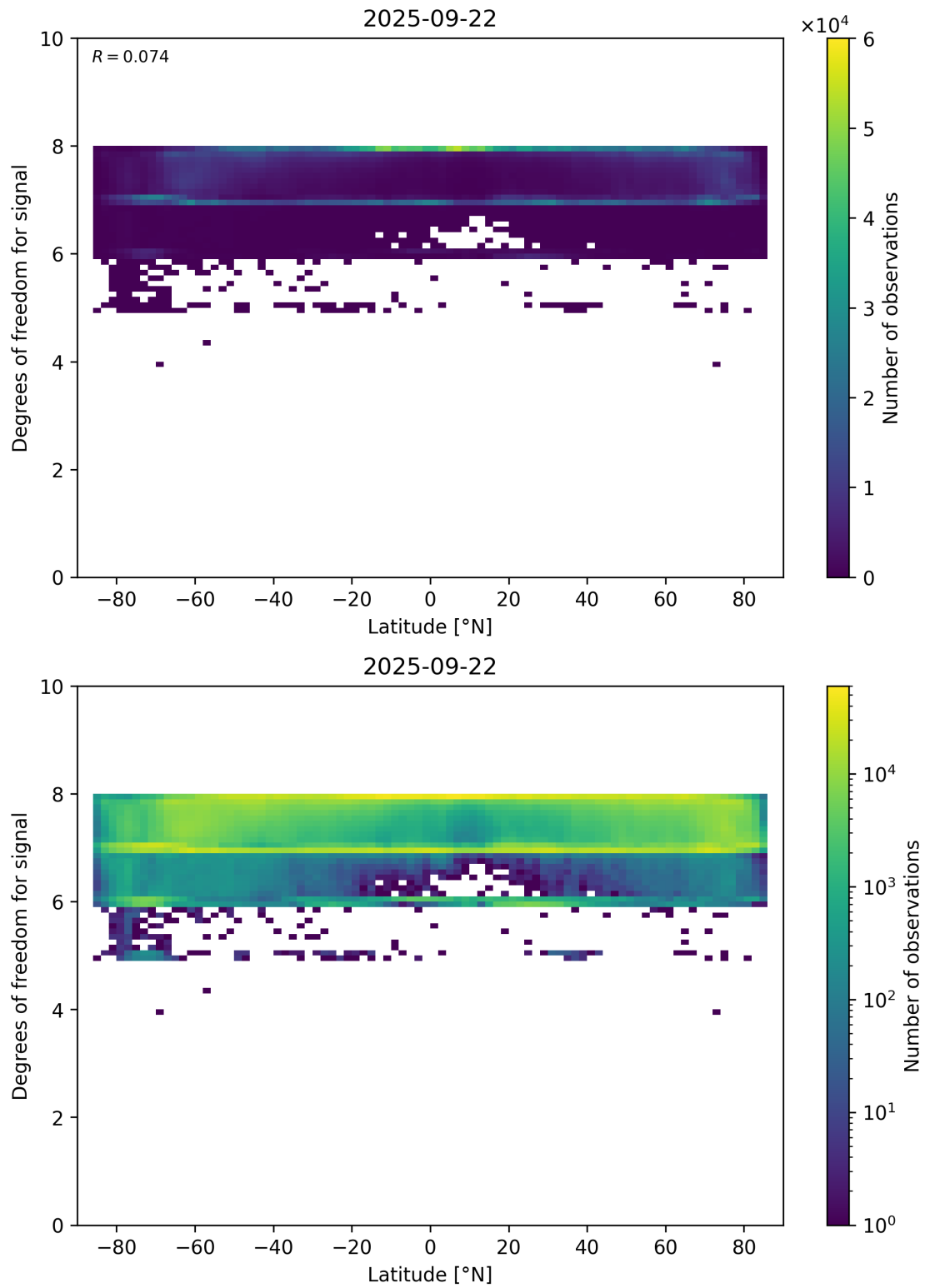
Figure 55: Scatter density plot of “Latitude” against “Degrees of freedom for signal” for 2025-09-22 to 2025-09-23.
