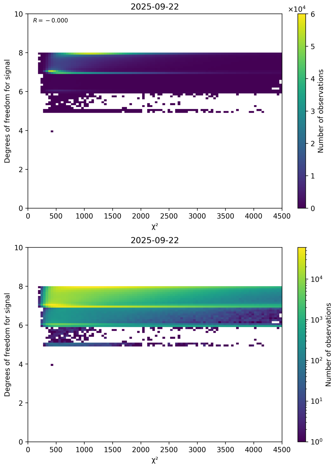
Figure 48: Scatter density plot of " \chi^2 " against "Degrees of freedom for signal" for 2025-09-22 to 2025-09-23.
