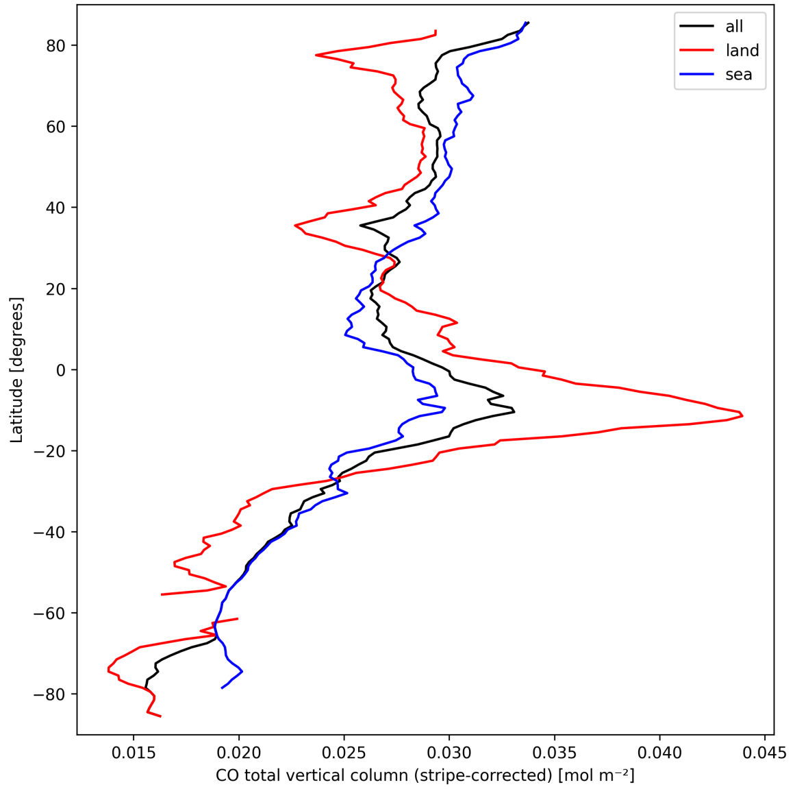
Figure 11: Zonal average of “CO total vertical column (stripe-corrected)” for 2025-09-22 to 2025-09-23.
