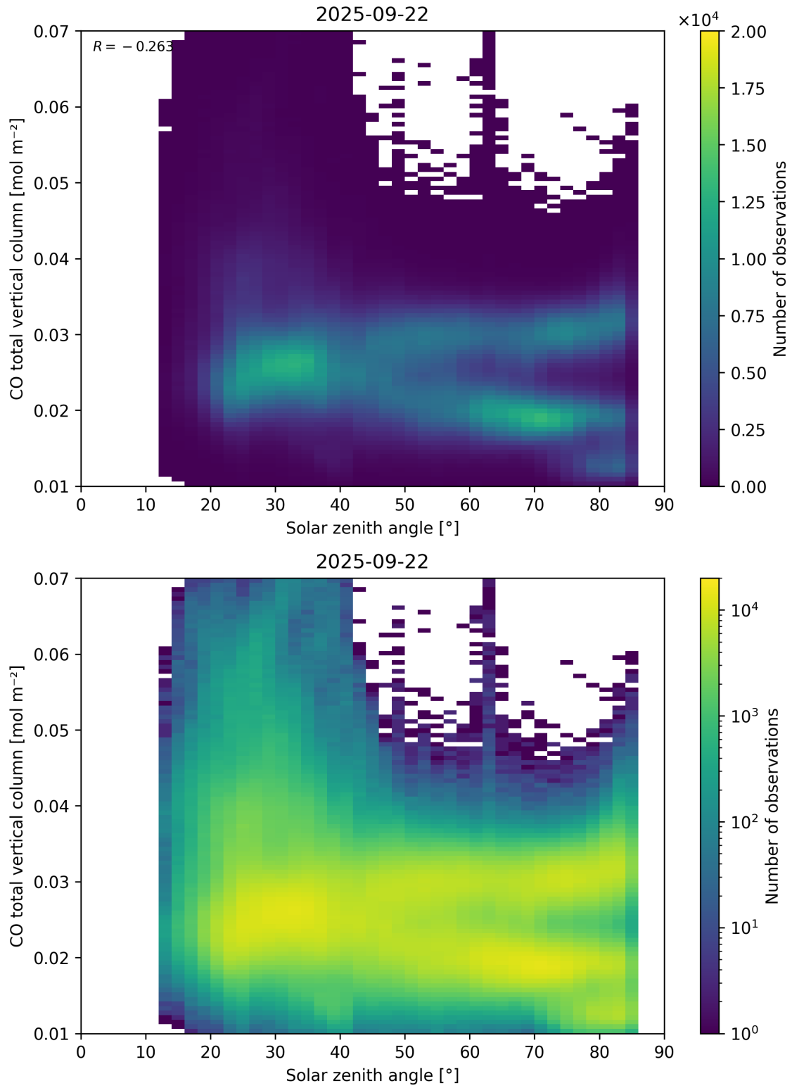
Figure 61: Scatter density plot of “Solar zenith angle” against “CO total vertical column” for 2025-09-22 to 2025-09-23.
