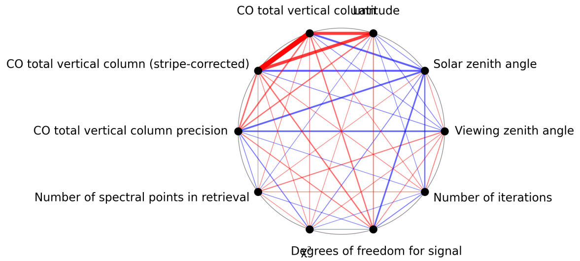
Figure 1: Map of correlation graph for 2025-09-22 to 2025-09-23.
