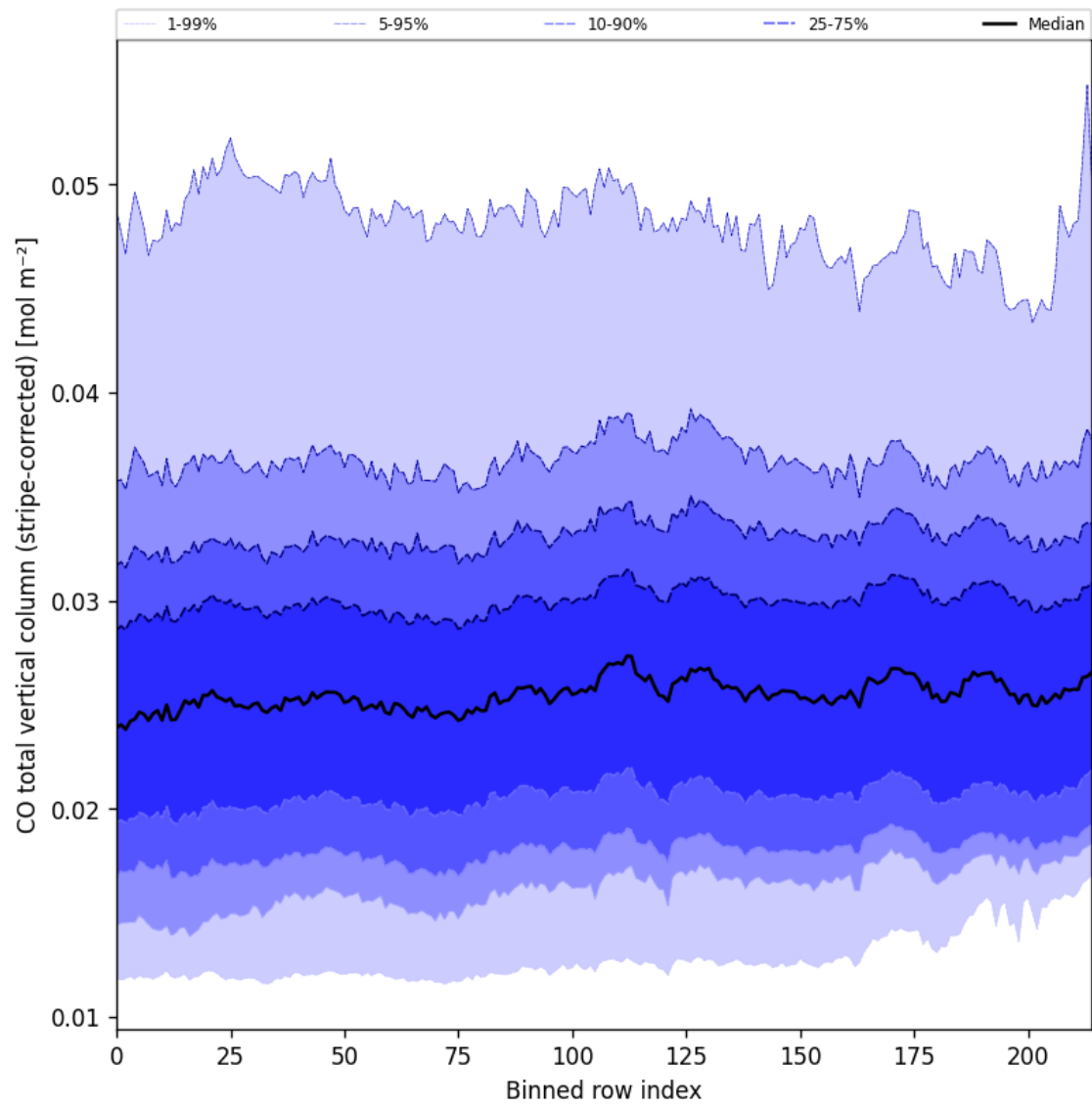
Figure 27: Along track statistics of “CO total vertical column (stripe-corrected)” for 2025-09-22 to 2025-09-23
