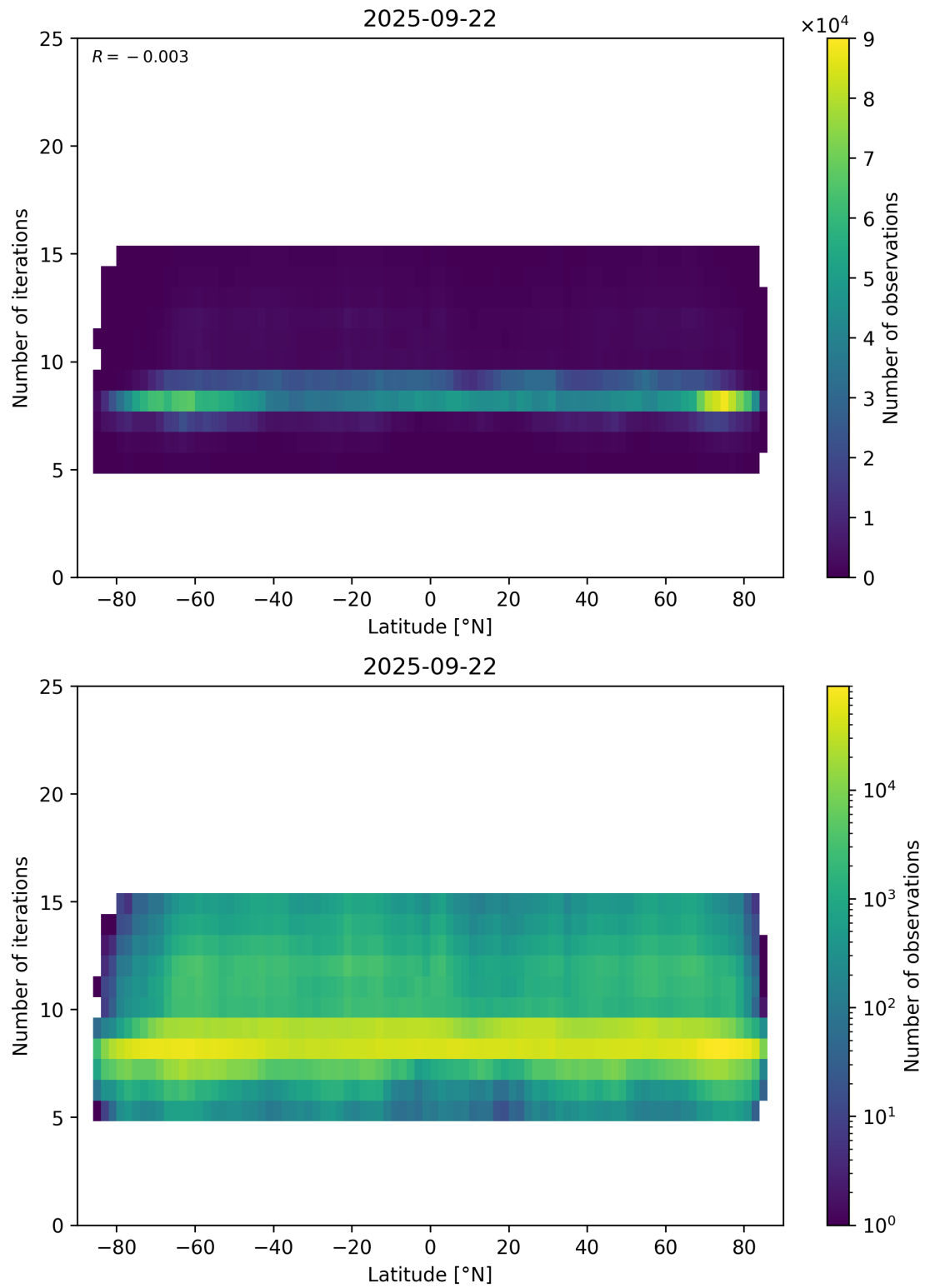
Figure 56: Scatter density plot of “Latitude” against “Number of iterations” for 2025-09-22 to 2025-09-23.
