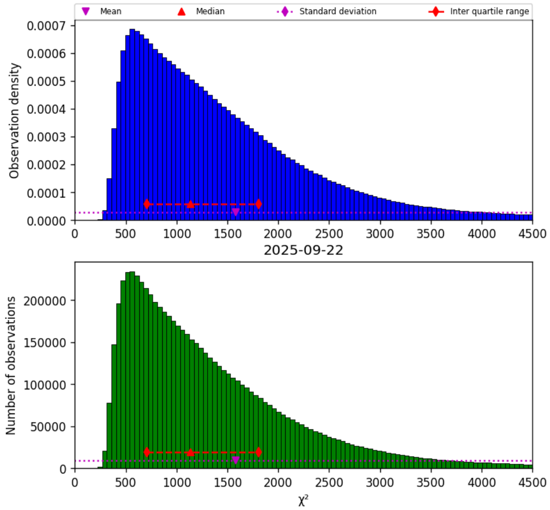
Figure 22: Histogram of " \chi^2 " for 2025-09-22 to 2025-09-23
