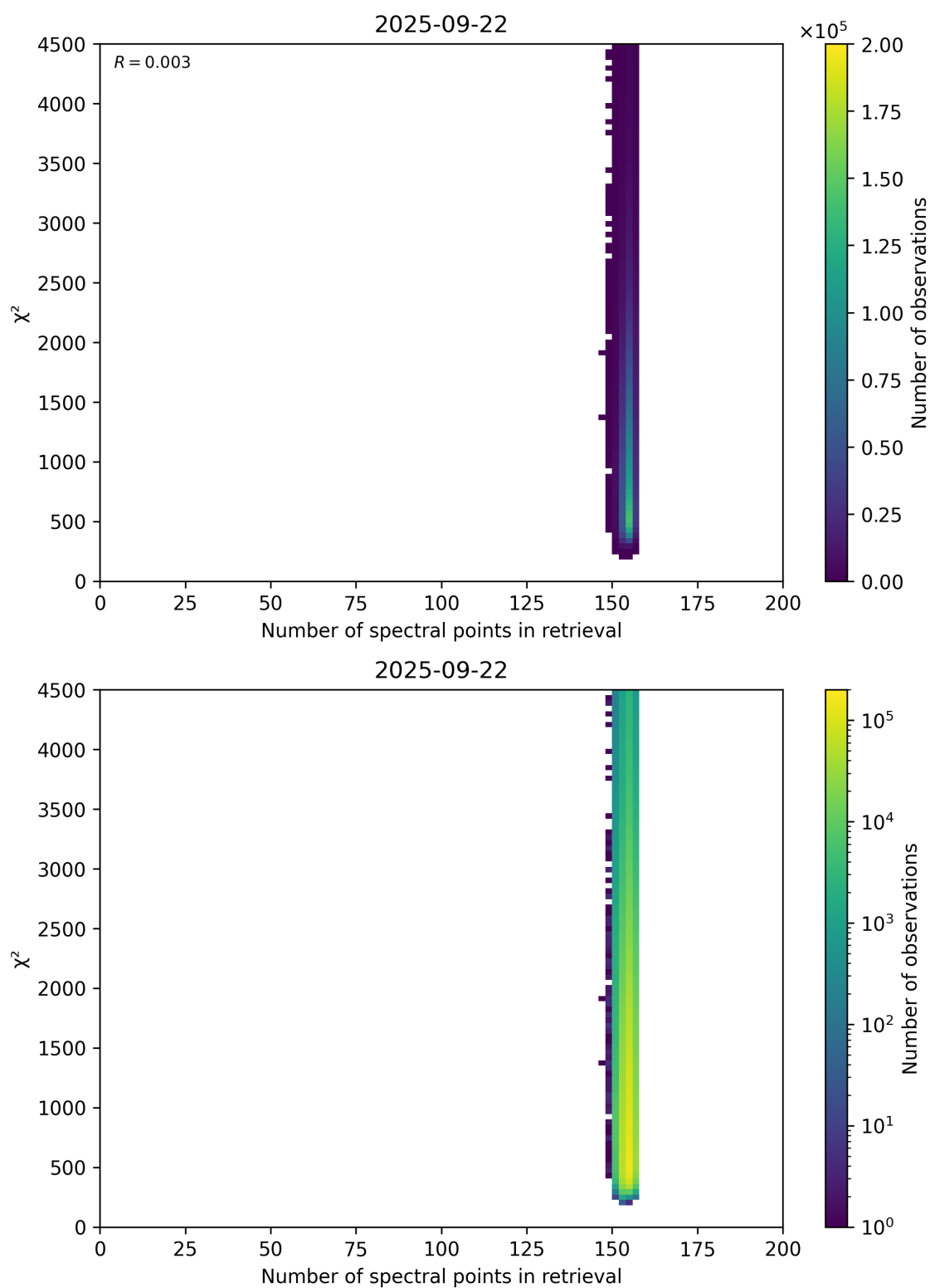
Figure 58: Scatter density plot of “Number of spectral points in retrieval” against “ \chi^2 ” for 2025-09-22 to 2025-09-23.
