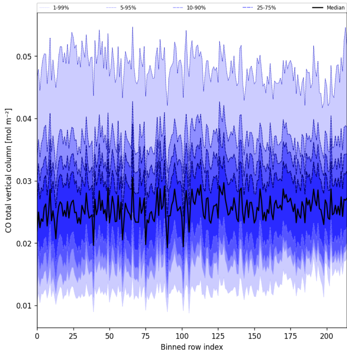
Figure 26: Along track statistics of “CO total vertical column” for 2025-09-22 to 2025-09-23
