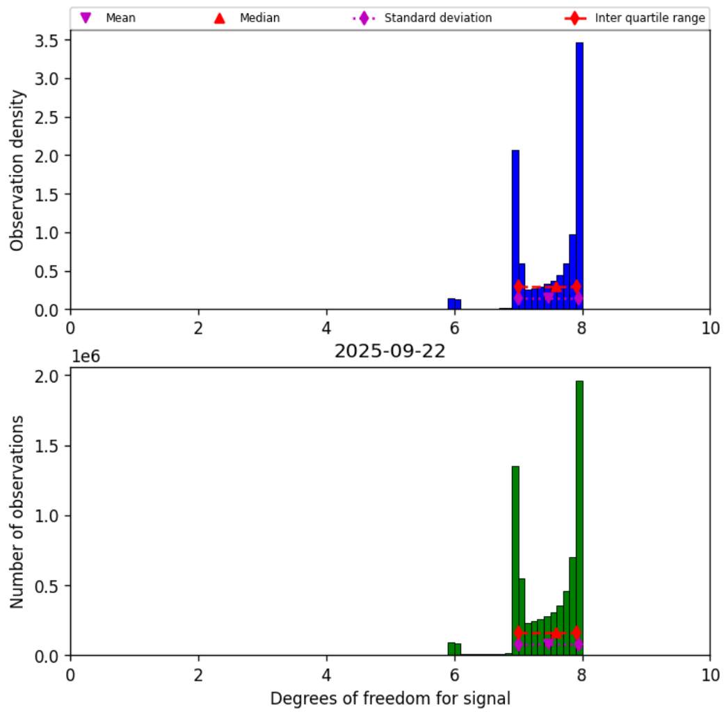
Figure 23: Histogram of “Degrees of freedom for signal” for 2025-09-22 to 2025-09-23
