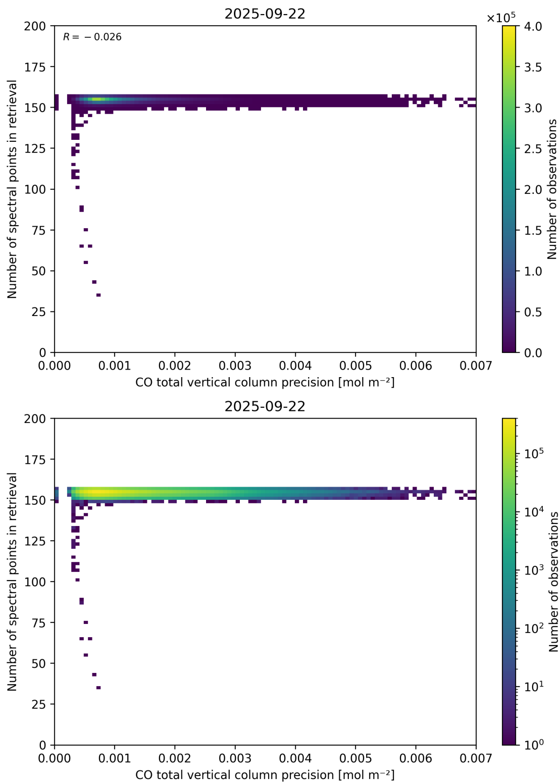
Figure 47: Scatter density plot of “CO total vertical column precision” against “Number of spectral points in retrieval” for 2025-09-22 to 2025-09-23.
