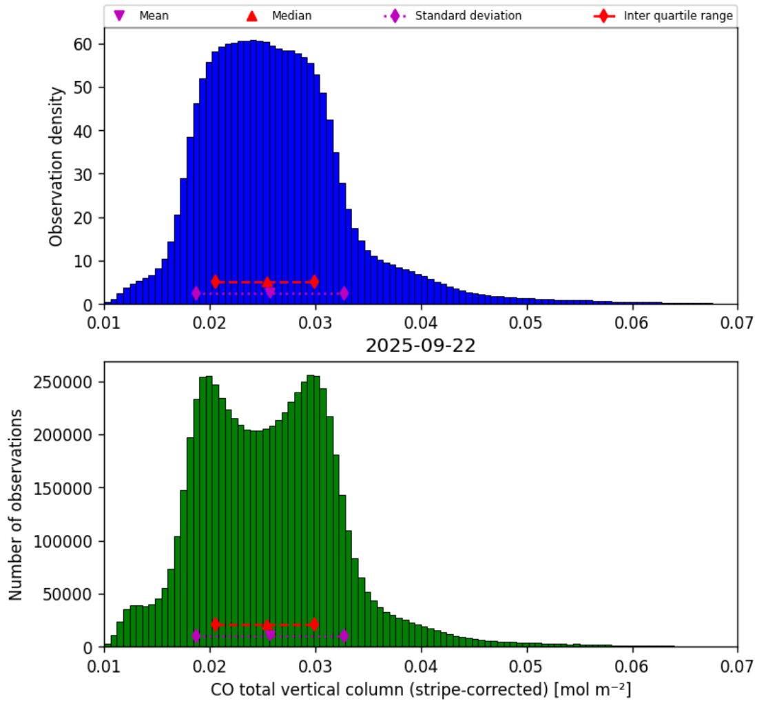
Figure 19: Histogram of “CO total vertical column (stripe-corrected)” for 2025-09-22 to 2025-09-23
