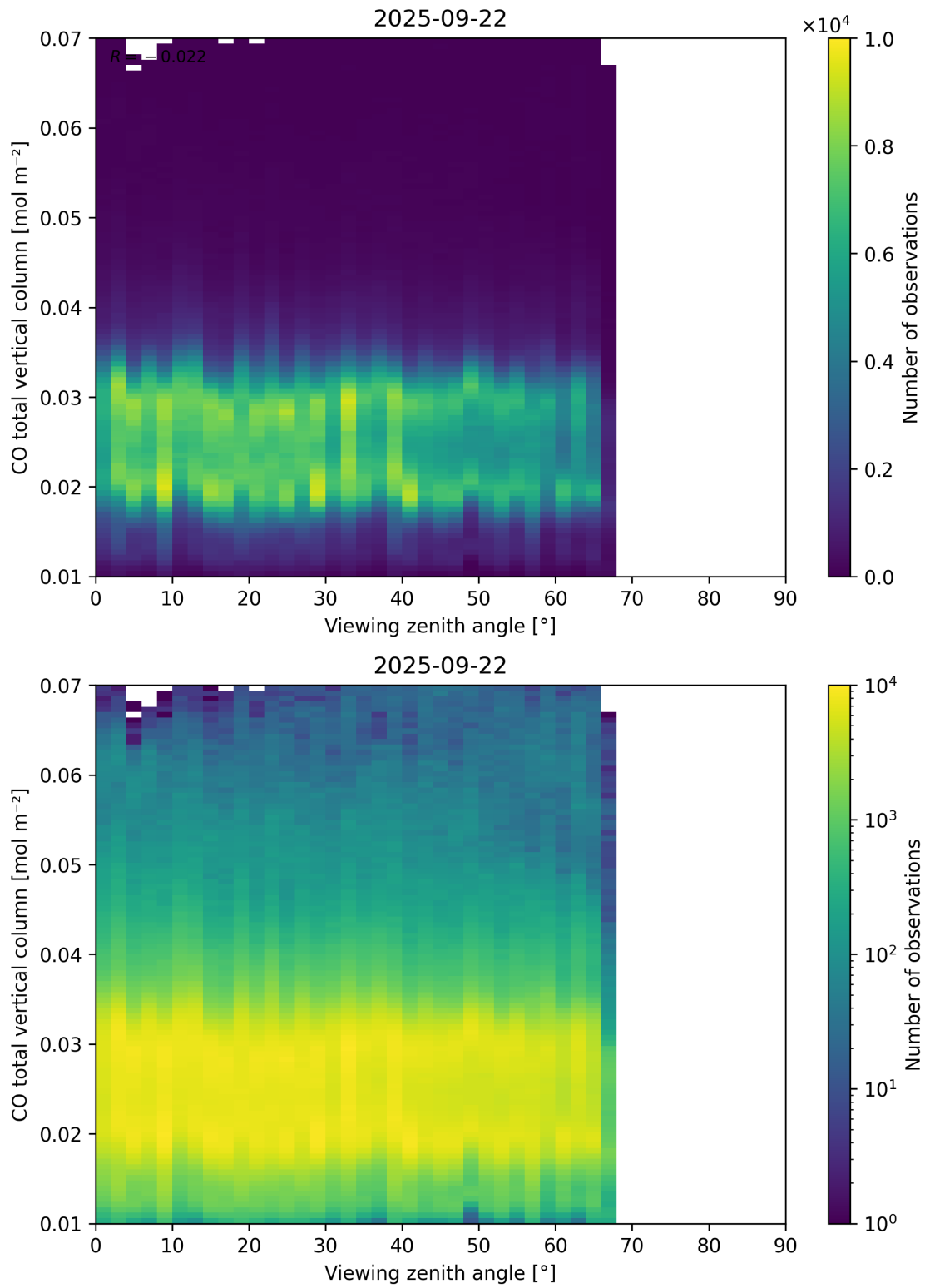
Figure 69: Scatter density plot of “Viewing zenith angle” against “CO total vertical column” for 2025-09-22 to 2025-09-23.
