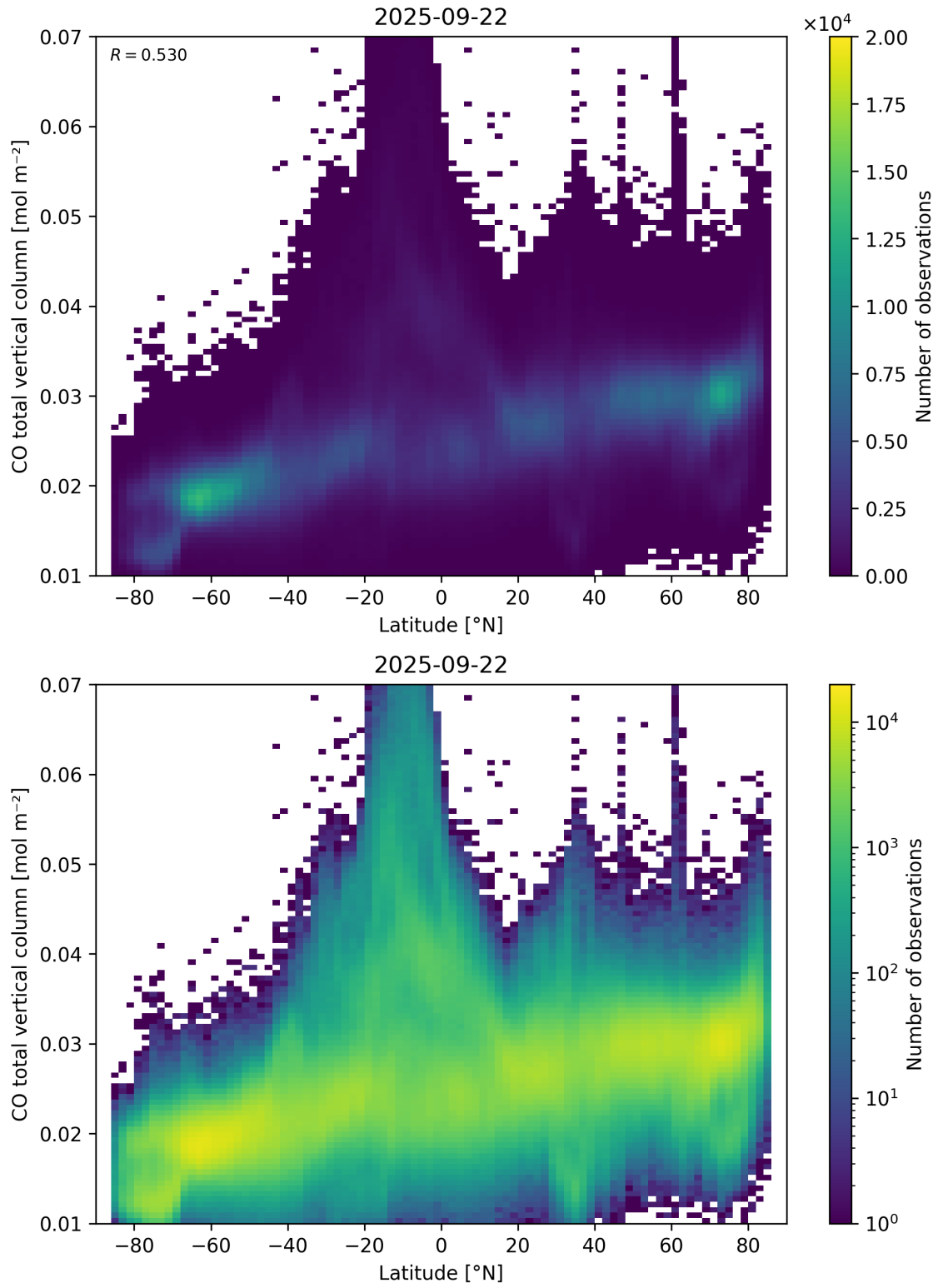
Figure 51: Scatter density plot of “Latitude” against “CO total vertical column” for 2025-09-22 to 2025-09-23.
