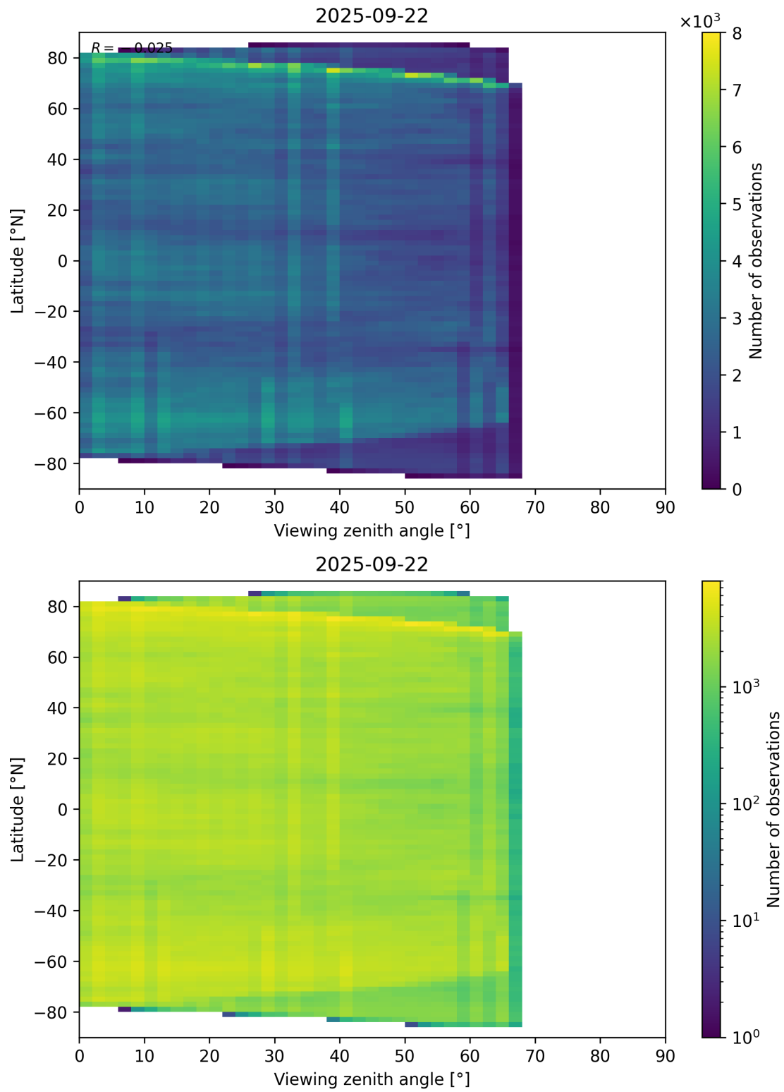
Figure 74: Scatter density plot of “Viewing zenith angle” against “Latitude” for 2025-09-22 to 2025-09-23.
