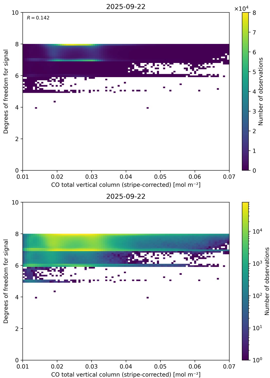
Figure 38: Scatter density plot of “CO total vertical column (stripe-corrected)” against “Degrees of freedom for signal” for 2025-09-22 to 2025-09-23.
