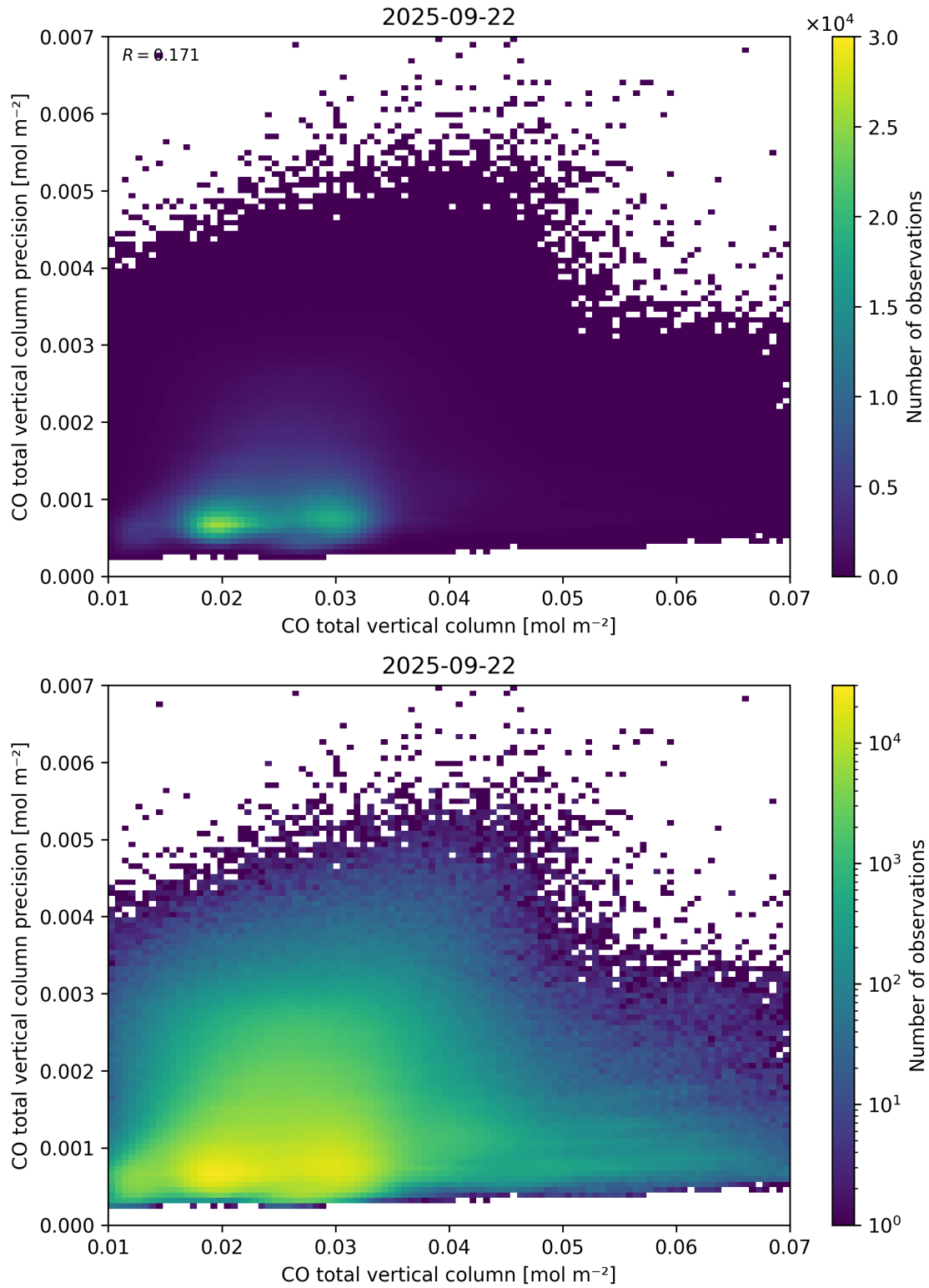
Figure 34: Scatter density plot of “CO total vertical column” against “CO total vertical column precision” for 2025-09-22 to 2025-09-23.
