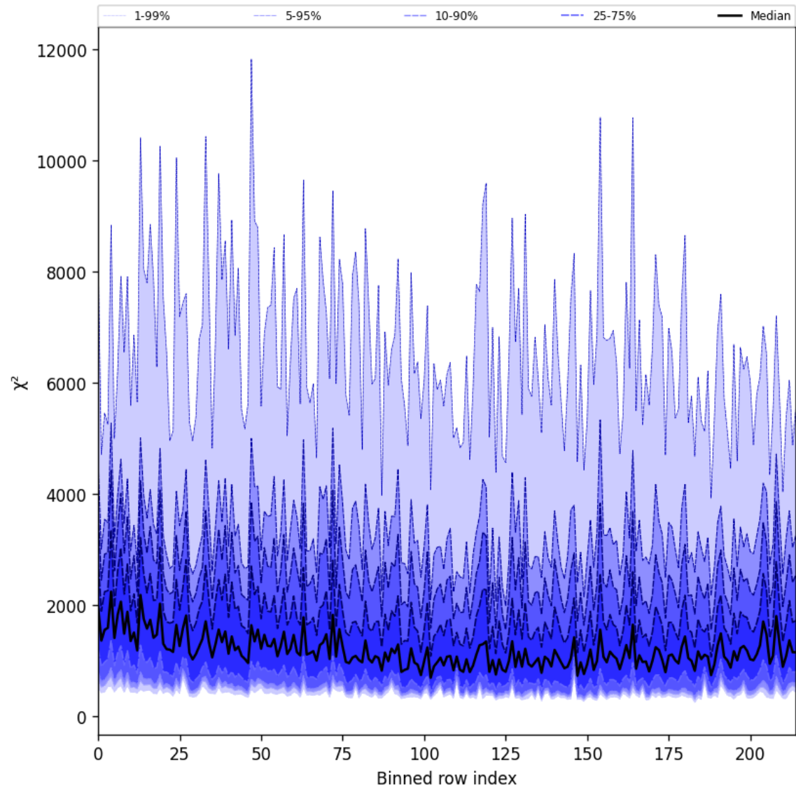
Figure 30: Along track statistics of “ \chi^2 ” for 2025-09-22 to 2025-09-23
