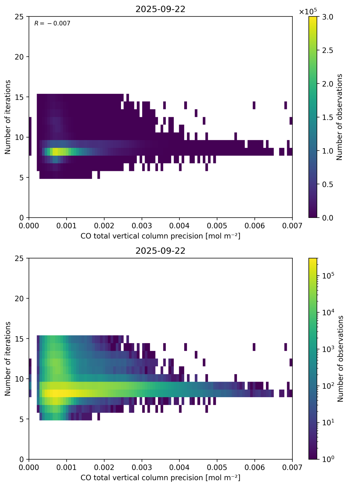
Figure 46: Scatter density plot of “CO total vertical column precision” against “Number of iterations” for 2025-09-22 to 2025-09-23.
