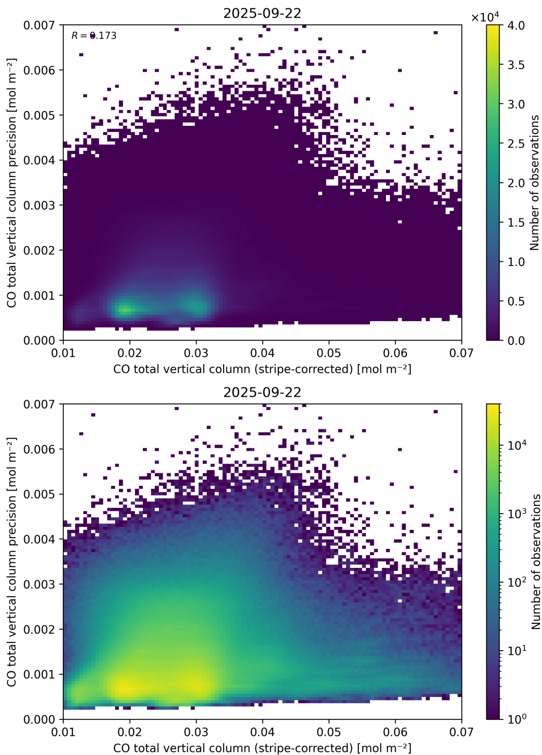
Figure 36: Scatter density plot of “CO total vertical column (stripe-corrected)” against “CO total vertical column precision” for 2025-09-22 to 2025-09-23.
