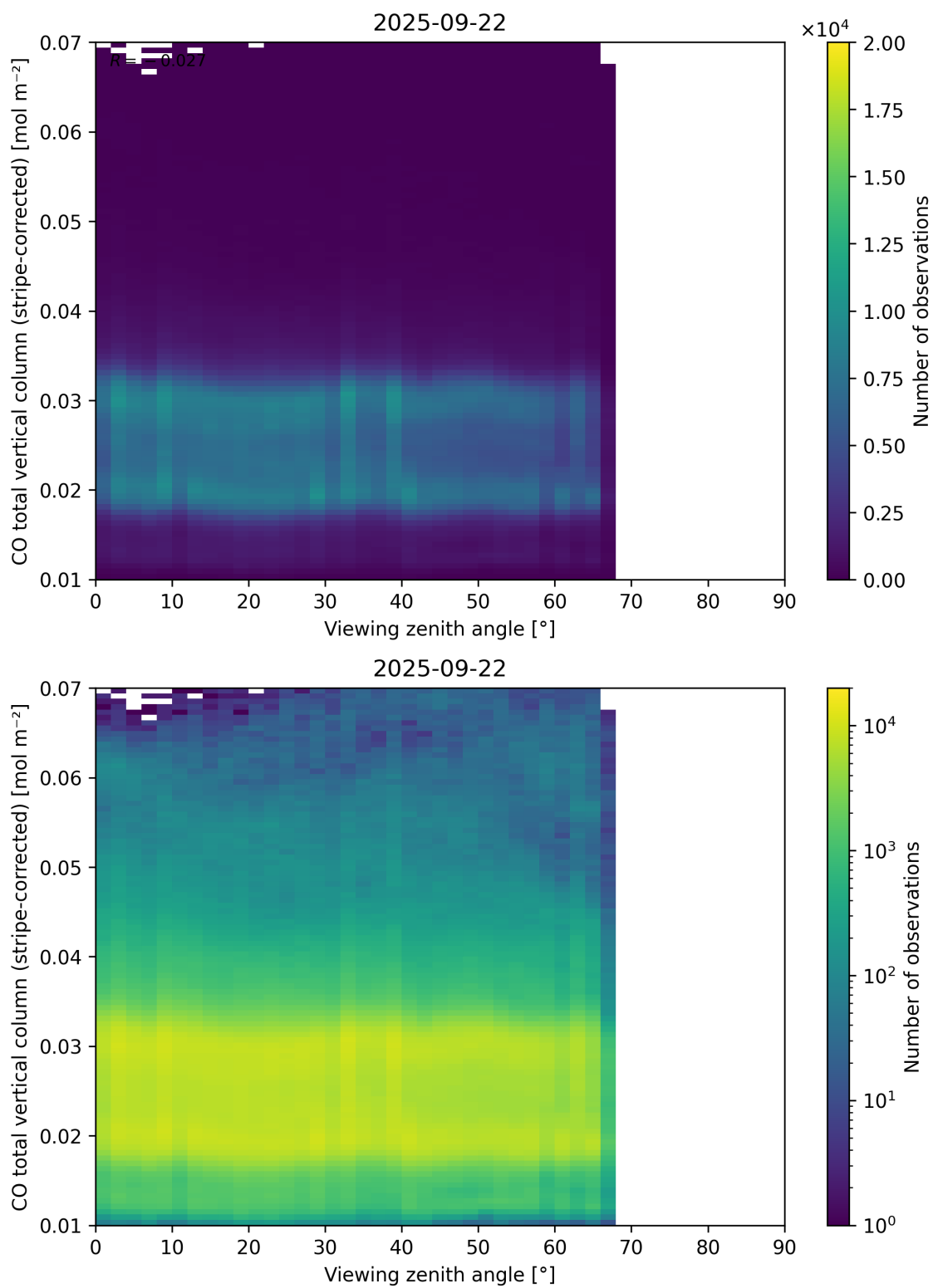
Figure 70: Scatter density plot of “Viewing zenith angle” against “CO total vertical column (stripe-corrected)” for 2025-09-22 to 2025-09-23.
