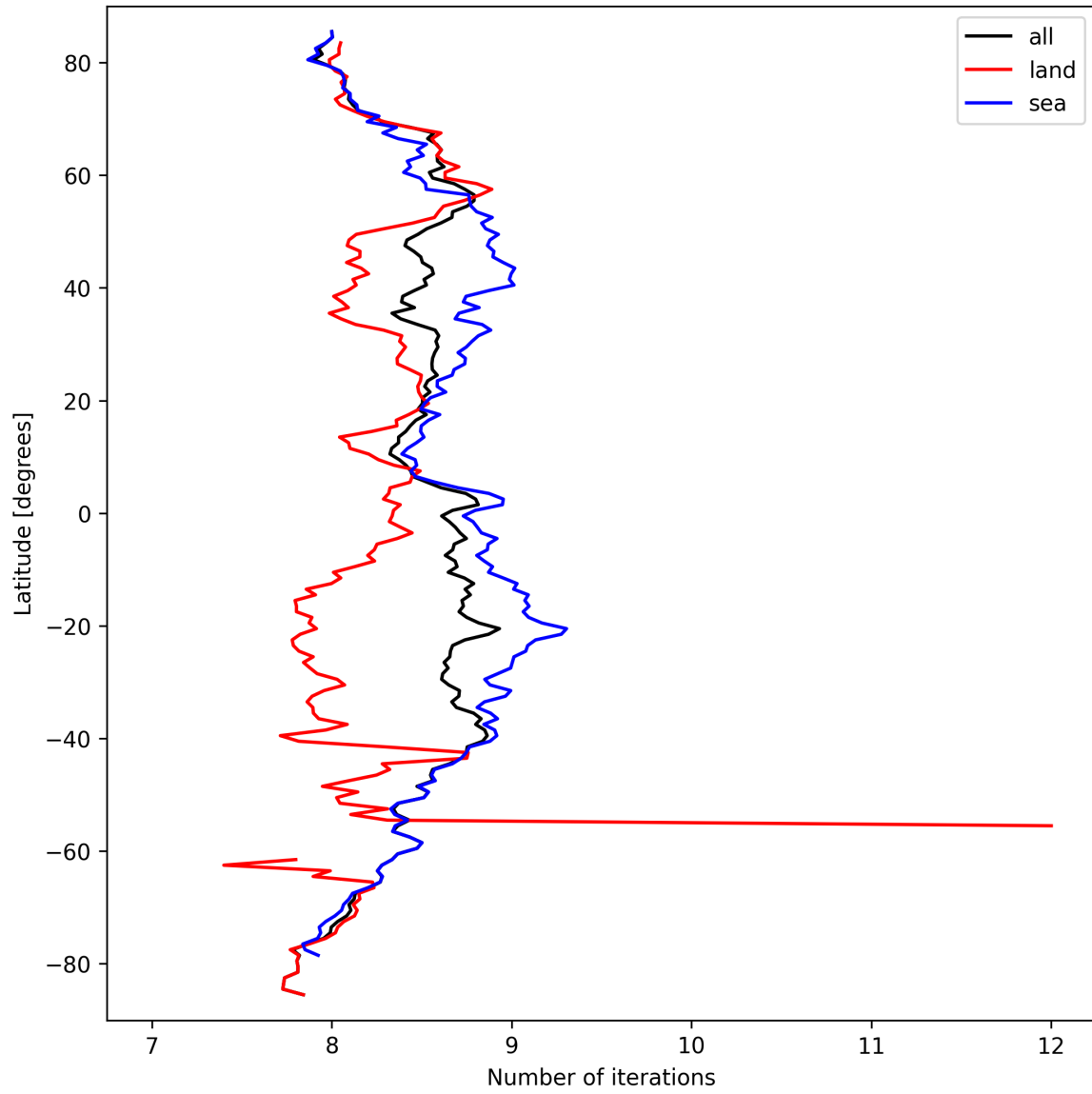
Figure 16: Zonal average of “Number of iterations” for 2025-09-22 to 2025-09-23.
