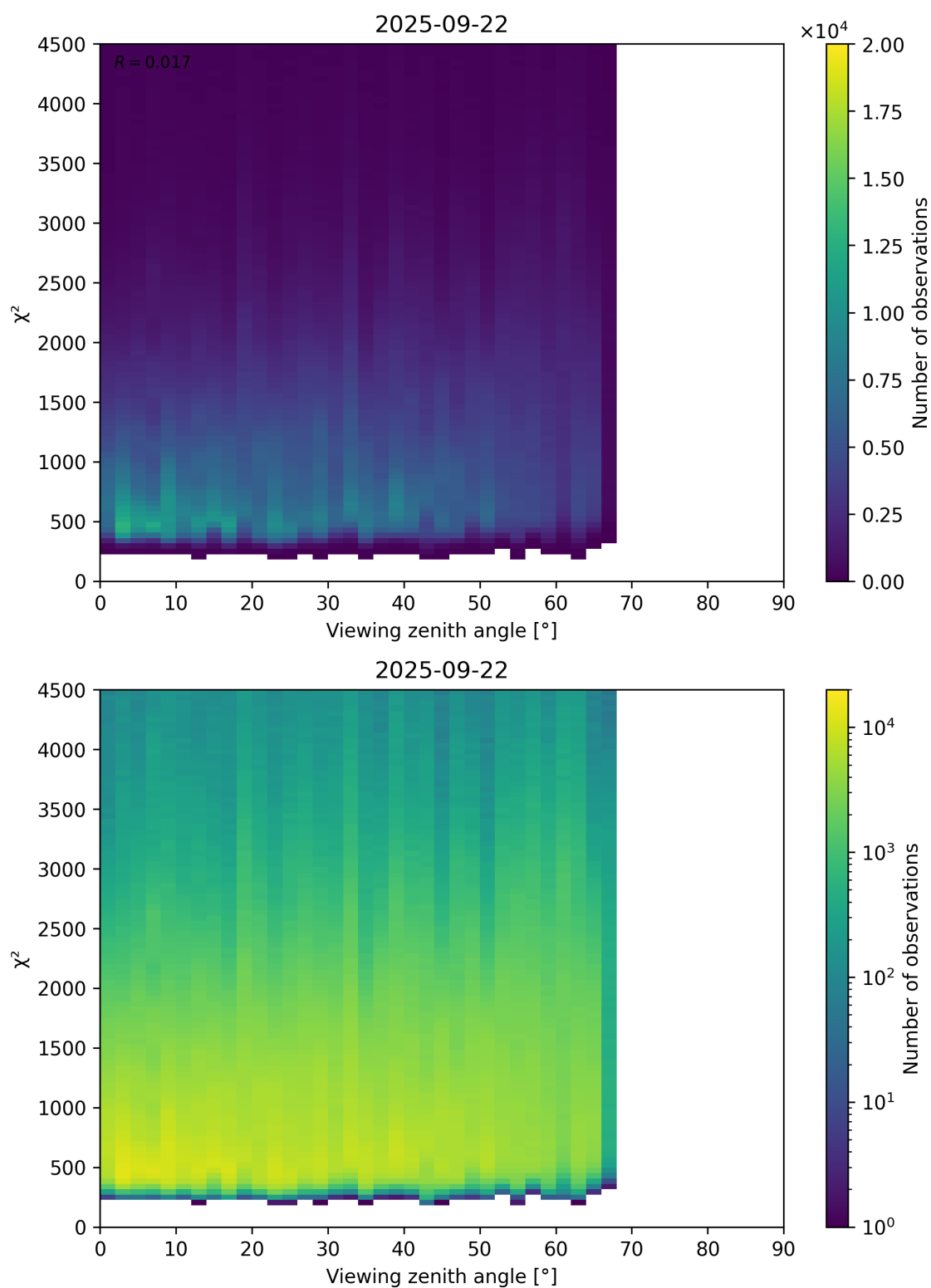
Figure 72: Scatter density plot of “Viewing zenith angle” against “ \chi^2 ” for 2025-09-22 to 2025-09-23.
