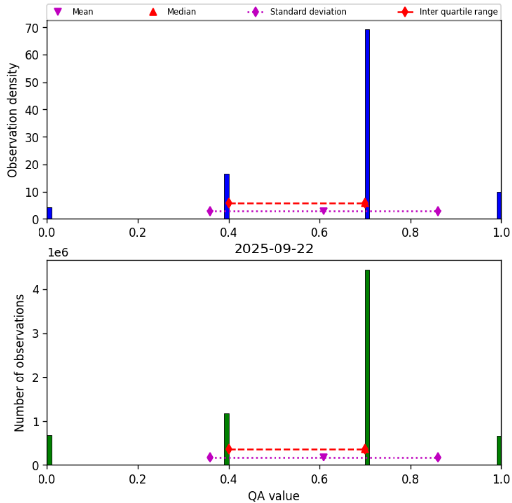
Figure 17: Histogram of “QA value” for 2025-09-22 to 2025-09-23
