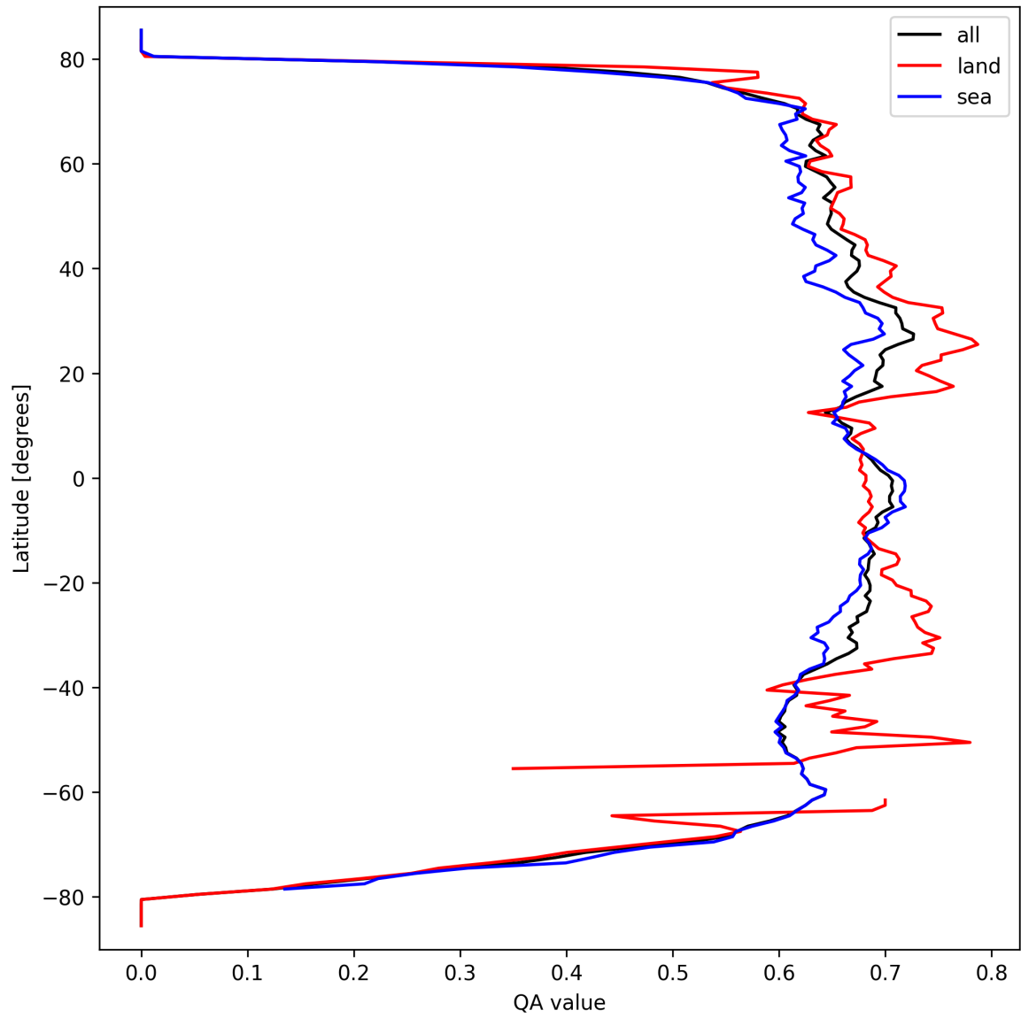
Figure 9: Zonal average of “QA value” for 2025-09-22 to 2025-09-23.
