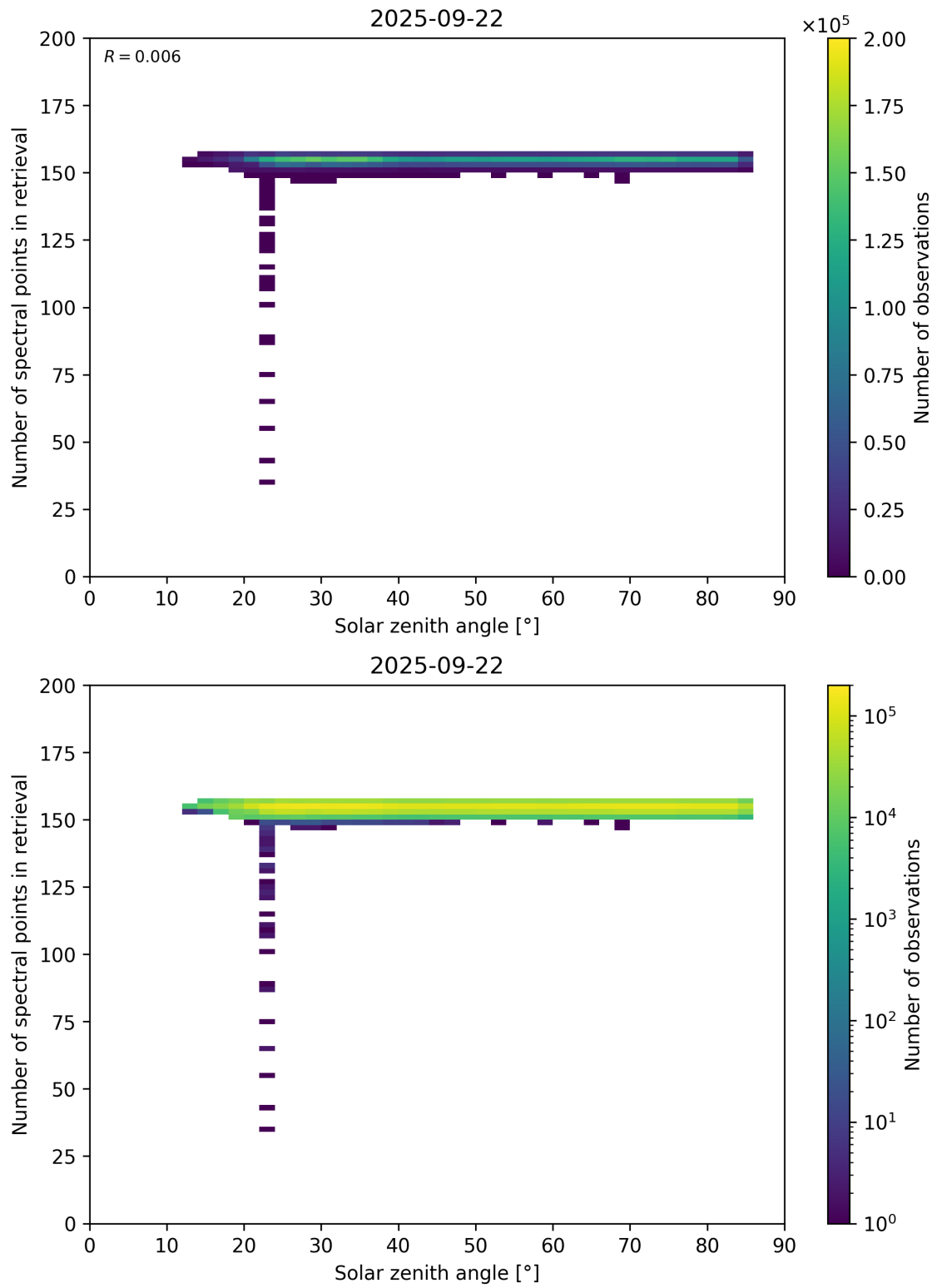
Figure 68: Scatter density plot of “Solar zenith angle” against “Number of spectral points in retrieval” for 2025-09-22 to 2025-09-23.
