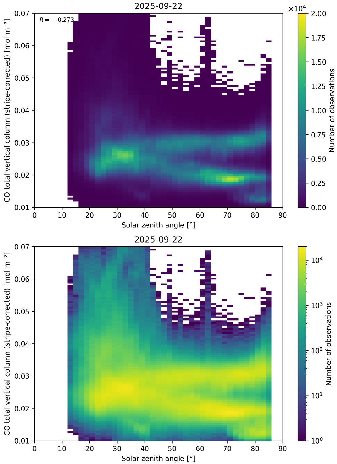
Figure 62: Scatter density plot of “Solar zenith angle” against “CO total vertical column (stripe-corrected)” for 2025-09-22 to 2025-09-23.
