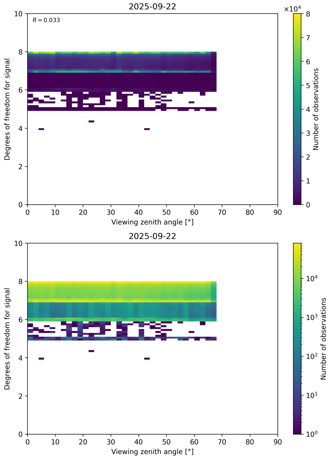
Figure 73: Scatter density plot of “Viewing zenith angle” against “Degrees of freedom for signal” for 2025-09-22 to 2025-09-23.
