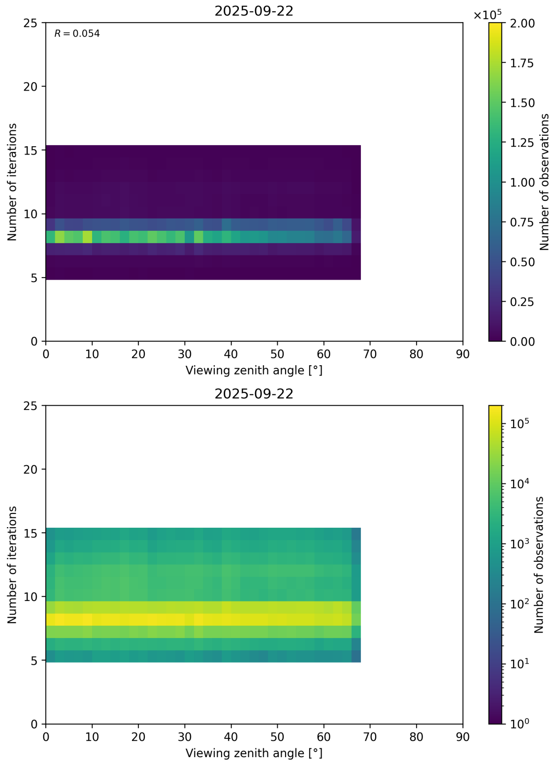
Figure 75: Scatter density plot of “Viewing zenith angle” against “Number of iterations” for 2025-09-22 to 2025-09-23.
