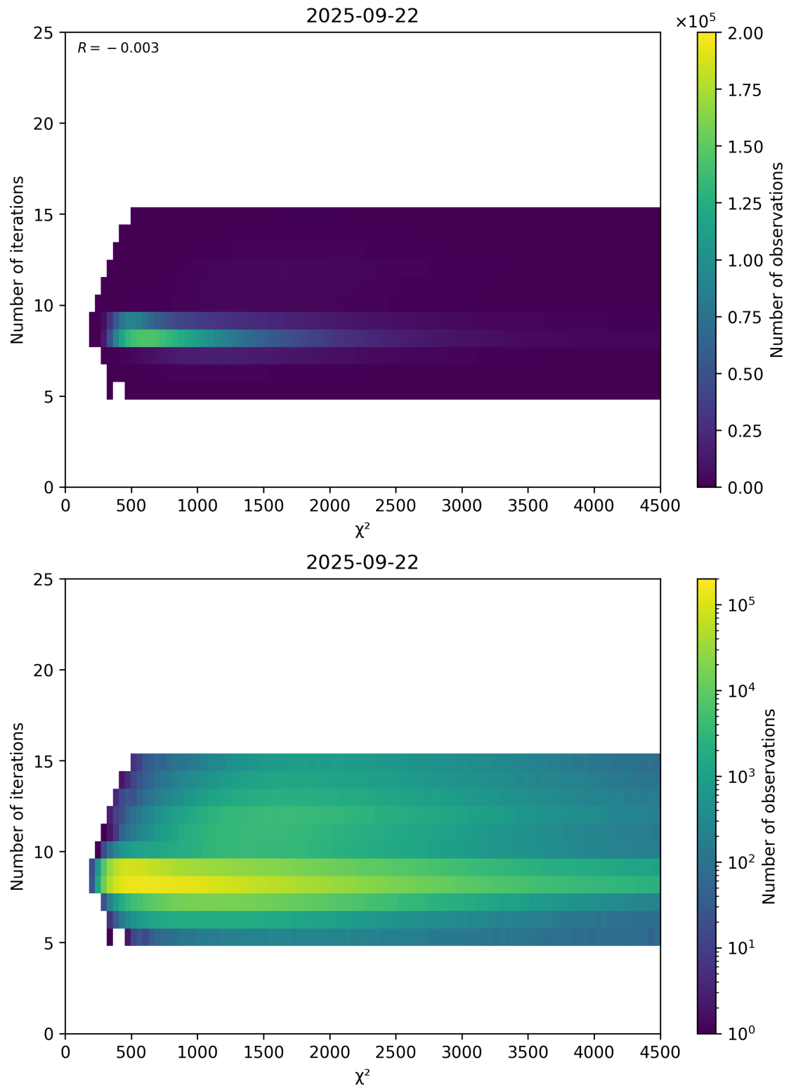
Figure 49: Scatter density plot of “ \chi^2 ” against “Number of iterations” for 2025-09-22 to 2025-09-23.
