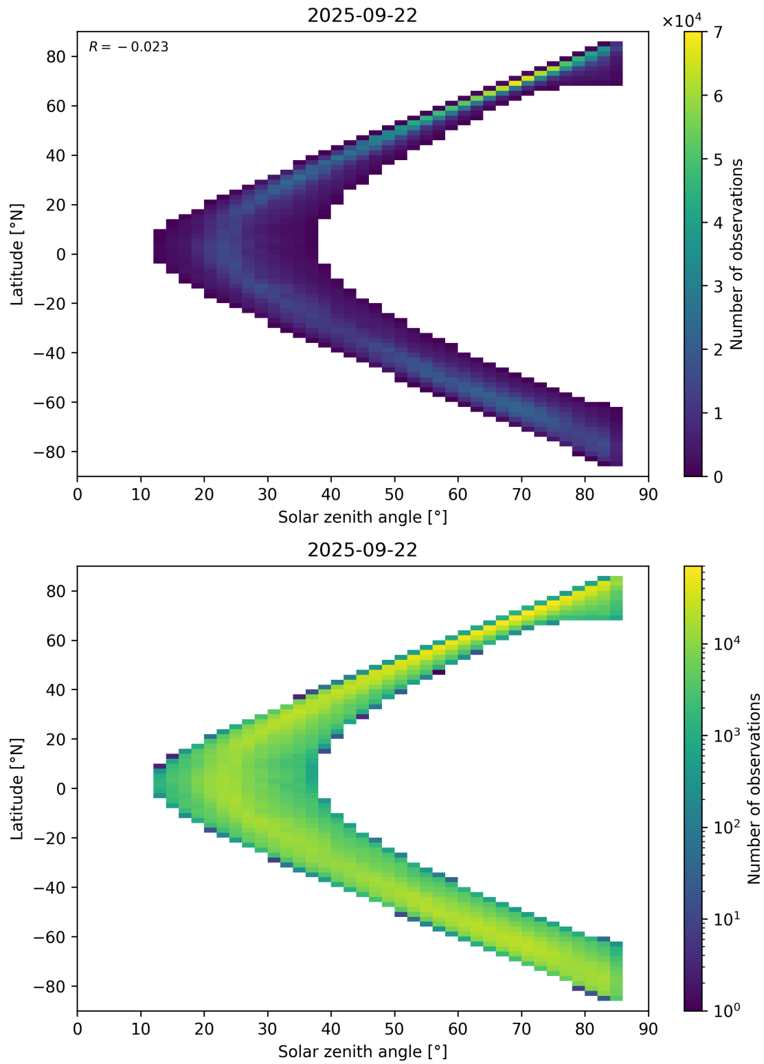
Figure 66: Scatter density plot of “Solar zenith angle” against “Latitude” for 2025-09-22 to 2025-09-23.
