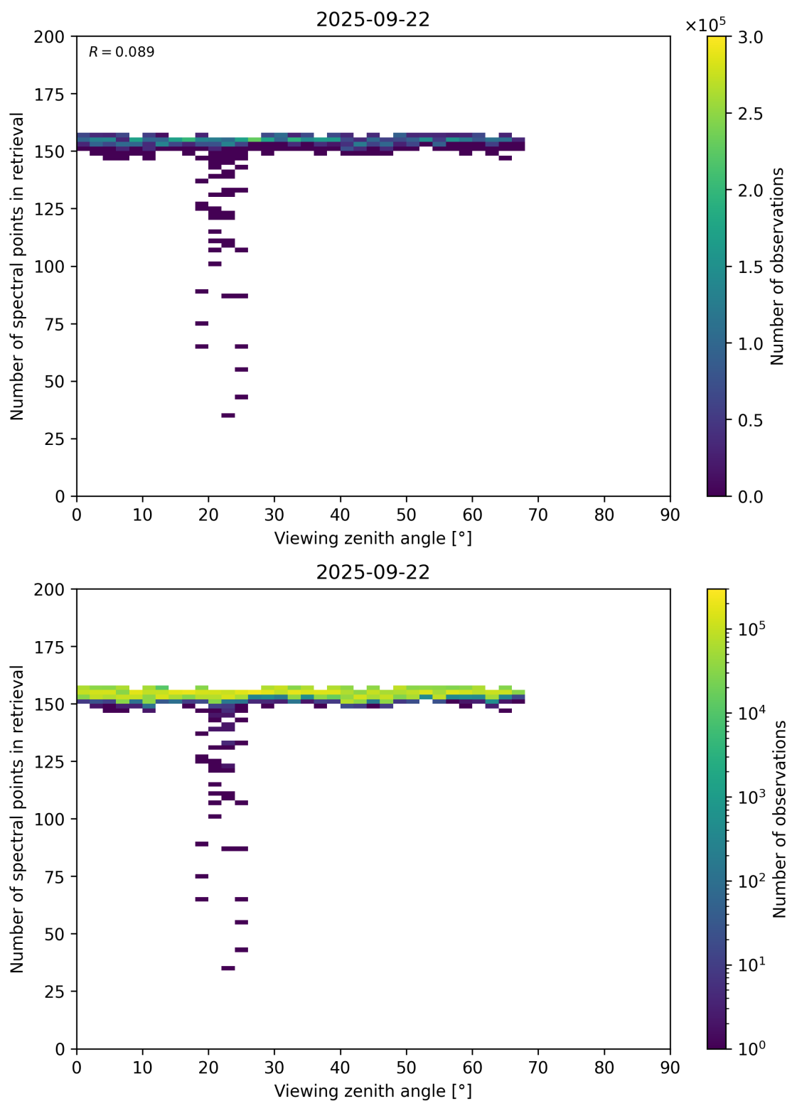
Figure 76: Scatter density plot of “Viewing zenith angle” against “Number of spectral points in retrieval” for 2025-09-22 to 2025-09-23.
