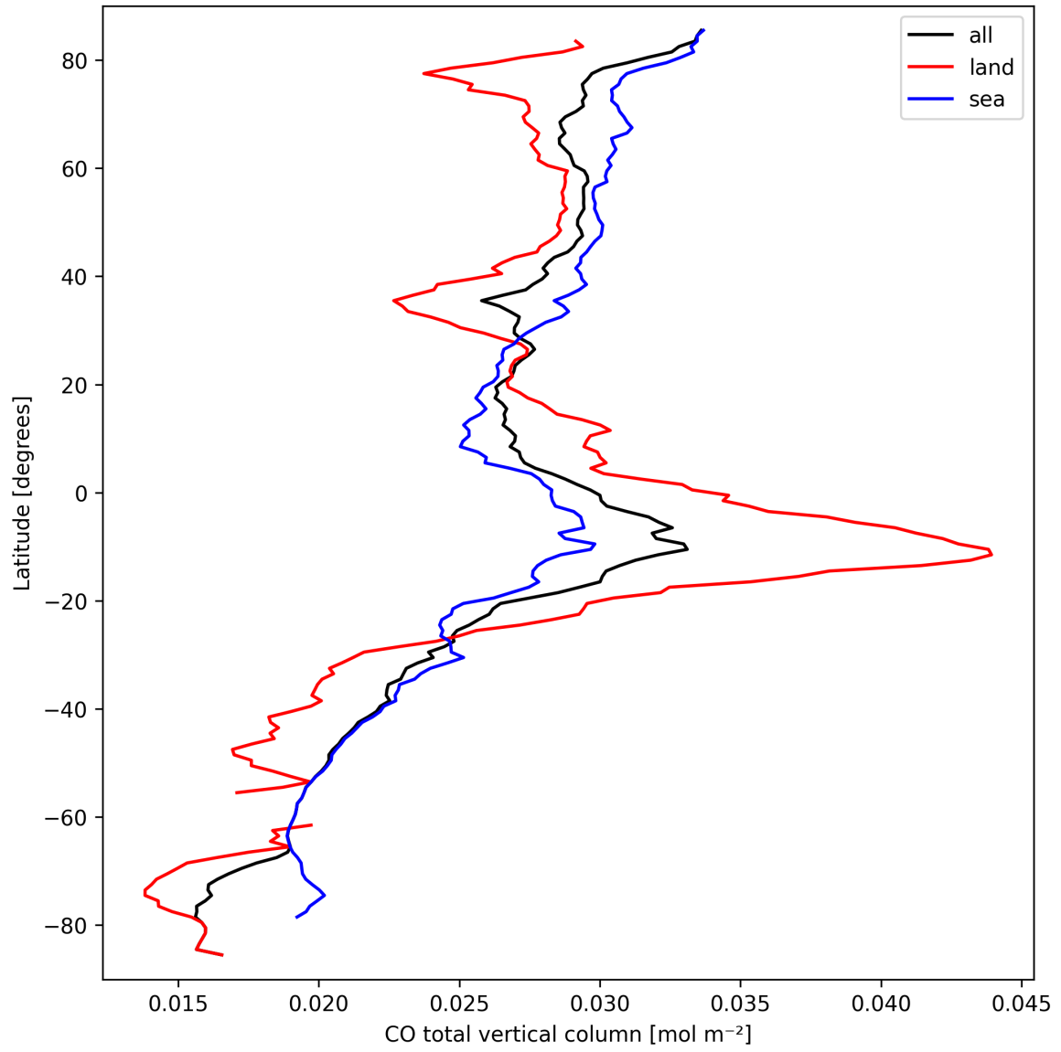
Figure 10: Zonal average of “CO total vertical column” for 2025-09-22 to 2025-09-23.
